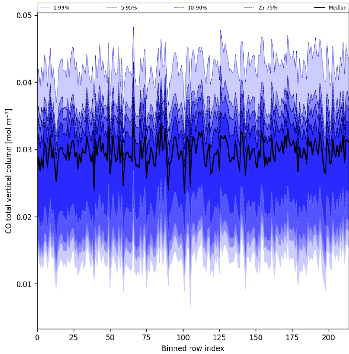
Figure 21: Along track statistics of “CO total vertical column” for 2025-05-06 to 2025-05-07
