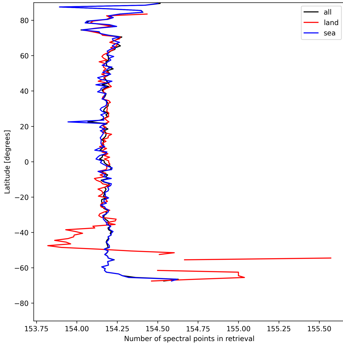
Figure 9: Zonal average of “Number of spectral points in retrieval” for 2025-05-06 to 2025-05-07.
