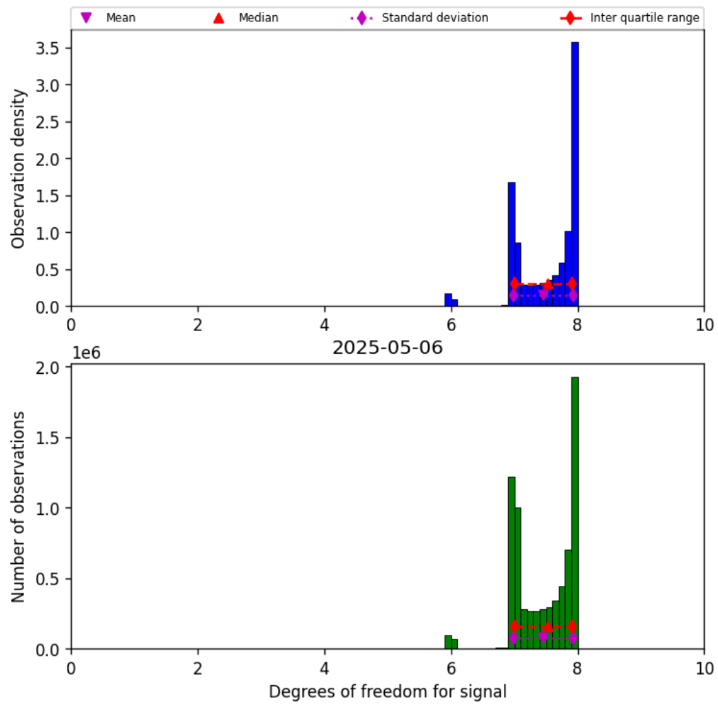
Figure 18: Histogram of “Degrees of freedom for signal” for 2025-05-06 to 2025-05-07
