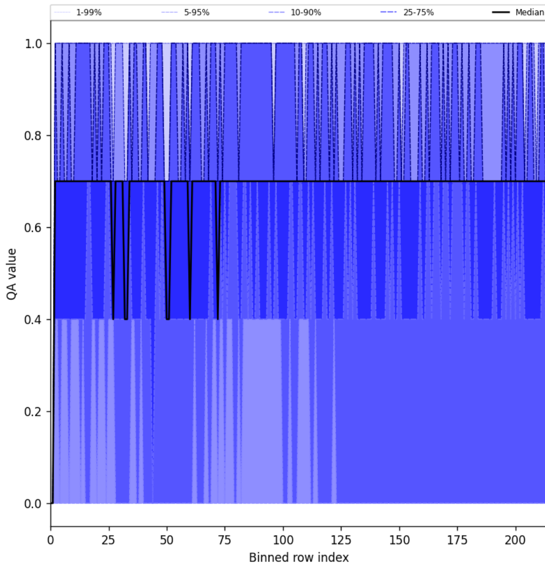
Figure 20: Along track statistics of “QA value” for 2025-05-06 to 2025-05-07
