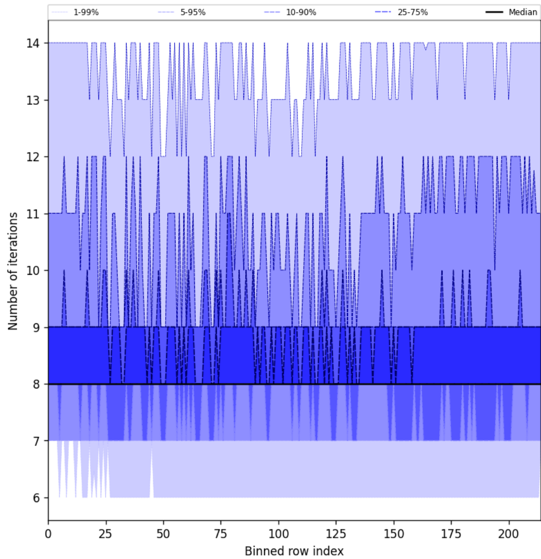
Figure 26: Along track statistics of “Number of iterations” for 2025-05-06 to 2025-05-07
