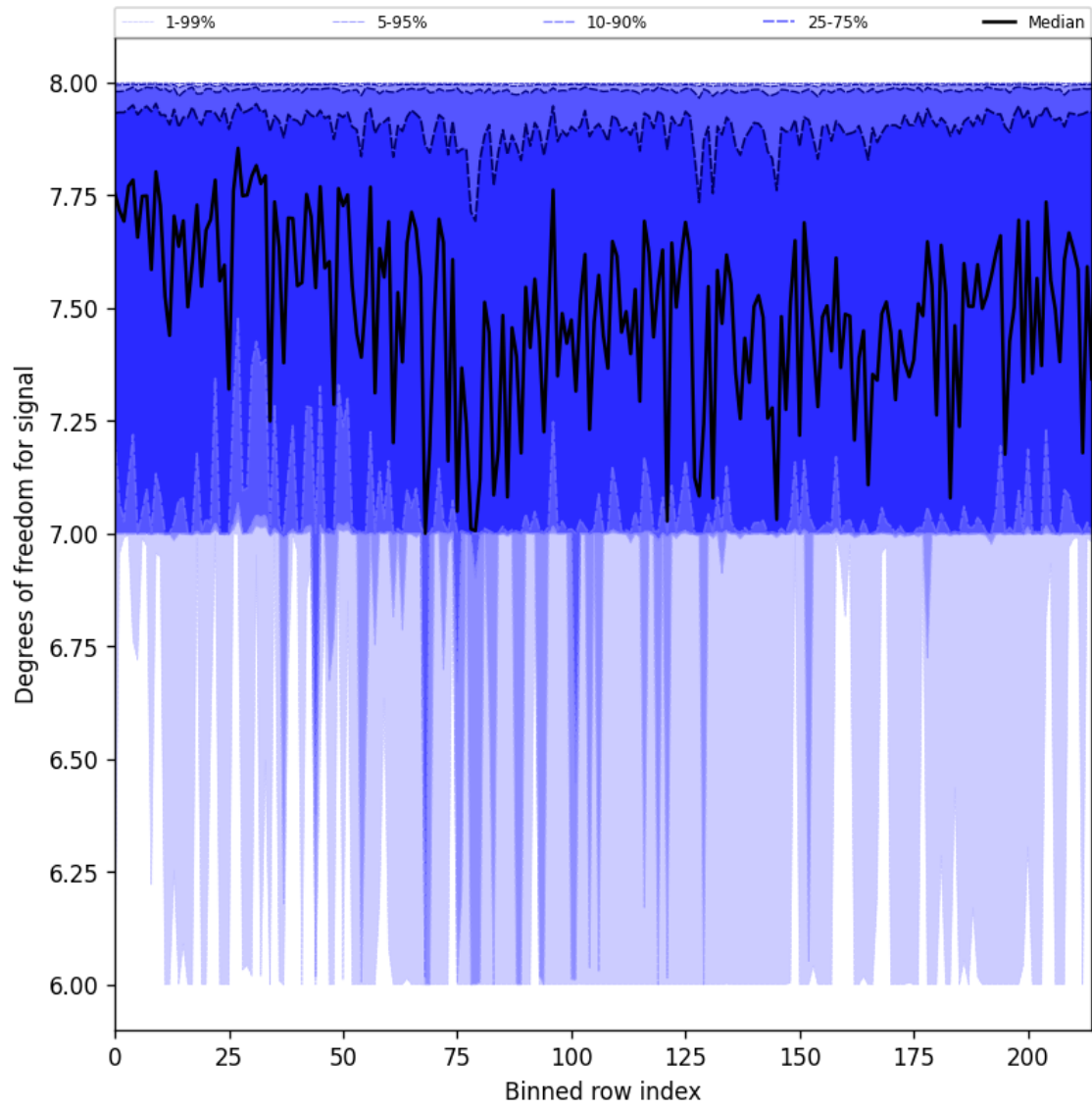
Figure 25: Along track statistics of “Degrees of freedom for signal” for 2025-05-06 to 2025-05-07
