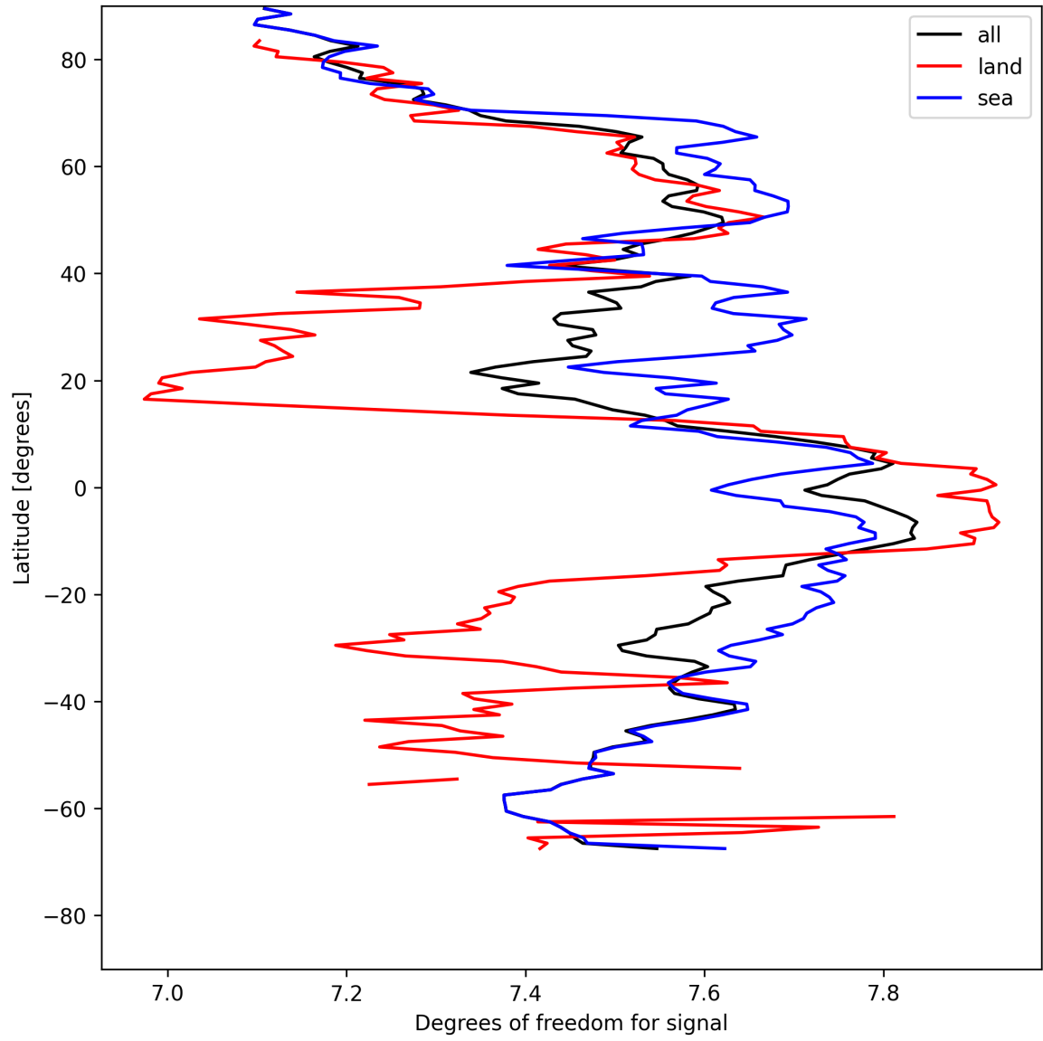
Figure 11: Zonal average of “Degrees of freedom for signal” for 2025-05-06 to 2025-05-07.
