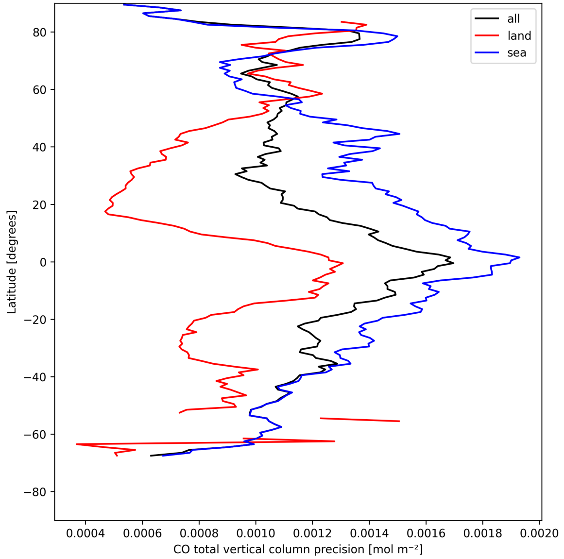
Figure 8: Zonal average of “CO total vertical column precision” for 2025-05-06 to 2025-05-07.
