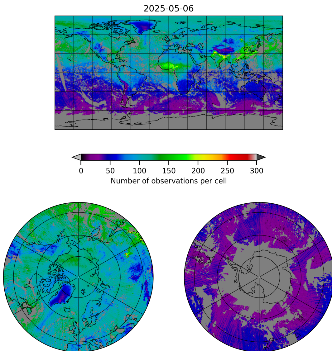
Figure 5: Map of the number of observations for 2025-05-06 to 2025-05-07
