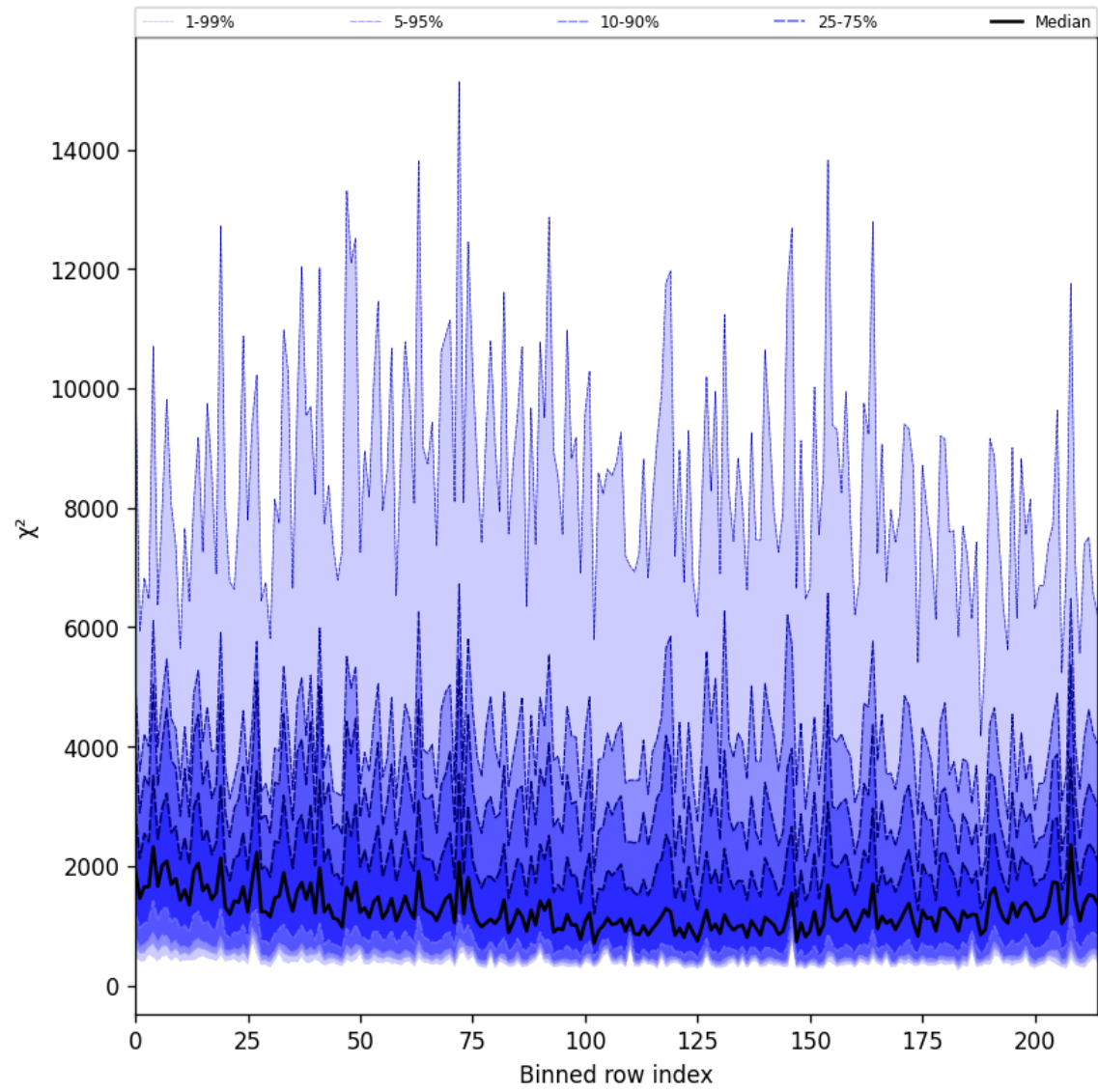
Figure 24: Along track statistics of “ \chi^2 ” for 2025-05-06 to 2025-05-07
