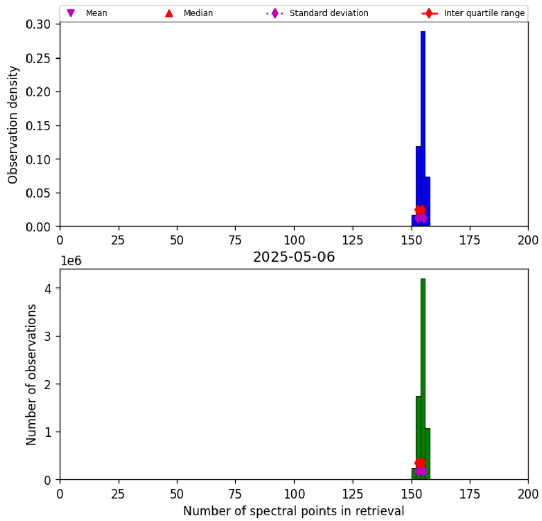
Figure 16: Histogram of “Number of spectral points in retrieval” for 2025-05-06 to 2025-05-07
