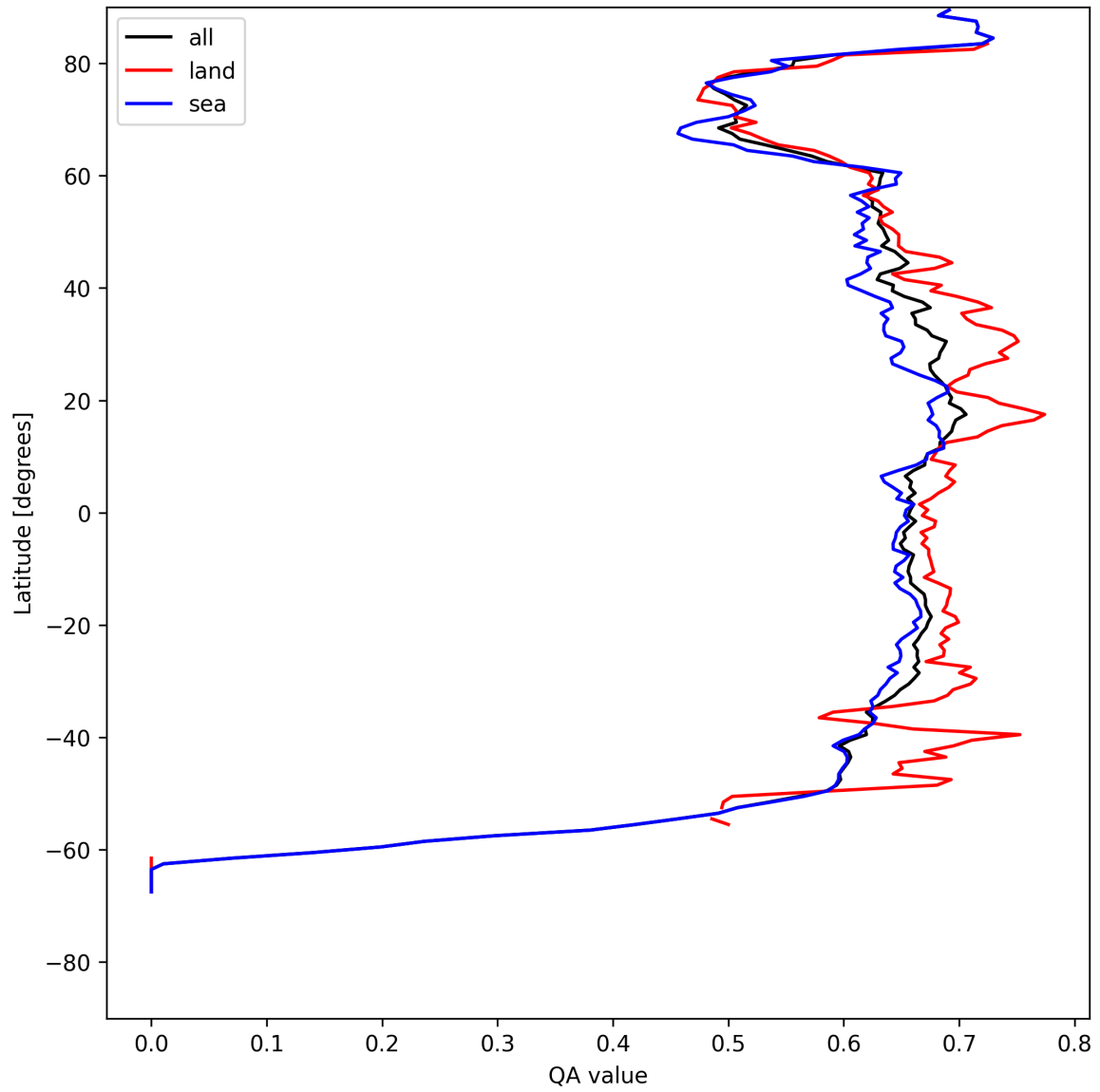
Figure 6: Zonal average of “QA value” for 2025-05-06 to 2025-05-07.
