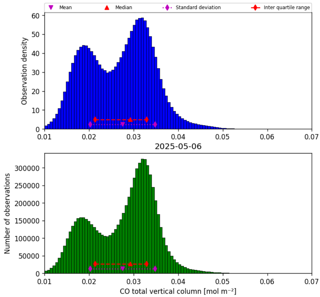
Figure 14: Histogram of “CO total vertical column” for 2025-05-06 to 2025-05-07
