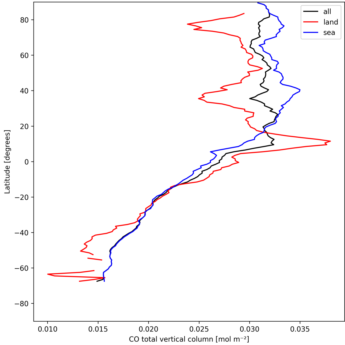
Figure 7: Zonal average of “CO total vertical column” for 2025-05-06 to 2025-05-07.
