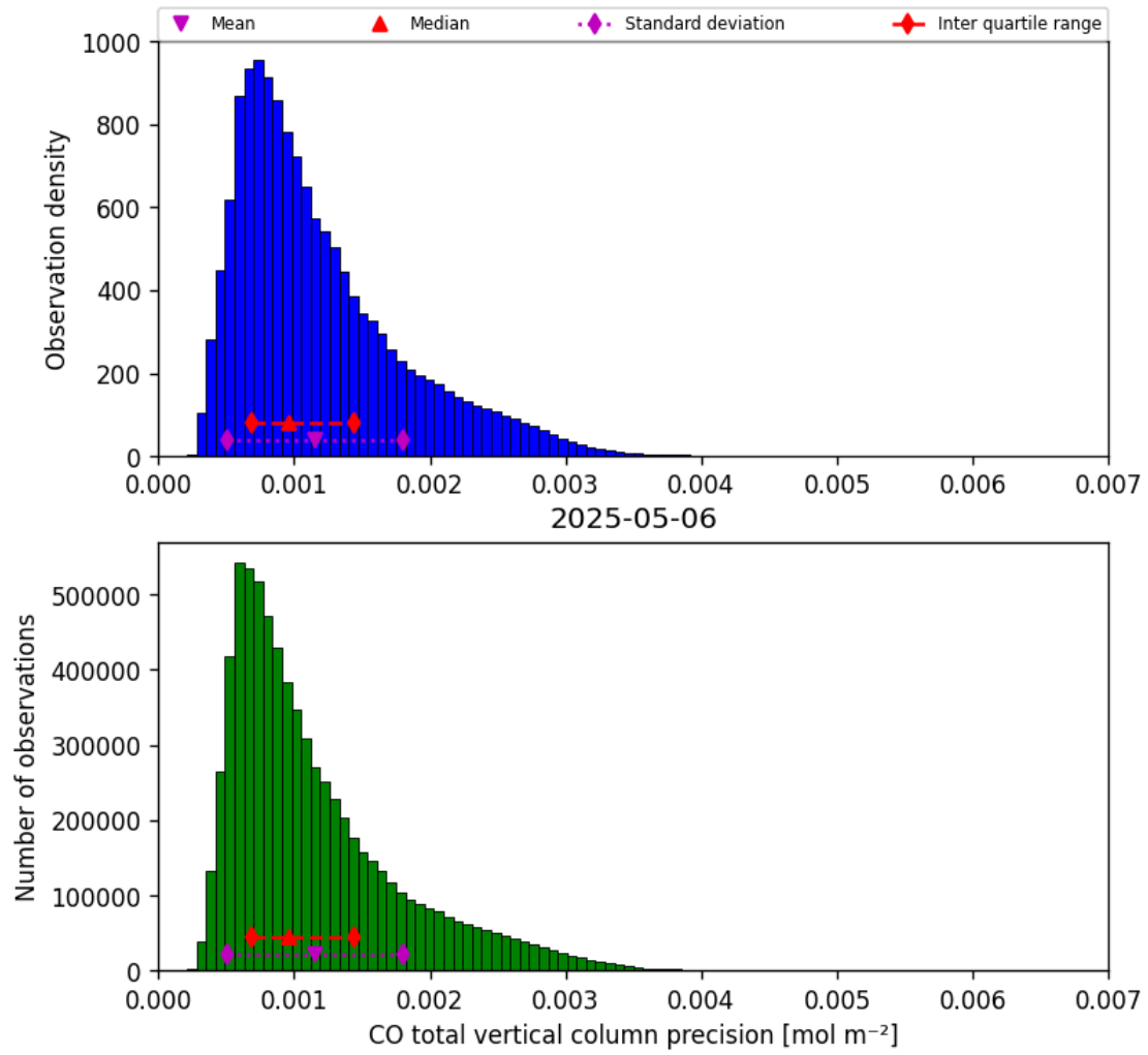
Figure 15: Histogram of “CO total vertical column precision” for 2025-05-06 to 2025-05-07
