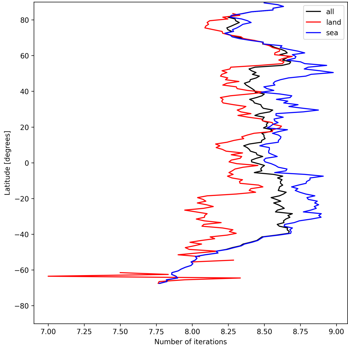
Figure 12: Zonal average of “Number of iterations” for 2025-05-06 to 2025-05-07.
