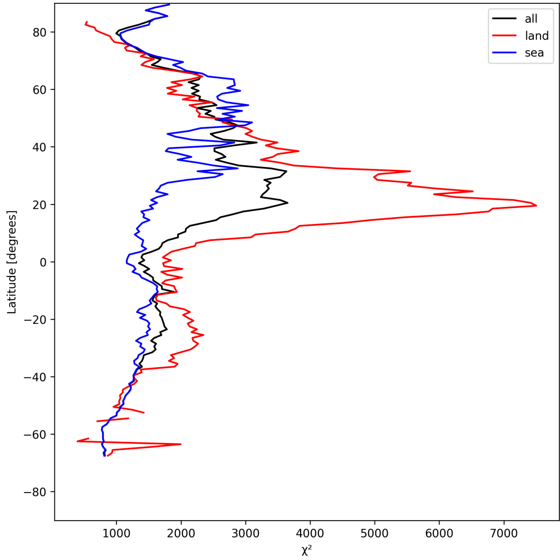
Figure 10: Zonal average of “ \chi^2 ” for 2025-05-06 to 2025-05-07.
