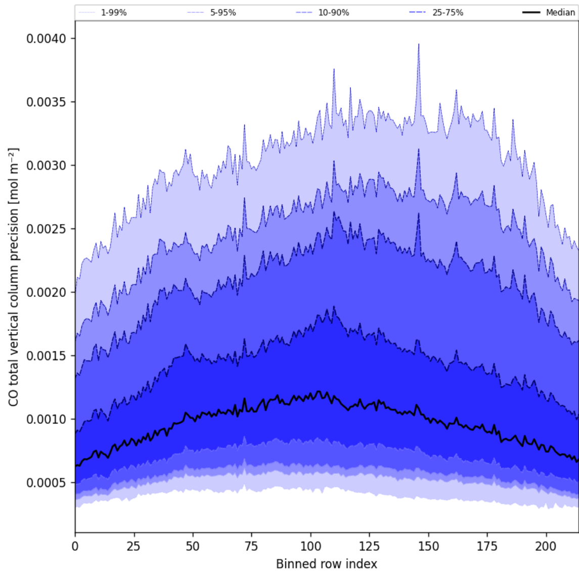
Figure 22: Along track statistics of “CO total vertical column precision” for 2025-05-06 to 2025-05-07
