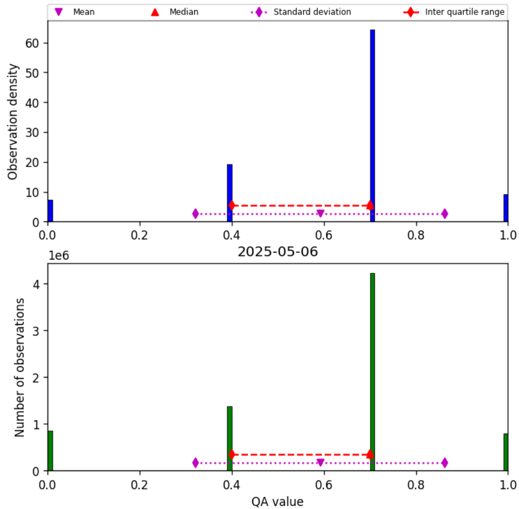
Figure 13: Histogram of “QA value” for 2025-05-06 to 2025-05-07
