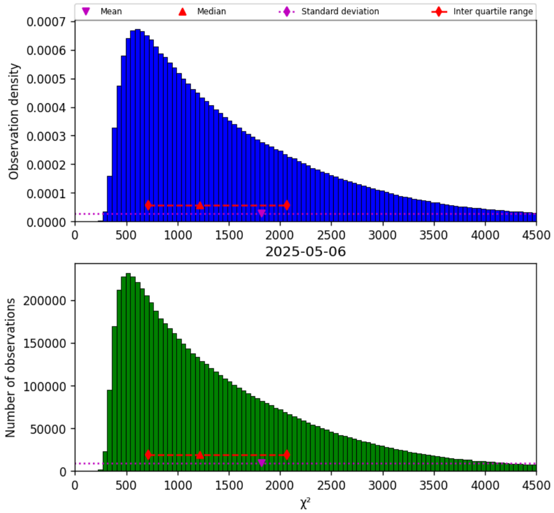
Figure 17: Histogram of “ \chi^2 ” for 2025-05-06 to 2025-05-07
