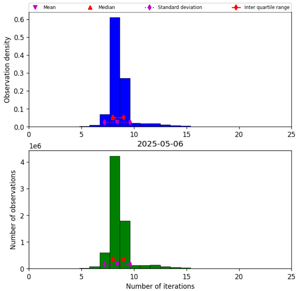
Figure 19: Histogram of “Number of iterations” for 2025-05-06 to 2025-05-07
