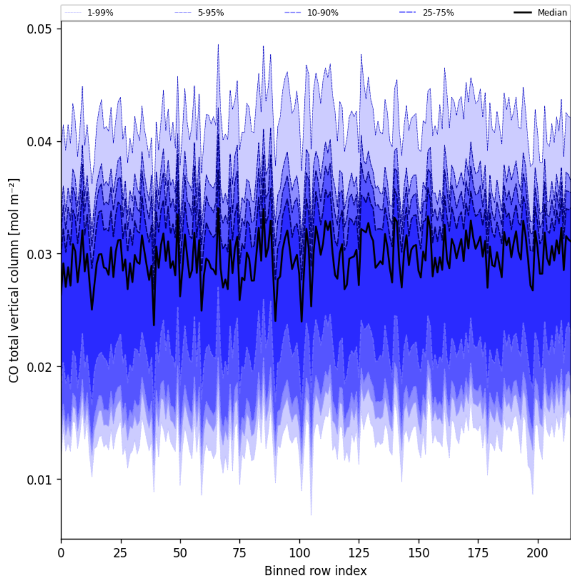
Figure 21: Along track statistics of “CO total vertical column” for 2025-05-07 to 2025-05-08
