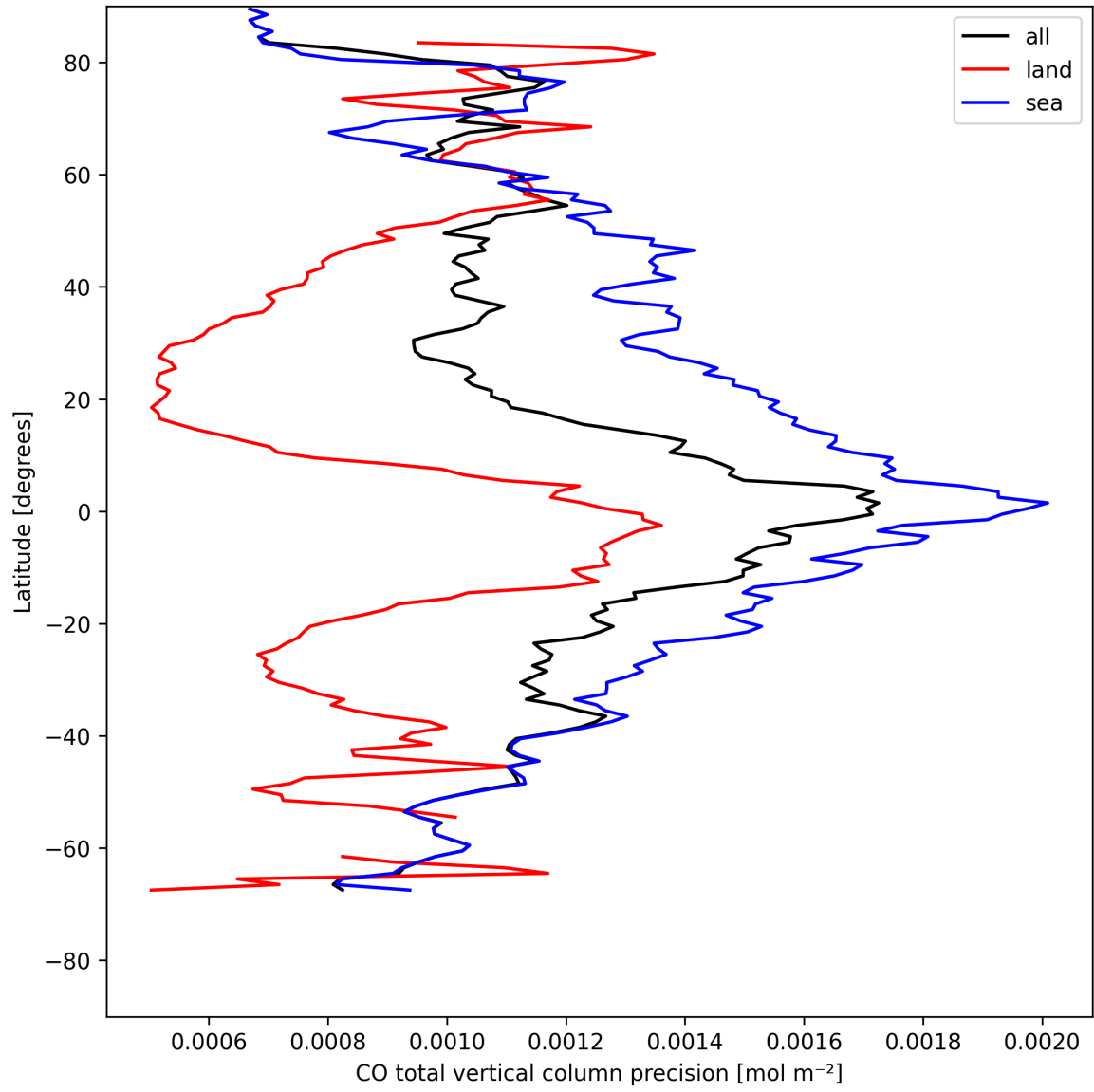
Figure 8: Zonal average of “CO total vertical column precision” for 2025-05-07 to 2025-05-08.
