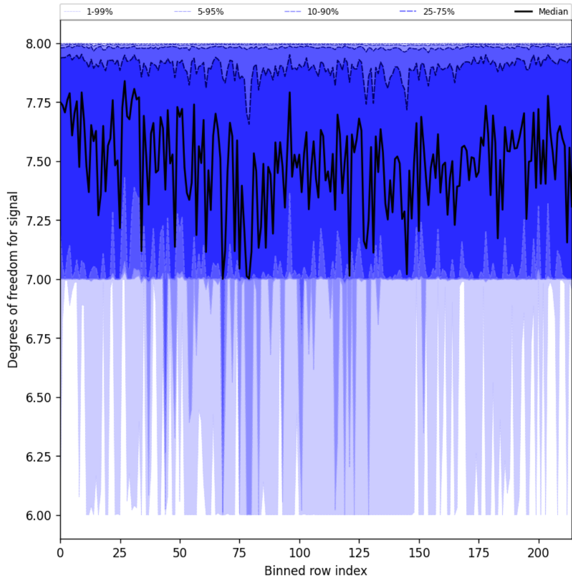
Figure 25: Along track statistics of “Degrees of freedom for signal” for 2025-05-07 to 2025-05-08
