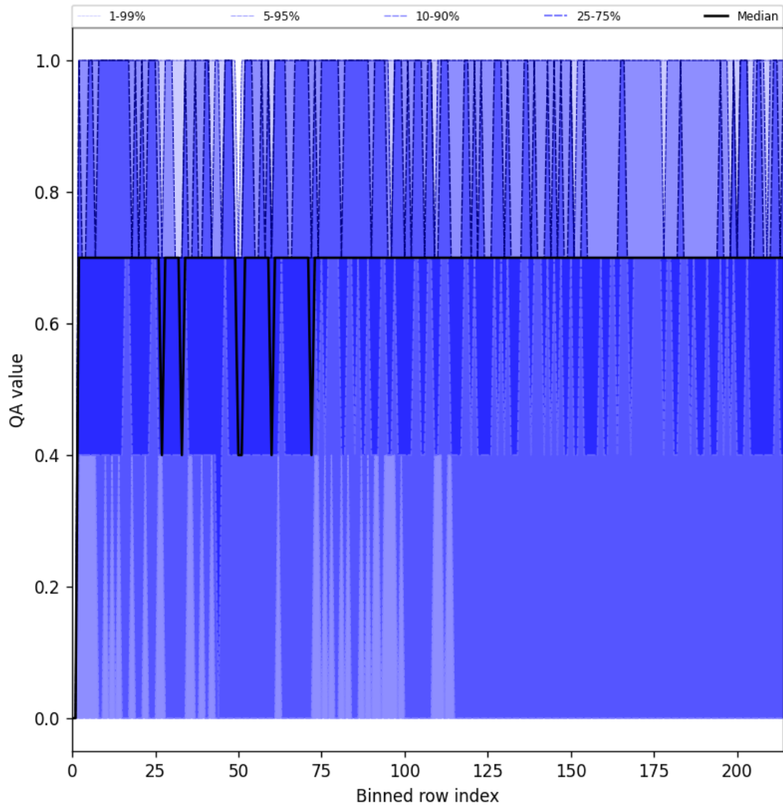
Figure 20: Along track statistics of “QA value” for 2025-05-07 to 2025-05-08
