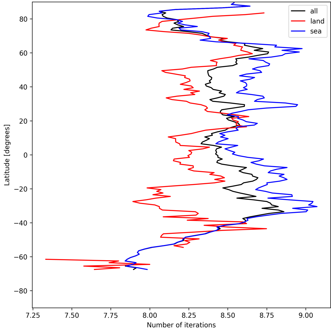
Figure 12: Zonal average of “Number of iterations” for 2025-05-07 to 2025-05-08.
