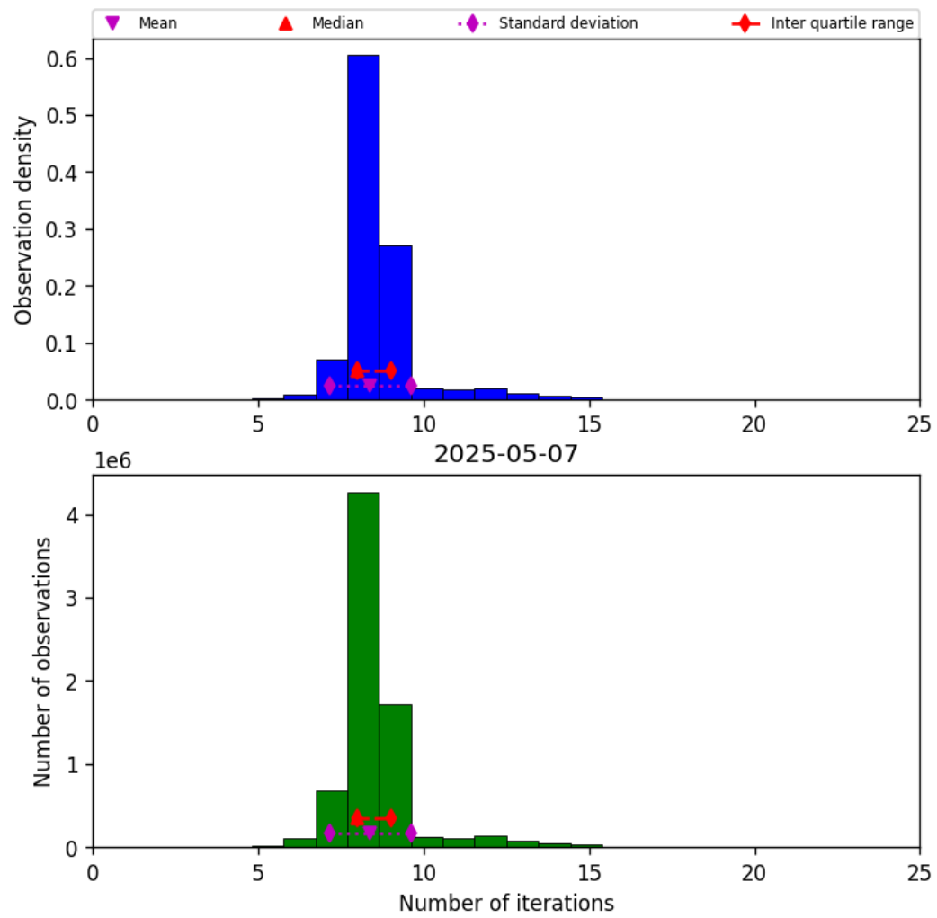
Figure 19: Histogram of “Number of iterations” for 2025-05-07 to 2025-05-08
