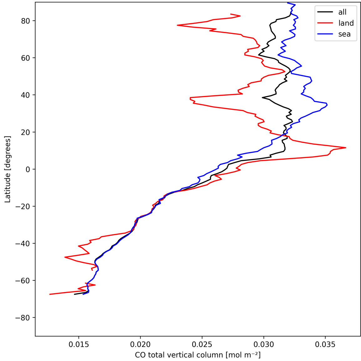
Figure 7: Zonal average of “CO total vertical column” for 2025-05-07 to 2025-05-08.
