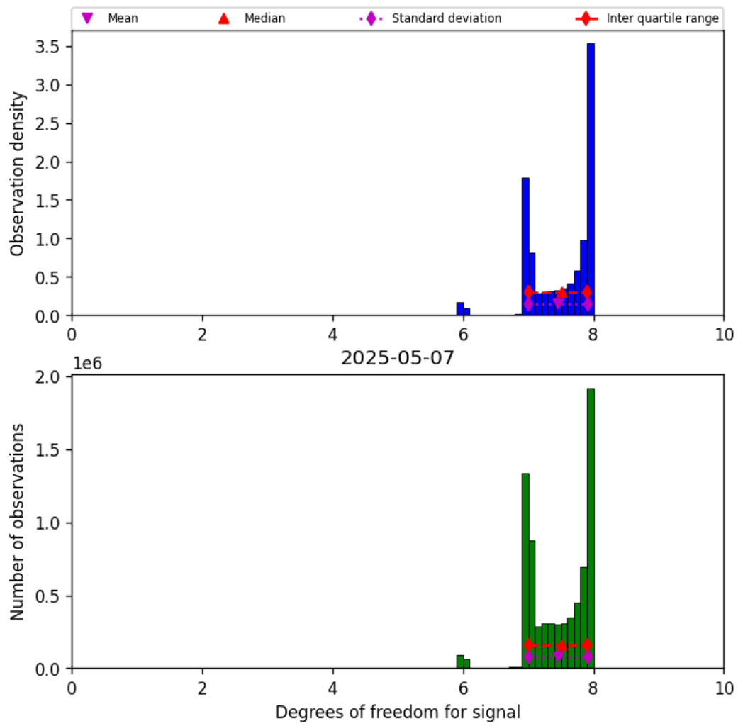
Figure 18: Histogram of “Degrees of freedom for signal” for 2025-05-07 to 2025-05-08
