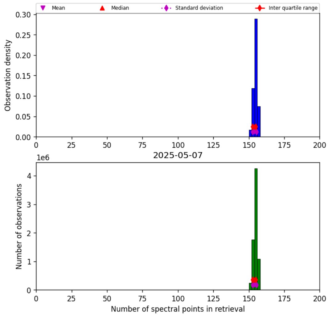
Figure 16: Histogram of “Number of spectral points in retrieval” for 2025-05-07 to 2025-05-08
