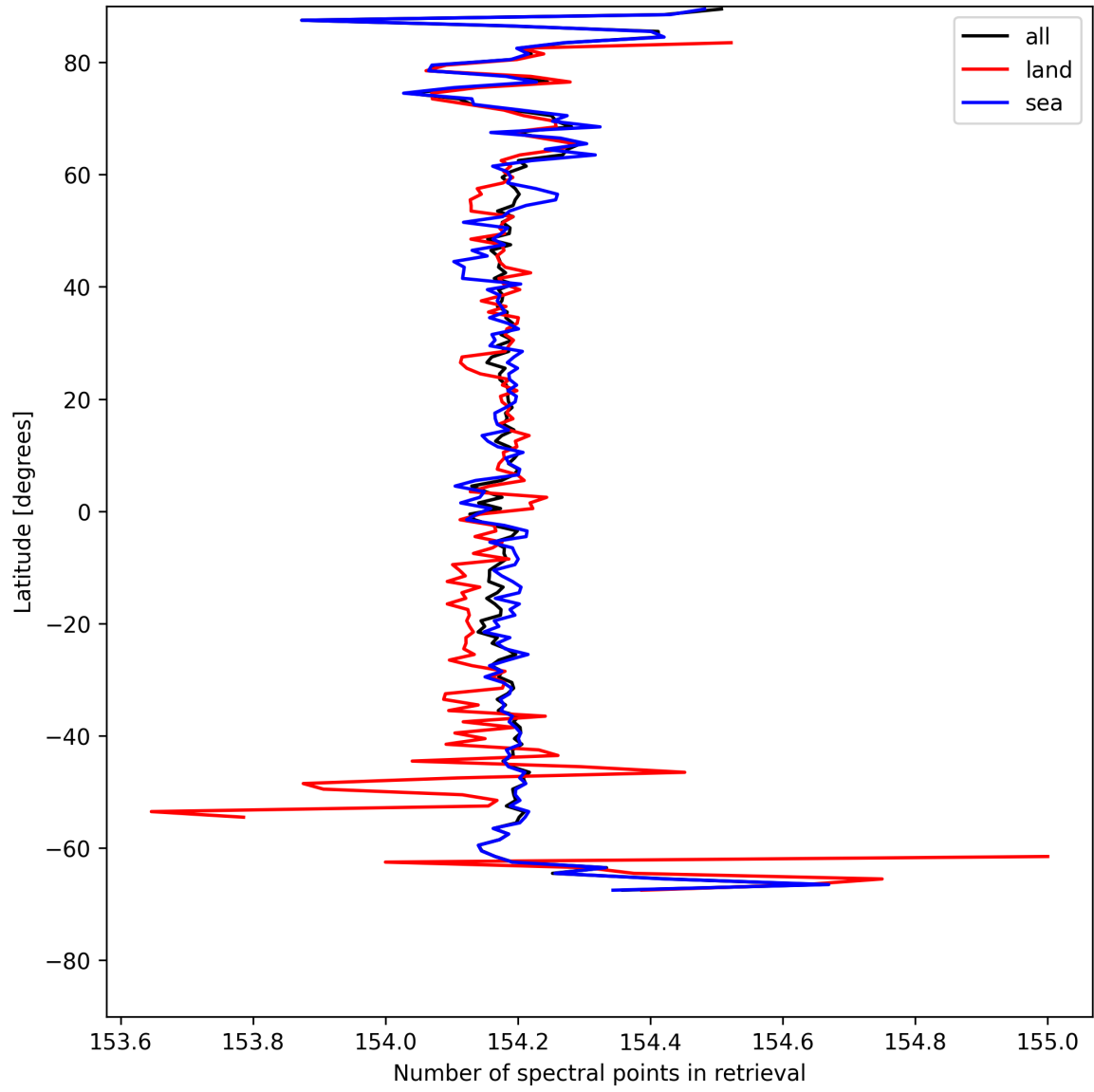
Figure 9: Zonal average of “Number of spectral points in retrieval” for 2025-05-07 to 2025-05-08.
