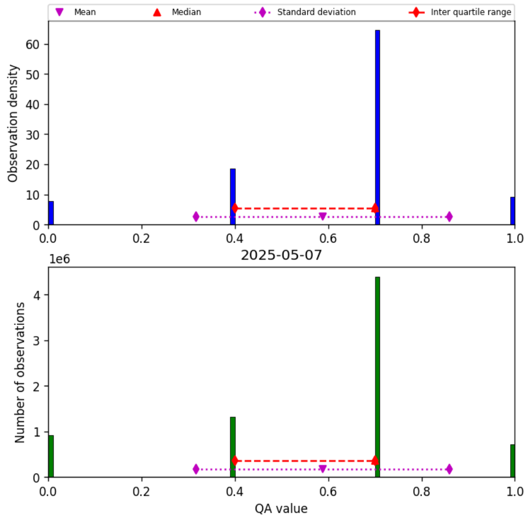
Figure 13: Histogram of “QA value” for 2025-05-07 to 2025-05-08
