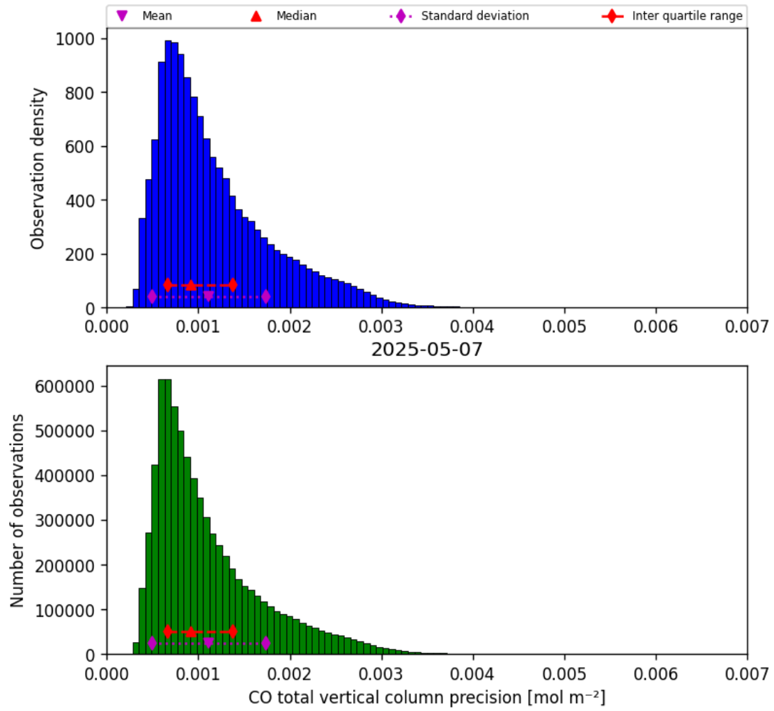
Figure 15: Histogram of “CO total vertical column precision” for 2025-05-07 to 2025-05-08
