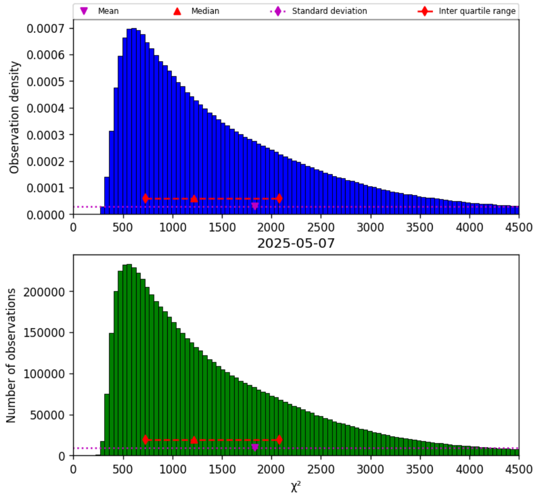
Figure 17: Histogram of " \chi^2 " for 2025-05-07 to 2025-05-08
