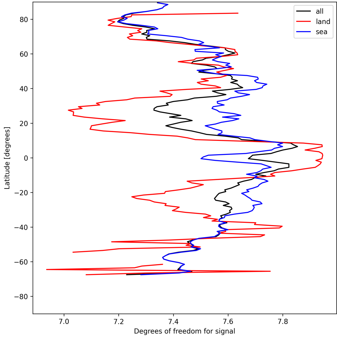
Figure 11: Zonal average of “Degrees of freedom for signal” for 2025-05-07 to 2025-05-08.
