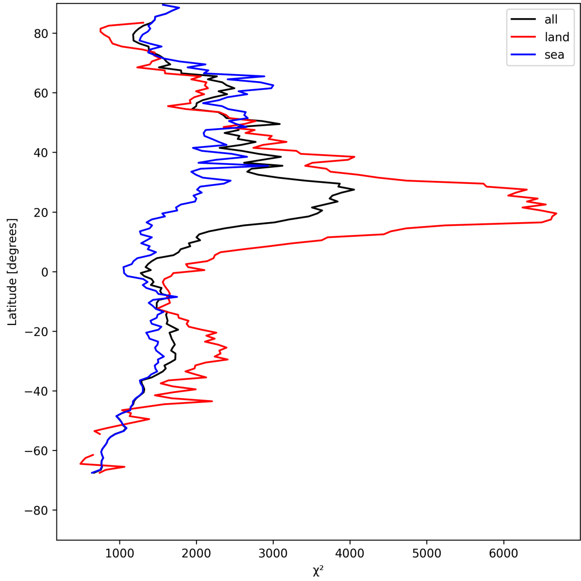
Figure 10: Zonal average of “ \chi^2 ” for 2025-05-07 to 2025-05-08.
