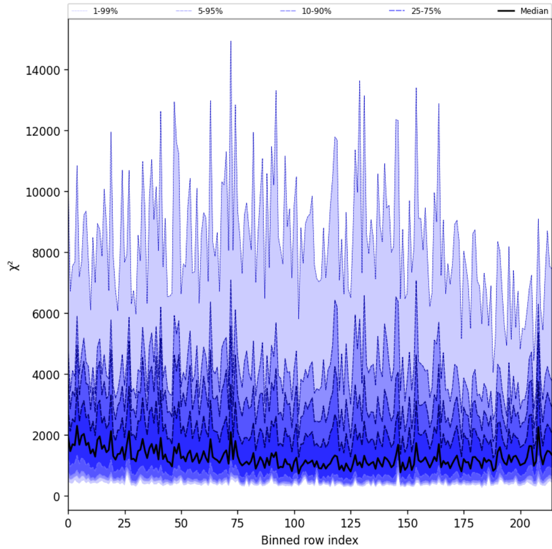
Figure 24: Along track statistics of “ \chi^2 ” for 2025-05-07 to 2025-05-08
