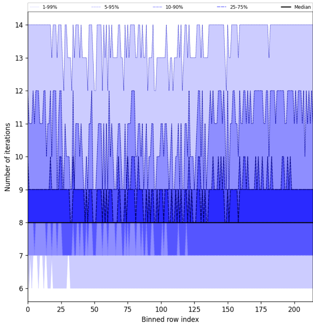
Figure 26: Along track statistics of “Number of iterations” for 2025-05-07 to 2025-05-08
