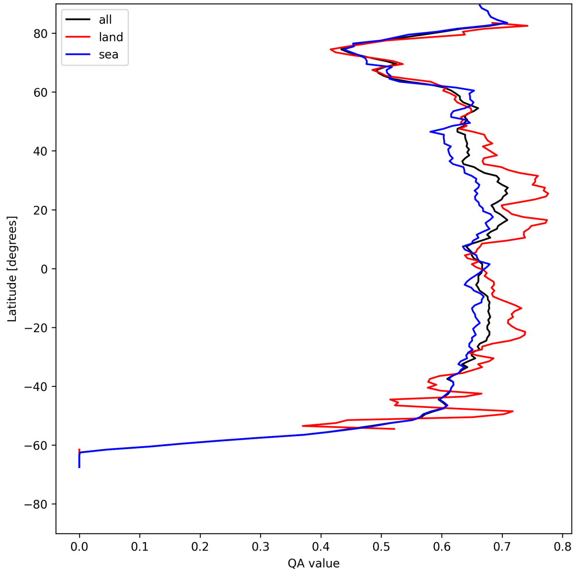
Figure 6: Zonal average of “QA value” for 2025-05-07 to 2025-05-08.
