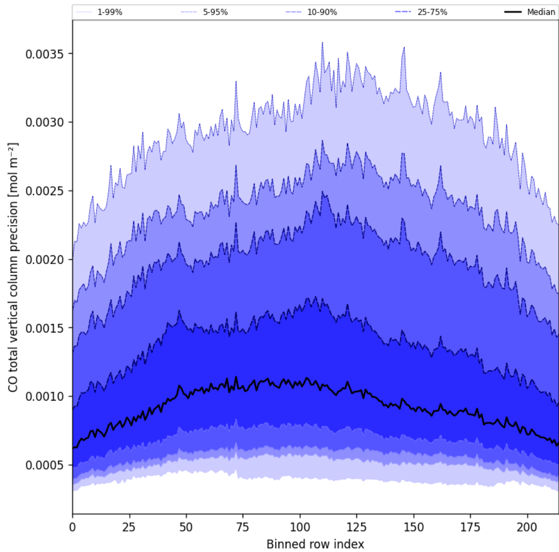
Figure 22: Along track statistics of “CO total vertical column precision” for 2025-05-07 to 2025-05-08
