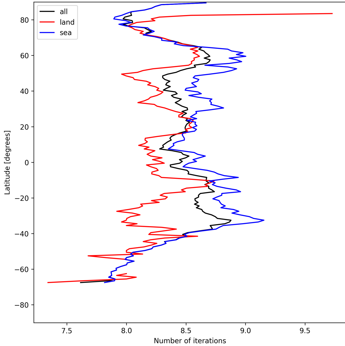
Figure 12: Zonal average of “Number of iterations” for 2025-05-08 to 2025-05-08.
