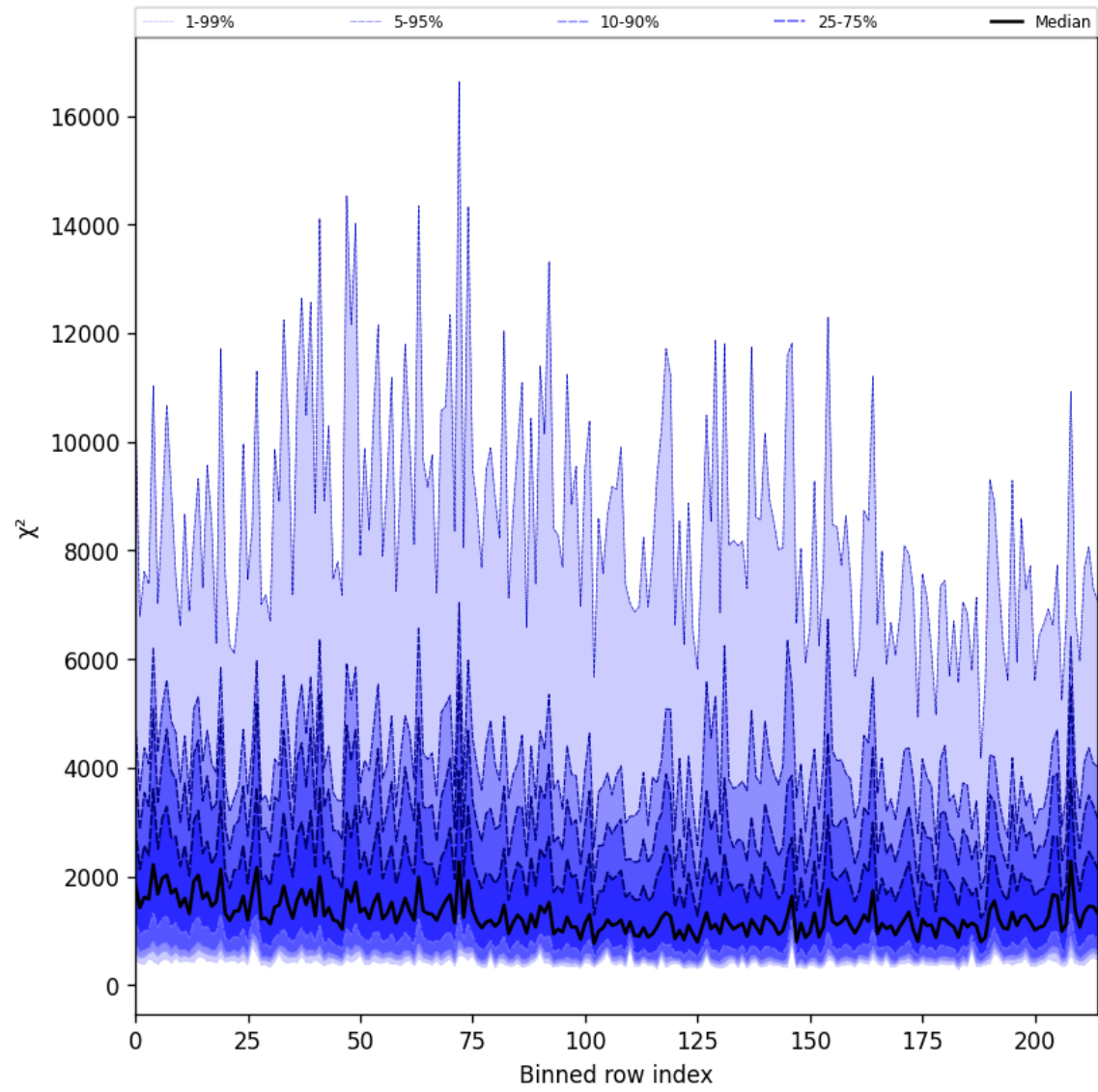
Figure 24: Along track statistics of “ \chi^2 ” for 2025-05-08 to 2025-05-08
