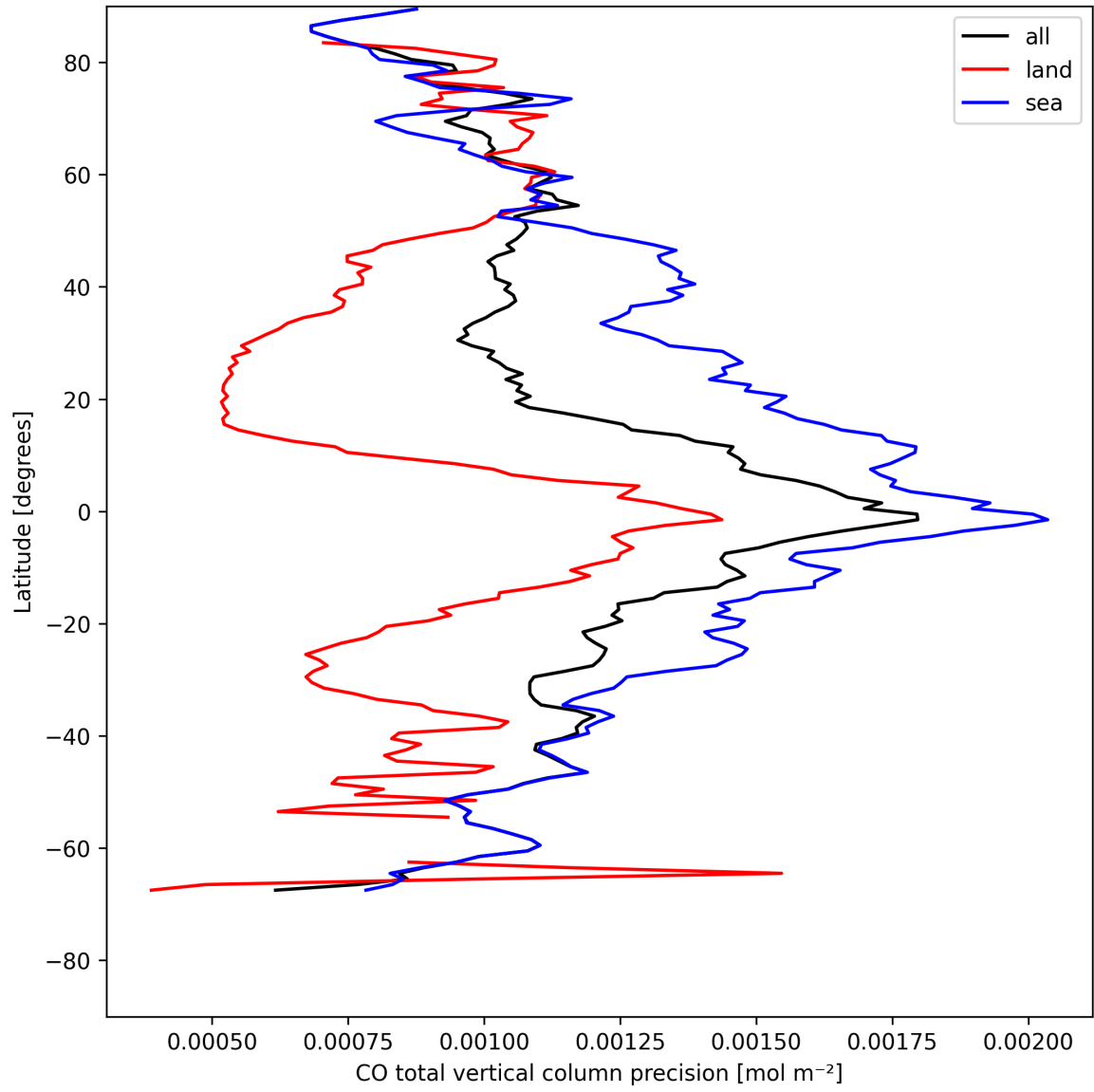
Figure 8: Zonal average of “CO total vertical column precision” for 2025-05-08 to 2025-05-08.
