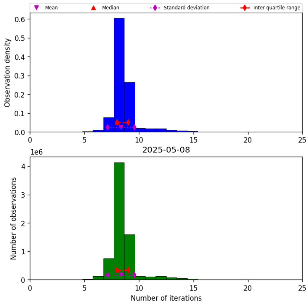
Figure 19: Histogram of “Number of iterations” for 2025-05-08 to 2025-05-08
