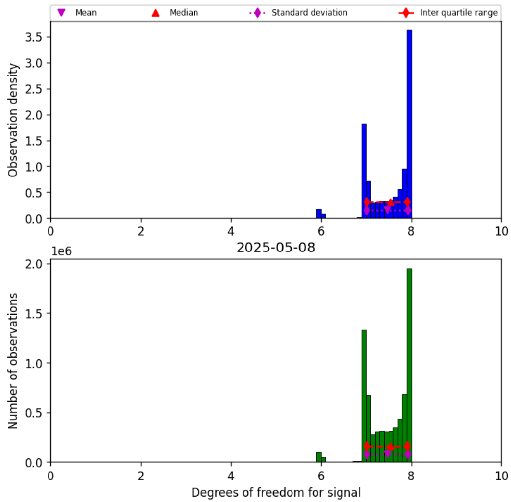
Figure 18: Histogram of “Degrees of freedom for signal” for 2025-05-08 to 2025-05-08
