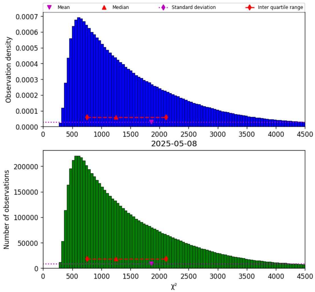
Figure 17: Histogram of " \chi^2 " for 2025-05-08 to 2025-05-08
