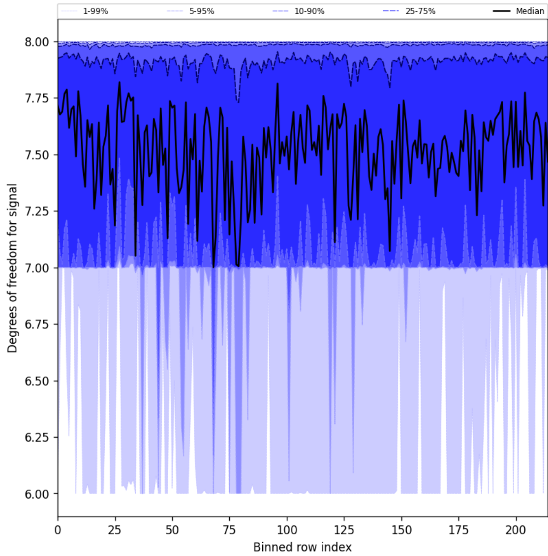
Figure 25: Along track statistics of “Degrees of freedom for signal” for 2025-05-08 to 2025-05-08
