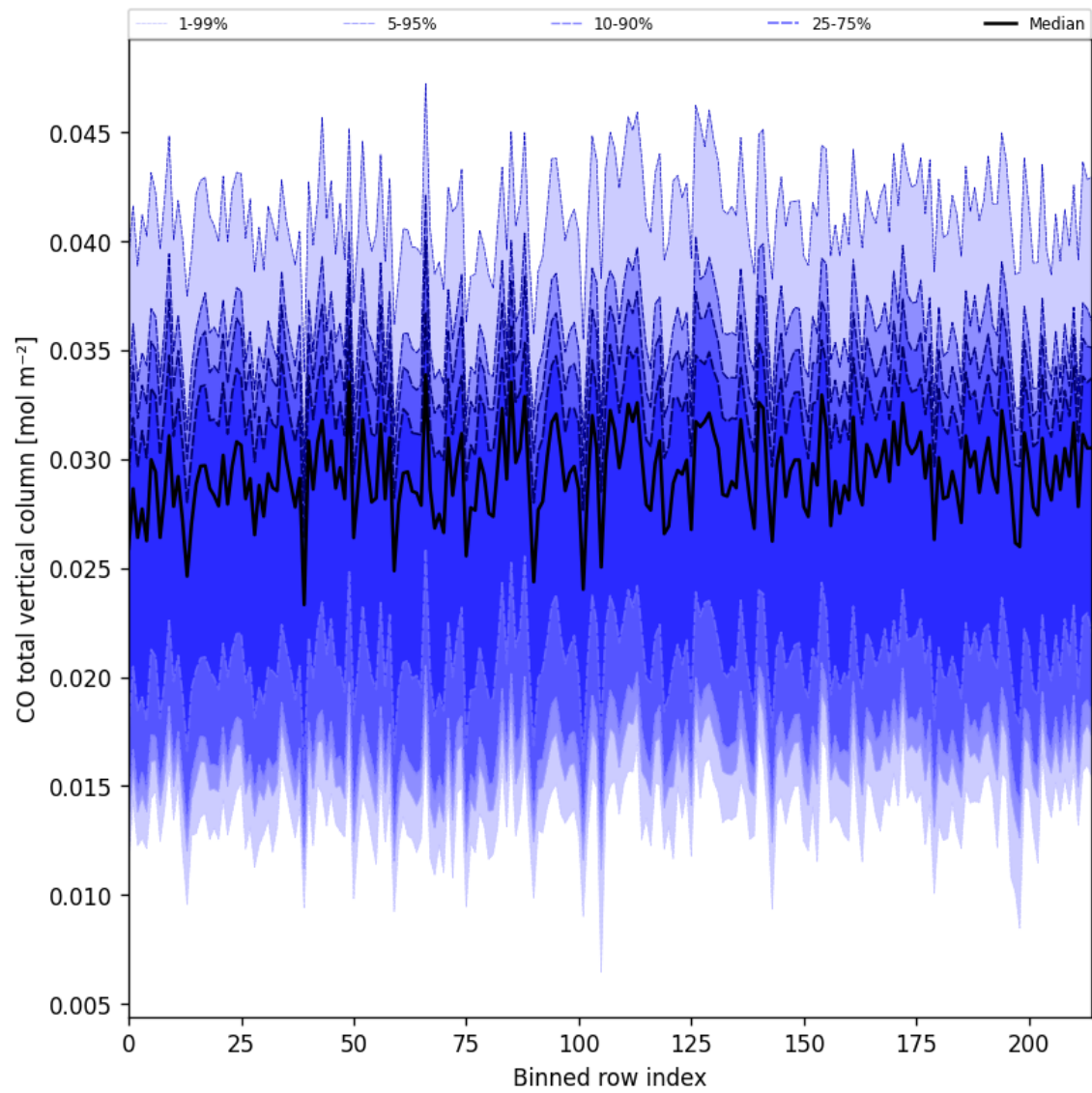
Figure 21: Along track statistics of "CO total vertical column" for 2025-05-08 to 2025-05-08
