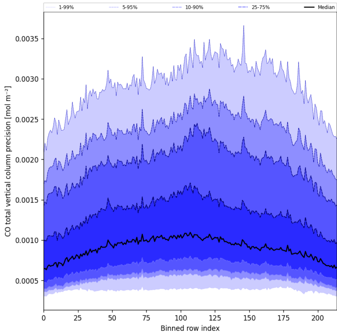
Figure 22: Along track statistics of “CO total vertical column precision” for 2025-05-08 to 2025-05-08
