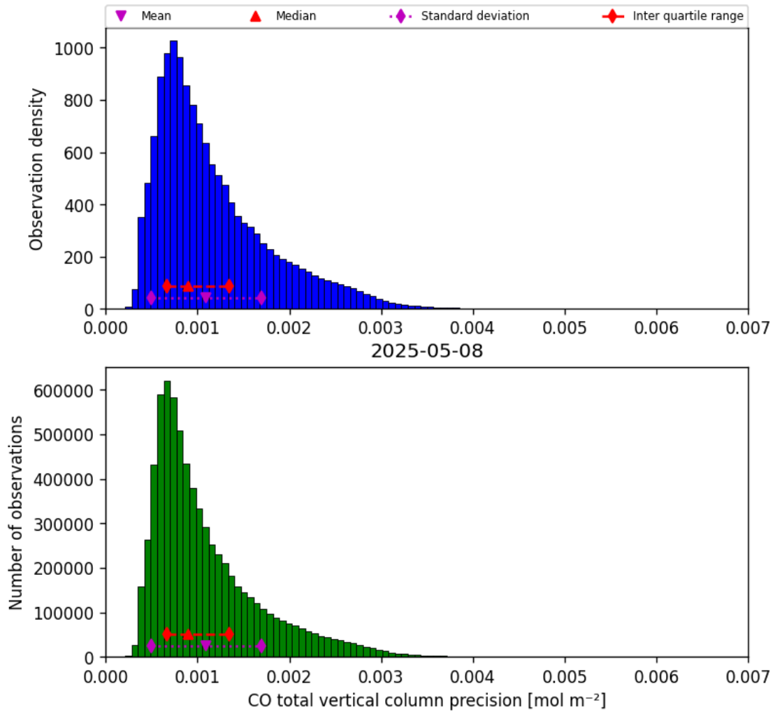
Figure 15: Histogram of “CO total vertical column precision” for 2025-05-08 to 2025-05-08
