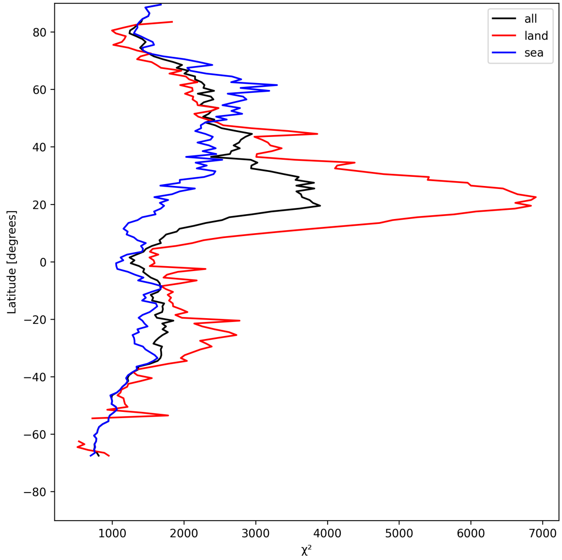
Figure 10: Zonal average of “ \chi^2 ” for 2025-05-08 to 2025-05-08.
