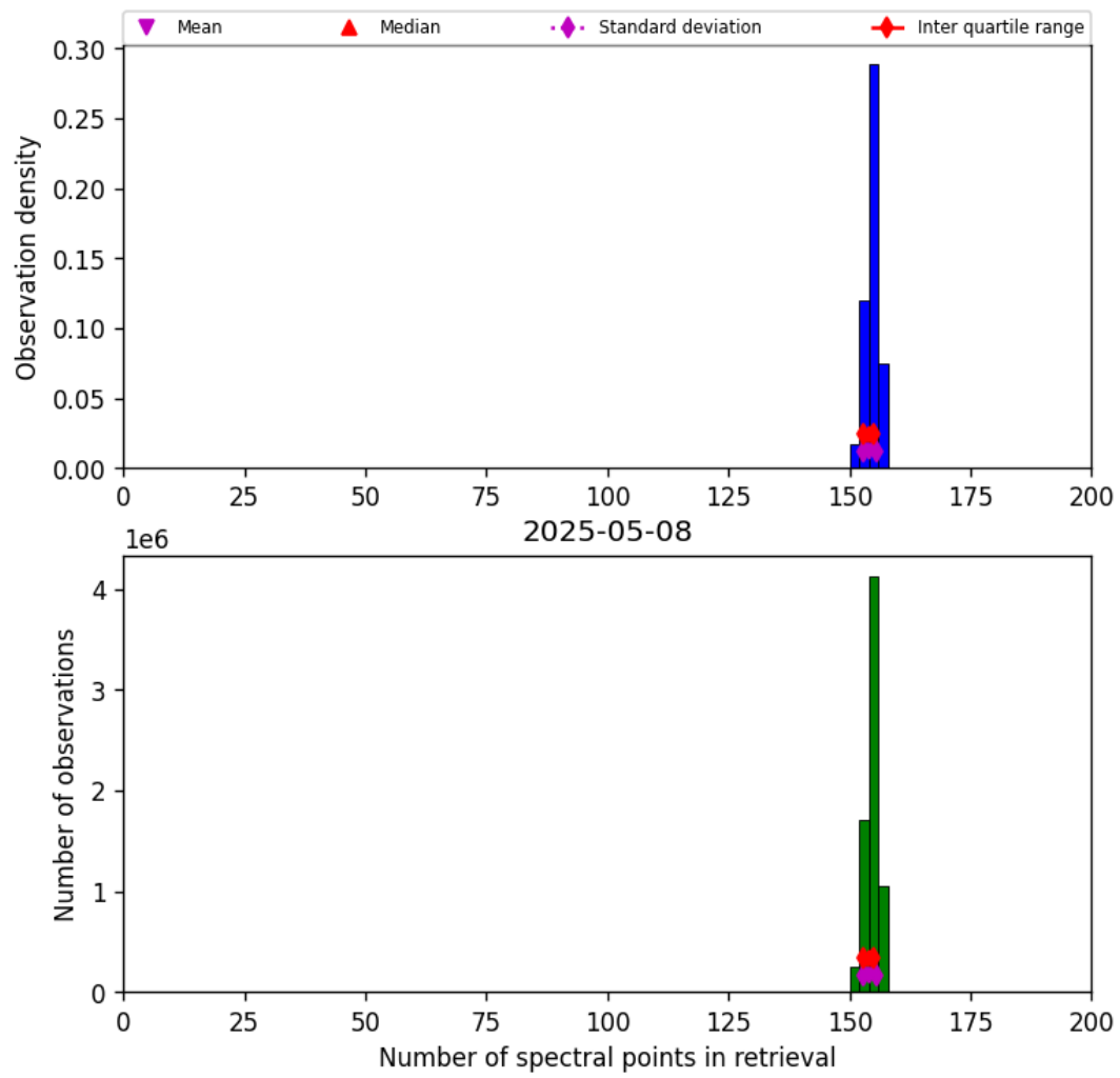
Figure 16: Histogram of “Number of spectral points in retrieval” for 2025-05-08 to 2025-05-08
