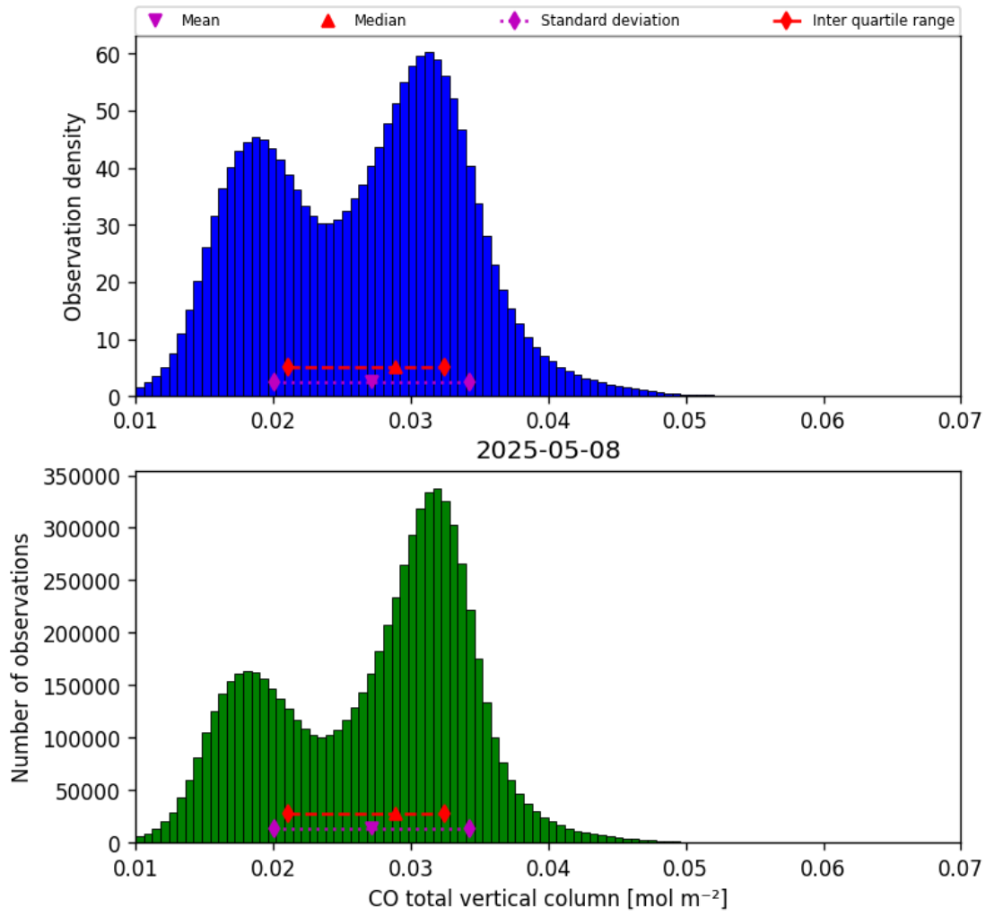
Figure 14: Histogram of “CO total vertical column” for 2025-05-08 to 2025-05-08
