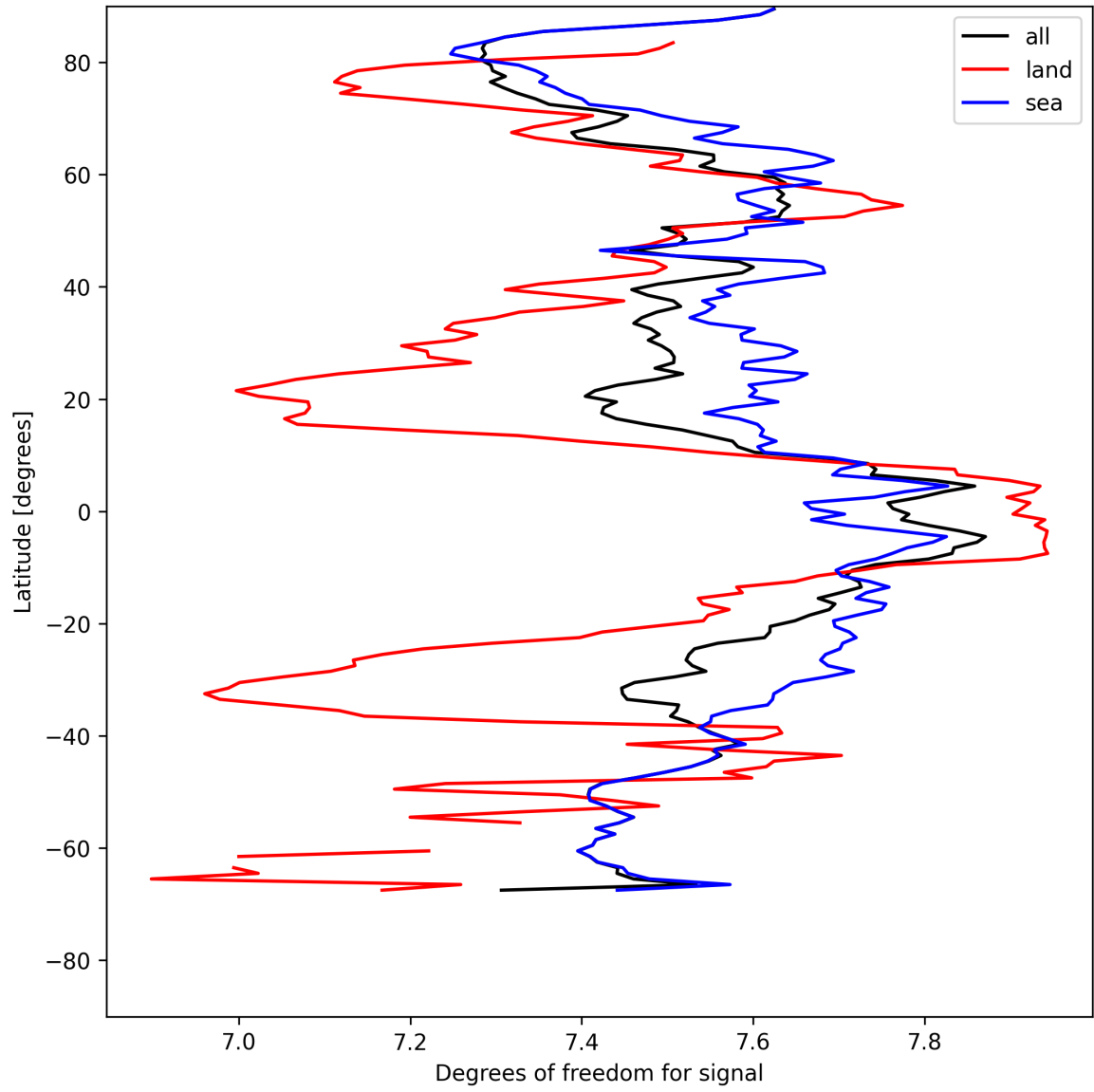
Figure 11: Zonal average of “Degrees of freedom for signal” for 2025-05-09 to 2025-05-10.
