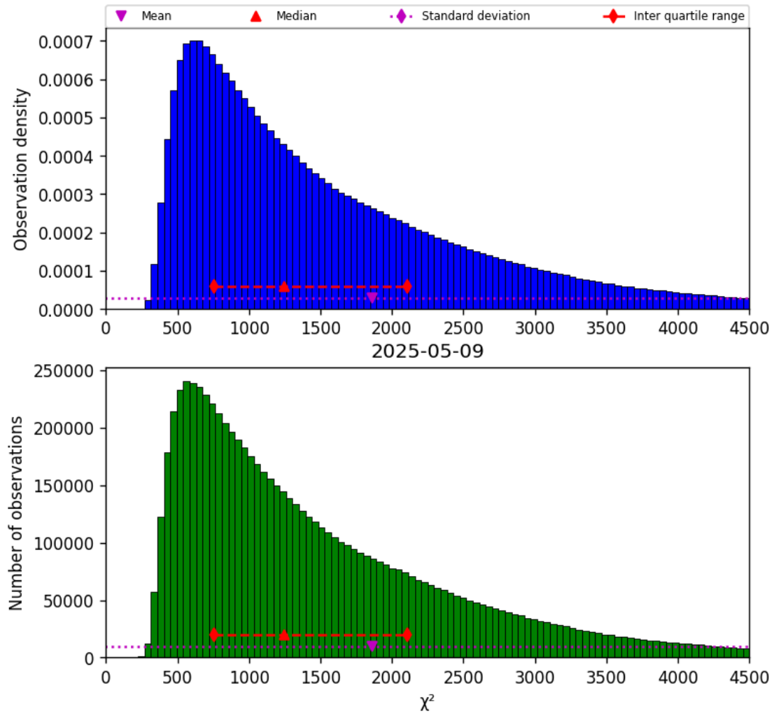
Figure 17: Histogram of “ \chi^2 ” for 2025-05-09 to 2025-05-10
