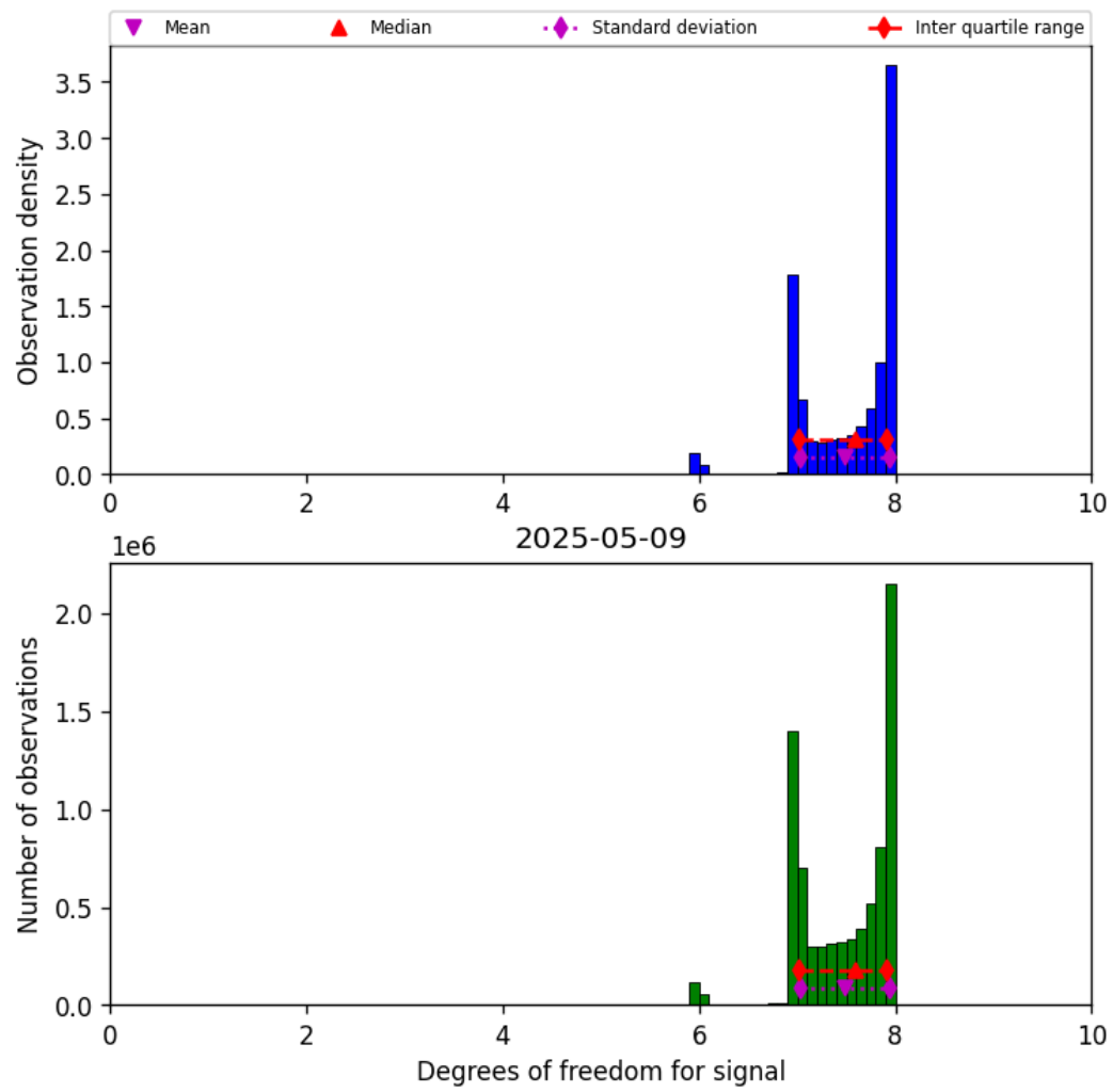
Figure 18: Histogram of “Degrees of freedom for signal” for 2025-05-09 to 2025-05-10
