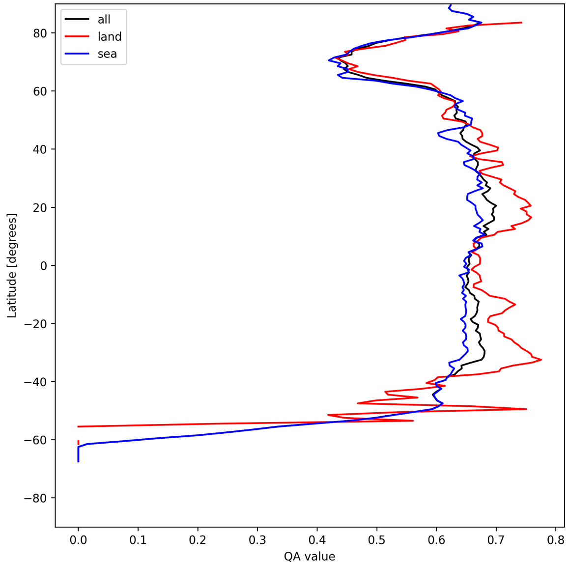
Figure 6: Zonal average of “QA value” for 2025-05-09 to 2025-05-10.
