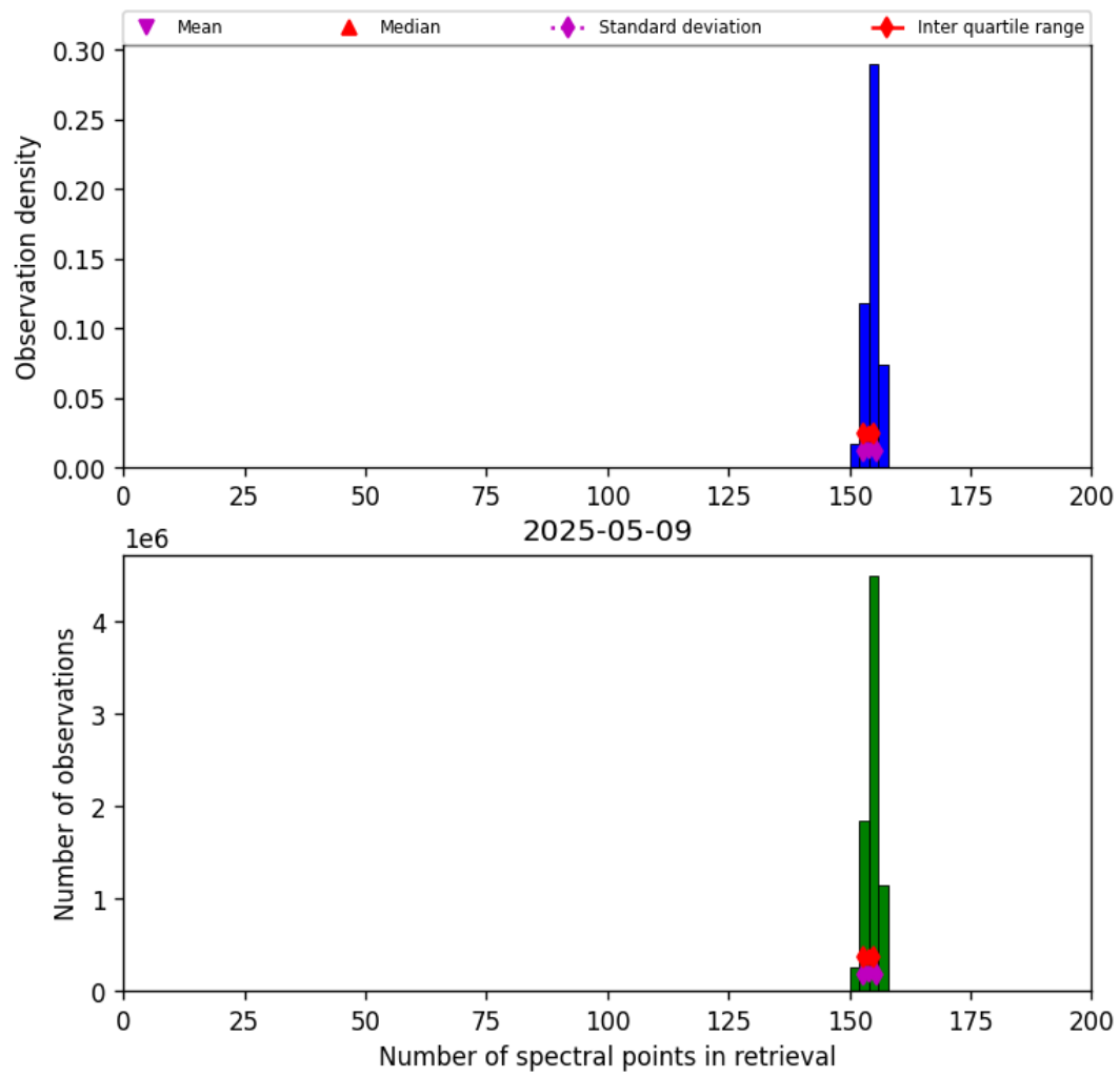
Figure 16: Histogram of “Number of spectral points in retrieval” for 2025-05-09 to 2025-05-10
