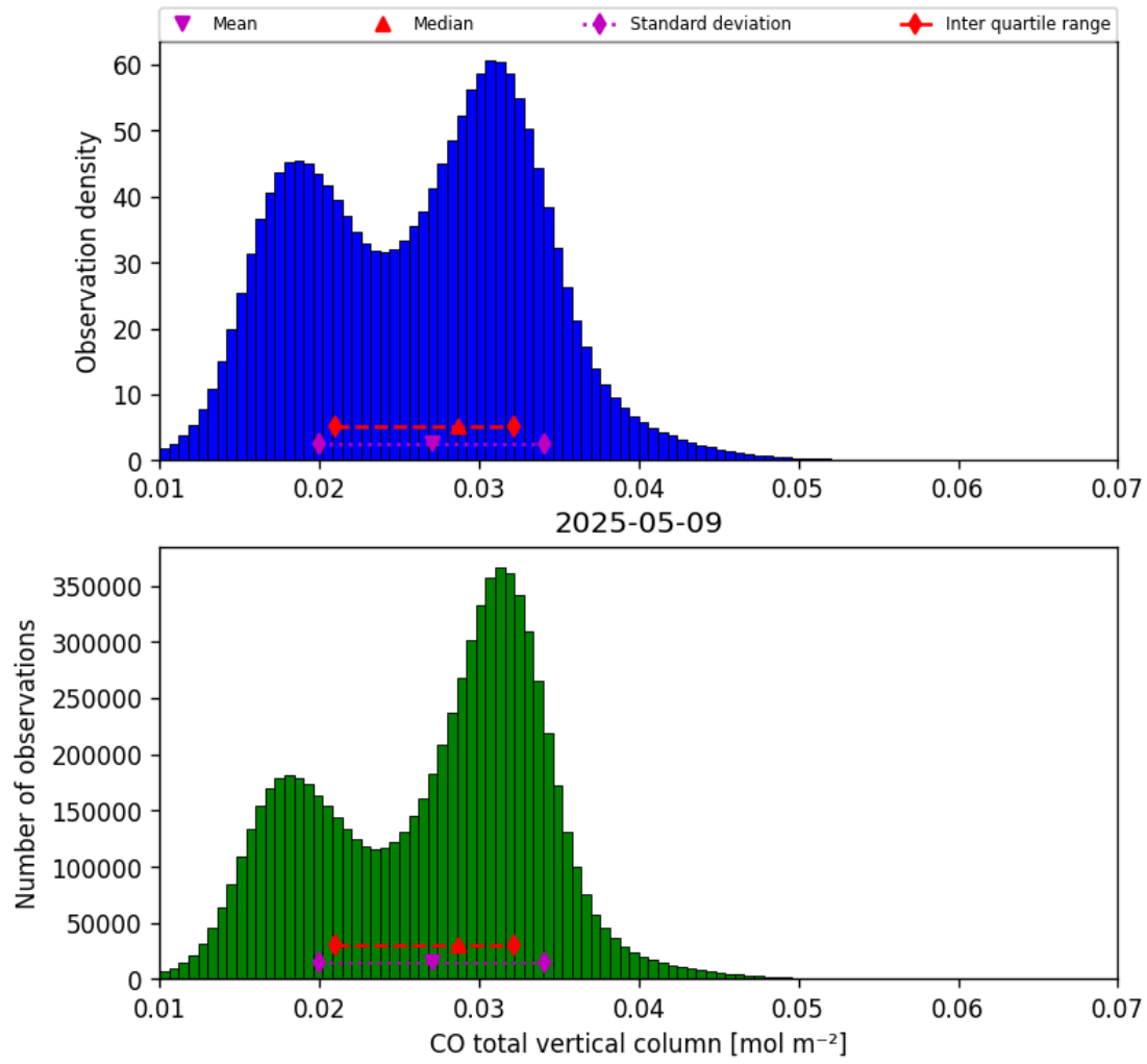
Figure 14: Histogram of “CO total vertical column” for 2025-05-09 to 2025-05-10
