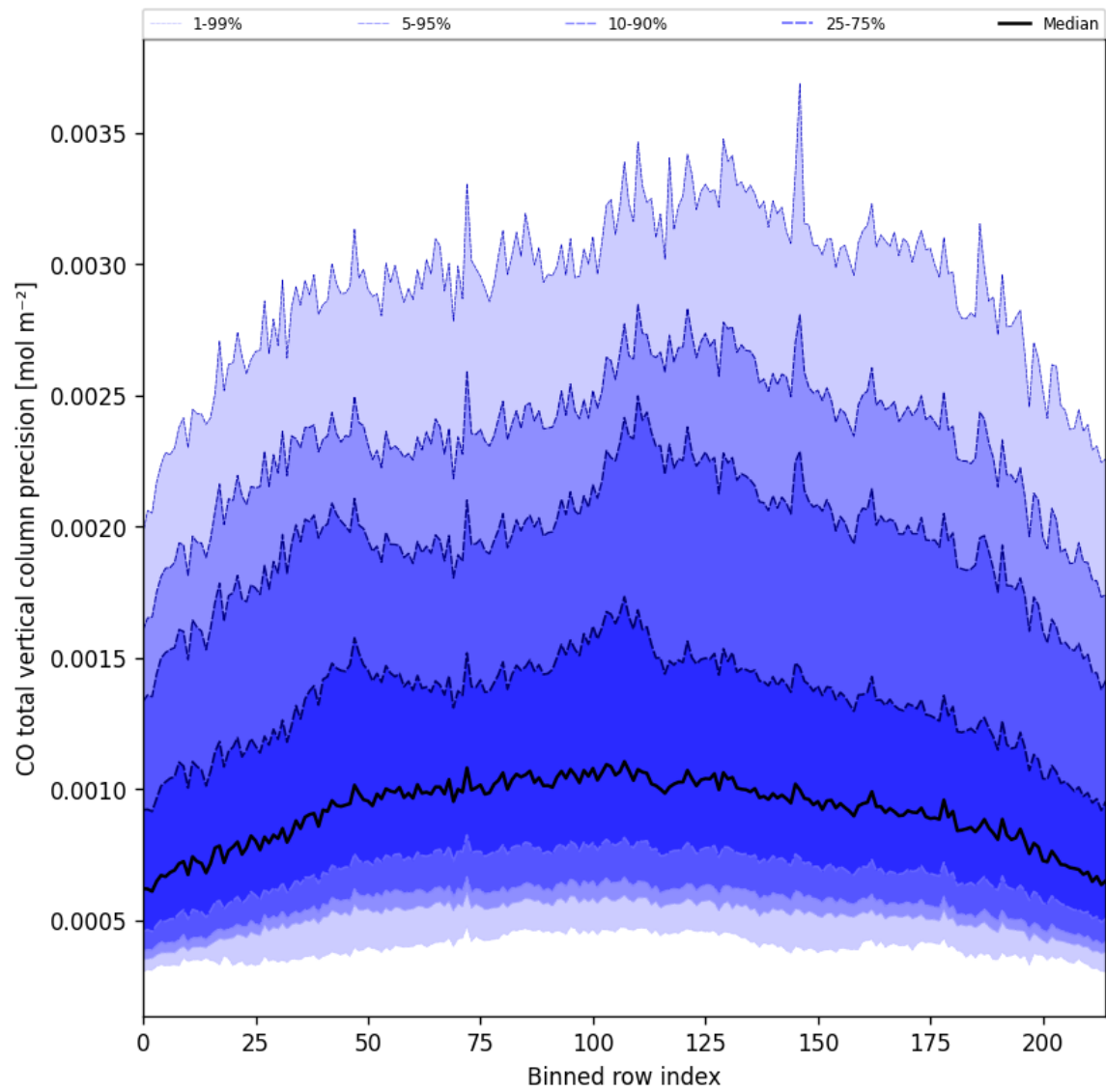
Figure 22: Along track statistics of “CO total vertical column precision” for 2025-05-09 to 2025-05-10
