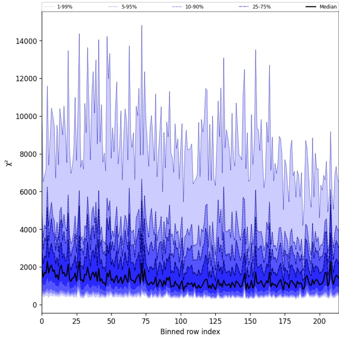
Figure 24: Along track statistics of “ \chi^2 ” for 2025-05-09 to 2025-05-10
