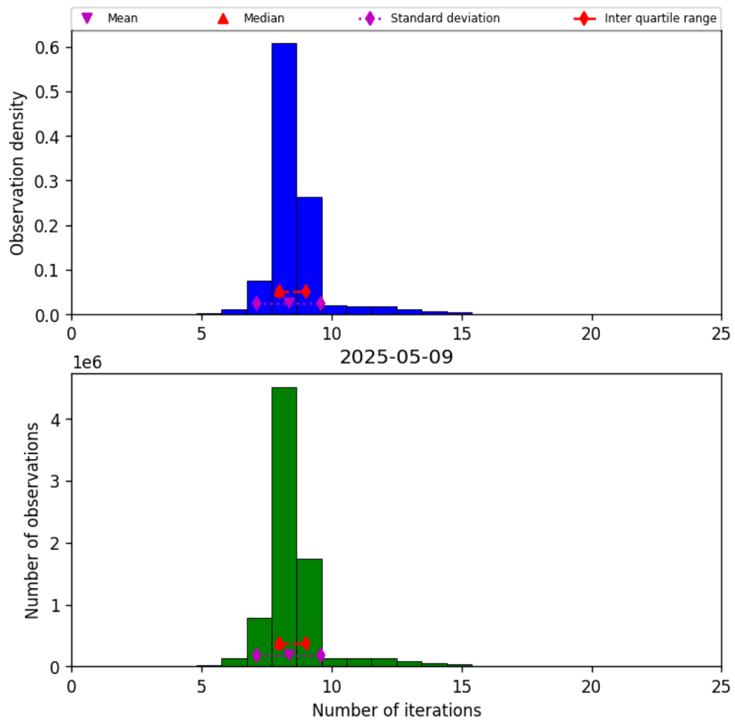
Figure 19: Histogram of “Number of iterations” for 2025-05-09 to 2025-05-10
