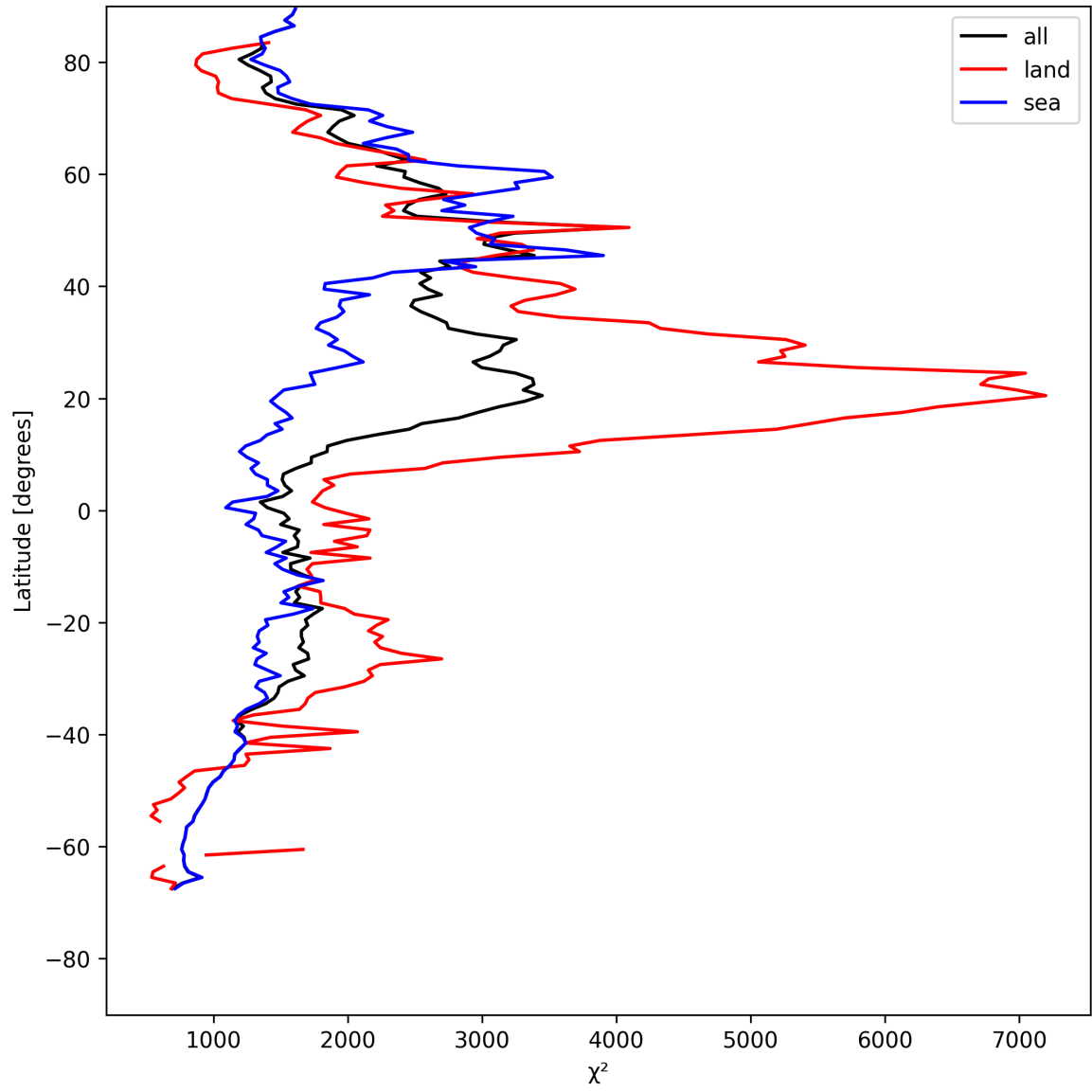
Figure 10: Zonal average of “ \chi^2 ” for 2025-05-09 to 2025-05-10.
