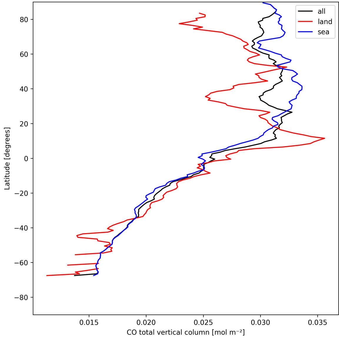
Figure 7: Zonal average of “CO total vertical column” for 2025-05-09 to 2025-05-10.
