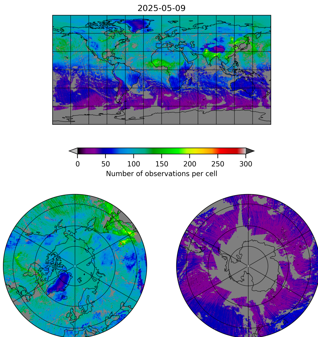
Figure 5: Map of the number of observations for 2025-05-09 to 2025-05-10
