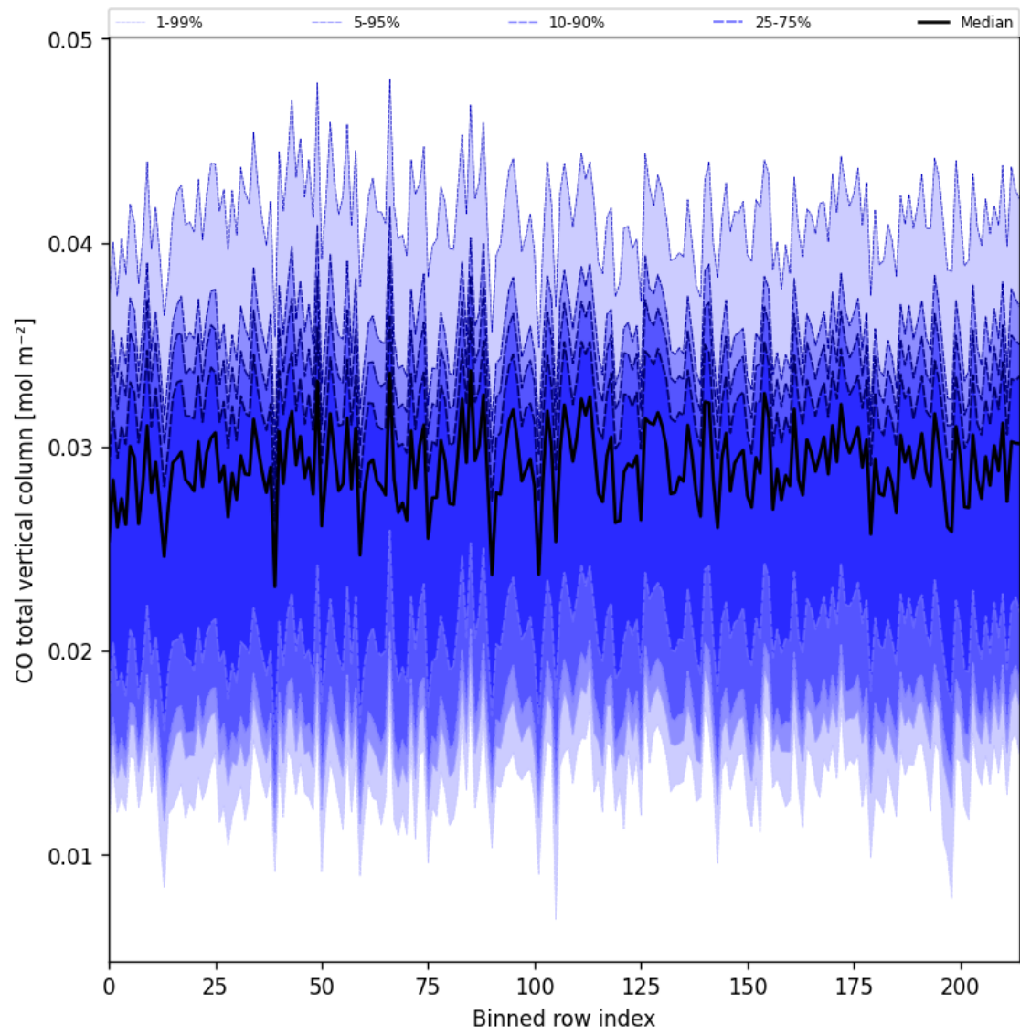
Figure 21: Along track statistics of “CO total vertical column” for 2025-05-09 to 2025-05-10
