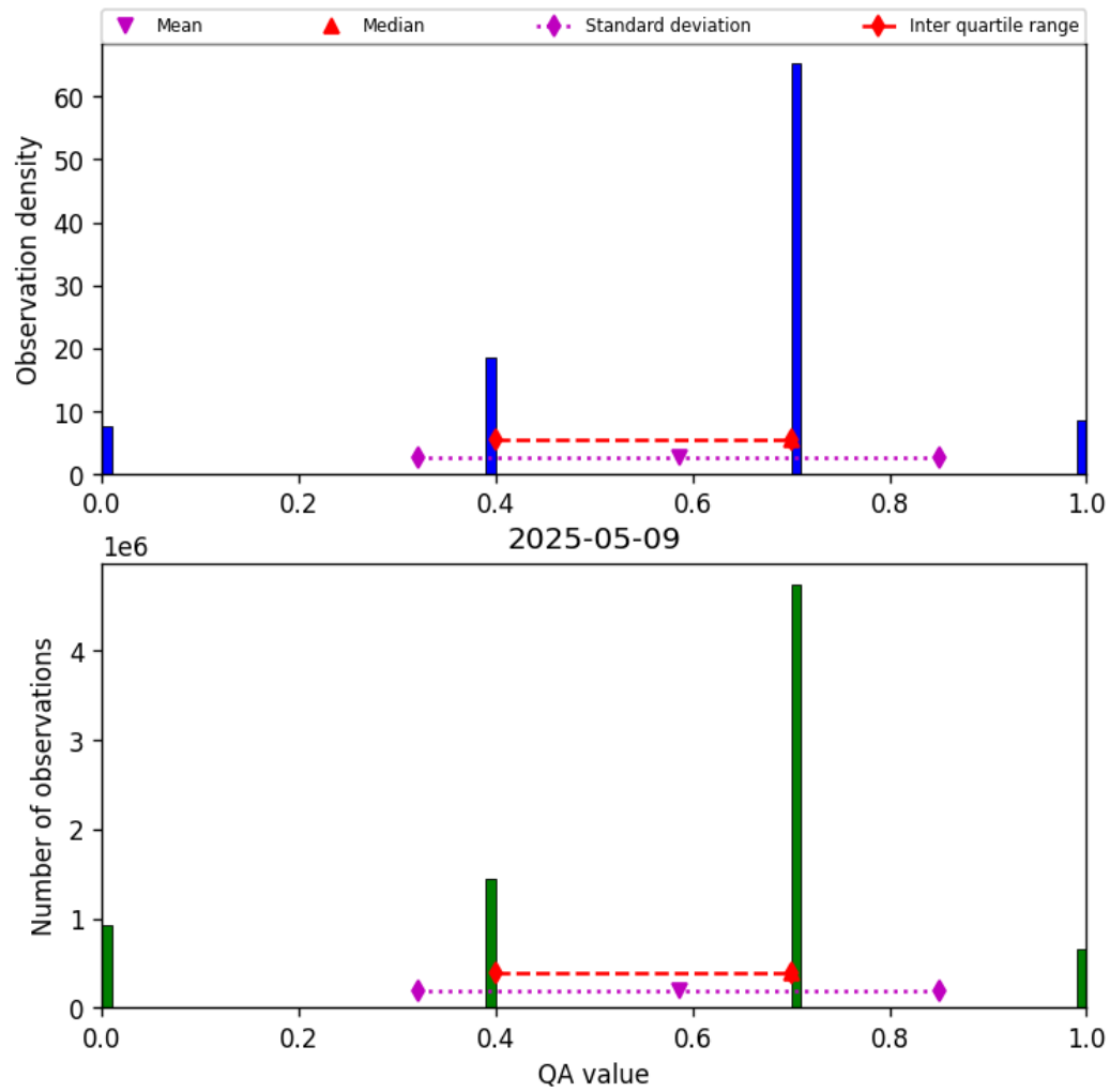
Figure 13: Histogram of “QA value” for 2025-05-09 to 2025-05-10
