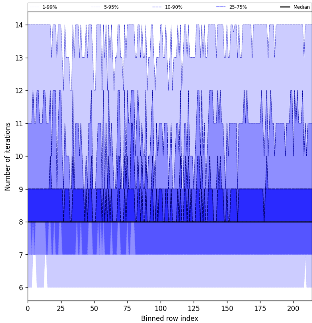
Figure 26: Along track statistics of “Number of iterations” for 2025-05-09 to 2025-05-10
