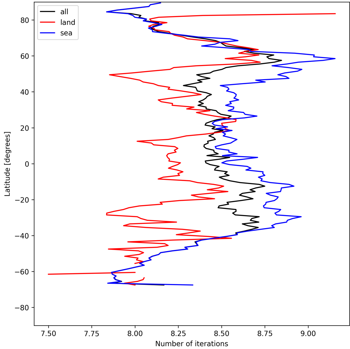
Figure 12: Zonal average of “Number of iterations” for 2025-05-09 to 2025-05-10.
