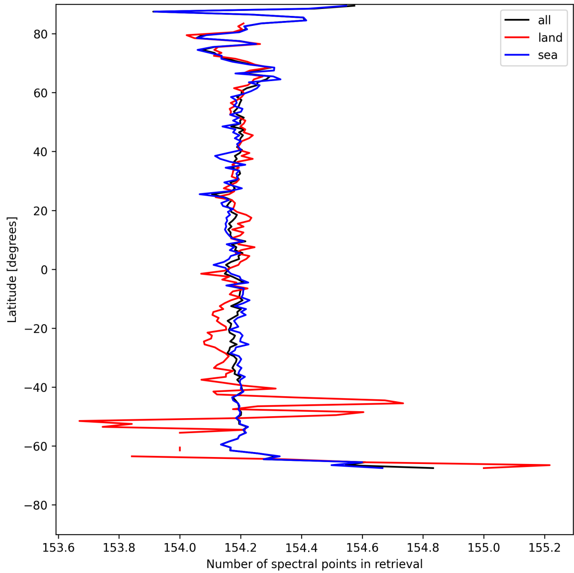
Figure 9: Zonal average of “Number of spectral points in retrieval” for 2025-05-09 to 2025-05-10.
