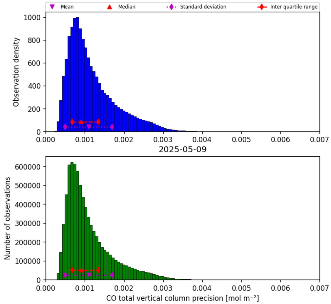
Figure 15: Histogram of “CO total vertical column precision” for 2025-05-09 to 2025-05-10
