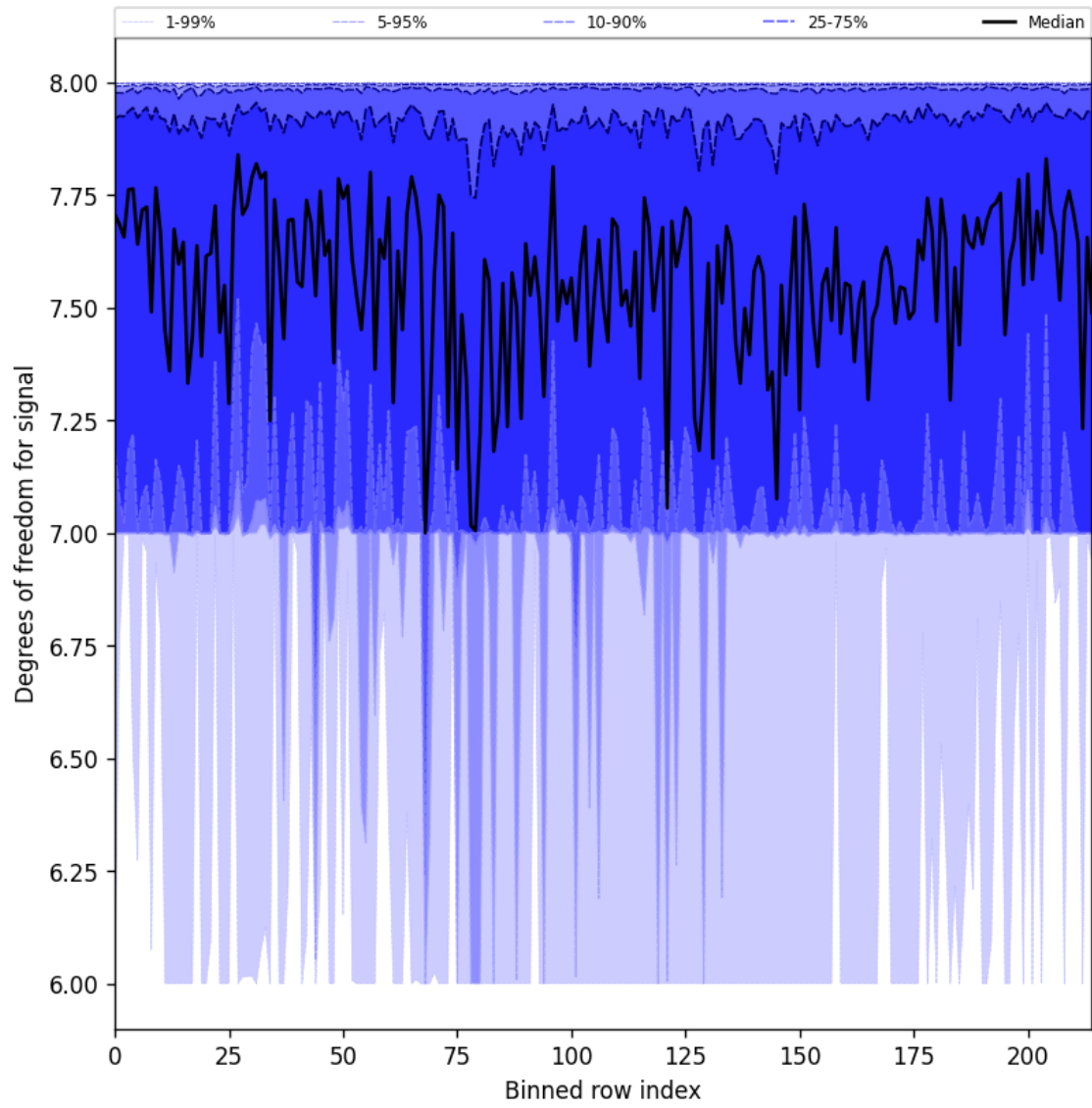
Figure 25: Along track statistics of “Degrees of freedom for signal” for 2025-05-09 to 2025-05-10
