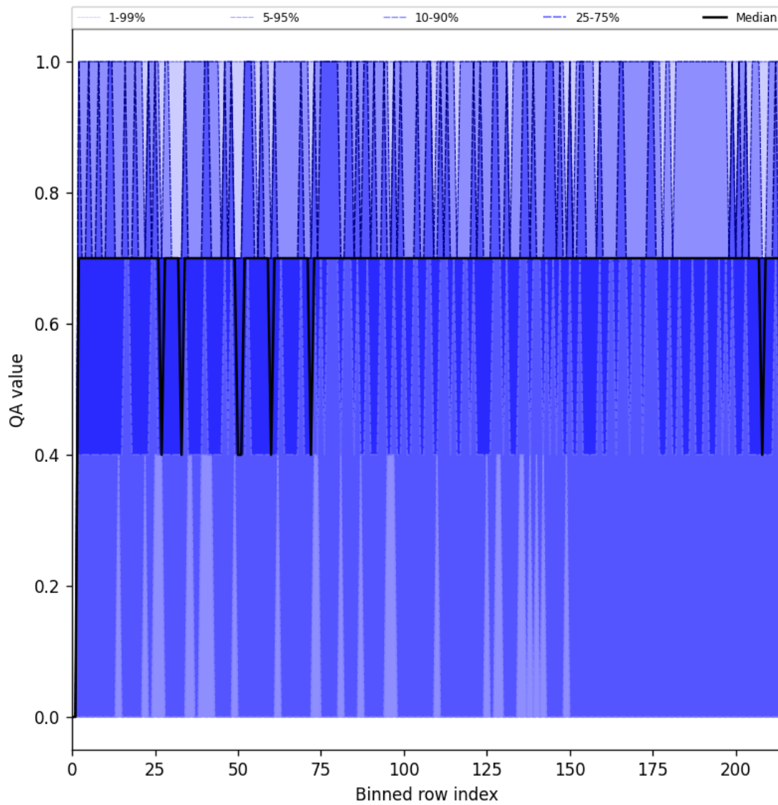
Figure 20: Along track statistics of “QA value” for 2025-05-09 to 2025-05-10
