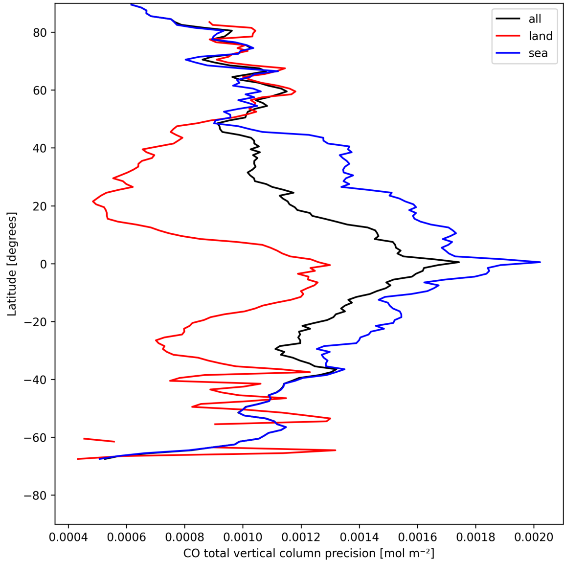
Figure 8: Zonal average of “CO total vertical column precision” for 2025-05-09 to 2025-05-10.
