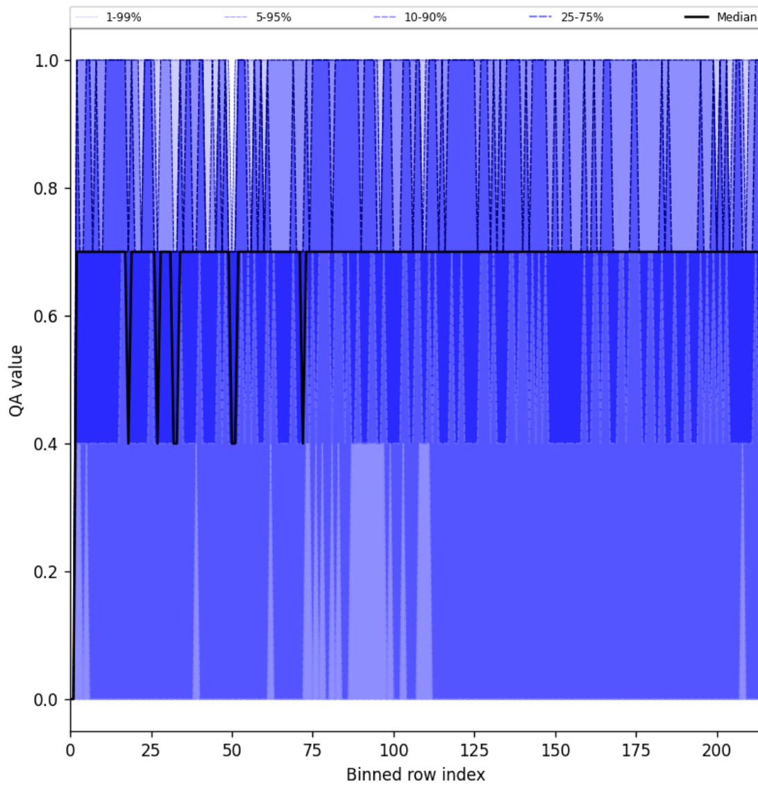
Figure 20: Along track statistics of “QA value” for 2025-05-11 to 2025-05-12
