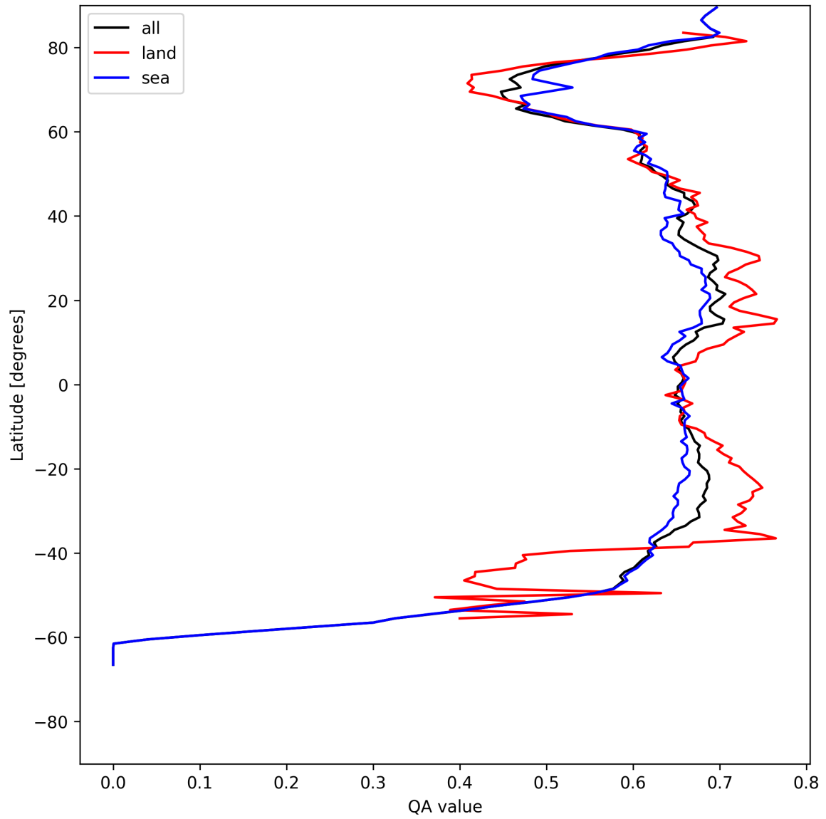
Figure 6: Zonal average of “QA value” for 2025-05-11 to 2025-05-12.
