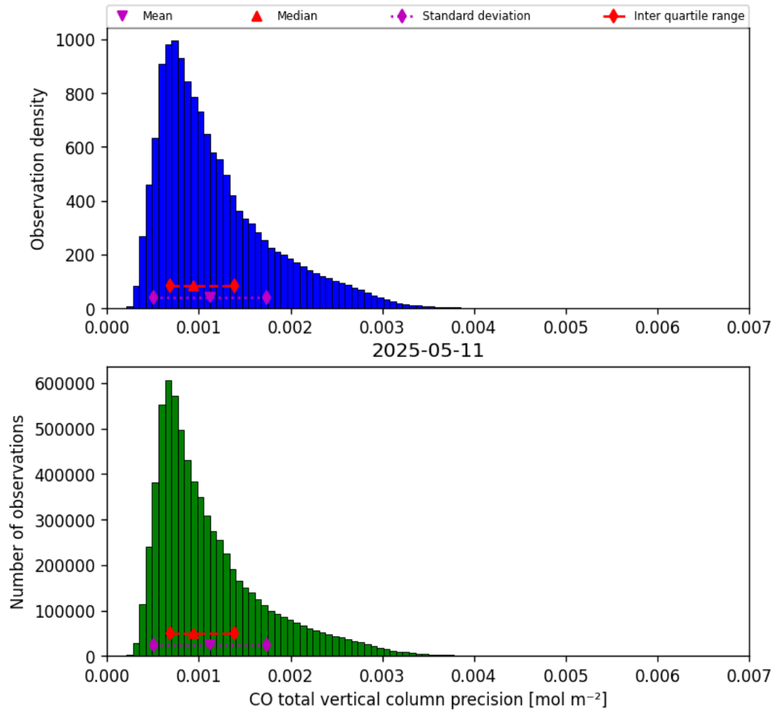
Figure 15: Histogram of “CO total vertical column precision” for 2025-05-11 to 2025-05-12
