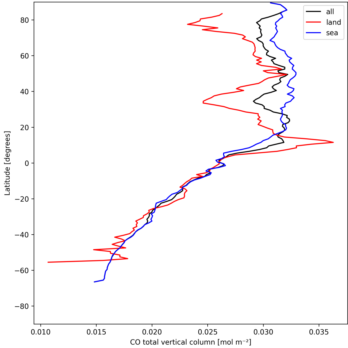
Figure 7: Zonal average of “CO total vertical column” for 2025-05-11 to 2025-05-12.
