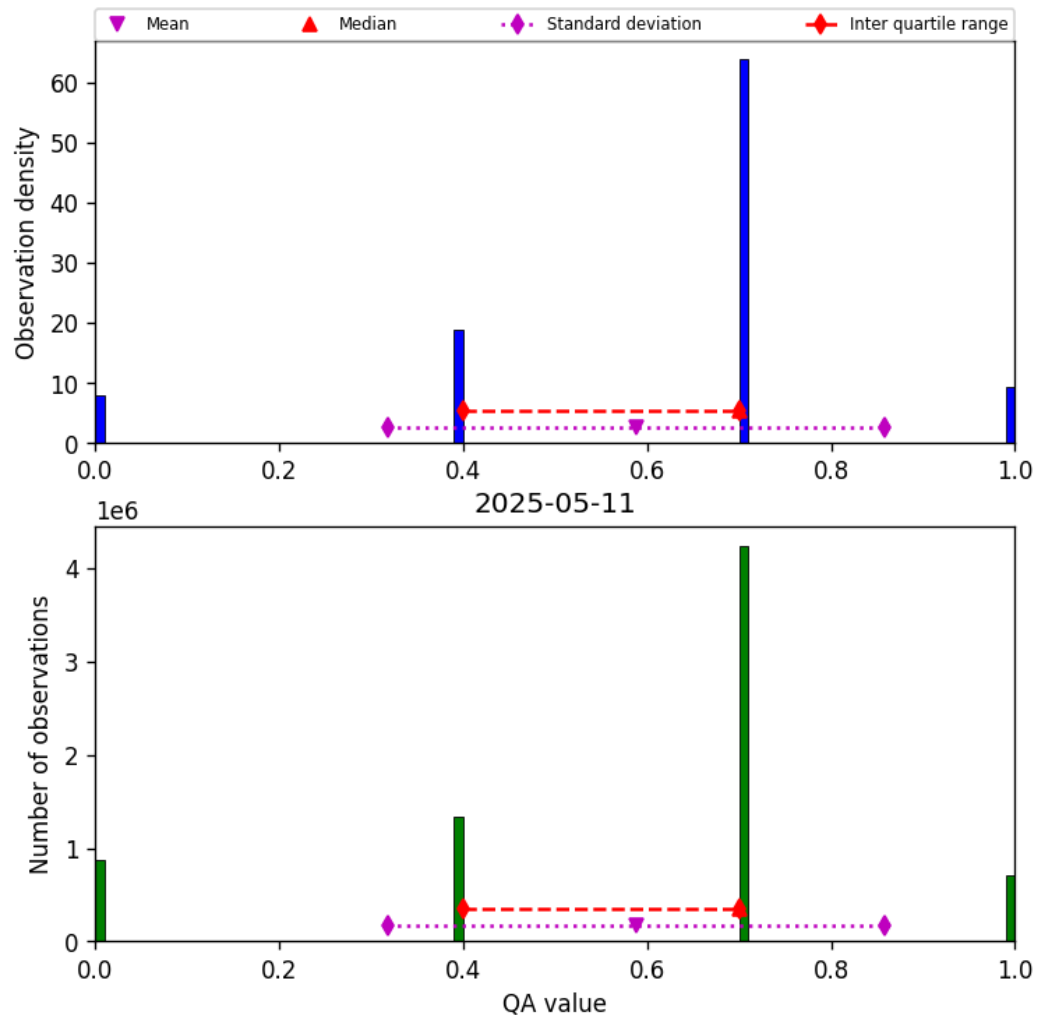
Figure 13: Histogram of “QA value” for 2025-05-11 to 2025-05-12
