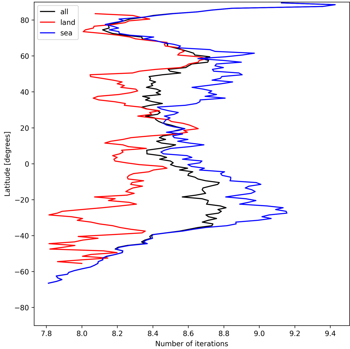
Figure 12: Zonal average of “Number of iterations” for 2025-05-11 to 2025-05-12.
