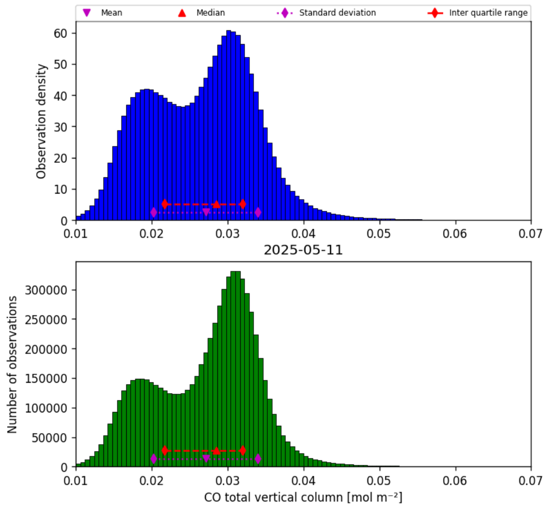
Figure 14: Histogram of “CO total vertical column” for 2025-05-11 to 2025-05-12
