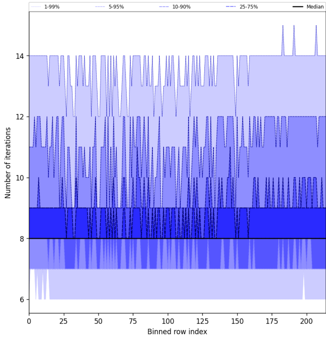
Figure 26: Along track statistics of “Number of iterations” for 2025-05-11 to 2025-05-12
