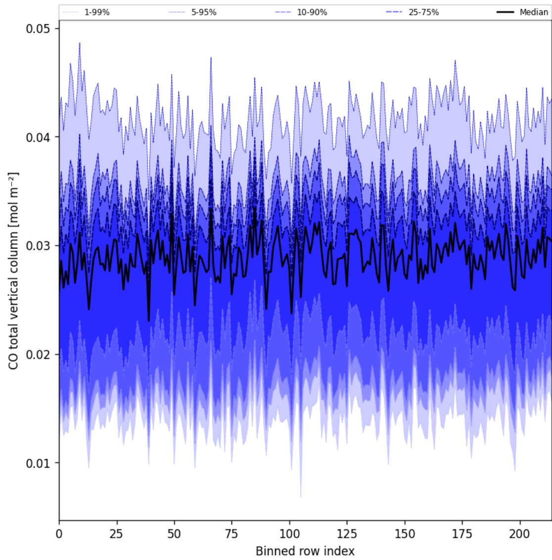
Figure 21: Along track statistics of “CO total vertical column” for 2025-05-11 to 2025-05-12
