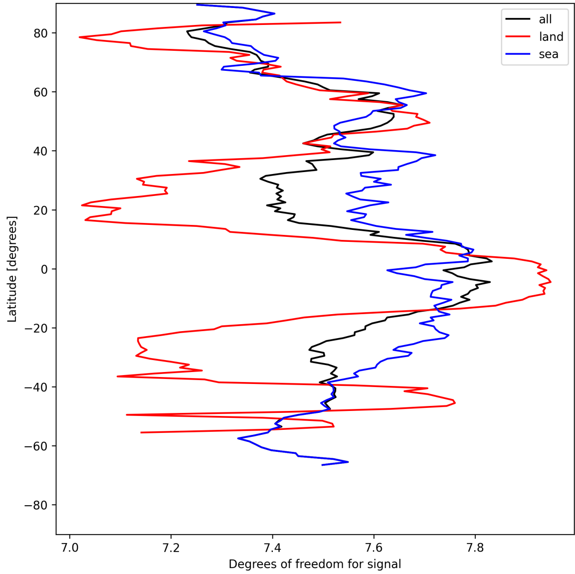
Figure 11: Zonal average of “Degrees of freedom for signal” for 2025-05-11 to 2025-05-12.
