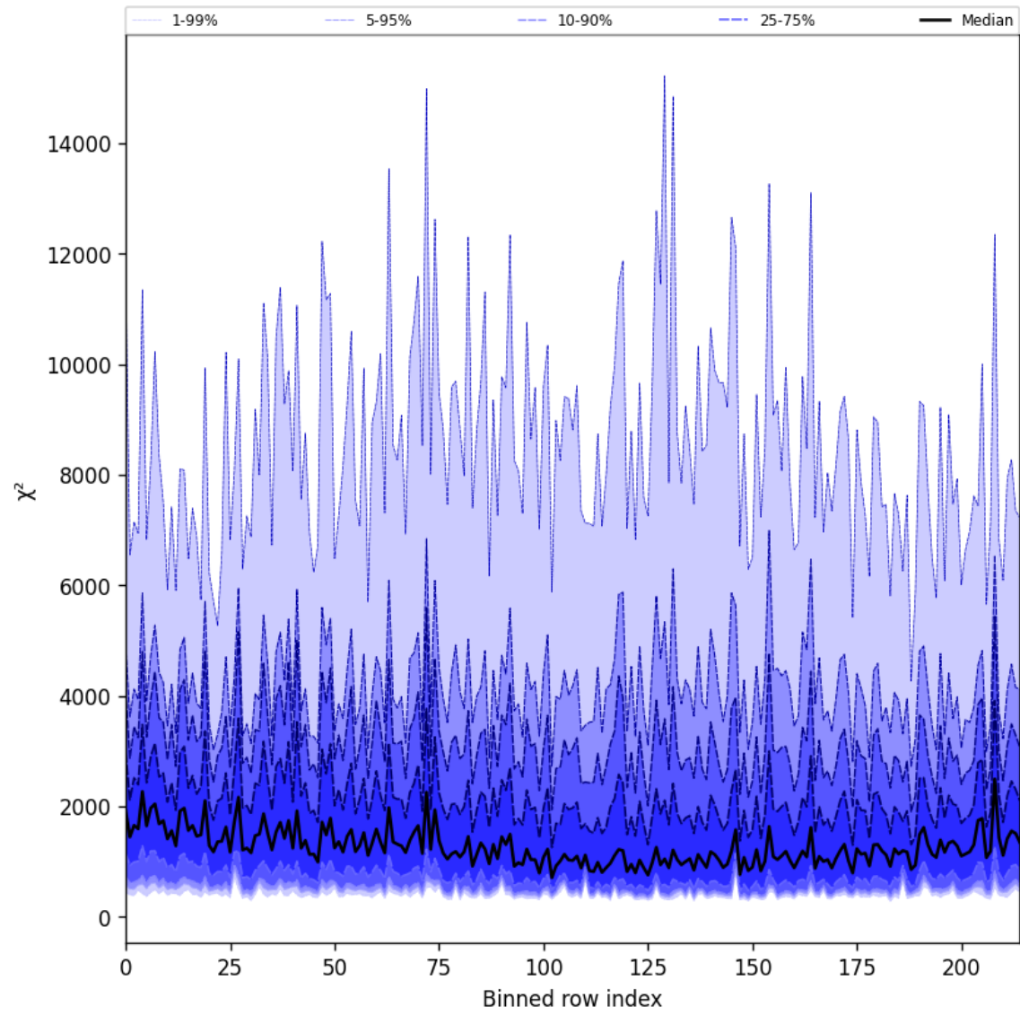
Figure 24: Along track statistics of “ \chi^2 ” for 2025-05-11 to 2025-05-12
