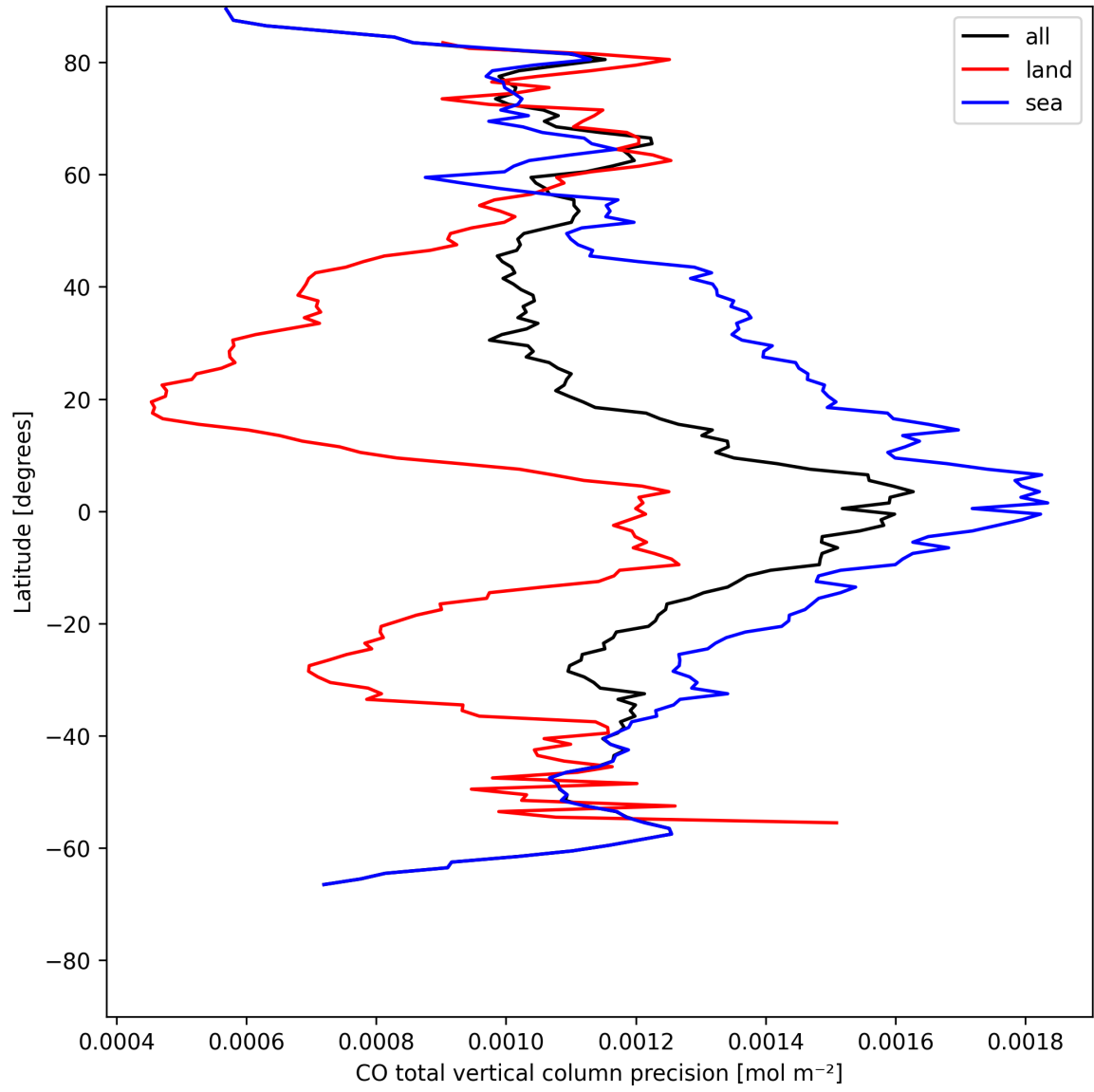
Figure 8: Zonal average of "CO total vertical column precision" for 2025-05-11 to 2025-05-12.
