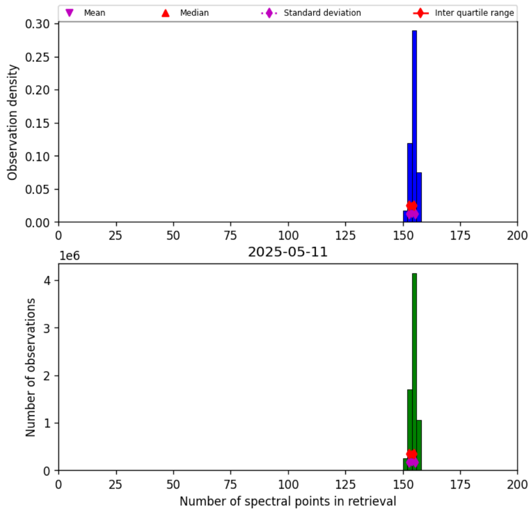
Figure 16: Histogram of “Number of spectral points in retrieval” for 2025-05-11 to 2025-05-12
