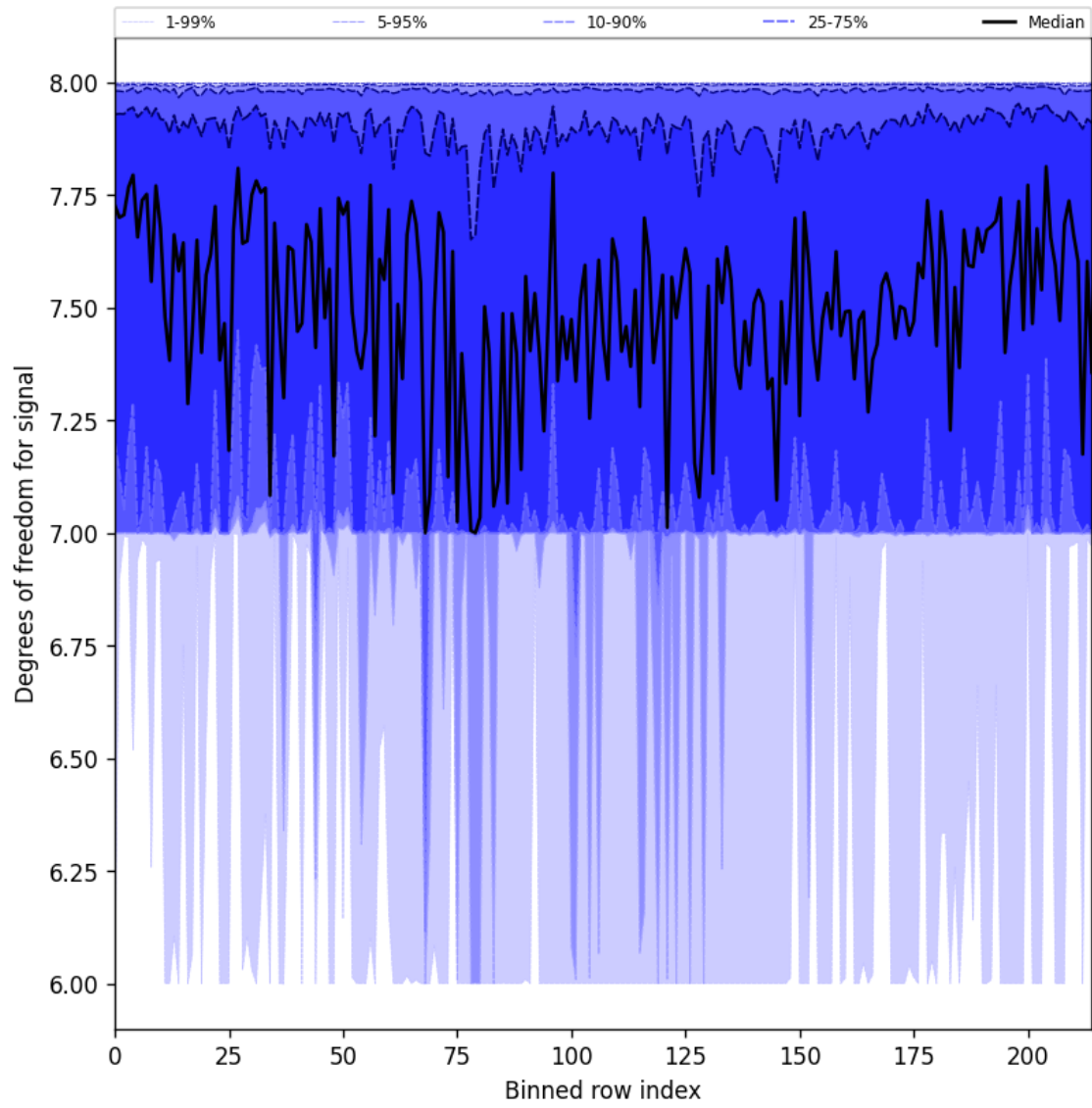
Figure 25: Along track statistics of “Degrees of freedom for signal” for 2025-05-11 to 2025-05-12
