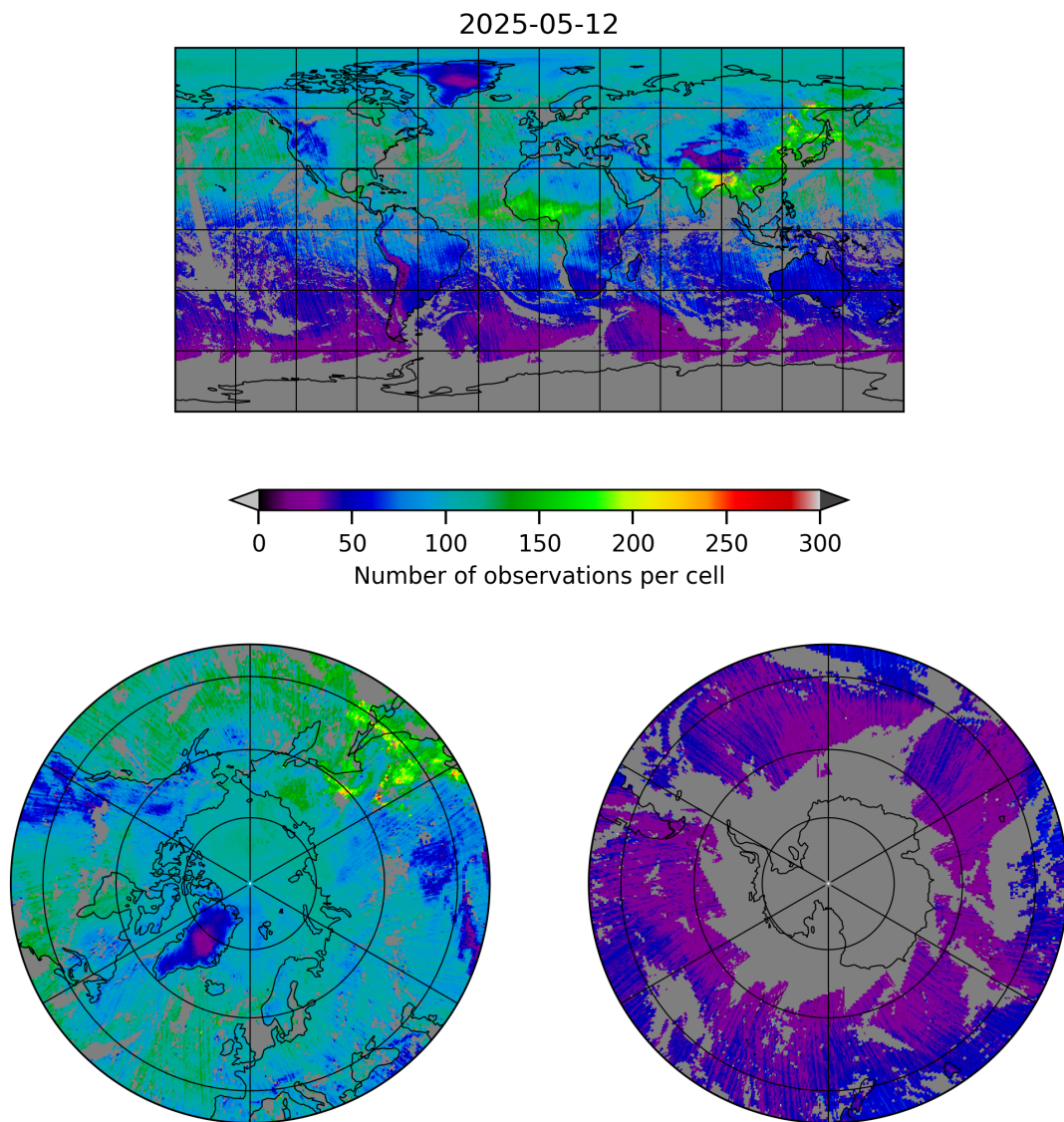
Figure 5: Map of the number of observations for 2025-05-12 to 2025-05-13
