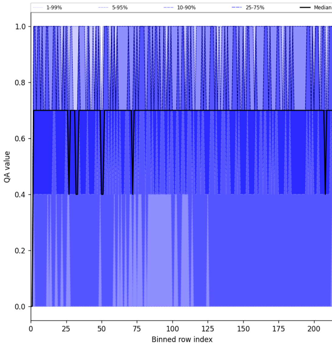
Figure 20: Along track statistics of “QA value” for 2025-05-12 to 2025-05-13
