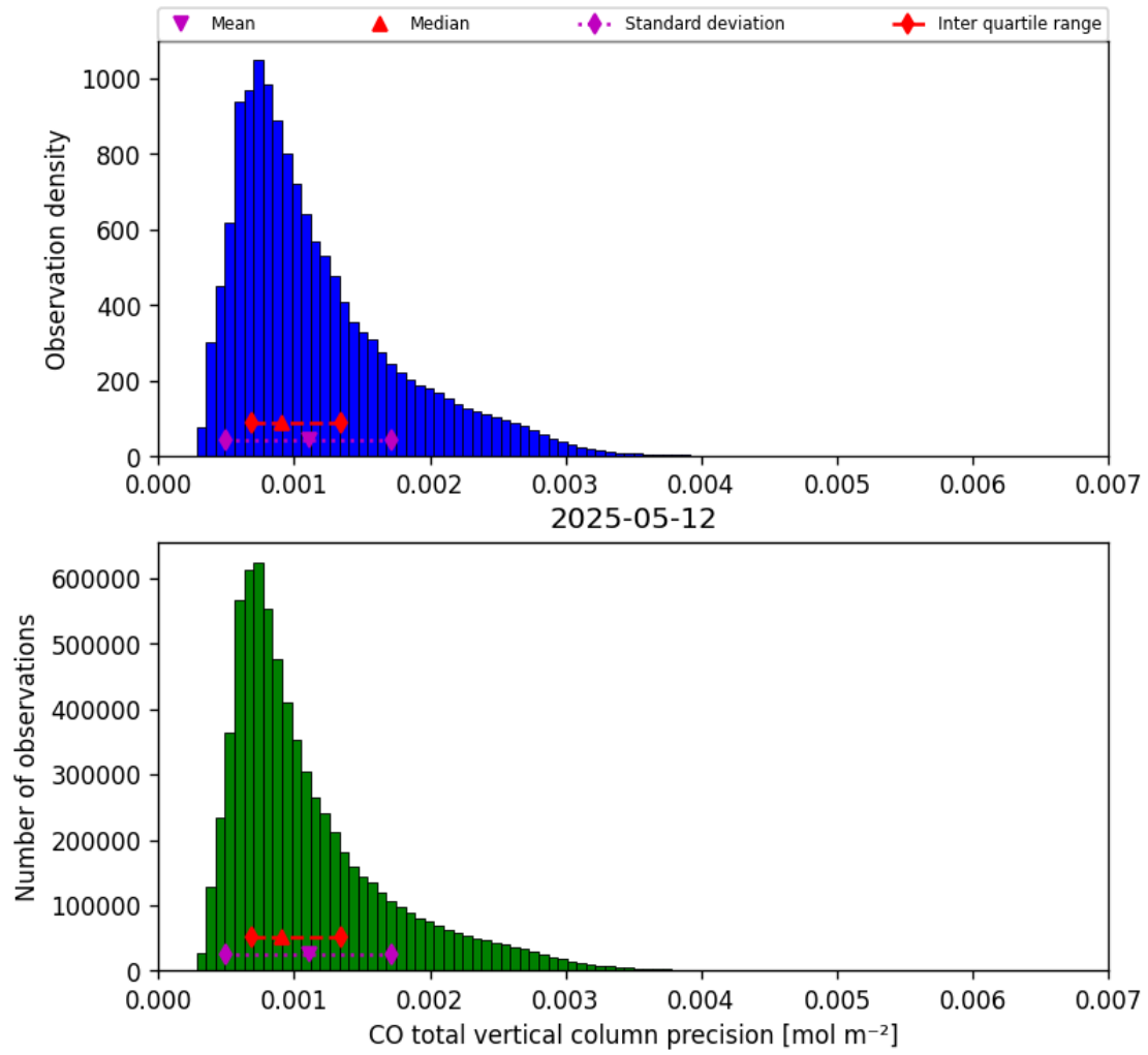
Figure 15: Histogram of “CO total vertical column precision” for 2025-05-12 to 2025-05-13
