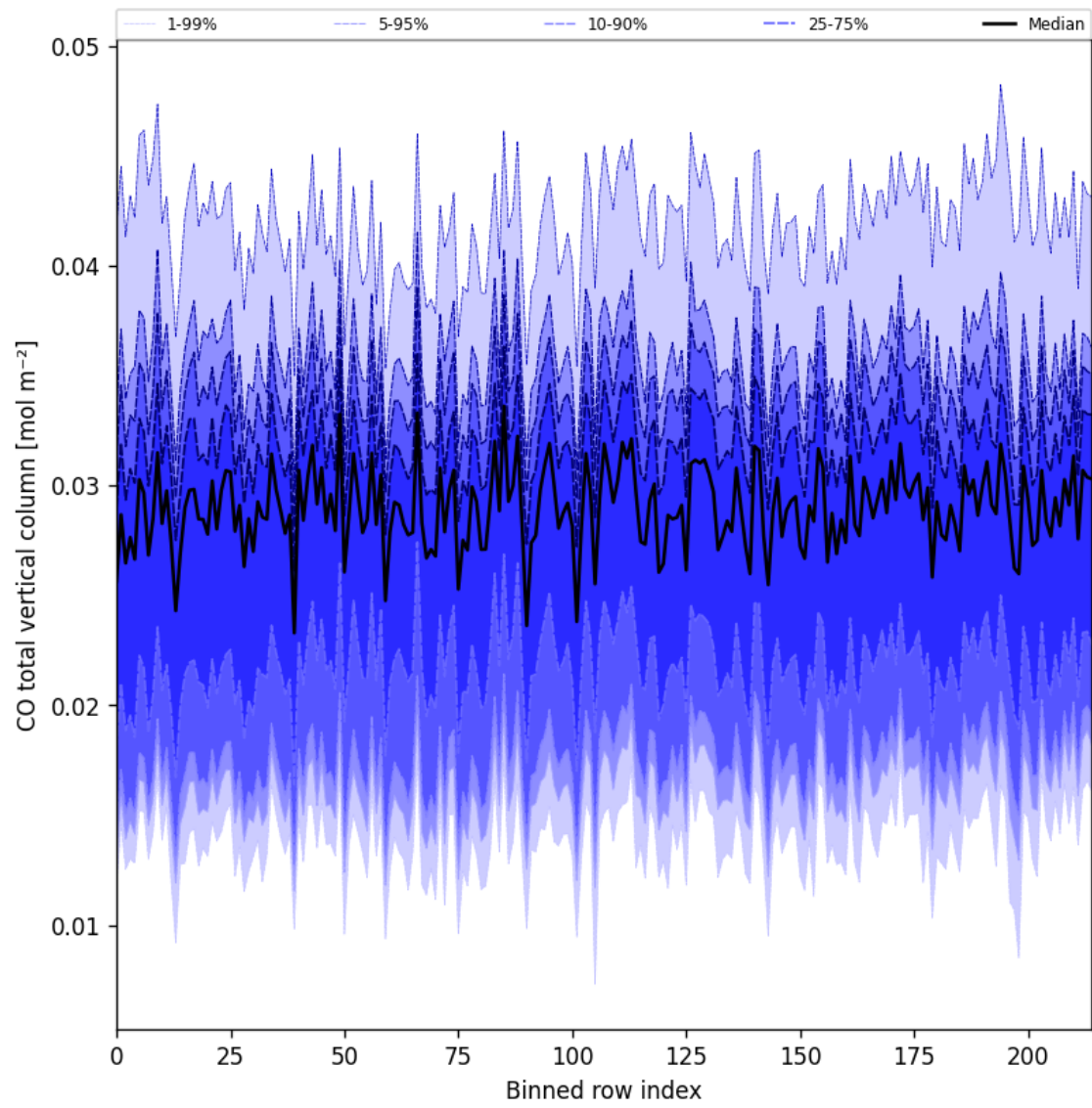
Figure 21: Along track statistics of “CO total vertical column” for 2025-05-12 to 2025-05-13
