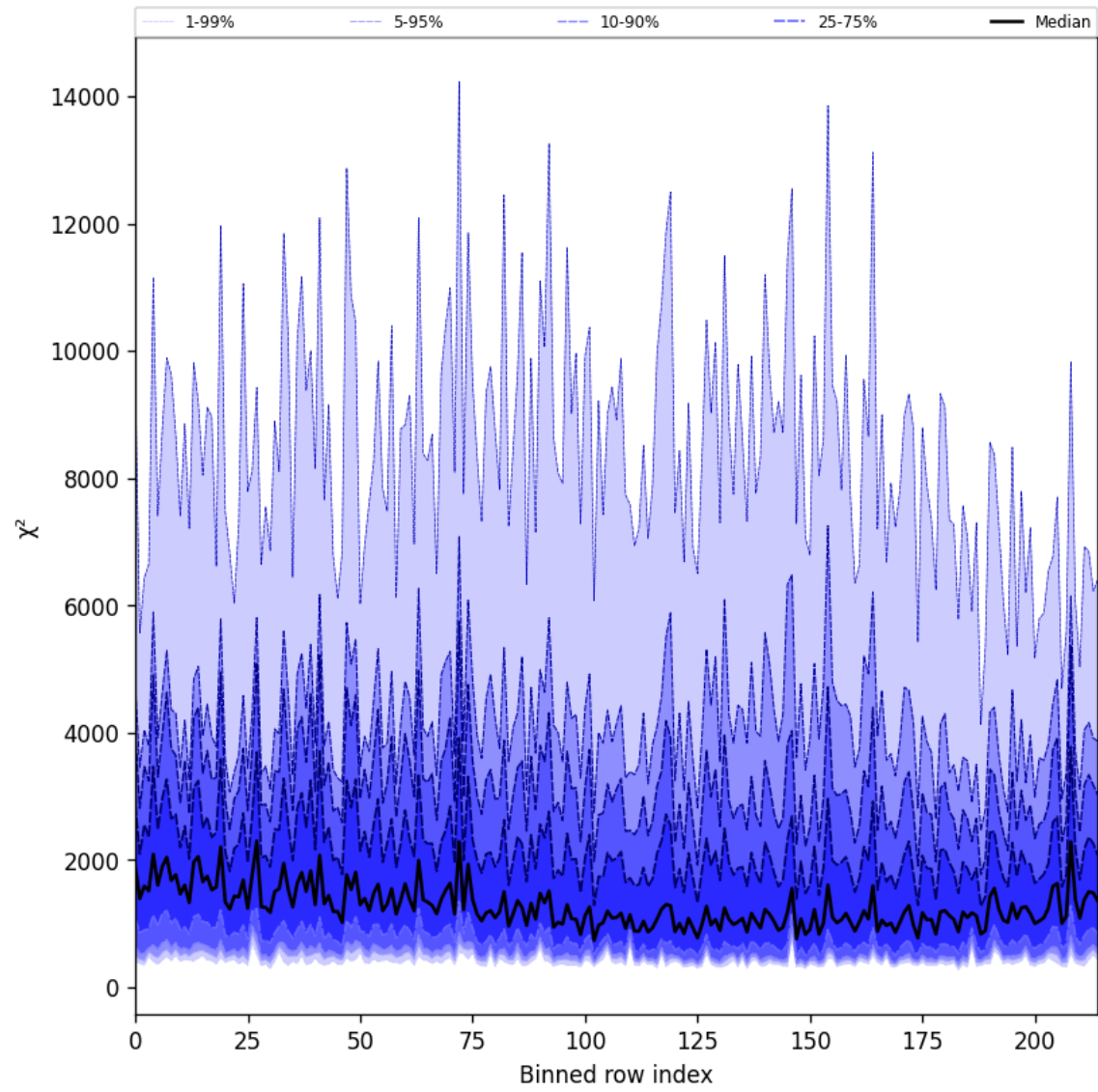
Figure 24: Along track statistics of “ \chi^2 ” for 2025-05-12 to 2025-05-13
