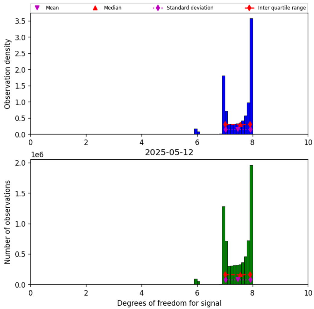
Figure 18: Histogram of “Degrees of freedom for signal” for 2025-05-12 to 2025-05-13
