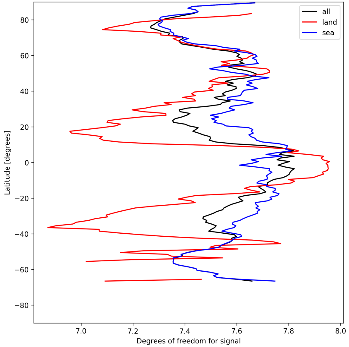
Figure 11: Zonal average of “Degrees of freedom for signal” for 2025-05-12 to 2025-05-13.
