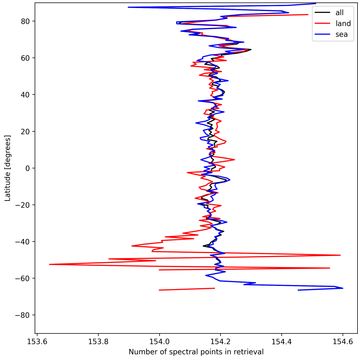
Figure 9: Zonal average of “Number of spectral points in retrieval” for 2025-05-12 to 2025-05-13.
