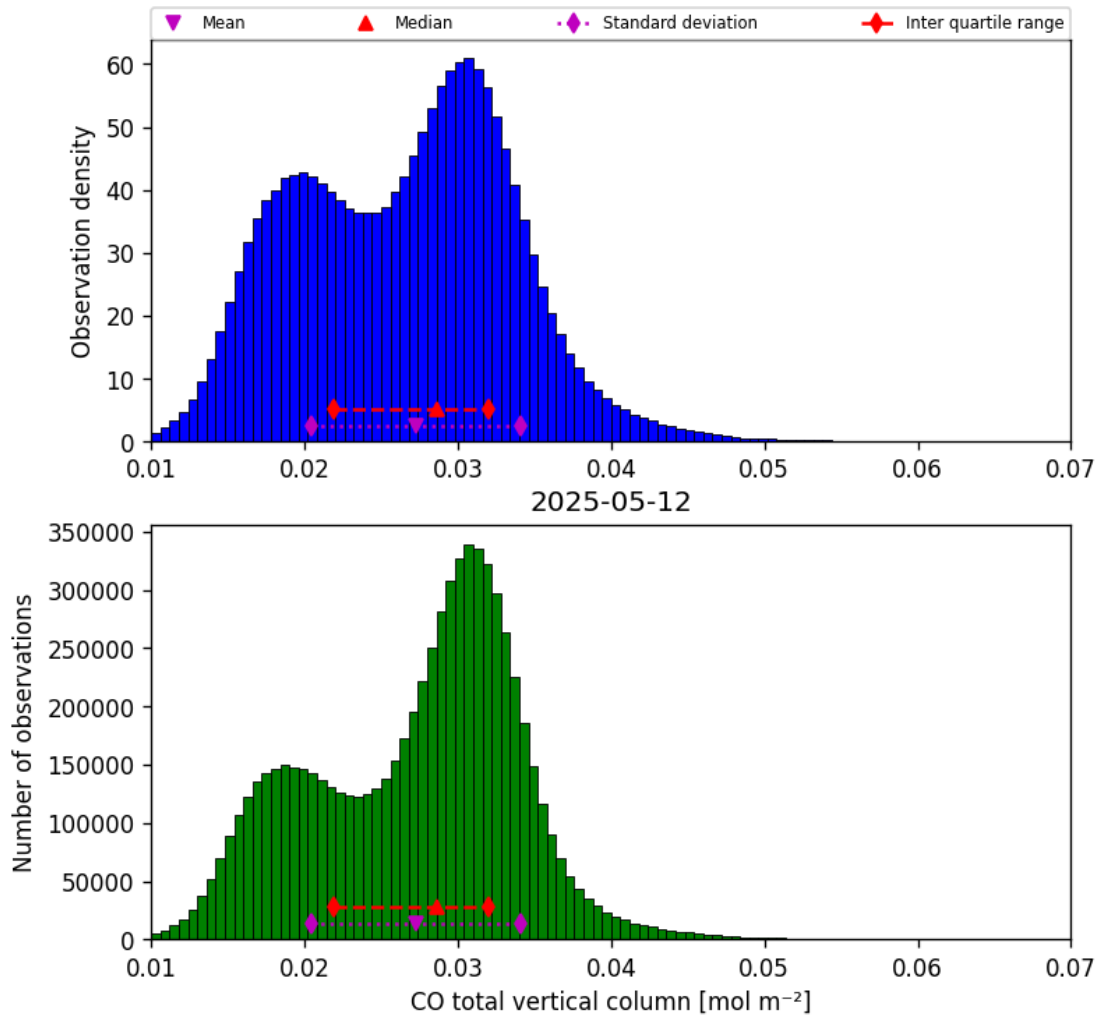
Figure 14: Histogram of “CO total vertical column” for 2025-05-12 to 2025-05-13
