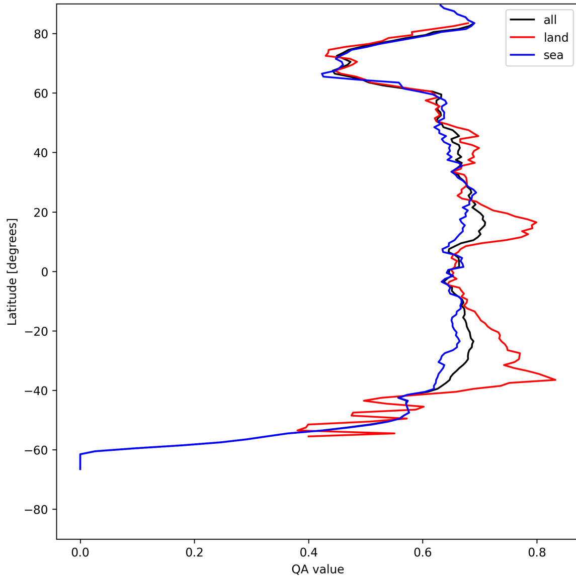
Figure 6: Zonal average of “QA value” for 2025-05-12 to 2025-05-13.
