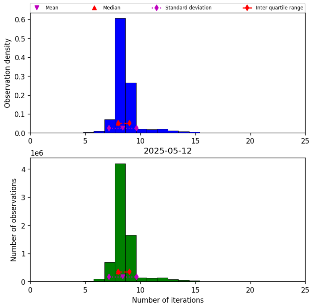
Figure 19: Histogram of “Number of iterations” for 2025-05-12 to 2025-05-13
