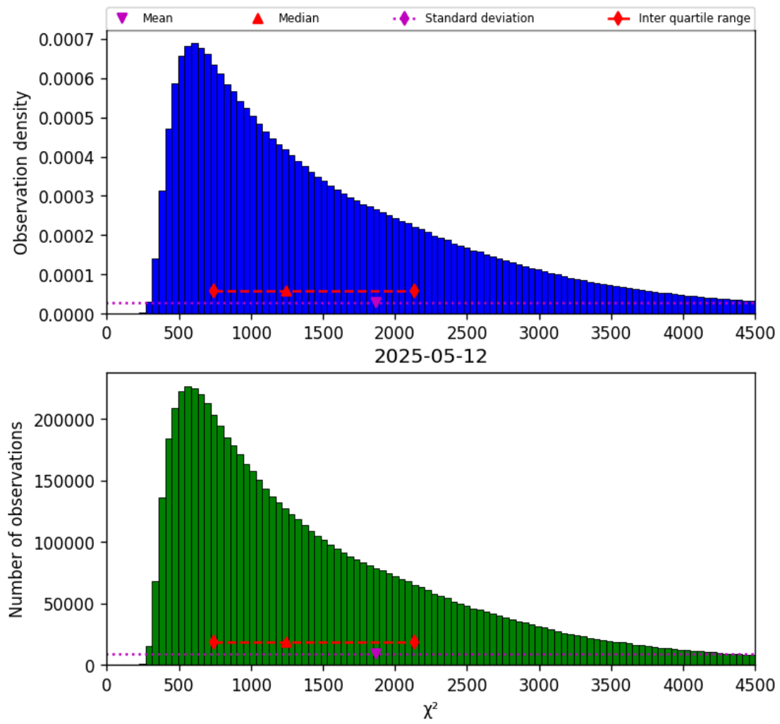
Figure 17: Histogram of " \chi^2 " for 2025-05-12 to 2025-05-13
