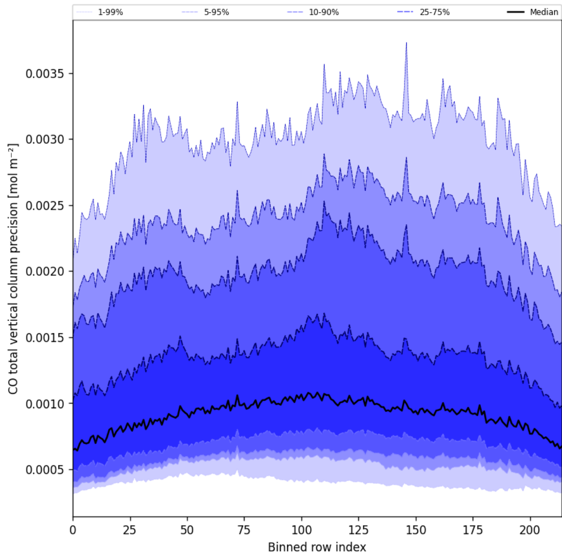
Figure 22: Along track statistics of “CO total vertical column precision” for 2025-05-12 to 2025-05-13
