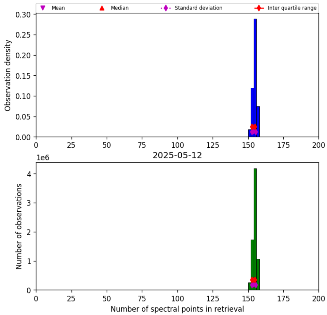
Figure 16: Histogram of “Number of spectral points in retrieval” for 2025-05-12 to 2025-05-13
