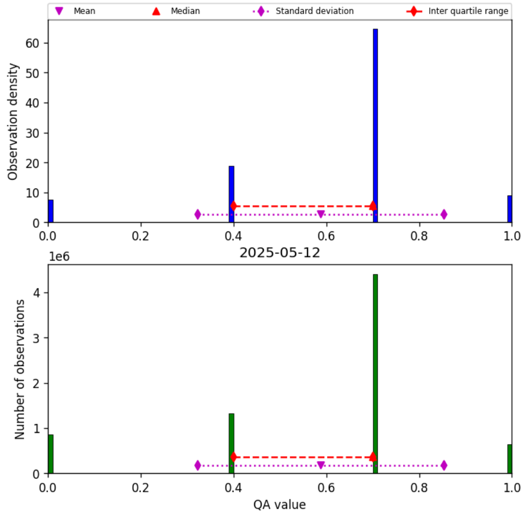
Figure 13: Histogram of “QA value” for 2025-05-12 to 2025-05-13
