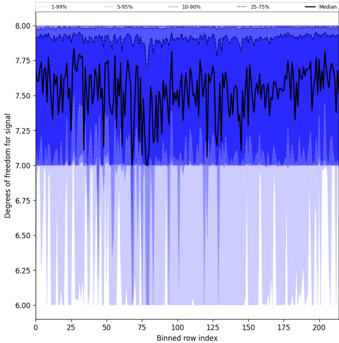
Figure 25: Along track statistics of “Degrees of freedom for signal” for 2025-05-12 to 2025-05-13
