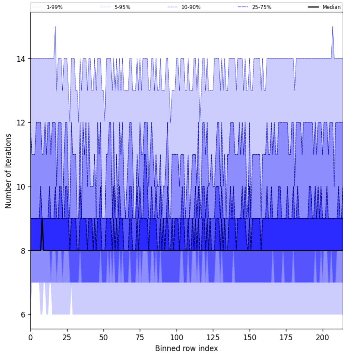
Figure 26: Along track statistics of “Number of iterations” for 2025-05-12 to 2025-05-13
