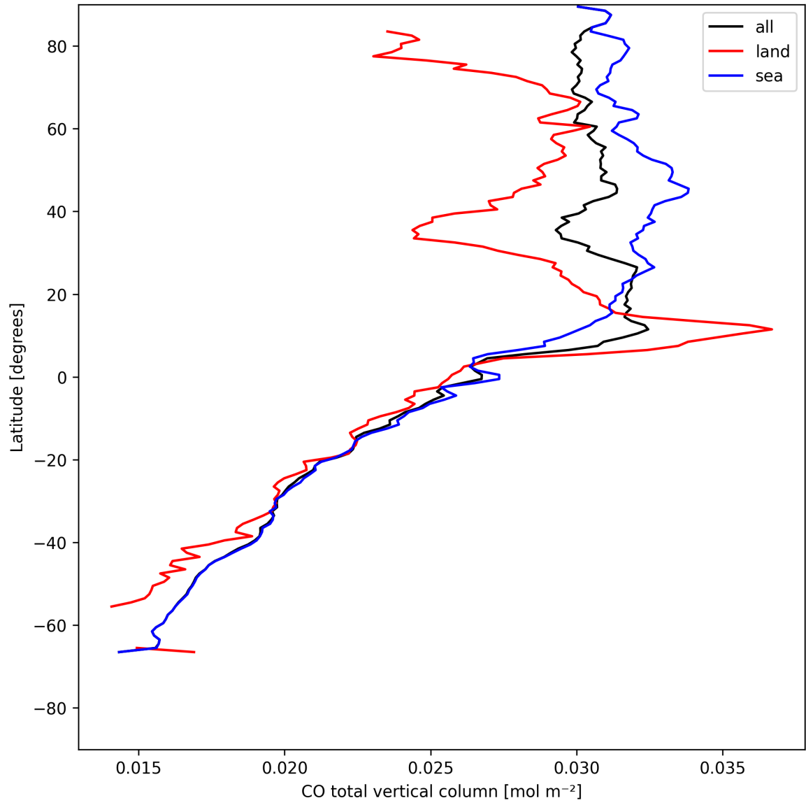
Figure 7: Zonal average of “CO total vertical column” for 2025-05-12 to 2025-05-13.
