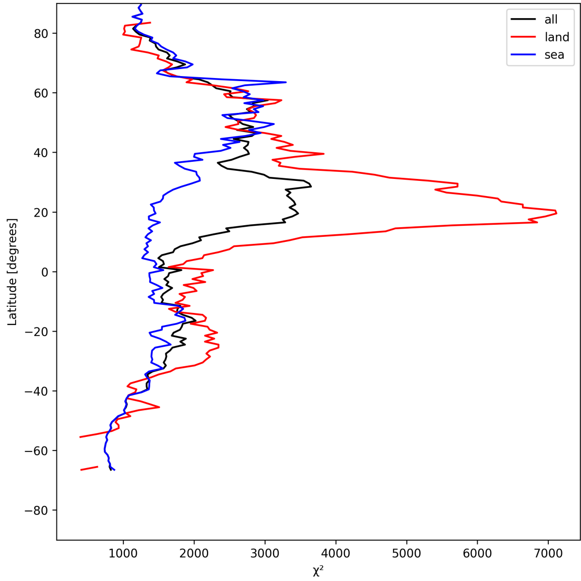
Figure 10: Zonal average of “ \chi^2 ” for 2025-05-12 to 2025-05-13.
