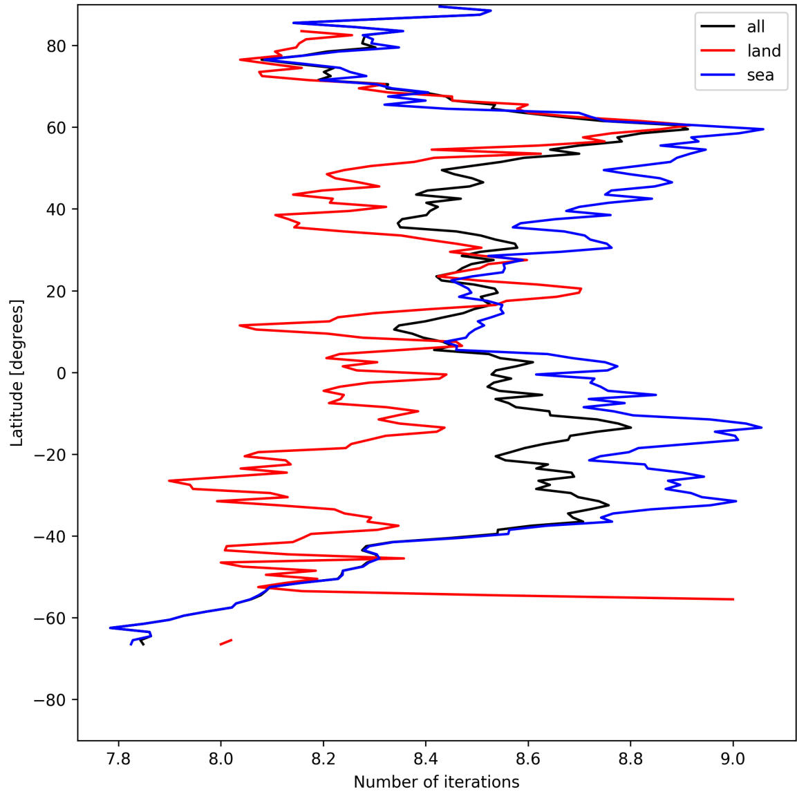
Figure 12: Zonal average of “Number of iterations” for 2025-05-12 to 2025-05-13.
