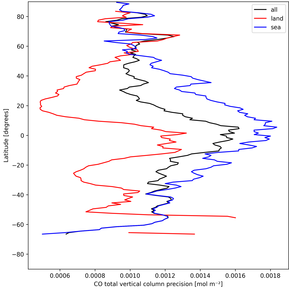
Figure 8: Zonal average of “CO total vertical column precision” for 2025-05-12 to 2025-05-13.
