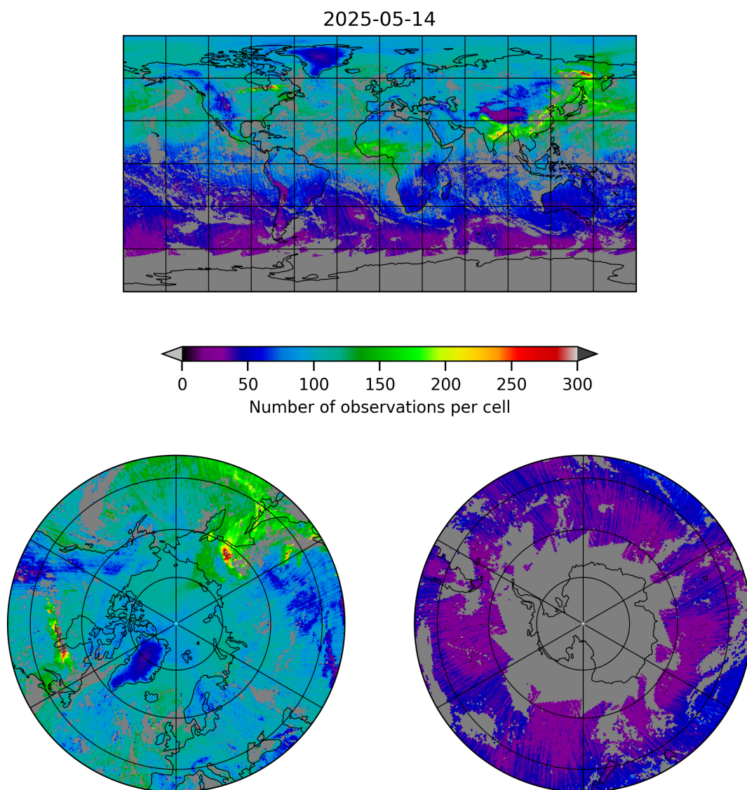
Figure 5: Map of the number of observations for 2025-05-14 to 2025-05-15
