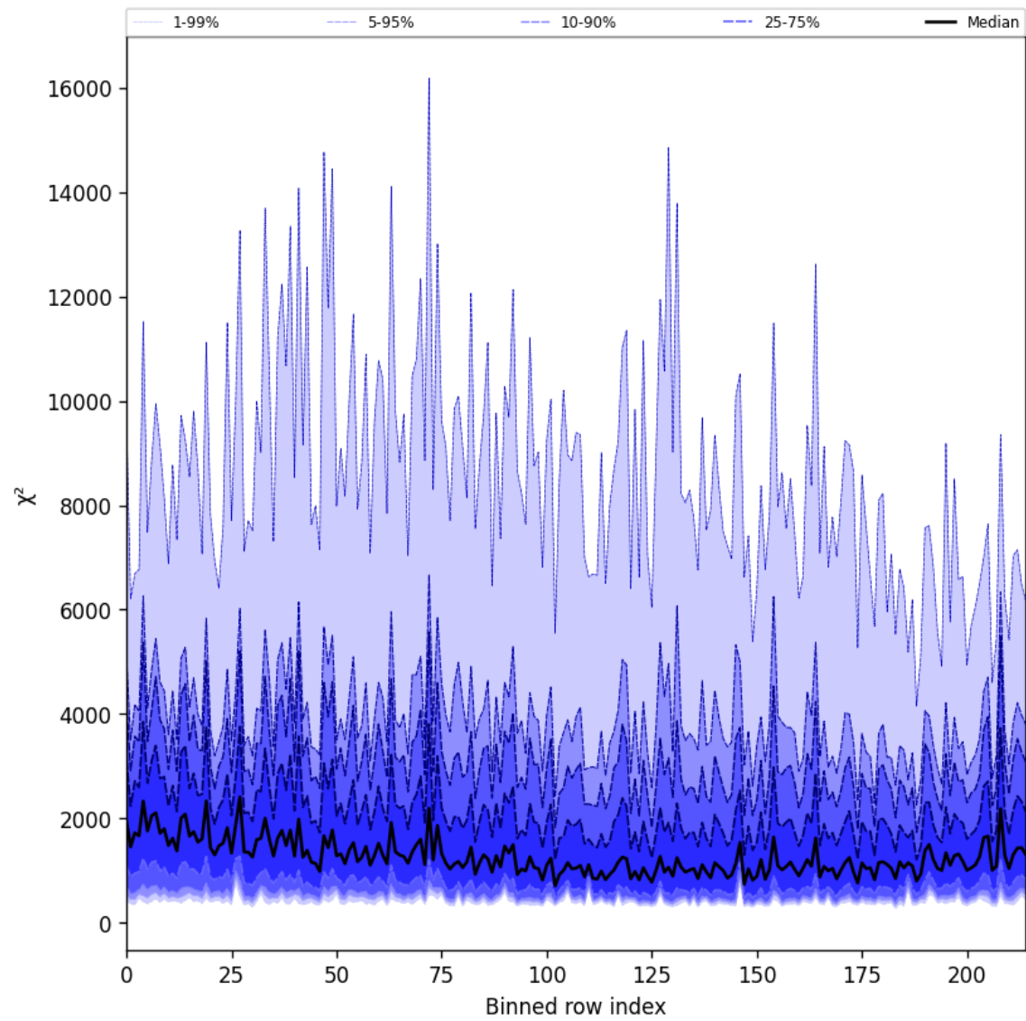
Figure 24: Along track statistics of “ \chi^2 ” for 2025-05-14 to 2025-05-15
