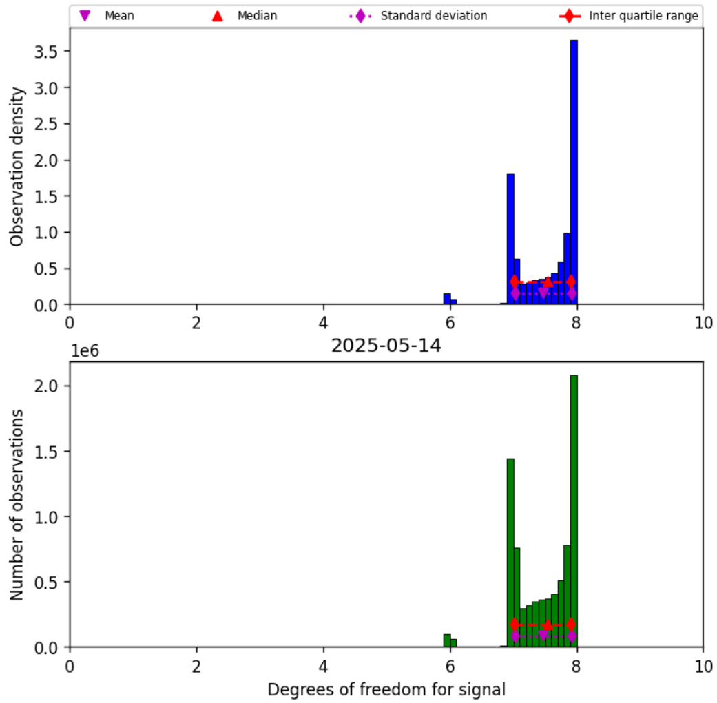
Figure 18: Histogram of “Degrees of freedom for signal” for 2025-05-14 to 2025-05-15
