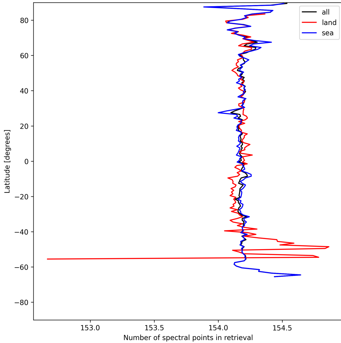
Figure 9: Zonal average of “Number of spectral points in retrieval” for 2025-05-14 to 2025-05-15.
