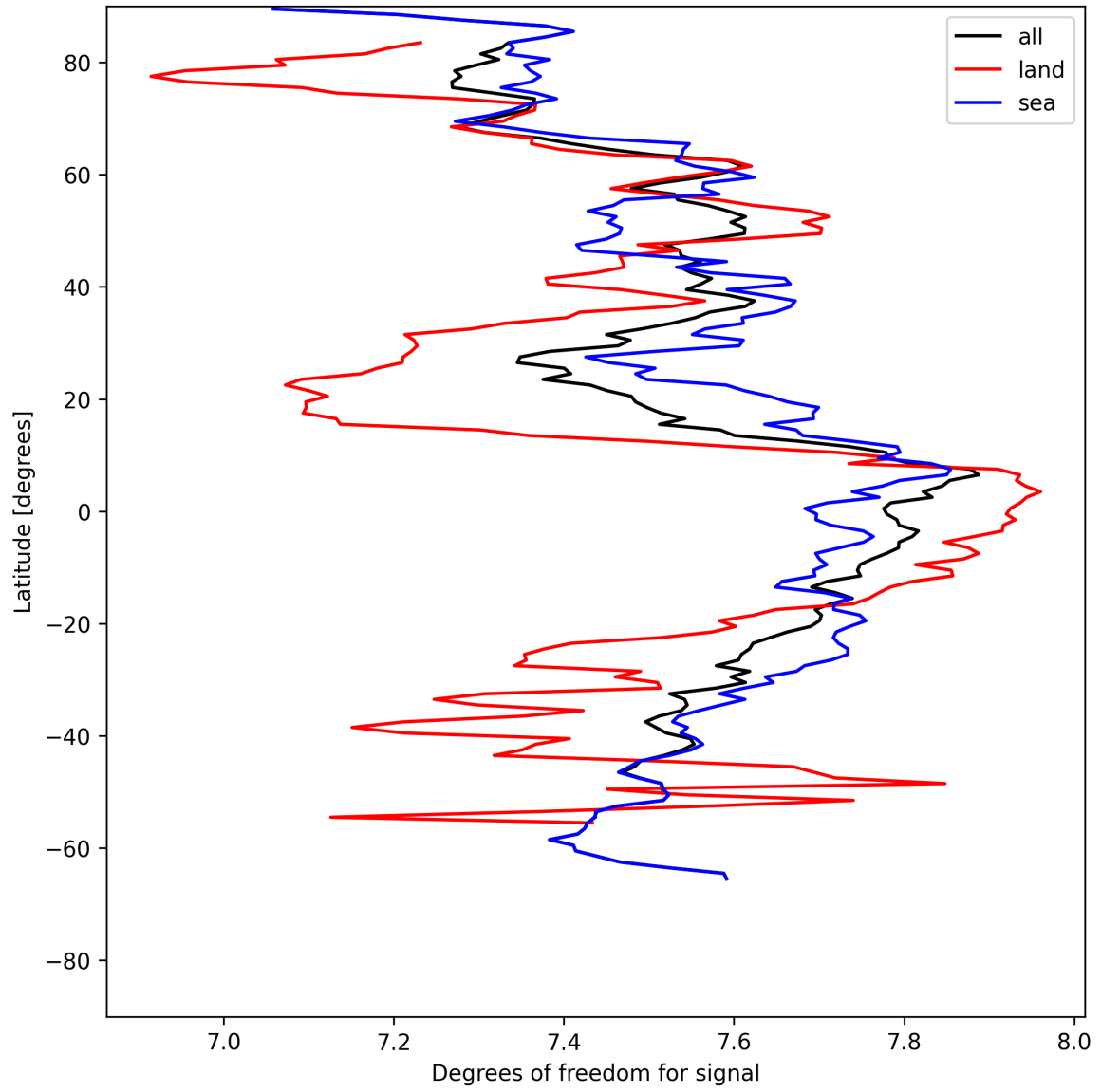
Figure 11: Zonal average of “Degrees of freedom for signal” for 2025-05-14 to 2025-05-15.
