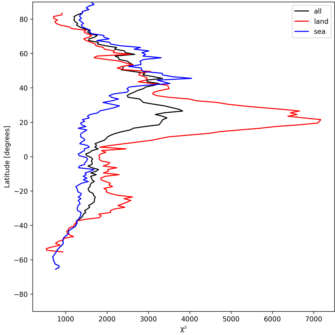
Figure 10: Zonal average of “ \chi^2 ” for 2025-05-14 to 2025-05-15.
