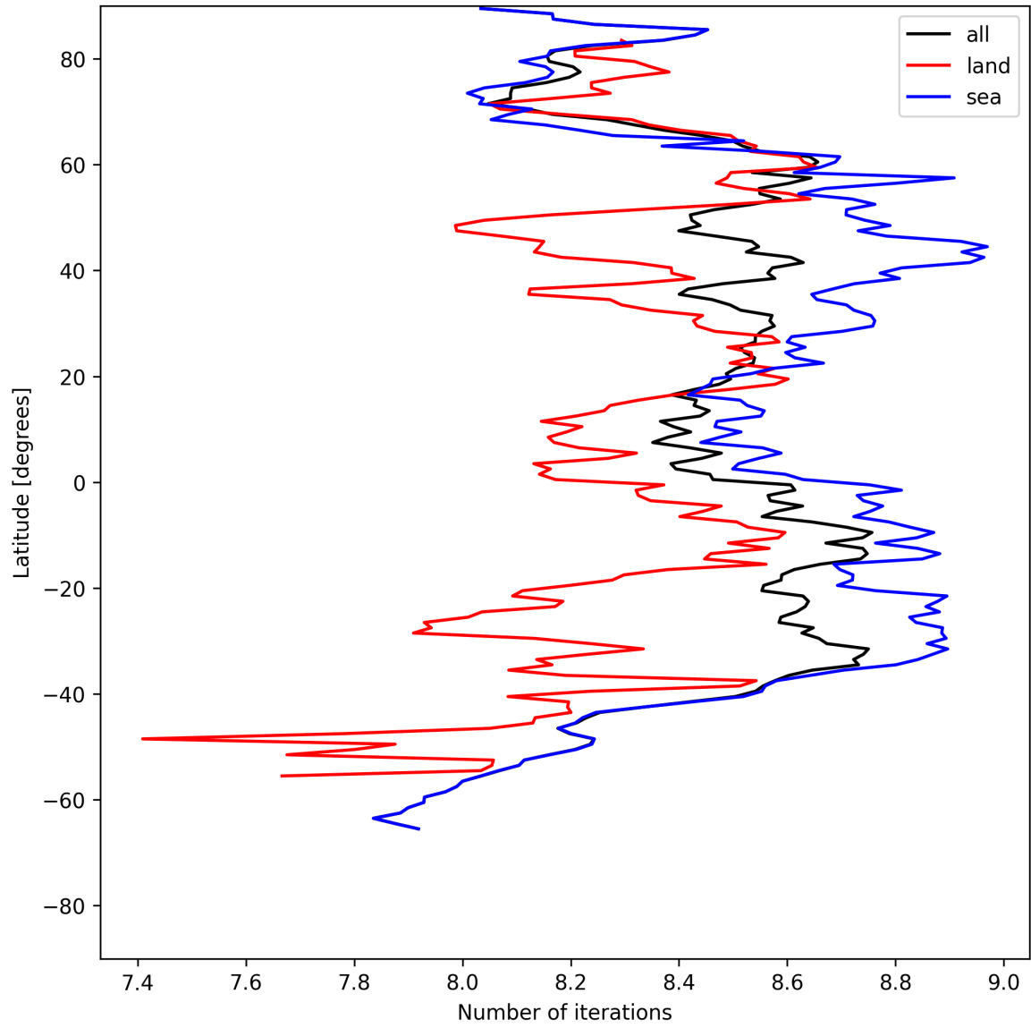
Figure 12: Zonal average of “Number of iterations” for 2025-05-14 to 2025-05-15.
