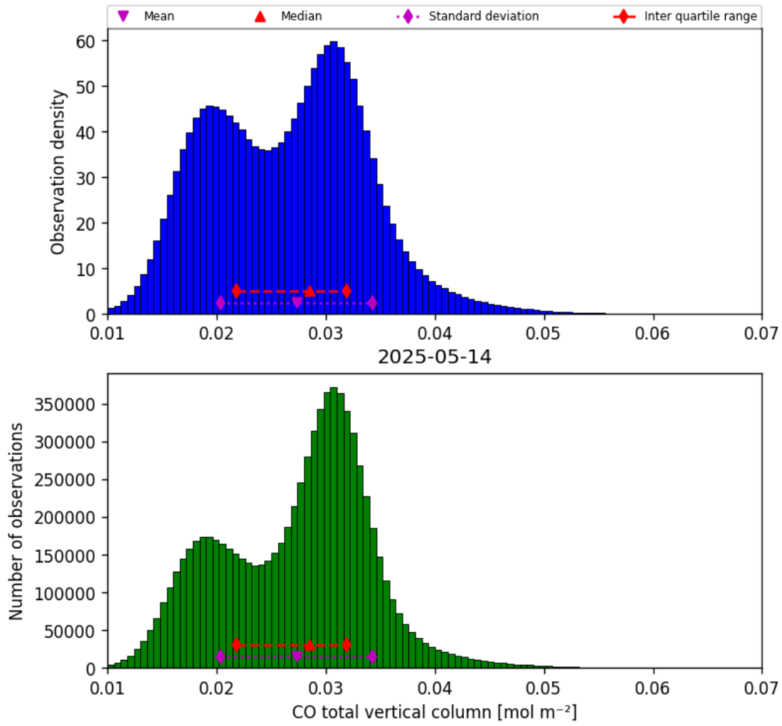
Figure 14: Histogram of “CO total vertical column” for 2025-05-14 to 2025-05-15
