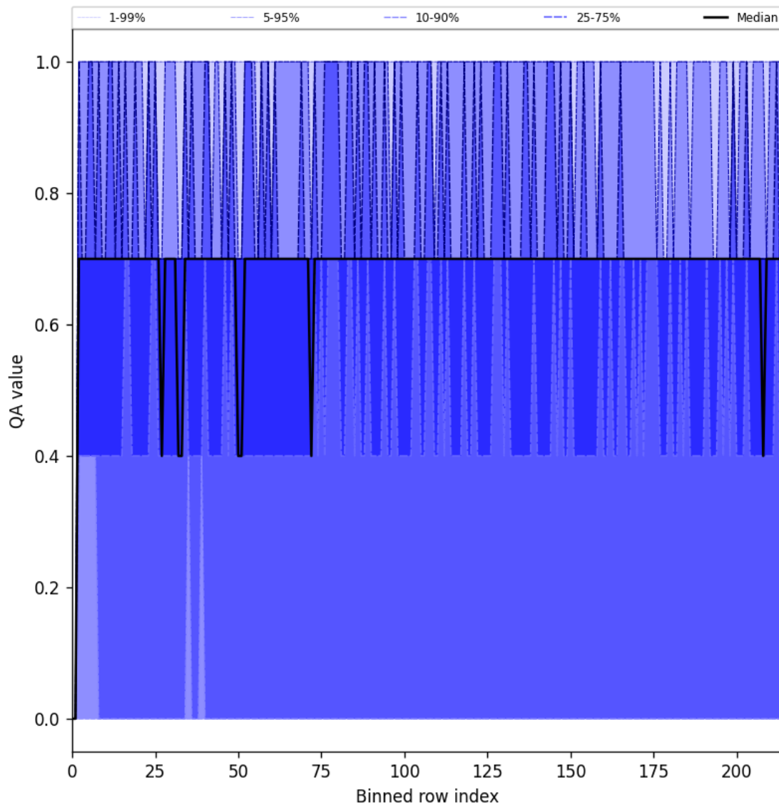
Figure 20: Along track statistics of “QA value” for 2025-05-14 to 2025-05-15
