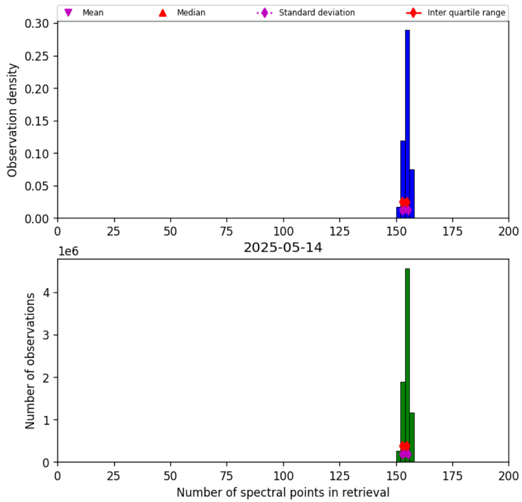
Figure 16: Histogram of “Number of spectral points in retrieval” for 2025-05-14 to 2025-05-15
