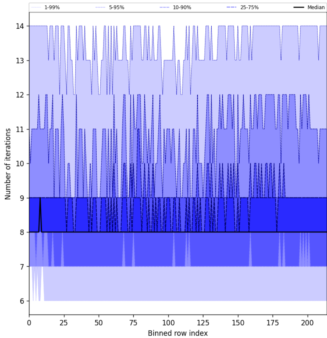
Figure 26: Along track statistics of “Number of iterations” for 2025-05-14 to 2025-05-15
