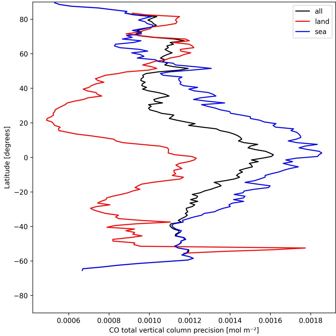
Figure 8: Zonal average of “CO total vertical column precision” for 2025-05-14 to 2025-05-15.
