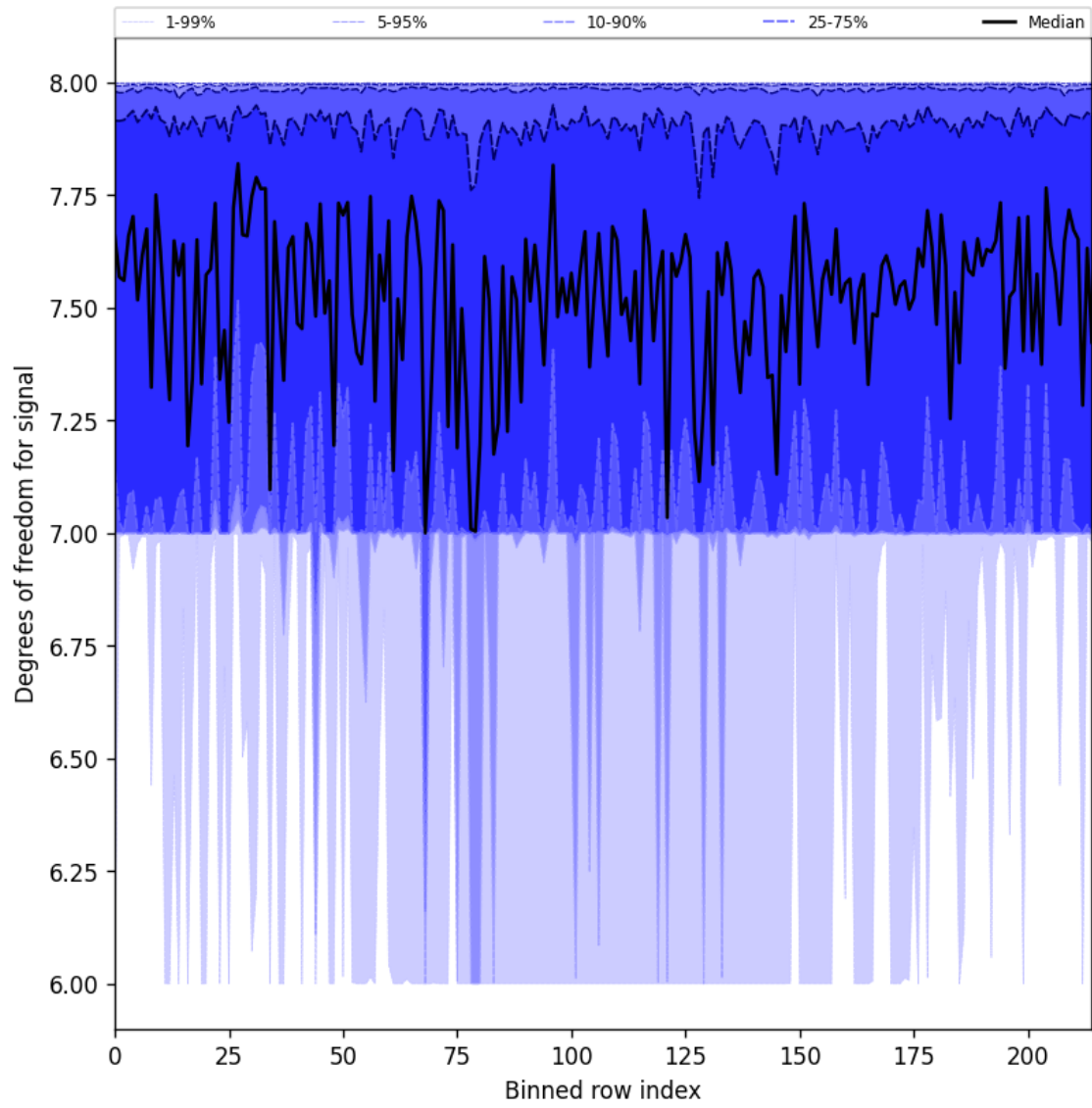
Figure 25: Along track statistics of “Degrees of freedom for signal” for 2025-05-14 to 2025-05-15
