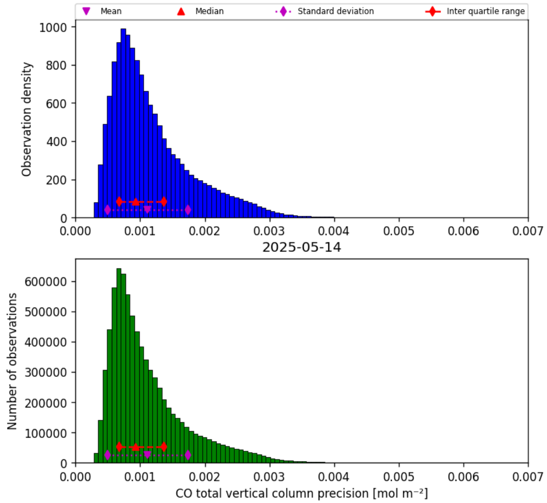
Figure 15: Histogram of “CO total vertical column precision” for 2025-05-14 to 2025-05-15
