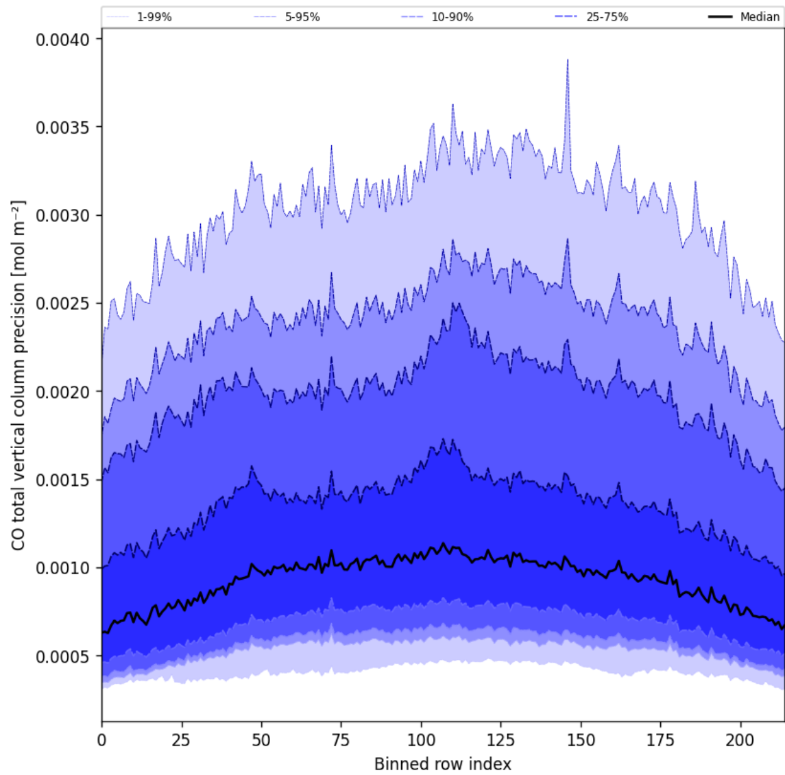
Figure 22: Along track statistics of “CO total vertical column precision” for 2025-05-14 to 2025-05-15
