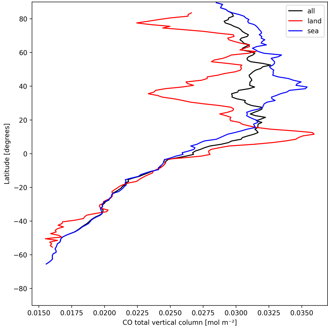
Figure 7: Zonal average of “CO total vertical column” for 2025-05-14 to 2025-05-15.
