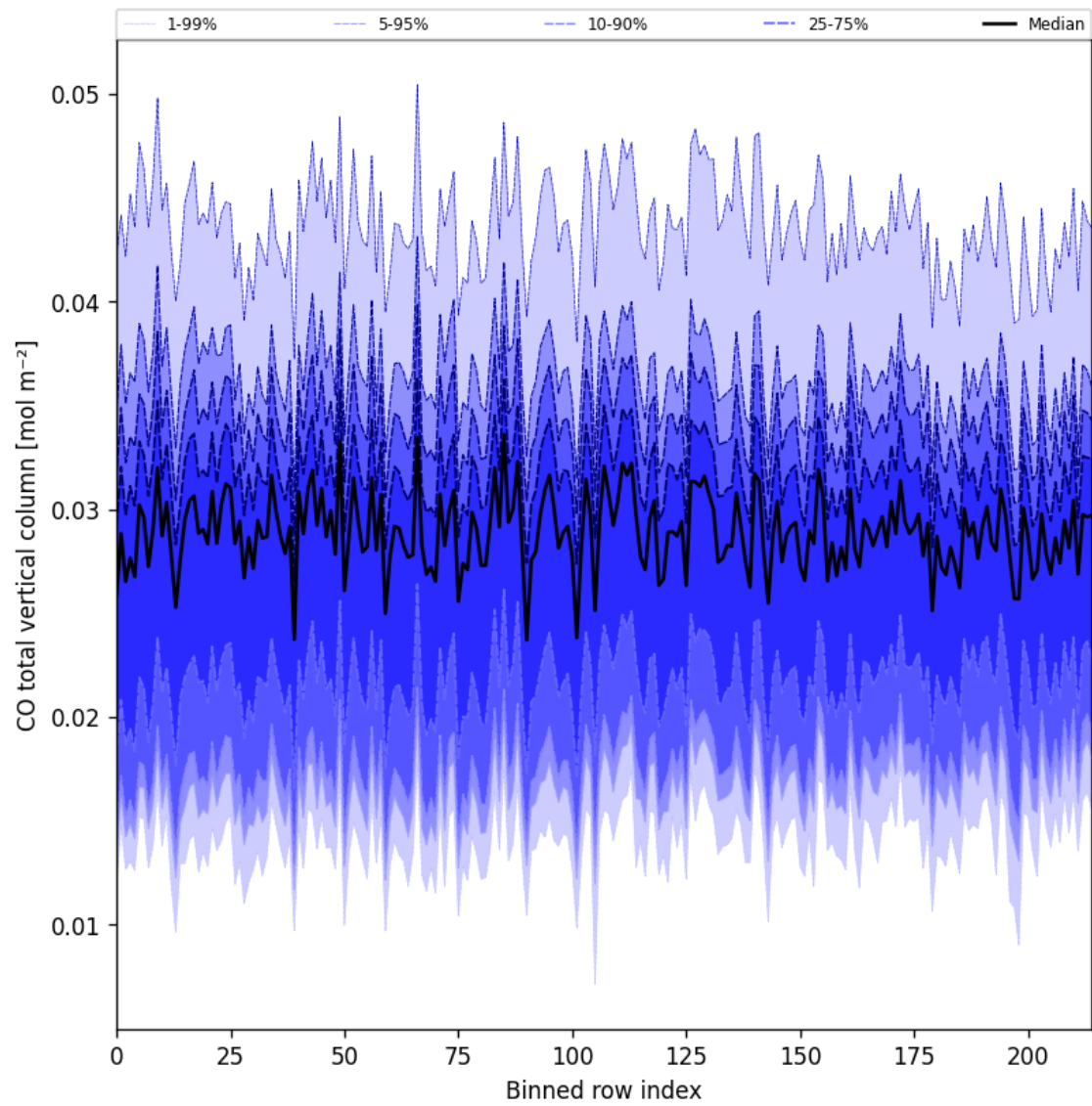
Figure 21: Along track statistics of “CO total vertical column” for 2025-05-14 to 2025-05-15
