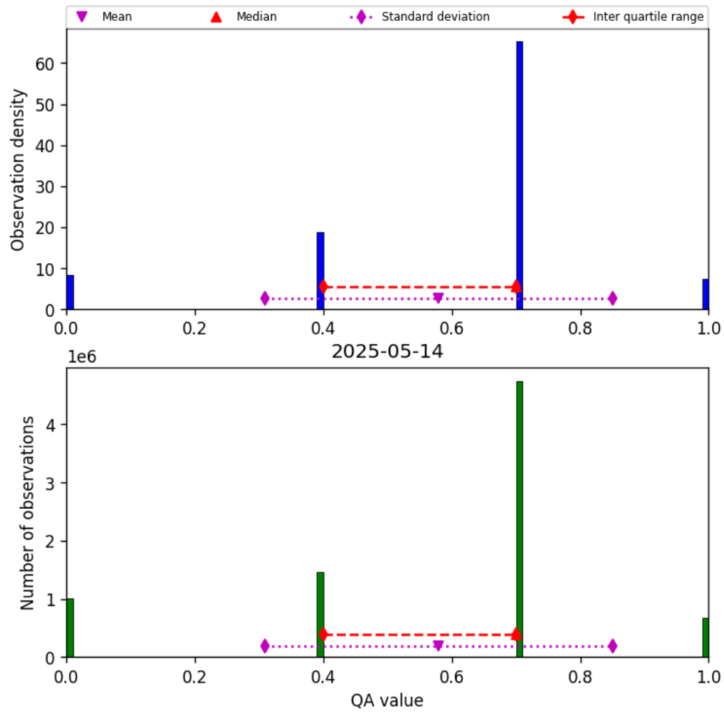
Figure 13: Histogram of “QA value” for 2025-05-14 to 2025-05-15
