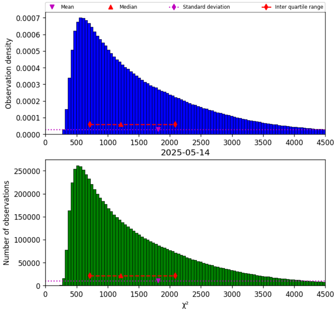
Figure 17: Histogram of “ \chi^2 ” for 2025-05-14 to 2025-05-15
