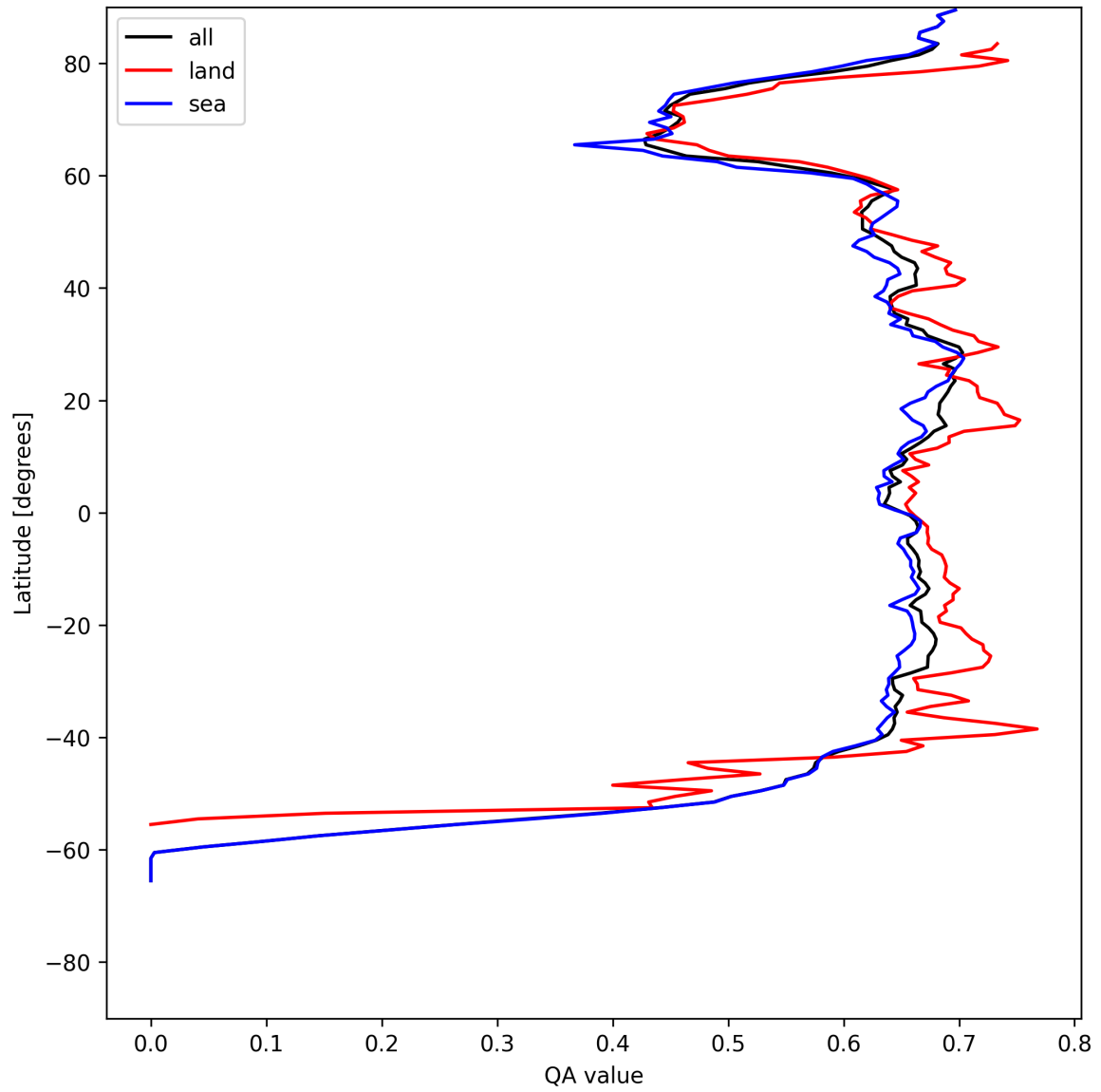
Figure 6: Zonal average of “QA value” for 2025-05-14 to 2025-05-15.
