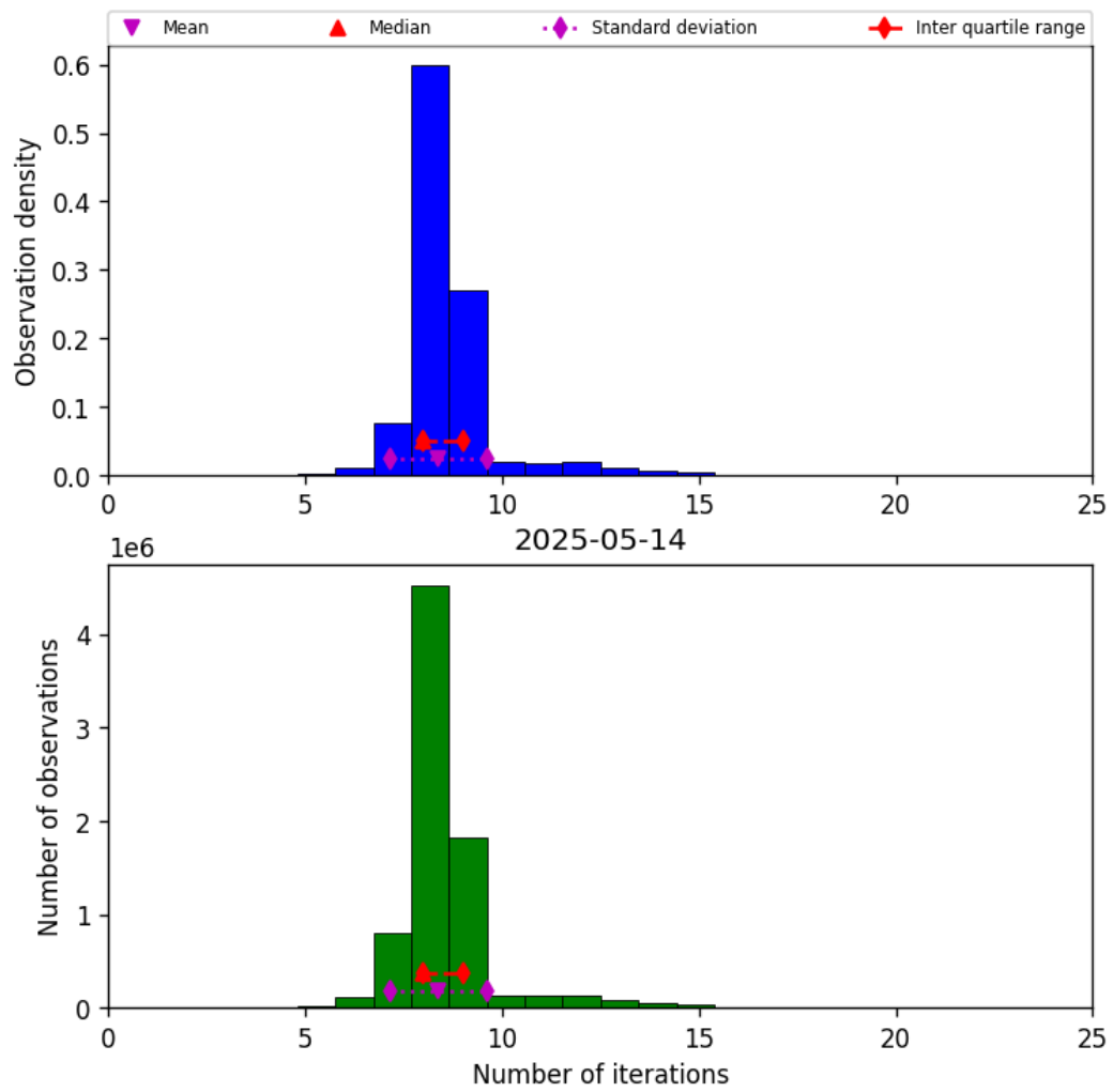
Figure 19: Histogram of “Number of iterations” for 2025-05-14 to 2025-05-15
