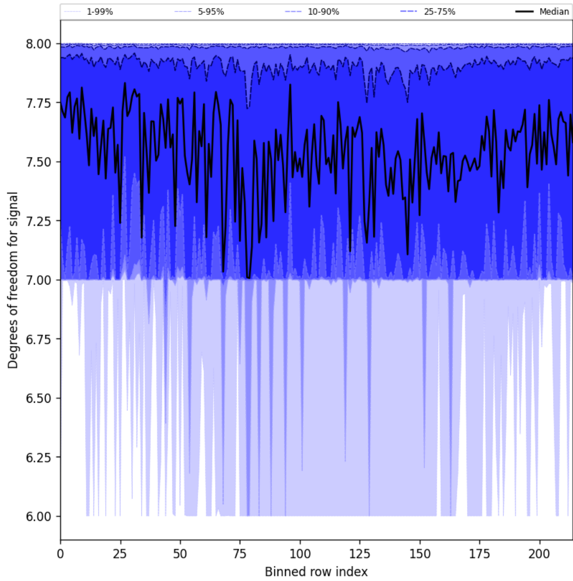
Figure 25: Along track statistics of “Degrees of freedom for signal” for 2025-05-16 to 2025-05-17
