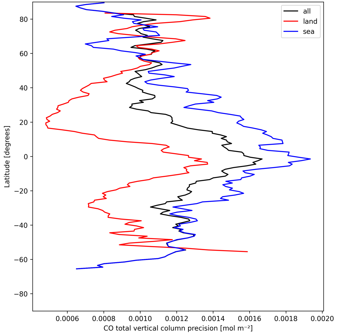
Figure 8: Zonal average of “CO total vertical column precision” for 2025-05-16 to 2025-05-17.
