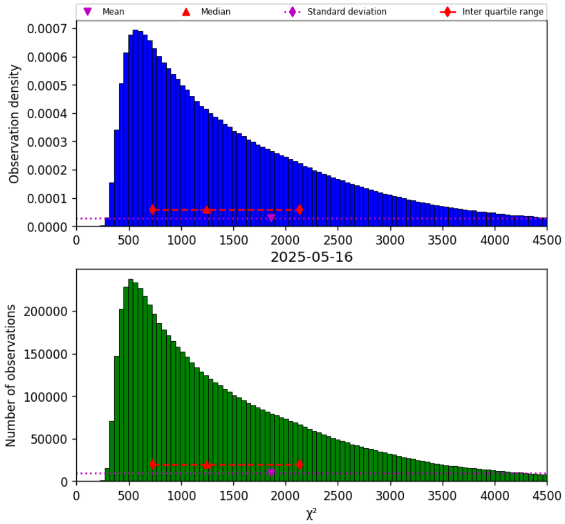
Figure 17: Histogram of “ \chi^2 ” for 2025-05-16 to 2025-05-17
