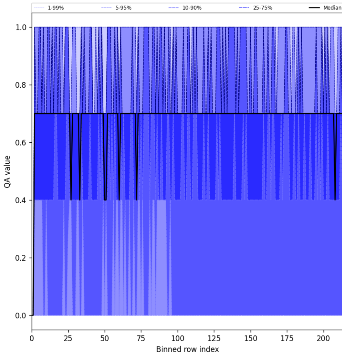
Figure 20: Along track statistics of “QA value” for 2025-05-16 to 2025-05-17
