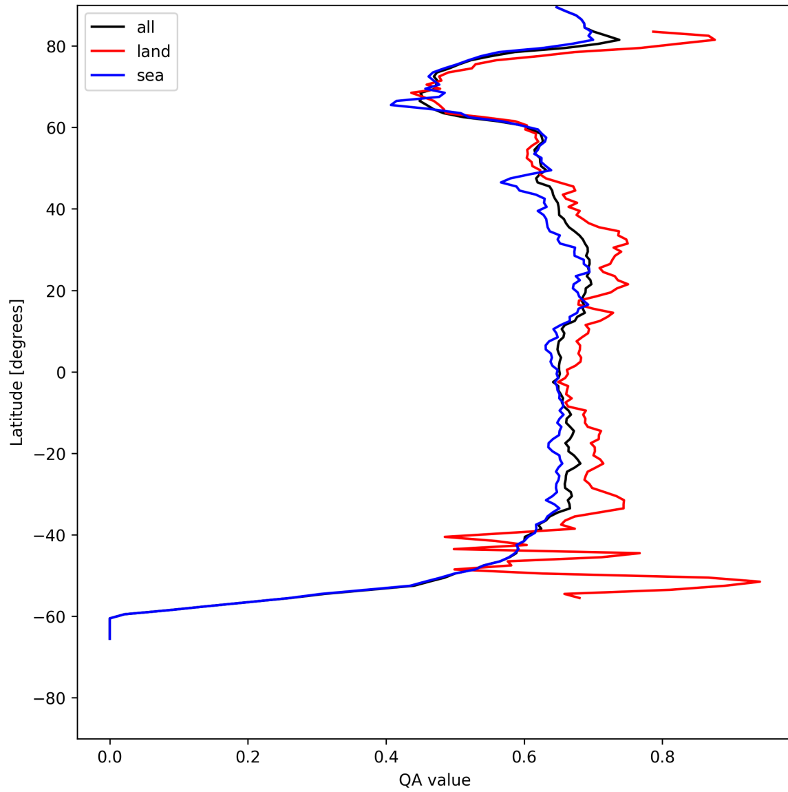
Figure 6: Zonal average of “QA value” for 2025-05-16 to 2025-05-17.
