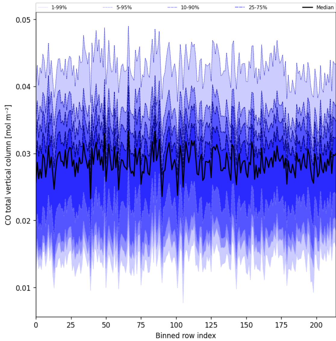
Figure 21: Along track statistics of “CO total vertical column” for 2025-05-16 to 2025-05-17
