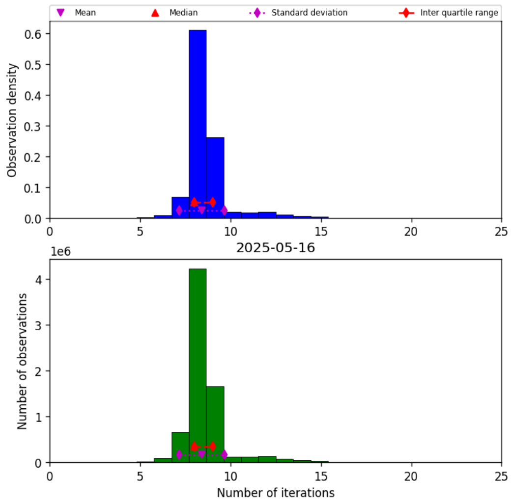
Figure 19: Histogram of “Number of iterations” for 2025-05-16 to 2025-05-17
