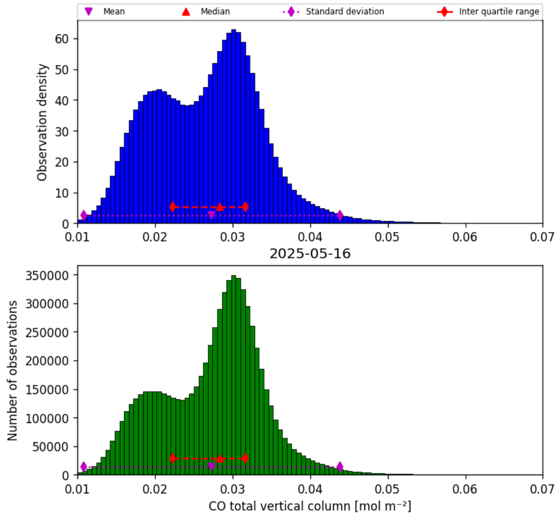
Figure 14: Histogram of “CO total vertical column” for 2025-05-16 to 2025-05-17
