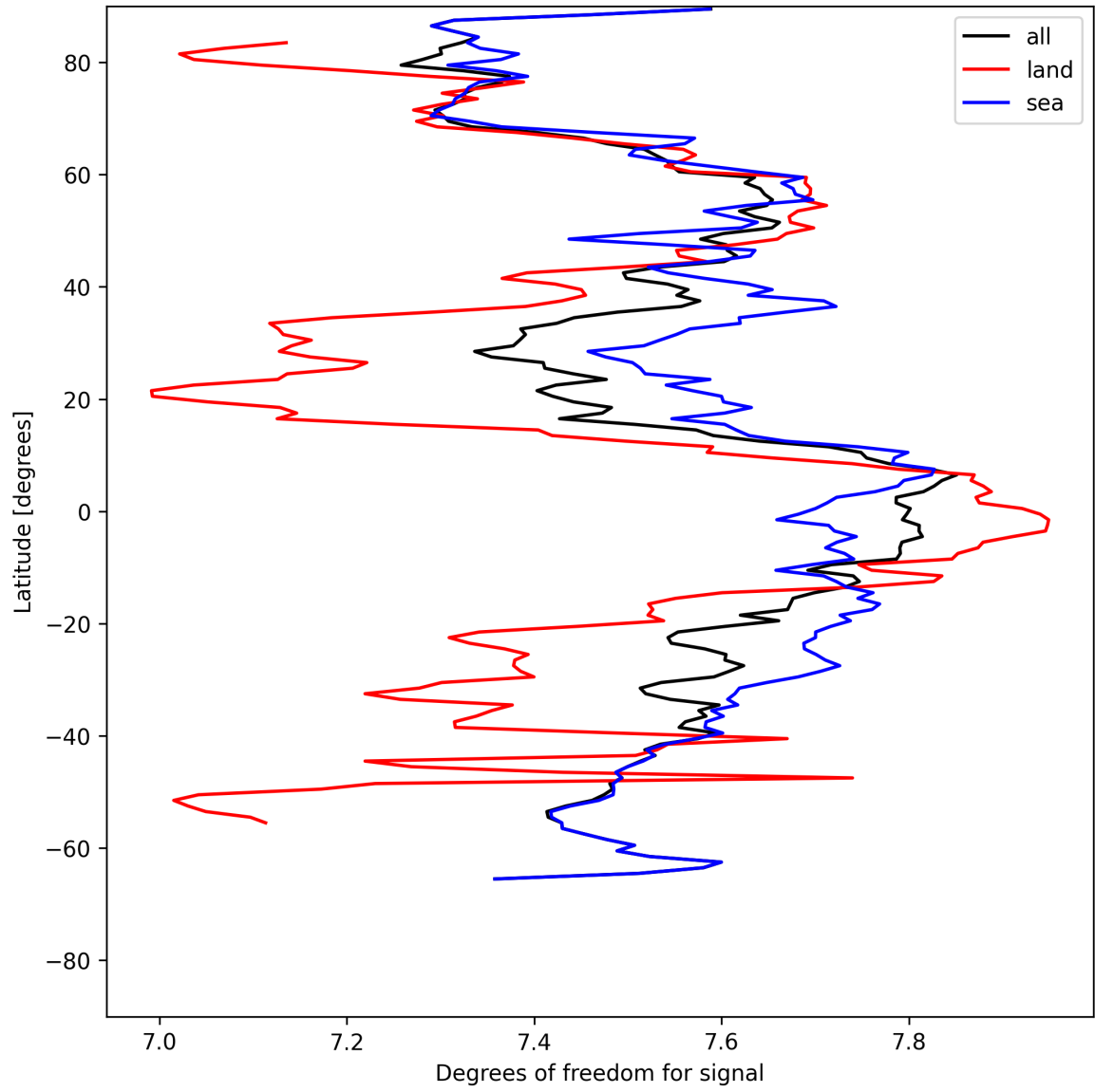
Figure 11: Zonal average of “Degrees of freedom for signal” for 2025-05-16 to 2025-05-17.
