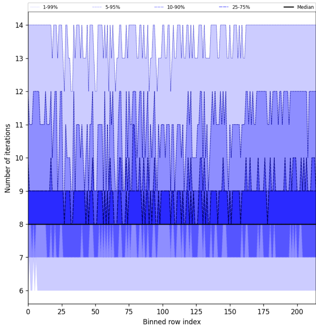
Figure 26: Along track statistics of “Number of iterations” for 2025-05-16 to 2025-05-17
