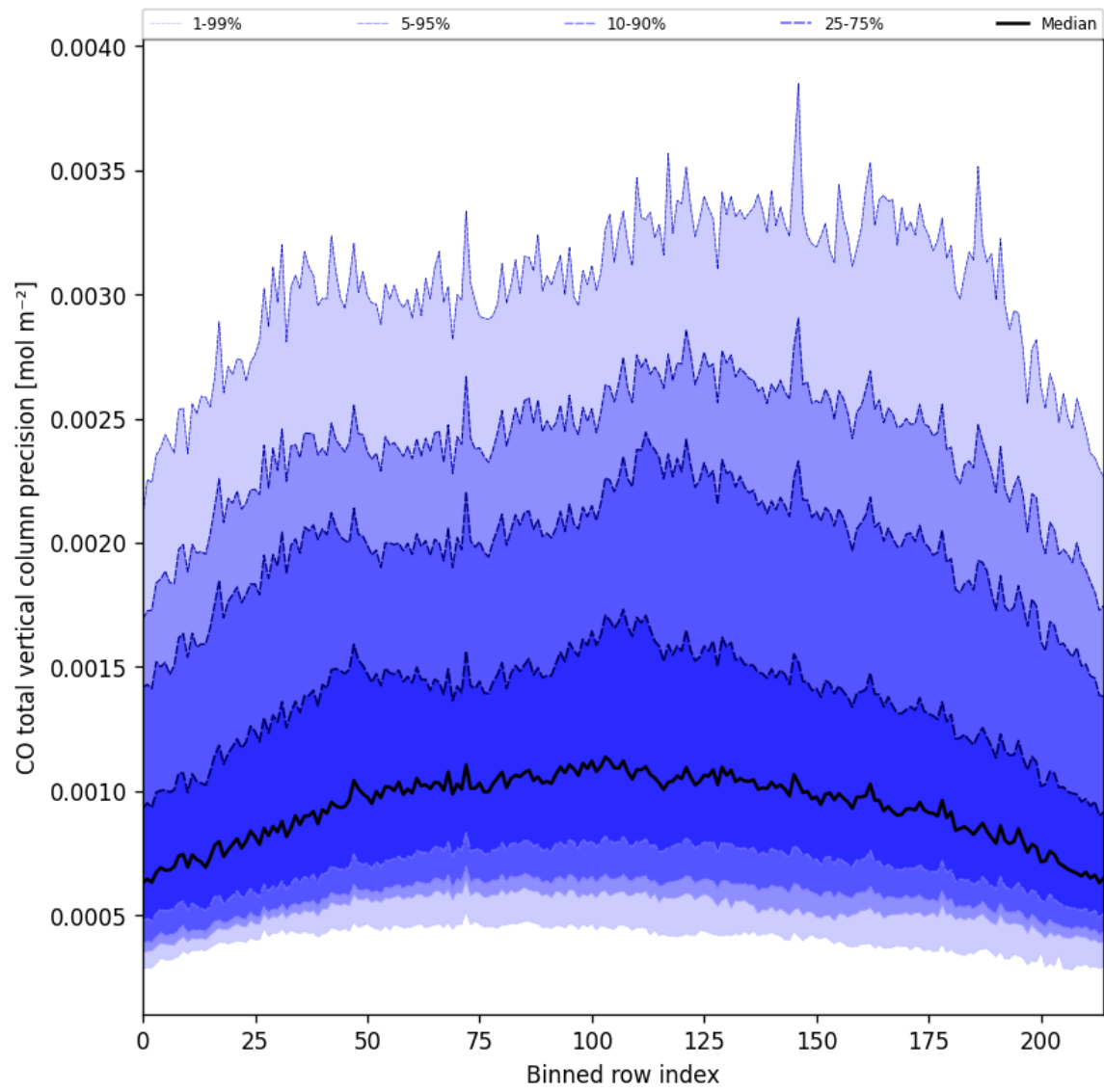
Figure 22: Along track statistics of “CO total vertical column precision” for 2025-05-16 to 2025-05-17
