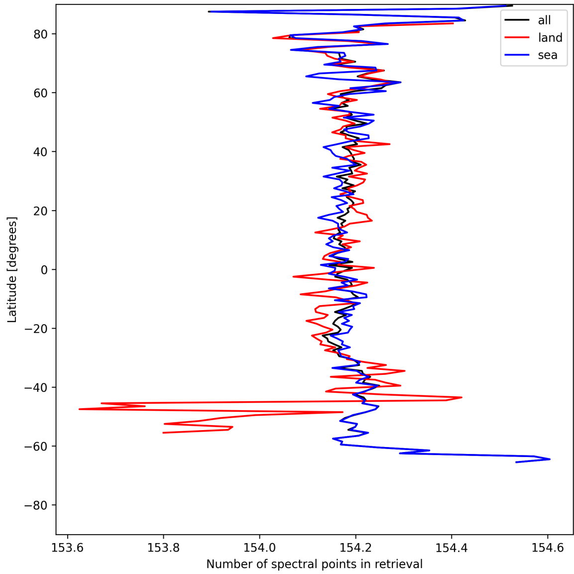
Figure 9: Zonal average of “Number of spectral points in retrieval” for 2025-05-16 to 2025-05-17.
