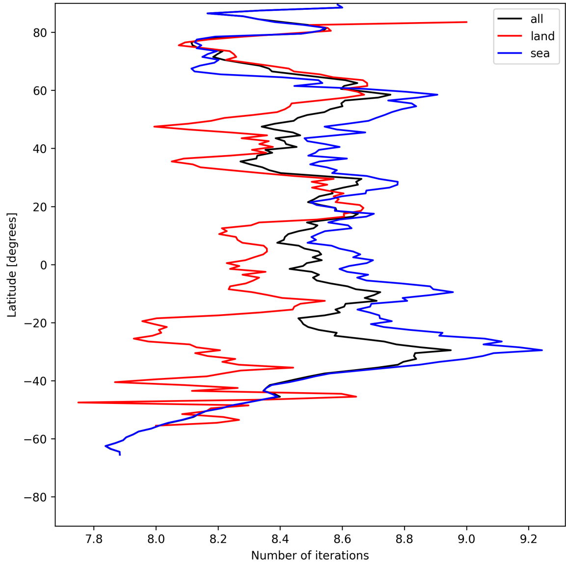
Figure 12: Zonal average of “Number of iterations” for 2025-05-16 to 2025-05-17.
