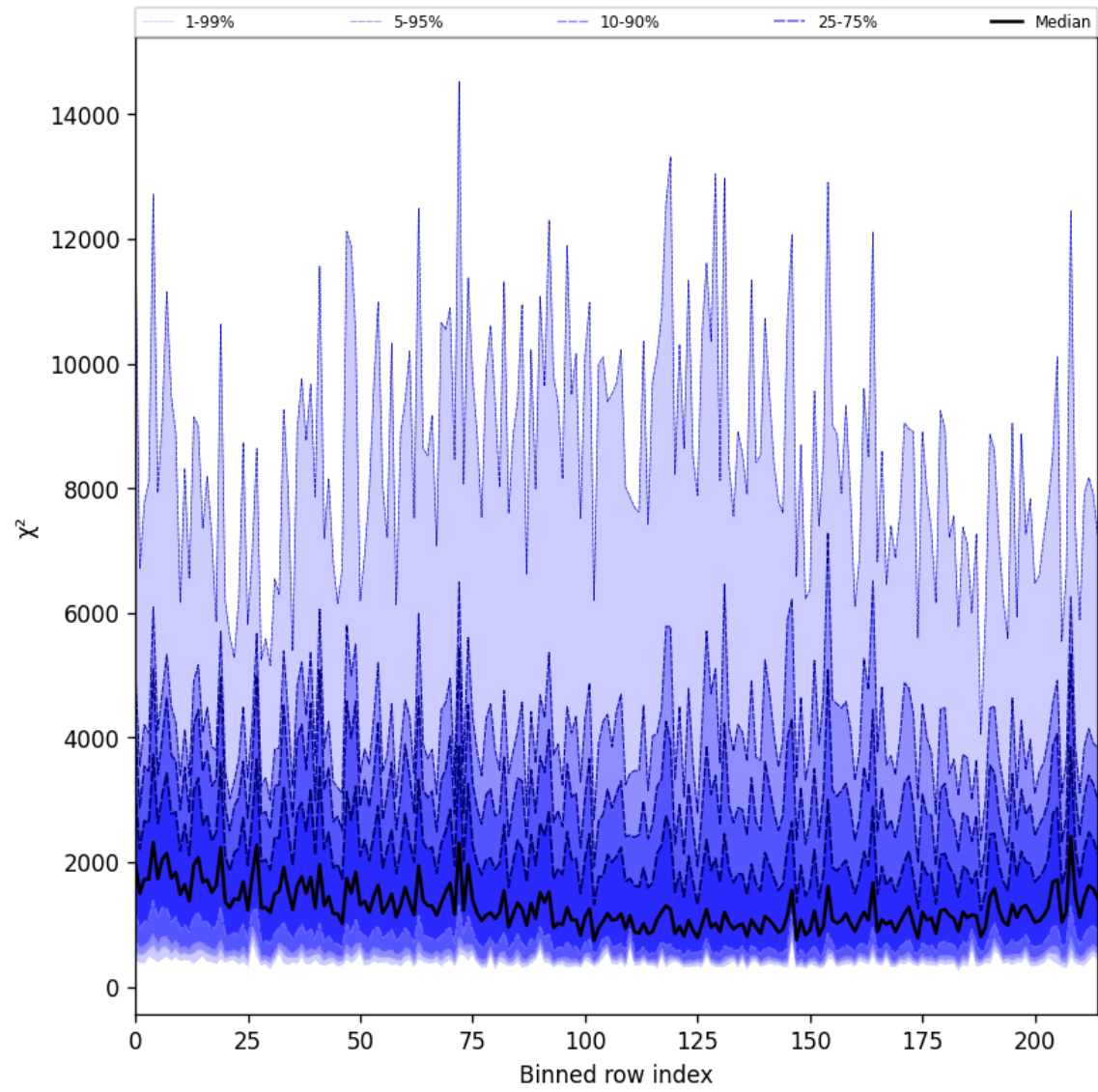
Figure 24: Along track statistics of “ \chi^2 ” for 2025-05-16 to 2025-05-17
