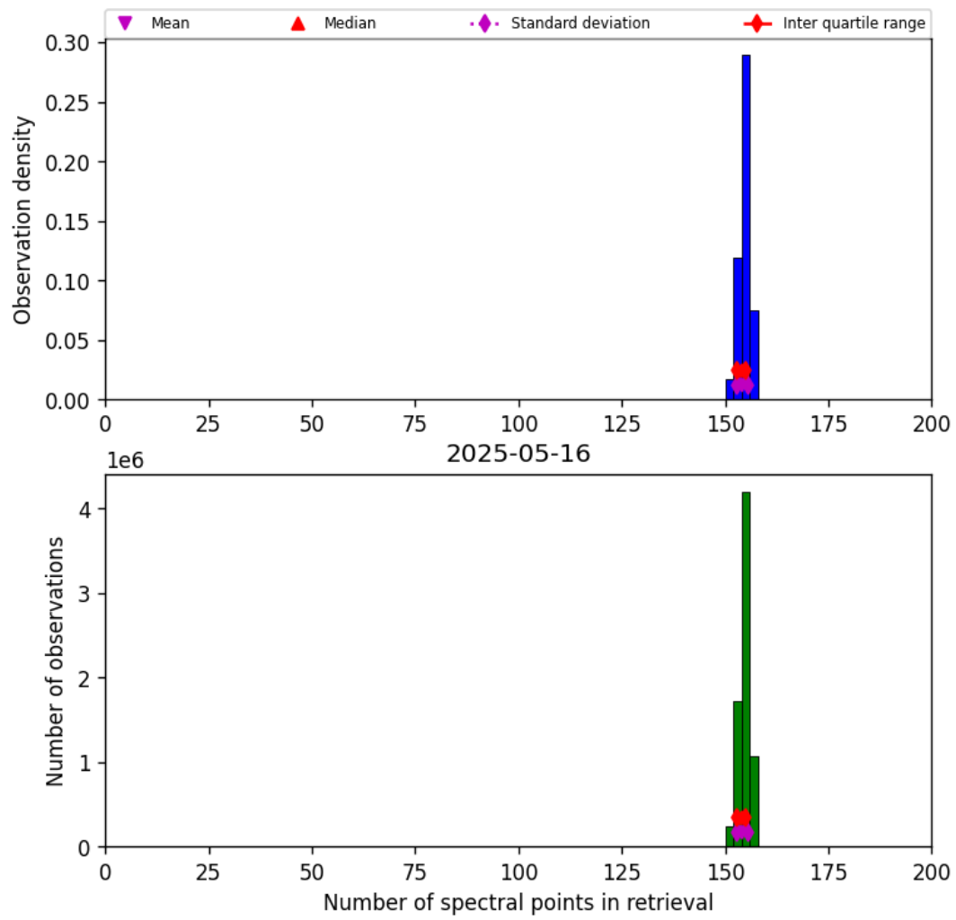
Figure 16: Histogram of “Number of spectral points in retrieval” for 2025-05-16 to 2025-05-17
