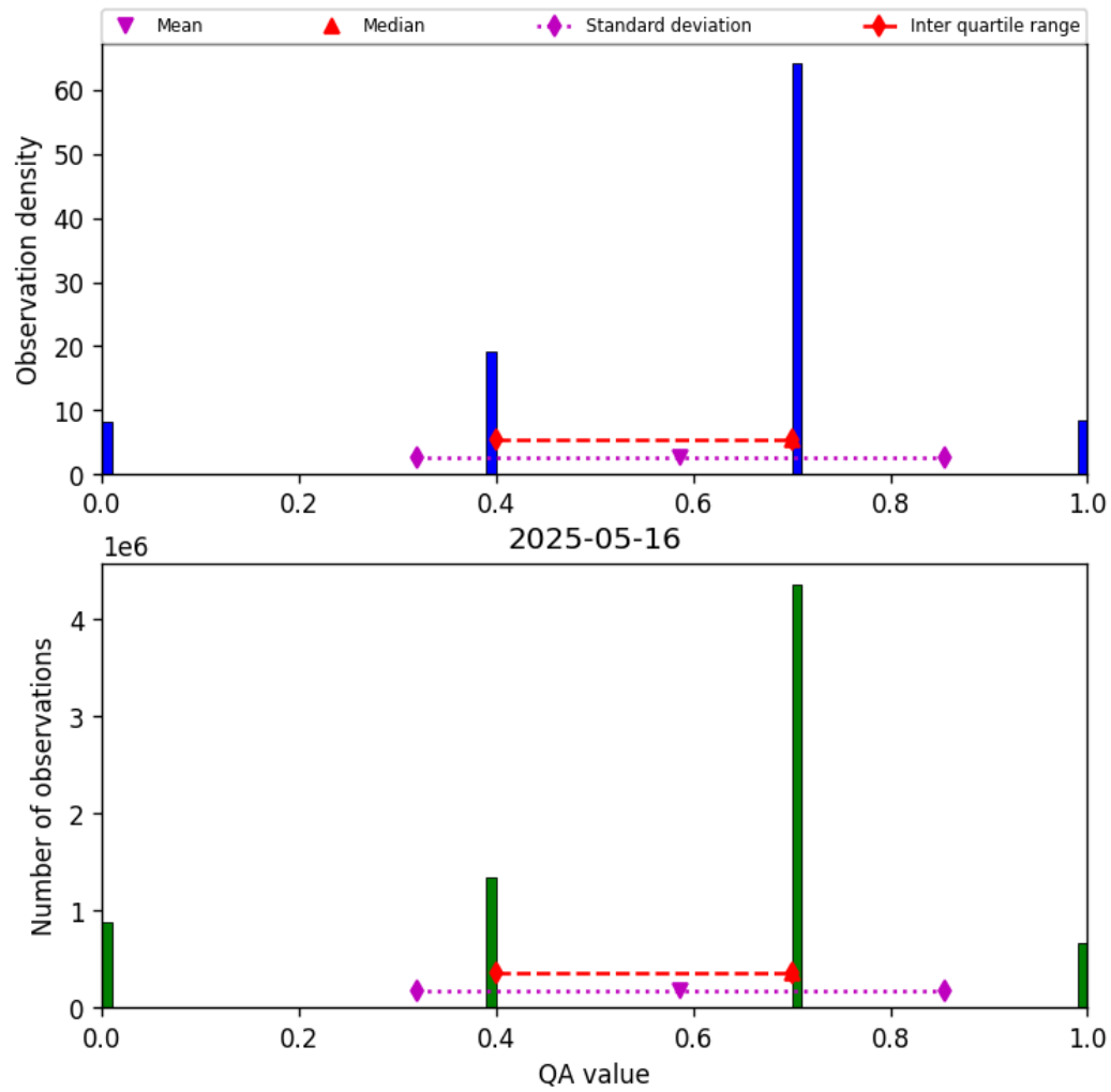
Figure 13: Histogram of “QA value” for 2025-05-16 to 2025-05-17
