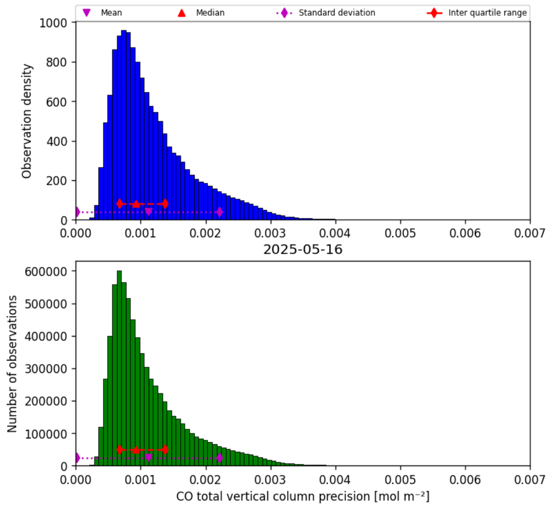
Figure 15: Histogram of “CO total vertical column precision” for 2025-05-16 to 2025-05-17
