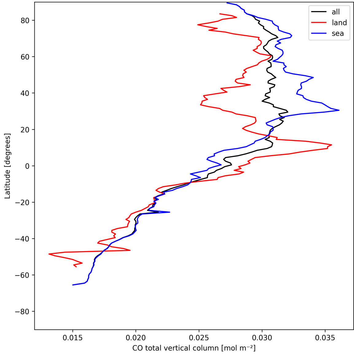
Figure 7: Zonal average of “CO total vertical column” for 2025-05-16 to 2025-05-17.
