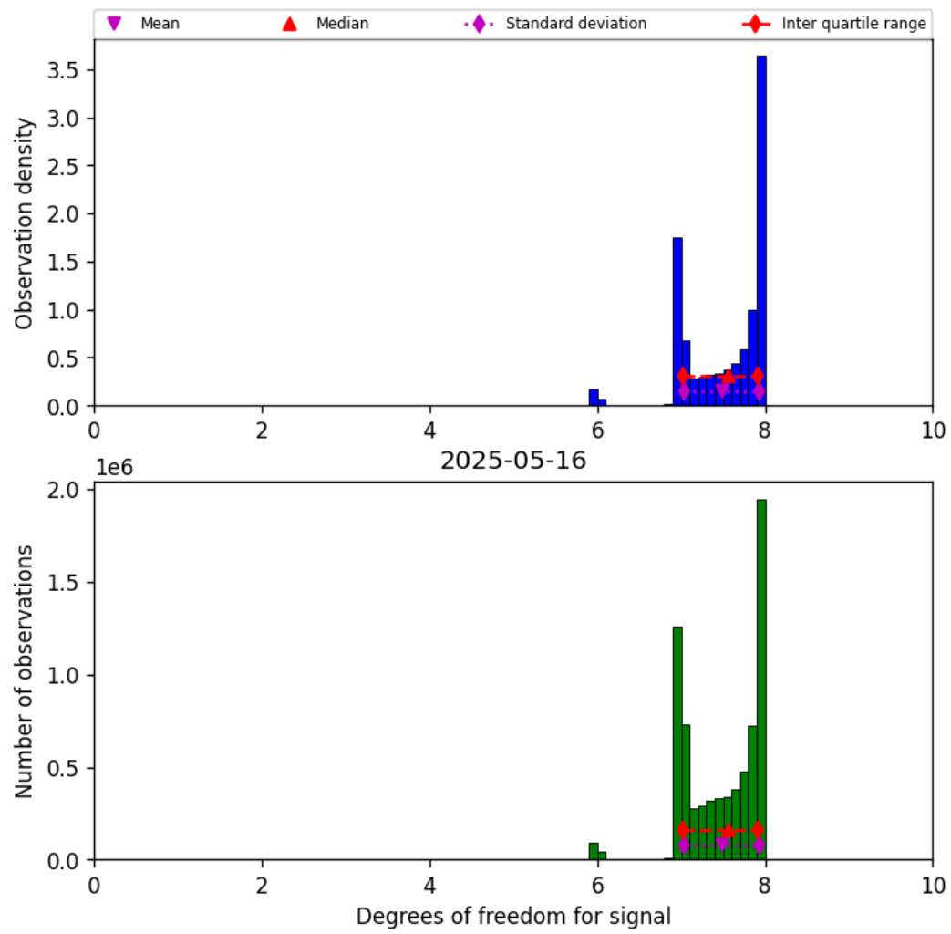
Figure 18: Histogram of “Degrees of freedom for signal” for 2025-05-16 to 2025-05-17
