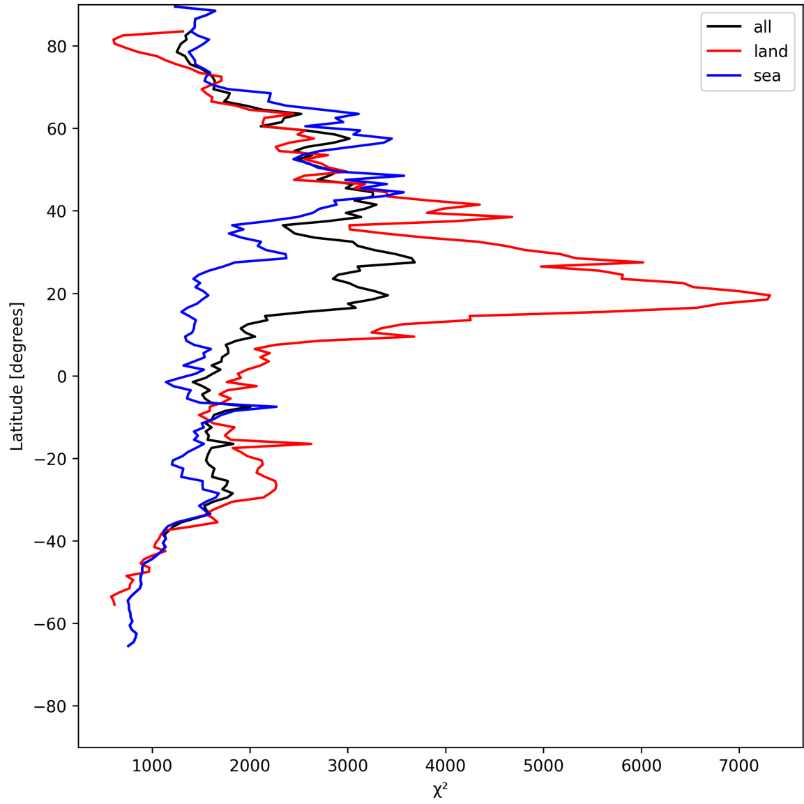
Figure 10: Zonal average of “ \chi^2 ” for 2025-05-16 to 2025-05-17.
