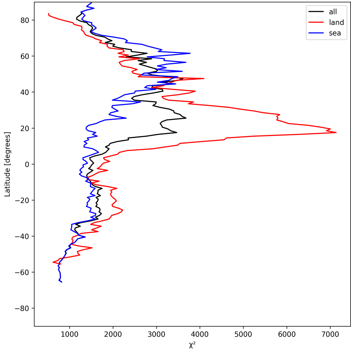
Figure 10: Zonal average of “ \chi^2 ” for 2025-05-17 to 2025-05-18.
