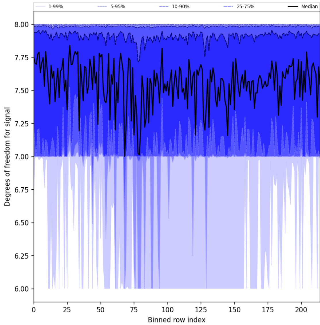
Figure 25: Along track statistics of “Degrees of freedom for signal” for 2025-05-17 to 2025-05-18
