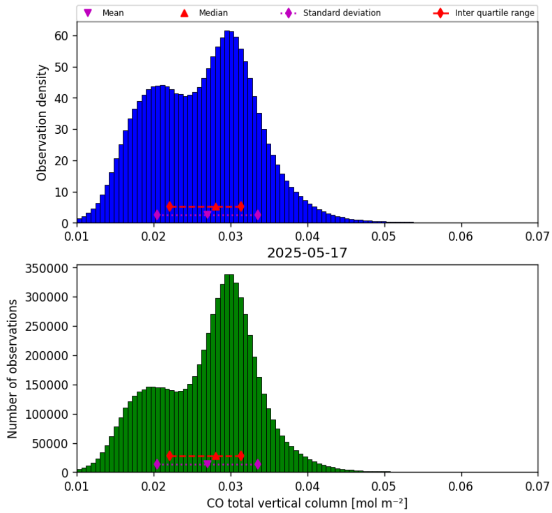
Figure 14: Histogram of “CO total vertical column” for 2025-05-17 to 2025-05-18
