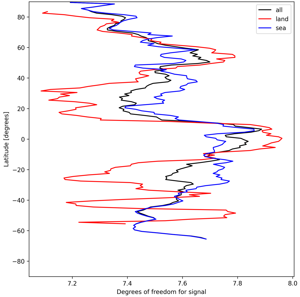
Figure 11: Zonal average of “Degrees of freedom for signal” for 2025-05-17 to 2025-05-18.
