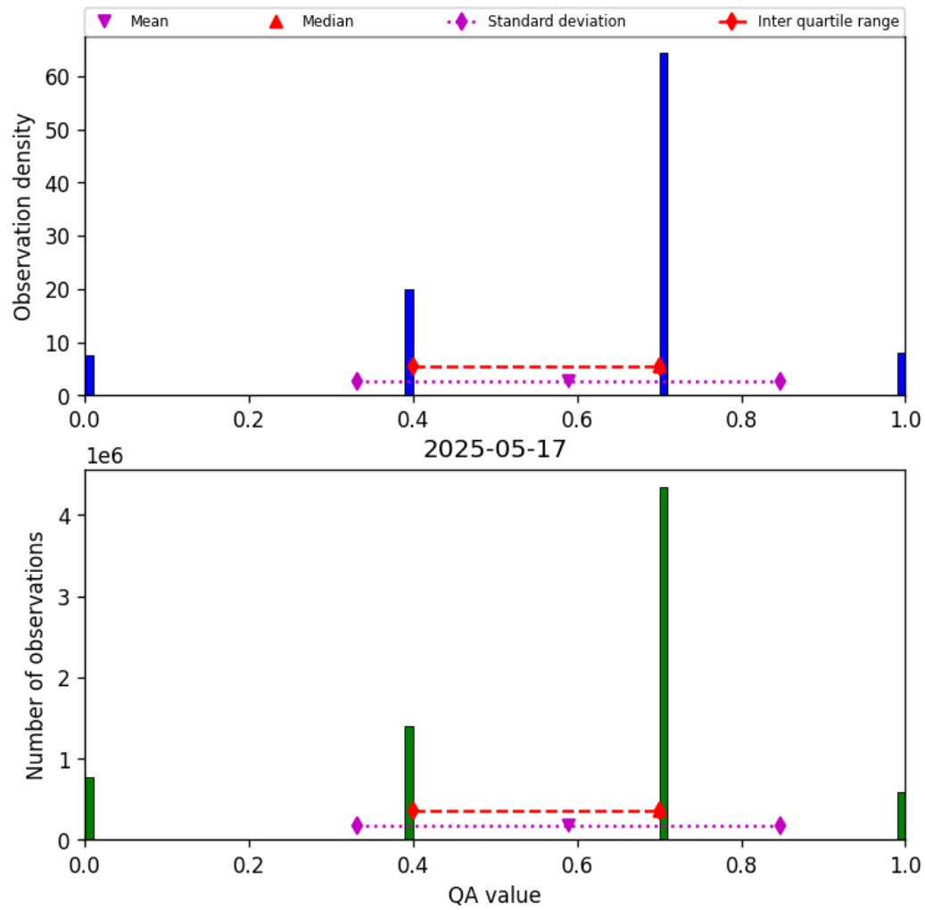
Figure 13: Histogram of “QA value” for 2025-05-17 to 2025-05-18
