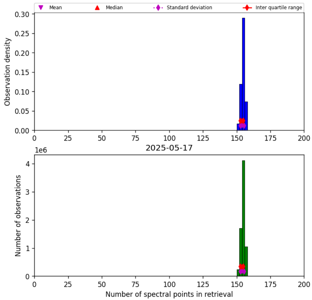
Figure 16: Histogram of “Number of spectral points in retrieval” for 2025-05-17 to 2025-05-18
