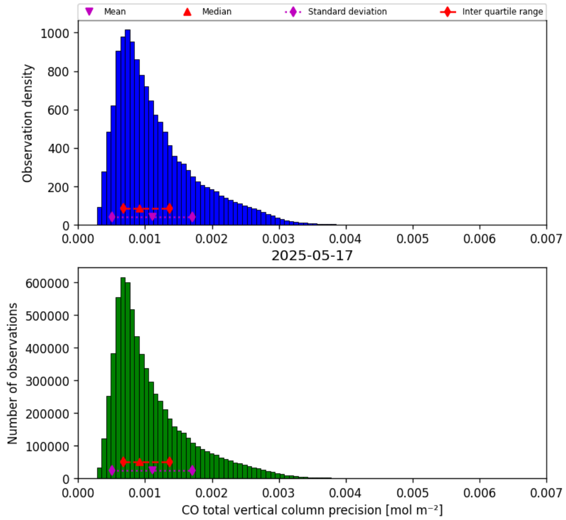
Figure 15: Histogram of “CO total vertical column precision” for 2025-05-17 to 2025-05-18
