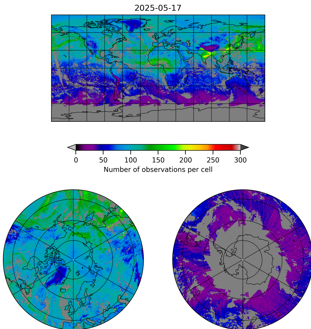
Figure 5: Map of the number of observations for 2025-05-17 to 2025-05-18
