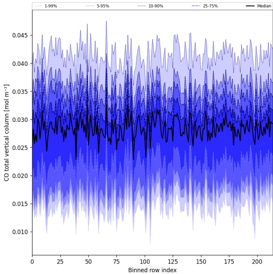
Figure 21: Along track statistics of “CO total vertical column” for 2025-05-17 to 2025-05-18
