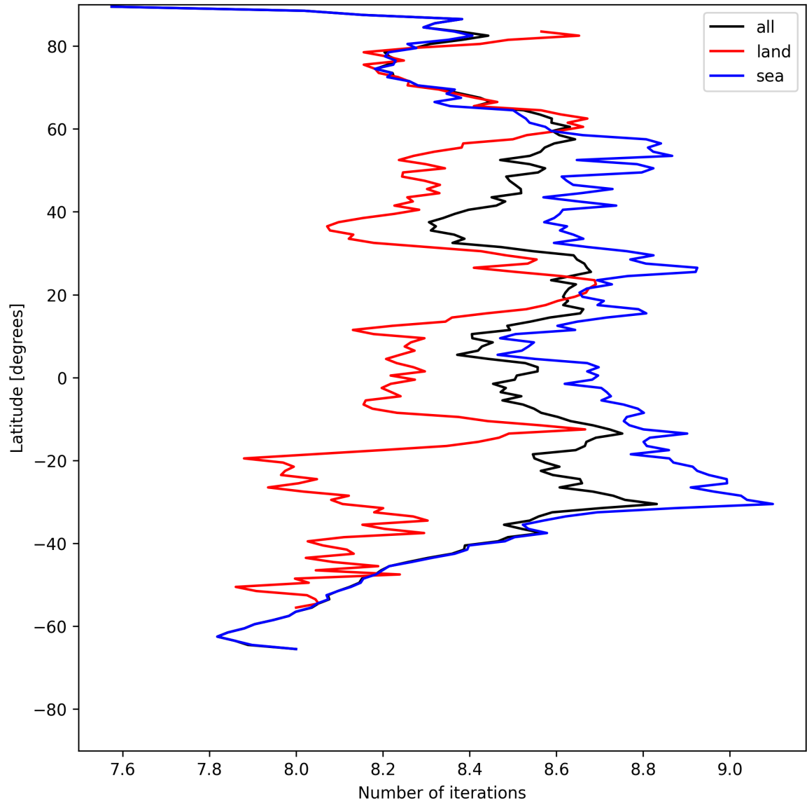
Figure 12: Zonal average of “Number of iterations” for 2025-05-17 to 2025-05-18.
