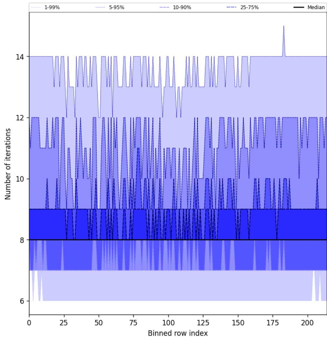
Figure 26: Along track statistics of “Number of iterations” for 2025-05-17 to 2025-05-18
