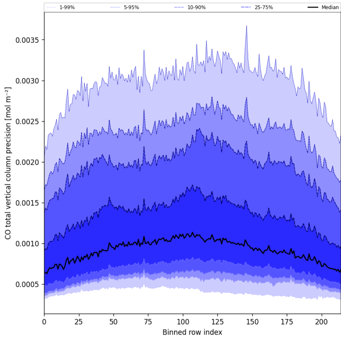
Figure 22: Along track statistics of “CO total vertical column precision” for 2025-05-17 to 2025-05-18
