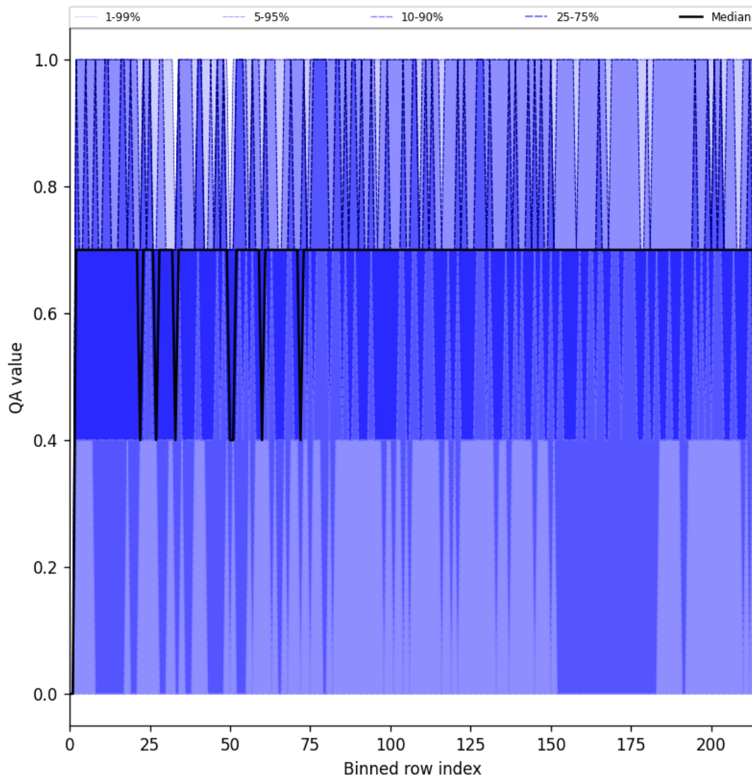
Figure 20: Along track statistics of “QA value” for 2025-05-17 to 2025-05-18
