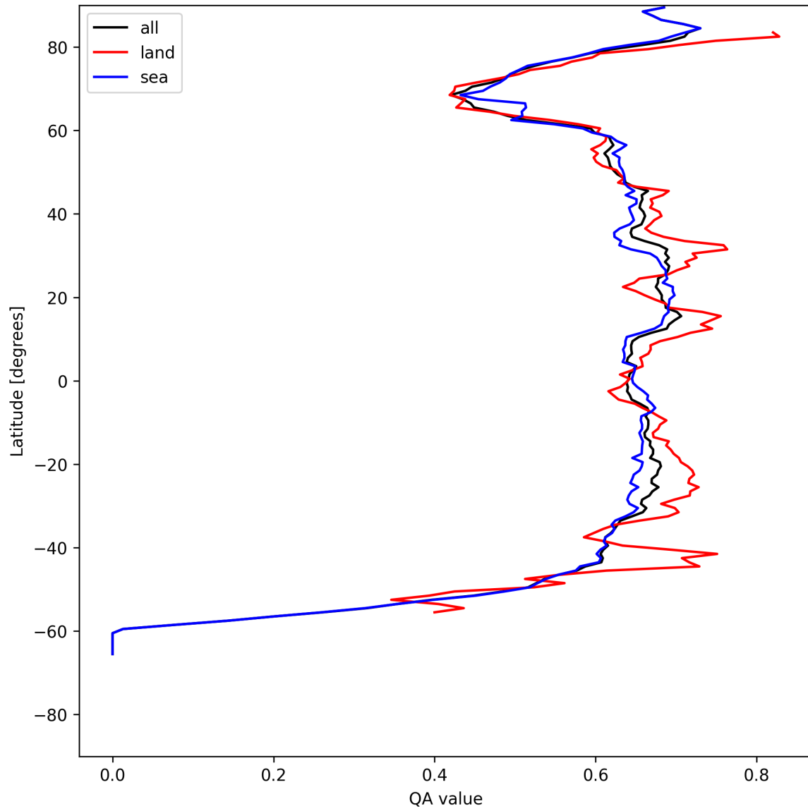
Figure 6: Zonal average of “QA value” for 2025-05-17 to 2025-05-18.
