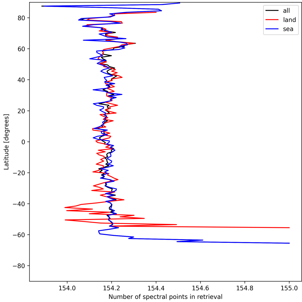
Figure 9: Zonal average of “Number of spectral points in retrieval” for 2025-05-17 to 2025-05-18.
