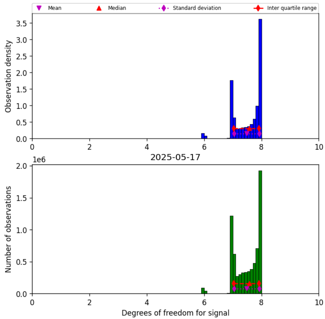
Figure 18: Histogram of “Degrees of freedom for signal” for 2025-05-17 to 2025-05-18
