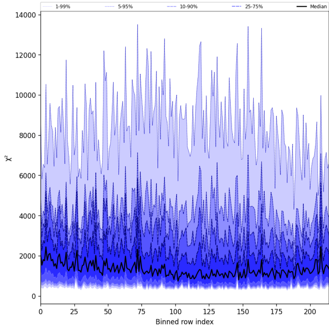
Figure 24: Along track statistics of “ \chi^2 ” for 2025-05-17 to 2025-05-18
