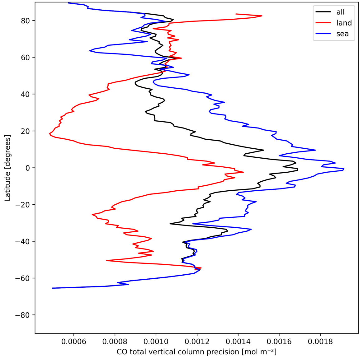
Figure 8: Zonal average of “CO total vertical column precision” for 2025-05-17 to 2025-05-18.
