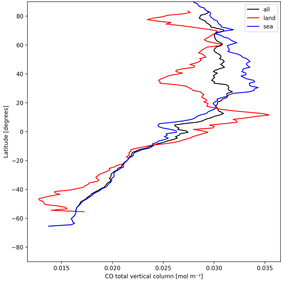
Figure 7: Zonal average of “CO total vertical column” for 2025-05-17 to 2025-05-18.
