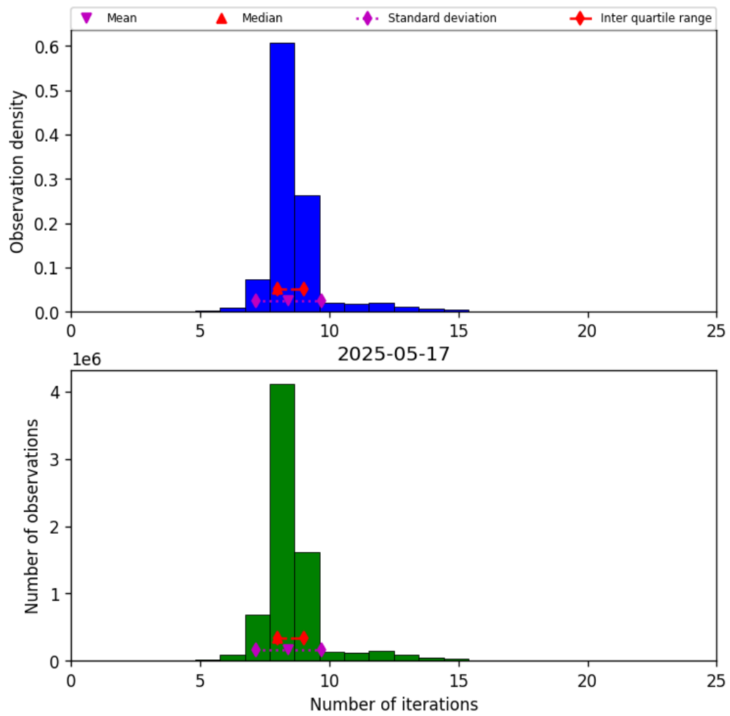
Figure 19: Histogram of “Number of iterations” for 2025-05-17 to 2025-05-18
