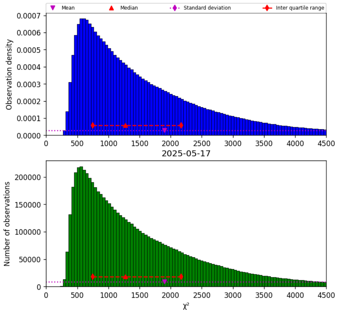
Figure 17: Histogram of “ \chi^2 ” for 2025-05-17 to 2025-05-18
