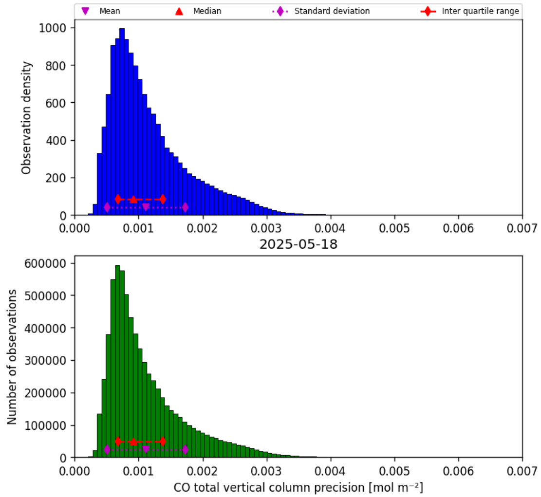
Figure 15: Histogram of “CO total vertical column precision” for 2025-05-18 to 2025-05-19
