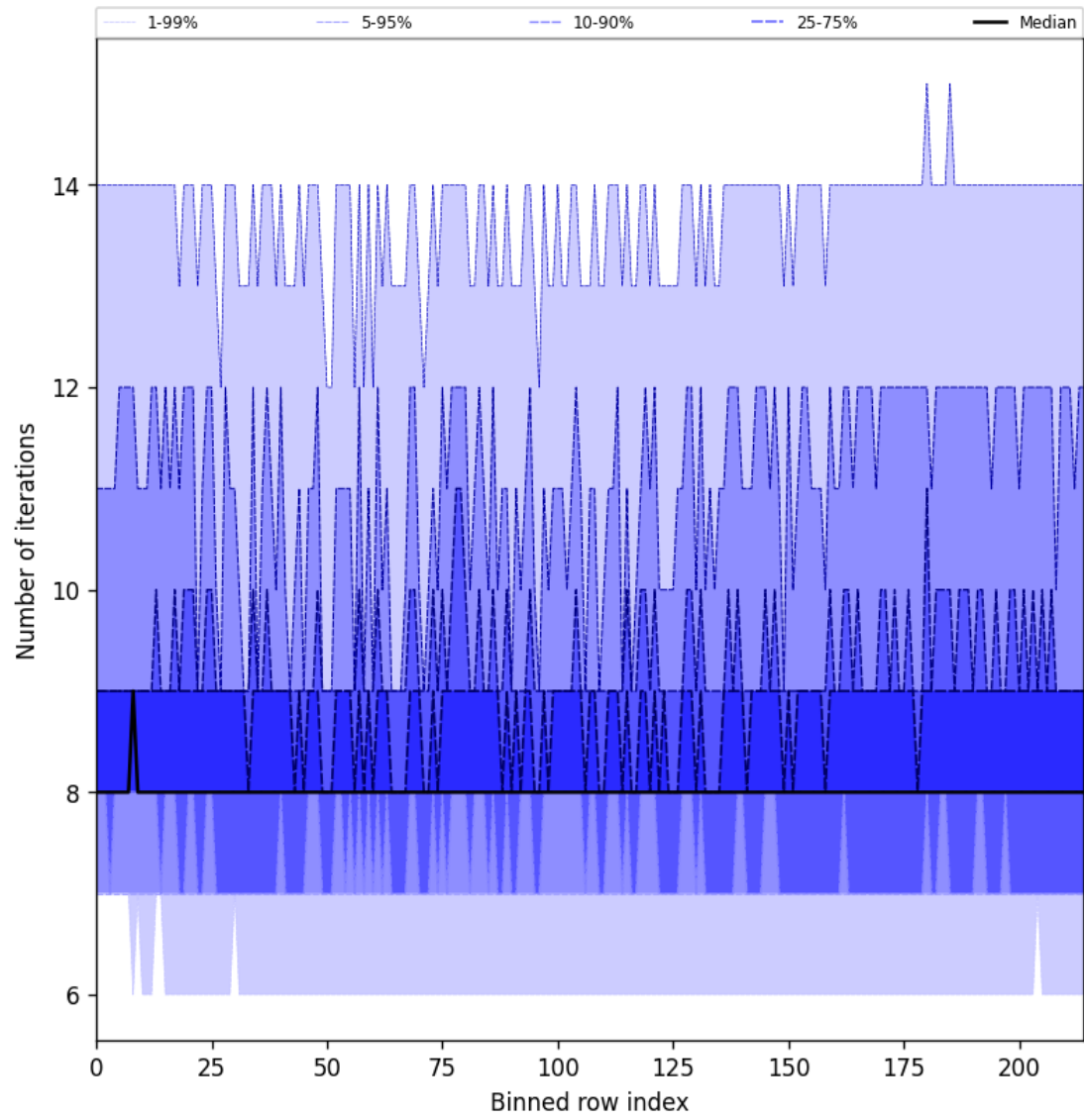
Figure 26: Along track statistics of “Number of iterations” for 2025-05-18 to 2025-05-19
