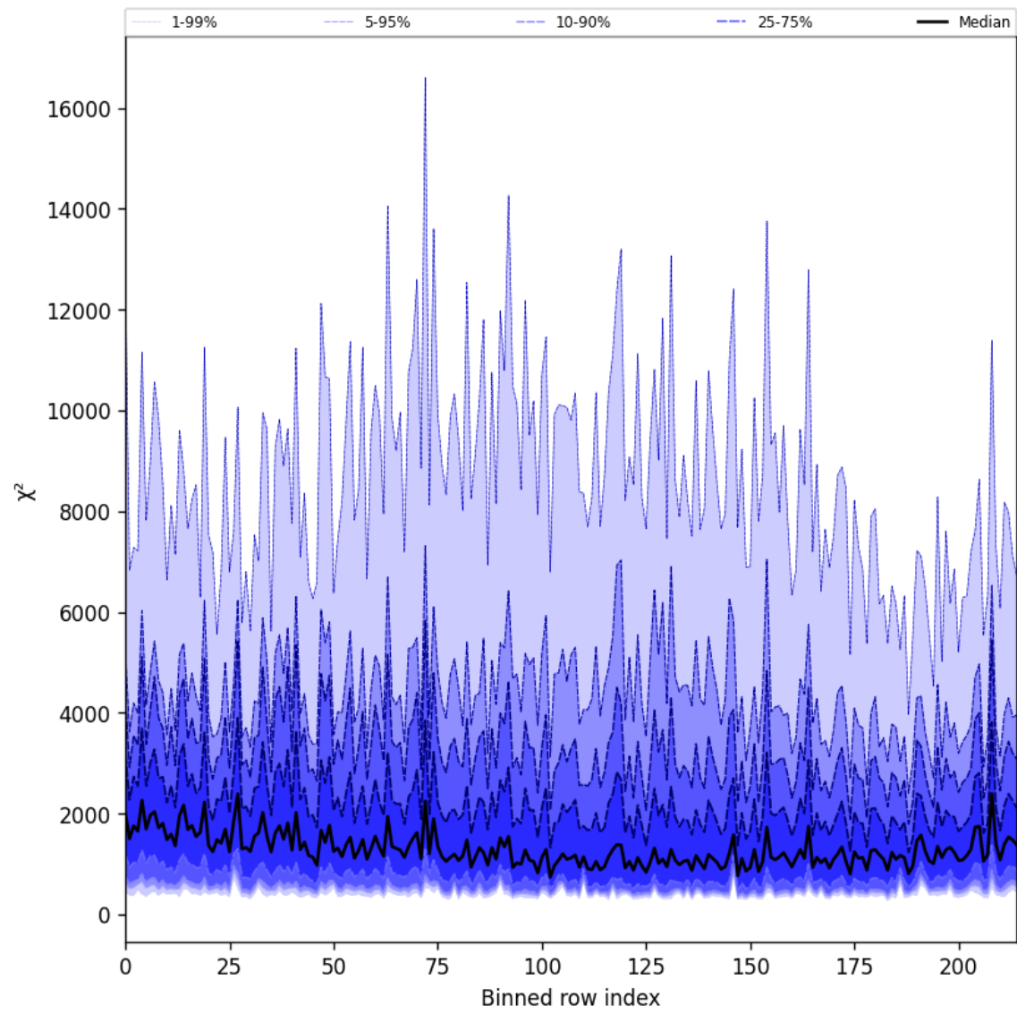
Figure 24: Along track statistics of “ \chi^2 ” for 2025-05-18 to 2025-05-19
