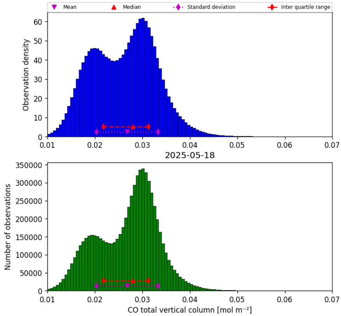
Figure 14: Histogram of “CO total vertical column” for 2025-05-18 to 2025-05-19
