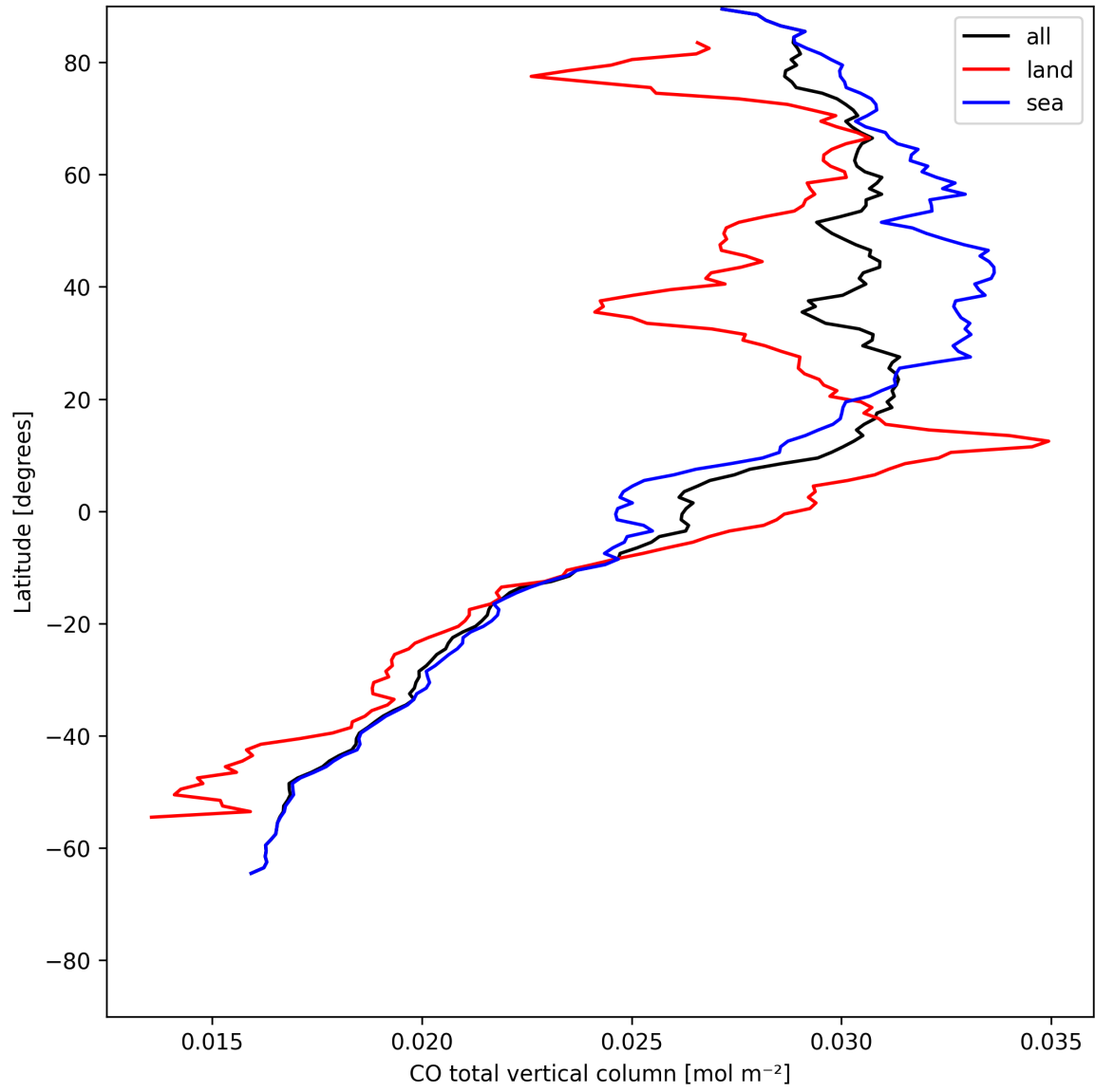
Figure 7: Zonal average of “CO total vertical column” for 2025-05-18 to 2025-05-19.
