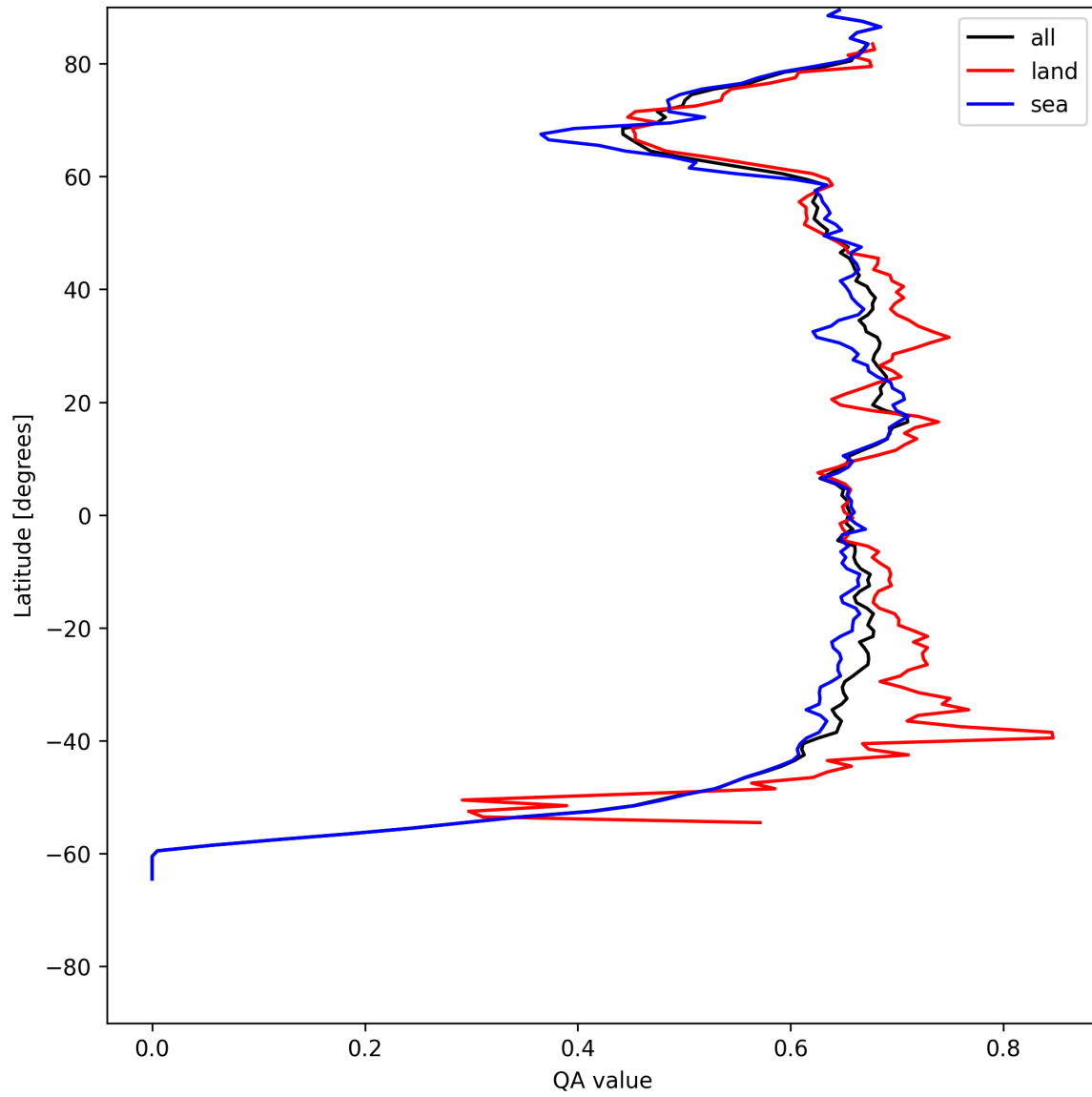
Figure 6: Zonal average of “QA value” for 2025-05-18 to 2025-05-19.
