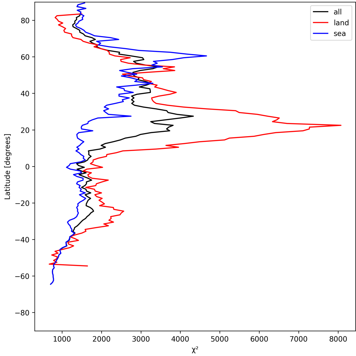
Figure 10: Zonal average of “ \chi^2 ” for 2025-05-18 to 2025-05-19.
