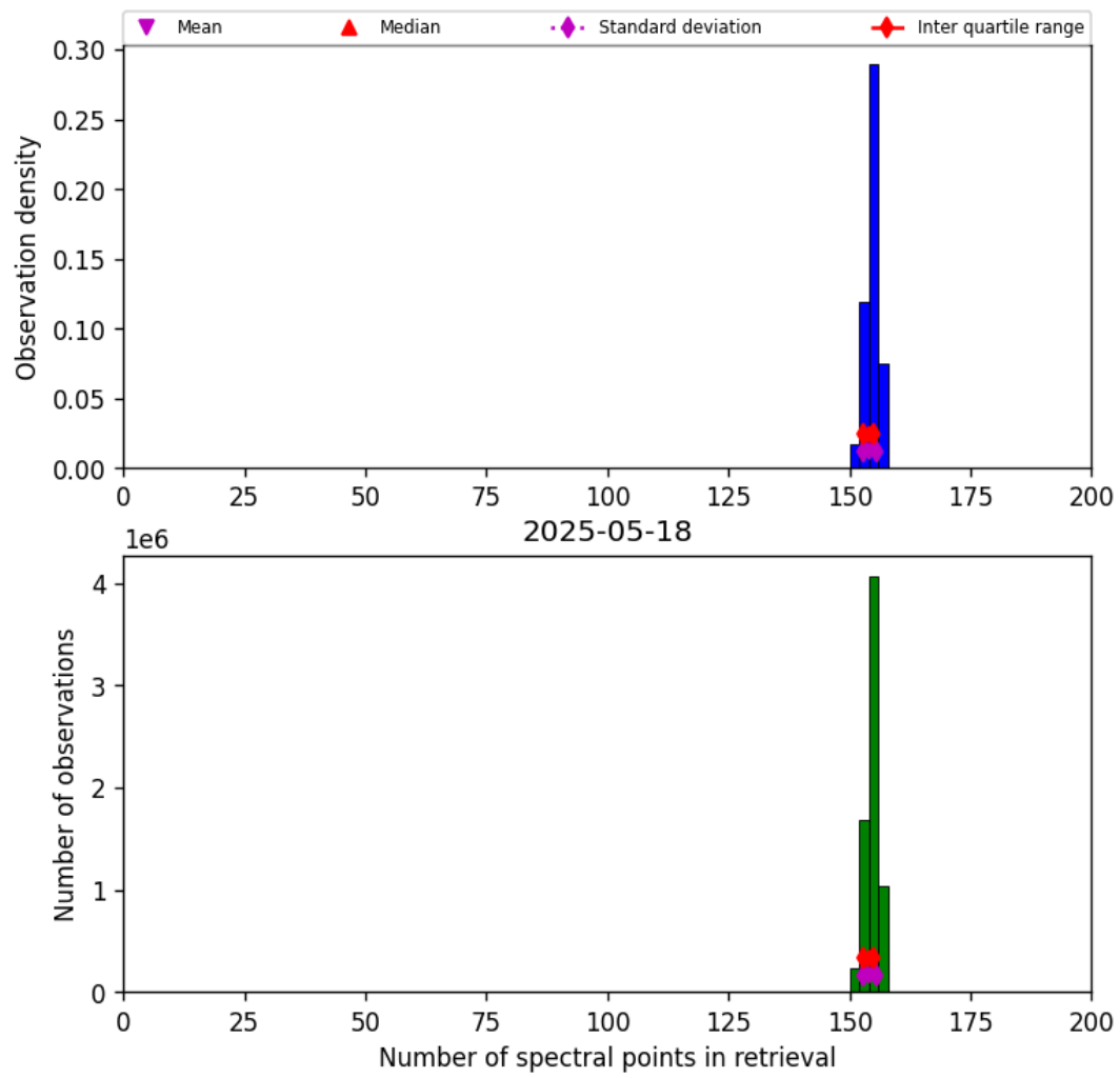
Figure 16: Histogram of “Number of spectral points in retrieval” for 2025-05-18 to 2025-05-19
