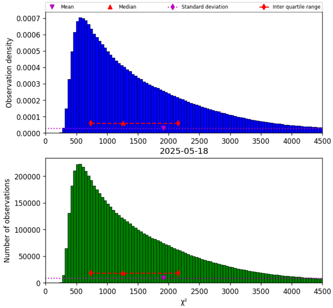
Figure 17: Histogram of “ \chi^2 ” for 2025-05-18 to 2025-05-19
