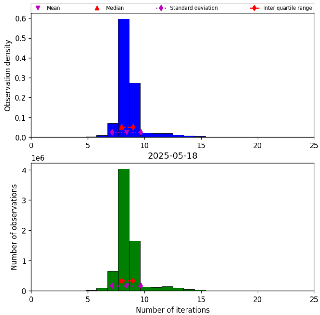
Figure 19: Histogram of “Number of iterations” for 2025-05-18 to 2025-05-19
