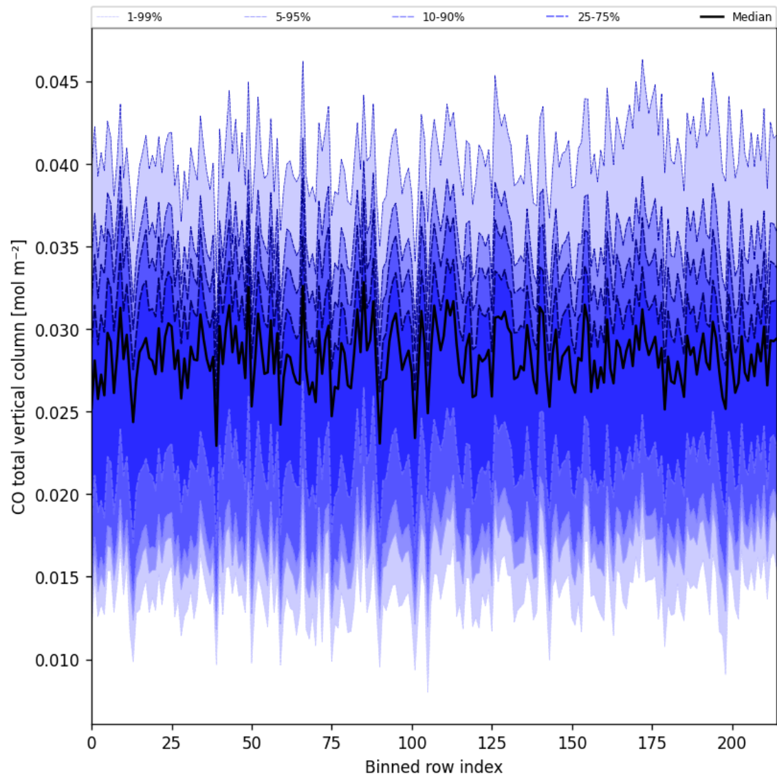
Figure 21: Along track statistics of “CO total vertical column” for 2025-05-18 to 2025-05-19
