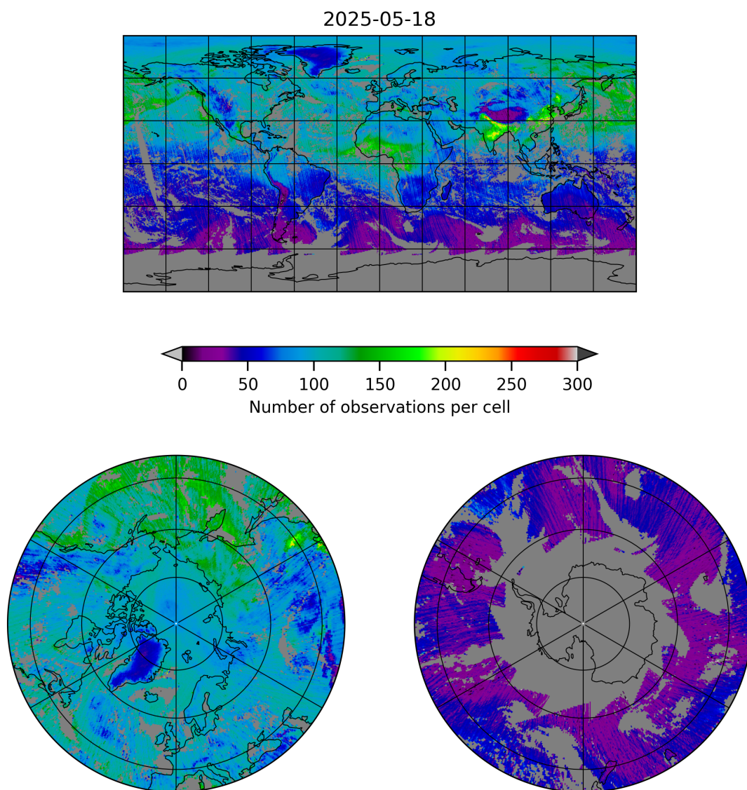
Figure 5: Map of the number of observations for 2025-05-18 to 2025-05-19
