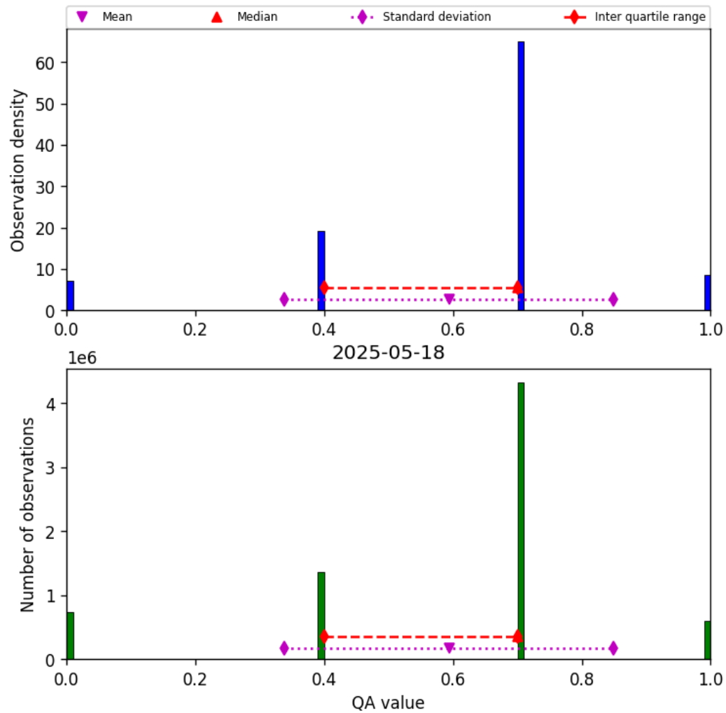
Figure 13: Histogram of “QA value” for 2025-05-18 to 2025-05-19
