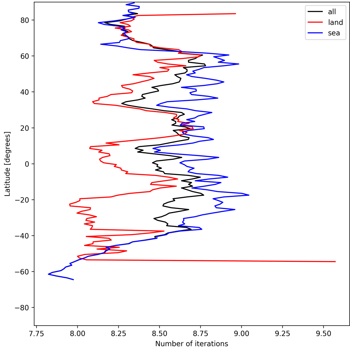
Figure 12: Zonal average of “Number of iterations” for 2025-05-18 to 2025-05-19.
