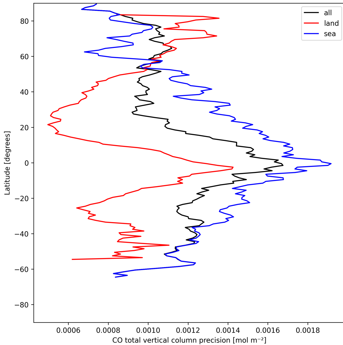
Figure 8: Zonal average of “CO total vertical column precision” for 2025-05-18 to 2025-05-19.
