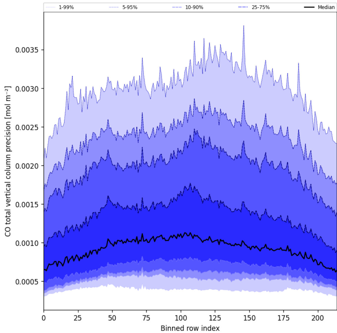
Figure 22: Along track statistics of “CO total vertical column precision” for 2025-05-18 to 2025-05-19
