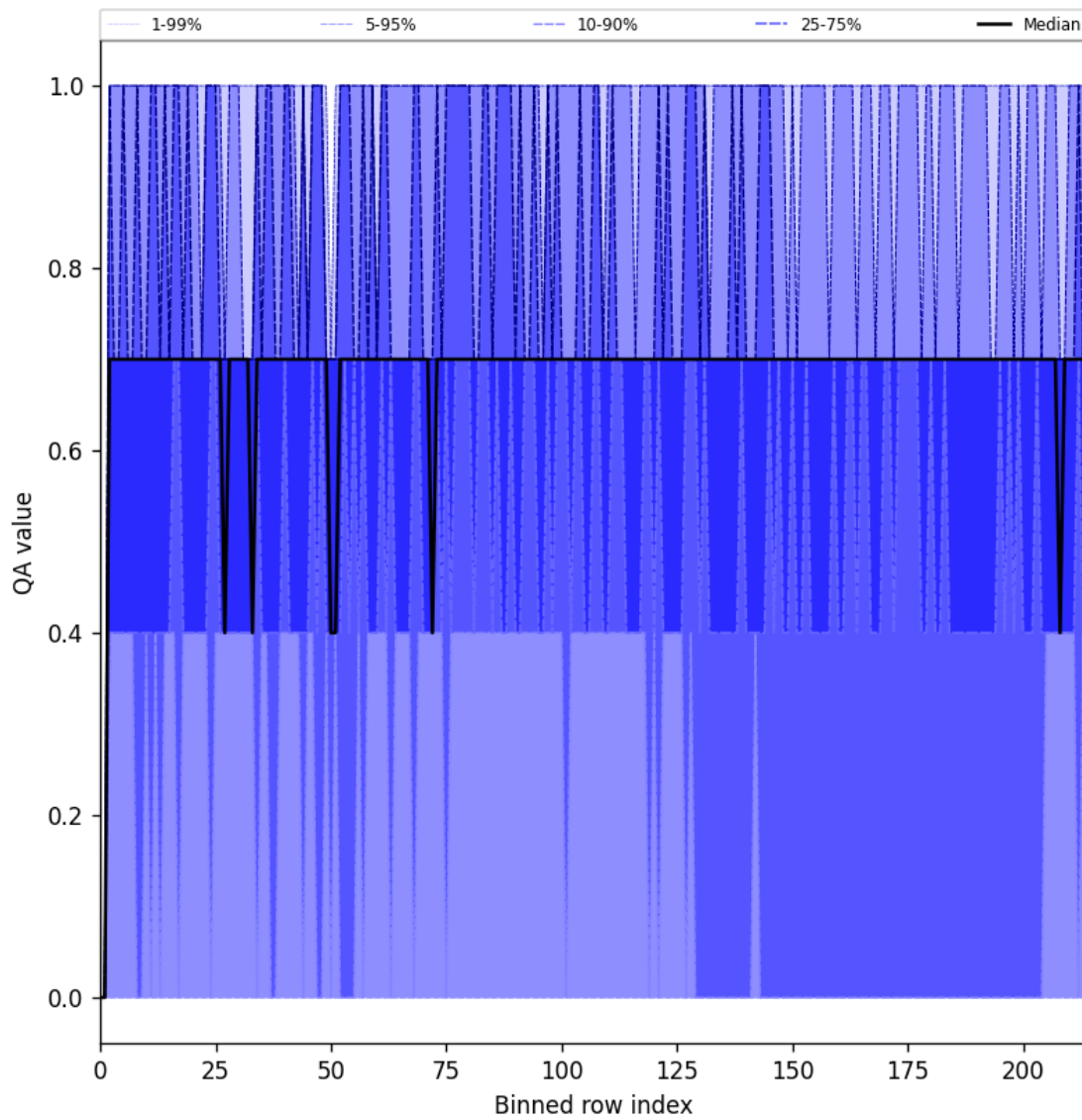
Figure 20: Along track statistics of “QA value” for 2025-05-18 to 2025-05-19
