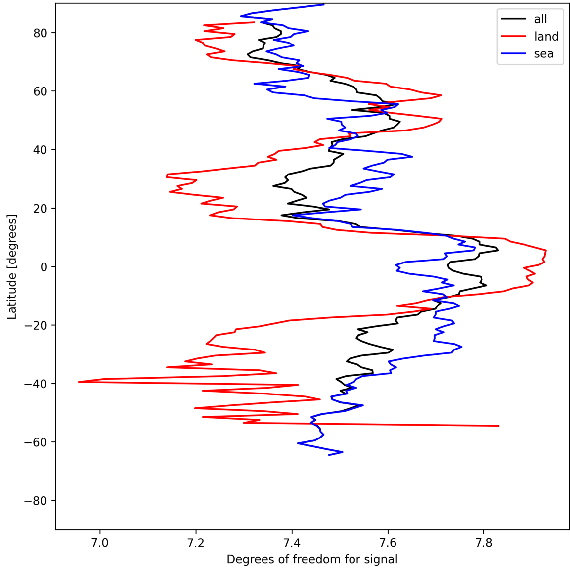
Figure 11: Zonal average of “Degrees of freedom for signal” for 2025-05-18 to 2025-05-19.
