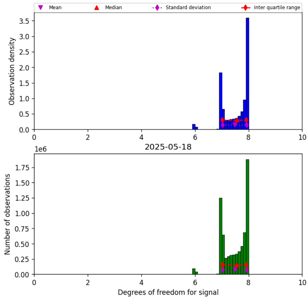
Figure 18: Histogram of “Degrees of freedom for signal” for 2025-05-18 to 2025-05-19
