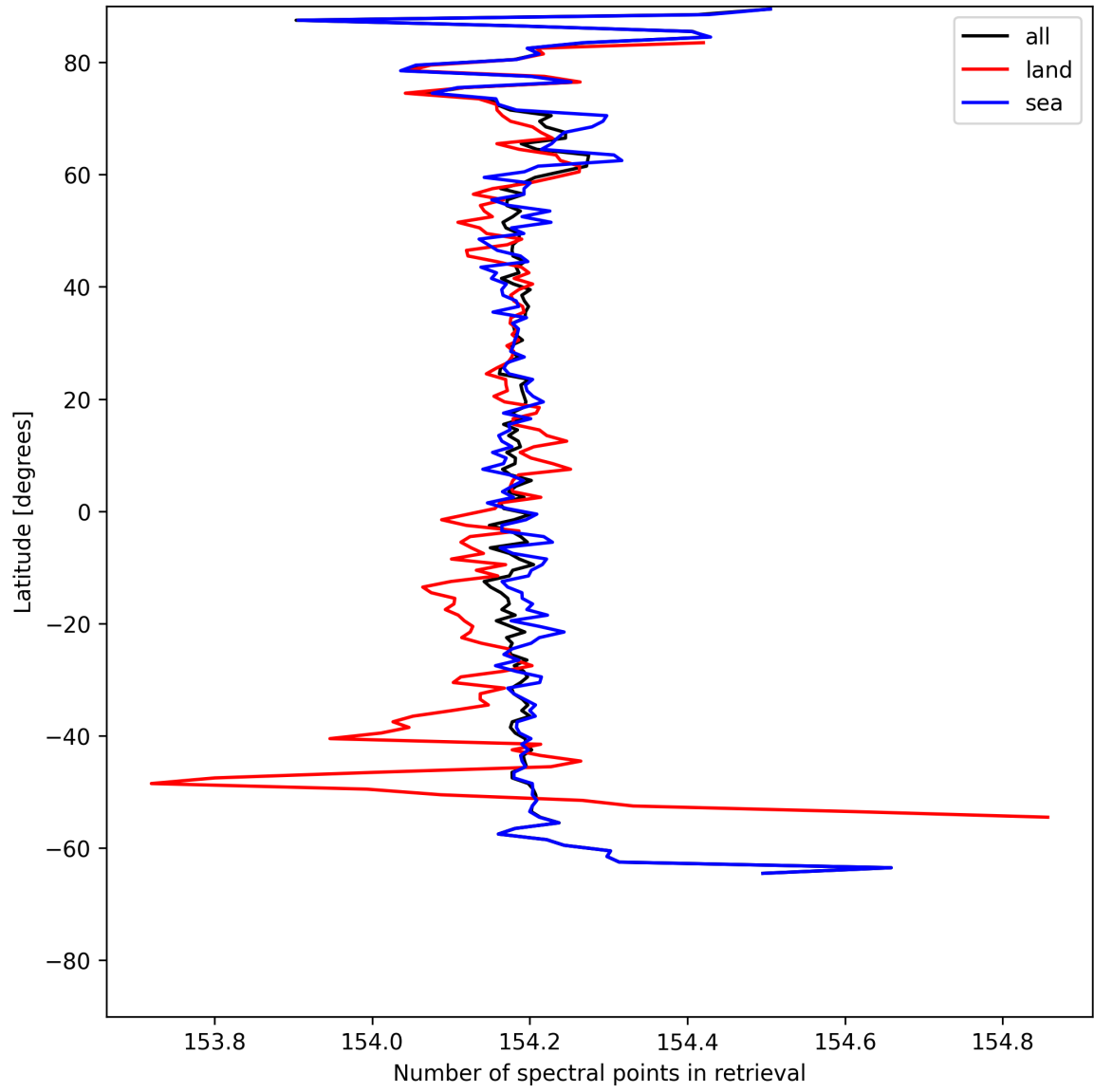
Figure 9: Zonal average of “Number of spectral points in retrieval” for 2025-05-18 to 2025-05-19.
