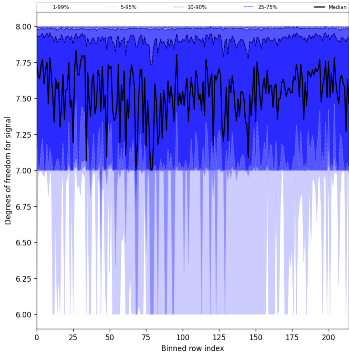
Figure 25: Along track statistics of “Degrees of freedom for signal” for 2025-05-18 to 2025-05-19
