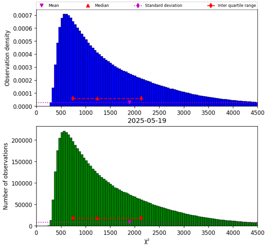
Figure 17: Histogram of " \chi^2 " for 2025-05-19 to 2025-05-19
