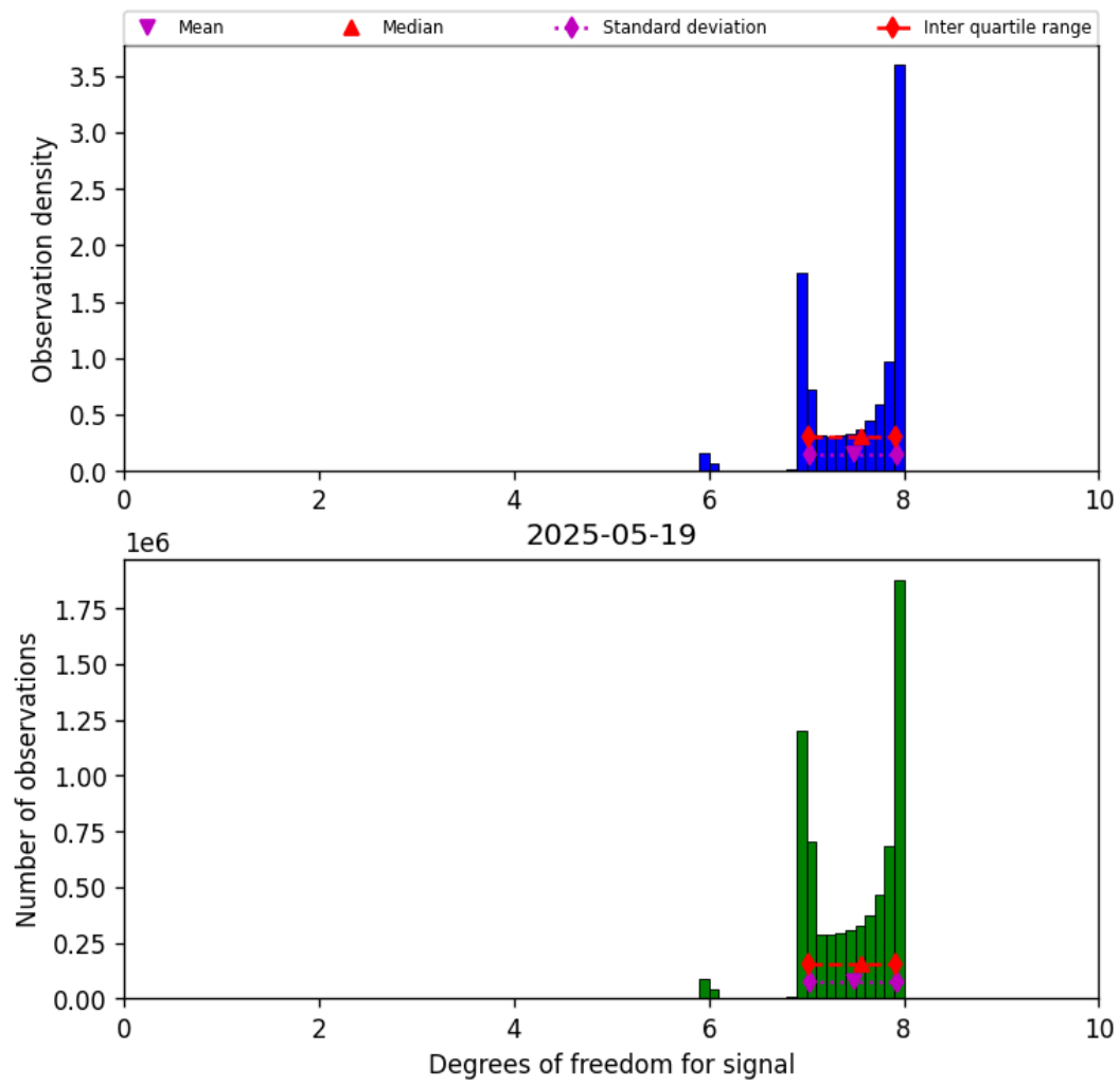
Figure 18: Histogram of “Degrees of freedom for signal” for 2025-05-19 to 2025-05-19
