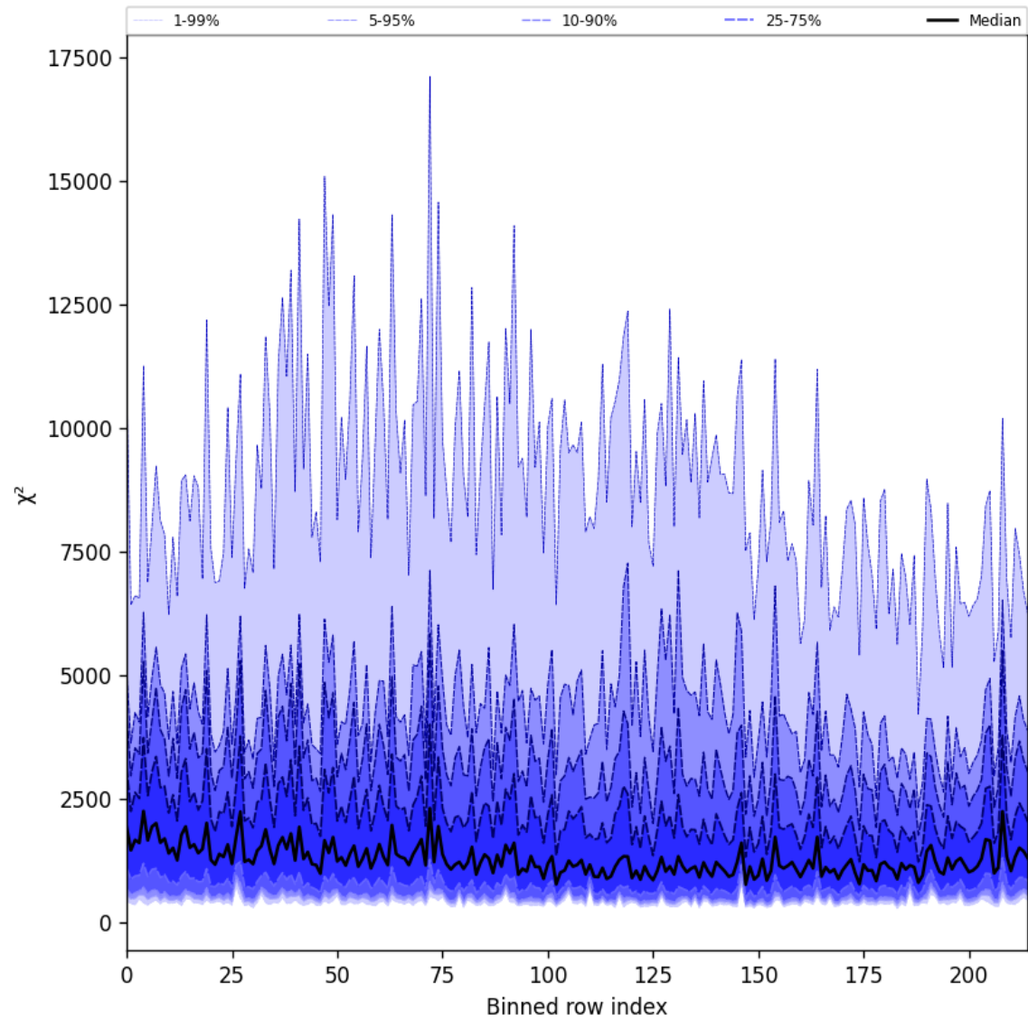
Figure 24: Along track statistics of “ \chi^2 ” for 2025-05-19 to 2025-05-19
