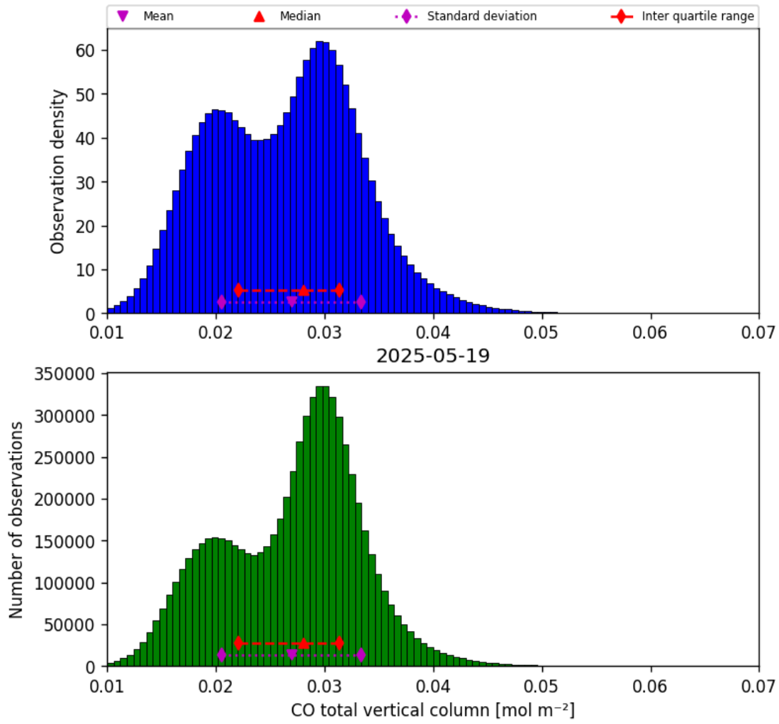
Figure 14: Histogram of “CO total vertical column” for 2025-05-19 to 2025-05-19
