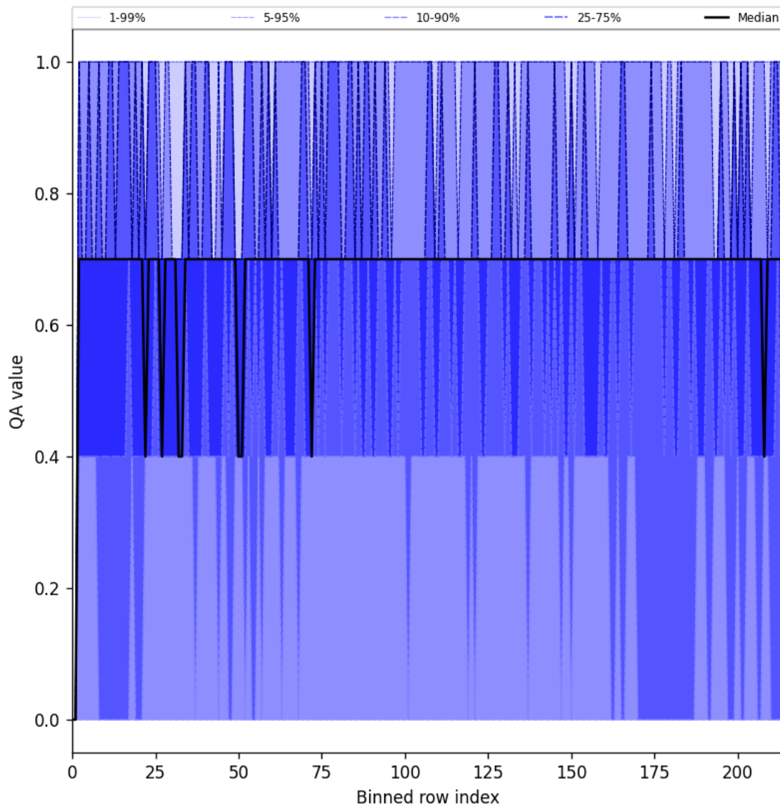
Figure 20: Along track statistics of “QA value” for 2025-05-19 to 2025-05-19
