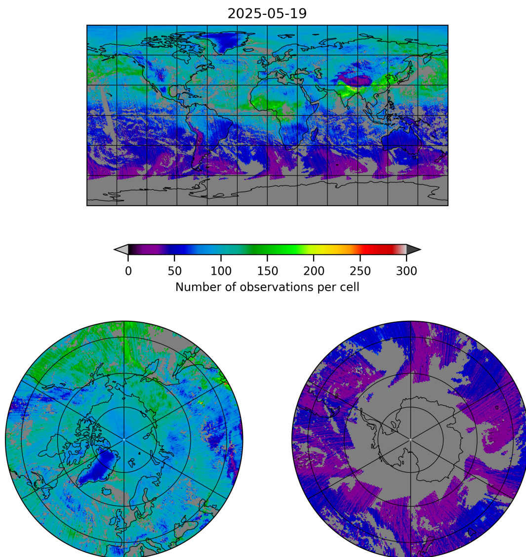
Figure 5: Map of the number of observations for 2025-05-19 to 2025-05-19
