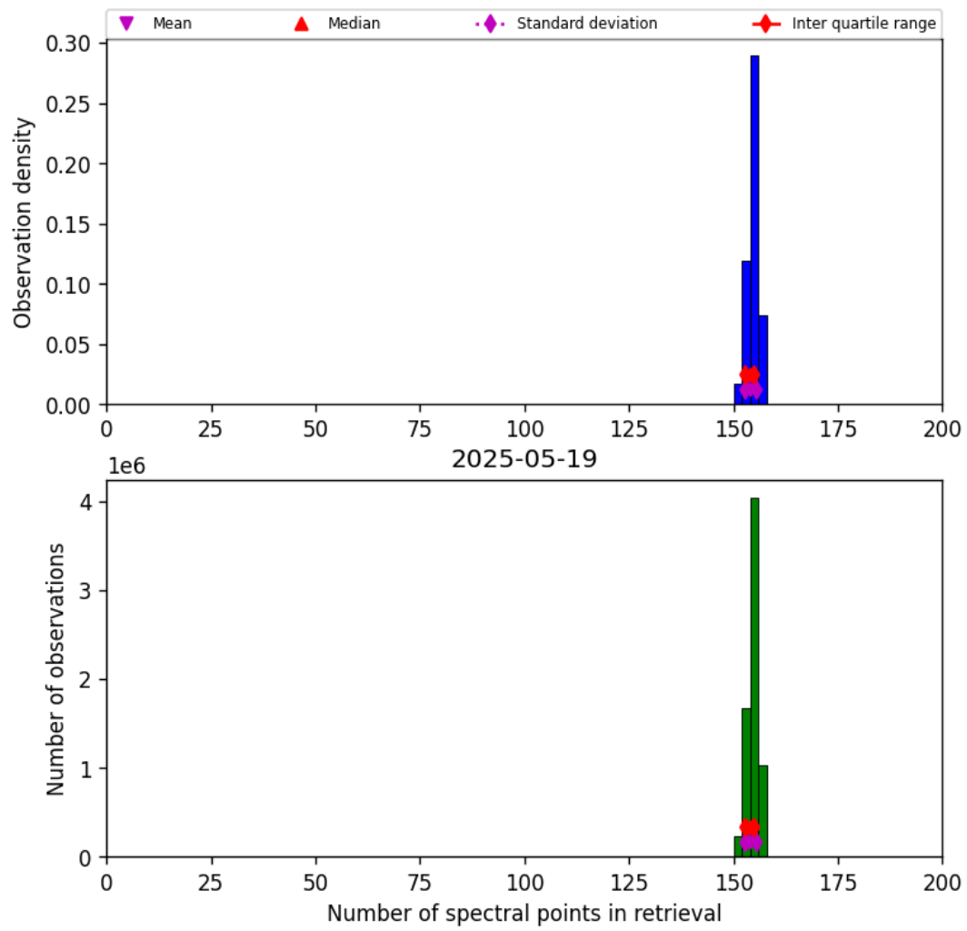
Figure 16: Histogram of “Number of spectral points in retrieval” for 2025-05-19 to 2025-05-19
