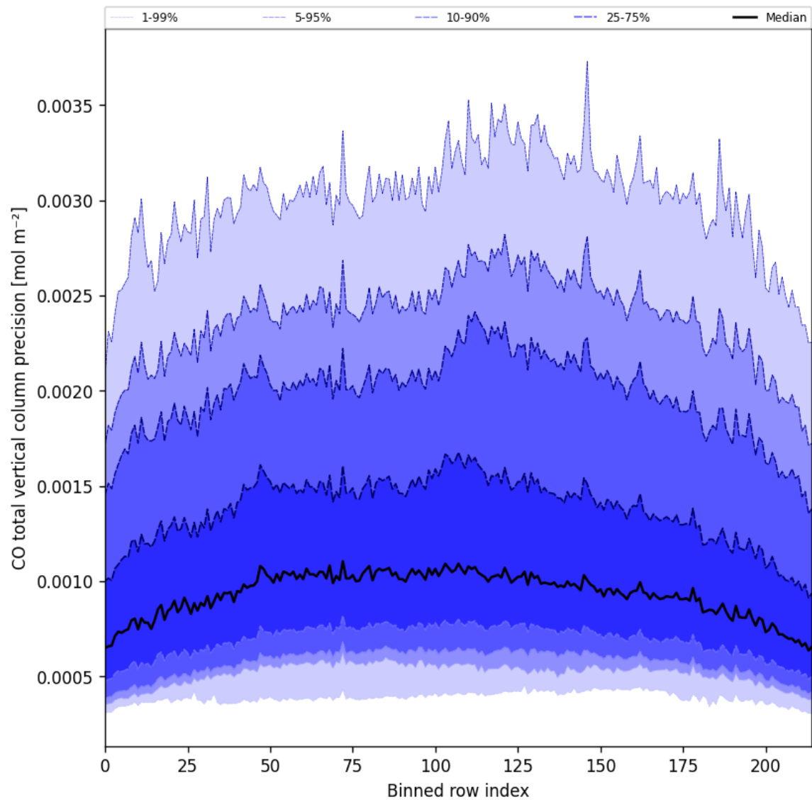
Figure 22: Along track statistics of “CO total vertical column precision” for 2025-05-19 to 2025-05-19
