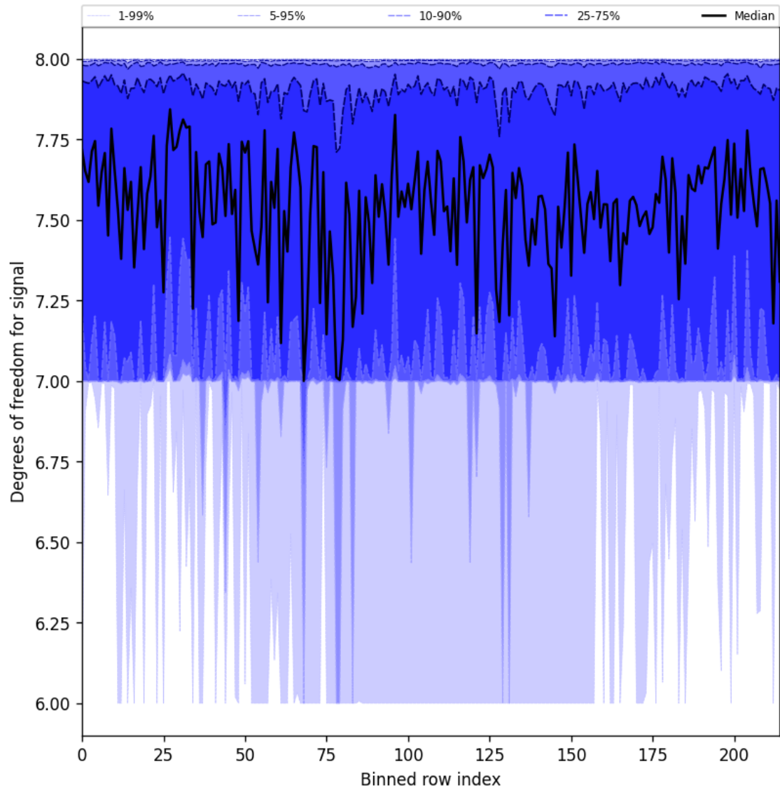
Figure 25: Along track statistics of “Degrees of freedom for signal” for 2025-05-19 to 2025-05-19
