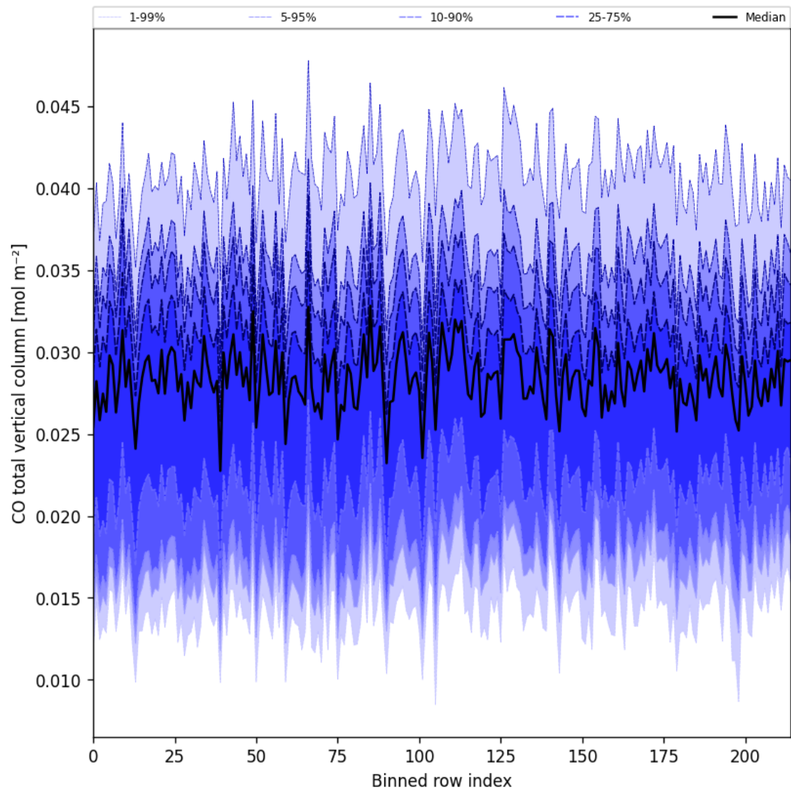
Figure 21: Along track statistics of “CO total vertical column” for 2025-05-19 to 2025-05-19
