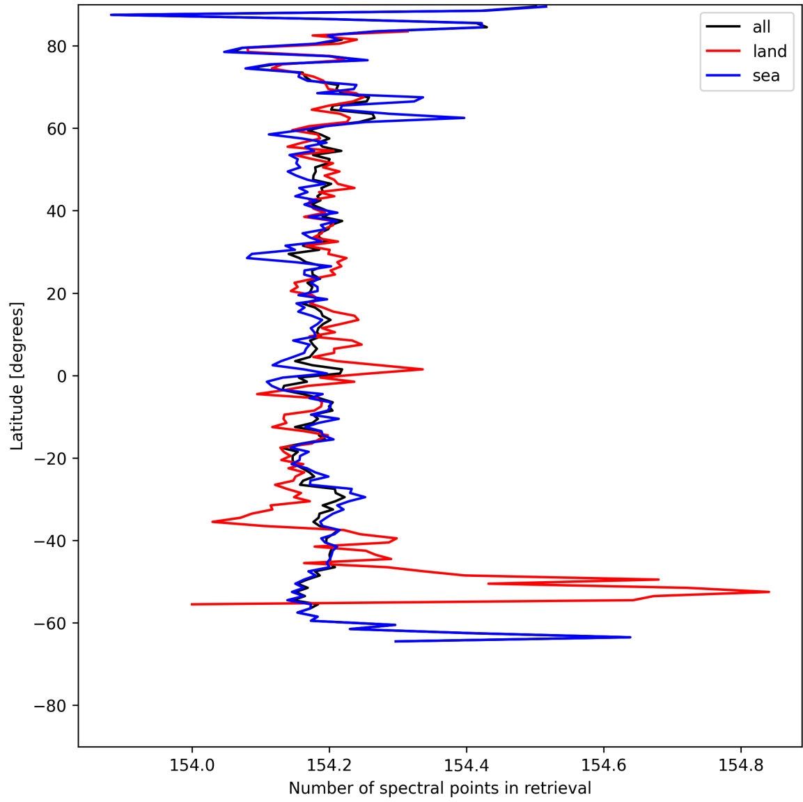
Figure 9: Zonal average of “Number of spectral points in retrieval” for 2025-05-19 to 2025-05-19.
