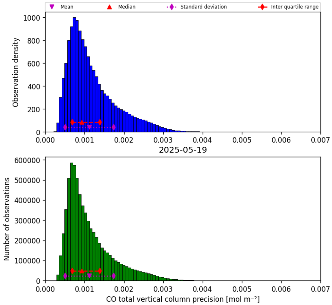
Figure 15: Histogram of “CO total vertical column precision” for 2025-05-19 to 2025-05-19
