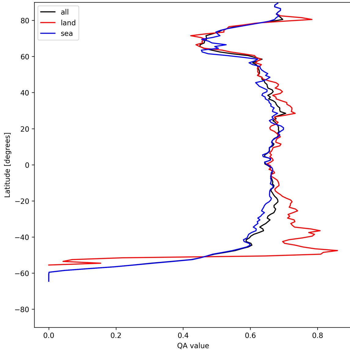
Figure 6: Zonal average of “QA value” for 2025-05-19 to 2025-05-19.
