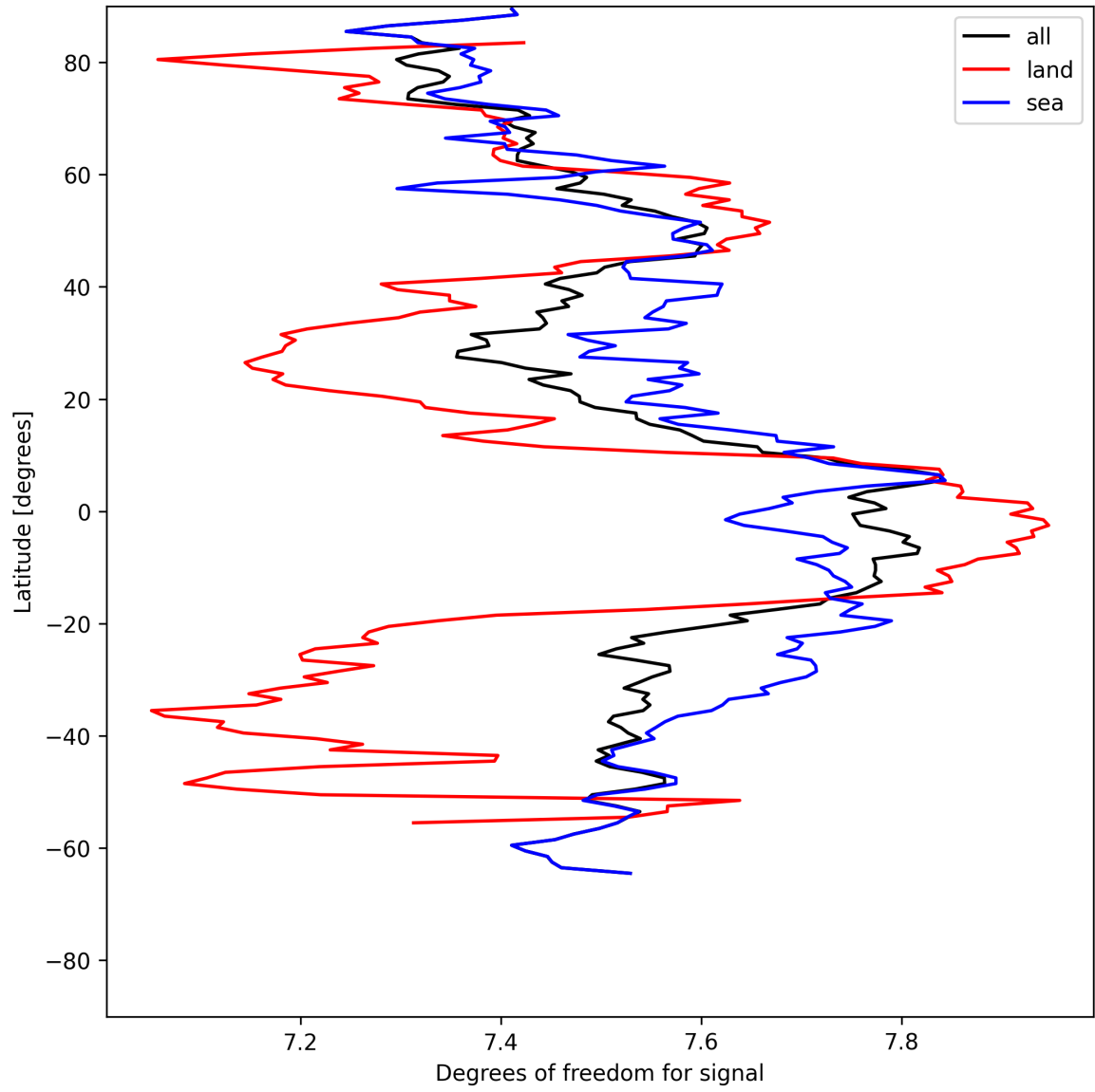
Figure 11: Zonal average of “Degrees of freedom for signal” for 2025-05-19 to 2025-05-19.
