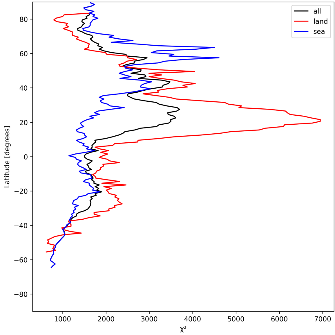
Figure 10: Zonal average of “ \chi^2 ” for 2025-05-19 to 2025-05-19.
