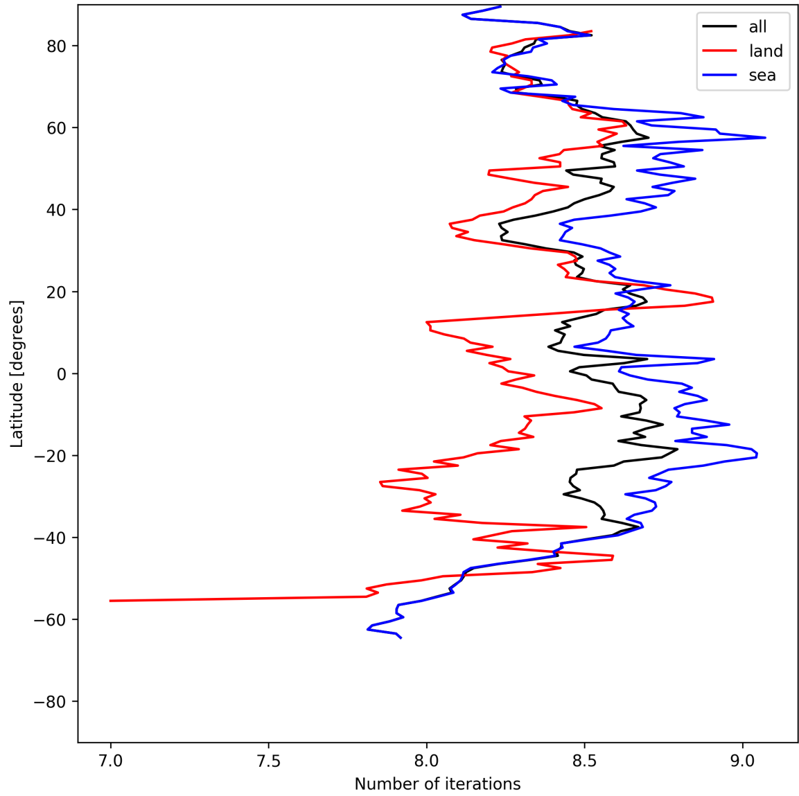
Figure 12: Zonal average of “Number of iterations” for 2025-05-19 to 2025-05-19.
