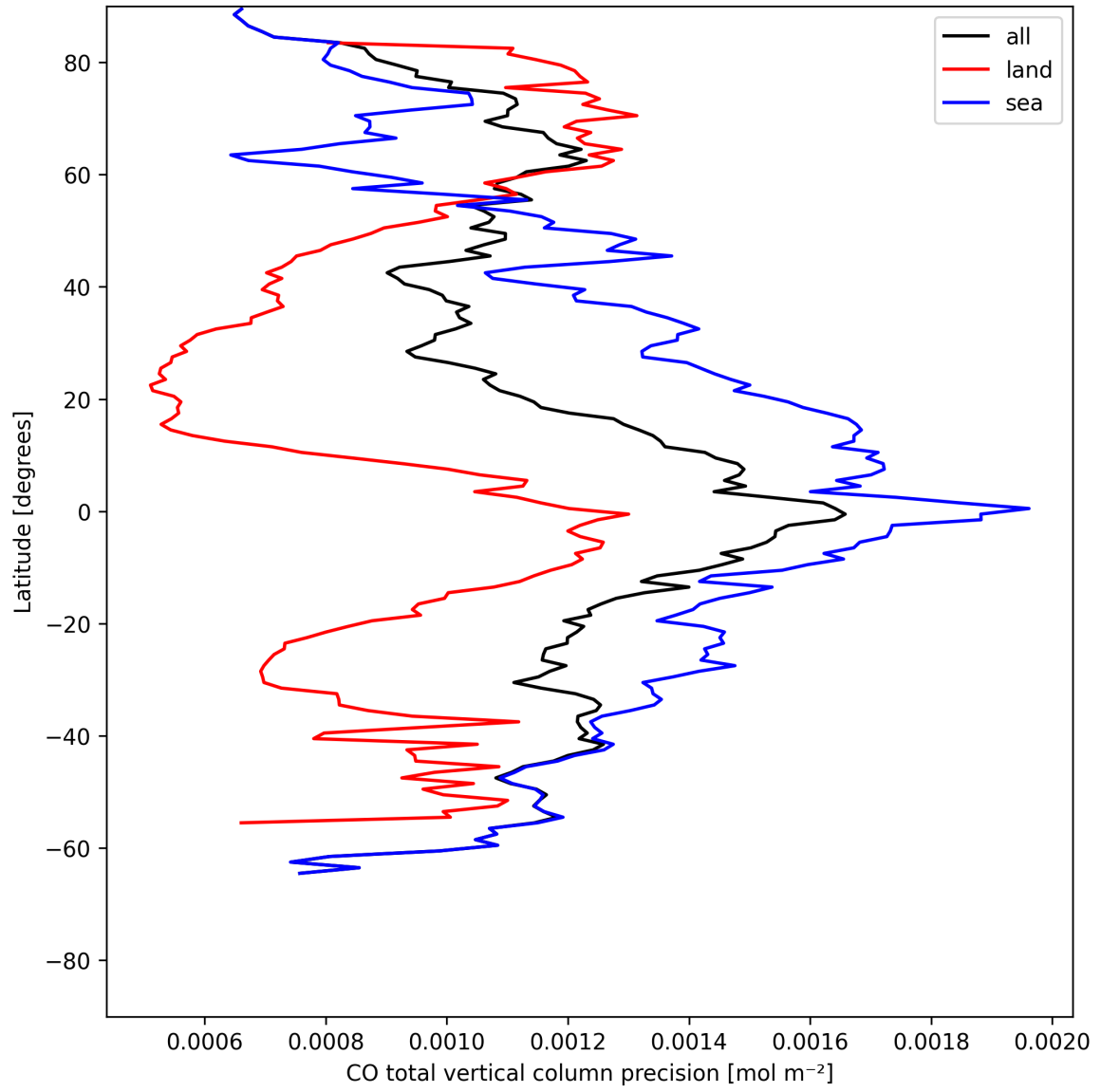
Figure 8: Zonal average of “CO total vertical column precision” for 2025-05-19 to 2025-05-19.
