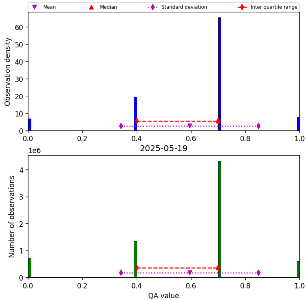
Figure 13: Histogram of “QA value” for 2025-05-19 to 2025-05-19
