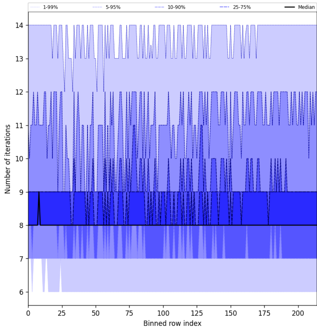
Figure 26: Along track statistics of “Number of iterations” for 2025-05-19 to 2025-05-19
