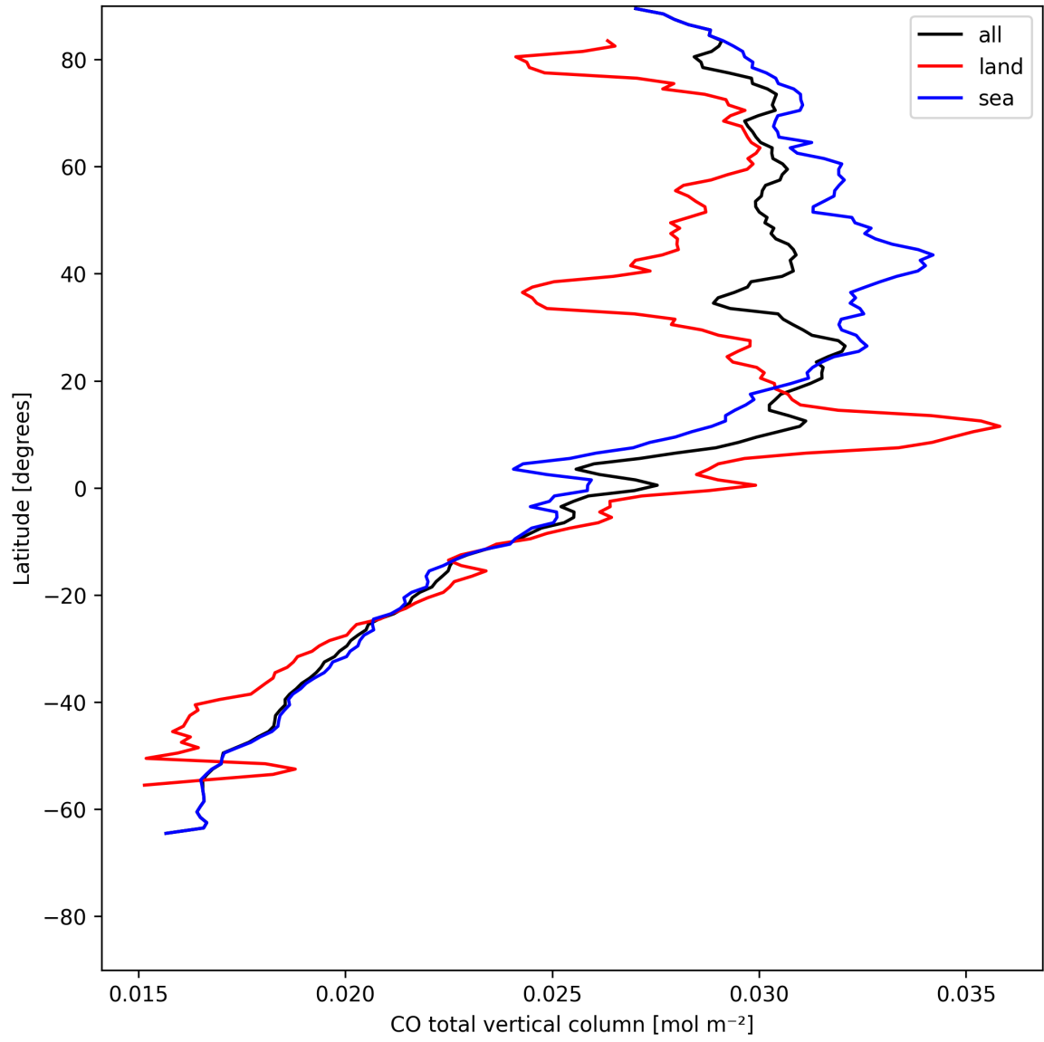
Figure 7: Zonal average of “CO total vertical column” for 2025-05-19 to 2025-05-19.
