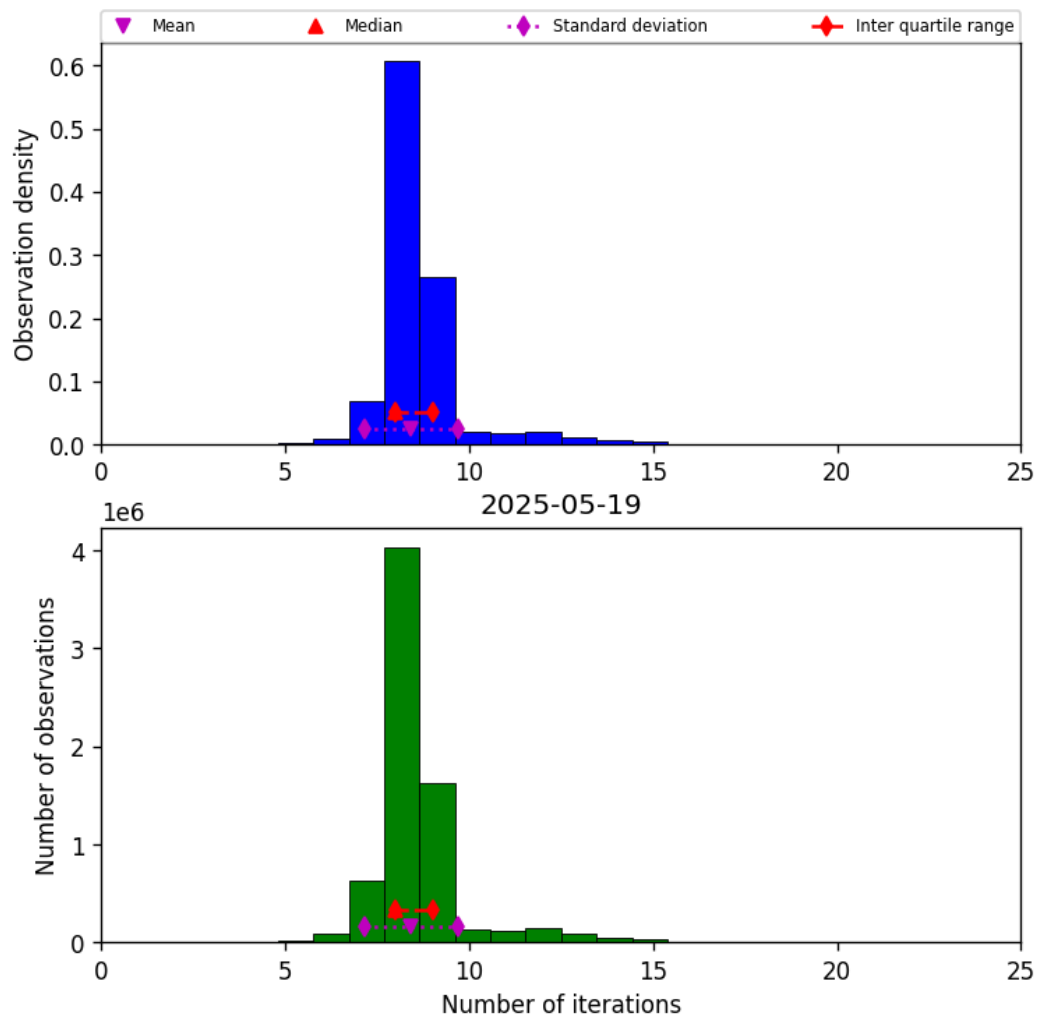
Figure 19: Histogram of “Number of iterations” for 2025-05-19 to 2025-05-19
