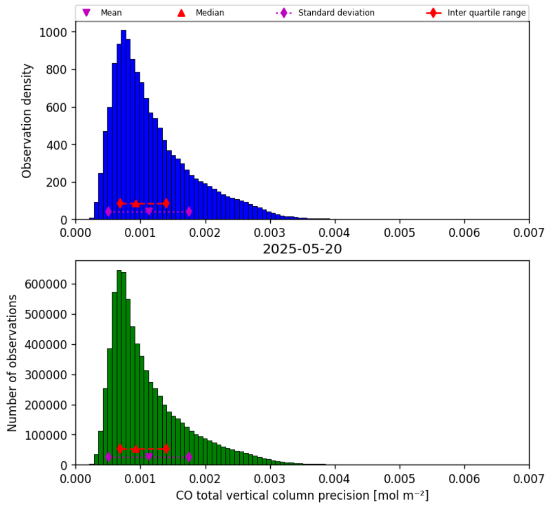
Figure 15: Histogram of “CO total vertical column precision” for 2025-05-20 to 2025-05-21
