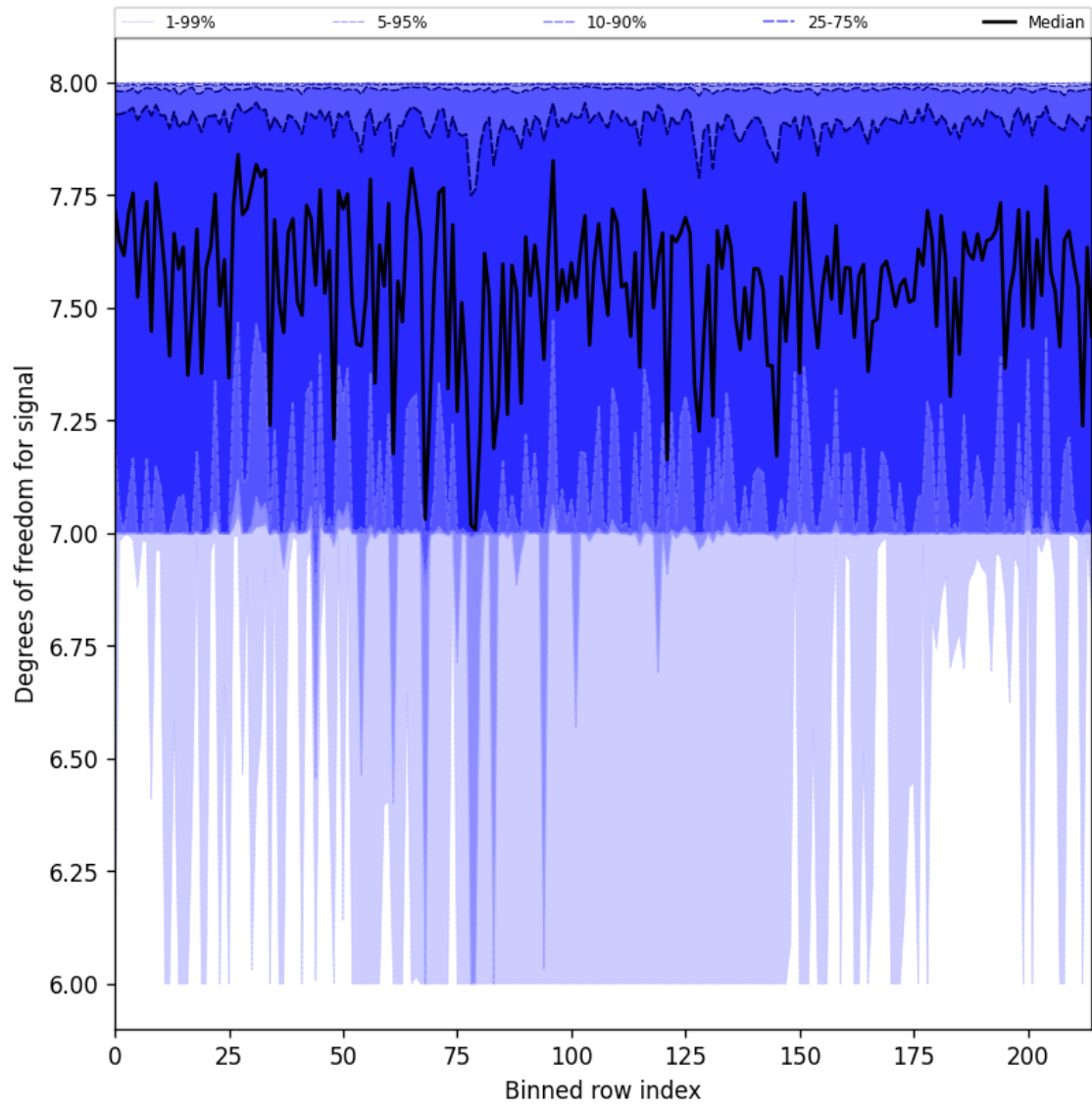
Figure 25: Along track statistics of “Degrees of freedom for signal” for 2025-05-20 to 2025-05-21
