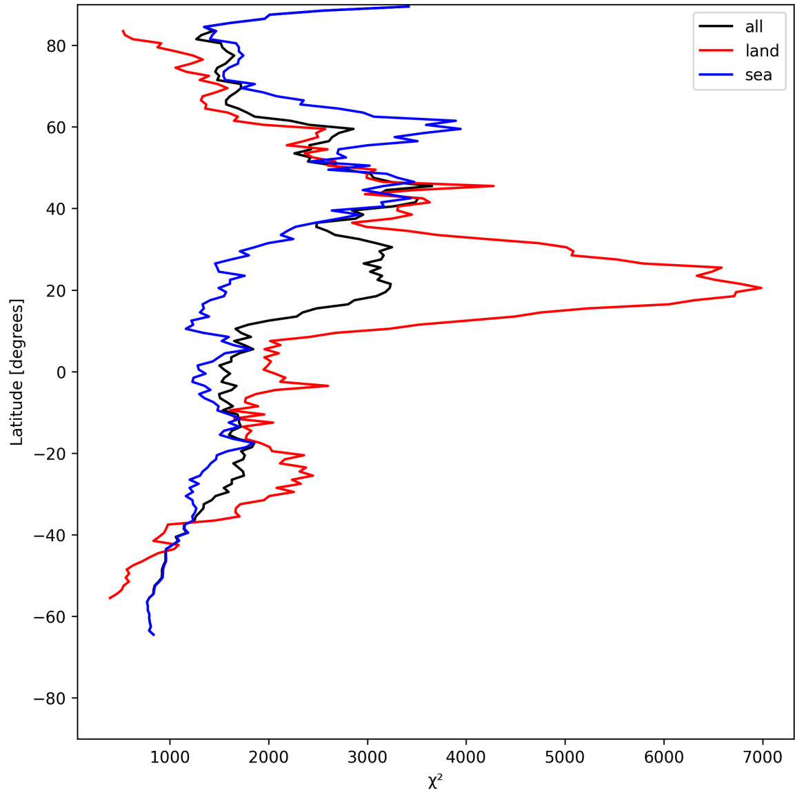
Figure 10: Zonal average of “ \chi^2 ” for 2025-05-20 to 2025-05-21.
