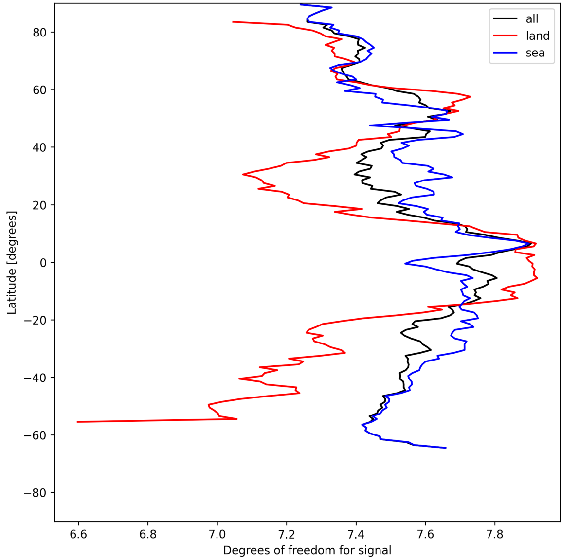
Figure 11: Zonal average of “Degrees of freedom for signal” for 2025-05-20 to 2025-05-21.
