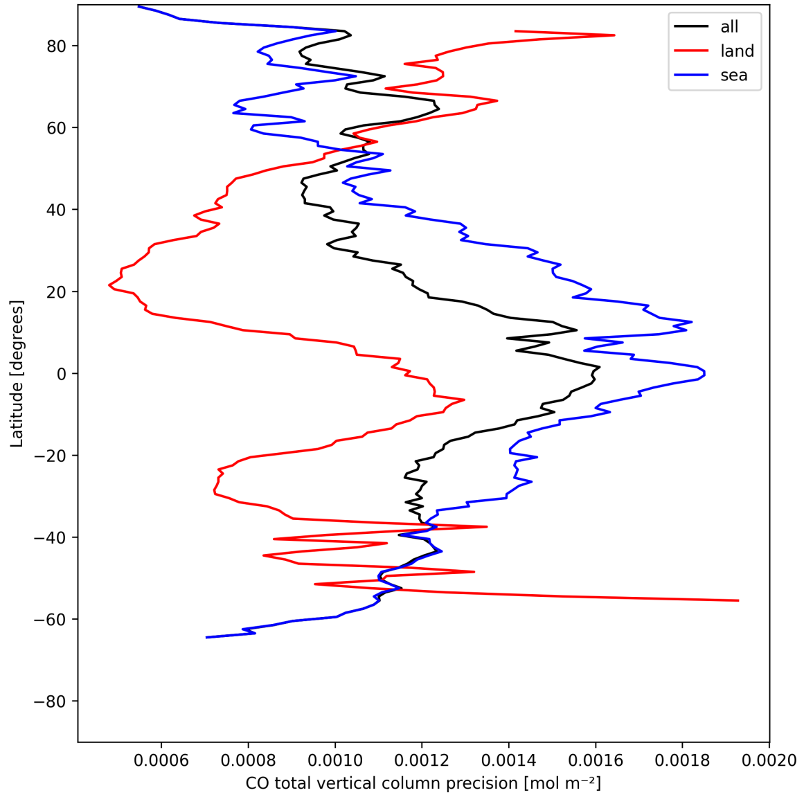
Figure 8: Zonal average of “CO total vertical column precision” for 2025-05-20 to 2025-05-21.
