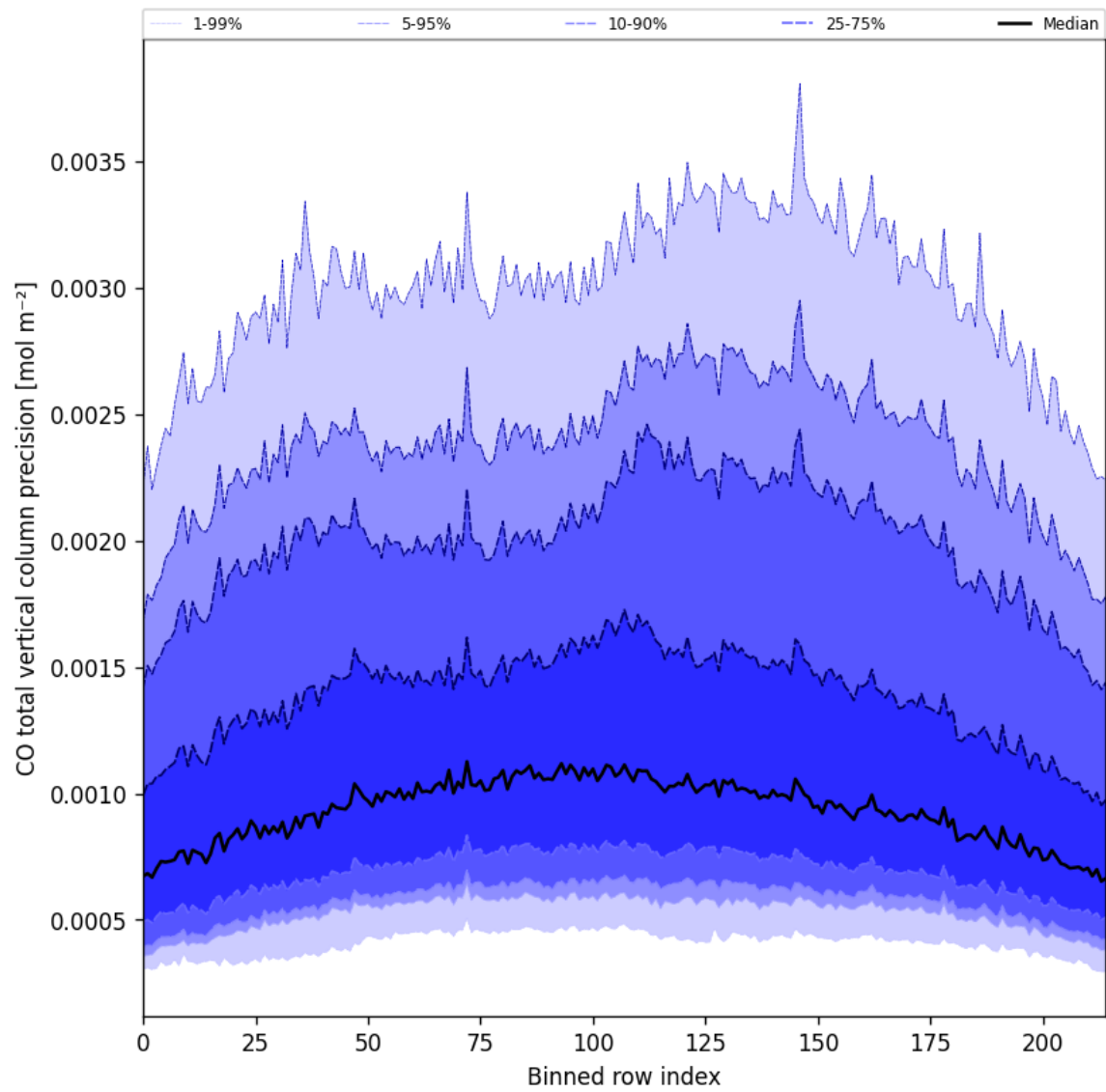
Figure 22: Along track statistics of “CO total vertical column precision” for 2025-05-20 to 2025-05-21
