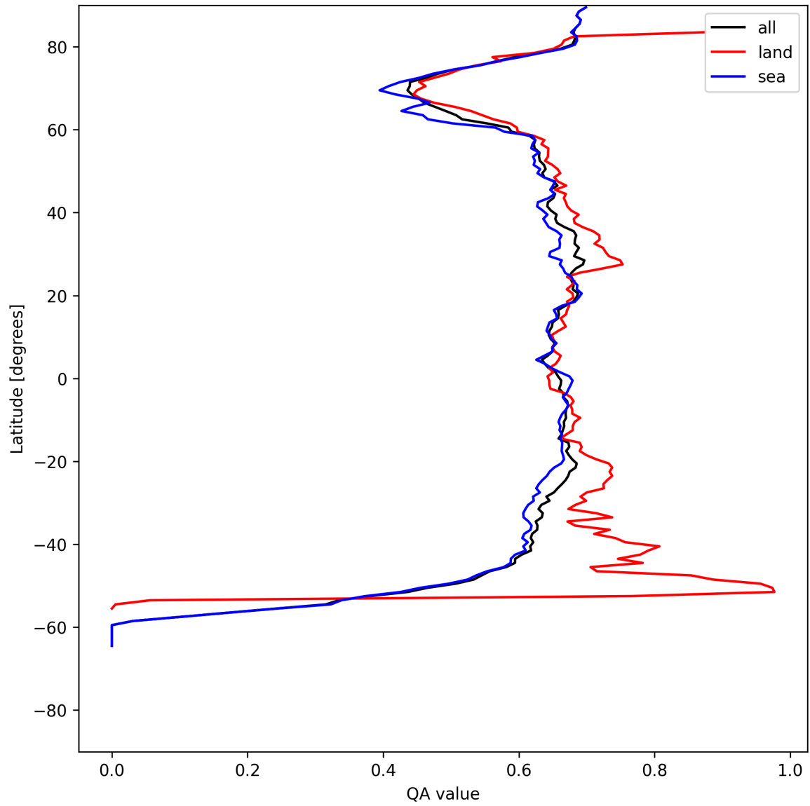
Figure 6: Zonal average of “QA value” for 2025-05-20 to 2025-05-21.
