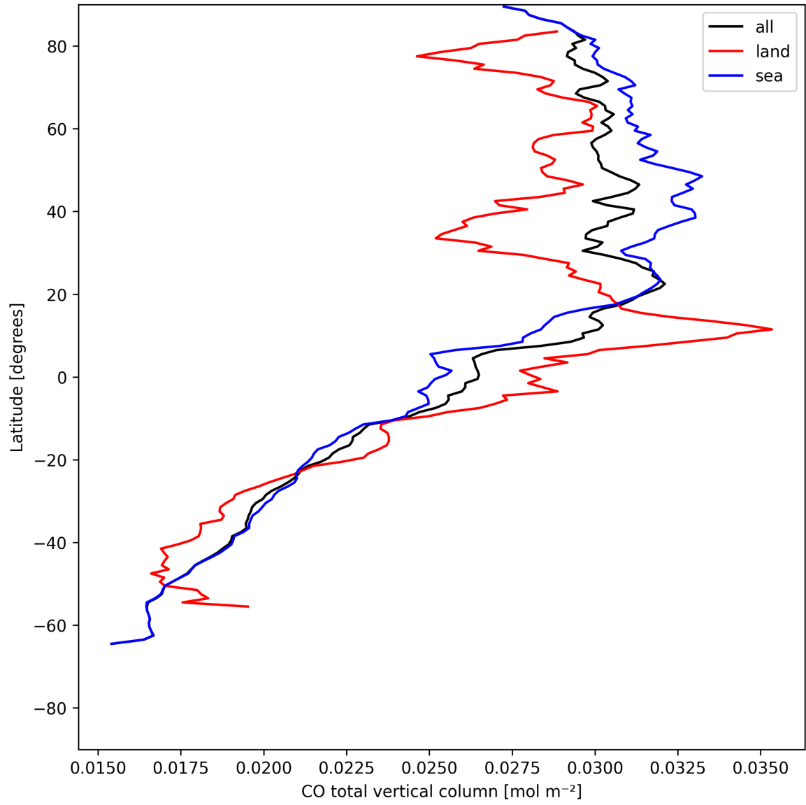
Figure 7: Zonal average of “CO total vertical column” for 2025-05-20 to 2025-05-21.
