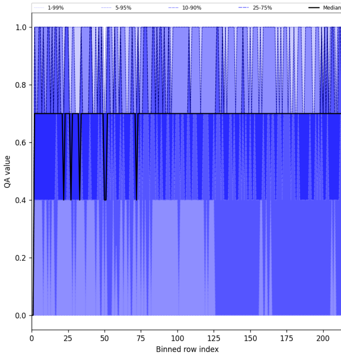
Figure 20: Along track statistics of “QA value” for 2025-05-20 to 2025-05-21
