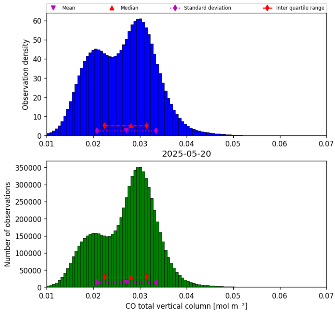
Figure 14: Histogram of “CO total vertical column” for 2025-05-20 to 2025-05-21
