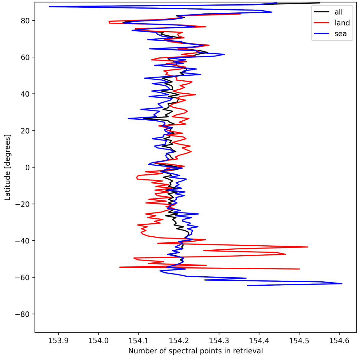
Figure 9: Zonal average of “Number of spectral points in retrieval” for 2025-05-20 to 2025-05-21.
