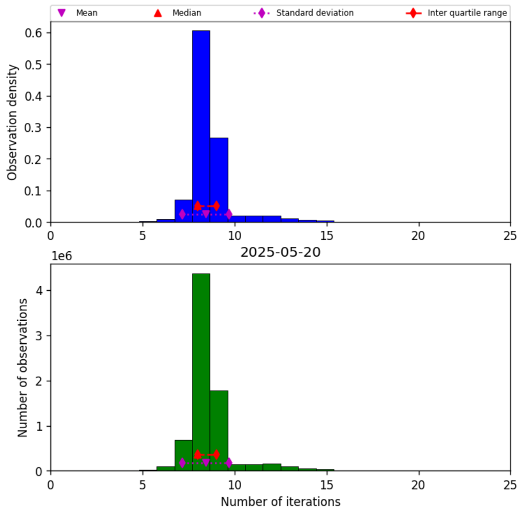
Figure 19: Histogram of “Number of iterations” for 2025-05-20 to 2025-05-21
