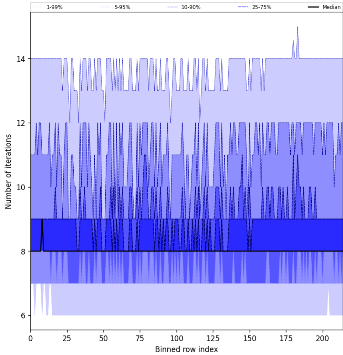
Figure 26: Along track statistics of “Number of iterations” for 2025-05-20 to 2025-05-21
