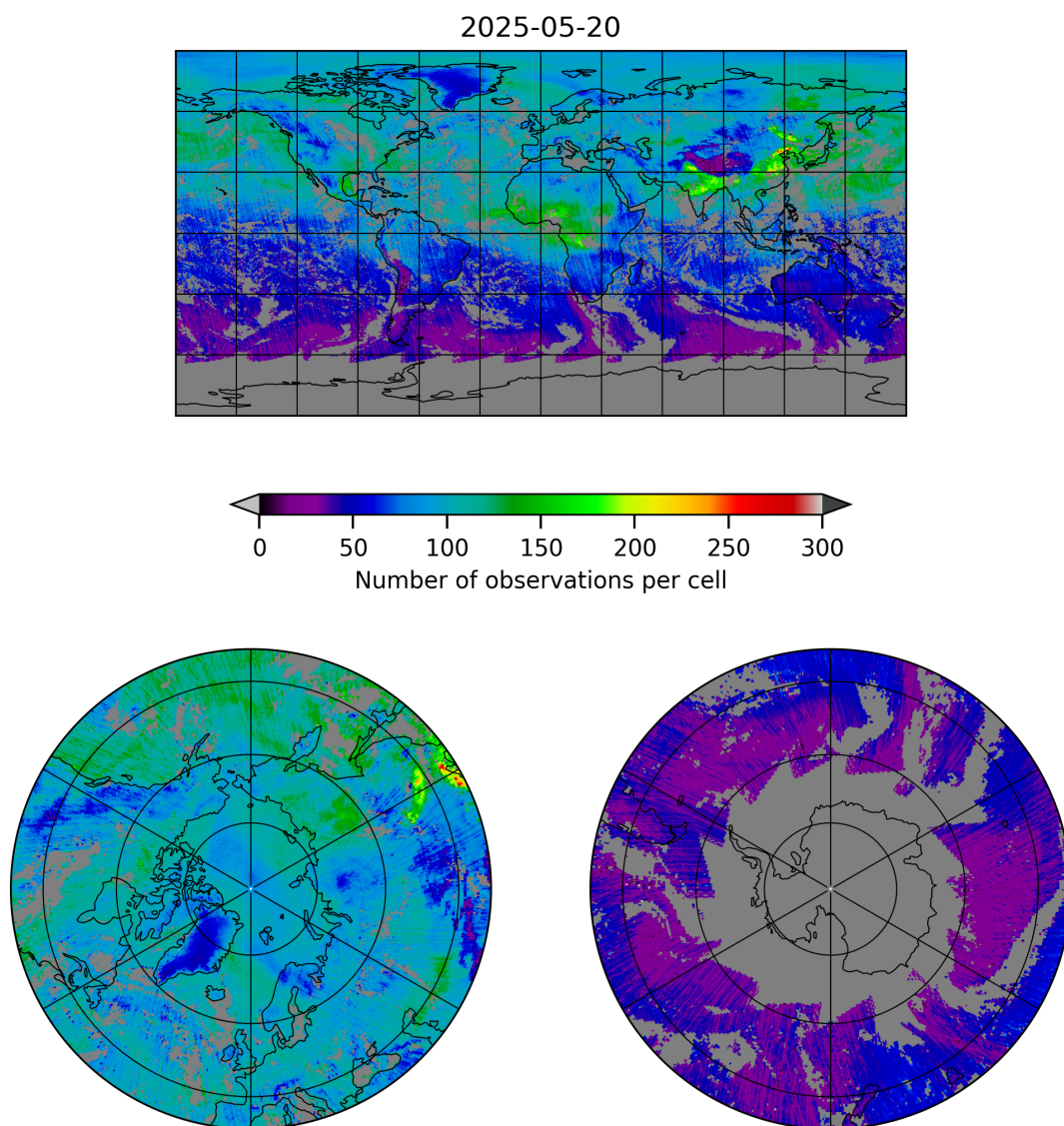
Figure 5: Map of the number of observations for 2025-05-20 to 2025-05-21
