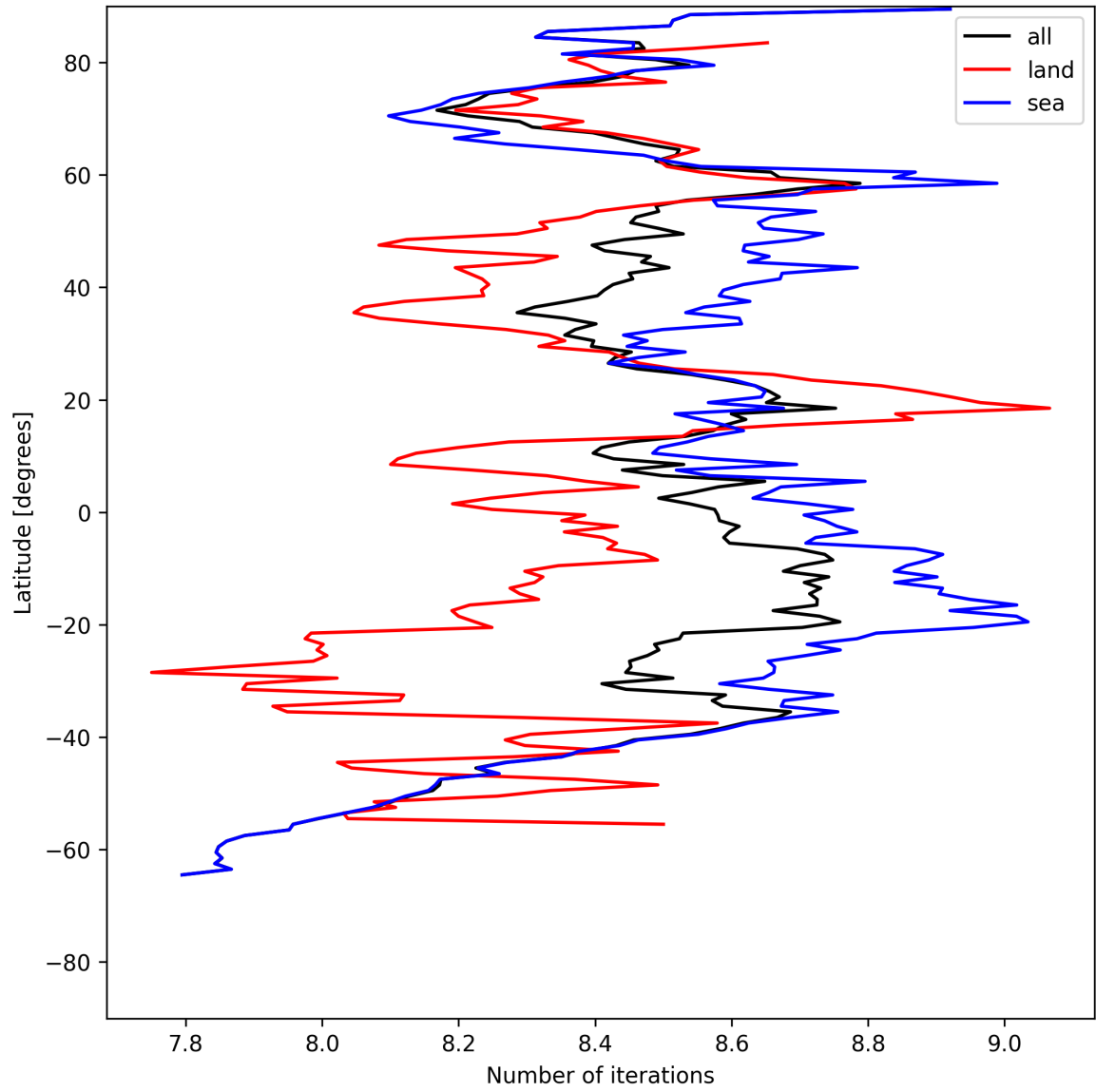
Figure 12: Zonal average of “Number of iterations” for 2025-05-20 to 2025-05-21.
