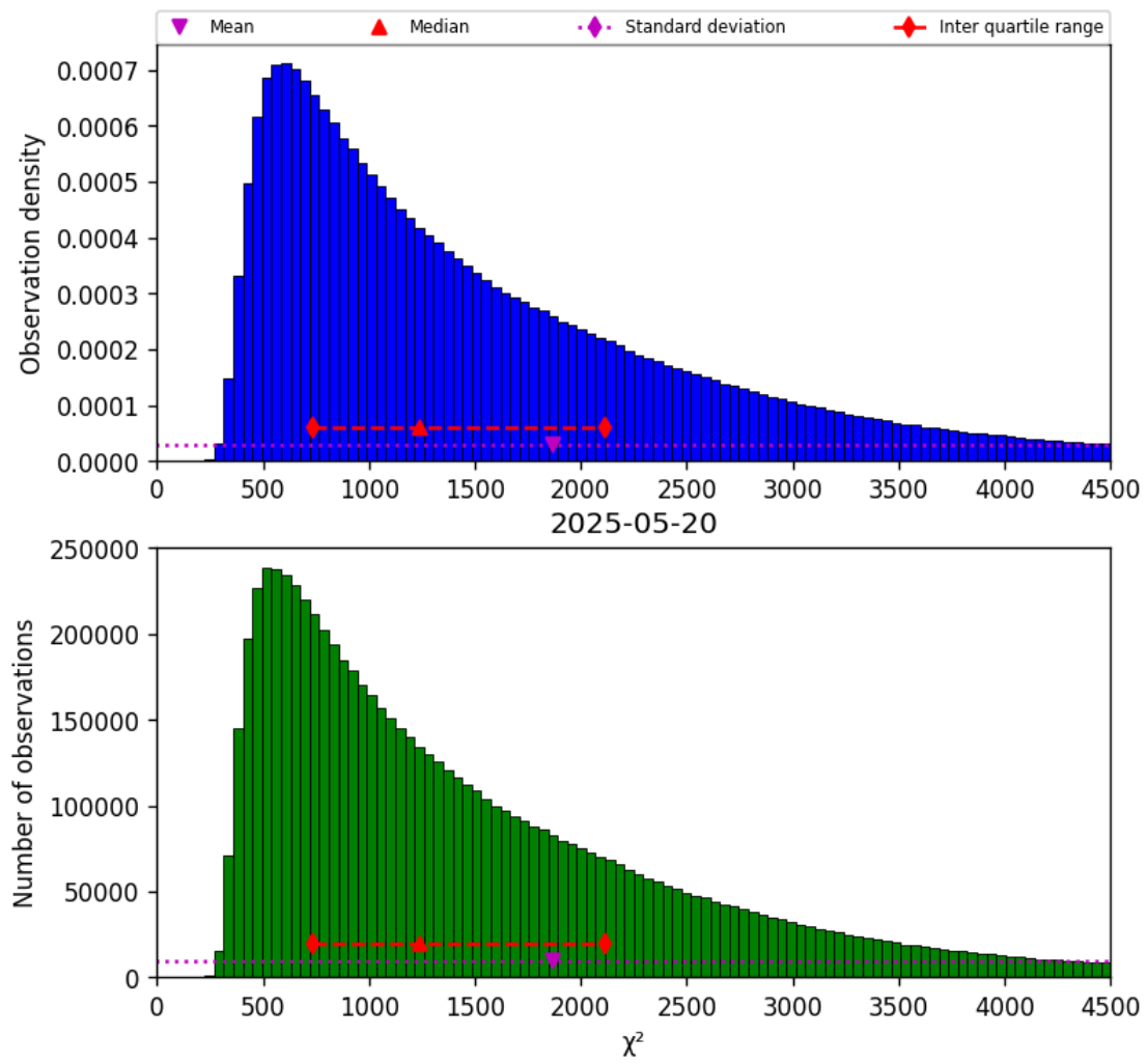
Figure 17: Histogram of “ \chi^2 ” for 2025-05-20 to 2025-05-21
