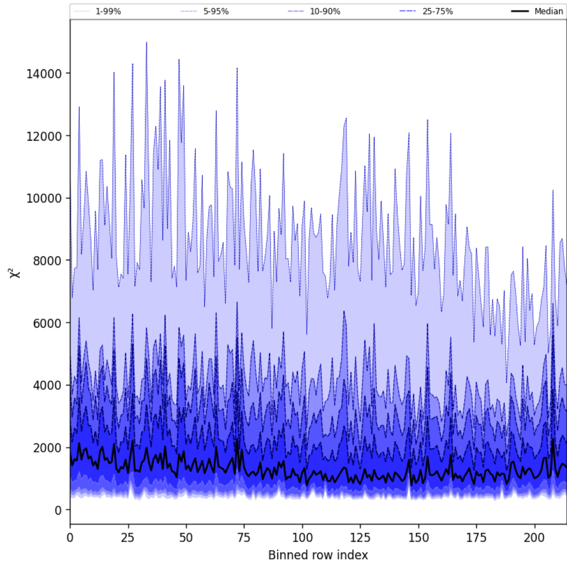
Figure 24: Along track statistics of “ \chi^2 ” for 2025-05-20 to 2025-05-21
