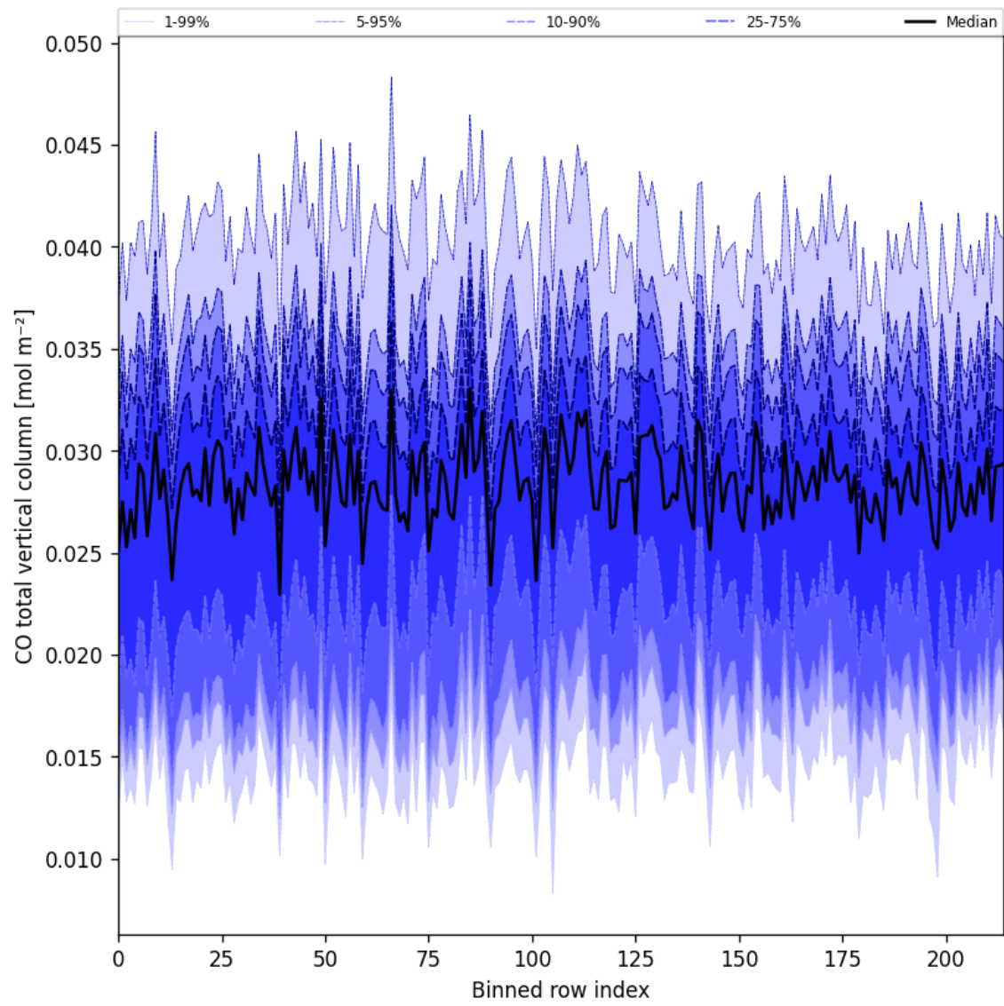
Figure 21: Along track statistics of “CO total vertical column” for 2025-05-20 to 2025-05-21
