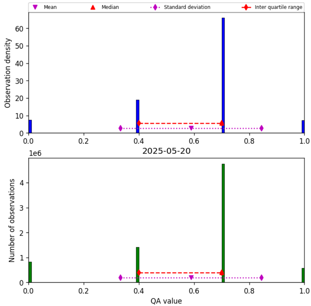
Figure 13: Histogram of “QA value” for 2025-05-20 to 2025-05-21
