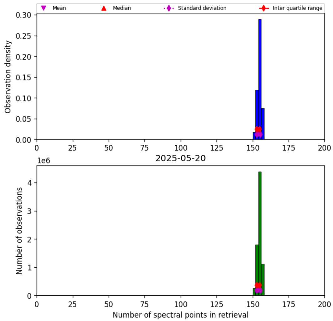
Figure 16: Histogram of “Number of spectral points in retrieval” for 2025-05-20 to 2025-05-21
