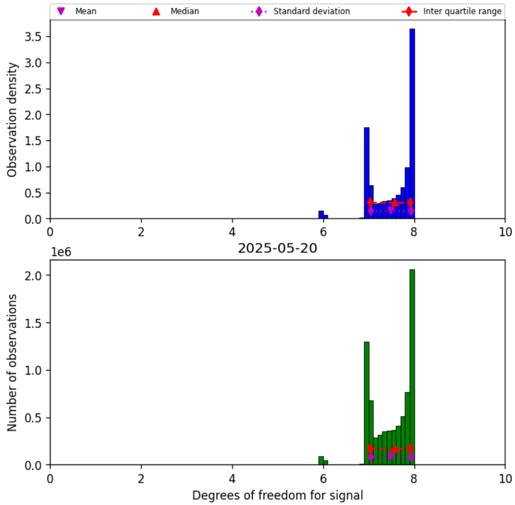
Figure 18: Histogram of “Degrees of freedom for signal” for 2025-05-20 to 2025-05-21
