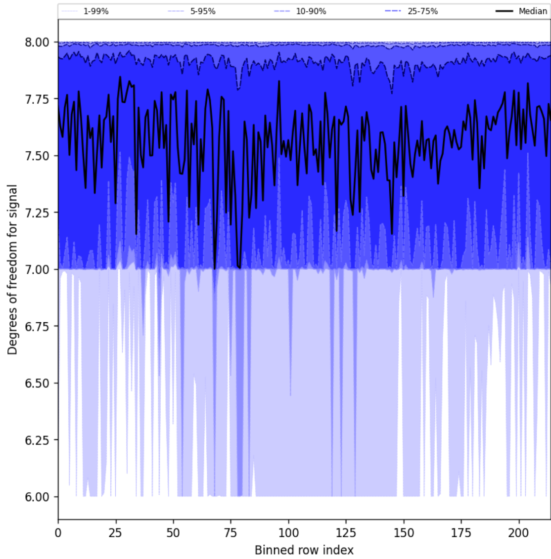
Figure 25: Along track statistics of “Degrees of freedom for signal” for 2025-05-21 to 2025-05-22
