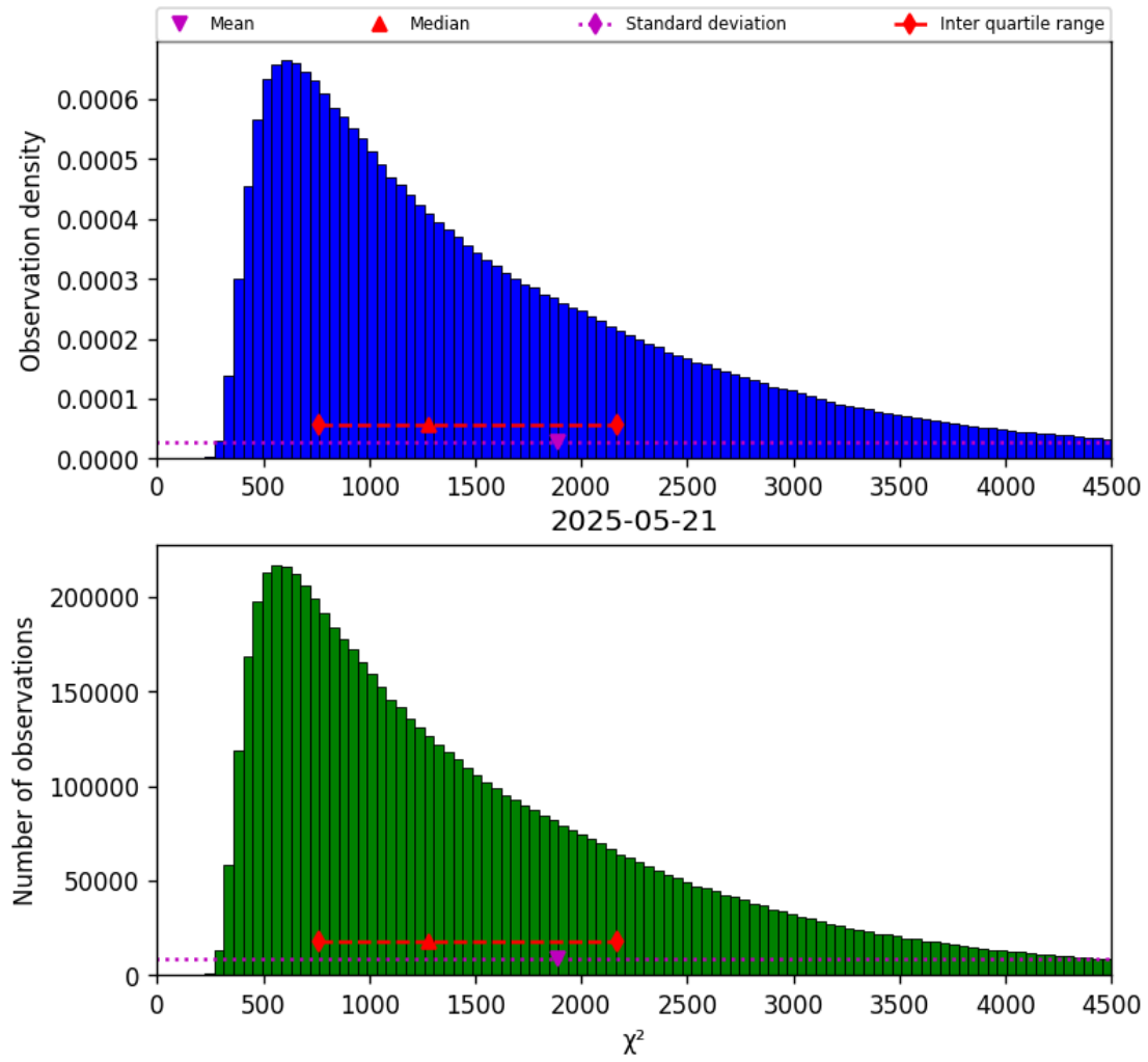
Figure 17: Histogram of “ \chi^2 ” for 2025-05-21 to 2025-05-22
