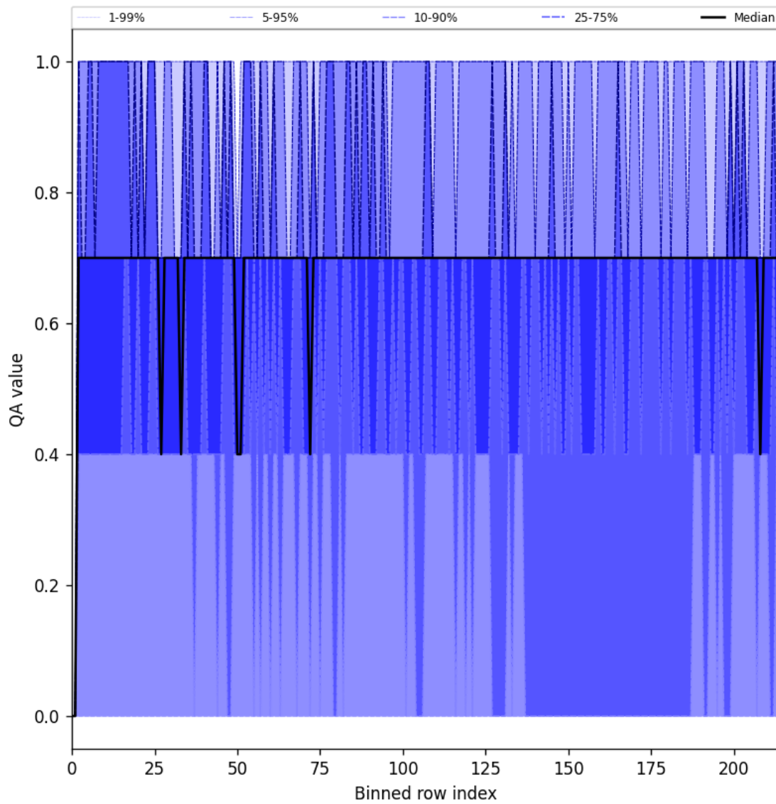
Figure 20: Along track statistics of “QA value” for 2025-05-21 to 2025-05-22
