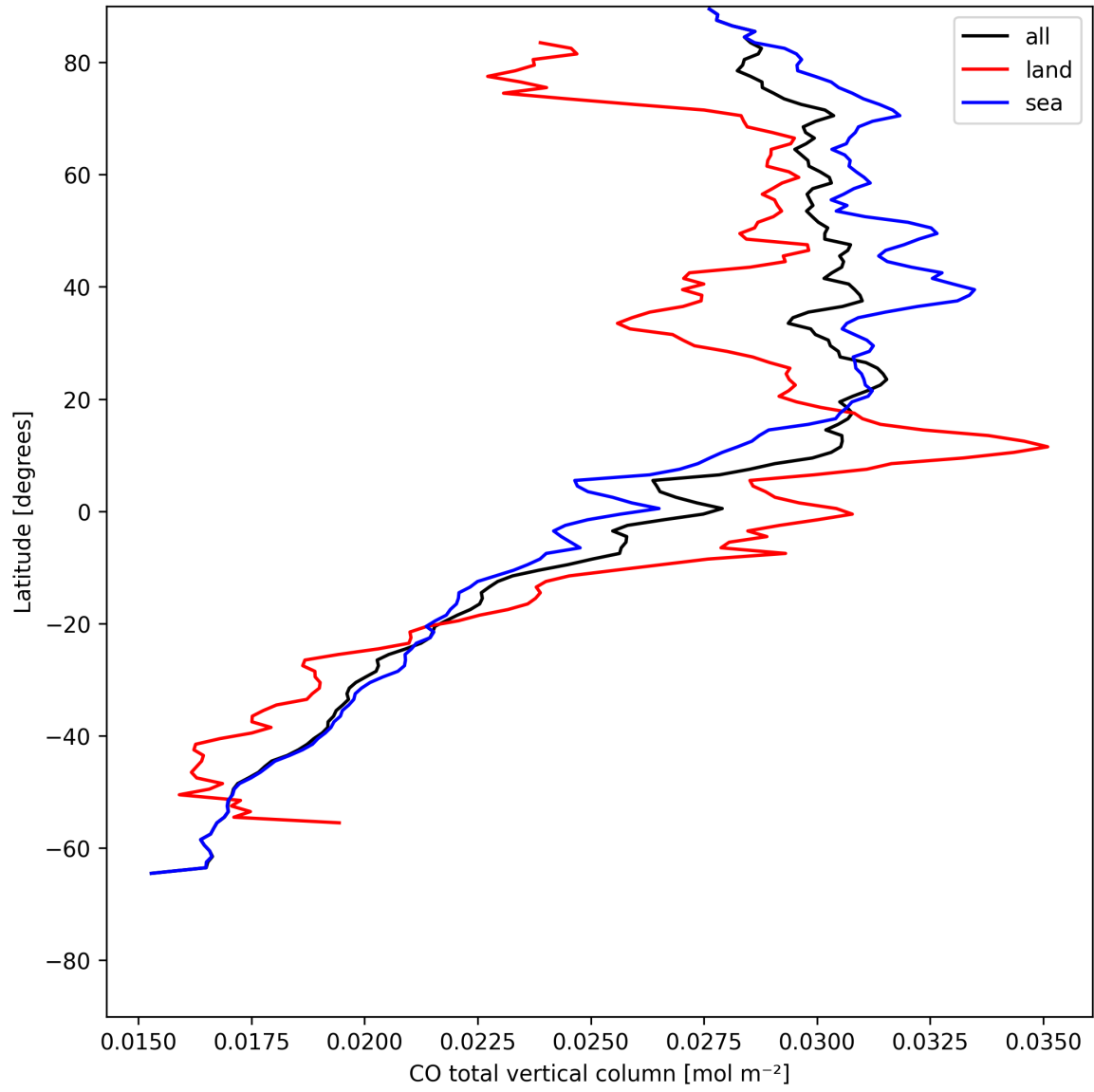
Figure 7: Zonal average of “CO total vertical column” for 2025-05-21 to 2025-05-22.
