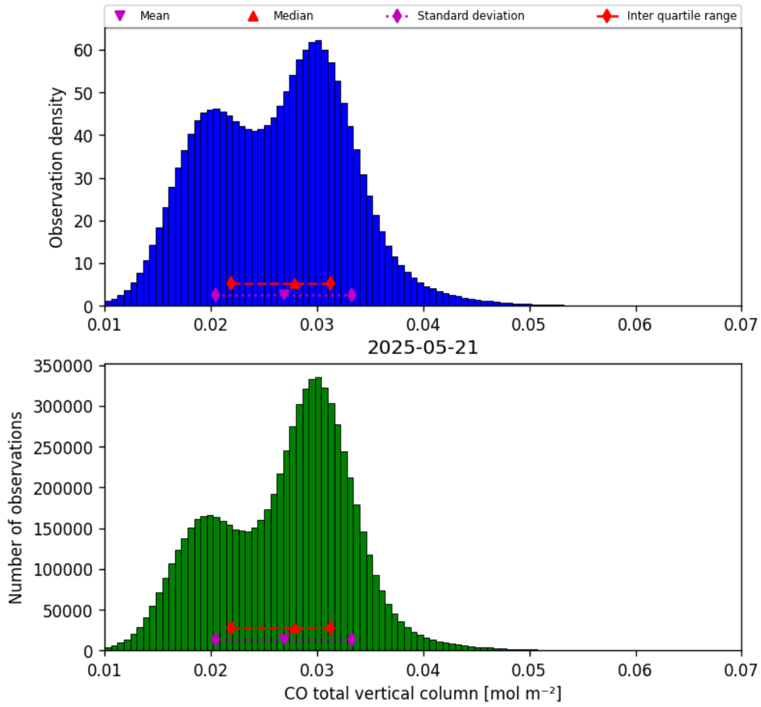
Figure 14: Histogram of “CO total vertical column” for 2025-05-21 to 2025-05-22
