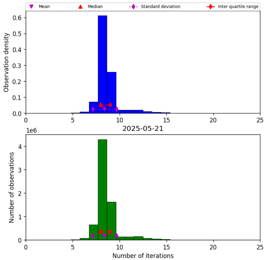
Figure 19: Histogram of “Number of iterations” for 2025-05-21 to 2025-05-22
