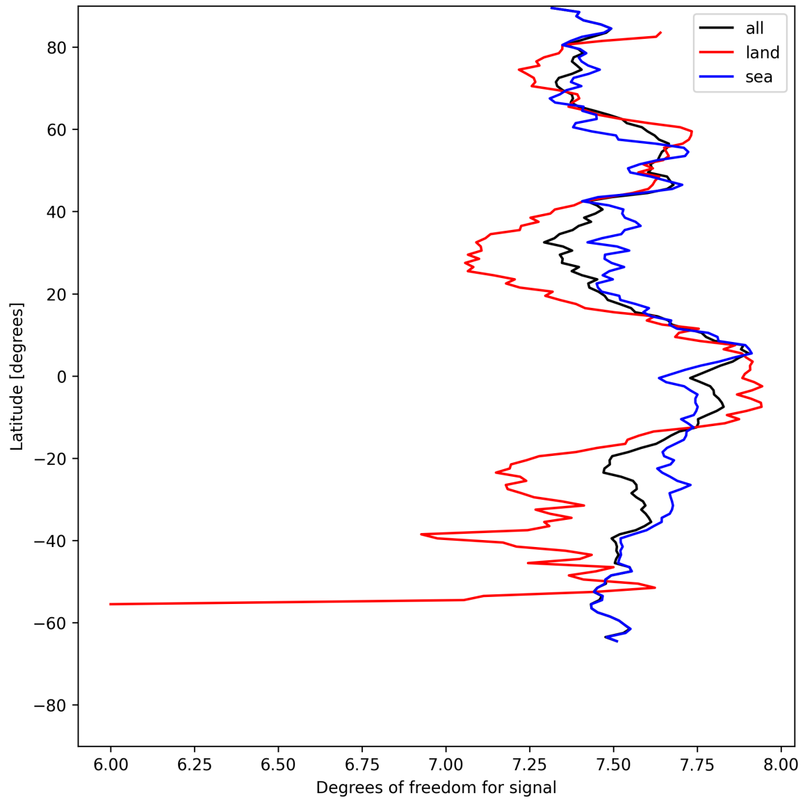
Figure 11: Zonal average of “Degrees of freedom for signal” for 2025-05-21 to 2025-05-22.
