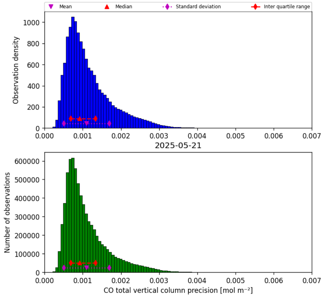
Figure 15: Histogram of “CO total vertical column precision” for 2025-05-21 to 2025-05-22
