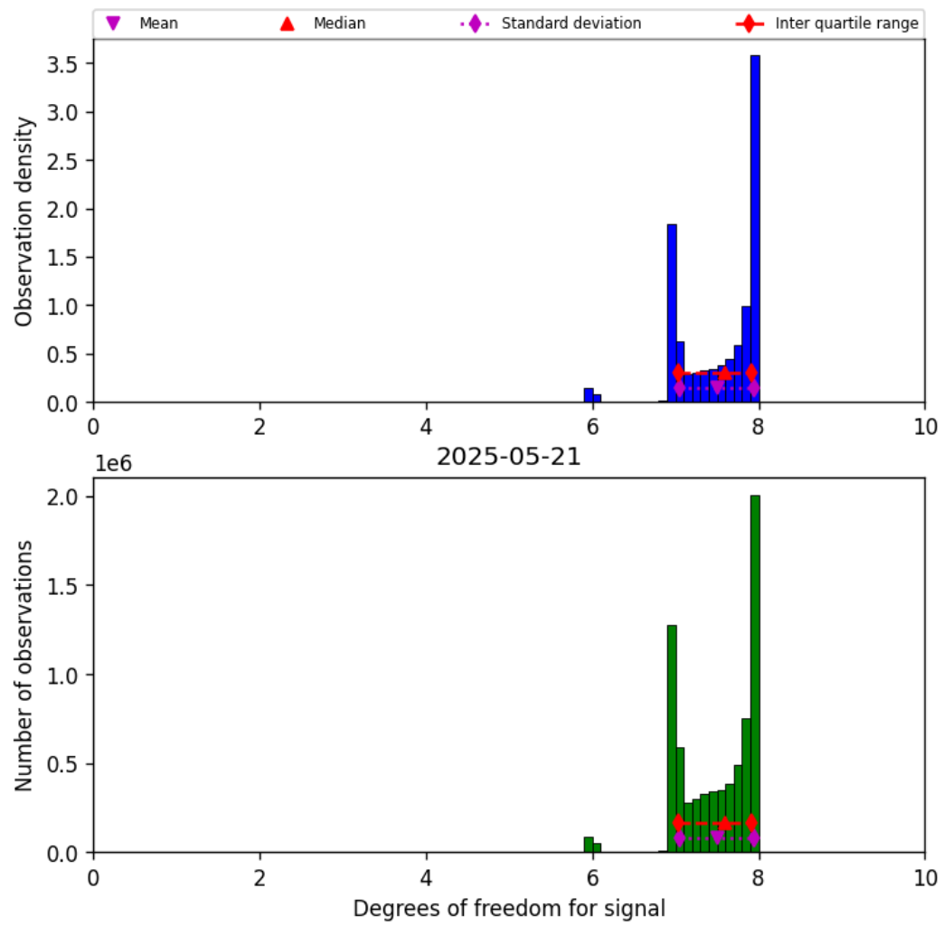
Figure 18: Histogram of “Degrees of freedom for signal” for 2025-05-21 to 2025-05-22
