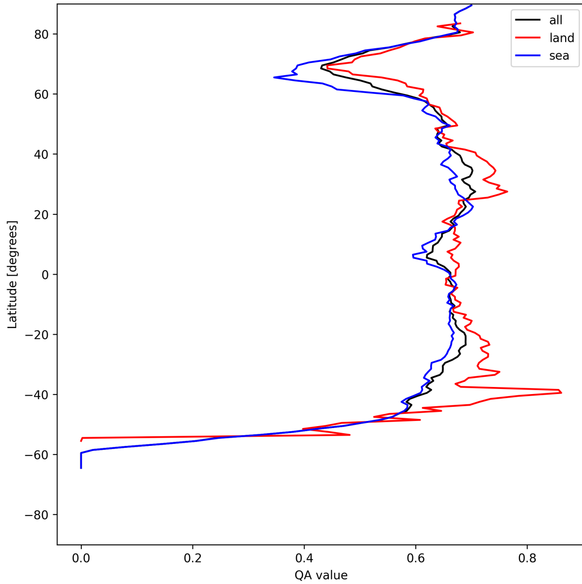
Figure 6: Zonal average of “QA value” for 2025-05-21 to 2025-05-22.
