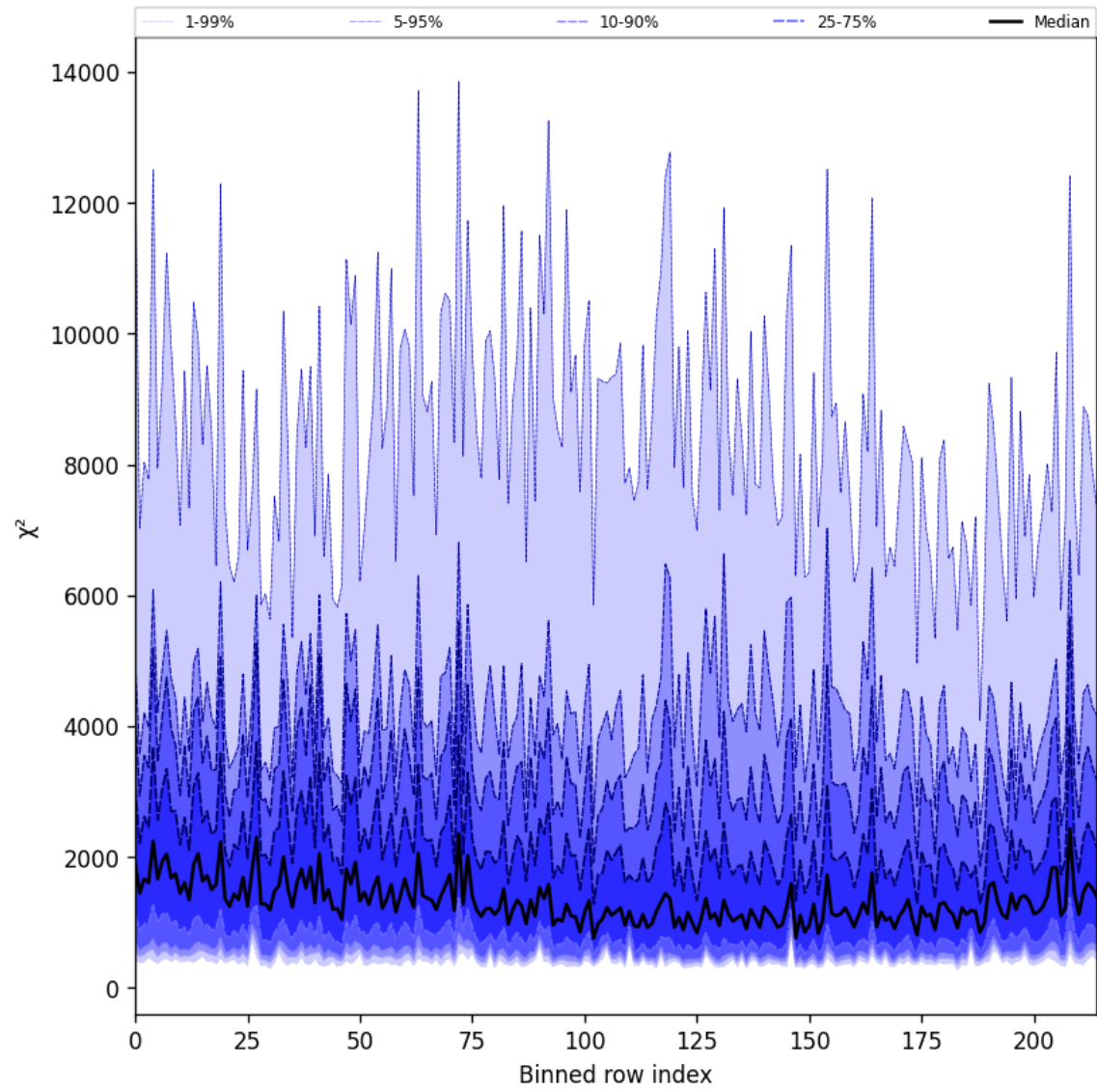
Figure 24: Along track statistics of “ \chi^2 ” for 2025-05-21 to 2025-05-22
