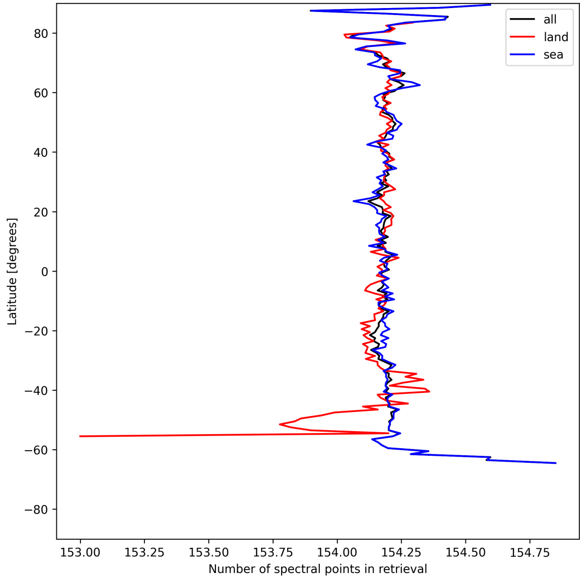
Figure 9: Zonal average of “Number of spectral points in retrieval” for 2025-05-21 to 2025-05-22.
