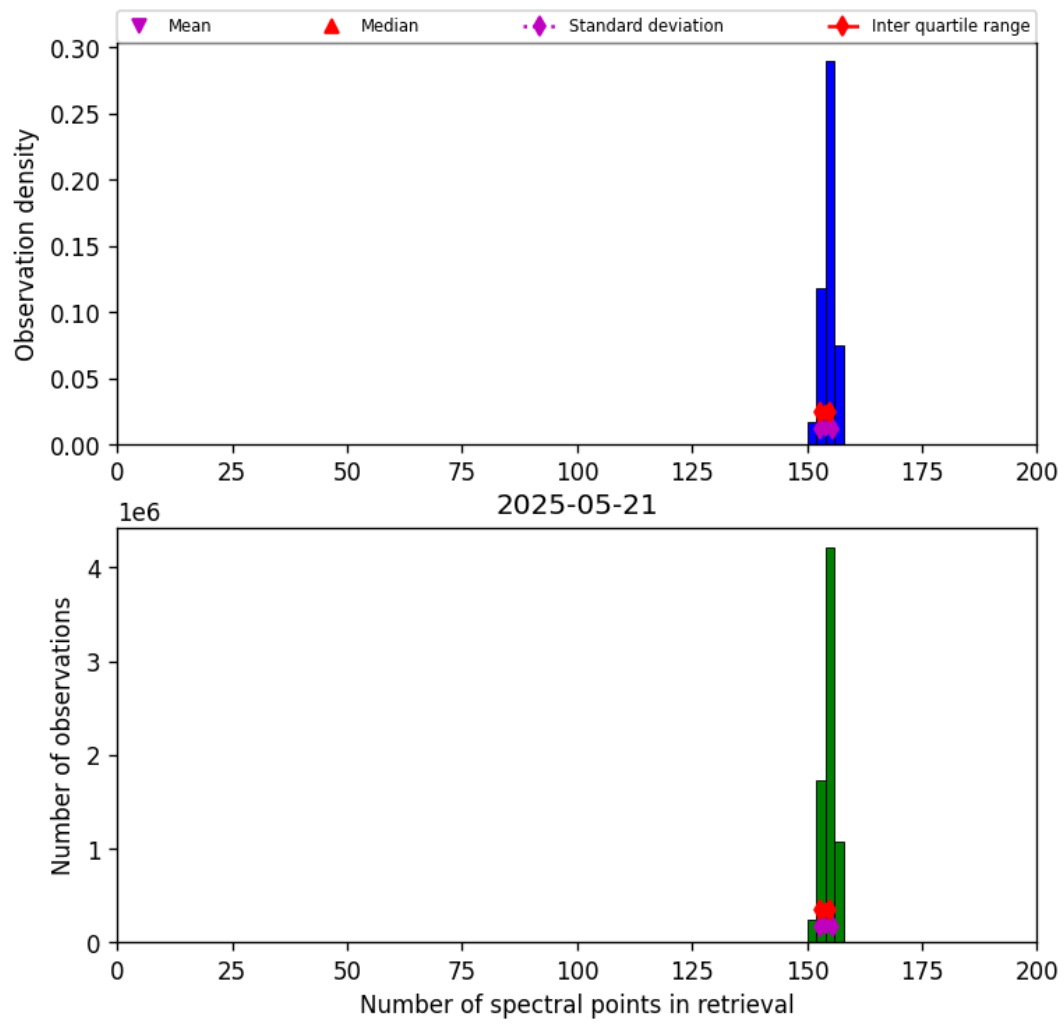
Figure 16: Histogram of “Number of spectral points in retrieval” for 2025-05-21 to 2025-05-22
