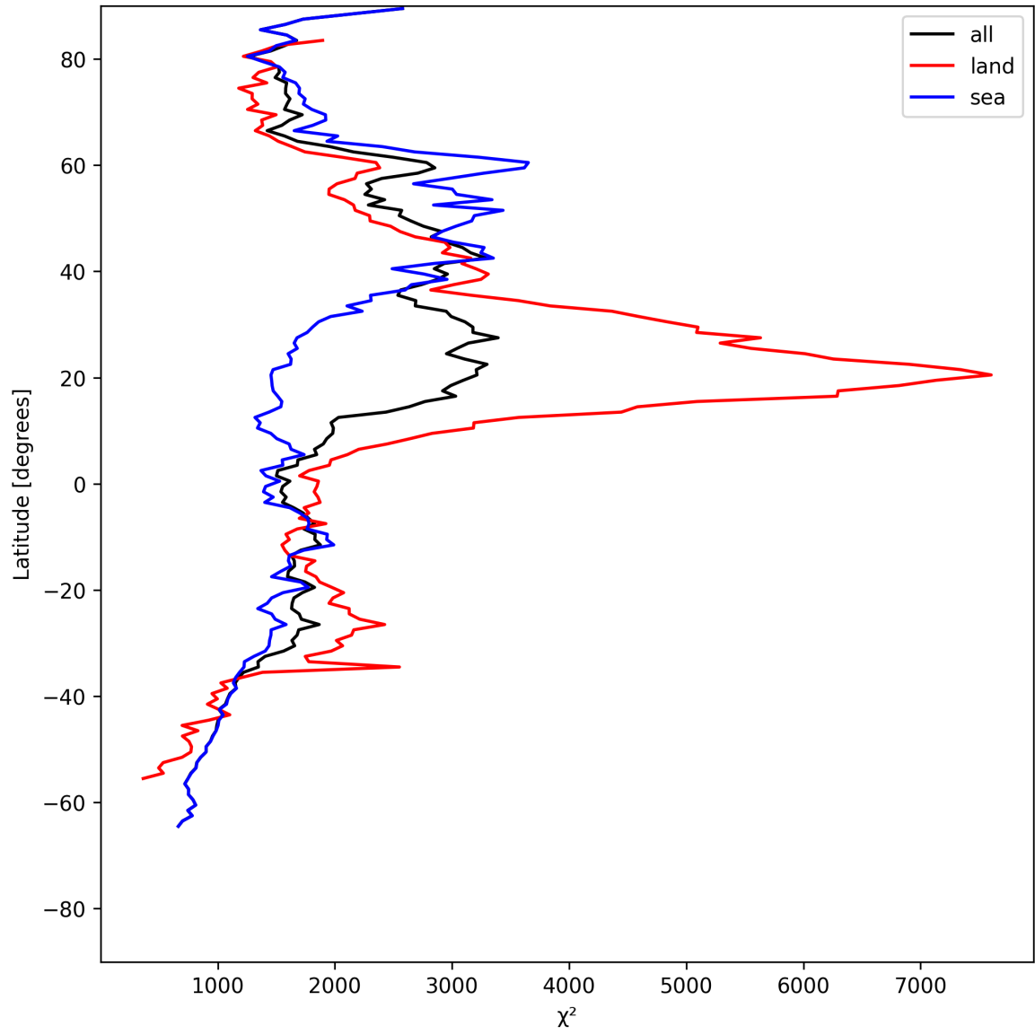
Figure 10: Zonal average of “ \chi^2 ” for 2025-05-21 to 2025-05-22.
