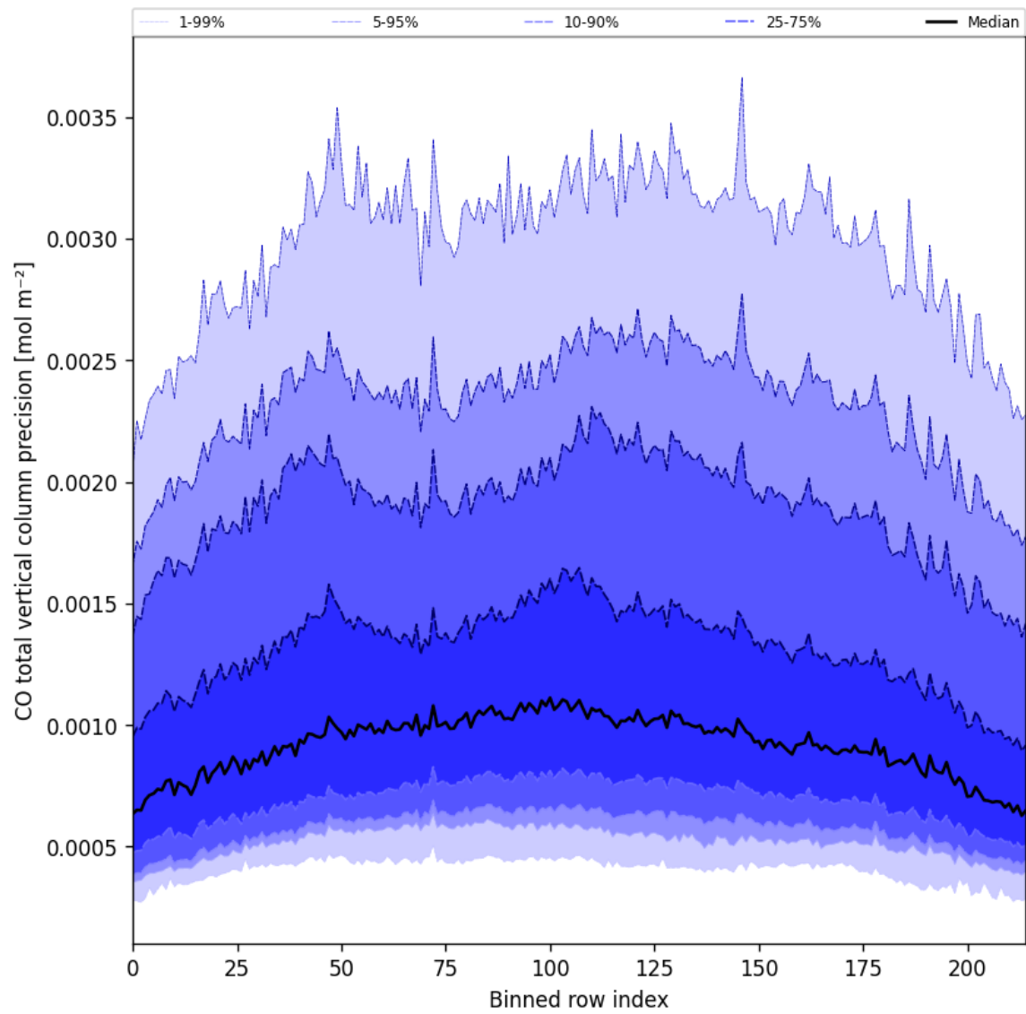
Figure 22: Along track statistics of “CO total vertical column precision” for 2025-05-21 to 2025-05-22
