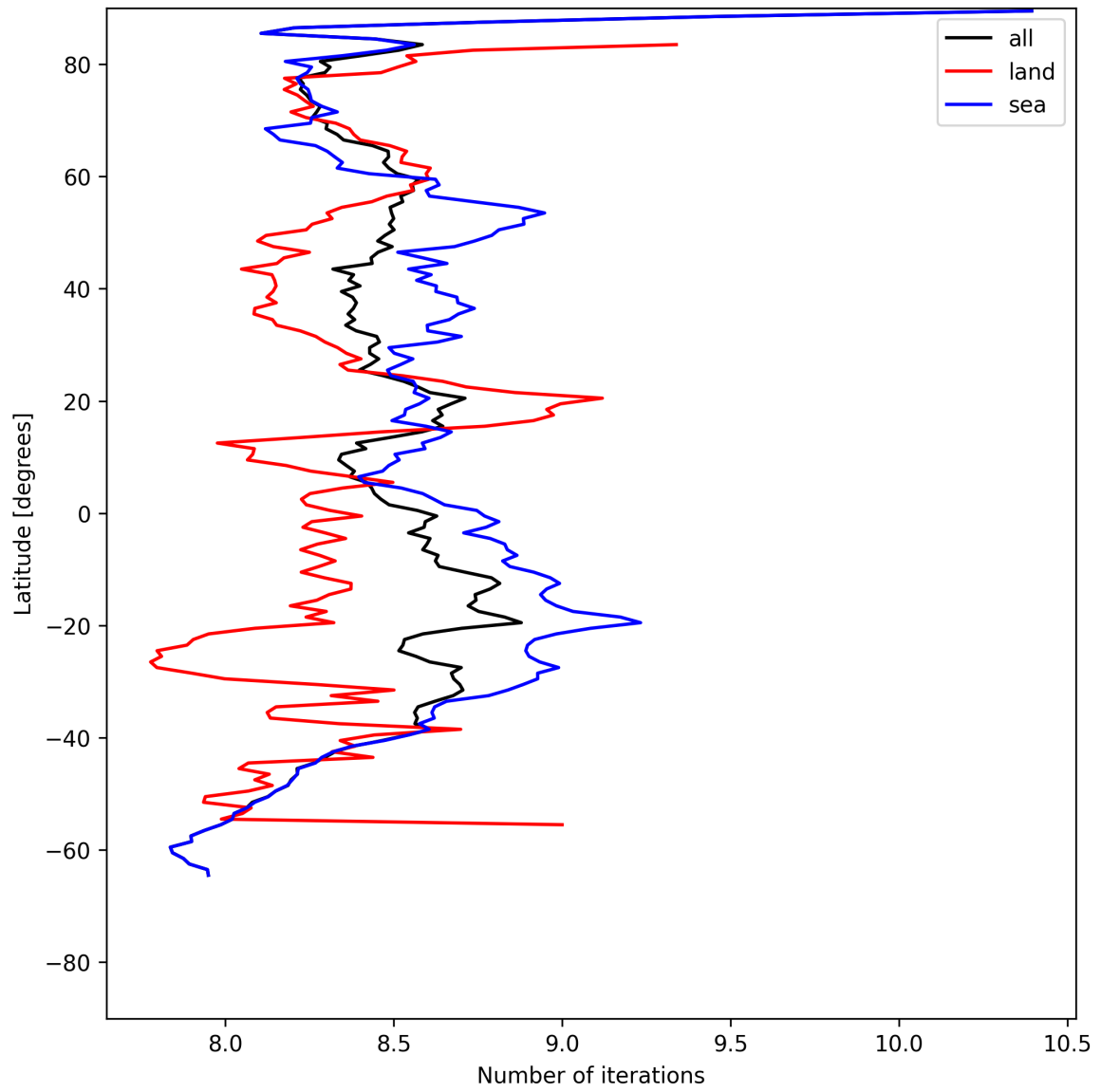
Figure 12: Zonal average of “Number of iterations” for 2025-05-21 to 2025-05-22.
