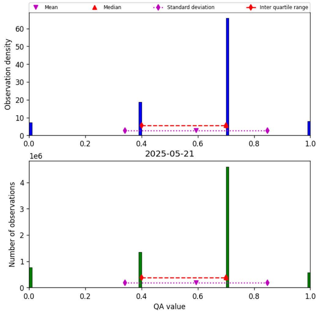
Figure 13: Histogram of “QA value” for 2025-05-21 to 2025-05-22
