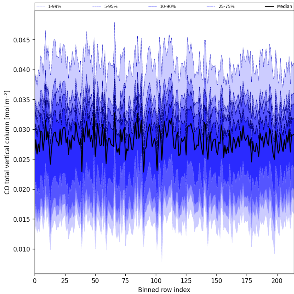
Figure 21: Along track statistics of “CO total vertical column” for 2025-05-21 to 2025-05-22
