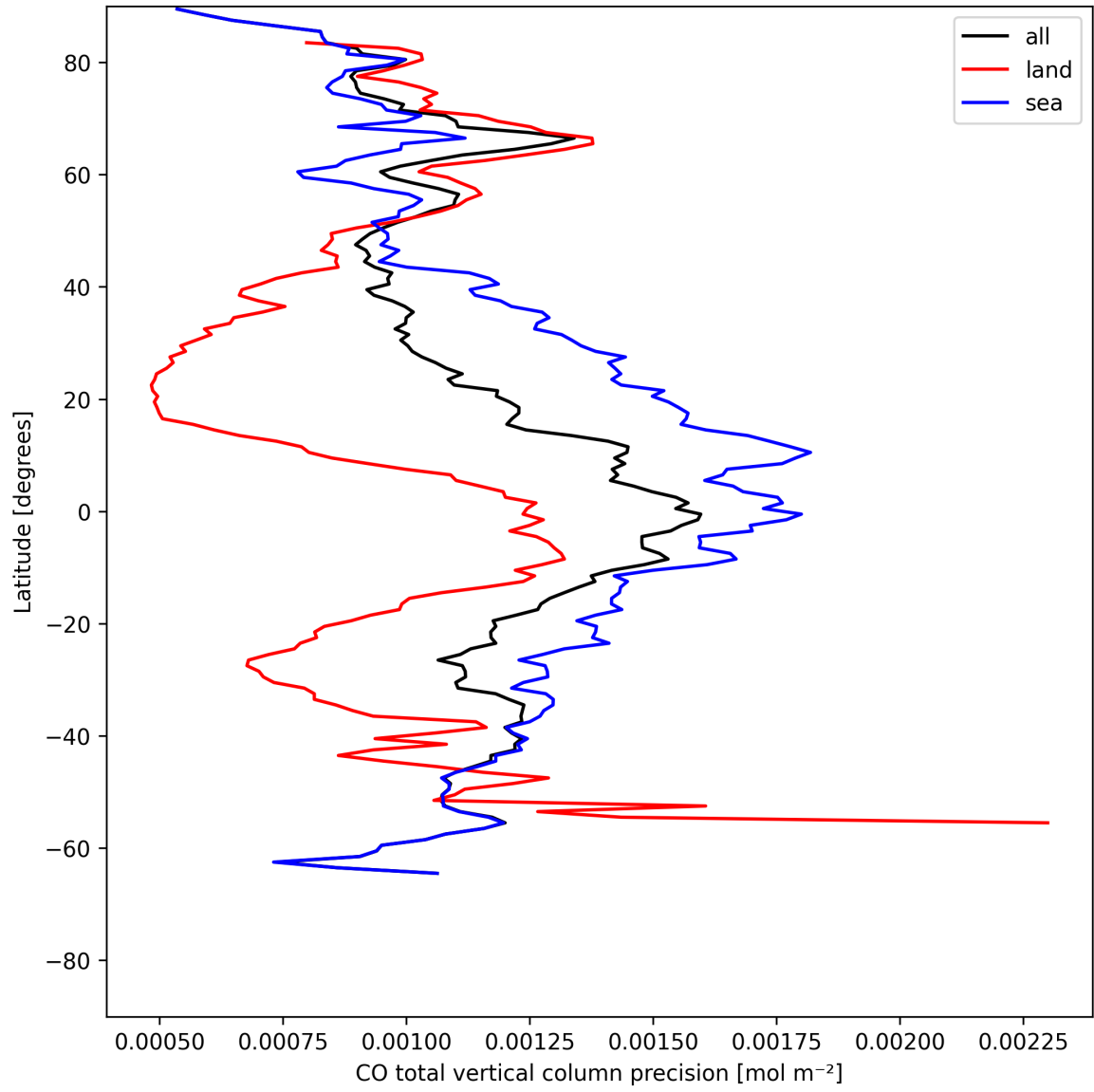
Figure 8: Zonal average of “CO total vertical column precision” for 2025-05-21 to 2025-05-22.
