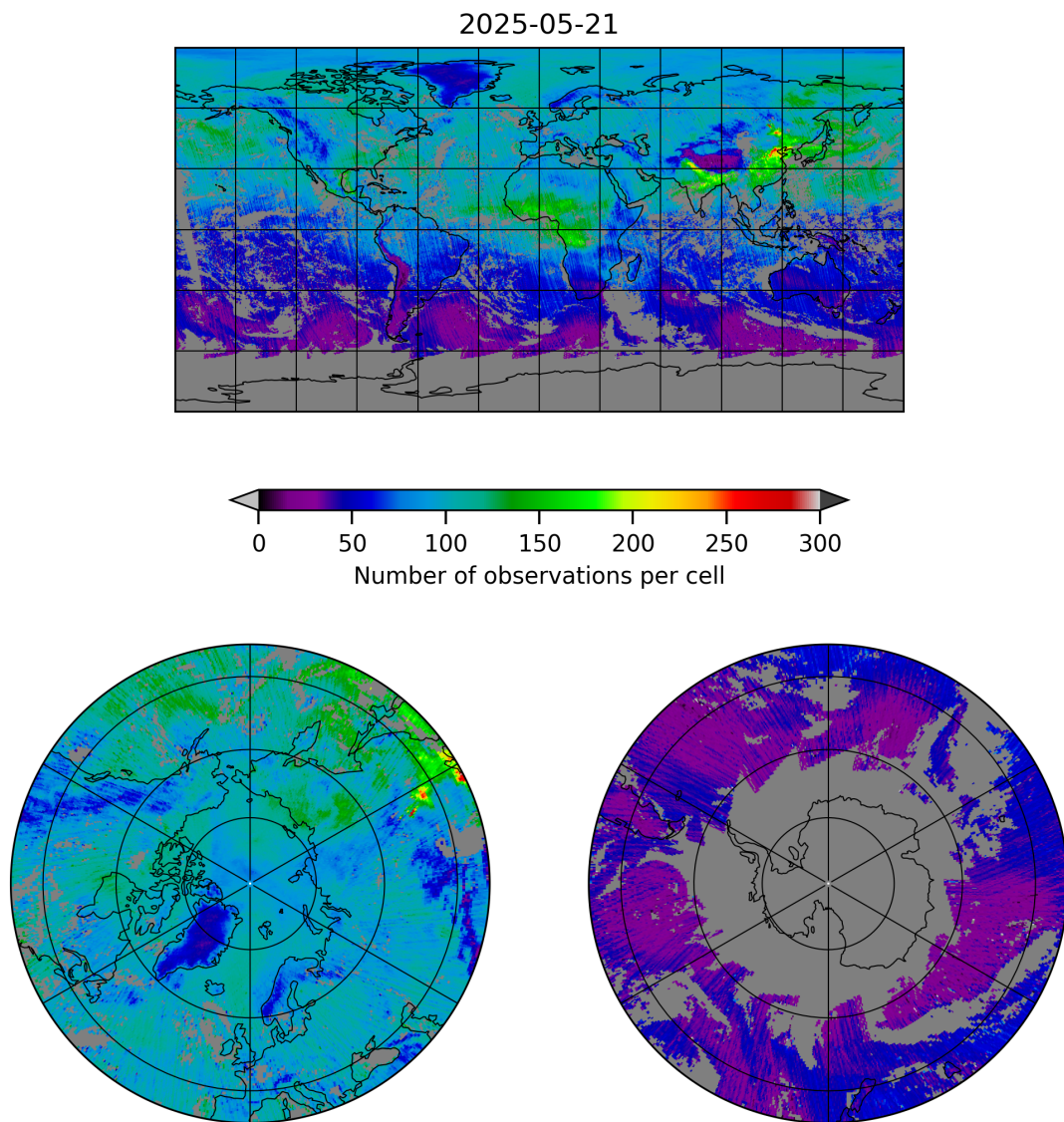
Figure 5: Map of the number of observations for 2025-05-21 to 2025-05-22
