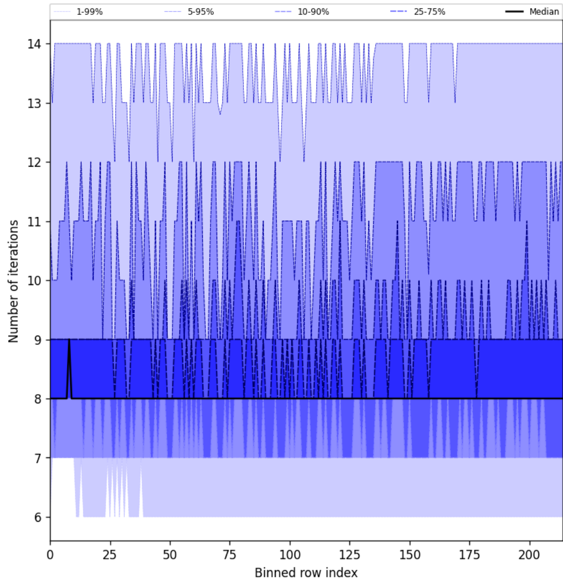
Figure 26: Along track statistics of “Number of iterations” for 2025-05-21 to 2025-05-22
