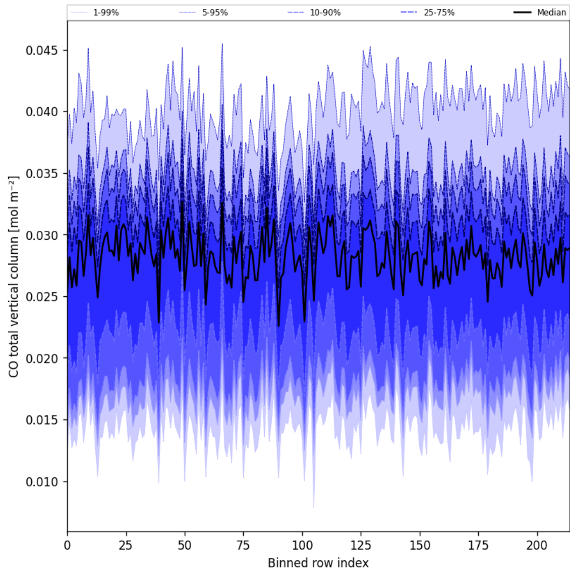
Figure 21: Along track statistics of “CO total vertical column” for 2025-05-22 to 2025-05-23
