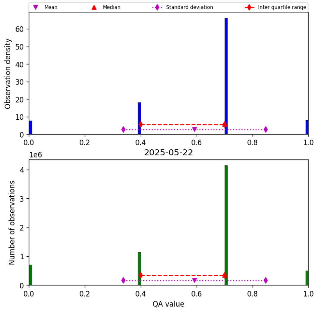
Figure 13: Histogram of “QA value” for 2025-05-22 to 2025-05-23
