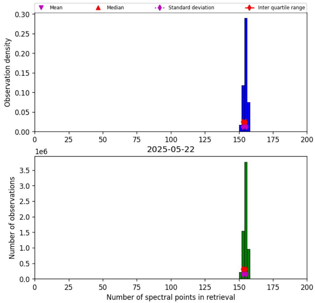
Figure 16: Histogram of “Number of spectral points in retrieval” for 2025-05-22 to 2025-05-23
