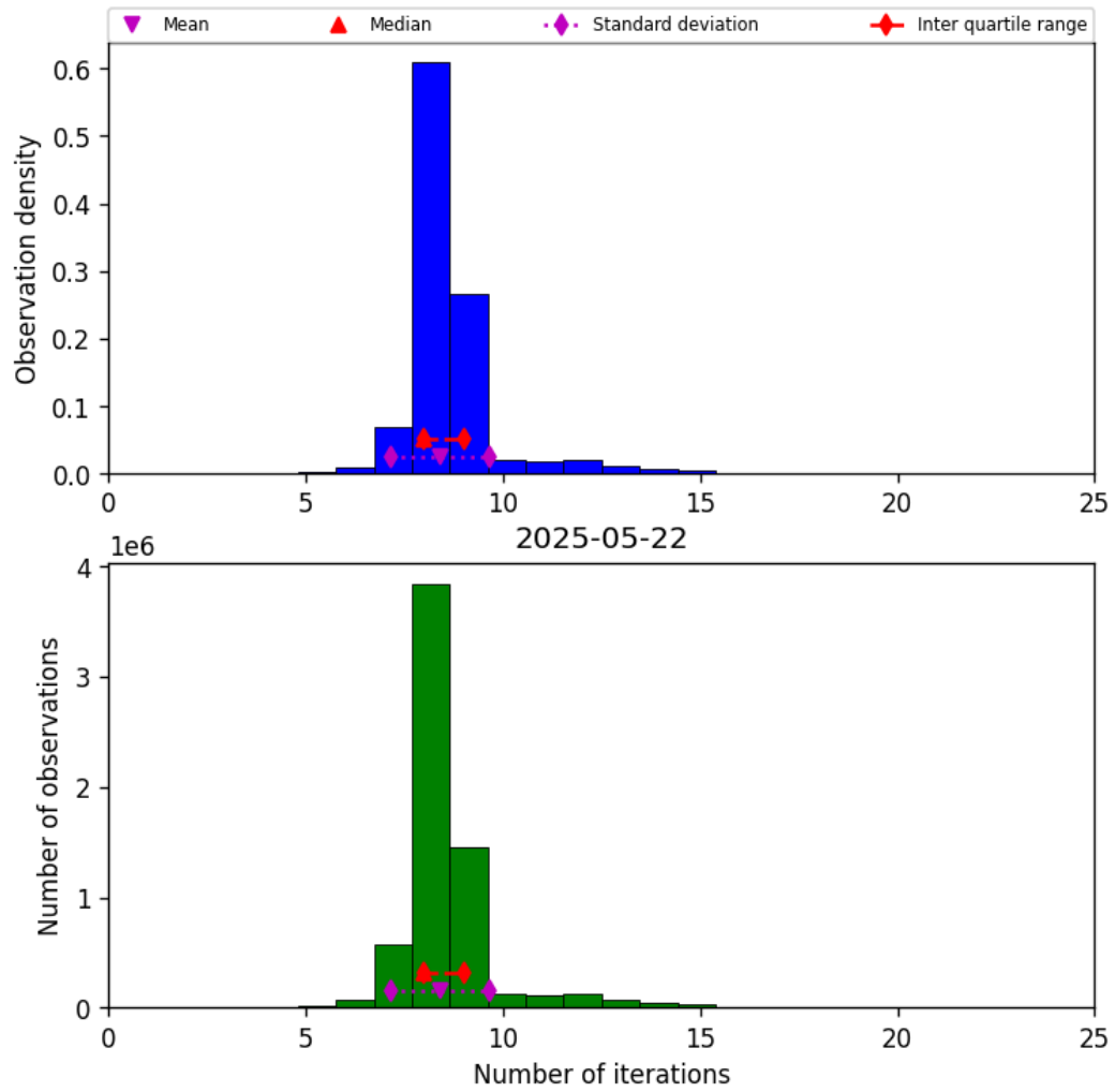
Figure 19: Histogram of “Number of iterations” for 2025-05-22 to 2025-05-23
