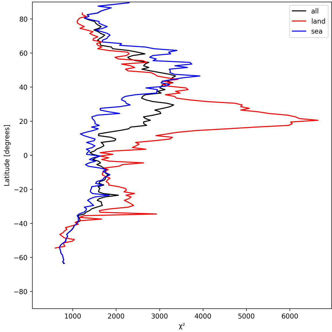
Figure 10: Zonal average of “ \chi^2 ” for 2025-05-22 to 2025-05-23.
