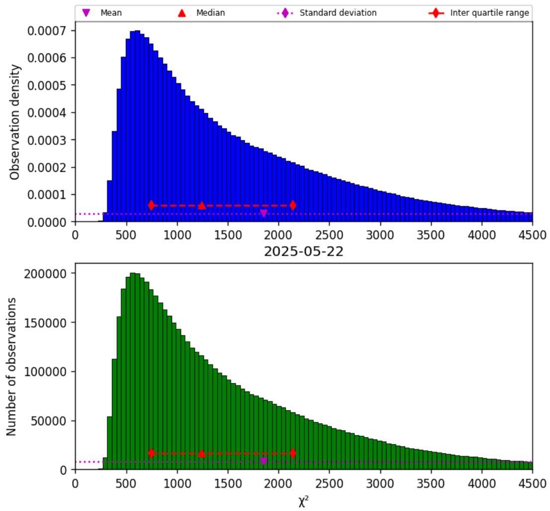
Figure 17: Histogram of “ \chi^2 ” for 2025-05-22 to 2025-05-23
