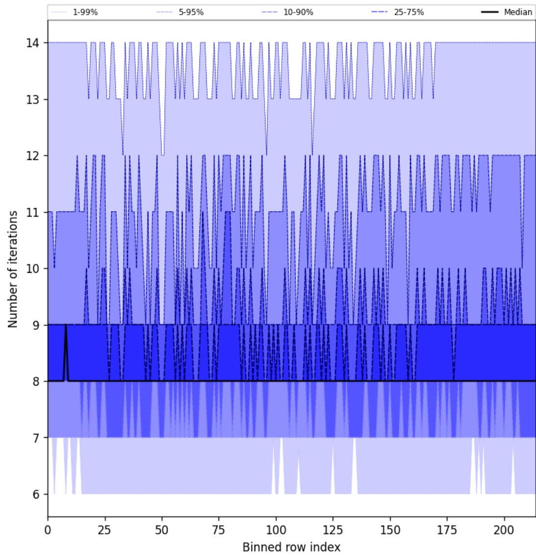
Figure 26: Along track statistics of “Number of iterations” for 2025-05-22 to 2025-05-23
