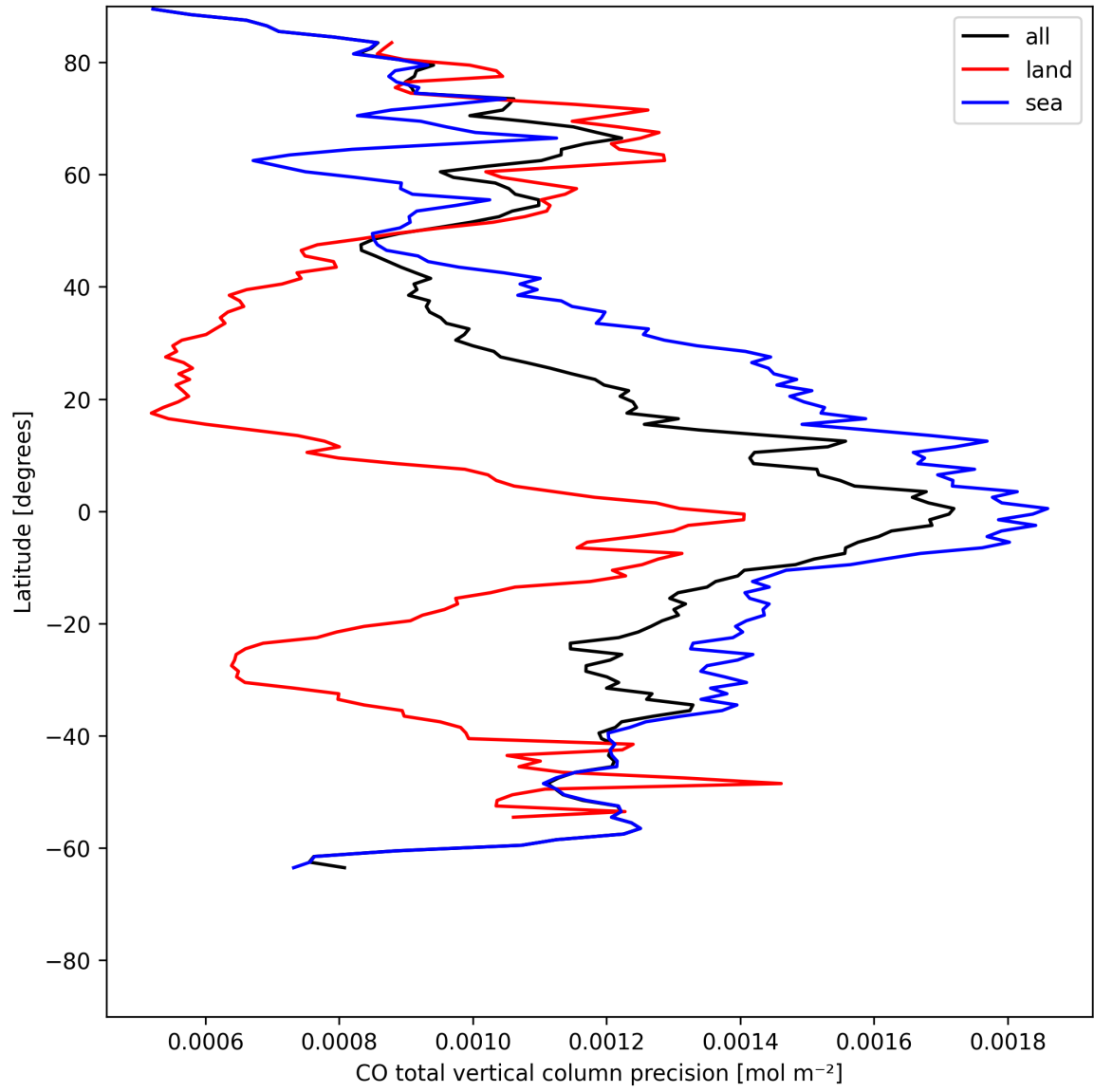
Figure 8: Zonal average of “CO total vertical column precision” for 2025-05-22 to 2025-05-23.
