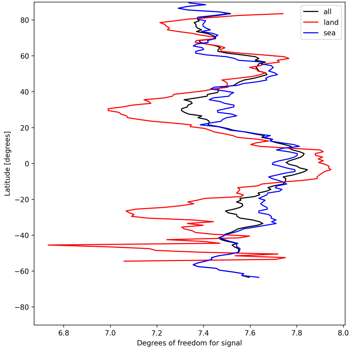
Figure 11: Zonal average of “Degrees of freedom for signal” for 2025-05-22 to 2025-05-23.
