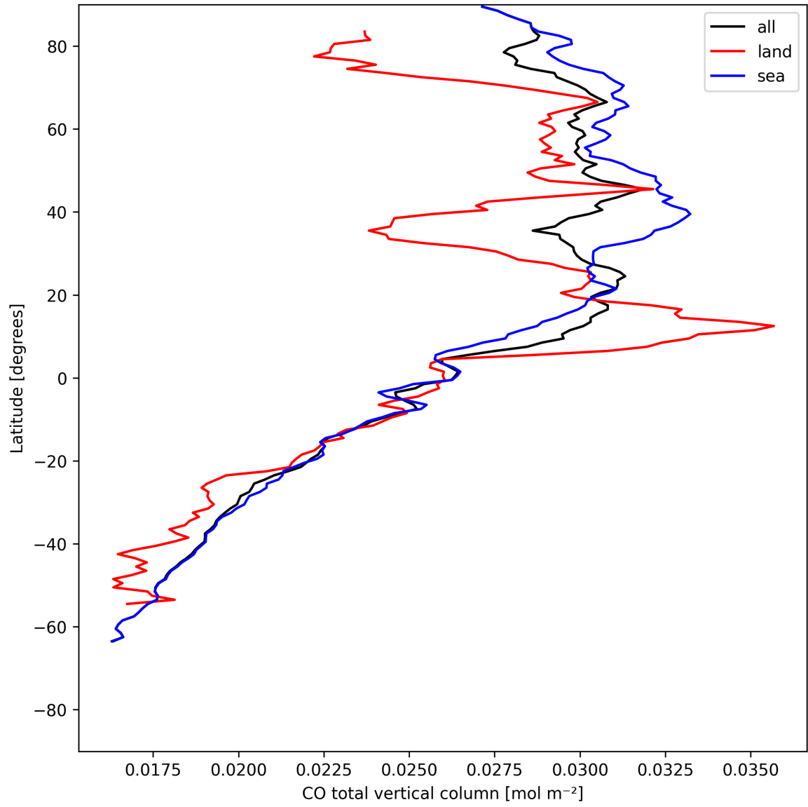
Figure 7: Zonal average of “CO total vertical column” for 2025-05-22 to 2025-05-23.
