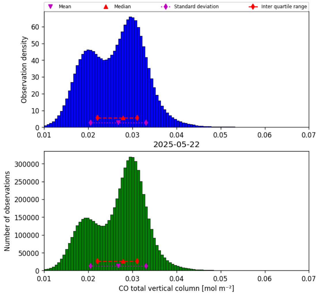
Figure 14: Histogram of “CO total vertical column” for 2025-05-22 to 2025-05-23
