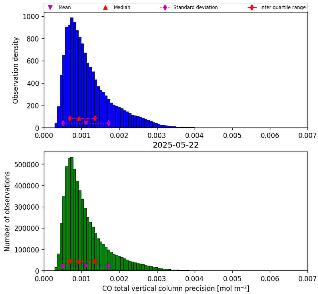
Figure 15: Histogram of “CO total vertical column precision” for 2025-05-22 to 2025-05-23
