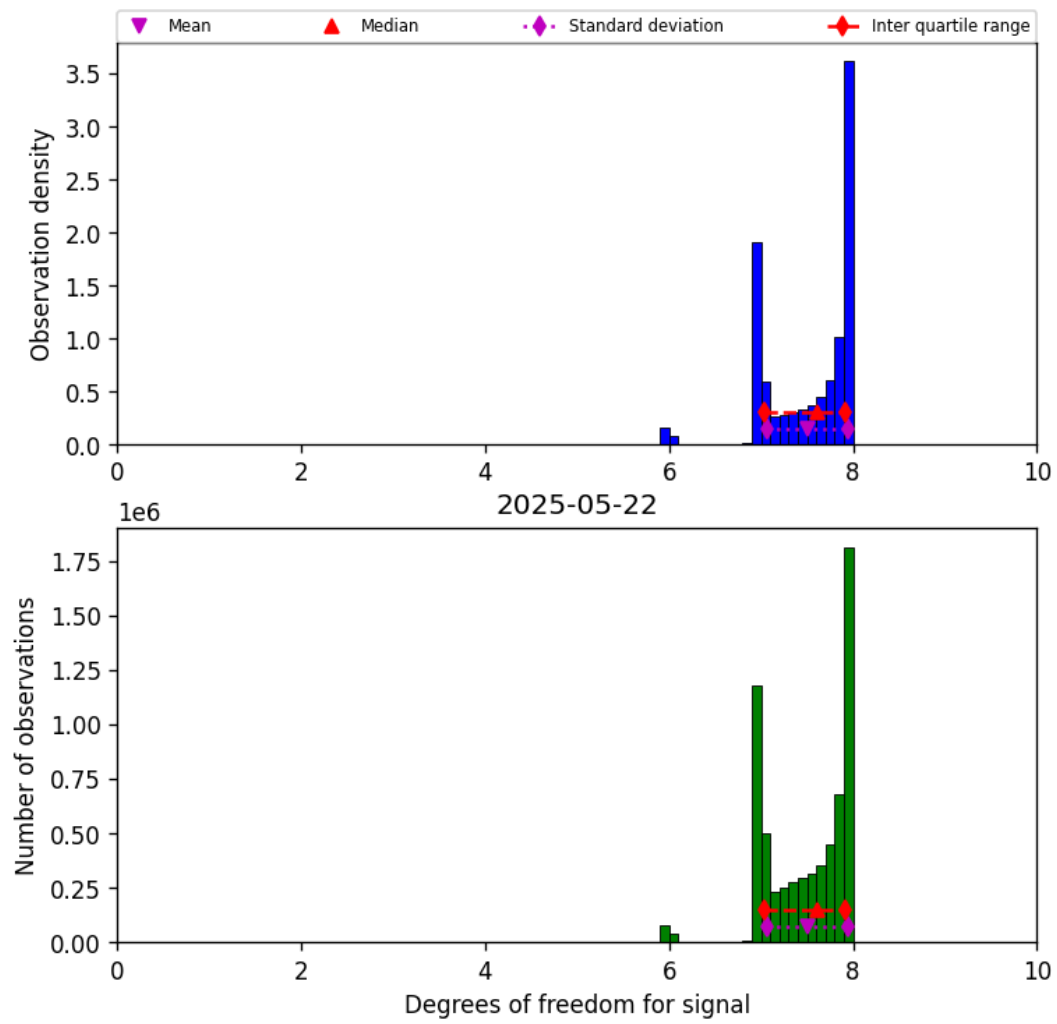
Figure 18: Histogram of “Degrees of freedom for signal” for 2025-05-22 to 2025-05-23
