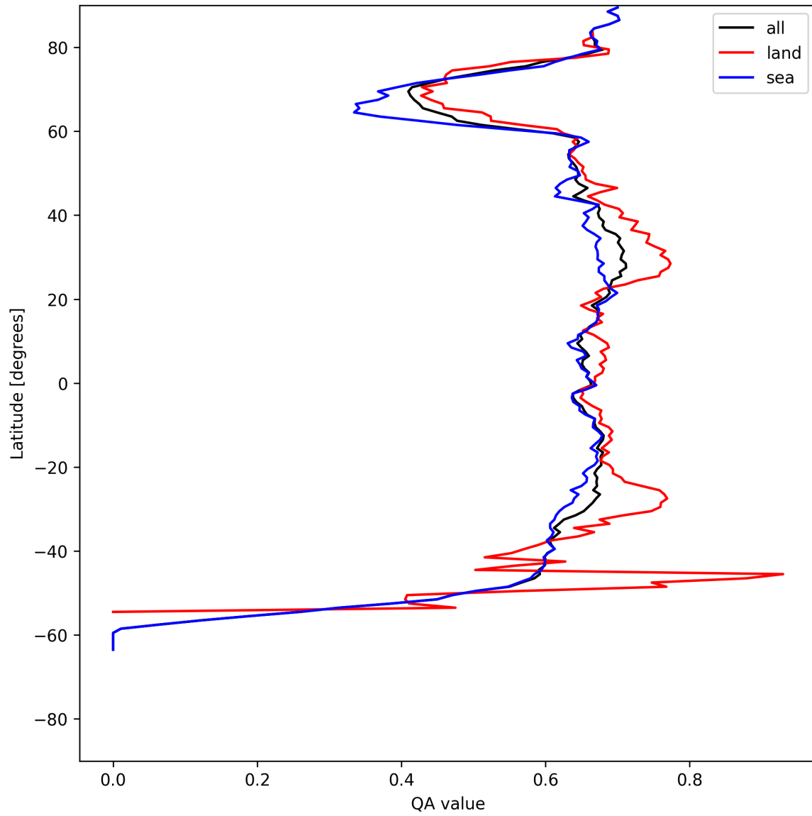
Figure 6: Zonal average of “QA value” for 2025-05-22 to 2025-05-23.
