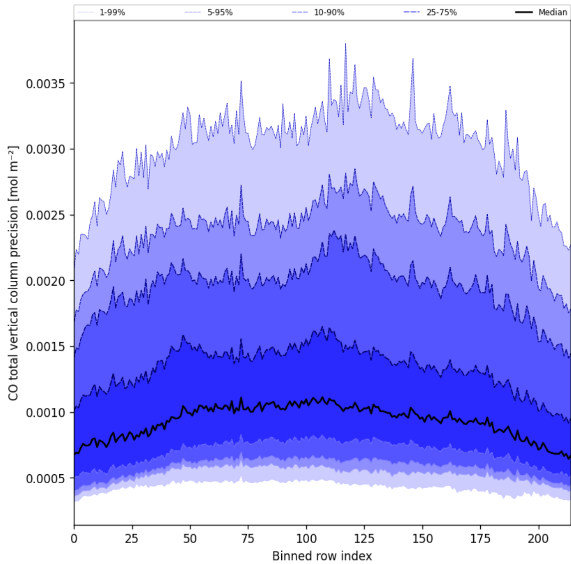
Figure 22: Along track statistics of “CO total vertical column precision” for 2025-05-22 to 2025-05-23
