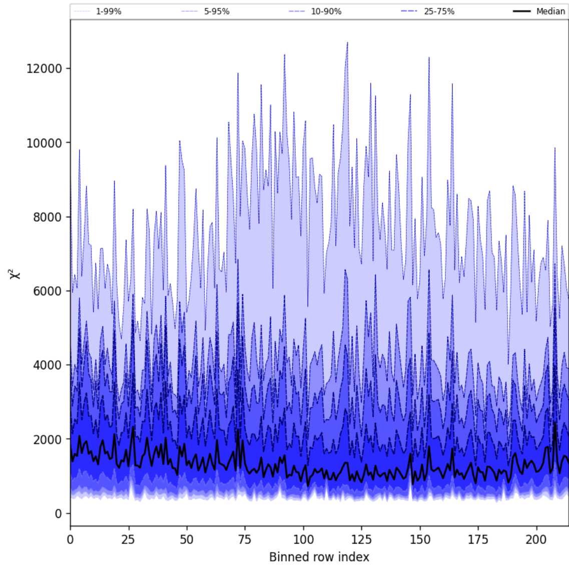
Figure 24: Along track statistics of “ \chi^2 ” for 2025-05-22 to 2025-05-23
