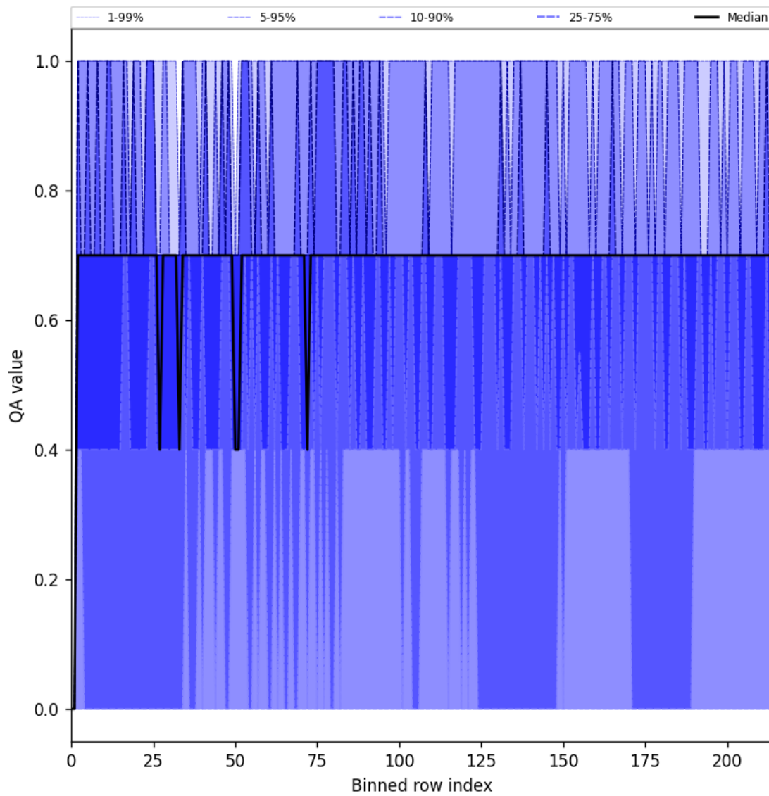
Figure 20: Along track statistics of “QA value” for 2025-05-22 to 2025-05-23
