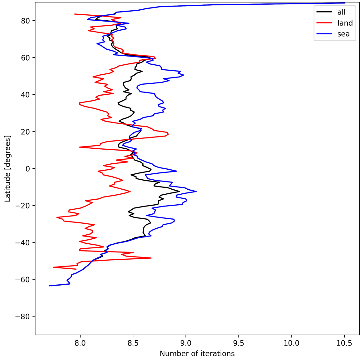
Figure 12: Zonal average of “Number of iterations” for 2025-05-22 to 2025-05-23.
