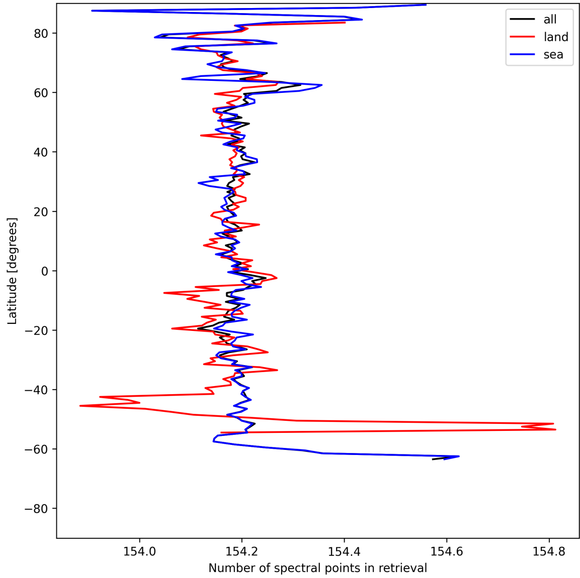
Figure 9: Zonal average of “Number of spectral points in retrieval” for 2025-05-22 to 2025-05-23.
