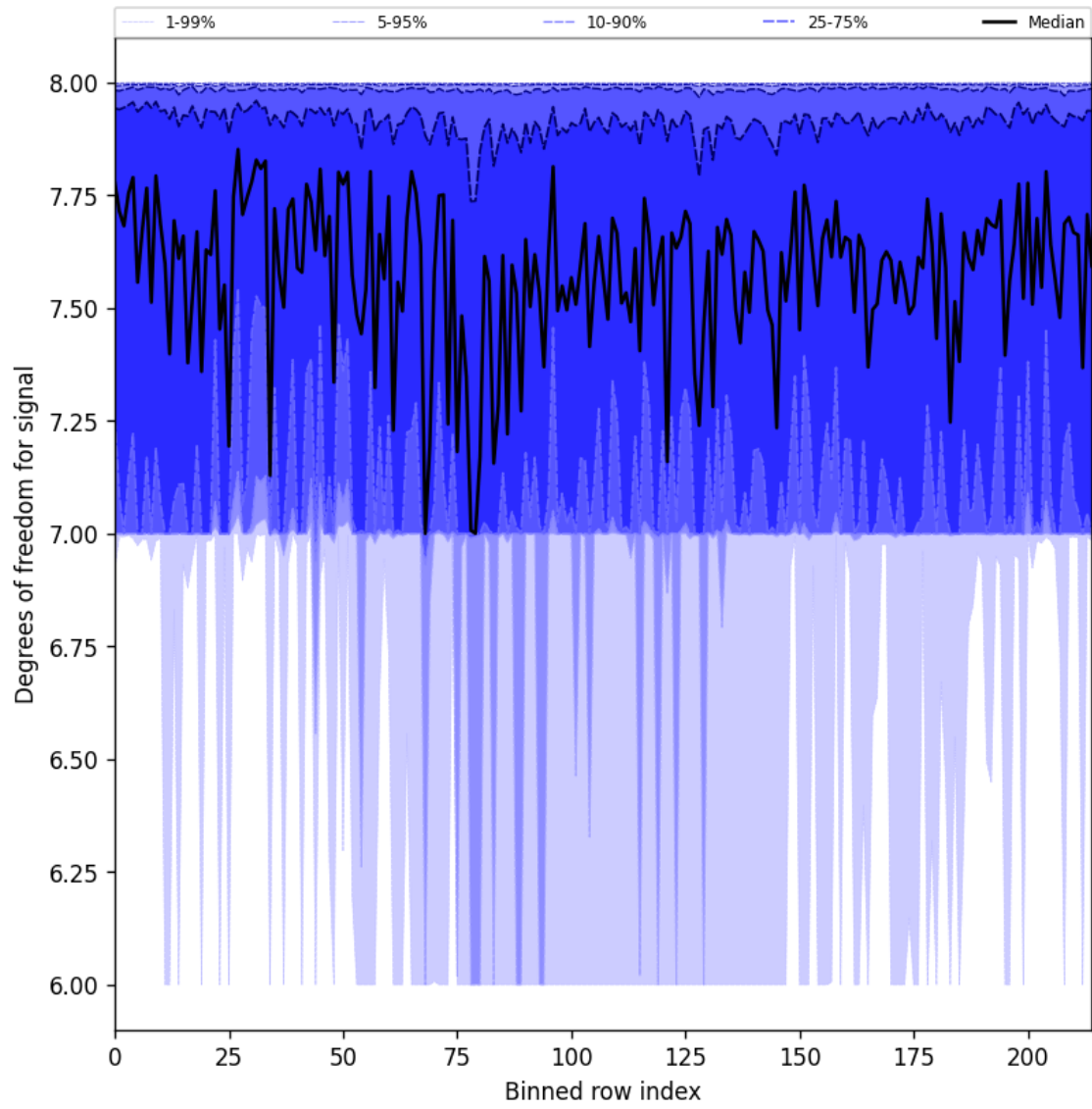
Figure 25: Along track statistics of “Degrees of freedom for signal” for 2025-05-22 to 2025-05-23
