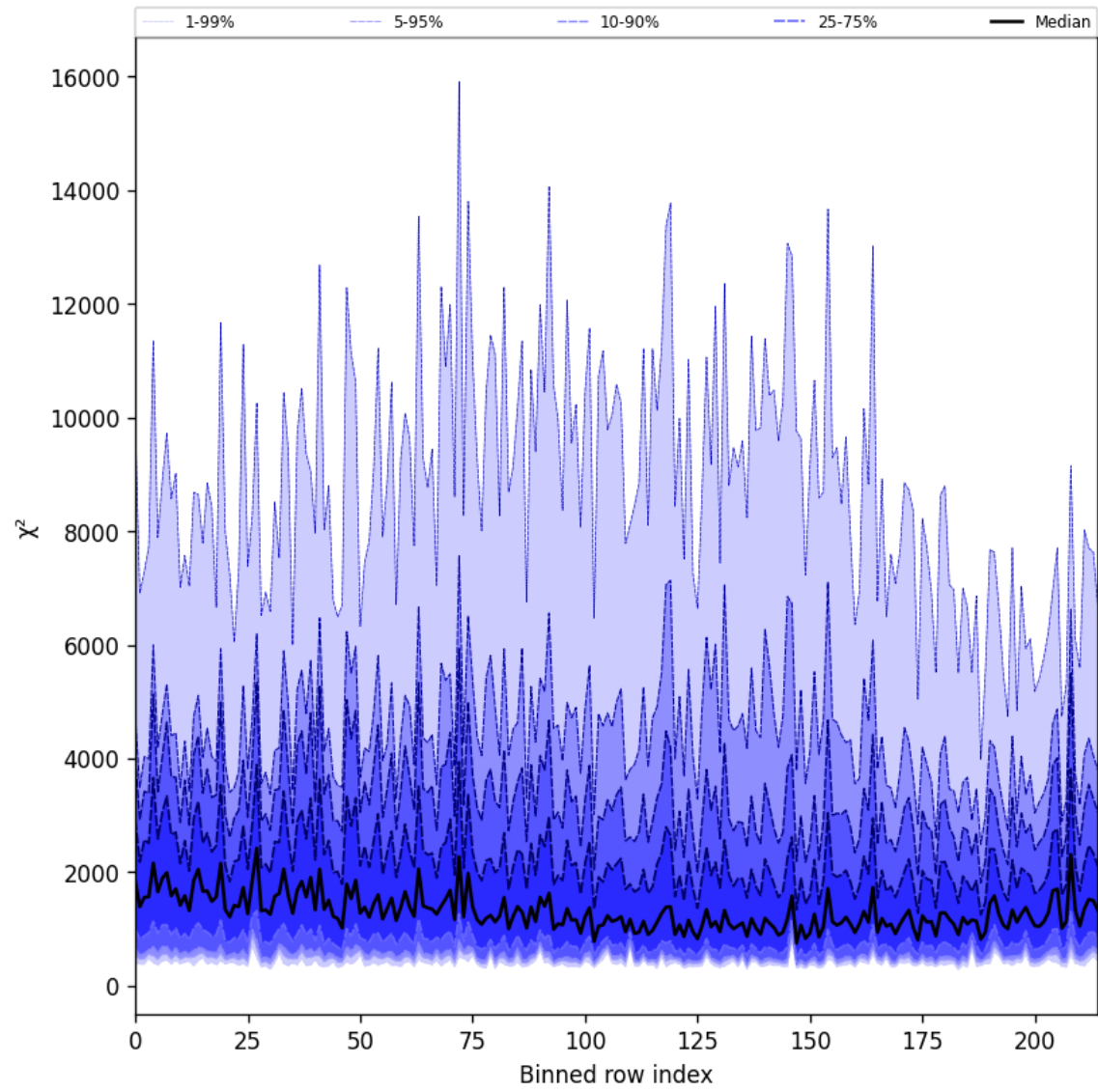
Figure 24: Along track statistics of “ \chi^2 ” for 2025-05-23 to 2025-05-24
