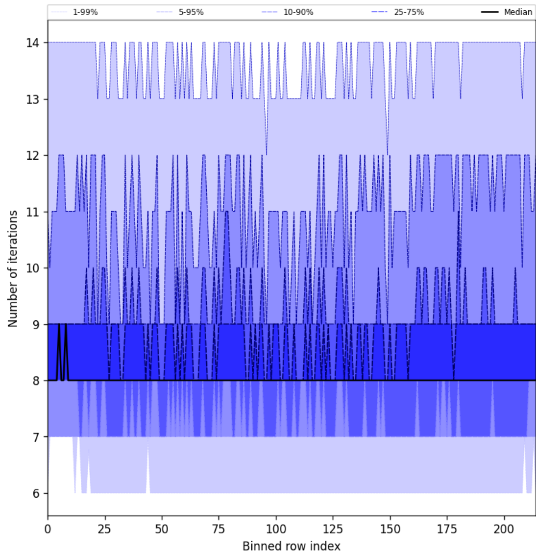
Figure 26: Along track statistics of “Number of iterations” for 2025-05-23 to 2025-05-24
