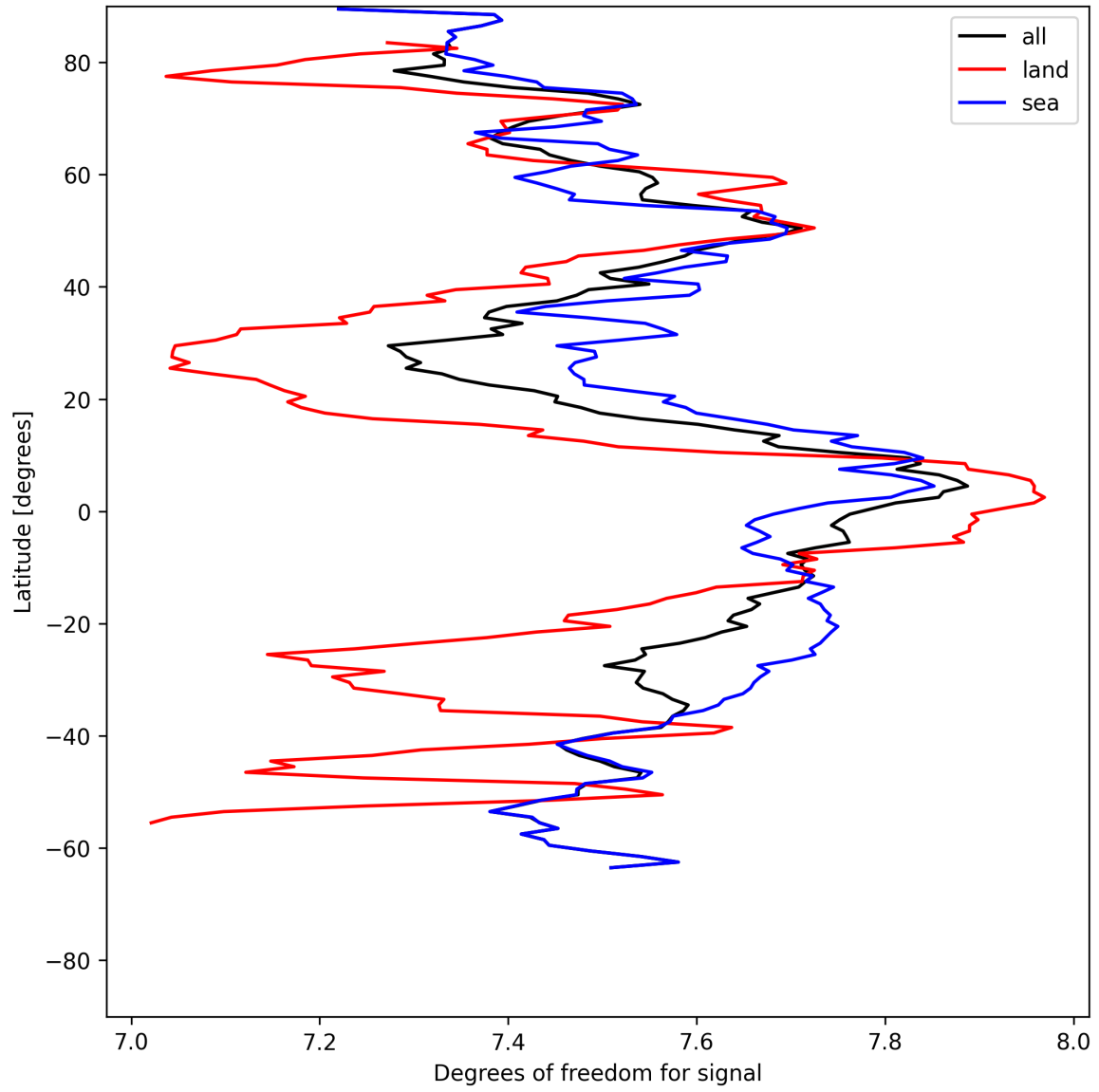
Figure 11: Zonal average of “Degrees of freedom for signal” for 2025-05-23 to 2025-05-24.
