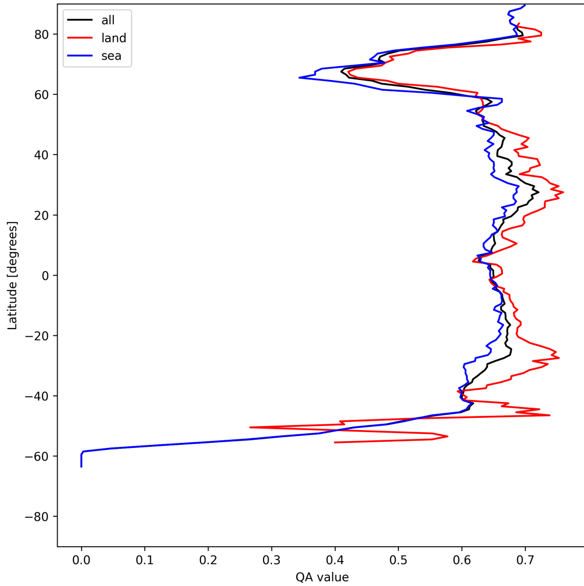
Figure 6: Zonal average of “QA value” for 2025-05-23 to 2025-05-24.
