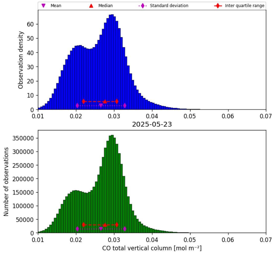
Figure 14: Histogram of “CO total vertical column” for 2025-05-23 to 2025-05-24
