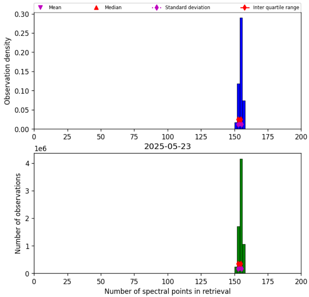
Figure 16: Histogram of “Number of spectral points in retrieval” for 2025-05-23 to 2025-05-24
