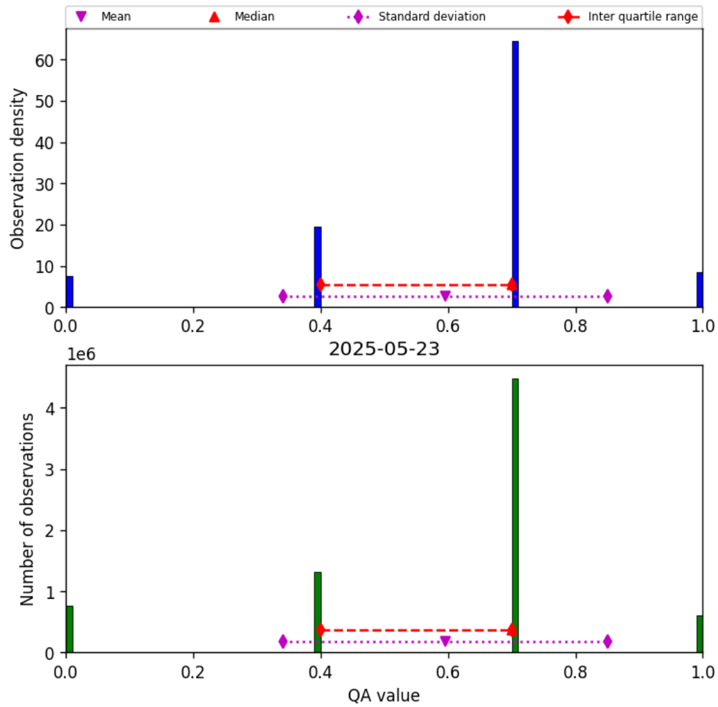
Figure 13: Histogram of “QA value” for 2025-05-23 to 2025-05-24
