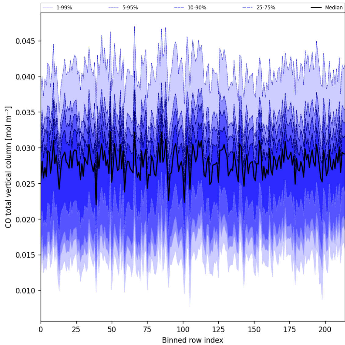
Figure 21: Along track statistics of "CO total vertical column" for 2025-05-23 to 2025-05-24
