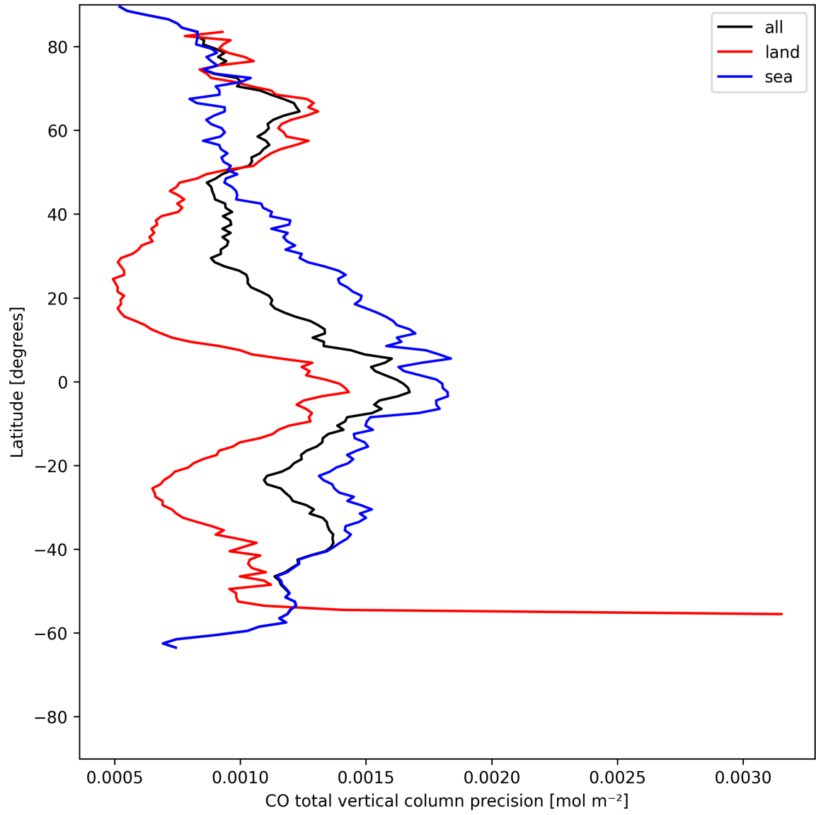
Figure 8: Zonal average of “CO total vertical column precision” for 2025-05-23 to 2025-05-24.
