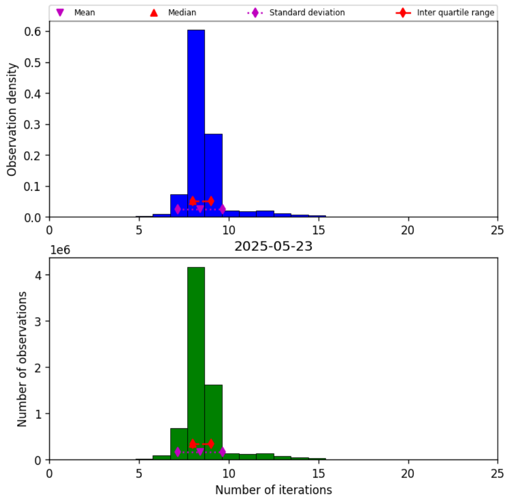
Figure 19: Histogram of “Number of iterations” for 2025-05-23 to 2025-05-24
