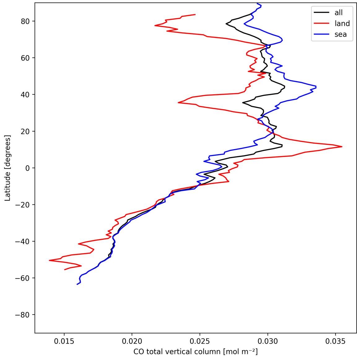
Figure 7: Zonal average of “CO total vertical column” for 2025-05-23 to 2025-05-24.
