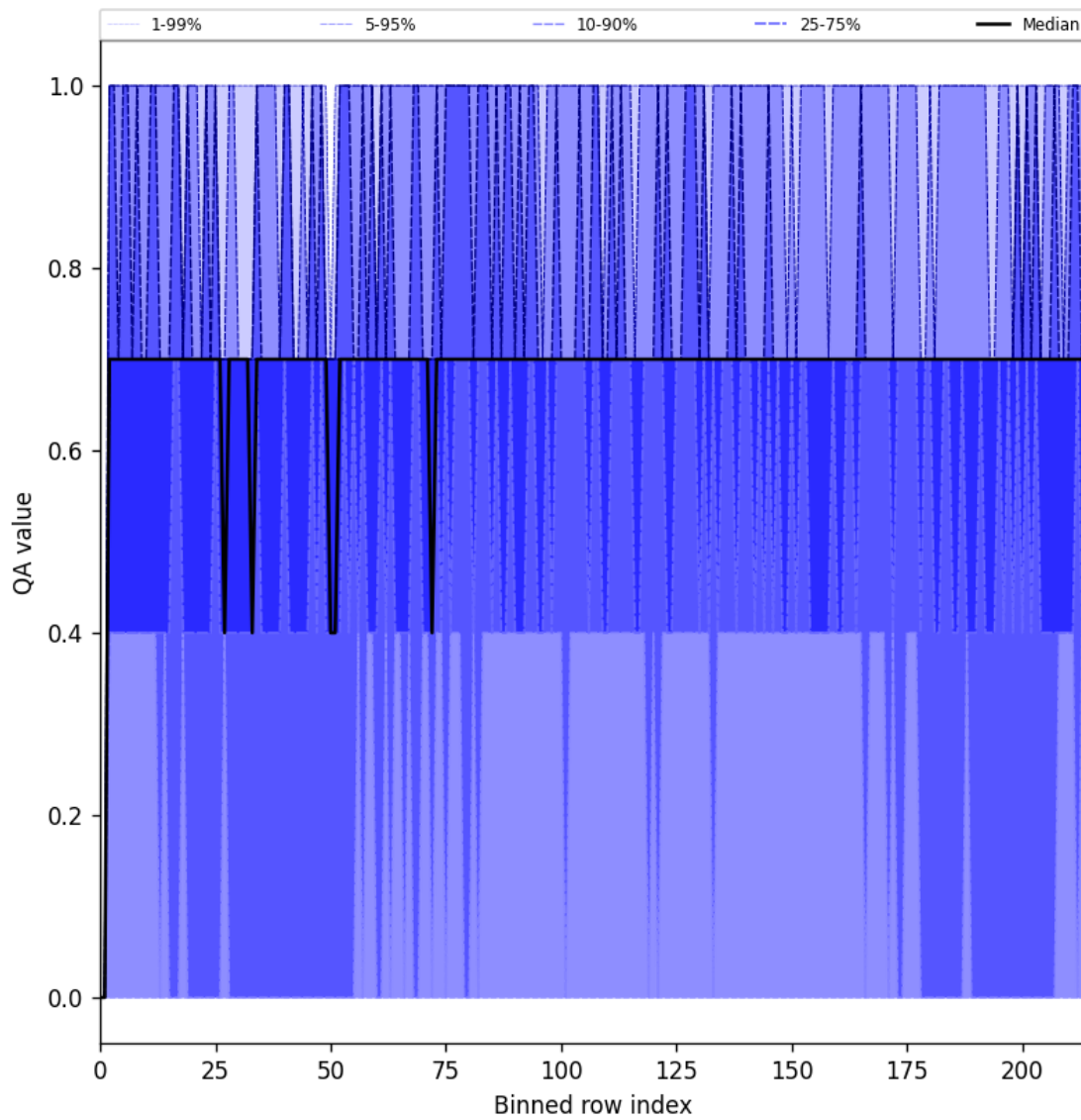
Figure 20: Along track statistics of “QA value” for 2025-05-23 to 2025-05-24
