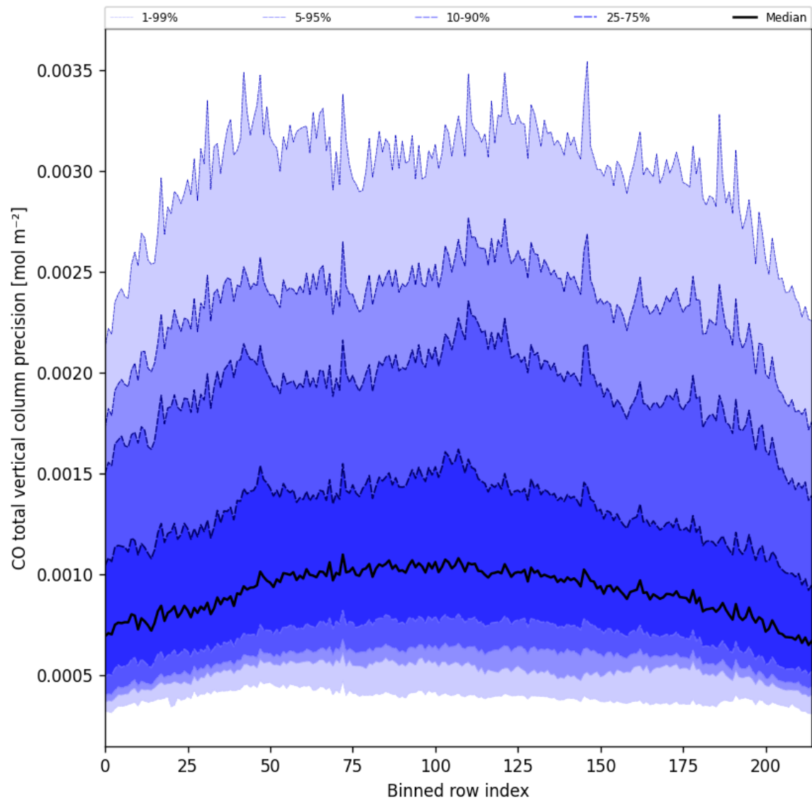
Figure 22: Along track statistics of “CO total vertical column precision” for 2025-05-23 to 2025-05-24
