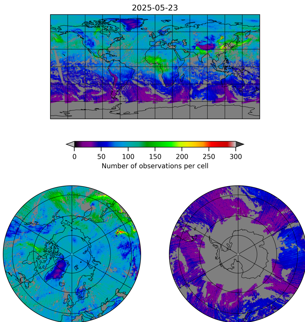
Figure 5: Map of the number of observations for 2025-05-23 to 2025-05-24
