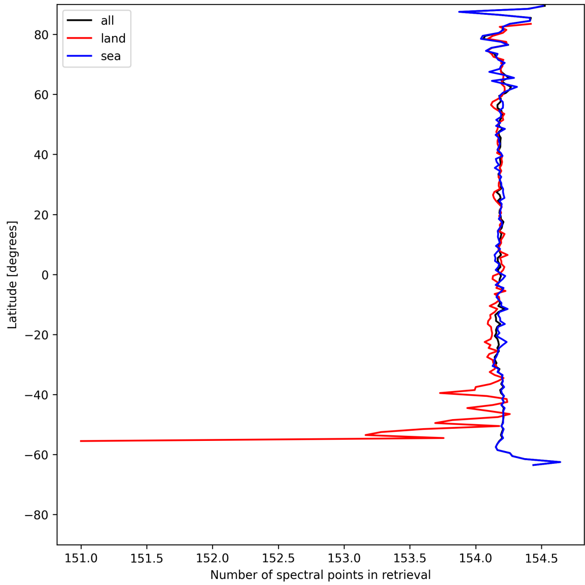
Figure 9: Zonal average of “Number of spectral points in retrieval” for 2025-05-23 to 2025-05-24.
