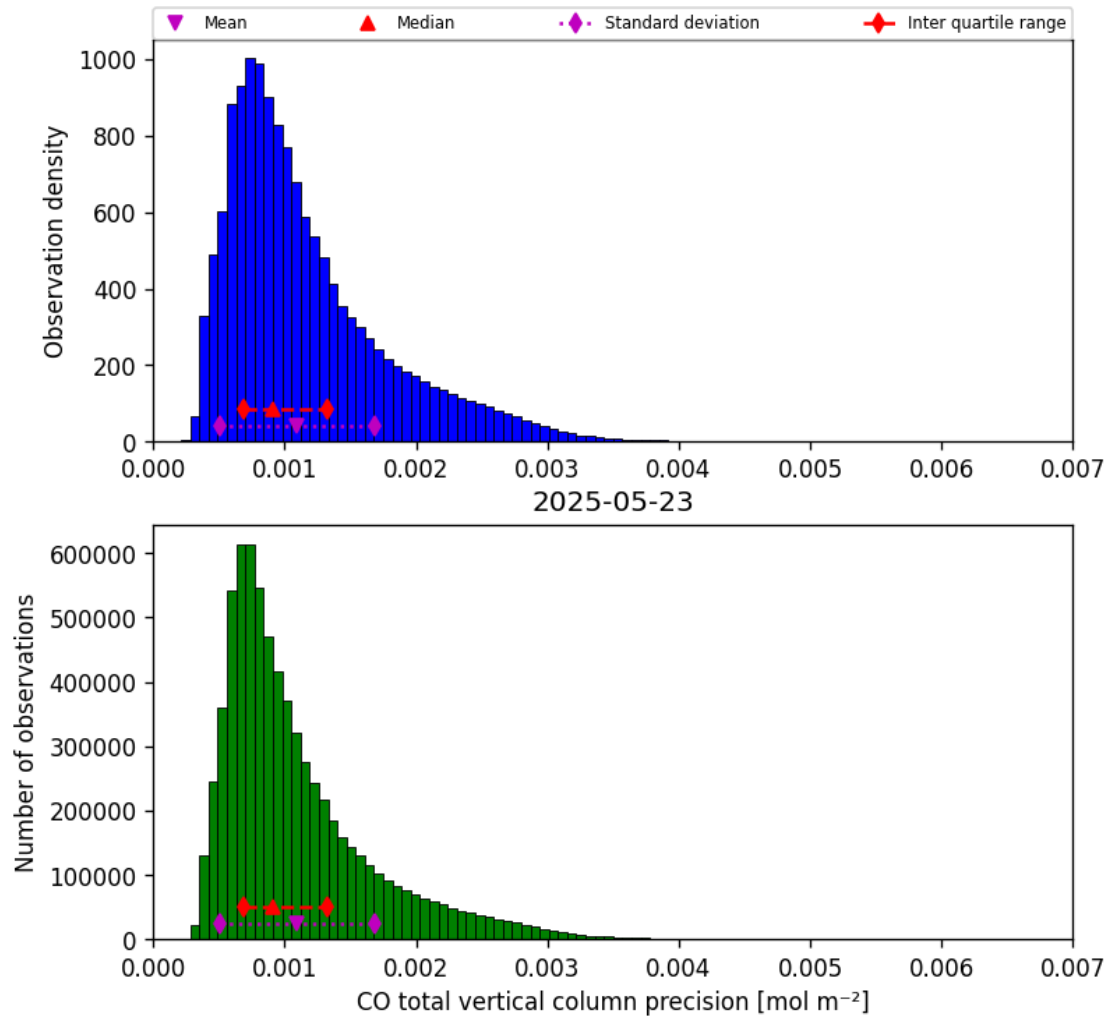
Figure 15: Histogram of “CO total vertical column precision” for 2025-05-23 to 2025-05-24
