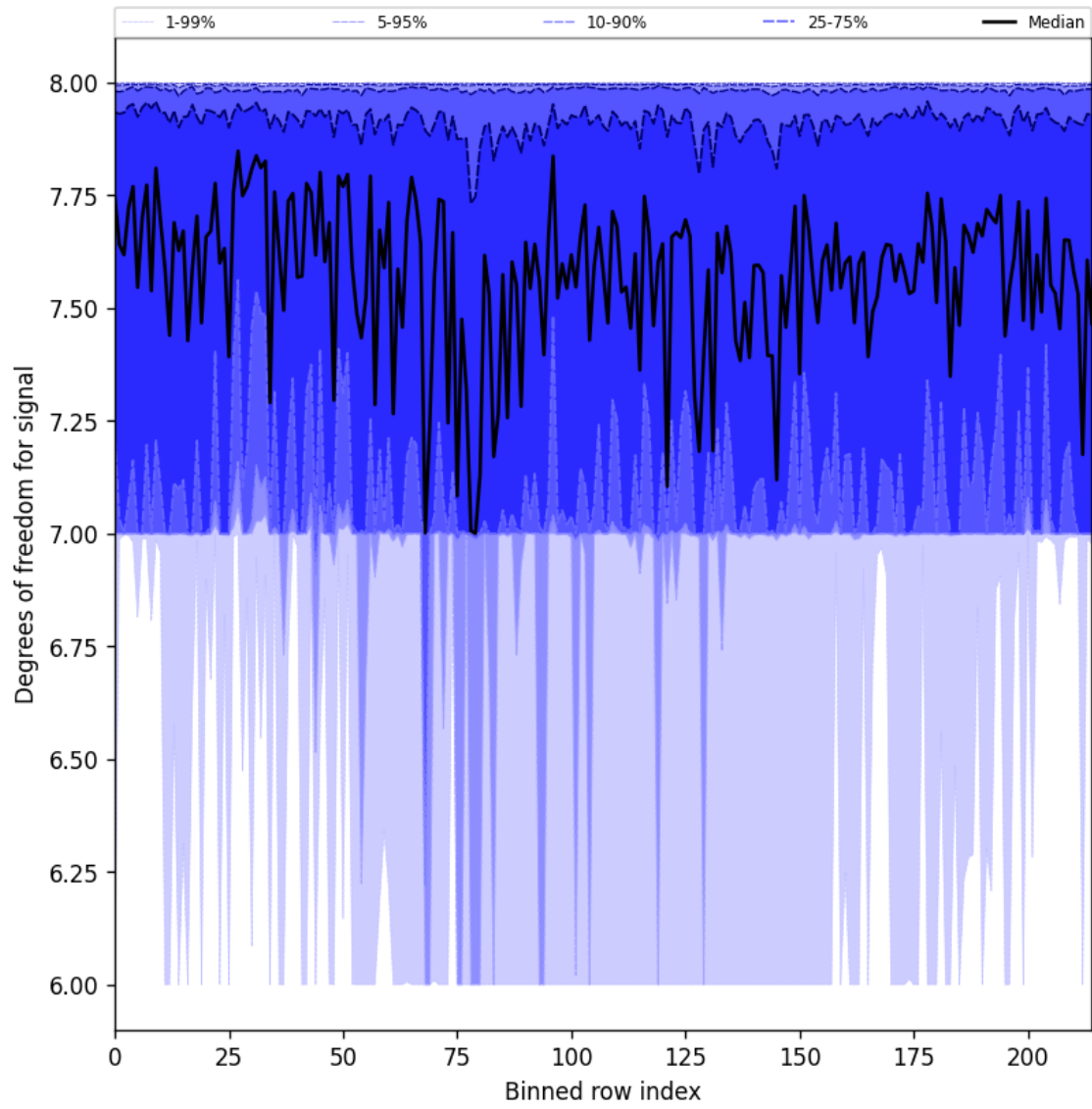
Figure 25: Along track statistics of “Degrees of freedom for signal” for 2025-05-23 to 2025-05-24
