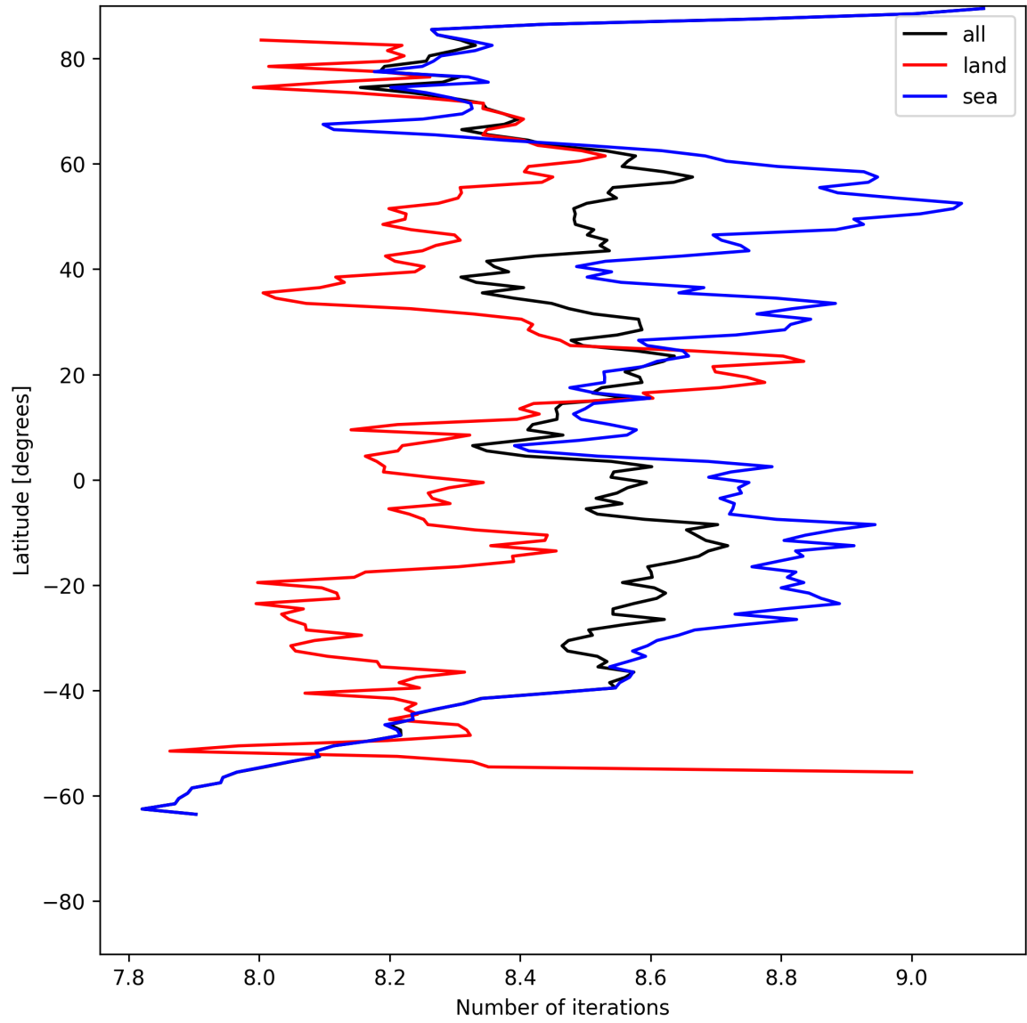
Figure 12: Zonal average of “Number of iterations” for 2025-05-23 to 2025-05-24.
