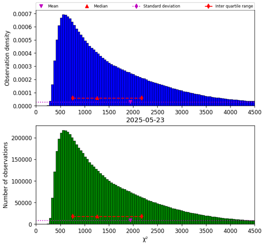
Figure 17: Histogram of “ \chi^2 ” for 2025-05-23 to 2025-05-24
