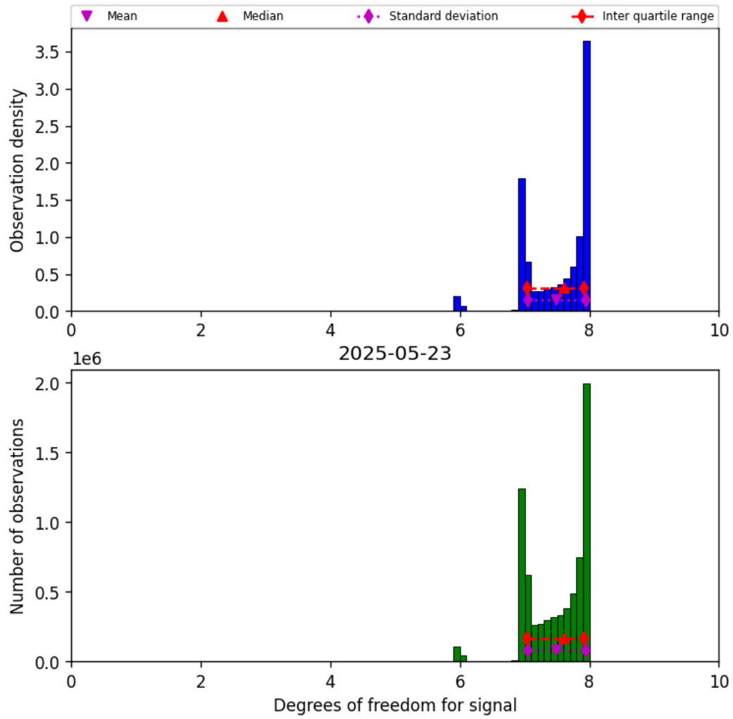
Figure 18: Histogram of “Degrees of freedom for signal” for 2025-05-23 to 2025-05-24
