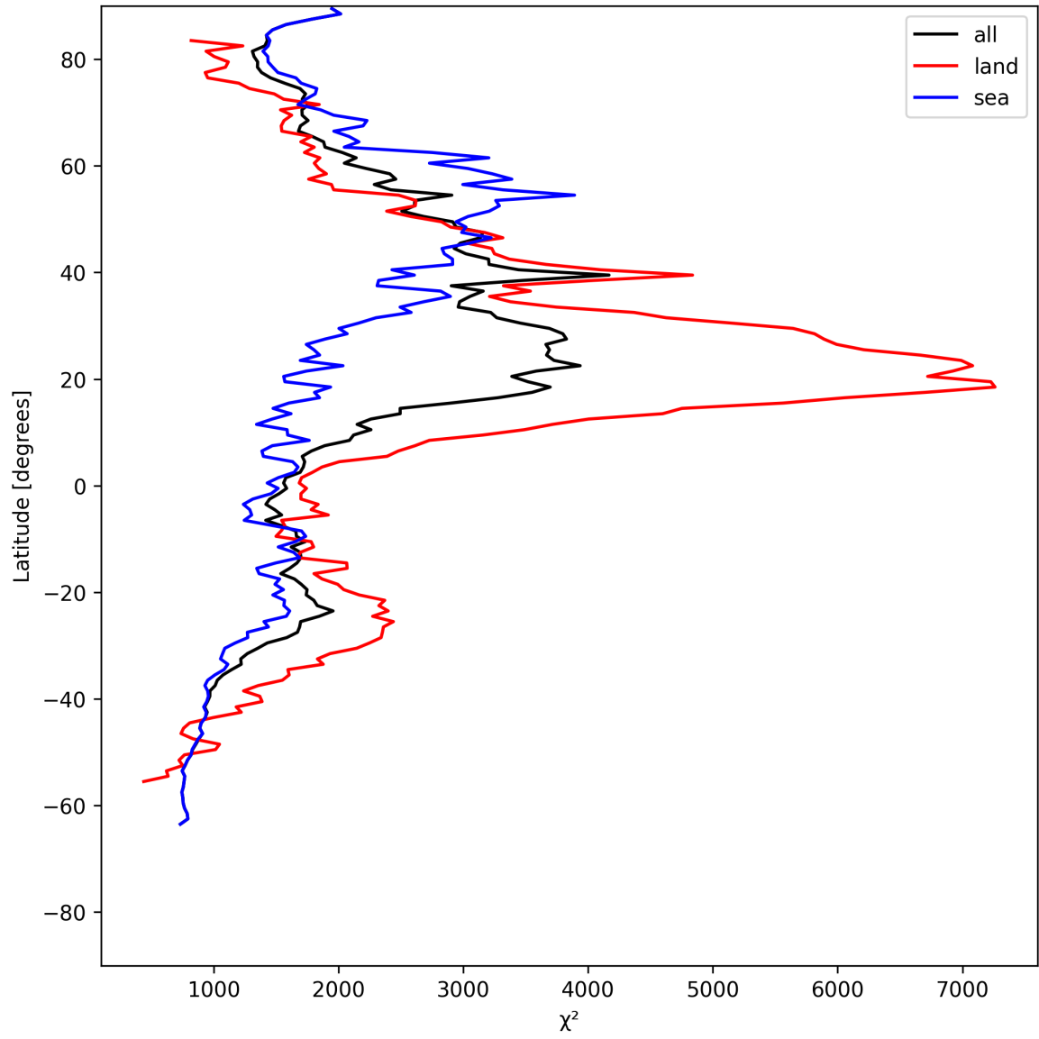
Figure 10: Zonal average of “ \chi^2 ” for 2025-05-23 to 2025-05-24.
