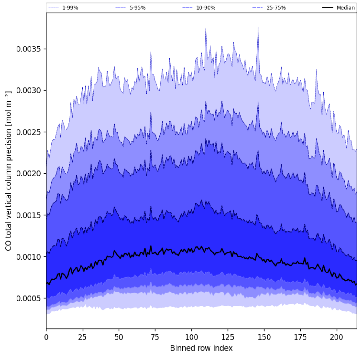
Figure 22: Along track statistics of “CO total vertical column precision” for 2025-05-24 to 2025-05-24
