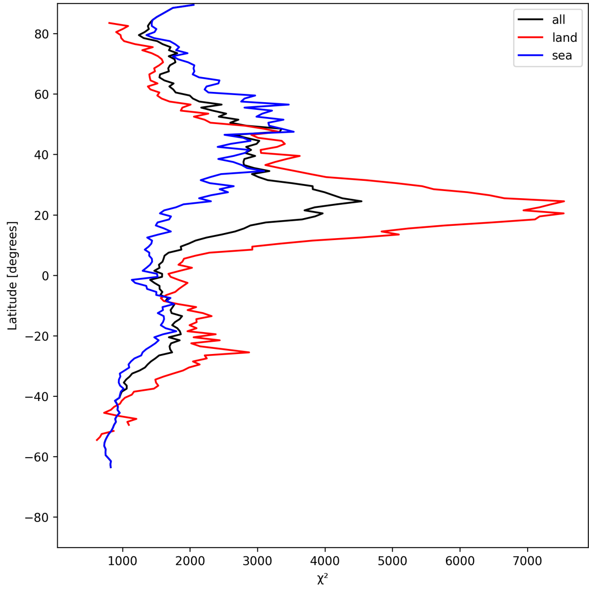
Figure 10: Zonal average of “ \chi^2 ” for 2025-05-24 to 2025-05-24.
