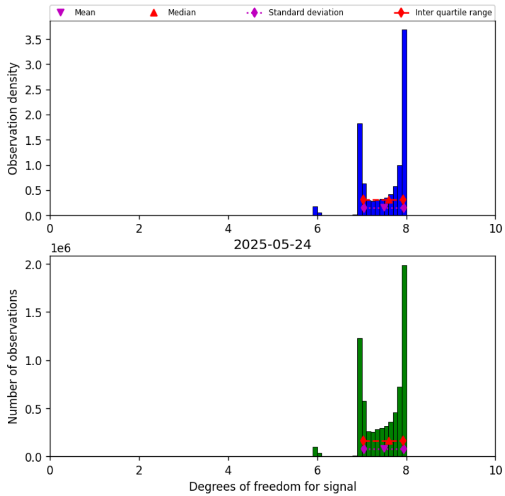
Figure 18: Histogram of “Degrees of freedom for signal” for 2025-05-24 to 2025-05-24
