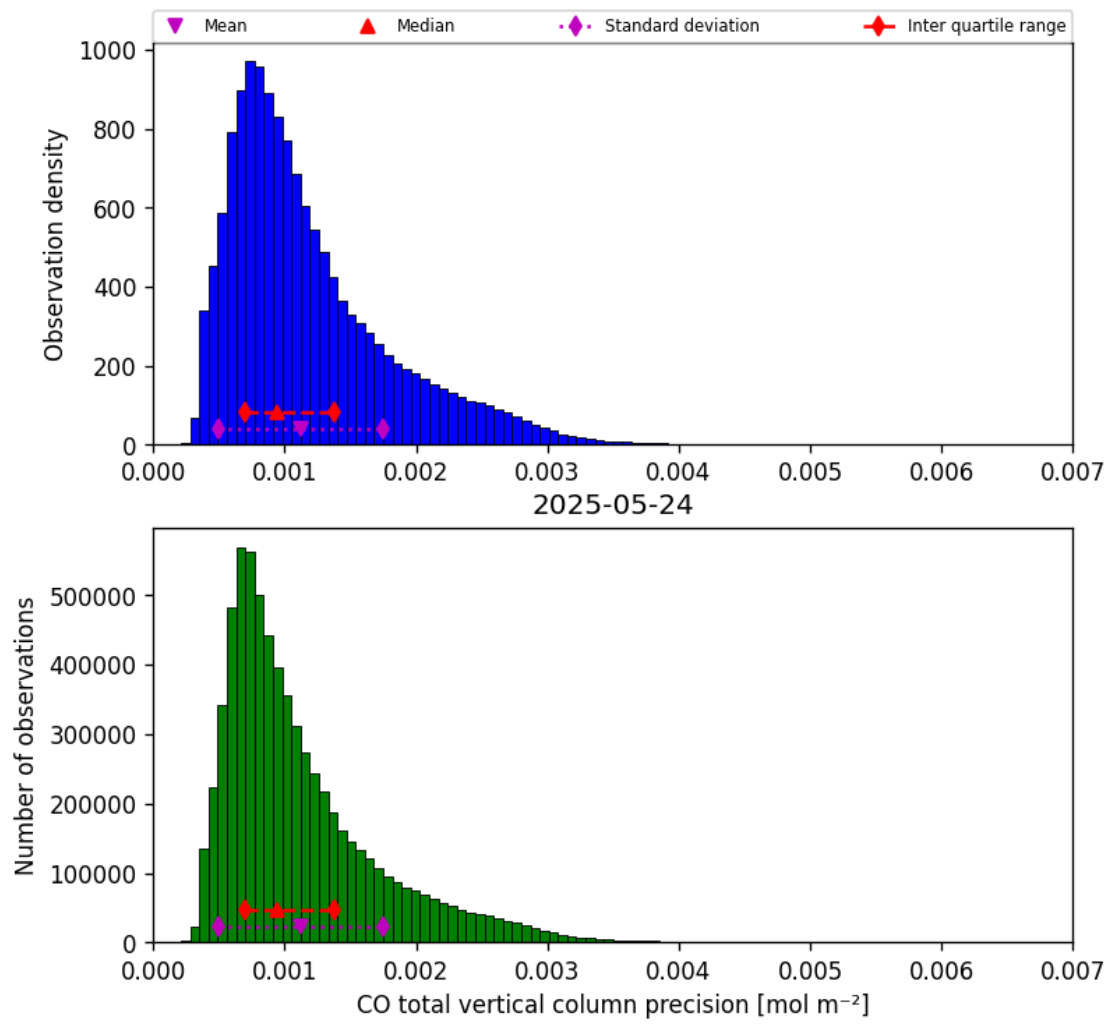
Figure 15: Histogram of “CO total vertical column precision” for 2025-05-24 to 2025-05-24
