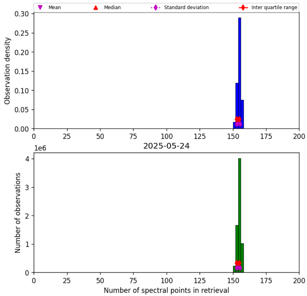
Figure 16: Histogram of “Number of spectral points in retrieval” for 2025-05-24 to 2025-05-24
