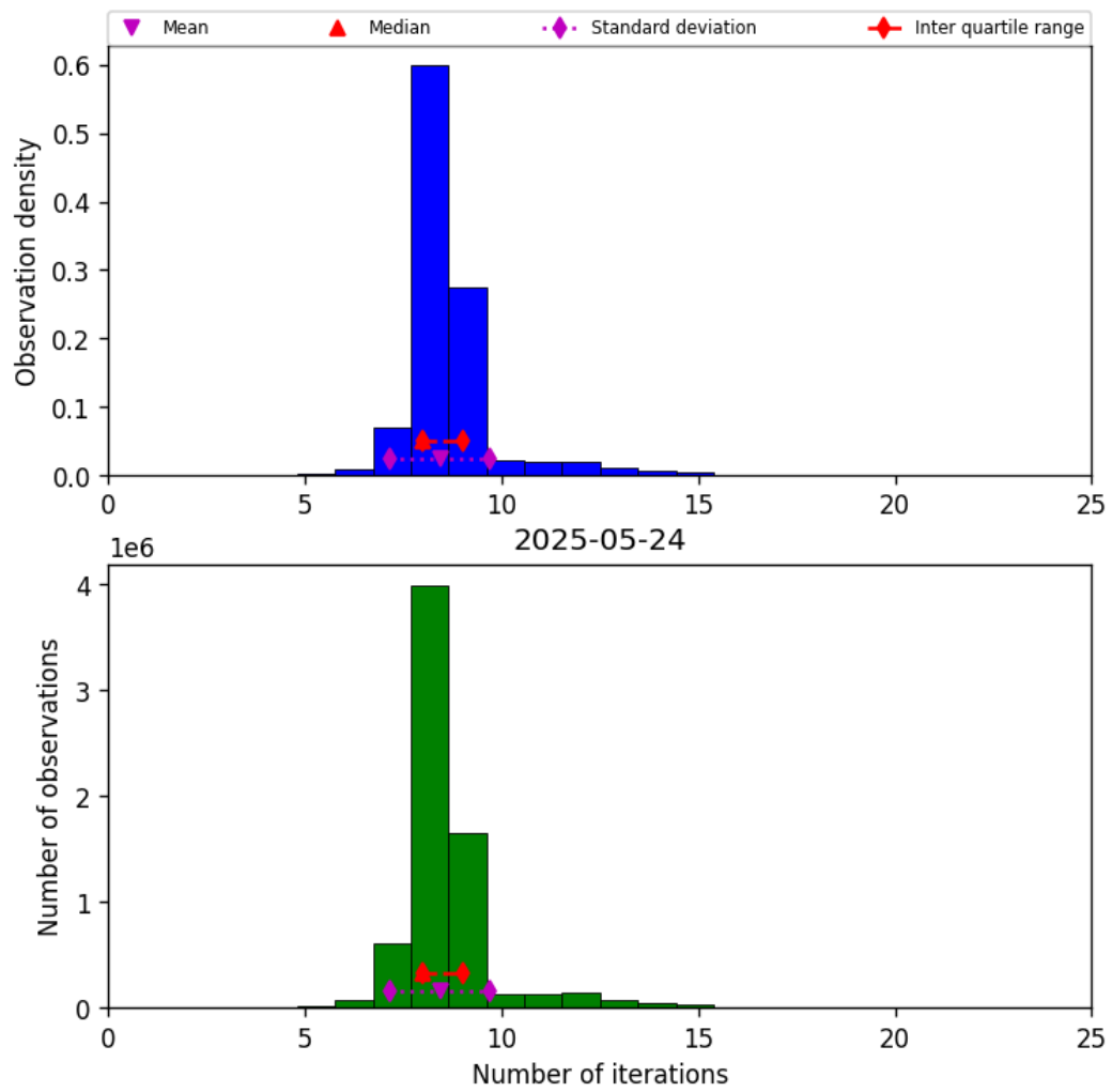
Figure 19: Histogram of “Number of iterations” for 2025-05-24 to 2025-05-24
