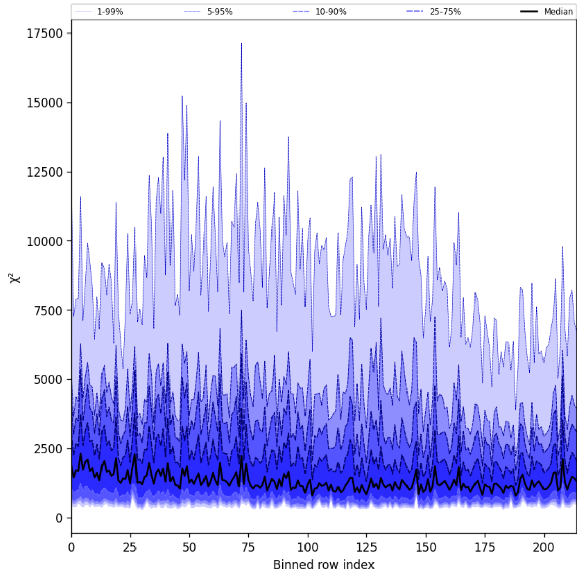
Figure 24: Along track statistics of “ \chi^2 ” for 2025-05-24 to 2025-05-24
