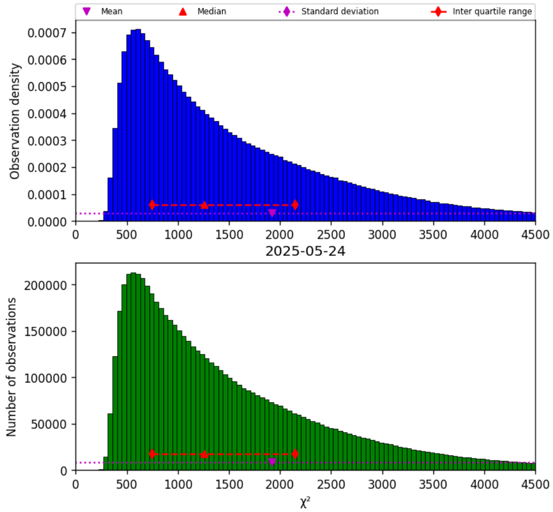
Figure 17: Histogram of " \chi^2 " for 2025-05-24 to 2025-05-24
