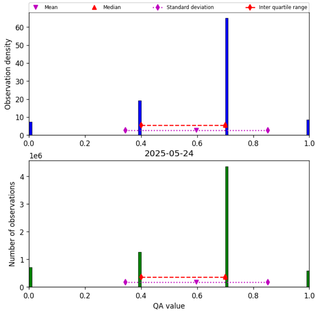
Figure 13: Histogram of “QA value” for 2025-05-24 to 2025-05-24
