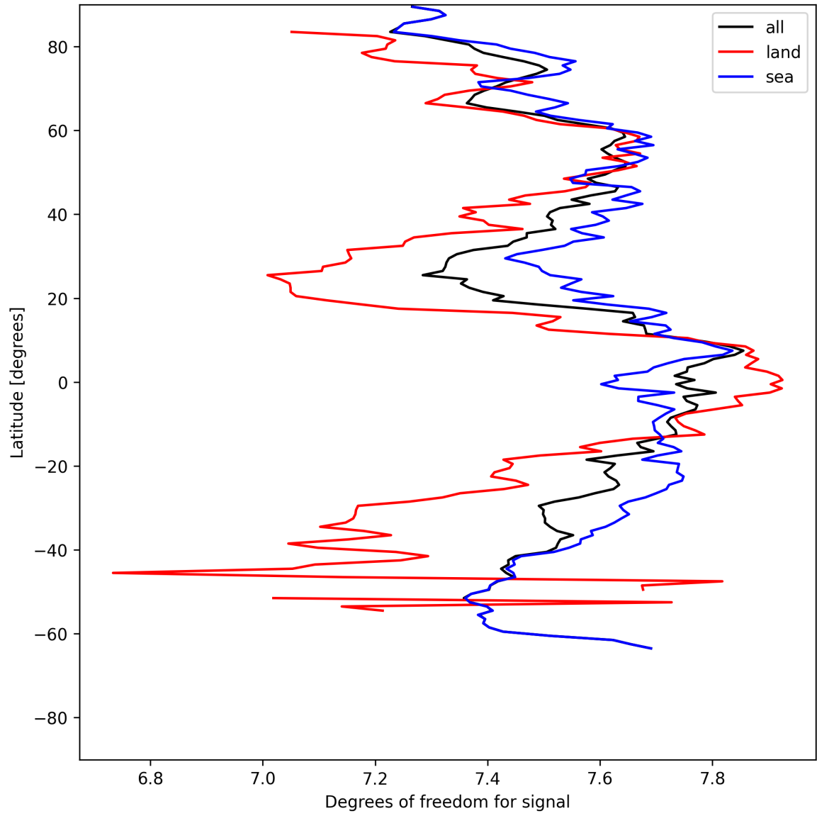
Figure 11: Zonal average of “Degrees of freedom for signal” for 2025-05-24 to 2025-05-24.
