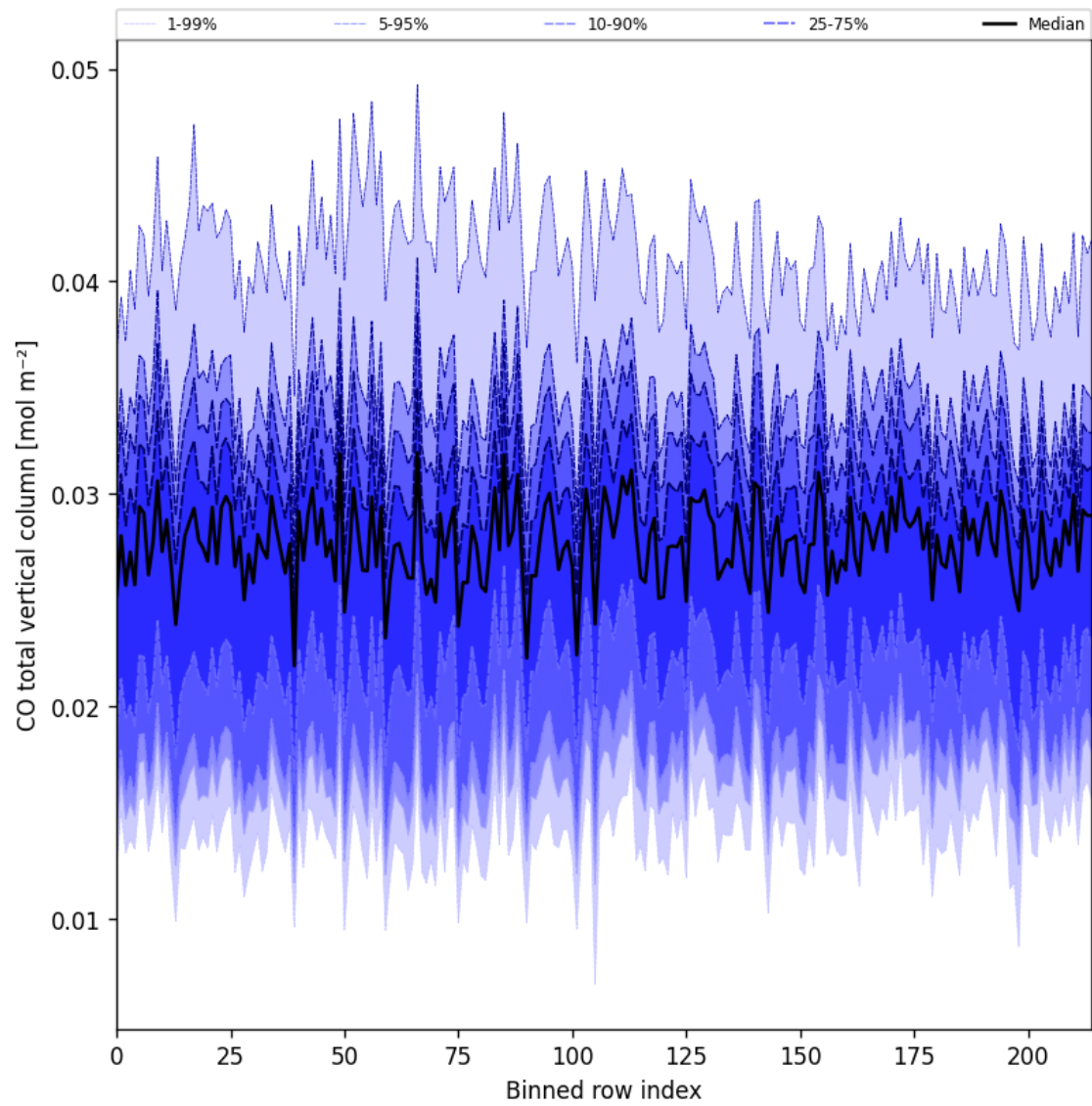
Figure 21: Along track statistics of “CO total vertical column” for 2025-05-24 to 2025-05-24
