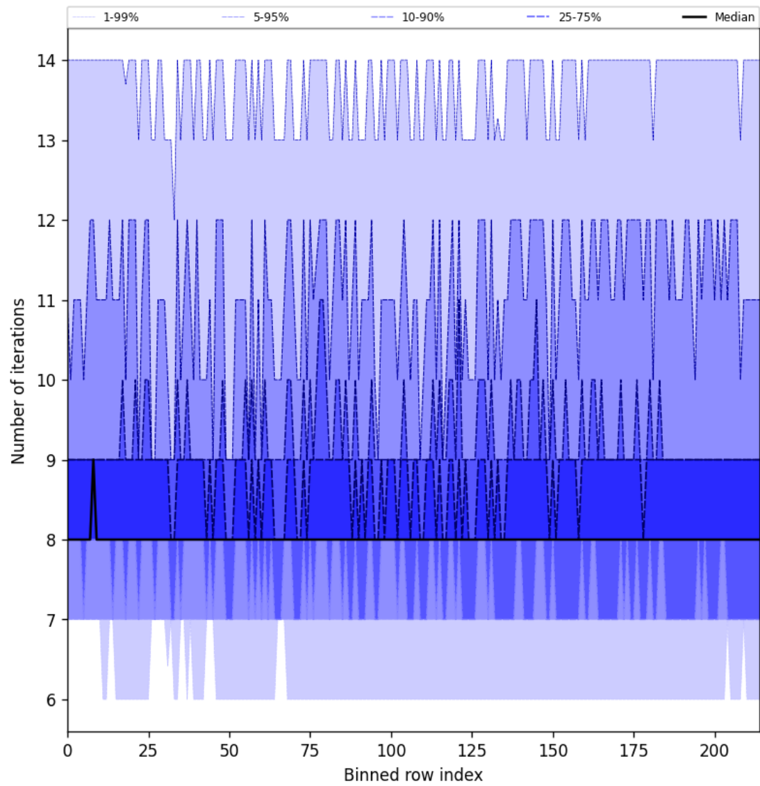
Figure 26: Along track statistics of “Number of iterations” for 2025-05-24 to 2025-05-24
