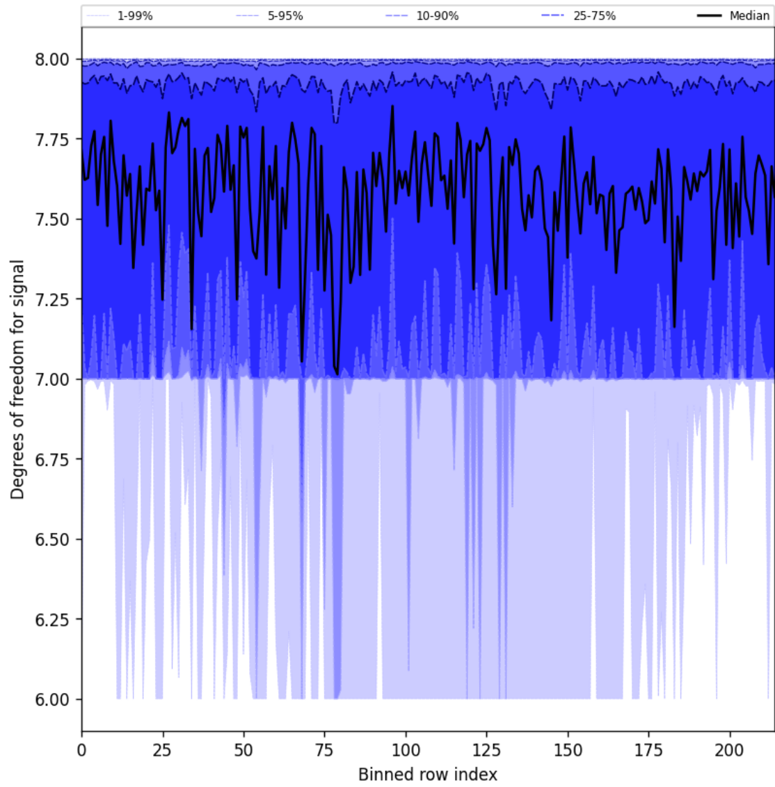
Figure 25: Along track statistics of “Degrees of freedom for signal” for 2025-05-24 to 2025-05-24
