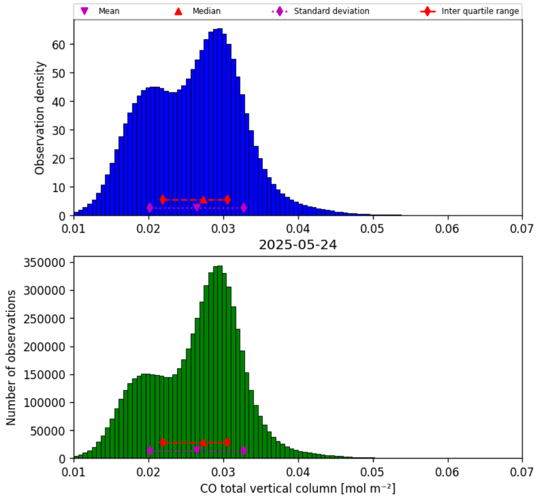
Figure 14: Histogram of “CO total vertical column” for 2025-05-24 to 2025-05-24
