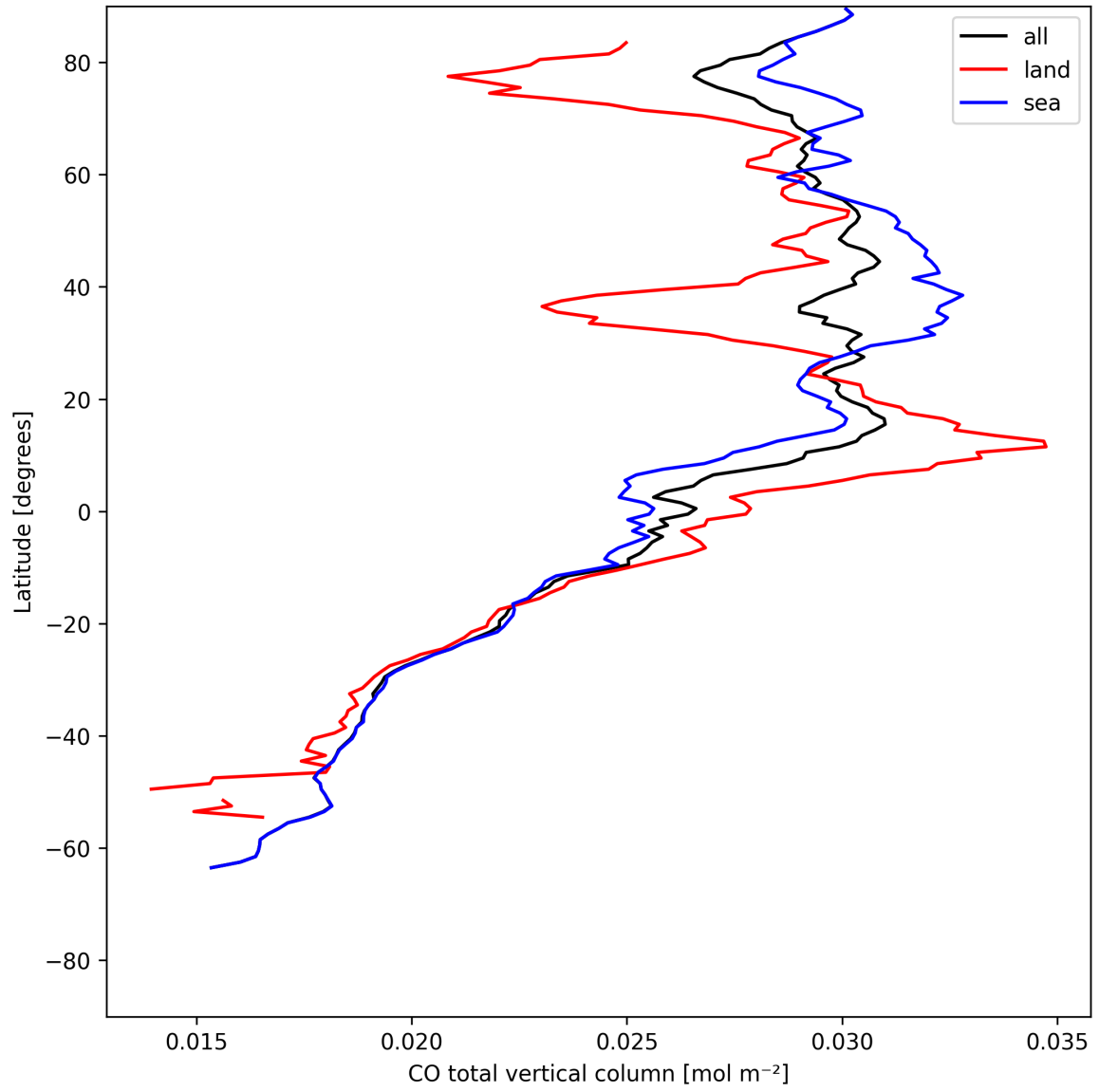
Figure 7: Zonal average of “CO total vertical column” for 2025-05-24 to 2025-05-24.
