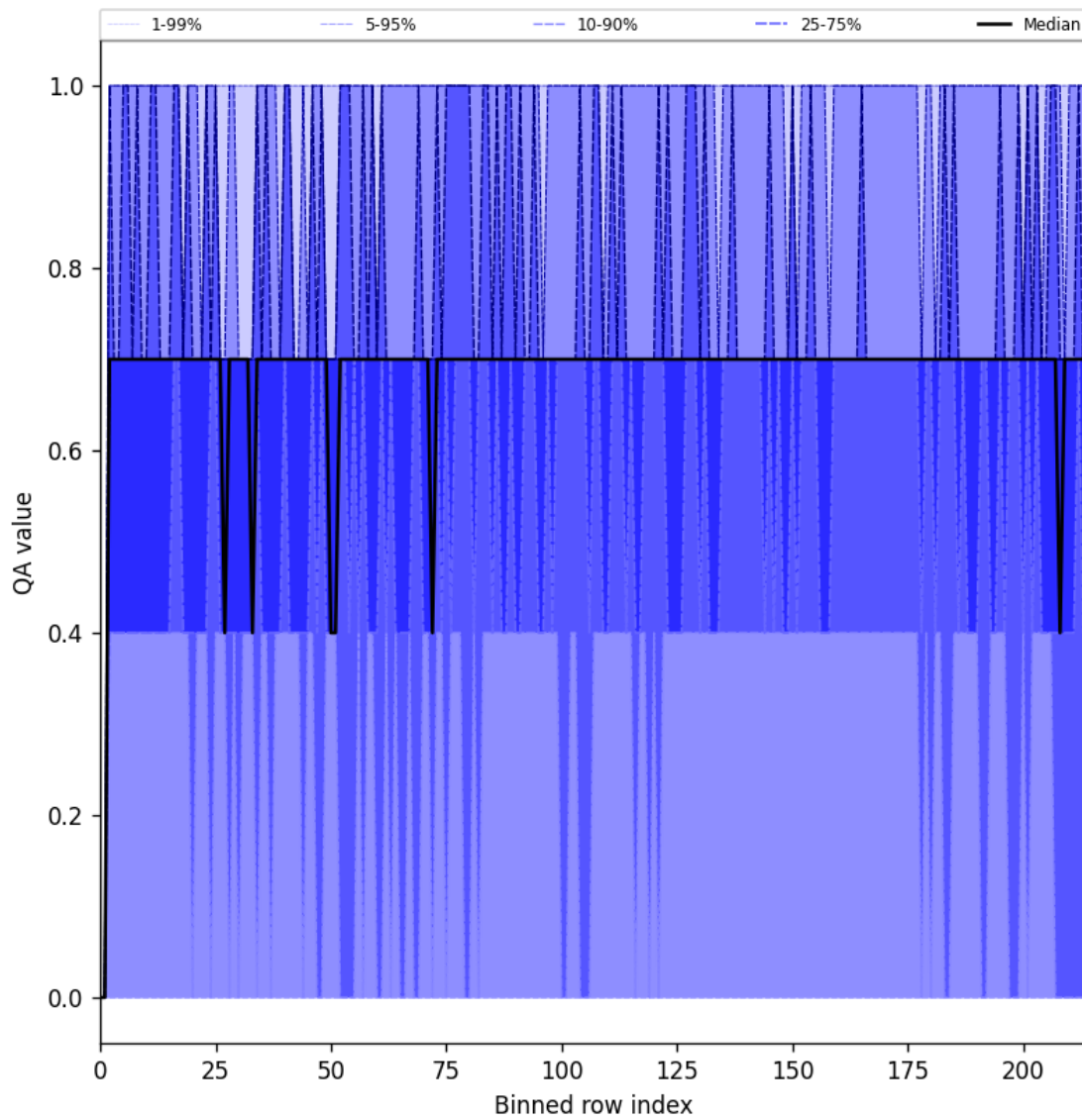
Figure 20: Along track statistics of “QA value” for 2025-05-24 to 2025-05-24
