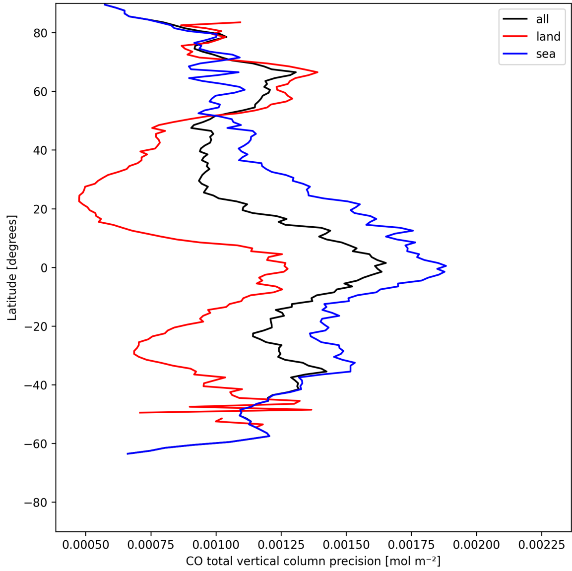
Figure 8: Zonal average of “CO total vertical column precision” for 2025-05-24 to 2025-05-24.
