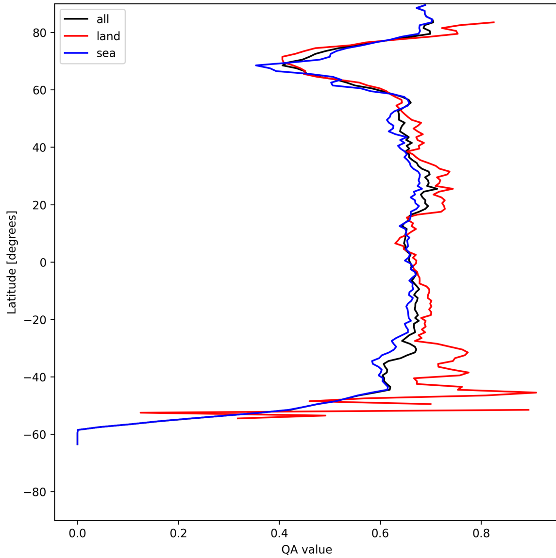
Figure 6: Zonal average of “QA value” for 2025-05-24 to 2025-05-24.
