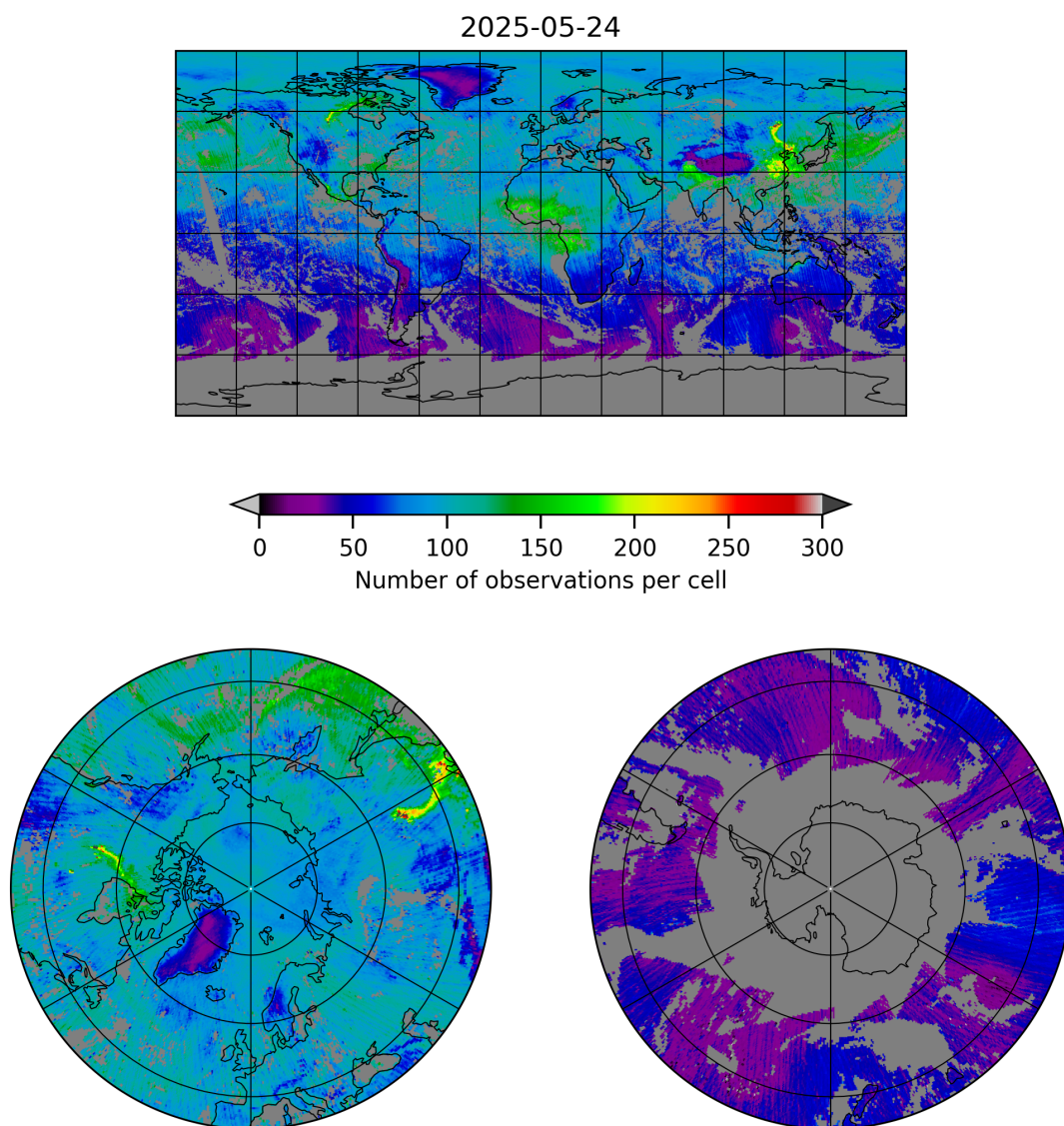
Figure 5: Map of the number of observations for 2025-05-24 to 2025-05-24
