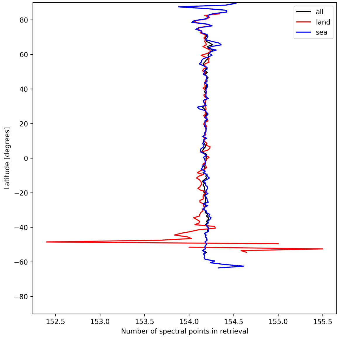
Figure 9: Zonal average of “Number of spectral points in retrieval” for 2025-05-24 to 2025-05-24.
