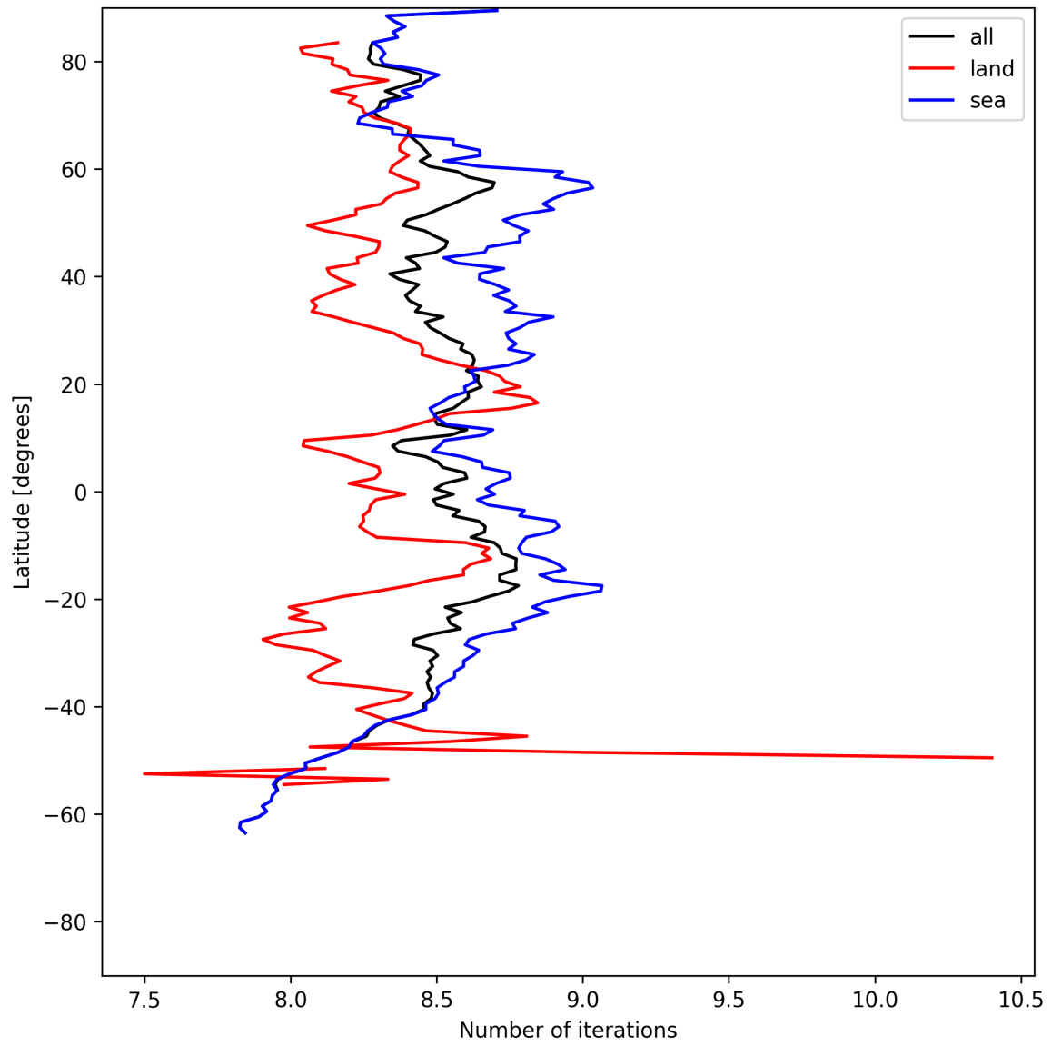
Figure 12: Zonal average of “Number of iterations” for 2025-05-24 to 2025-05-24.
