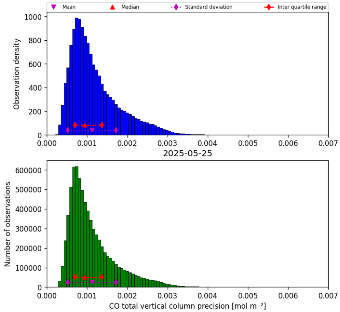
Figure 15: Histogram of “CO total vertical column precision” for 2025-05-25 to 2025-05-26
