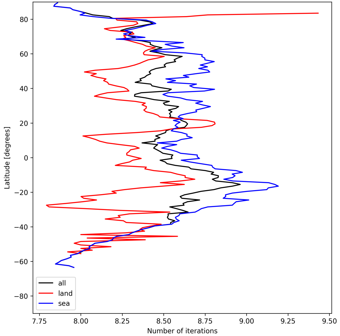
Figure 12: Zonal average of “Number of iterations” for 2025-05-25 to 2025-05-26.
