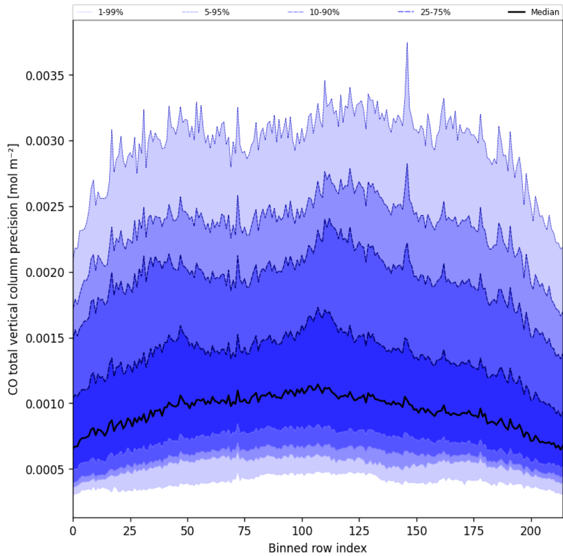
Figure 22: Along track statistics of "CO total vertical column precision" for 2025-05-25 to 2025-05-26
