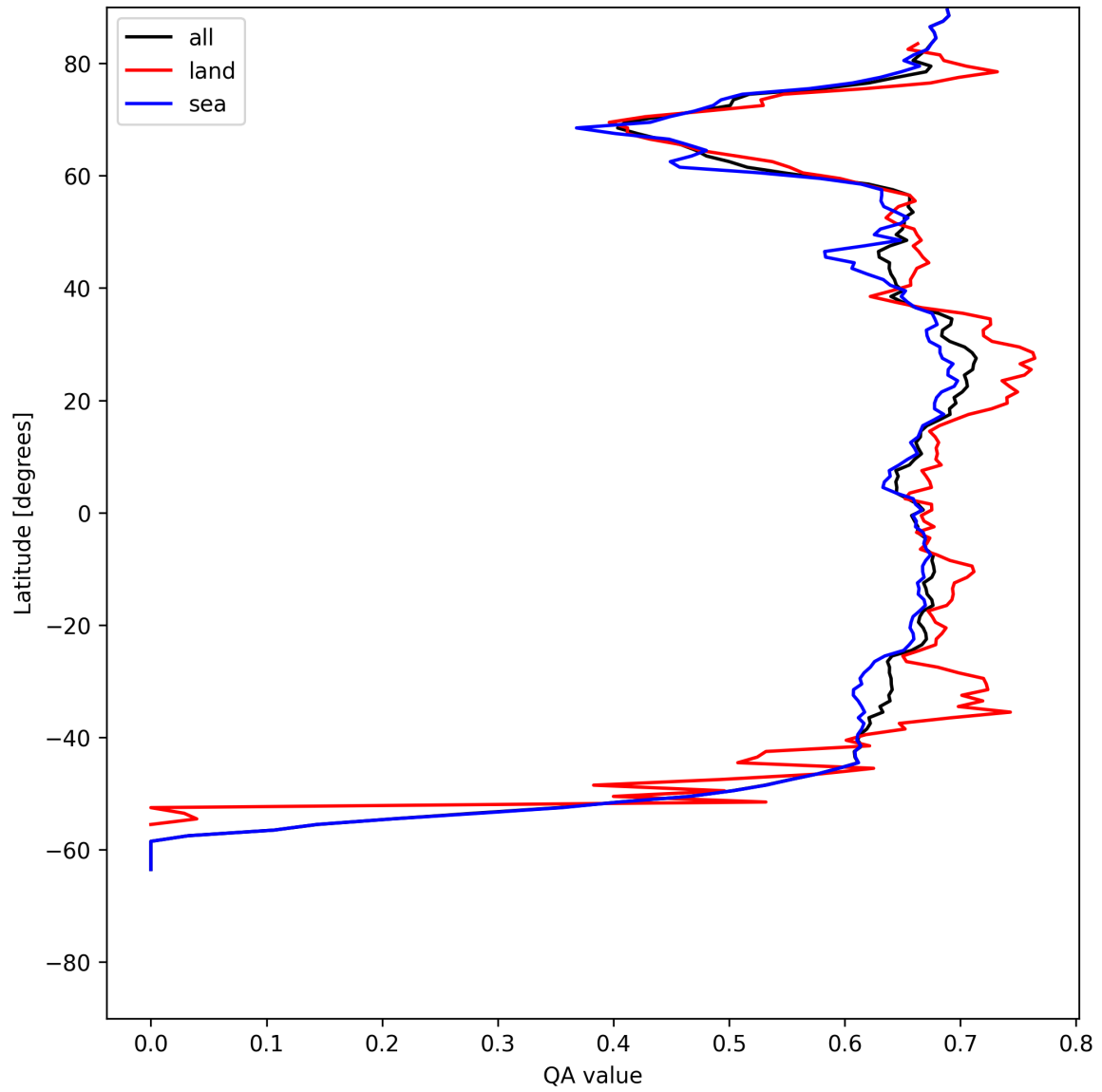
Figure 6: Zonal average of “QA value” for 2025-05-25 to 2025-05-26.
