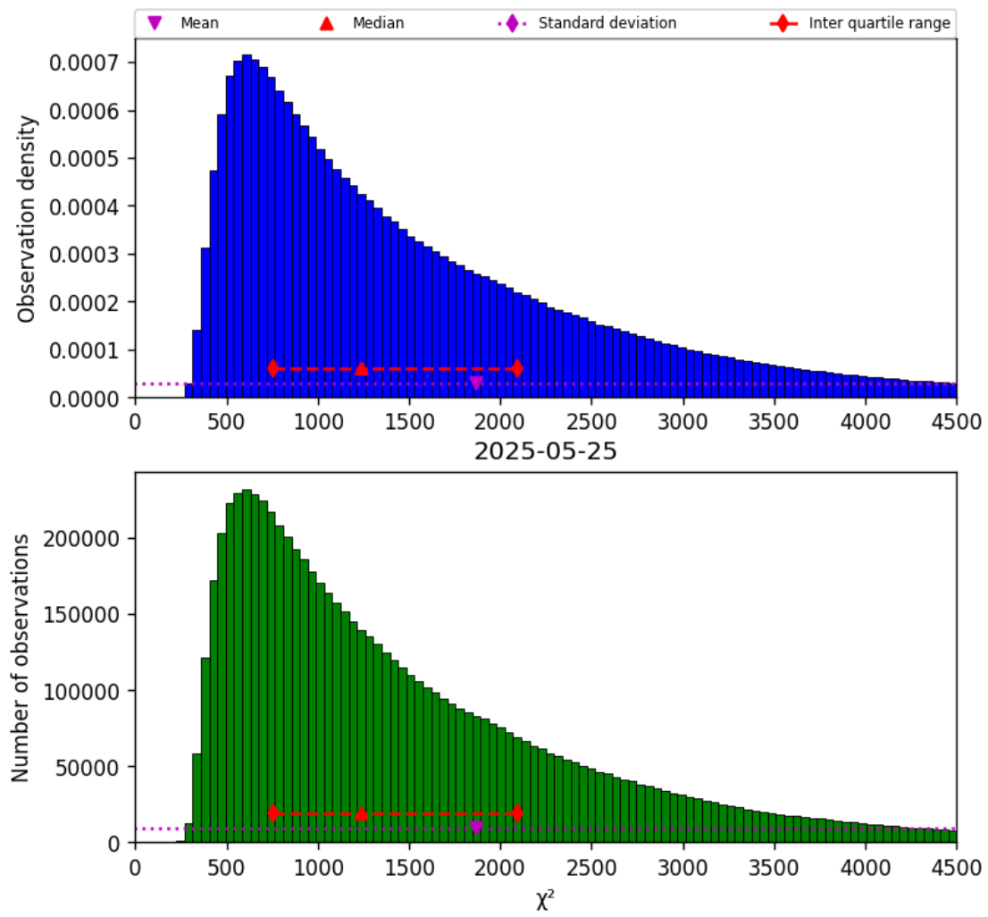
Figure 17: Histogram of “ \chi^2 ” for 2025-05-25 to 2025-05-26
