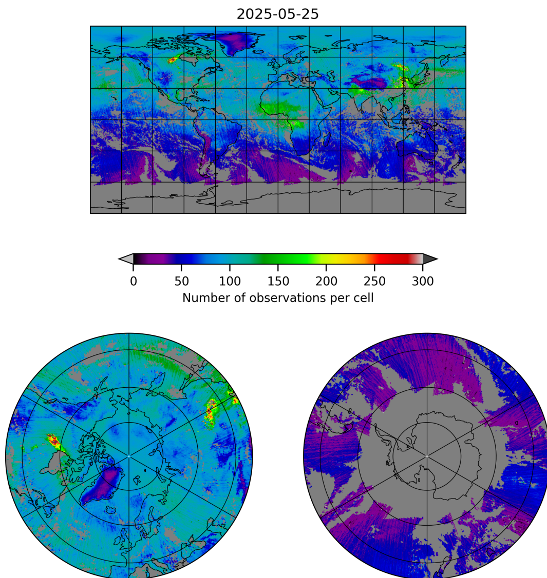
Figure 5: Map of the number of observations for 2025-05-25 to 2025-05-26
