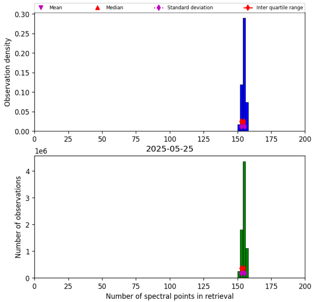
Figure 16: Histogram of “Number of spectral points in retrieval” for 2025-05-25 to 2025-05-26
