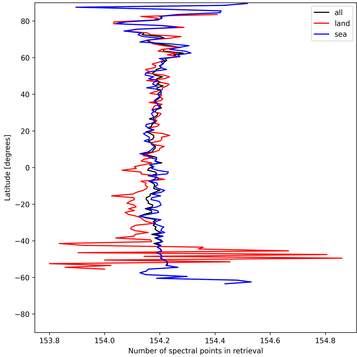
Figure 9: Zonal average of “Number of spectral points in retrieval” for 2025-05-25 to 2025-05-26.
