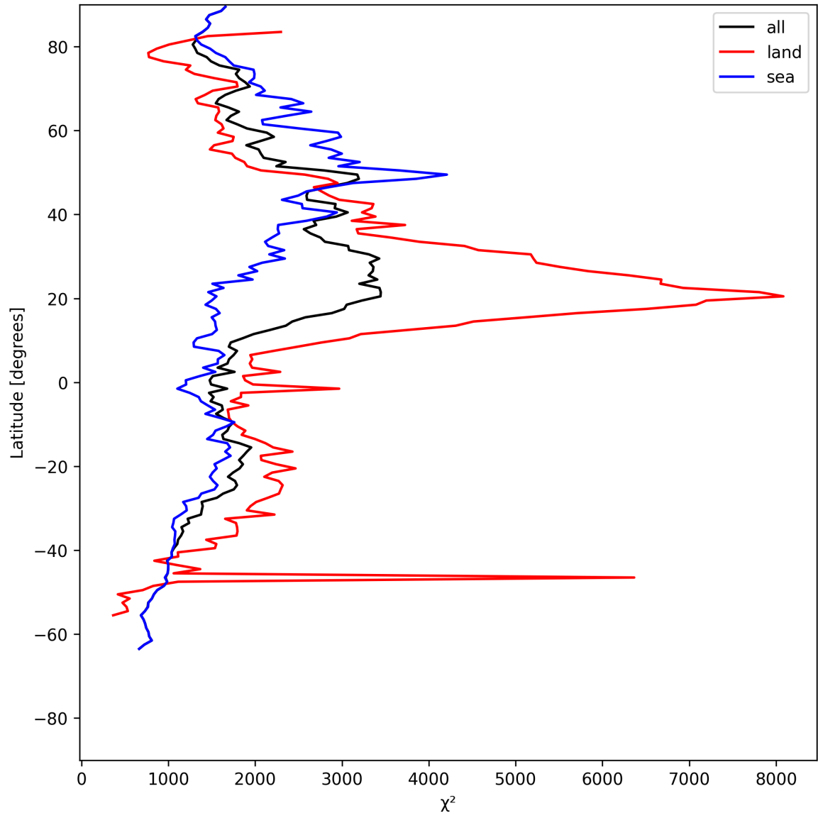
Figure 10: Zonal average of “ \chi^2 ” for 2025-05-25 to 2025-05-26.
