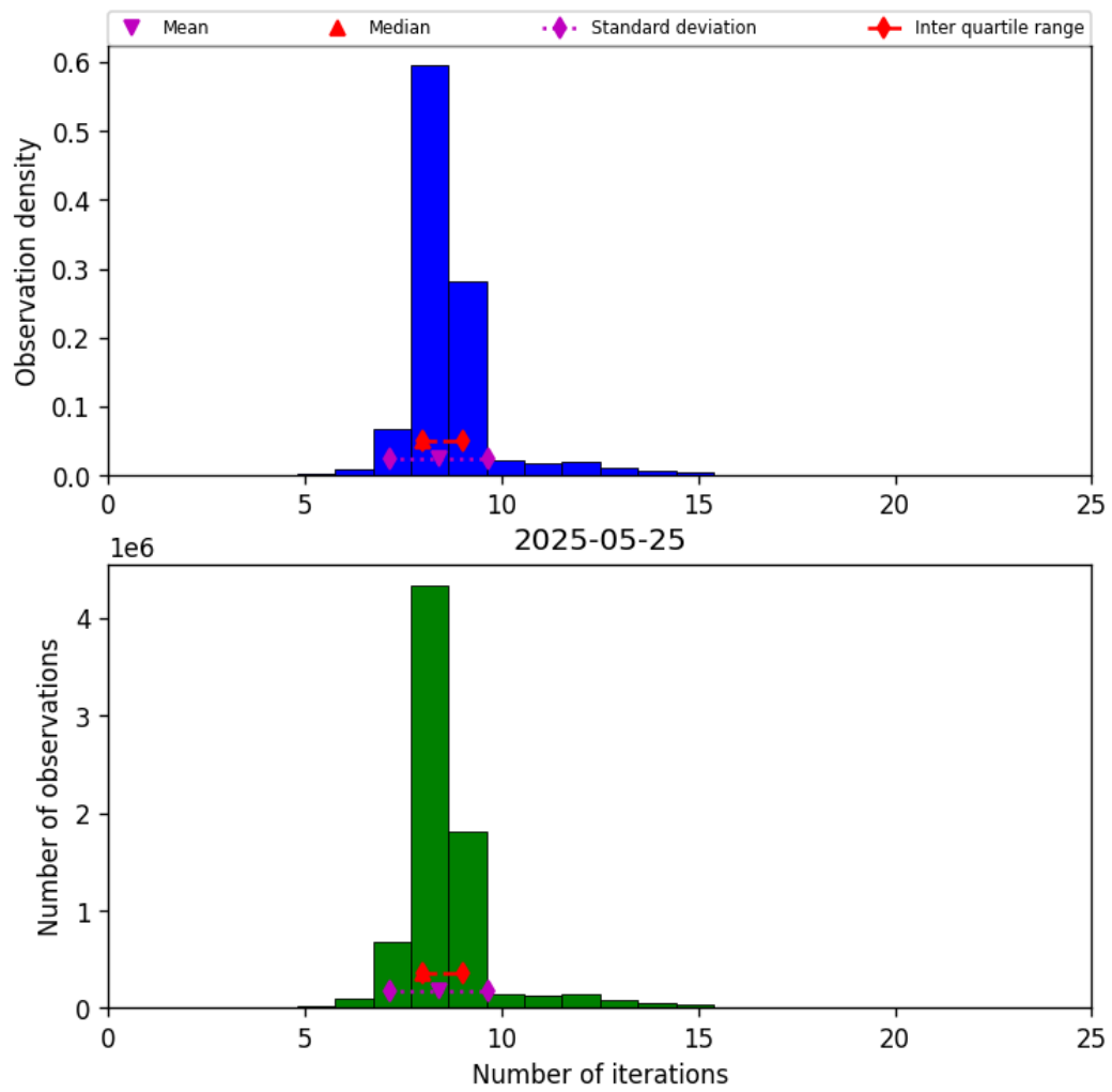
Figure 19: Histogram of “Number of iterations” for 2025-05-25 to 2025-05-26
