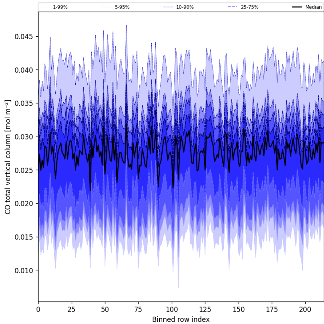
Figure 21: Along track statistics of “CO total vertical column” for 2025-05-25 to 2025-05-26
