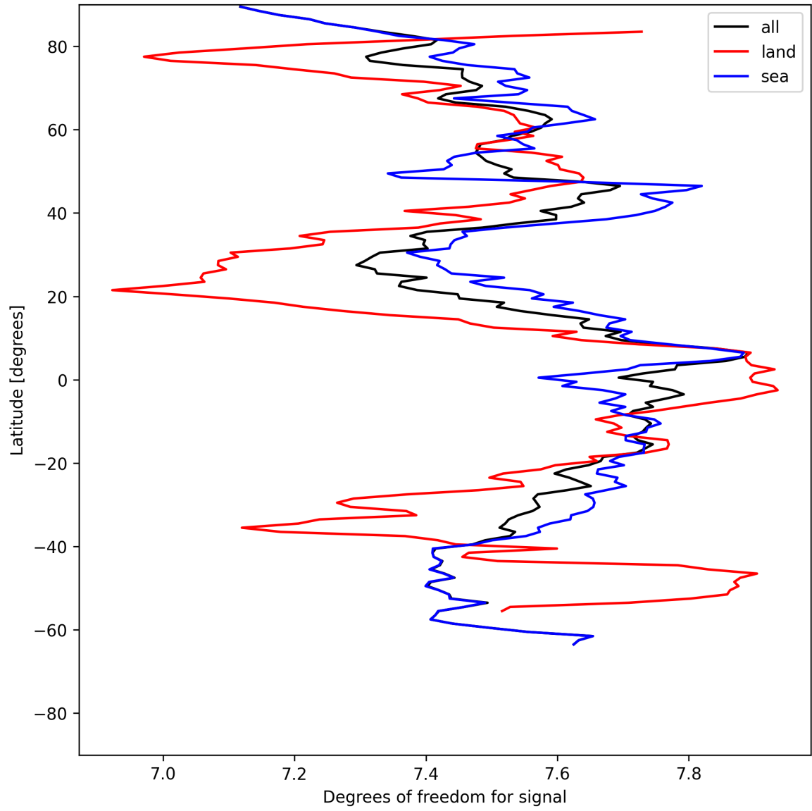
Figure 11: Zonal average of “Degrees of freedom for signal” for 2025-05-25 to 2025-05-26.
