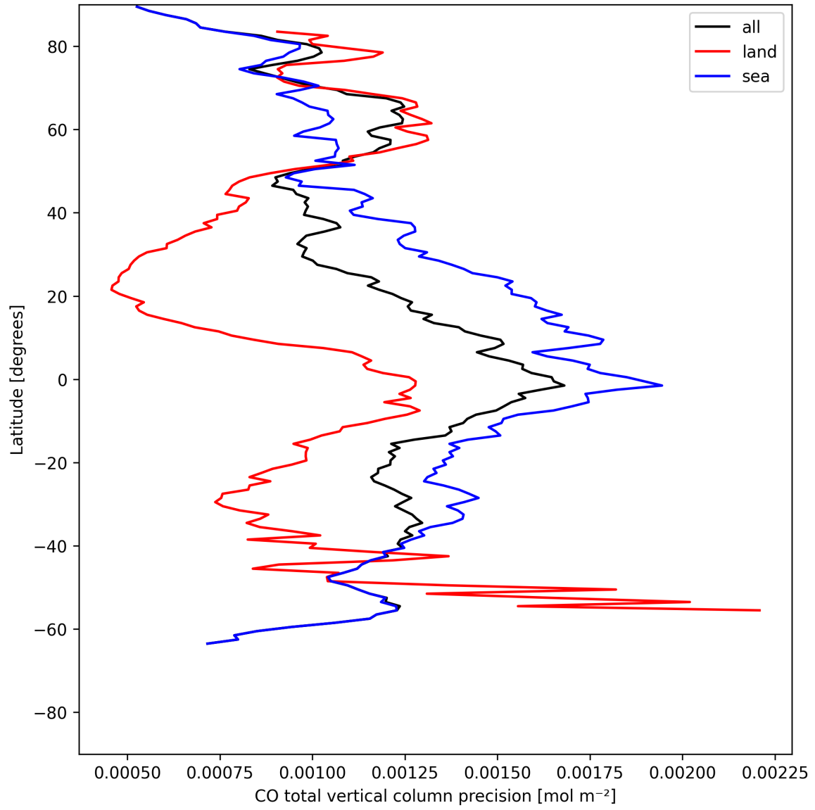
Figure 8: Zonal average of “CO total vertical column precision” for 2025-05-25 to 2025-05-26.
