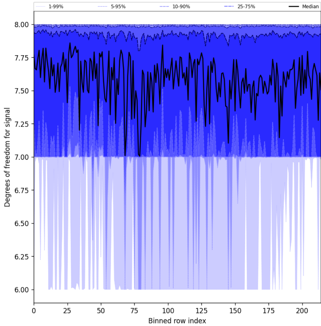
Figure 25: Along track statistics of “Degrees of freedom for signal” for 2025-05-25 to 2025-05-26
