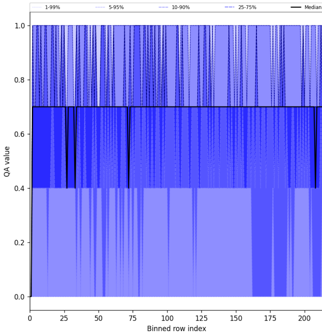
Figure 20: Along track statistics of “QA value” for 2025-05-25 to 2025-05-26
