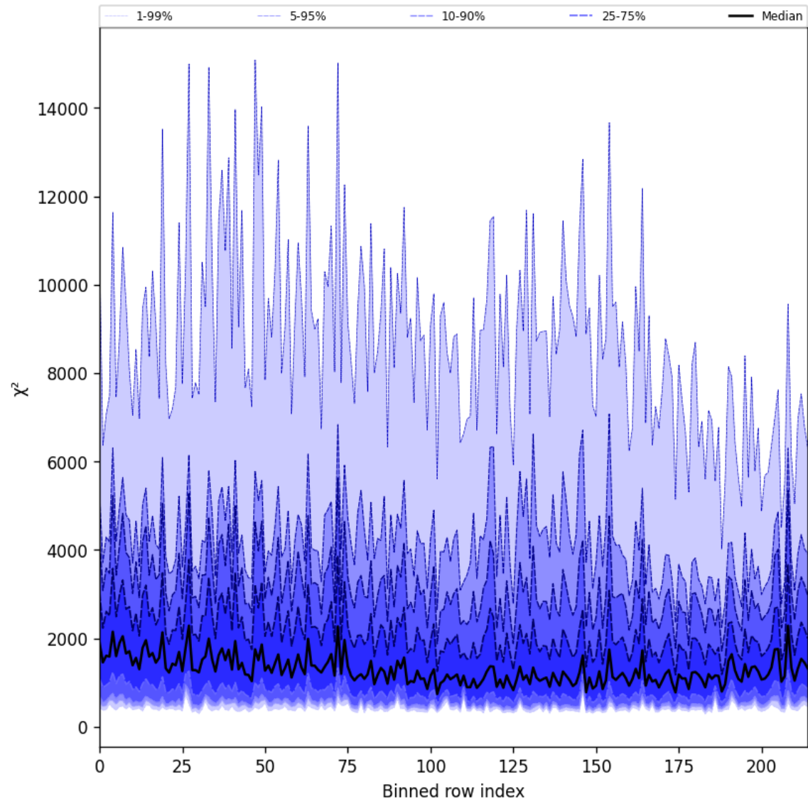
Figure 24: Along track statistics of “ \chi^2 ” for 2025-05-25 to 2025-05-26
