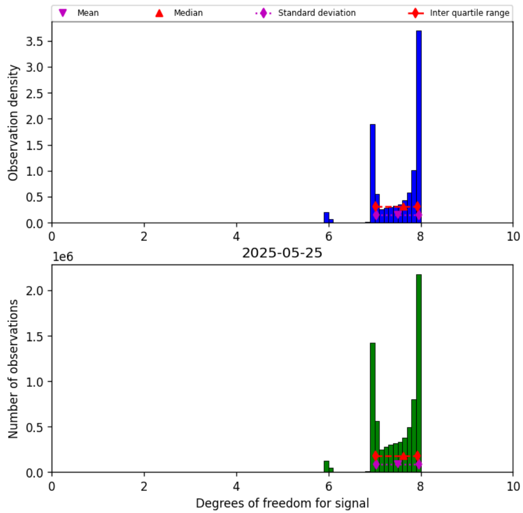
Figure 18: Histogram of “Degrees of freedom for signal” for 2025-05-25 to 2025-05-26
