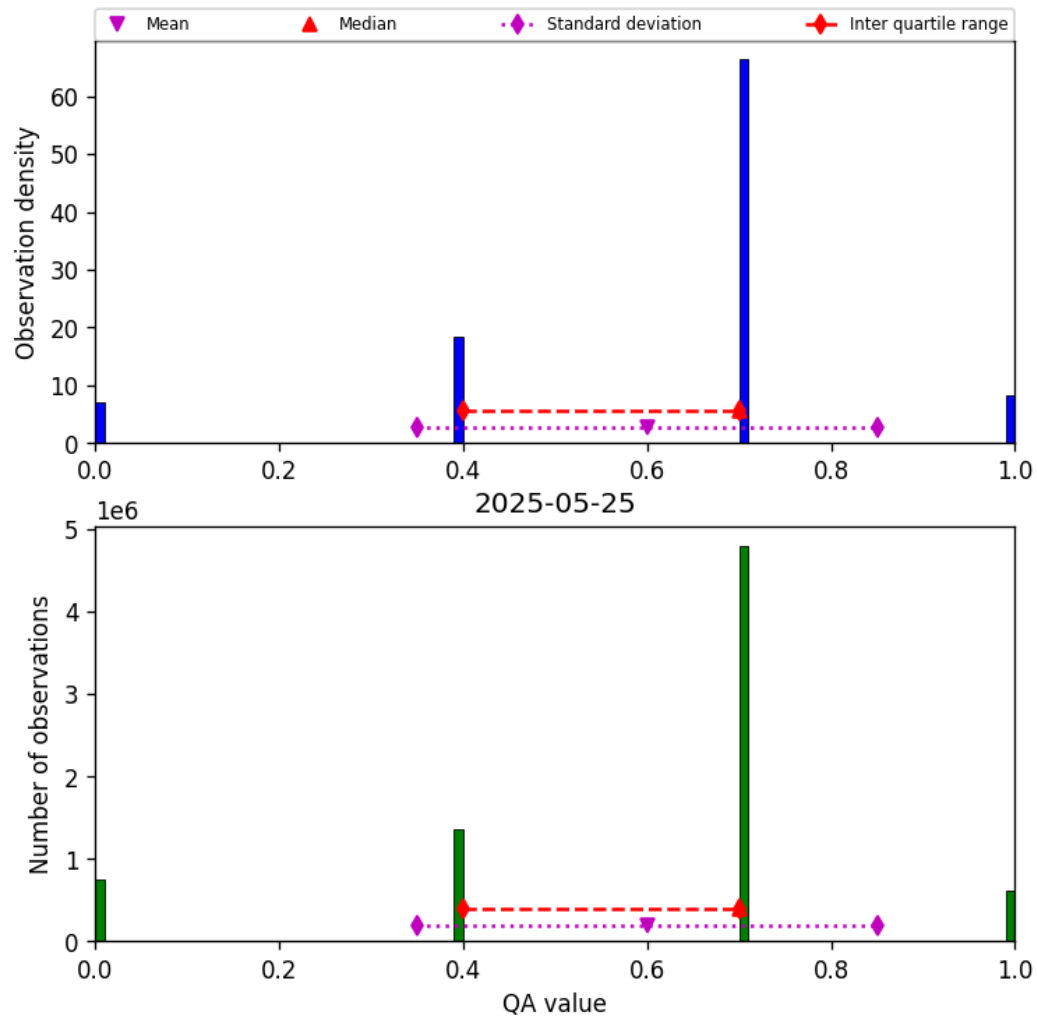
Figure 13: Histogram of “QA value” for 2025-05-25 to 2025-05-26
