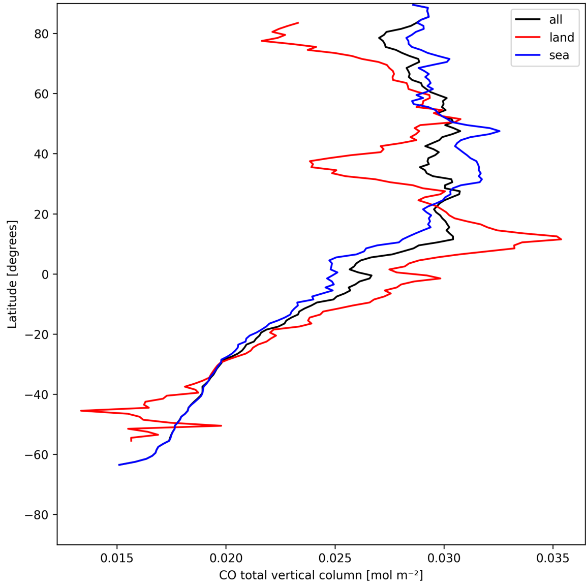
Figure 7: Zonal average of “CO total vertical column” for 2025-05-25 to 2025-05-26.
