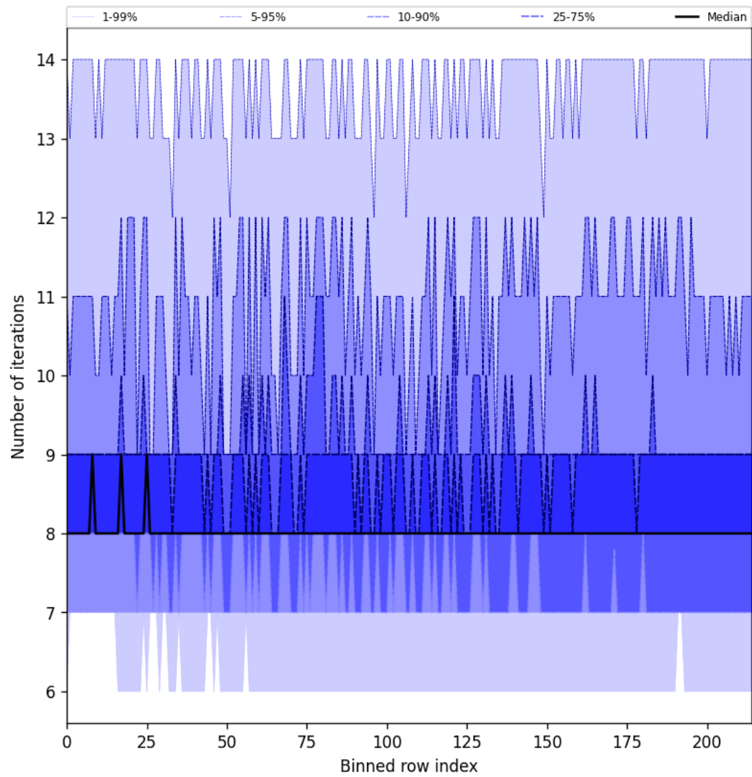
Figure 26: Along track statistics of “Number of iterations” for 2025-05-25 to 2025-05-26
