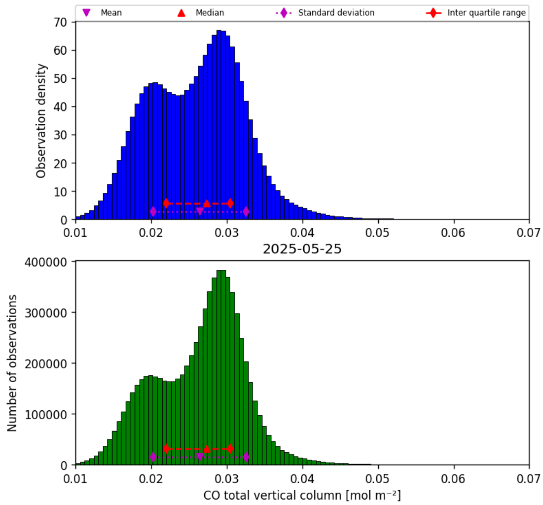
Figure 14: Histogram of “CO total vertical column” for 2025-05-25 to 2025-05-26
