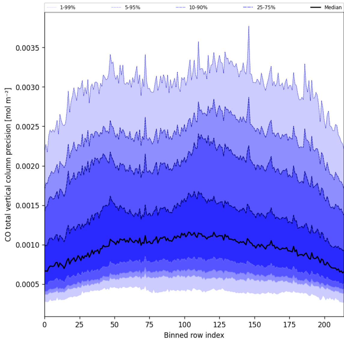
Figure 22: Along track statistics of “CO total vertical column precision” for 2025-05-26 to 2025-05-27
