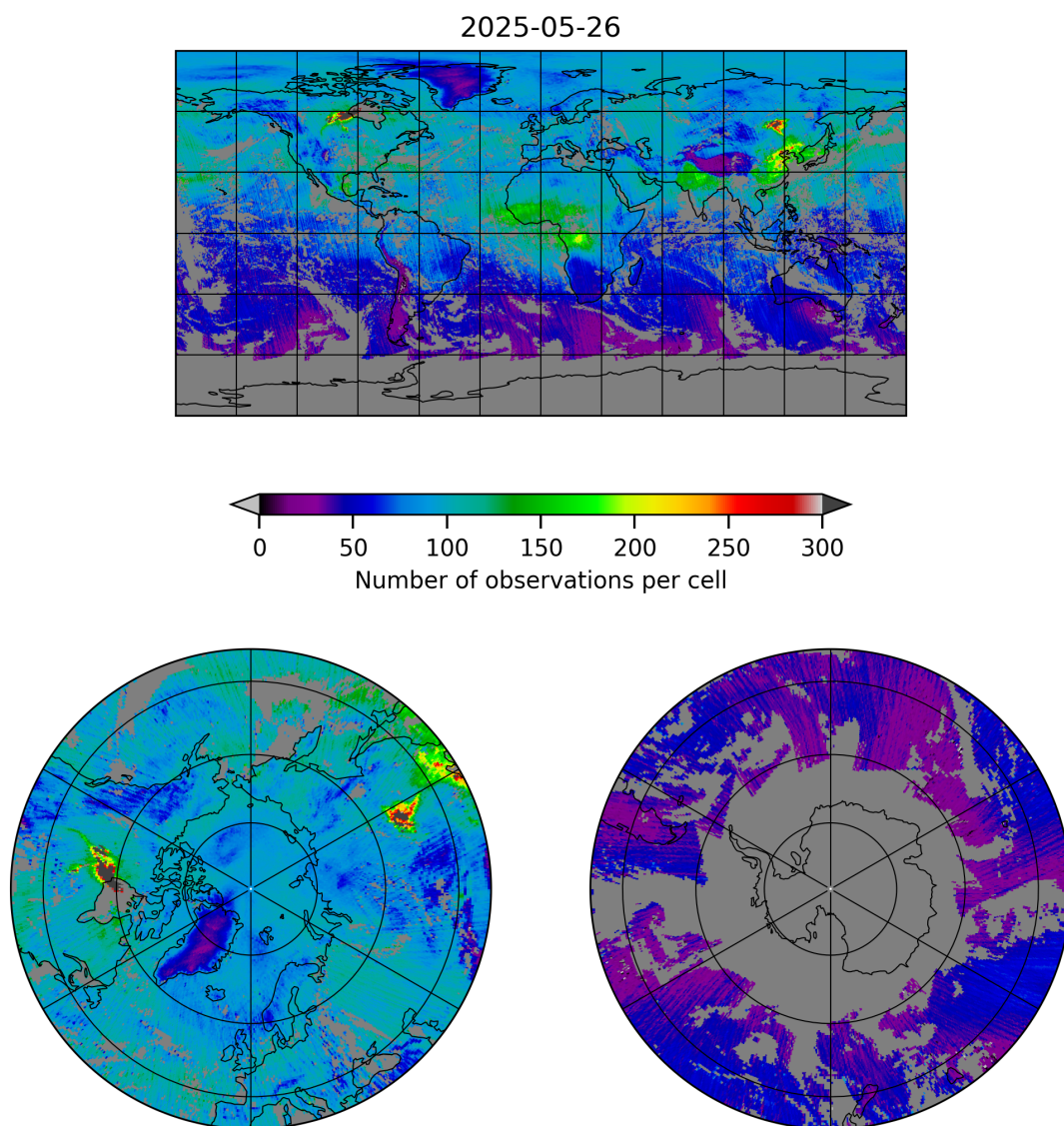
Figure 5: Map of the number of observations for 2025-05-26 to 2025-05-27
