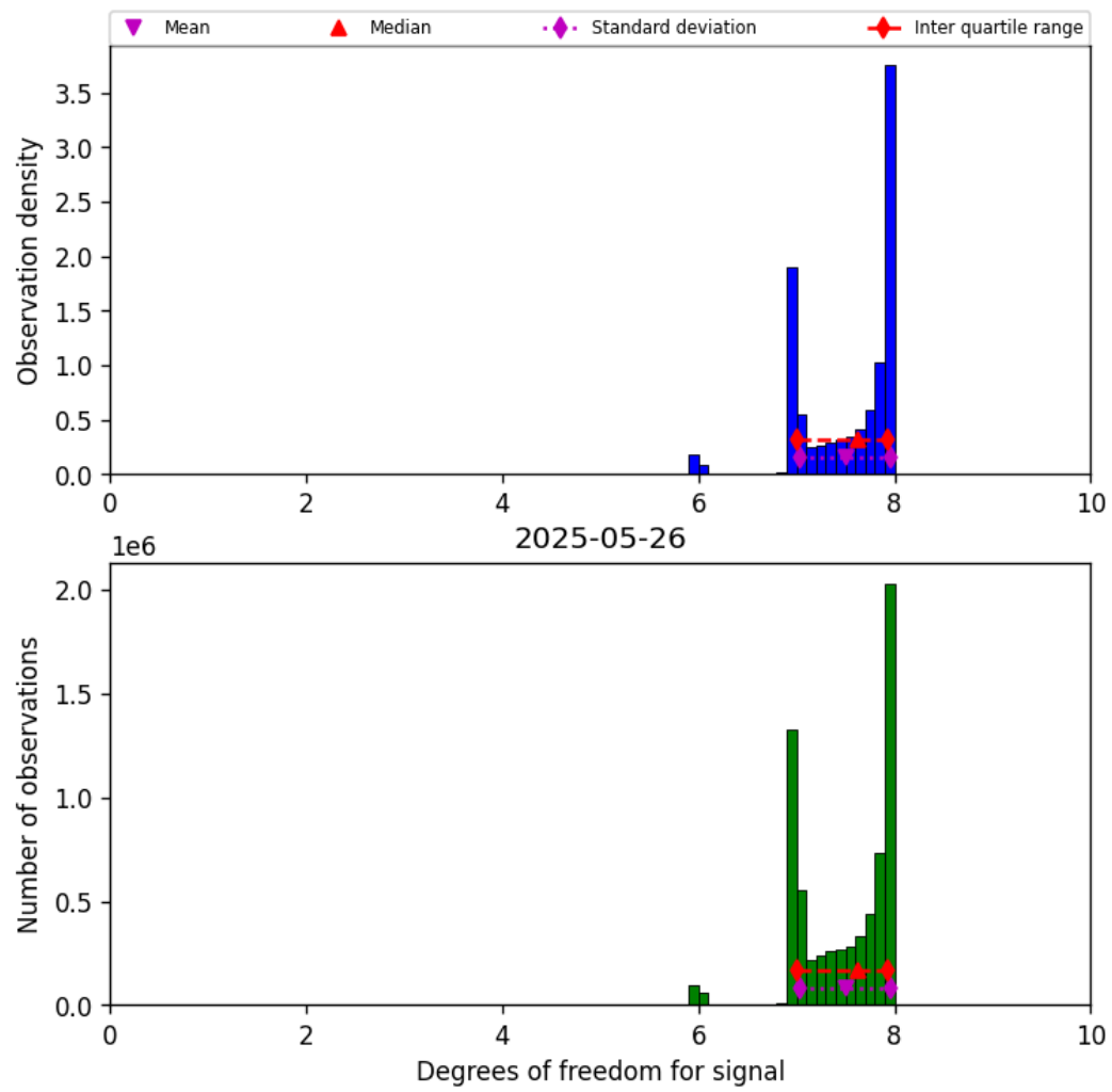
Figure 18: Histogram of “Degrees of freedom for signal” for 2025-05-26 to 2025-05-27
