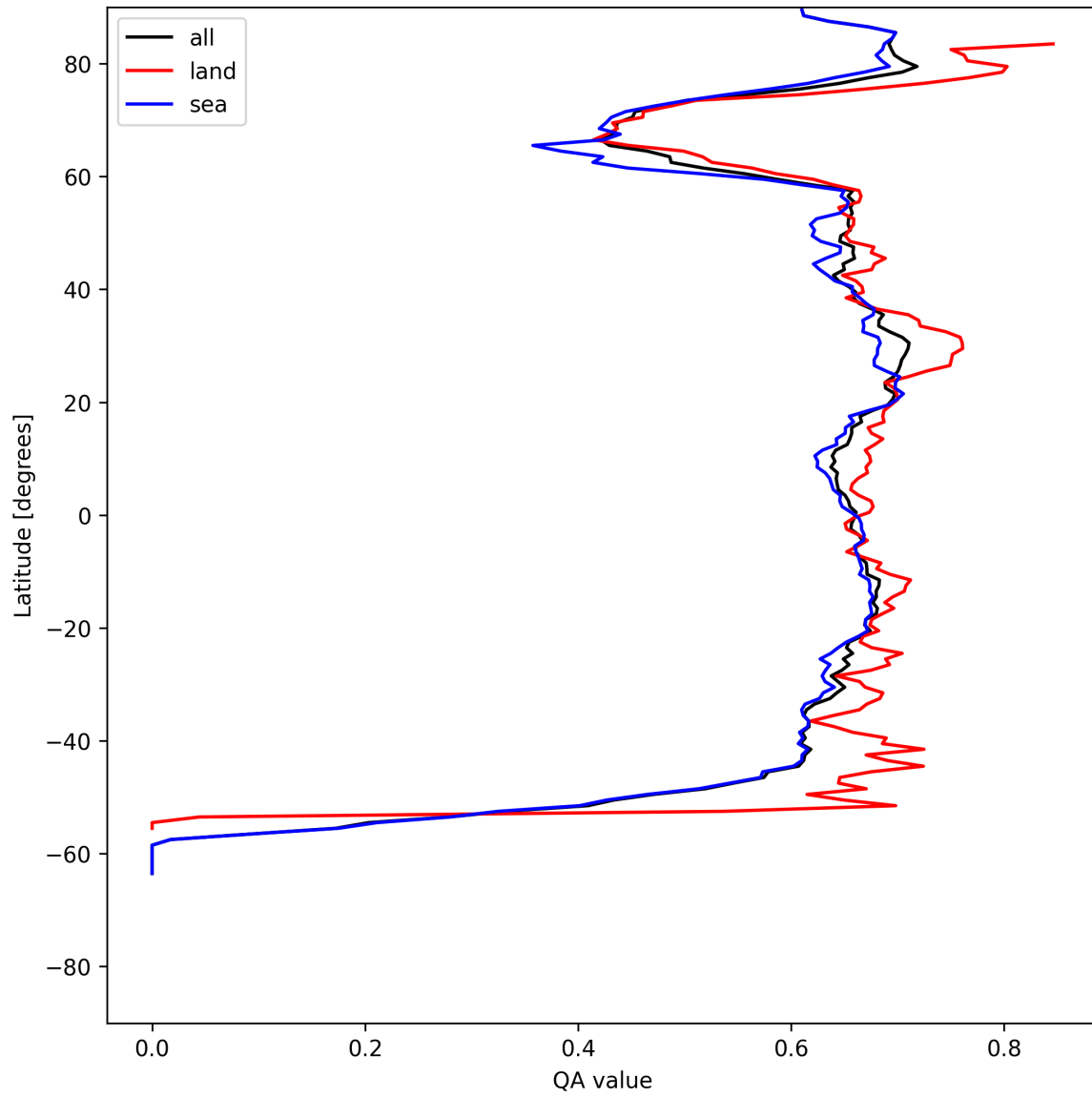
Figure 6: Zonal average of “QA value” for 2025-05-26 to 2025-05-27.
