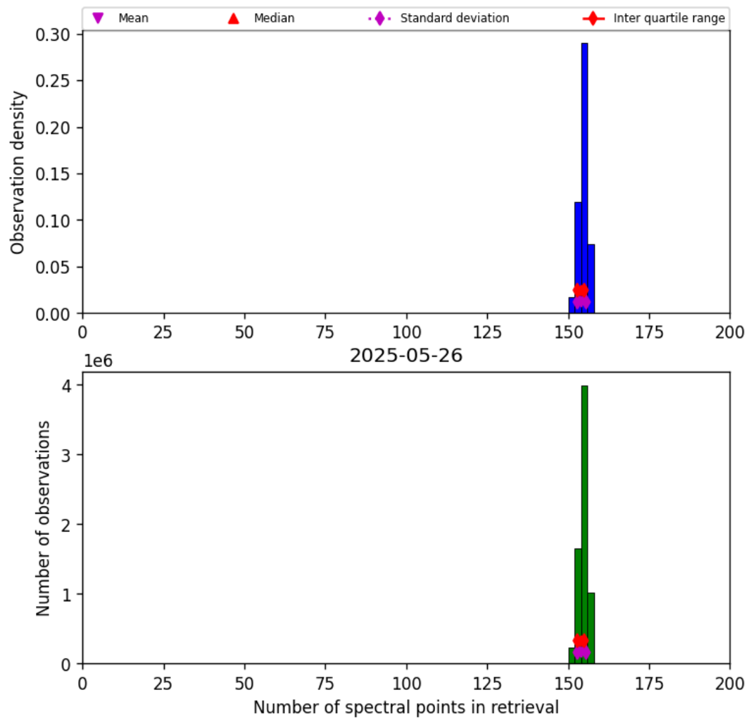
Figure 16: Histogram of "Number of spectral points in retrieval" for 2025-05-26 to 2025-05-27
