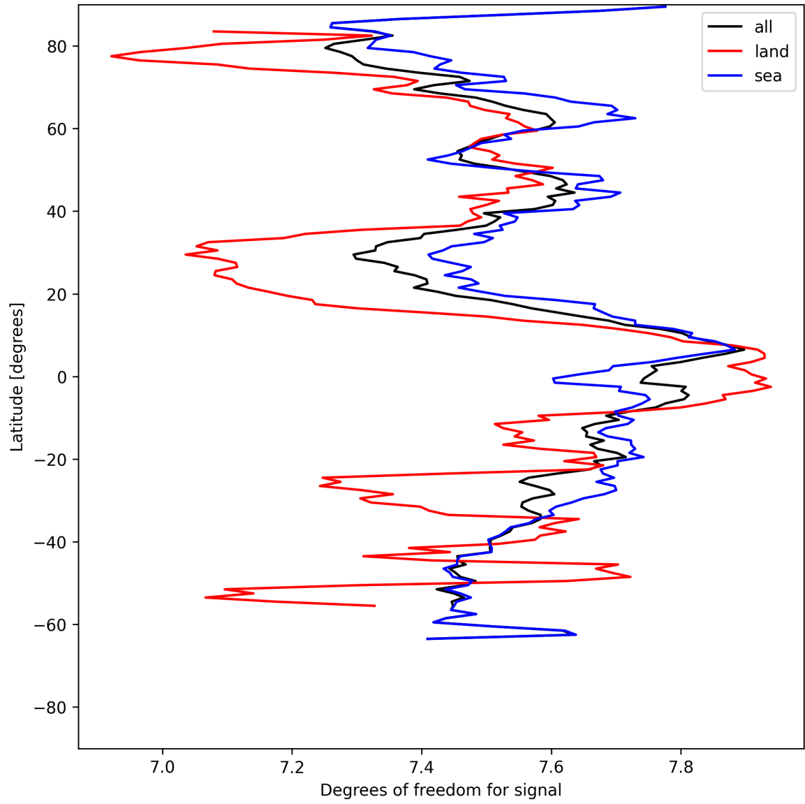
Figure 11: Zonal average of “Degrees of freedom for signal” for 2025-05-26 to 2025-05-27.
