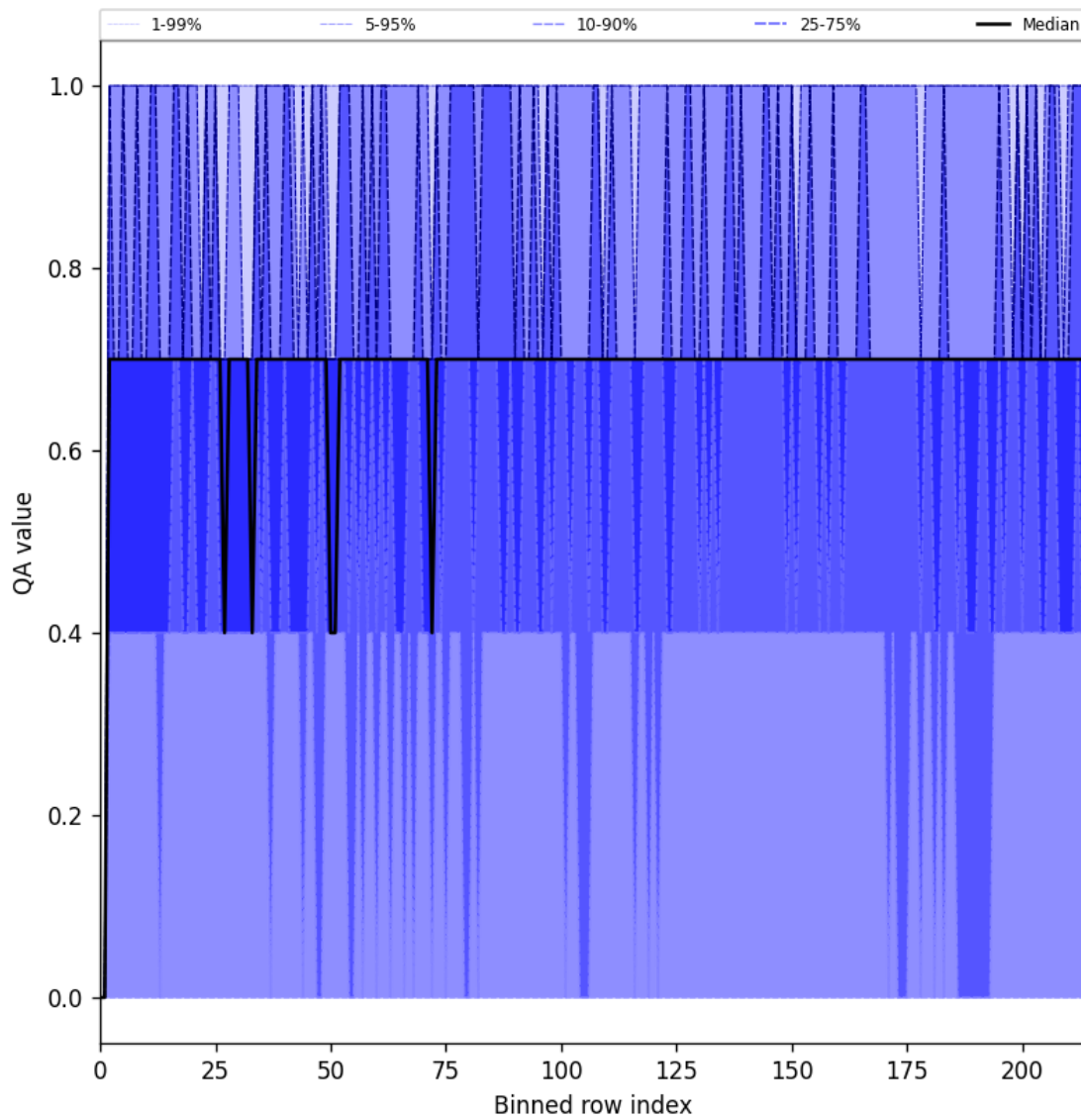
Figure 20: Along track statistics of “QA value” for 2025-05-26 to 2025-05-27
