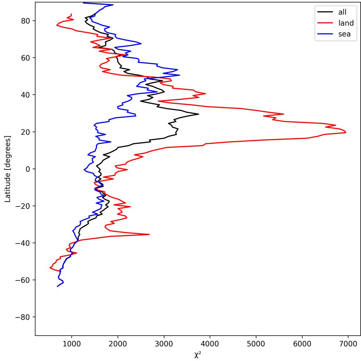
Figure 10: Zonal average of “ \chi^2 ” for 2025-05-26 to 2025-05-27.
