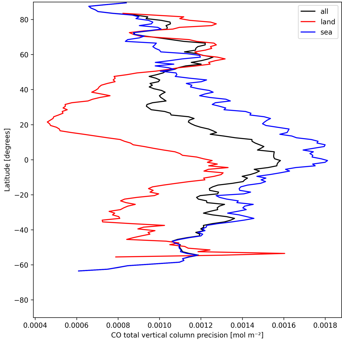
Figure 8: Zonal average of “CO total vertical column precision” for 2025-05-26 to 2025-05-27.
