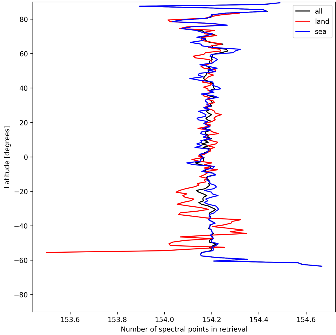
Figure 9: Zonal average of “Number of spectral points in retrieval” for 2025-05-26 to 2025-05-27.
