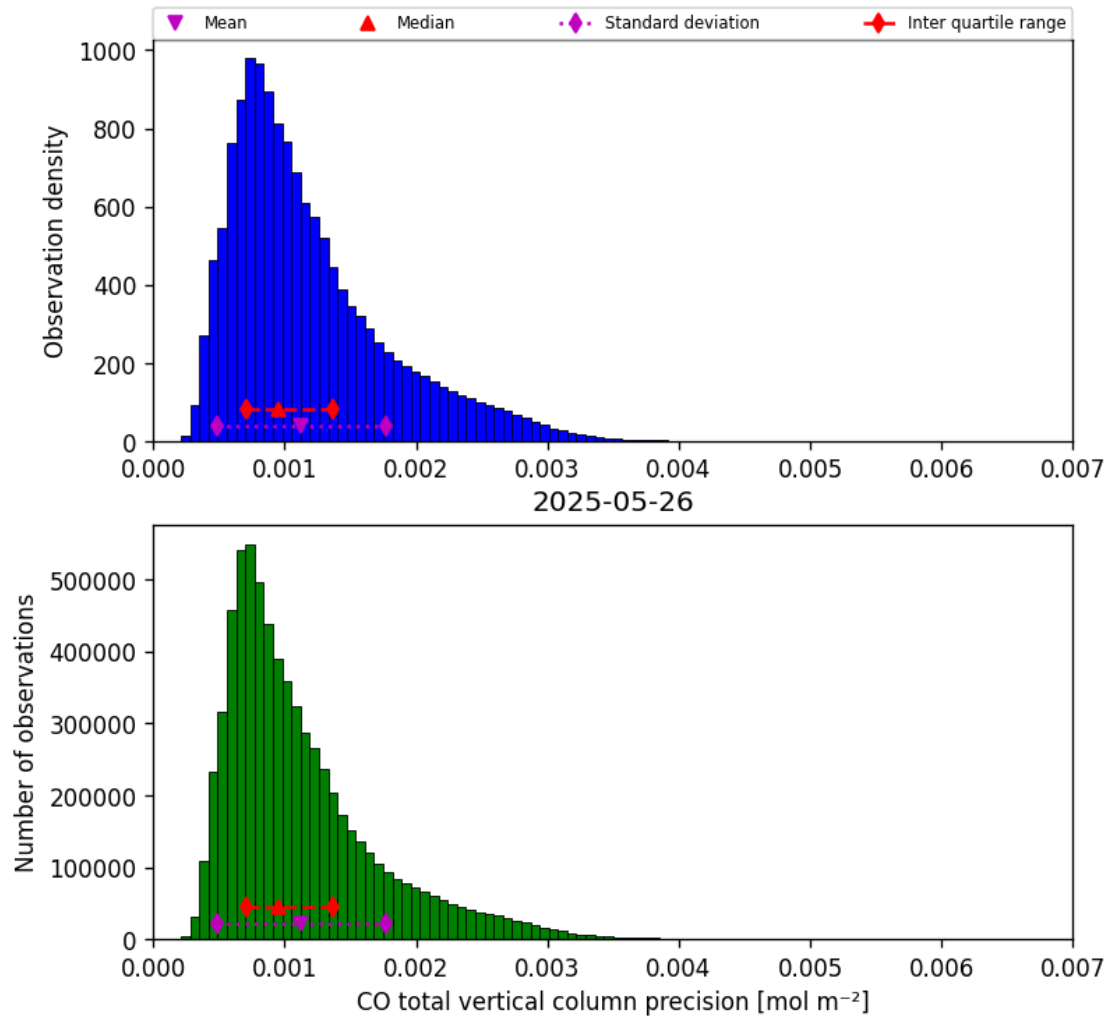
Figure 15: Histogram of “CO total vertical column precision” for 2025-05-26 to 2025-05-27
