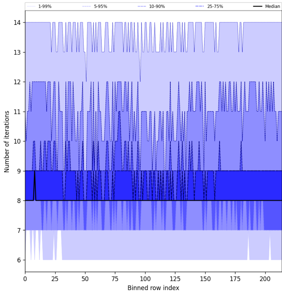
Figure 26: Along track statistics of “Number of iterations” for 2025-05-26 to 2025-05-27
