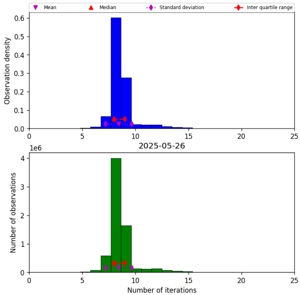
Figure 19: Histogram of “Number of iterations” for 2025-05-26 to 2025-05-27
