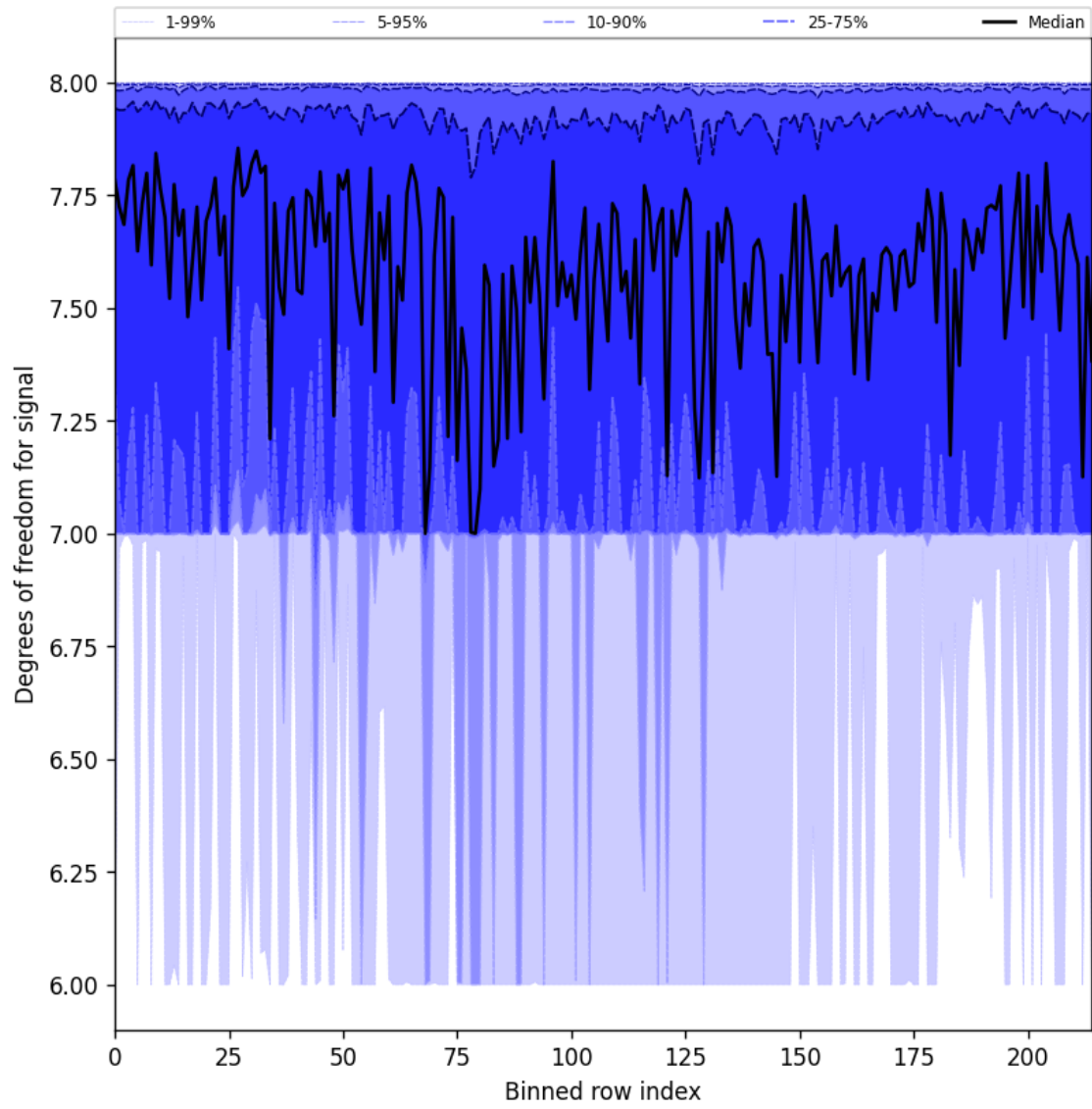
Figure 25: Along track statistics of “Degrees of freedom for signal” for 2025-05-26 to 2025-05-27
