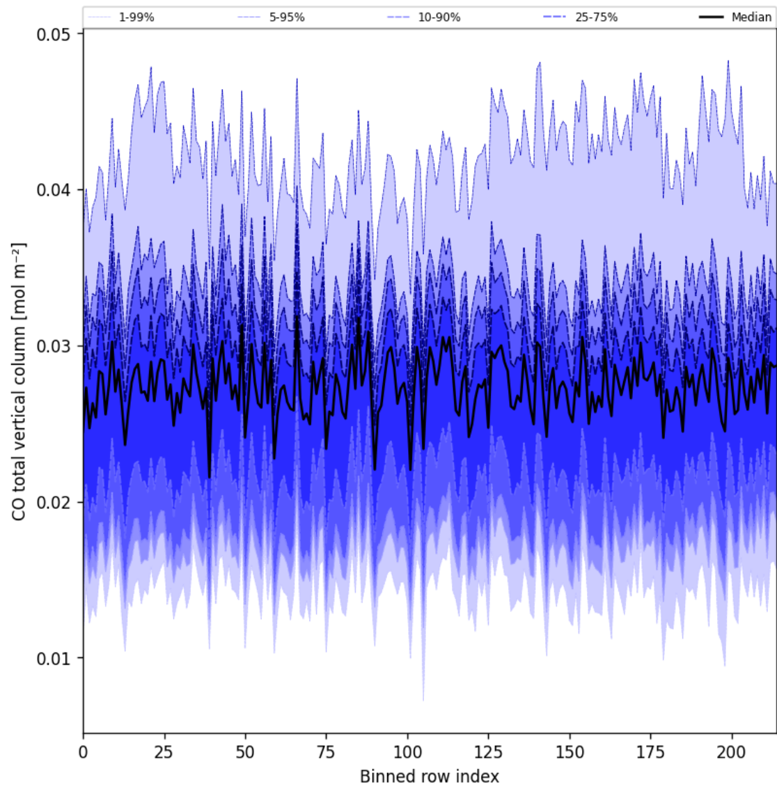
Figure 21: Along track statistics of “CO total vertical column” for 2025-05-26 to 2025-05-27
