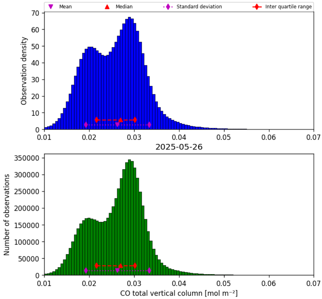
Figure 14: Histogram of “CO total vertical column” for 2025-05-26 to 2025-05-27
