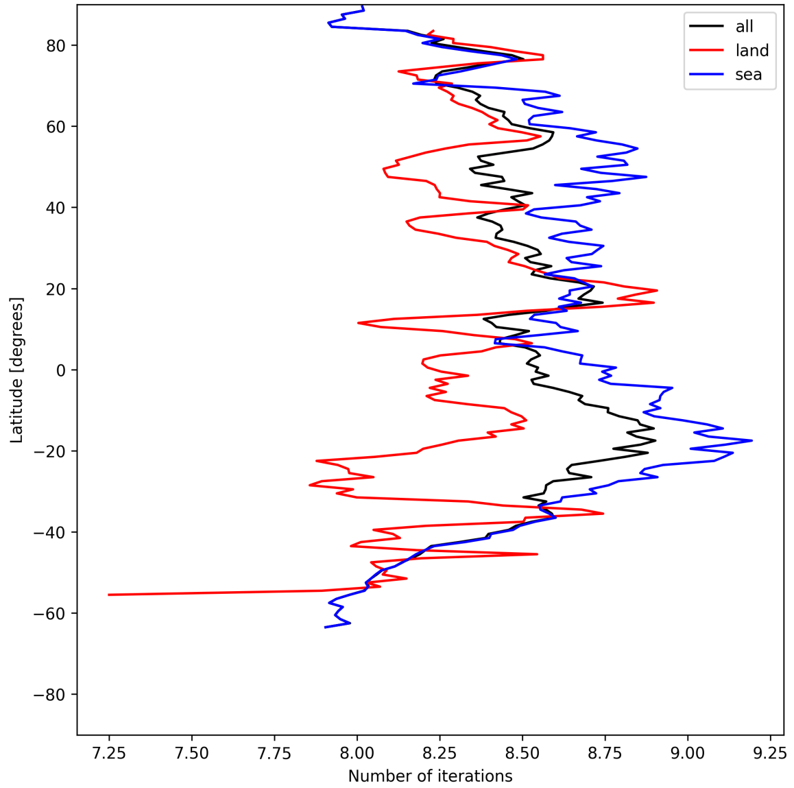
Figure 12: Zonal average of “Number of iterations” for 2025-05-26 to 2025-05-27.
