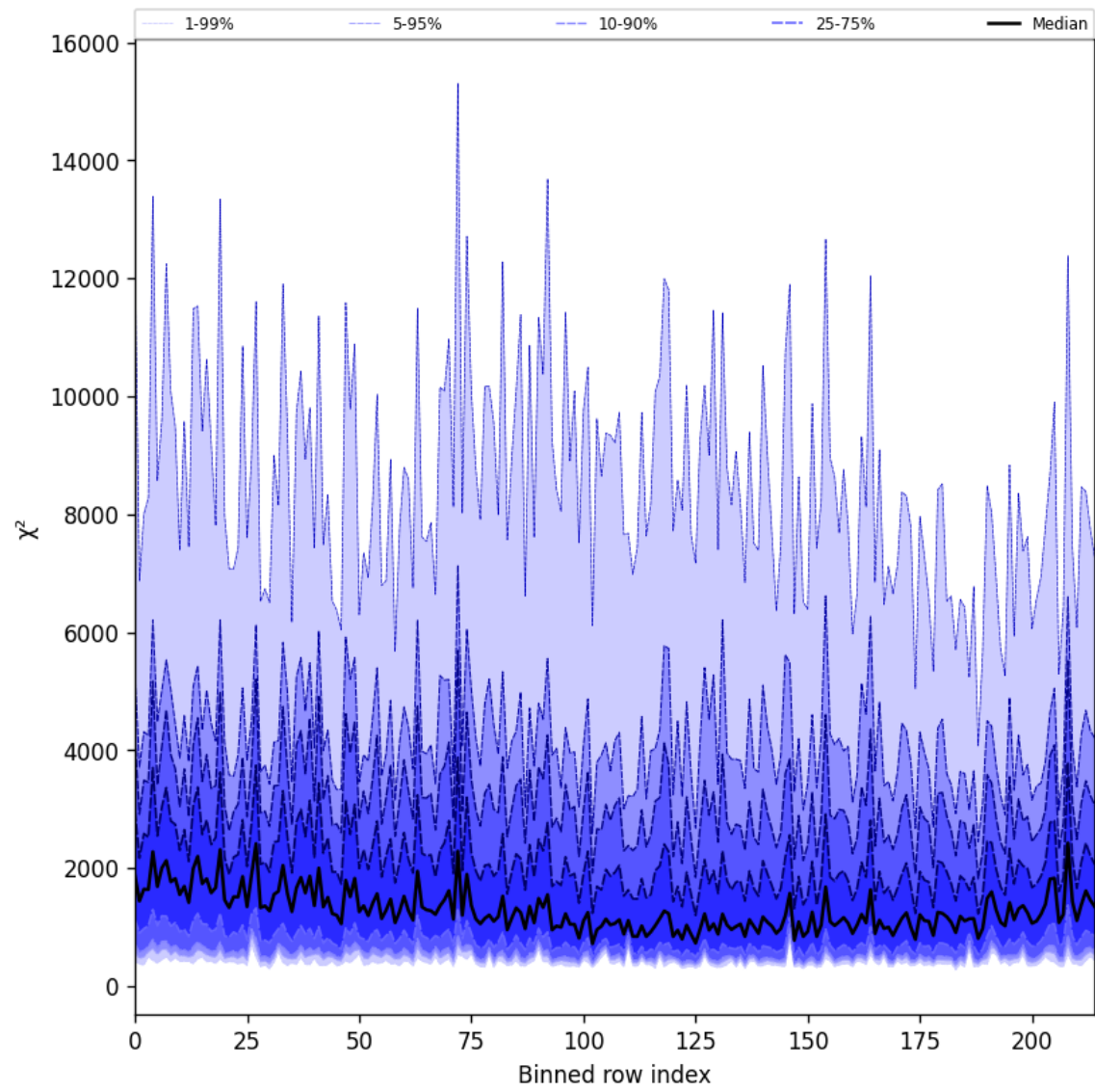
Figure 24: Along track statistics of “ \chi^2 ” for 2025-05-26 to 2025-05-27
