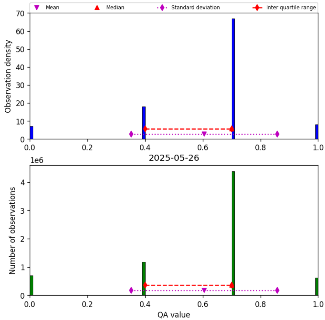
Figure 13: Histogram of “QA value” for 2025-05-26 to 2025-05-27
