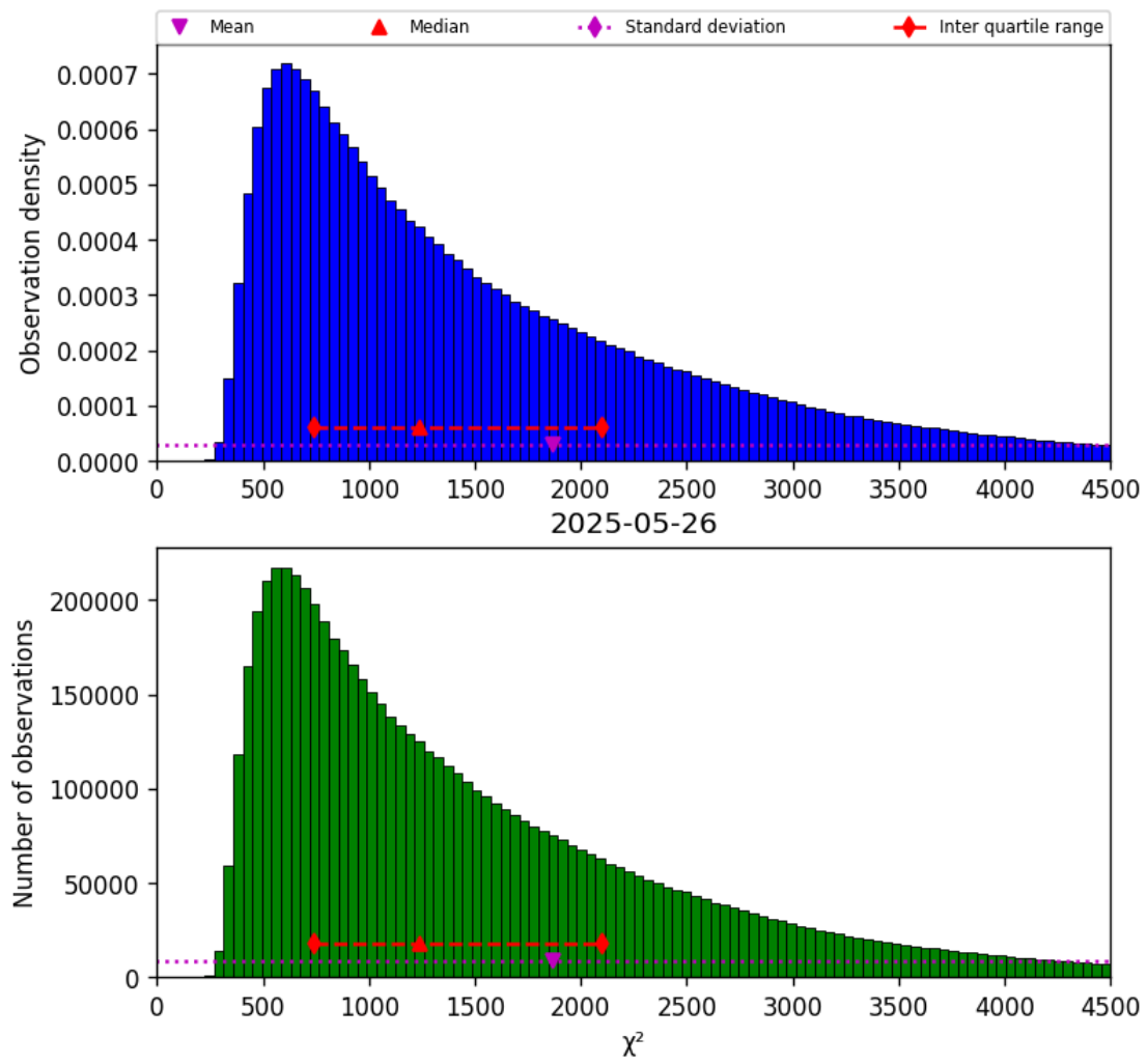
Figure 17: Histogram of “ \chi^2 ” for 2025-05-26 to 2025-05-27
