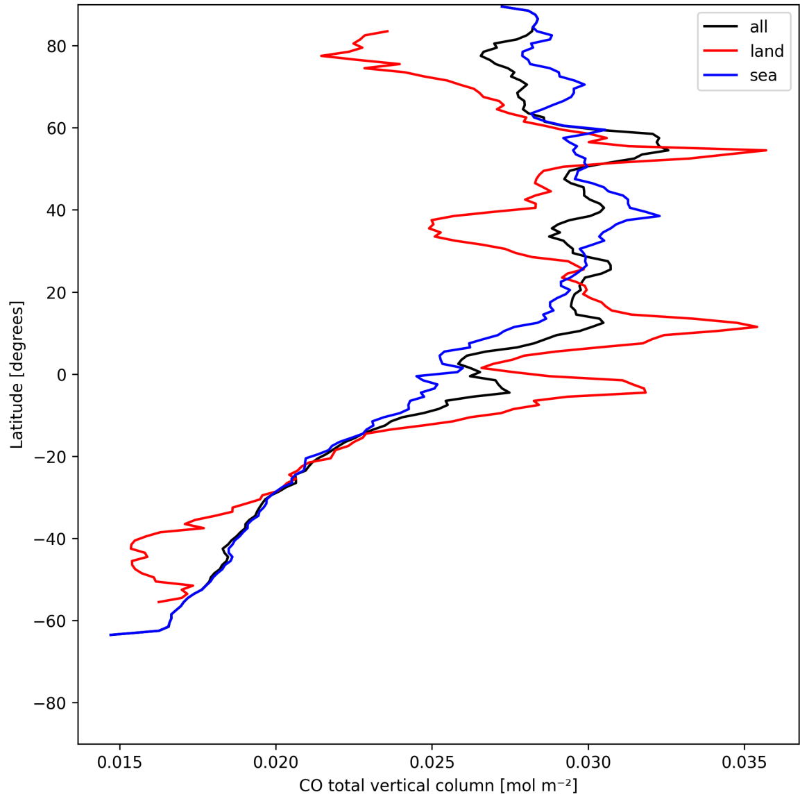
Figure 7: Zonal average of “CO total vertical column” for 2025-05-26 to 2025-05-27.
