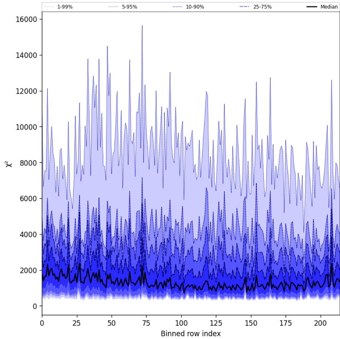
Figure 24: Along track statistics of “ \chi^2 ” for 2025-05-27 to 2025-05-28
