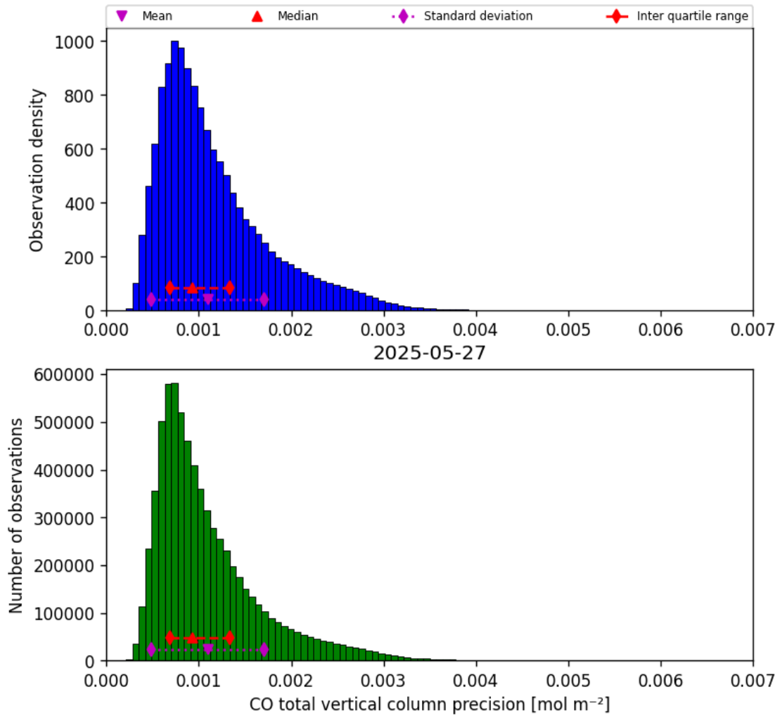
Figure 15: Histogram of “CO total vertical column precision” for 2025-05-27 to 2025-05-28
