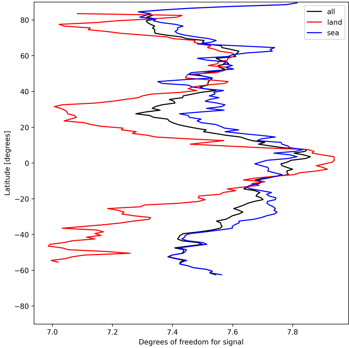
Figure 11: Zonal average of “Degrees of freedom for signal” for 2025-05-27 to 2025-05-28.
