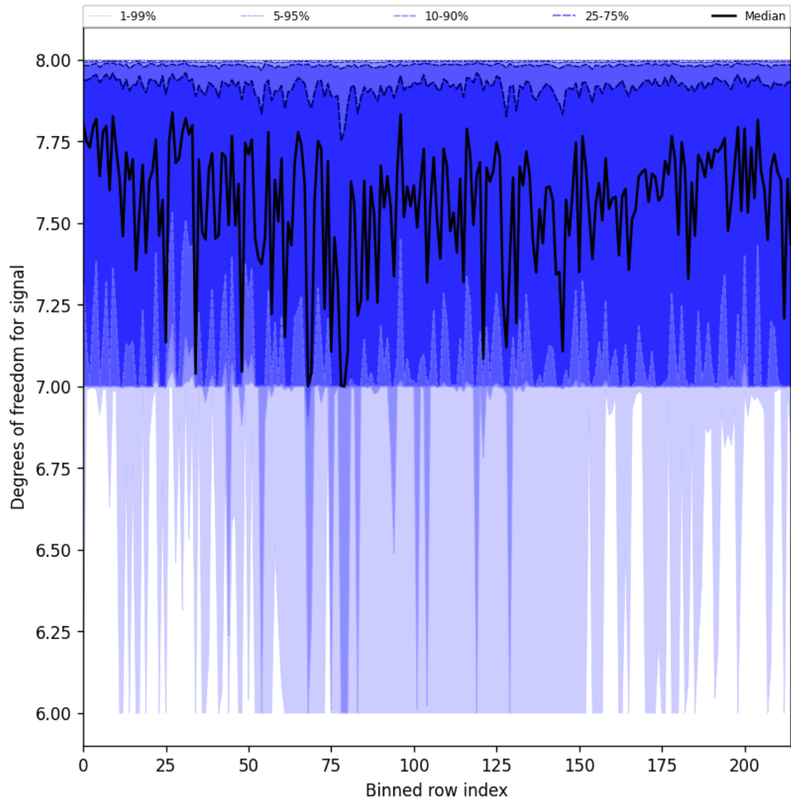
Figure 25: Along track statistics of “Degrees of freedom for signal” for 2025-05-27 to 2025-05-28
