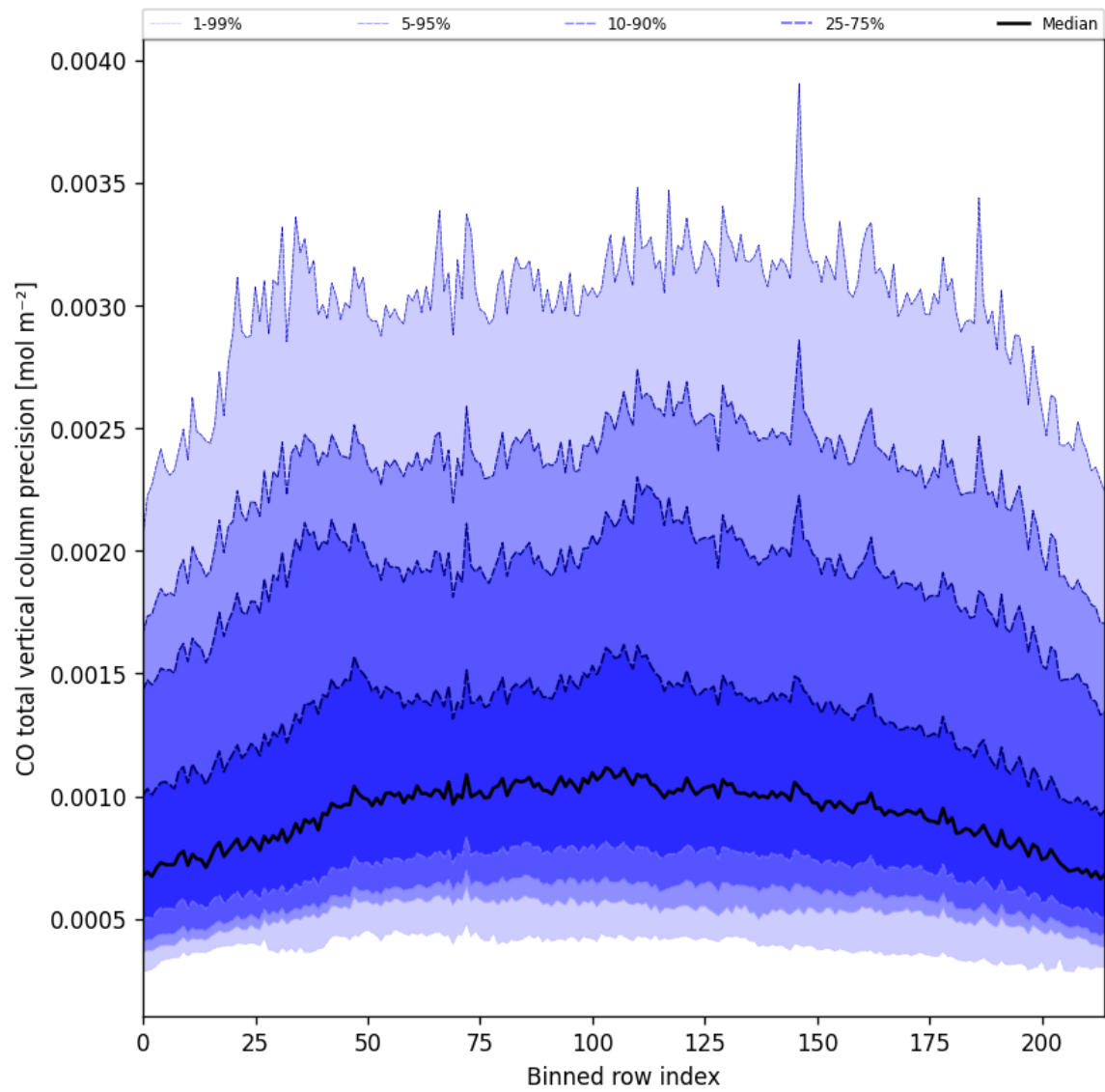
Figure 22: Along track statistics of “CO total vertical column precision” for 2025-05-27 to 2025-05-28
