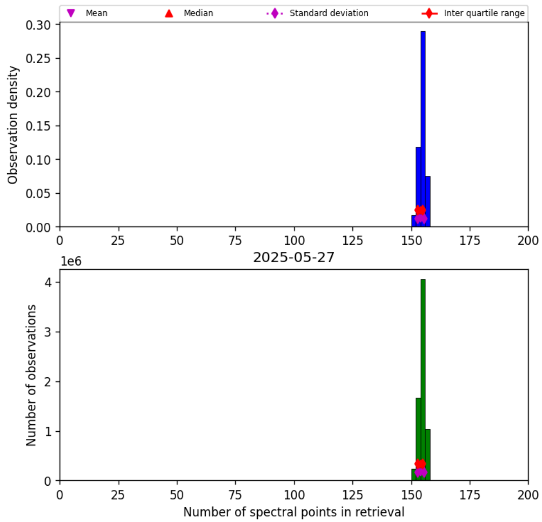
Figure 16: Histogram of “Number of spectral points in retrieval” for 2025-05-27 to 2025-05-28
