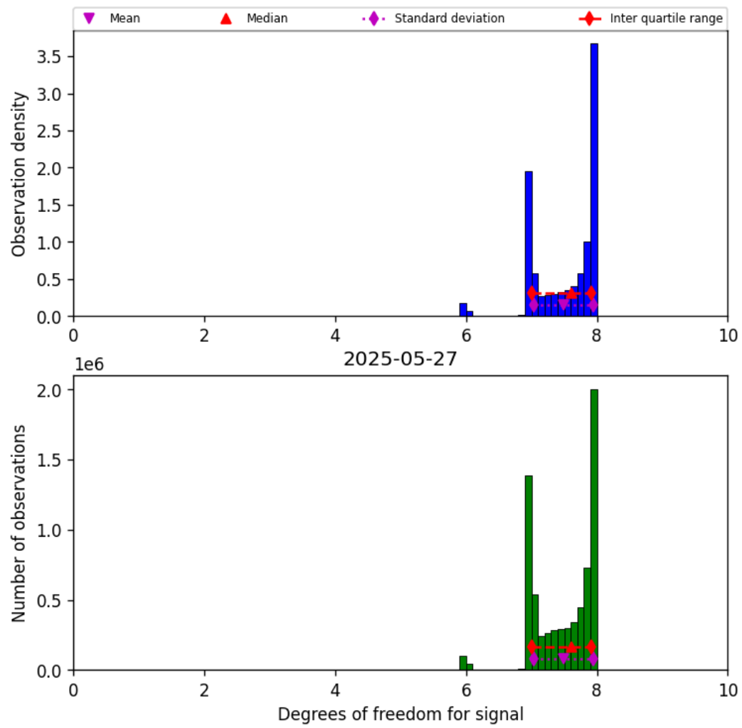
Figure 18: Histogram of “Degrees of freedom for signal” for 2025-05-27 to 2025-05-28
