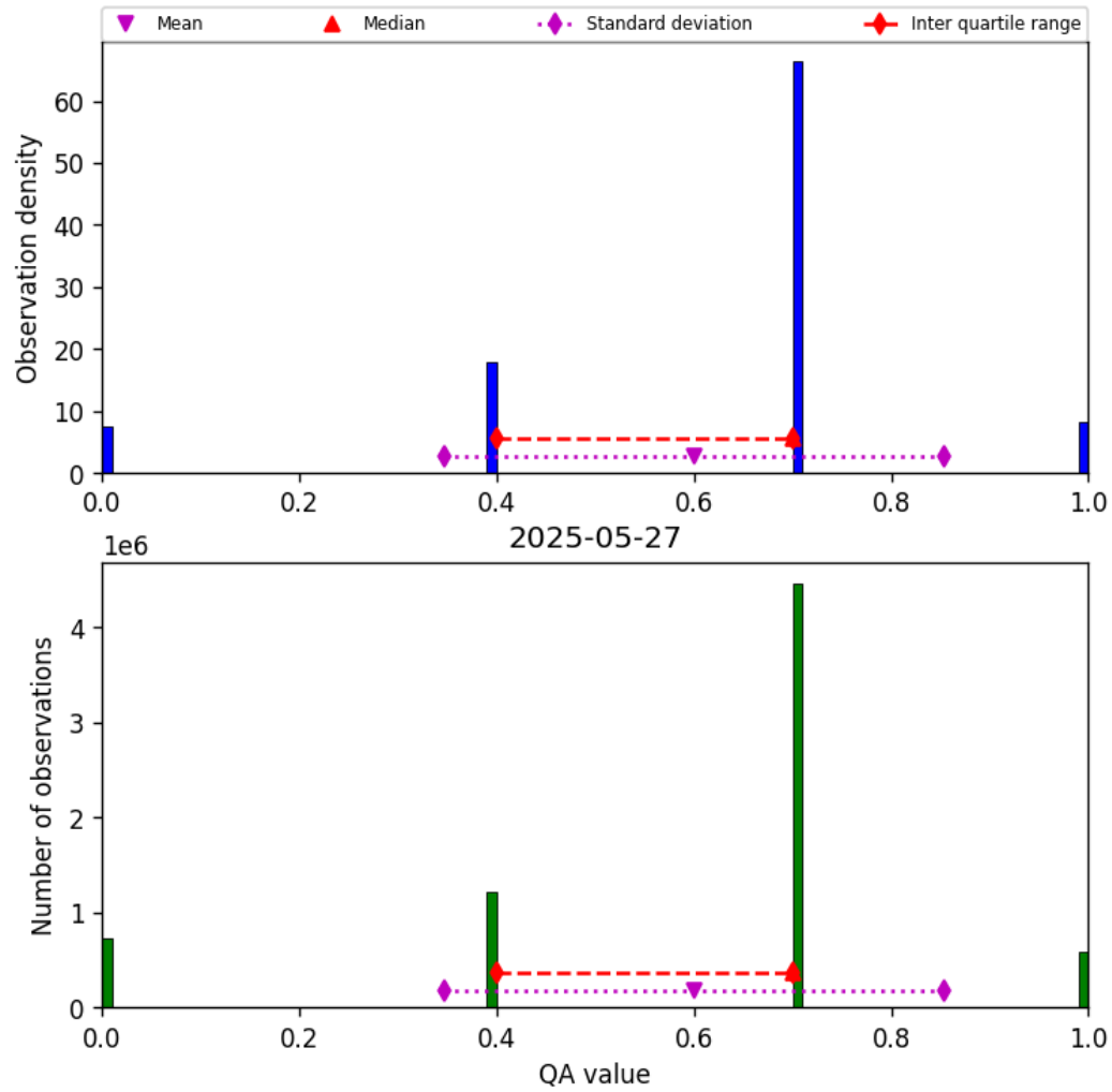
Figure 13: Histogram of “QA value” for 2025-05-27 to 2025-05-28
