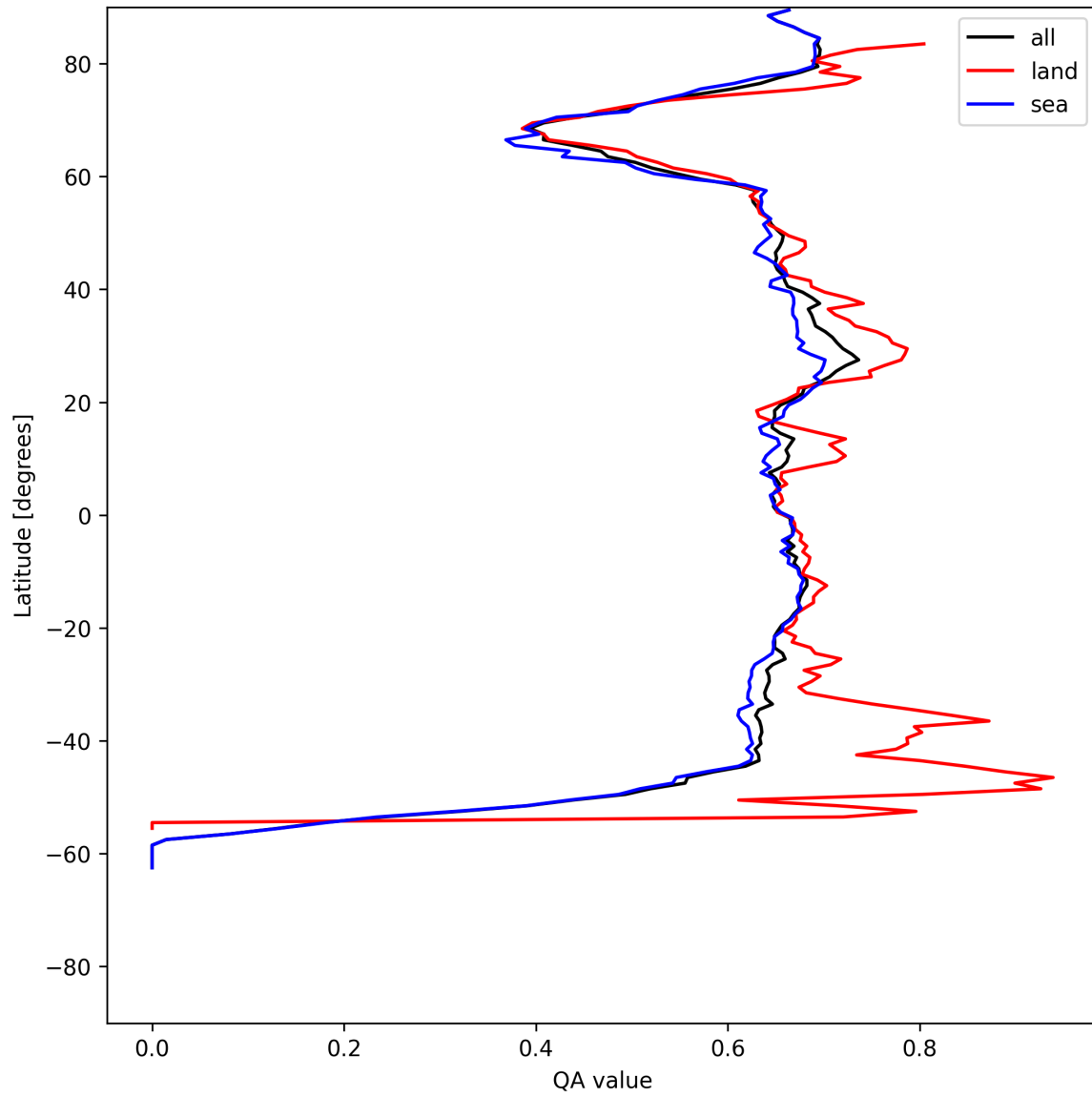
Figure 6: Zonal average of “QA value” for 2025-05-27 to 2025-05-28.
