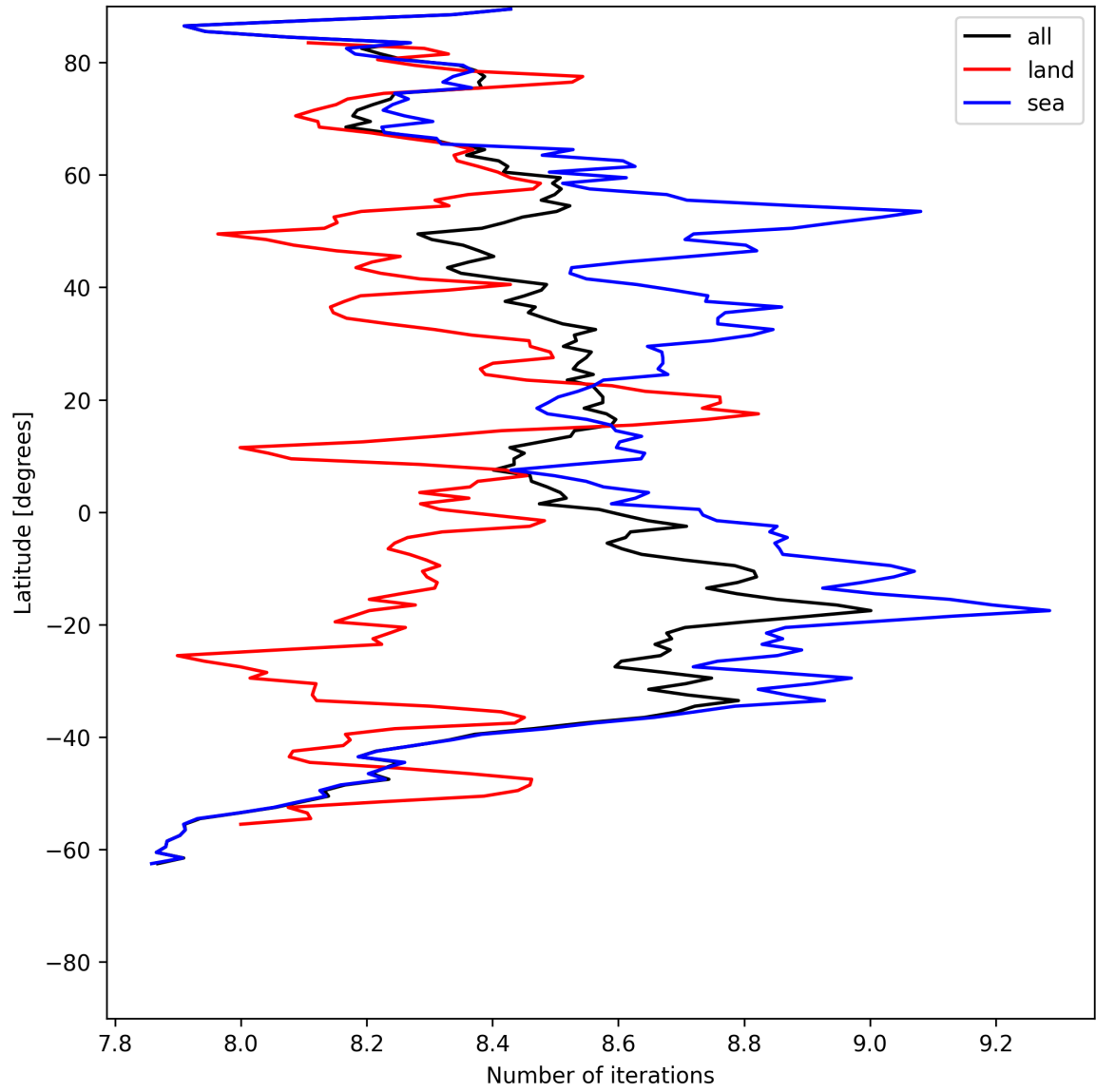
Figure 12: Zonal average of “Number of iterations” for 2025-05-27 to 2025-05-28.
