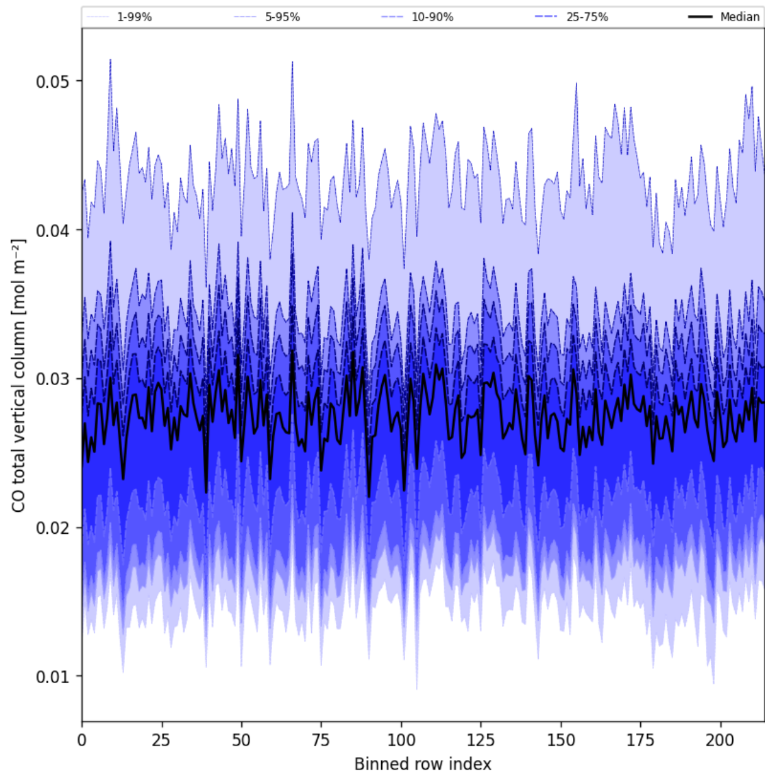
Figure 21: Along track statistics of “CO total vertical column” for 2025-05-27 to 2025-05-28
