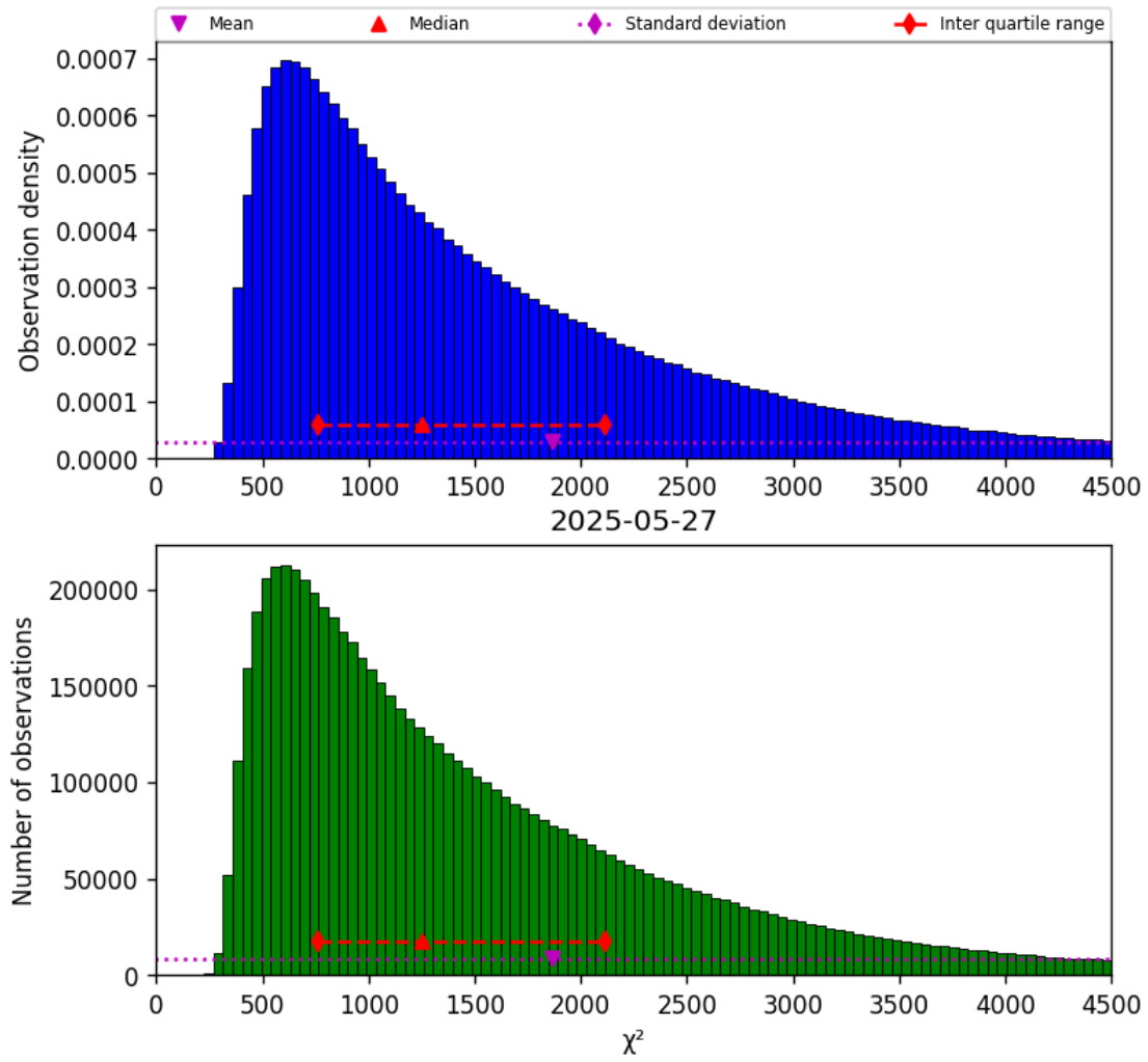
Figure 17: Histogram of “ \chi^2 ” for 2025-05-27 to 2025-05-28
