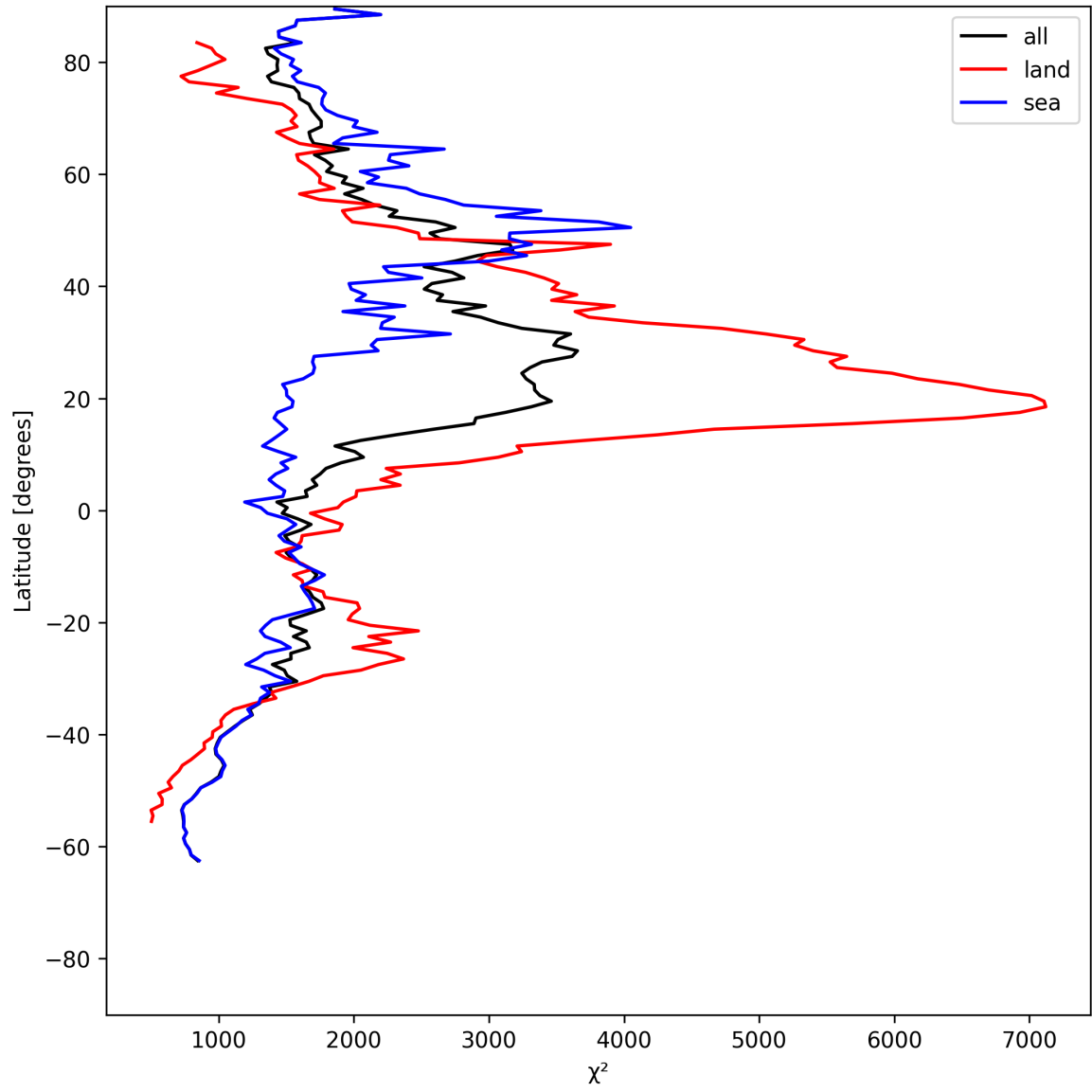
Figure 10: Zonal average of “ \chi^2 ” for 2025-05-27 to 2025-05-28.
