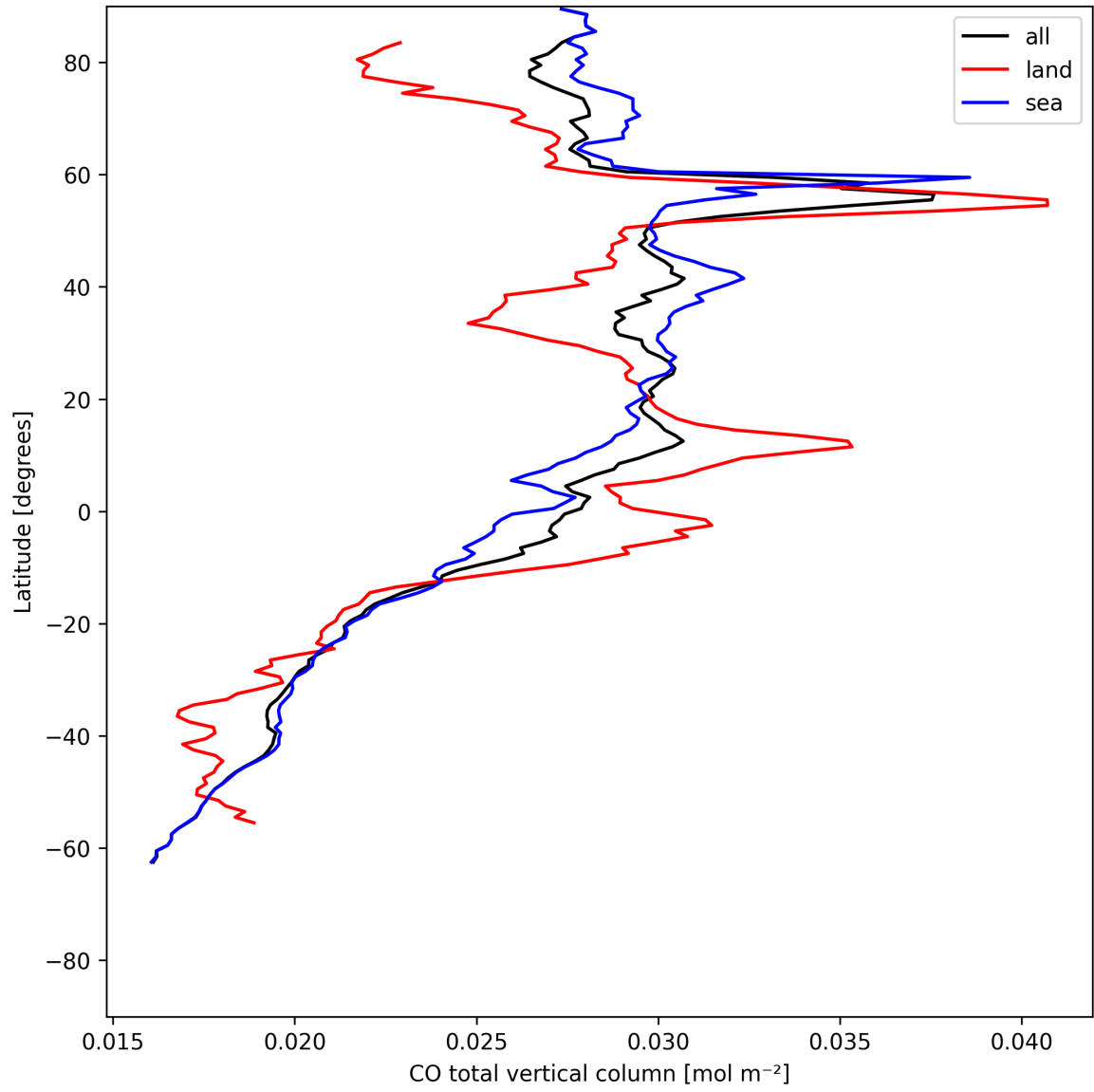
Figure 7: Zonal average of “CO total vertical column” for 2025-05-27 to 2025-05-28.
