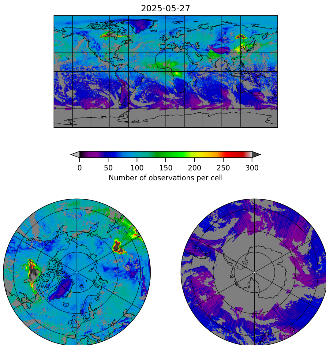
Figure 5: Map of the number of observations for 2025-05-27 to 2025-05-28
