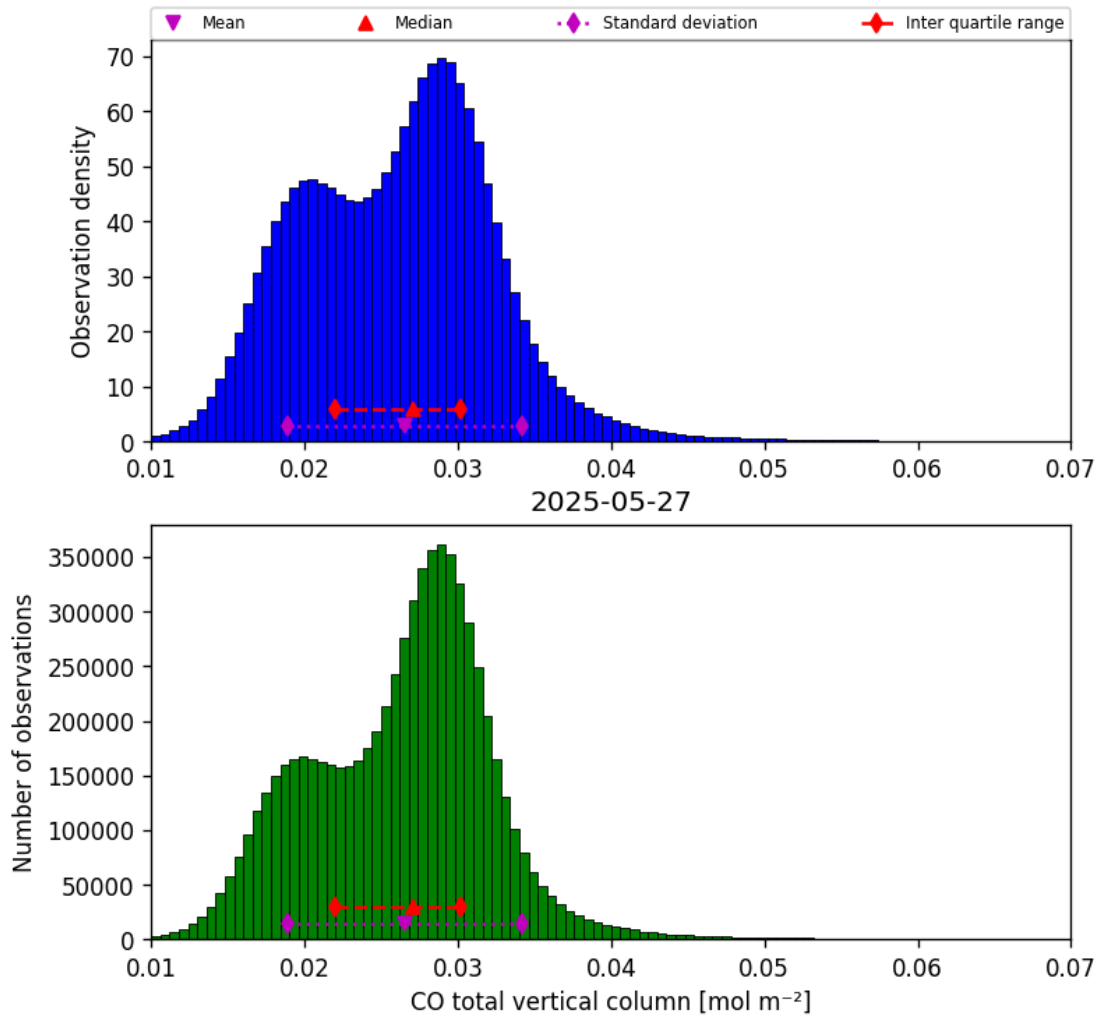
Figure 14: Histogram of “CO total vertical column” for 2025-05-27 to 2025-05-28
