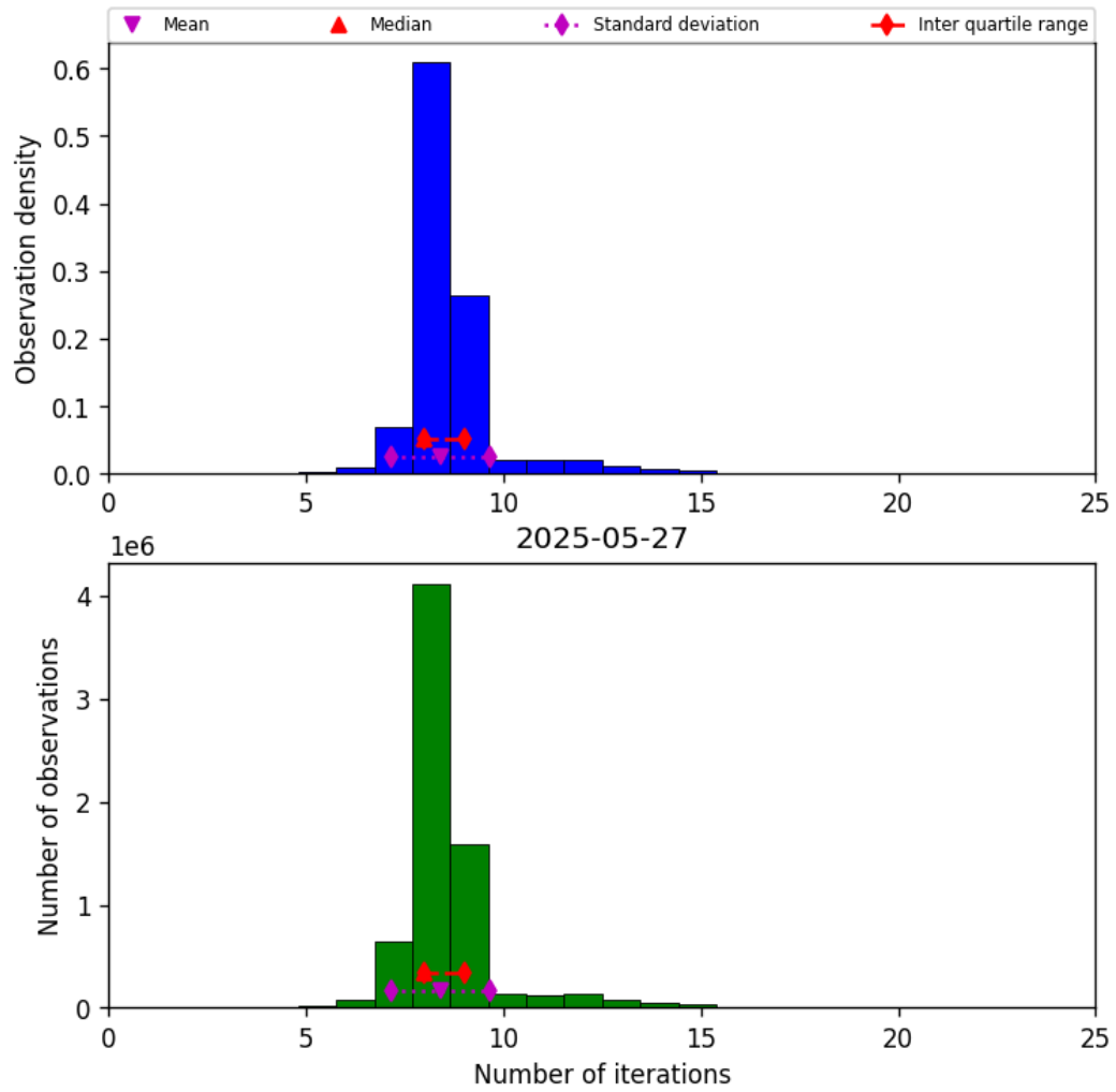
Figure 19: Histogram of “Number of iterations” for 2025-05-27 to 2025-05-28
