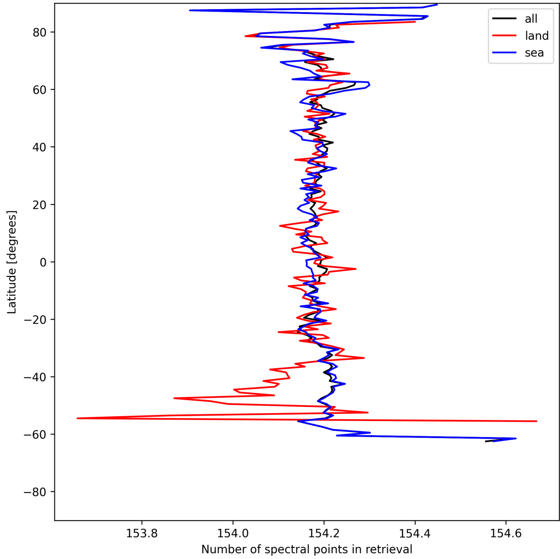
Figure 9: Zonal average of “Number of spectral points in retrieval” for 2025-05-27 to 2025-05-28.
