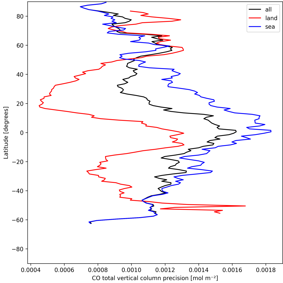
Figure 8: Zonal average of “CO total vertical column precision” for 2025-05-27 to 2025-05-28.
