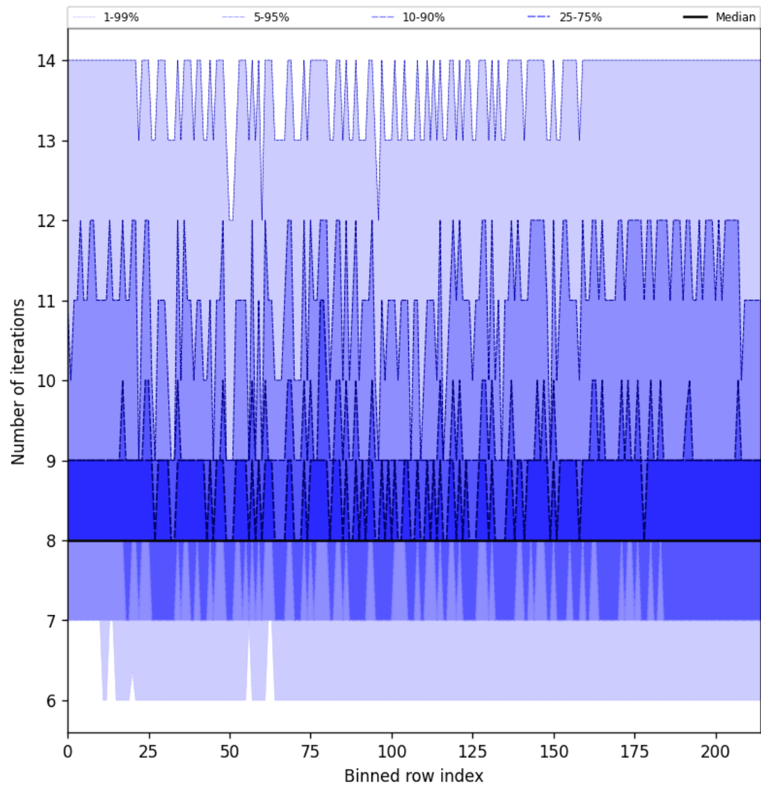
Figure 26: Along track statistics of “Number of iterations” for 2025-05-27 to 2025-05-28
