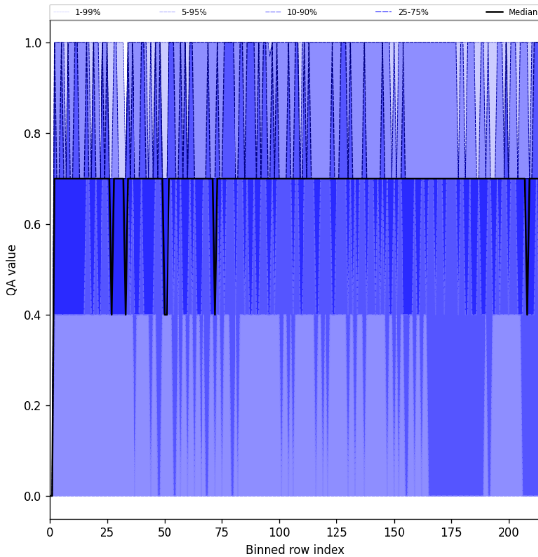
Figure 20: Along track statistics of “QA value” for 2025-05-27 to 2025-05-28
