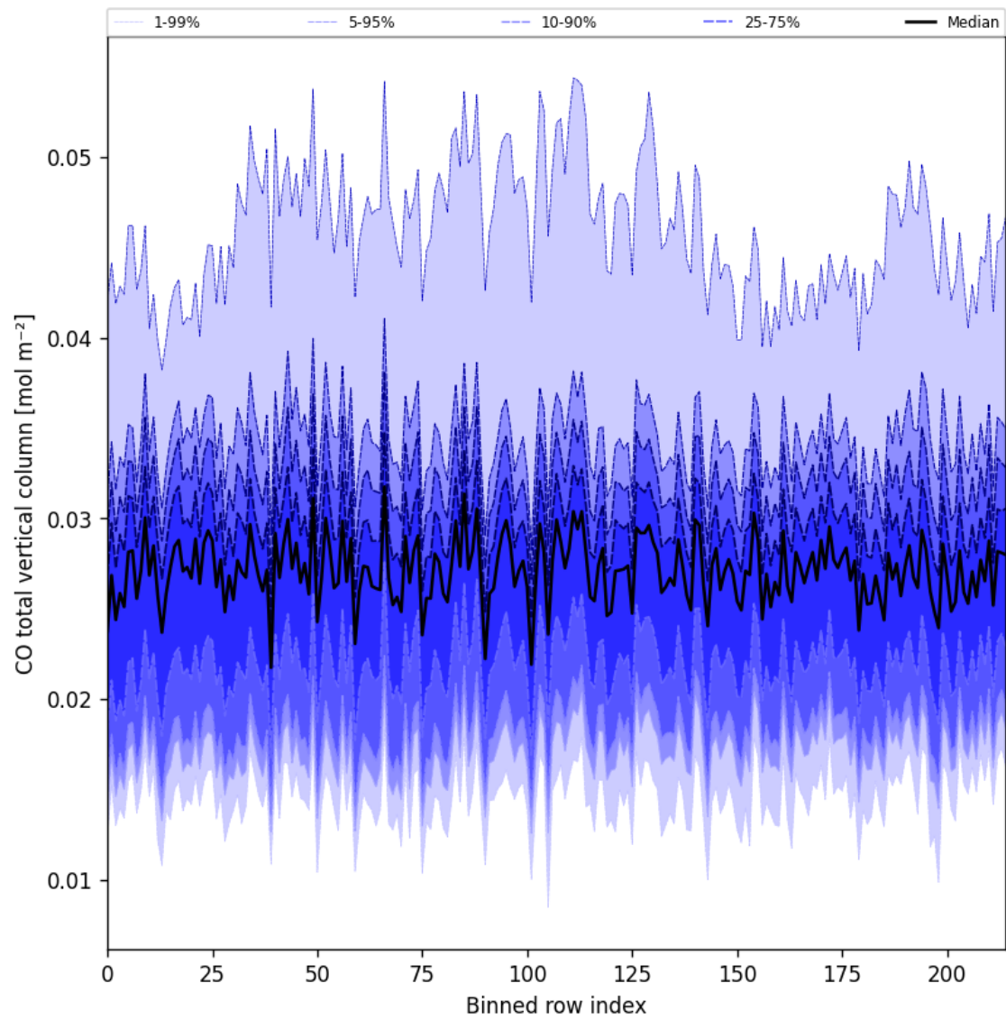
Figure 21: Along track statistics of “CO total vertical column” for 2025-05-28 to 2025-05-29
