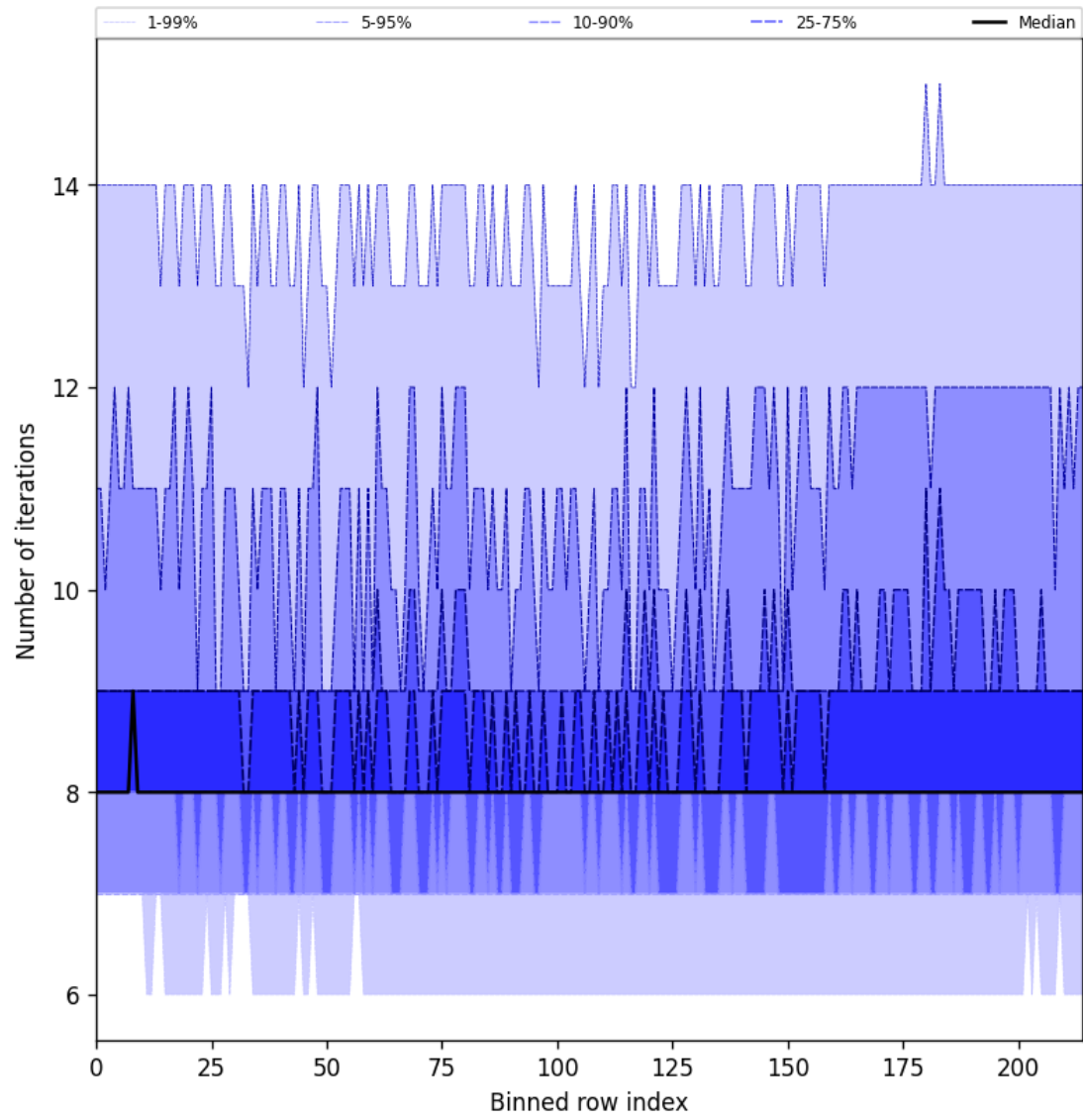
Figure 26: Along track statistics of “Number of iterations” for 2025-05-28 to 2025-05-29
