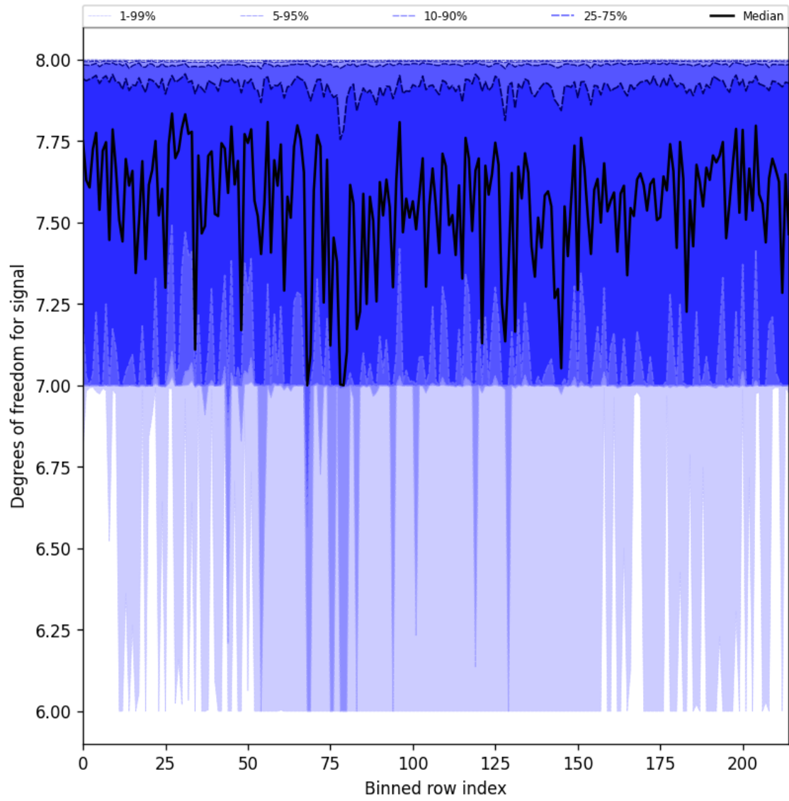
Figure 25: Along track statistics of “Degrees of freedom for signal” for 2025-05-28 to 2025-05-29
