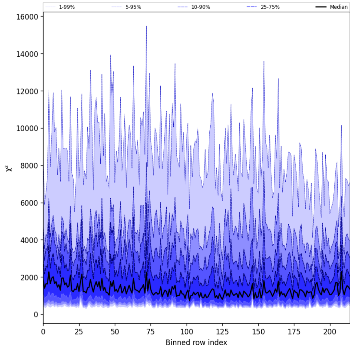
Figure 24: Along track statistics of “ \chi^2 ” for 2025-05-28 to 2025-05-29
