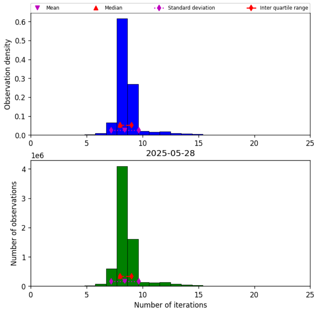
Figure 19: Histogram of “Number of iterations” for 2025-05-28 to 2025-05-29
