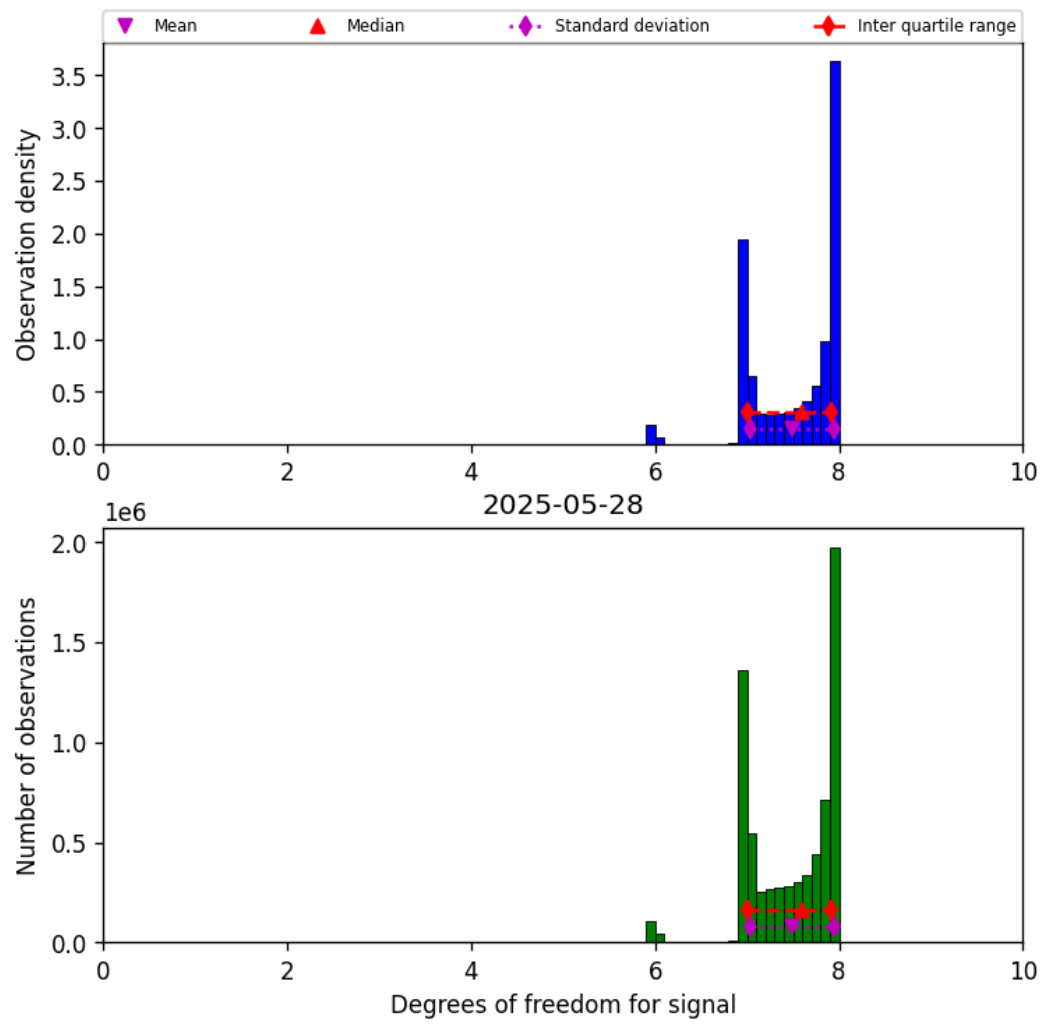
Figure 18: Histogram of “Degrees of freedom for signal” for 2025-05-28 to 2025-05-29
