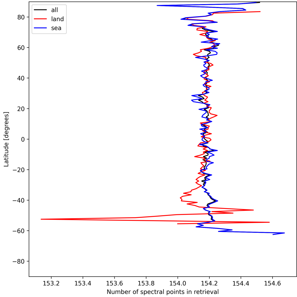
Figure 9: Zonal average of “Number of spectral points in retrieval” for 2025-05-28 to 2025-05-29.
