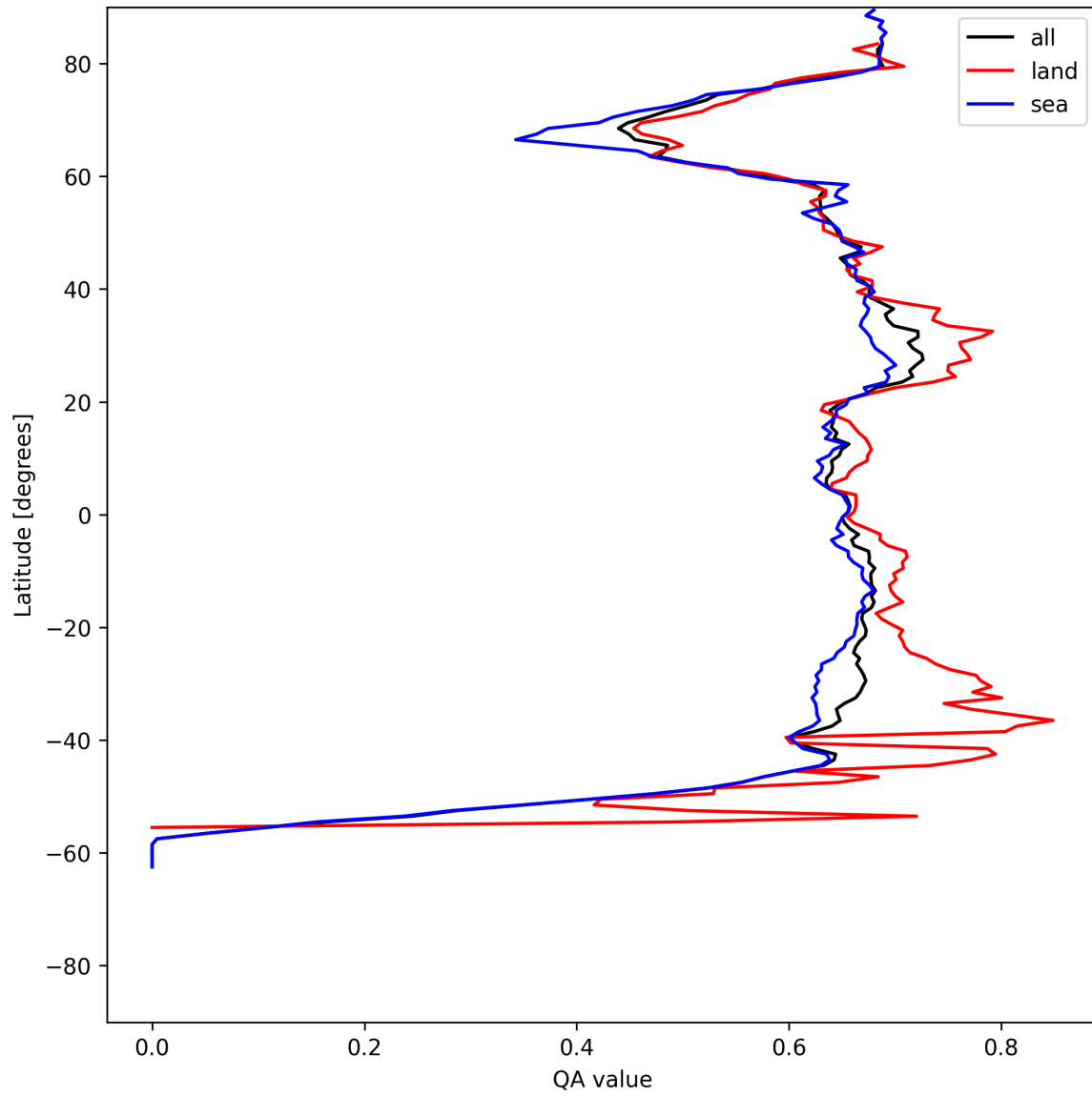
Figure 6: Zonal average of “QA value” for 2025-05-28 to 2025-05-29.
