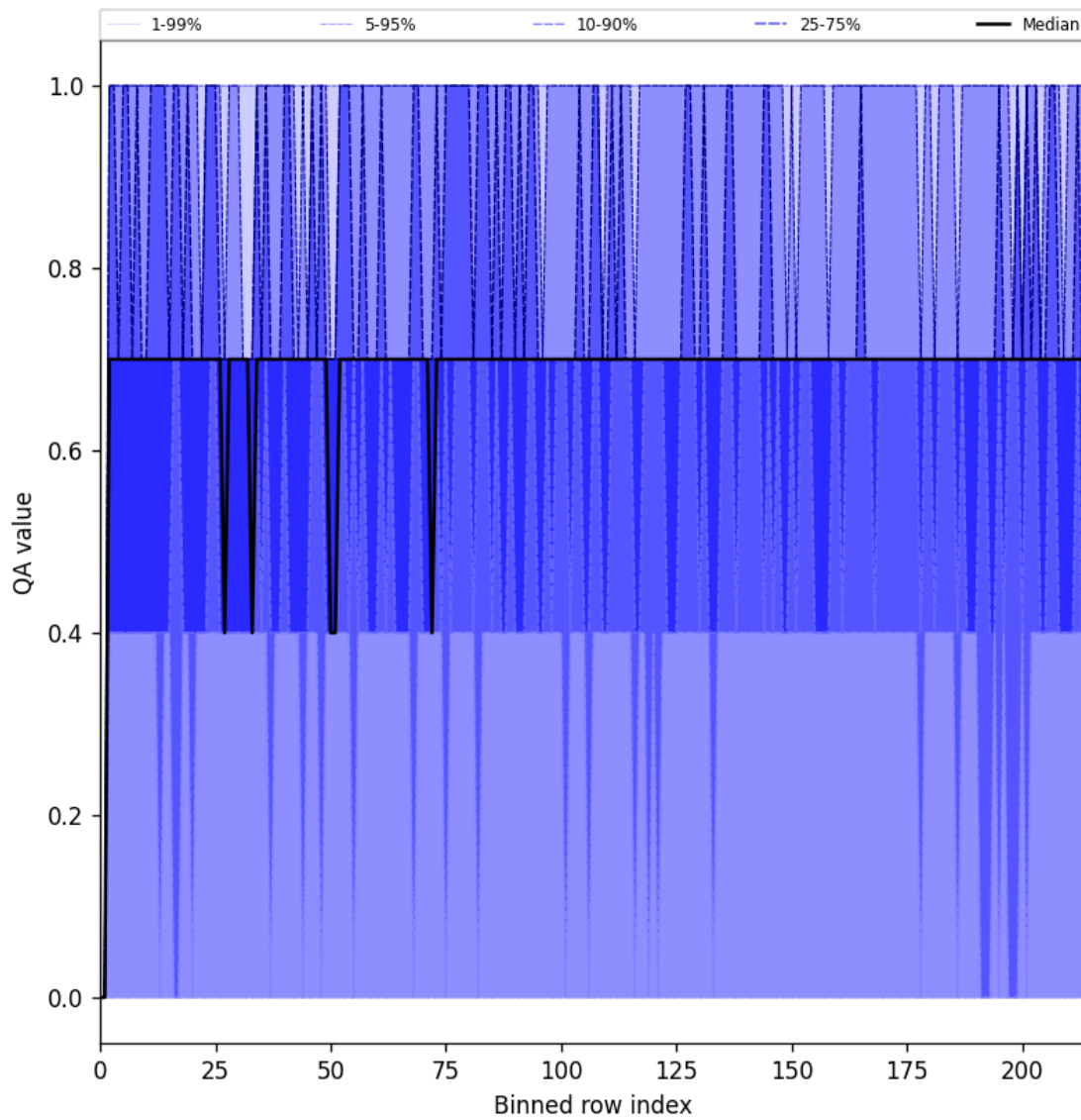
Figure 20: Along track statistics of “QA value” for 2025-05-28 to 2025-05-29
