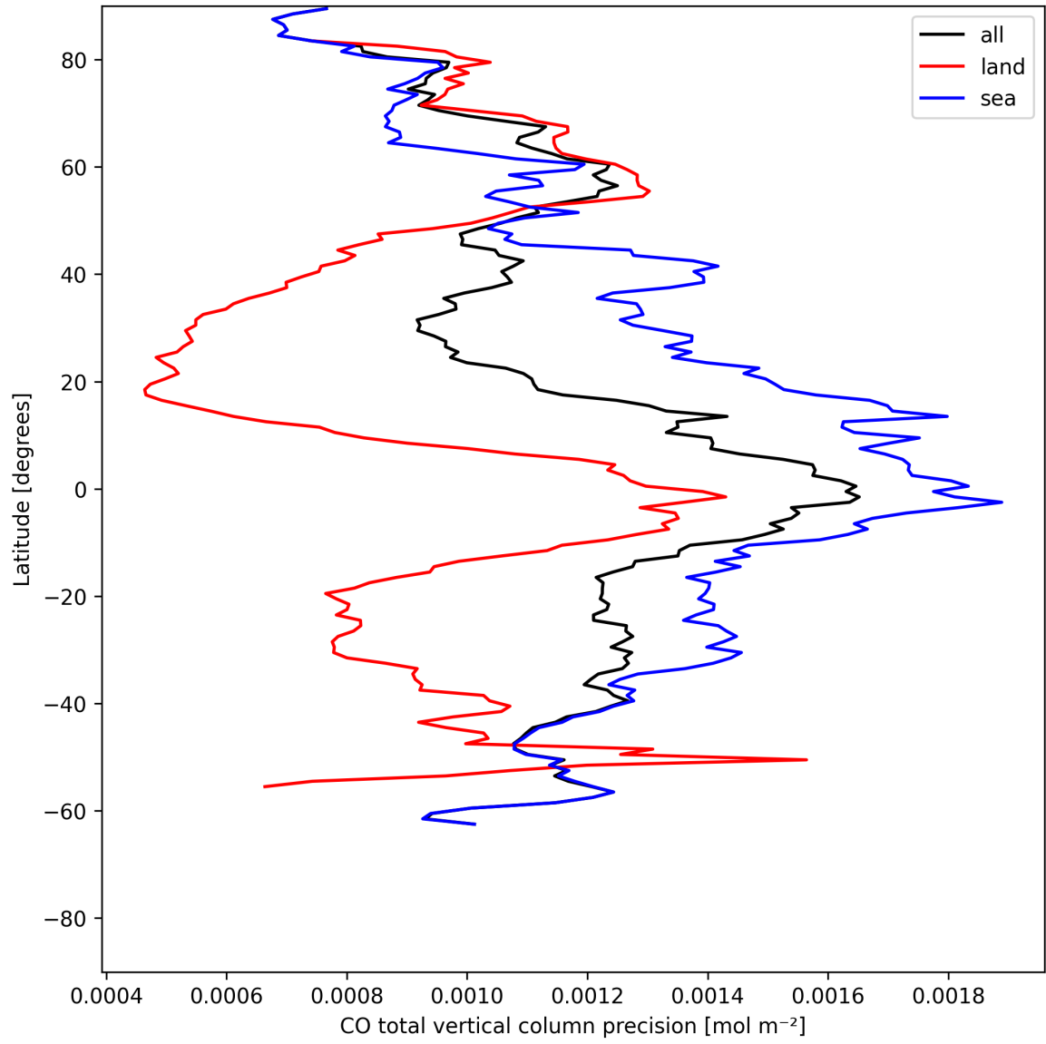
Figure 8: Zonal average of “CO total vertical column precision” for 2025-05-28 to 2025-05-29.
