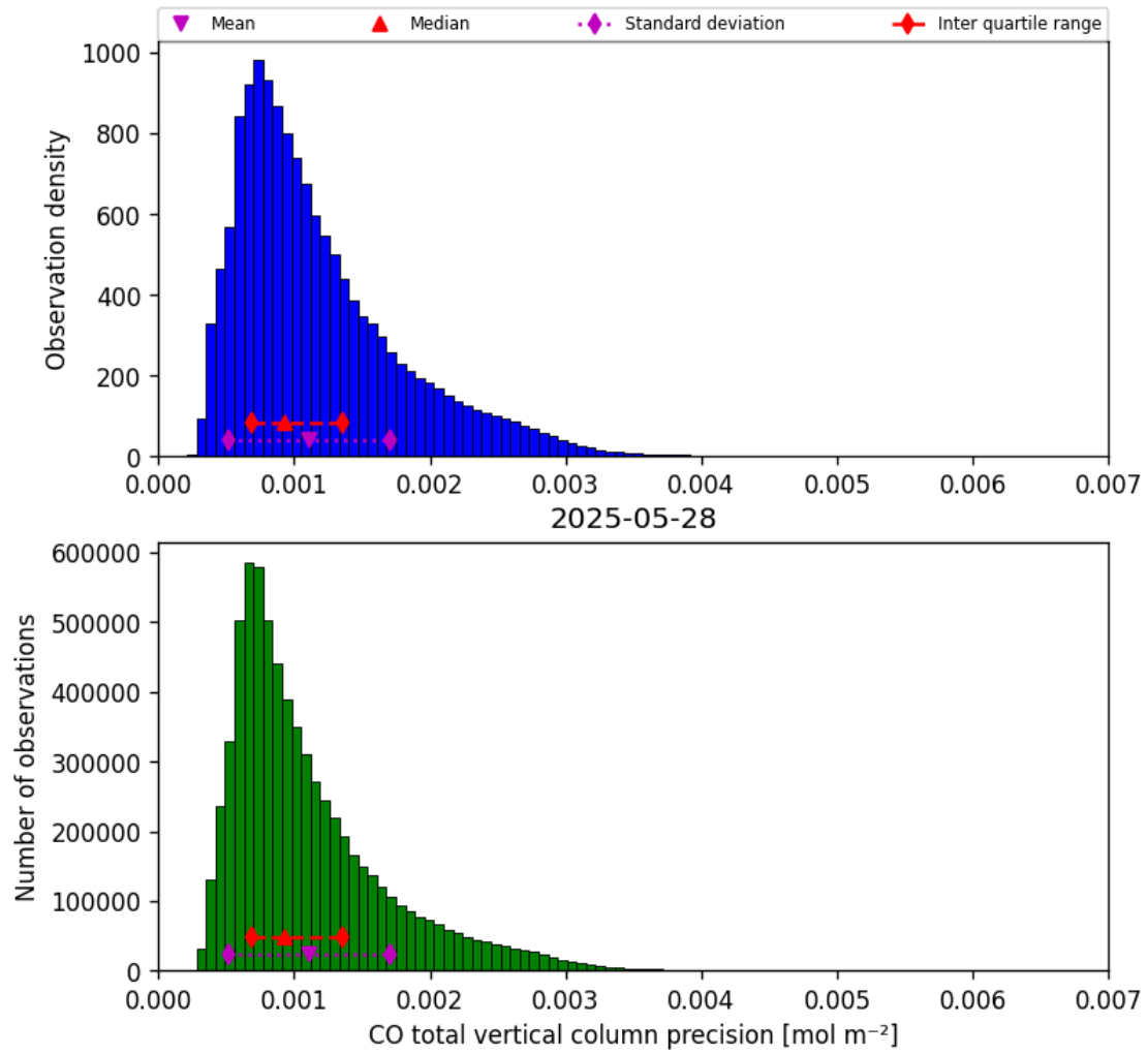
Figure 15: Histogram of “CO total vertical column precision” for 2025-05-28 to 2025-05-29
