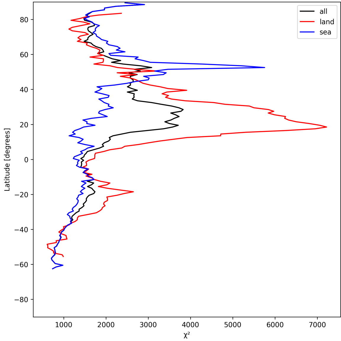
Figure 10: Zonal average of “ \chi^2 ” for 2025-05-28 to 2025-05-29.
