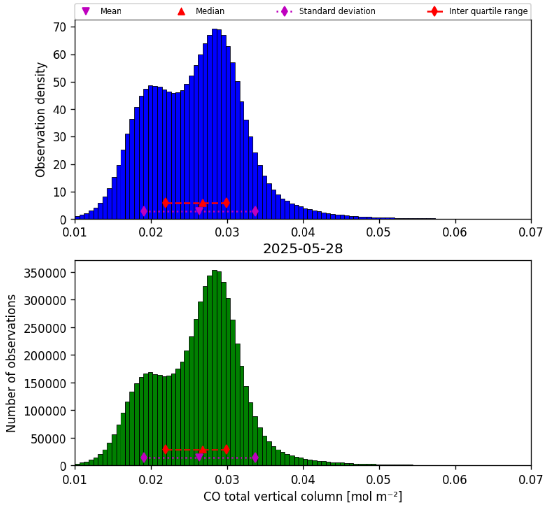
Figure 14: Histogram of “CO total vertical column” for 2025-05-28 to 2025-05-29
