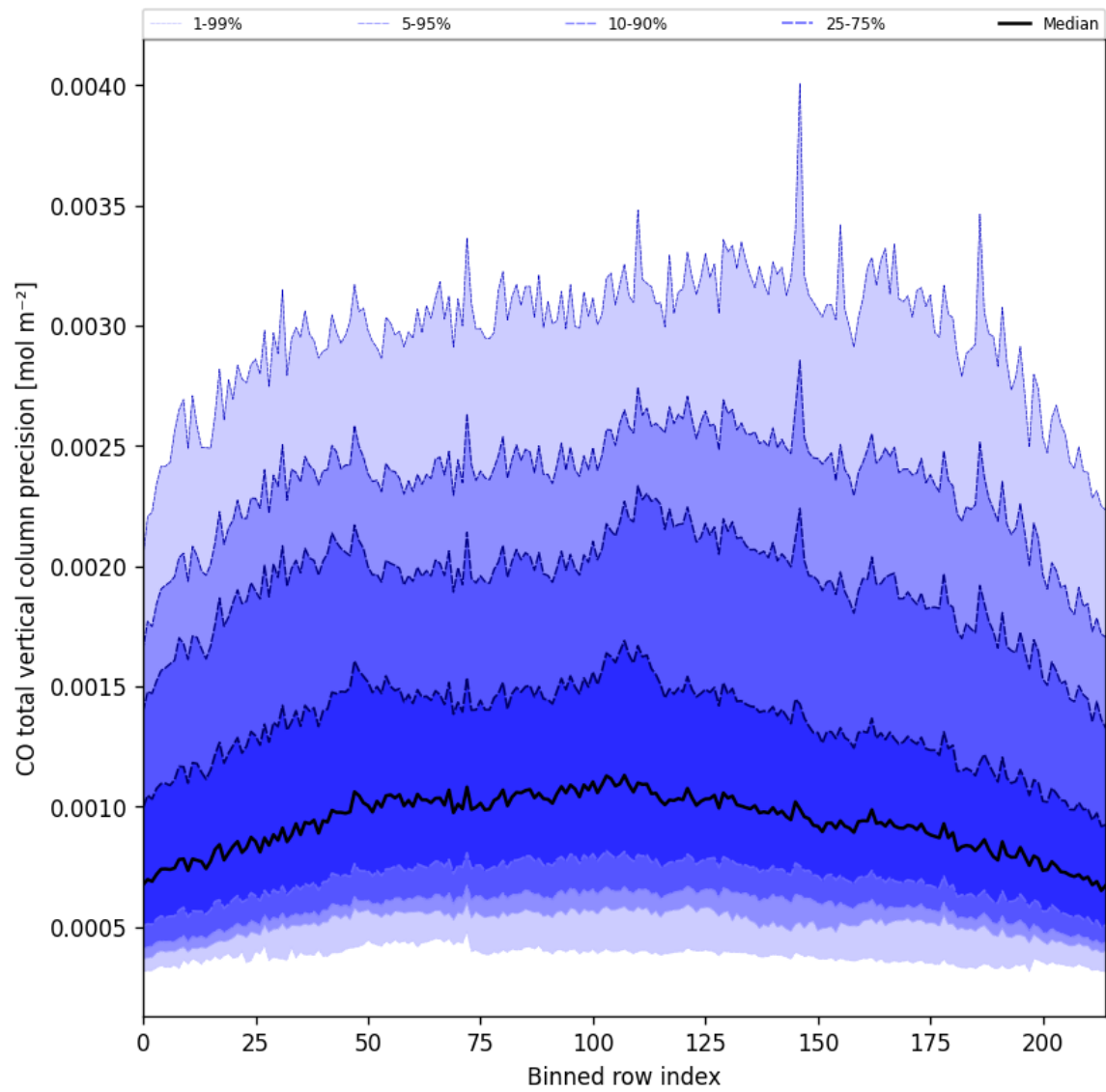
Figure 22: Along track statistics of “CO total vertical column precision” for 2025-05-28 to 2025-05-29
