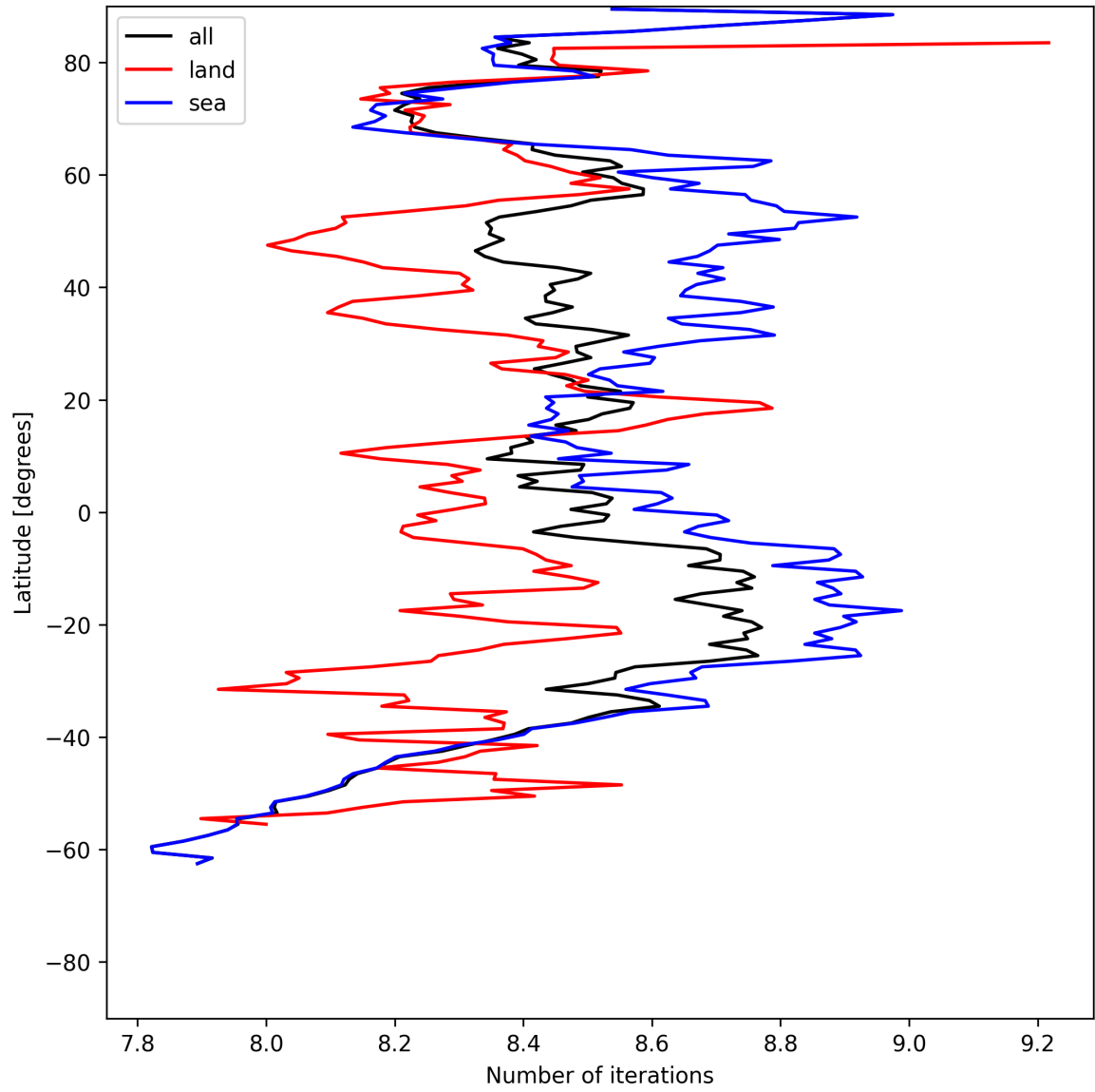
Figure 12: Zonal average of “Number of iterations” for 2025-05-28 to 2025-05-29.
