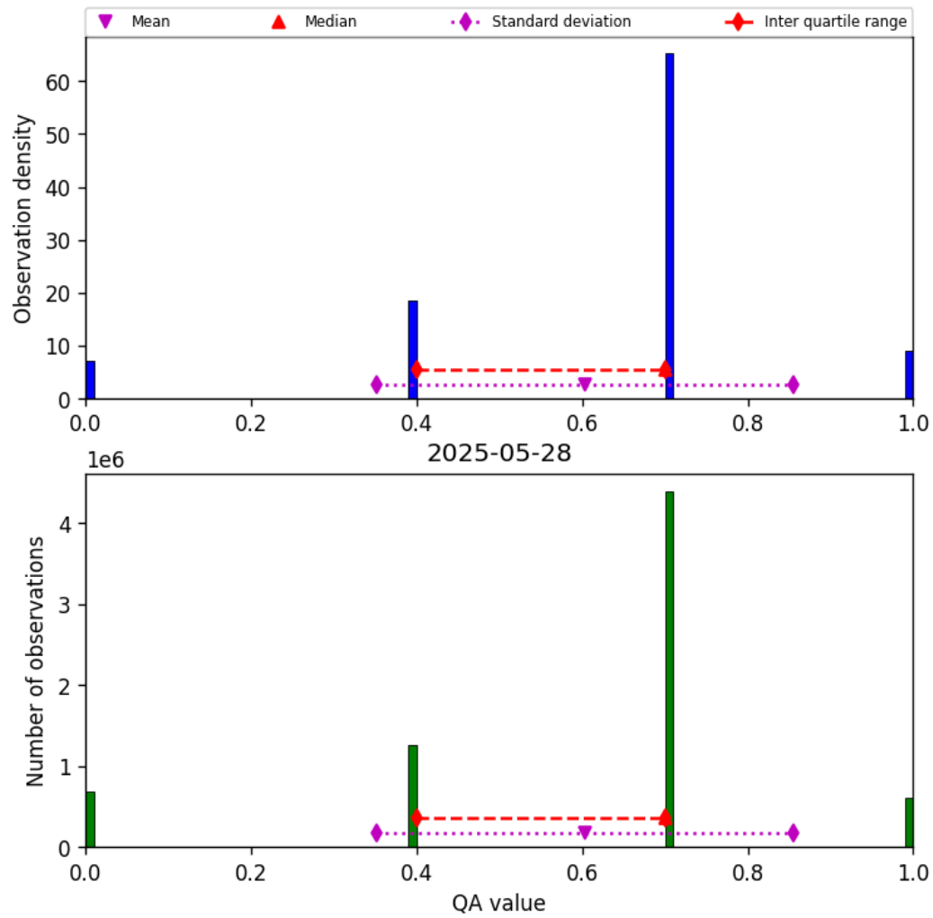
Figure 13: Histogram of “QA value” for 2025-05-28 to 2025-05-29
