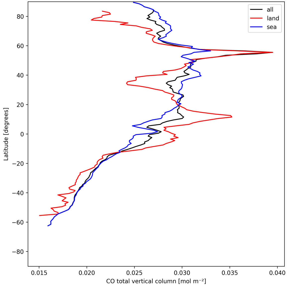
Figure 7: Zonal average of “CO total vertical column” for 2025-05-28 to 2025-05-29.
