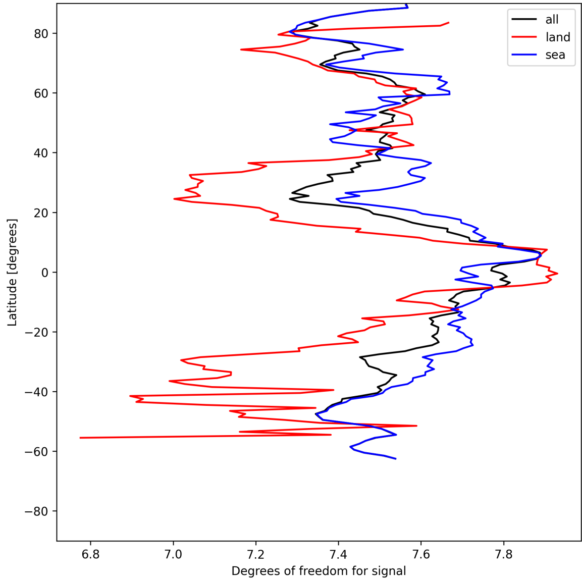
Figure 11: Zonal average of “Degrees of freedom for signal” for 2025-05-28 to 2025-05-29.
