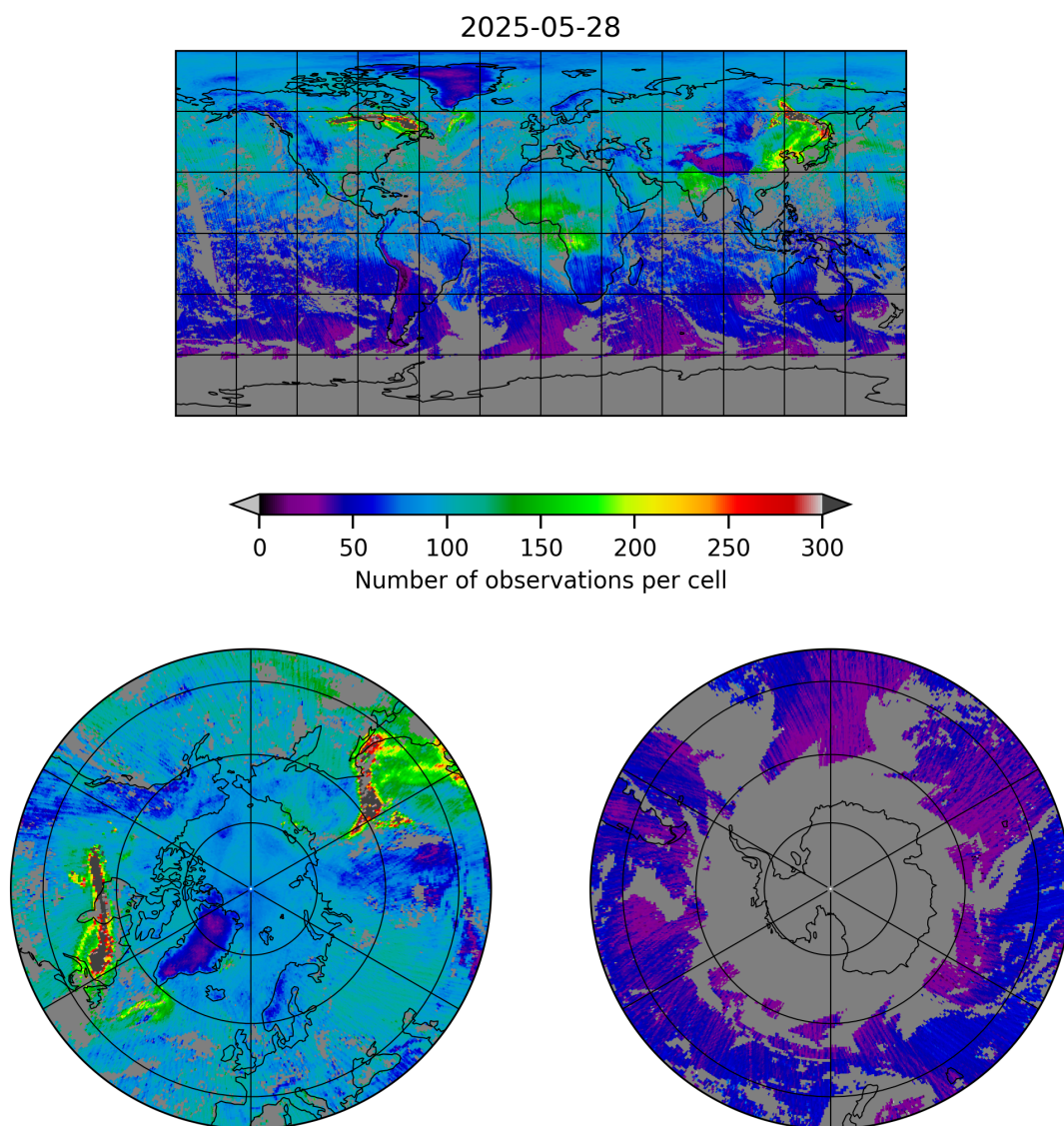
Figure 5: Map of the number of observations for 2025-05-28 to 2025-05-29
