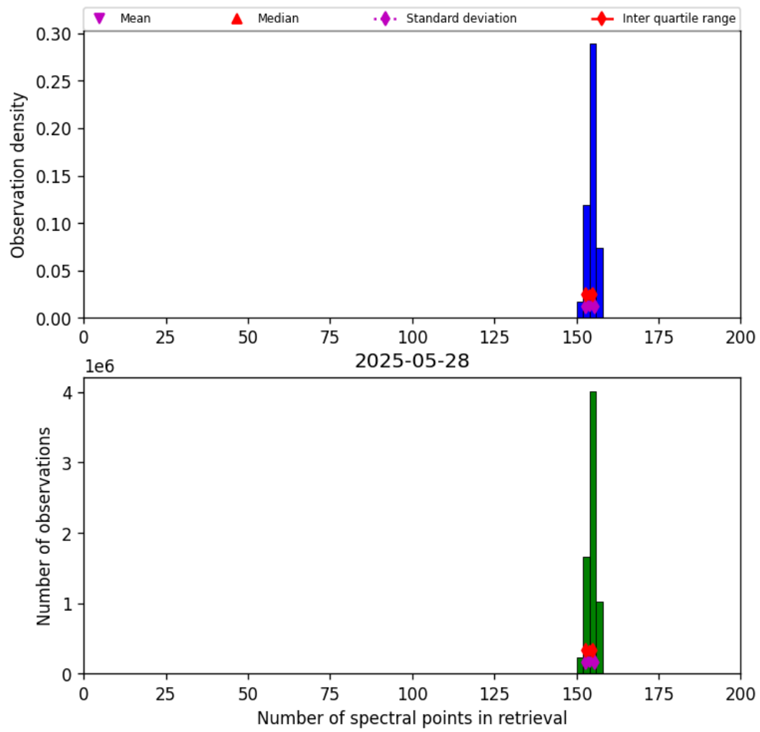
Figure 16: Histogram of “Number of spectral points in retrieval” for 2025-05-28 to 2025-05-29
