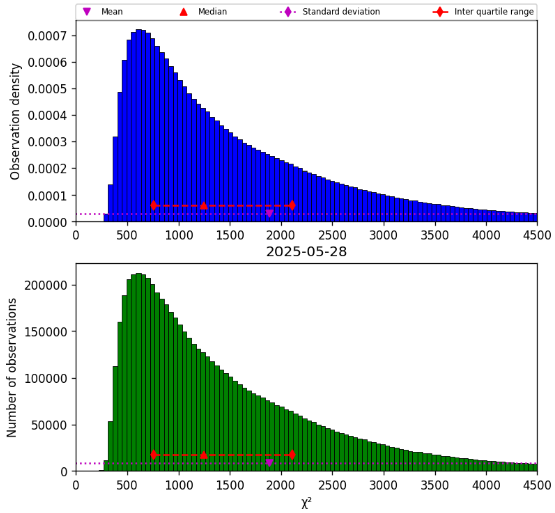
Figure 17: Histogram of “ \chi^2 ” for 2025-05-28 to 2025-05-29
