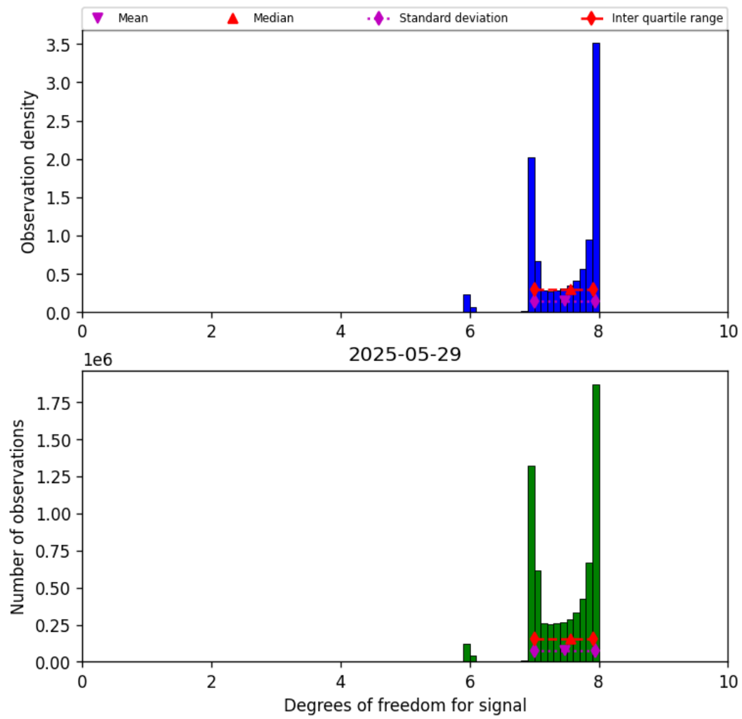
Figure 18: Histogram of “Degrees of freedom for signal” for 2025-05-29 to 2025-05-29
