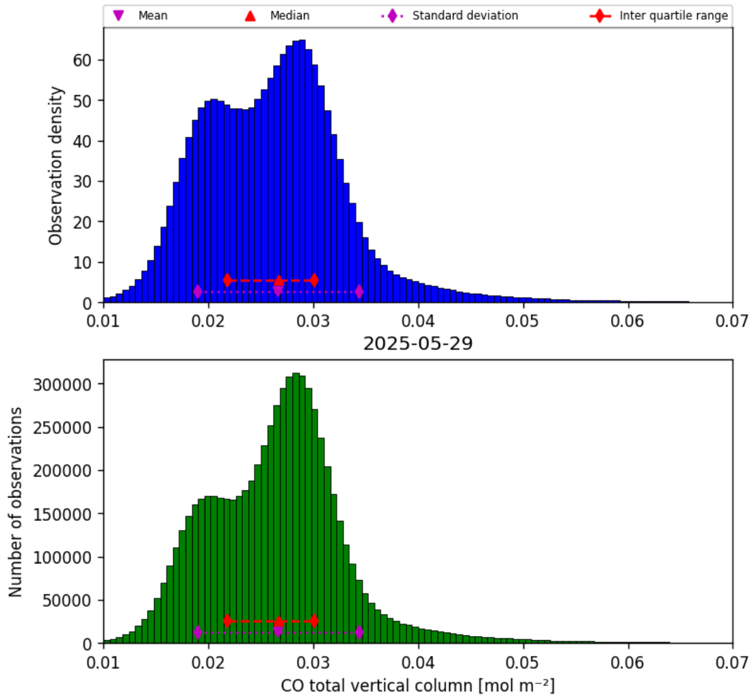
Figure 14: Histogram of “CO total vertical column” for 2025-05-29 to 2025-05-29
