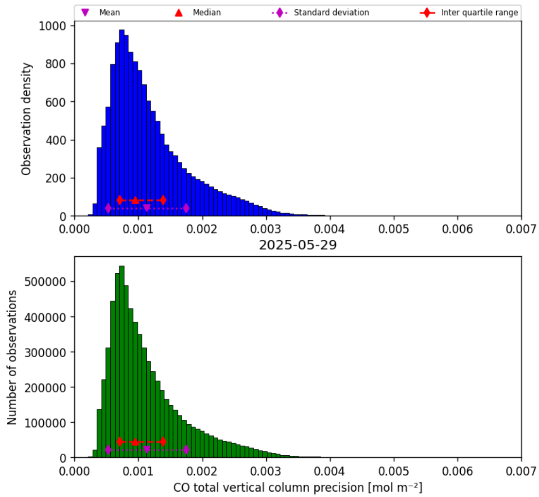
Figure 15: Histogram of “CO total vertical column precision” for 2025-05-29 to 2025-05-29
