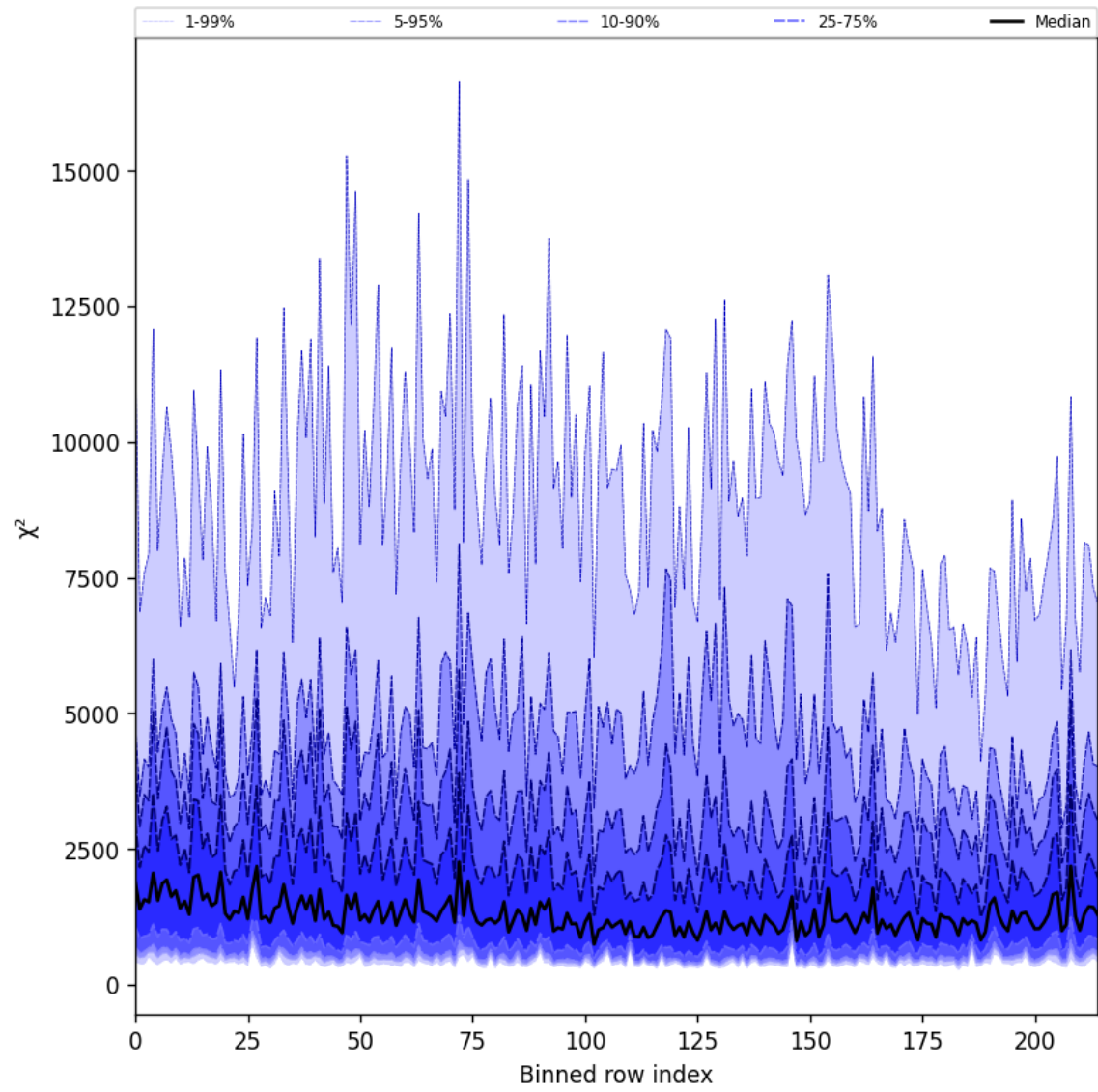
Figure 24: Along track statistics of “ \chi^2 ” for 2025-05-29 to 2025-05-29
