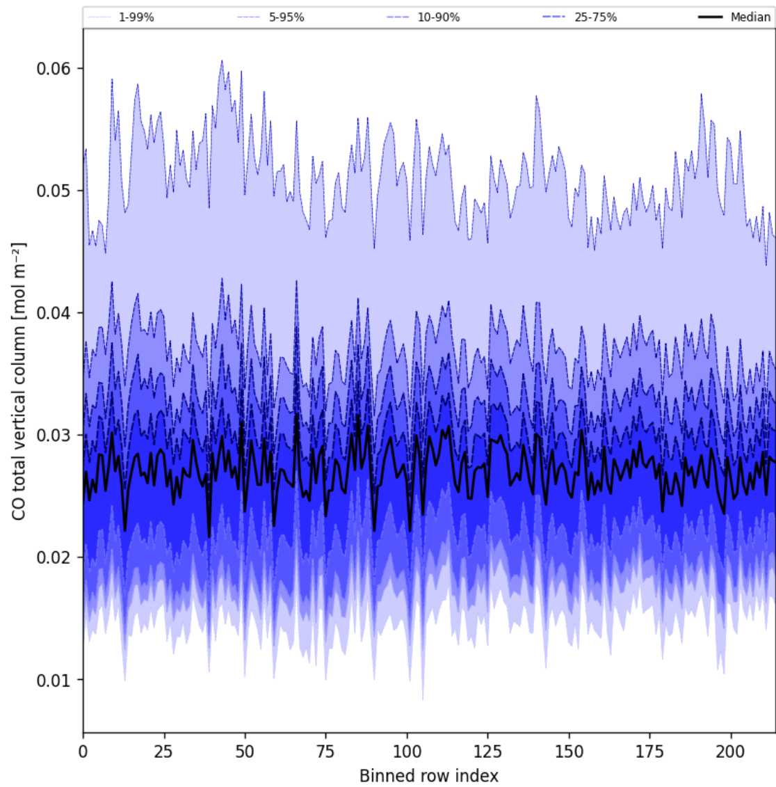
Figure 21: Along track statistics of “CO total vertical column” for 2025-05-29 to 2025-05-29
