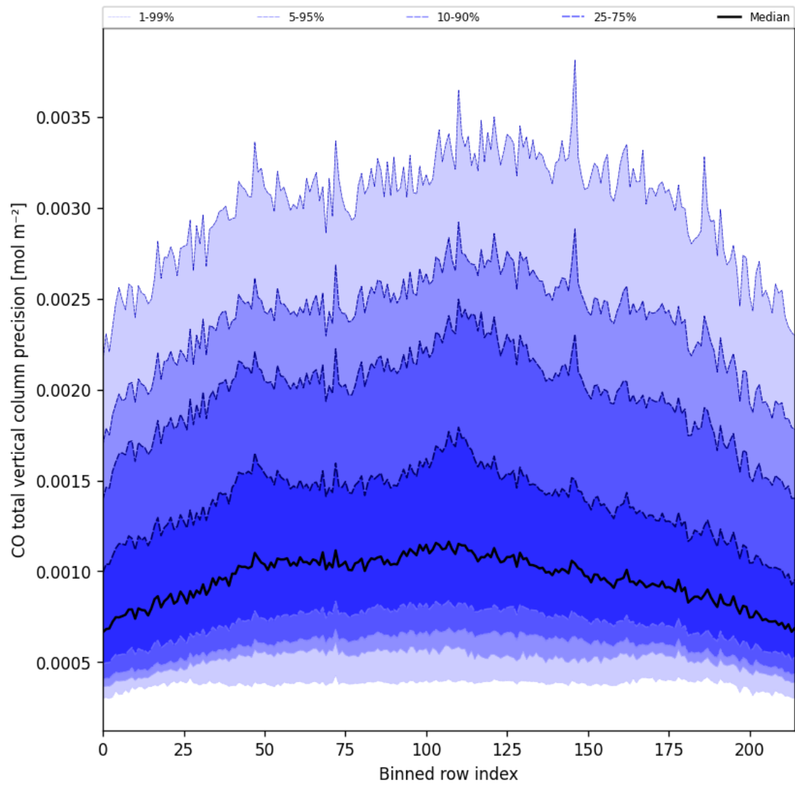
Figure 22: Along track statistics of “CO total vertical column precision” for 2025-05-29 to 2025-05-29
