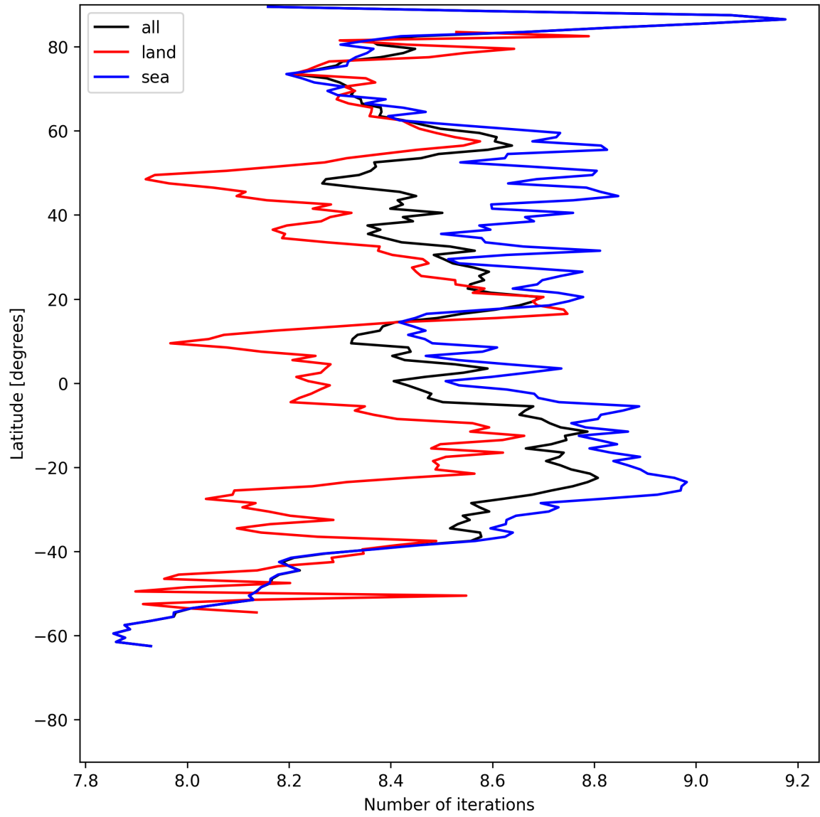
Figure 12: Zonal average of “Number of iterations” for 2025-05-29 to 2025-05-29.
