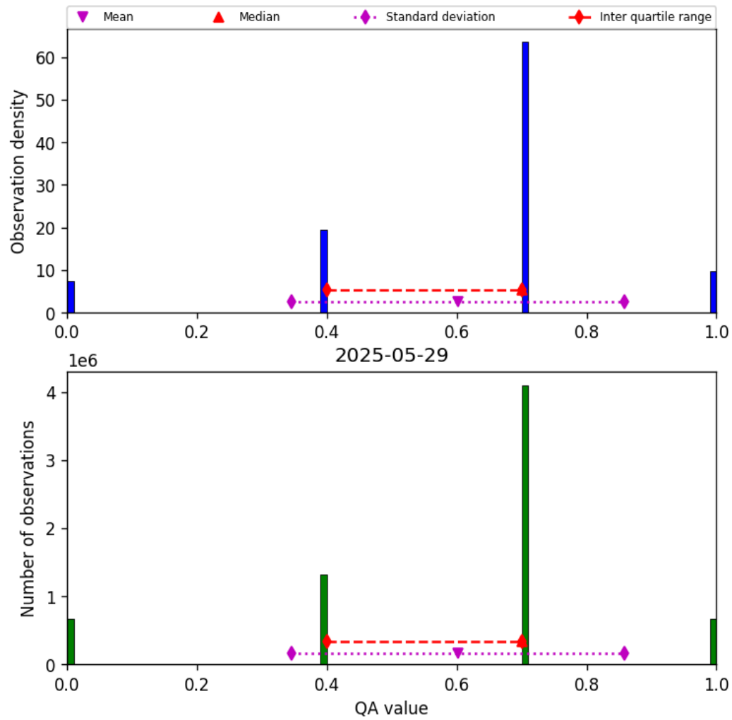
Figure 13: Histogram of “QA value” for 2025-05-29 to 2025-05-29
