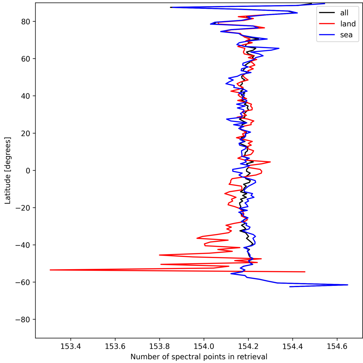
Figure 9: Zonal average of “Number of spectral points in retrieval” for 2025-05-29 to 2025-05-29.
