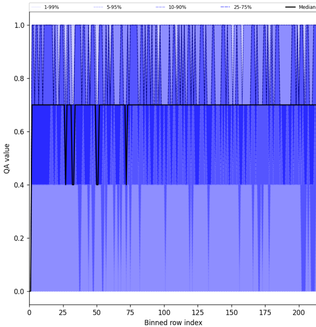
Figure 20: Along track statistics of “QA value” for 2025-05-29 to 2025-05-29
