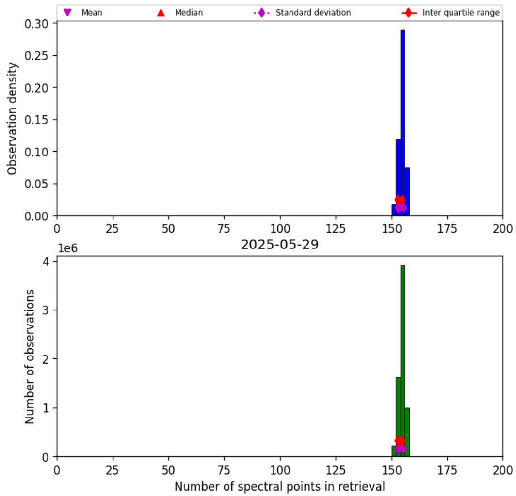
Figure 16: Histogram of “Number of spectral points in retrieval” for 2025-05-29 to 2025-05-29
