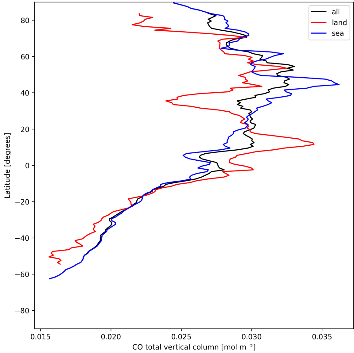
Figure 7: Zonal average of “CO total vertical column” for 2025-05-29 to 2025-05-29.
