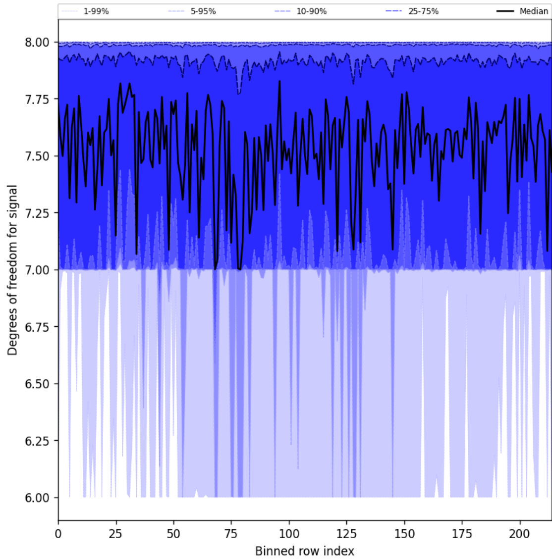
Figure 25: Along track statistics of “Degrees of freedom for signal” for 2025-05-29 to 2025-05-29
