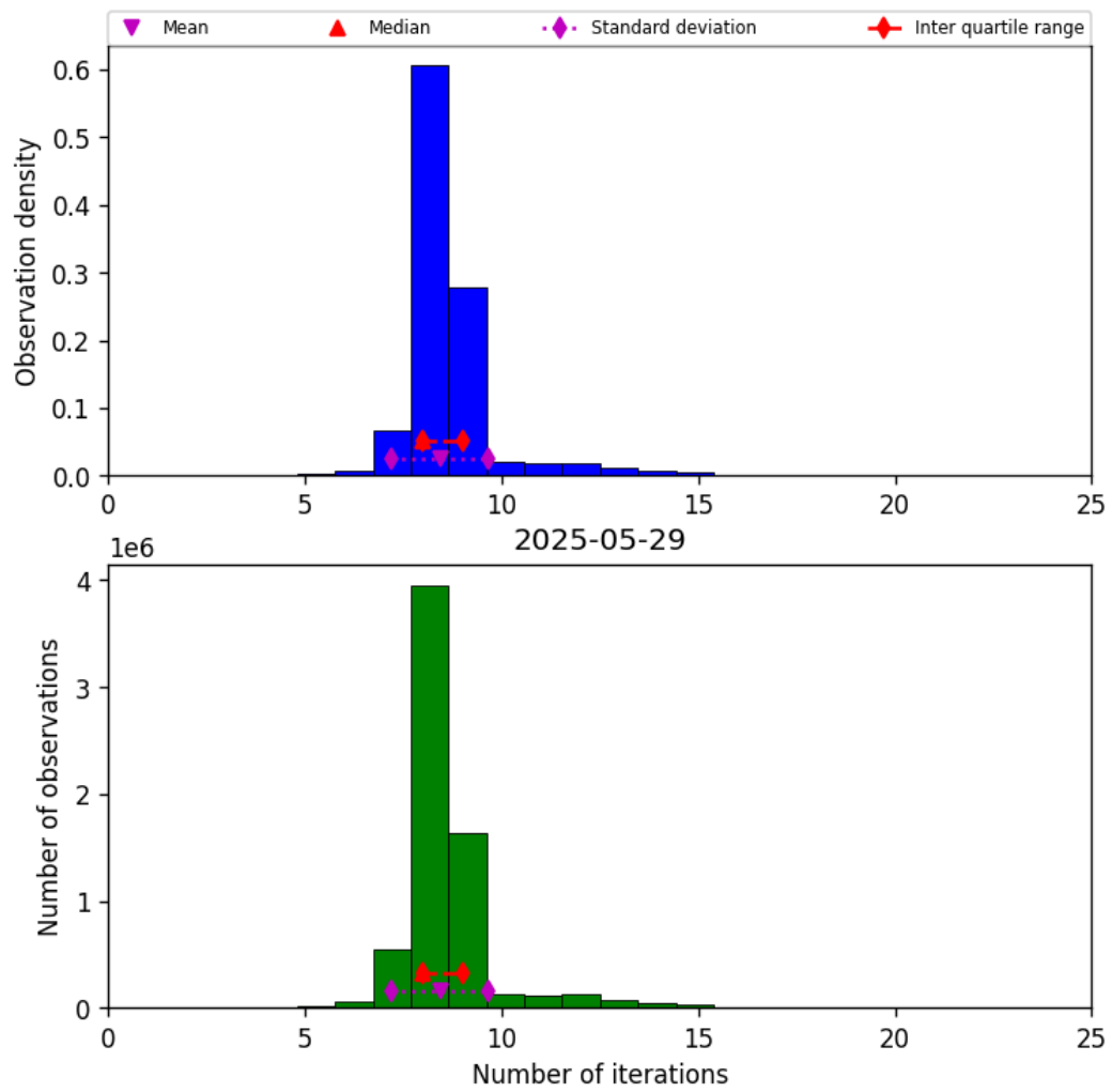
Figure 19: Histogram of “Number of iterations” for 2025-05-29 to 2025-05-29
