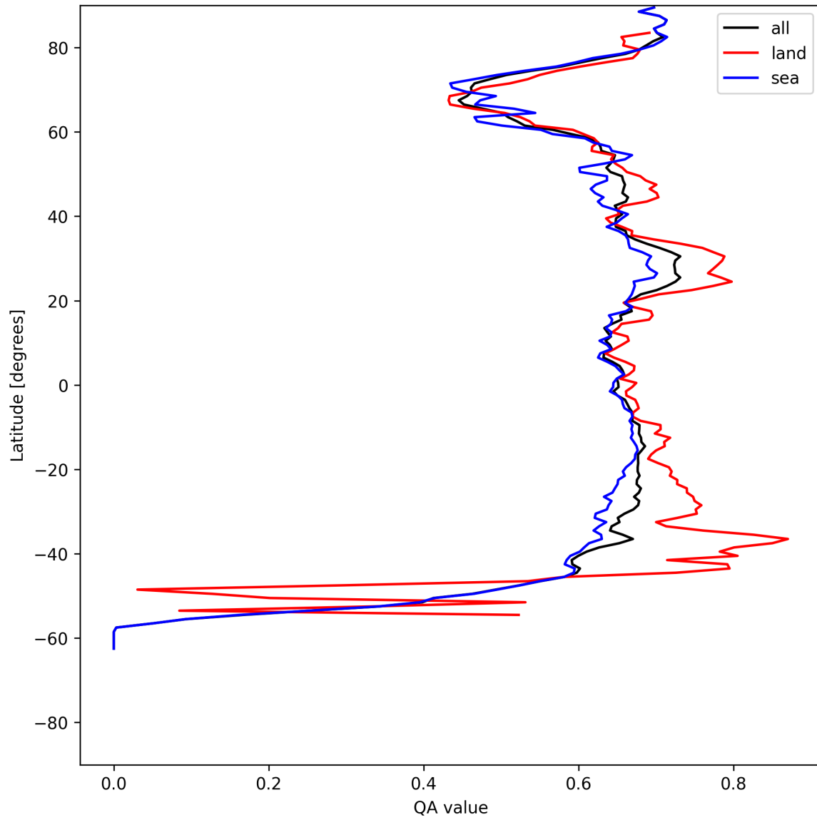
Figure 6: Zonal average of “QA value” for 2025-05-29 to 2025-05-29.
