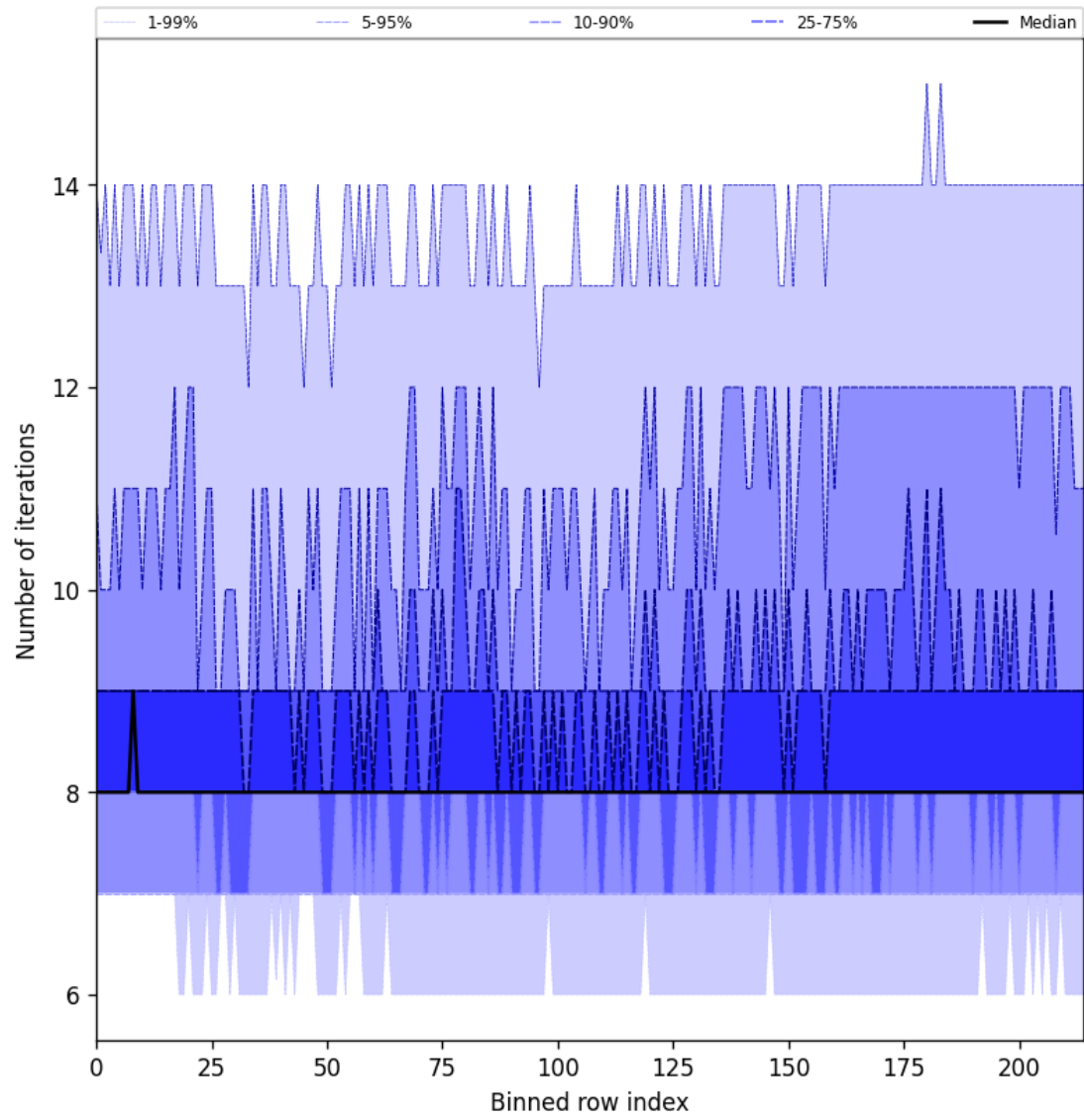
Figure 26: Along track statistics of “Number of iterations” for 2025-05-29 to 2025-05-29
