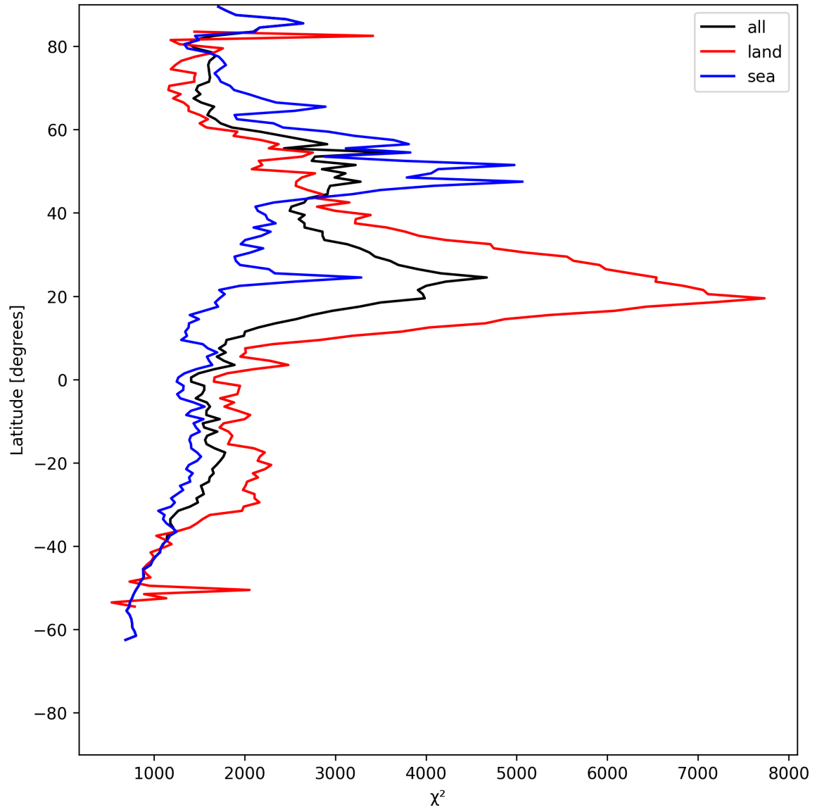
Figure 10: Zonal average of “ \chi^2 ” for 2025-05-29 to 2025-05-29.
