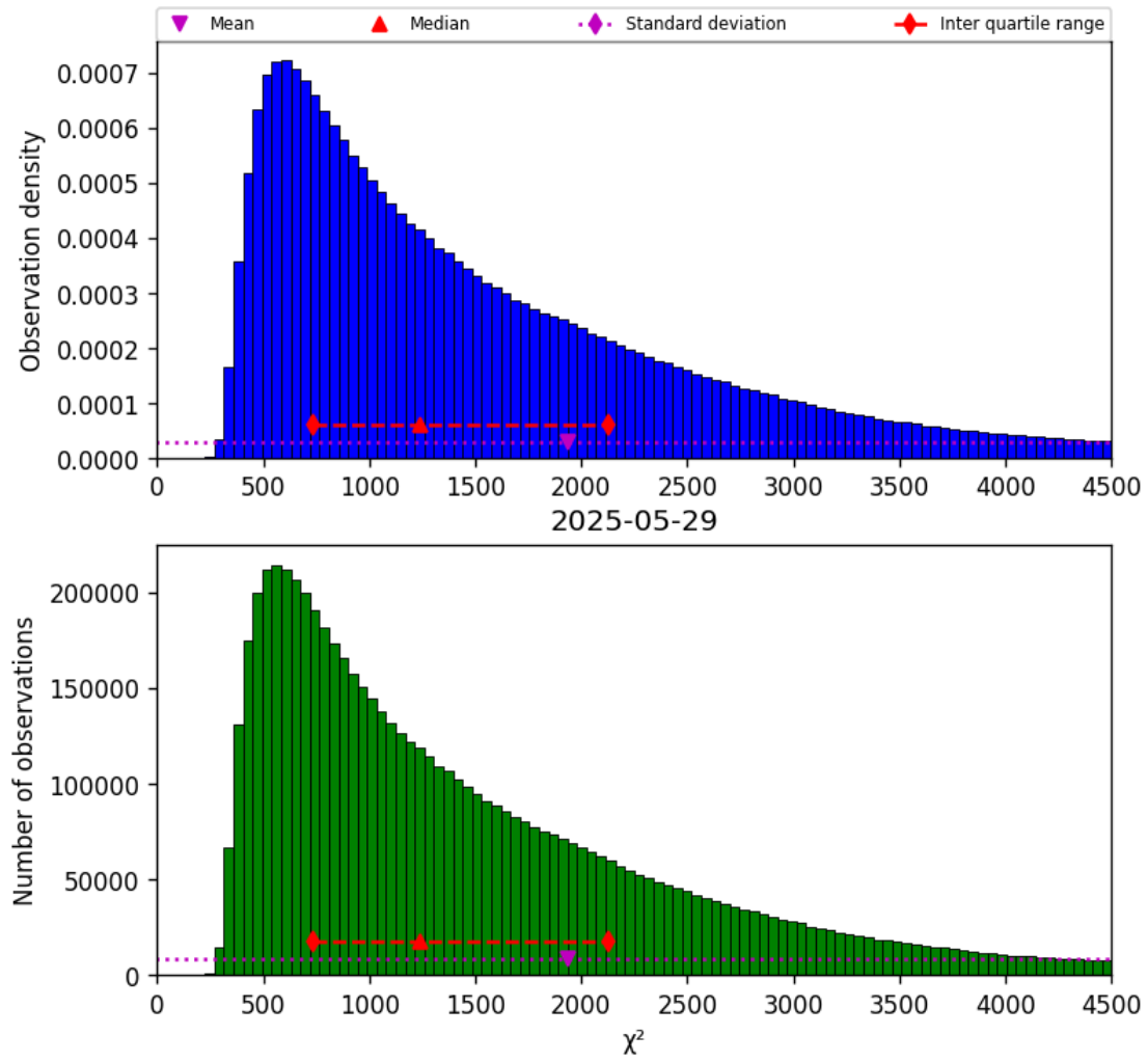
Figure 17: Histogram of " \chi^2 " for 2025-05-29 to 2025-05-29
