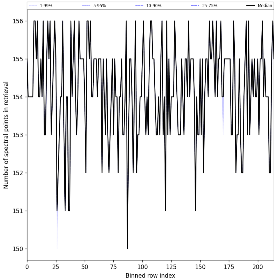
Figure 23: Along track statistics of “Number of spectral points in retrieval” for 2025-05-29 to 2025-05-29
