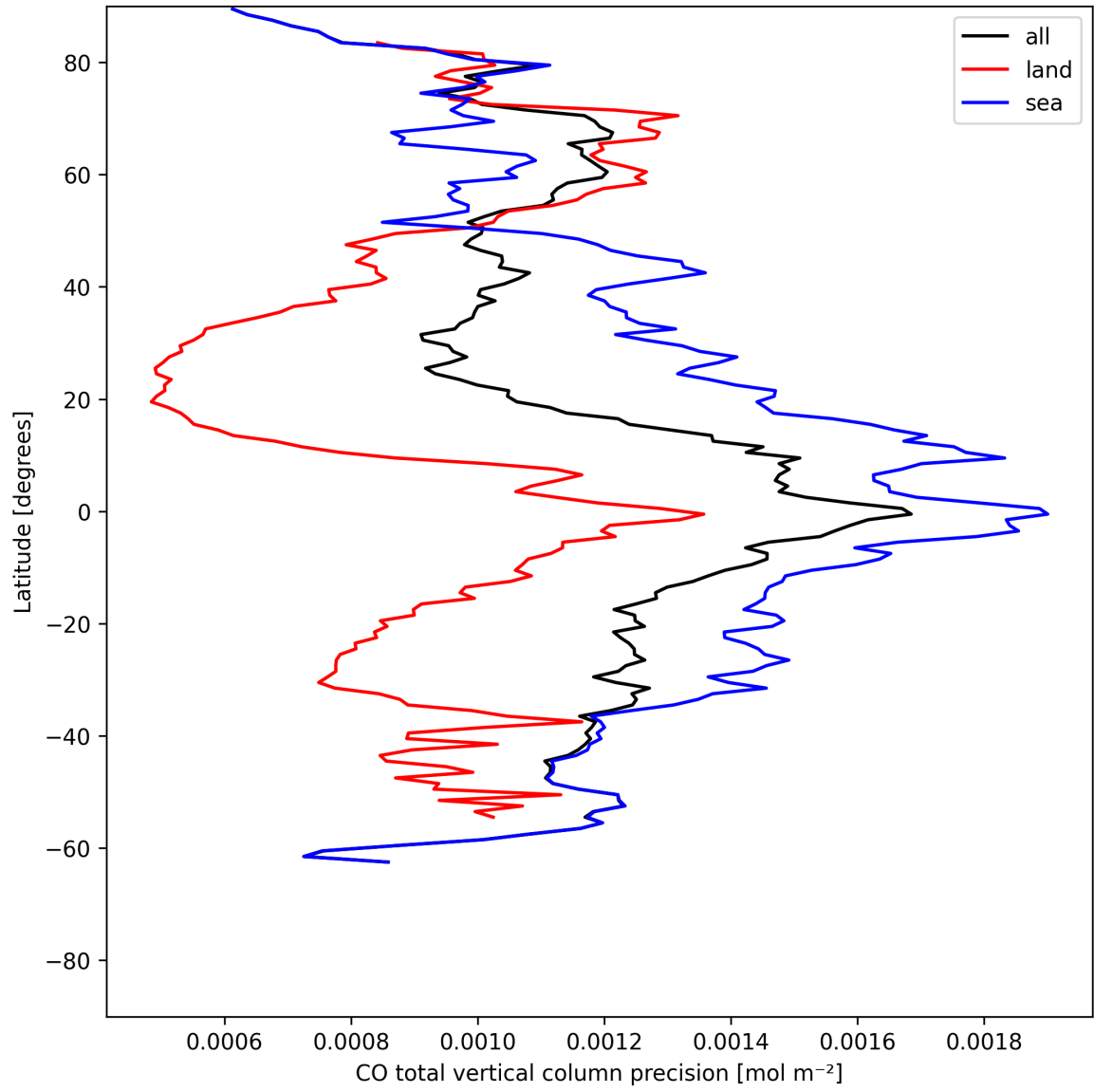
Figure 8: Zonal average of “CO total vertical column precision” for 2025-05-29 to 2025-05-29.
