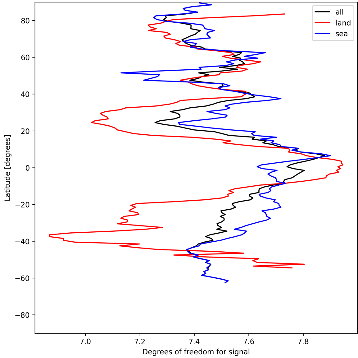
Figure 11: Zonal average of “Degrees of freedom for signal” for 2025-05-29 to 2025-05-29.
