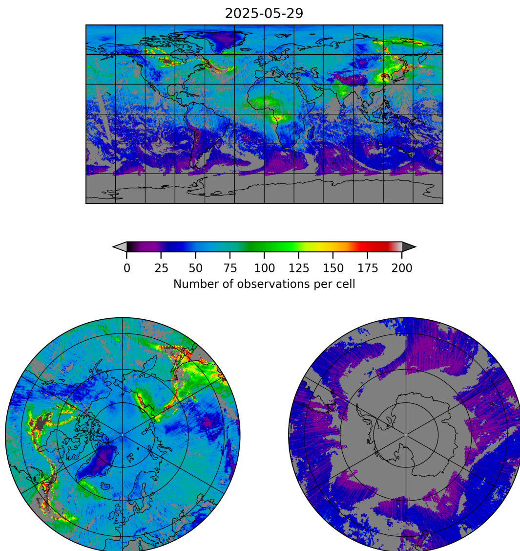
Figure 5: Map of the number of observations for 2025-05-29 to 2025-05-29
