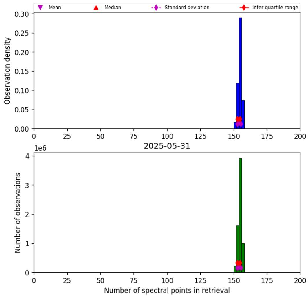
Figure 16: Histogram of “Number of spectral points in retrieval” for 2025-05-31 to 2025-06-01
