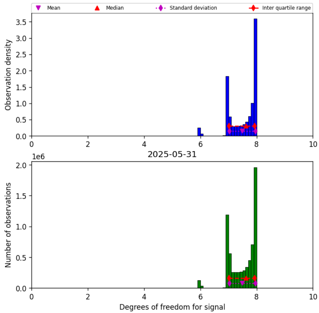
Figure 18: Histogram of “Degrees of freedom for signal” for 2025-05-31 to 2025-06-01
