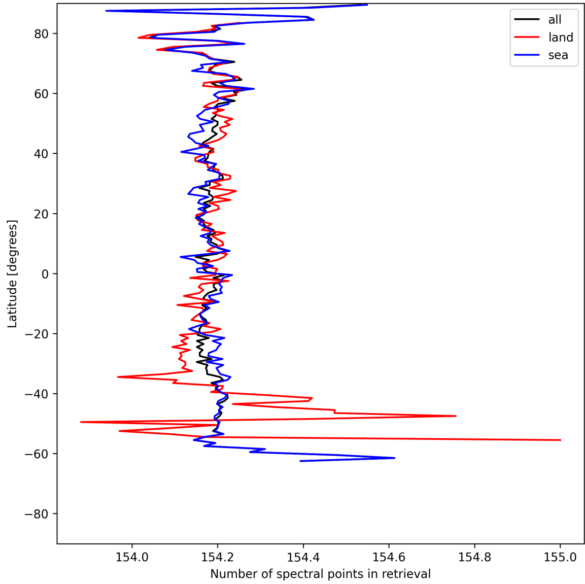
Figure 9: Zonal average of “Number of spectral points in retrieval” for 2025-05-31 to 2025-06-01.
