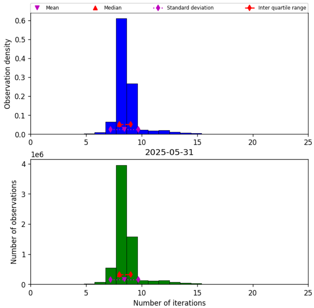
Figure 19: Histogram of “Number of iterations” for 2025-05-31 to 2025-06-01
