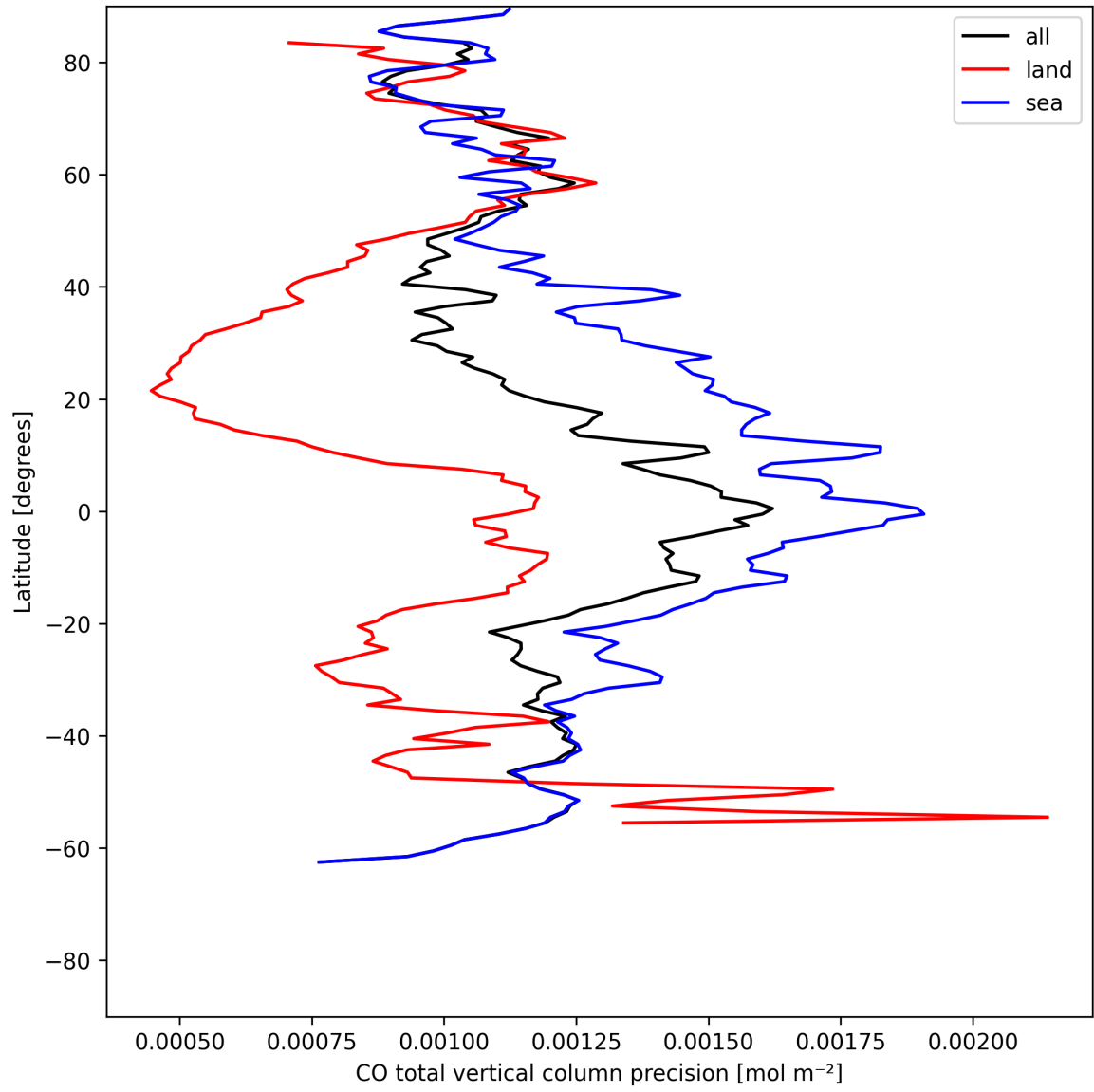
Figure 8: Zonal average of “CO total vertical column precision” for 2025-05-31 to 2025-06-01.
