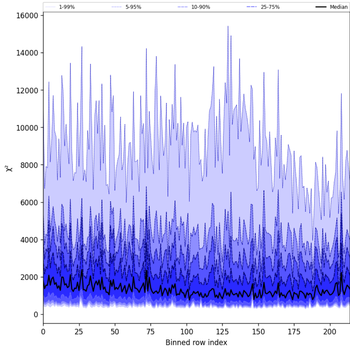
Figure 24: Along track statistics of “ \chi^2 ” for 2025-05-31 to 2025-06-01
