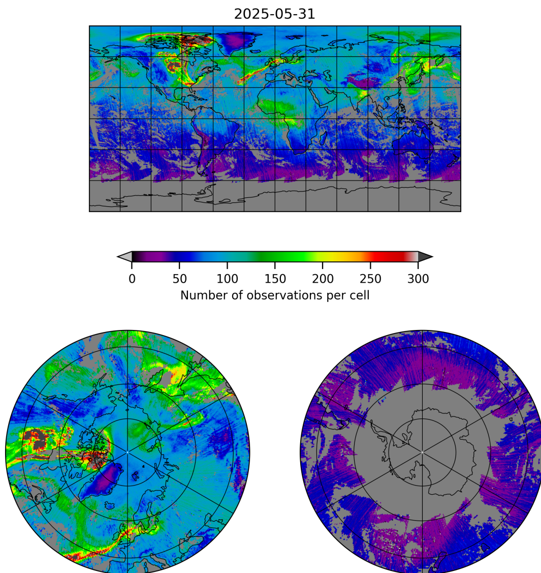
Figure 5: Map of the number of observations for 2025-05-31 to 2025-06-01
