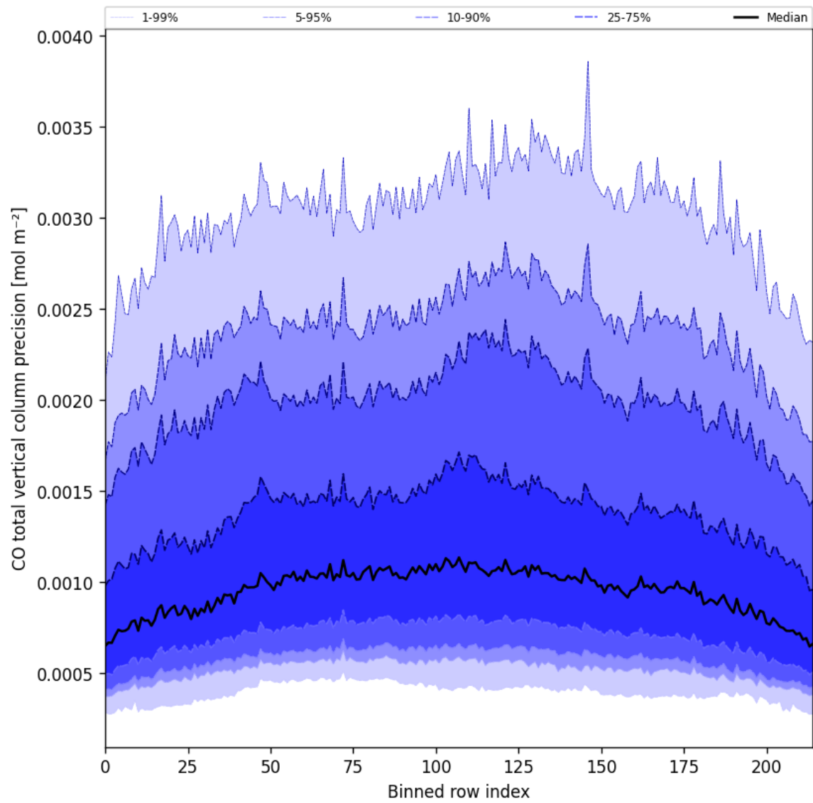
Figure 22: Along track statistics of “CO total vertical column precision” for 2025-05-31 to 2025-06-01
