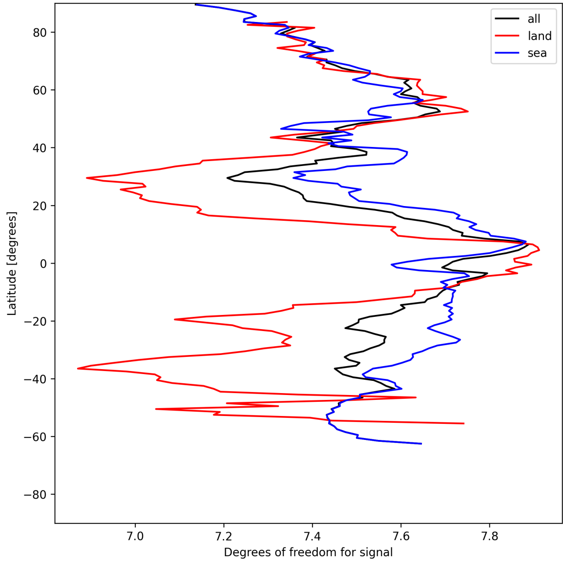
Figure 11: Zonal average of “Degrees of freedom for signal” for 2025-05-31 to 2025-06-01.
