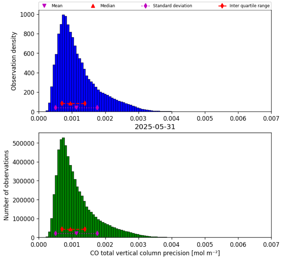
Figure 15: Histogram of “CO total vertical column precision” for 2025-05-31 to 2025-06-01
