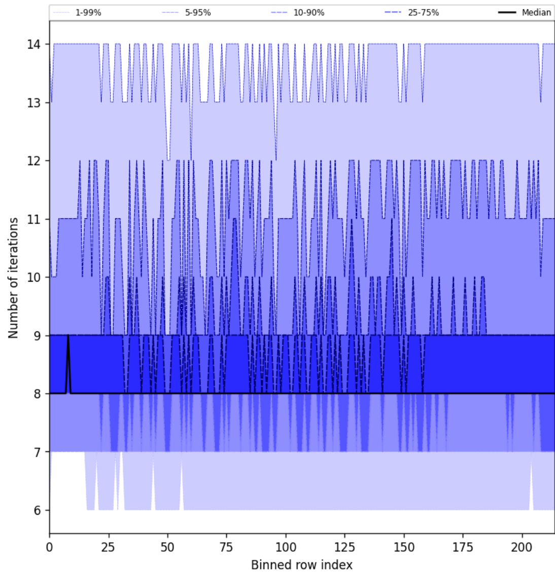
Figure 26: Along track statistics of “Number of iterations” for 2025-05-31 to 2025-06-01
