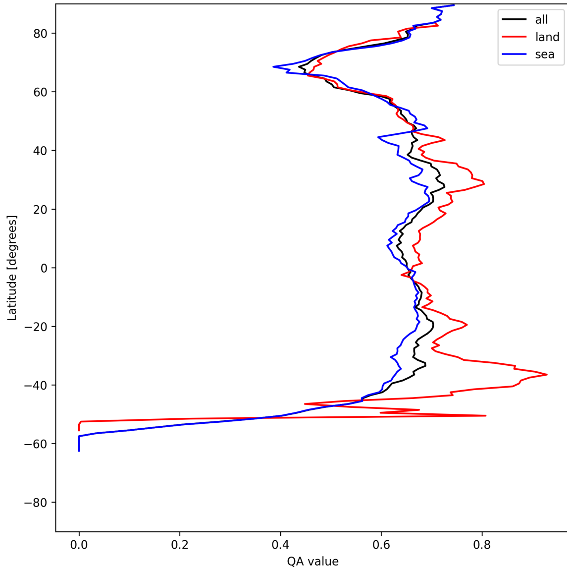
Figure 6: Zonal average of “QA value” for 2025-05-31 to 2025-06-01.
