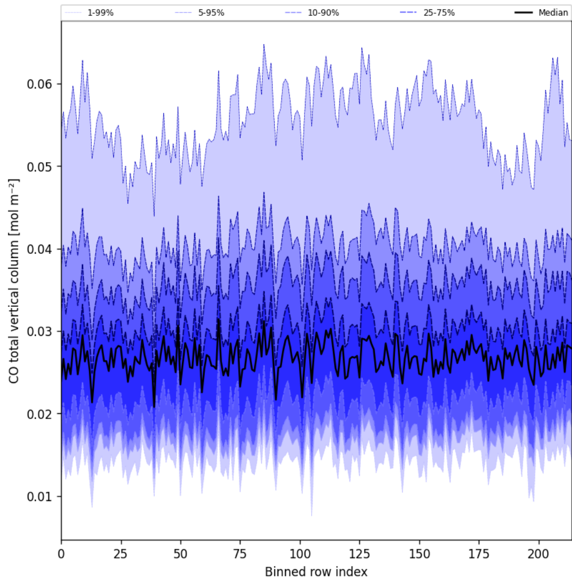
Figure 21: Along track statistics of “CO total vertical column” for 2025-05-31 to 2025-06-01
