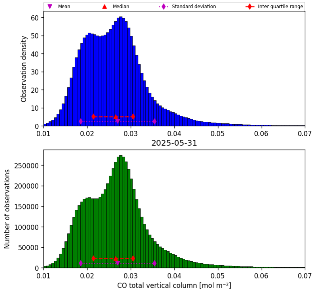
Figure 14: Histogram of “CO total vertical column” for 2025-05-31 to 2025-06-01
