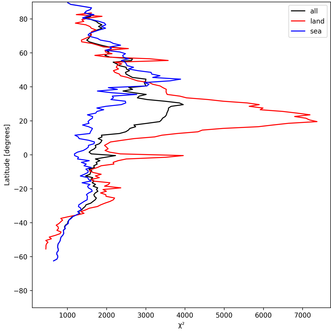
Figure 10: Zonal average of “ \chi^2 ” for 2025-05-31 to 2025-06-01.
