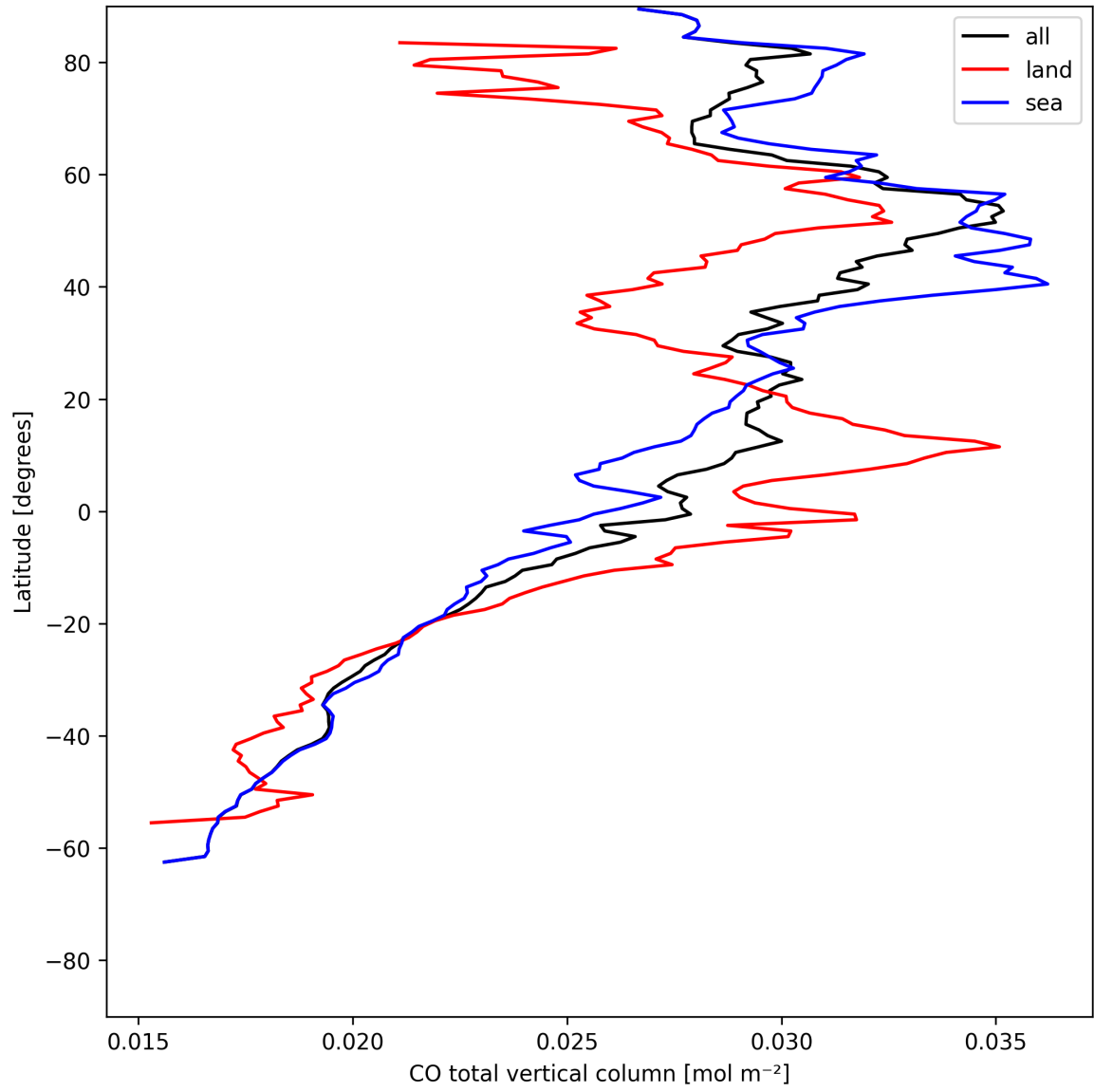
Figure 7: Zonal average of “CO total vertical column” for 2025-05-31 to 2025-06-01.
