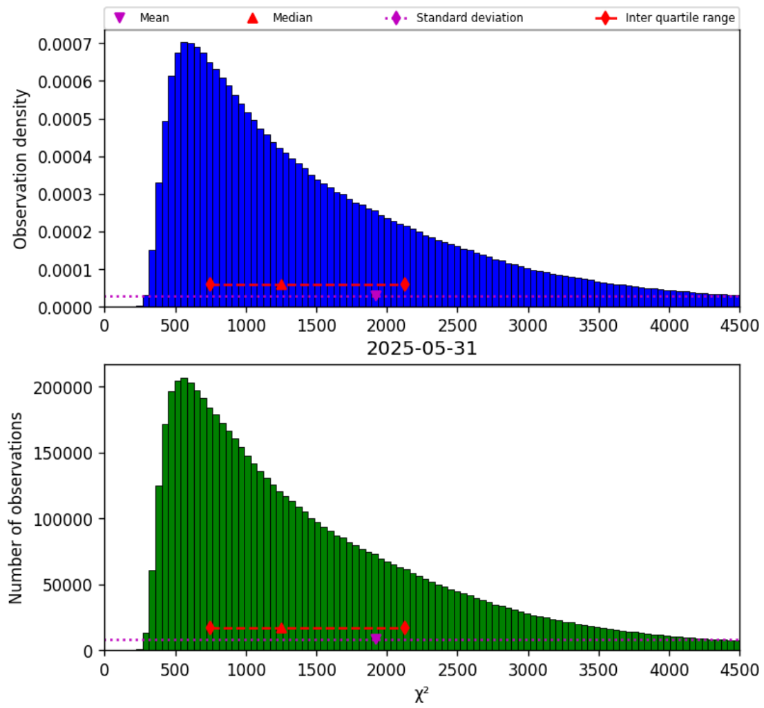
Figure 17: Histogram of " \chi^2 " for 2025-05-31 to 2025-06-01
