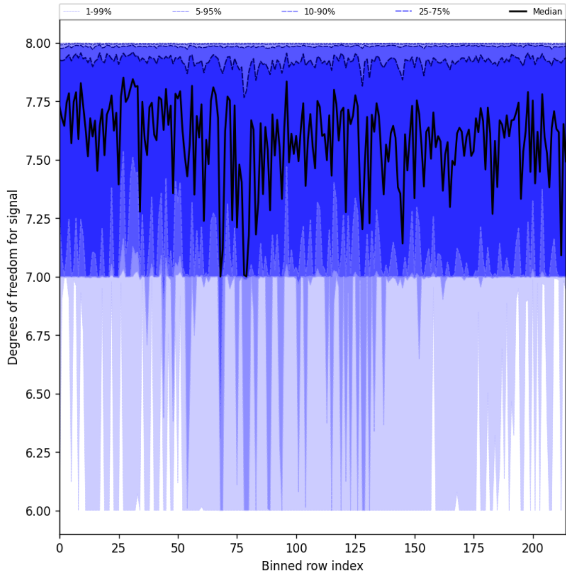
Figure 25: Along track statistics of “Degrees of freedom for signal” for 2025-05-31 to 2025-06-01
