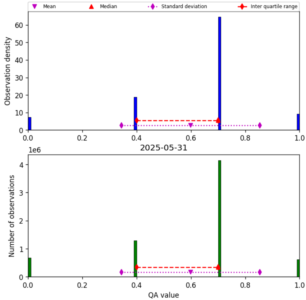
Figure 13: Histogram of “QA value” for 2025-05-31 to 2025-06-01
