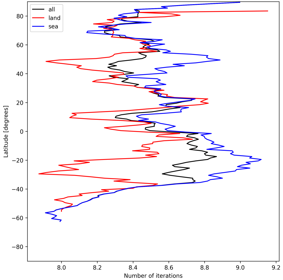
Figure 12: Zonal average of “Number of iterations” for 2025-05-31 to 2025-06-01.
