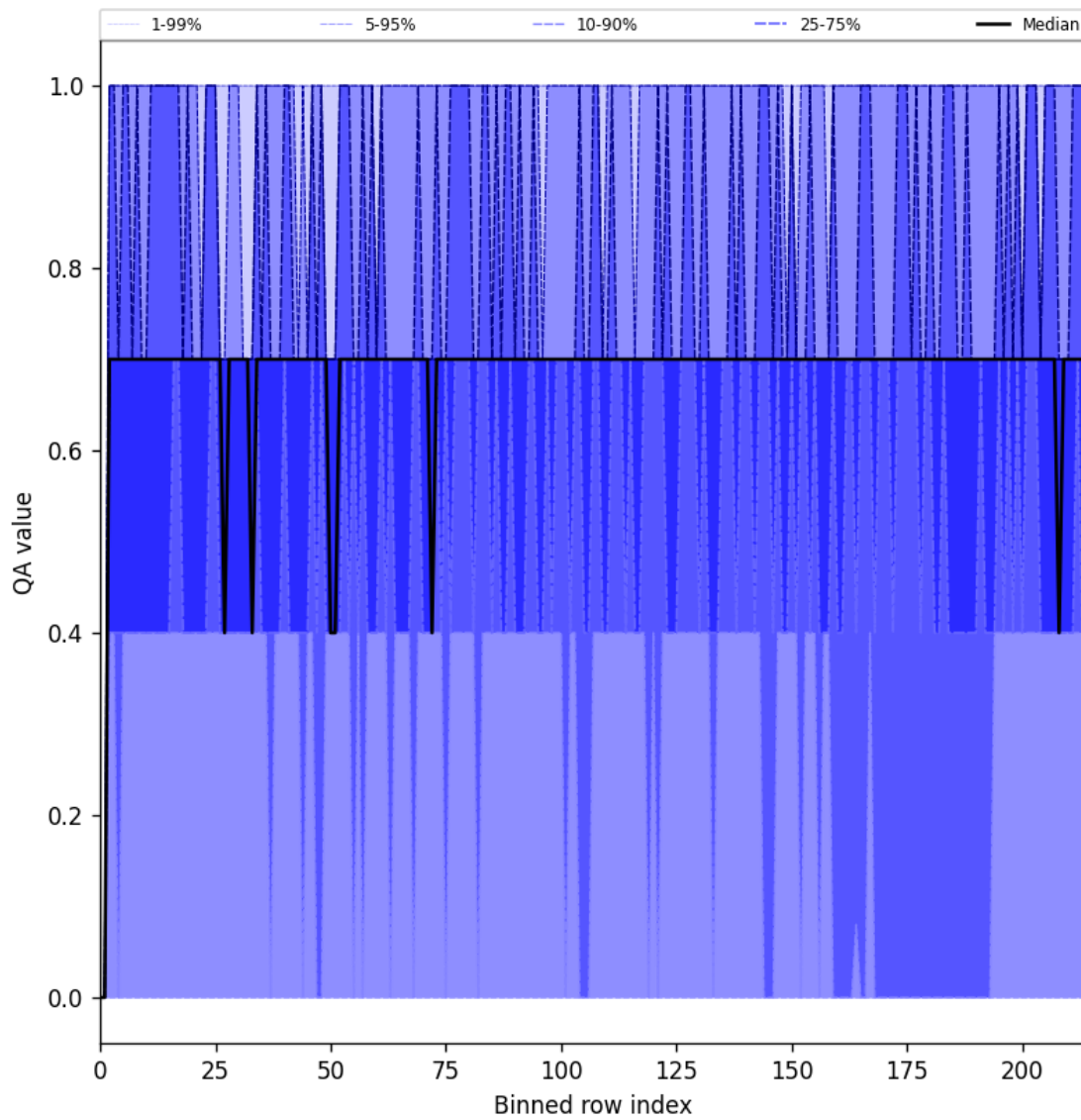
Figure 20: Along track statistics of “QA value” for 2025-05-31 to 2025-06-01
