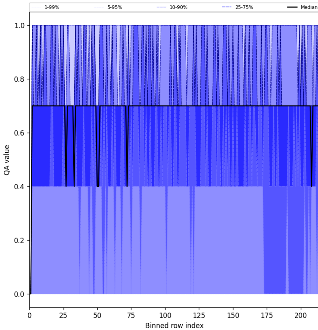
Figure 20: Along track statistics of “QA value” for 2025-06-01 to 2025-06-02
