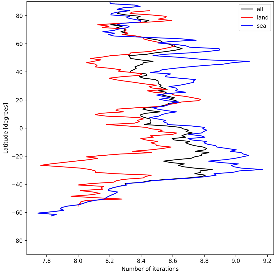
Figure 12: Zonal average of “Number of iterations” for 2025-06-01 to 2025-06-02.
