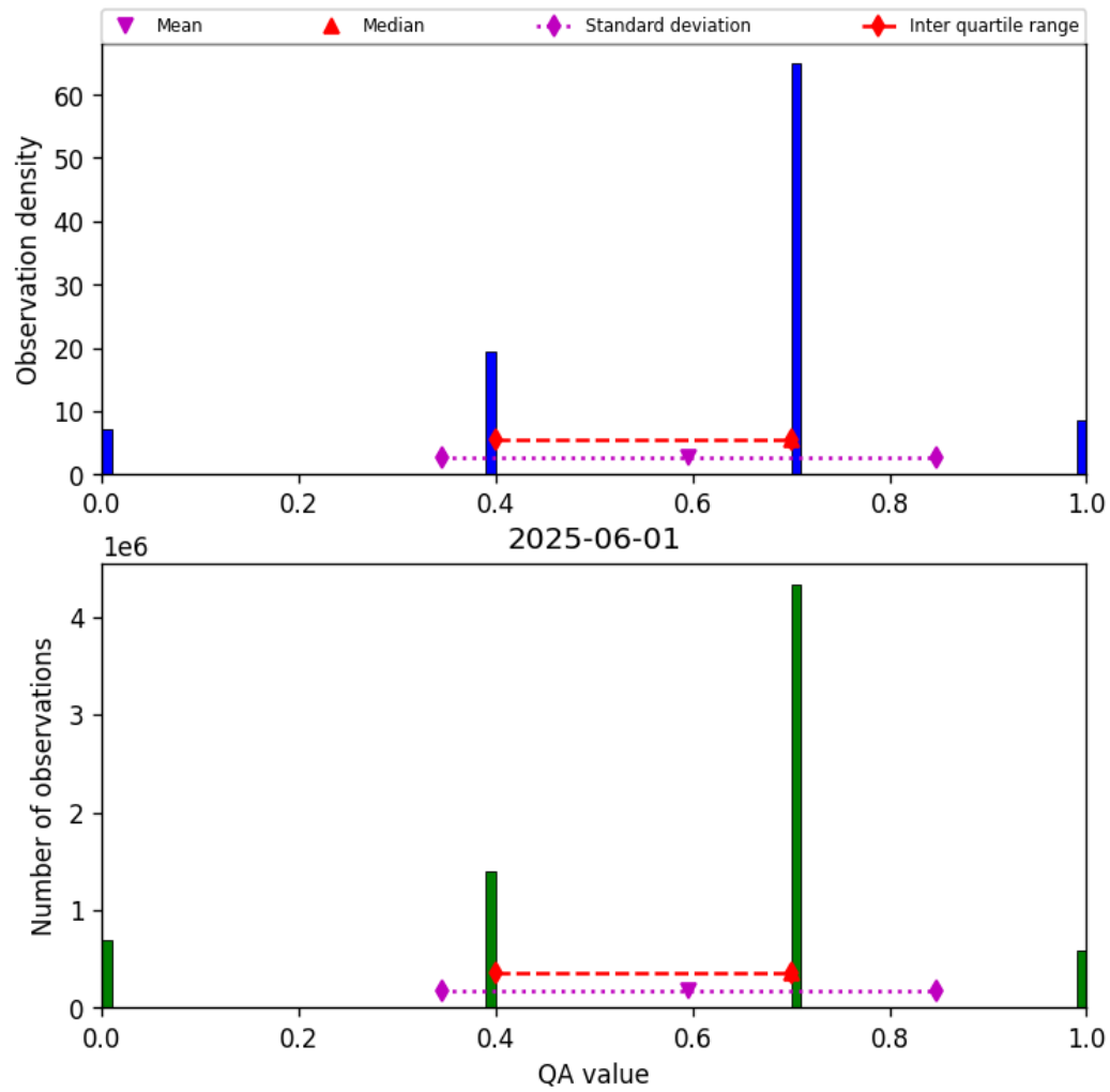
Figure 13: Histogram of “QA value” for 2025-06-01 to 2025-06-02
