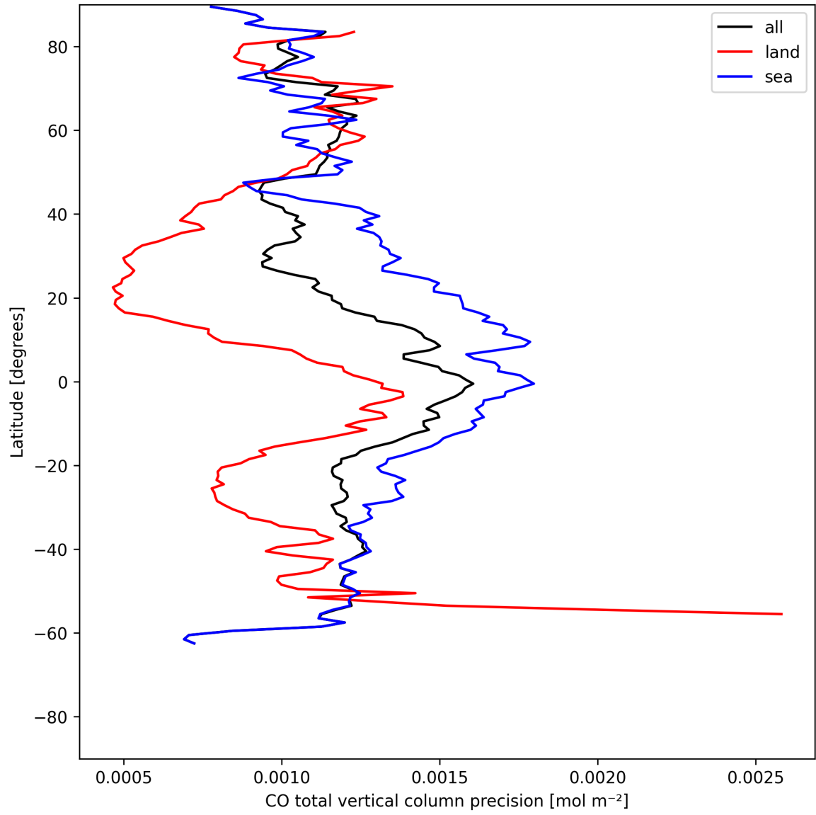
Figure 8: Zonal average of “CO total vertical column precision” for 2025-06-01 to 2025-06-02.
