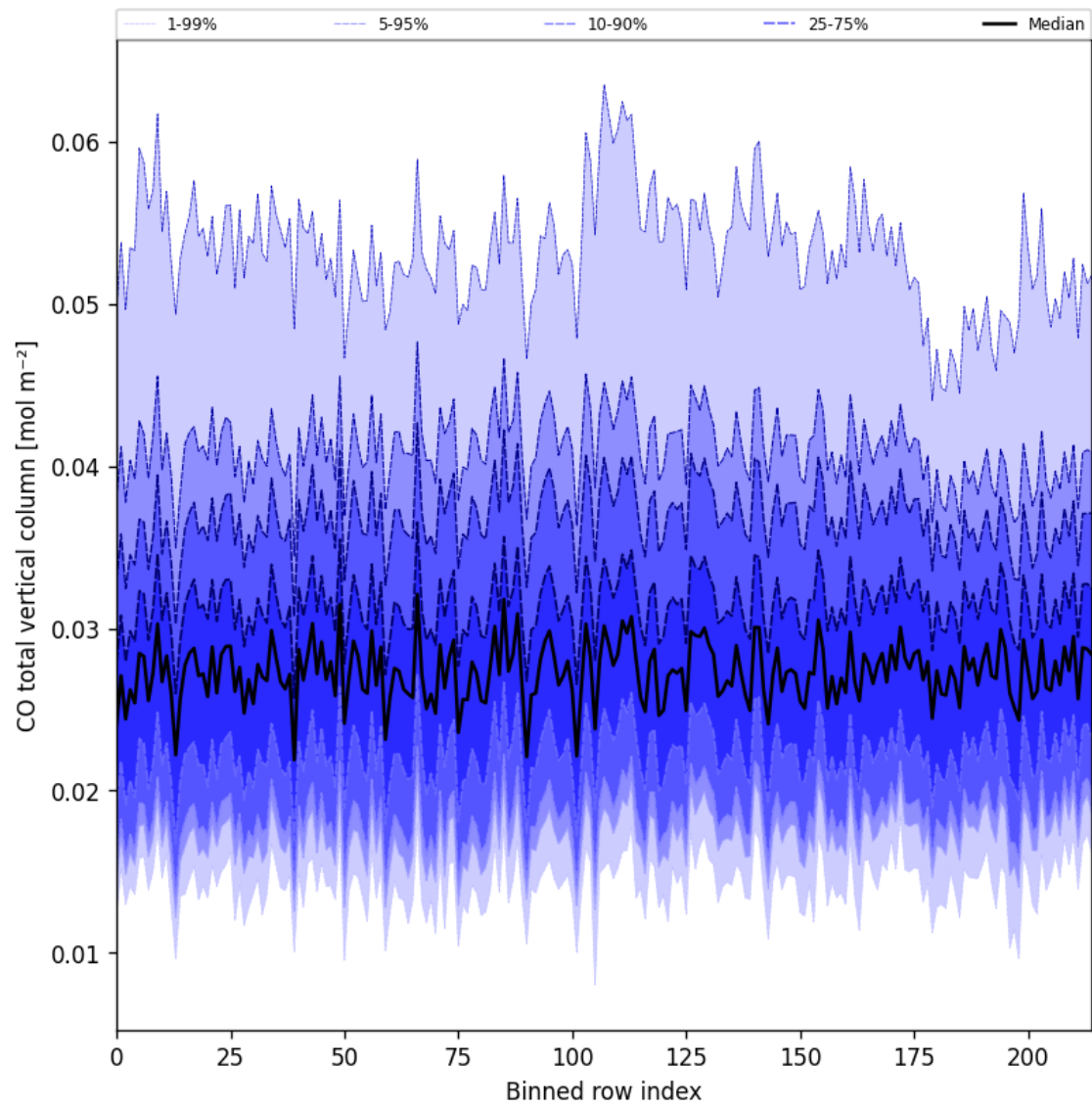
Figure 21: Along track statistics of “CO total vertical column” for 2025-06-01 to 2025-06-02
