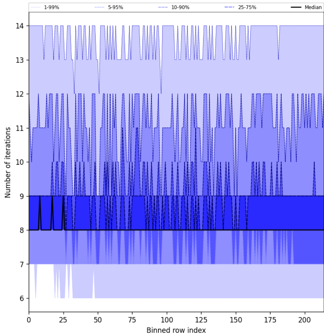
Figure 26: Along track statistics of “Number of iterations” for 2025-06-01 to 2025-06-02
