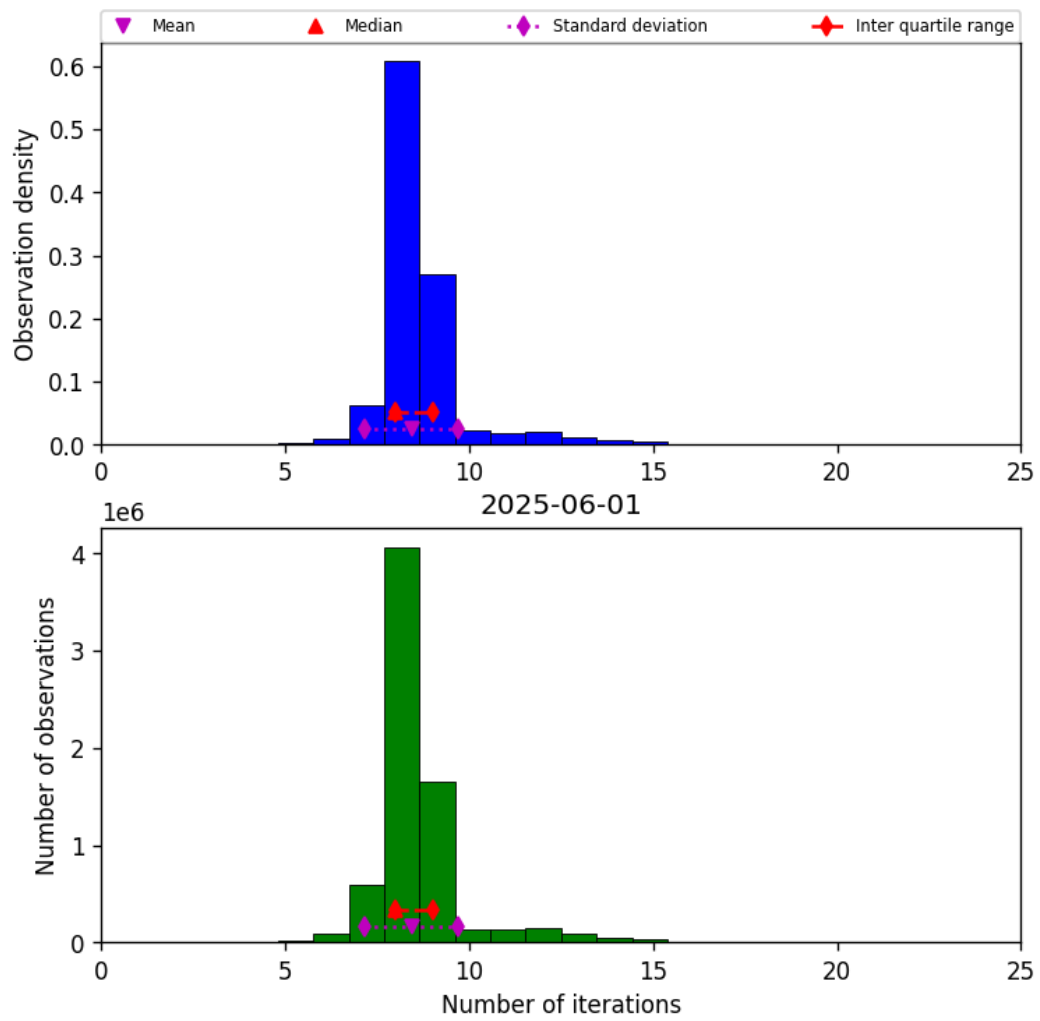
Figure 19: Histogram of “Number of iterations” for 2025-06-01 to 2025-06-02
