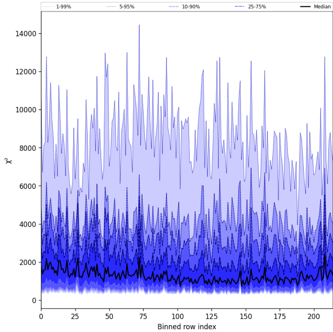
Figure 24: Along track statistics of “ \chi^2 ” for 2025-06-01 to 2025-06-02
