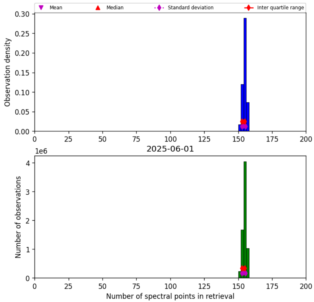
Figure 16: Histogram of “Number of spectral points in retrieval” for 2025-06-01 to 2025-06-02
