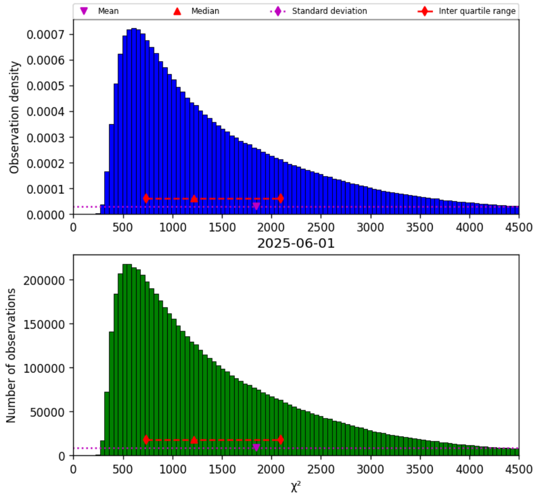
Figure 17: Histogram of " \chi^2 " for 2025-06-01 to 2025-06-02
