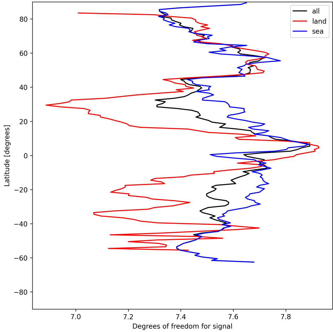
Figure 11: Zonal average of “Degrees of freedom for signal” for 2025-06-01 to 2025-06-02.
