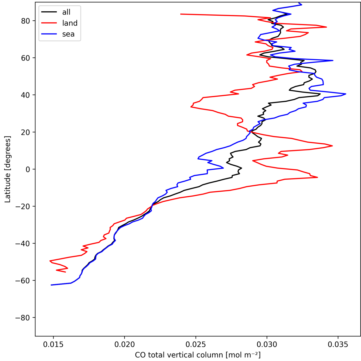
Figure 7: Zonal average of “CO total vertical column” for 2025-06-01 to 2025-06-02.
