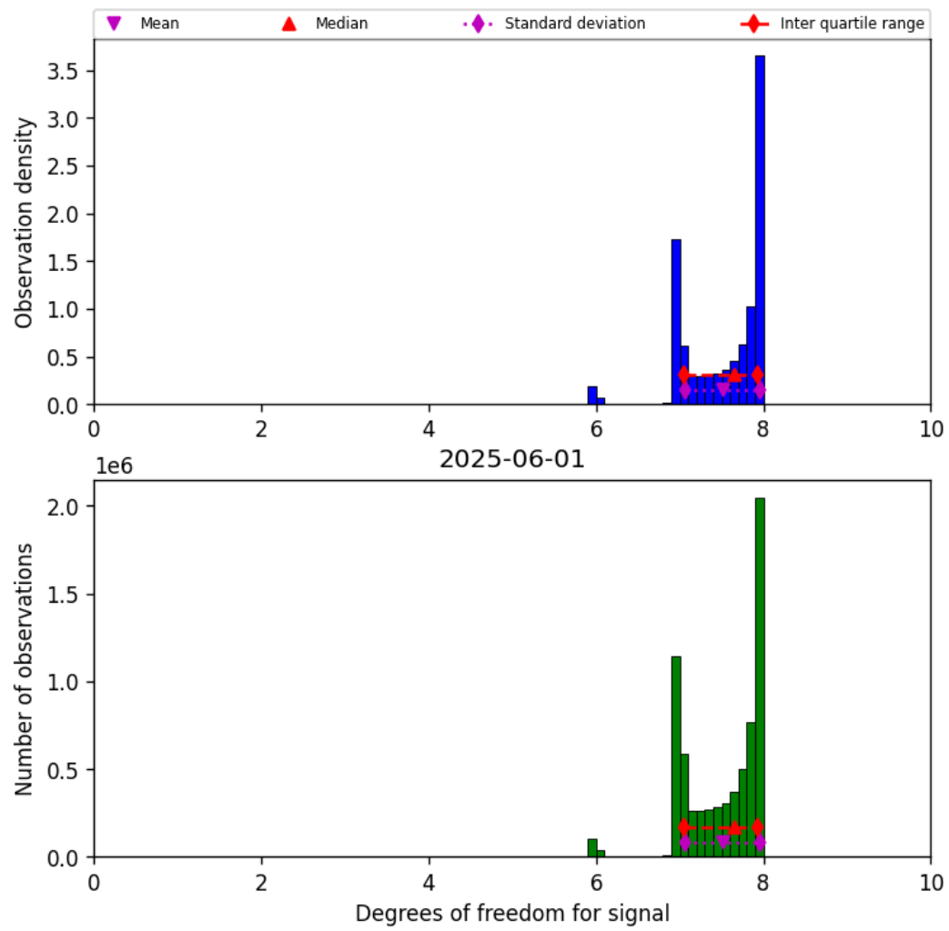
Figure 18: Histogram of “Degrees of freedom for signal” for 2025-06-01 to 2025-06-02
