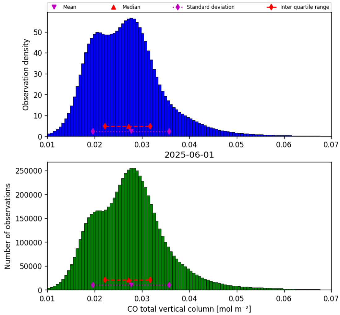
Figure 14: Histogram of “CO total vertical column” for 2025-06-01 to 2025-06-02
