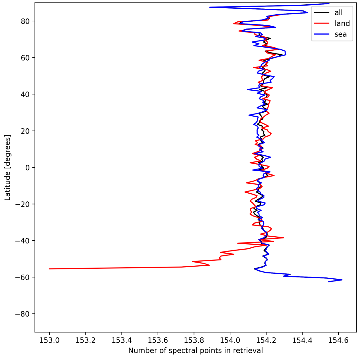
Figure 9: Zonal average of “Number of spectral points in retrieval” for 2025-06-01 to 2025-06-02.
