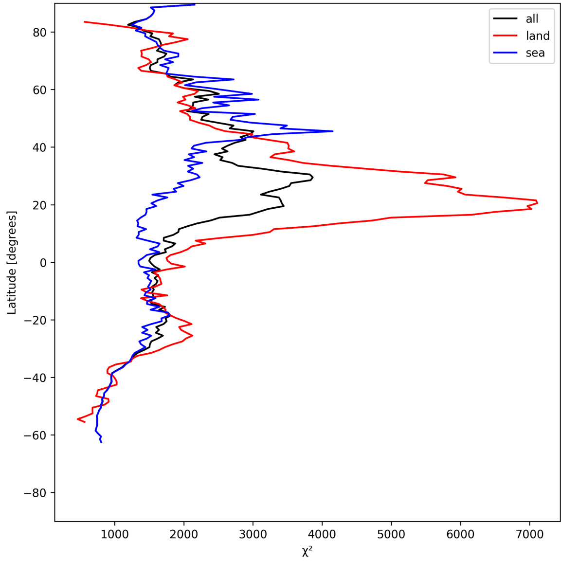
Figure 10: Zonal average of “ \chi^2 ” for 2025-06-01 to 2025-06-02.
