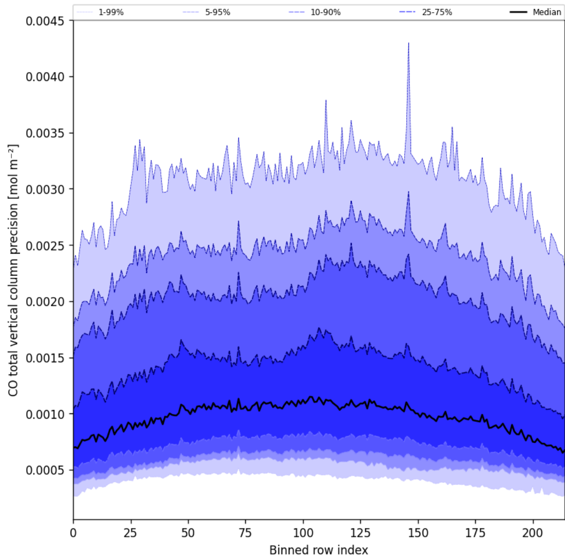
Figure 22: Along track statistics of “CO total vertical column precision” for 2025-06-01 to 2025-06-02
