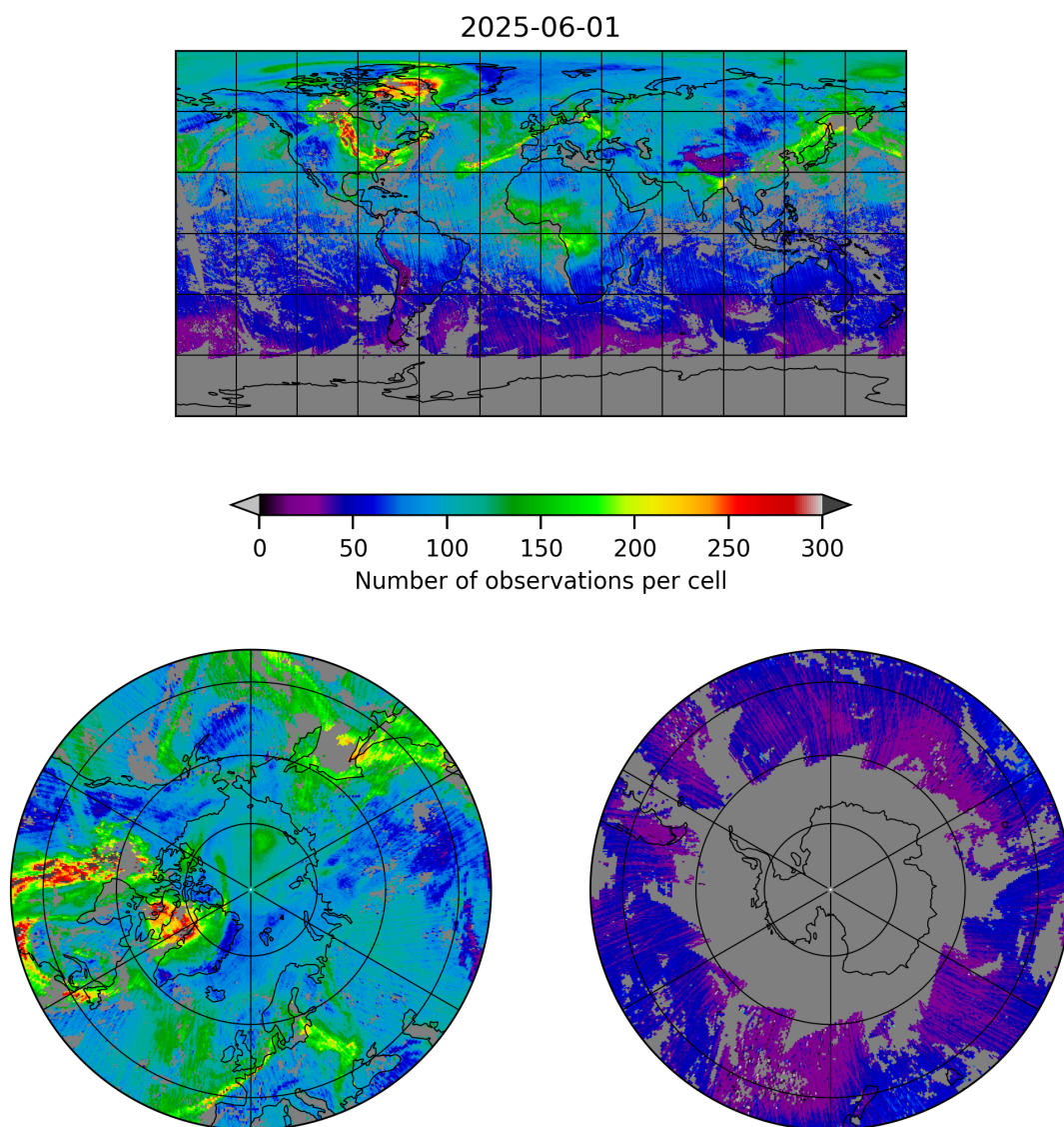
Figure 5: Map of the number of observations for 2025-06-01 to 2025-06-02
