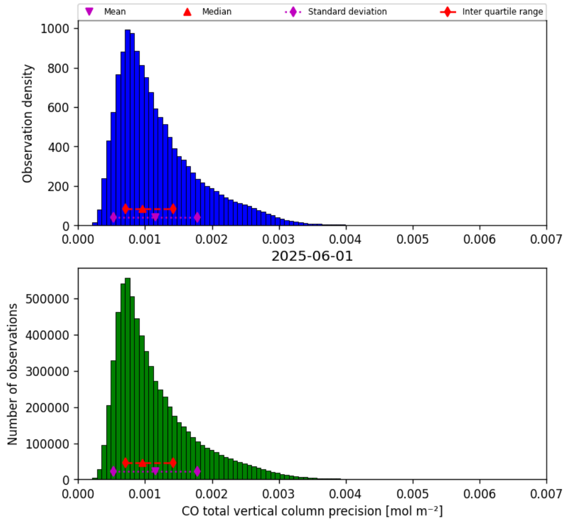
Figure 15: Histogram of “CO total vertical column precision” for 2025-06-01 to 2025-06-02
