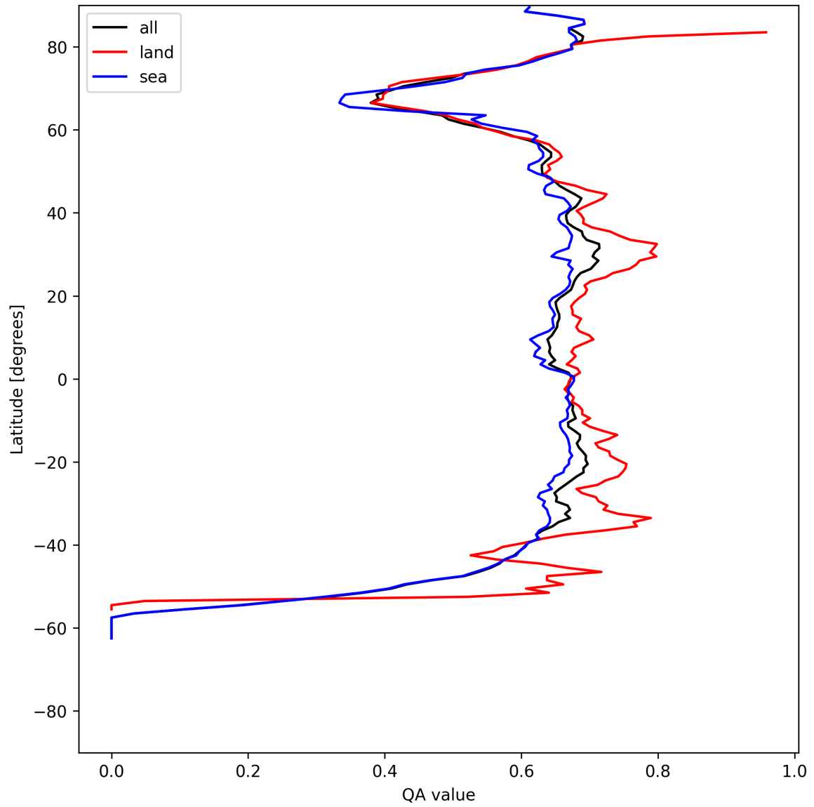
Figure 6: Zonal average of “QA value” for 2025-06-01 to 2025-06-02.
