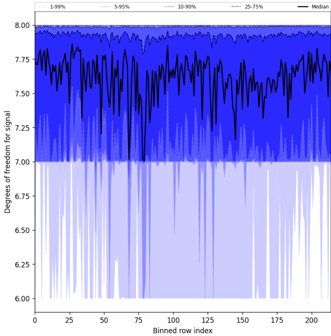
Figure 25: Along track statistics of “Degrees of freedom for signal” for 2025-06-01 to 2025-06-02
