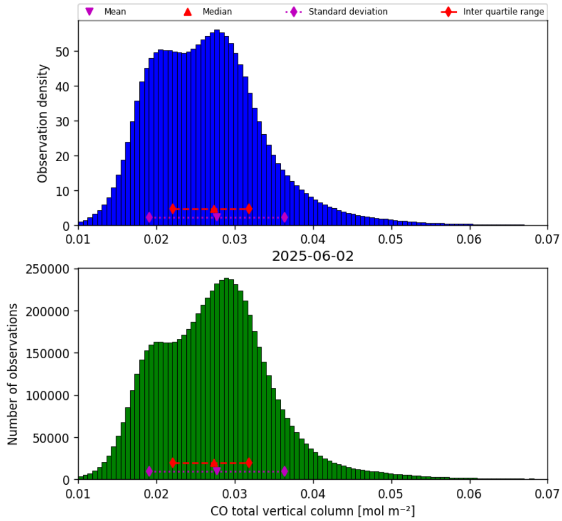
Figure 14: Histogram of “CO total vertical column” for 2025-06-02 to 2025-06-03
