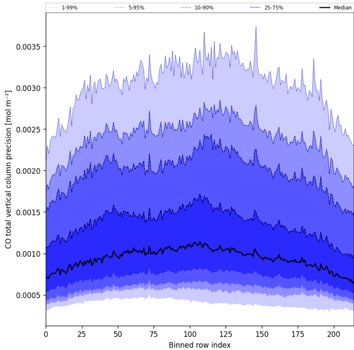
Figure 22: Along track statistics of “CO total vertical column precision” for 2025-06-02 to 2025-06-03
