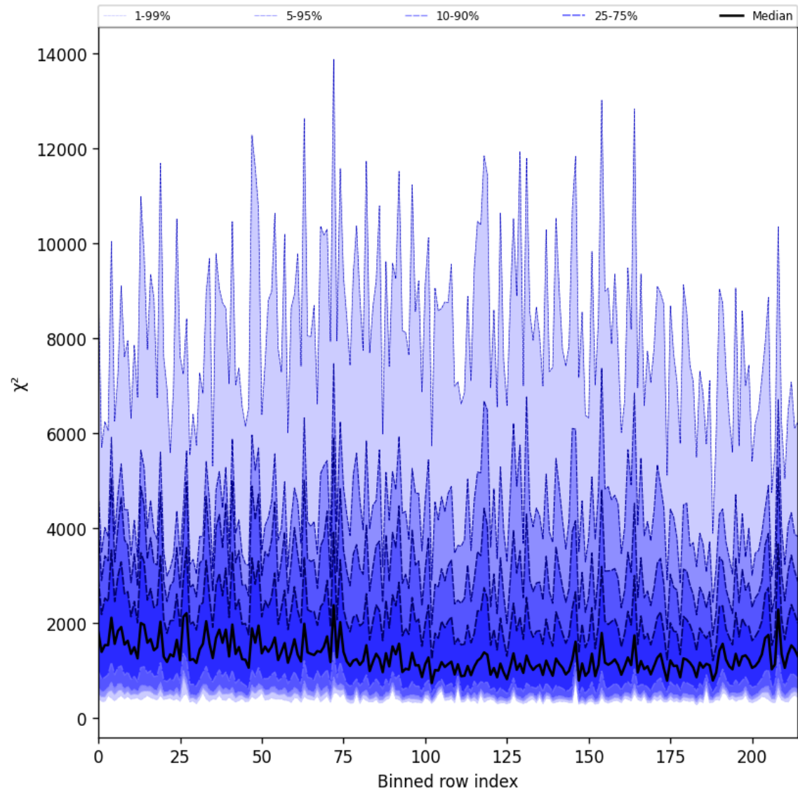
Figure 24: Along track statistics of “ \chi^2 ” for 2025-06-02 to 2025-06-03
