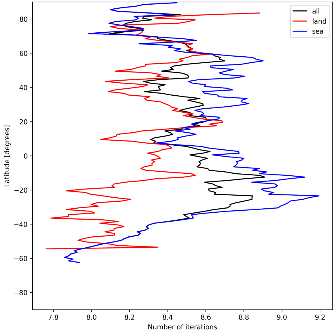
Figure 12: Zonal average of “Number of iterations” for 2025-06-02 to 2025-06-03.
