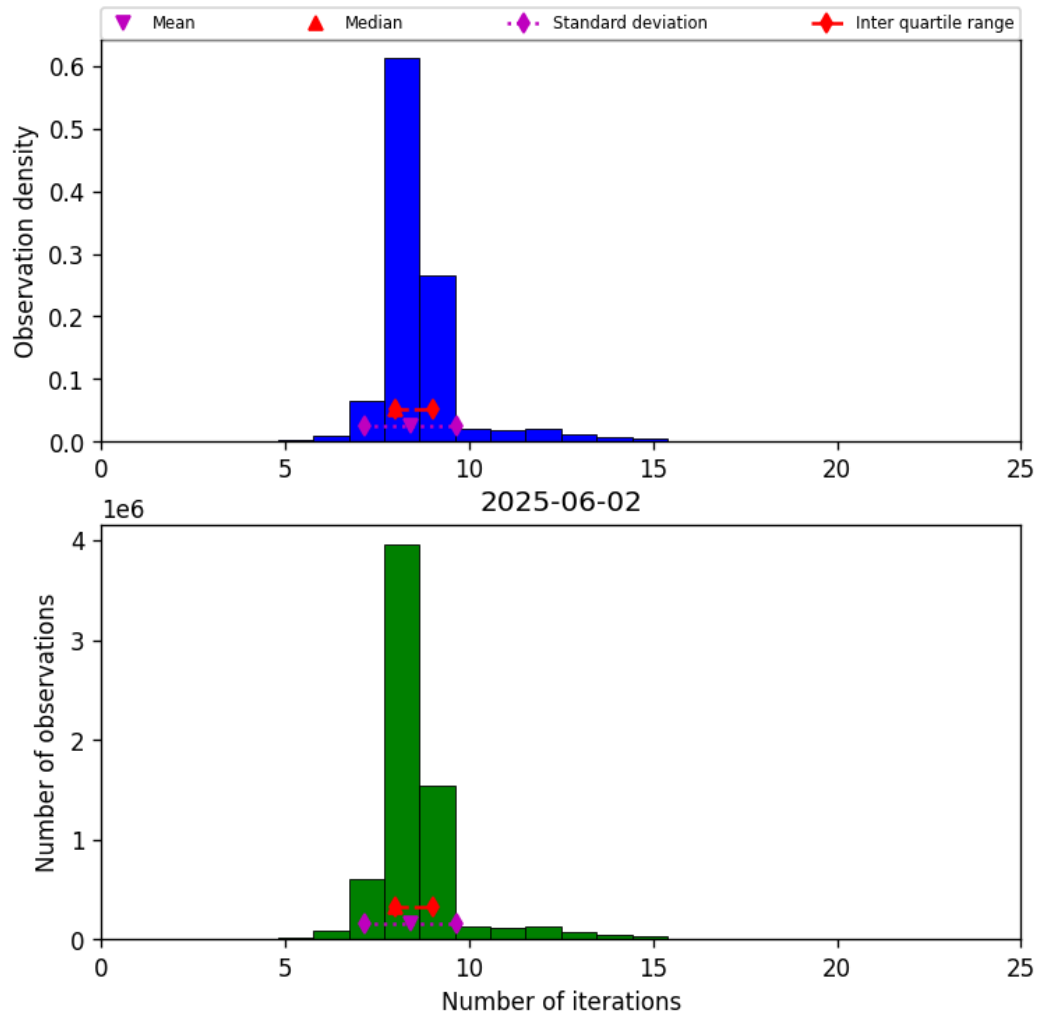
Figure 19: Histogram of “Number of iterations” for 2025-06-02 to 2025-06-03
