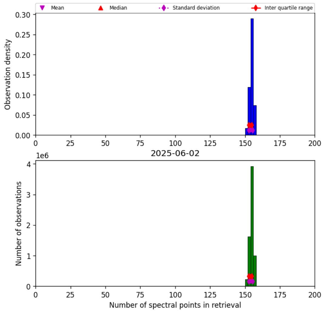
Figure 16: Histogram of “Number of spectral points in retrieval” for 2025-06-02 to 2025-06-03
