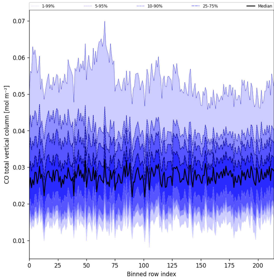
Figure 21: Along track statistics of “CO total vertical column” for 2025-06-02 to 2025-06-03
