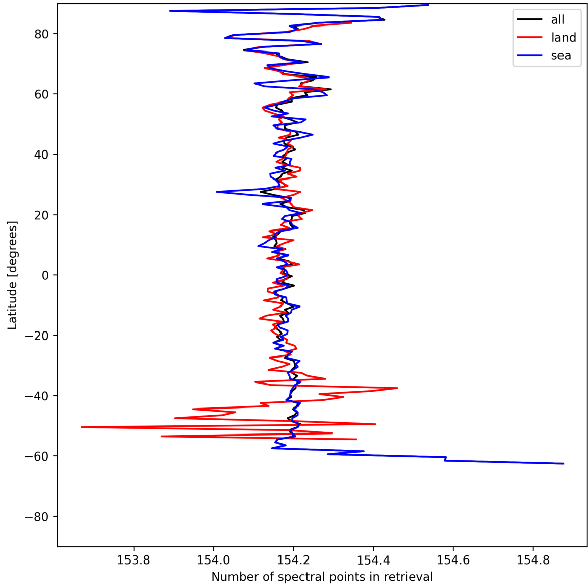
Figure 9: Zonal average of “Number of spectral points in retrieval” for 2025-06-02 to 2025-06-03.
