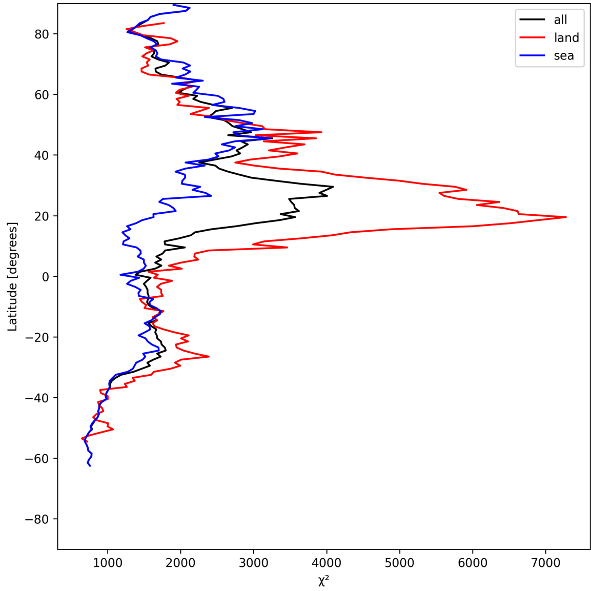
Figure 10: Zonal average of “ \chi^2 ” for 2025-06-02 to 2025-06-03.
