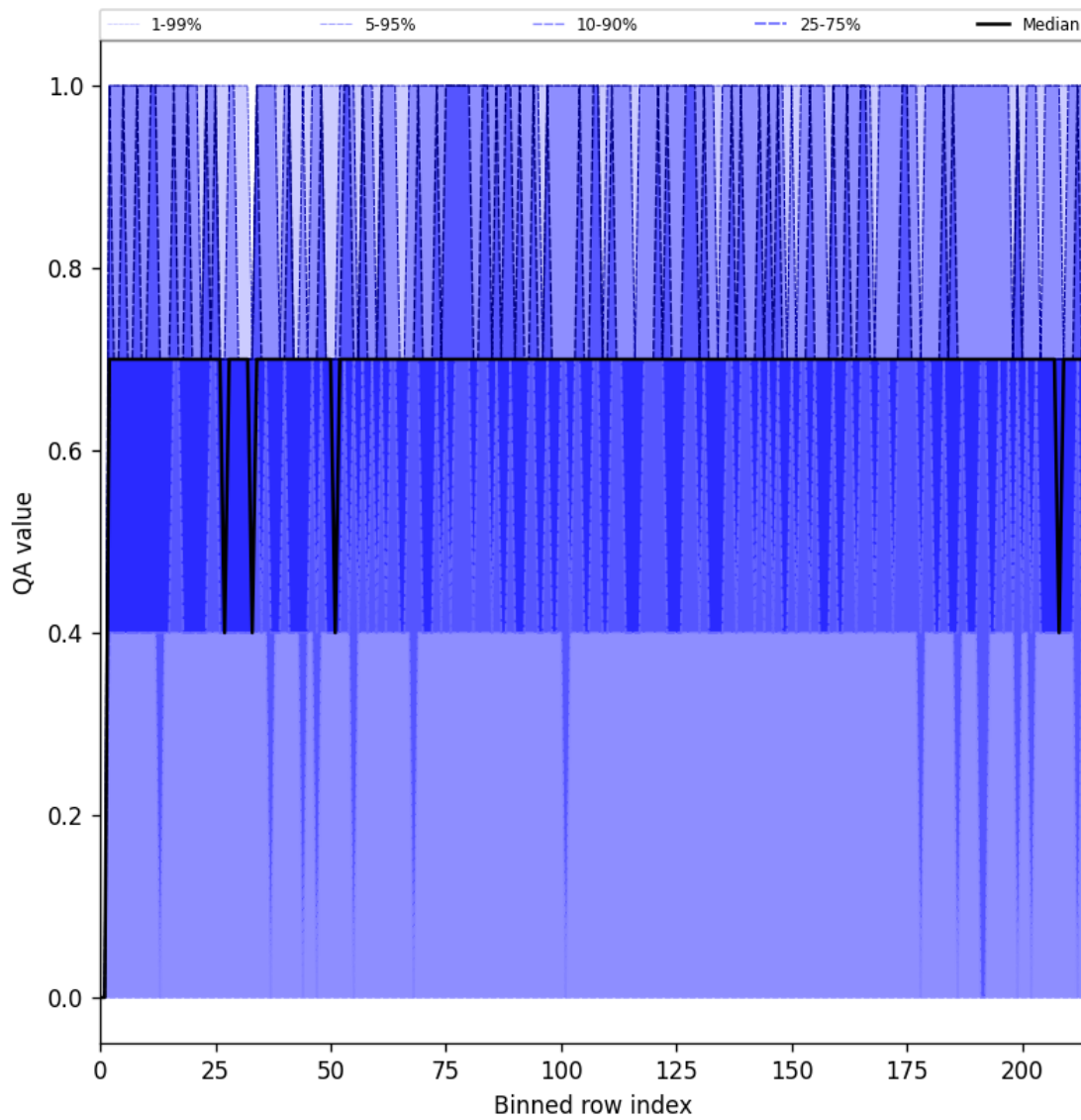
Figure 20: Along track statistics of “QA value” for 2025-06-02 to 2025-06-03
