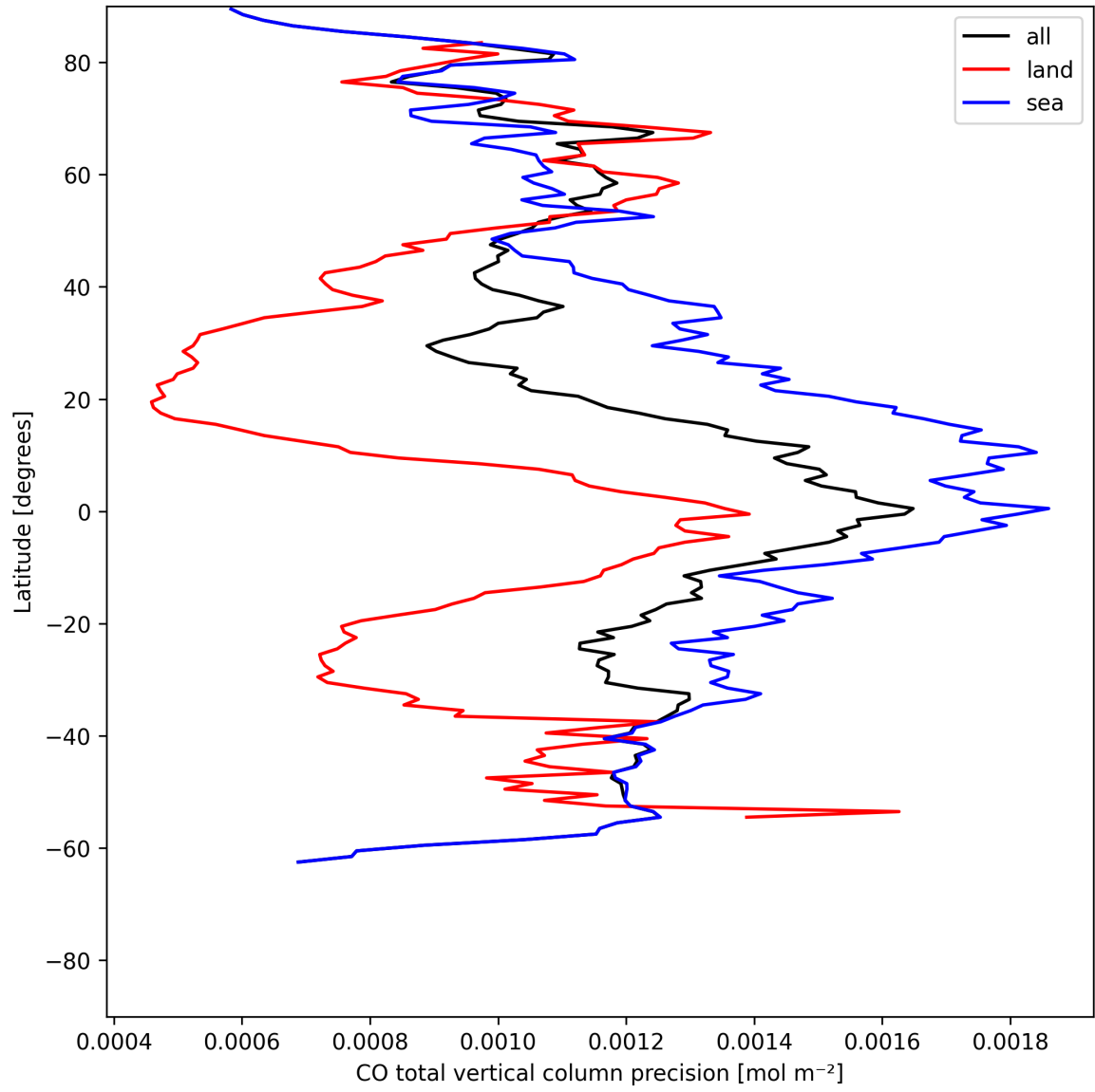
Figure 8: Zonal average of "CO total vertical column precision" for 2025-06-02 to 2025-06-03.
