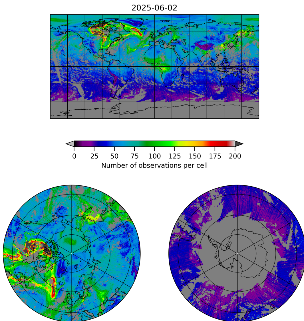
Figure 5: Map of the number of observations for 2025-06-02 to 2025-06-03
