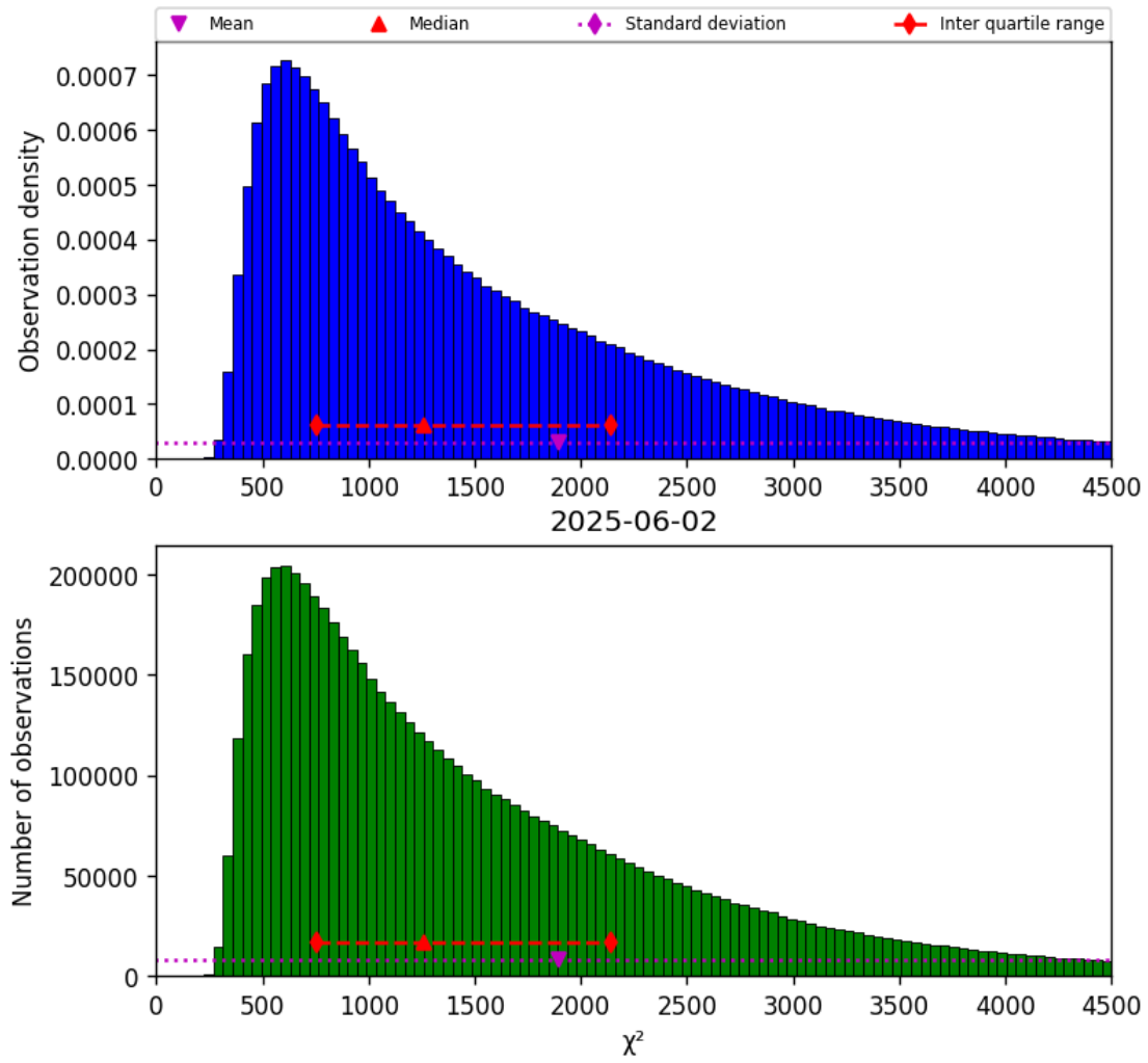
Figure 17: Histogram of " \chi^2 " for 2025-06-02 to 2025-06-03
