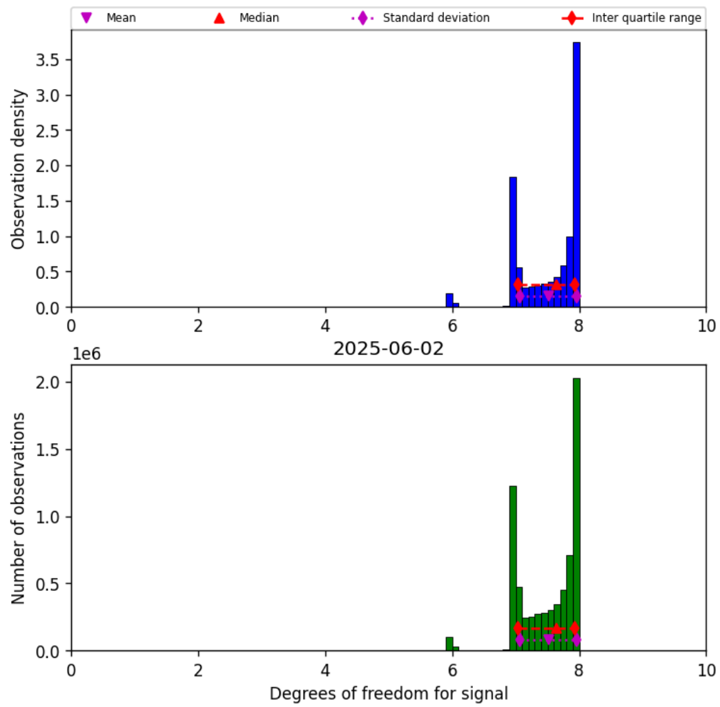
Figure 18: Histogram of “Degrees of freedom for signal” for 2025-06-02 to 2025-06-03
