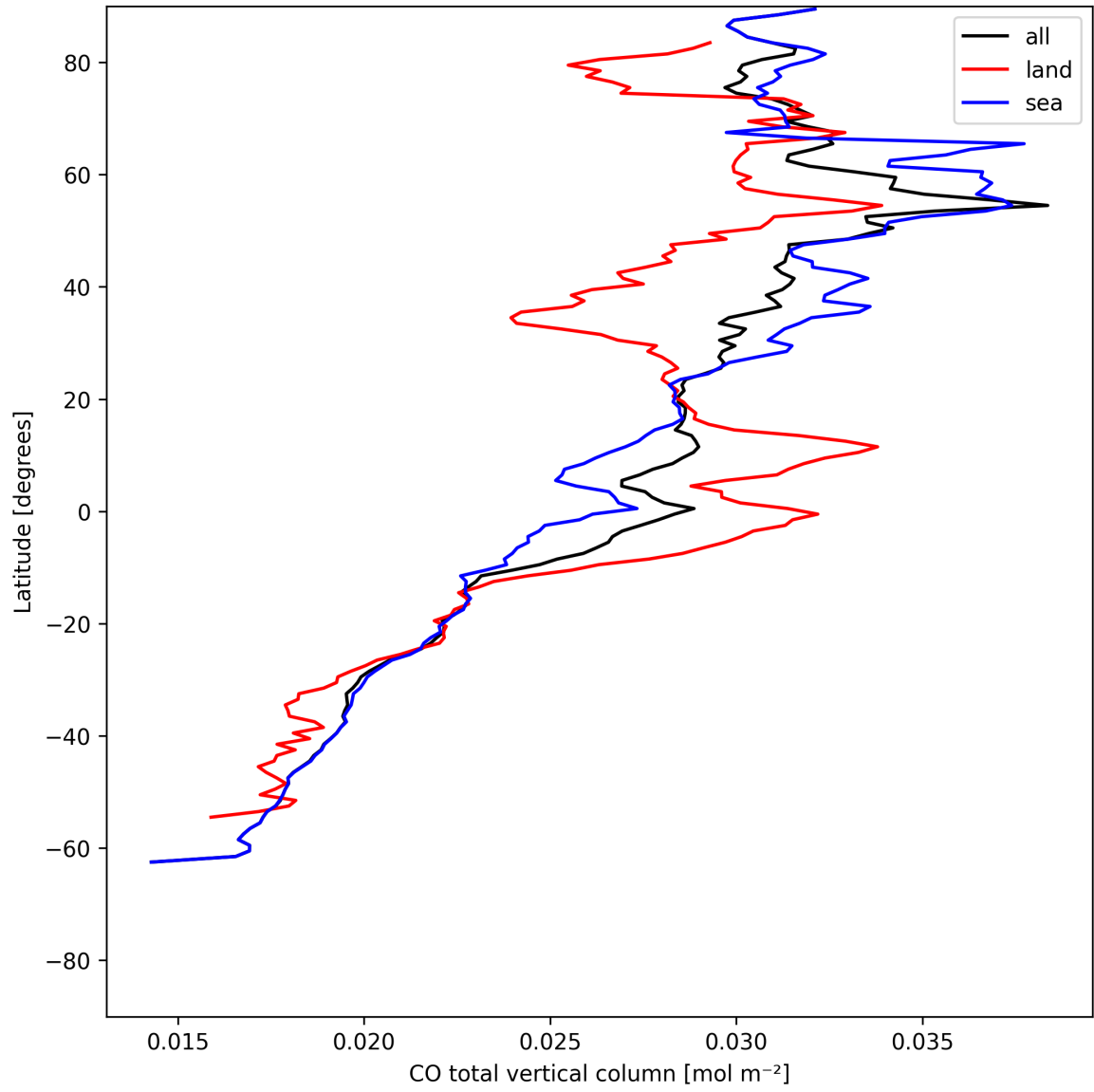
Figure 7: Zonal average of “CO total vertical column” for 2025-06-02 to 2025-06-03.
