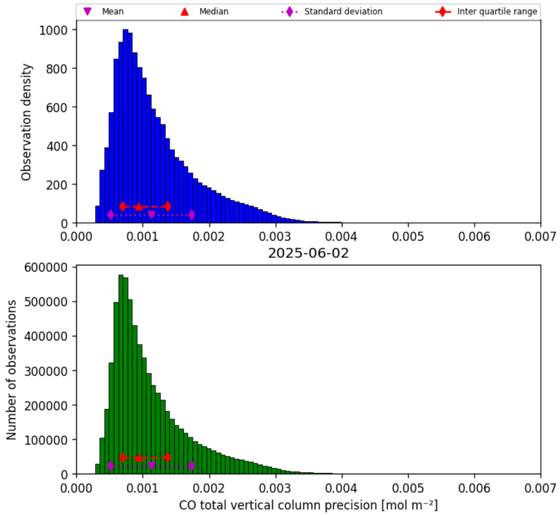
Figure 15: Histogram of “CO total vertical column precision” for 2025-06-02 to 2025-06-03
