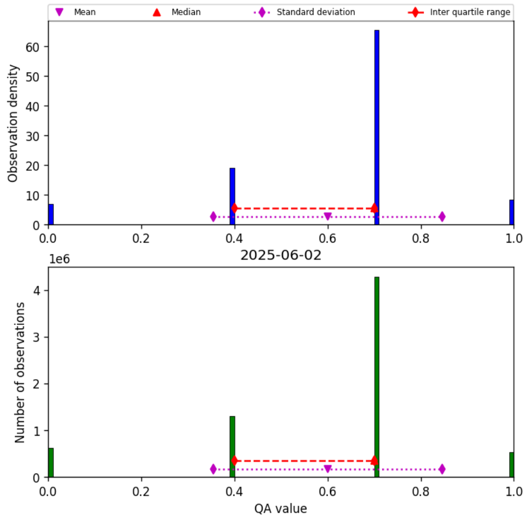
Figure 13: Histogram of “QA value” for 2025-06-02 to 2025-06-03
