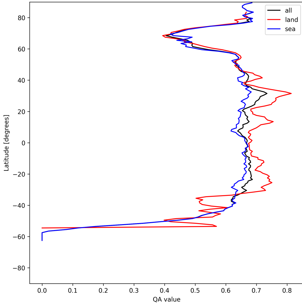
Figure 6: Zonal average of “QA value” for 2025-06-02 to 2025-06-03.
