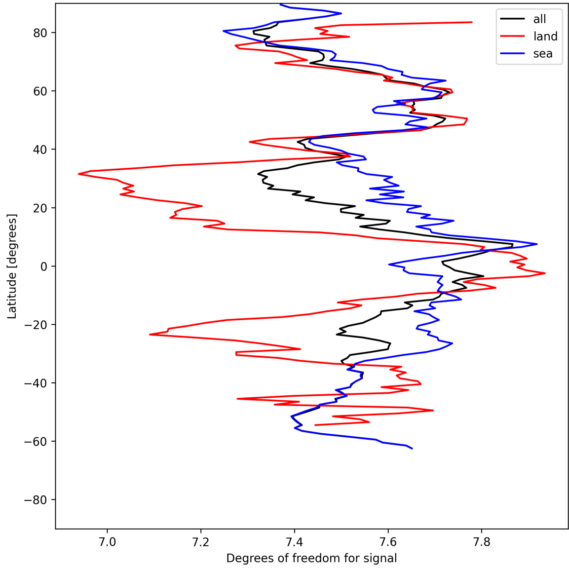
Figure 11: Zonal average of “Degrees of freedom for signal” for 2025-06-02 to 2025-06-03.
