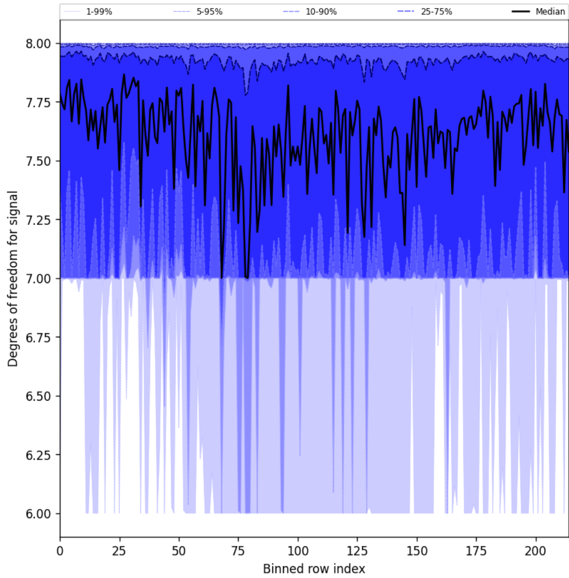
Figure 25: Along track statistics of “Degrees of freedom for signal” for 2025-06-02 to 2025-06-03
