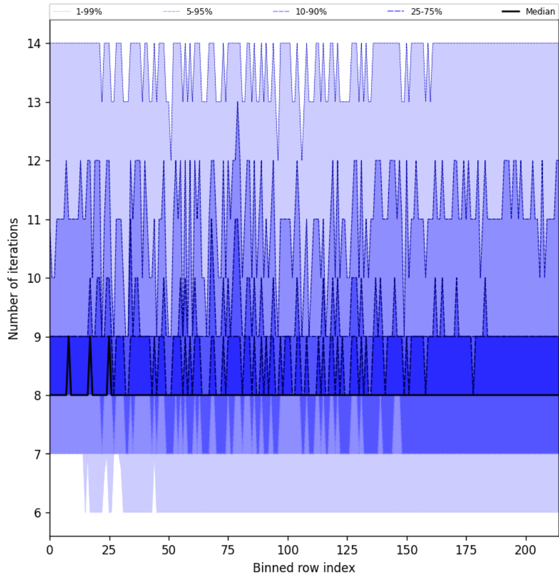
Figure 26: Along track statistics of “Number of iterations” for 2025-06-02 to 2025-06-03
