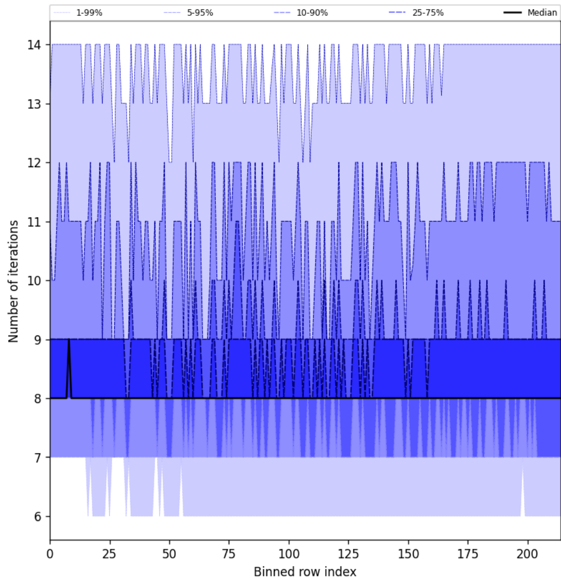
Figure 26: Along track statistics of “Number of iterations” for 2025-06-03 to 2025-06-04
