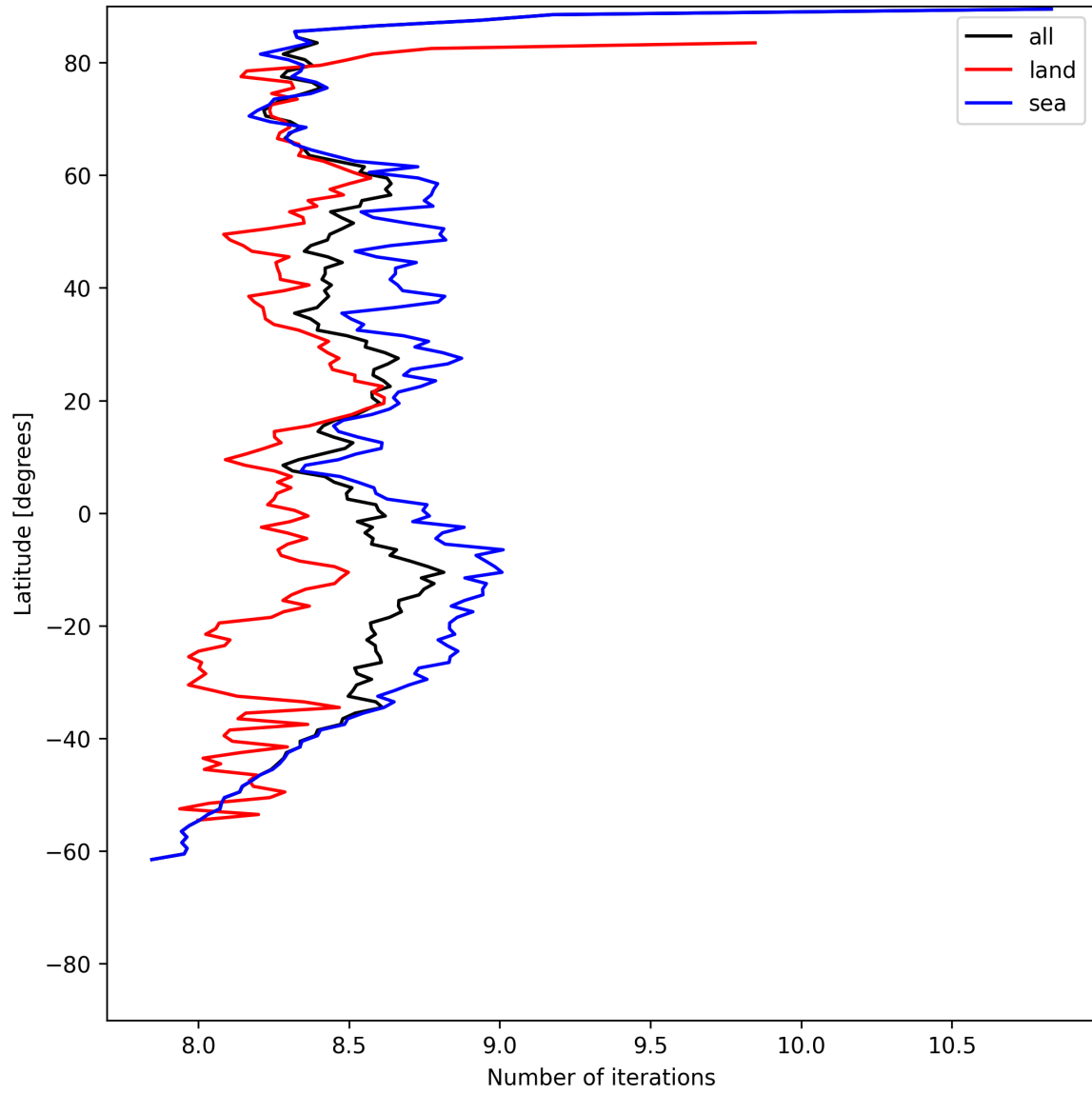
Figure 12: Zonal average of “Number of iterations” for 2025-06-03 to 2025-06-04.
