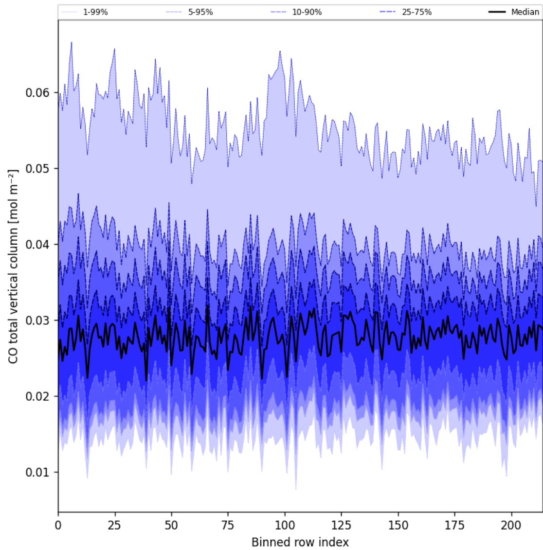
Figure 21: Along track statistics of “CO total vertical column” for 2025-06-03 to 2025-06-04
