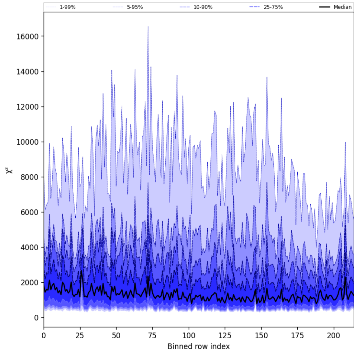
Figure 24: Along track statistics of “ \chi^2 ” for 2025-06-03 to 2025-06-04
