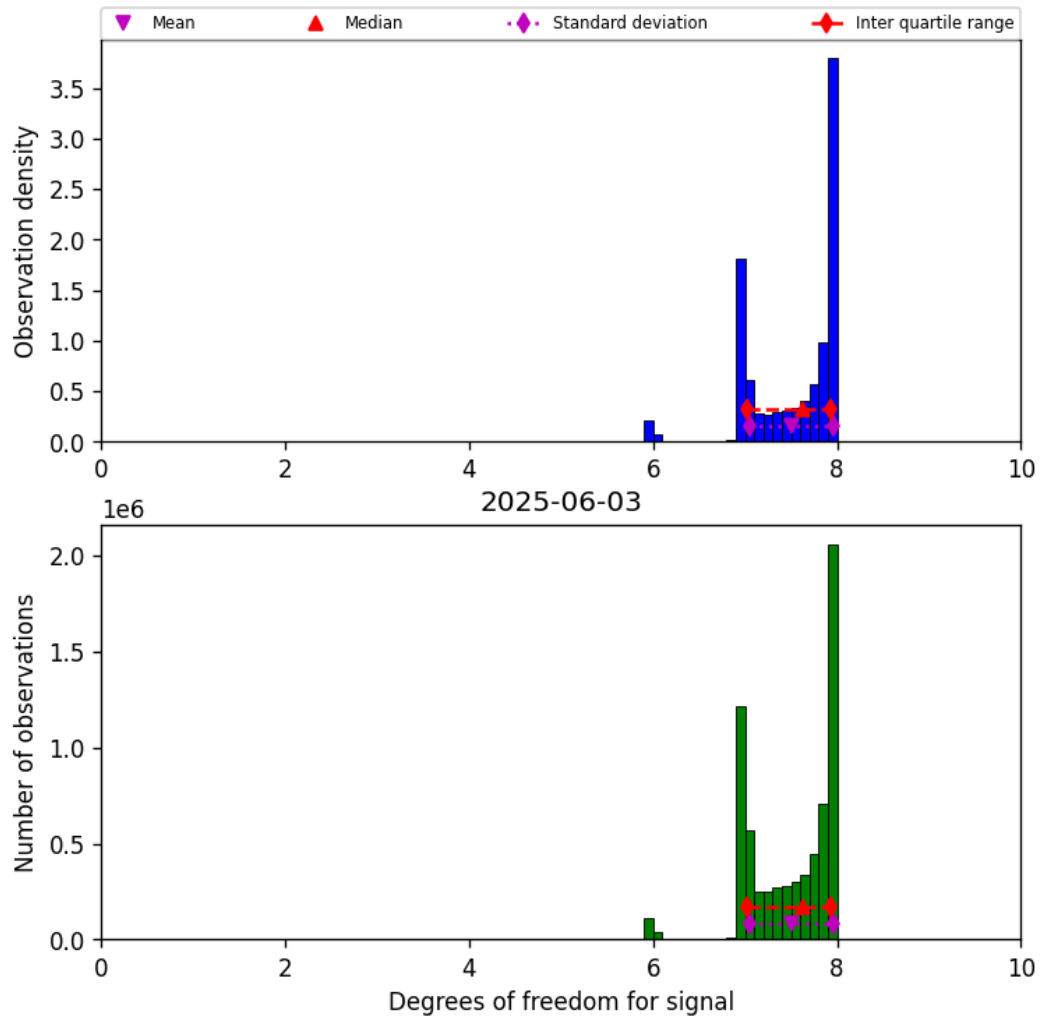
Figure 18: Histogram of “Degrees of freedom for signal” for 2025-06-03 to 2025-06-04
