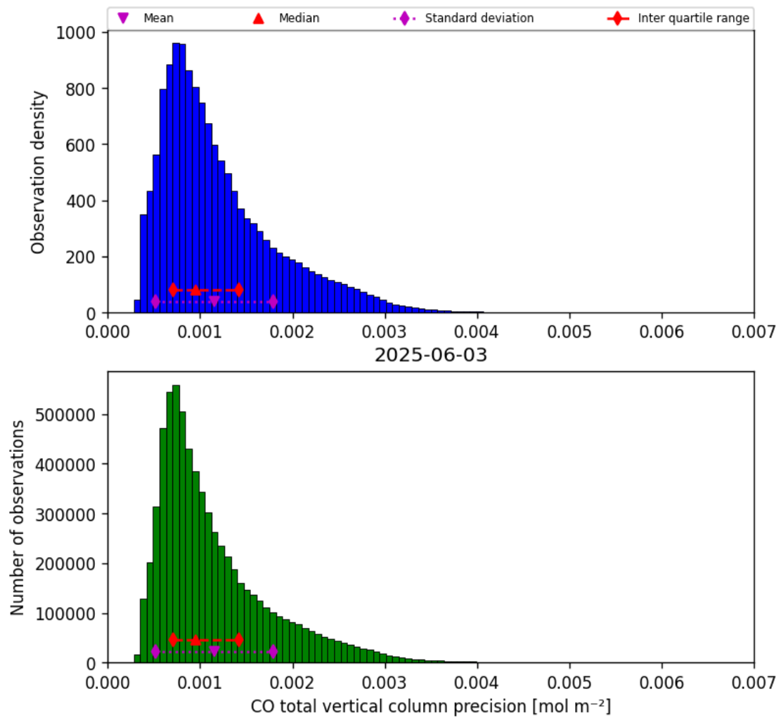
Figure 15: Histogram of “CO total vertical column precision” for 2025-06-03 to 2025-06-04
