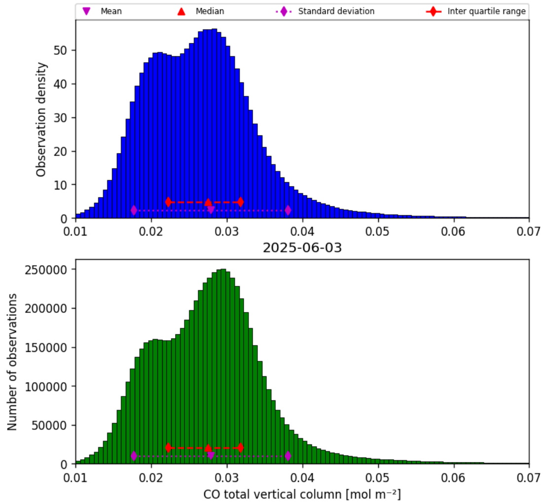
Figure 14: Histogram of “CO total vertical column” for 2025-06-03 to 2025-06-04
