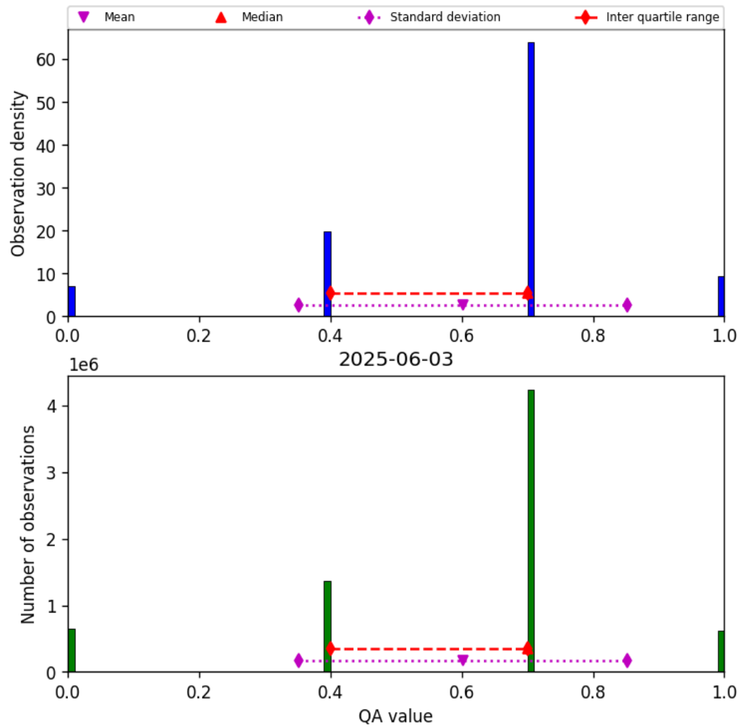
Figure 13: Histogram of “QA value” for 2025-06-03 to 2025-06-04
