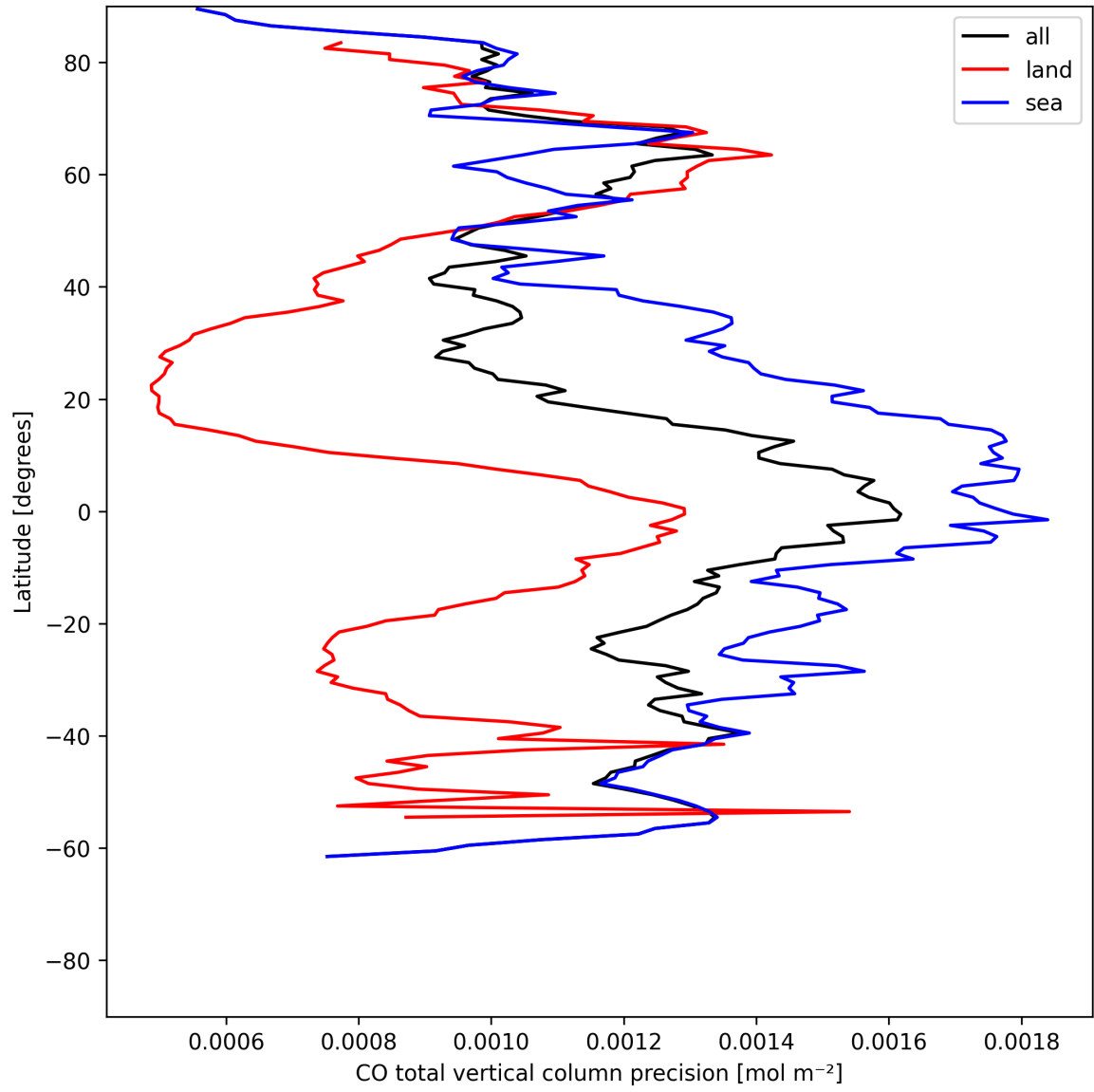
Figure 8: Zonal average of “CO total vertical column precision” for 2025-06-03 to 2025-06-04.
