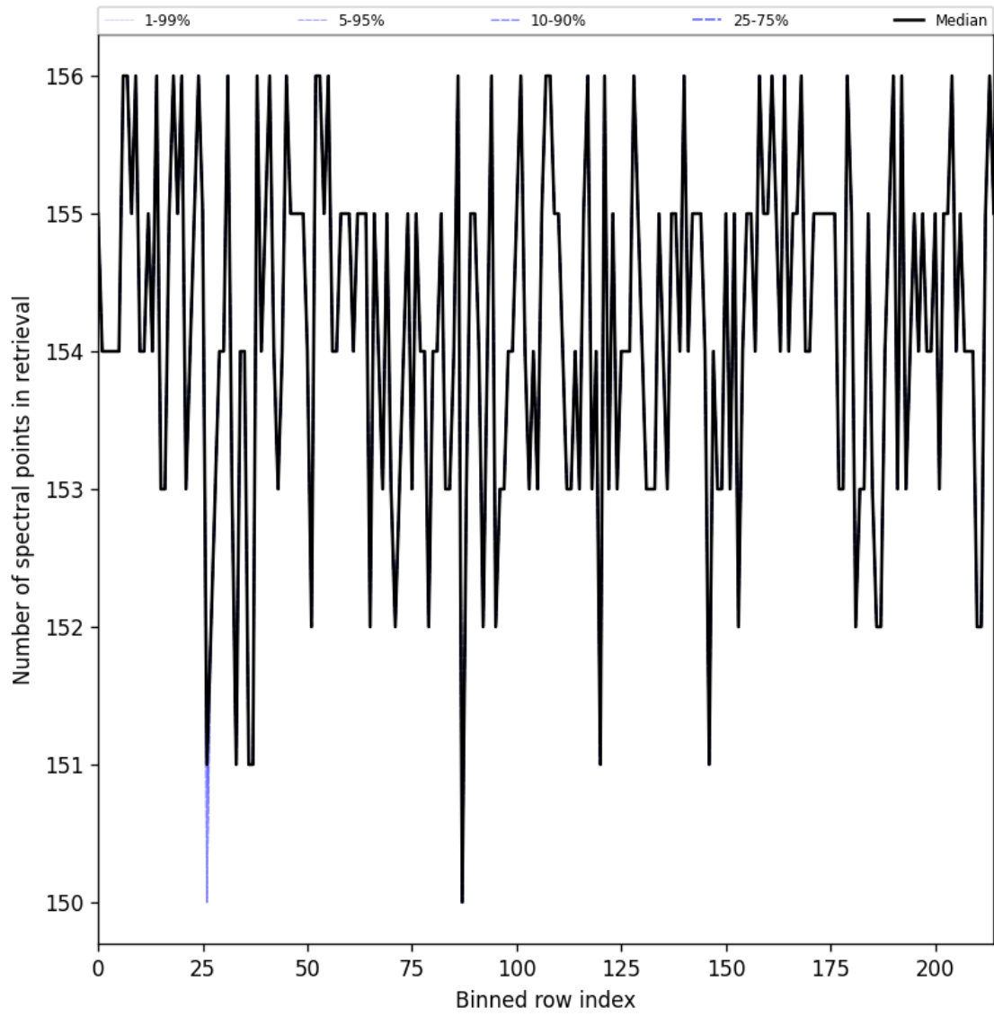
Figure 23: Along track statistics of “Number of spectral points in retrieval” for 2025-06-03 to 2025-06-04
