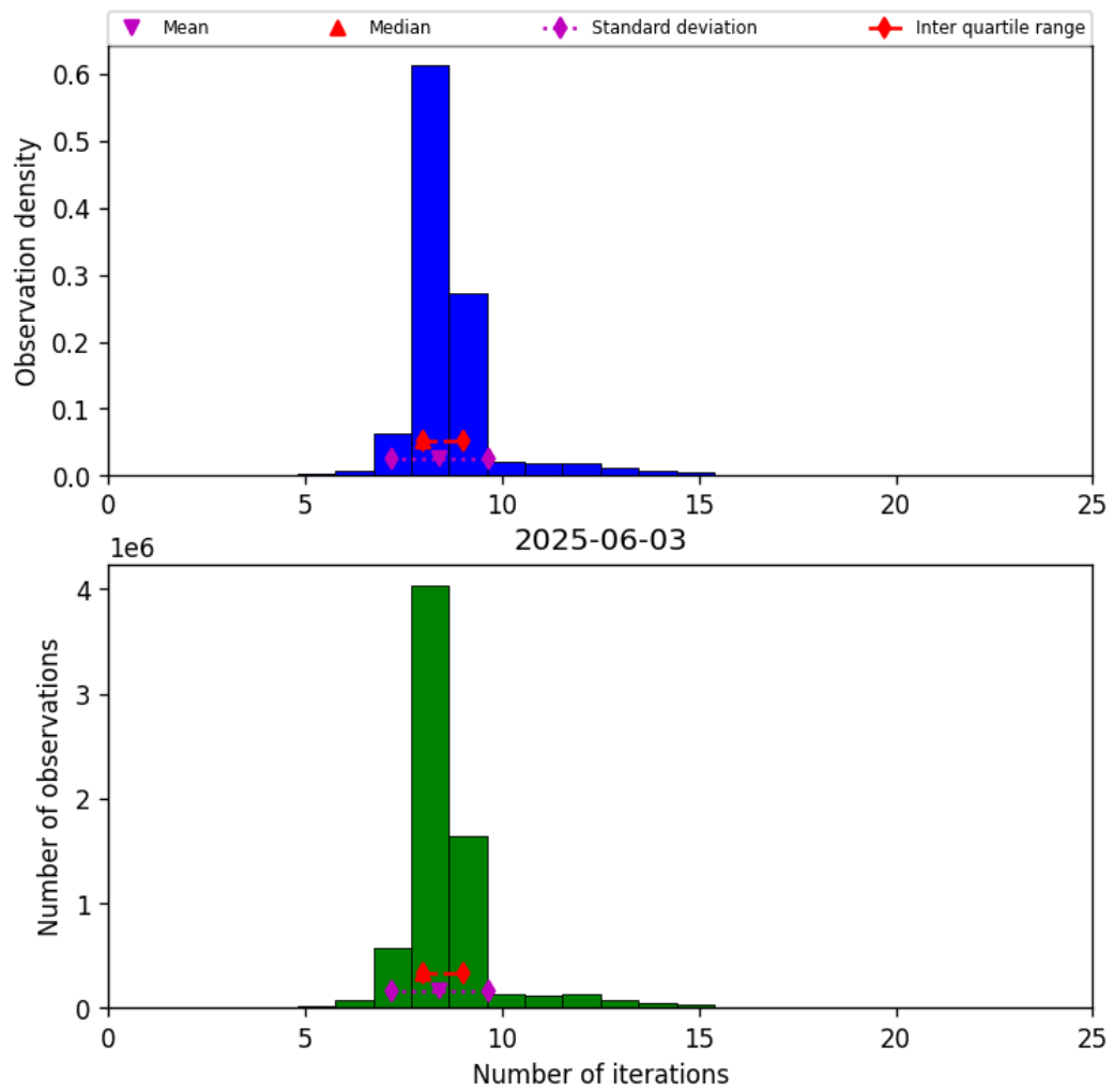
Figure 19: Histogram of “Number of iterations” for 2025-06-03 to 2025-06-04
