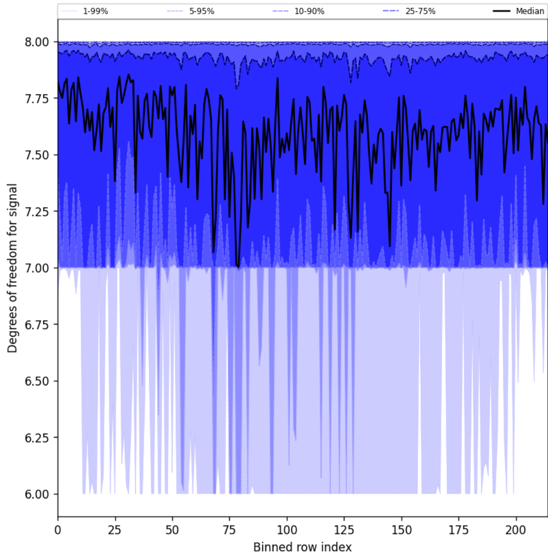
Figure 25: Along track statistics of “Degrees of freedom for signal” for 2025-06-03 to 2025-06-04
