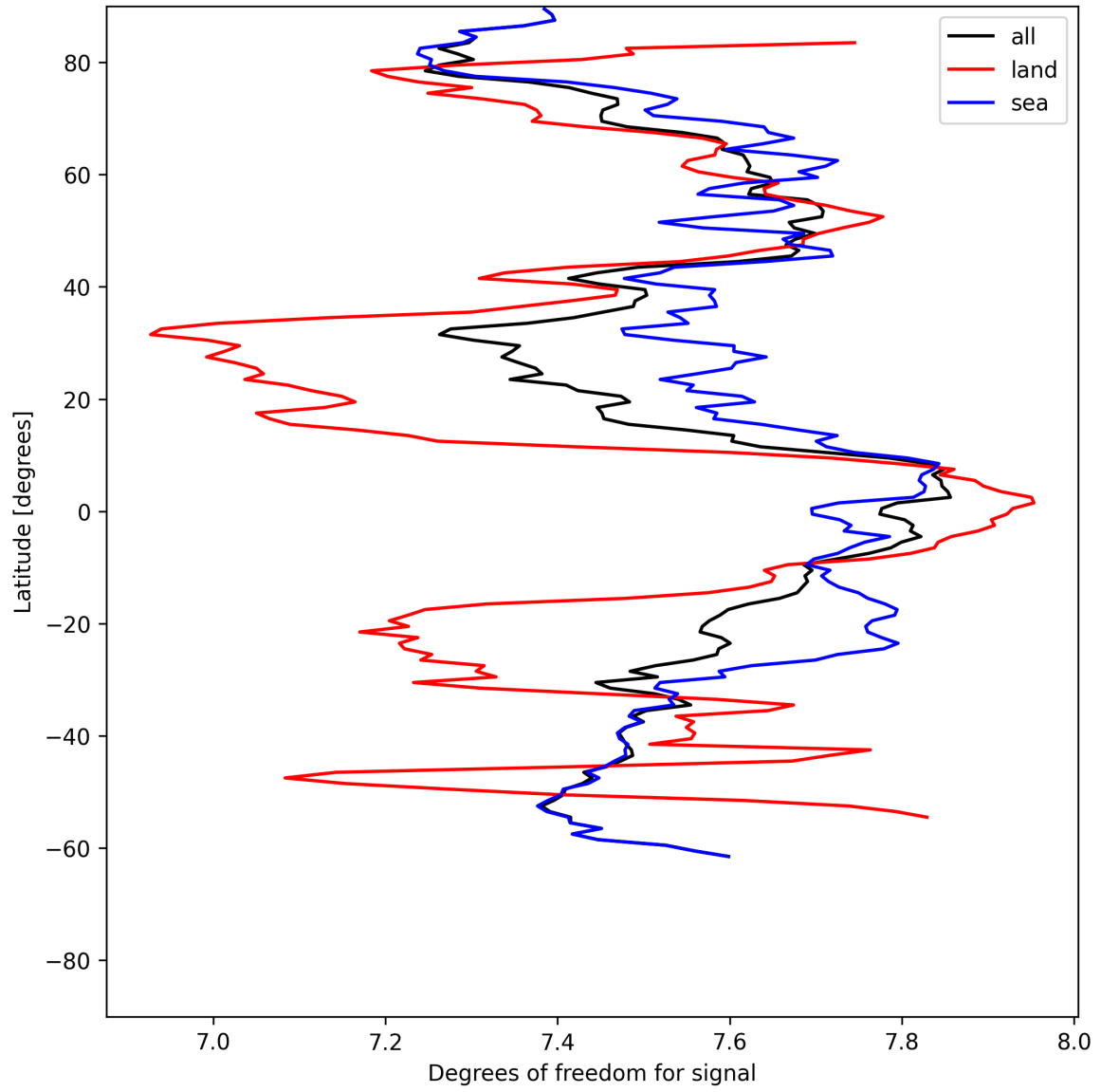
Figure 11: Zonal average of “Degrees of freedom for signal” for 2025-06-03 to 2025-06-04.
