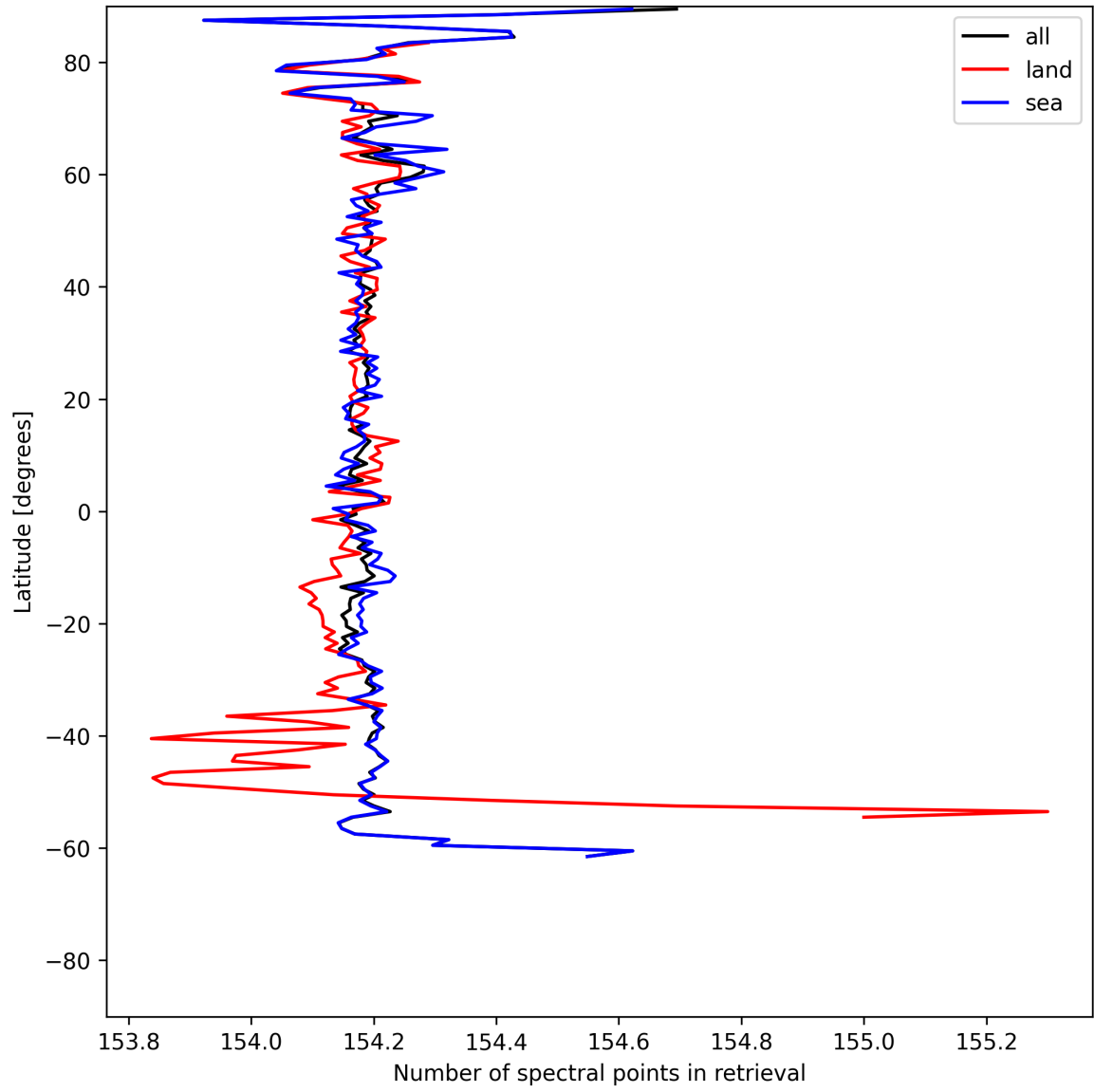
Figure 9: Zonal average of “Number of spectral points in retrieval” for 2025-06-03 to 2025-06-04.
