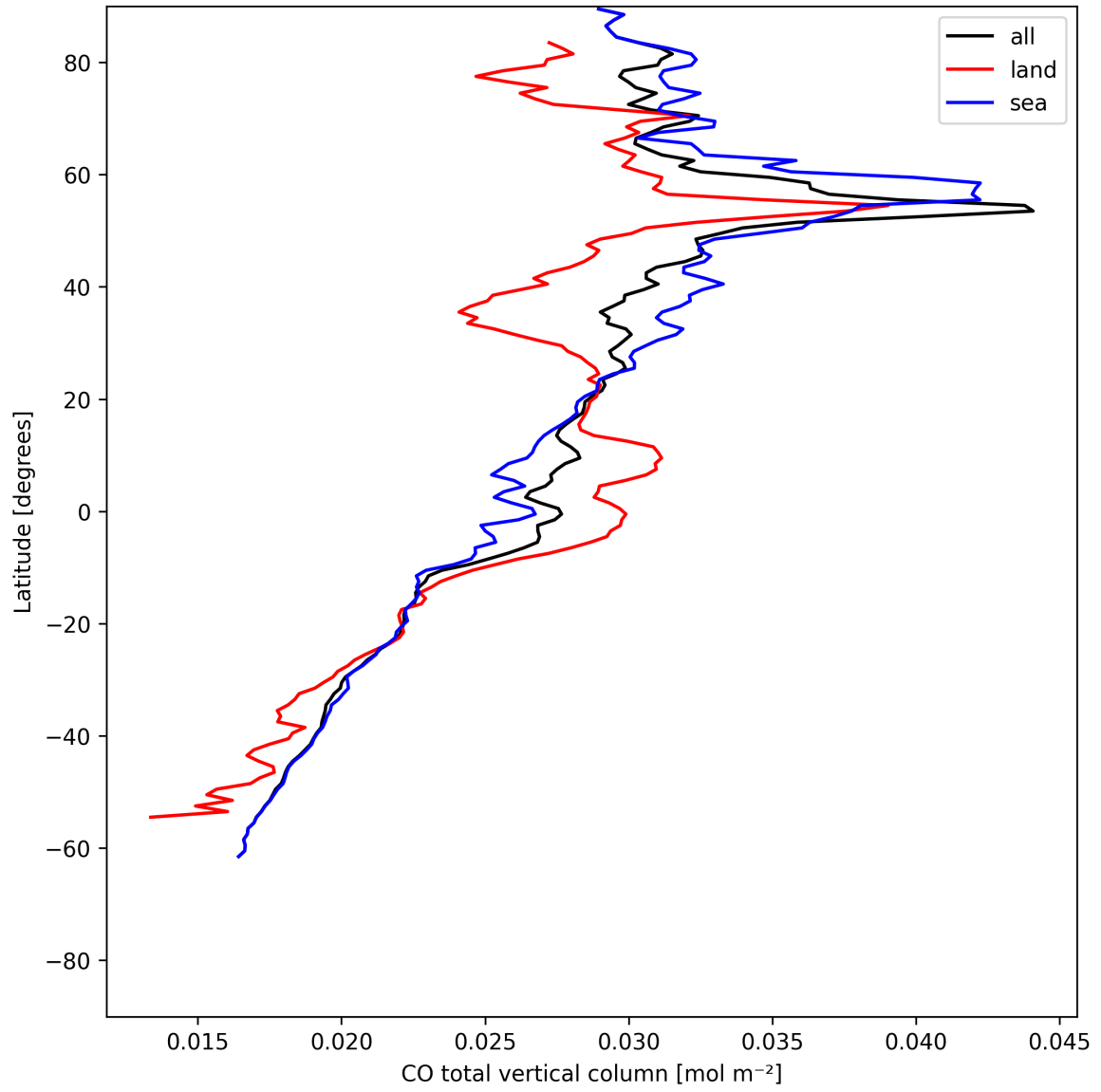
Figure 7: Zonal average of “CO total vertical column” for 2025-06-03 to 2025-06-04.
