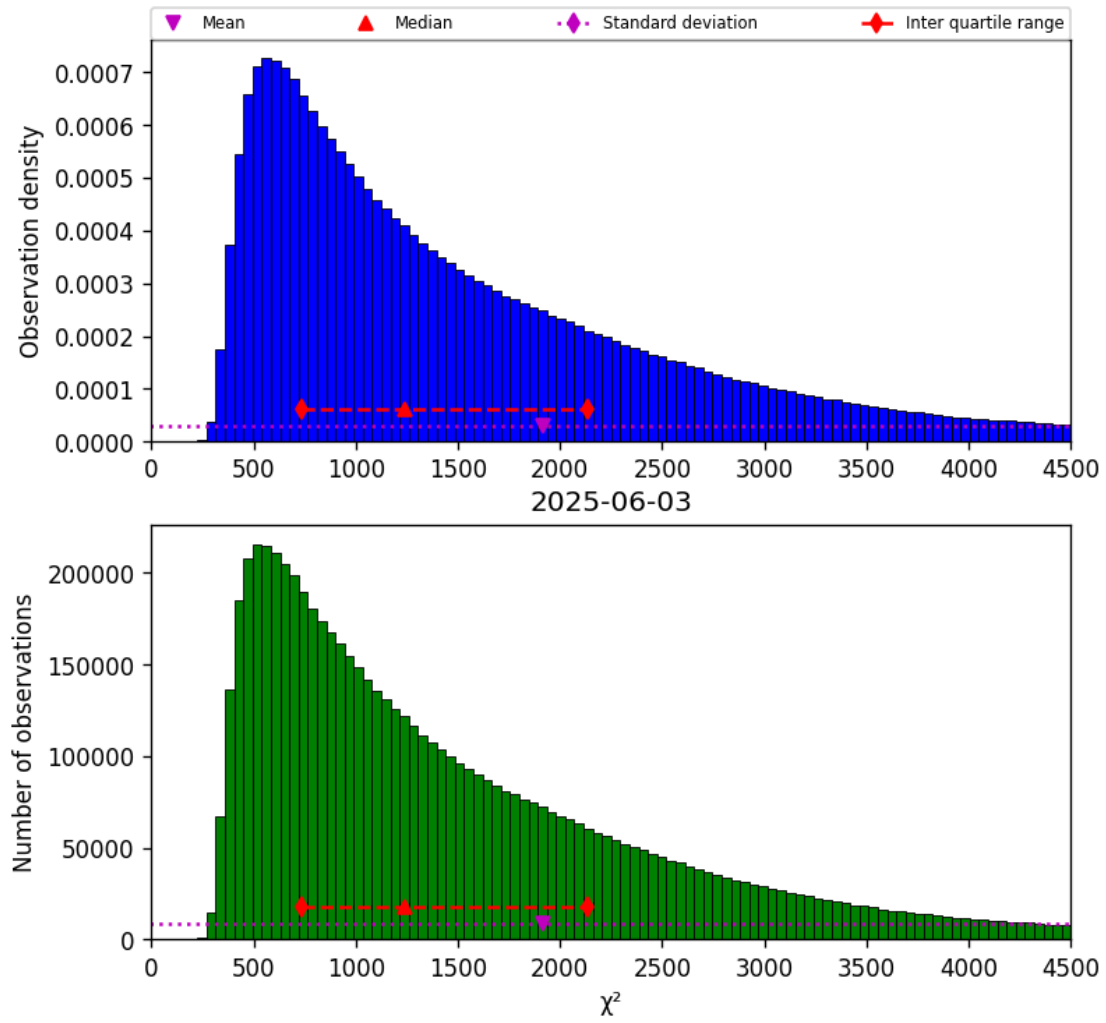
Figure 17: Histogram of " \chi^2 " for 2025-06-03 to 2025-06-04
