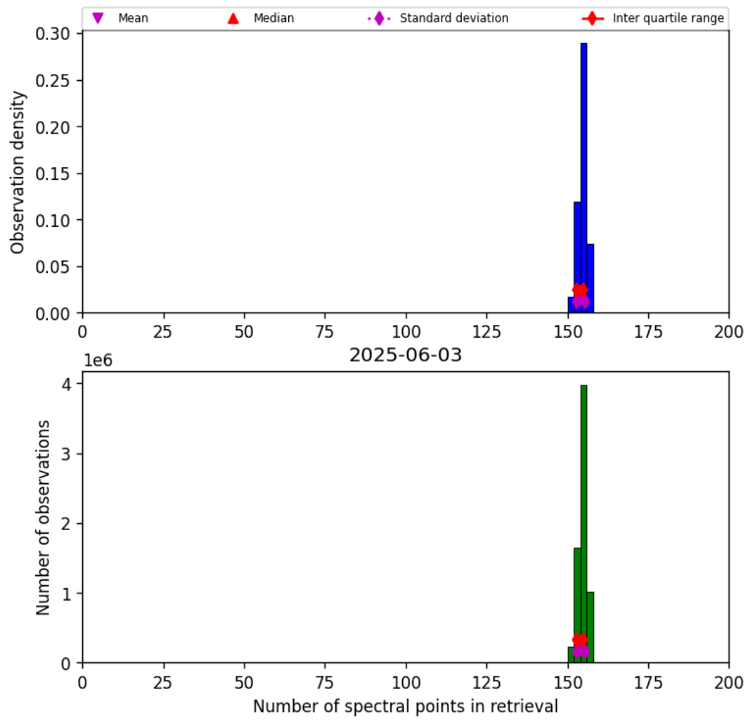
Figure 16: Histogram of “Number of spectral points in retrieval” for 2025-06-03 to 2025-06-04
