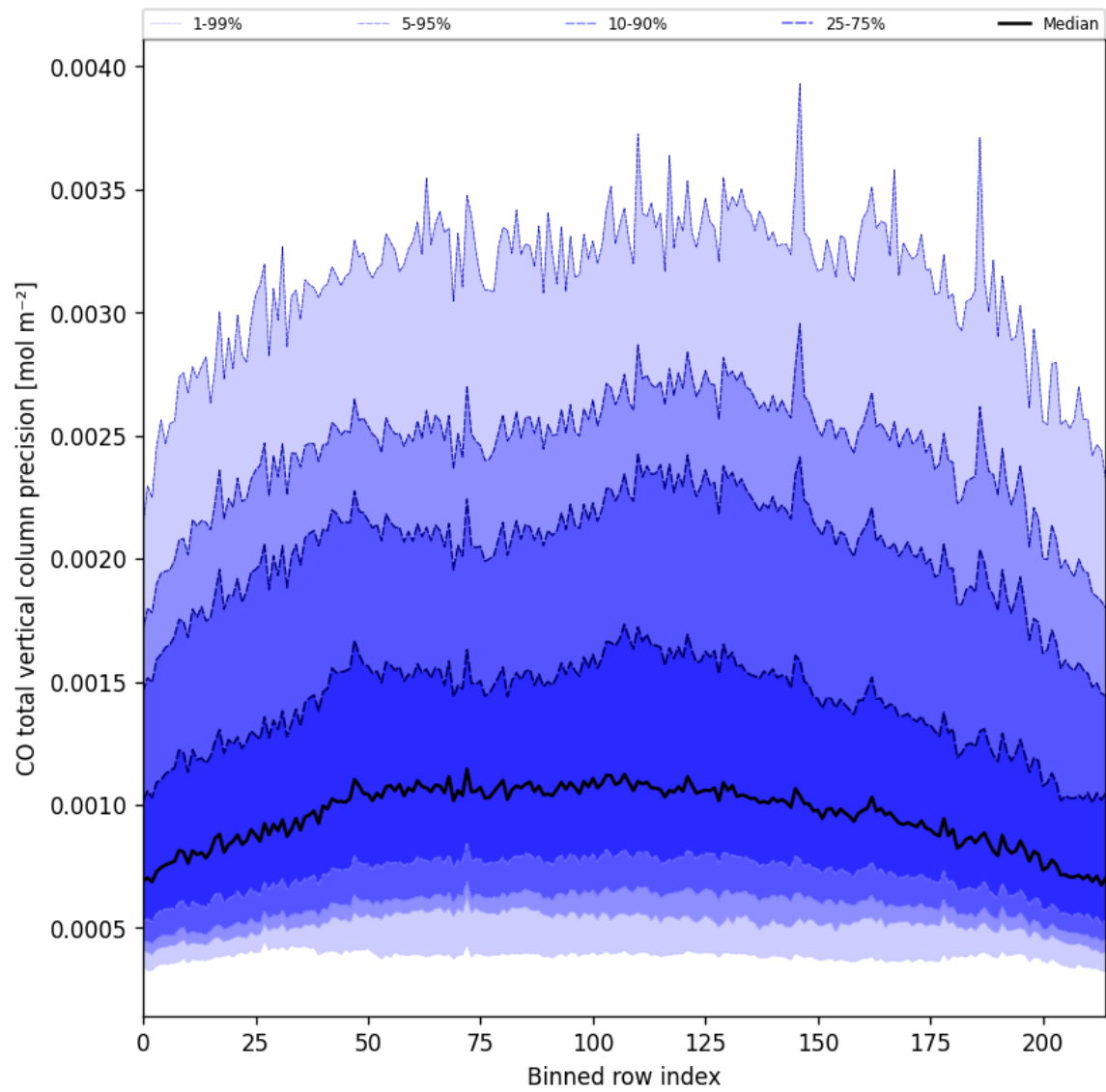
Figure 22: Along track statistics of “CO total vertical column precision” for 2025-06-03 to 2025-06-04
