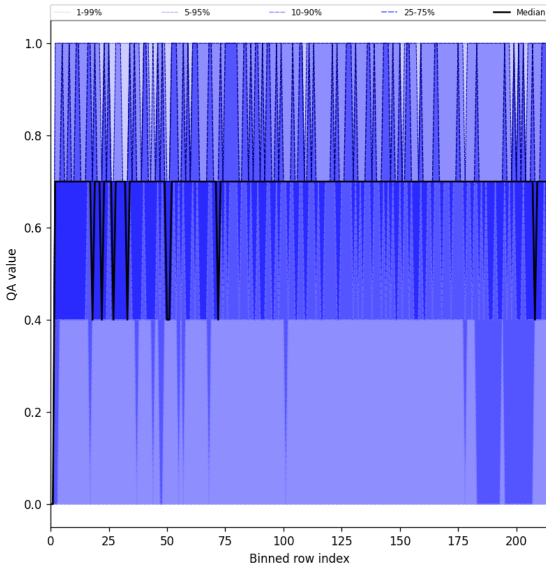
Figure 20: Along track statistics of “QA value” for 2025-06-03 to 2025-06-04
