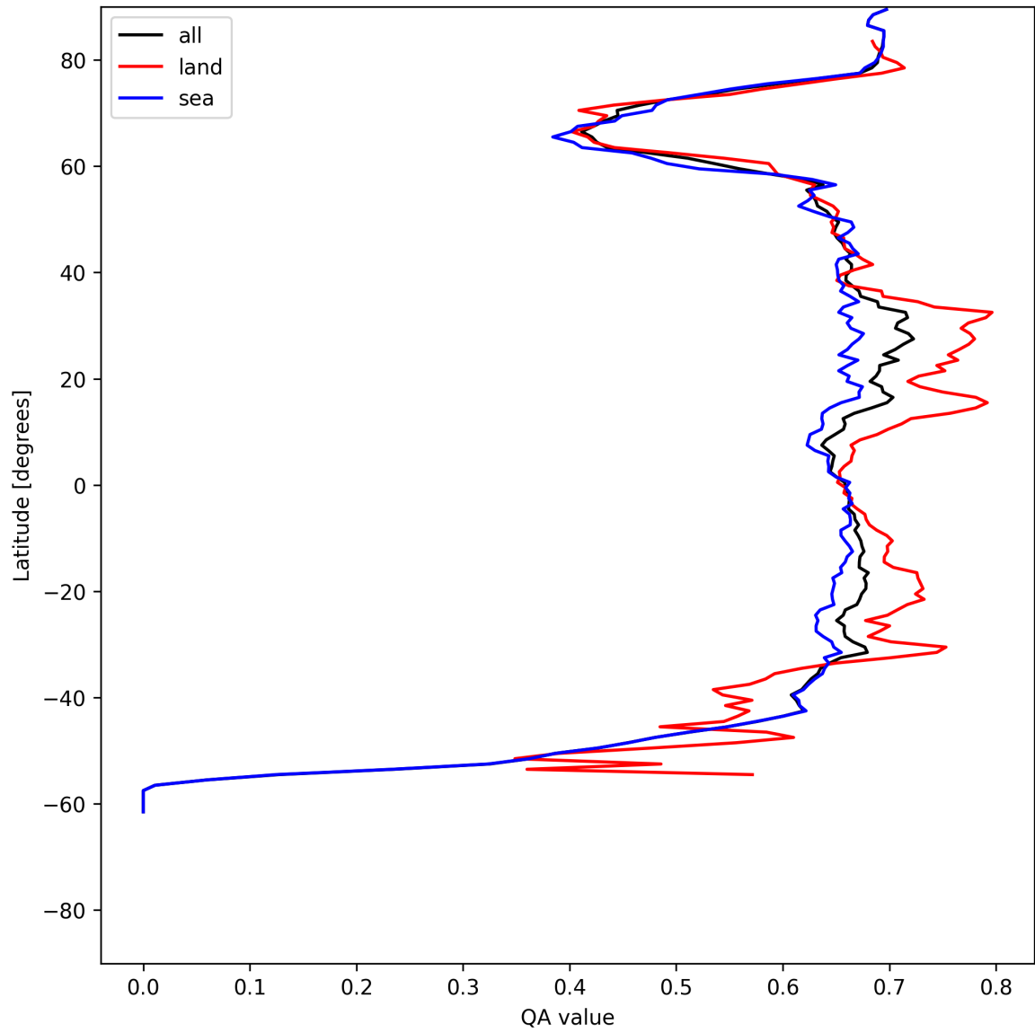
Figure 6: Zonal average of “QA value” for 2025-06-03 to 2025-06-04.
