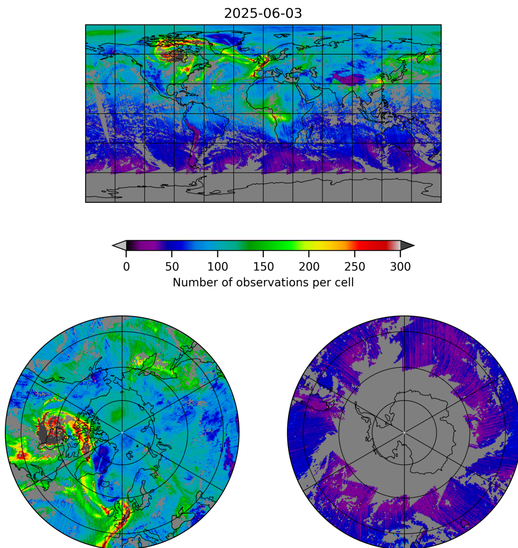
Figure 5: Map of the number of observations for 2025-06-03 to 2025-06-04
