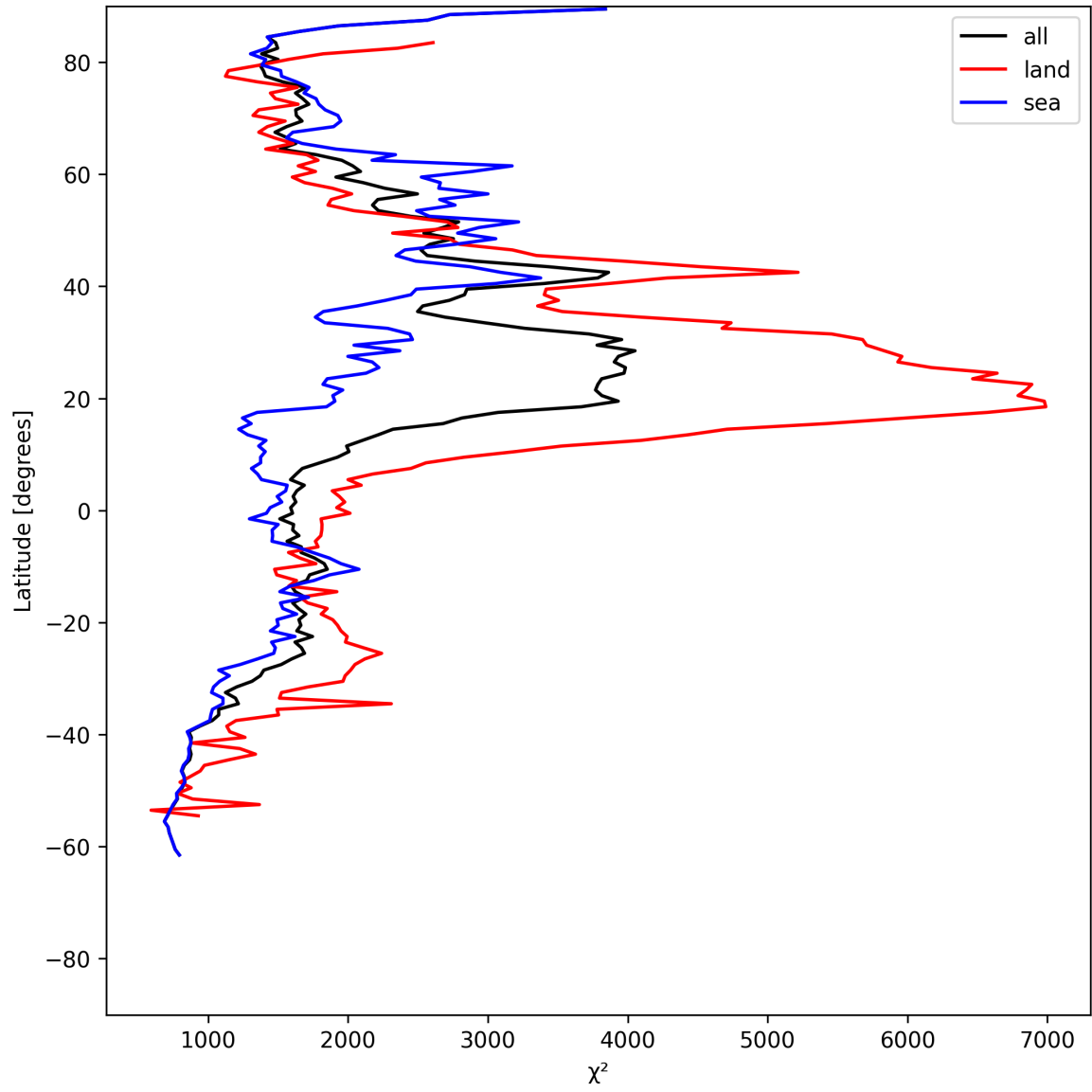
Figure 10: Zonal average of “ \chi^2 ” for 2025-06-03 to 2025-06-04.
