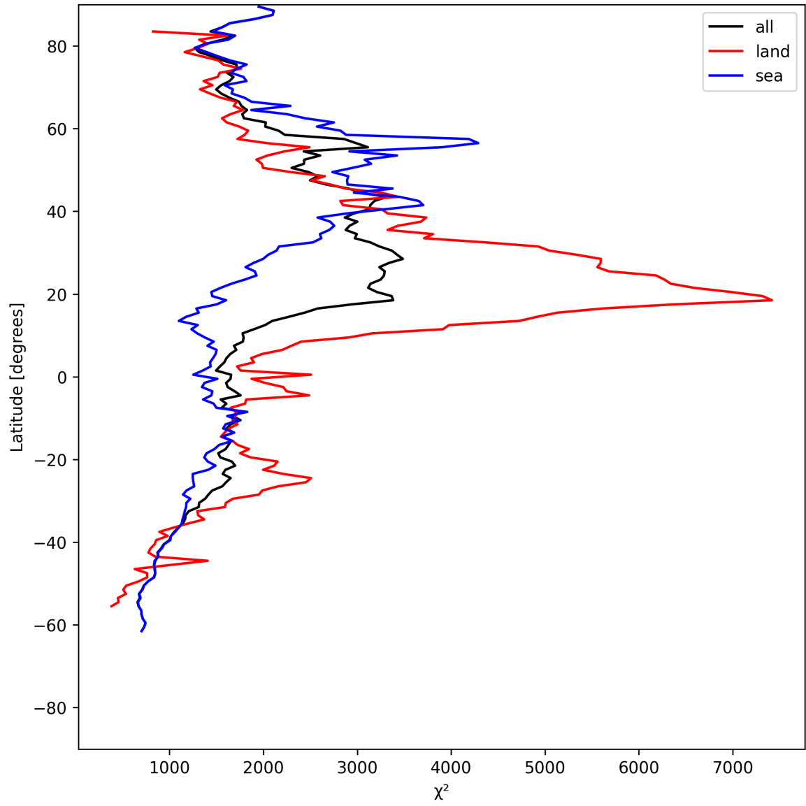
Figure 10: Zonal average of “ \chi^2 ” for 2025-06-05 to 2025-06-06.
