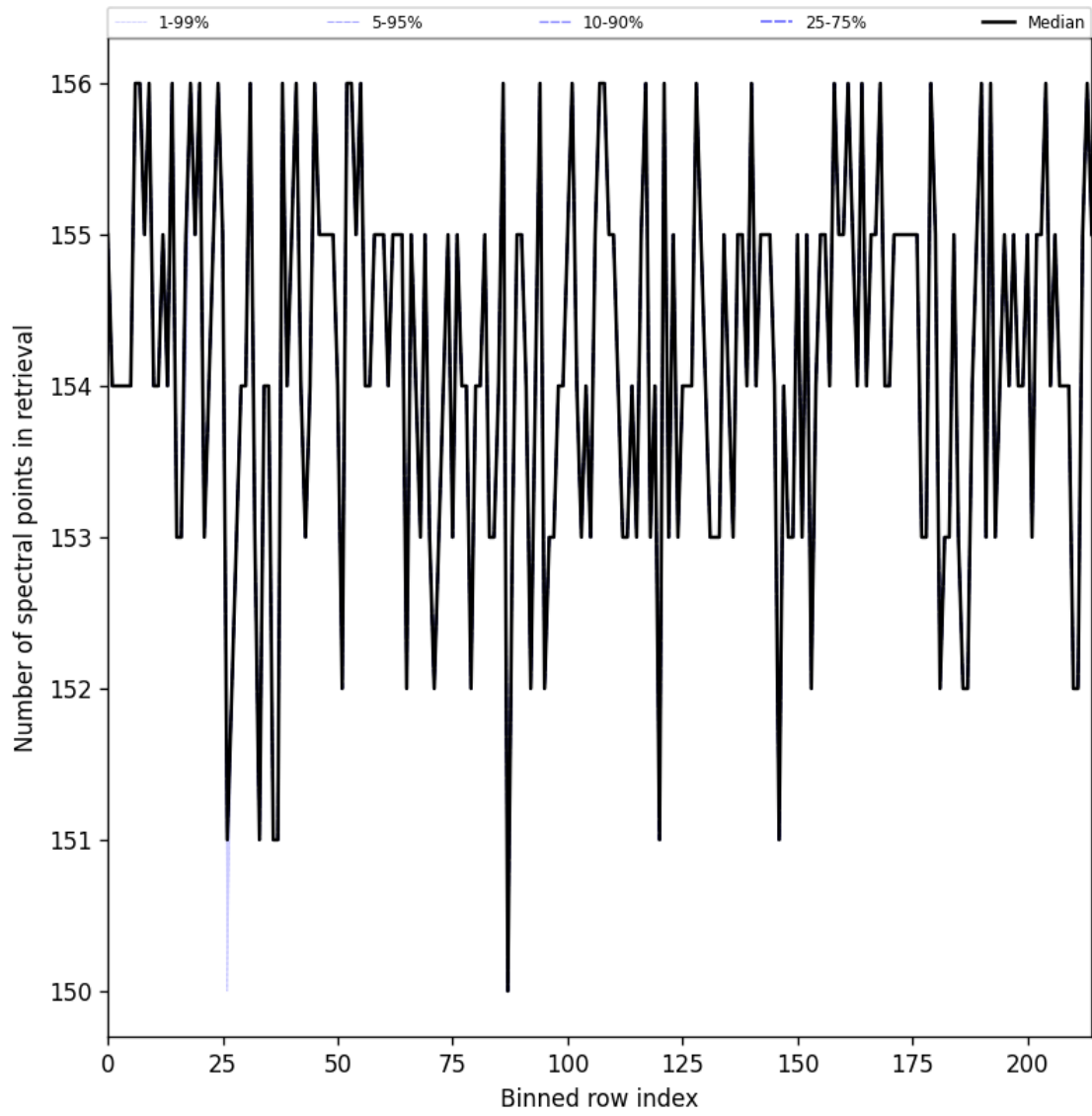
Figure 23: Along track statistics of “Number of spectral points in retrieval” for 2025-06-05 to 2025-06-06
