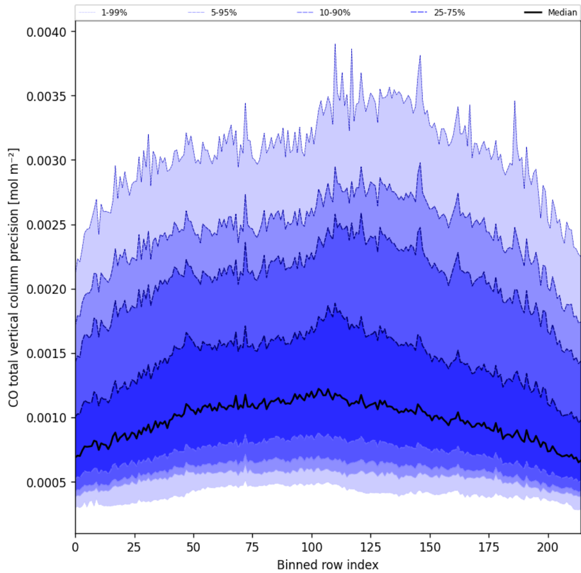
Figure 22: Along track statistics of “CO total vertical column precision” for 2025-06-05 to 2025-06-06
