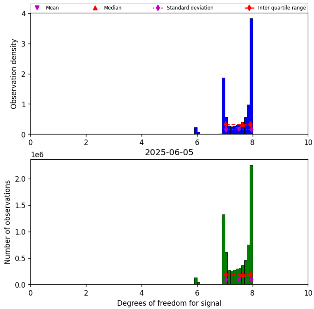
Figure 18: Histogram of “Degrees of freedom for signal” for 2025-06-05 to 2025-06-06
