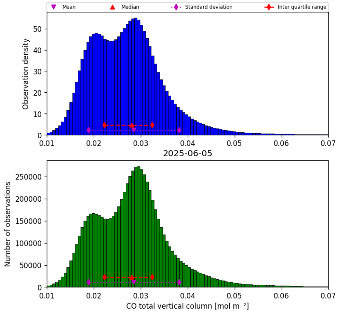
Figure 14: Histogram of “CO total vertical column” for 2025-06-05 to 2025-06-06
