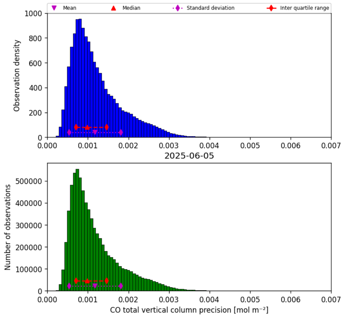
Figure 15: Histogram of “CO total vertical column precision” for 2025-06-05 to 2025-06-06
