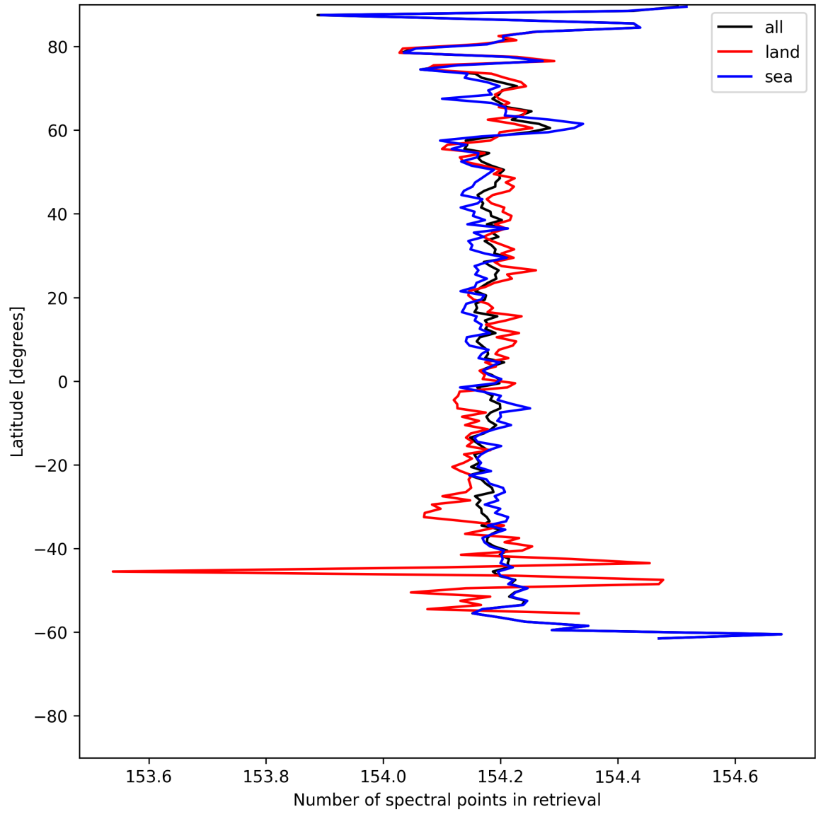
Figure 9: Zonal average of “Number of spectral points in retrieval” for 2025-06-05 to 2025-06-06.
