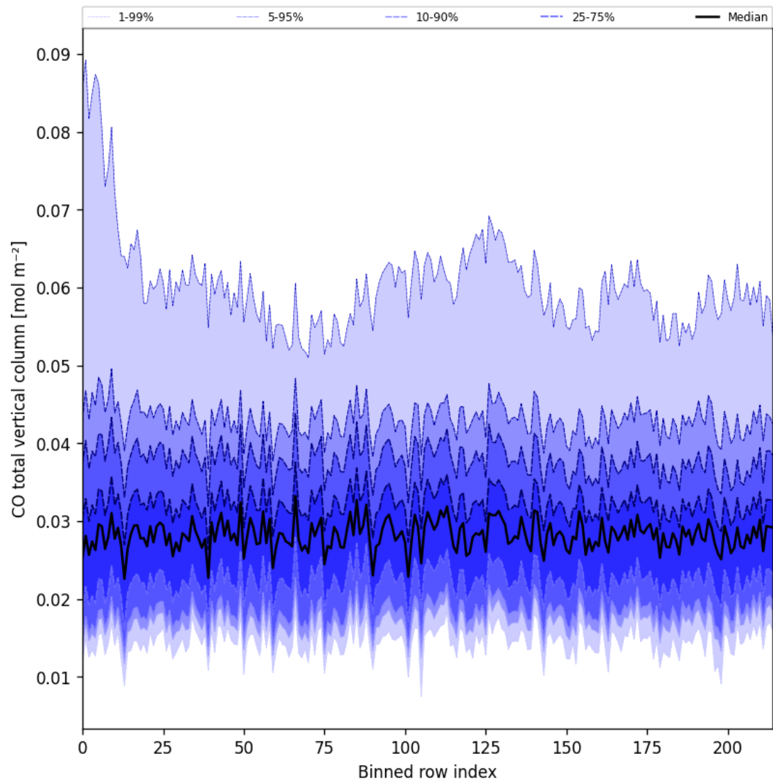
Figure 21: Along track statistics of “CO total vertical column” for 2025-06-05 to 2025-06-06
