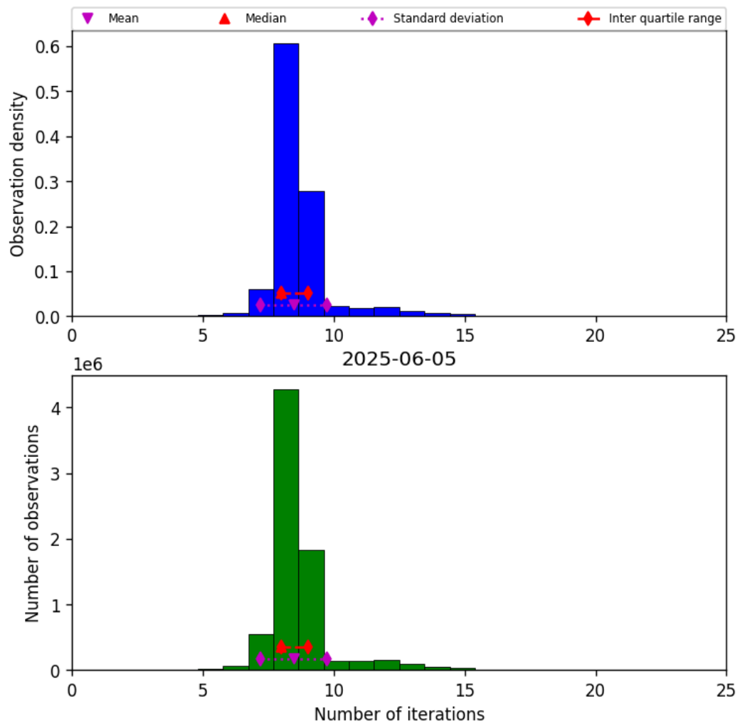
Figure 19: Histogram of “Number of iterations” for 2025-06-05 to 2025-06-06
