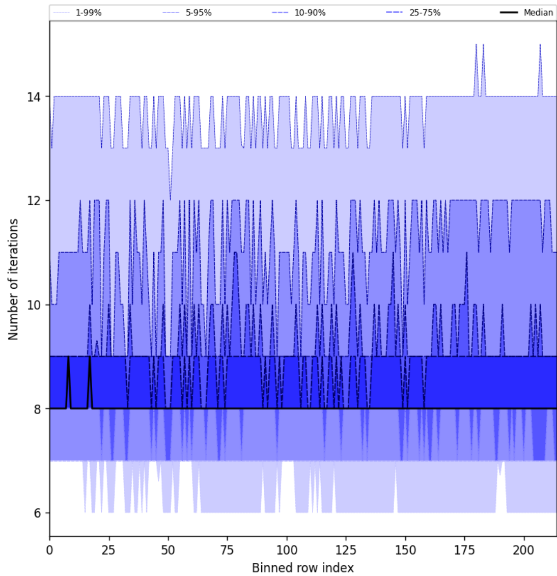
Figure 26: Along track statistics of “Number of iterations” for 2025-06-05 to 2025-06-06
