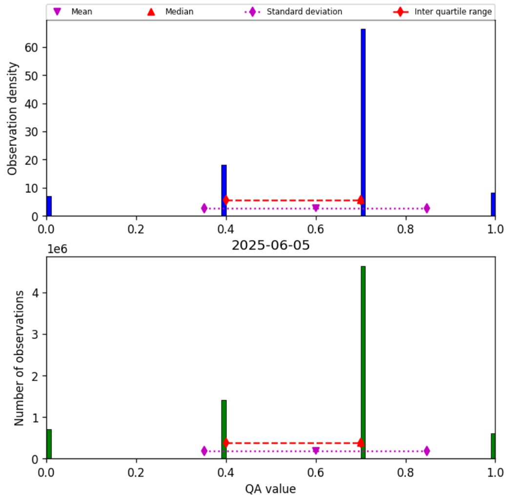
Figure 13: Histogram of “QA value” for 2025-06-05 to 2025-06-06
