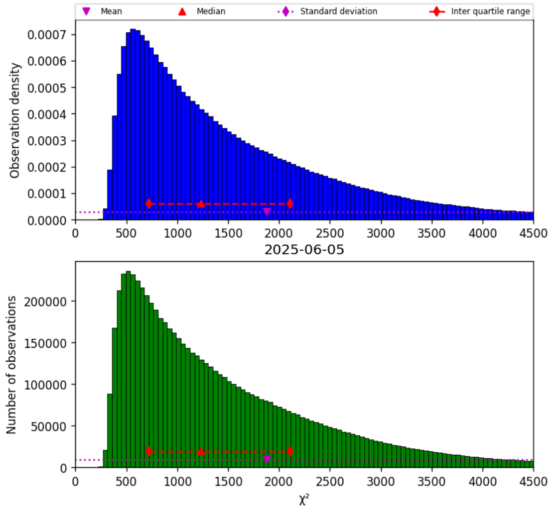
Figure 17: Histogram of " \chi^2 " for 2025-06-05 to 2025-06-06
