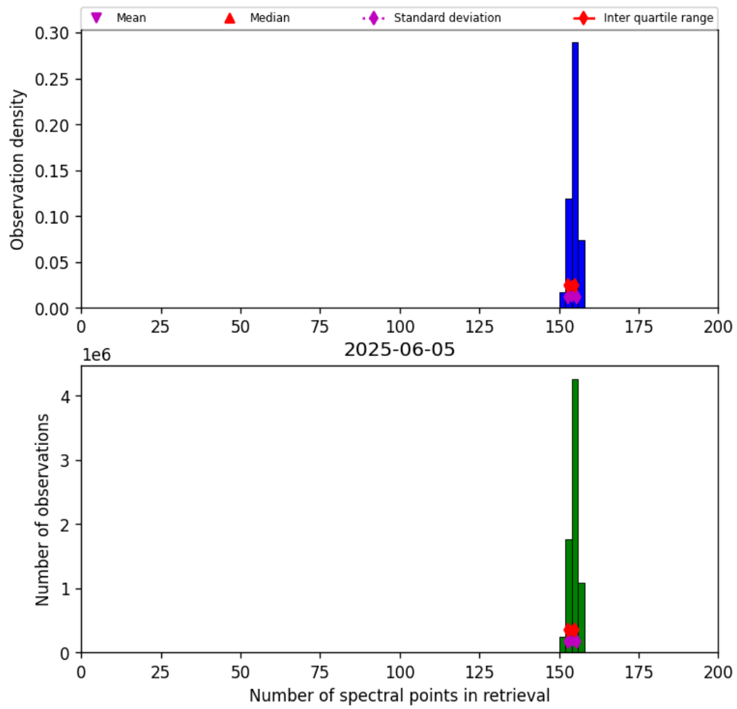
Figure 16: Histogram of “Number of spectral points in retrieval” for 2025-06-05 to 2025-06-06
