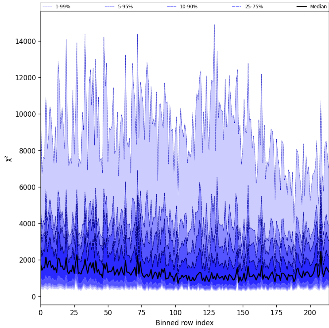
Figure 24: Along track statistics of “ \chi^2 ” for 2025-06-05 to 2025-06-06
