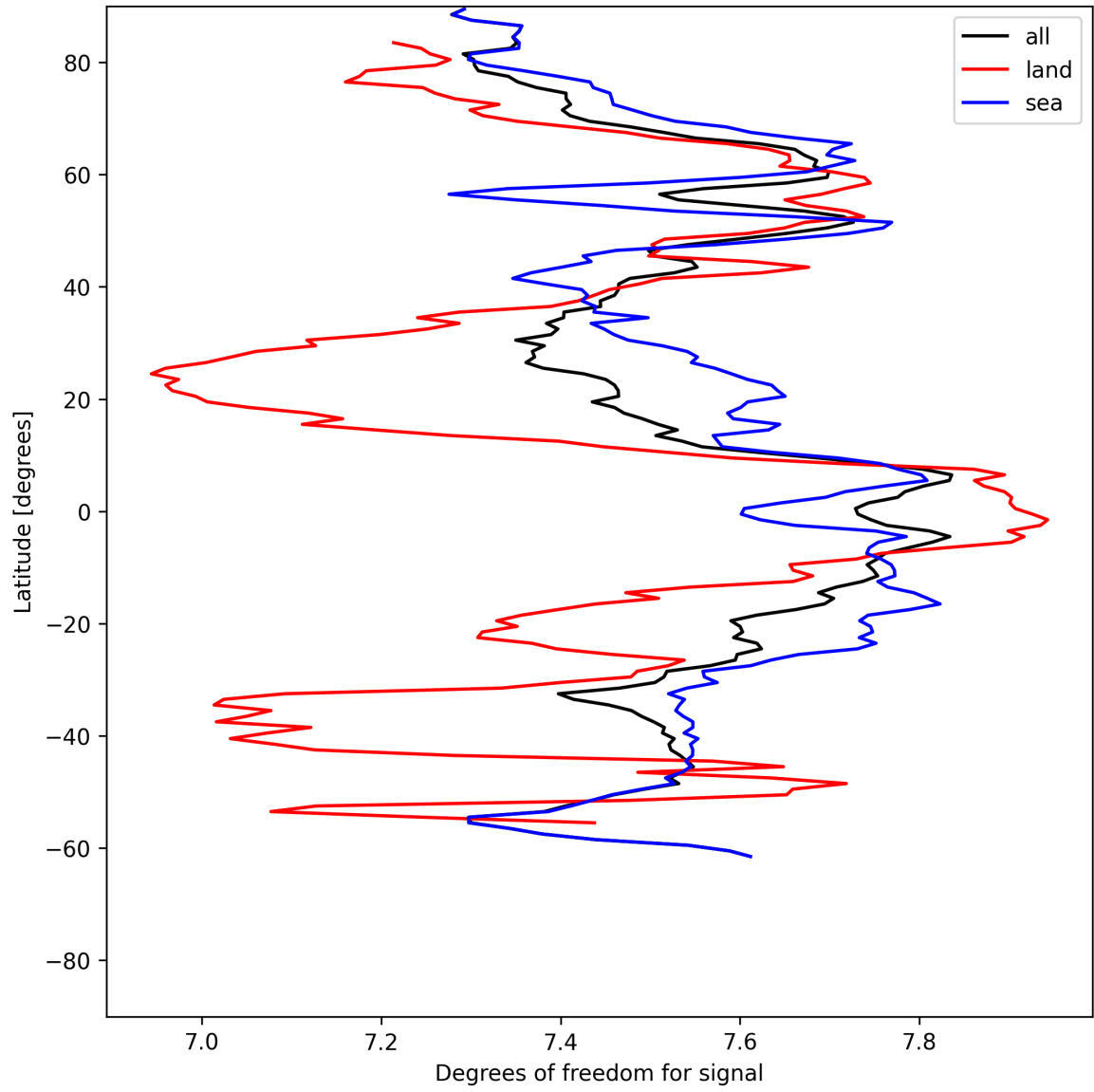
Figure 11: Zonal average of “Degrees of freedom for signal” for 2025-06-05 to 2025-06-06.
