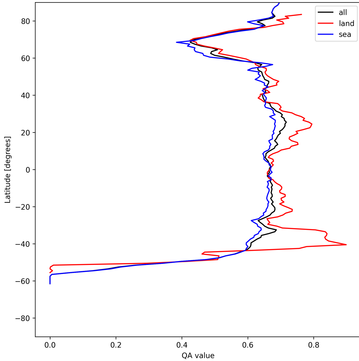
Figure 6: Zonal average of “QA value” for 2025-06-05 to 2025-06-06.
