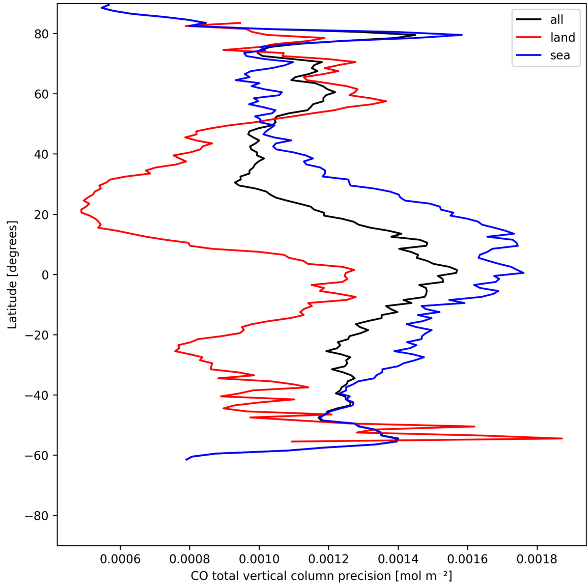
Figure 8: Zonal average of “CO total vertical column precision” for 2025-06-05 to 2025-06-06.
