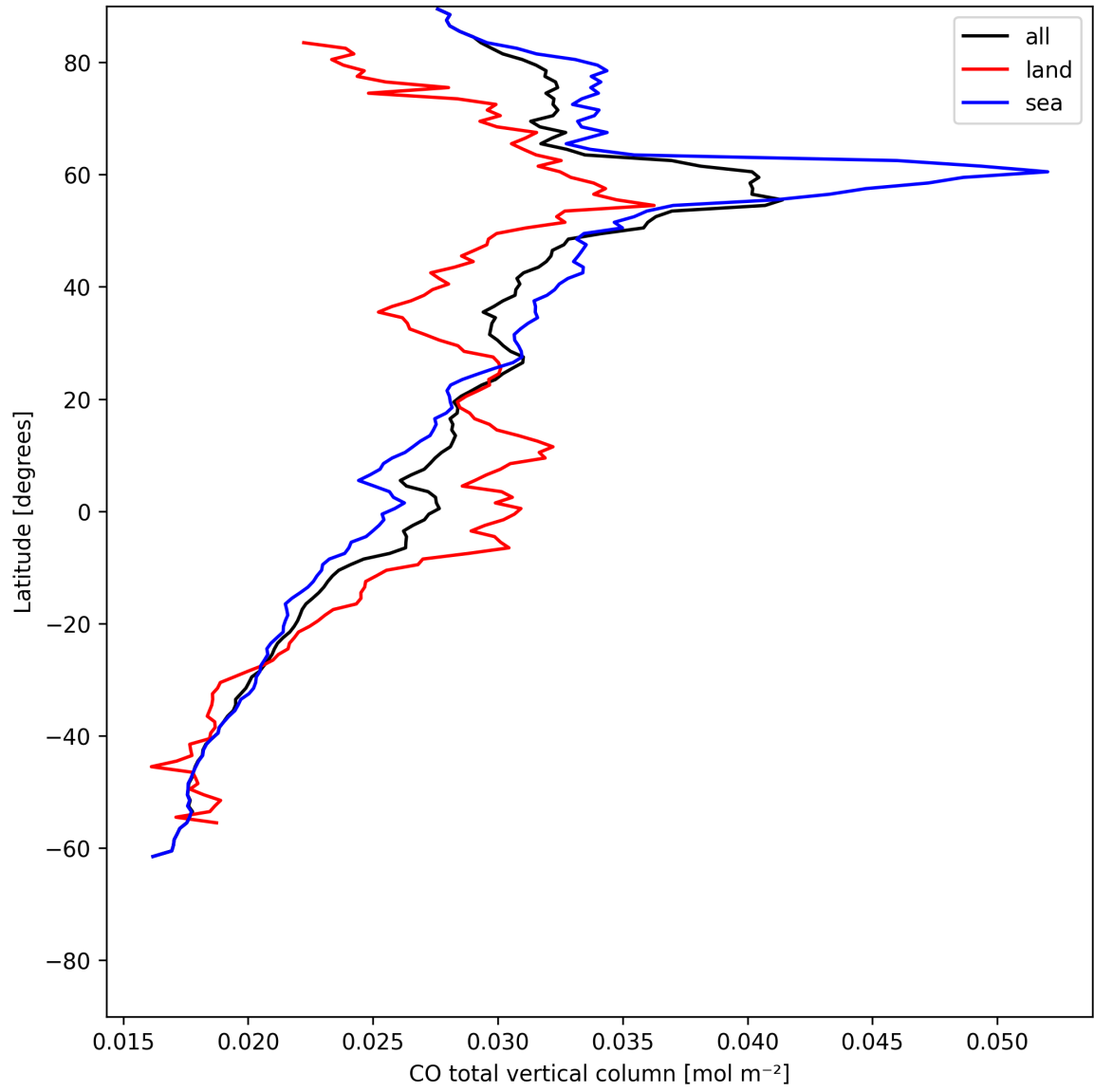
Figure 7: Zonal average of “CO total vertical column” for 2025-06-05 to 2025-06-06.
