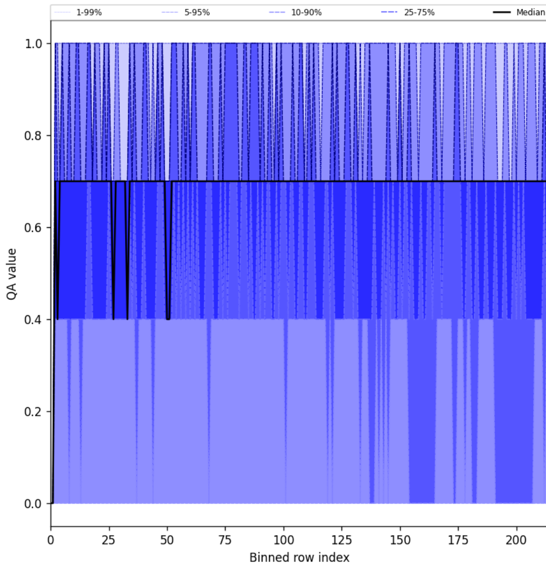
Figure 20: Along track statistics of “QA value” for 2025-06-05 to 2025-06-06
