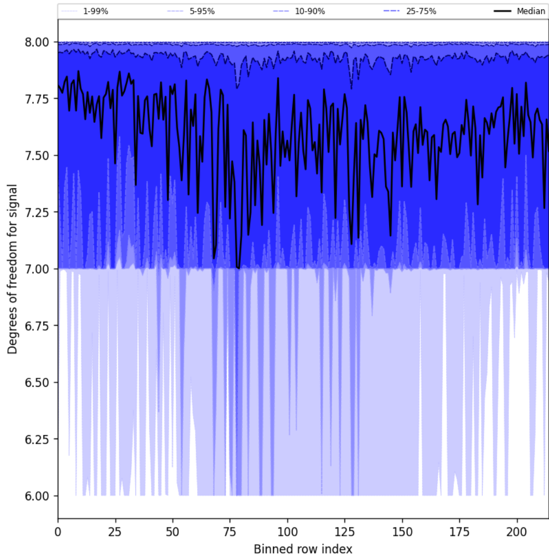
Figure 25: Along track statistics of “Degrees of freedom for signal” for 2025-06-05 to 2025-06-06
