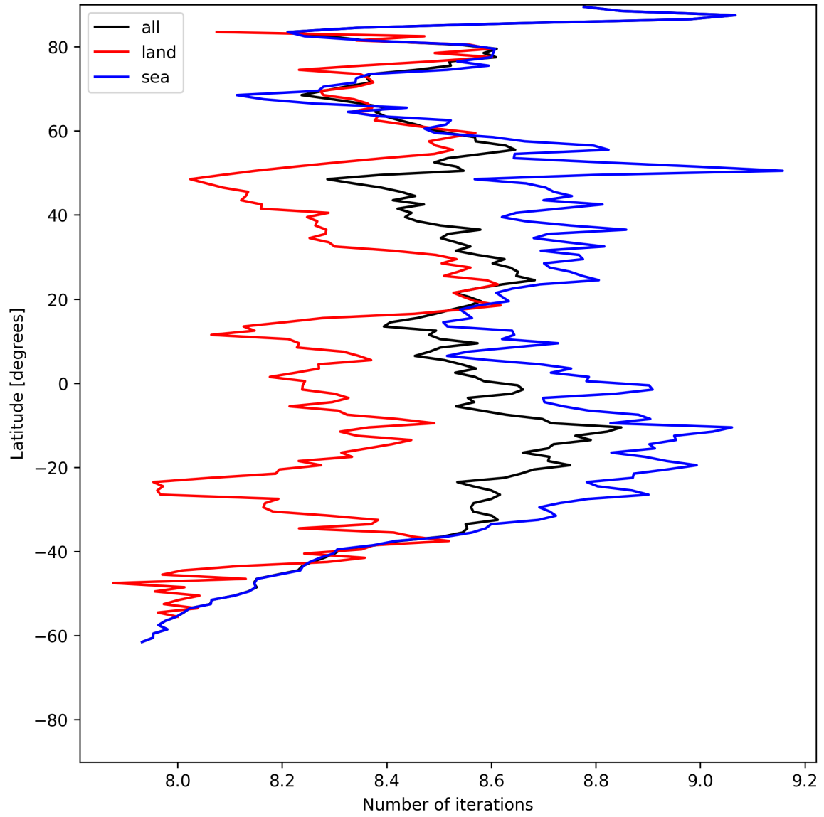
Figure 12: Zonal average of “Number of iterations” for 2025-06-05 to 2025-06-06.
