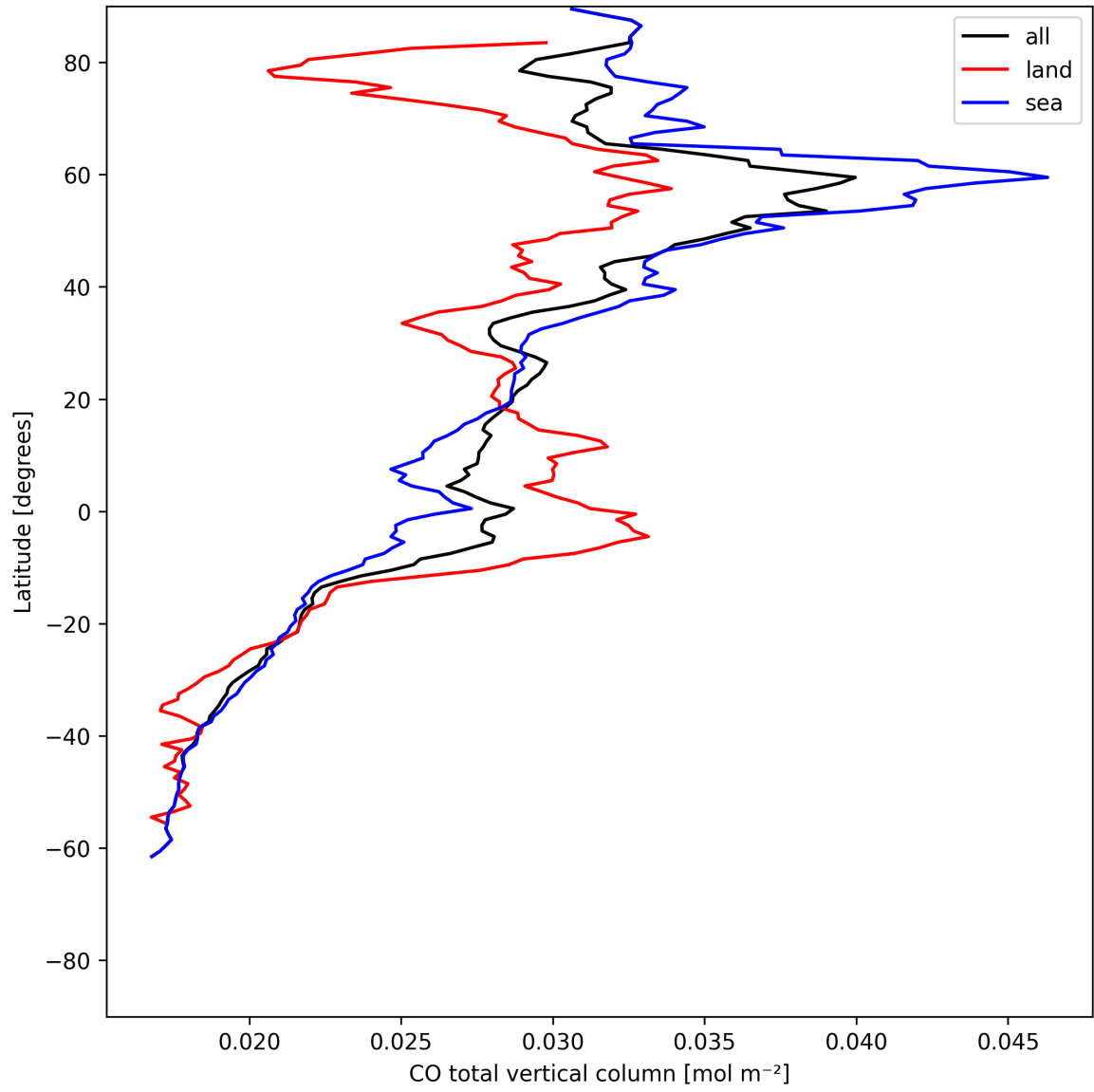
Figure 7: Zonal average of “CO total vertical column” for 2025-06-07 to 2025-06-08.
