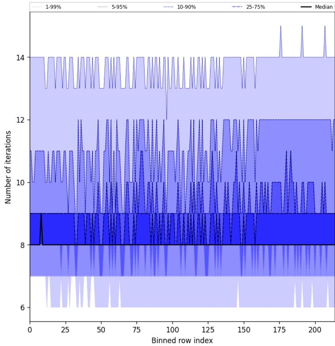
Figure 26: Along track statistics of “Number of iterations” for 2025-06-07 to 2025-06-08
