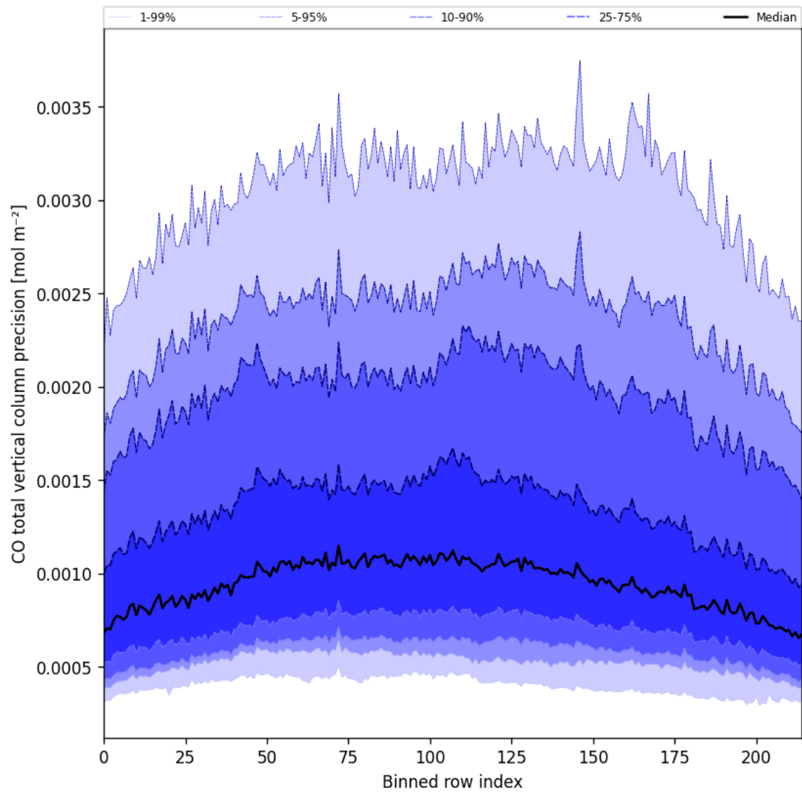
Figure 22: Along track statistics of “CO total vertical column precision” for 2025-06-07 to 2025-06-08
