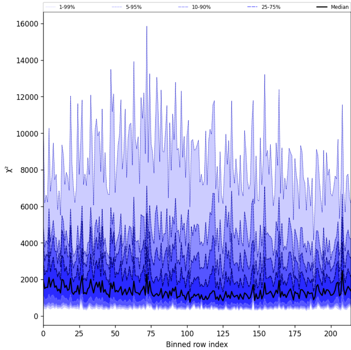
Figure 24: Along track statistics of “ \chi^2 ” for 2025-06-07 to 2025-06-08
