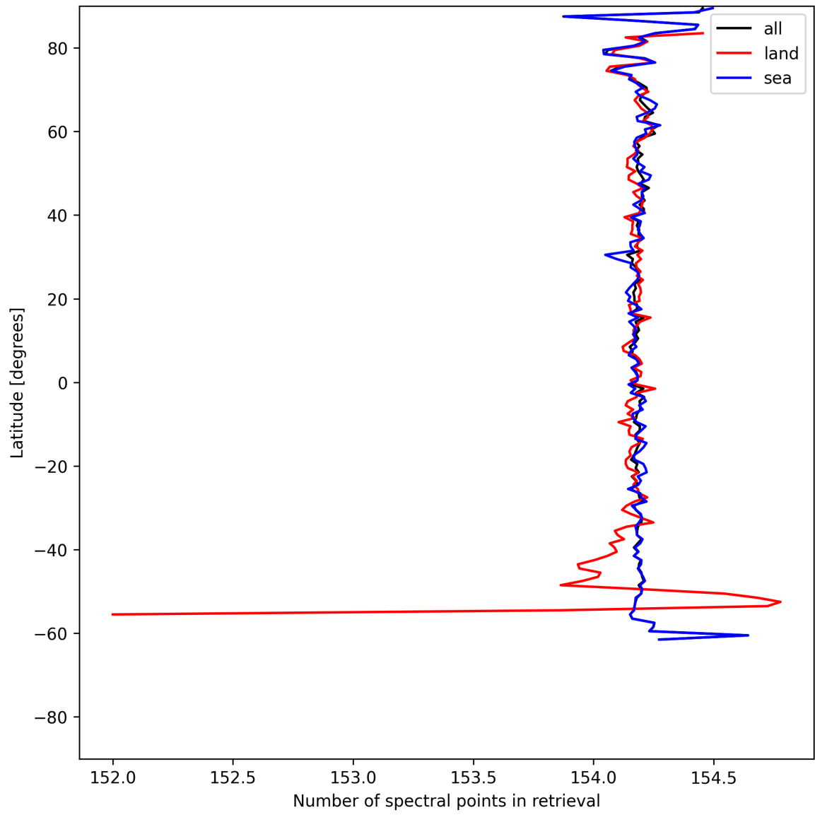
Figure 9: Zonal average of “Number of spectral points in retrieval” for 2025-06-07 to 2025-06-08.
