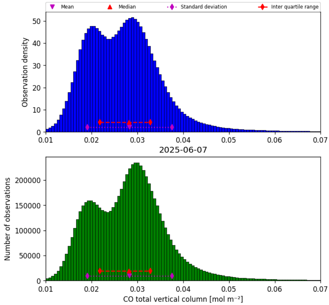
Figure 14: Histogram of “CO total vertical column” for 2025-06-07 to 2025-06-08
