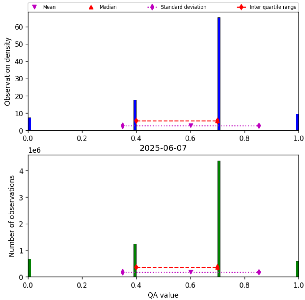
Figure 13: Histogram of “QA value” for 2025-06-07 to 2025-06-08
