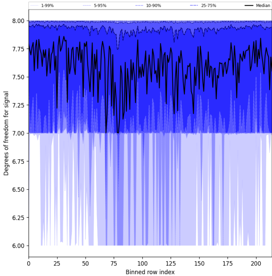
Figure 25: Along track statistics of “Degrees of freedom for signal” for 2025-06-07 to 2025-06-08
