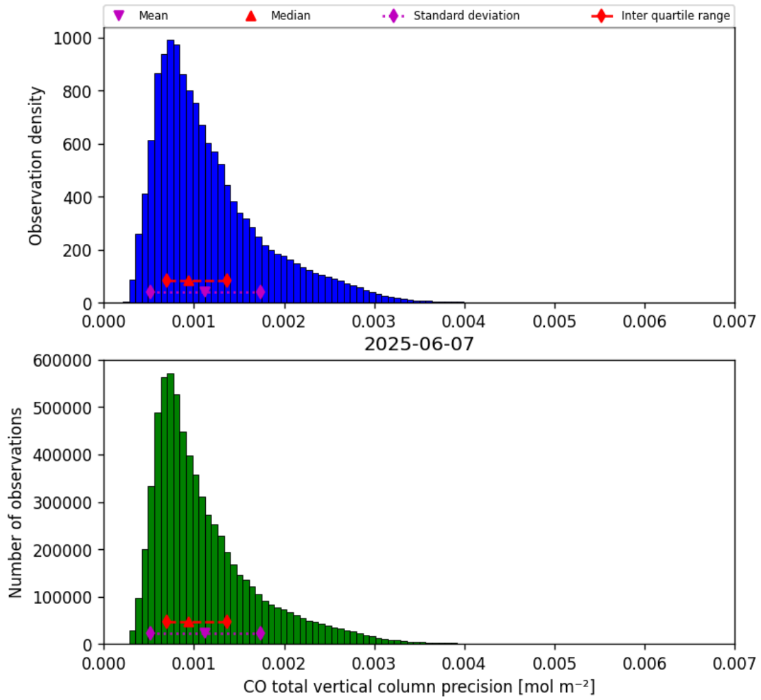
Figure 15: Histogram of “CO total vertical column precision” for 2025-06-07 to 2025-06-08
