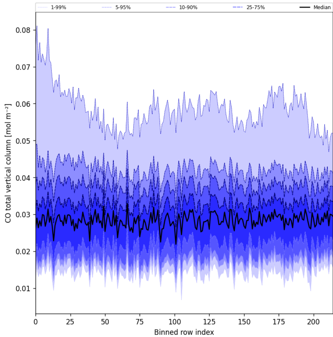
Figure 21: Along track statistics of “CO total vertical column” for 2025-06-07 to 2025-06-08
