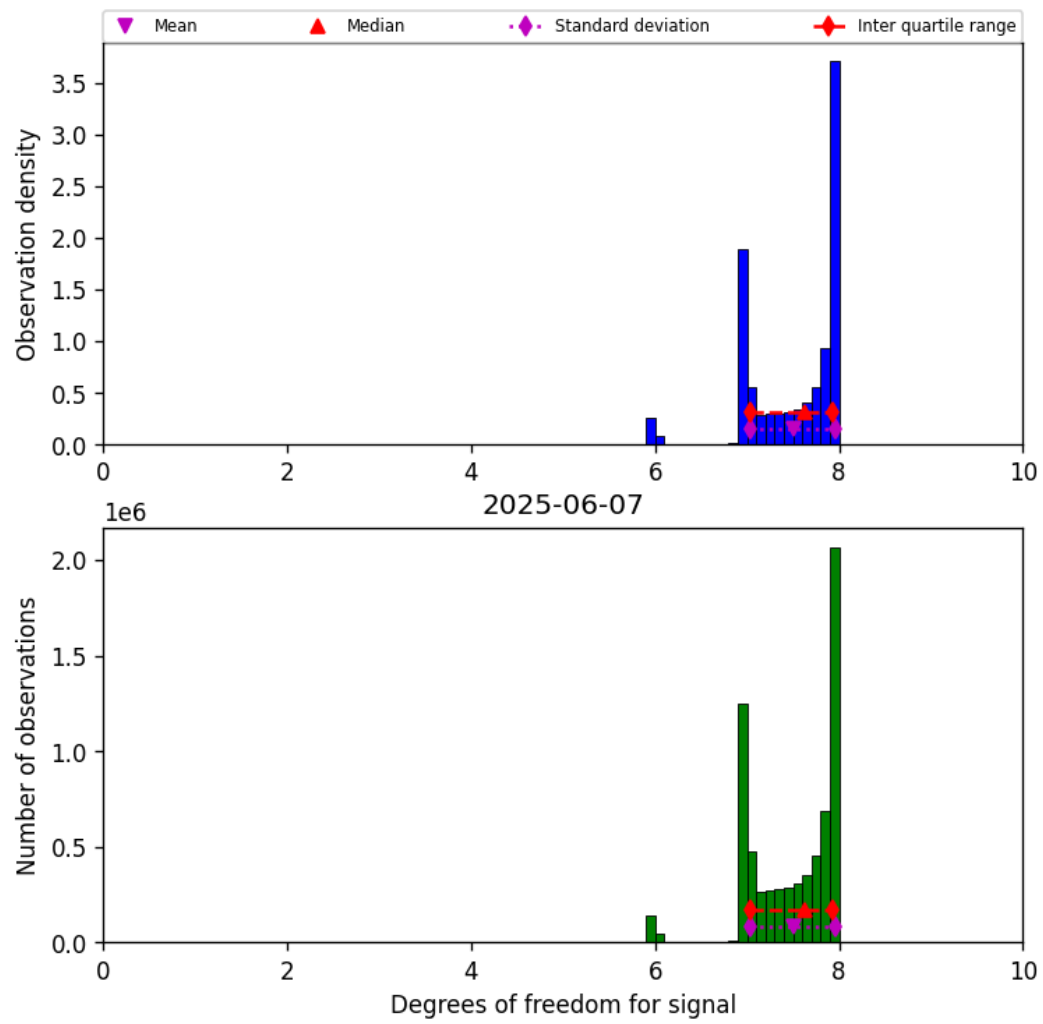
Figure 18: Histogram of “Degrees of freedom for signal” for 2025-06-07 to 2025-06-08
