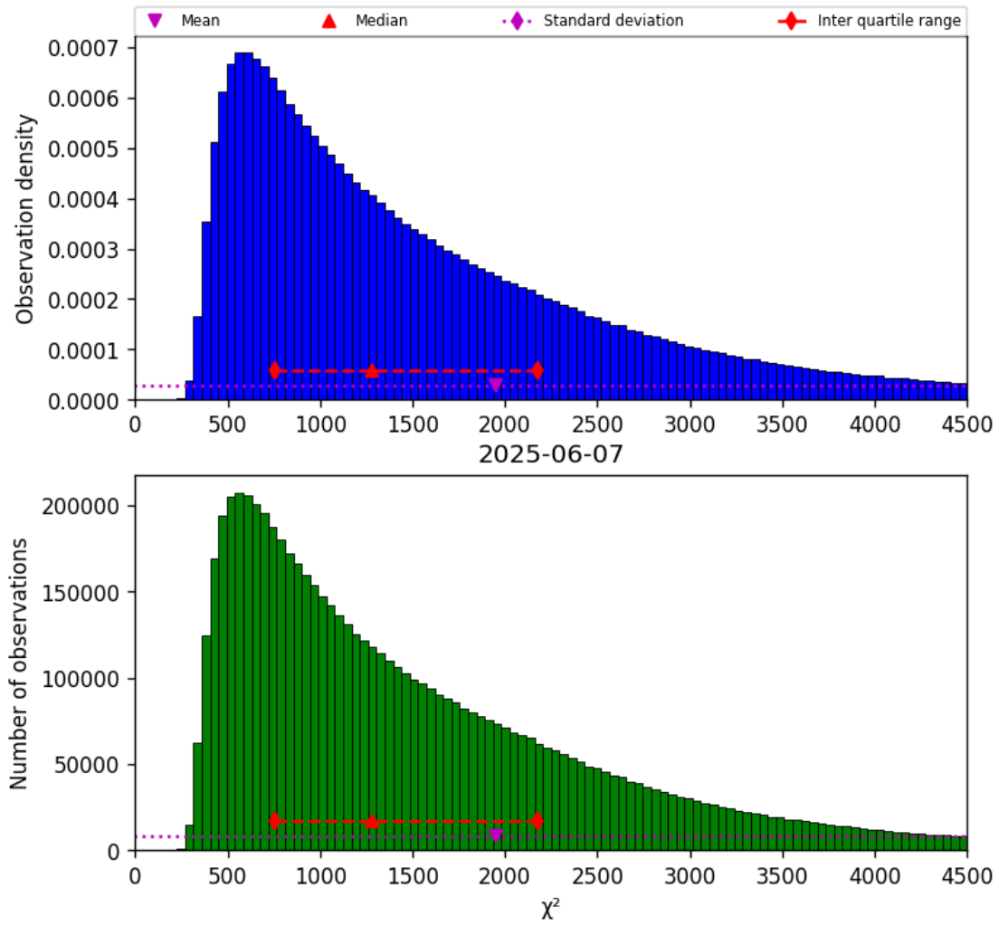
Figure 17: Histogram of " \chi^2 " for 2025-06-07 to 2025-06-08
