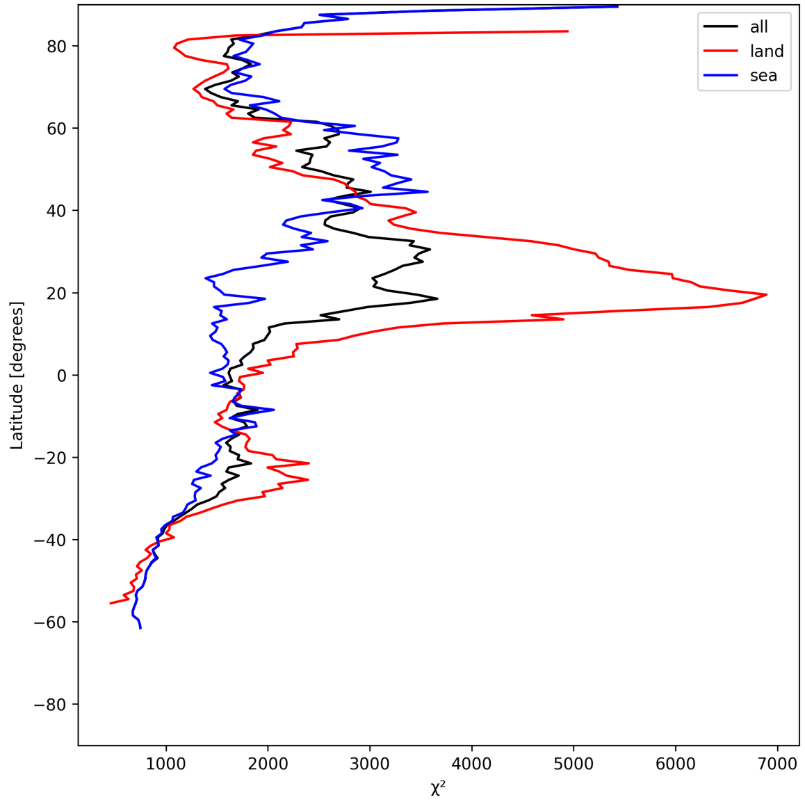
Figure 10: Zonal average of “ \chi^2 ” for 2025-06-07 to 2025-06-08.
