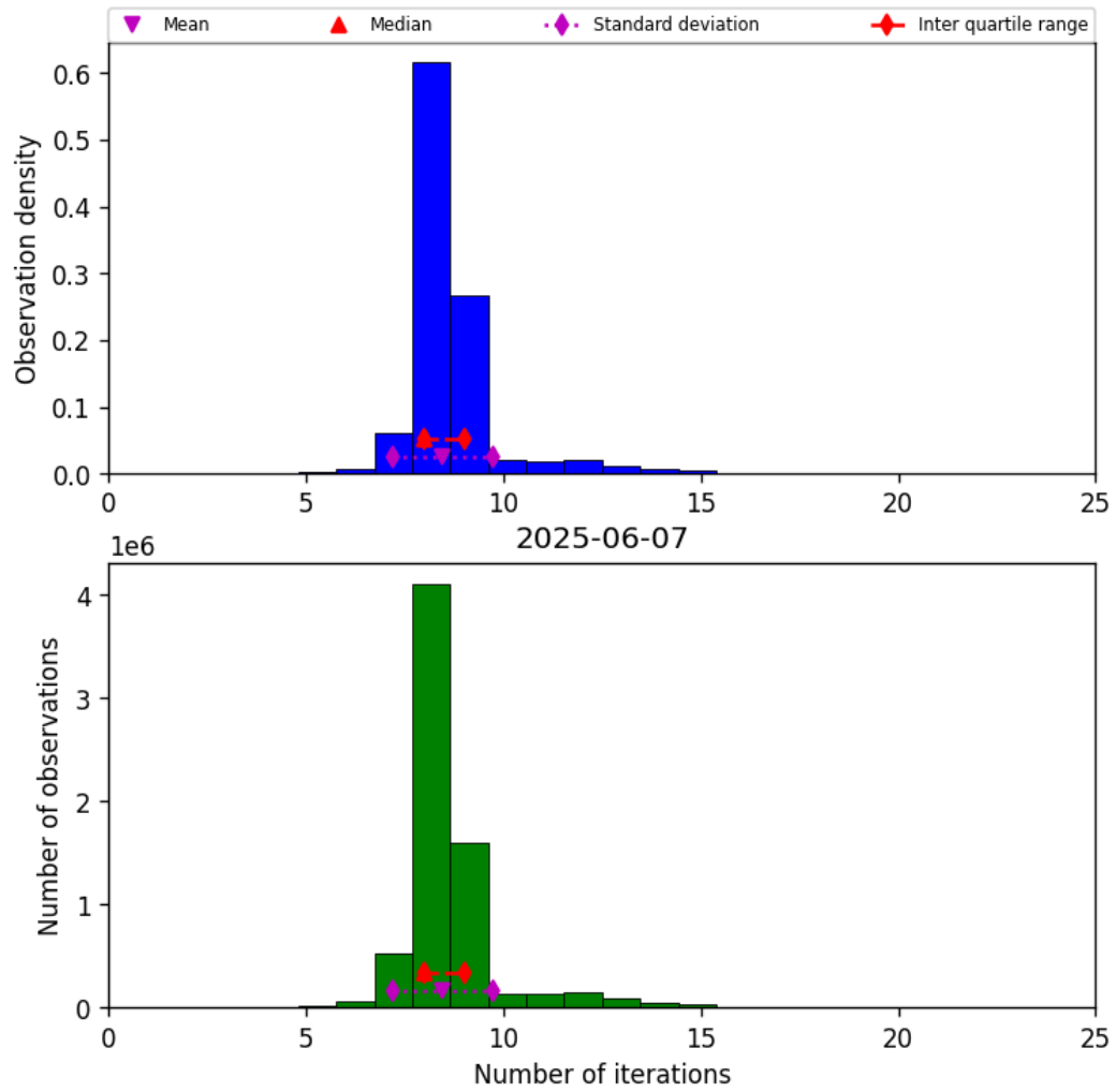
Figure 19: Histogram of “Number of iterations” for 2025-06-07 to 2025-06-08
