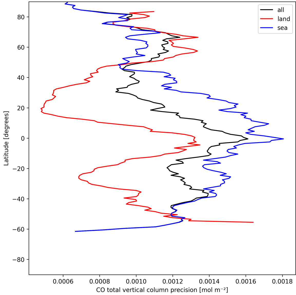
Figure 8: Zonal average of “CO total vertical column precision” for 2025-06-07 to 2025-06-08.
