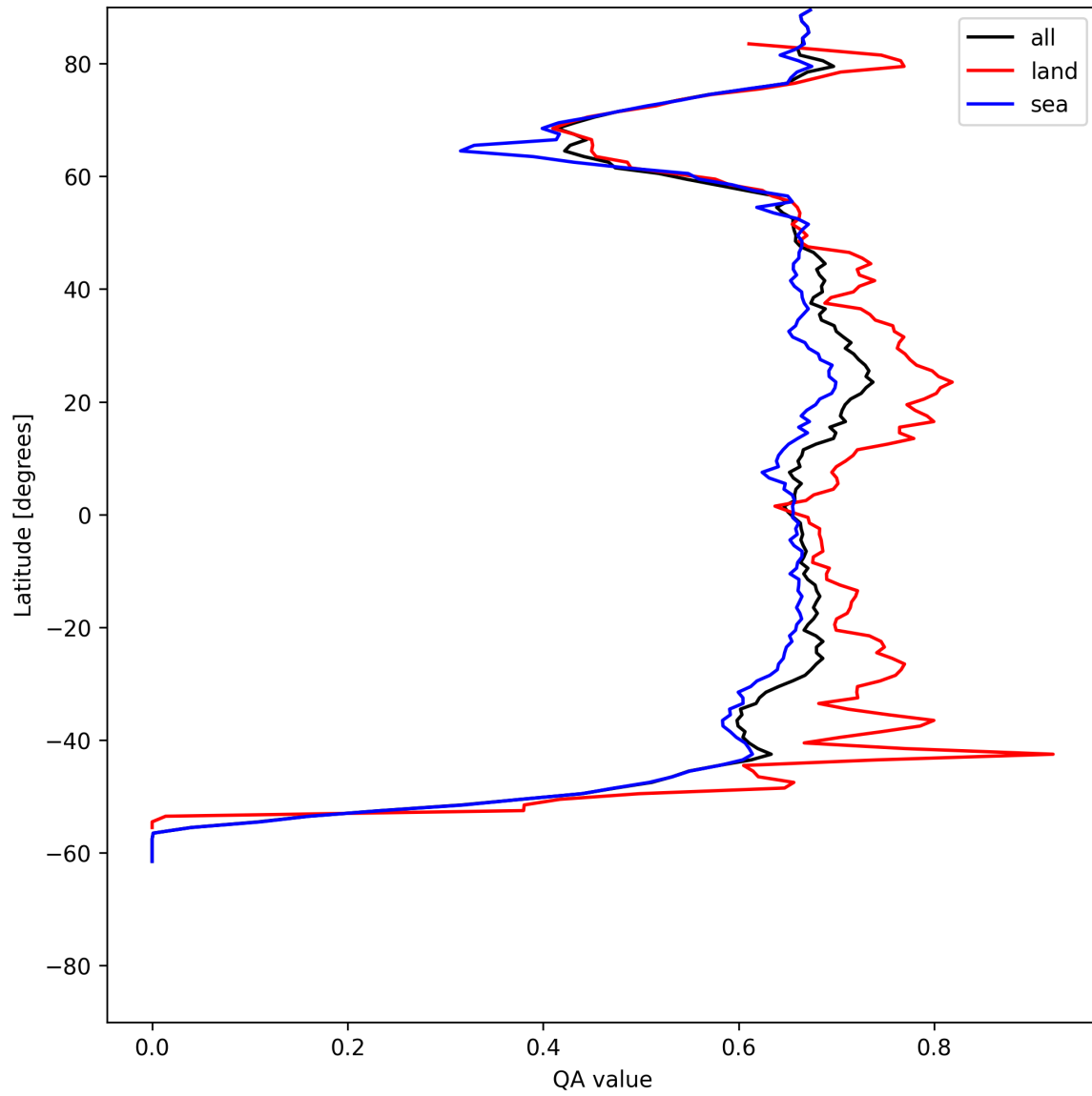
Figure 6: Zonal average of “QA value” for 2025-06-07 to 2025-06-08.
