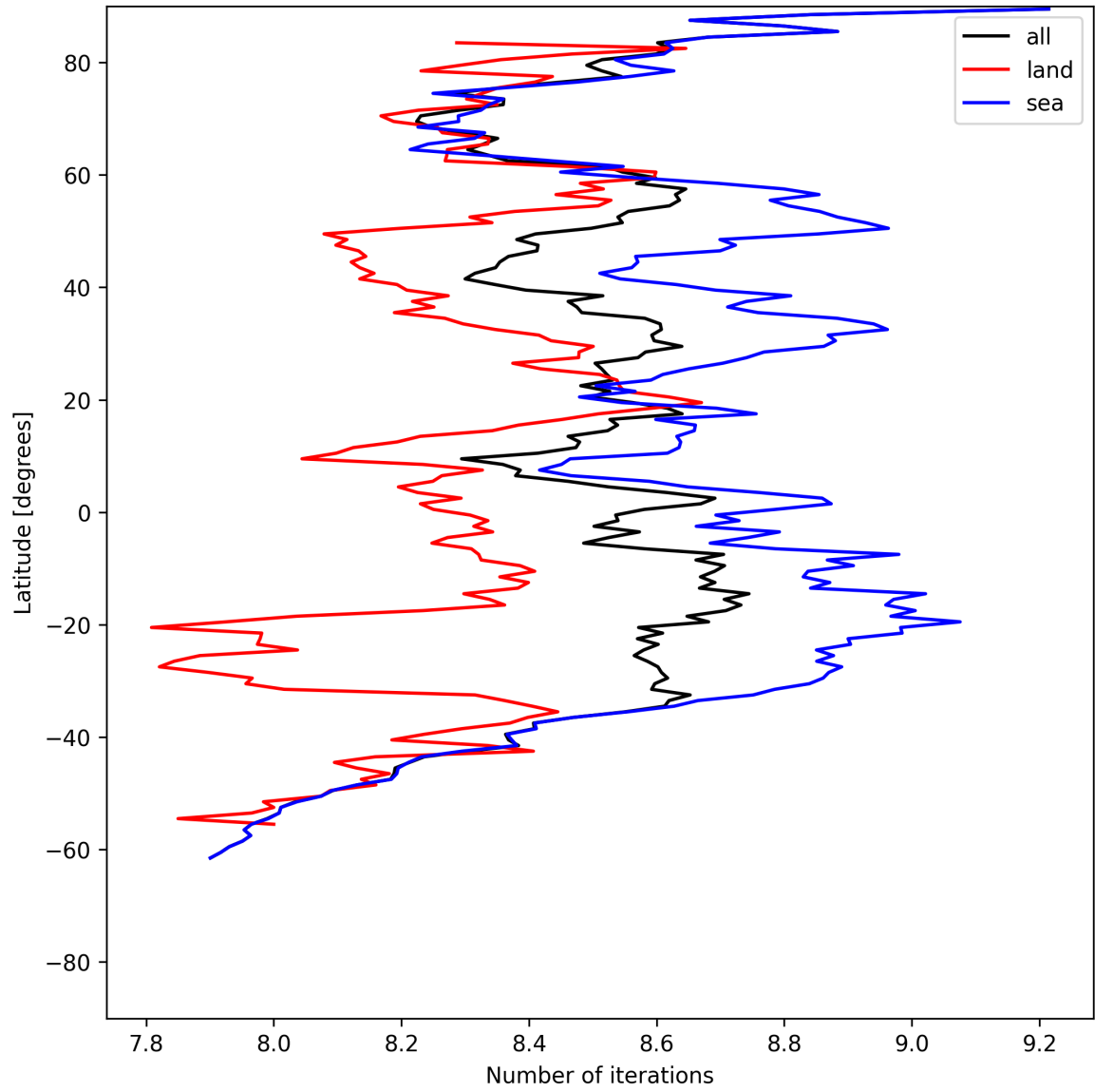
Figure 12: Zonal average of “Number of iterations” for 2025-06-07 to 2025-06-08.
