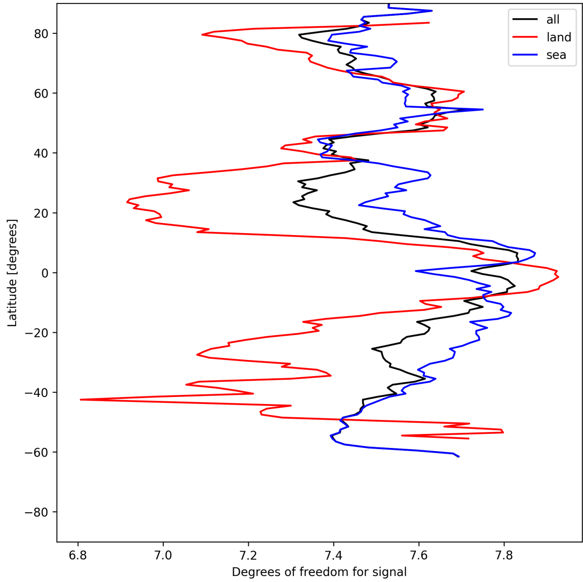
Figure 11: Zonal average of “Degrees of freedom for signal” for 2025-06-07 to 2025-06-08.
