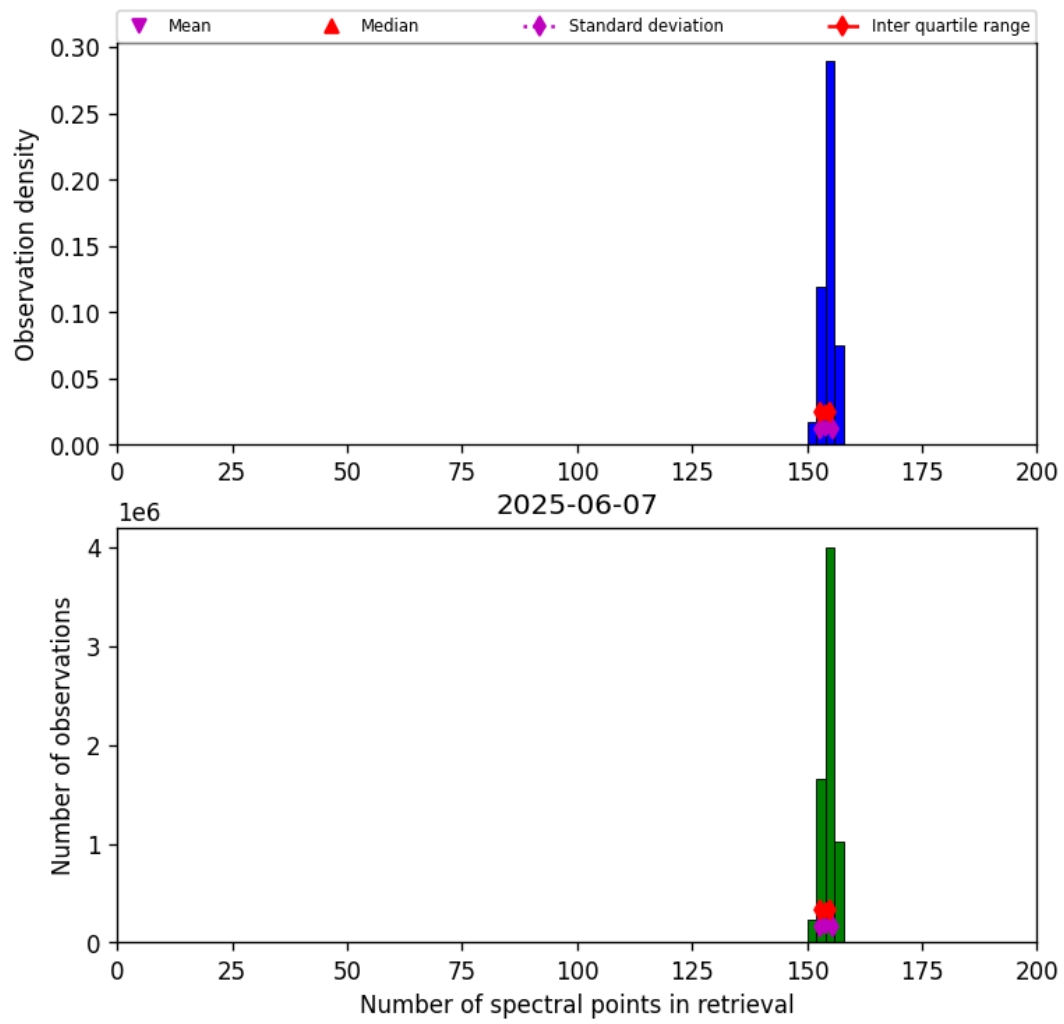
Figure 16: Histogram of “Number of spectral points in retrieval” for 2025-06-07 to 2025-06-08
