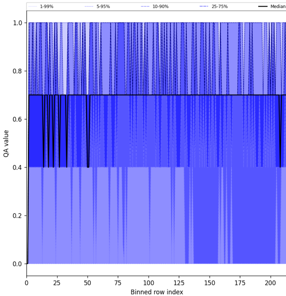
Figure 20: Along track statistics of “QA value” for 2025-06-08 to 2025-06-09
