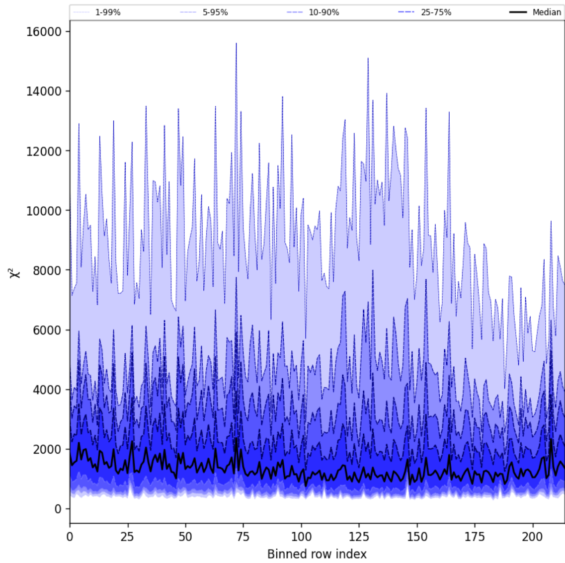
Figure 24: Along track statistics of “ \chi^2 ” for 2025-06-08 to 2025-06-09
