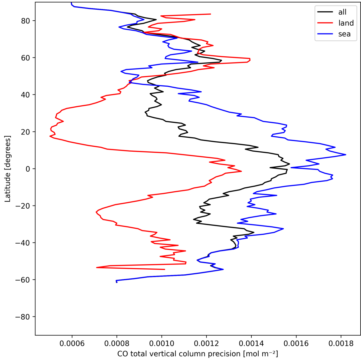
Figure 8: Zonal average of “CO total vertical column precision” for 2025-06-08 to 2025-06-09.
