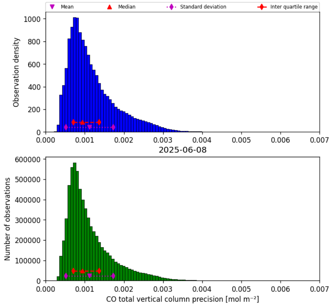
Figure 15: Histogram of “CO total vertical column precision” for 2025-06-08 to 2025-06-09
