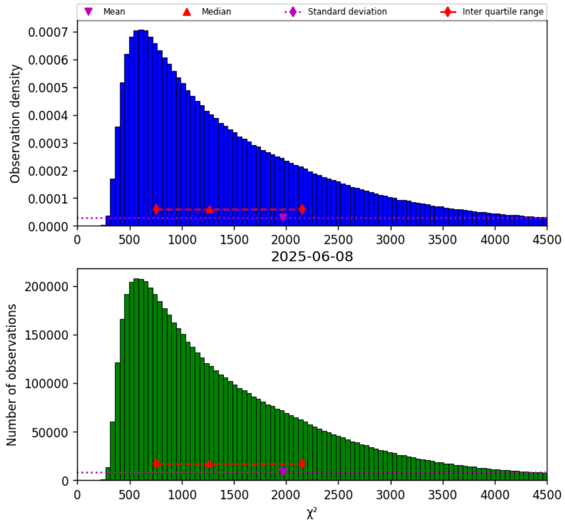
Figure 17: Histogram of " \chi^2 " for 2025-06-08 to 2025-06-09
