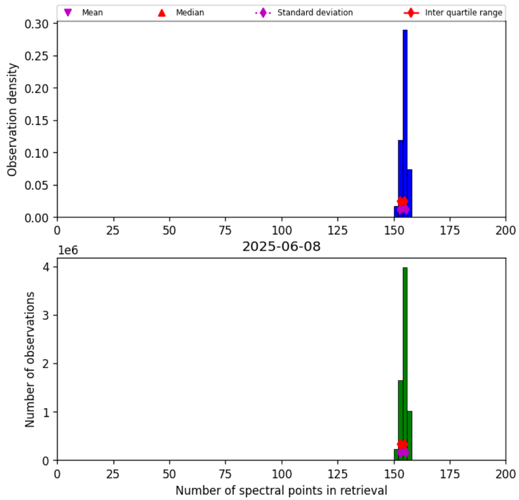
Figure 16: Histogram of “Number of spectral points in retrieval” for 2025-06-08 to 2025-06-09
