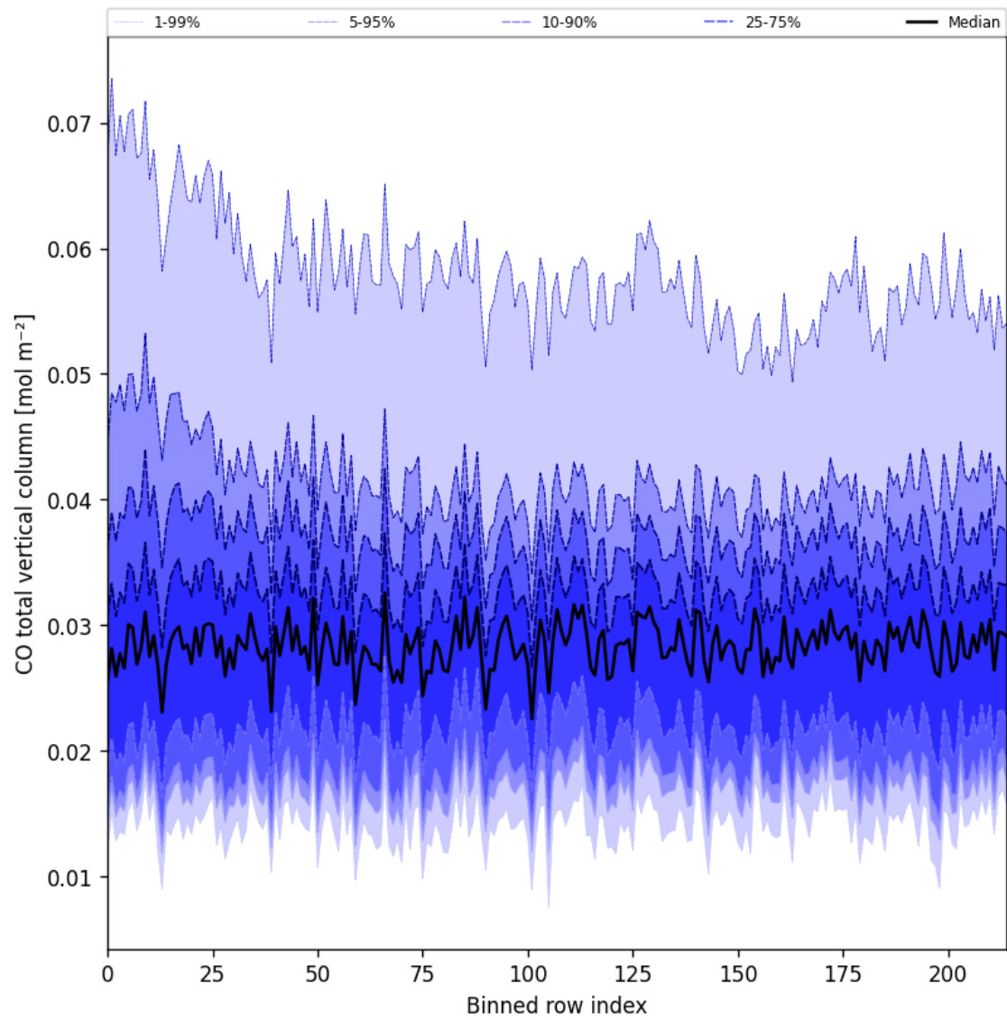
Figure 21: Along track statistics of “CO total vertical column” for 2025-06-08 to 2025-06-09
