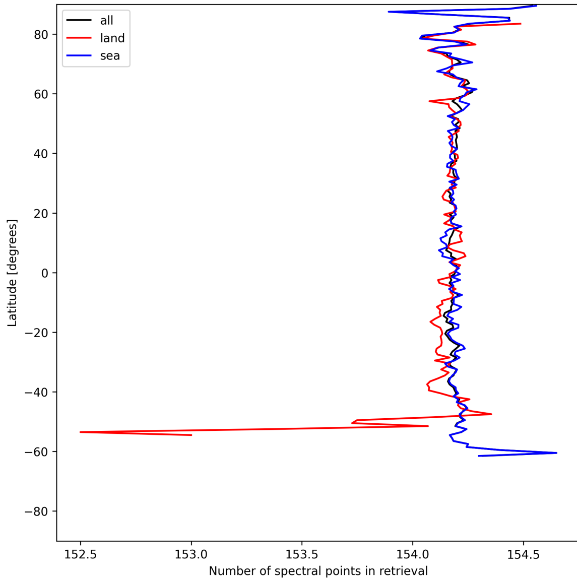
Figure 9: Zonal average of “Number of spectral points in retrieval” for 2025-06-08 to 2025-06-09.
