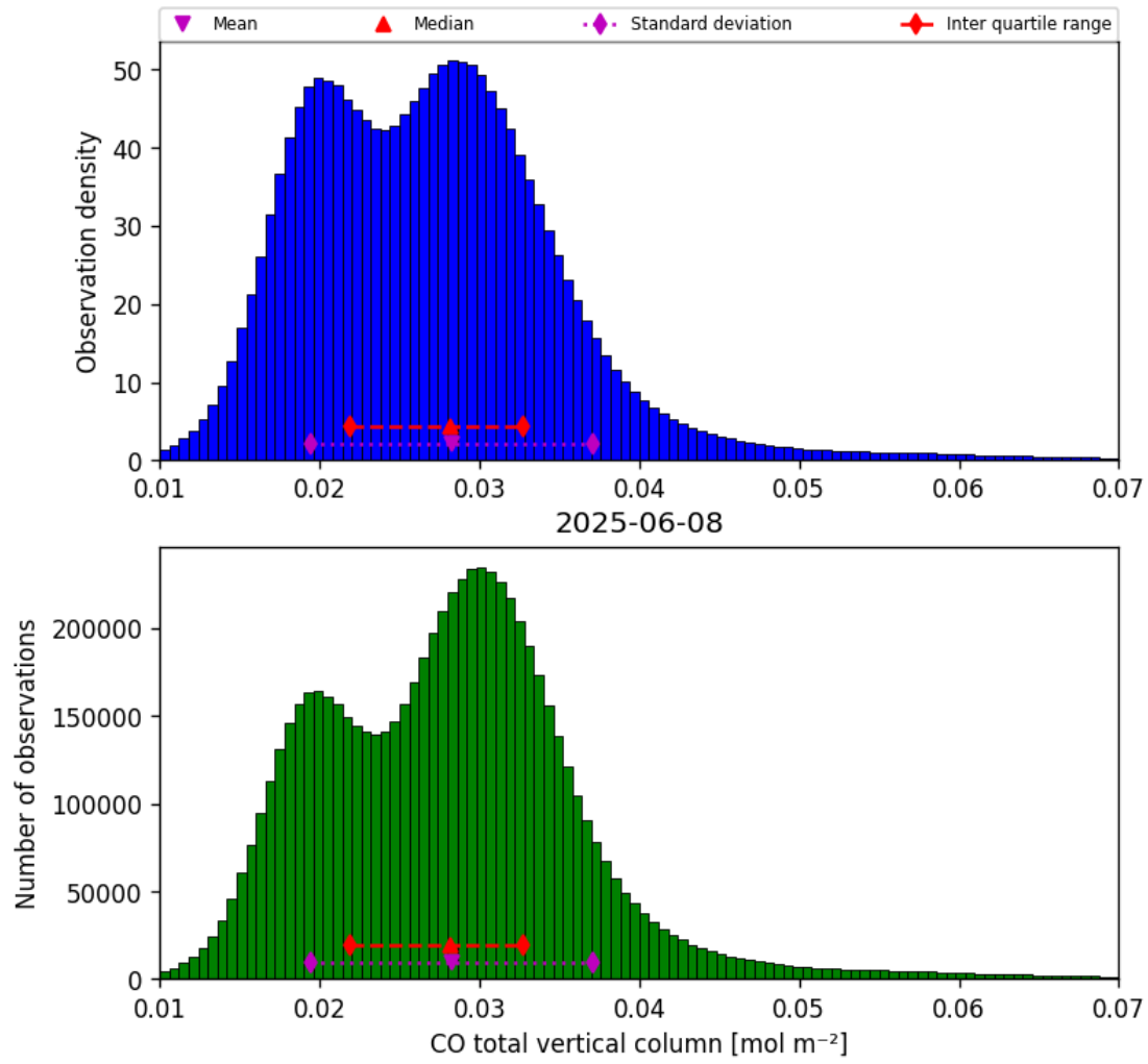
Figure 14: Histogram of “CO total vertical column” for 2025-06-08 to 2025-06-09
