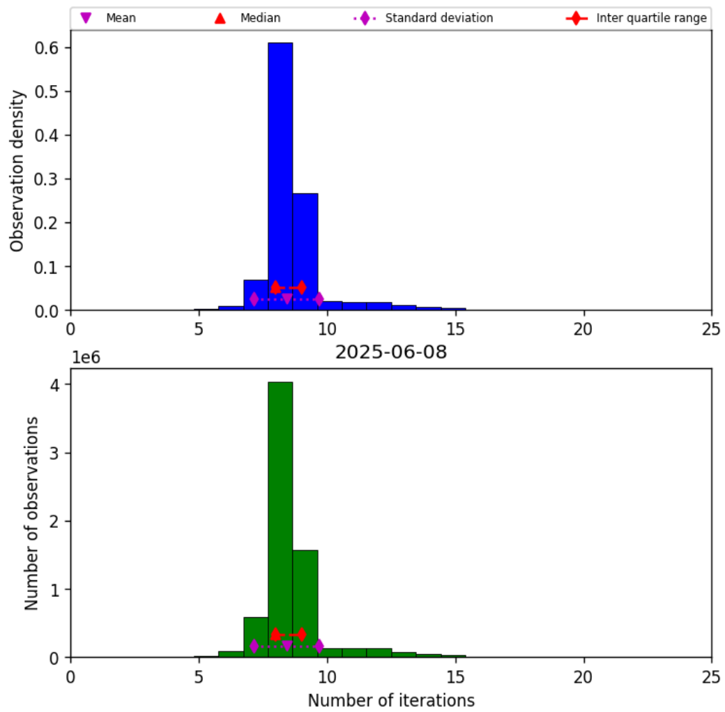
Figure 19: Histogram of “Number of iterations” for 2025-06-08 to 2025-06-09
