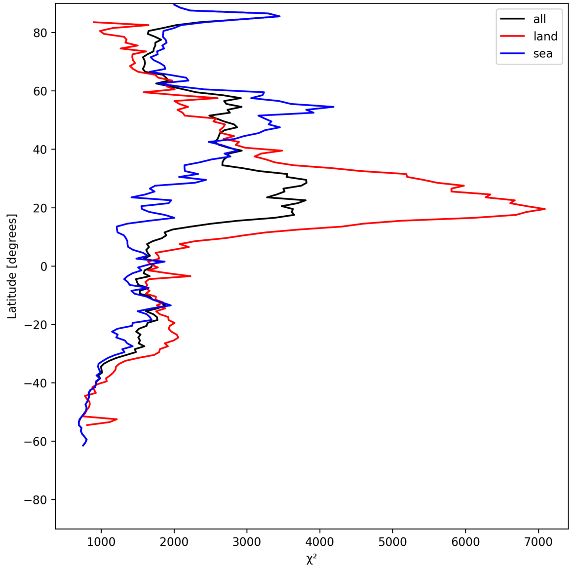
Figure 10: Zonal average of “ \chi^2 ” for 2025-06-08 to 2025-06-09.
