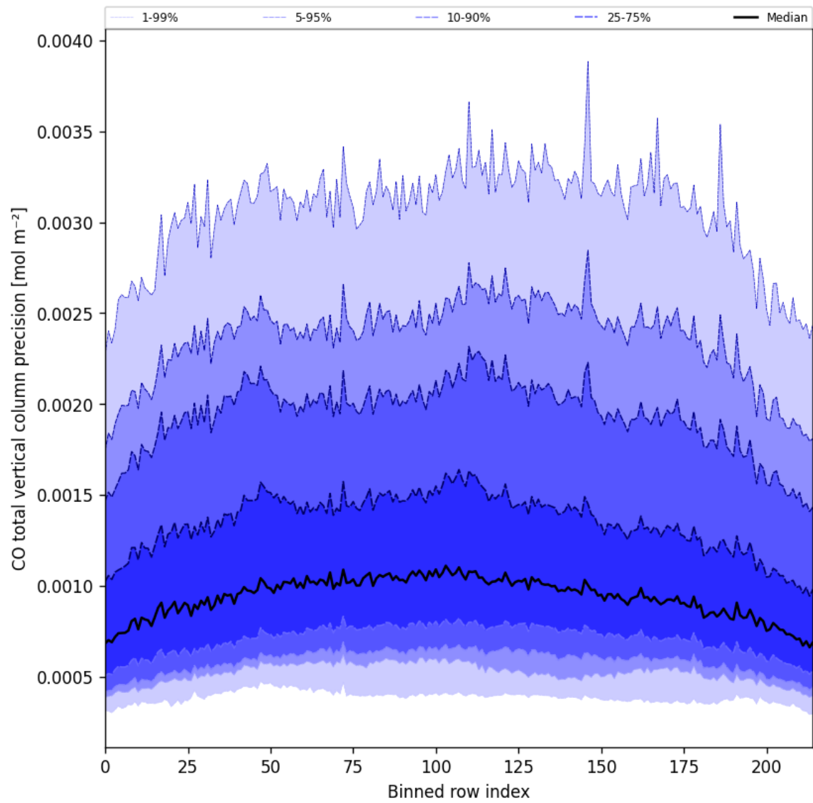
Figure 22: Along track statistics of “CO total vertical column precision” for 2025-06-08 to 2025-06-09
