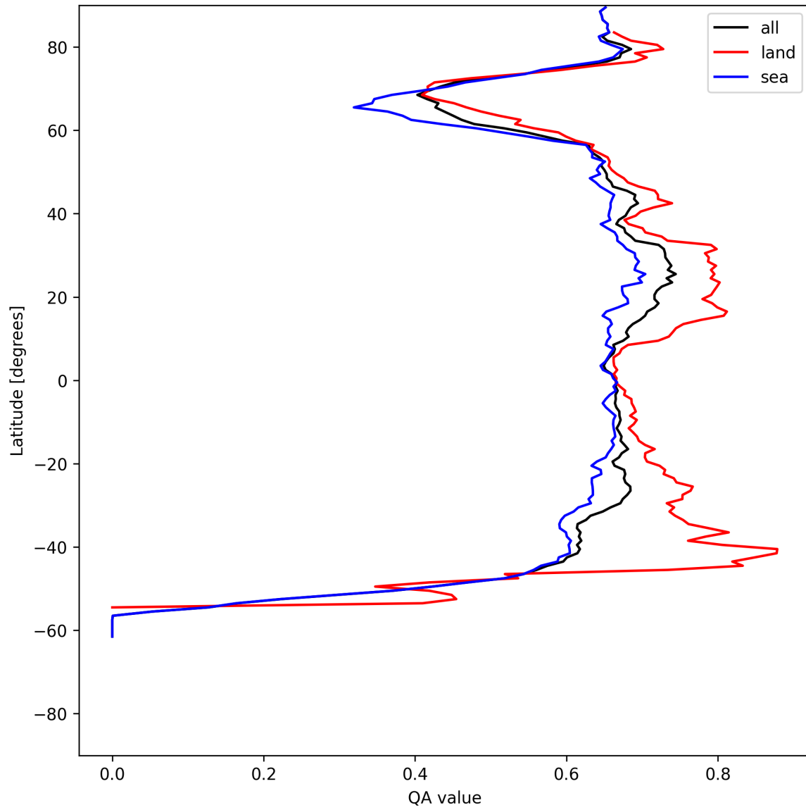
Figure 6: Zonal average of “QA value” for 2025-06-08 to 2025-06-09.
