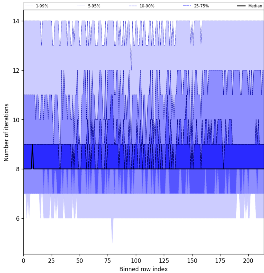
Figure 26: Along track statistics of “Number of iterations” for 2025-06-08 to 2025-06-09
