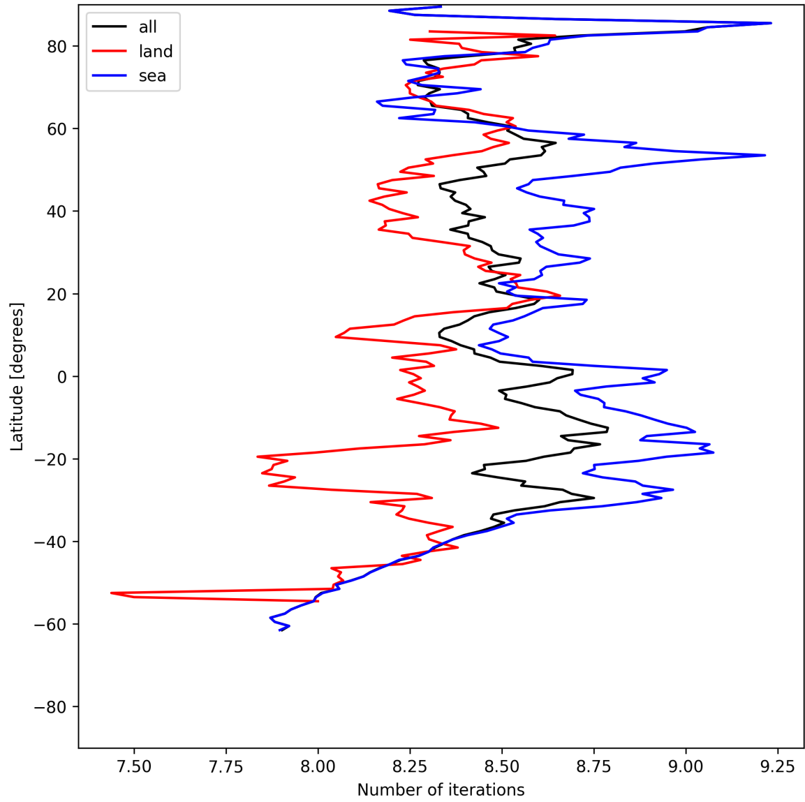
Figure 12: Zonal average of “Number of iterations” for 2025-06-08 to 2025-06-09.
