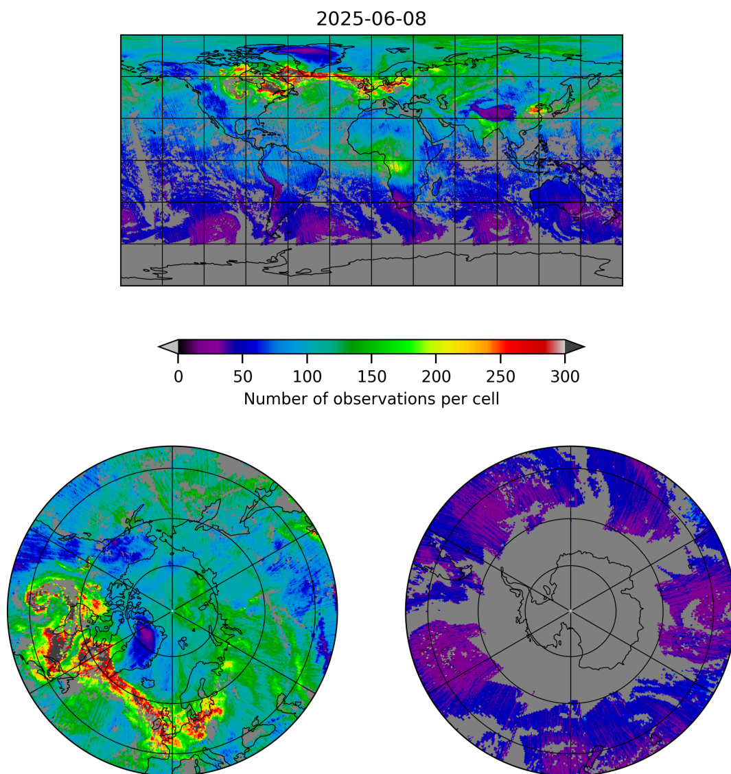
Figure 5: Map of the number of observations for 2025-06-08 to 2025-06-09
