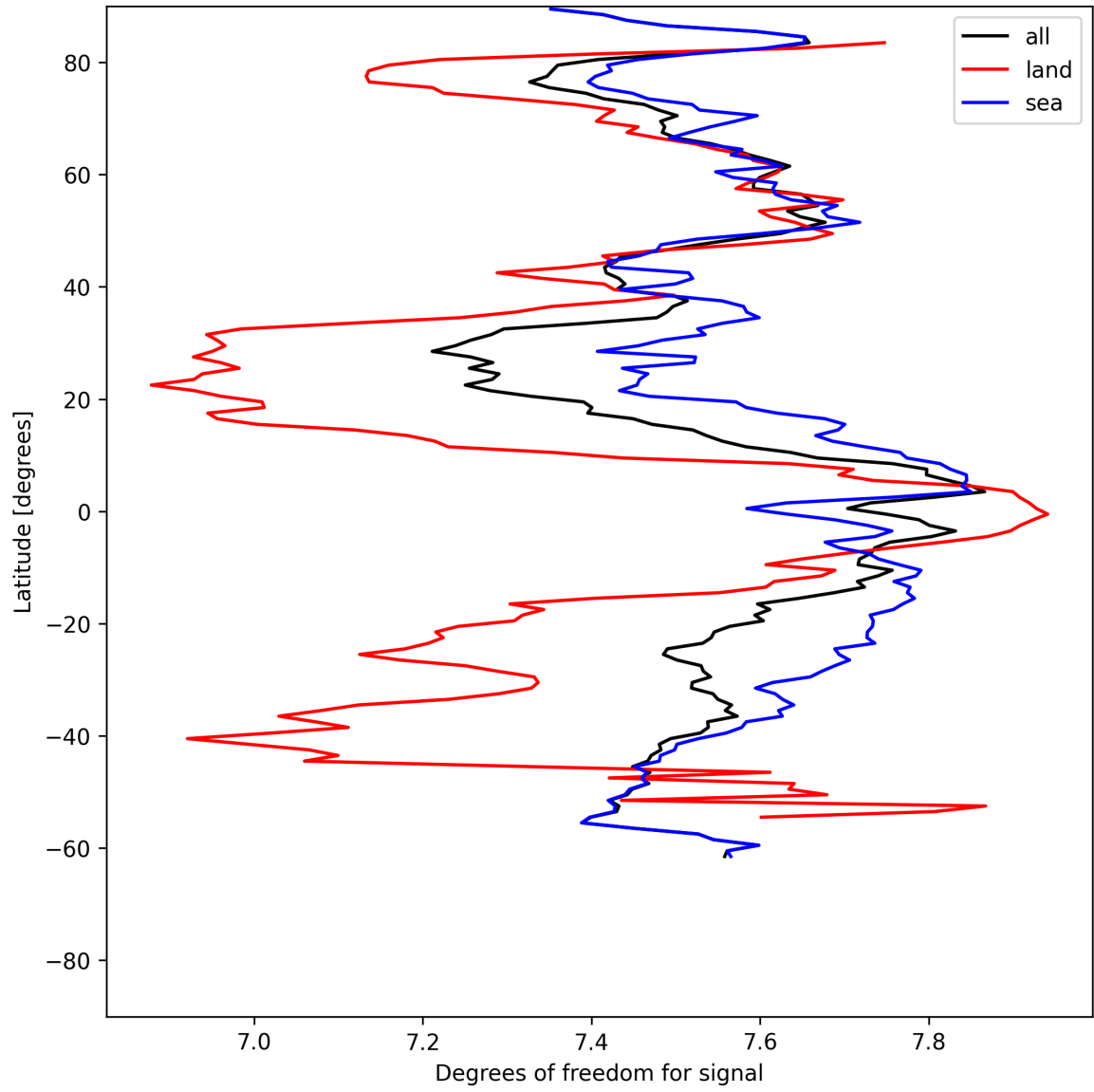
Figure 11: Zonal average of “Degrees of freedom for signal” for 2025-06-08 to 2025-06-09.
