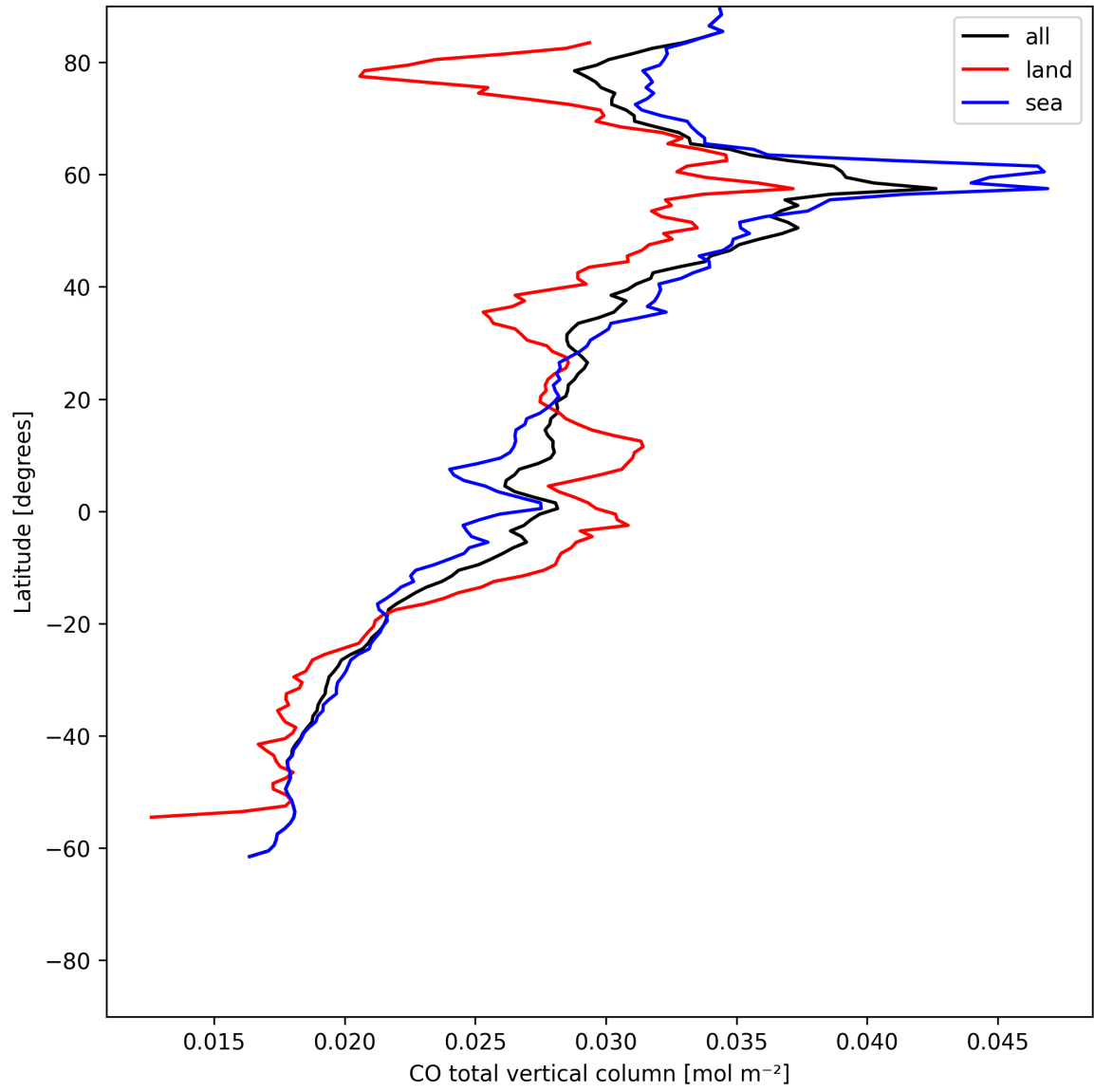
Figure 7: Zonal average of “CO total vertical column” for 2025-06-08 to 2025-06-09.
