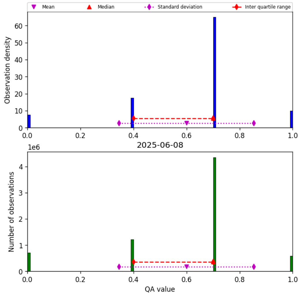
Figure 13: Histogram of “QA value” for 2025-06-08 to 2025-06-09
