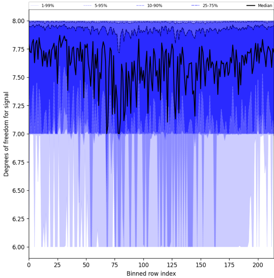
Figure 25: Along track statistics of “Degrees of freedom for signal” for 2025-06-08 to 2025-06-09
