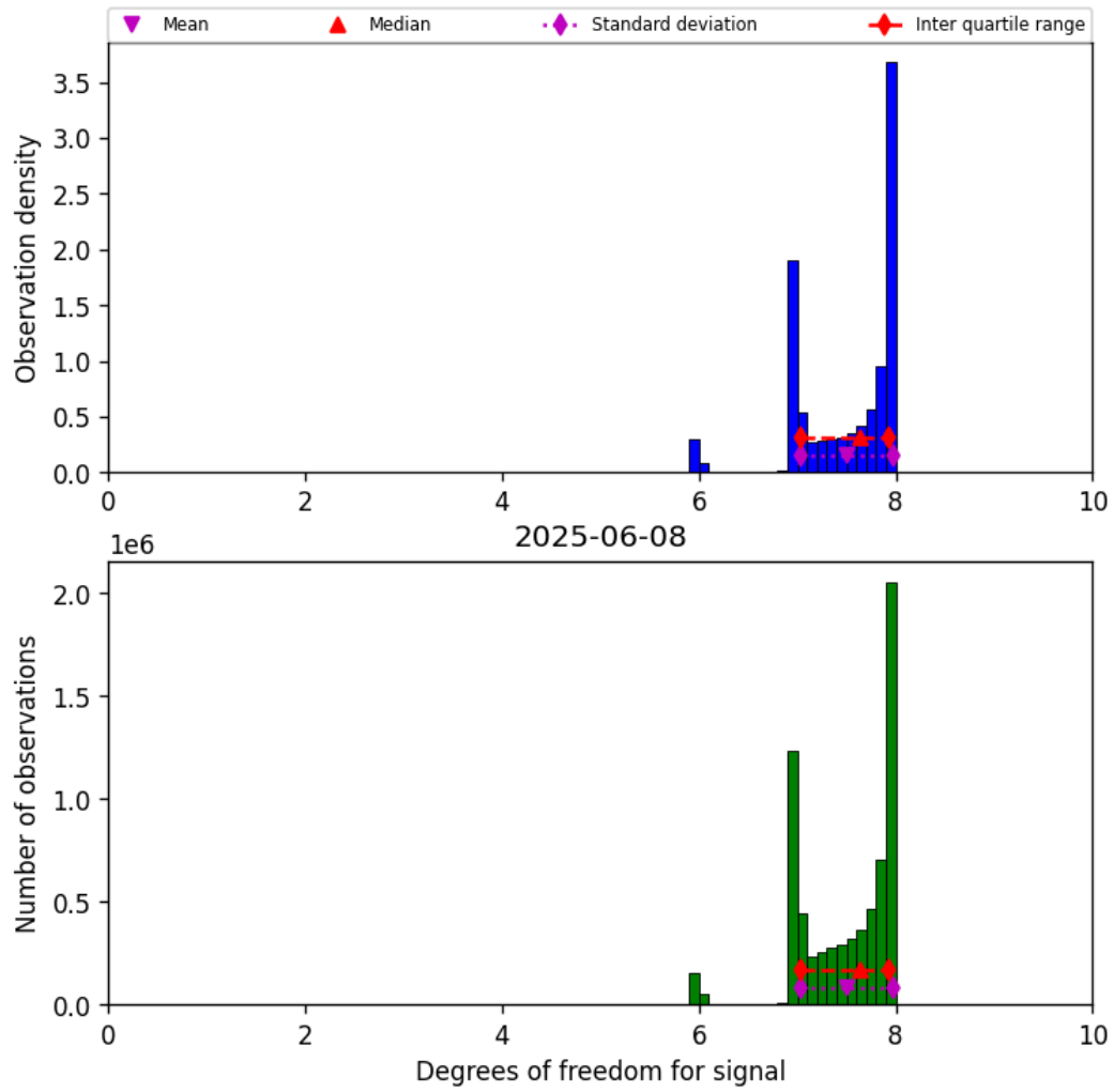
Figure 18: Histogram of “Degrees of freedom for signal” for 2025-06-08 to 2025-06-09
