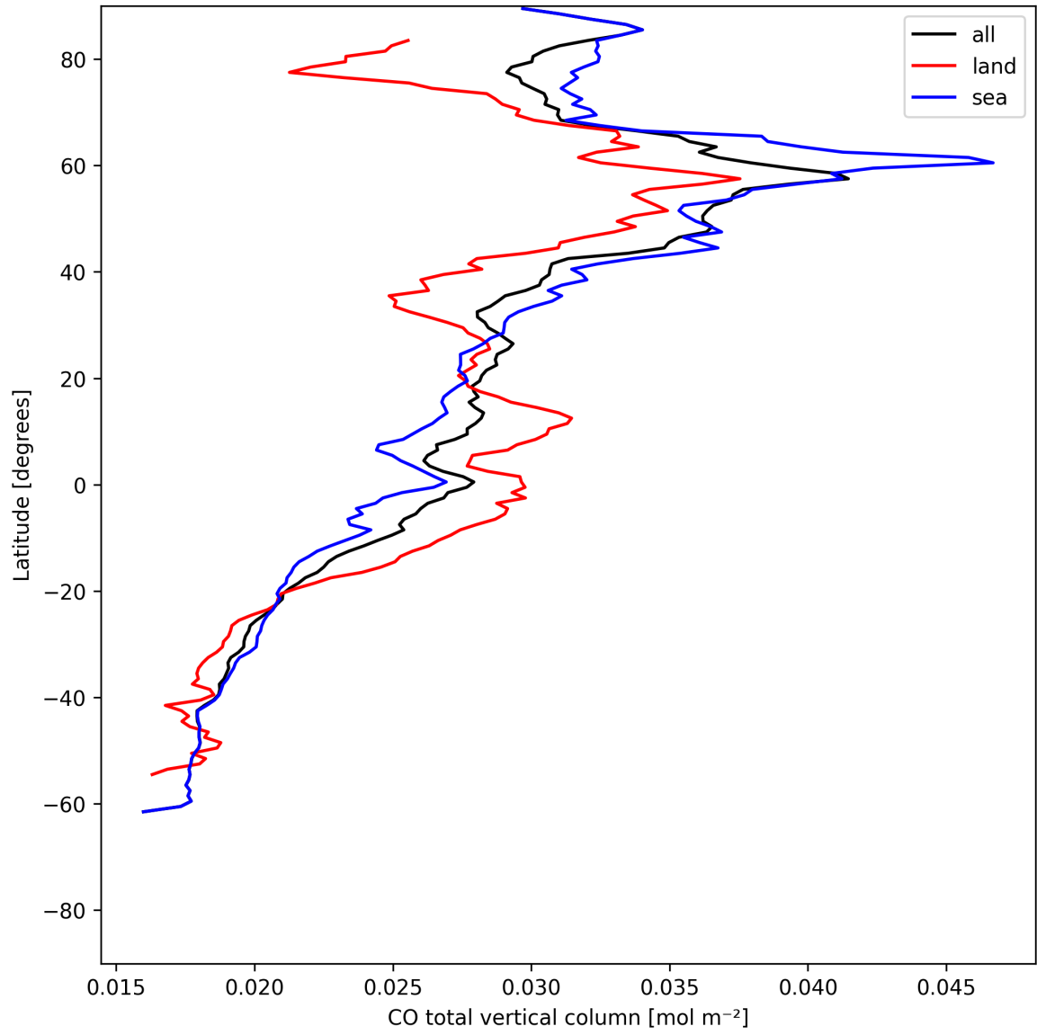
Figure 7: Zonal average of “CO total vertical column” for 2025-06-09 to 2025-06-09.
