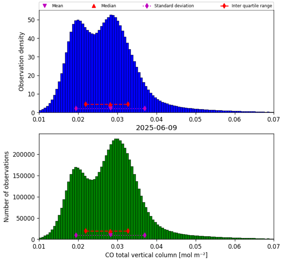
Figure 14: Histogram of “CO total vertical column” for 2025-06-09 to 2025-06-09
