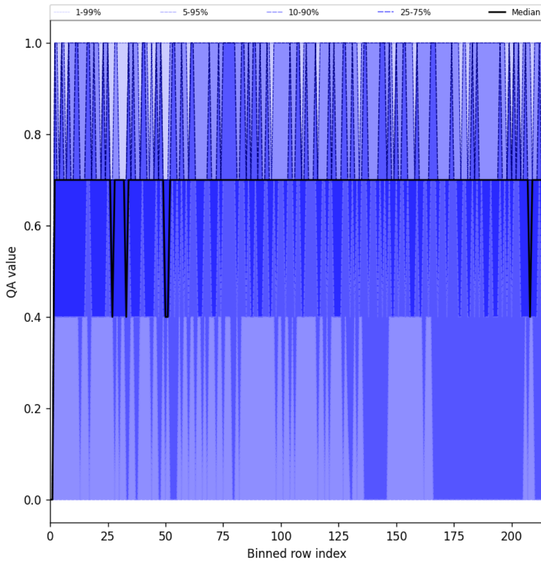
Figure 20: Along track statistics of “QA value” for 2025-06-09 to 2025-06-09
