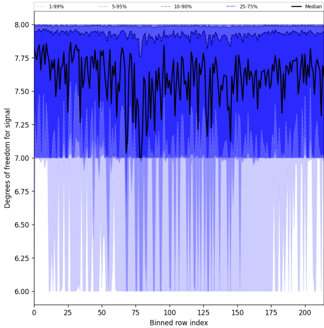
Figure 25: Along track statistics of “Degrees of freedom for signal” for 2025-06-09 to 2025-06-09
