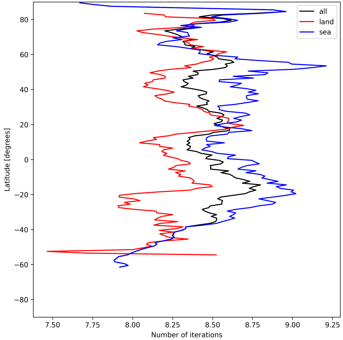
Figure 12: Zonal average of “Number of iterations” for 2025-06-09 to 2025-06-09.
