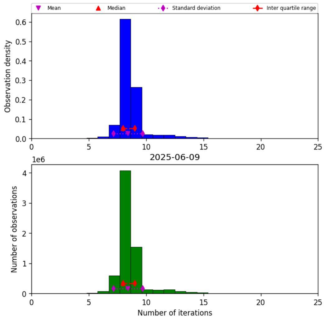
Figure 19: Histogram of “Number of iterations” for 2025-06-09 to 2025-06-09
