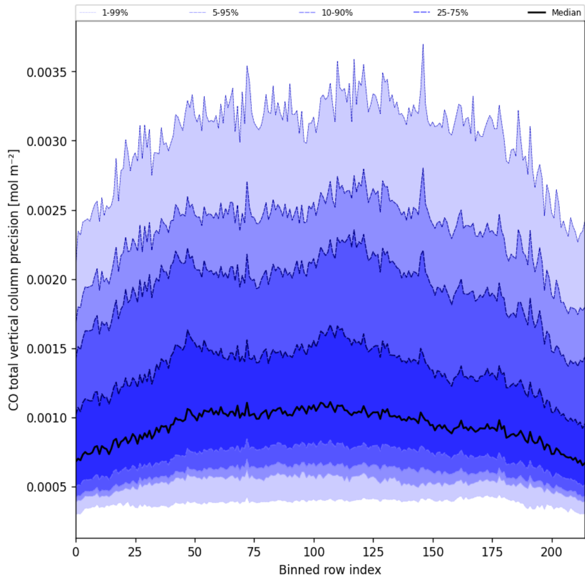
Figure 22: Along track statistics of “CO total vertical column precision” for 2025-06-09 to 2025-06-09
