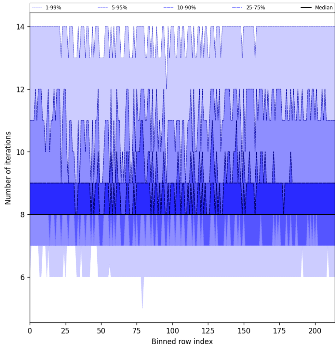
Figure 26: Along track statistics of “Number of iterations” for 2025-06-09 to 2025-06-09
