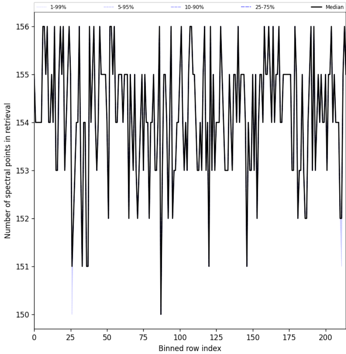
Figure 23: Along track statistics of “Number of spectral points in retrieval” for 2025-06-09 to 2025-06-09
