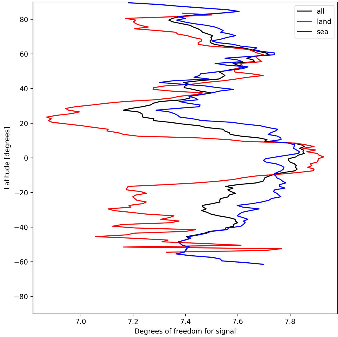
Figure 11: Zonal average of “Degrees of freedom for signal” for 2025-06-09 to 2025-06-09.
