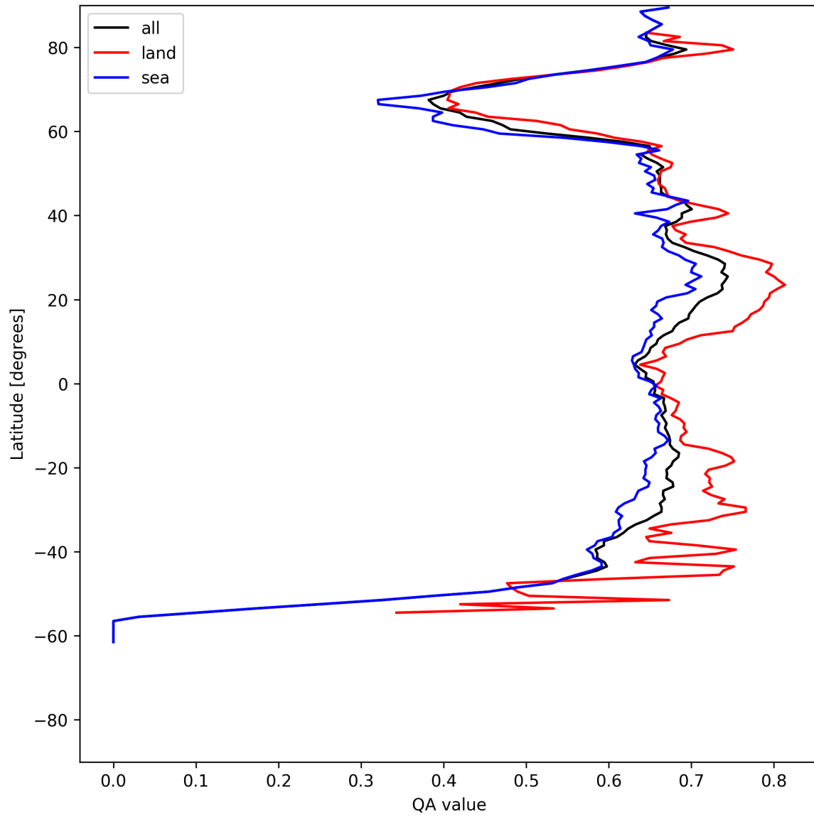
Figure 6: Zonal average of “QA value” for 2025-06-09 to 2025-06-09.
