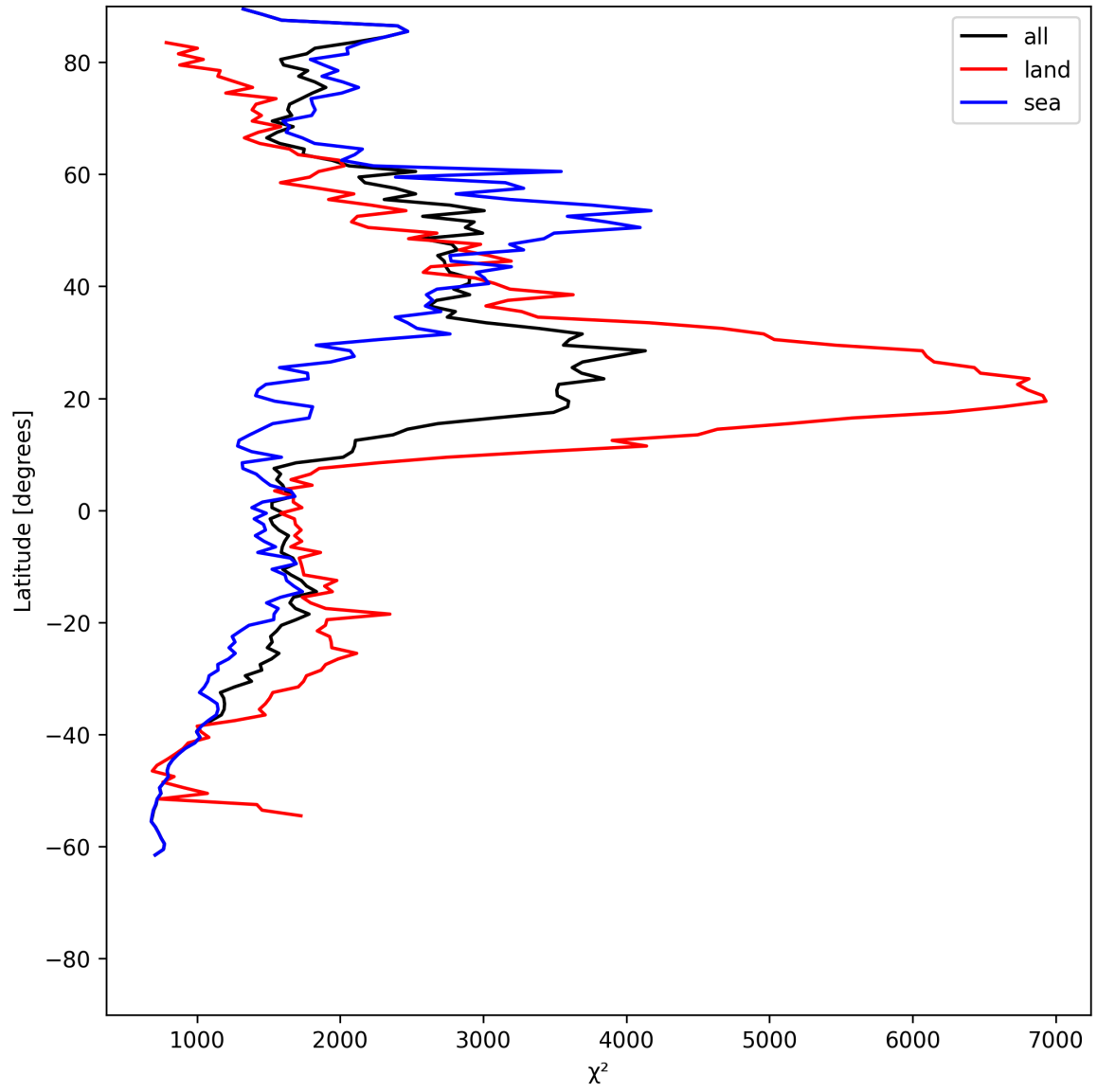
Figure 10: Zonal average of “ \chi^2 ” for 2025-06-09 to 2025-06-09.
