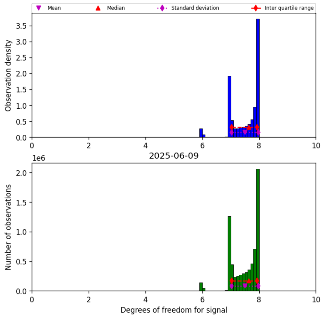
Figure 18: Histogram of “Degrees of freedom for signal” for 2025-06-09 to 2025-06-09
