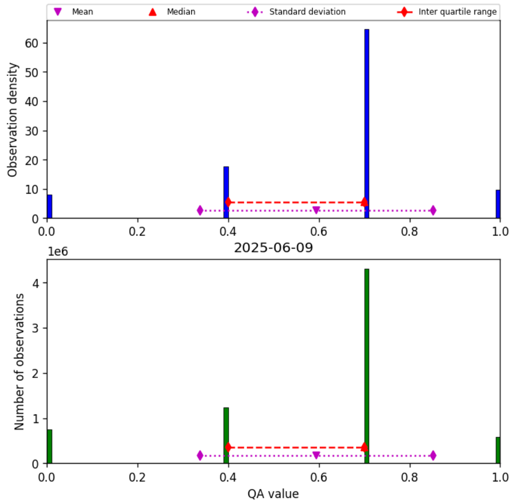
Figure 13: Histogram of “QA value” for 2025-06-09 to 2025-06-09
