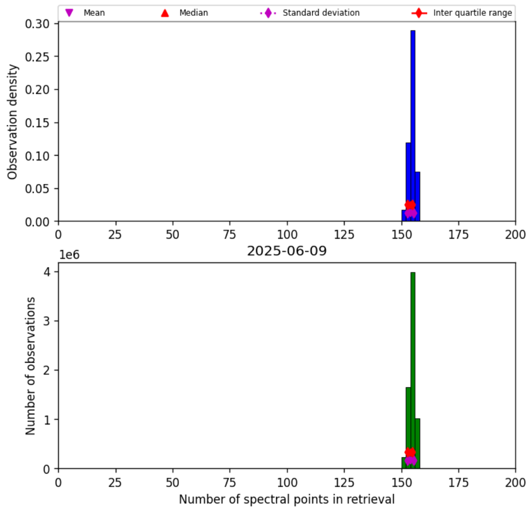
Figure 16: Histogram of “Number of spectral points in retrieval” for 2025-06-09 to 2025-06-09
