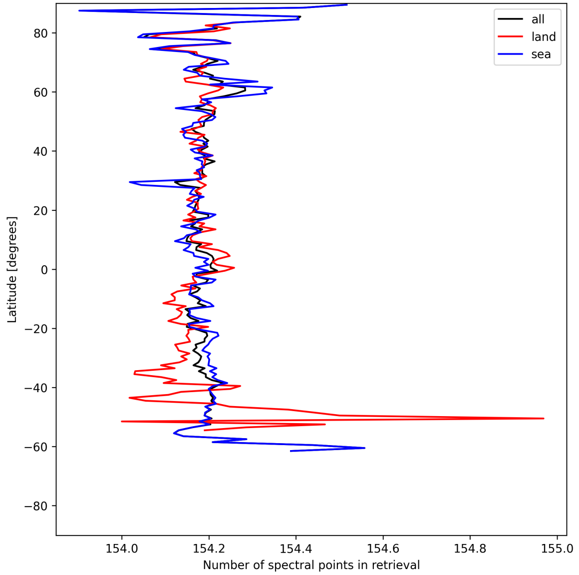
Figure 9: Zonal average of “Number of spectral points in retrieval” for 2025-06-09 to 2025-06-09.
