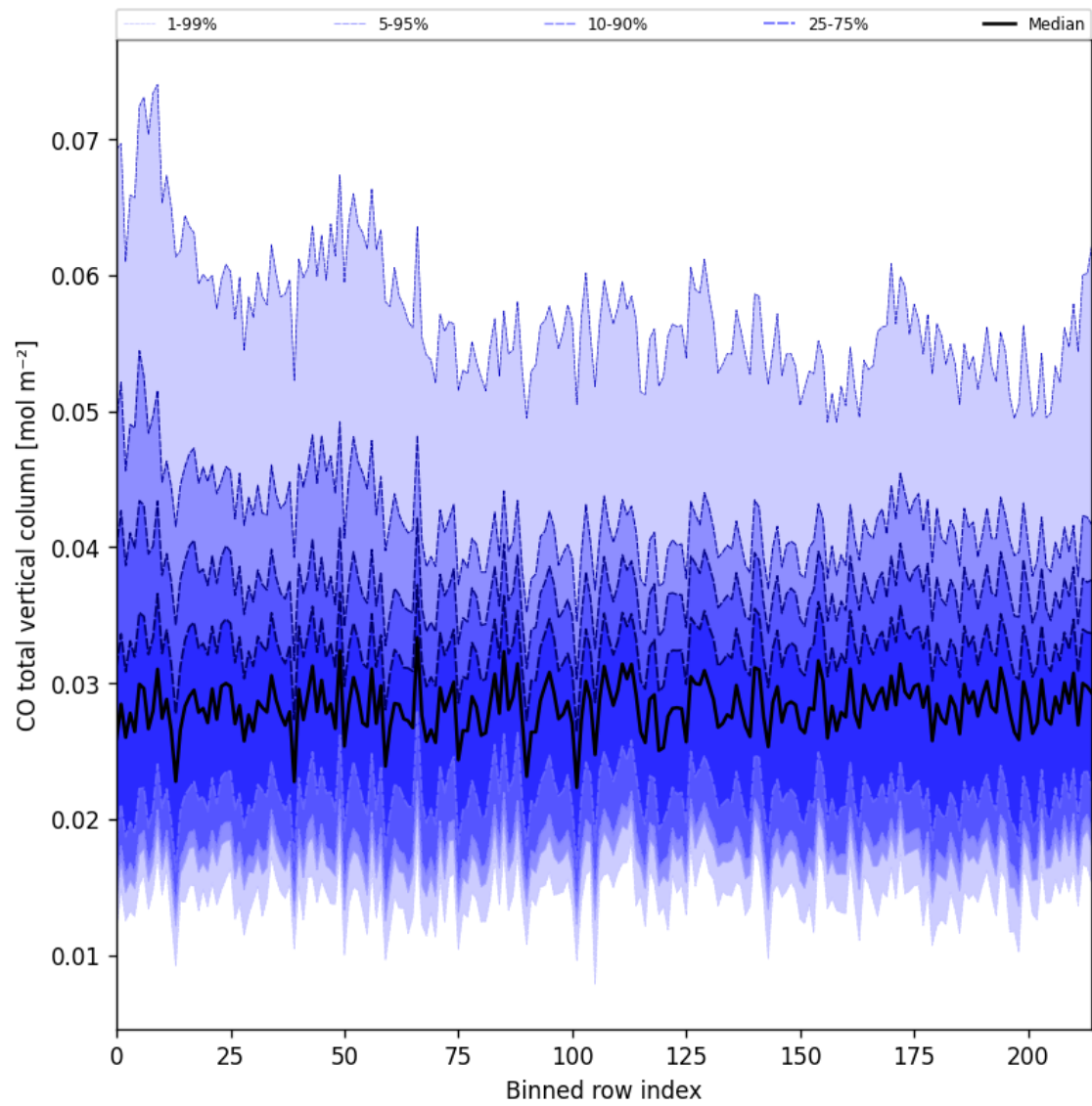
Figure 21: Along track statistics of “CO total vertical column” for 2025-06-09 to 2025-06-09
