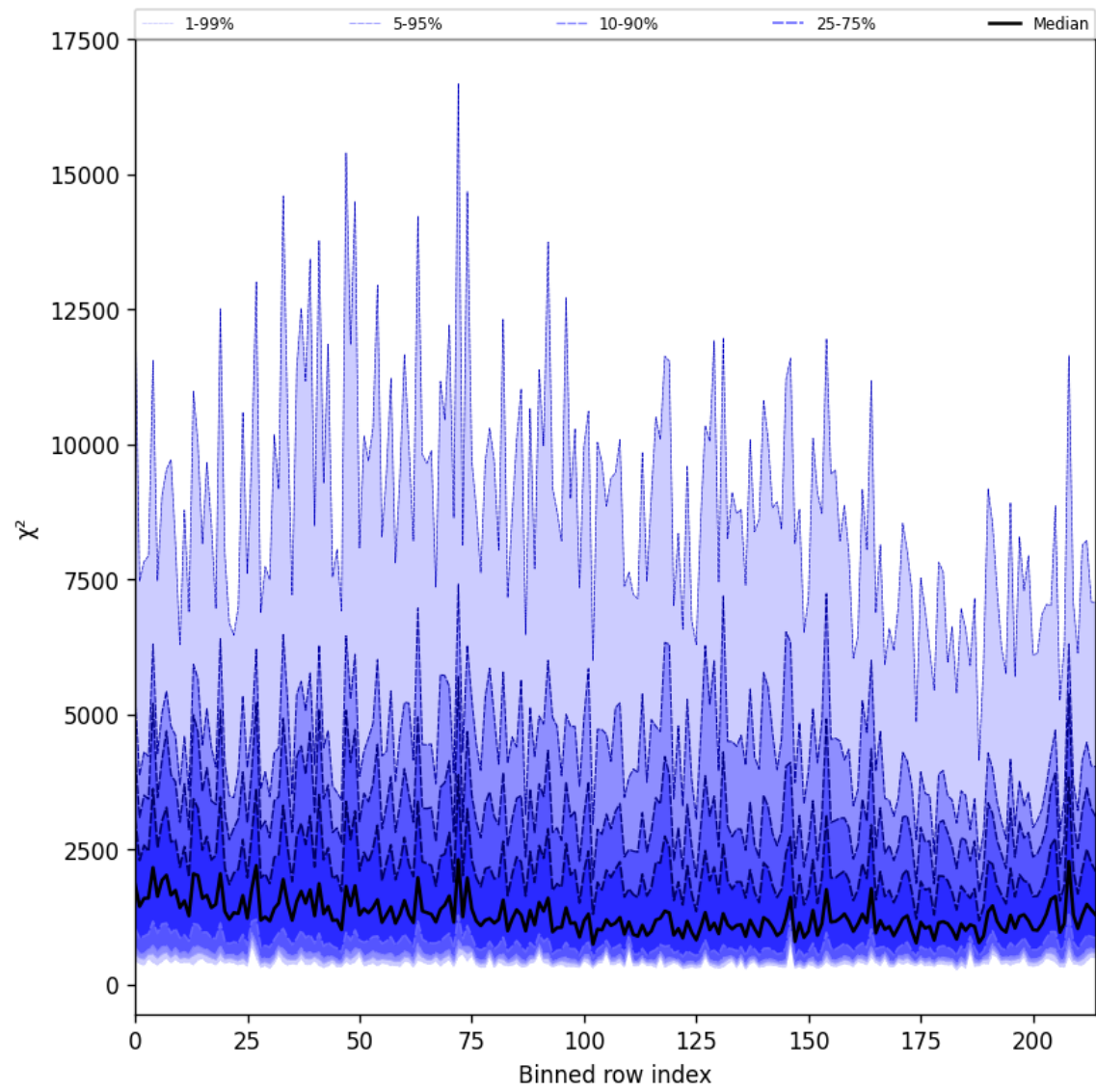
Figure 24: Along track statistics of “ \chi^2 ” for 2025-06-09 to 2025-06-09
