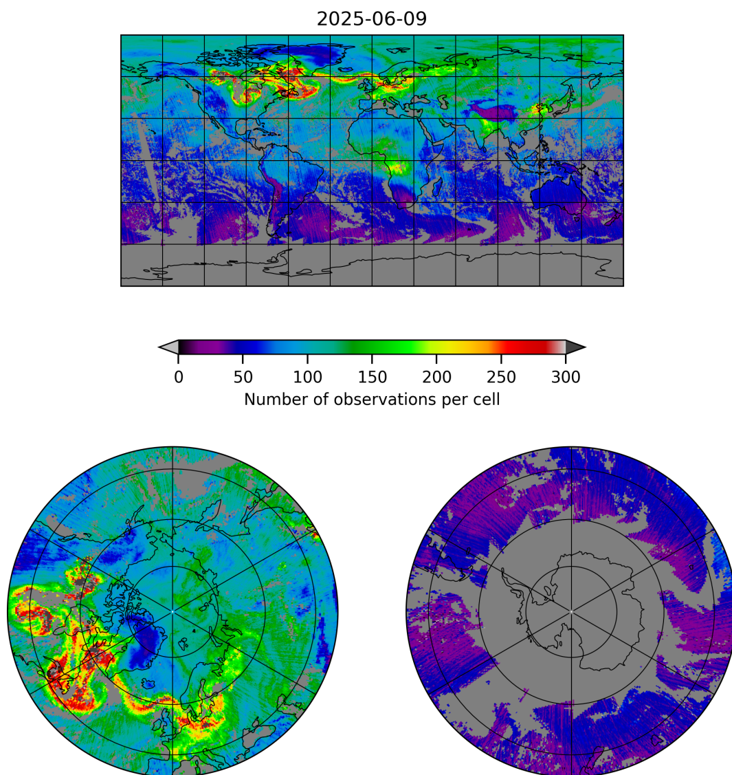
Figure 5: Map of the number of observations for 2025-06-09 to 2025-06-09
