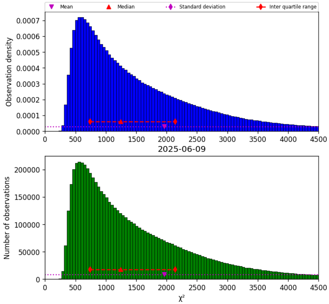
Figure 17: Histogram of “ \chi^2 ” for 2025-06-09 to 2025-06-09
