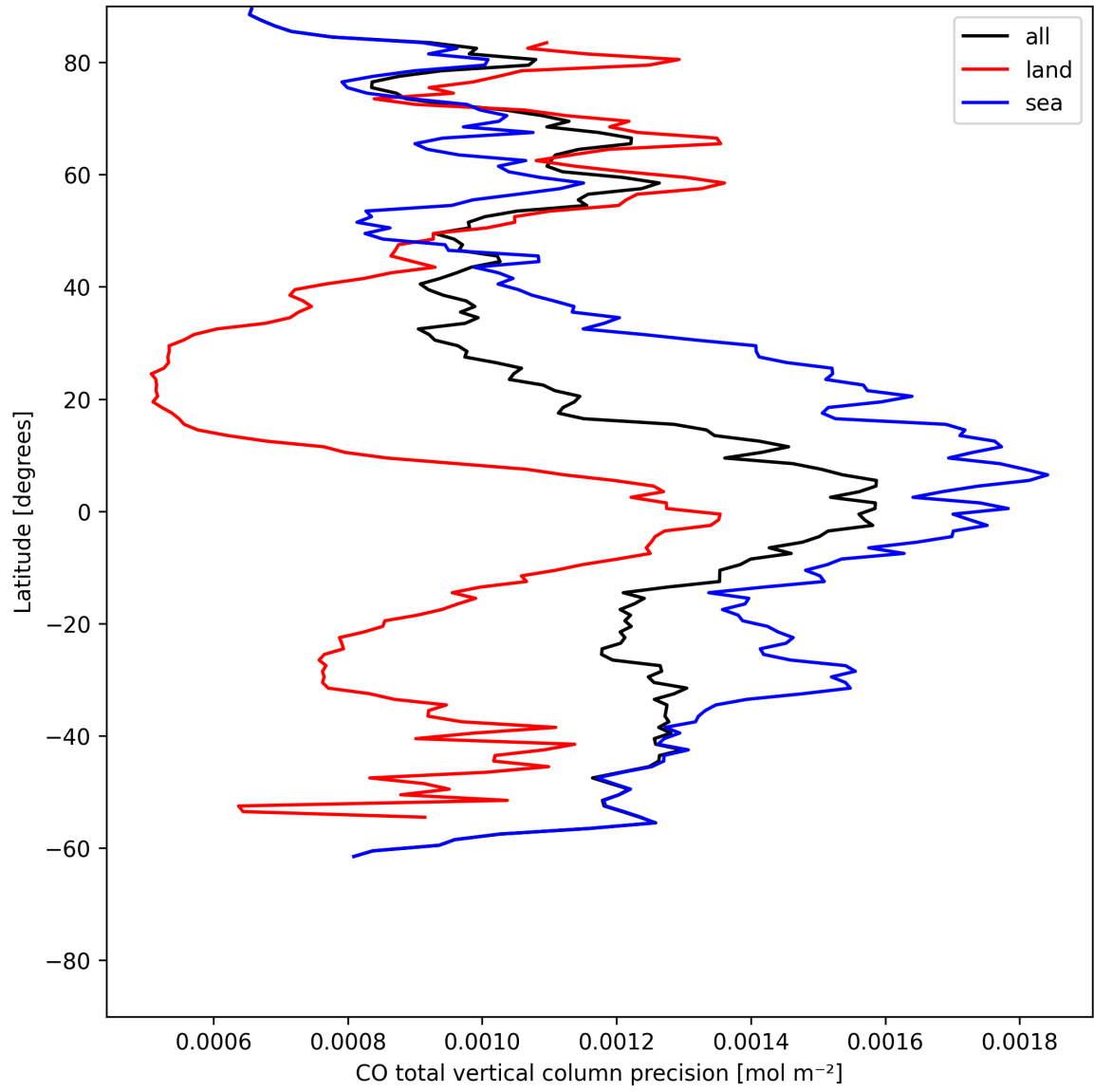
Figure 8: Zonal average of “CO total vertical column precision” for 2025-06-09 to 2025-06-09.
