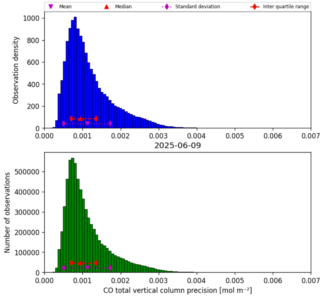
Figure 15: Histogram of “CO total vertical column precision” for 2025-06-09 to 2025-06-09
