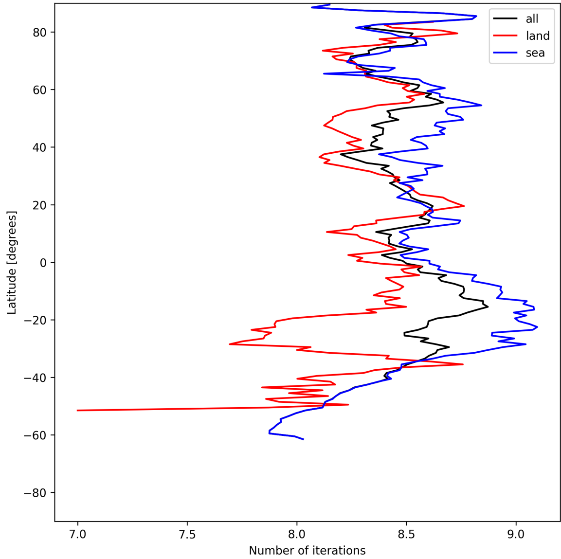
Figure 12: Zonal average of “Number of iterations” for 2025-06-11 to 2025-06-12.
