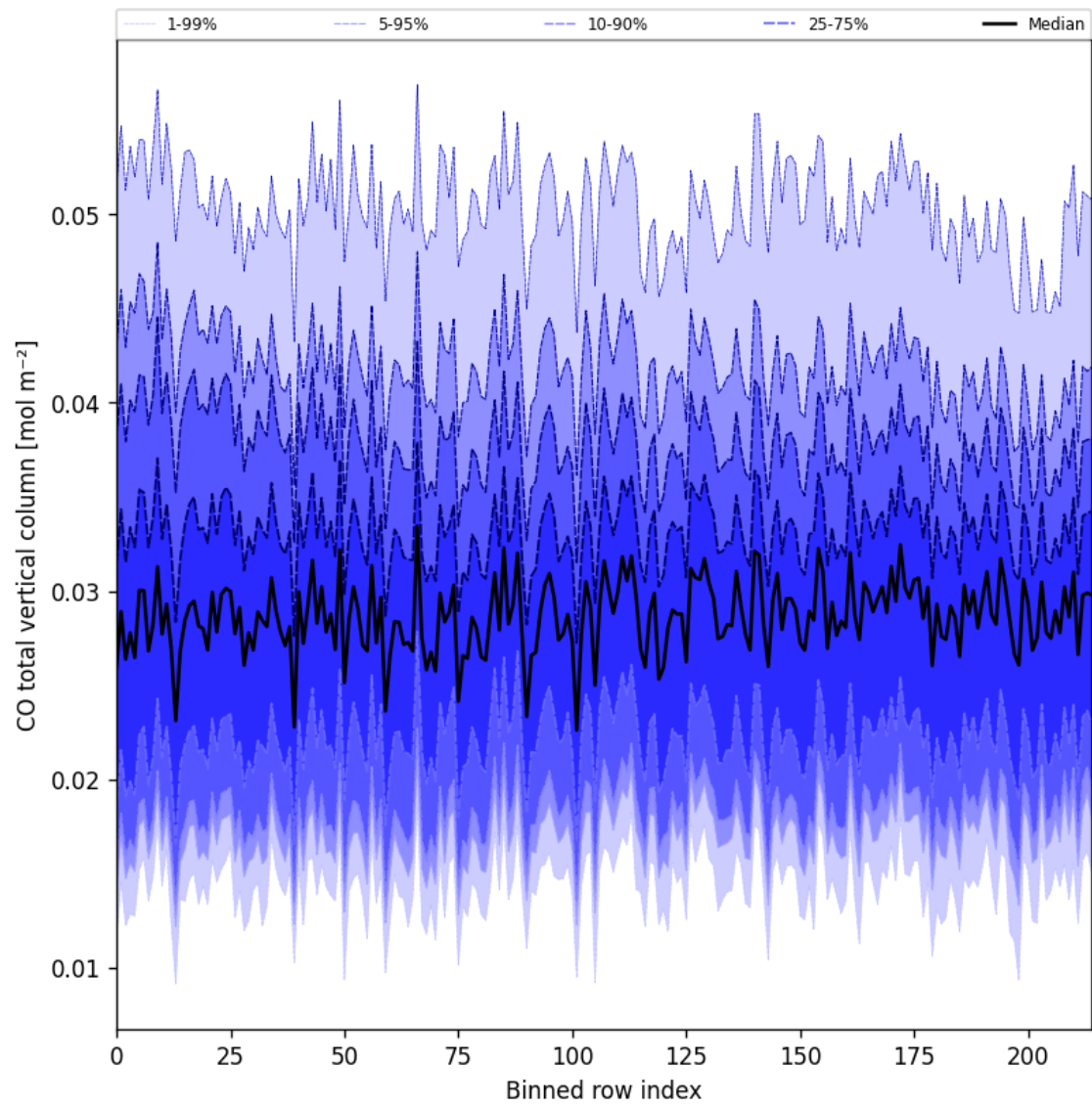
Figure 21: Along track statistics of “CO total vertical column” for 2025-06-11 to 2025-06-12
