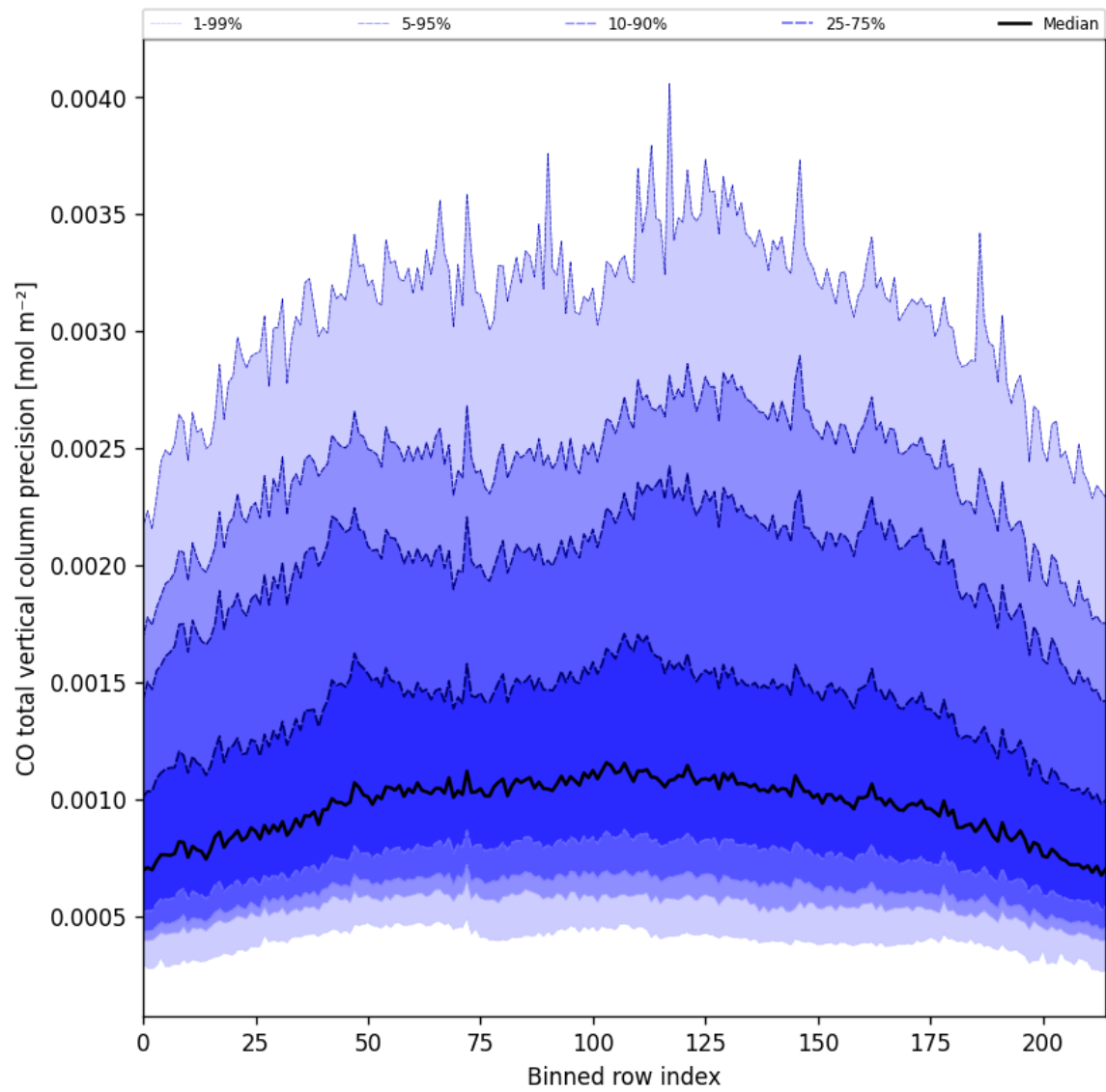
Figure 22: Along track statistics of “CO total vertical column precision” for 2025-06-11 to 2025-06-12
