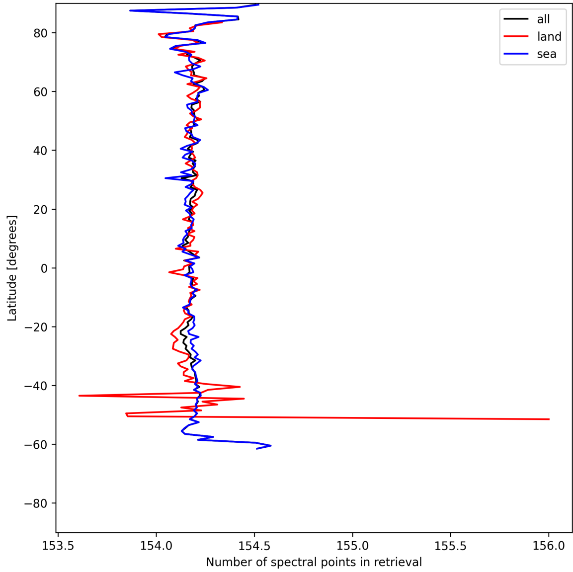
Figure 9: Zonal average of “Number of spectral points in retrieval” for 2025-06-11 to 2025-06-12.
