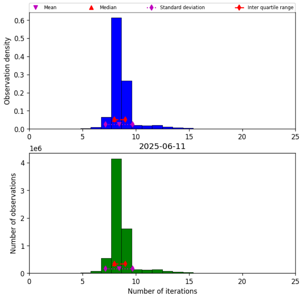
Figure 19: Histogram of “Number of iterations” for 2025-06-11 to 2025-06-12
