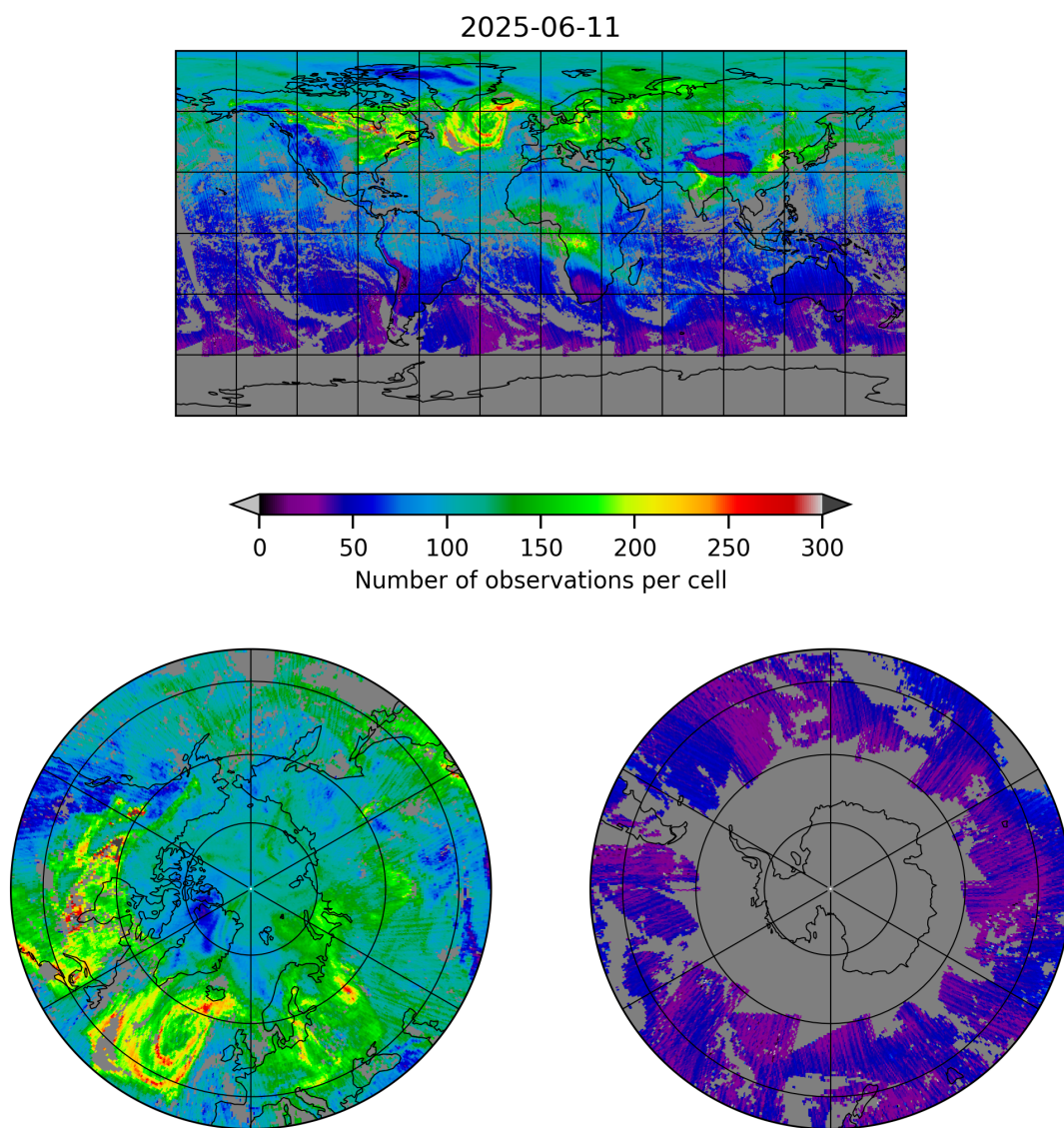
Figure 5: Map of the number of observations for 2025-06-11 to 2025-06-12
