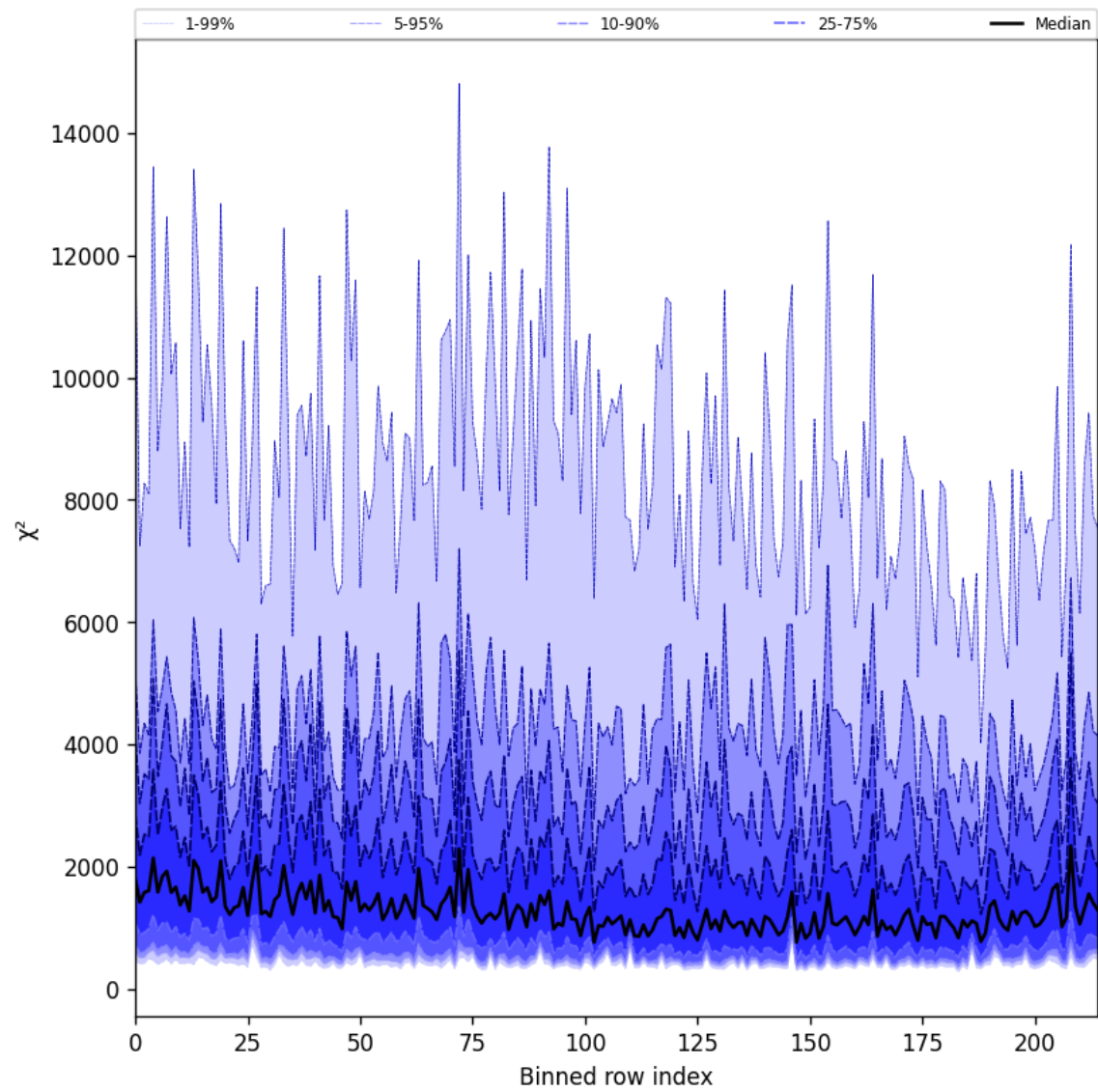
Figure 24: Along track statistics of “ \chi^2 ” for 2025-06-11 to 2025-06-12
