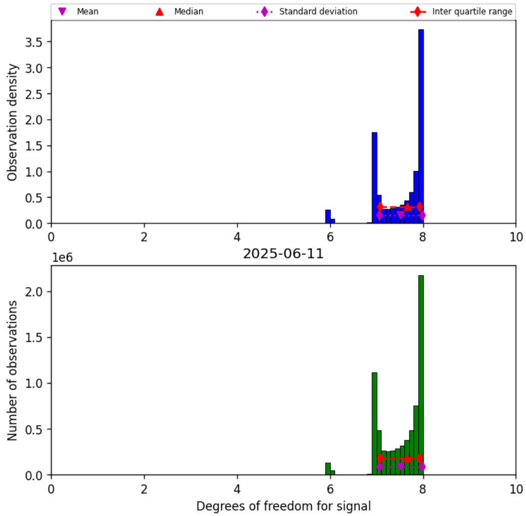
Figure 18: Histogram of “Degrees of freedom for signal” for 2025-06-11 to 2025-06-12
