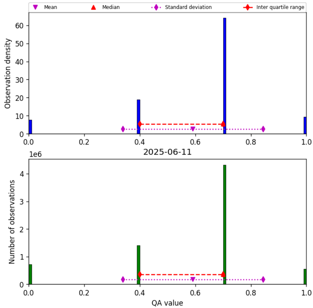
Figure 13: Histogram of “QA value” for 2025-06-11 to 2025-06-12
