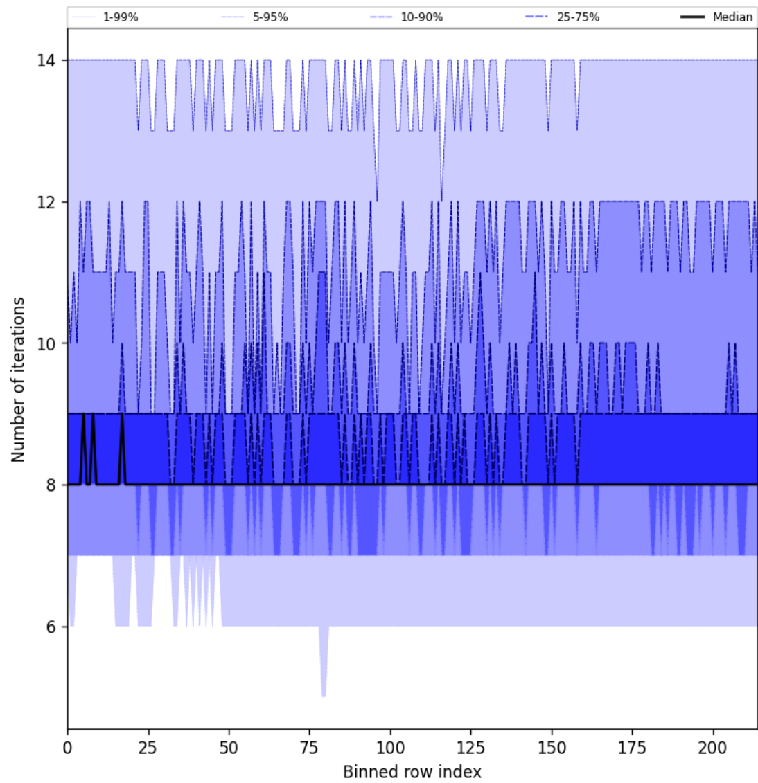
Figure 26: Along track statistics of “Number of iterations” for 2025-06-11 to 2025-06-12
