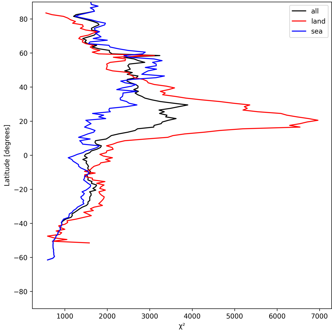
Figure 10: Zonal average of “ \chi^2 ” for 2025-06-11 to 2025-06-12.
