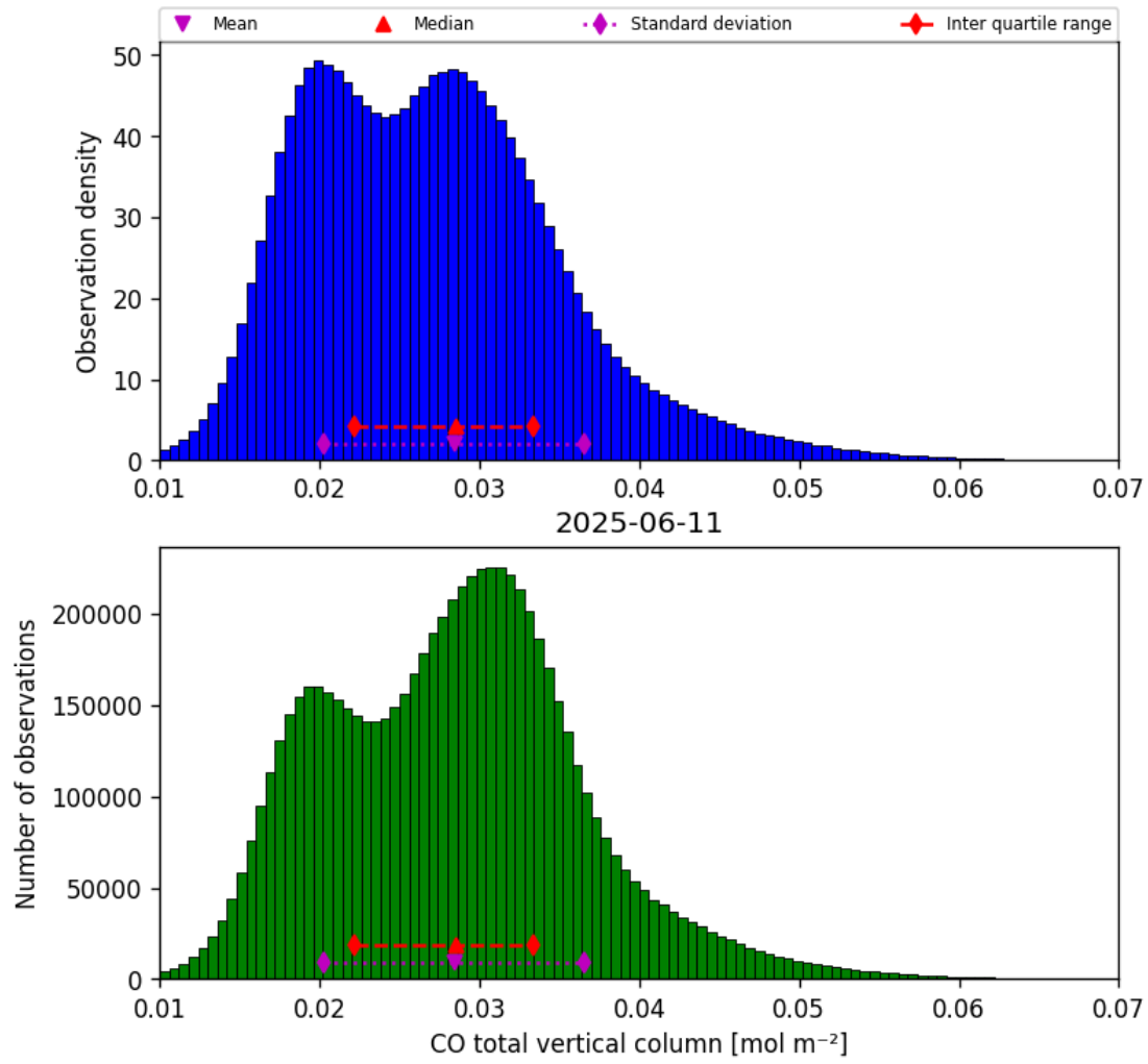
Figure 14: Histogram of “CO total vertical column” for 2025-06-11 to 2025-06-12
