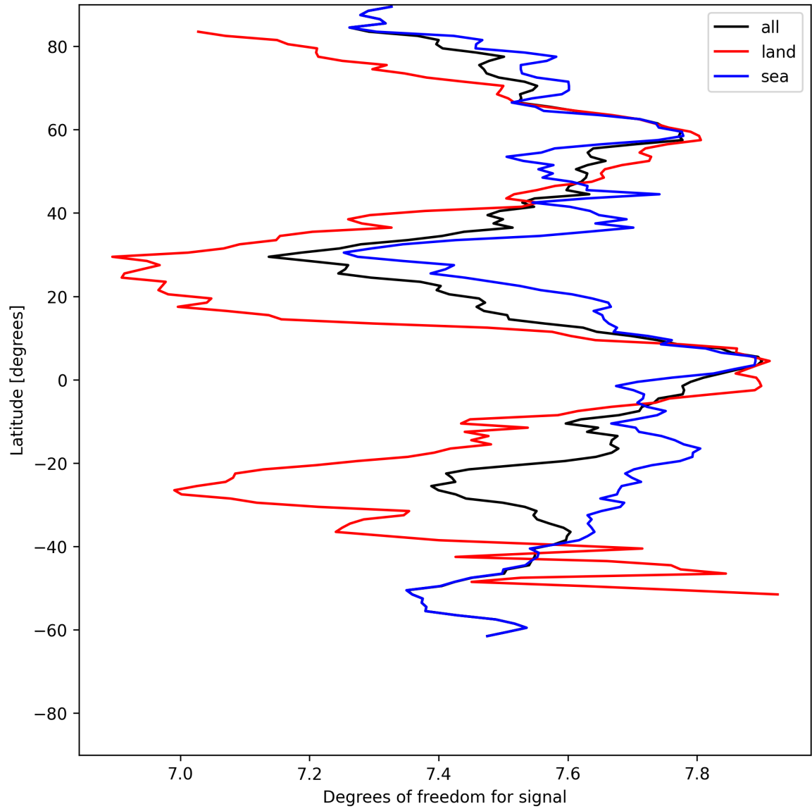
Figure 11: Zonal average of “Degrees of freedom for signal” for 2025-06-11 to 2025-06-12.
