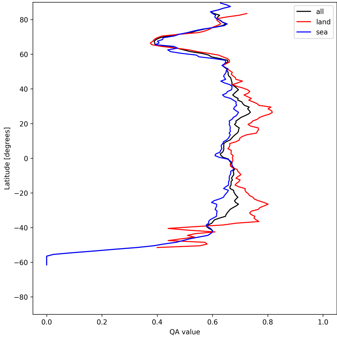
Figure 6: Zonal average of “QA value” for 2025-06-11 to 2025-06-12.
