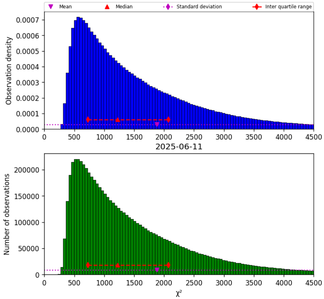
Figure 17: Histogram of “ \chi^2 ” for 2025-06-11 to 2025-06-12
