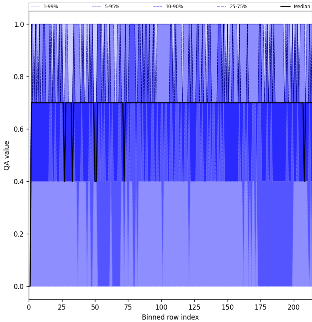
Figure 20: Along track statistics of “QA value” for 2025-06-11 to 2025-06-12
