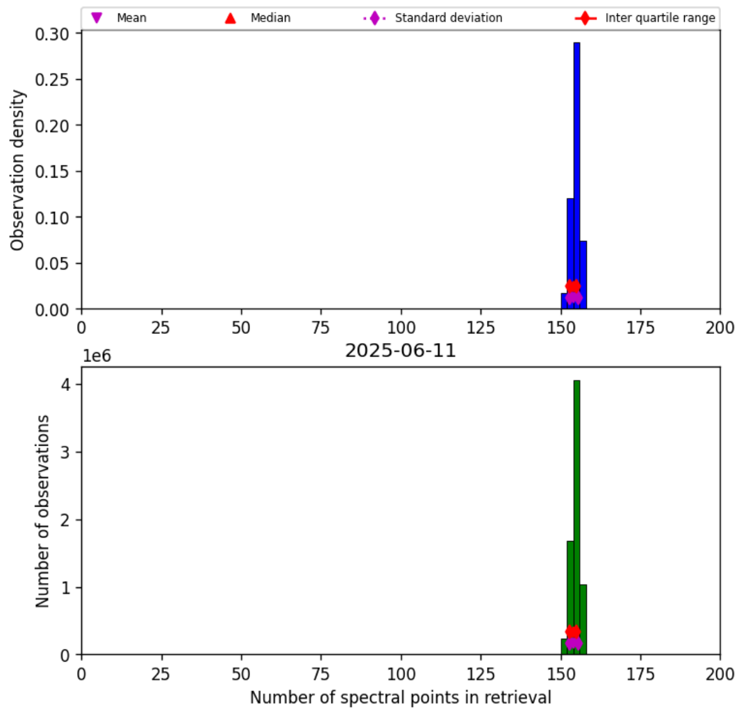
Figure 16: Histogram of “Number of spectral points in retrieval” for 2025-06-11 to 2025-06-12
