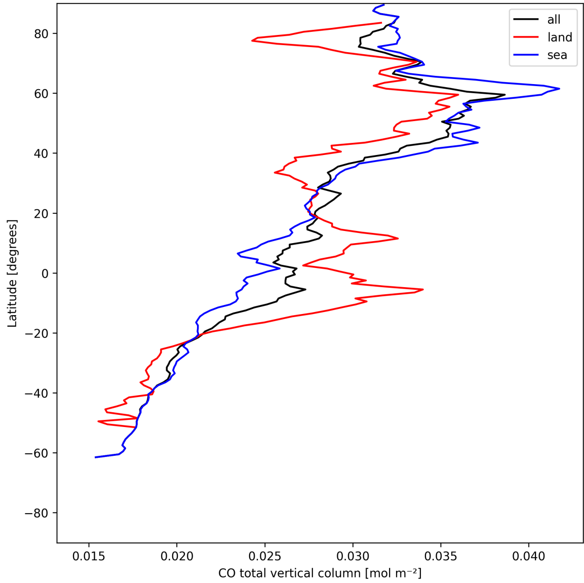
Figure 7: Zonal average of “CO total vertical column” for 2025-06-11 to 2025-06-12.
