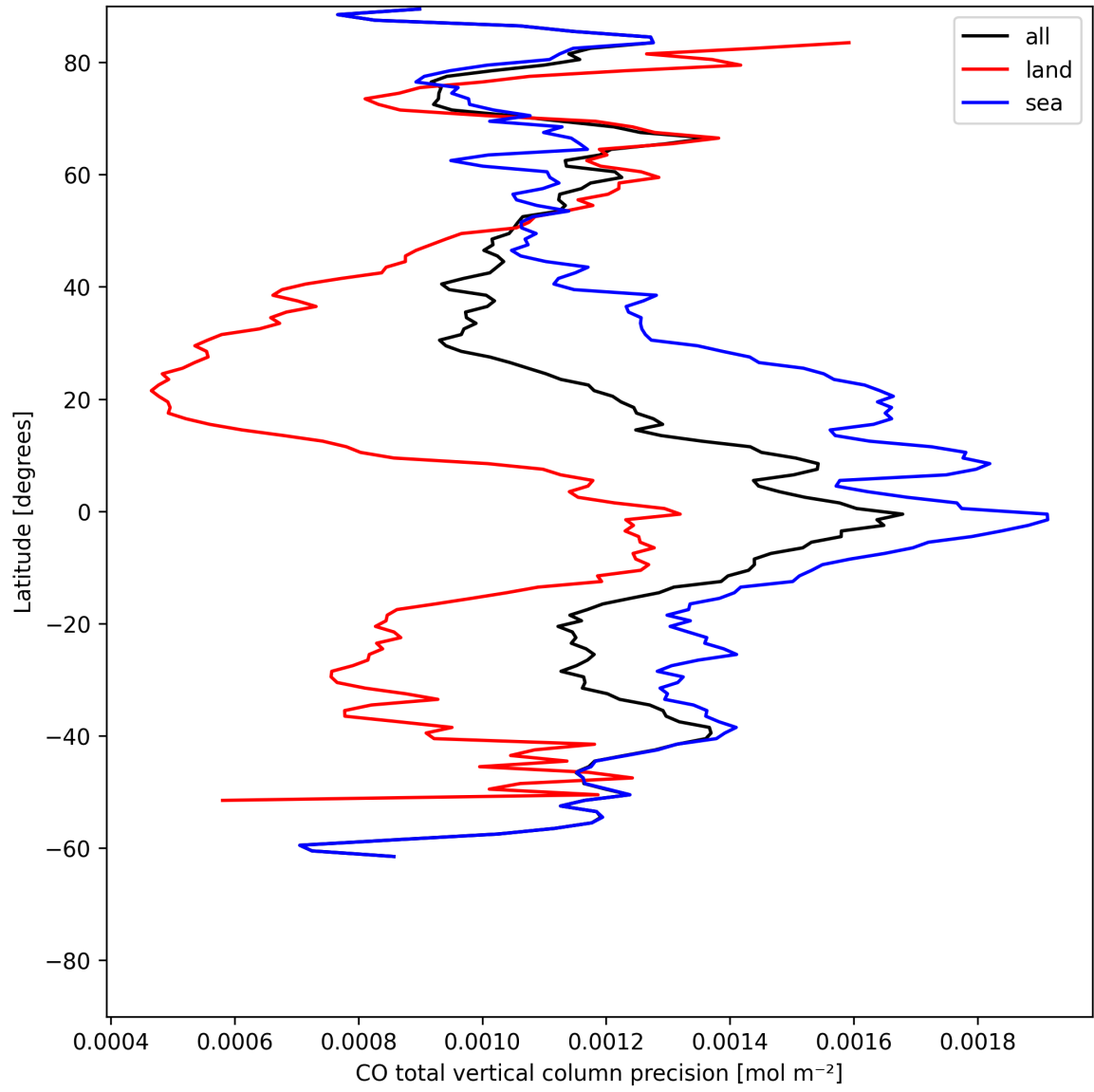
Figure 8: Zonal average of “CO total vertical column precision” for 2025-06-11 to 2025-06-12.
