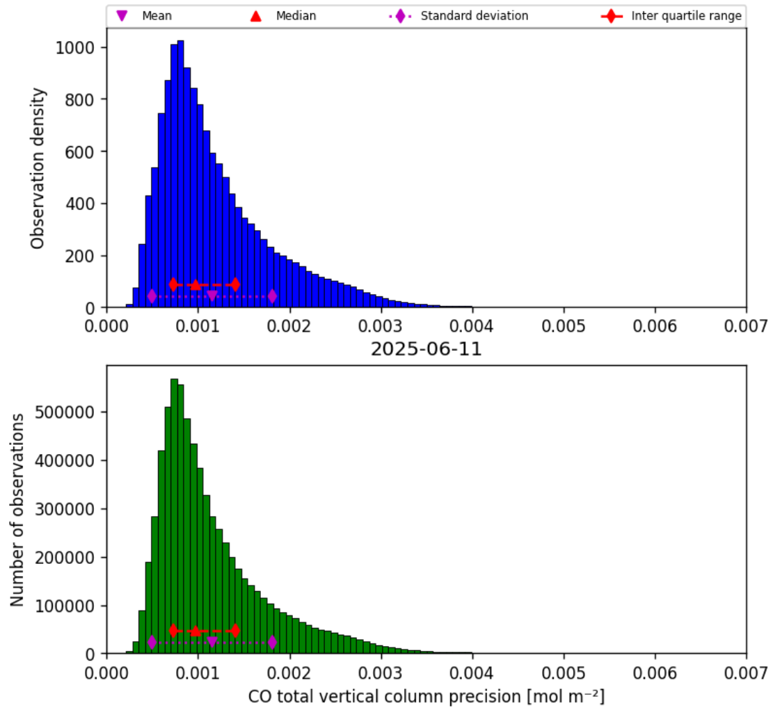
Figure 15: Histogram of “CO total vertical column precision” for 2025-06-11 to 2025-06-12
