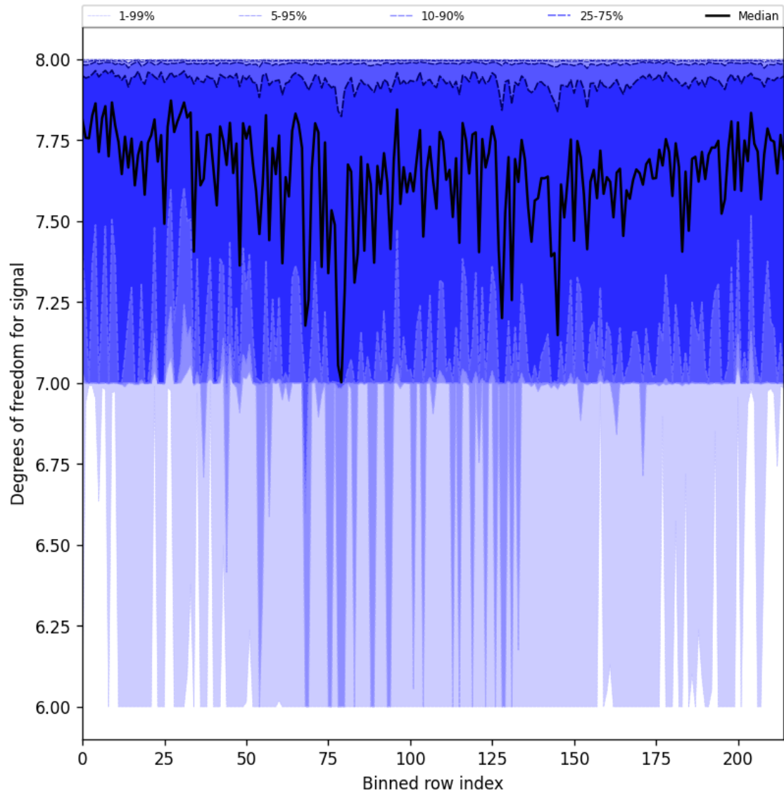
Figure 25: Along track statistics of “Degrees of freedom for signal” for 2025-06-11 to 2025-06-12
