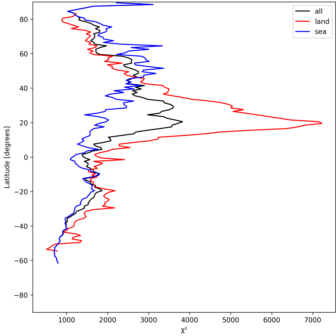
Figure 10: Zonal average of “ \chi^2 ” for 2025-06-12 to 2025-06-13.
