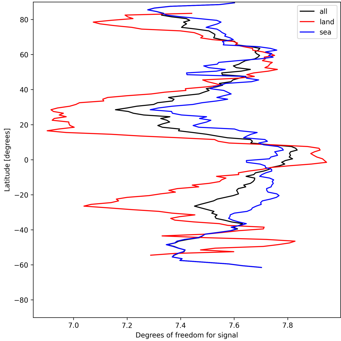
Figure 11: Zonal average of “Degrees of freedom for signal” for 2025-06-12 to 2025-06-13.
