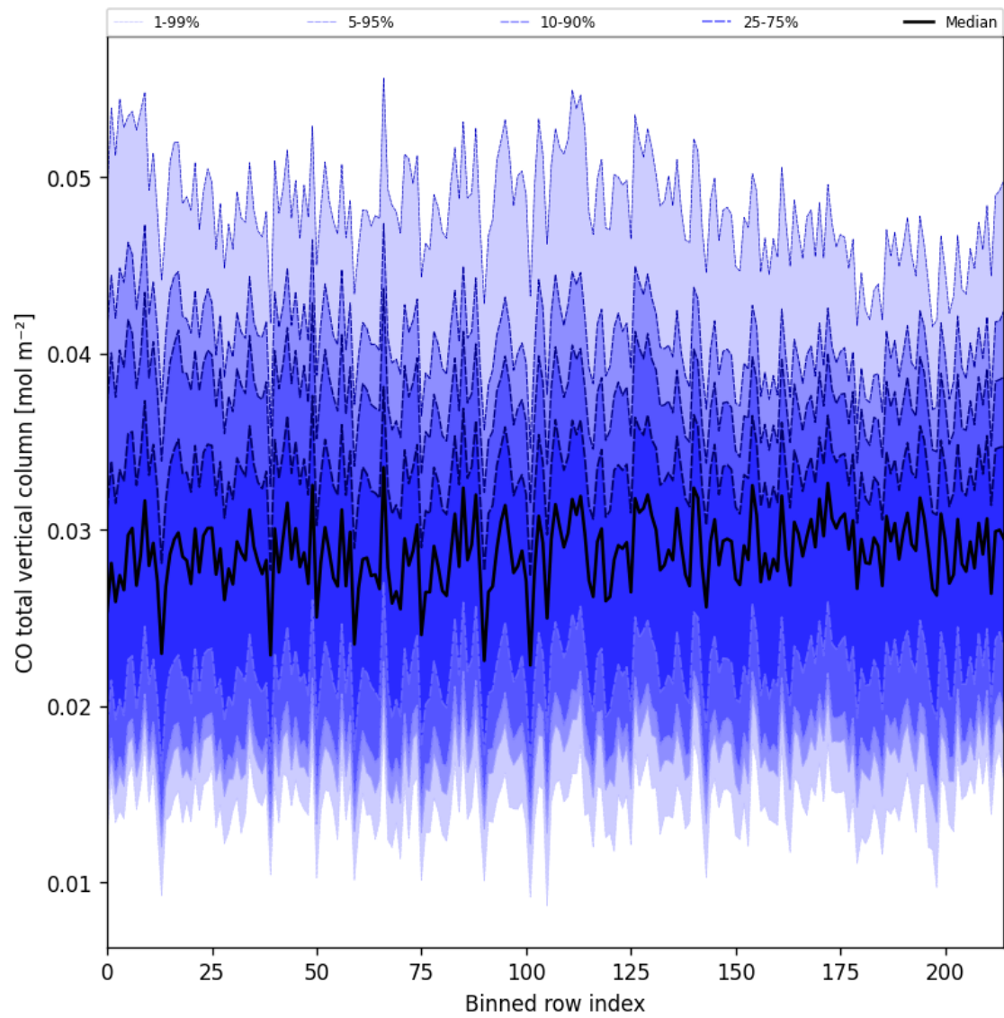
Figure 21: Along track statistics of “CO total vertical column” for 2025-06-12 to 2025-06-13
