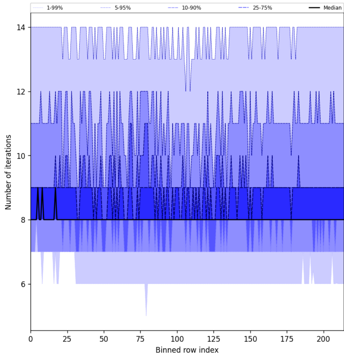
Figure 26: Along track statistics of “Number of iterations” for 2025-06-12 to 2025-06-13
