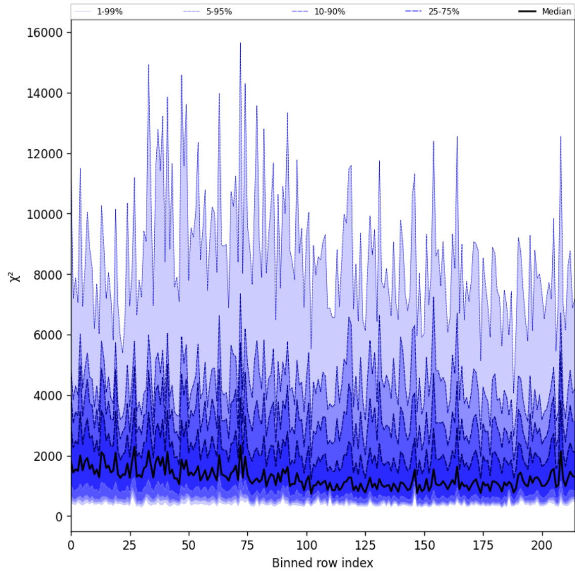
Figure 24: Along track statistics of “ \chi^2 ” for 2025-06-12 to 2025-06-13
