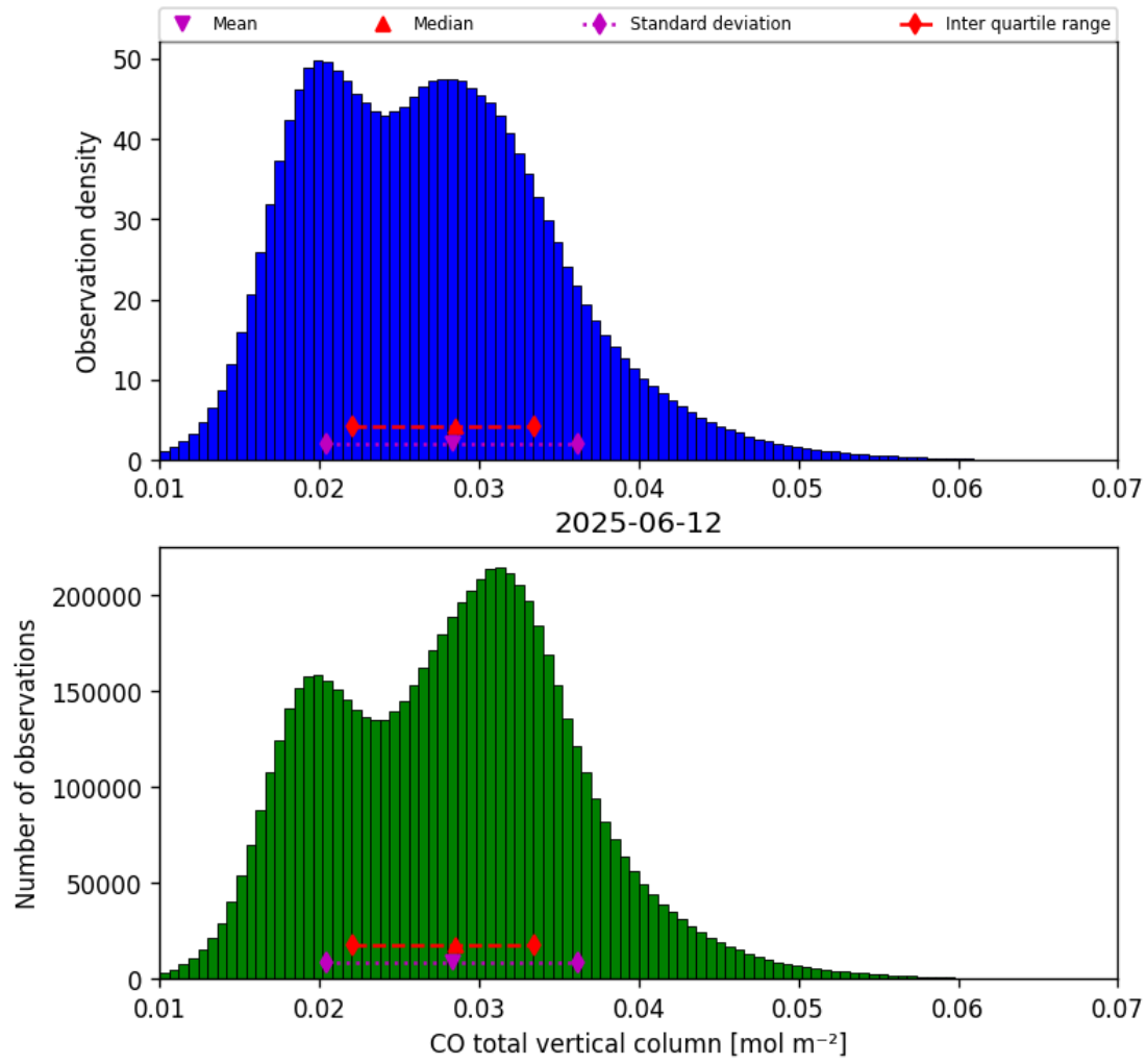
Figure 14: Histogram of “CO total vertical column” for 2025-06-12 to 2025-06-13
