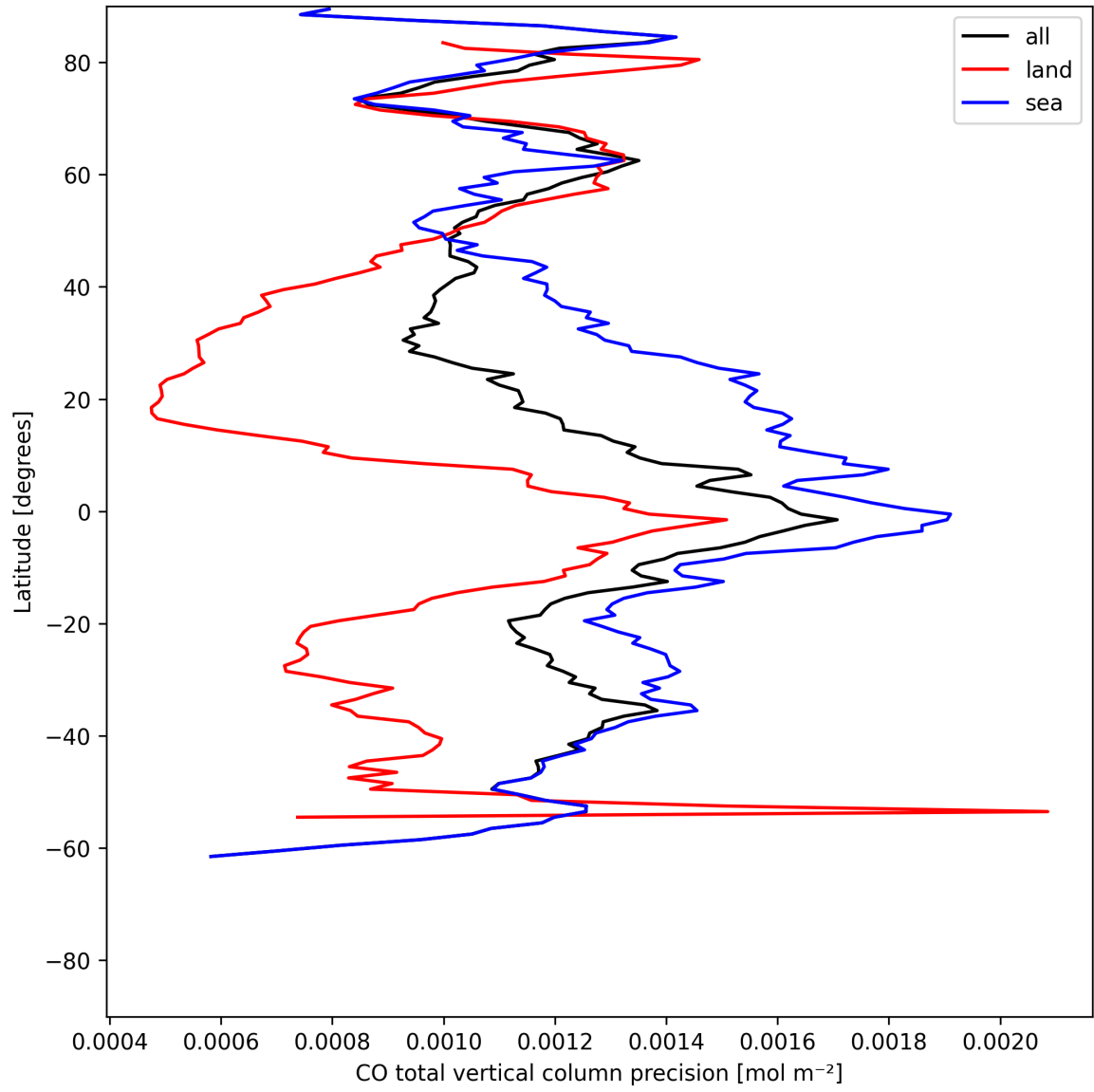
Figure 8: Zonal average of “CO total vertical column precision” for 2025-06-12 to 2025-06-13.
