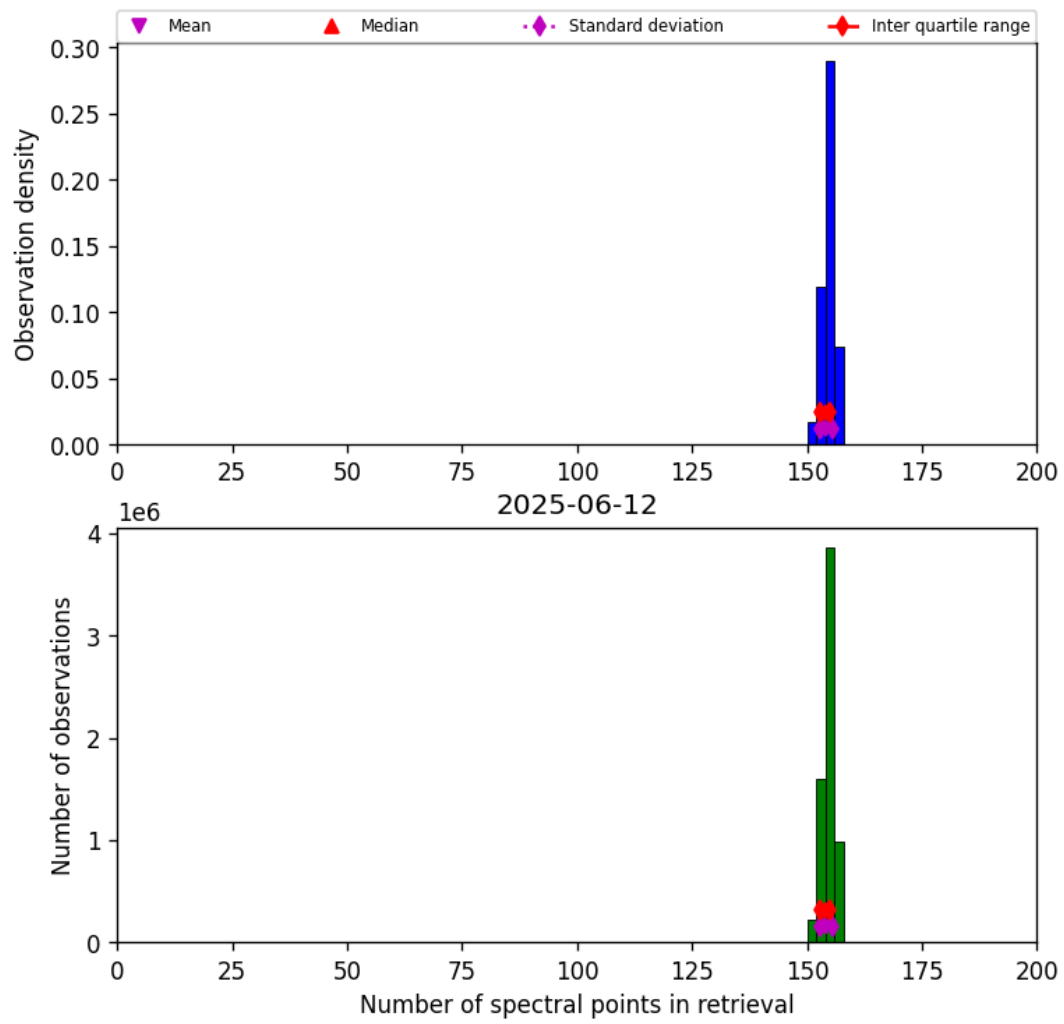
Figure 16: Histogram of “Number of spectral points in retrieval” for 2025-06-12 to 2025-06-13
