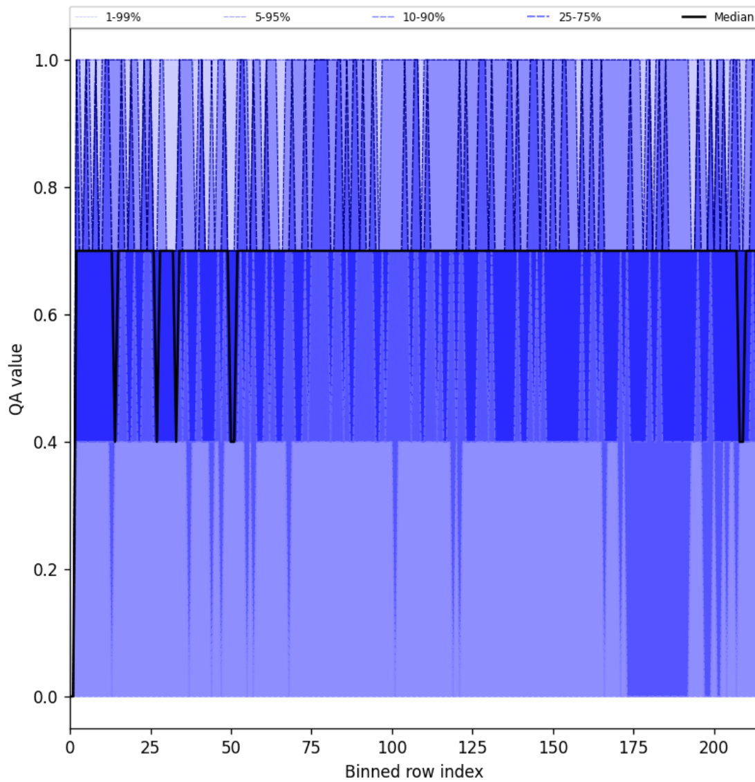
Figure 20: Along track statistics of “QA value” for 2025-06-12 to 2025-06-13
