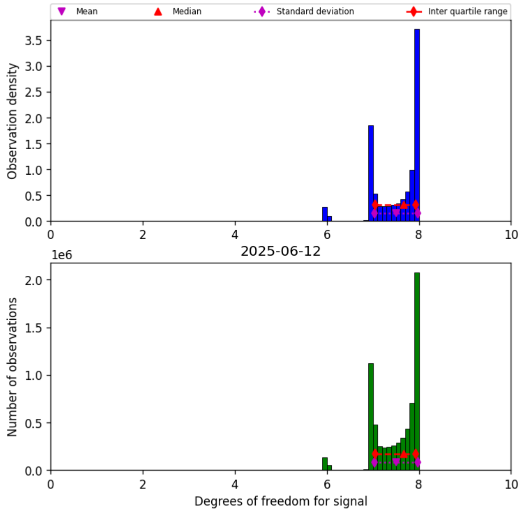
Figure 18: Histogram of “Degrees of freedom for signal” for 2025-06-12 to 2025-06-13
