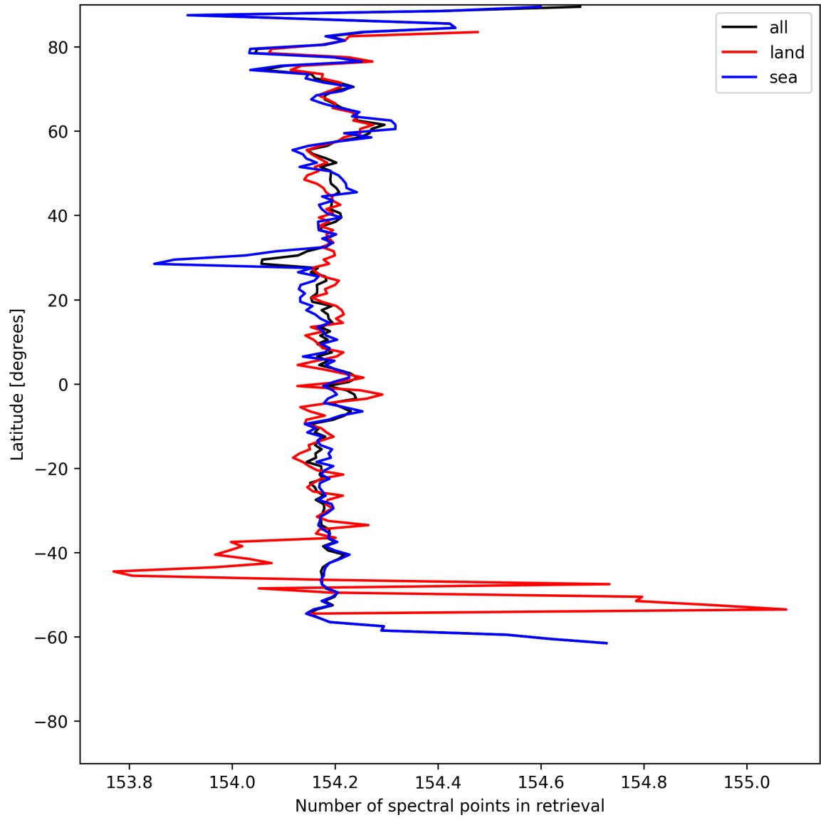
Figure 9: Zonal average of “Number of spectral points in retrieval” for 2025-06-12 to 2025-06-13.
