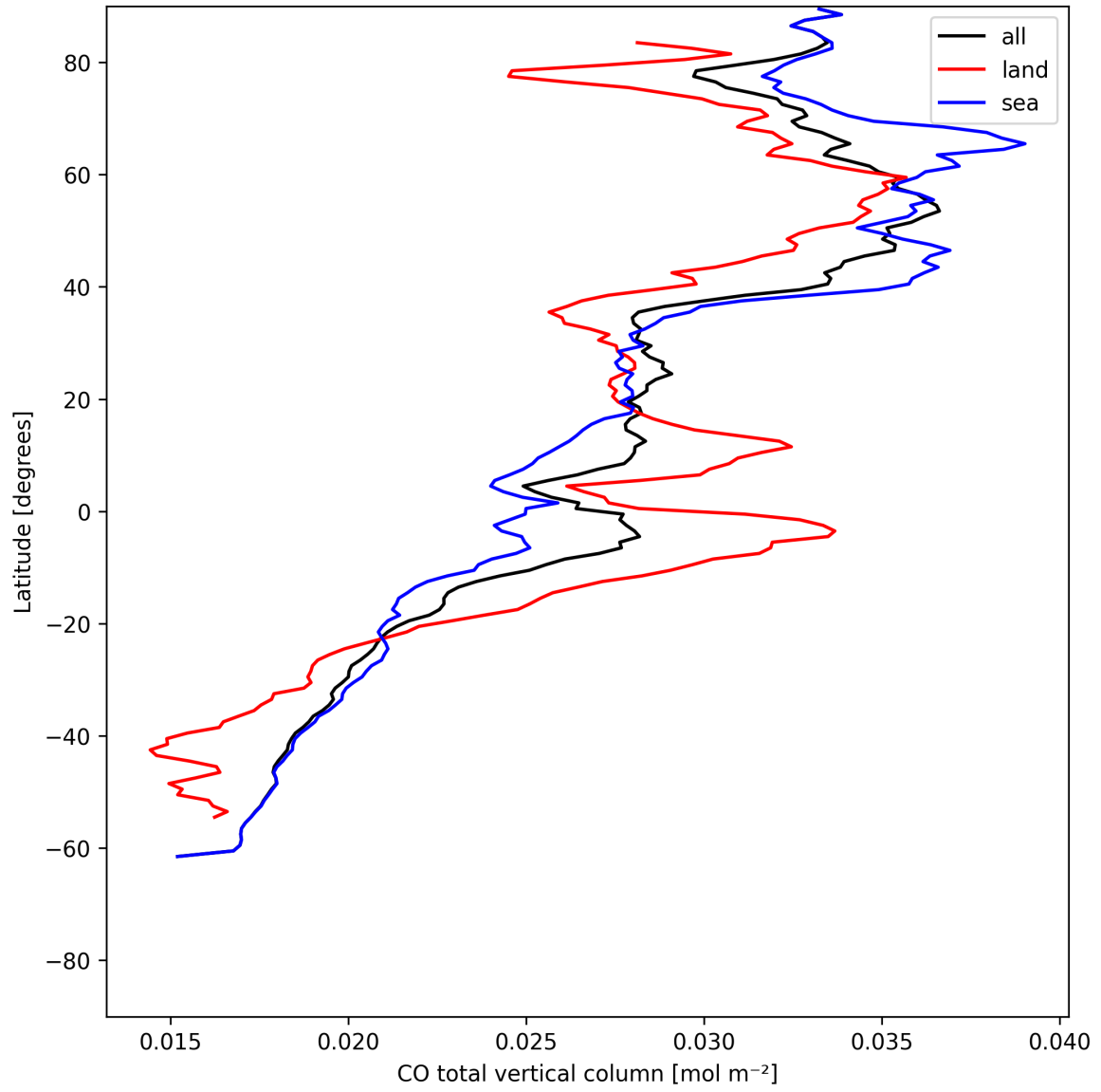
Figure 7: Zonal average of “CO total vertical column” for 2025-06-12 to 2025-06-13.
