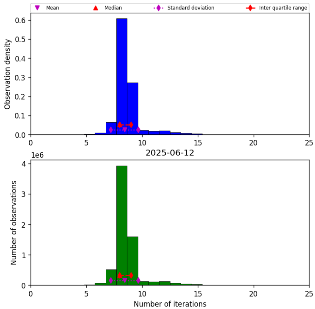
Figure 19: Histogram of “Number of iterations” for 2025-06-12 to 2025-06-13
