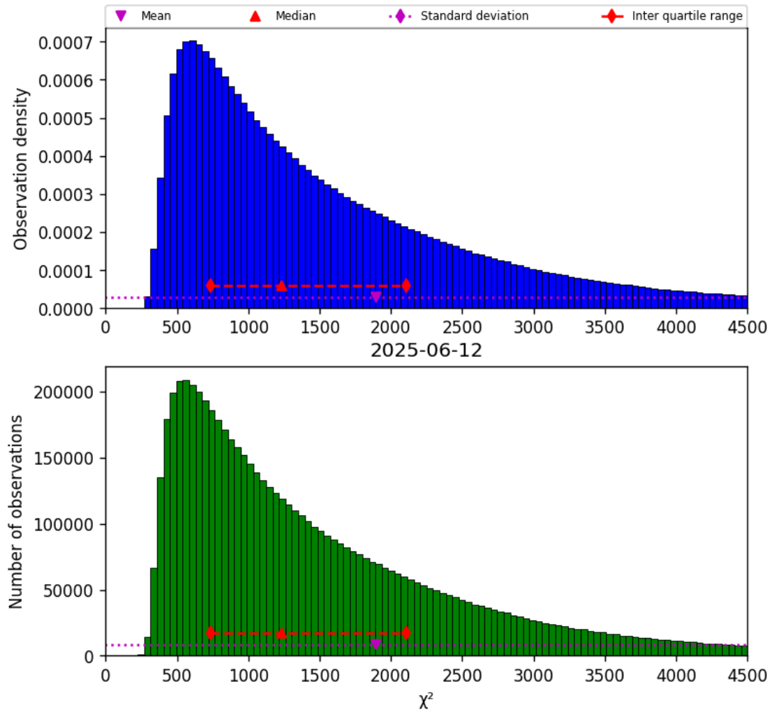
Figure 17: Histogram of “ \chi^2 ” for 2025-06-12 to 2025-06-13
