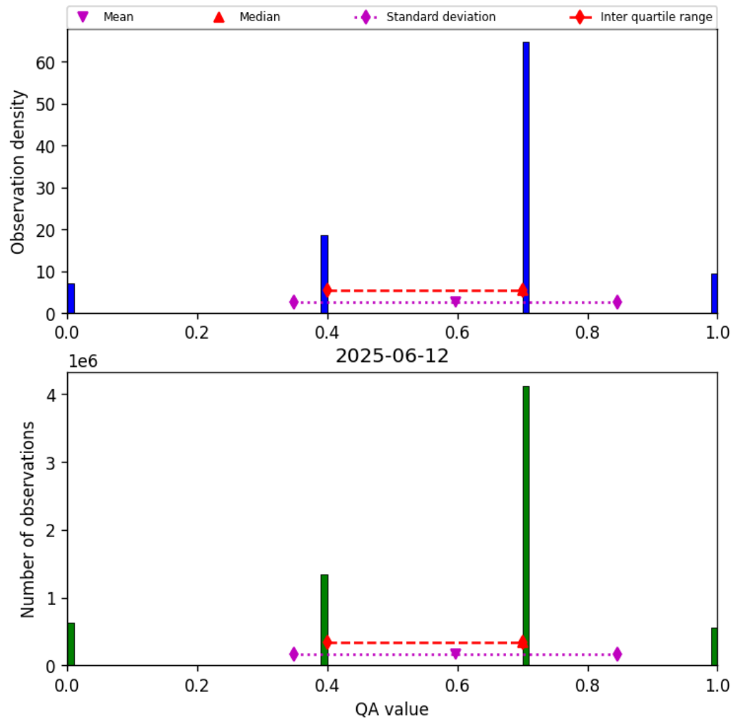
Figure 13: Histogram of “QA value” for 2025-06-12 to 2025-06-13
