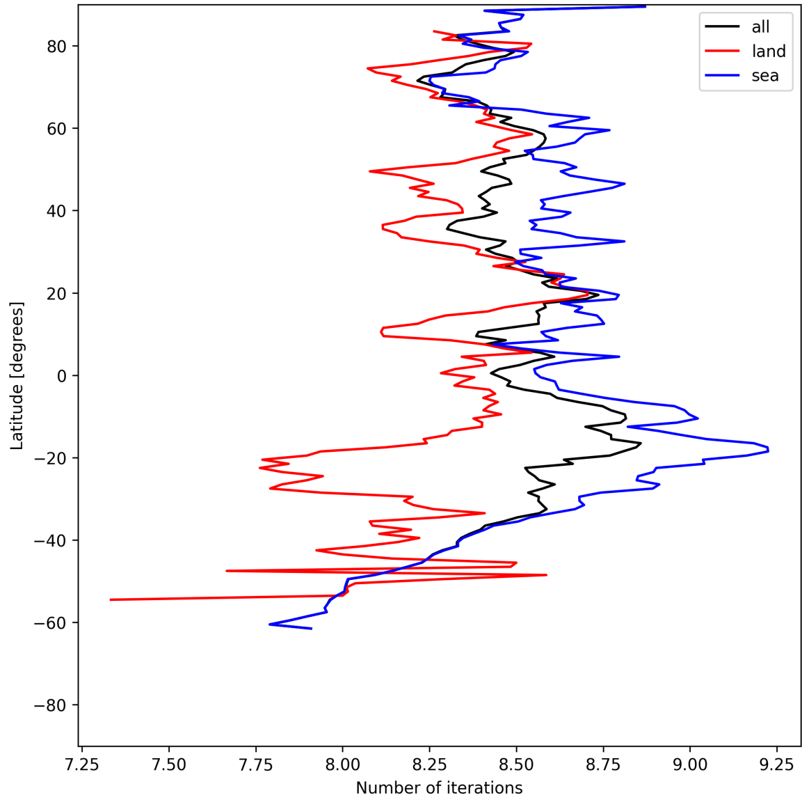
Figure 12: Zonal average of “Number of iterations” for 2025-06-12 to 2025-06-13.
