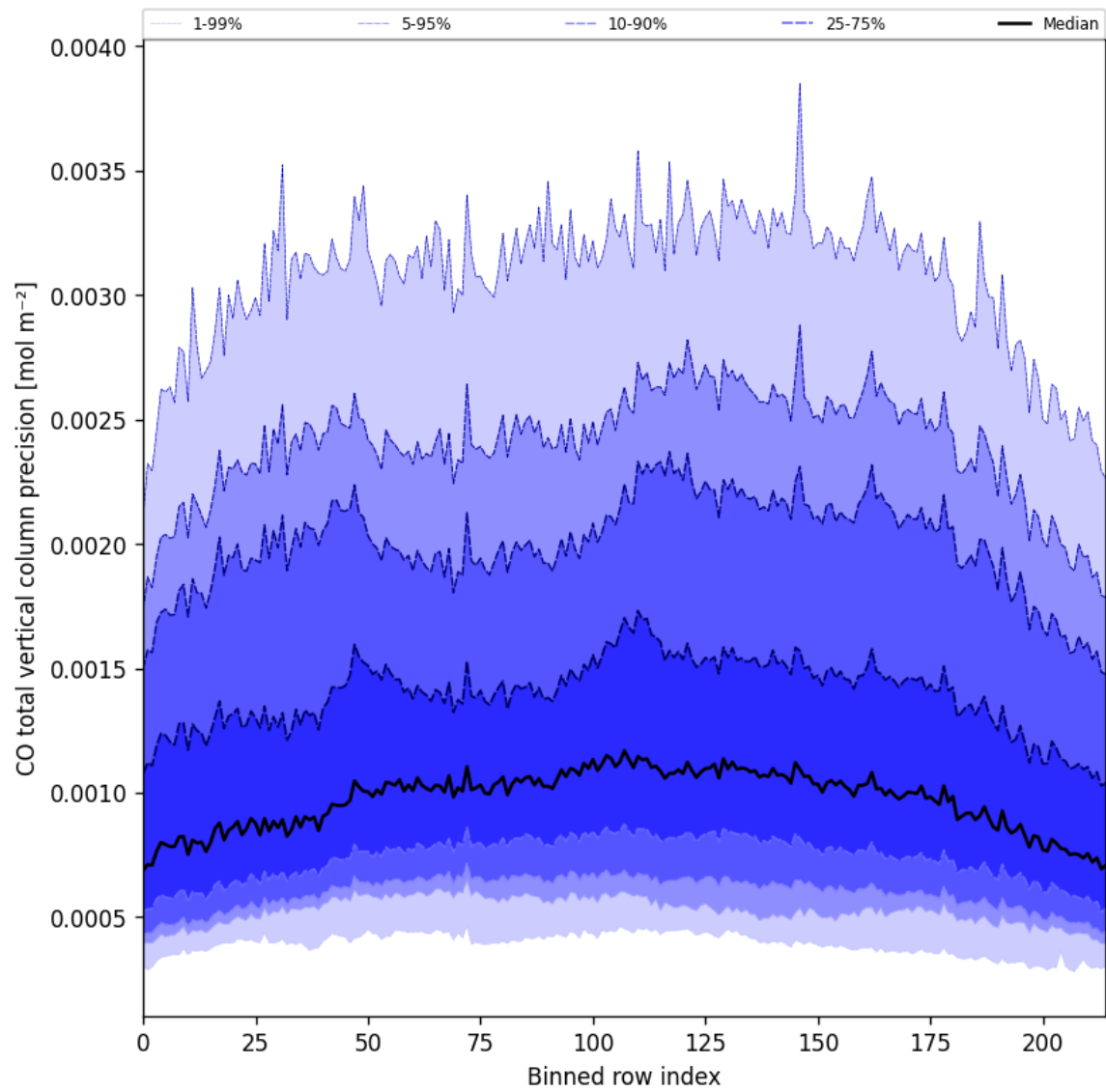
Figure 22: Along track statistics of “CO total vertical column precision” for 2025-06-12 to 2025-06-13
