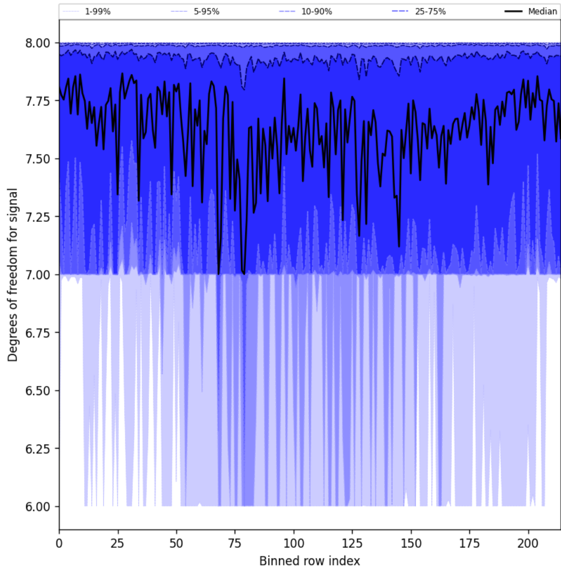
Figure 25: Along track statistics of “Degrees of freedom for signal” for 2025-06-12 to 2025-06-13
