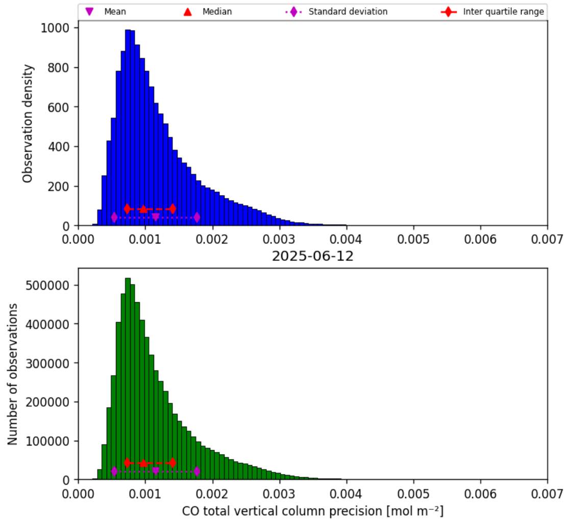
Figure 15: Histogram of “CO total vertical column precision” for 2025-06-12 to 2025-06-13
