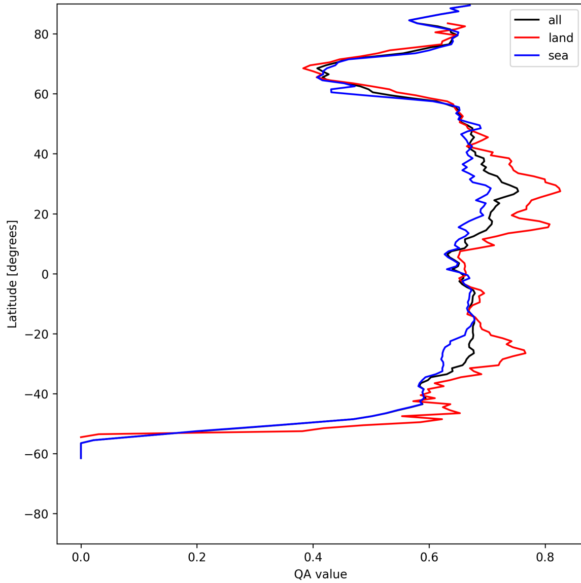
Figure 6: Zonal average of “QA value” for 2025-06-12 to 2025-06-13.
