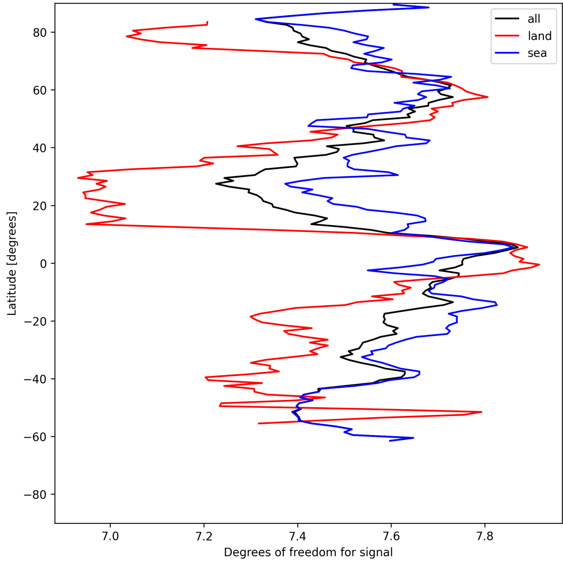
Figure 11: Zonal average of “Degrees of freedom for signal” for 2025-06-13 to 2025-06-14.
