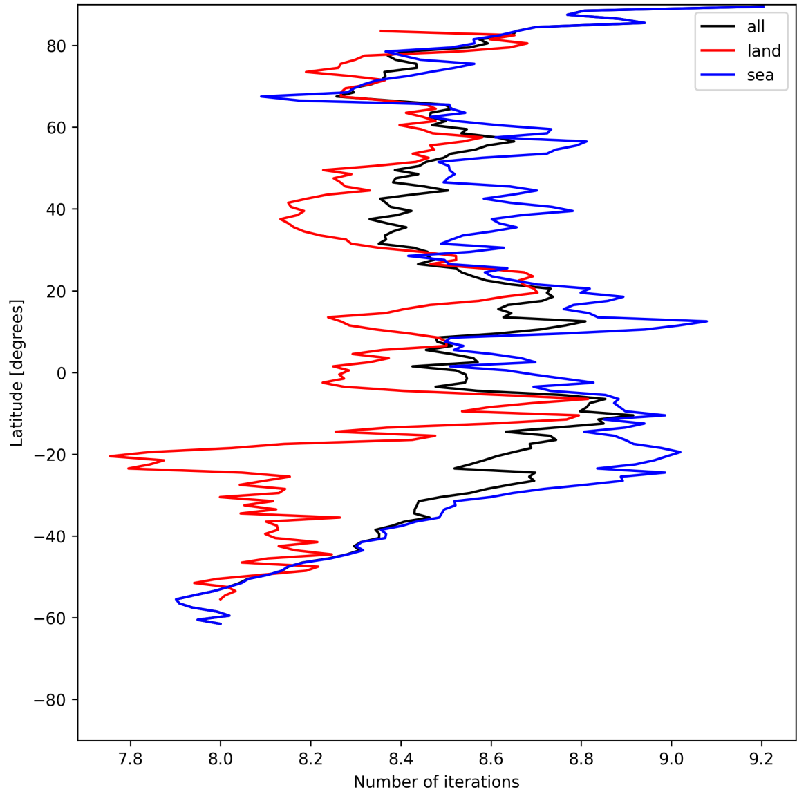
Figure 12: Zonal average of “Number of iterations” for 2025-06-13 to 2025-06-14.
