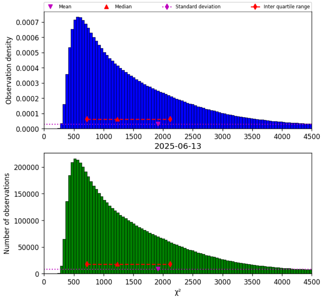
Figure 17: Histogram of “ \chi^2 ” for 2025-06-13 to 2025-06-14
