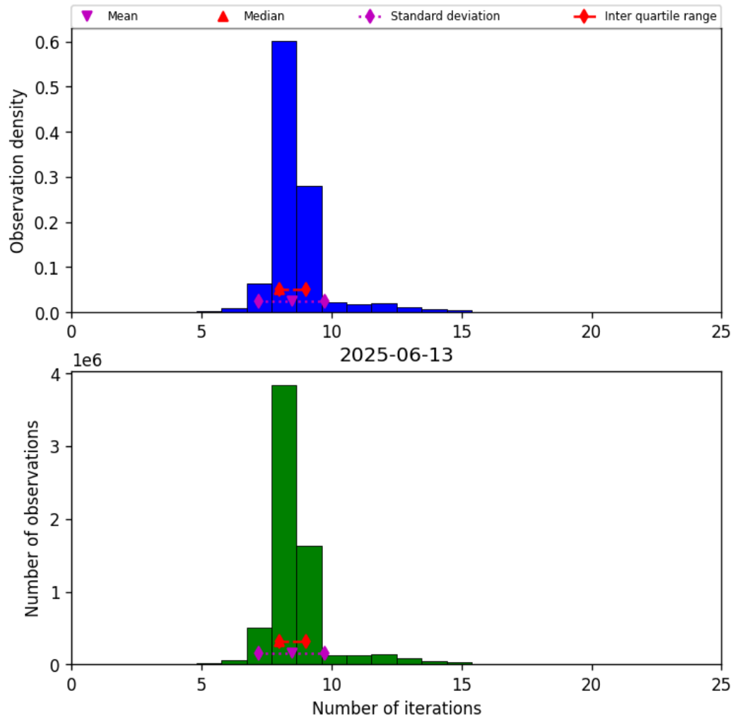
Figure 19: Histogram of “Number of iterations” for 2025-06-13 to 2025-06-14
