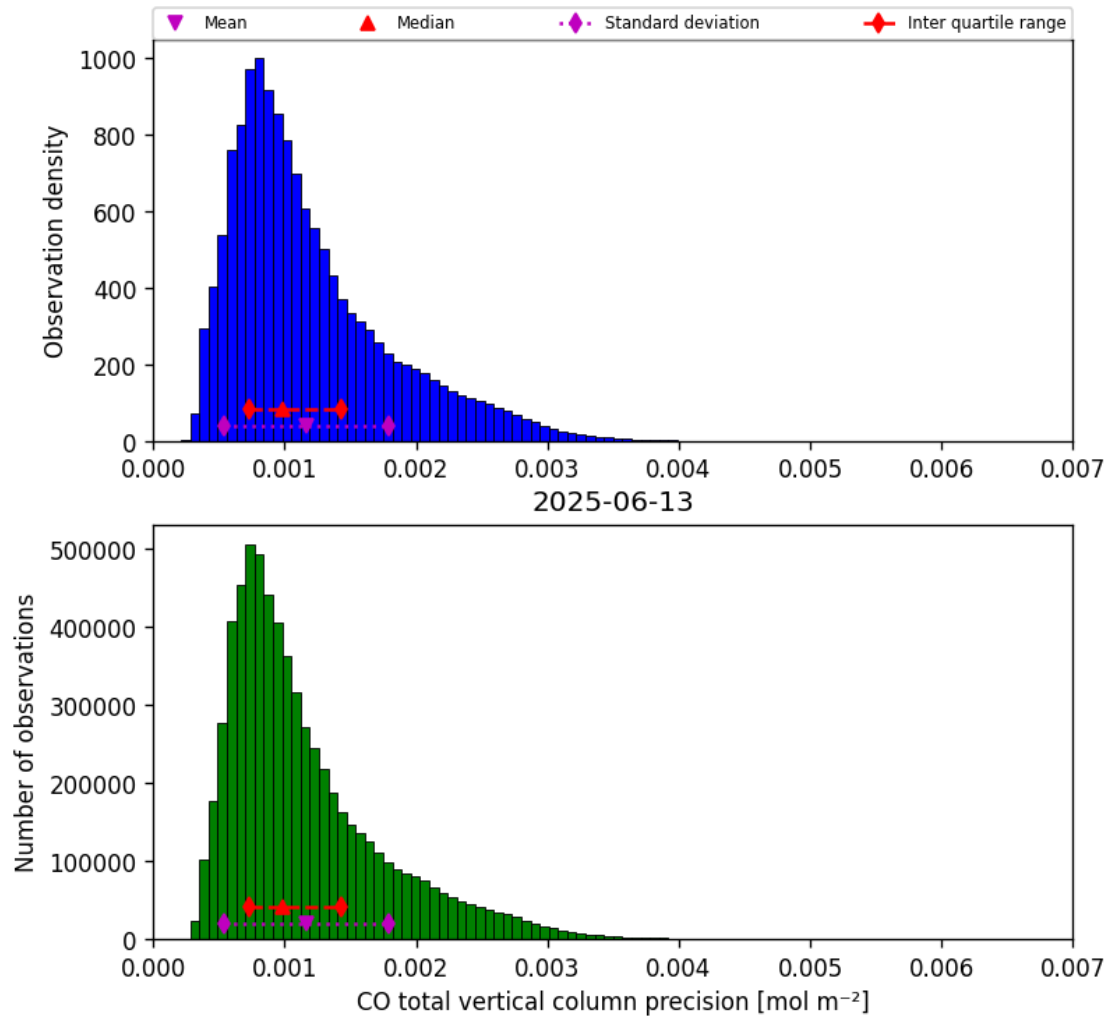
Figure 15: Histogram of “CO total vertical column precision” for 2025-06-13 to 2025-06-14
