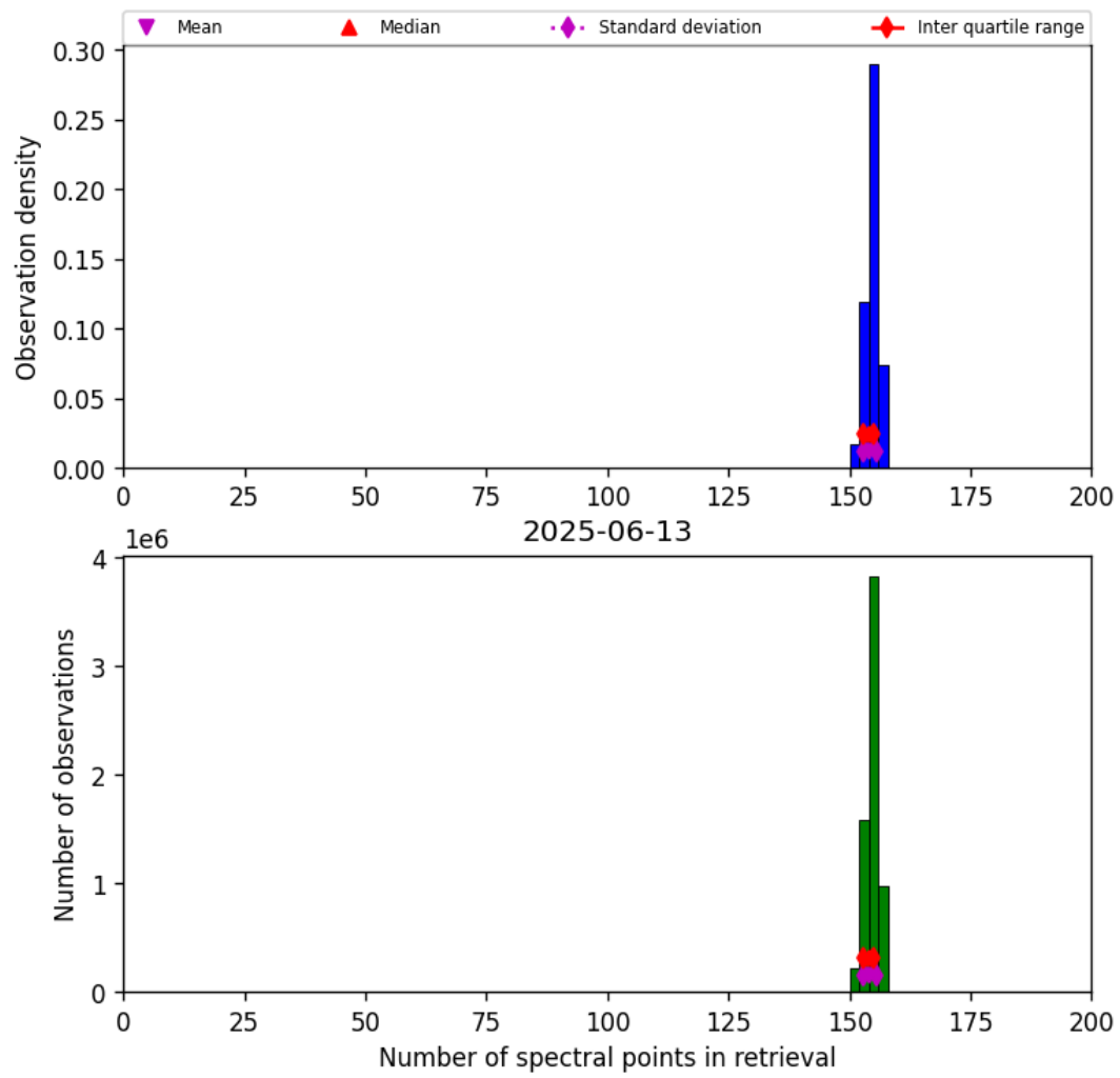
Figure 16: Histogram of “Number of spectral points in retrieval” for 2025-06-13 to 2025-06-14
