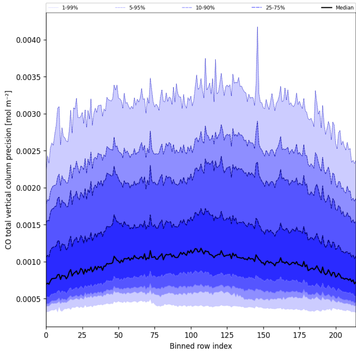
Figure 22: Along track statistics of “CO total vertical column precision” for 2025-06-13 to 2025-06-14
