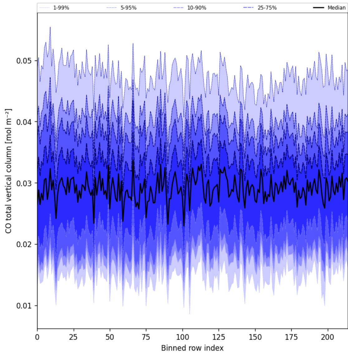
Figure 21: Along track statistics of “CO total vertical column” for 2025-06-13 to 2025-06-14
