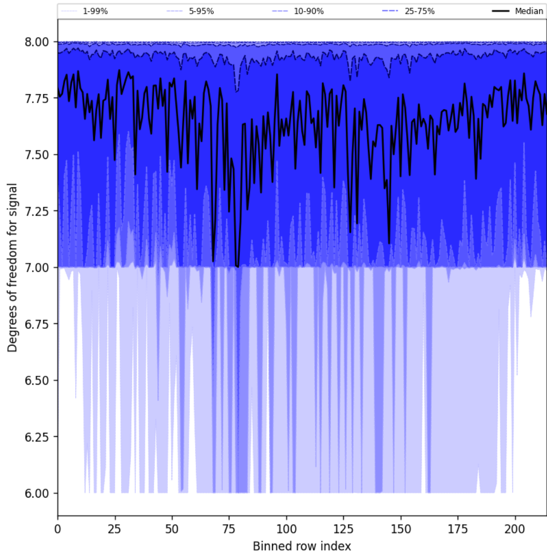
Figure 25: Along track statistics of “Degrees of freedom for signal” for 2025-06-13 to 2025-06-14
