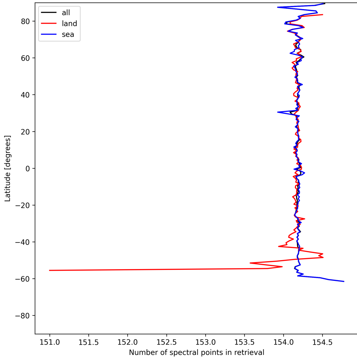
Figure 9: Zonal average of “Number of spectral points in retrieval” for 2025-06-13 to 2025-06-14.
