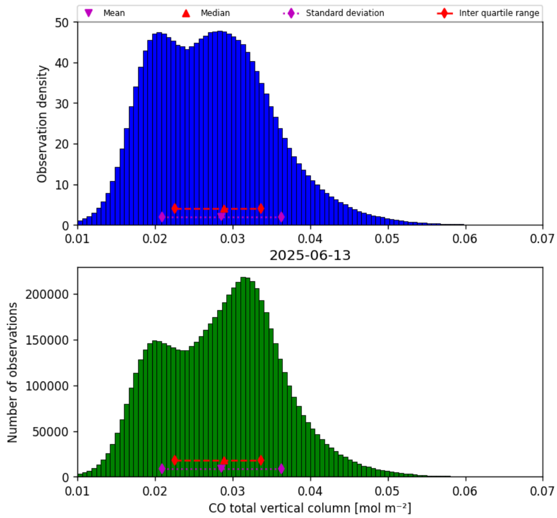
Figure 14: Histogram of “CO total vertical column” for 2025-06-13 to 2025-06-14
