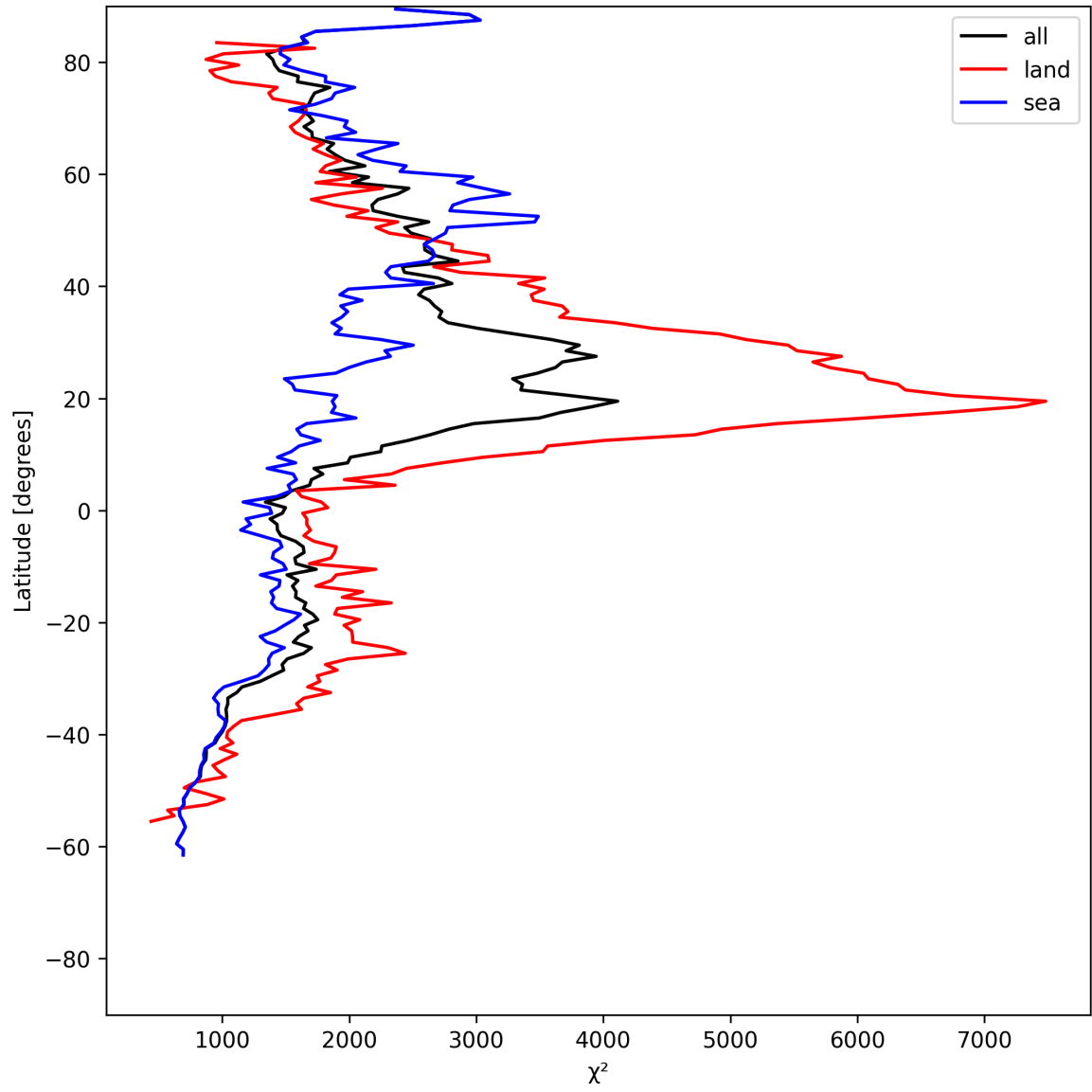
Figure 10: Zonal average of “ \chi^2 ” for 2025-06-13 to 2025-06-14.
