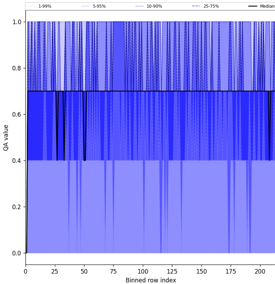
Figure 20: Along track statistics of “QA value” for 2025-06-13 to 2025-06-14
