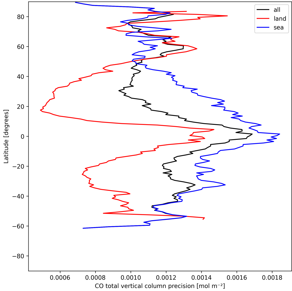
Figure 8: Zonal average of “CO total vertical column precision” for 2025-06-13 to 2025-06-14.
