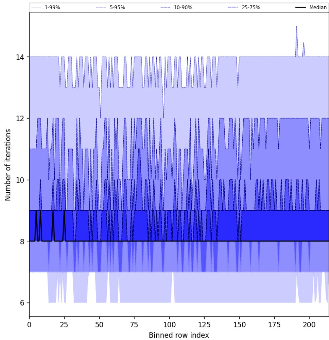
Figure 26: Along track statistics of “Number of iterations” for 2025-06-13 to 2025-06-14
