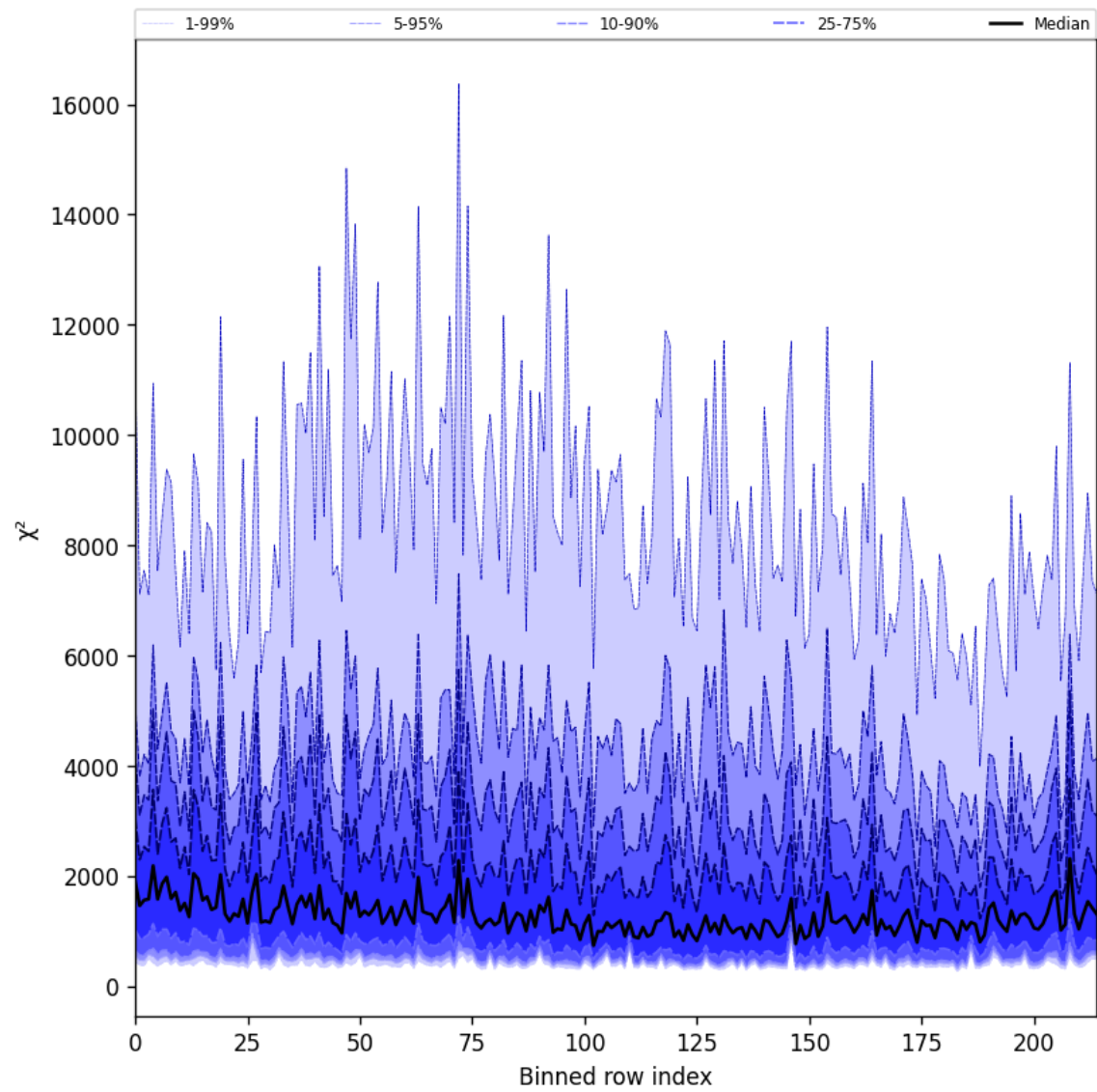
Figure 24: Along track statistics of “ \chi^2 ” for 2025-06-14 to 2025-06-14
