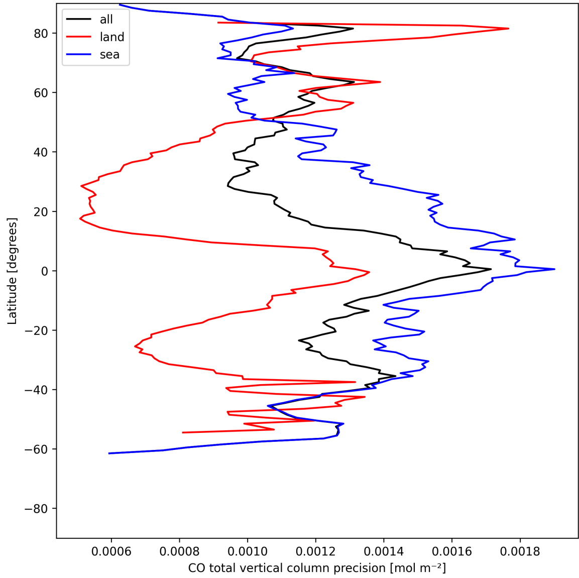
Figure 8: Zonal average of “CO total vertical column precision” for 2025-06-14 to 2025-06-14.
