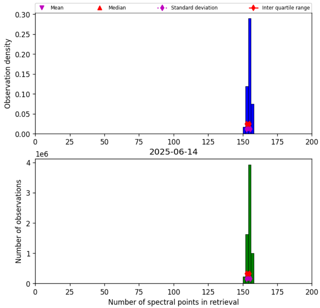
Figure 16: Histogram of “Number of spectral points in retrieval” for 2025-06-14 to 2025-06-14
