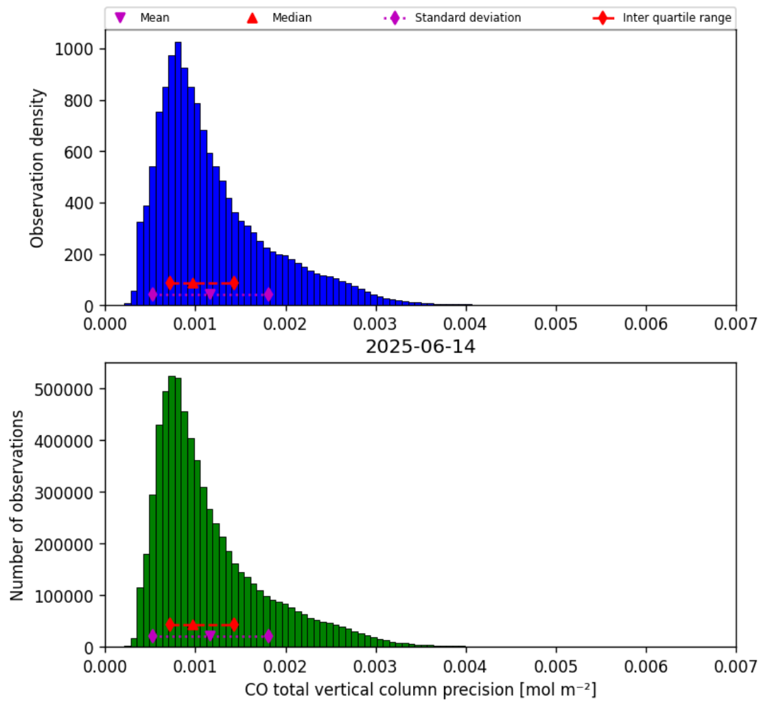
Figure 15: Histogram of “CO total vertical column precision” for 2025-06-14 to 2025-06-14
