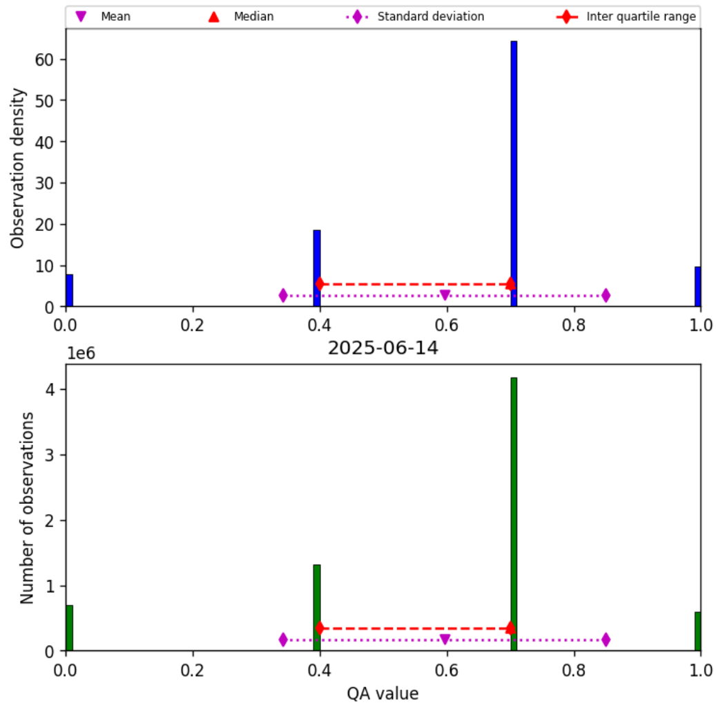
Figure 13: Histogram of “QA value” for 2025-06-14 to 2025-06-14
