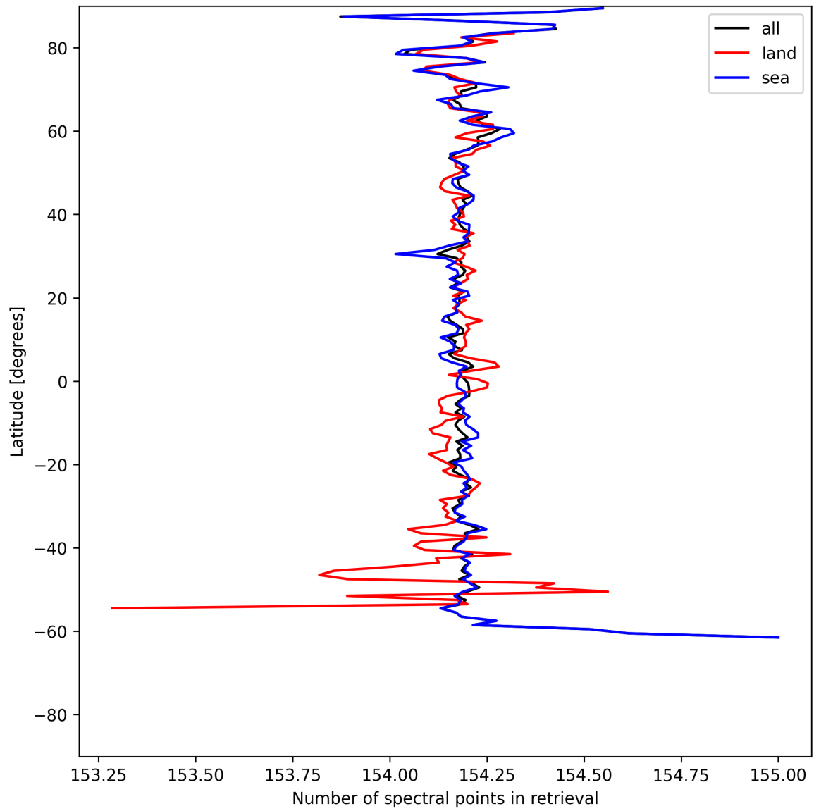
Figure 9: Zonal average of “Number of spectral points in retrieval” for 2025-06-14 to 2025-06-14.
