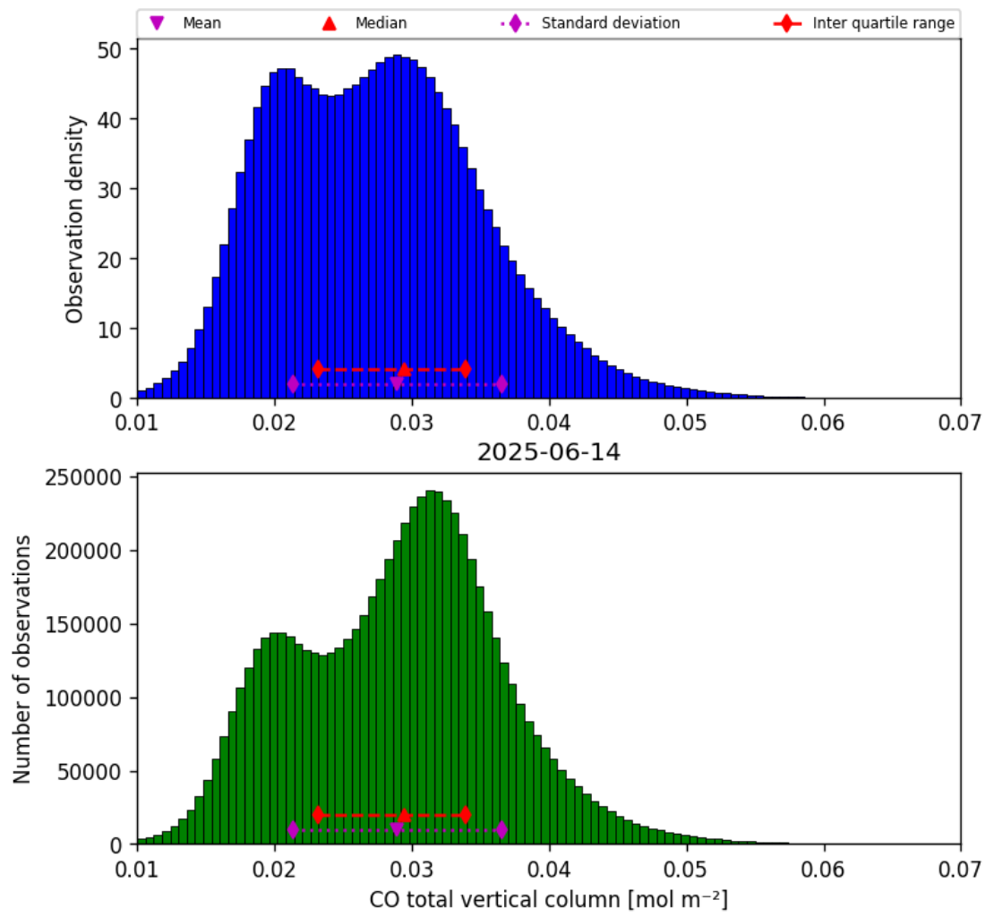
Figure 14: Histogram of “CO total vertical column” for 2025-06-14 to 2025-06-14
