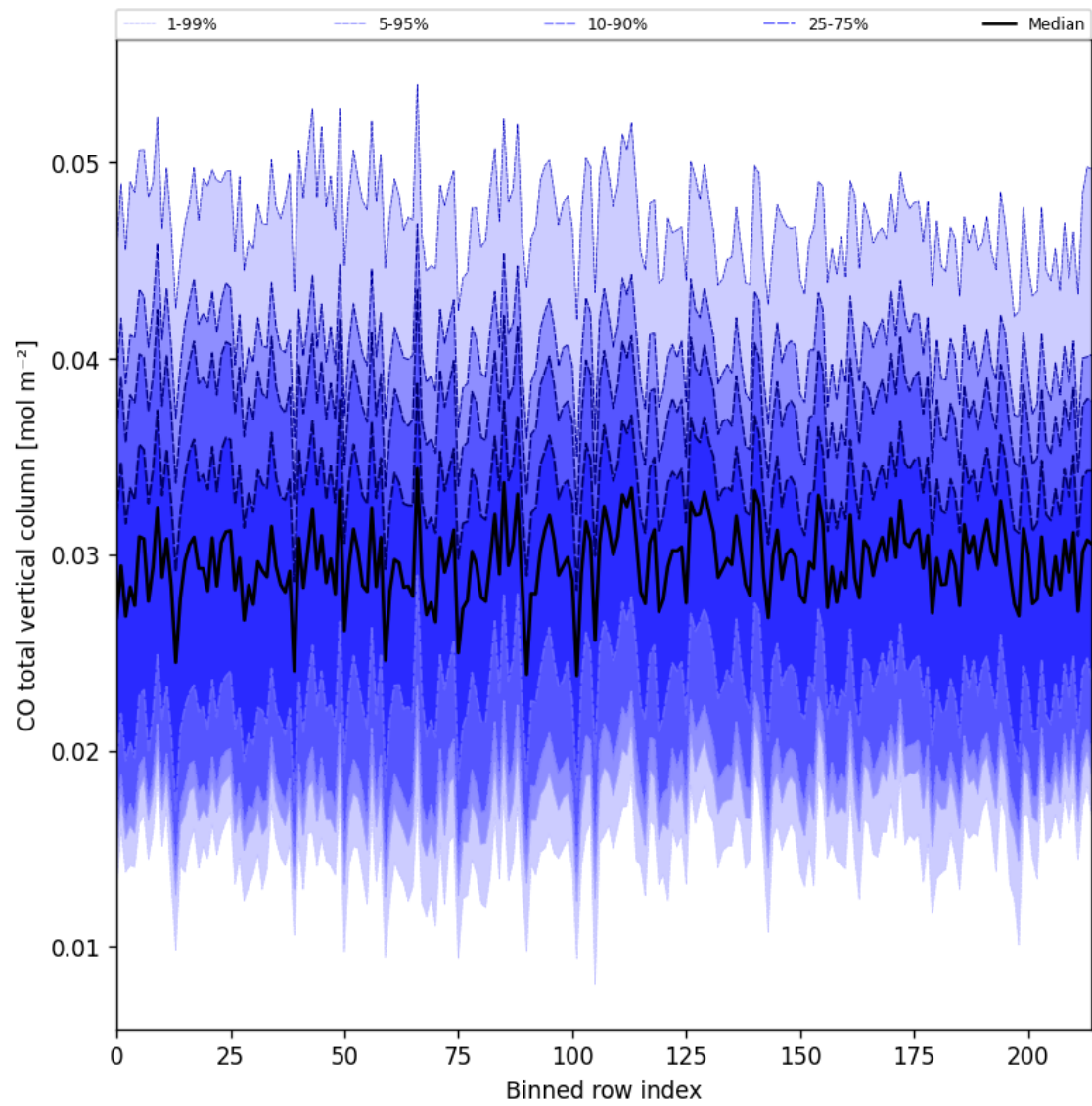
Figure 21: Along track statistics of “CO total vertical column” for 2025-06-14 to 2025-06-14
