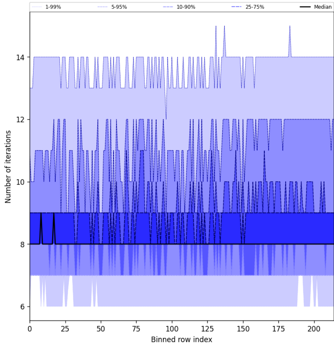
Figure 26: Along track statistics of “Number of iterations” for 2025-06-14 to 2025-06-14
