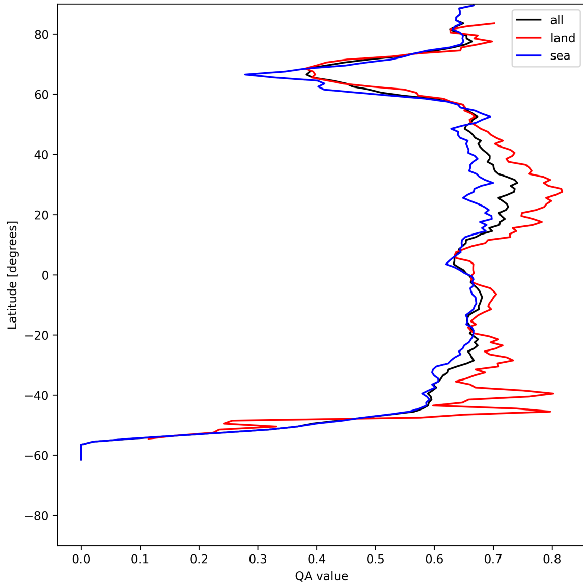
Figure 6: Zonal average of “QA value” for 2025-06-14 to 2025-06-14.
