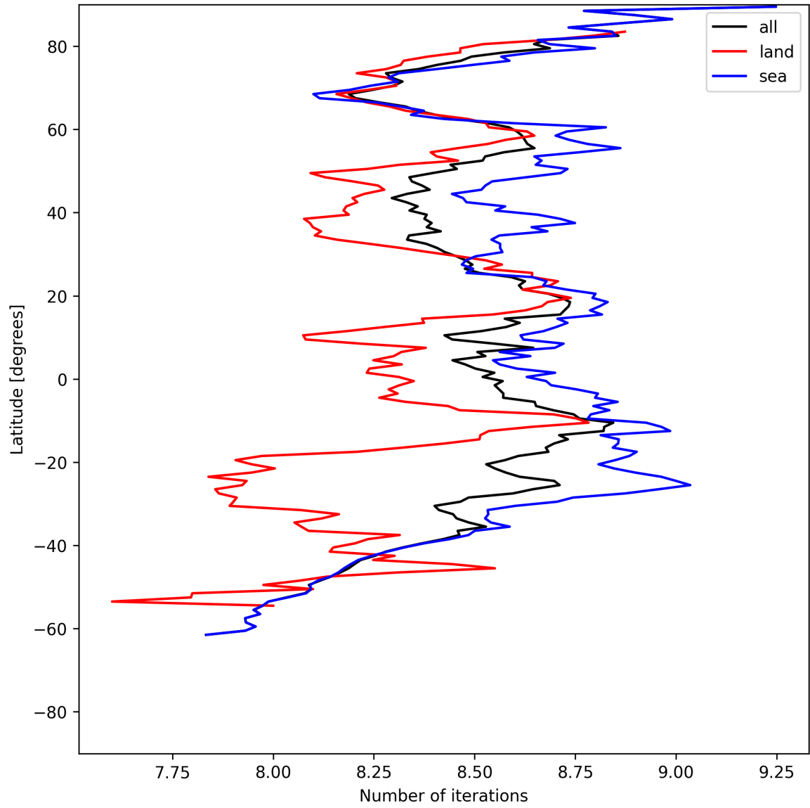
Figure 12: Zonal average of “Number of iterations” for 2025-06-14 to 2025-06-14.
