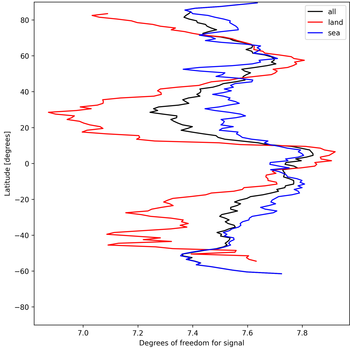
Figure 11: Zonal average of “Degrees of freedom for signal” for 2025-06-14 to 2025-06-14.
