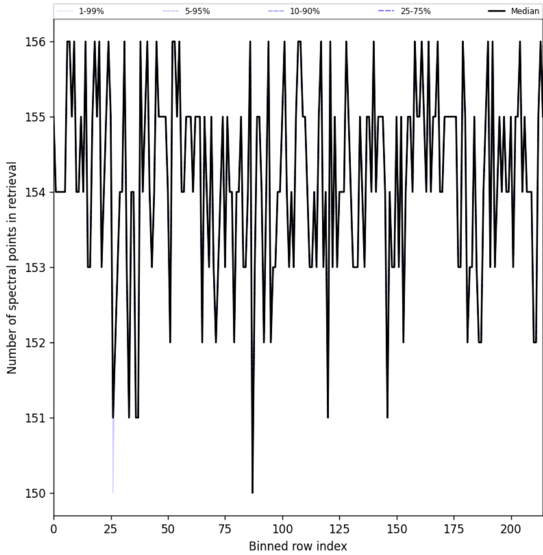
Figure 23: Along track statistics of “Number of spectral points in retrieval” for 2025-06-14 to 2025-06-14
