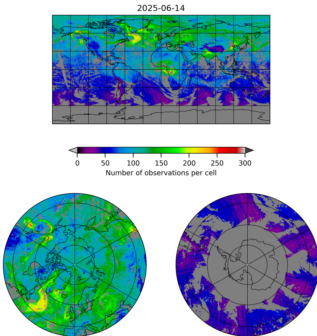
Figure 5: Map of the number of observations for 2025-06-14 to 2025-06-14
