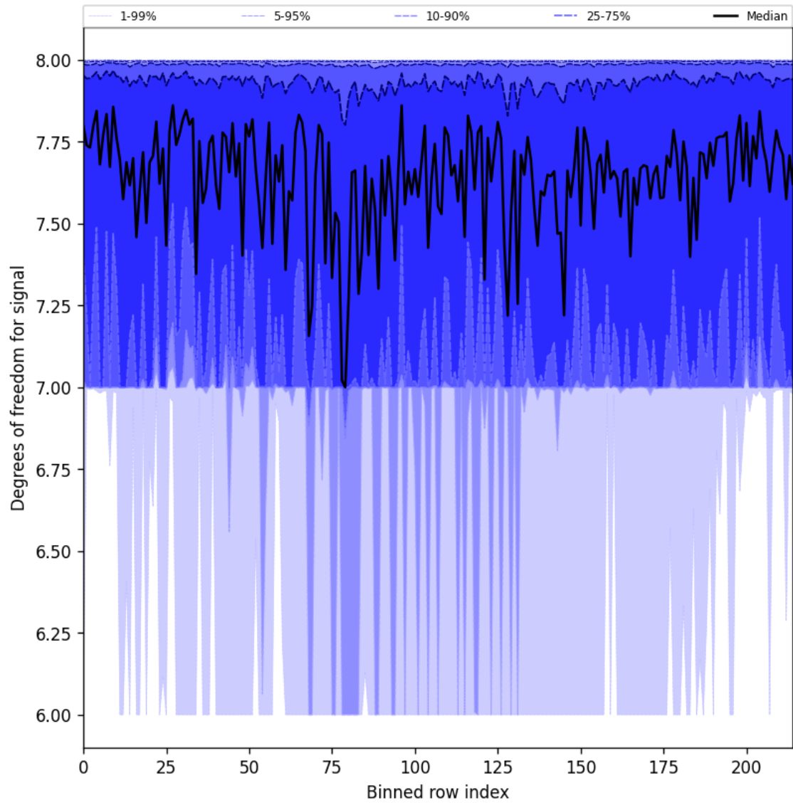
Figure 25: Along track statistics of “Degrees of freedom for signal” for 2025-06-14 to 2025-06-14
