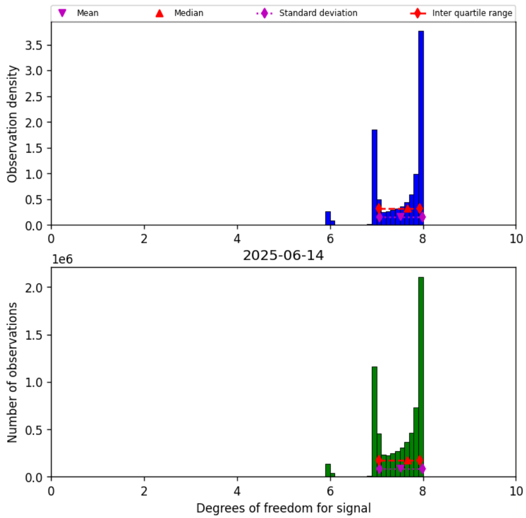
Figure 18: Histogram of “Degrees of freedom for signal” for 2025-06-14 to 2025-06-14
