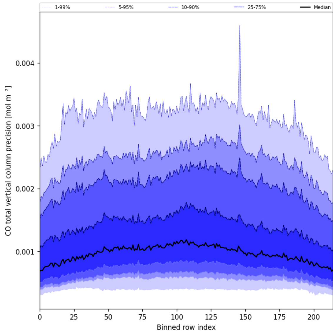
Figure 22: Along track statistics of “CO total vertical column precision” for 2025-06-14 to 2025-06-14
