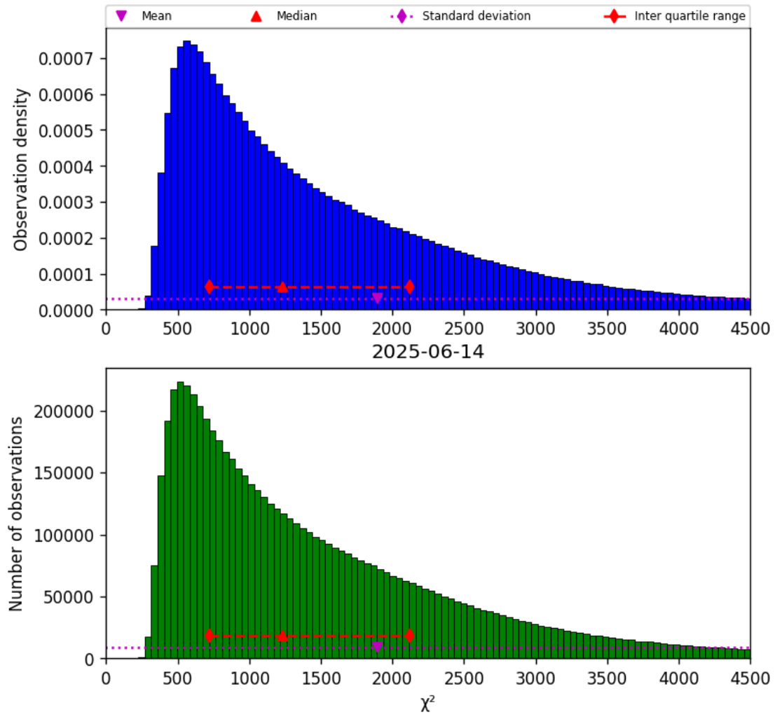
Figure 17: Histogram of " \chi^2 " for 2025-06-14 to 2025-06-14
