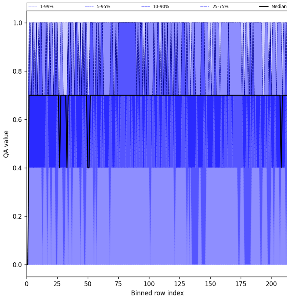
Figure 20: Along track statistics of “QA value” for 2025-06-14 to 2025-06-14
