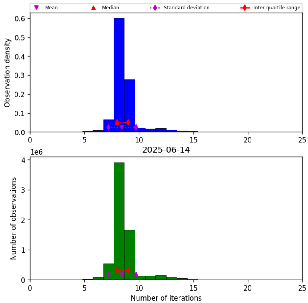
Figure 19: Histogram of “Number of iterations” for 2025-06-14 to 2025-06-14
