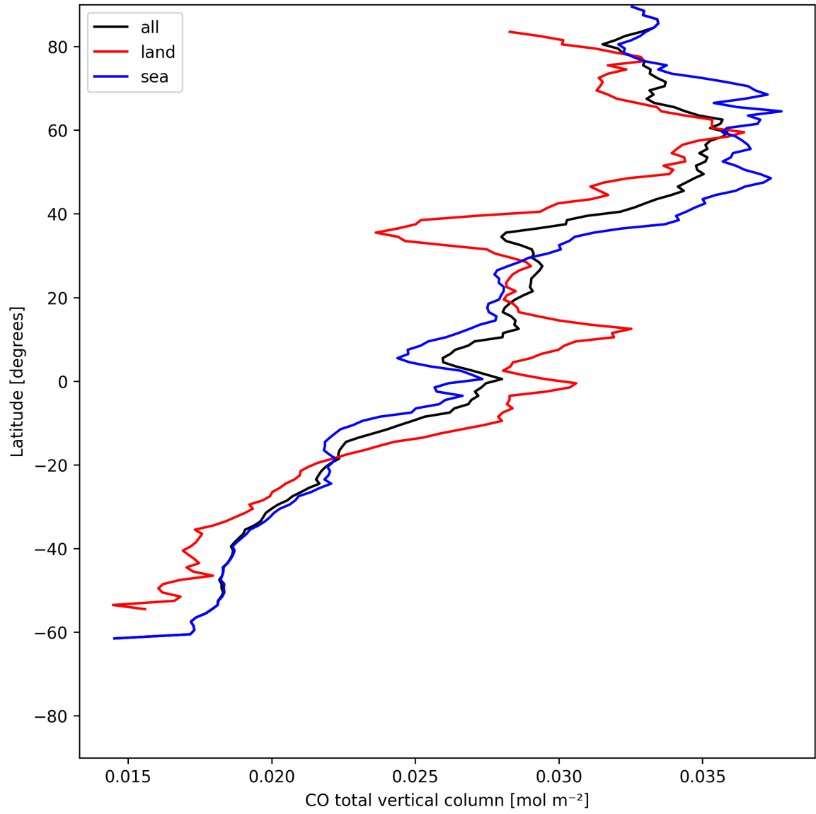
Figure 7: Zonal average of “CO total vertical column” for 2025-06-14 to 2025-06-14.
