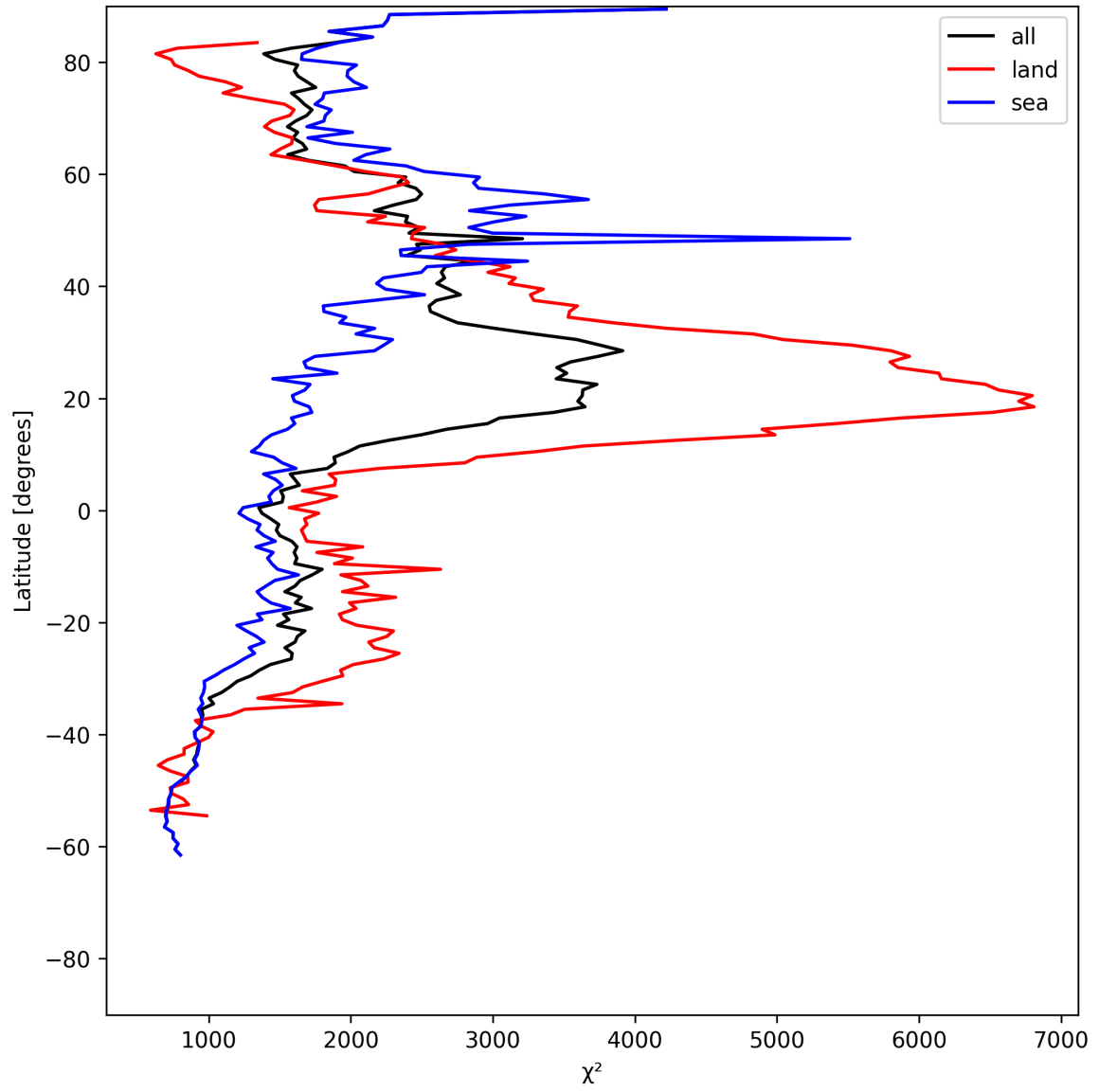
Figure 10: Zonal average of “ \chi^2 ” for 2025-06-14 to 2025-06-14.
