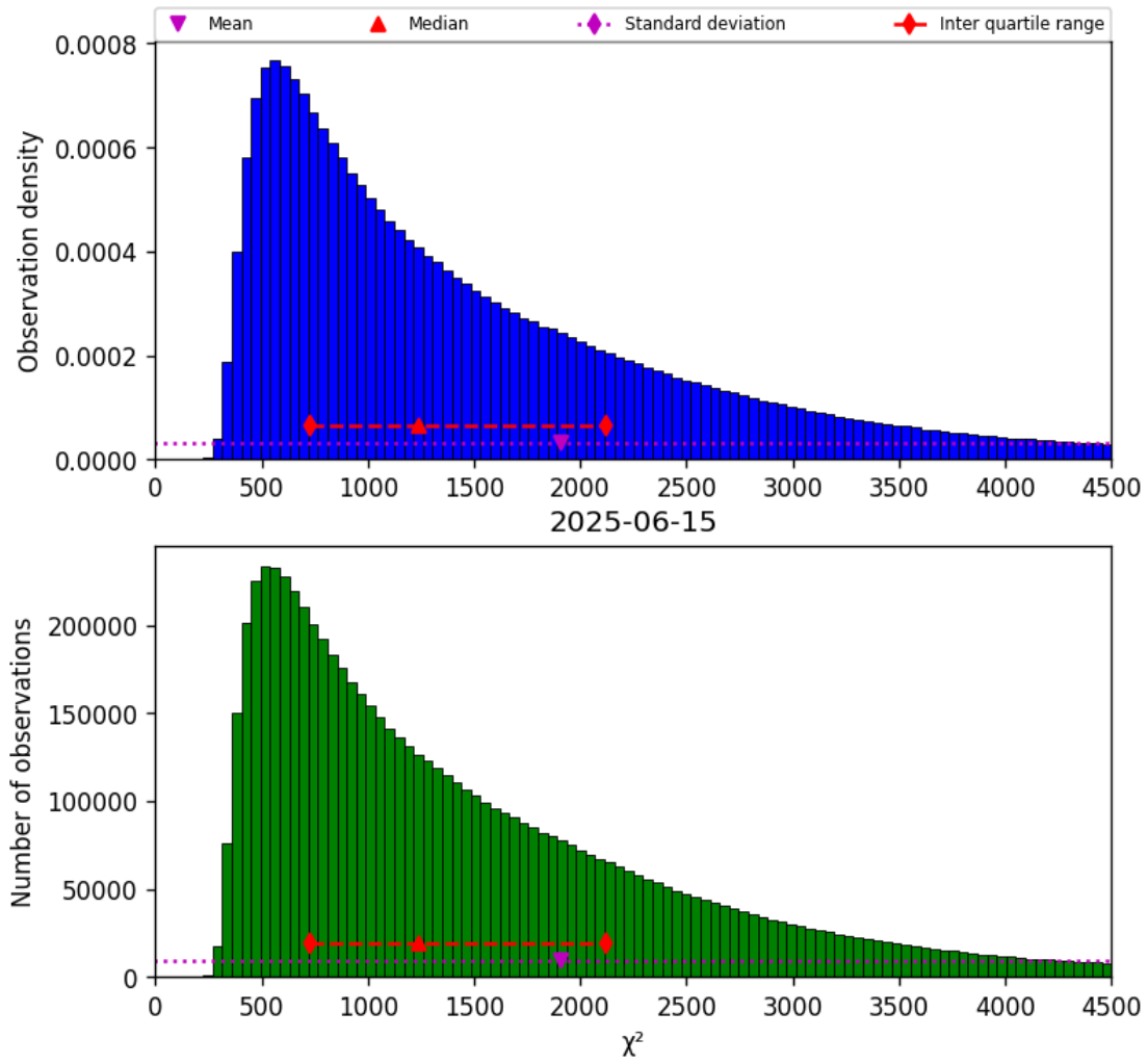
Figure 17: Histogram of “ \chi^2 ” for 2025-06-15 to 2025-06-16
