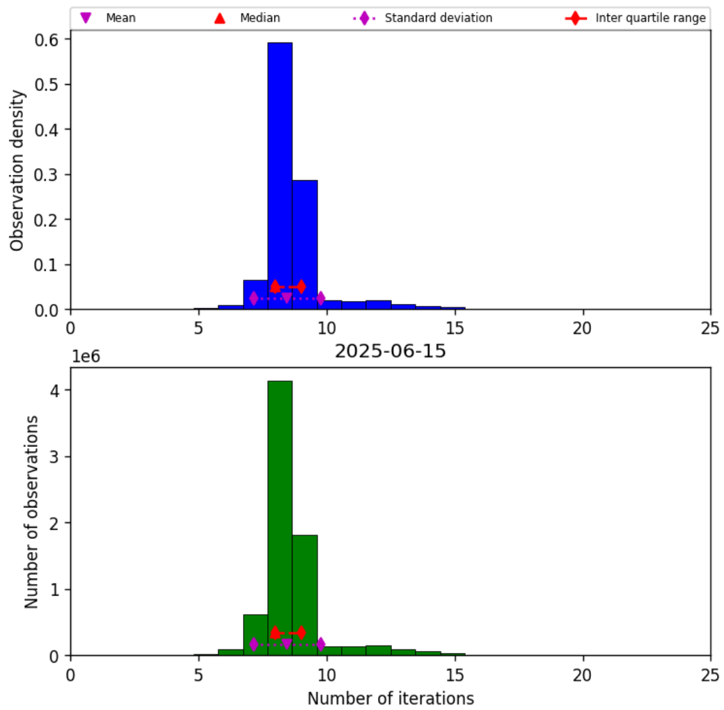
Figure 19: Histogram of “Number of iterations” for 2025-06-15 to 2025-06-16
