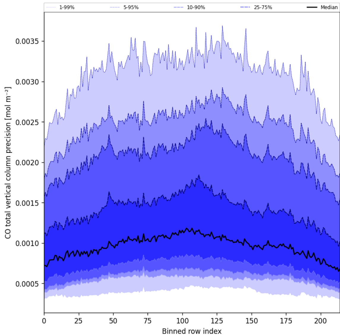
Figure 22: Along track statistics of “CO total vertical column precision” for 2025-06-15 to 2025-06-16
