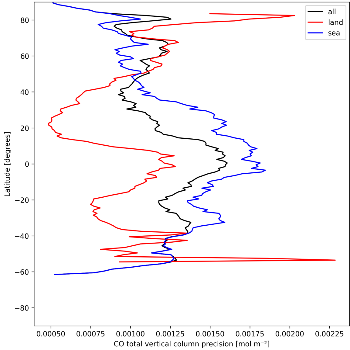
Figure 8: Zonal average of “CO total vertical column precision” for 2025-06-15 to 2025-06-16.
