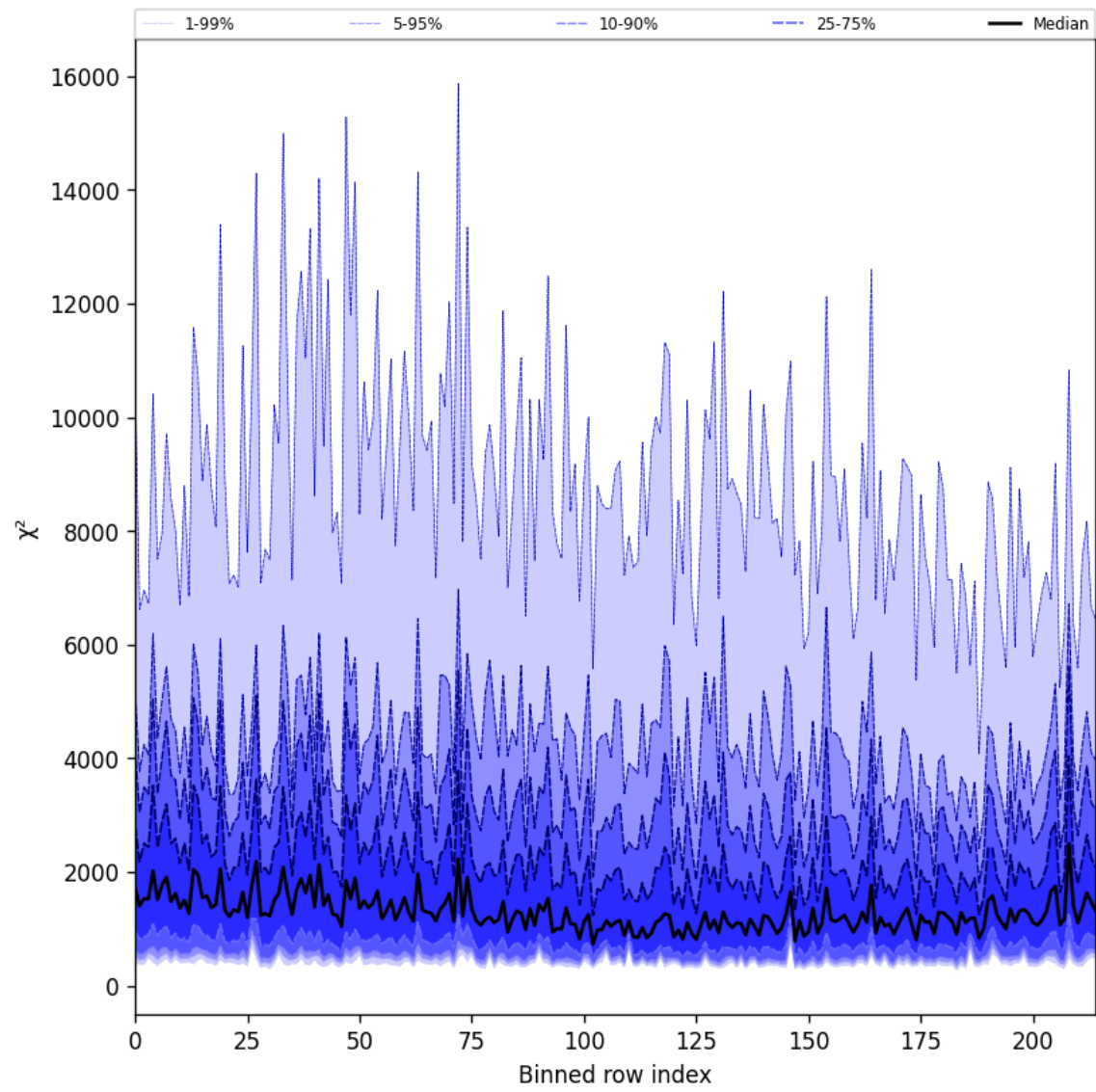
Figure 24: Along track statistics of “ \chi^2 ” for 2025-06-15 to 2025-06-16
