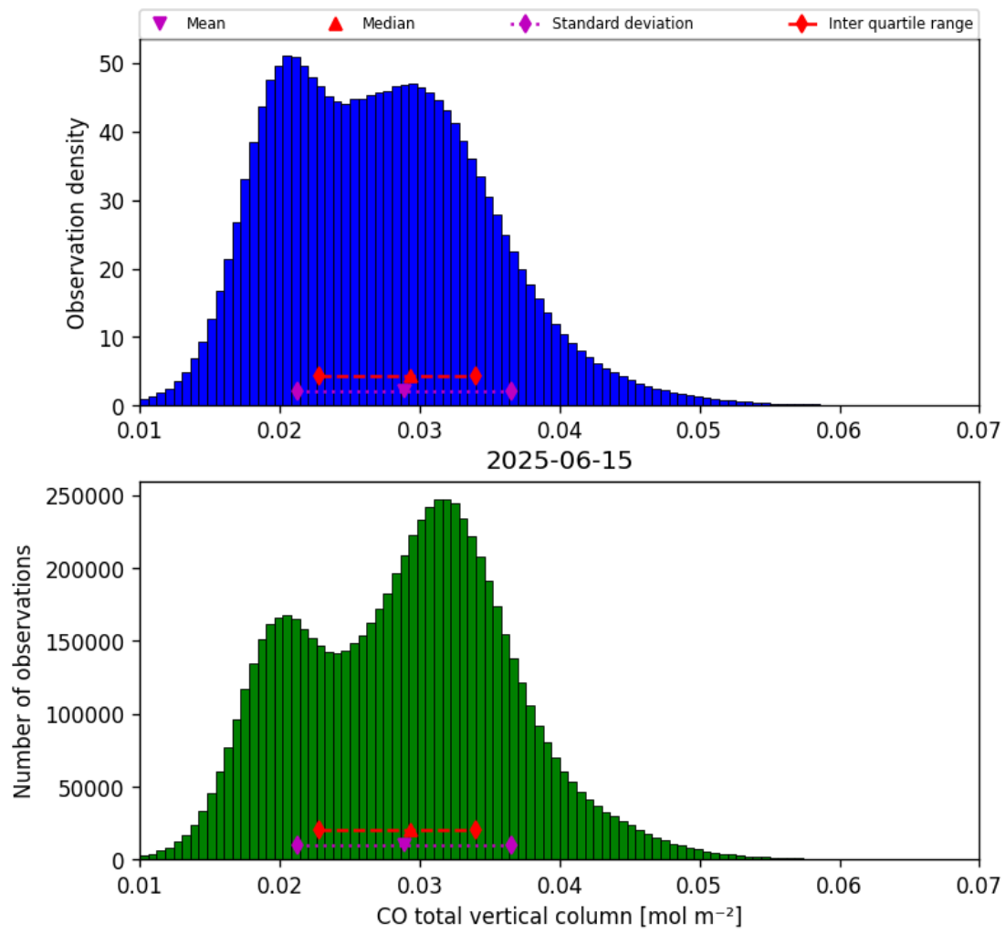
Figure 14: Histogram of “CO total vertical column” for 2025-06-15 to 2025-06-16
