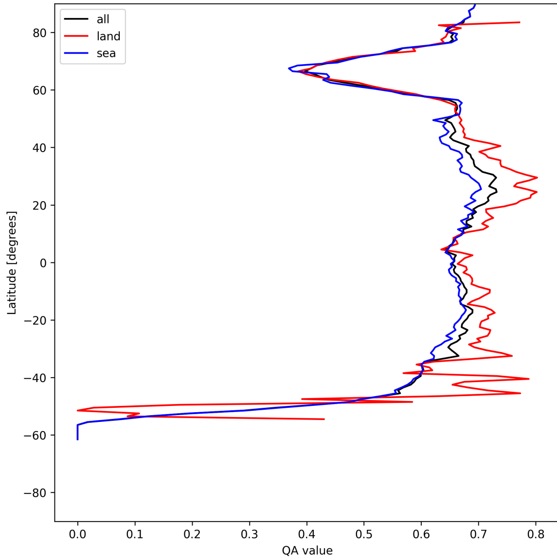
Figure 6: Zonal average of “QA value” for 2025-06-15 to 2025-06-16.
