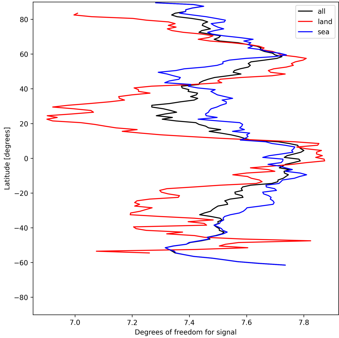
Figure 11: Zonal average of “Degrees of freedom for signal” for 2025-06-15 to 2025-06-16.
