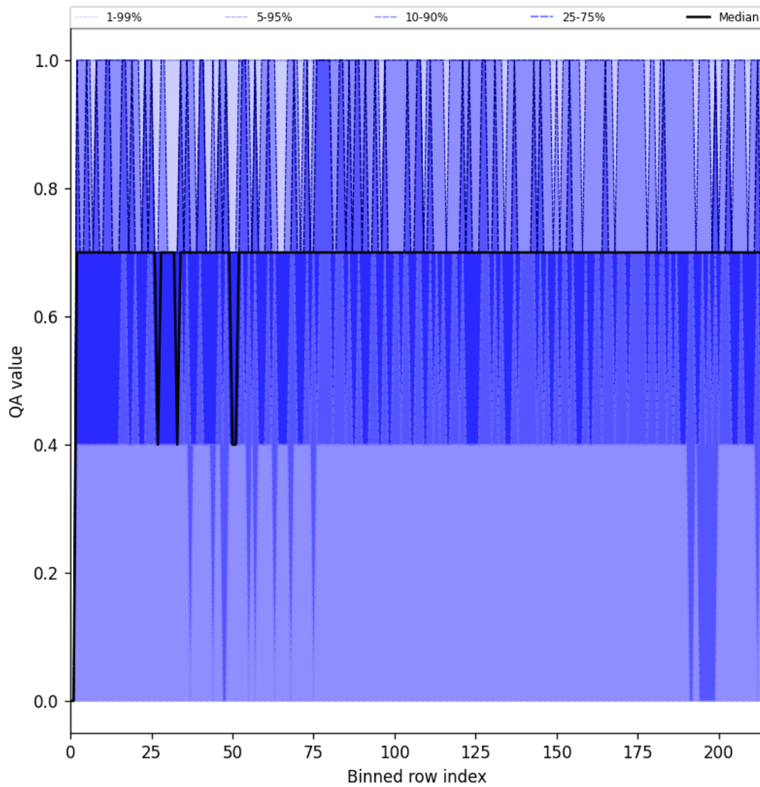
Figure 20: Along track statistics of “QA value” for 2025-06-15 to 2025-06-16
