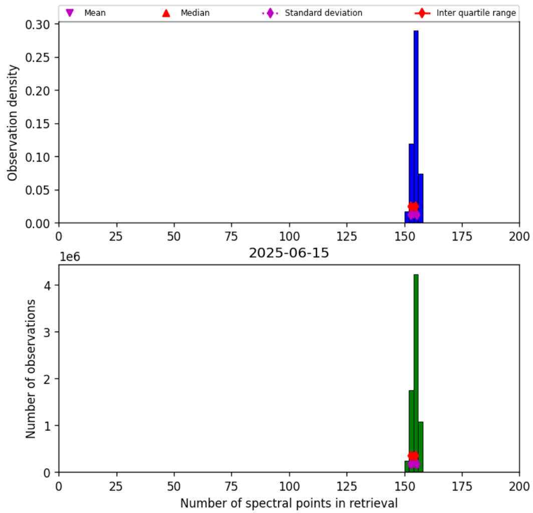
Figure 16: Histogram of “Number of spectral points in retrieval” for 2025-06-15 to 2025-06-16
