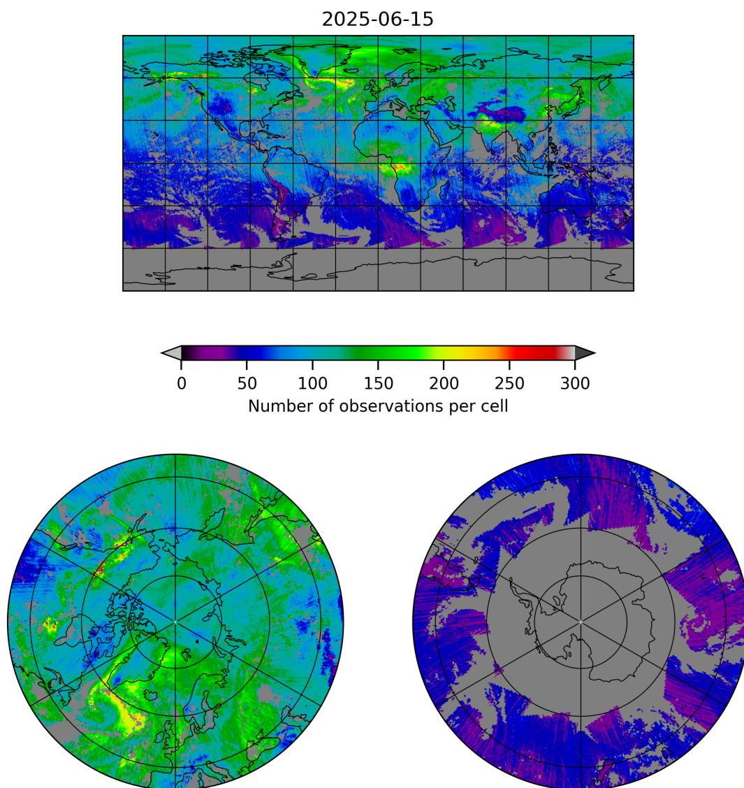
Figure 5: Map of the number of observations for 2025-06-15 to 2025-06-16
