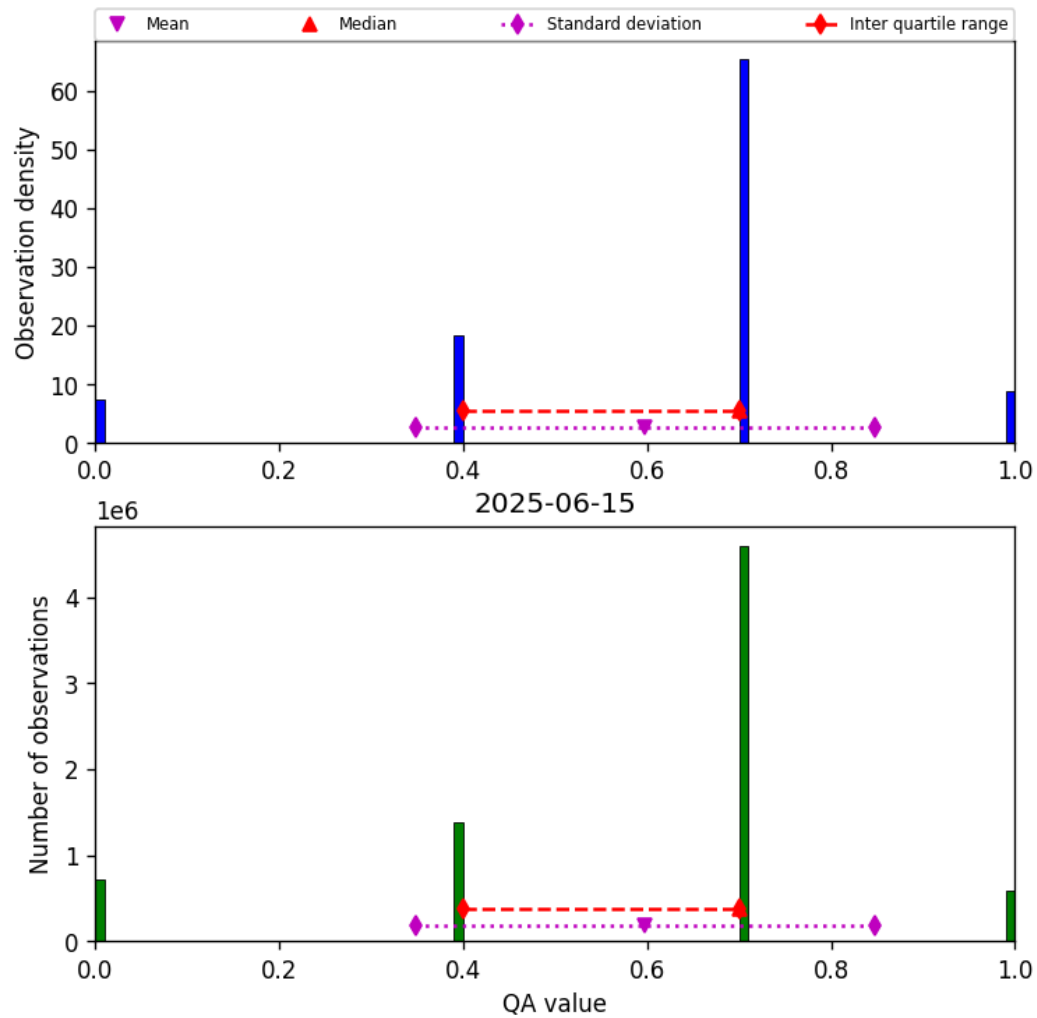
Figure 13: Histogram of “QA value” for 2025-06-15 to 2025-06-16
