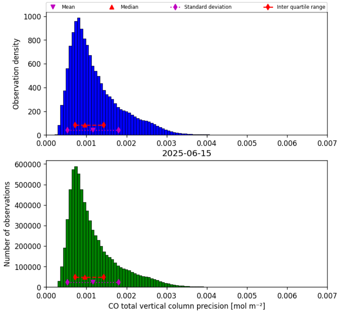
Figure 15: Histogram of “CO total vertical column precision” for 2025-06-15 to 2025-06-16
