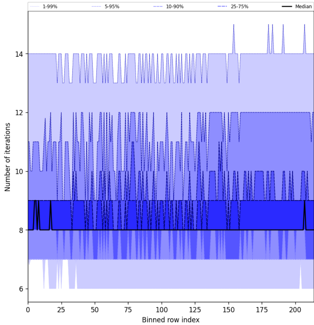
Figure 26: Along track statistics of “Number of iterations” for 2025-06-15 to 2025-06-16
