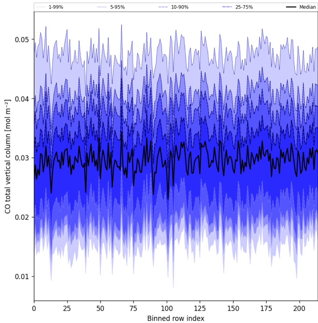
Figure 21: Along track statistics of “CO total vertical column” for 2025-06-15 to 2025-06-16
