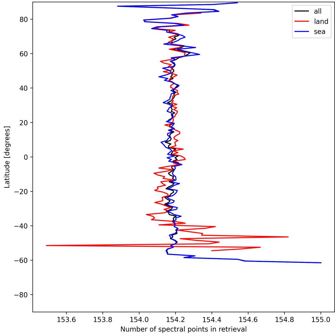
Figure 9: Zonal average of “Number of spectral points in retrieval” for 2025-06-15 to 2025-06-16.
