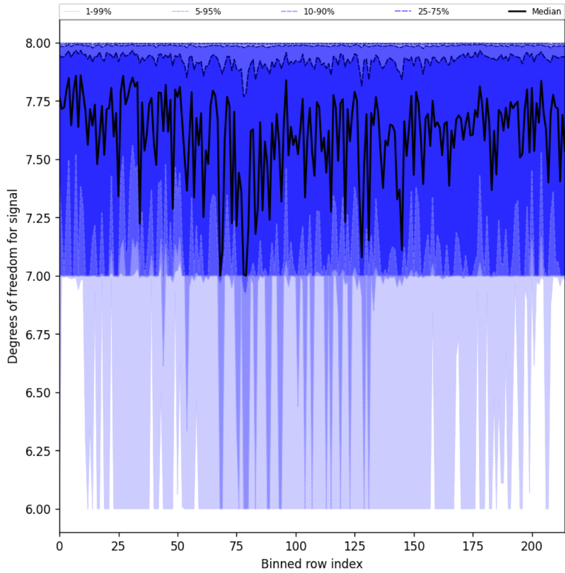
Figure 25: Along track statistics of “Degrees of freedom for signal” for 2025-06-15 to 2025-06-16
