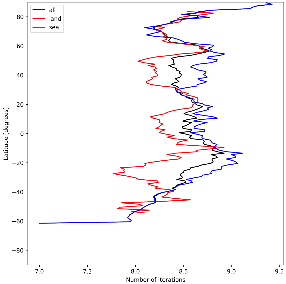
Figure 12: Zonal average of “Number of iterations” for 2025-06-15 to 2025-06-16.
