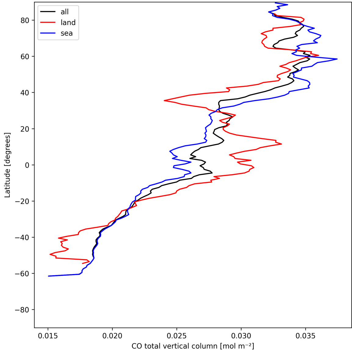
Figure 7: Zonal average of “CO total vertical column” for 2025-06-15 to 2025-06-16.
