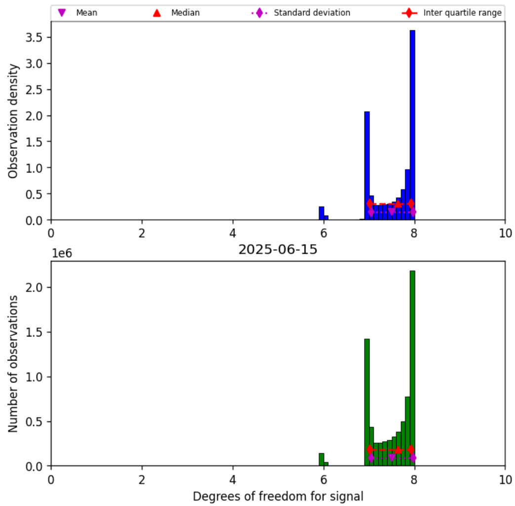
Figure 18: Histogram of “Degrees of freedom for signal” for 2025-06-15 to 2025-06-16
