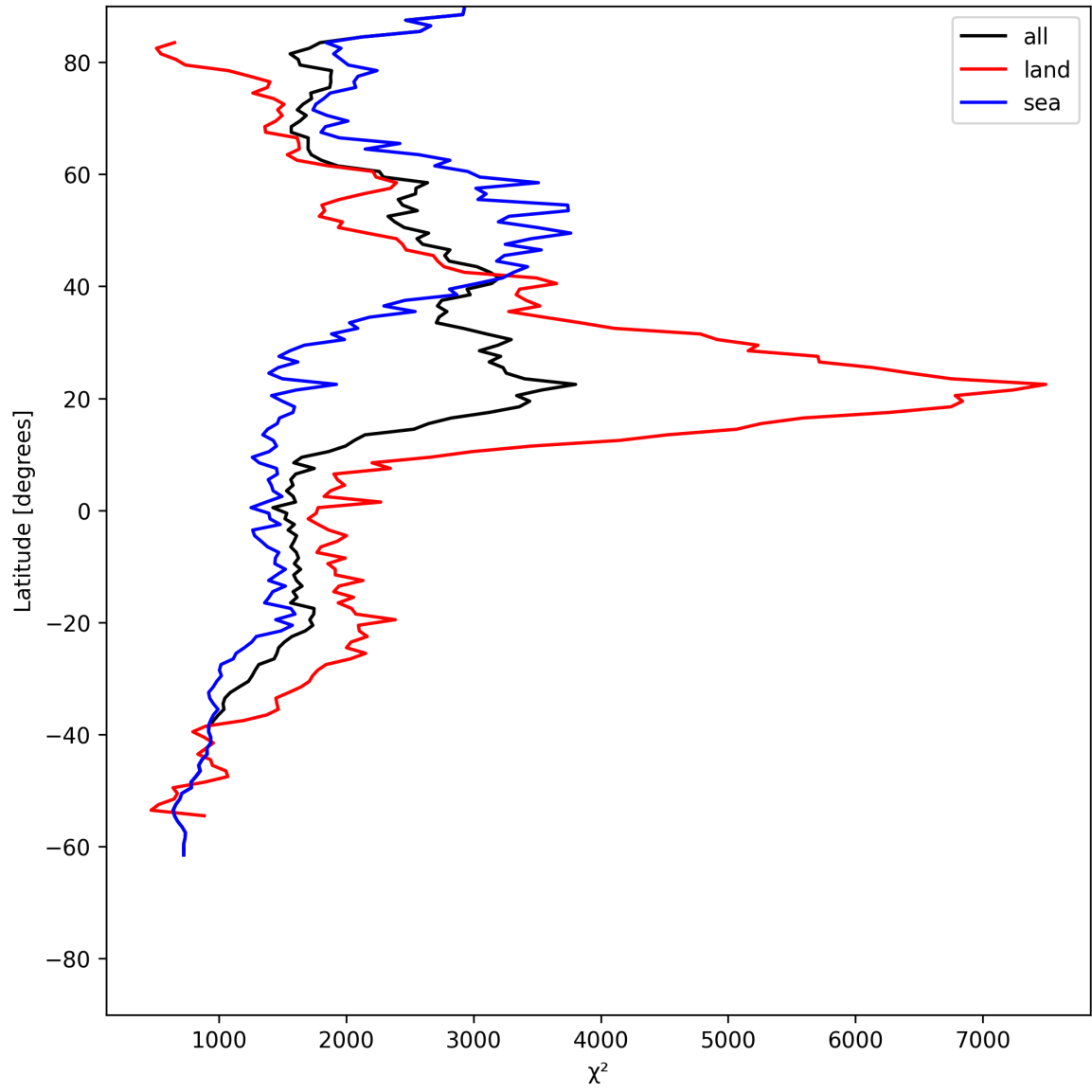
Figure 10: Zonal average of “ \chi^2 ” for 2025-06-15 to 2025-06-16.
