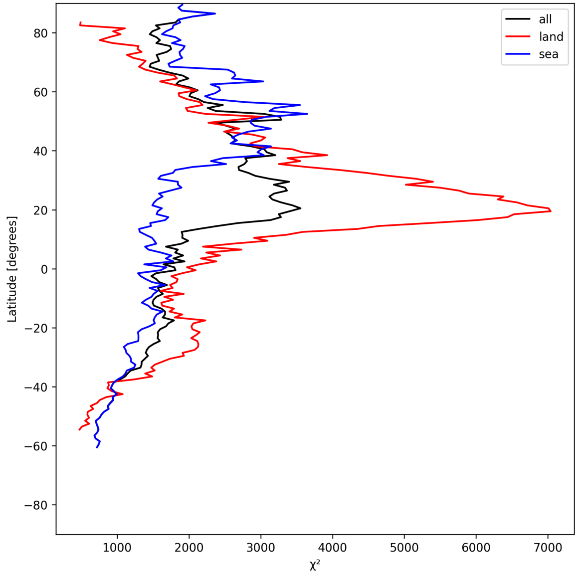
Figure 10: Zonal average of “ \chi^2 ” for 2025-06-16 to 2025-06-17.
