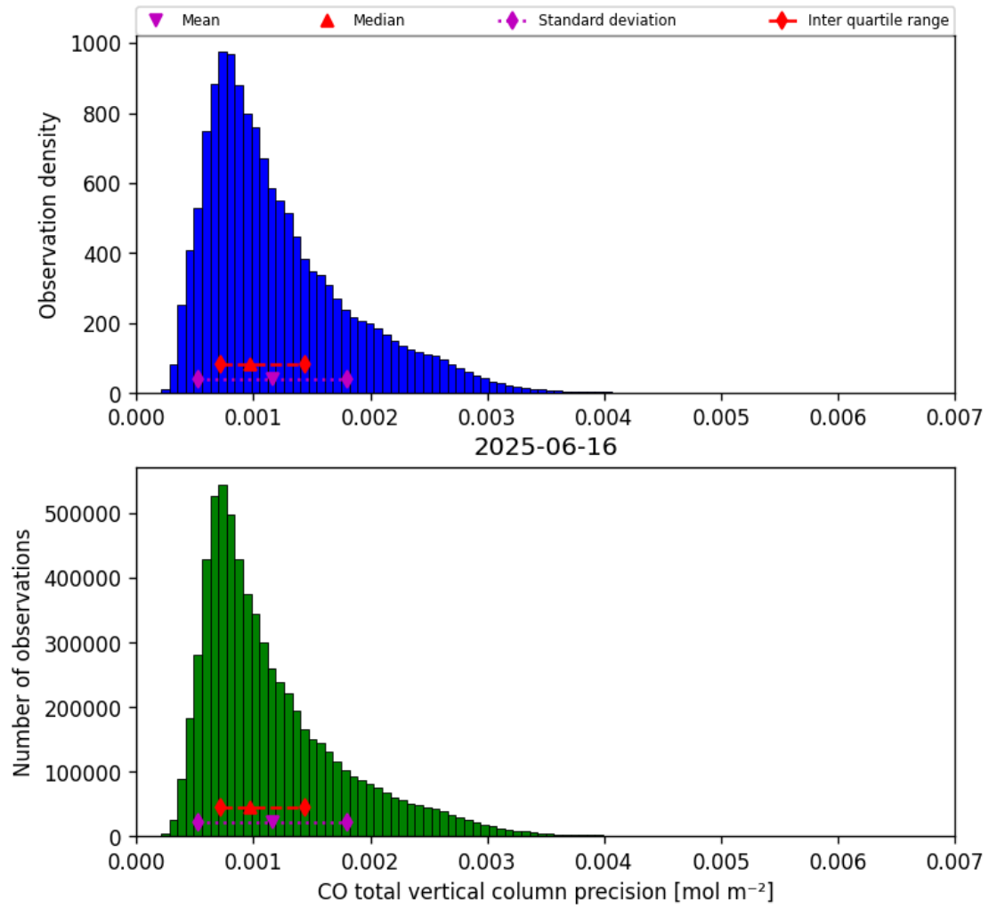
Figure 15: Histogram of “CO total vertical column precision” for 2025-06-16 to 2025-06-17
