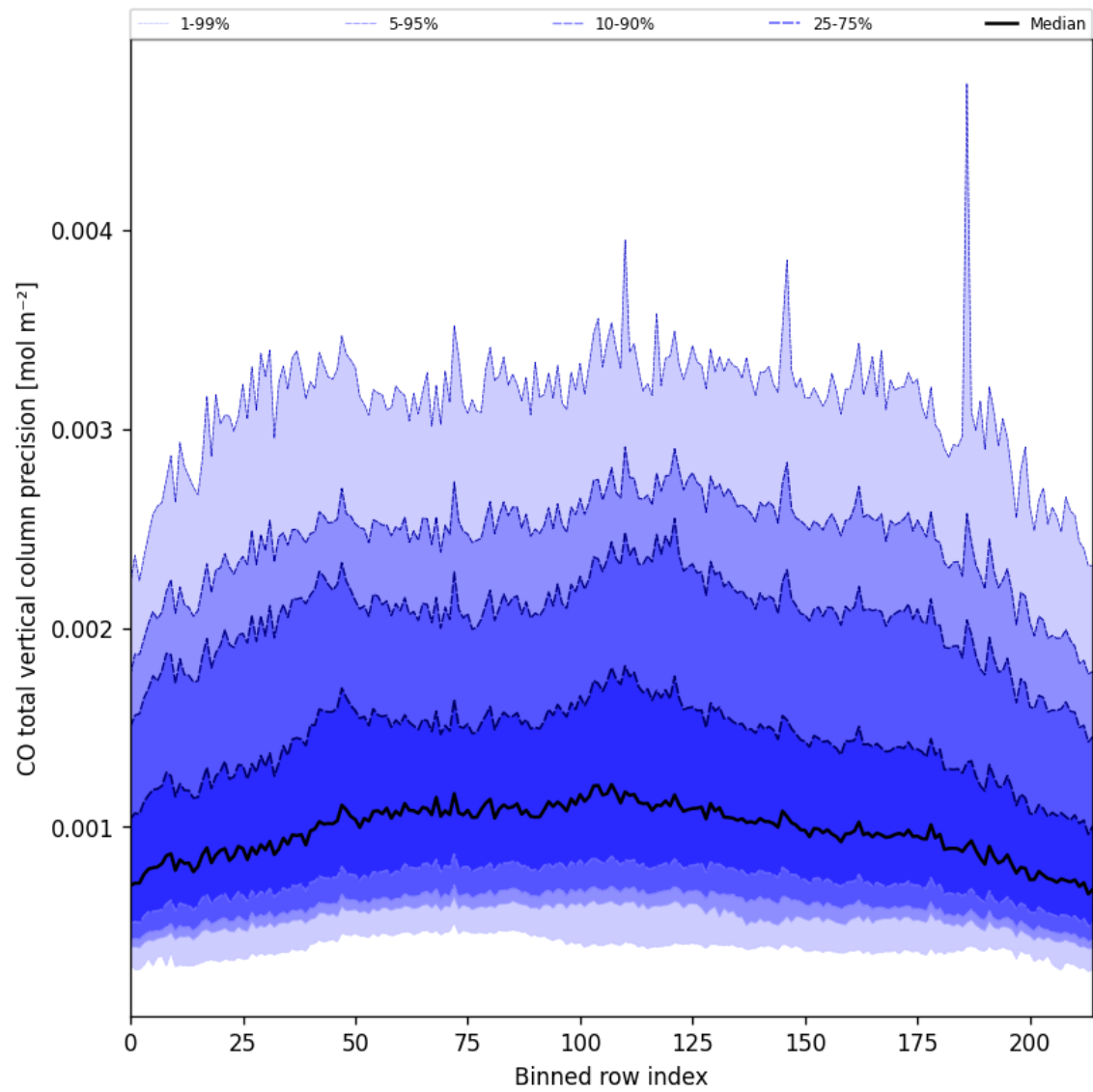
Figure 22: Along track statistics of “CO total vertical column precision” for 2025-06-16 to 2025-06-17
