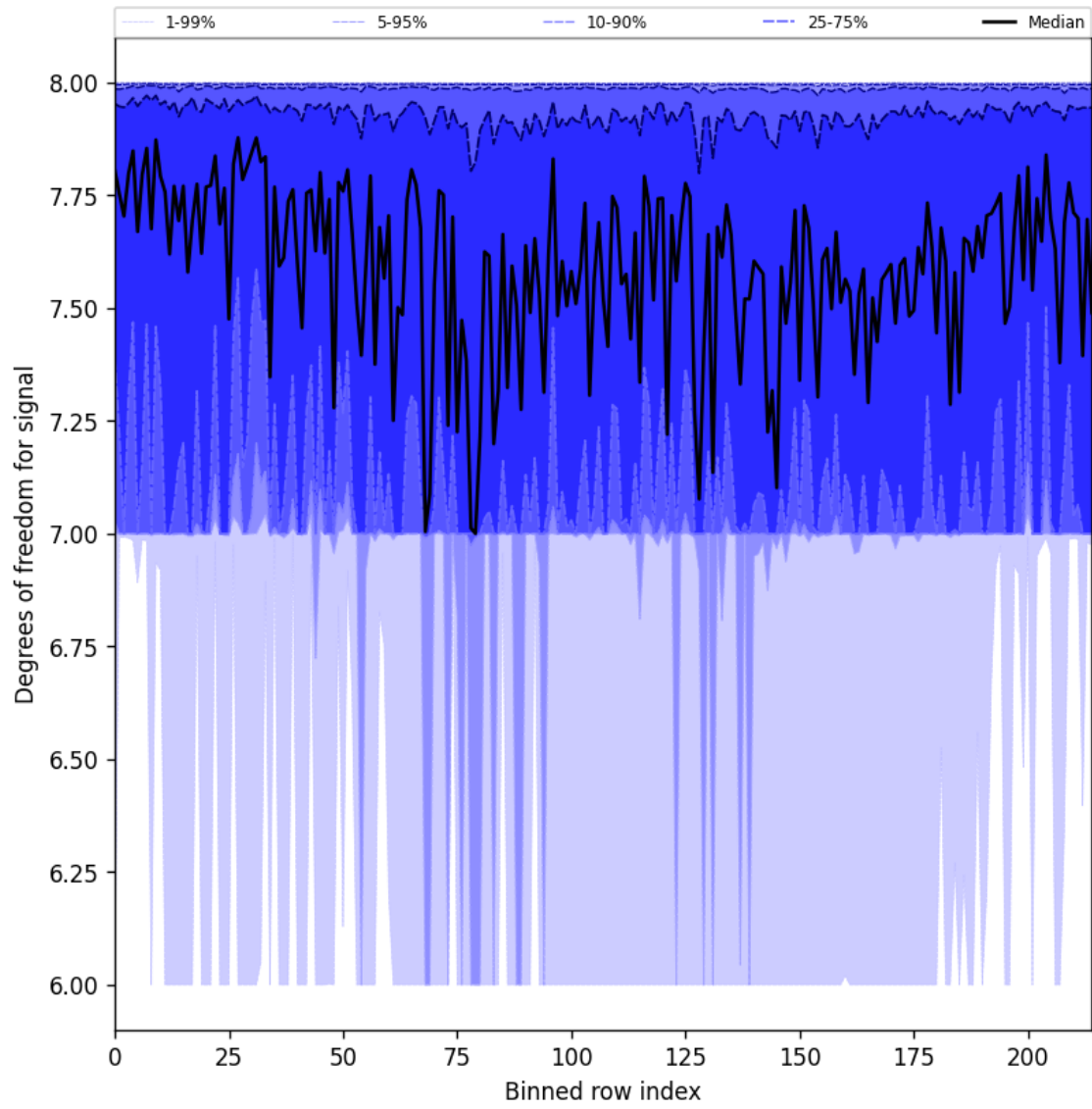
Figure 25: Along track statistics of “Degrees of freedom for signal” for 2025-06-16 to 2025-06-17
