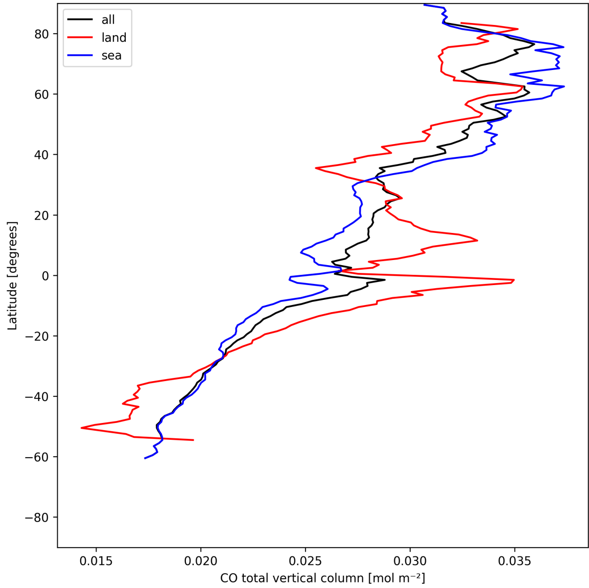
Figure 7: Zonal average of “CO total vertical column” for 2025-06-16 to 2025-06-17.
