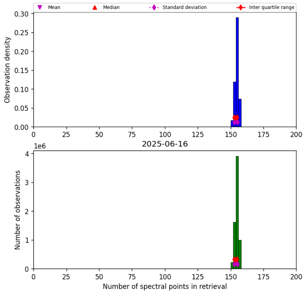
Figure 16: Histogram of “Number of spectral points in retrieval” for 2025-06-16 to 2025-06-17
