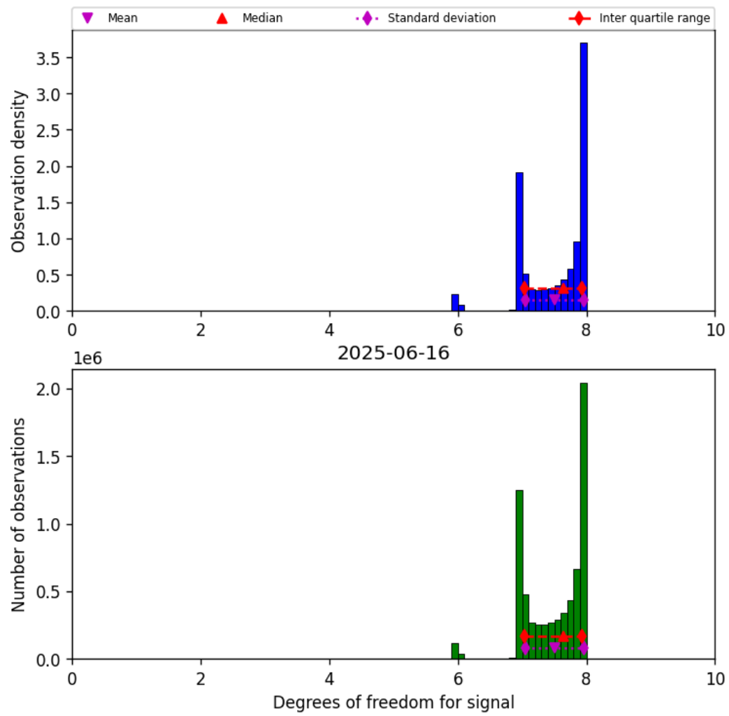
Figure 18: Histogram of “Degrees of freedom for signal” for 2025-06-16 to 2025-06-17
