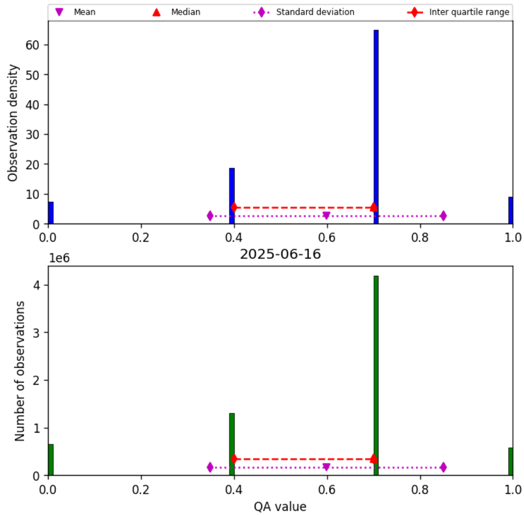
Figure 13: Histogram of “QA value” for 2025-06-16 to 2025-06-17
