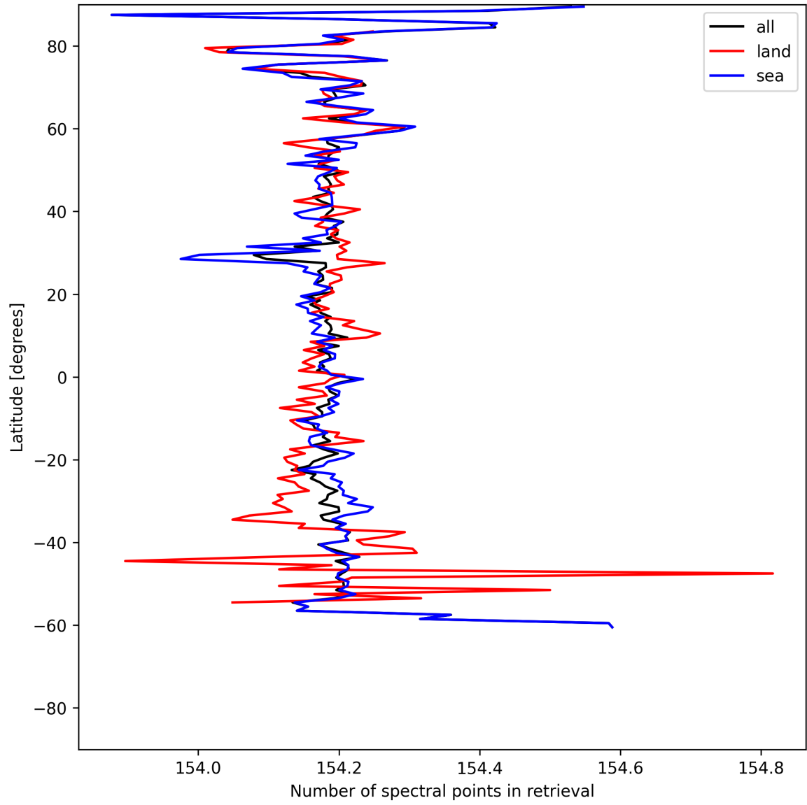
Figure 9: Zonal average of “Number of spectral points in retrieval” for 2025-06-16 to 2025-06-17.
