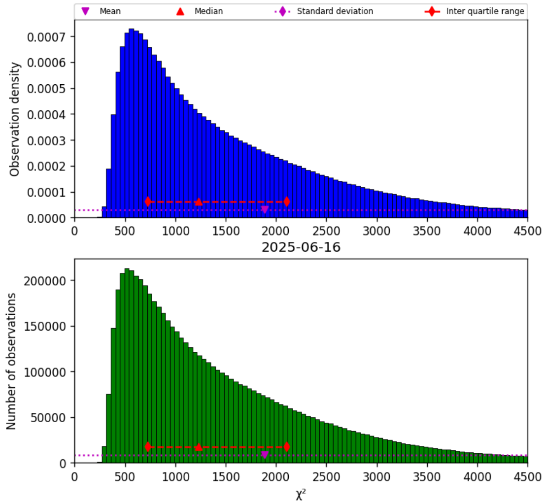
Figure 17: Histogram of “ \chi^2 ” for 2025-06-16 to 2025-06-17
