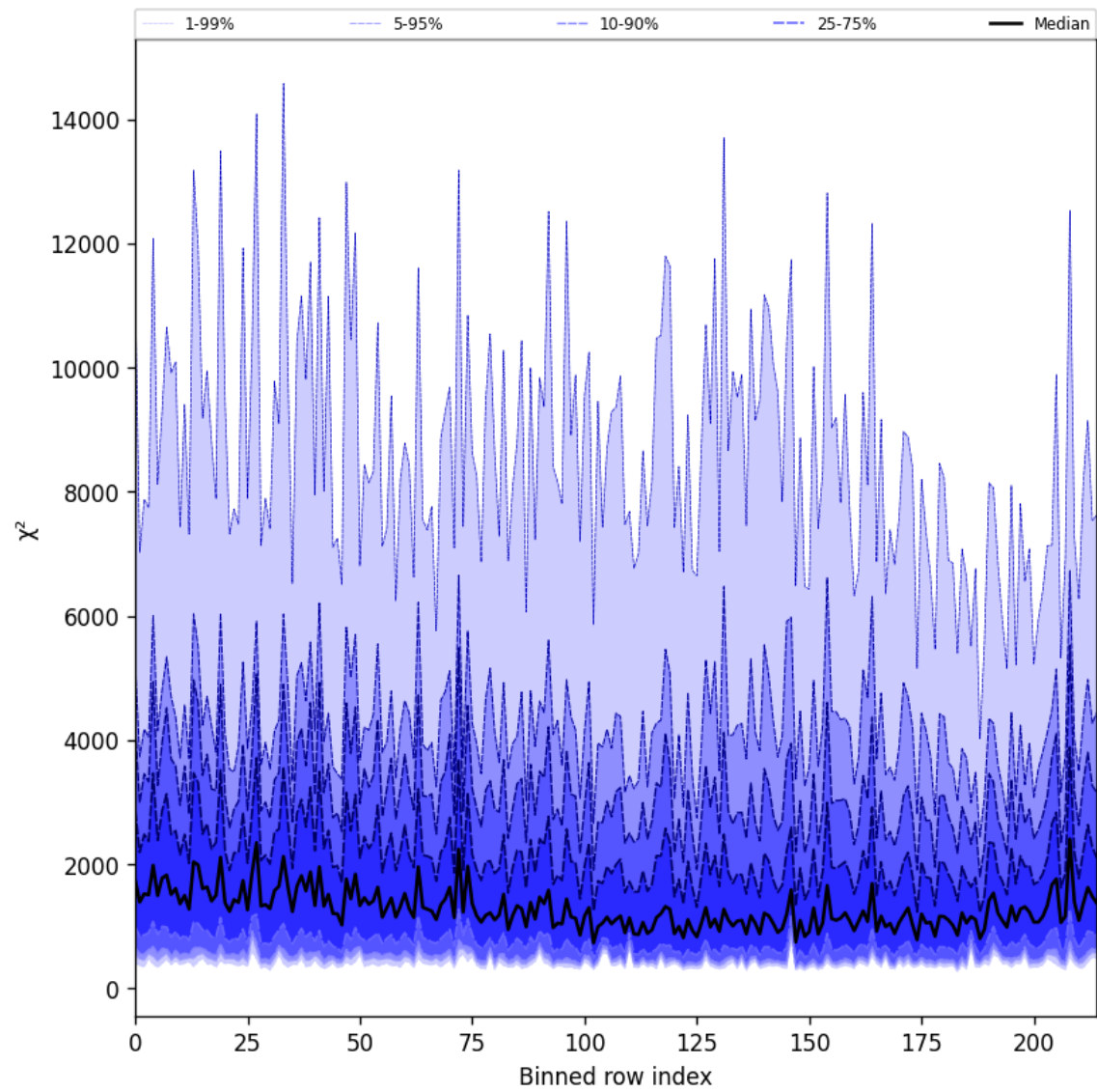
Figure 24: Along track statistics of “ \chi^2 ” for 2025-06-16 to 2025-06-17
