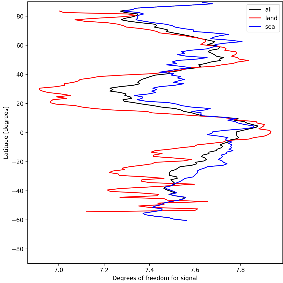
Figure 11: Zonal average of “Degrees of freedom for signal” for 2025-06-16 to 2025-06-17.
