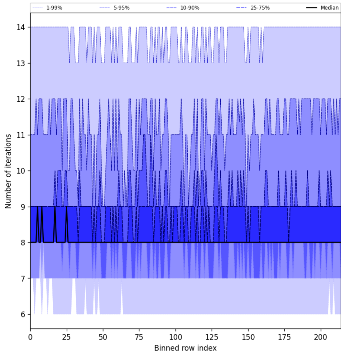
Figure 26: Along track statistics of “Number of iterations” for 2025-06-16 to 2025-06-17
