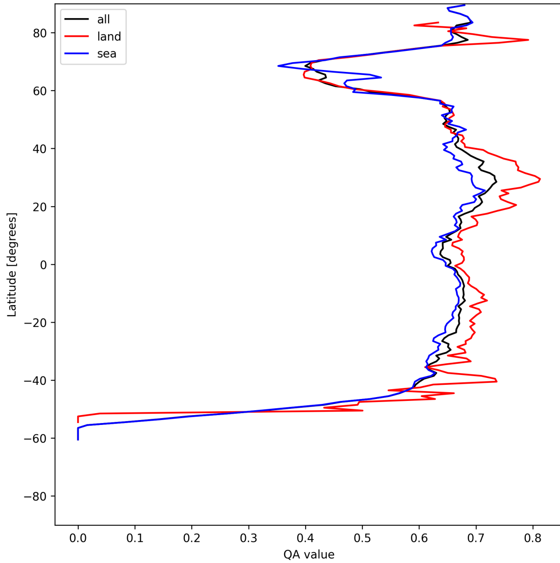
Figure 6: Zonal average of “QA value” for 2025-06-16 to 2025-06-17.
