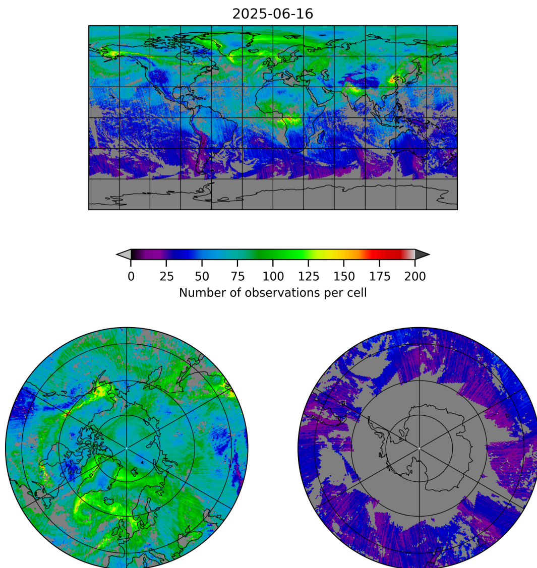
Figure 5: Map of the number of observations for 2025-06-16 to 2025-06-17
