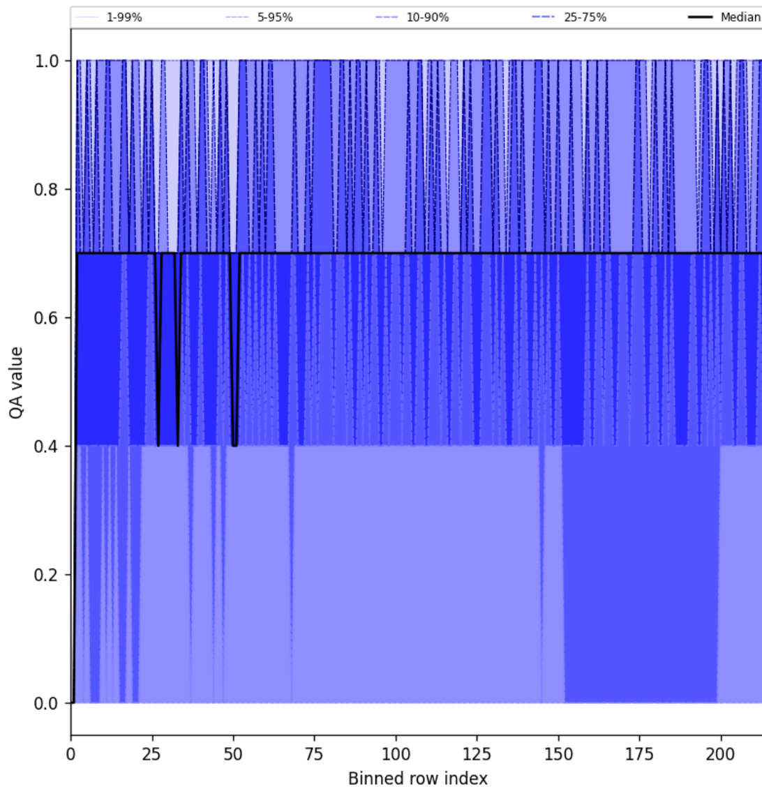
Figure 20: Along track statistics of “QA value” for 2025-06-16 to 2025-06-17
