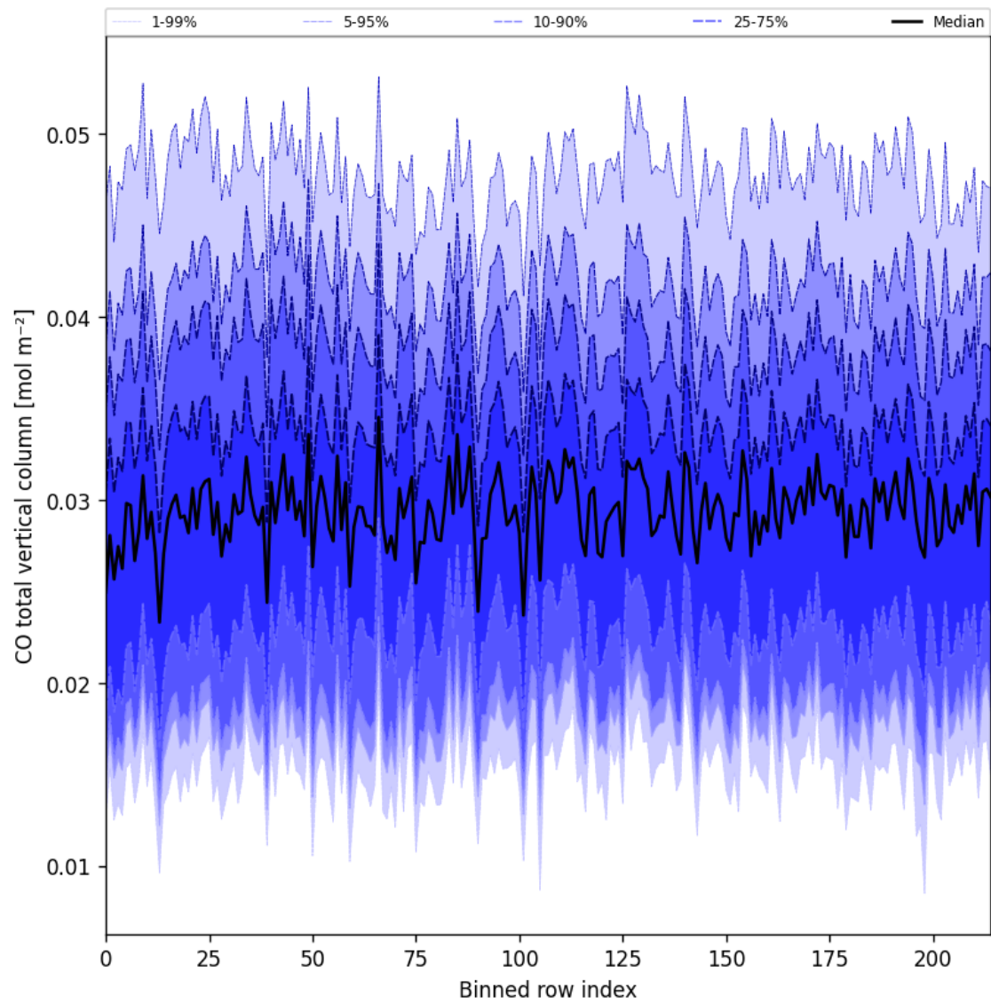
Figure 21: Along track statistics of “CO total vertical column” for 2025-06-16 to 2025-06-17
