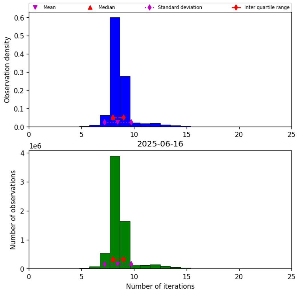
Figure 19: Histogram of “Number of iterations” for 2025-06-16 to 2025-06-17
