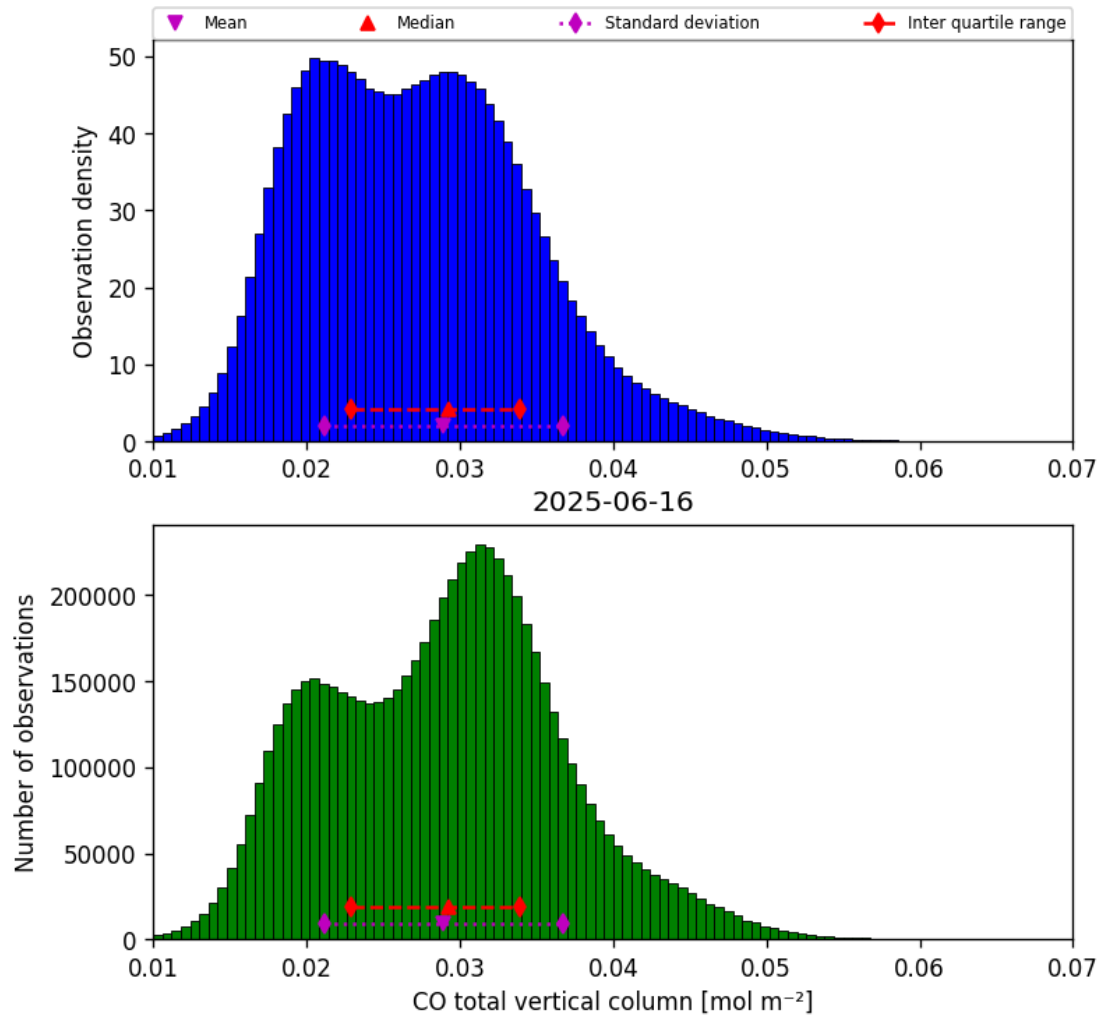
Figure 14: Histogram of “CO total vertical column” for 2025-06-16 to 2025-06-17
