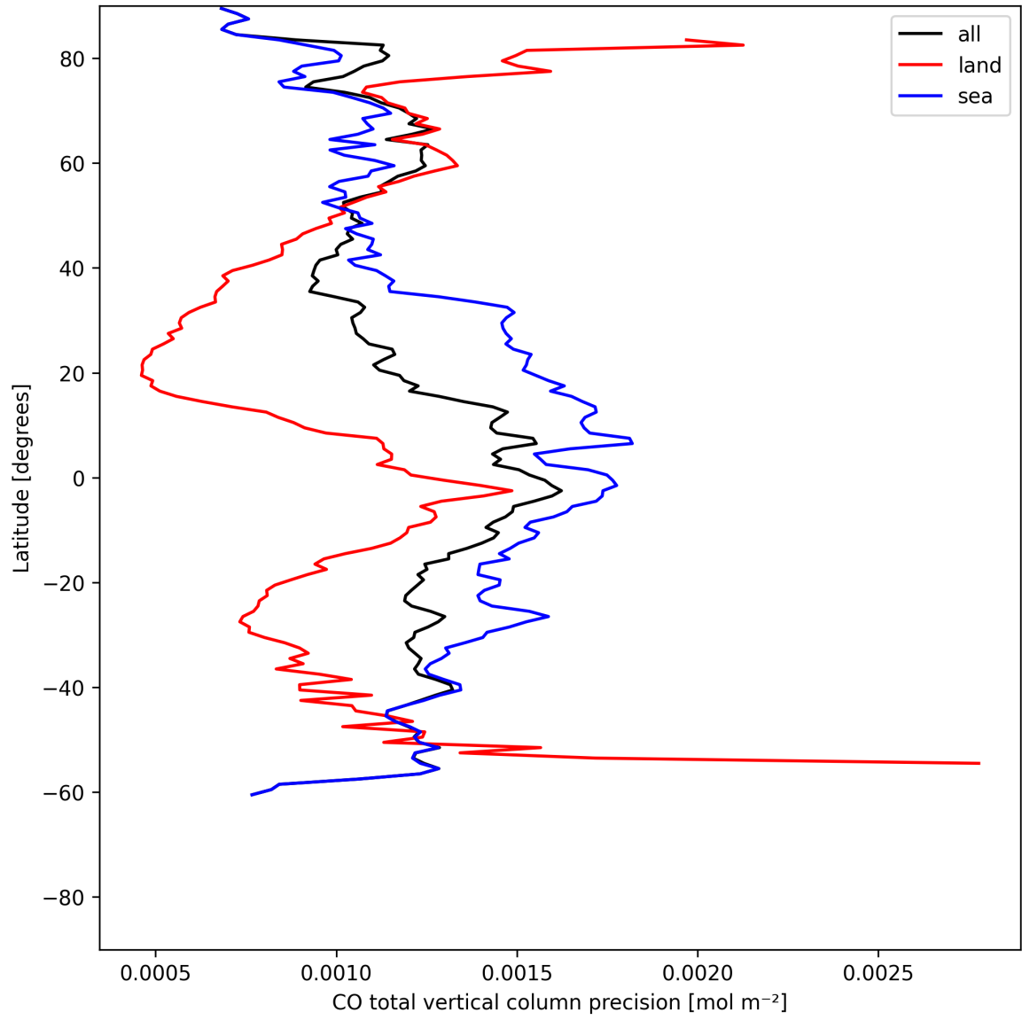
Figure 8: Zonal average of “CO total vertical column precision” for 2025-06-16 to 2025-06-17.
