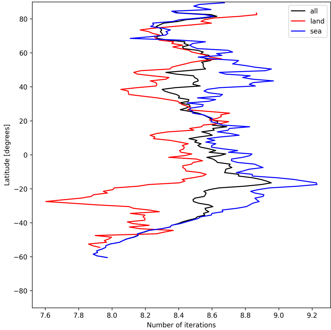
Figure 12: Zonal average of “Number of iterations” for 2025-06-16 to 2025-06-17.
