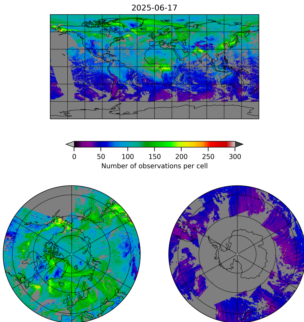
Figure 5: Map of the number of observations for 2025-06-17 to 2025-06-17
