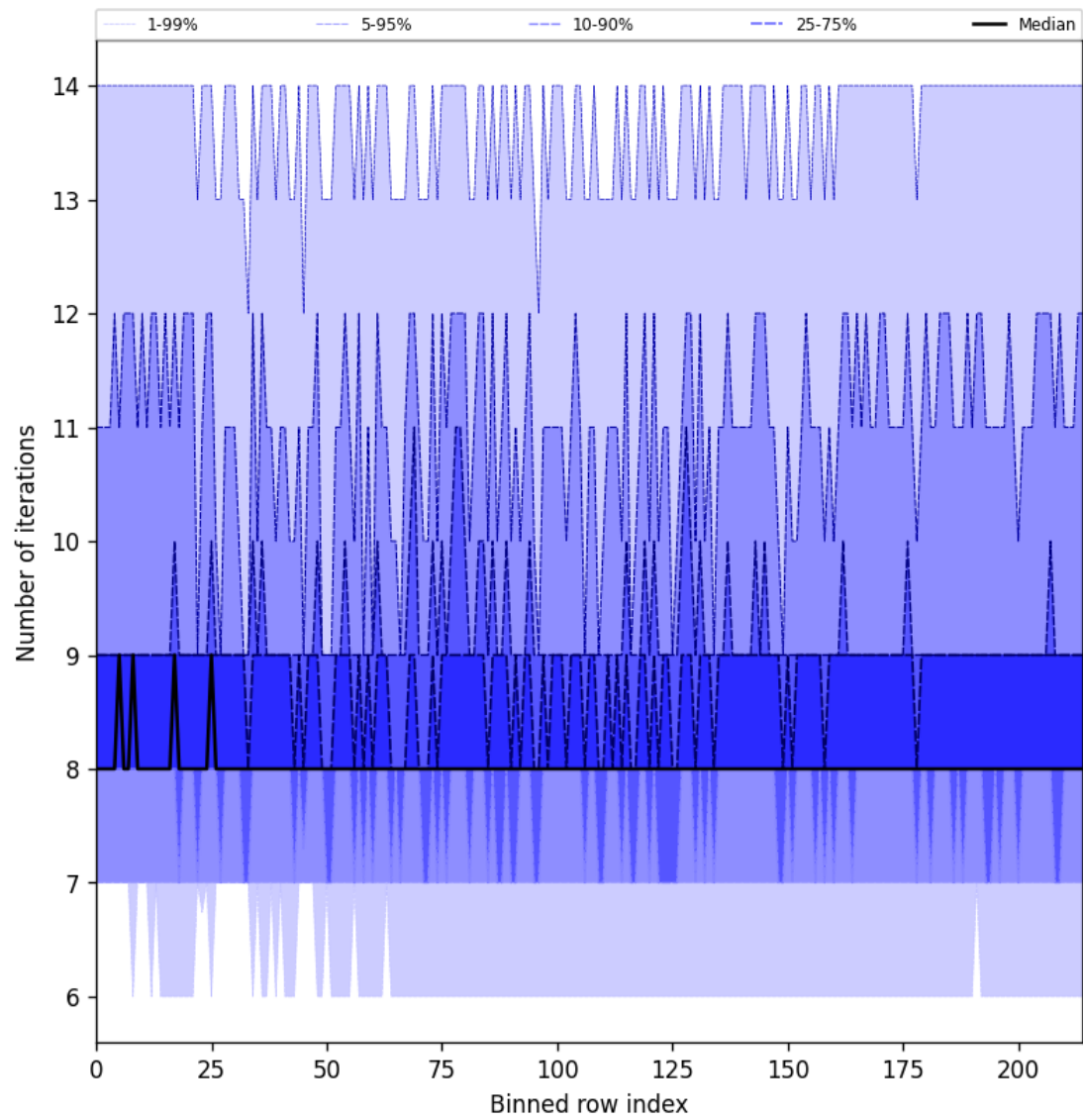
Figure 26: Along track statistics of “Number of iterations” for 2025-06-17 to 2025-06-17
