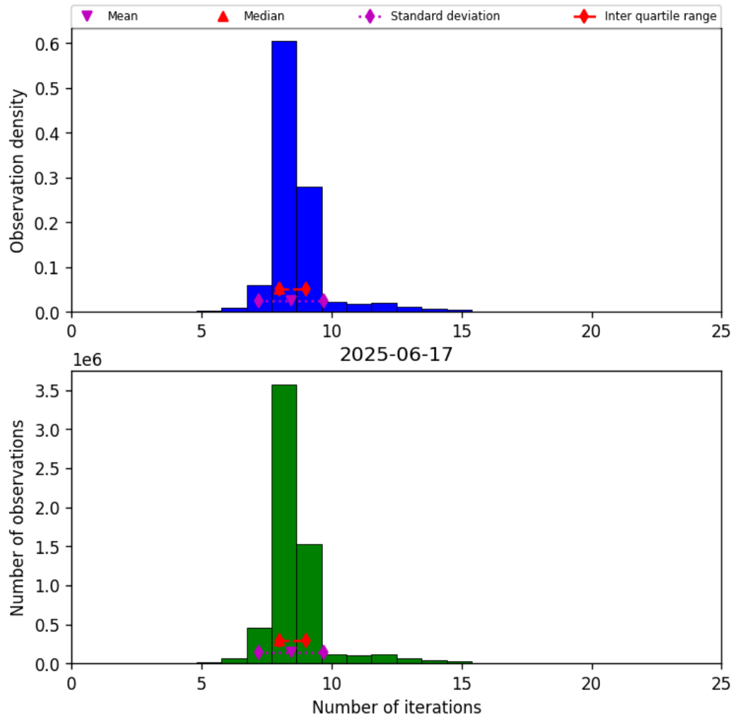
Figure 19: Histogram of “Number of iterations” for 2025-06-17 to 2025-06-17
