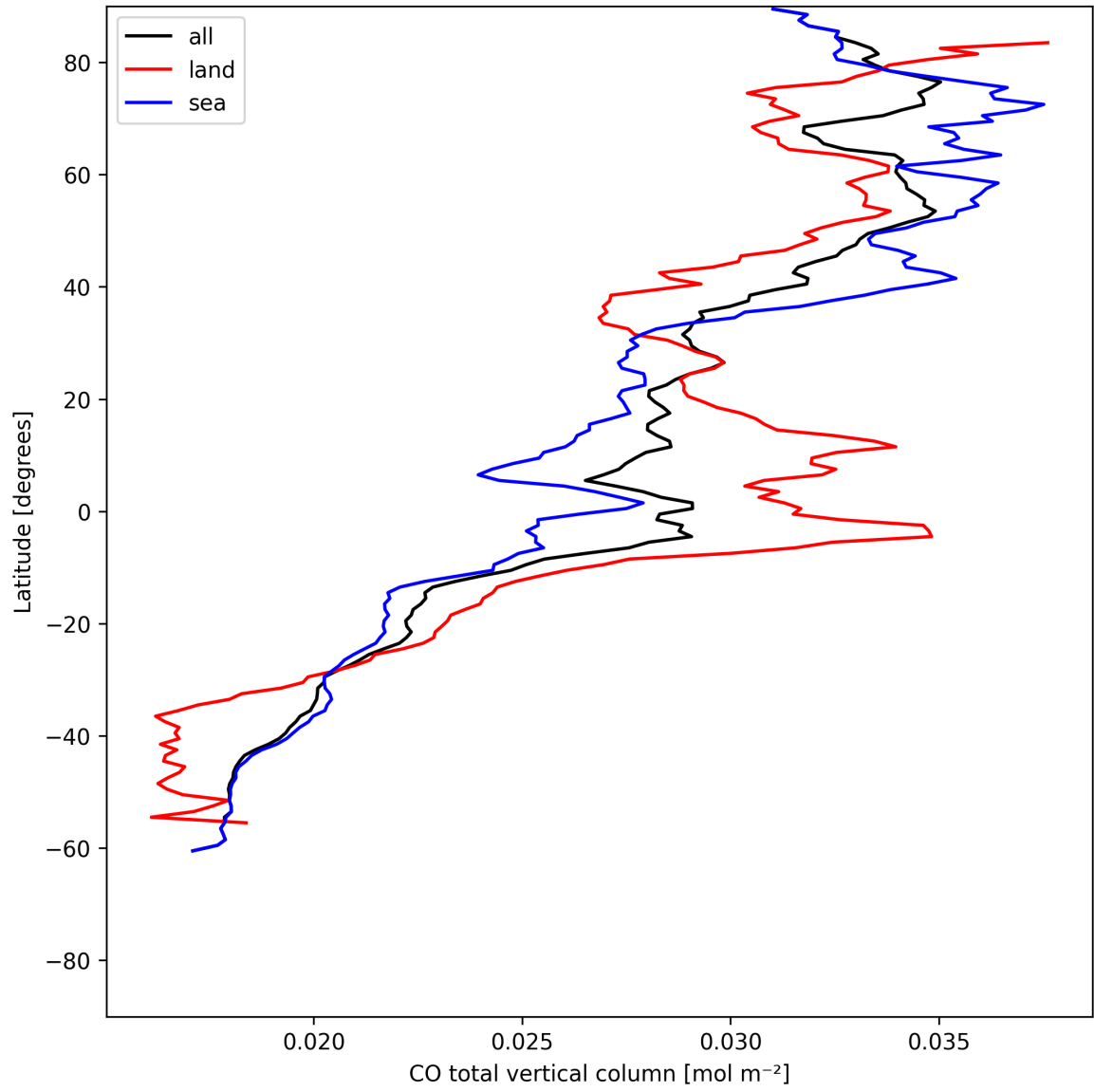
Figure 7: Zonal average of “CO total vertical column” for 2025-06-17 to 2025-06-17.
