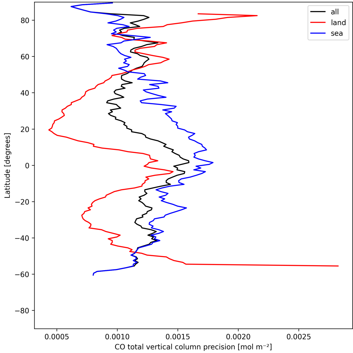
Figure 8: Zonal average of “CO total vertical column precision” for 2025-06-17 to 2025-06-17.
