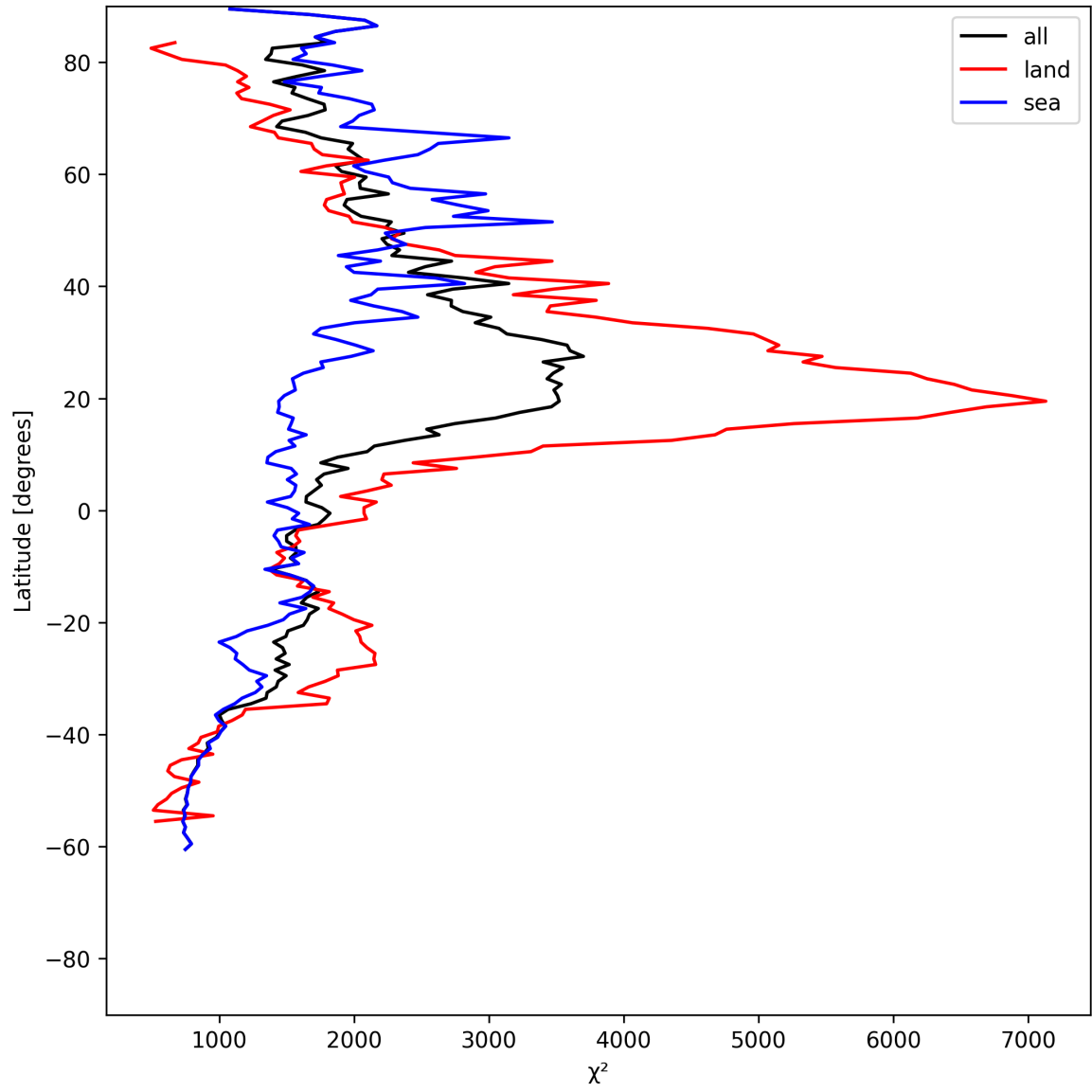
Figure 10: Zonal average of “ \chi^2 ” for 2025-06-17 to 2025-06-17.
