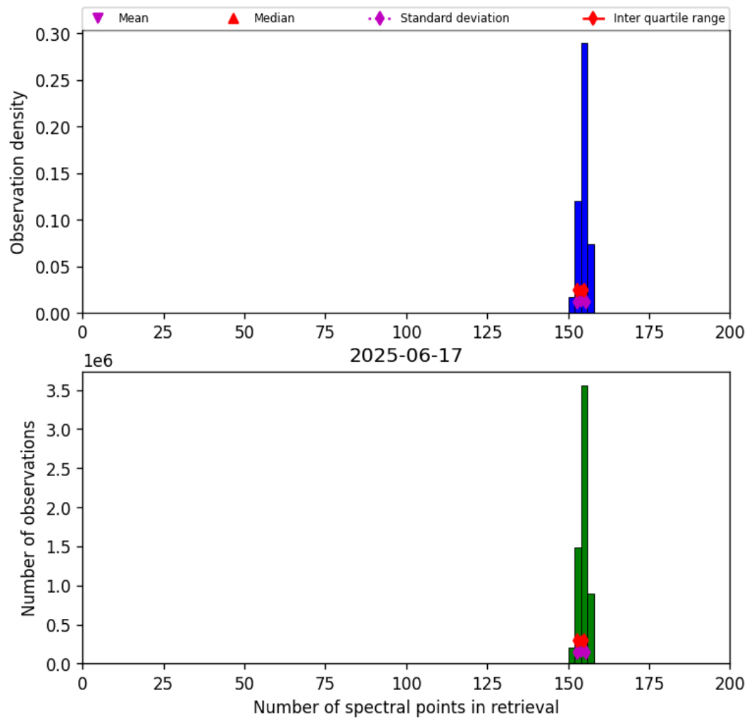
Figure 16: Histogram of “Number of spectral points in retrieval” for 2025-06-17 to 2025-06-17
