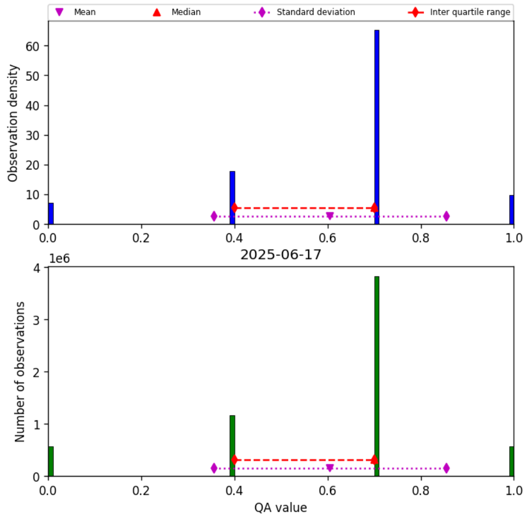
Figure 13: Histogram of “QA value” for 2025-06-17 to 2025-06-17
