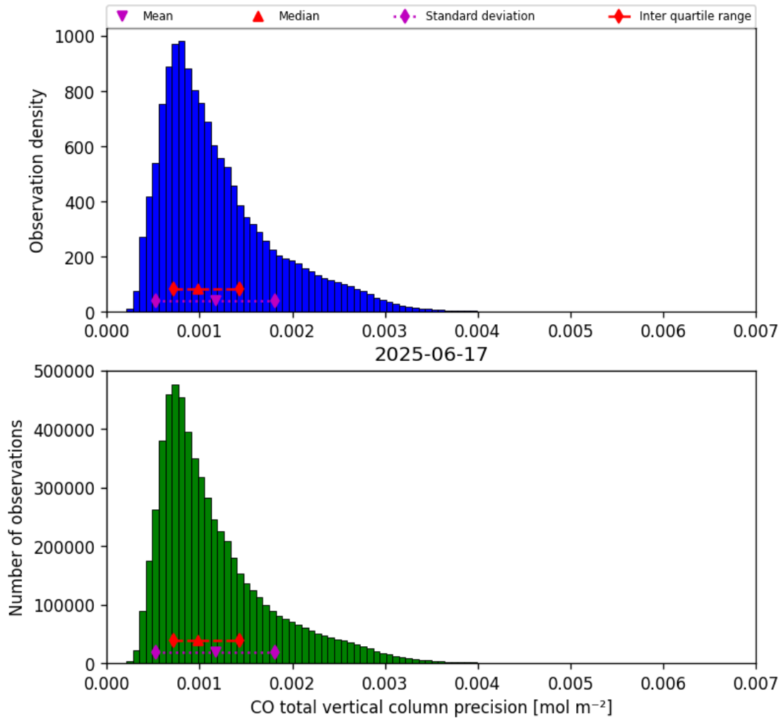
Figure 15: Histogram of “CO total vertical column precision” for 2025-06-17 to 2025-06-17
