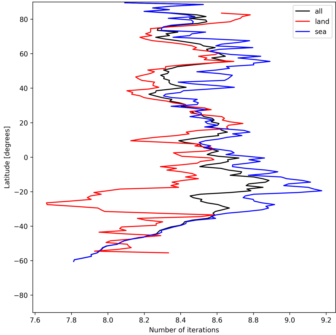
Figure 12: Zonal average of “Number of iterations” for 2025-06-17 to 2025-06-17.
