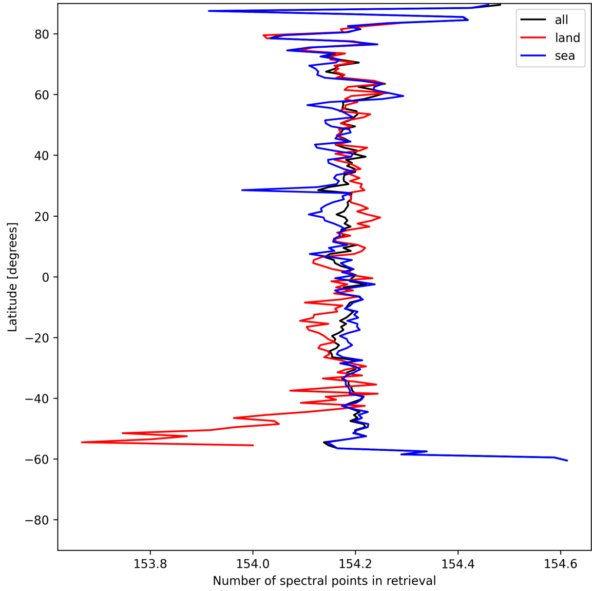
Figure 9: Zonal average of “Number of spectral points in retrieval” for 2025-06-17 to 2025-06-17.
