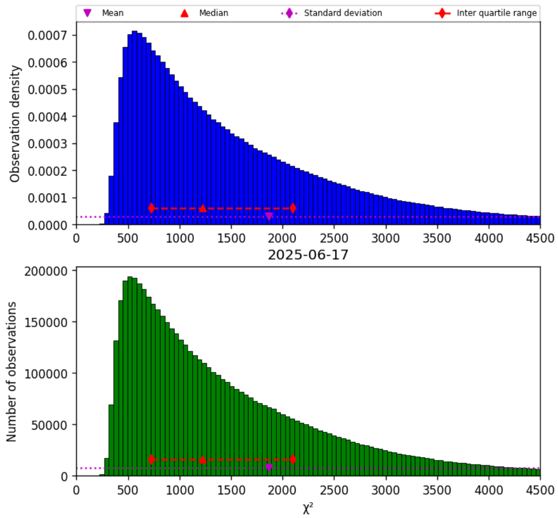
Figure 17: Histogram of " \chi^2 " for 2025-06-17 to 2025-06-17
