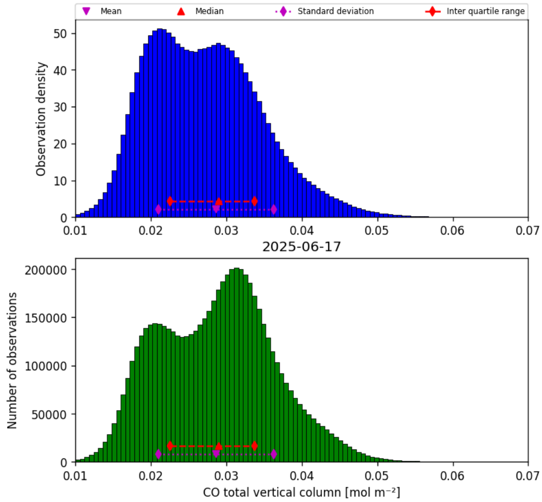
Figure 14: Histogram of “CO total vertical column” for 2025-06-17 to 2025-06-17
