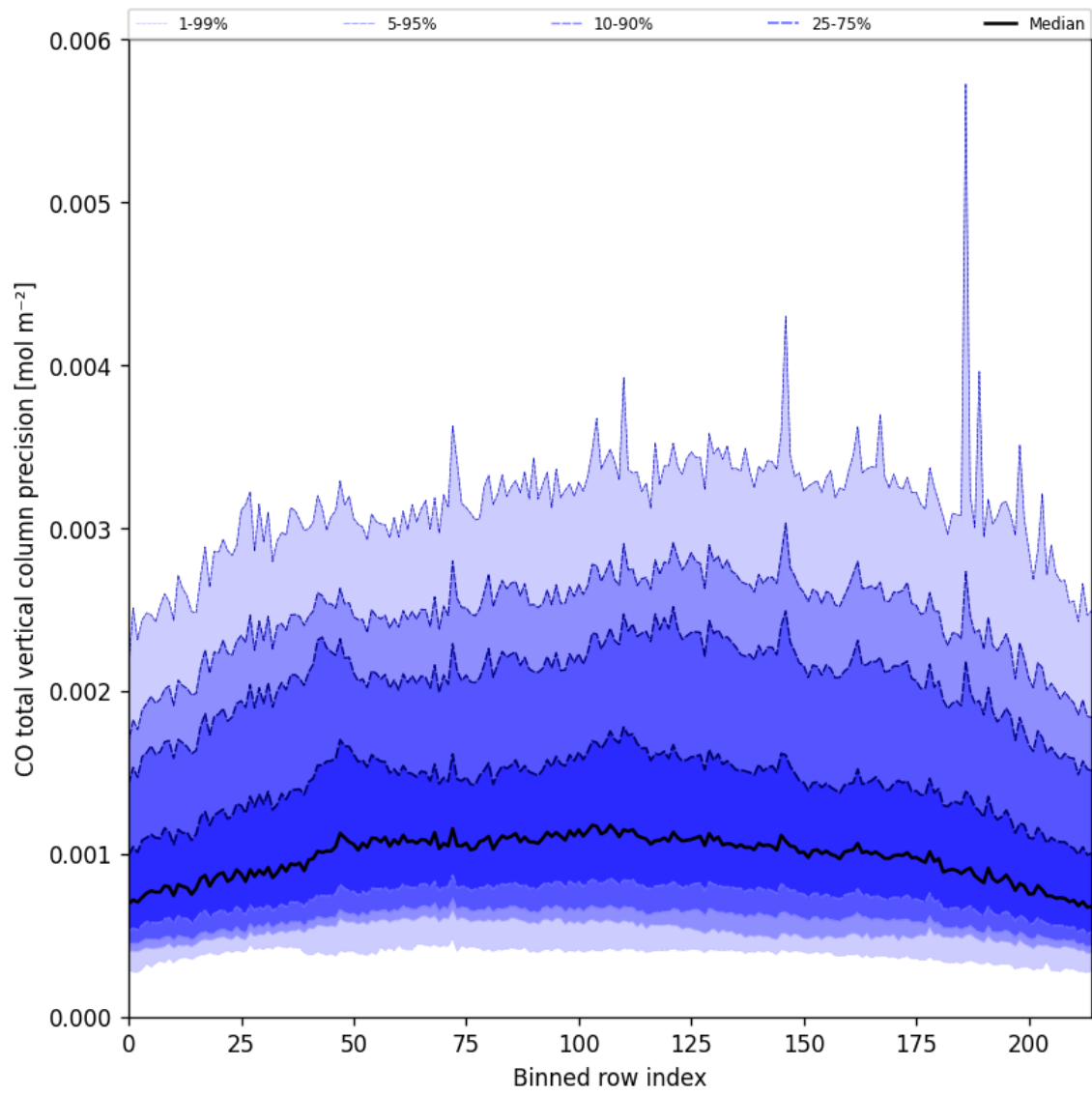
Figure 22: Along track statistics of “CO total vertical column precision” for 2025-06-17 to 2025-06-17
