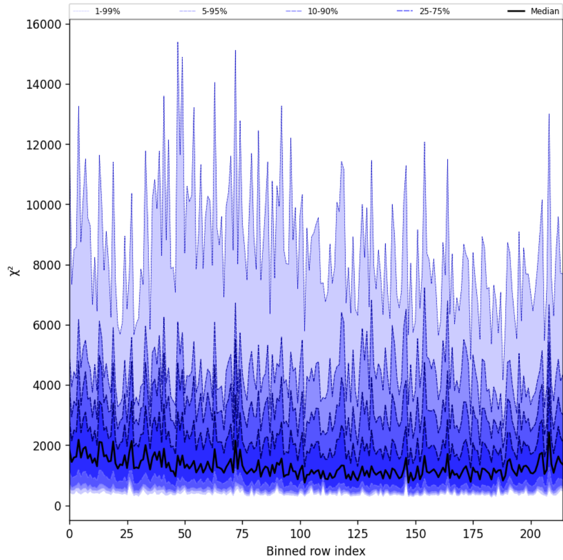
Figure 24: Along track statistics of “ \chi^2 ” for 2025-06-17 to 2025-06-17
