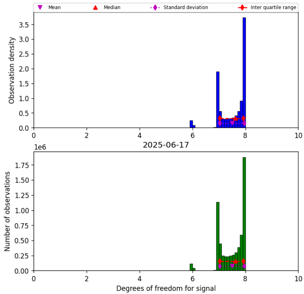
Figure 18: Histogram of “Degrees of freedom for signal” for 2025-06-17 to 2025-06-17
