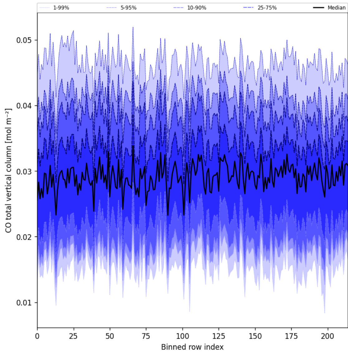
Figure 21: Along track statistics of “CO total vertical column” for 2025-06-17 to 2025-06-17
