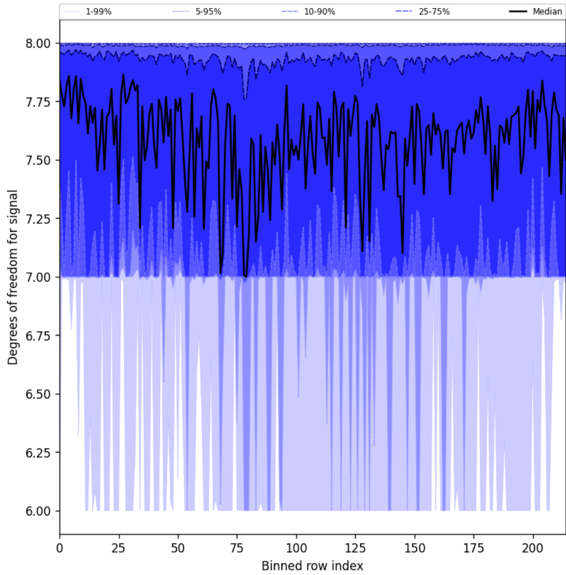
Figure 25: Along track statistics of “Degrees of freedom for signal” for 2025-06-17 to 2025-06-17
