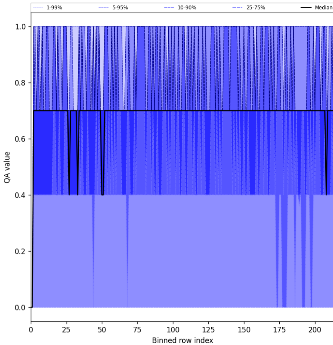
Figure 20: Along track statistics of “QA value” for 2025-06-17 to 2025-06-17
