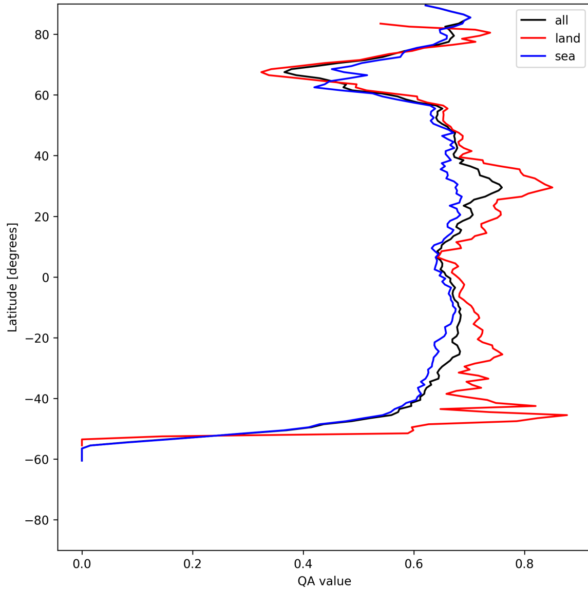
Figure 6: Zonal average of “QA value” for 2025-06-17 to 2025-06-17.
