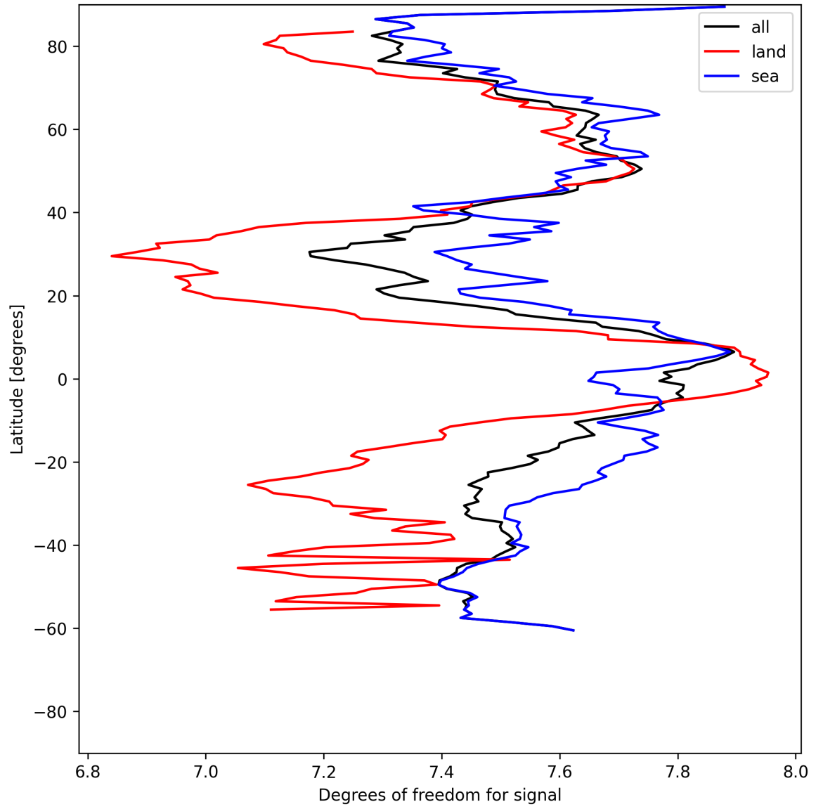
Figure 11: Zonal average of “Degrees of freedom for signal” for 2025-06-17 to 2025-06-17.
