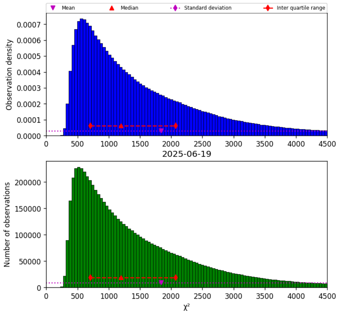
Figure 17: Histogram of “ \chi^2 ” for 2025-06-19 to 2025-06-20
