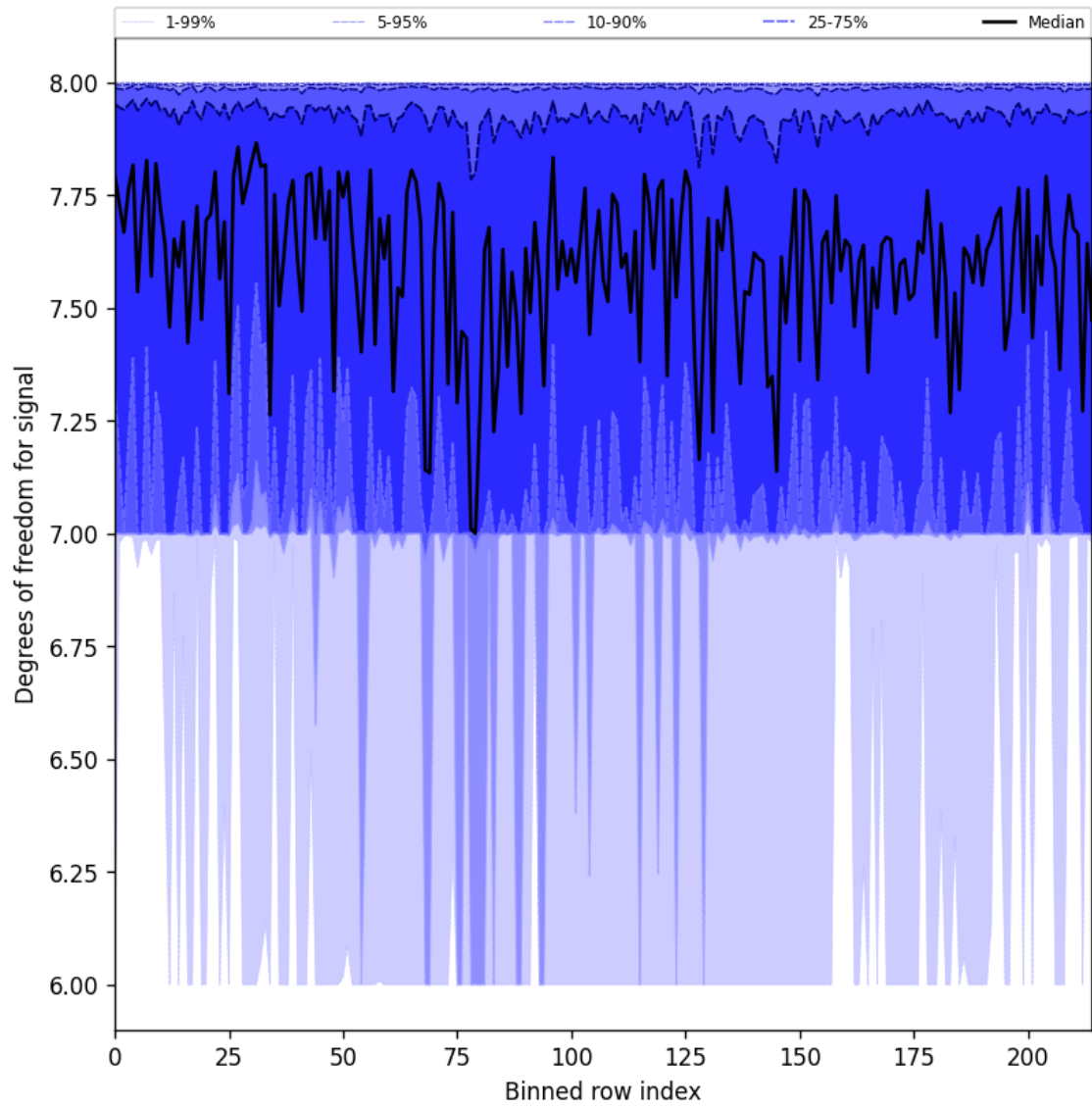
Figure 25: Along track statistics of “Degrees of freedom for signal” for 2025-06-19 to 2025-06-20
