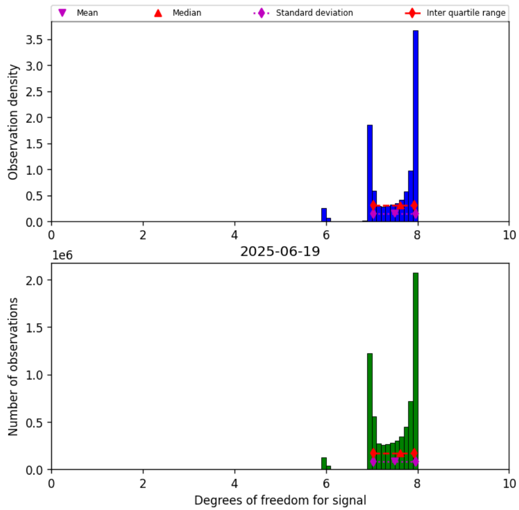
Figure 18: Histogram of “Degrees of freedom for signal” for 2025-06-19 to 2025-06-20
