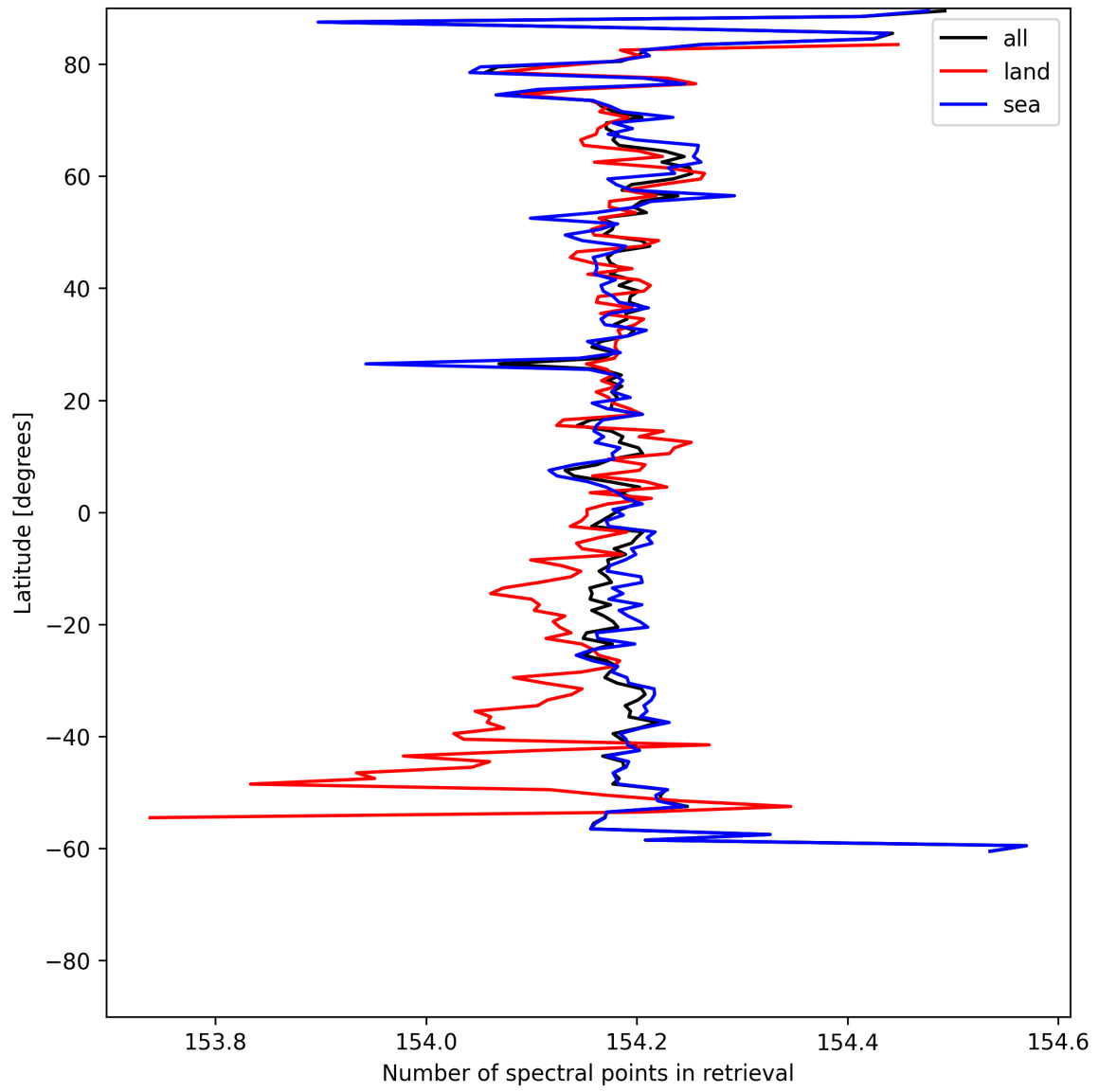
Figure 9: Zonal average of “Number of spectral points in retrieval” for 2025-06-19 to 2025-06-20.
