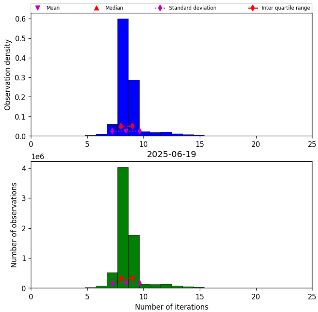
Figure 19: Histogram of “Number of iterations” for 2025-06-19 to 2025-06-20
