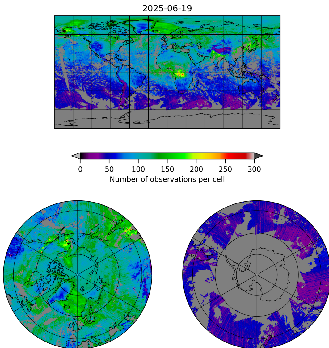
Figure 5: Map of the number of observations for 2025-06-19 to 2025-06-20
