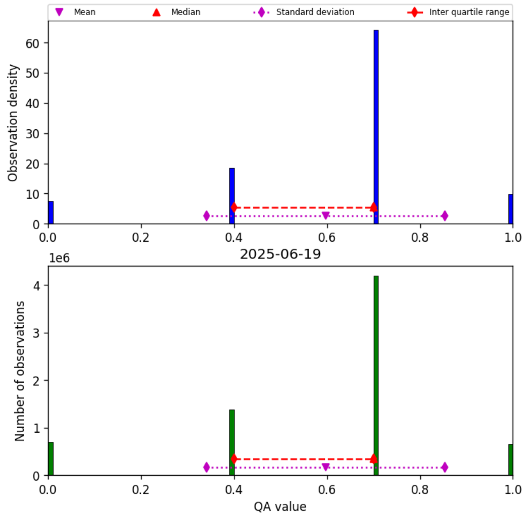
Figure 13: Histogram of “QA value” for 2025-06-19 to 2025-06-20
