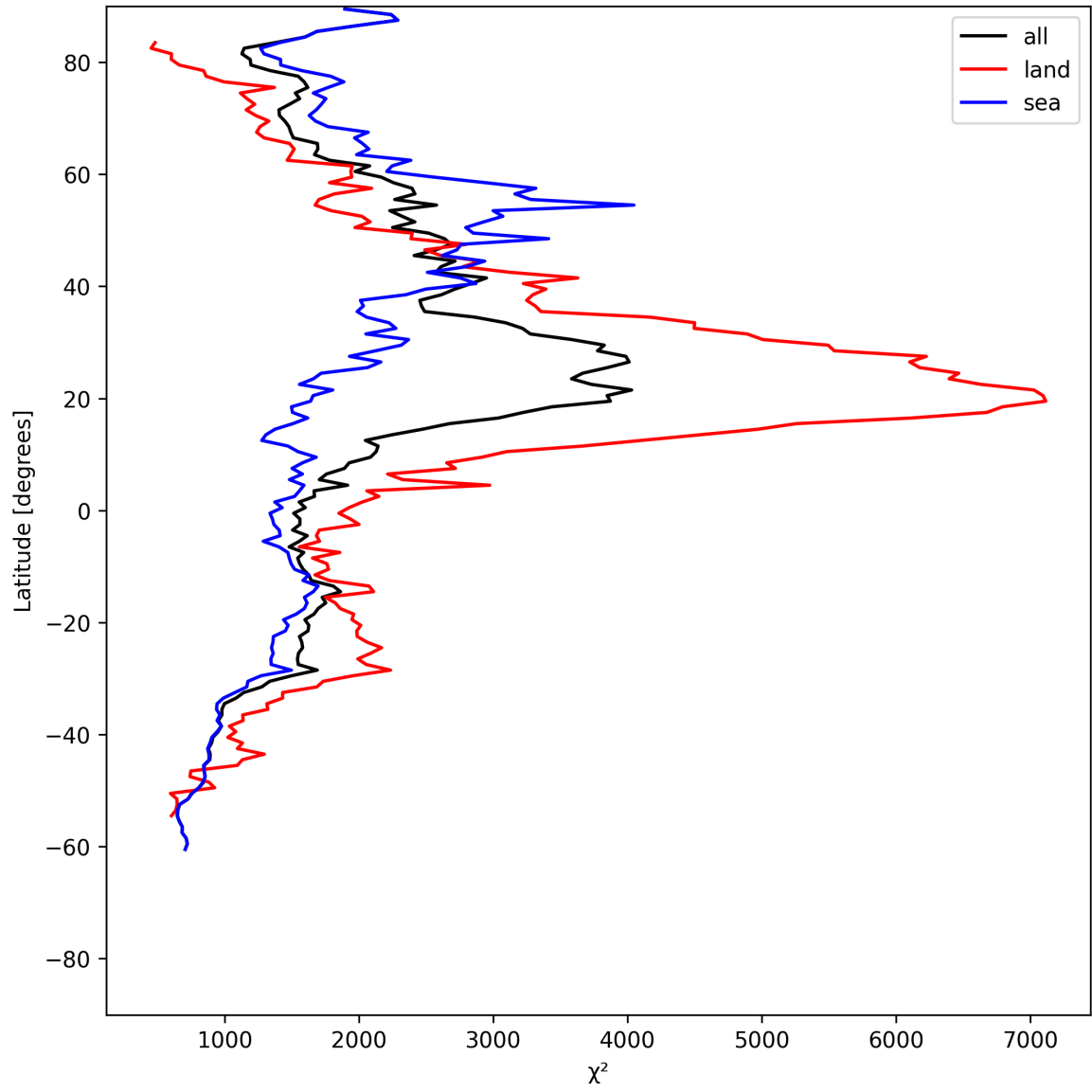
Figure 10: Zonal average of “ \chi^2 ” for 2025-06-19 to 2025-06-20.
