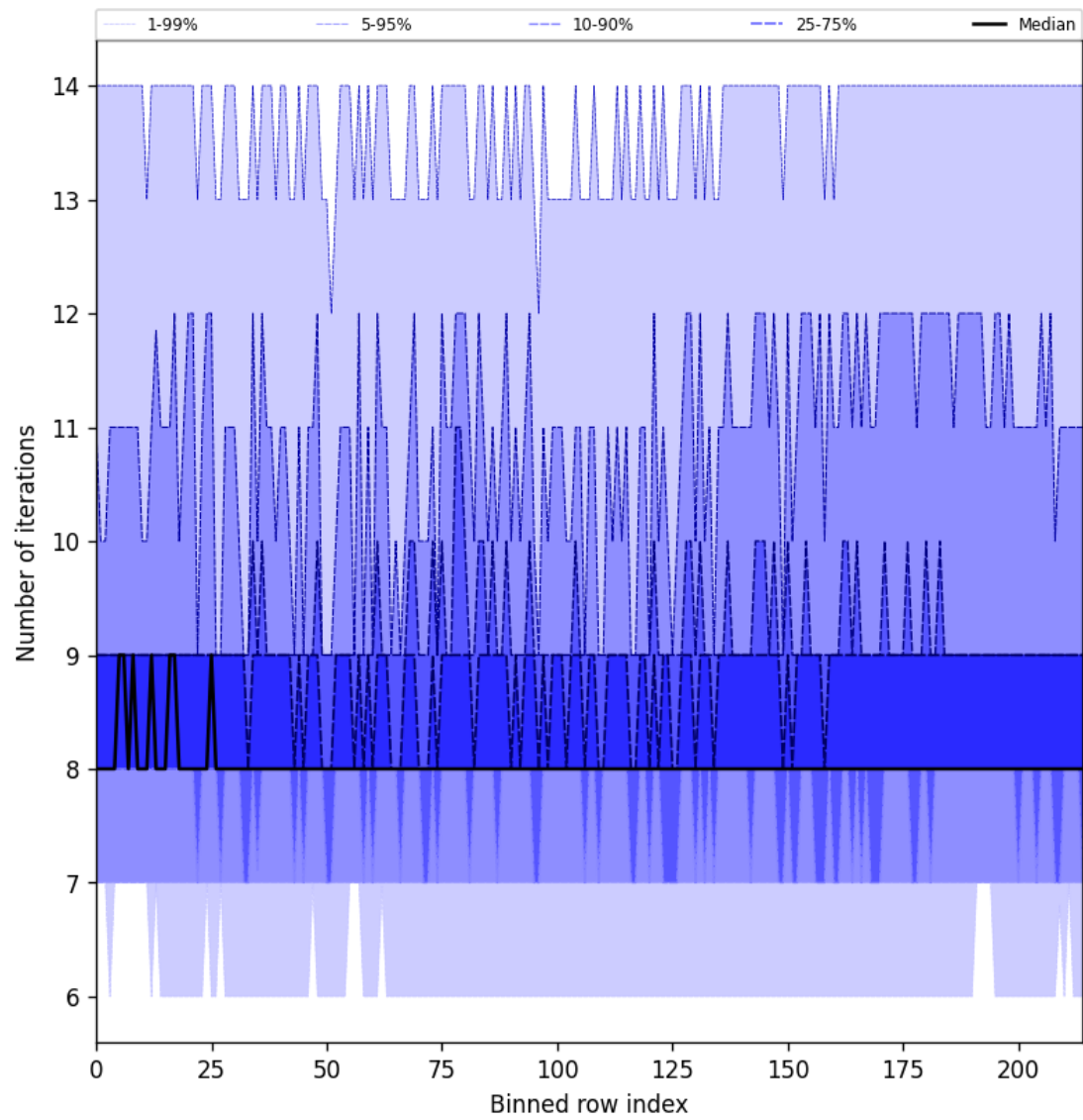
Figure 26: Along track statistics of “Number of iterations” for 2025-06-19 to 2025-06-20
