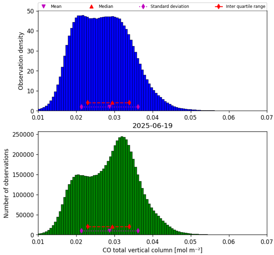
Figure 14: Histogram of “CO total vertical column” for 2025-06-19 to 2025-06-20
