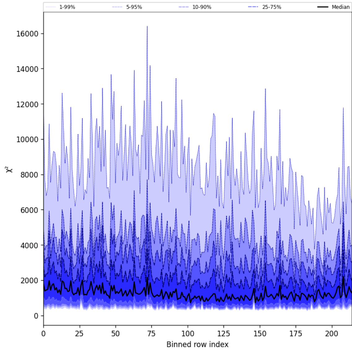
Figure 24: Along track statistics of “ \chi^2 ” for 2025-06-19 to 2025-06-20
