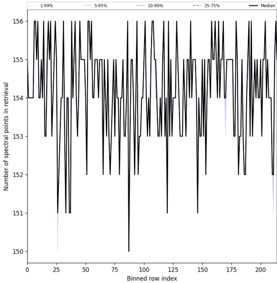
Figure 23: Along track statistics of “Number of spectral points in retrieval” for 2025-06-19 to 2025-06-20
