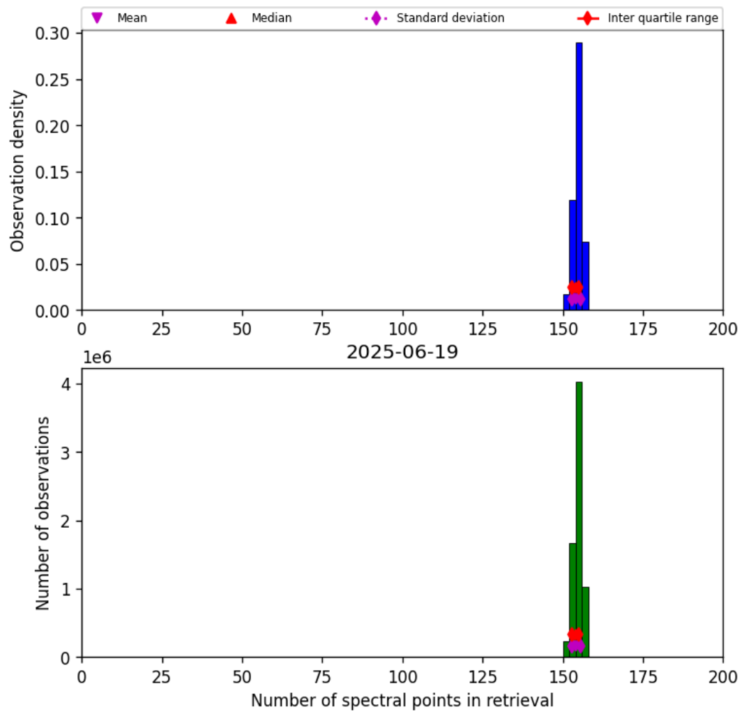
Figure 16: Histogram of “Number of spectral points in retrieval” for 2025-06-19 to 2025-06-20
