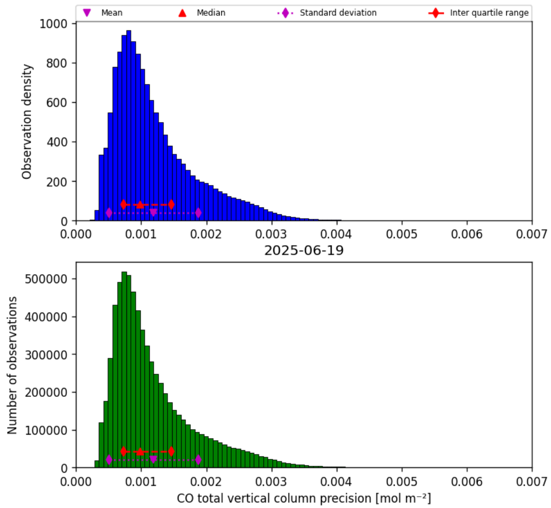
Figure 15: Histogram of “CO total vertical column precision” for 2025-06-19 to 2025-06-20
