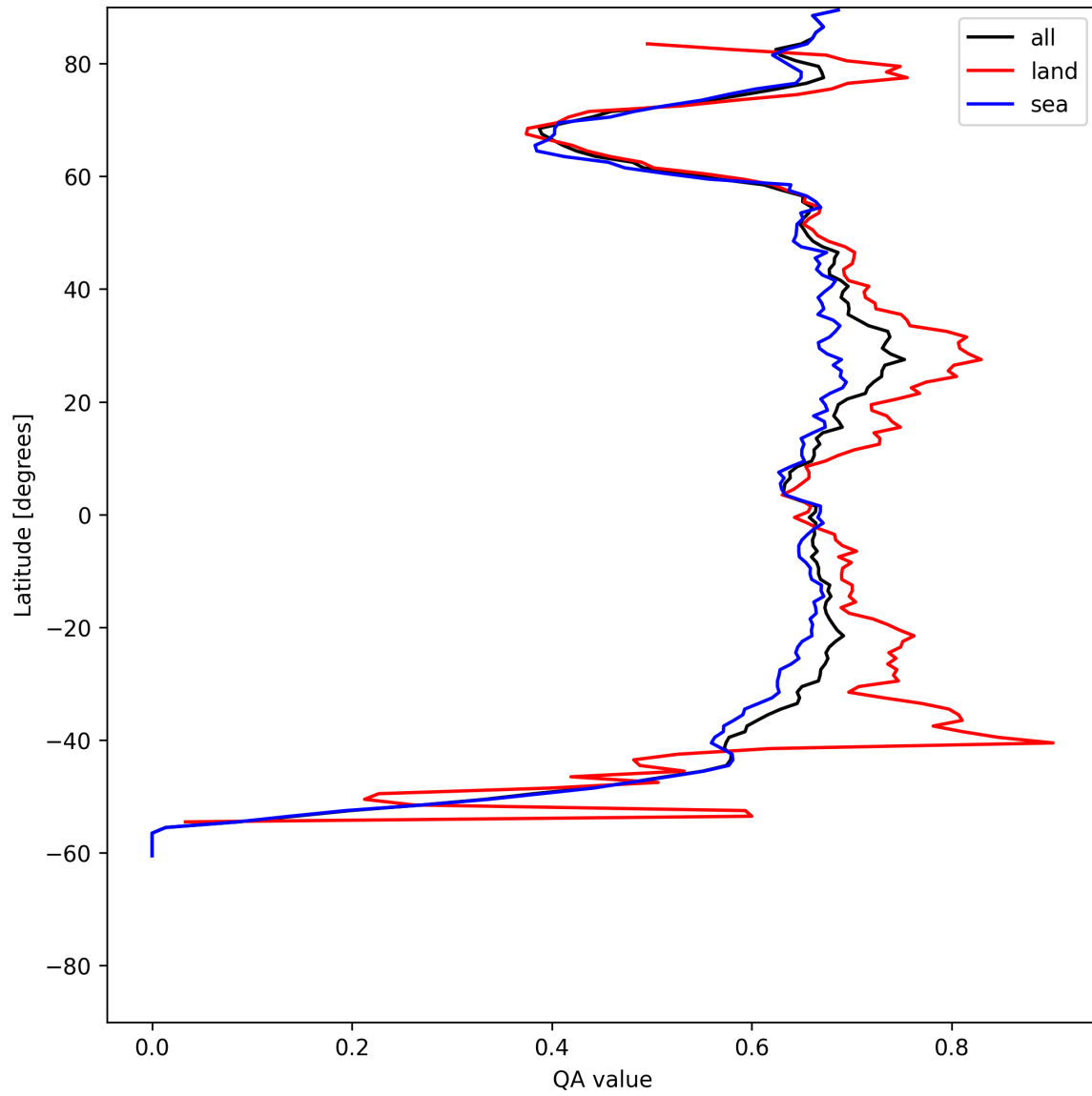
Figure 6: Zonal average of “QA value” for 2025-06-19 to 2025-06-20.
