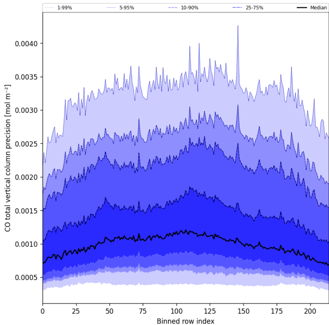
Figure 22: Along track statistics of “CO total vertical column precision” for 2025-06-19 to 2025-06-20
