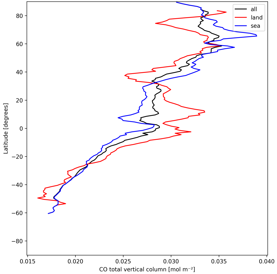
Figure 7: Zonal average of “CO total vertical column” for 2025-06-19 to 2025-06-20.
