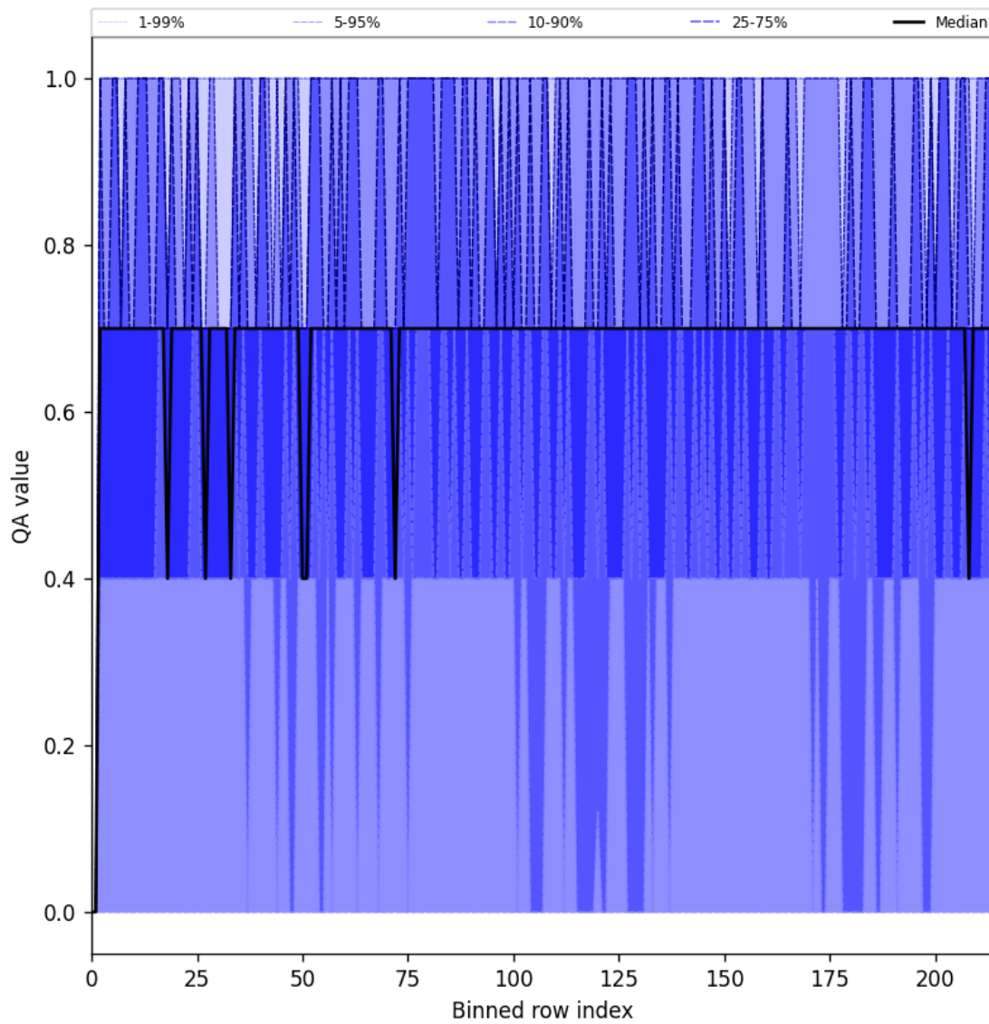
Figure 20: Along track statistics of “QA value” for 2025-06-19 to 2025-06-20
