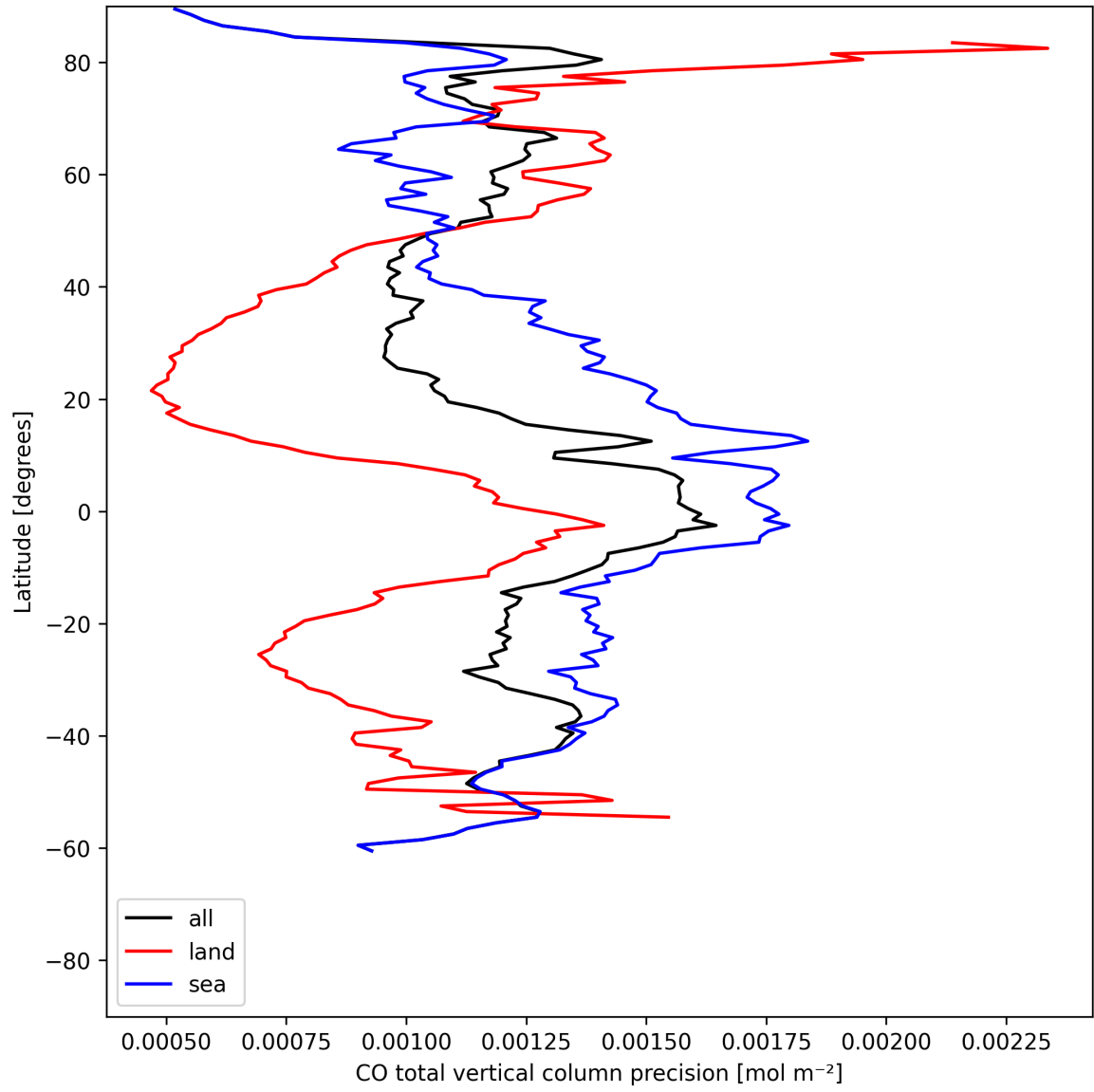
Figure 8: Zonal average of “CO total vertical column precision” for 2025-06-19 to 2025-06-20.
