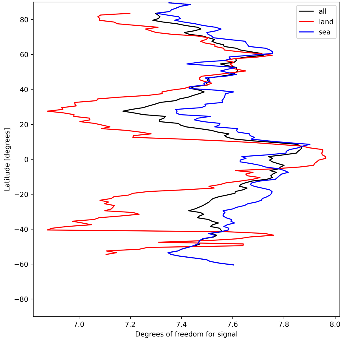
Figure 11: Zonal average of “Degrees of freedom for signal” for 2025-06-19 to 2025-06-20.
