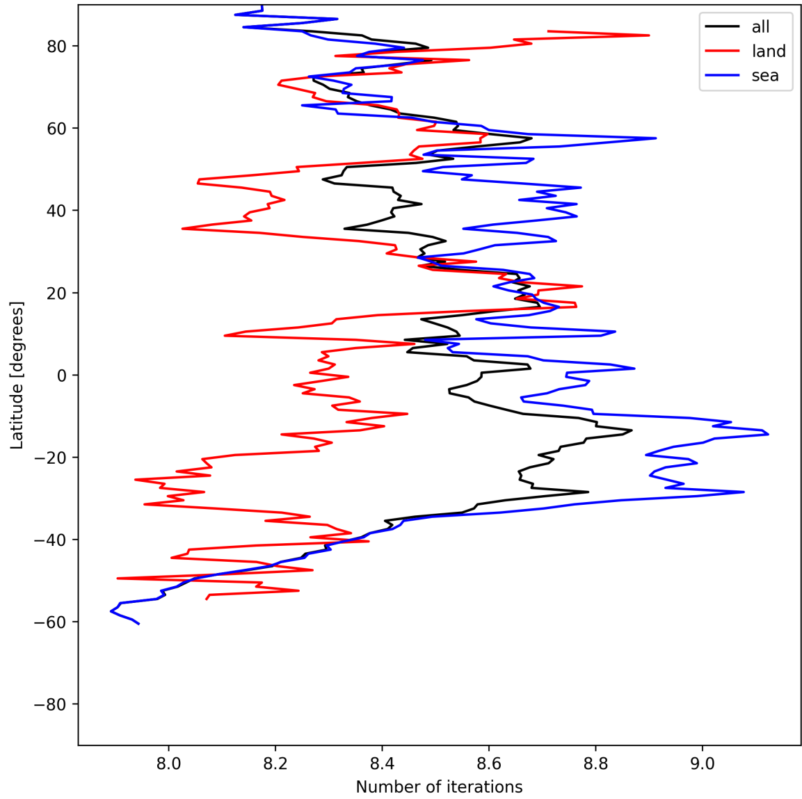
Figure 12: Zonal average of “Number of iterations” for 2025-06-19 to 2025-06-20.
