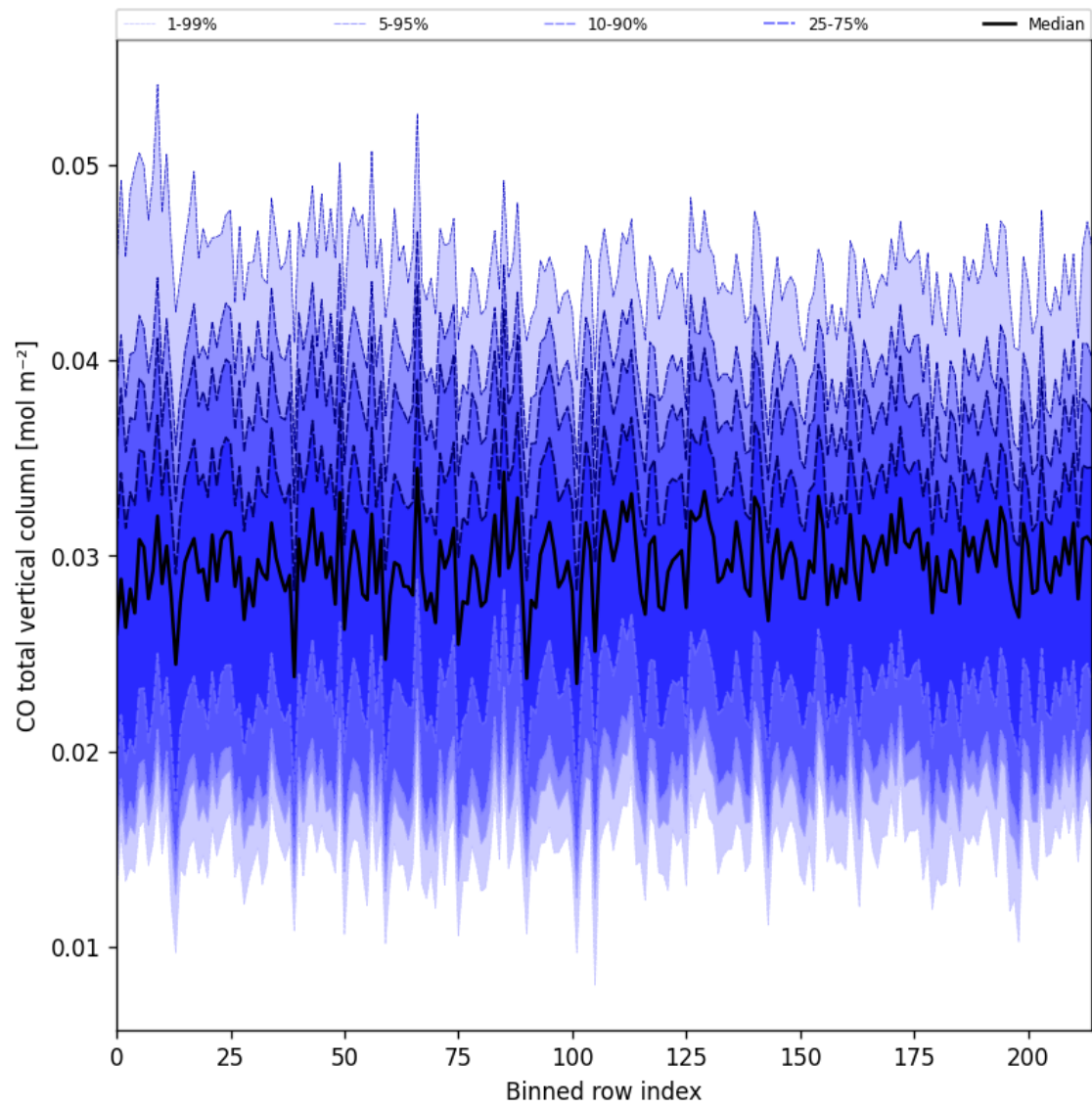
Figure 21: Along track statistics of “CO total vertical column” for 2025-06-19 to 2025-06-20
