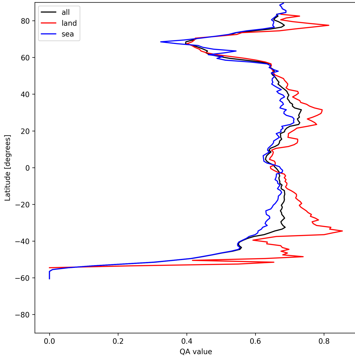
Figure 6: Zonal average of “QA value” for 2025-06-20 to 2025-06-20.
