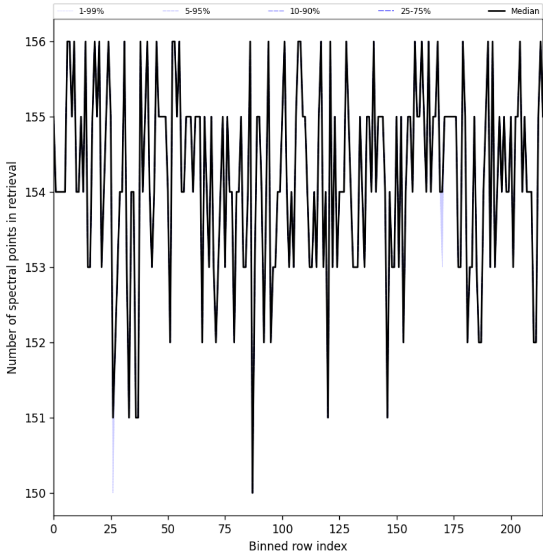
Figure 23: Along track statistics of “Number of spectral points in retrieval” for 2025-06-20 to 2025-06-20
