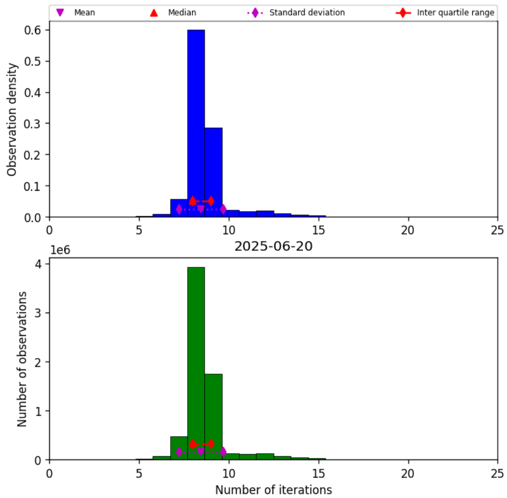
Figure 19: Histogram of “Number of iterations” for 2025-06-20 to 2025-06-20
