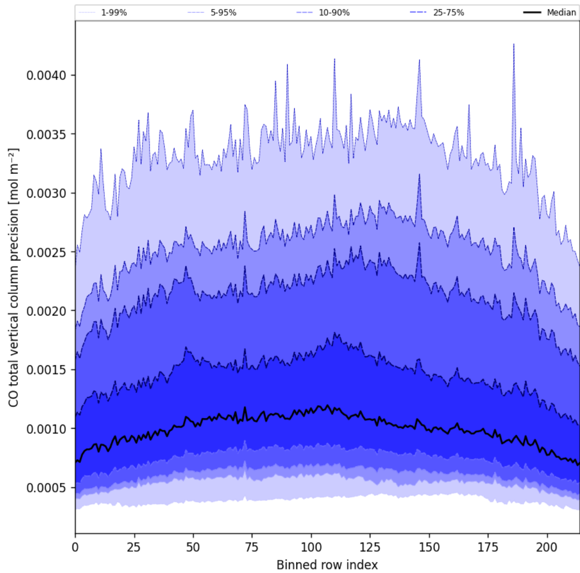
Figure 22: Along track statistics of “CO total vertical column precision” for 2025-06-20 to 2025-06-20
