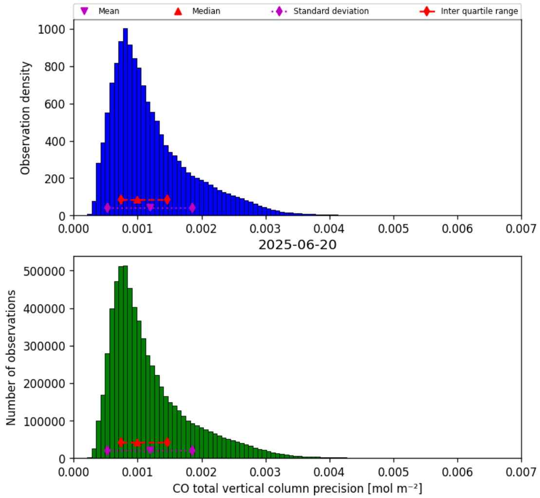
Figure 15: Histogram of “CO total vertical column precision” for 2025-06-20 to 2025-06-20
