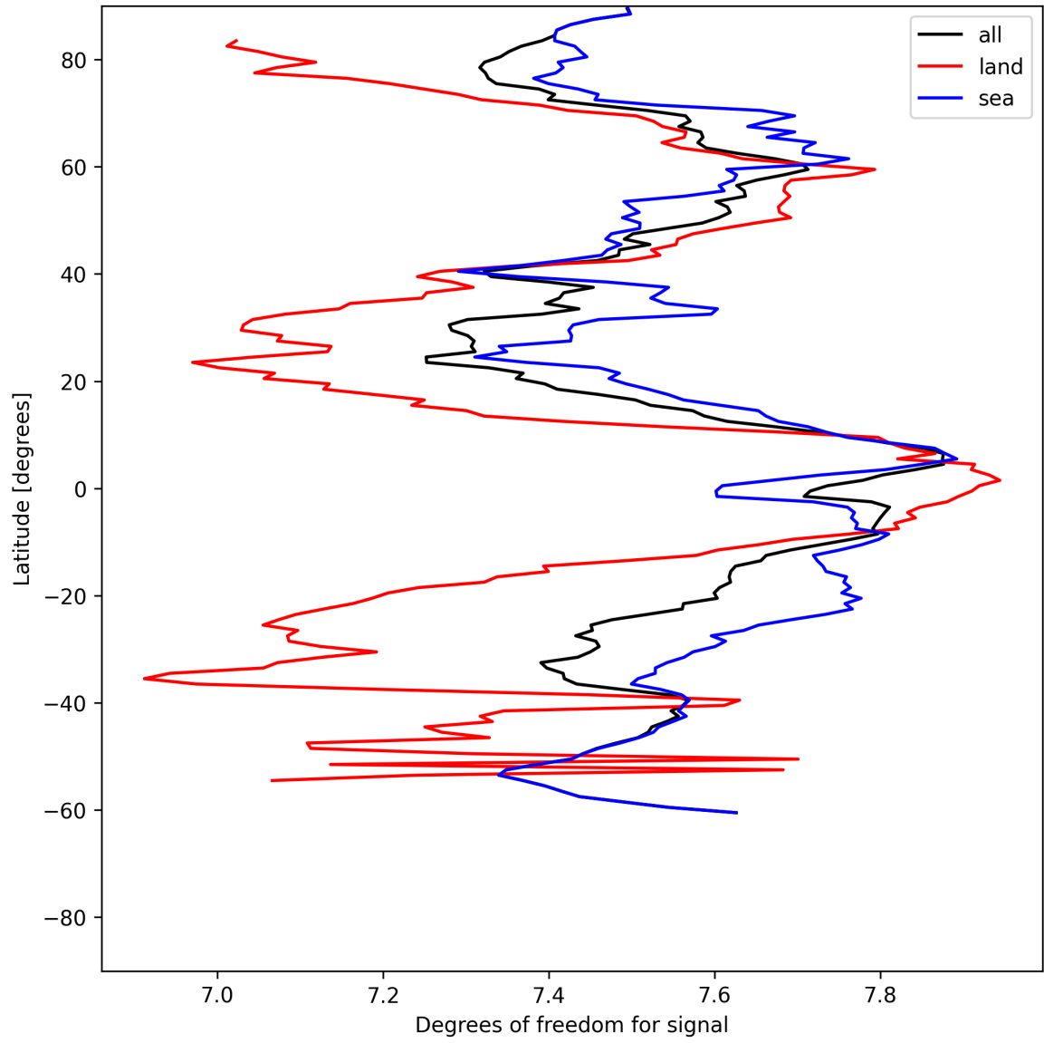
Figure 11: Zonal average of “Degrees of freedom for signal” for 2025-06-20 to 2025-06-20.
