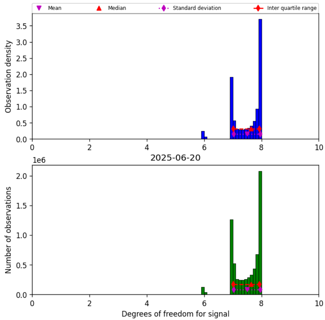
Figure 18: Histogram of “Degrees of freedom for signal” for 2025-06-20 to 2025-06-20
