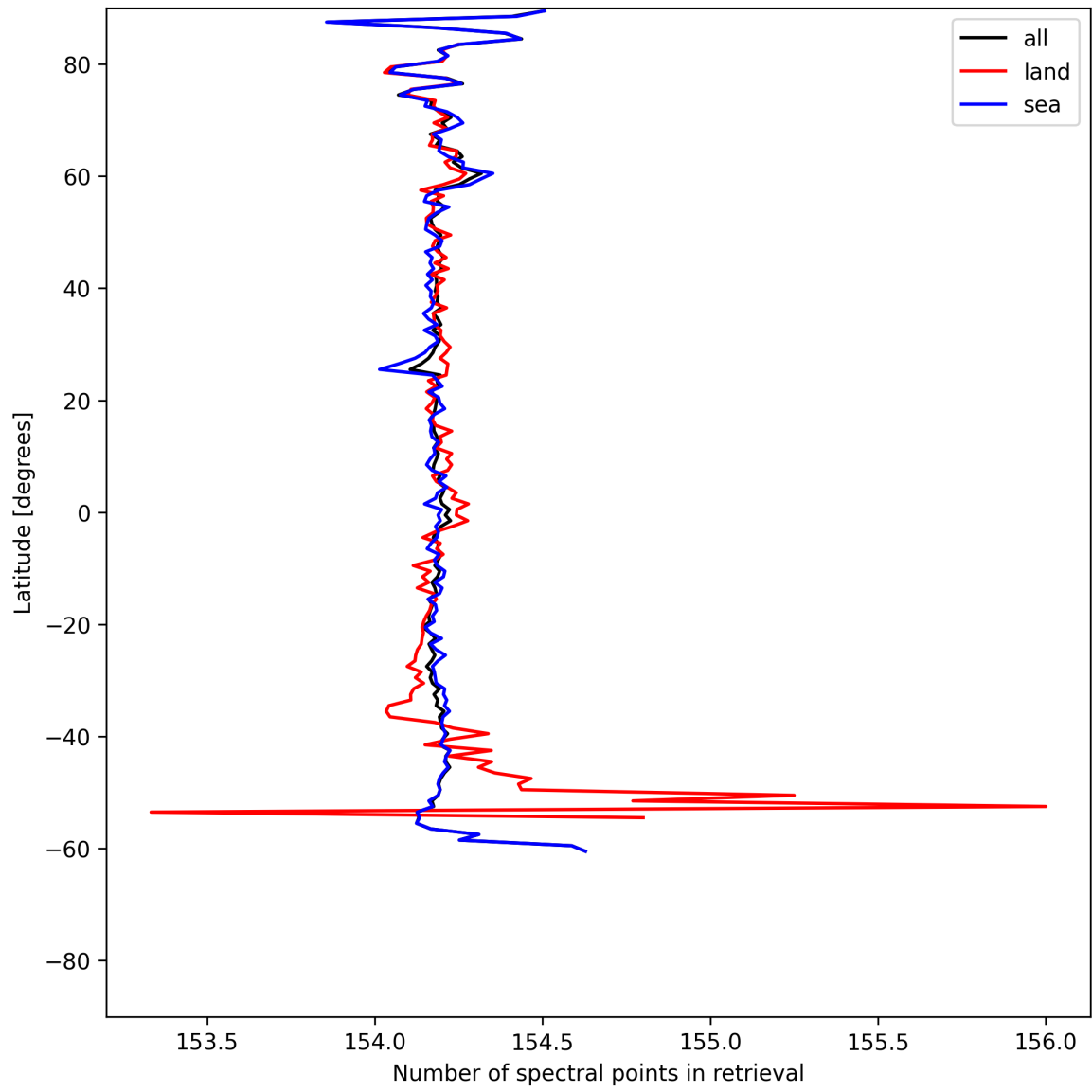
Figure 9: Zonal average of “Number of spectral points in retrieval” for 2025-06-20 to 2025-06-20.
