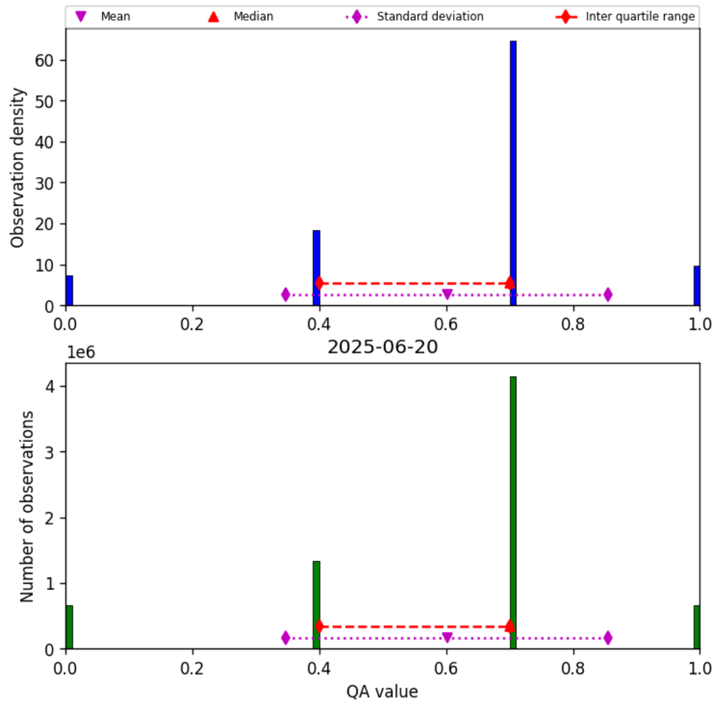
Figure 13: Histogram of “QA value” for 2025-06-20 to 2025-06-20
