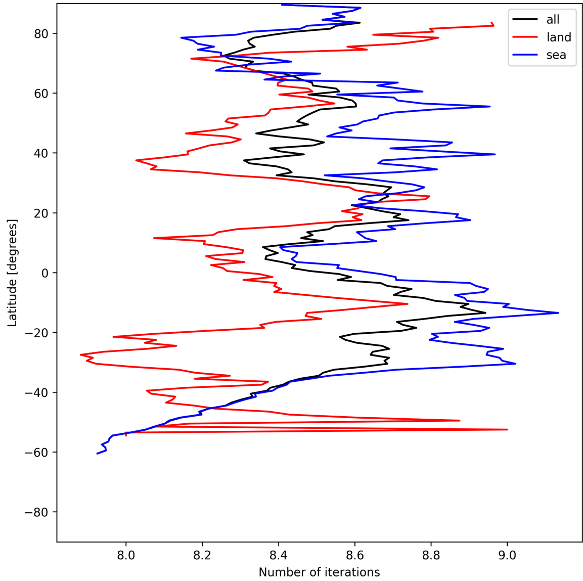
Figure 12: Zonal average of “Number of iterations” for 2025-06-20 to 2025-06-20.
