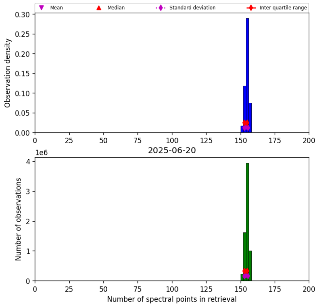
Figure 16: Histogram of “Number of spectral points in retrieval” for 2025-06-20 to 2025-06-20
