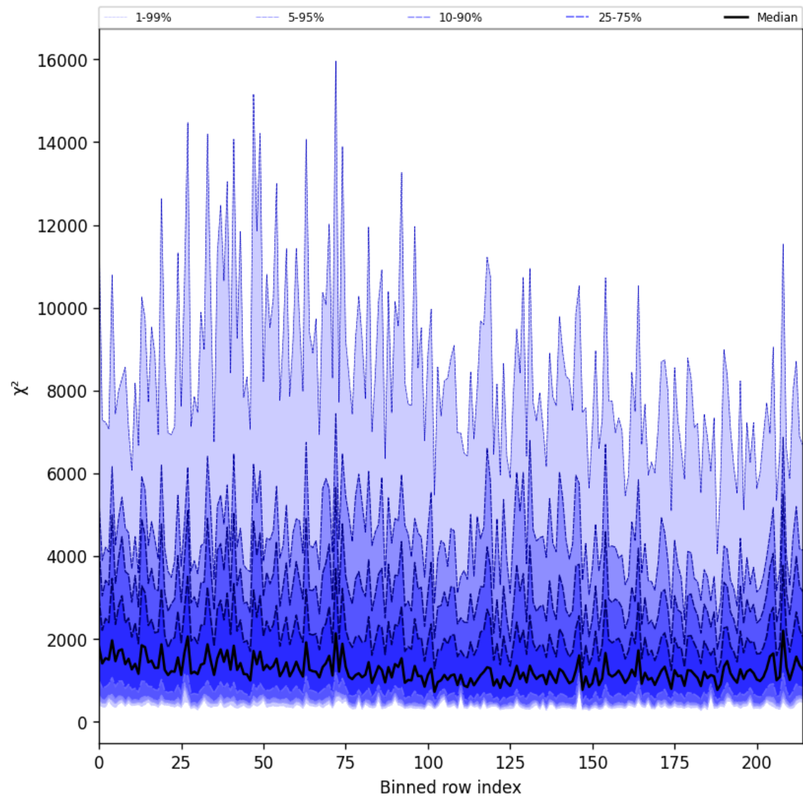
Figure 24: Along track statistics of “ \chi^2 ” for 2025-06-20 to 2025-06-20
