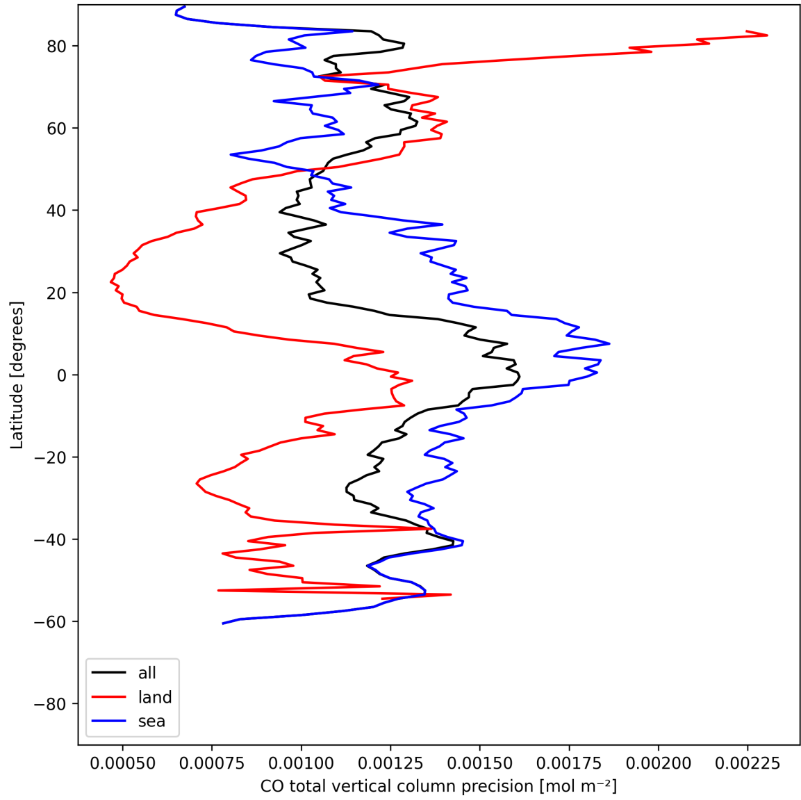
Figure 8: Zonal average of “CO total vertical column precision” for 2025-06-20 to 2025-06-20.
