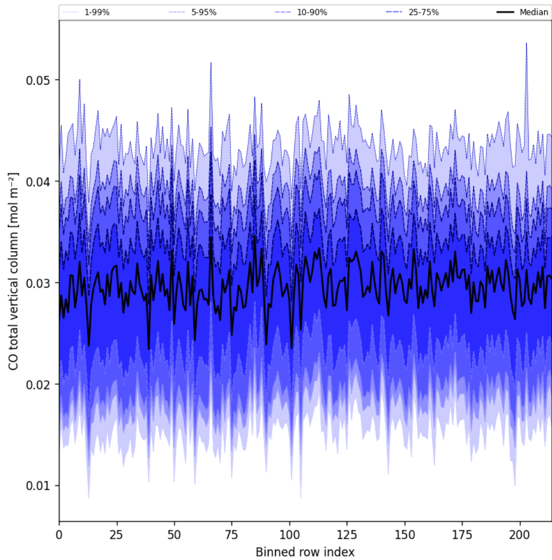
Figure 21: Along track statistics of “CO total vertical column” for 2025-06-20 to 2025-06-20
