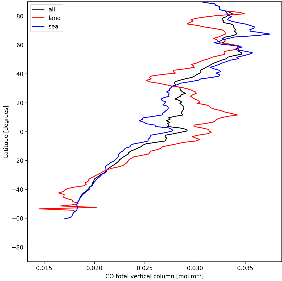
Figure 7: Zonal average of “CO total vertical column” for 2025-06-20 to 2025-06-20.
