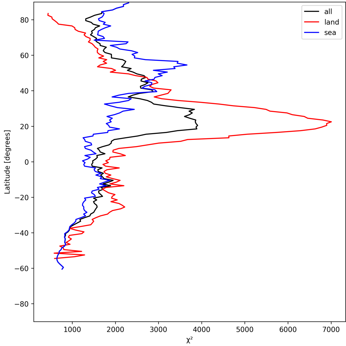
Figure 10: Zonal average of “ \chi^2 ” for 2025-06-20 to 2025-06-20.
