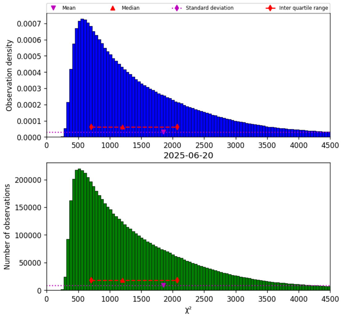
Figure 17: Histogram of " \chi^2 " for 2025-06-20 to 2025-06-20
