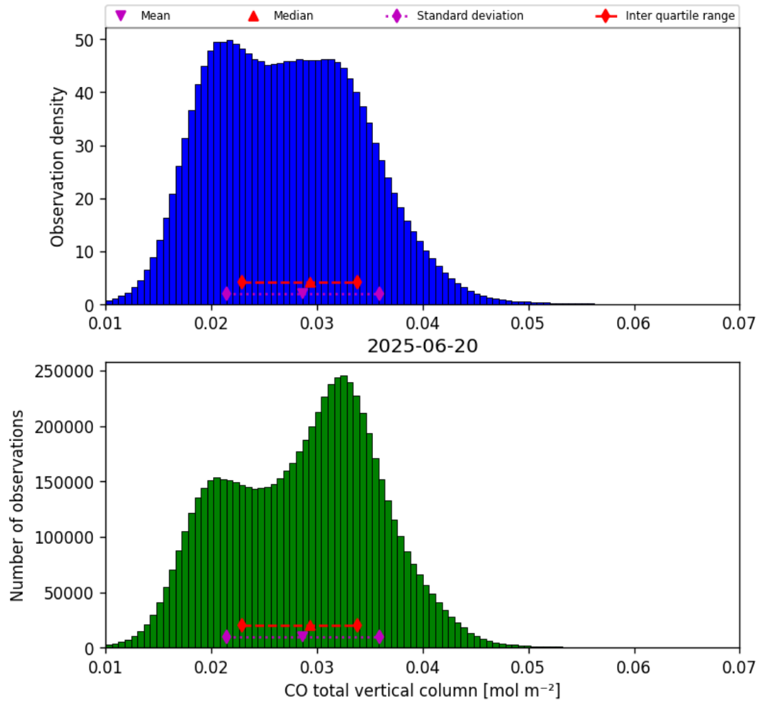
Figure 14: Histogram of “CO total vertical column” for 2025-06-20 to 2025-06-20
