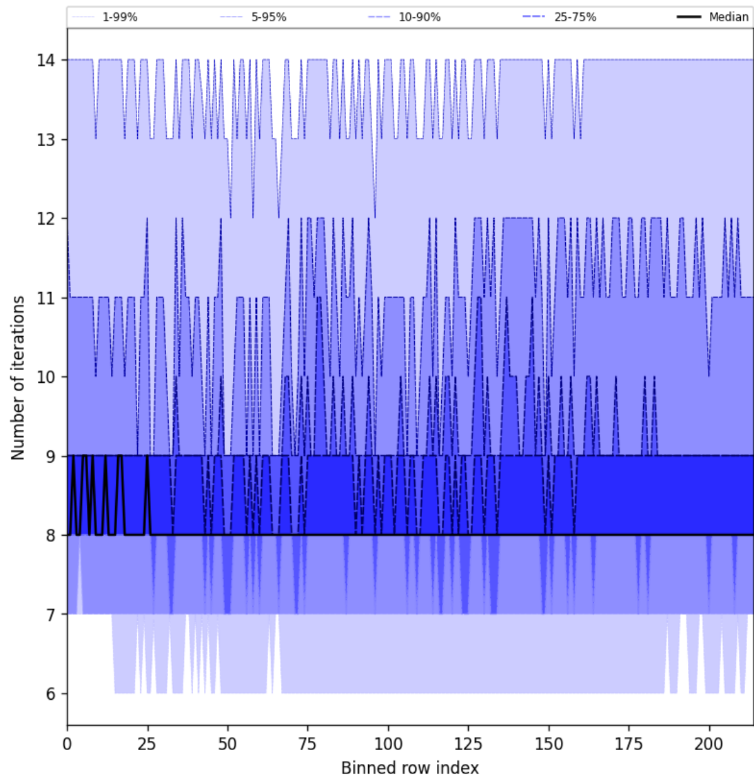
Figure 26: Along track statistics of “Number of iterations” for 2025-06-20 to 2025-06-20
