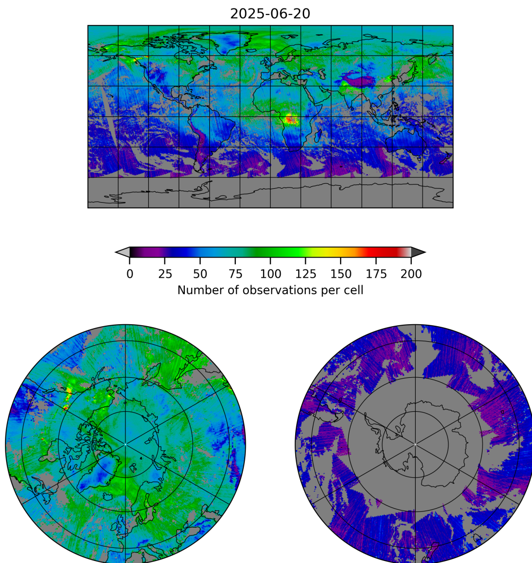
Figure 5: Map of the number of observations for 2025-06-20 to 2025-06-20
