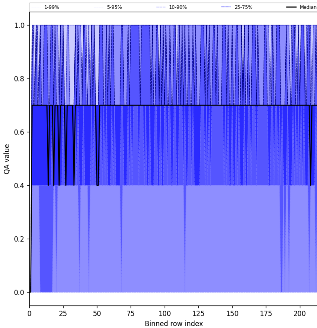
Figure 20: Along track statistics of “QA value” for 2025-06-20 to 2025-06-20
