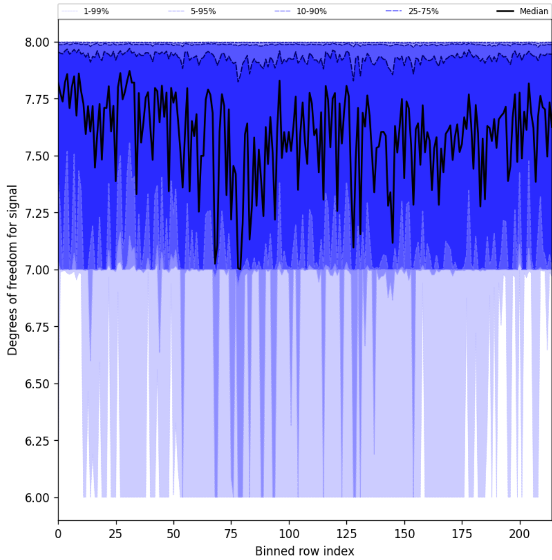
Figure 25: Along track statistics of “Degrees of freedom for signal” for 2025-06-20 to 2025-06-20
