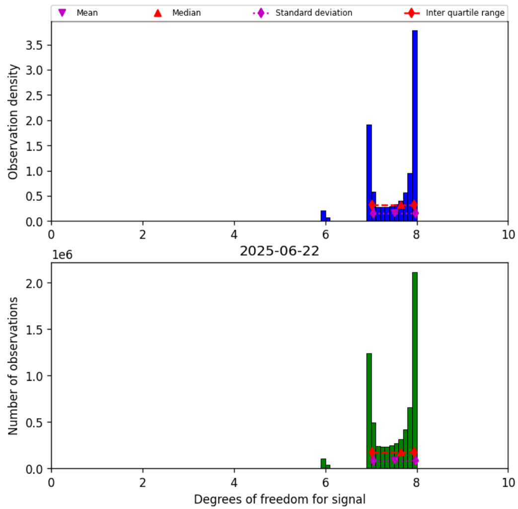
Figure 18: Histogram of “Degrees of freedom for signal” for 2025-06-22 to 2025-06-23
