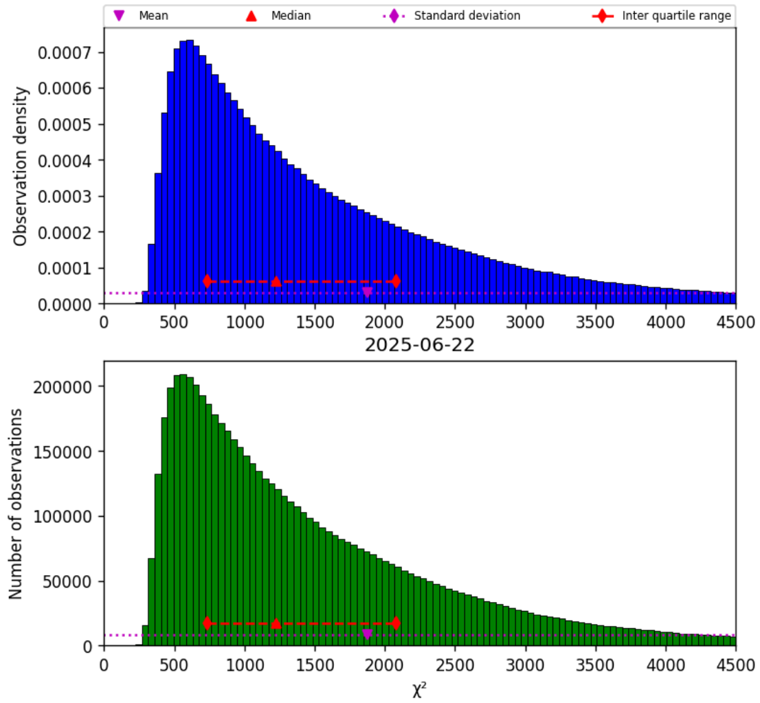
Figure 17: Histogram of “ \chi^2 ” for 2025-06-22 to 2025-06-23
