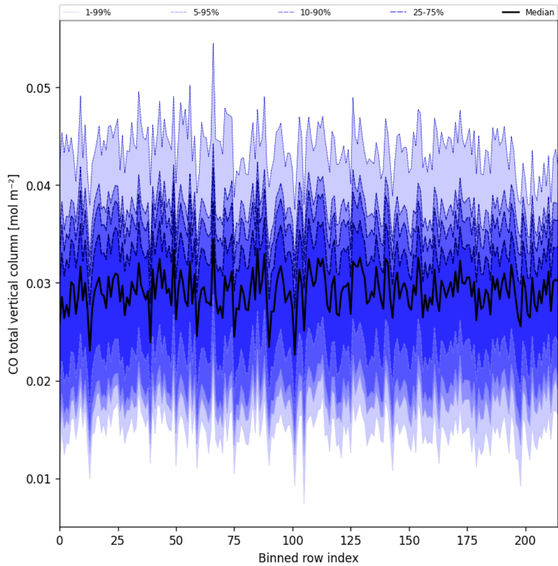
Figure 21: Along track statistics of “CO total vertical column” for 2025-06-22 to 2025-06-23
