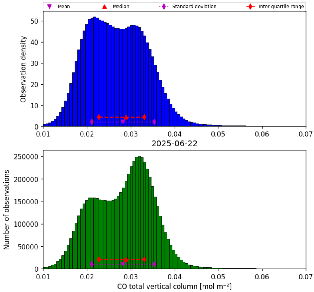
Figure 14: Histogram of “CO total vertical column” for 2025-06-22 to 2025-06-23
