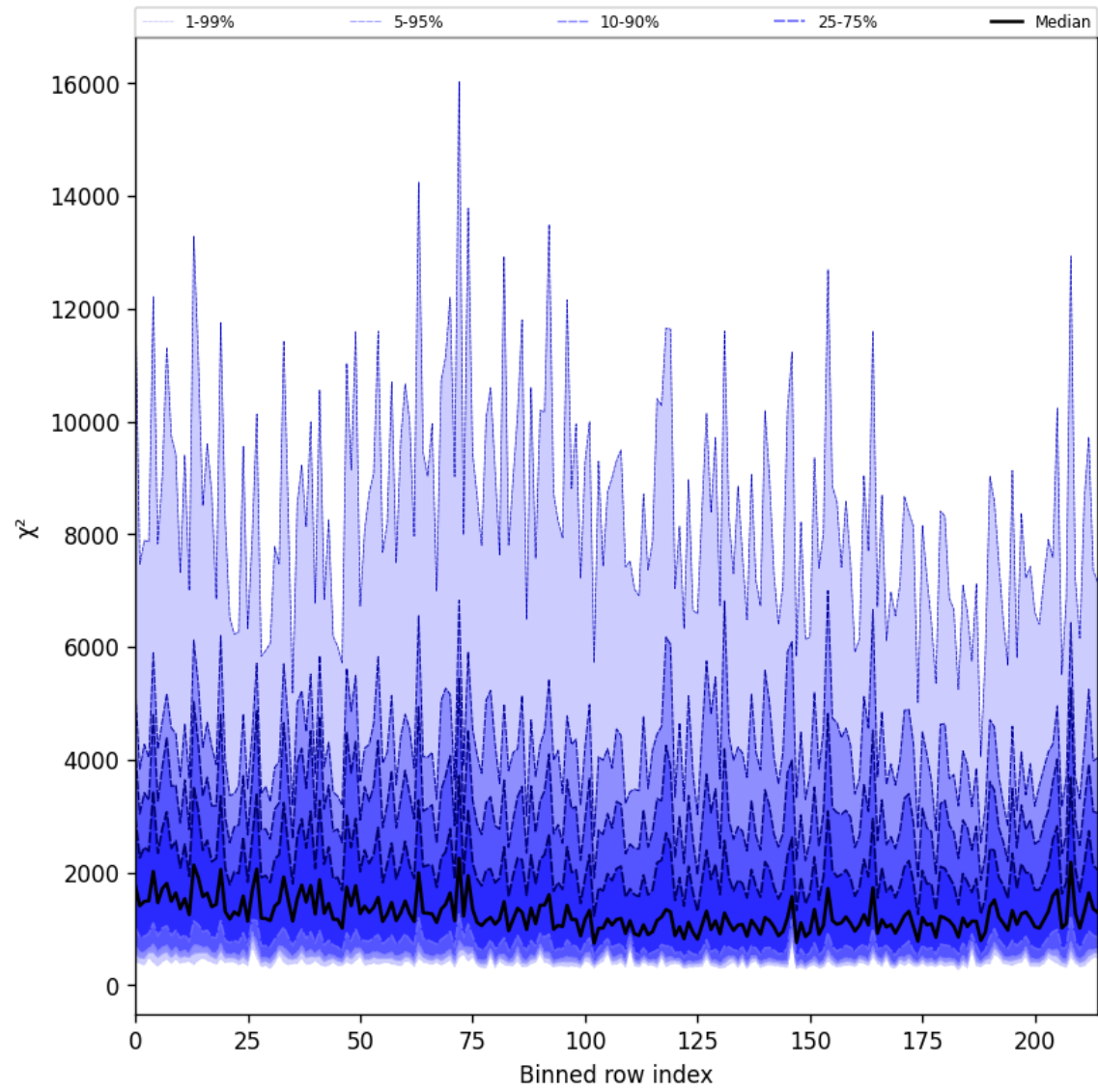
Figure 24: Along track statistics of “ \chi^2 ” for 2025-06-22 to 2025-06-23
