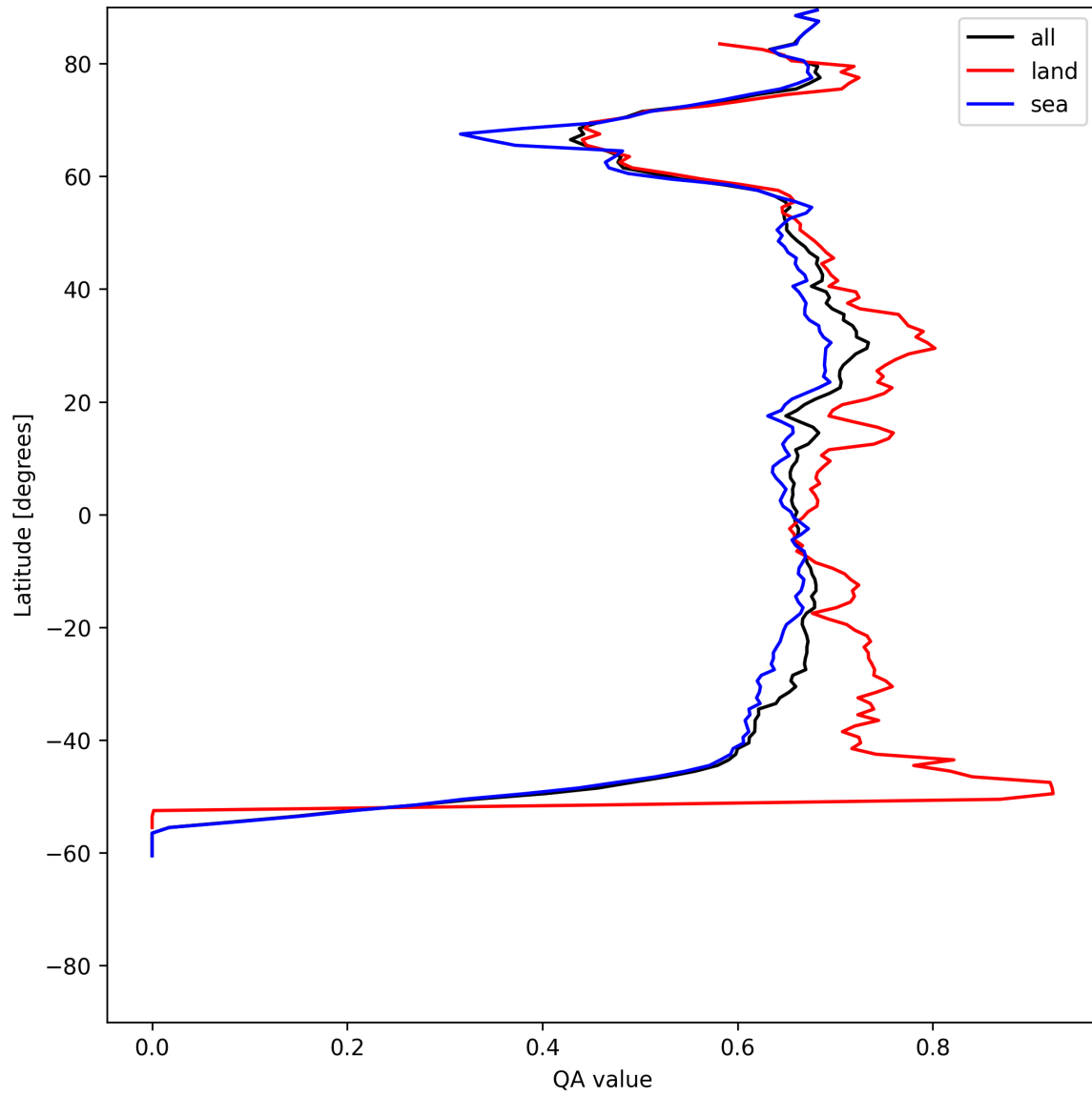
Figure 6: Zonal average of “QA value” for 2025-06-22 to 2025-06-23.
