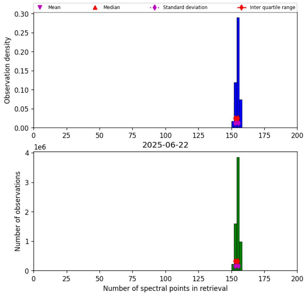
Figure 16: Histogram of “Number of spectral points in retrieval” for 2025-06-22 to 2025-06-23
