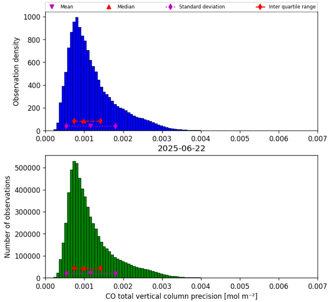
Figure 15: Histogram of “CO total vertical column precision” for 2025-06-22 to 2025-06-23
