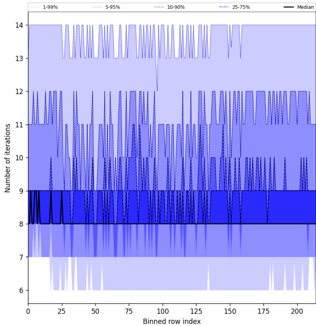
Figure 26: Along track statistics of “Number of iterations” for 2025-06-22 to 2025-06-23
