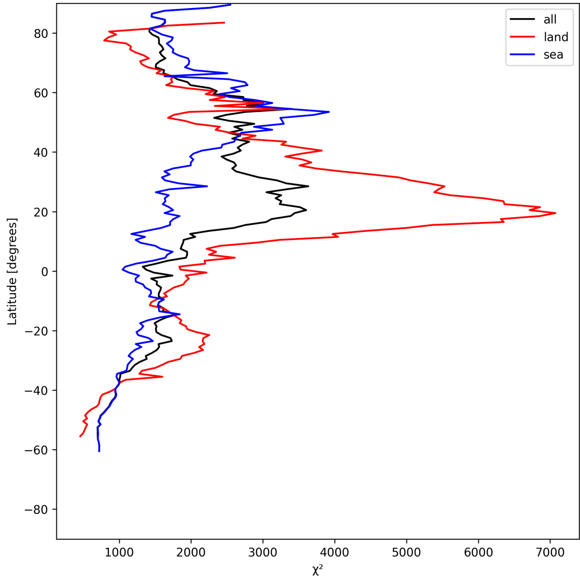
Figure 10: Zonal average of “ \chi^2 ” for 2025-06-22 to 2025-06-23.
