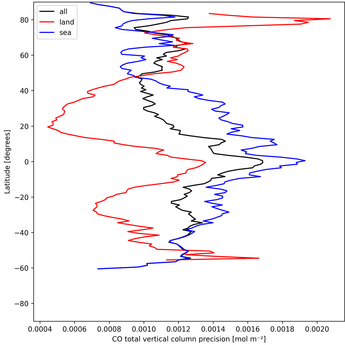
Figure 8: Zonal average of “CO total vertical column precision” for 2025-06-22 to 2025-06-23.
