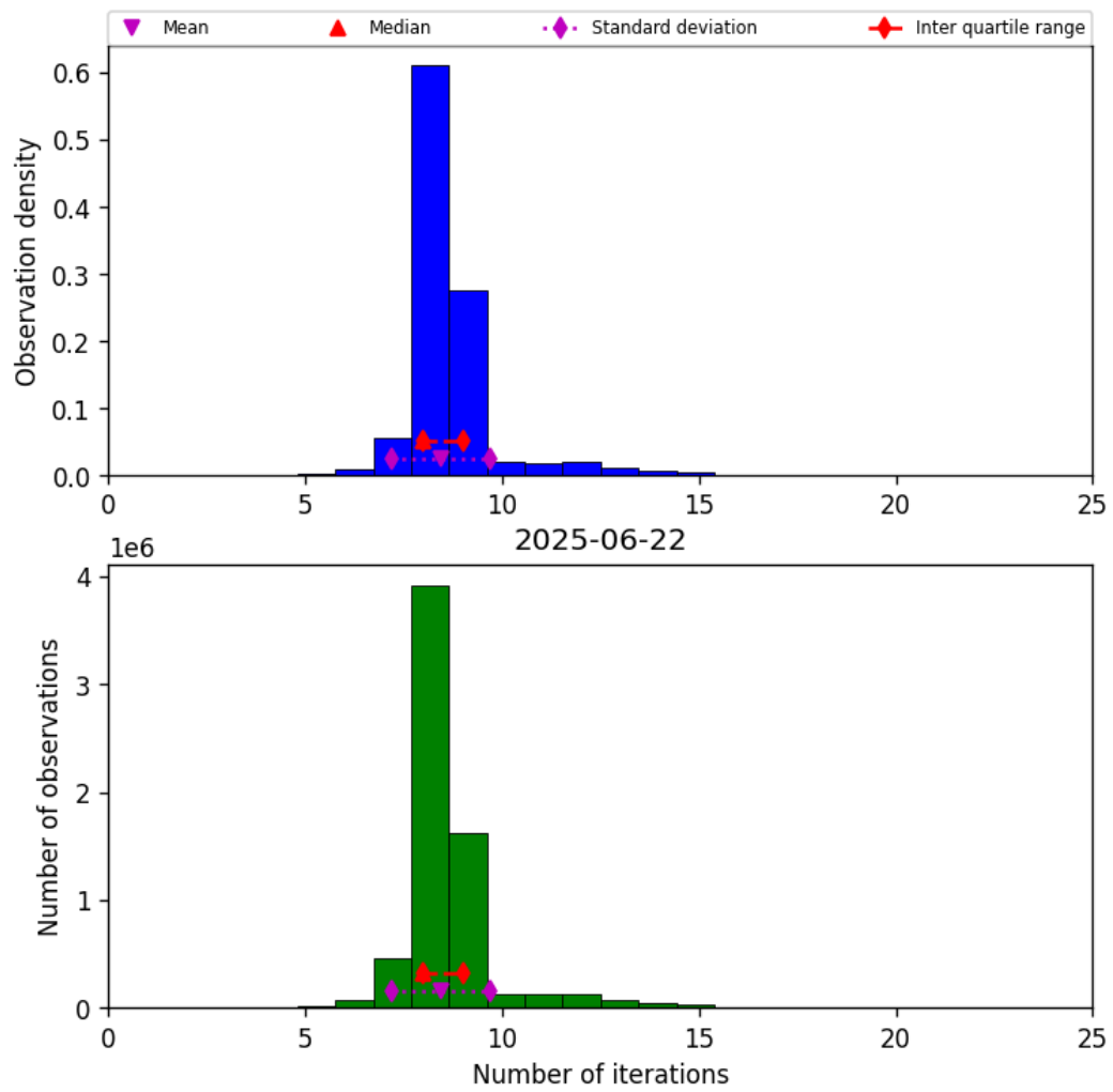
Figure 19: Histogram of “Number of iterations” for 2025-06-22 to 2025-06-23
