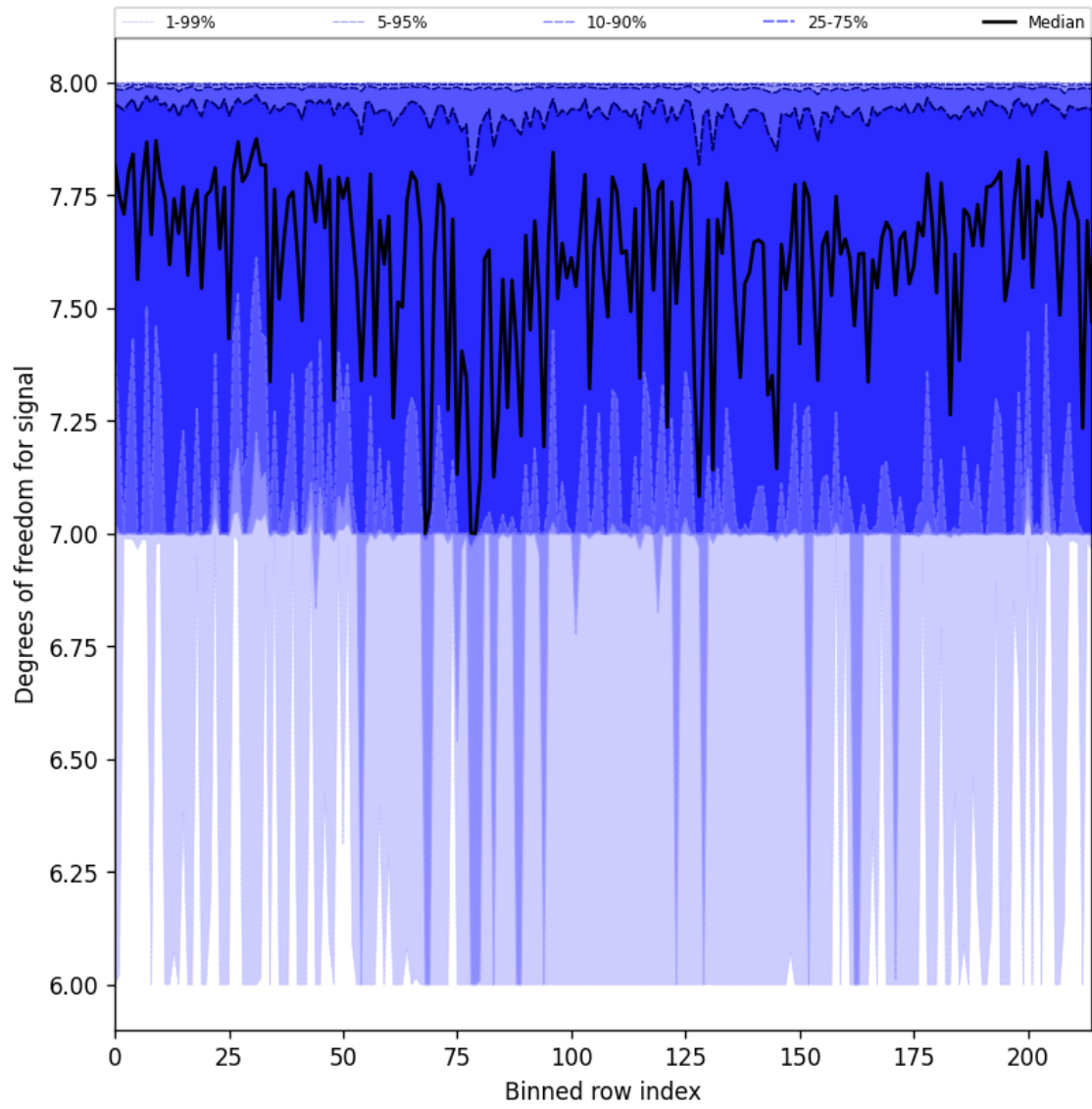
Figure 25: Along track statistics of “Degrees of freedom for signal” for 2025-06-22 to 2025-06-23
