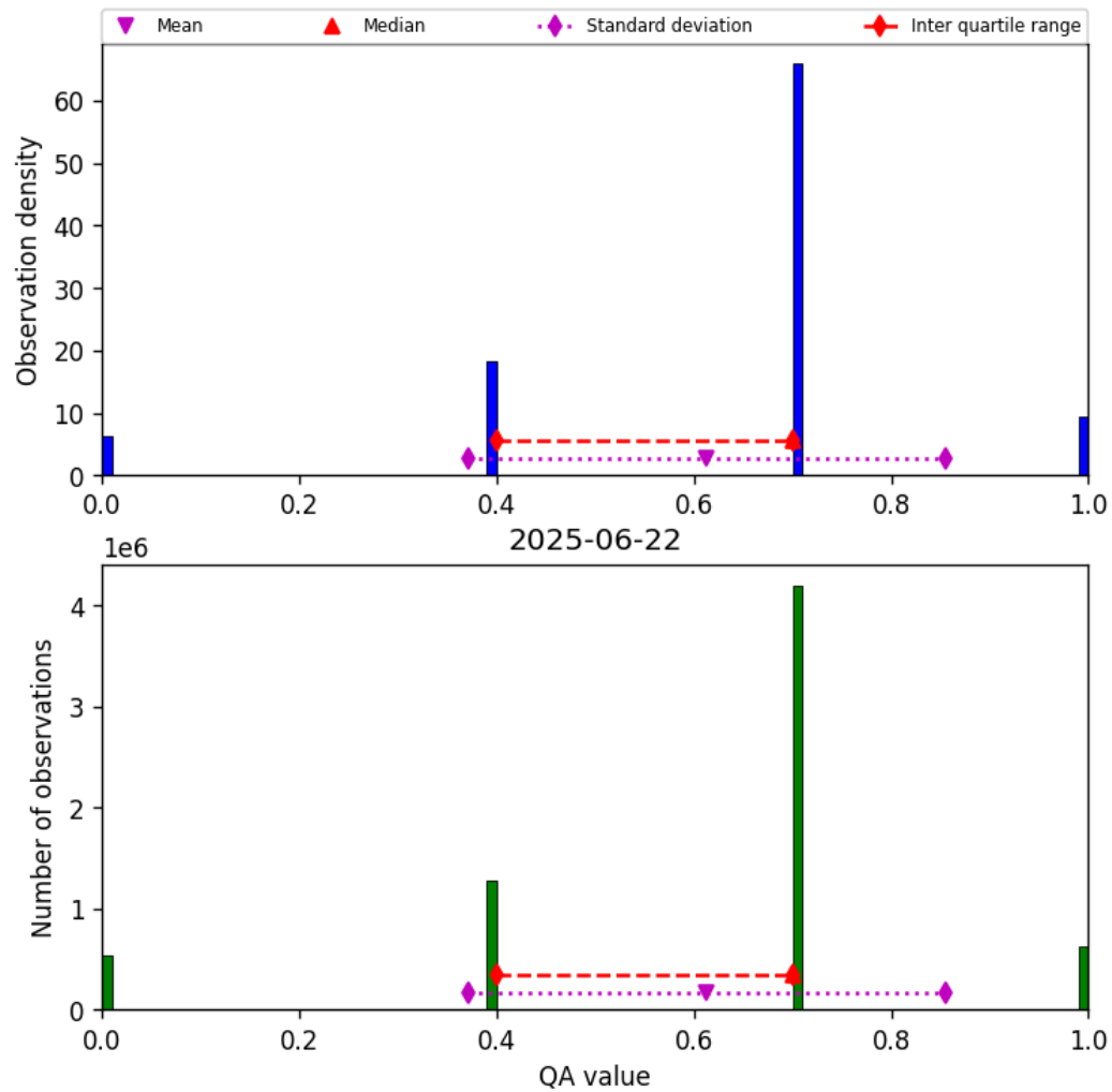
Figure 13: Histogram of “QA value” for 2025-06-22 to 2025-06-23
