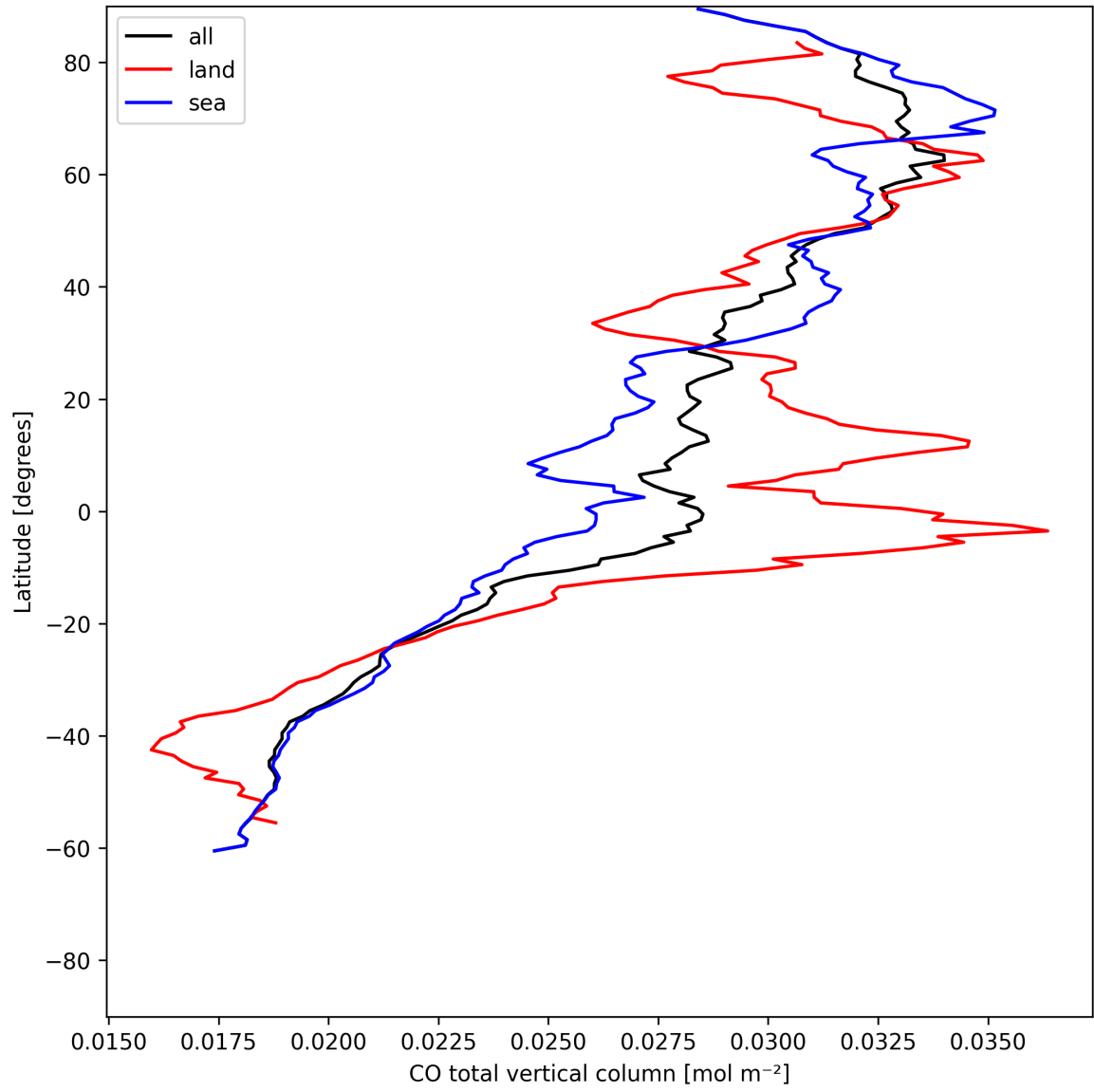
Figure 7: Zonal average of “CO total vertical column” for 2025-06-22 to 2025-06-23.
