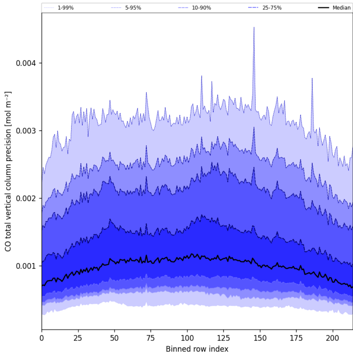
Figure 22: Along track statistics of “CO total vertical column precision” for 2025-06-22 to 2025-06-23
