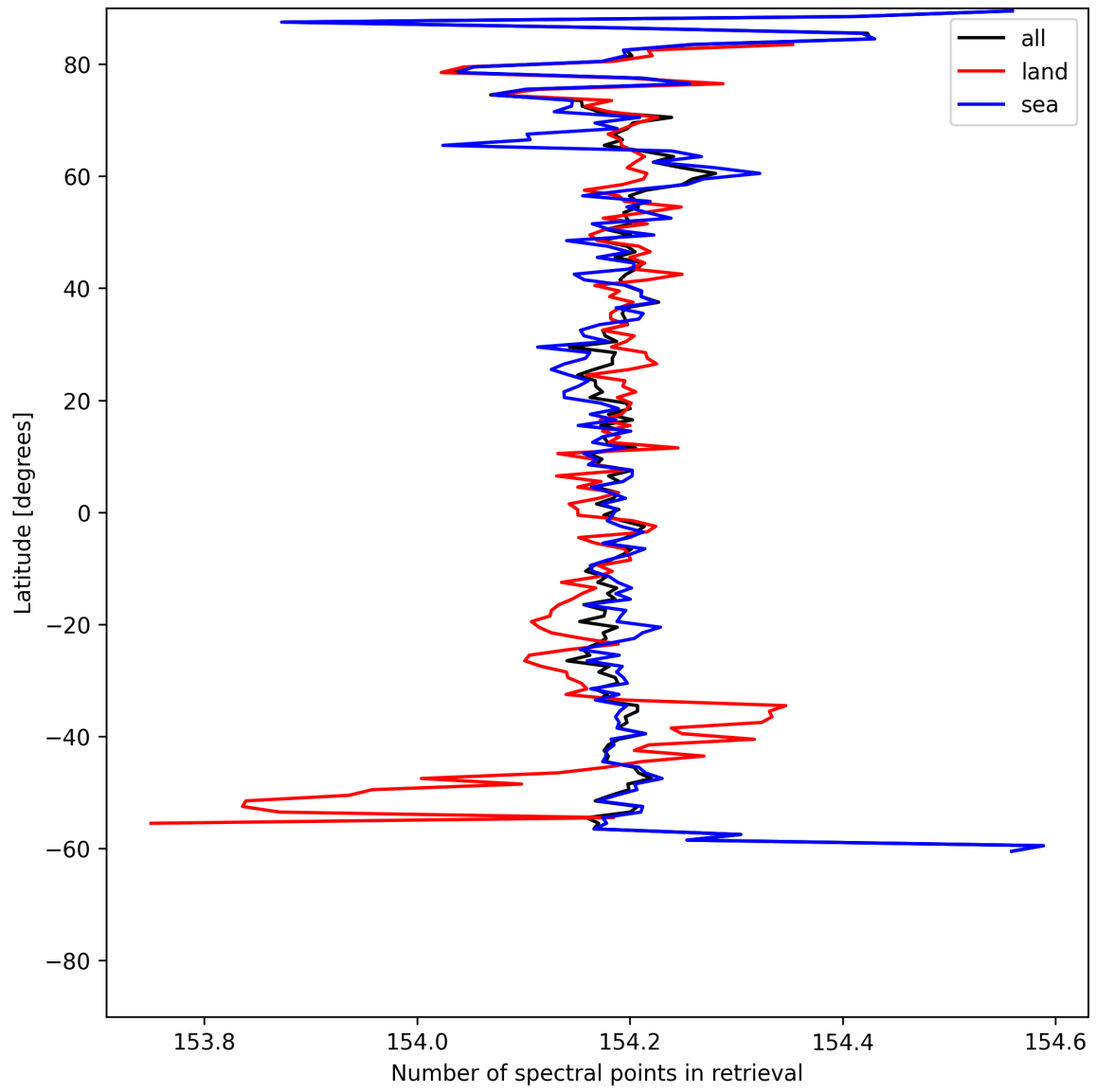
Figure 9: Zonal average of “Number of spectral points in retrieval” for 2025-06-22 to 2025-06-23.
