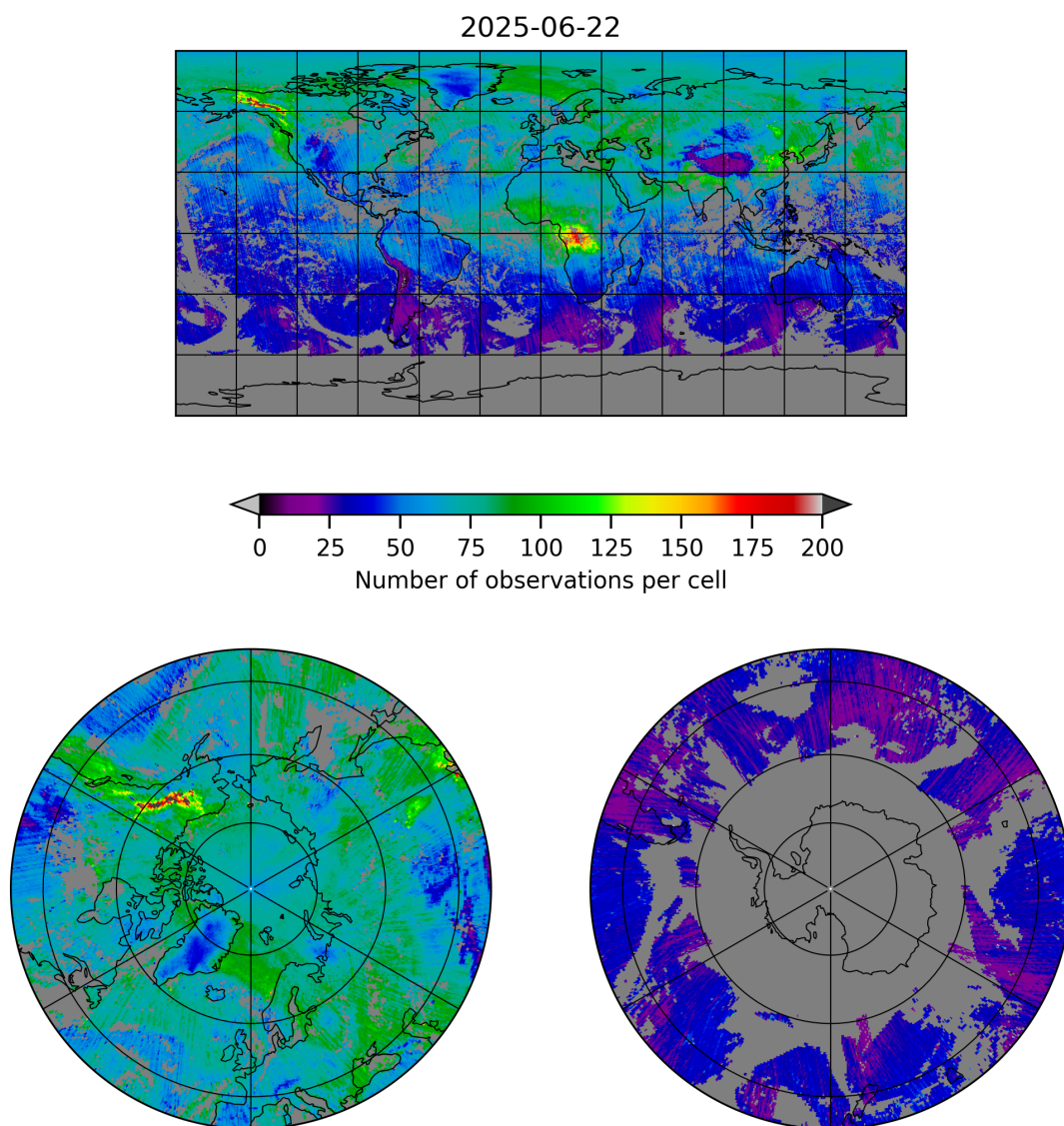
Figure 5: Map of the number of observations for 2025-06-22 to 2025-06-23
