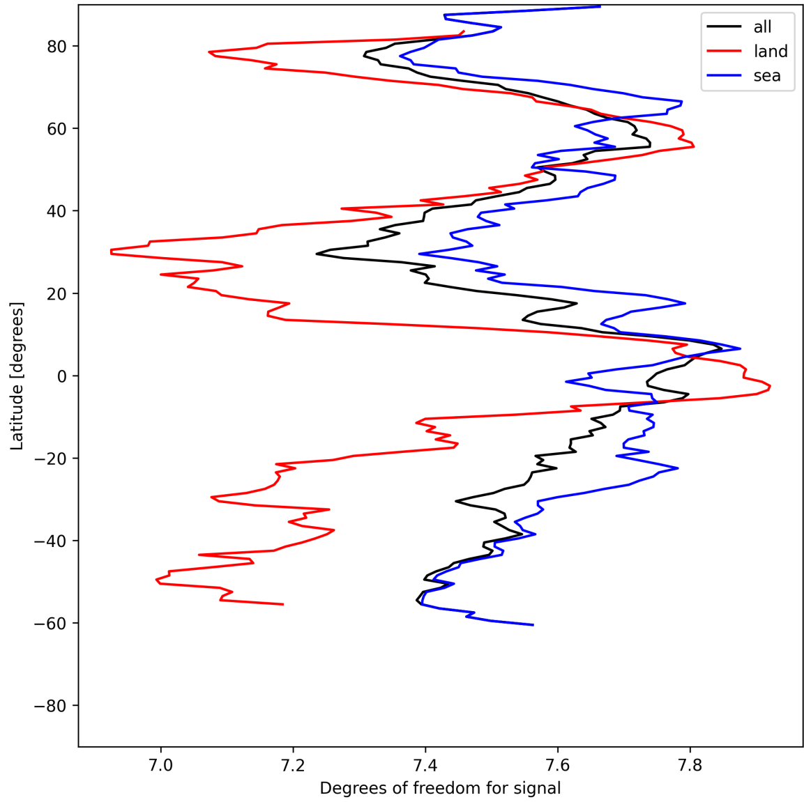
Figure 11: Zonal average of “Degrees of freedom for signal” for 2025-06-22 to 2025-06-23.
