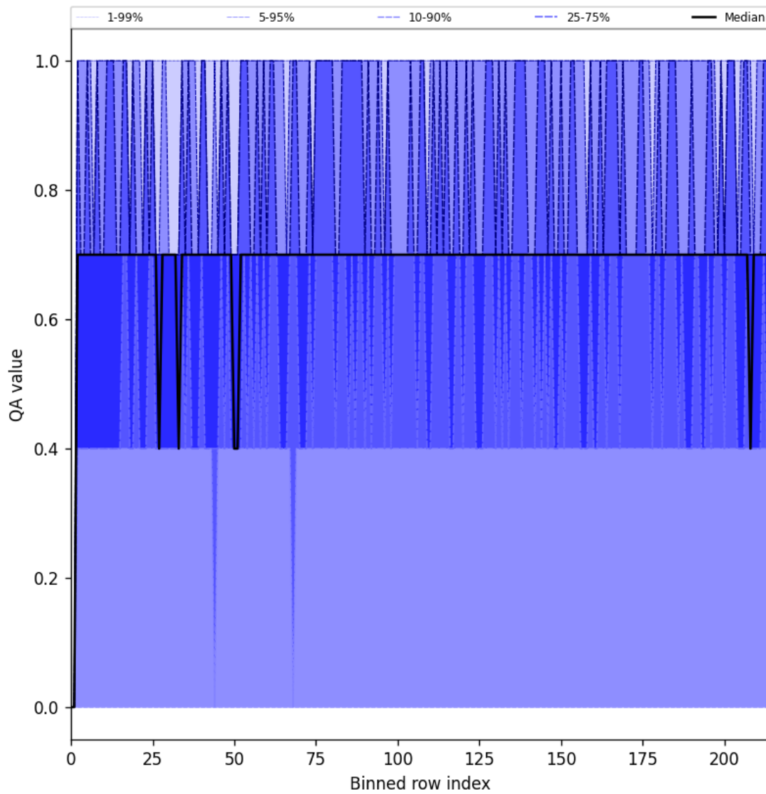
Figure 20: Along track statistics of “QA value” for 2025-06-22 to 2025-06-23
