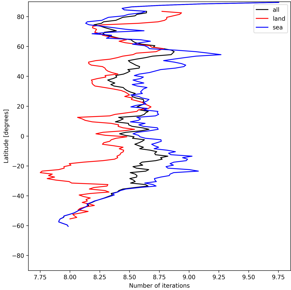
Figure 12: Zonal average of “Number of iterations” for 2025-06-22 to 2025-06-23.
