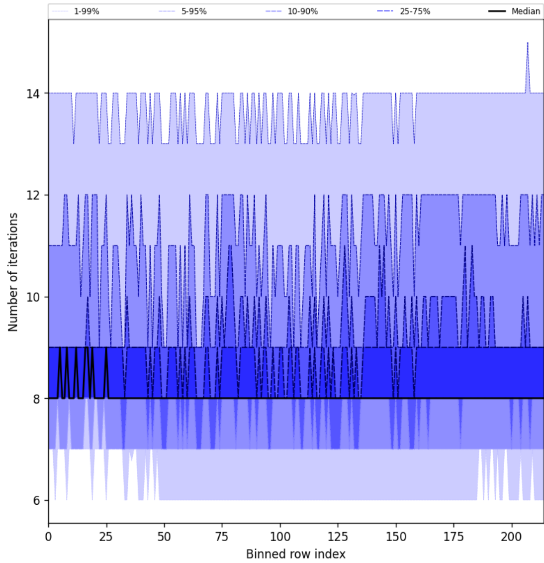
Figure 26: Along track statistics of “Number of iterations” for 2025-06-23 to 2025-06-24
