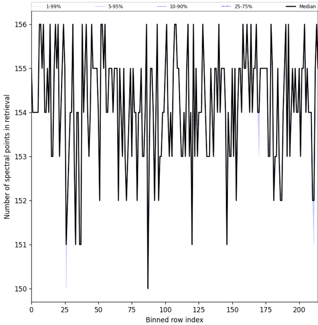
Figure 23: Along track statistics of “Number of spectral points in retrieval” for 2025-06-23 to 2025-06-24
