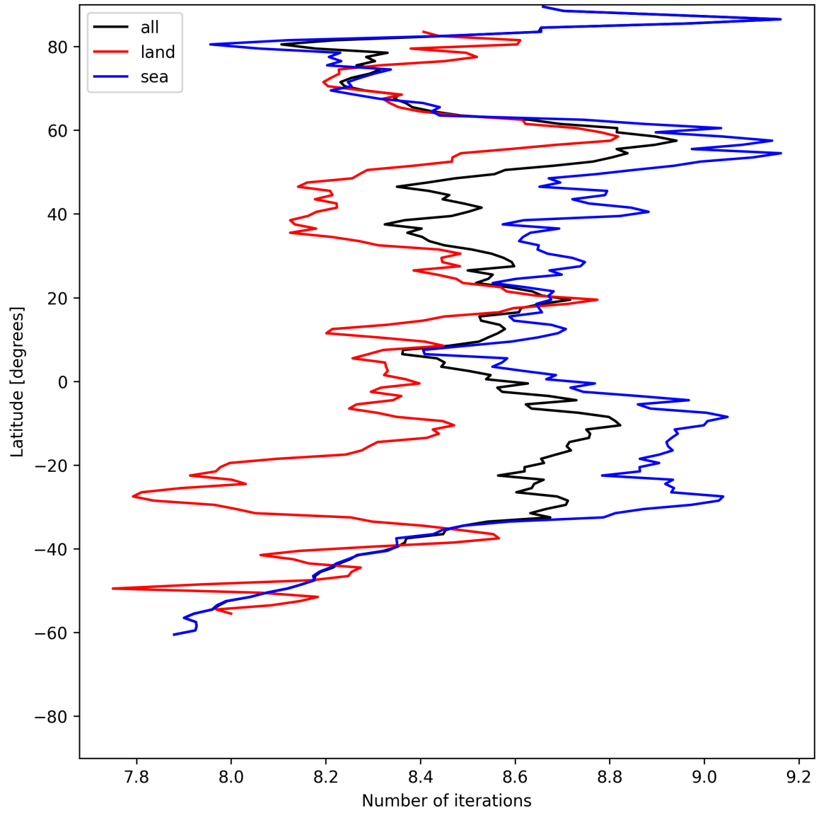
Figure 12: Zonal average of “Number of iterations” for 2025-06-23 to 2025-06-24.
