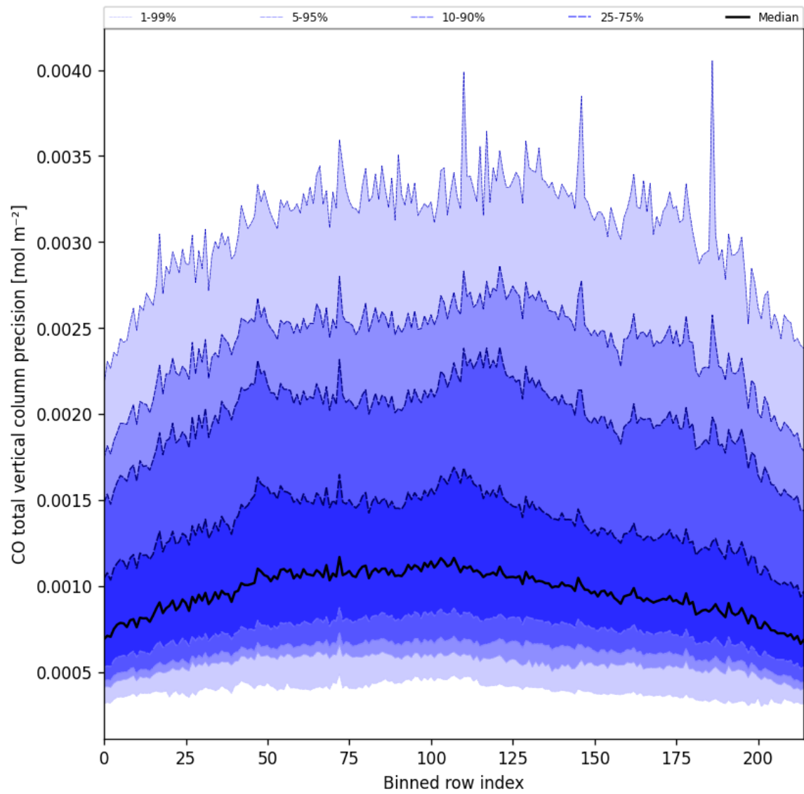
Figure 22: Along track statistics of “CO total vertical column precision” for 2025-06-23 to 2025-06-24
