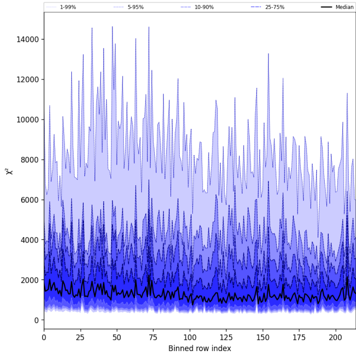
Figure 24: Along track statistics of “ \chi^2 ” for 2025-06-23 to 2025-06-24
