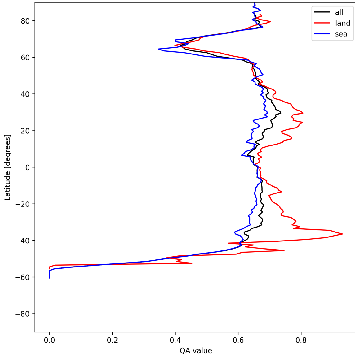
Figure 6: Zonal average of “QA value” for 2025-06-23 to 2025-06-24.
