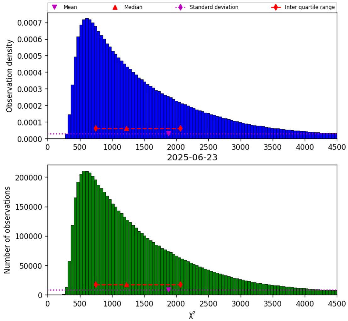
Figure 17: Histogram of “ \chi^2 ” for 2025-06-23 to 2025-06-24
