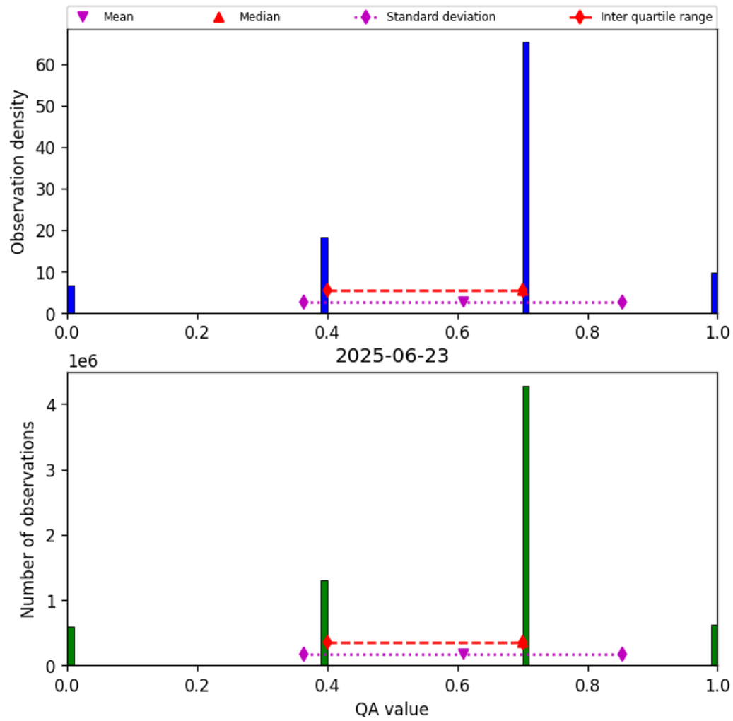
Figure 13: Histogram of “QA value” for 2025-06-23 to 2025-06-24
