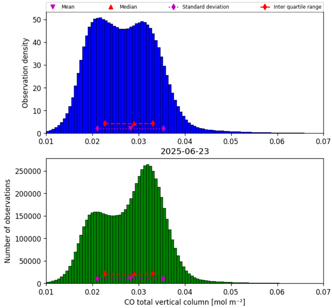
Figure 14: Histogram of “CO total vertical column” for 2025-06-23 to 2025-06-24
