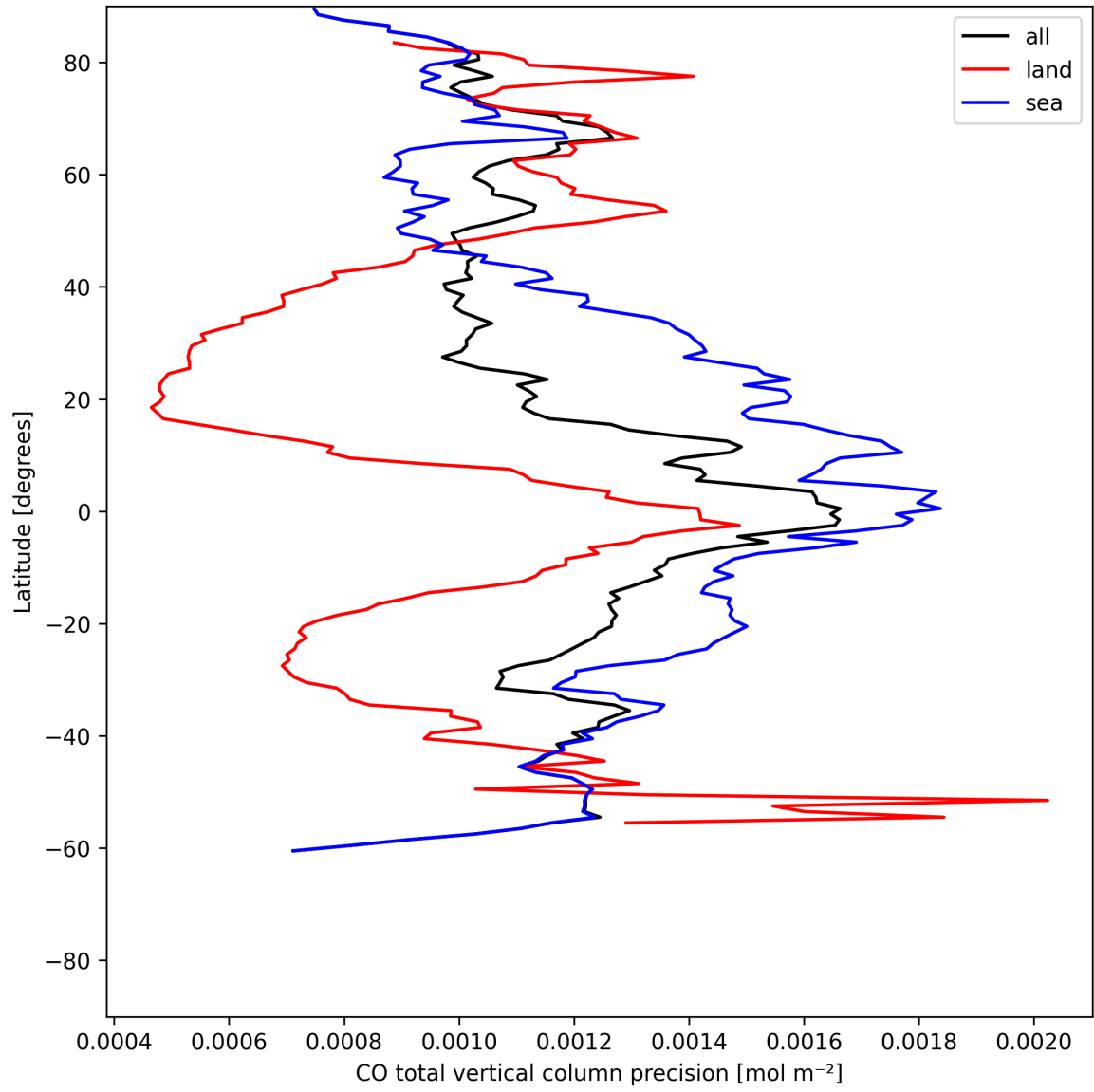
Figure 8: Zonal average of "CO total vertical column precision" for 2025-06-23 to 2025-06-24.
