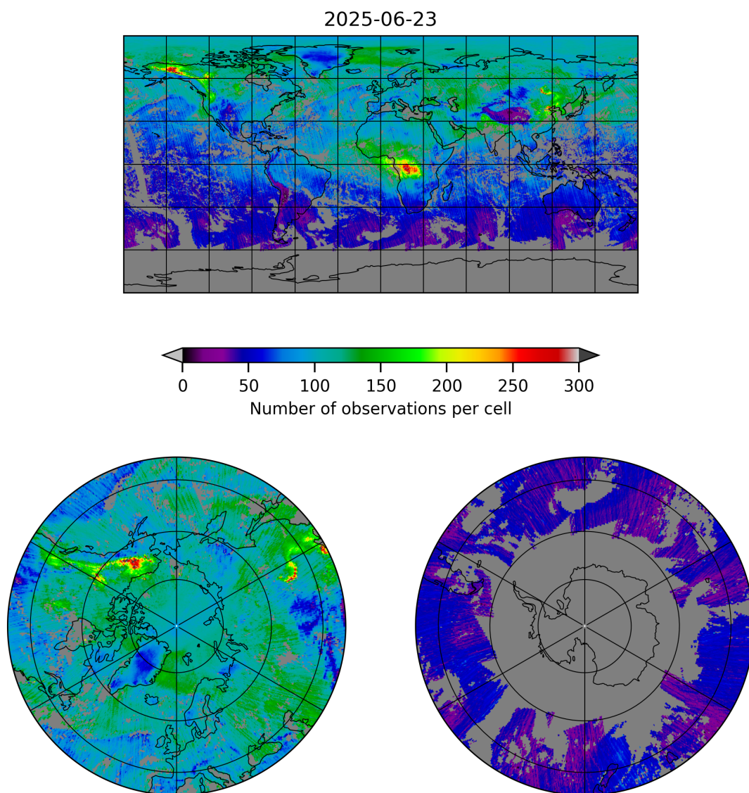
Figure 5: Map of the number of observations for 2025-06-23 to 2025-06-24
