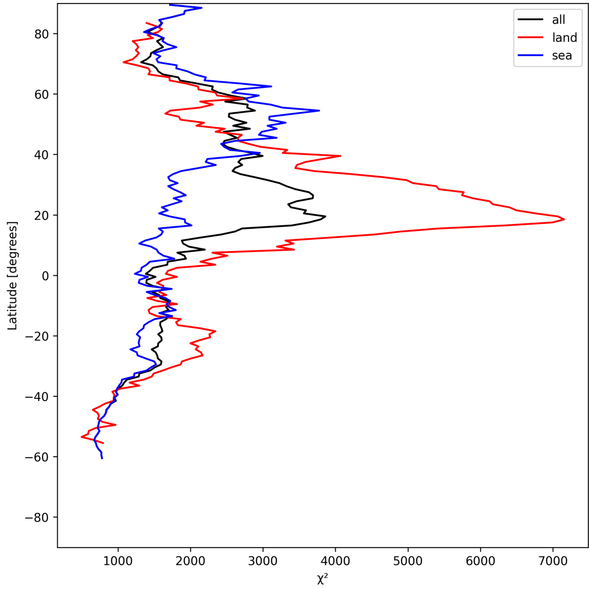
Figure 10: Zonal average of “ \chi^2 ” for 2025-06-23 to 2025-06-24.
