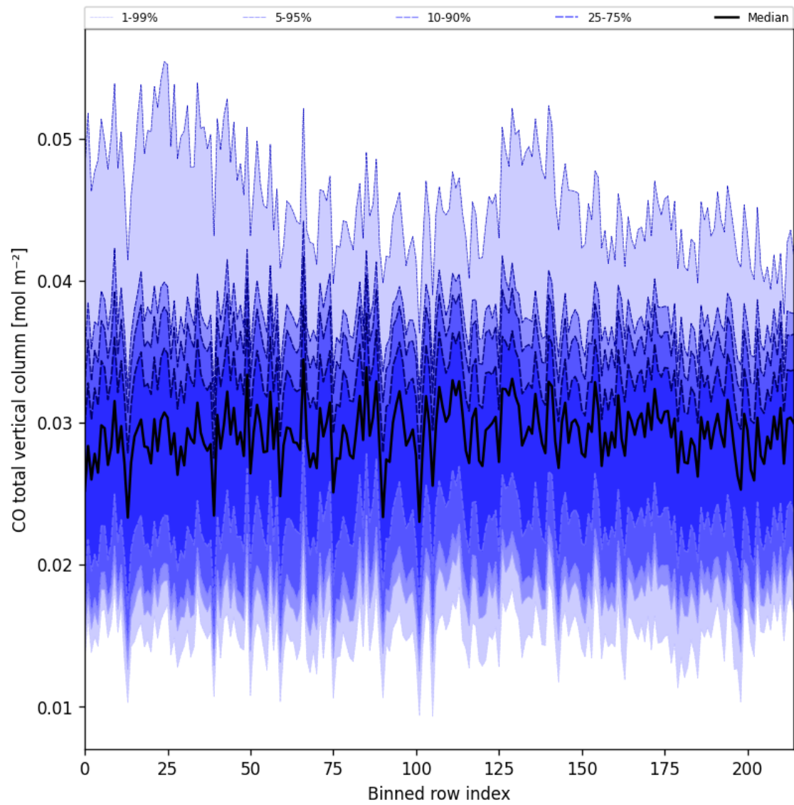
Figure 21: Along track statistics of “CO total vertical column” for 2025-06-23 to 2025-06-24
