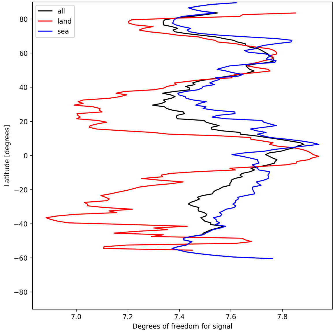
Figure 11: Zonal average of “Degrees of freedom for signal” for 2025-06-23 to 2025-06-24.
