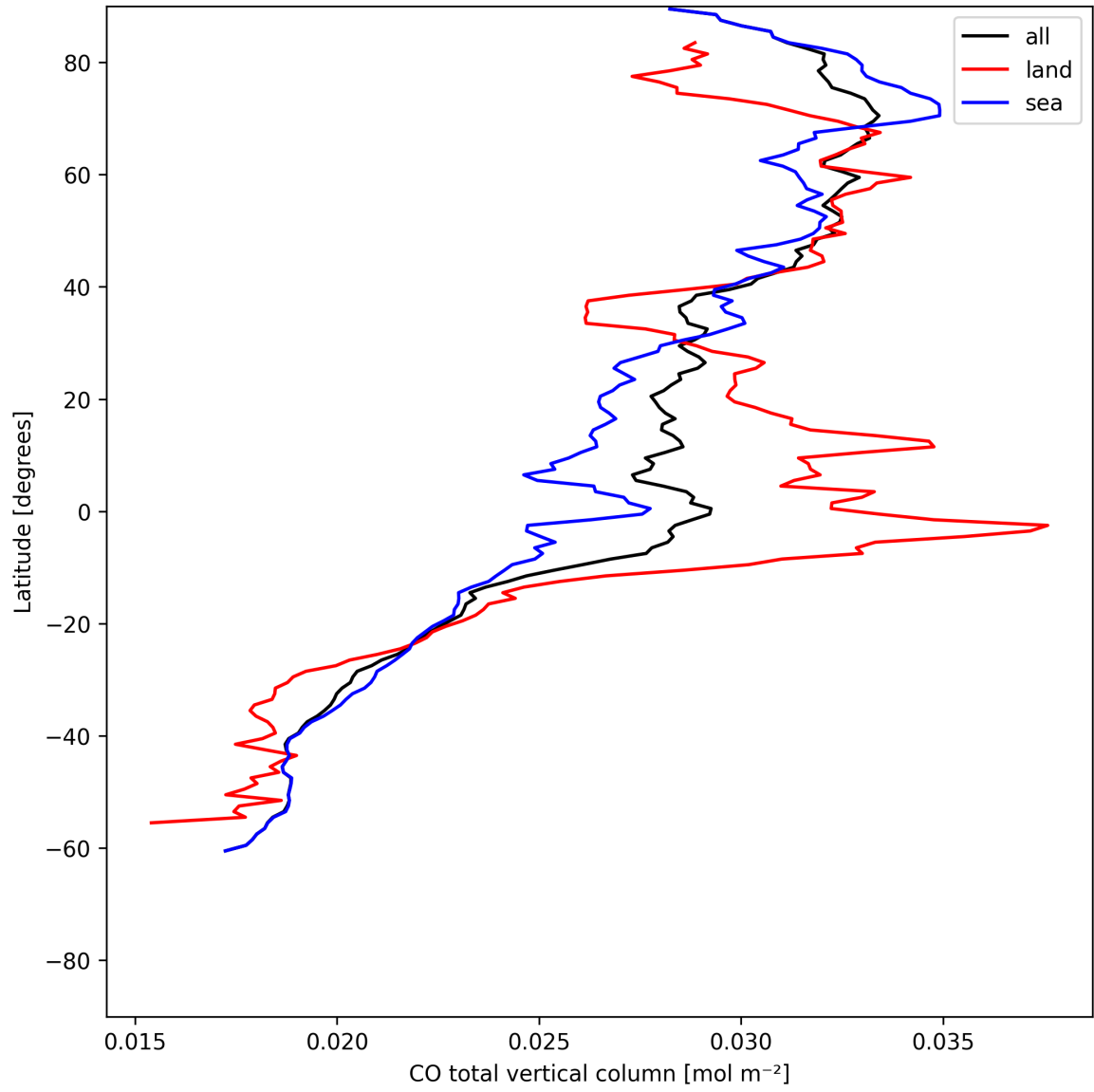
Figure 7: Zonal average of “CO total vertical column” for 2025-06-23 to 2025-06-24.
