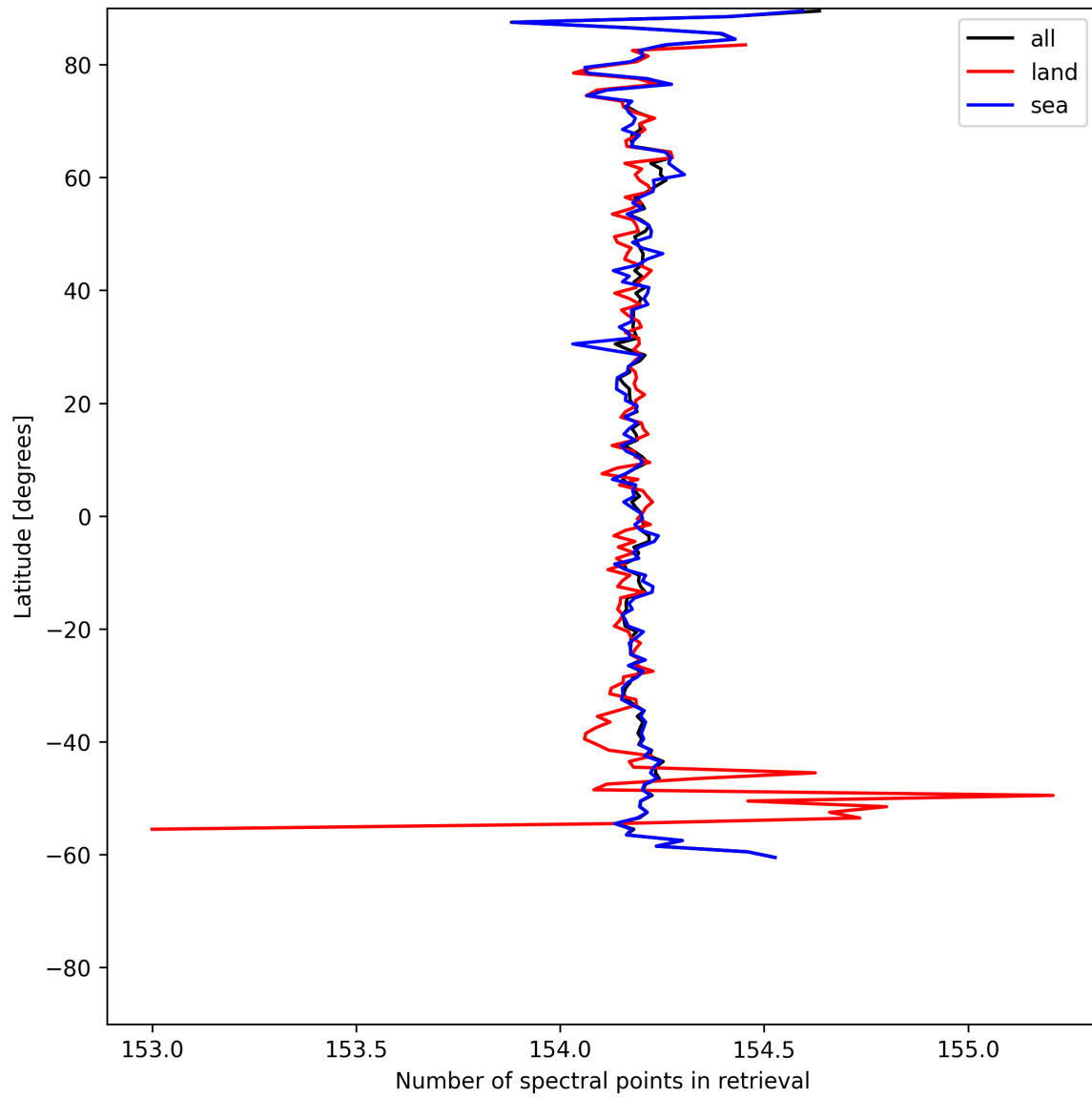
Figure 9: Zonal average of “Number of spectral points in retrieval” for 2025-06-23 to 2025-06-24.
