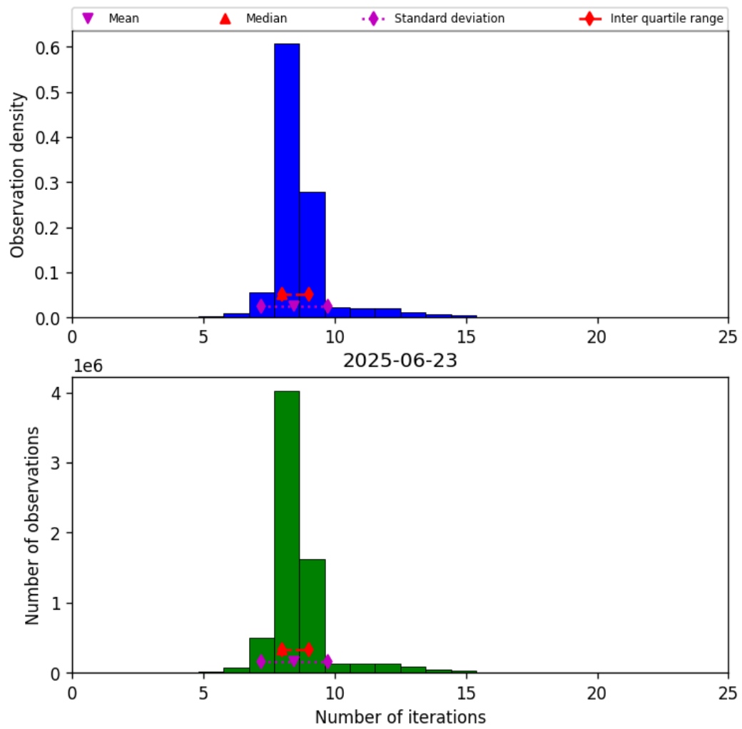
Figure 19: Histogram of “Number of iterations” for 2025-06-23 to 2025-06-24
