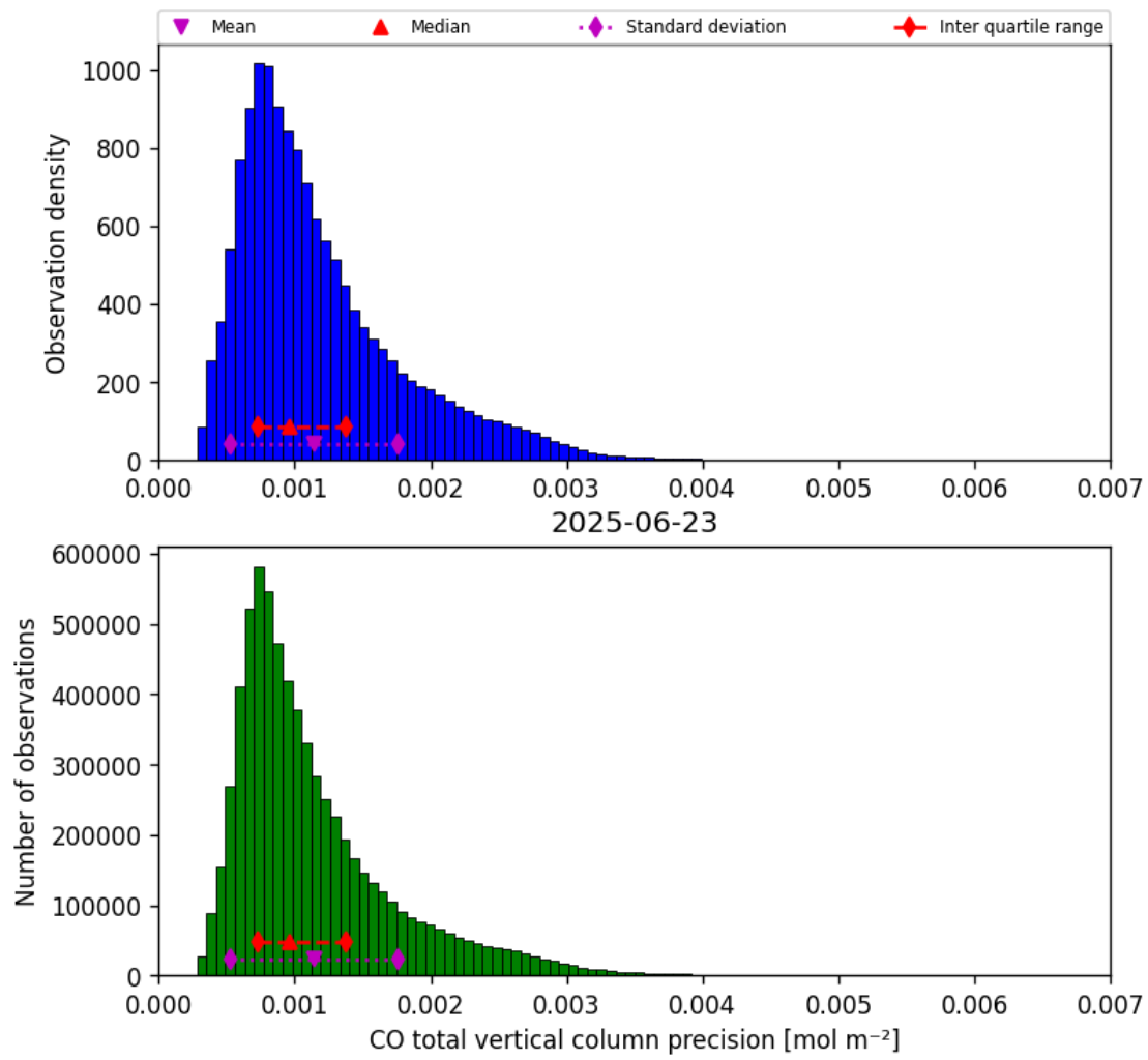
Figure 15: Histogram of “CO total vertical column precision” for 2025-06-23 to 2025-06-24
