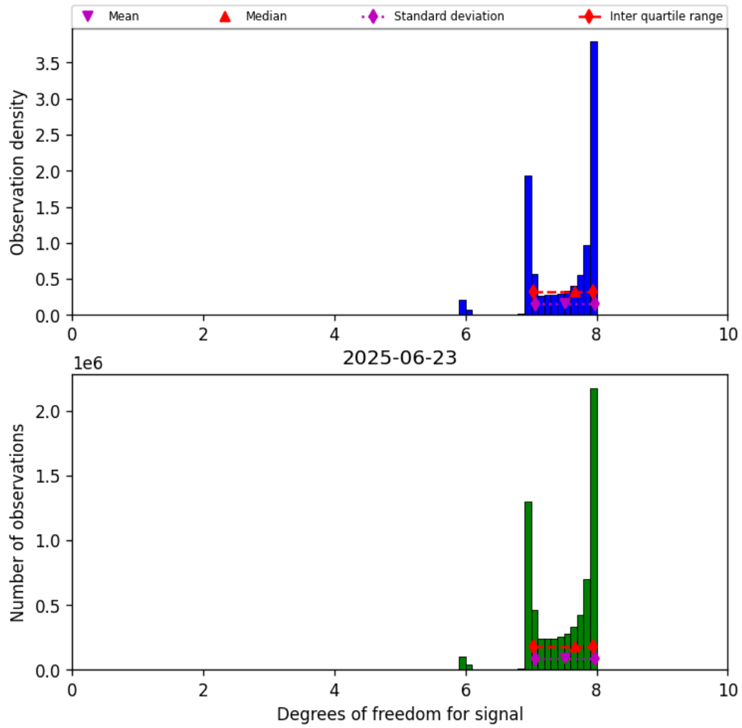
Figure 18: Histogram of “Degrees of freedom for signal” for 2025-06-23 to 2025-06-24
