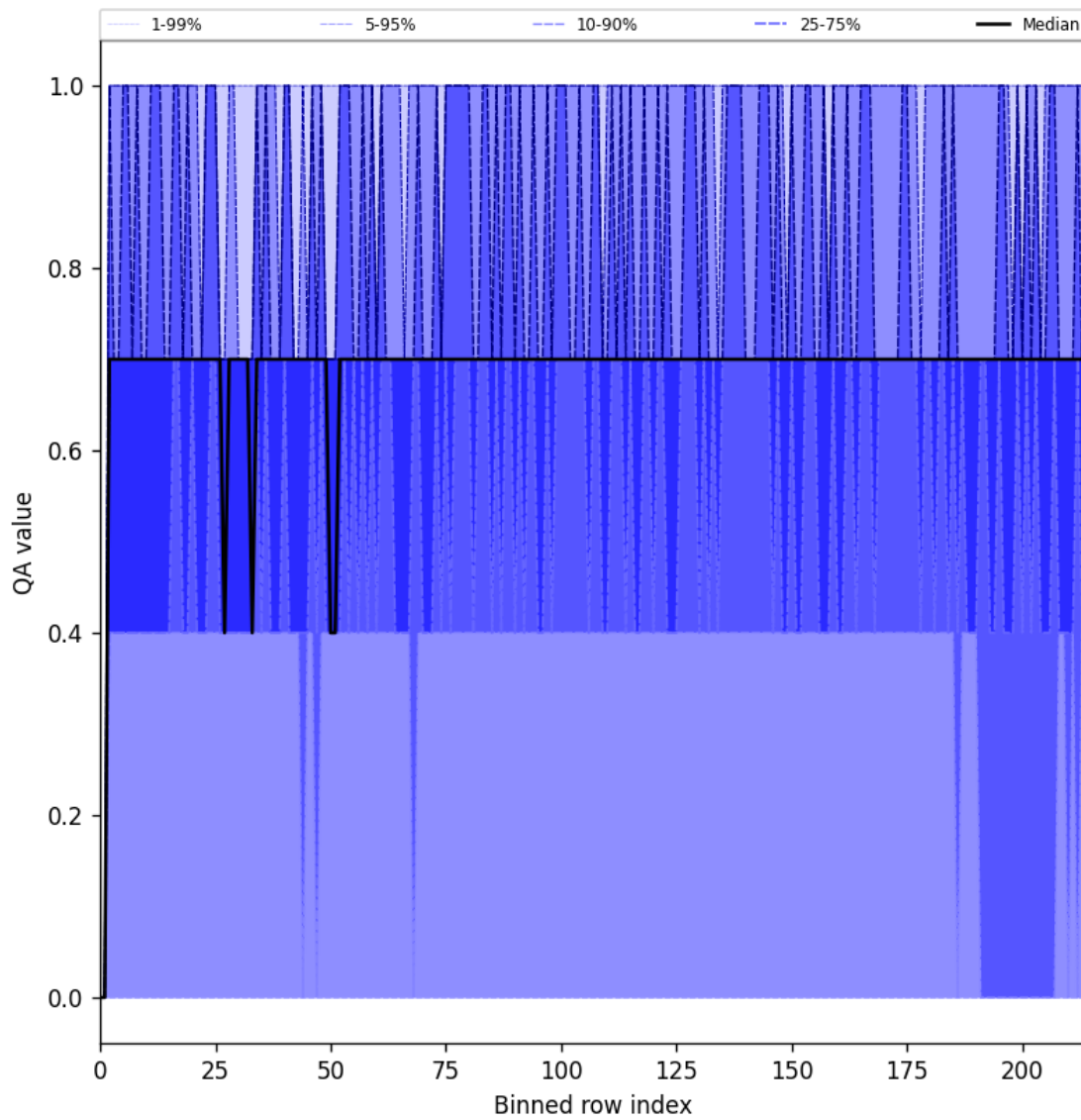
Figure 20: Along track statistics of “QA value” for 2025-06-23 to 2025-06-24
