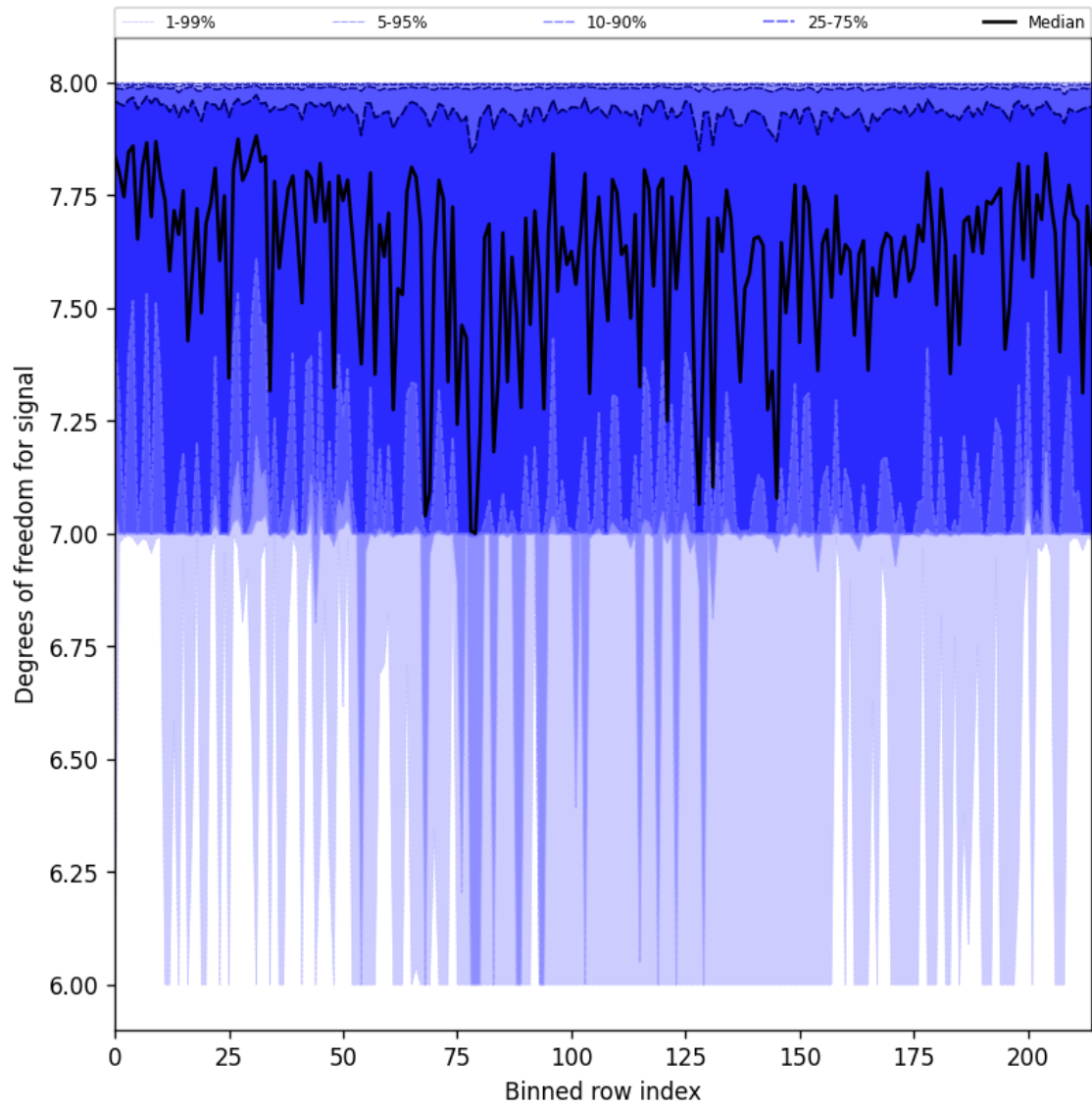
Figure 25: Along track statistics of “Degrees of freedom for signal” for 2025-06-23 to 2025-06-24
