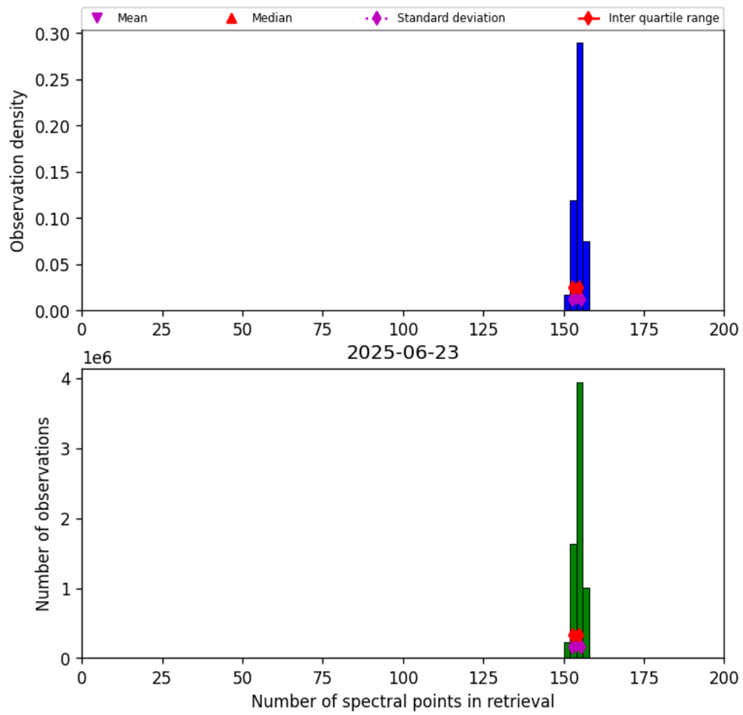
Figure 16: Histogram of "Number of spectral points in retrieval" for 2025-06-23 to 2025-06-24
