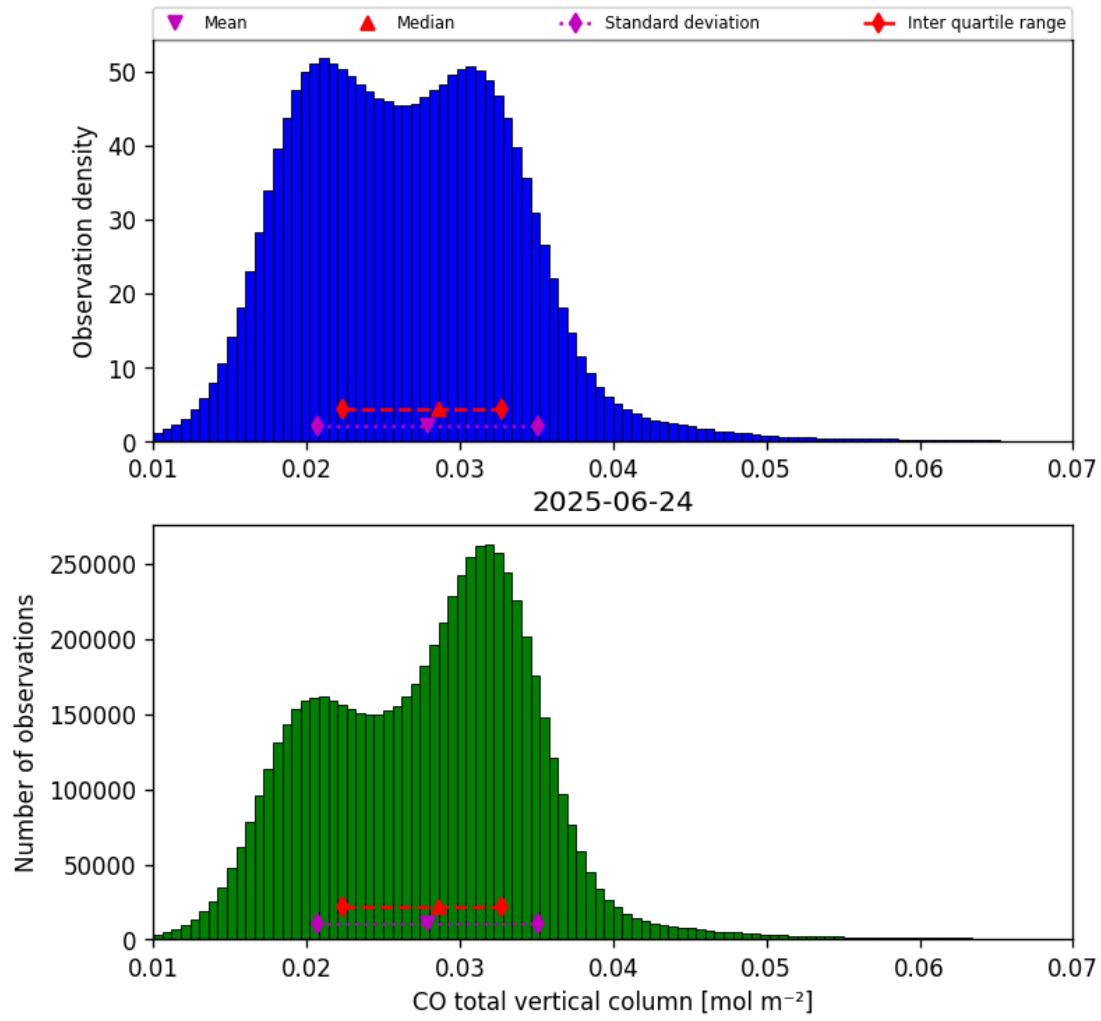
Figure 14: Histogram of “CO total vertical column” for 2025-06-24 to 2025-06-25
