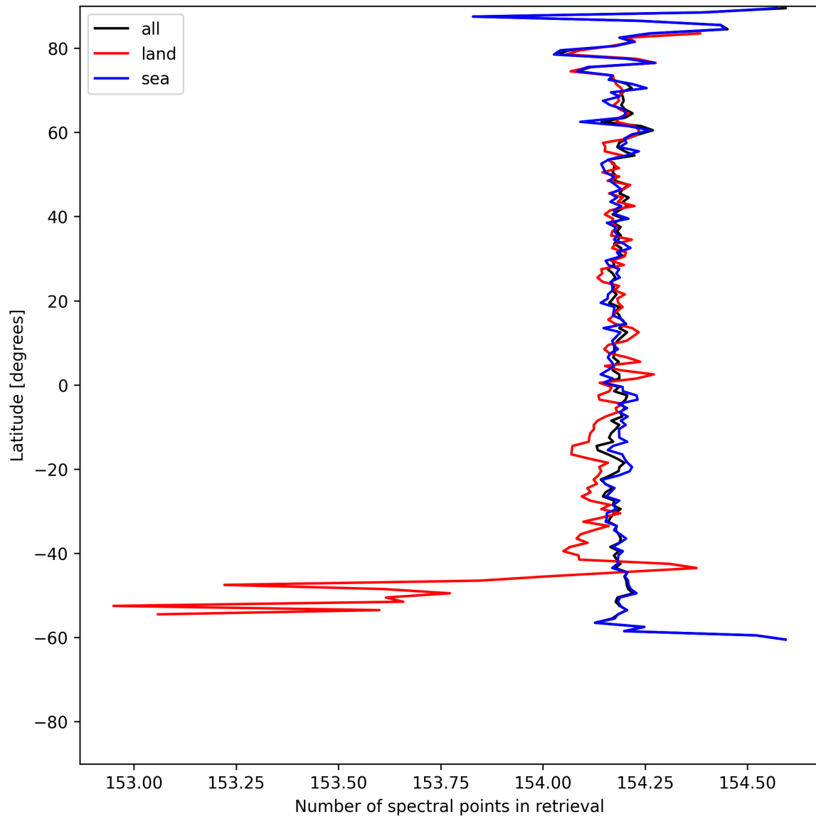
Figure 9: Zonal average of “Number of spectral points in retrieval” for 2025-06-24 to 2025-06-25.
