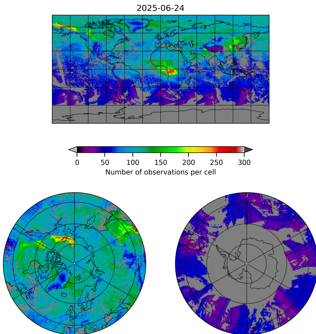
Figure 5: Map of the number of observations for 2025-06-24 to 2025-06-25
