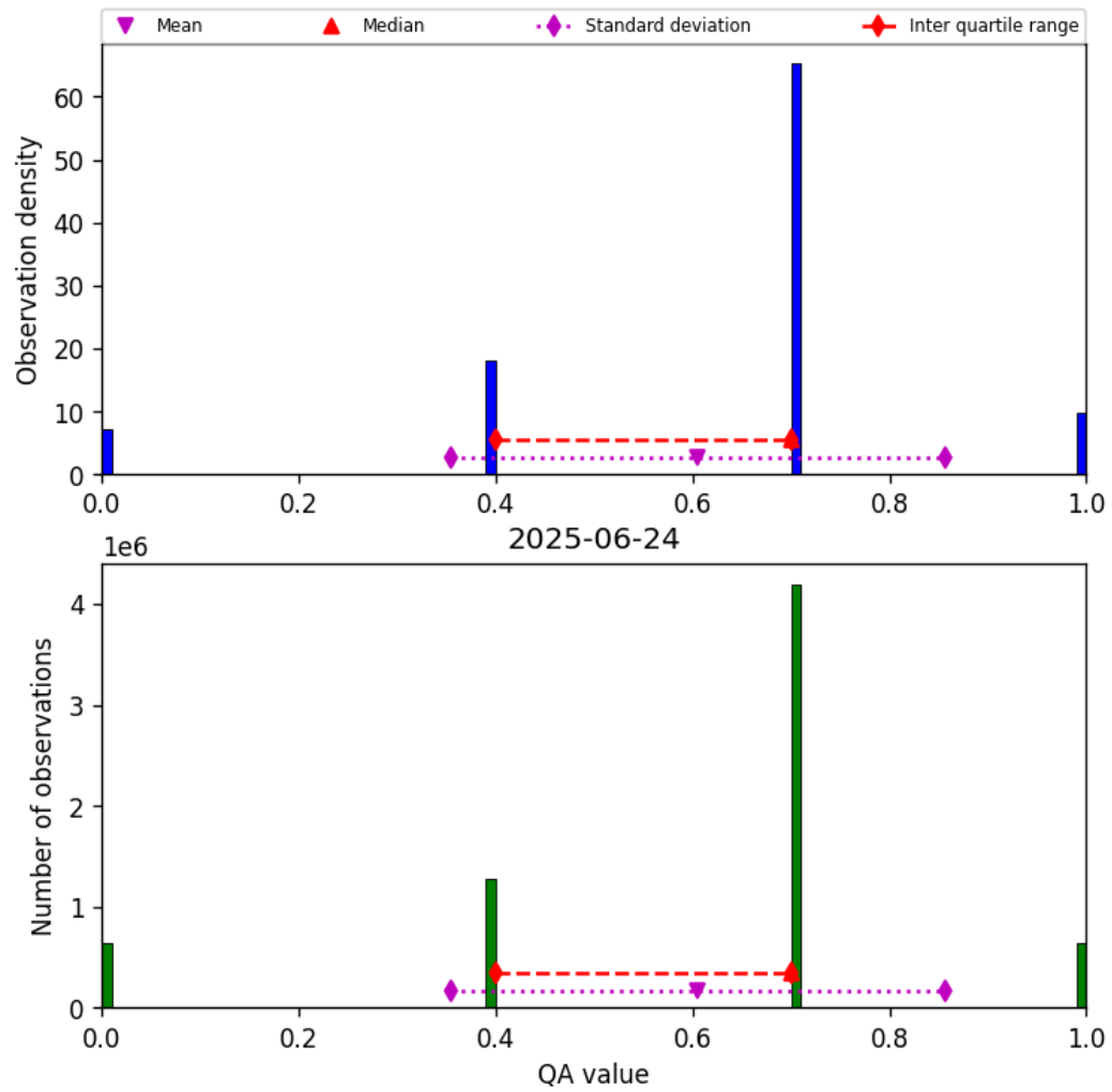
Figure 13: Histogram of “QA value” for 2025-06-24 to 2025-06-25
