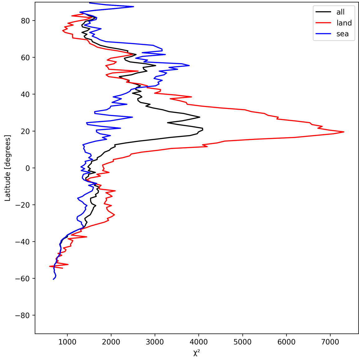
Figure 10: Zonal average of “ \chi^2 ” for 2025-06-24 to 2025-06-25.
