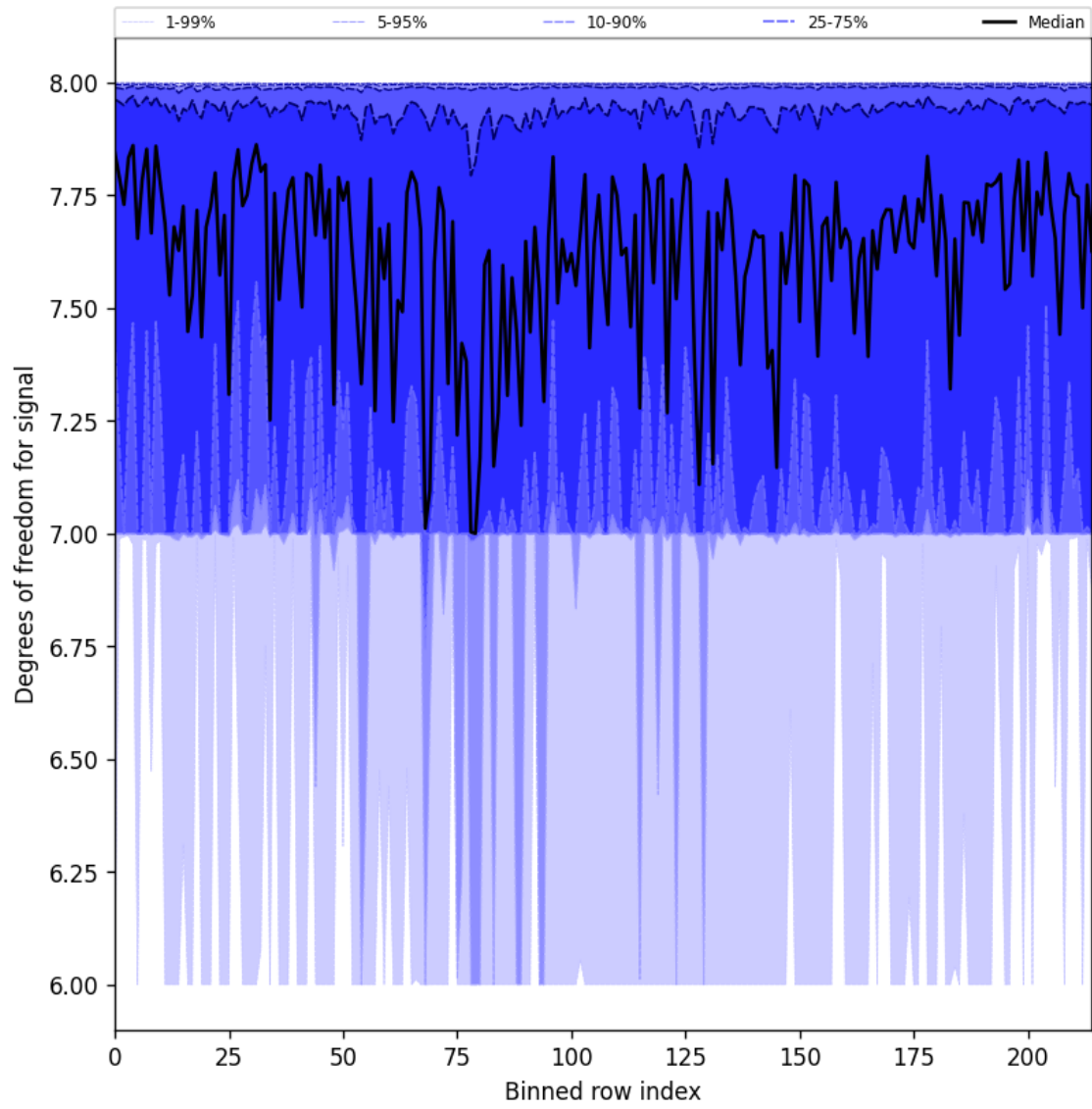
Figure 25: Along track statistics of “Degrees of freedom for signal” for 2025-06-24 to 2025-06-25
