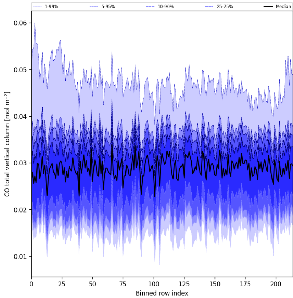
Figure 21: Along track statistics of “CO total vertical column” for 2025-06-24 to 2025-06-25
