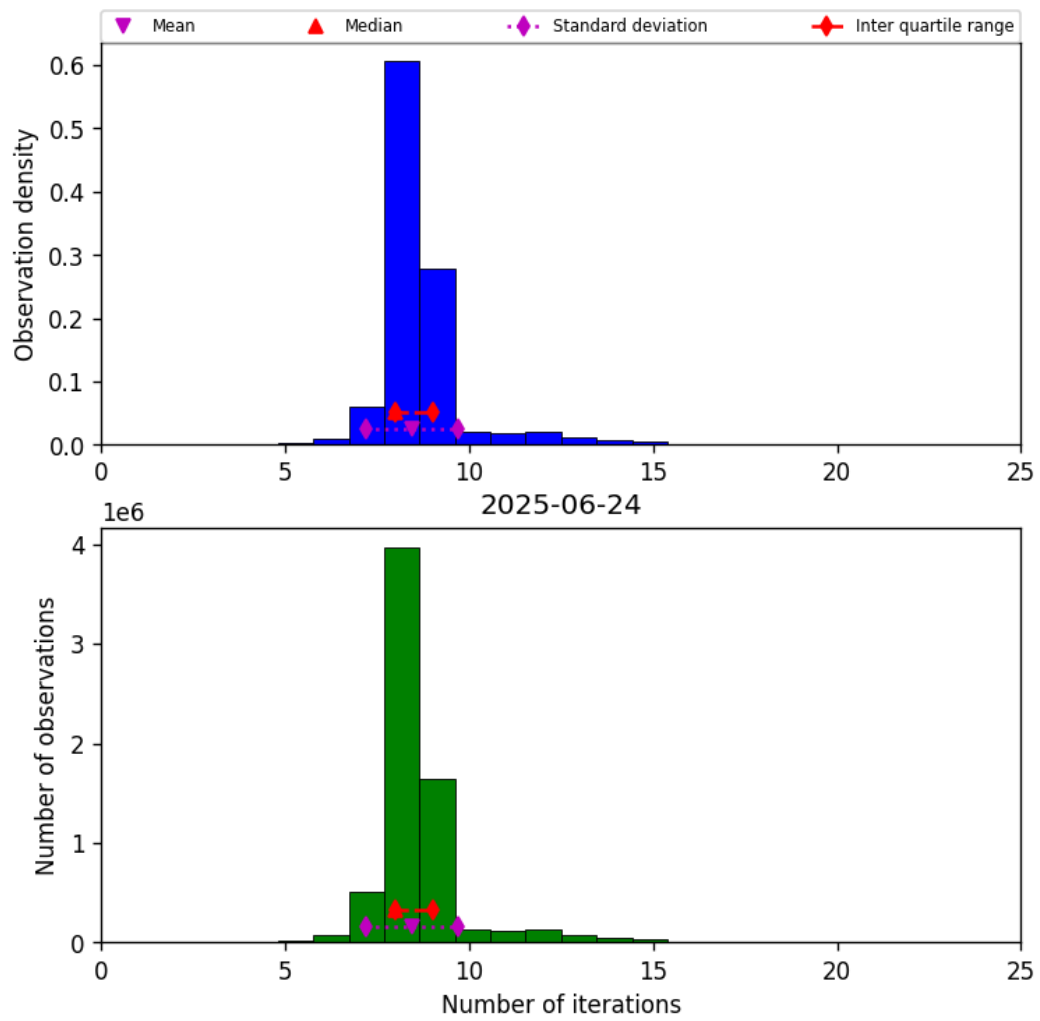
Figure 19: Histogram of “Number of iterations” for 2025-06-24 to 2025-06-25
