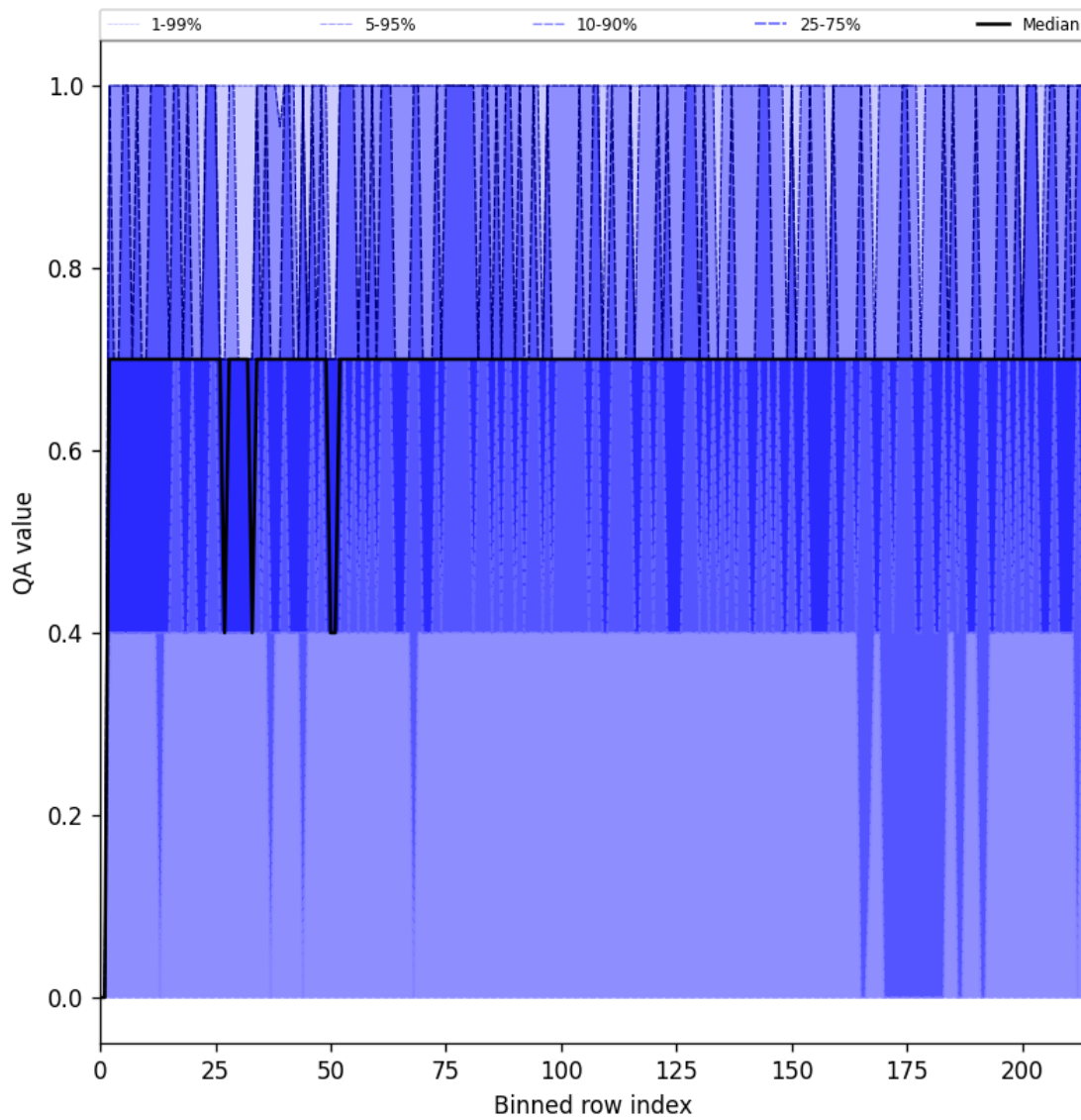
Figure 20: Along track statistics of “QA value” for 2025-06-24 to 2025-06-25
