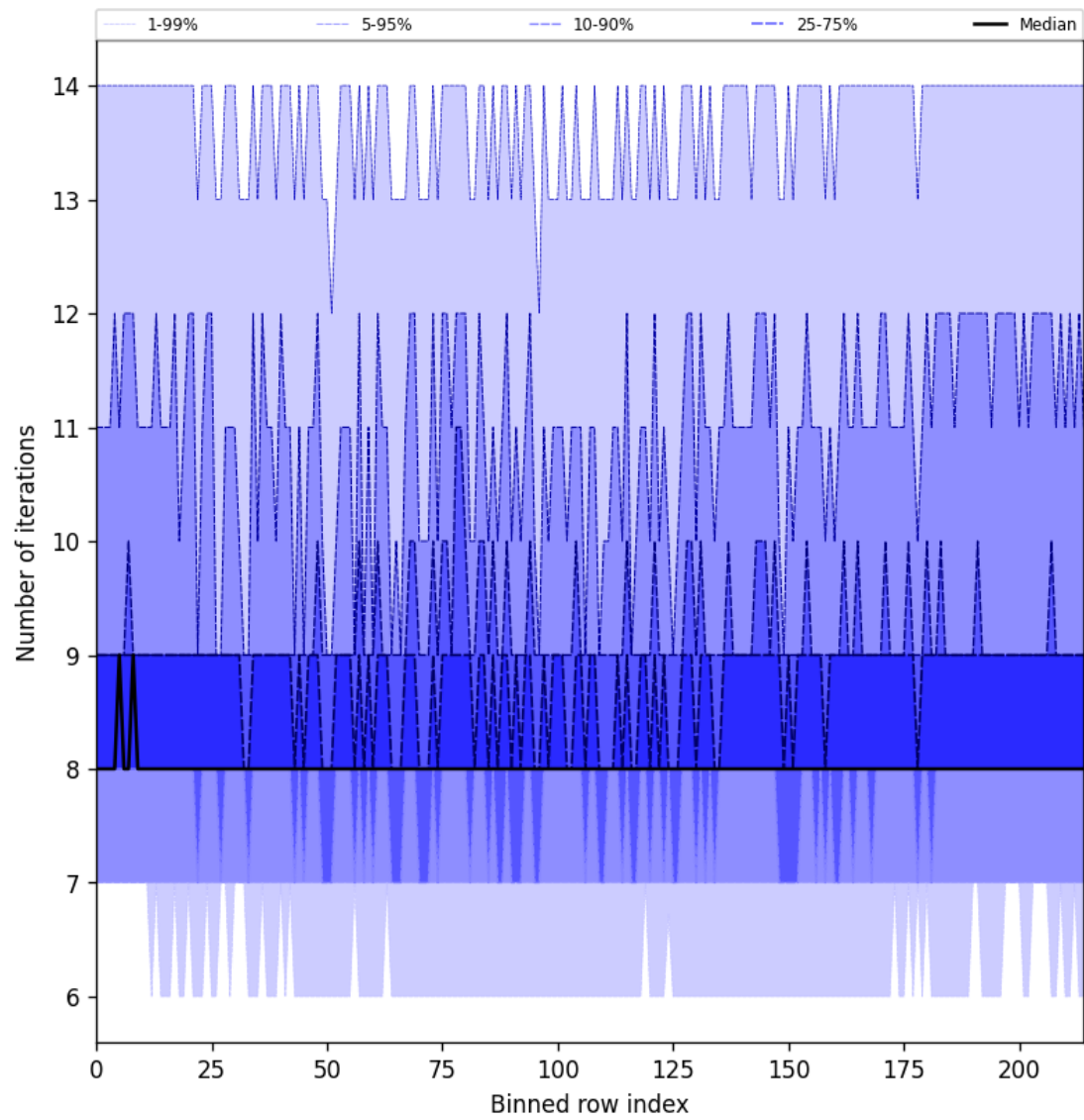
Figure 26: Along track statistics of “Number of iterations” for 2025-06-24 to 2025-06-25
