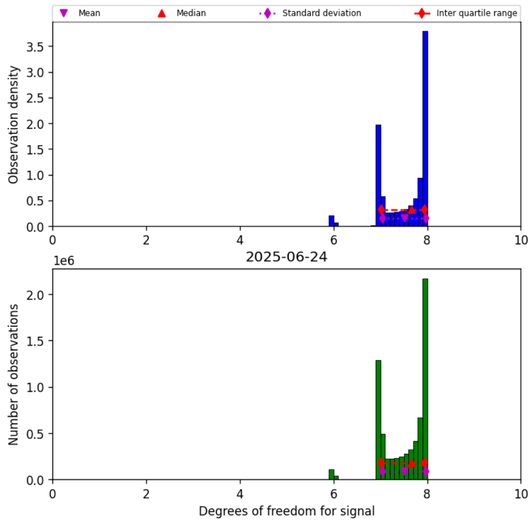
Figure 18: Histogram of “Degrees of freedom for signal” for 2025-06-24 to 2025-06-25
