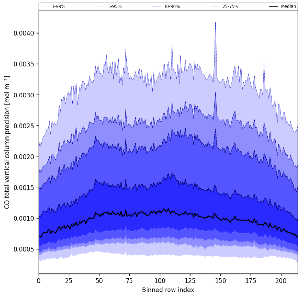
Figure 22: Along track statistics of “CO total vertical column precision” for 2025-06-24 to 2025-06-25
