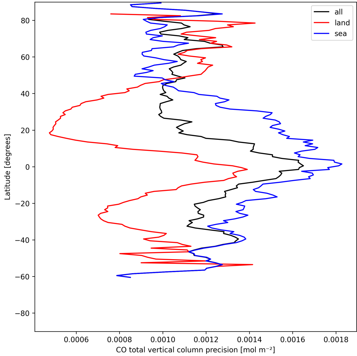
Figure 8: Zonal average of “CO total vertical column precision” for 2025-06-24 to 2025-06-25.
