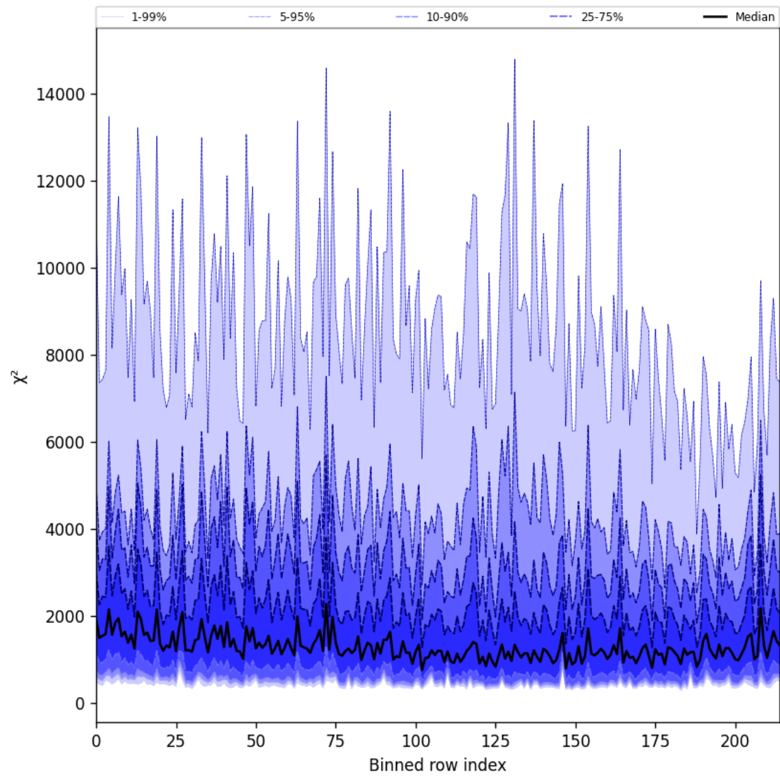
Figure 24: Along track statistics of “ \chi^2 ” for 2025-06-24 to 2025-06-25
