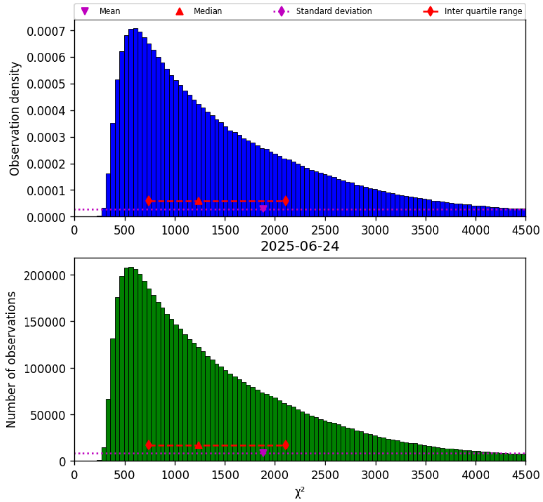
Figure 17: Histogram of “ \chi^2 ” for 2025-06-24 to 2025-06-25
