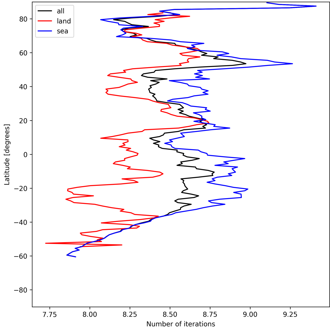
Figure 12: Zonal average of “Number of iterations” for 2025-06-24 to 2025-06-25.
