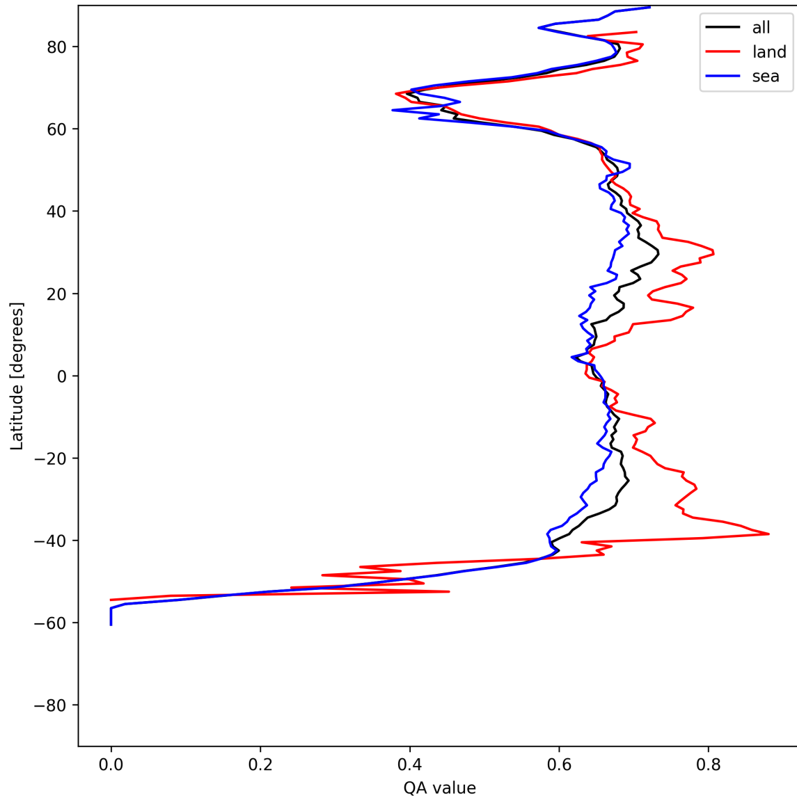
Figure 6: Zonal average of “QA value” for 2025-06-24 to 2025-06-25.
