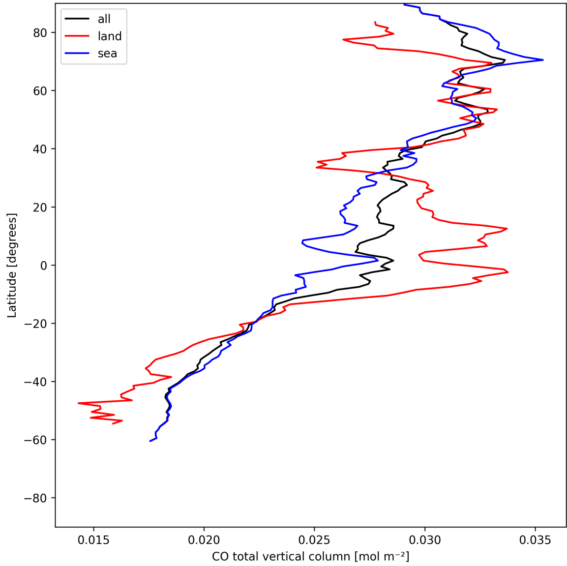
Figure 7: Zonal average of “CO total vertical column” for 2025-06-24 to 2025-06-25.
