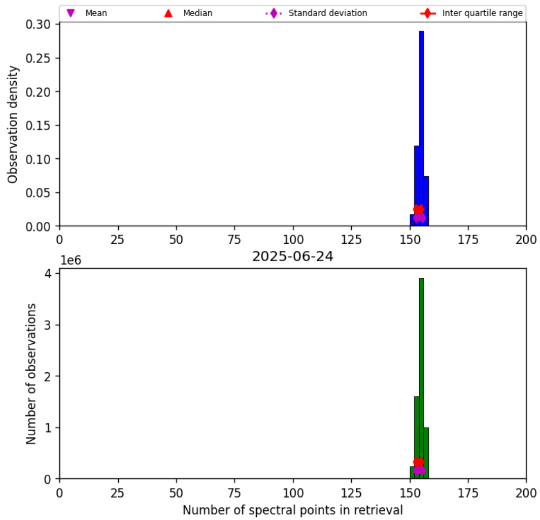
Figure 16: Histogram of “Number of spectral points in retrieval” for 2025-06-24 to 2025-06-25
