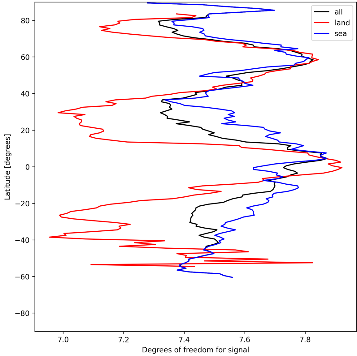
Figure 11: Zonal average of “Degrees of freedom for signal” for 2025-06-24 to 2025-06-25.
