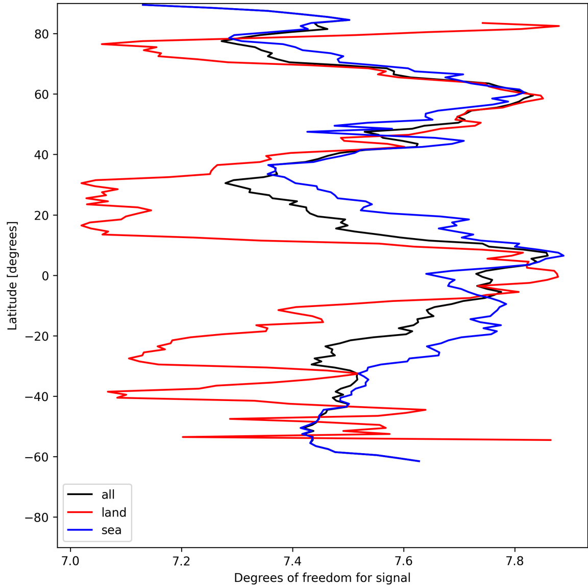
Figure 11: Zonal average of “Degrees of freedom for signal” for 2025-06-25 to 2025-06-25.
