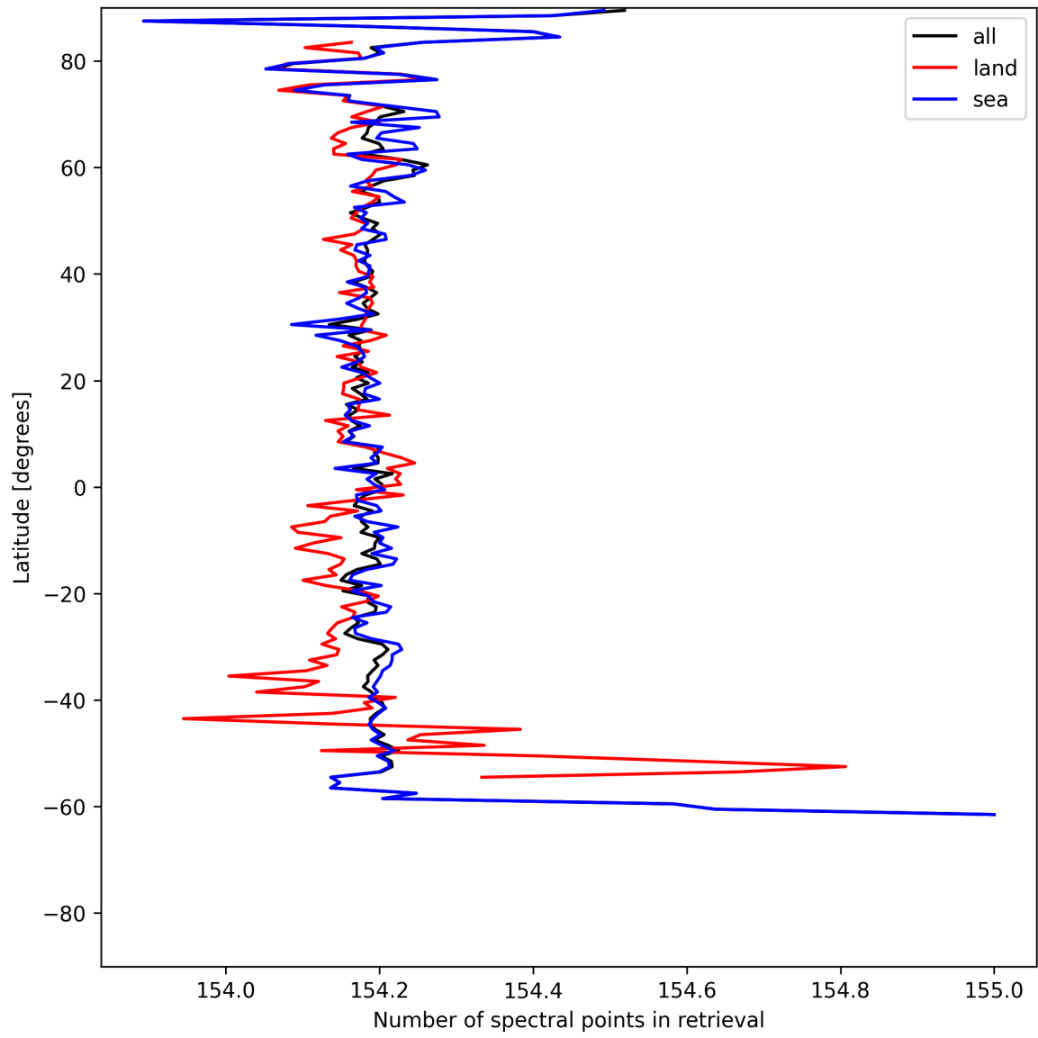
Figure 9: Zonal average of “Number of spectral points in retrieval” for 2025-06-25 to 2025-06-25.
