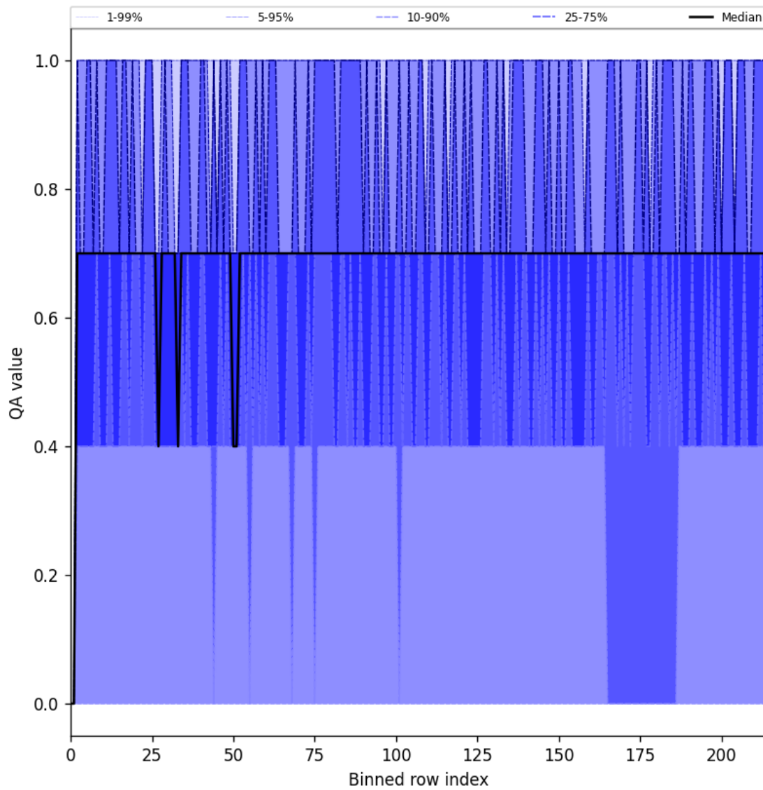
Figure 20: Along track statistics of “QA value” for 2025-06-25 to 2025-06-25
