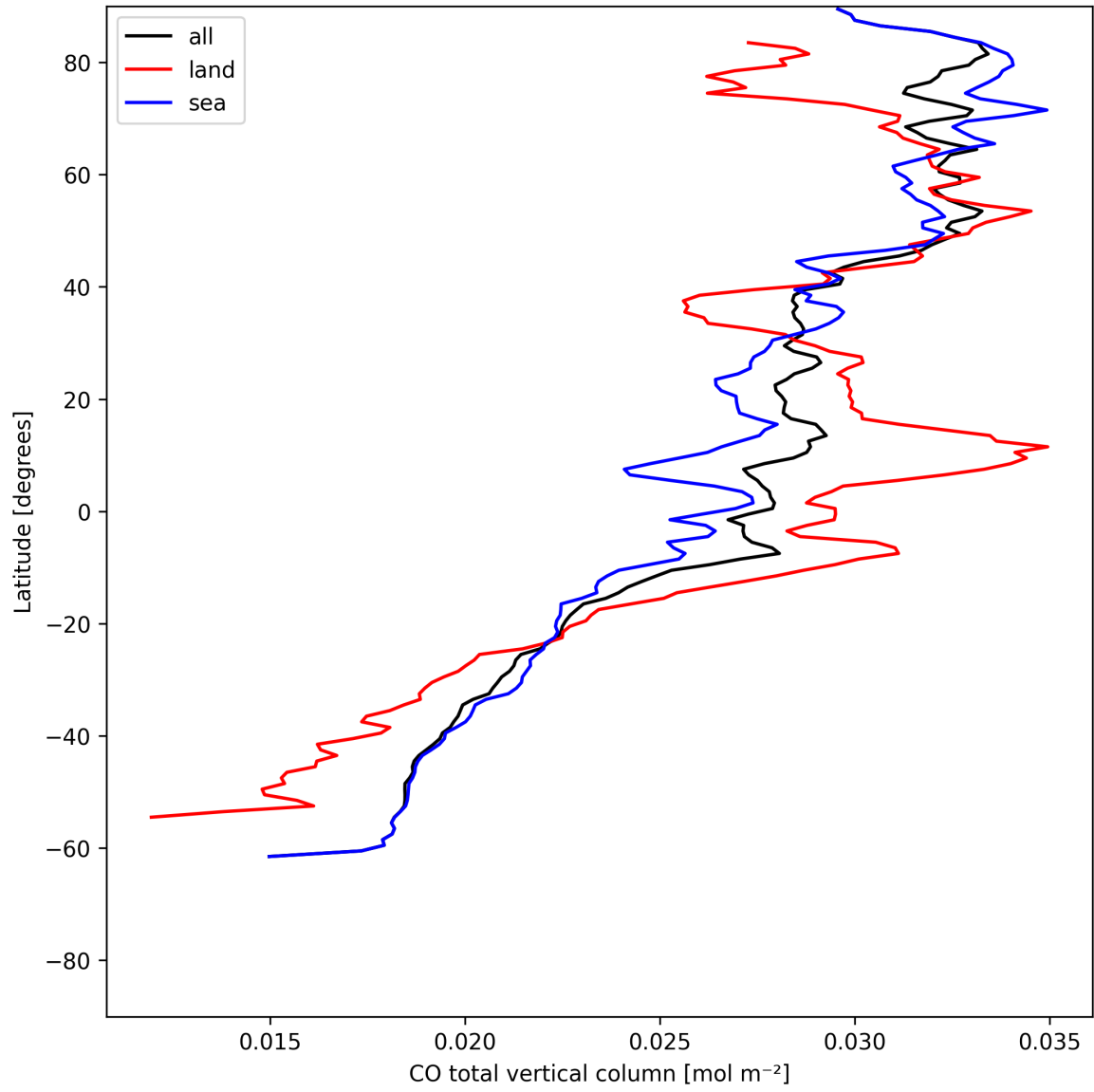
Figure 7: Zonal average of “CO total vertical column” for 2025-06-25 to 2025-06-25.
