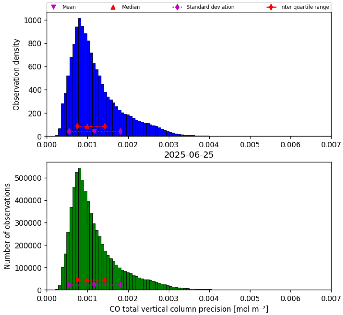
Figure 15: Histogram of “CO total vertical column precision” for 2025-06-25 to 2025-06-25
