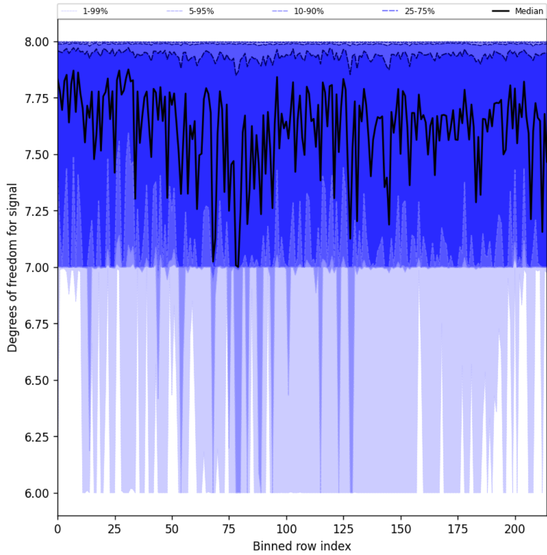
Figure 25: Along track statistics of “Degrees of freedom for signal” for 2025-06-25 to 2025-06-25
