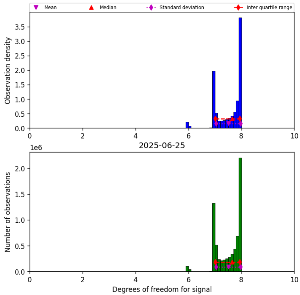
Figure 18: Histogram of “Degrees of freedom for signal” for 2025-06-25 to 2025-06-25
