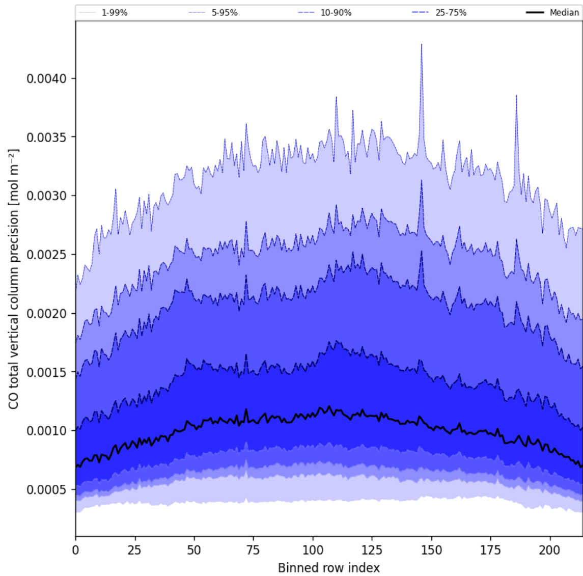
Figure 22: Along track statistics of “CO total vertical column precision” for 2025-06-25 to 2025-06-25
