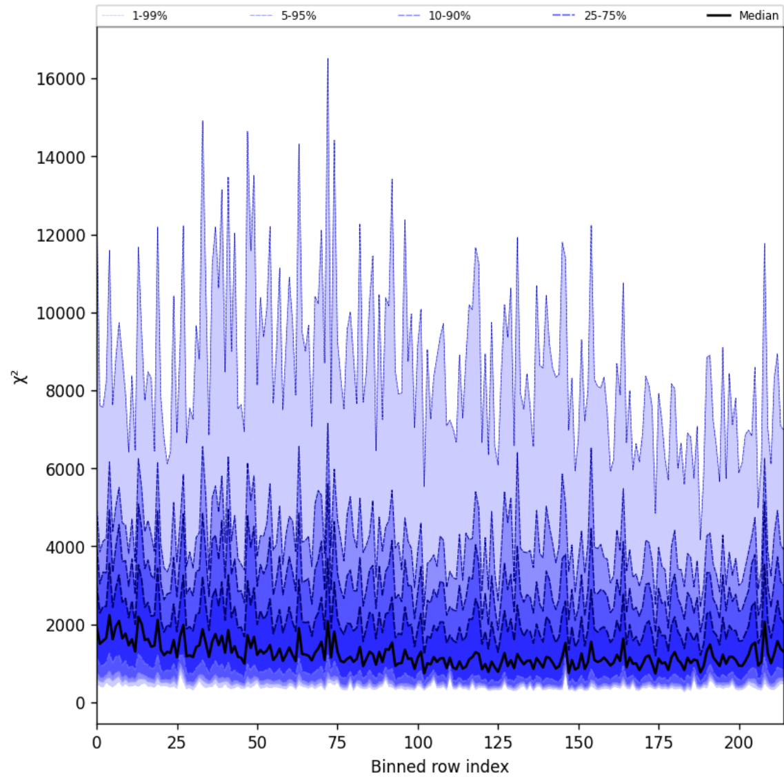
Figure 24: Along track statistics of “ \chi^2 ” for 2025-06-25 to 2025-06-25
