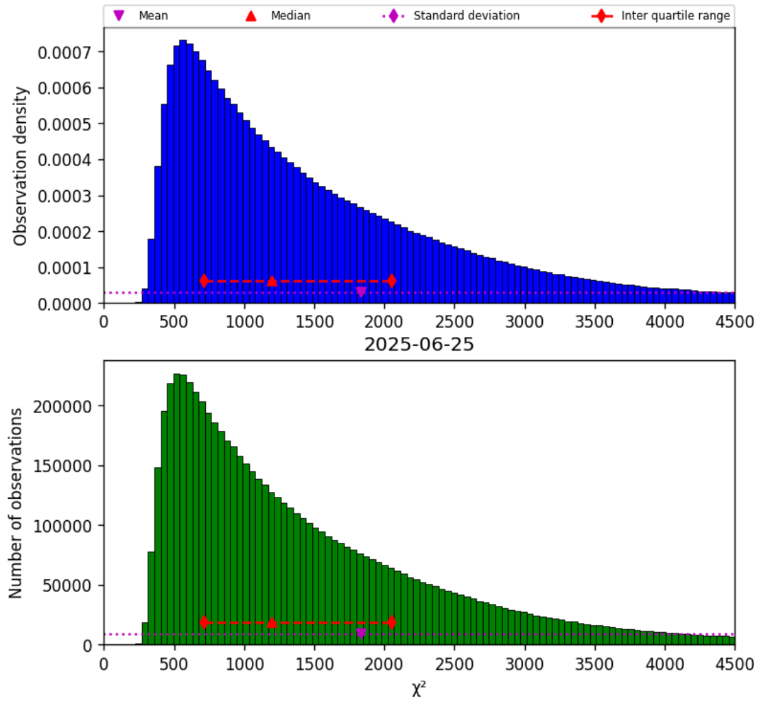
Figure 17: Histogram of “ \chi^2 ” for 2025-06-25 to 2025-06-25
