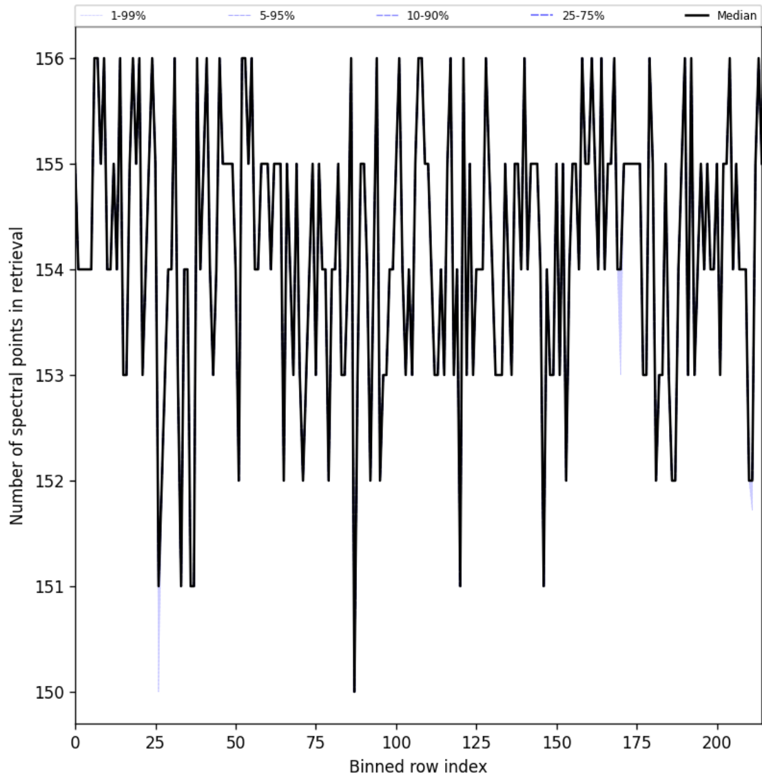
Figure 23: Along track statistics of “Number of spectral points in retrieval” for 2025-06-25 to 2025-06-25
