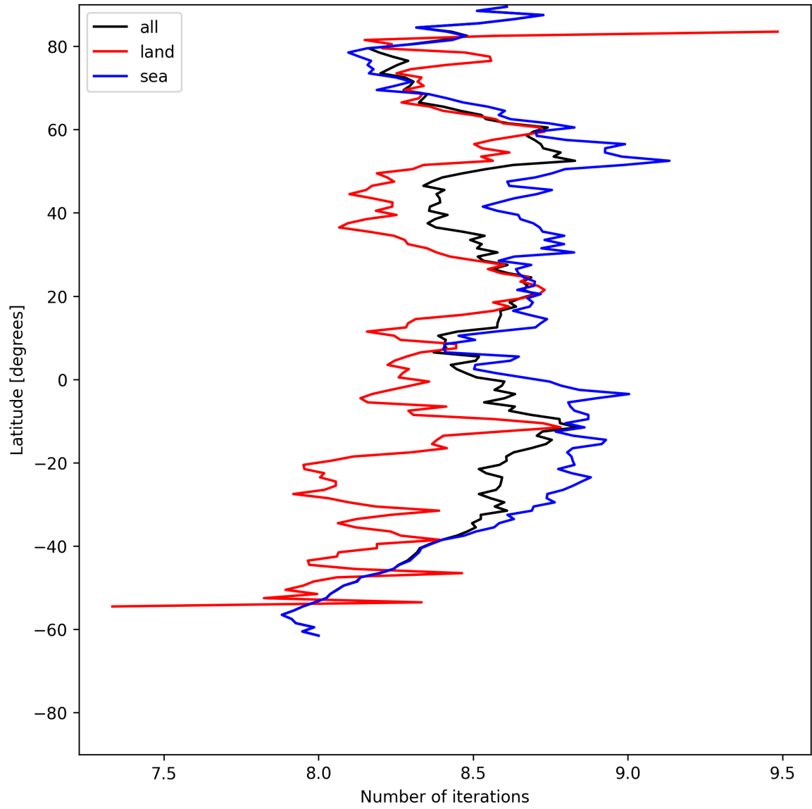
Figure 12: Zonal average of “Number of iterations” for 2025-06-25 to 2025-06-25.
