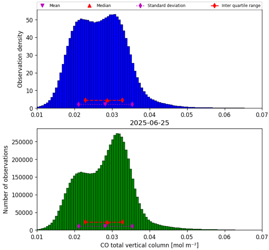
Figure 14: Histogram of “CO total vertical column” for 2025-06-25 to 2025-06-25
