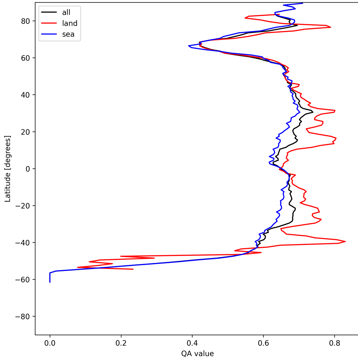
Figure 6: Zonal average of “QA value” for 2025-06-25 to 2025-06-25.
