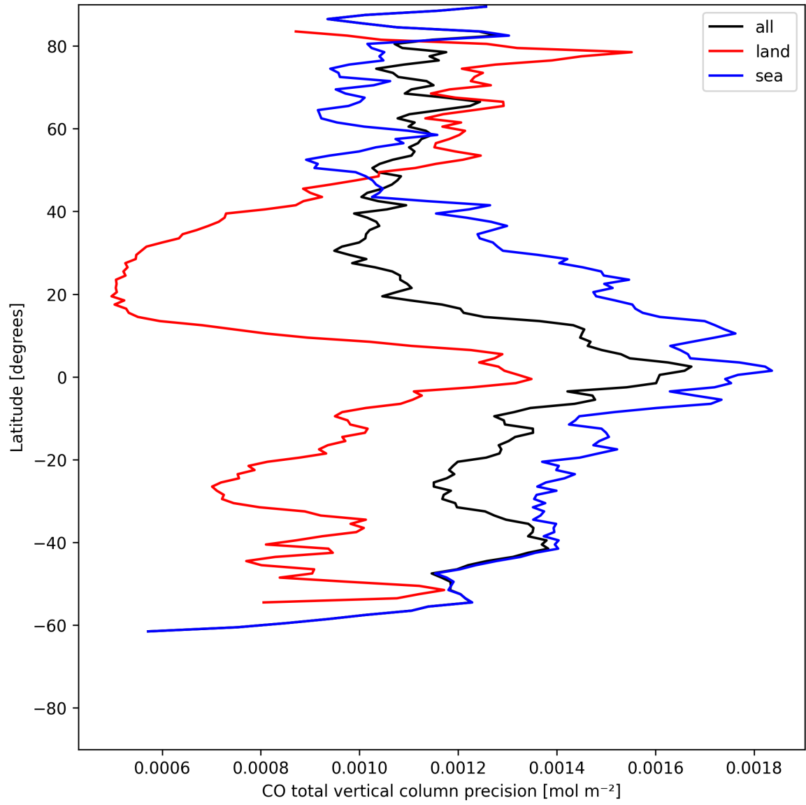
Figure 8: Zonal average of “CO total vertical column precision” for 2025-06-25 to 2025-06-25.
