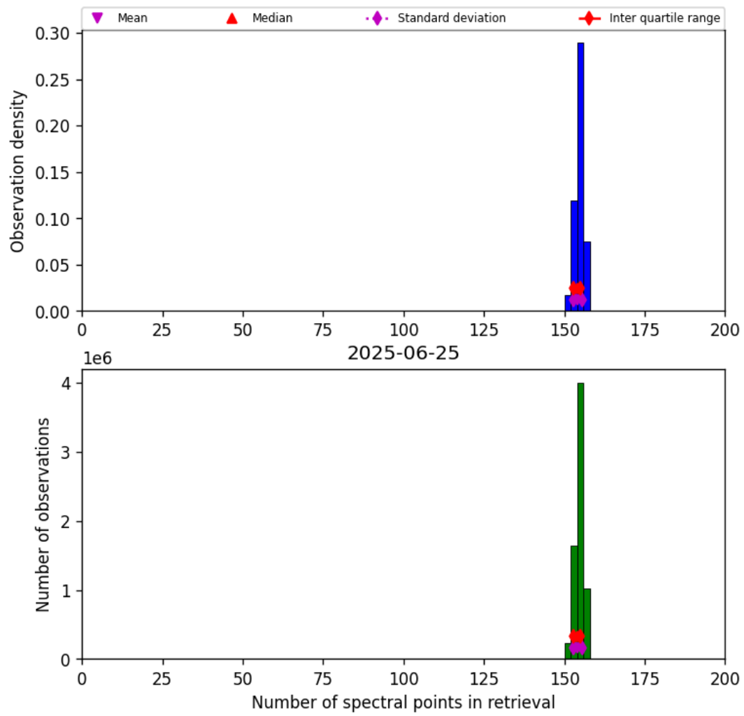
Figure 16: Histogram of “Number of spectral points in retrieval” for 2025-06-25 to 2025-06-25
