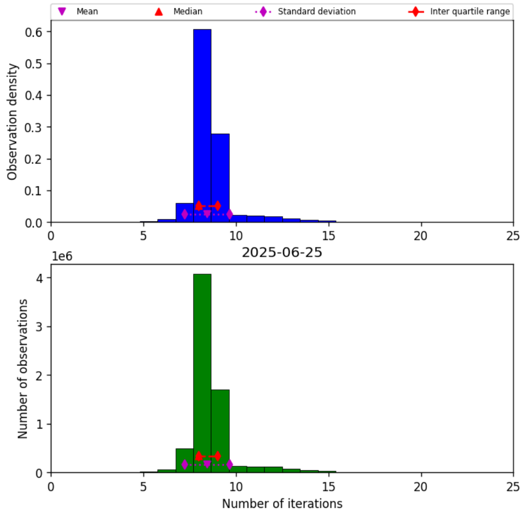
Figure 19: Histogram of “Number of iterations” for 2025-06-25 to 2025-06-25
