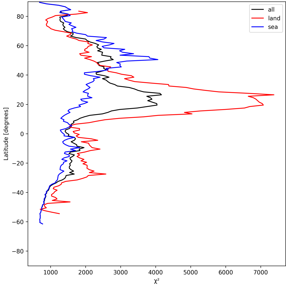
Figure 10: Zonal average of “ \chi^2 ” for 2025-06-25 to 2025-06-25.
