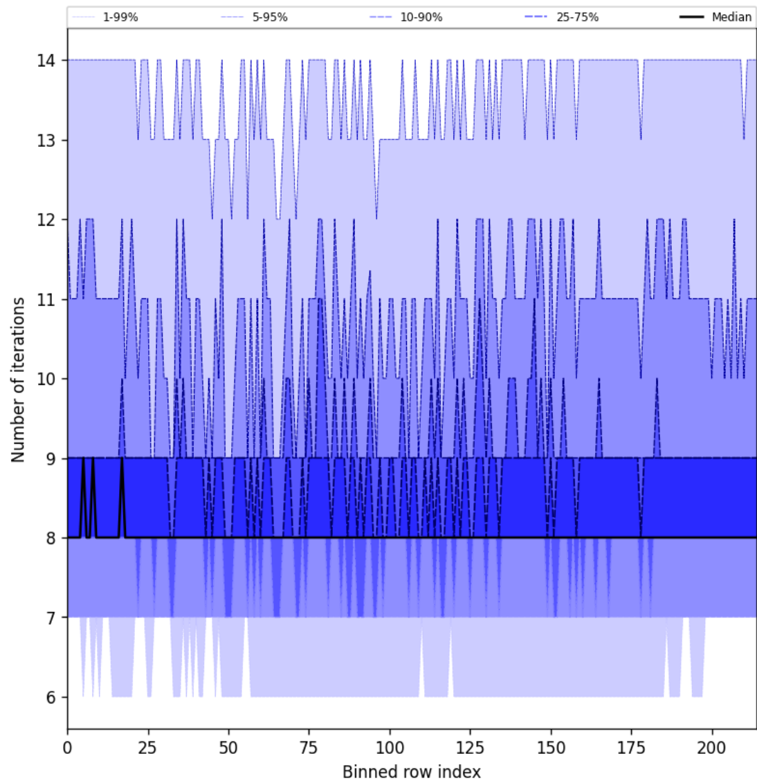
Figure 26: Along track statistics of “Number of iterations” for 2025-06-25 to 2025-06-25
