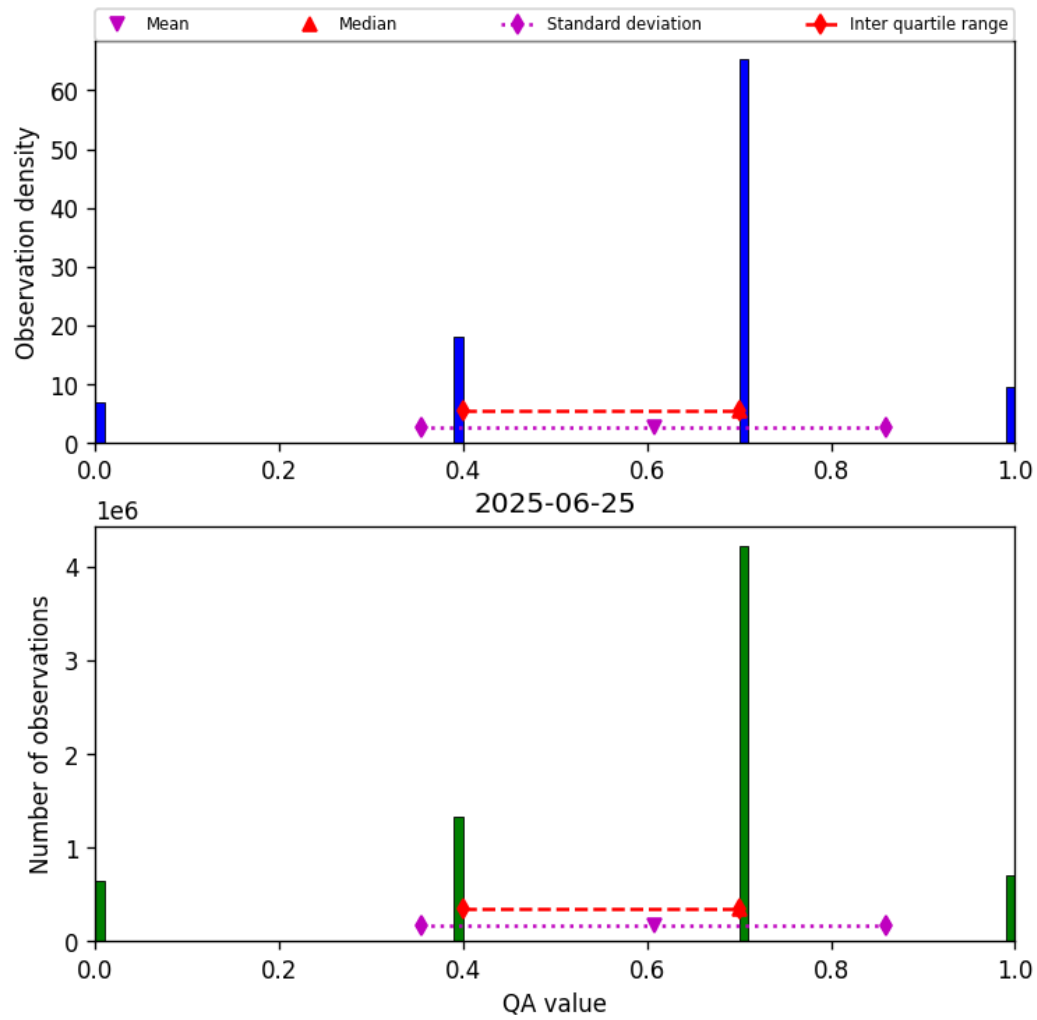
Figure 13: Histogram of “QA value” for 2025-06-25 to 2025-06-25
