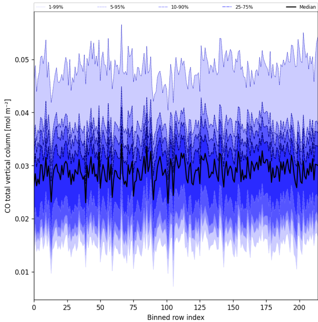
Figure 21: Along track statistics of “CO total vertical column” for 2025-06-25 to 2025-06-25
