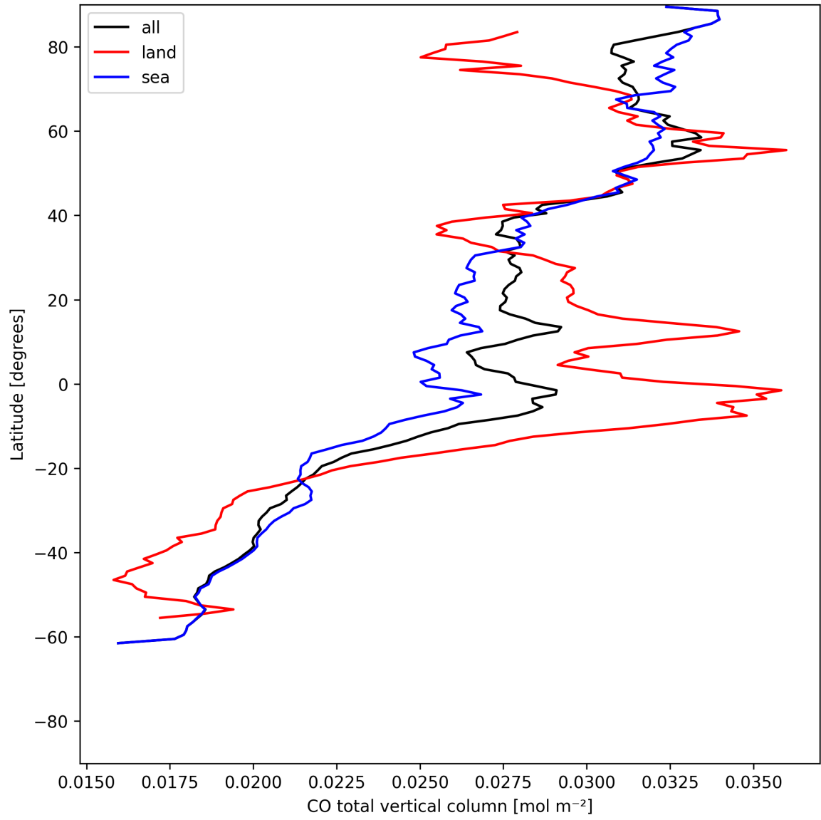
Figure 7: Zonal average of “CO total vertical column” for 2025-06-27 to 2025-06-28.
