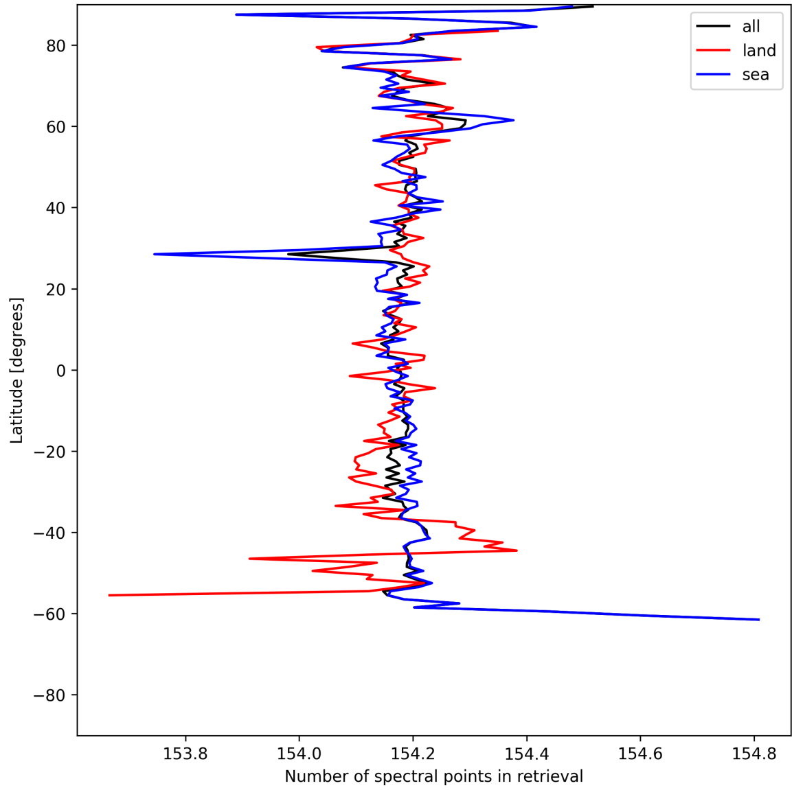
Figure 9: Zonal average of “Number of spectral points in retrieval” for 2025-06-27 to 2025-06-28.
