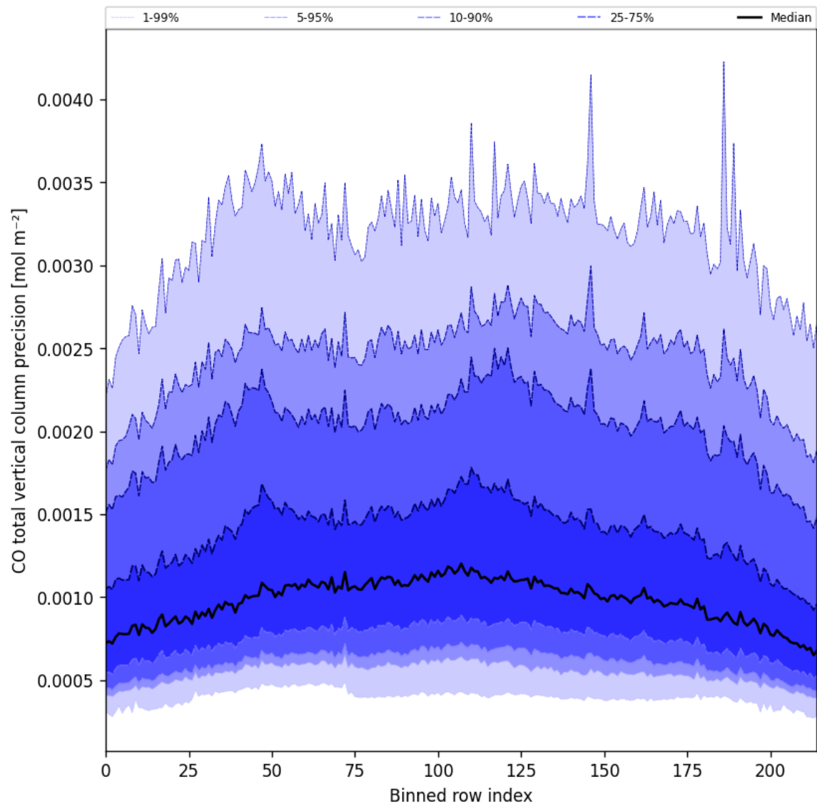
Figure 22: Along track statistics of “CO total vertical column precision” for 2025-06-27 to 2025-06-28
