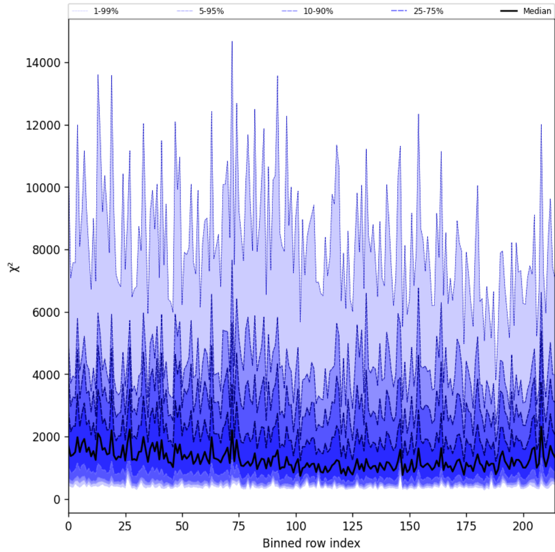
Figure 24: Along track statistics of “ \chi^2 ” for 2025-06-27 to 2025-06-28
