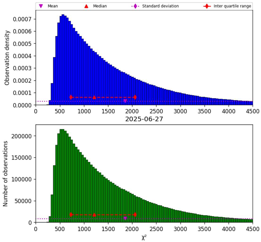
Figure 17: Histogram of “ \chi^2 ” for 2025-06-27 to 2025-06-28
