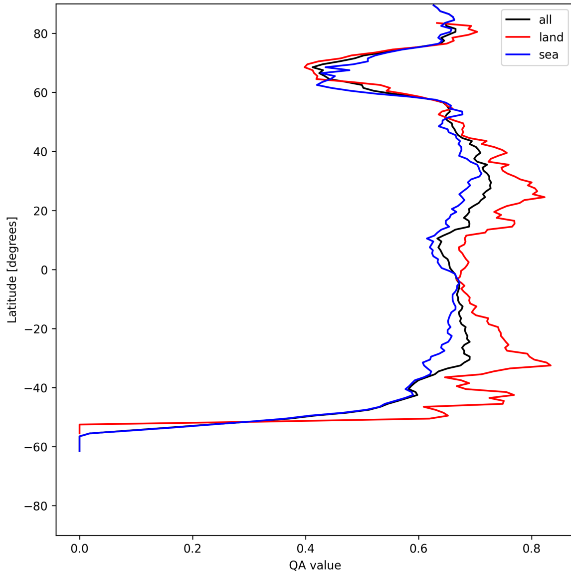
Figure 6: Zonal average of “QA value” for 2025-06-27 to 2025-06-28.
