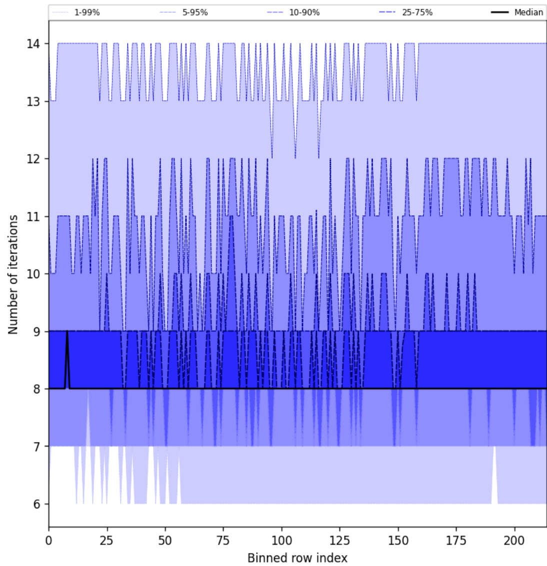
Figure 26: Along track statistics of “Number of iterations” for 2025-06-27 to 2025-06-28
