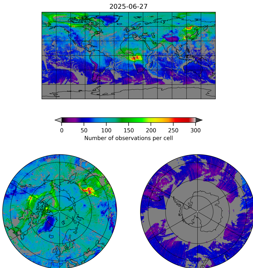
Figure 5: Map of the number of observations for 2025-06-27 to 2025-06-28
