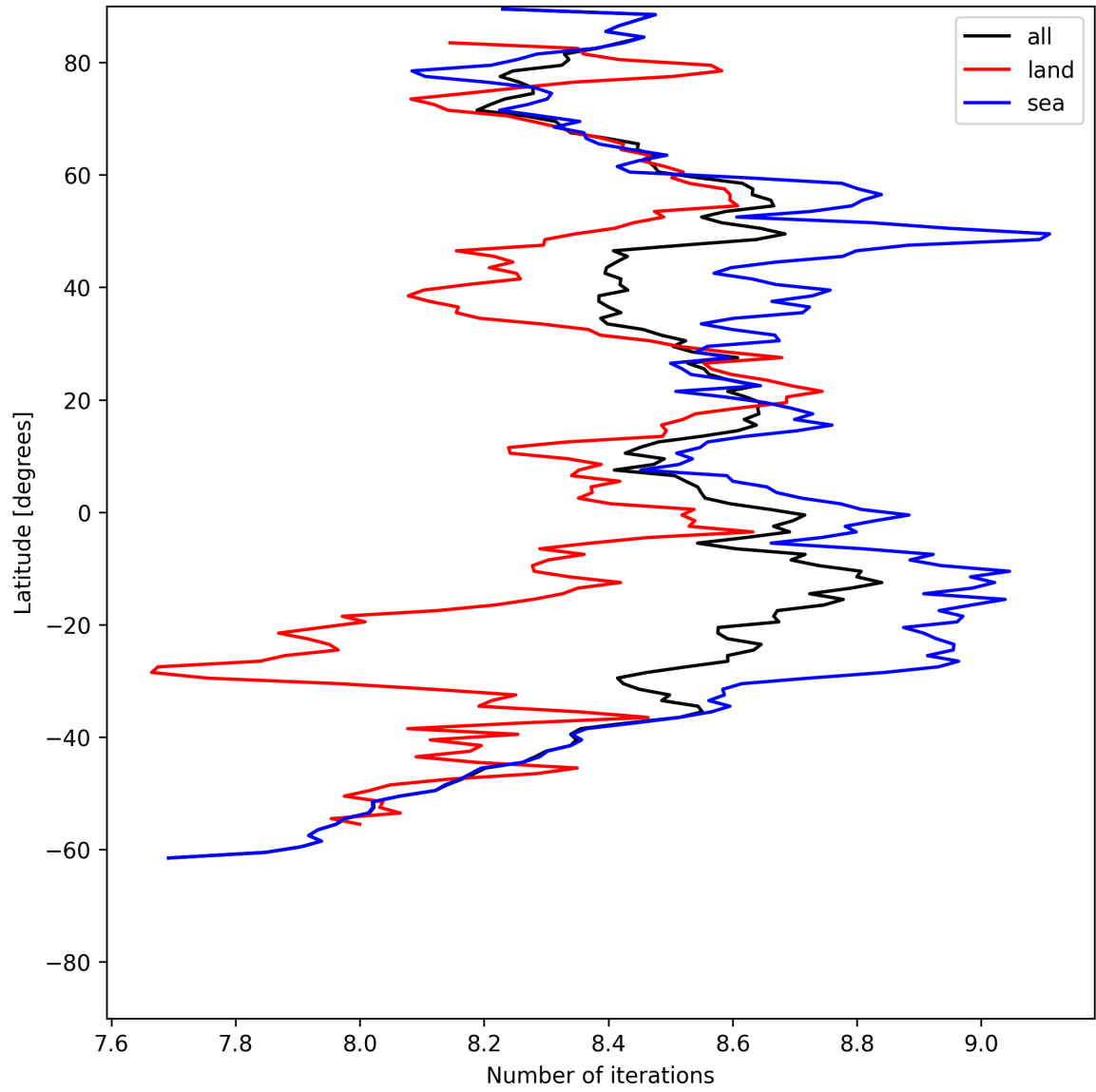
Figure 12: Zonal average of “Number of iterations” for 2025-06-27 to 2025-06-28.
