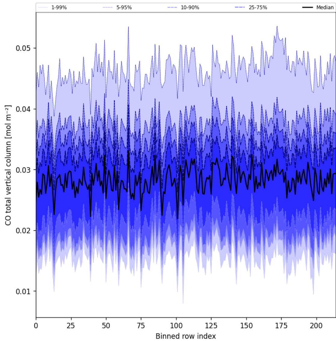
Figure 21: Along track statistics of “CO total vertical column” for 2025-06-27 to 2025-06-28
