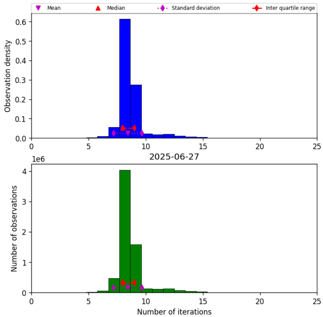
Figure 19: Histogram of “Number of iterations” for 2025-06-27 to 2025-06-28
