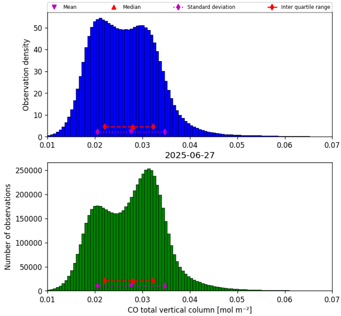
Figure 14: Histogram of “CO total vertical column” for 2025-06-27 to 2025-06-28
