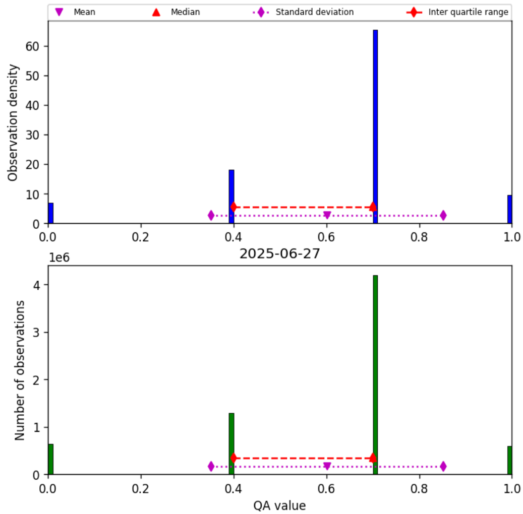
Figure 13: Histogram of “QA value” for 2025-06-27 to 2025-06-28
