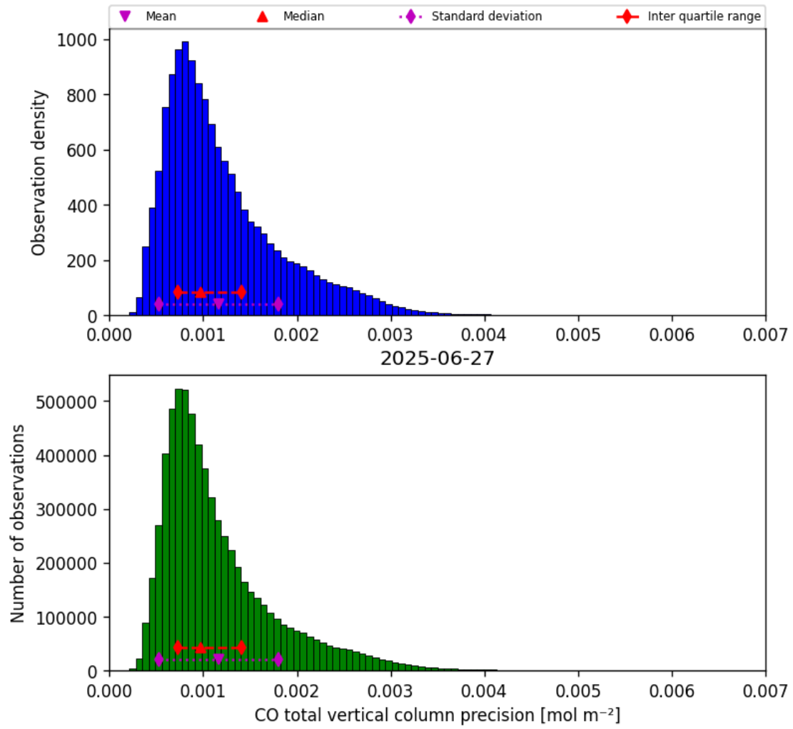
Figure 15: Histogram of “CO total vertical column precision” for 2025-06-27 to 2025-06-28
