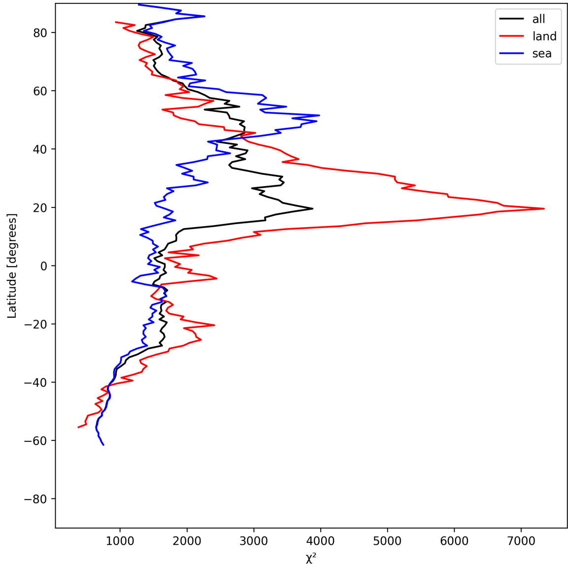
Figure 10: Zonal average of “ \chi^2 ” for 2025-06-27 to 2025-06-28.
