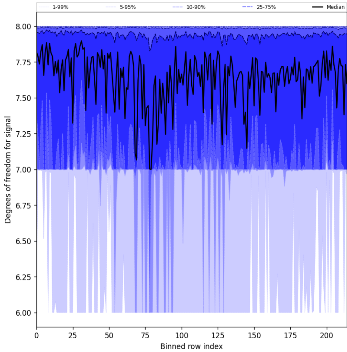
Figure 25: Along track statistics of “Degrees of freedom for signal” for 2025-06-27 to 2025-06-28
