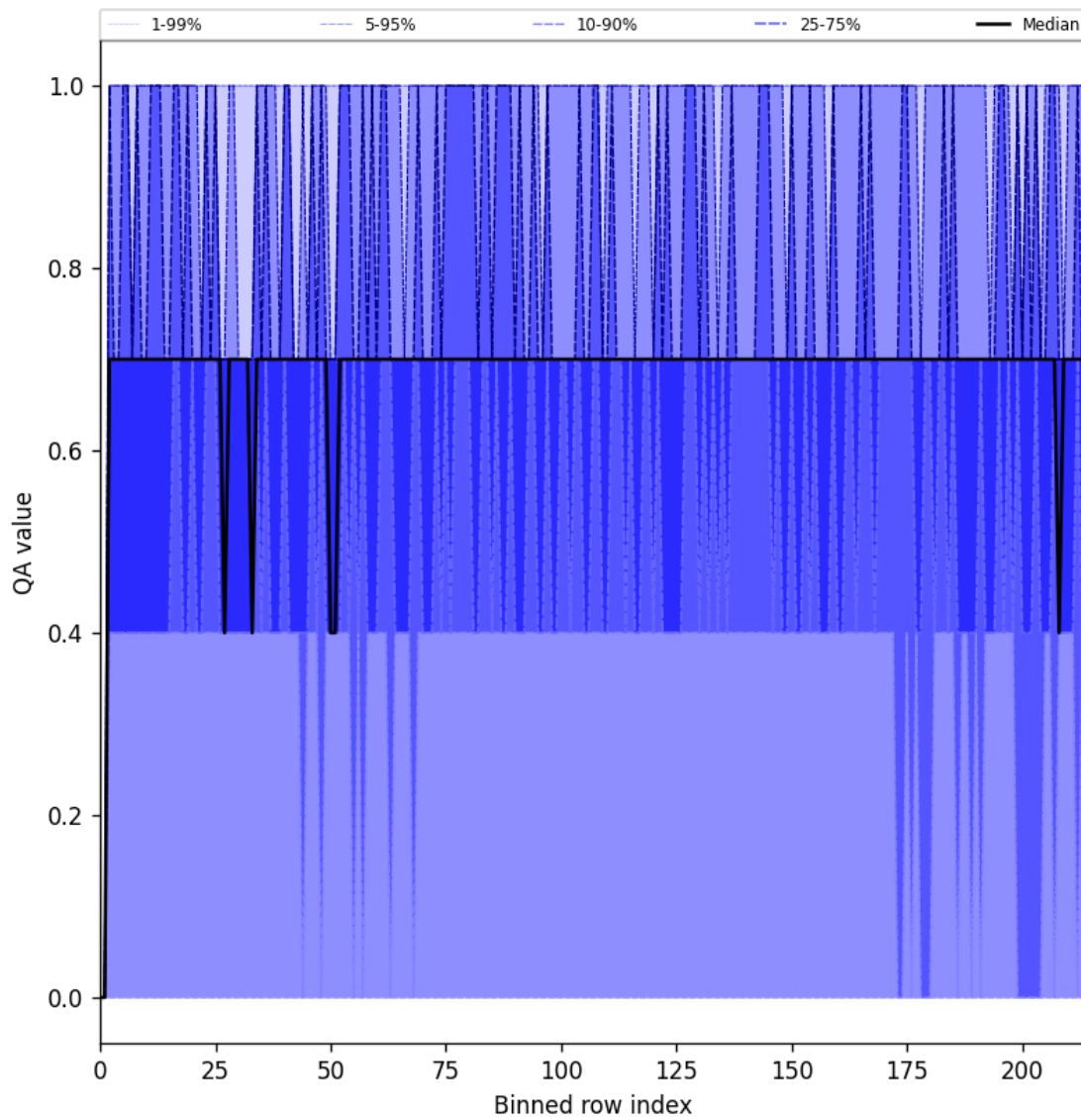
Figure 20: Along track statistics of “QA value” for 2025-06-27 to 2025-06-28
