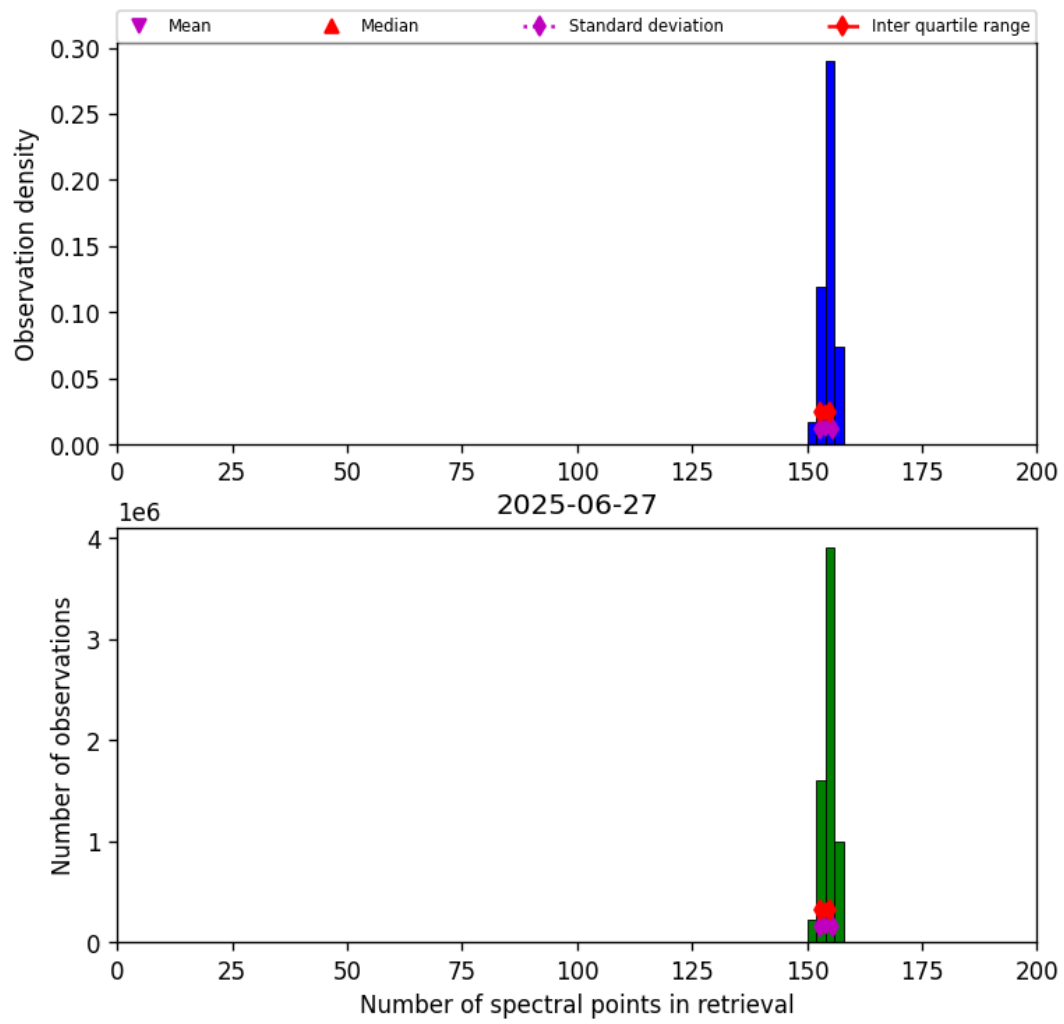
Figure 16: Histogram of “Number of spectral points in retrieval” for 2025-06-27 to 2025-06-28
