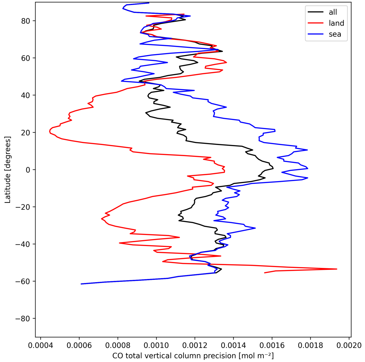
Figure 8: Zonal average of “CO total vertical column precision” for 2025-06-27 to 2025-06-28.
