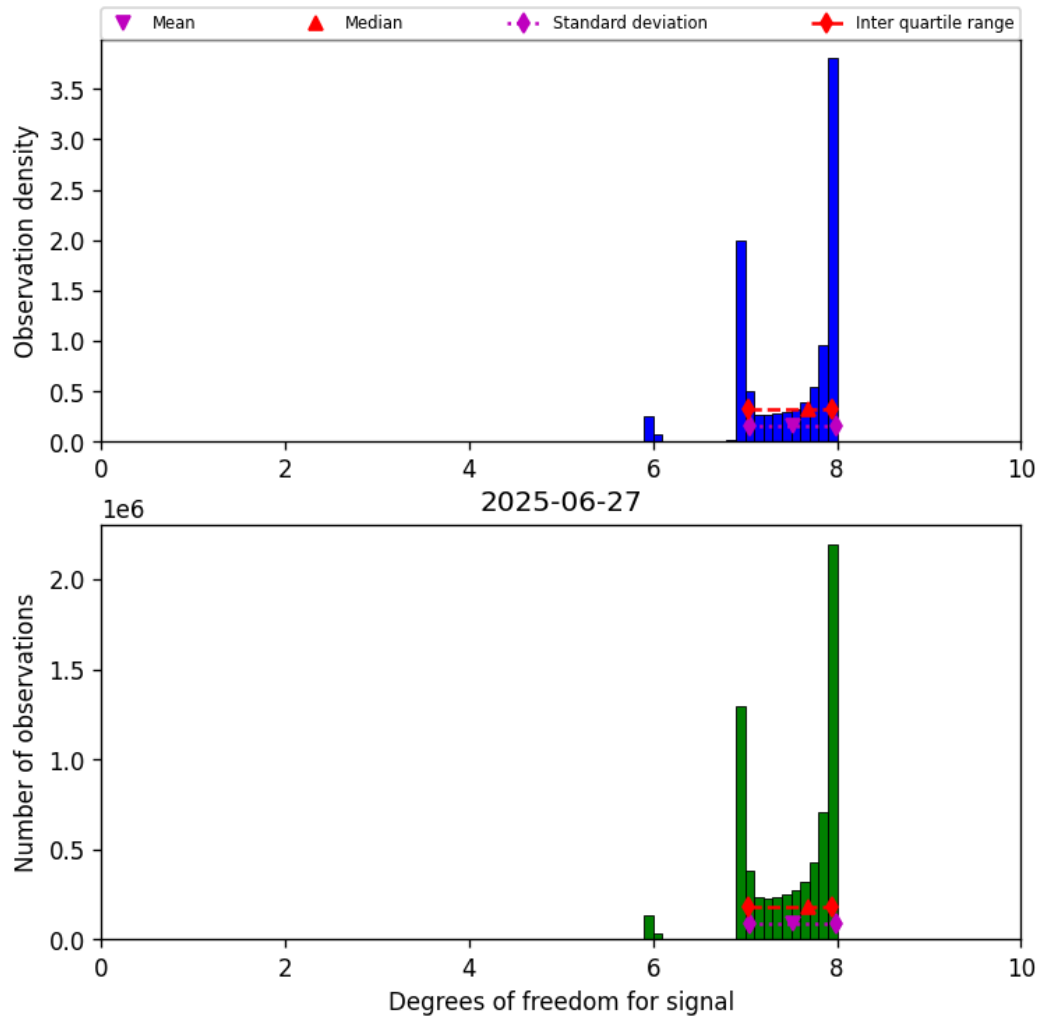
Figure 18: Histogram of “Degrees of freedom for signal” for 2025-06-27 to 2025-06-28
