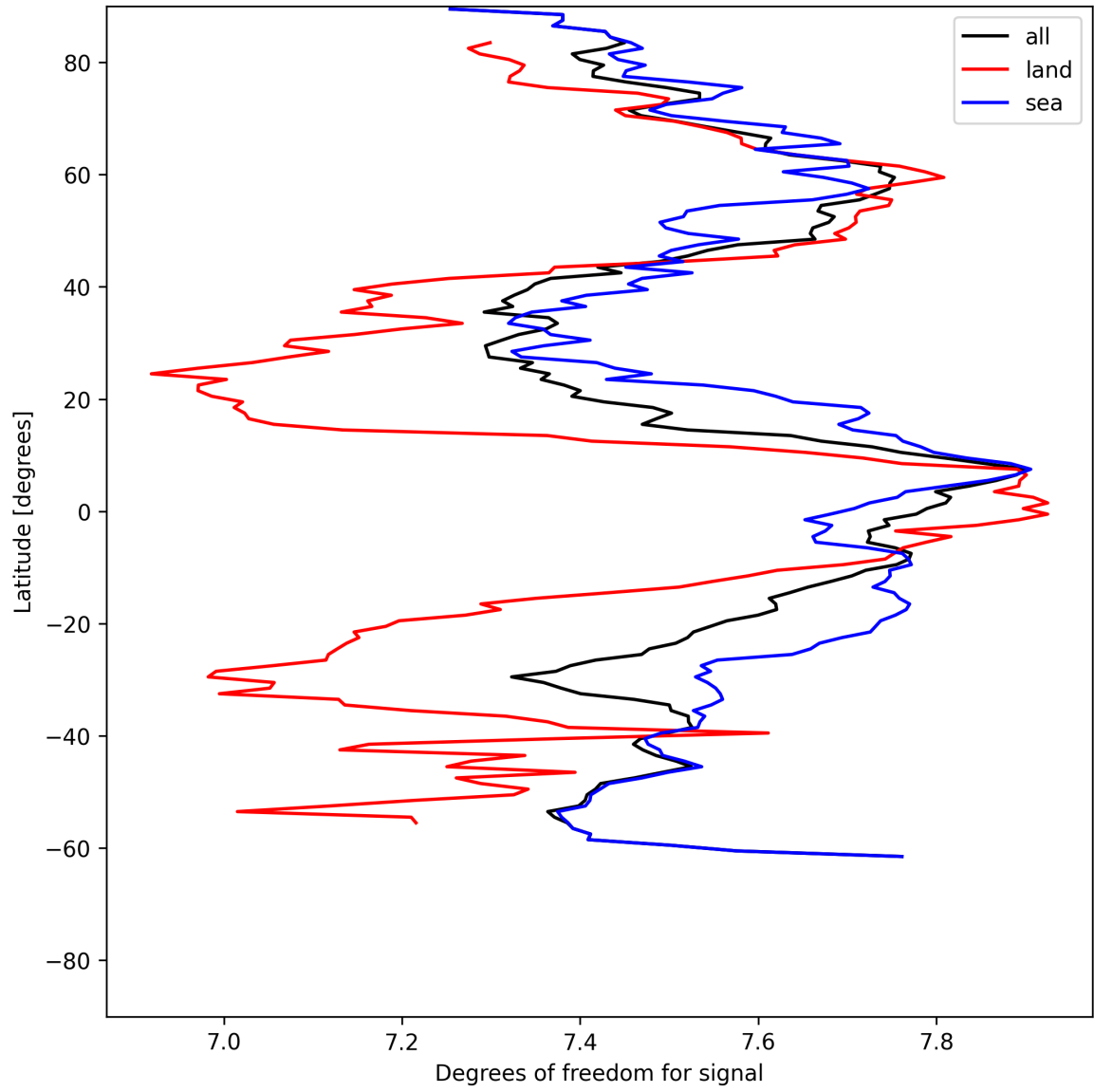
Figure 11: Zonal average of “Degrees of freedom for signal” for 2025-06-27 to 2025-06-28.
