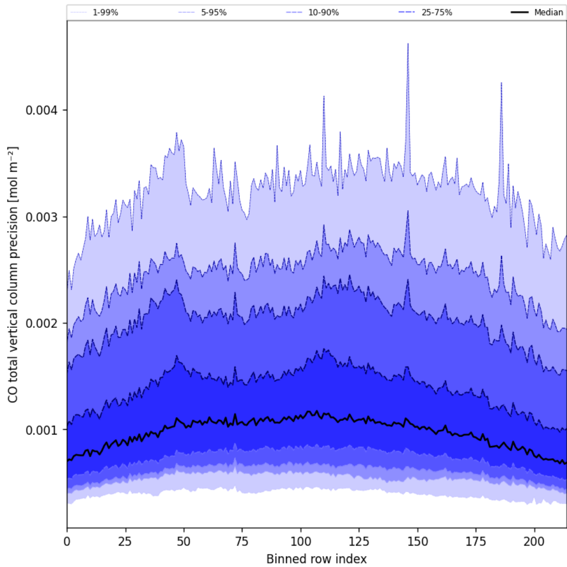
Figure 22: Along track statistics of “CO total vertical column precision” for 2025-06-28 to 2025-06-29
