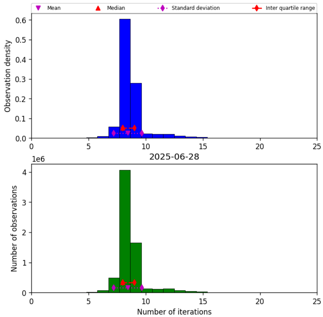
Figure 19: Histogram of “Number of iterations” for 2025-06-28 to 2025-06-29
