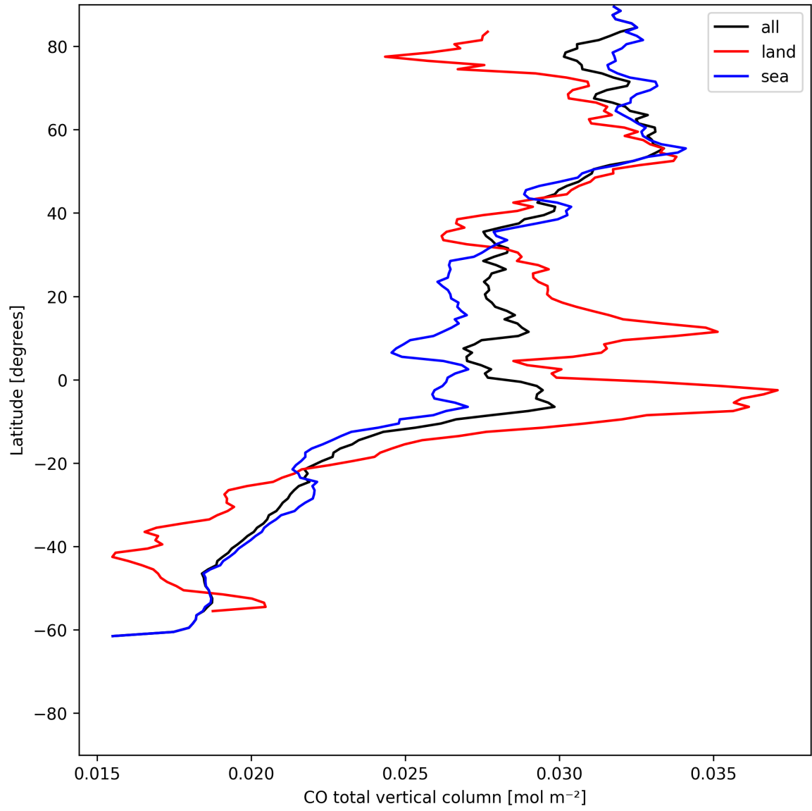
Figure 7: Zonal average of “CO total vertical column” for 2025-06-28 to 2025-06-29.
