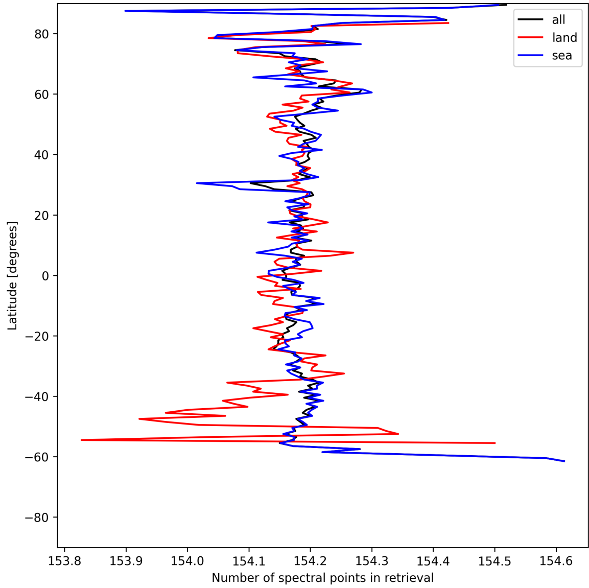
Figure 9: Zonal average of “Number of spectral points in retrieval” for 2025-06-28 to 2025-06-29.
