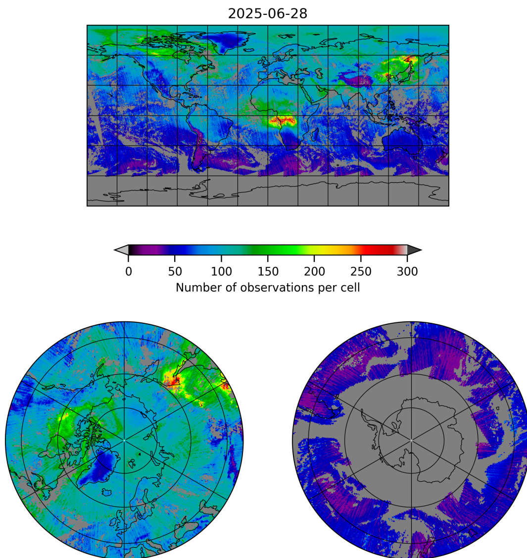
Figure 5: Map of the number of observations for 2025-06-28 to 2025-06-29
