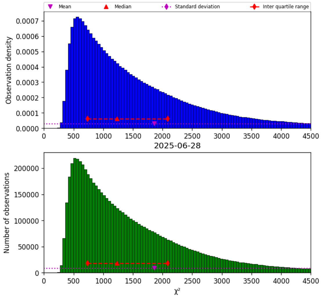
Figure 17: Histogram of “ \chi^2 ” for 2025-06-28 to 2025-06-29
