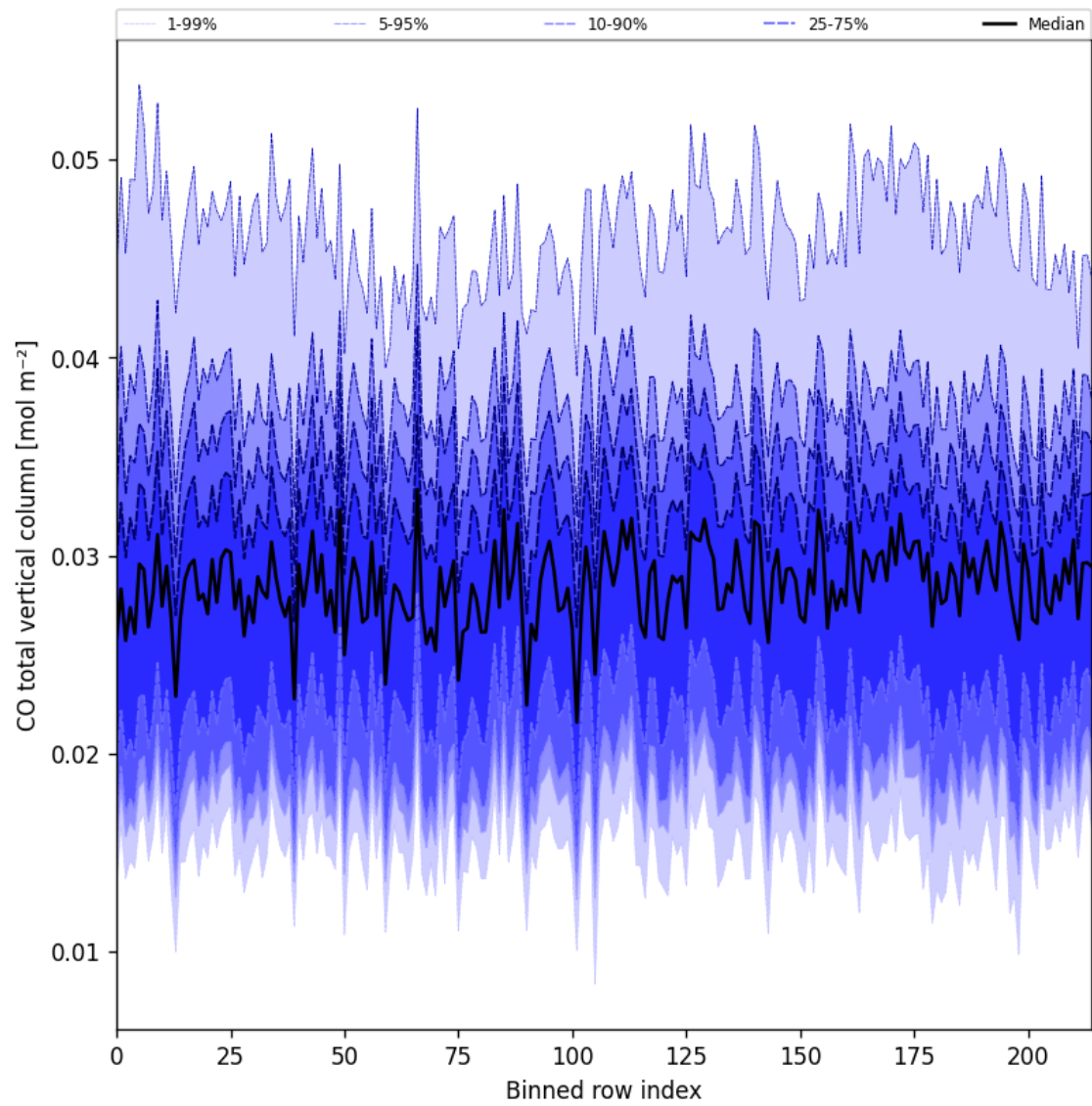
Figure 21: Along track statistics of “CO total vertical column” for 2025-06-28 to 2025-06-29
