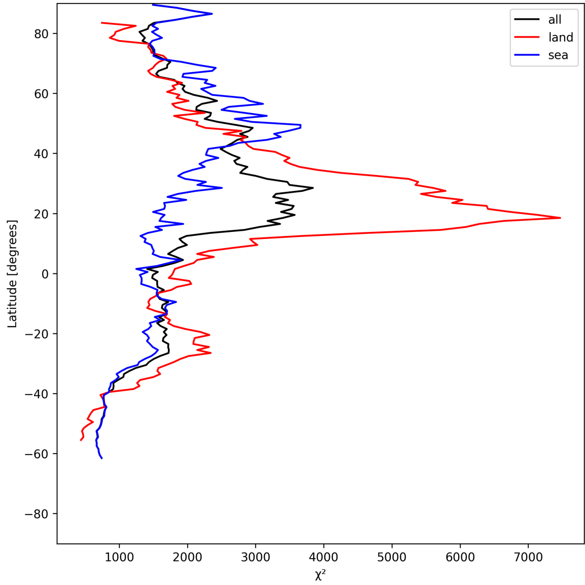
Figure 10: Zonal average of “ \chi^2 ” for 2025-06-28 to 2025-06-29.
