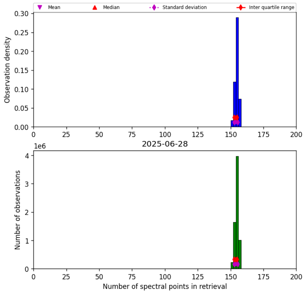
Figure 16: Histogram of “Number of spectral points in retrieval” for 2025-06-28 to 2025-06-29
