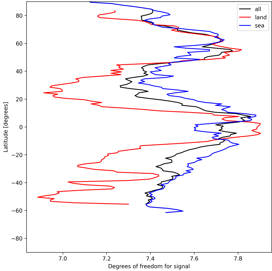
Figure 11: Zonal average of “Degrees of freedom for signal” for 2025-06-28 to 2025-06-29.
