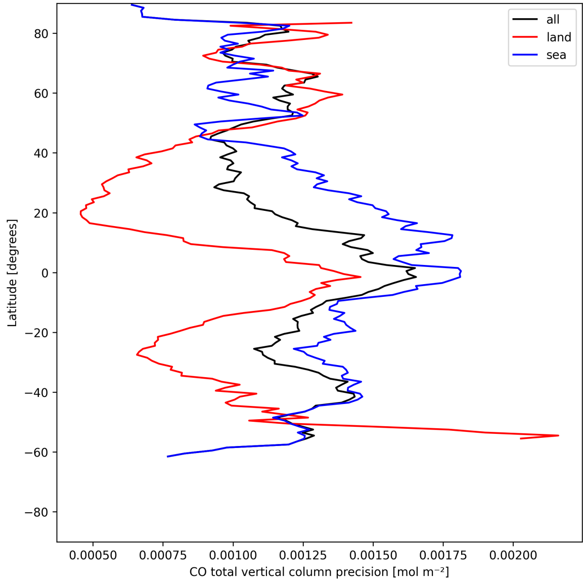
Figure 8: Zonal average of “CO total vertical column precision” for 2025-06-28 to 2025-06-29.
