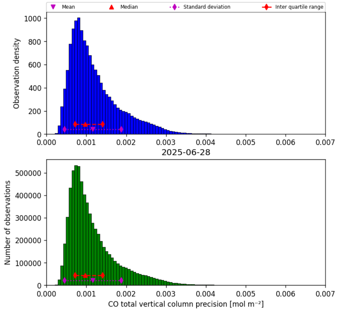
Figure 15: Histogram of “CO total vertical column precision” for 2025-06-28 to 2025-06-29
