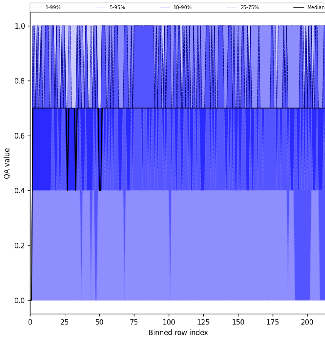
Figure 20: Along track statistics of “QA value” for 2025-06-28 to 2025-06-29
