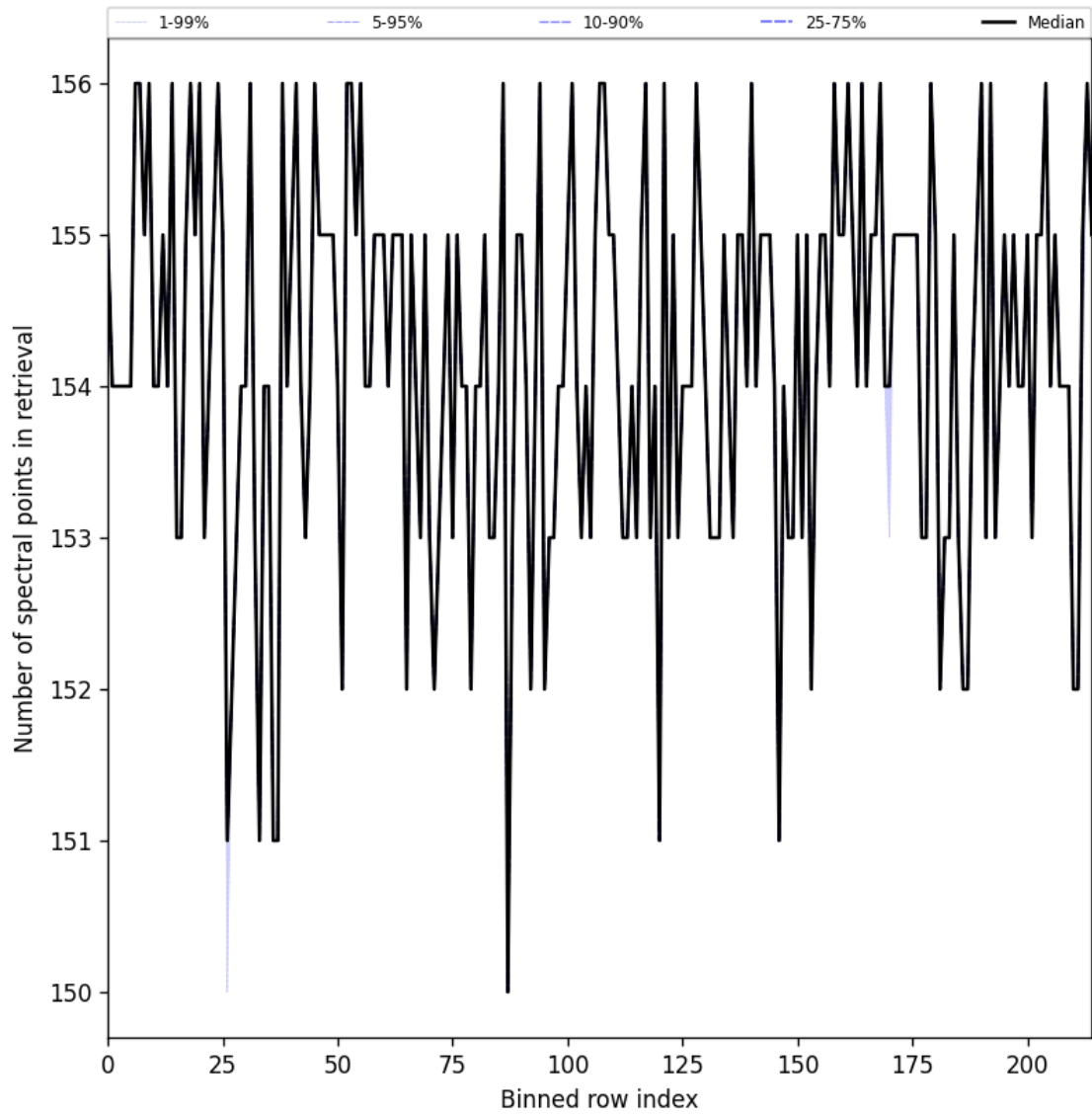
Figure 23: Along track statistics of “Number of spectral points in retrieval” for 2025-06-28 to 2025-06-29
