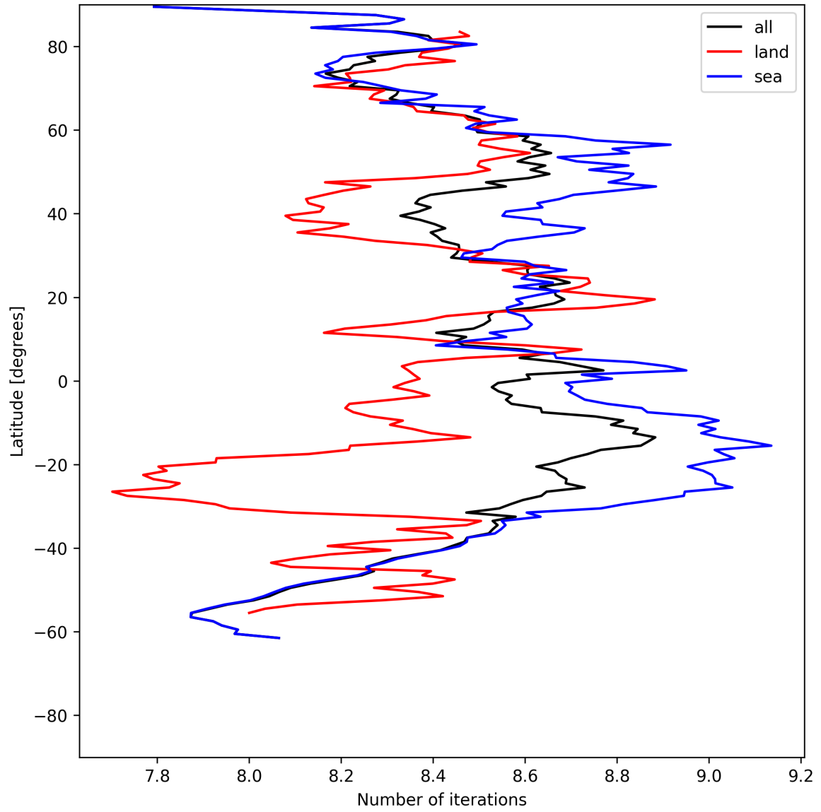
Figure 12: Zonal average of “Number of iterations” for 2025-06-28 to 2025-06-29.
