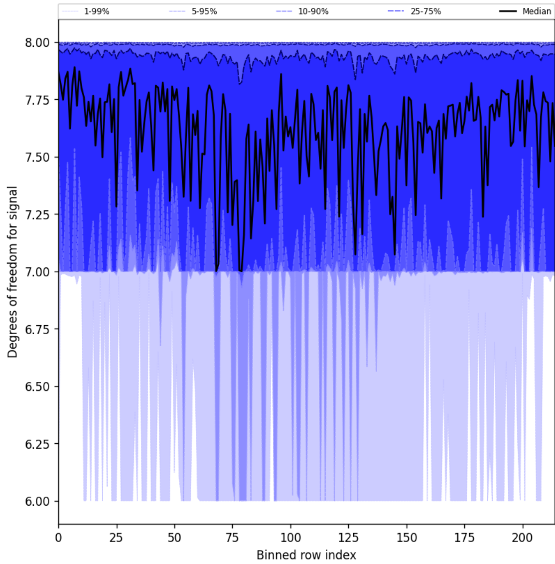
Figure 25: Along track statistics of “Degrees of freedom for signal” for 2025-06-28 to 2025-06-29
