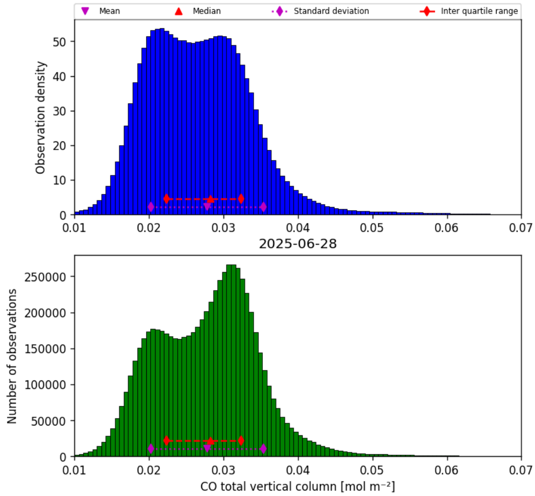
Figure 14: Histogram of “CO total vertical column” for 2025-06-28 to 2025-06-29
