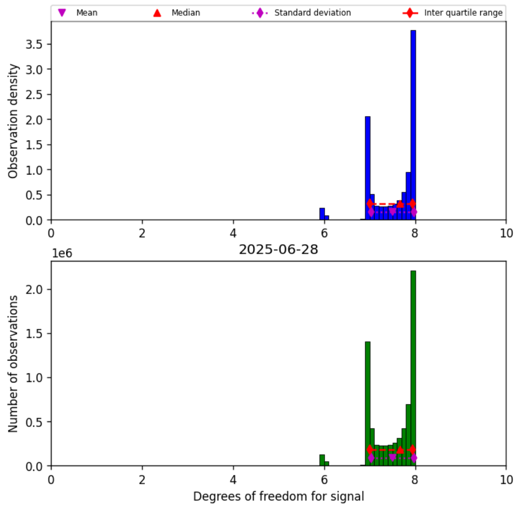
Figure 18: Histogram of “Degrees of freedom for signal” for 2025-06-28 to 2025-06-29
