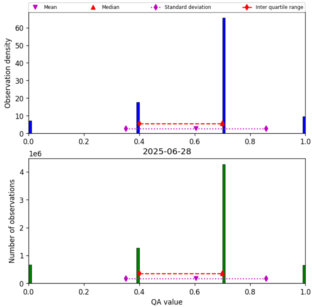
Figure 13: Histogram of “QA value” for 2025-06-28 to 2025-06-29
