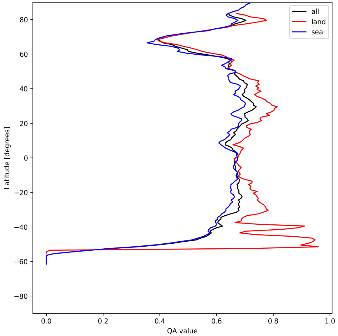
Figure 6: Zonal average of “QA value” for 2025-06-28 to 2025-06-29.
