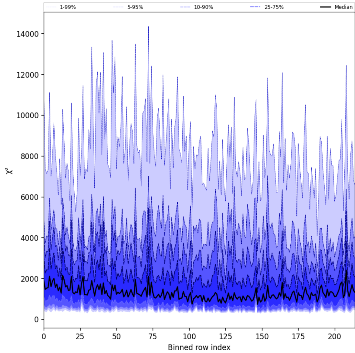
Figure 24: Along track statistics of “ \chi^2 ” for 2025-06-28 to 2025-06-29
