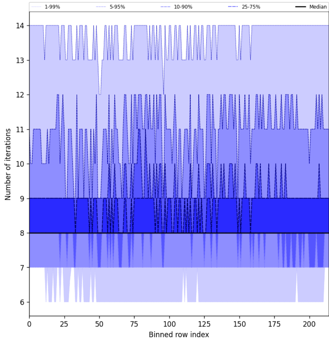
Figure 26: Along track statistics of “Number of iterations” for 2025-06-28 to 2025-06-29
