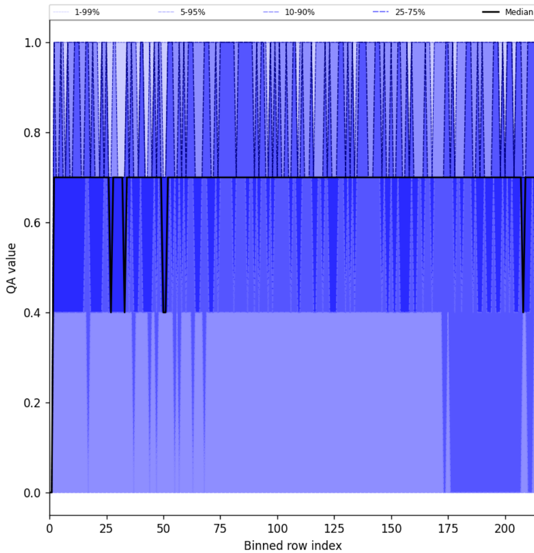
Figure 20: Along track statistics of “QA value” for 2025-06-29 to 2025-06-30
