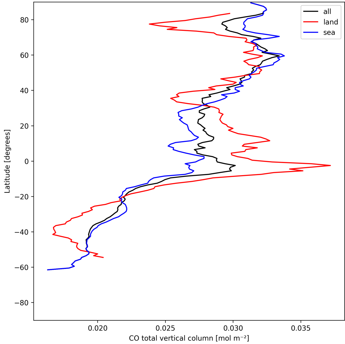
Figure 7: Zonal average of “CO total vertical column” for 2025-06-29 to 2025-06-30.
