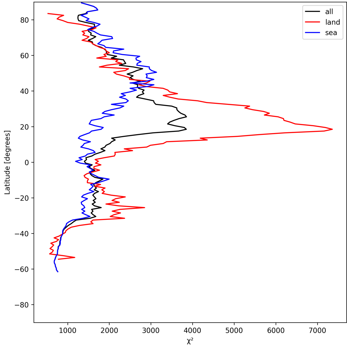
Figure 10: Zonal average of “ \chi^2 ” for 2025-06-29 to 2025-06-30.
