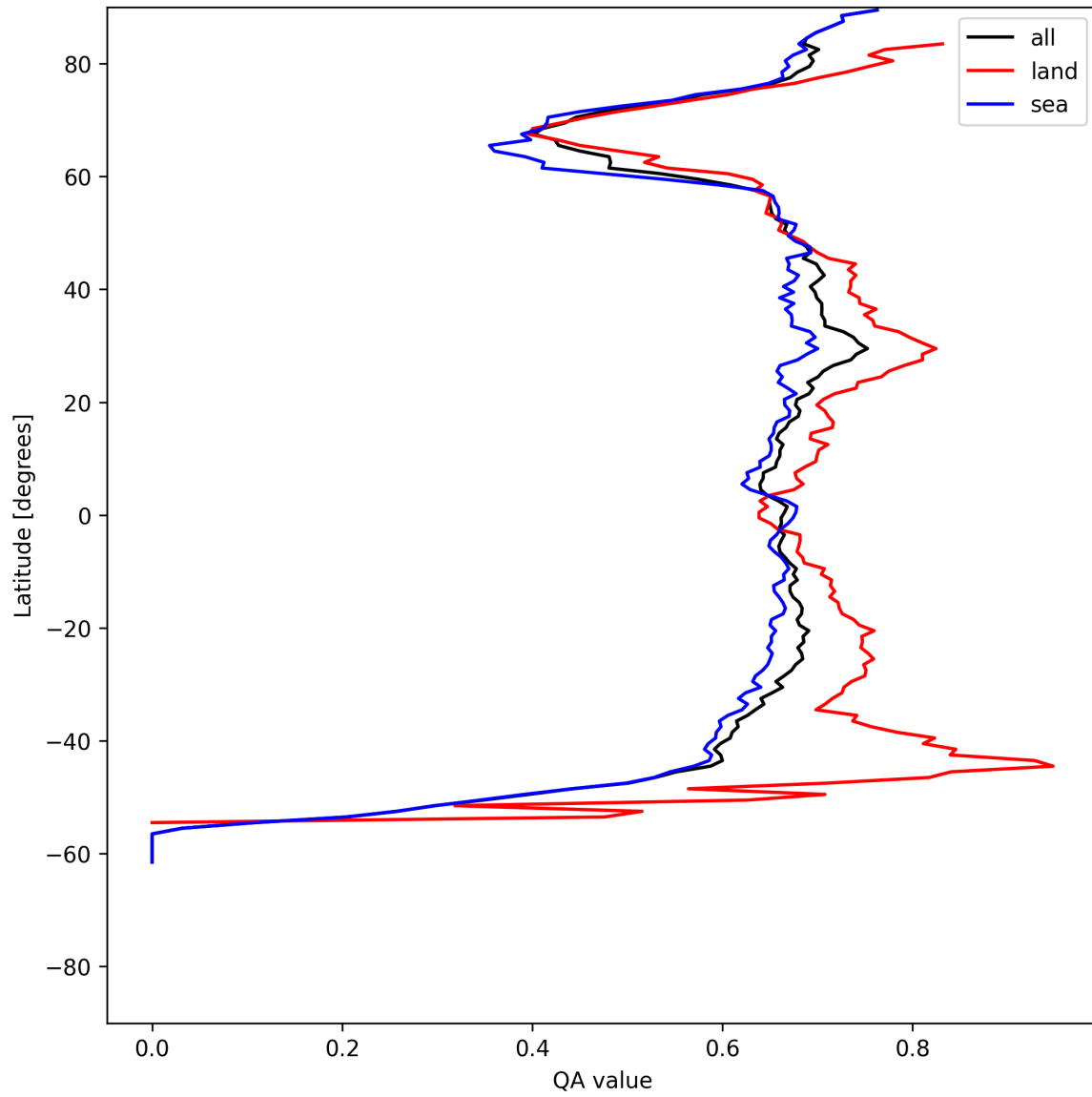
Figure 6: Zonal average of “QA value” for 2025-06-29 to 2025-06-30.
