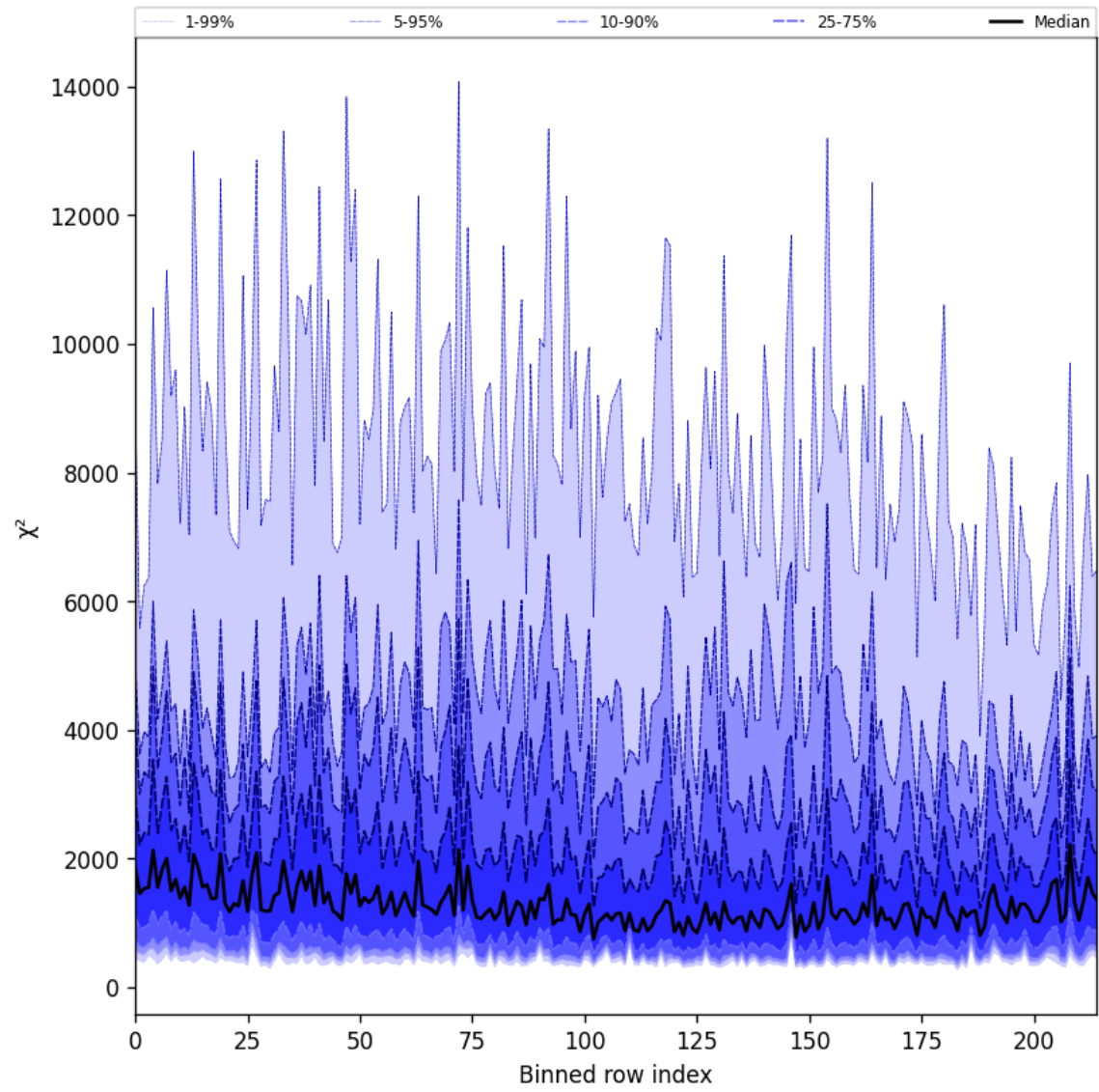
Figure 24: Along track statistics of “ \chi^2 ” for 2025-06-29 to 2025-06-30
