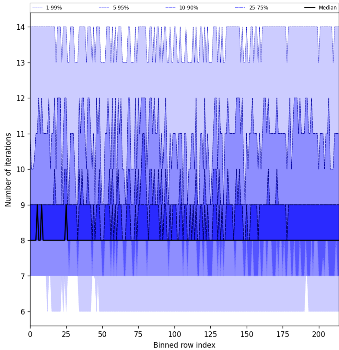
Figure 26: Along track statistics of “Number of iterations” for 2025-06-29 to 2025-06-30
