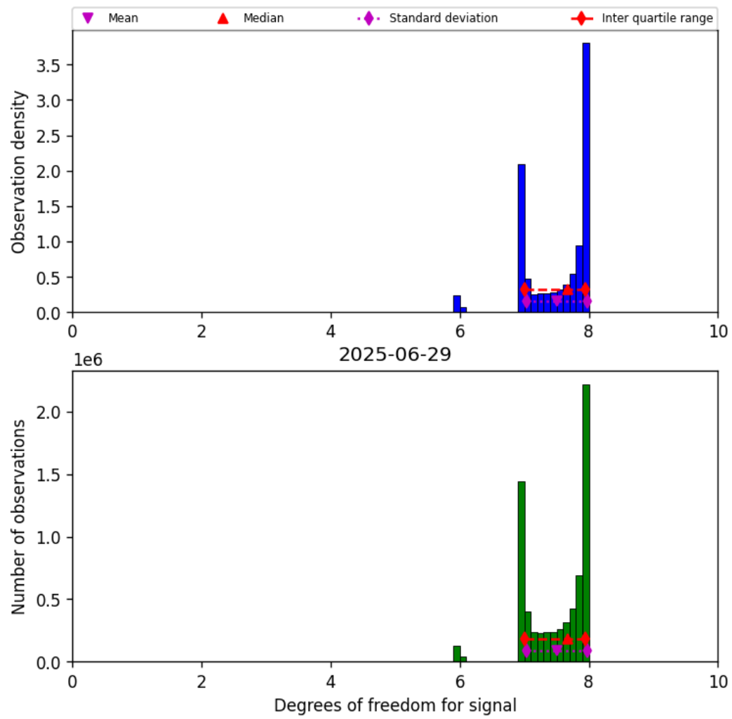
Figure 18: Histogram of “Degrees of freedom for signal” for 2025-06-29 to 2025-06-30
