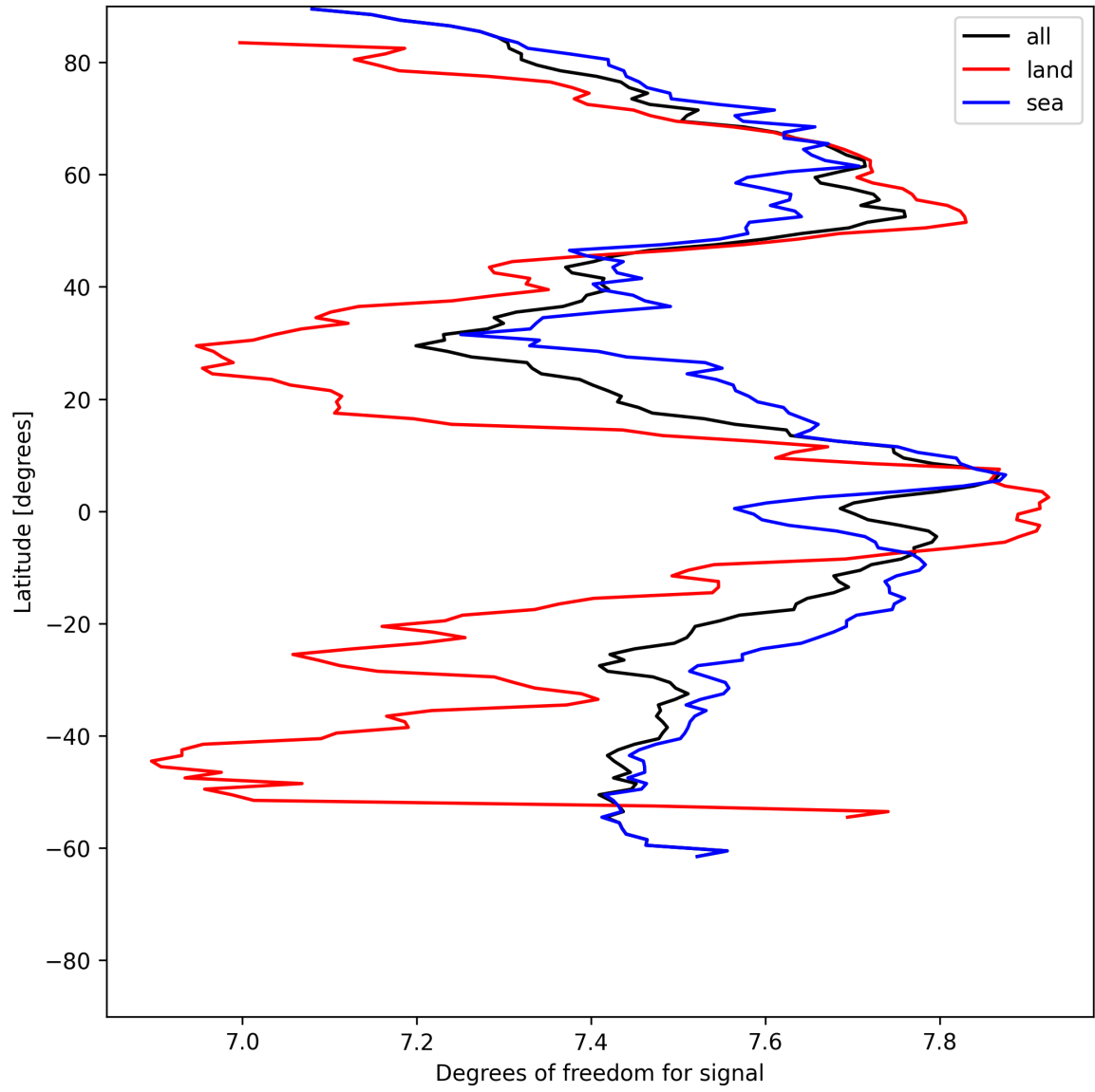
Figure 11: Zonal average of “Degrees of freedom for signal” for 2025-06-29 to 2025-06-30.
