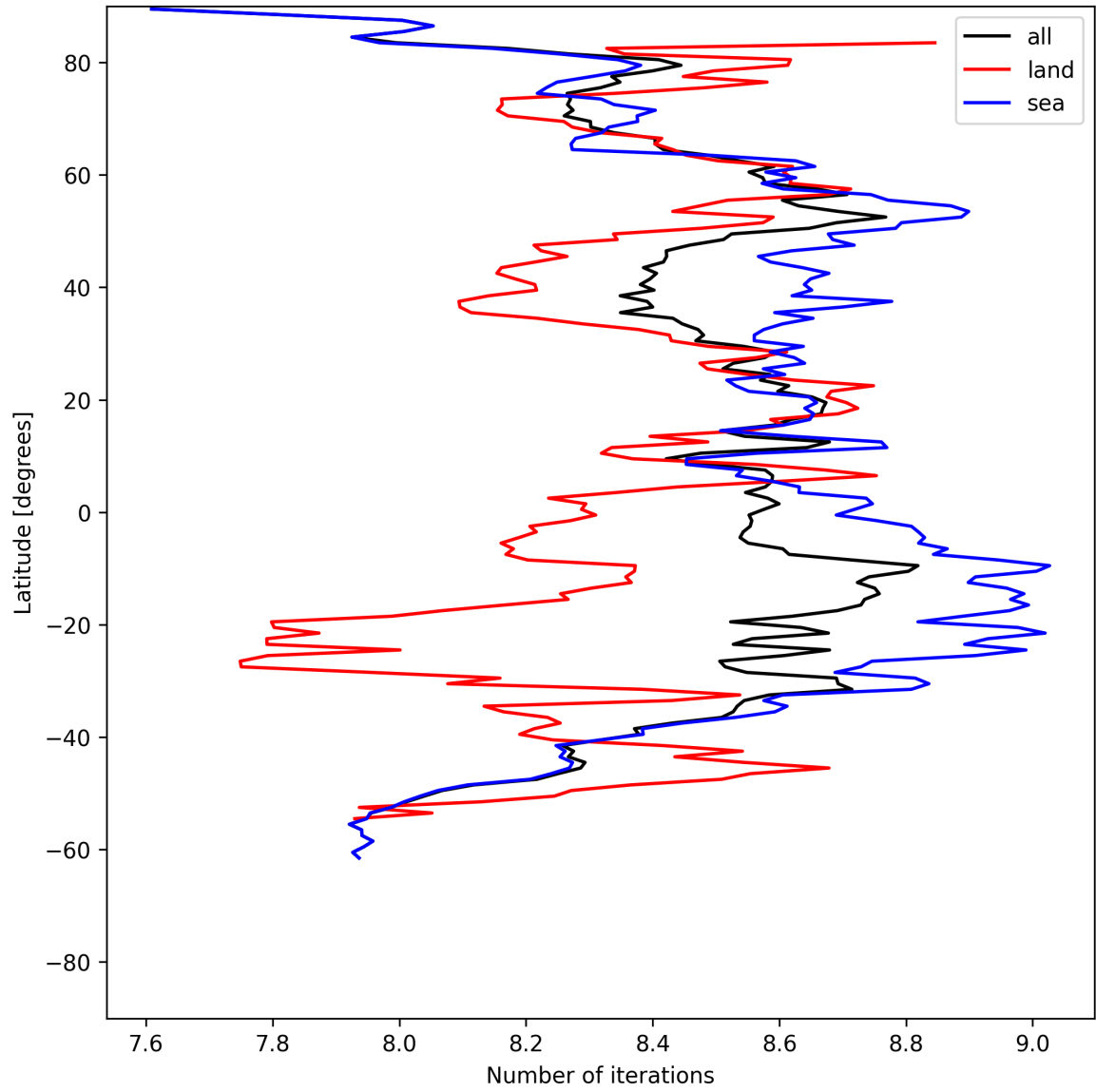
Figure 12: Zonal average of “Number of iterations” for 2025-06-29 to 2025-06-30.
