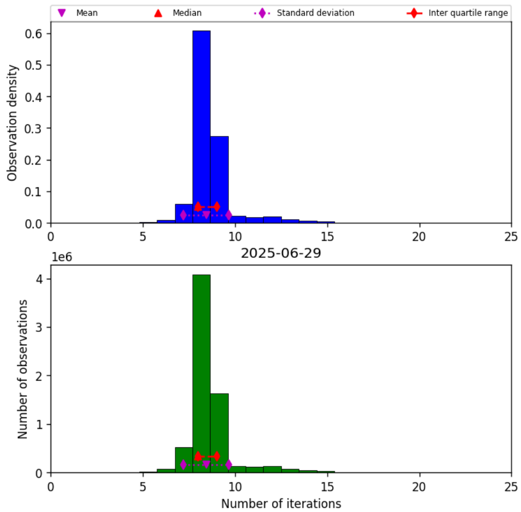
Figure 19: Histogram of “Number of iterations” for 2025-06-29 to 2025-06-30
