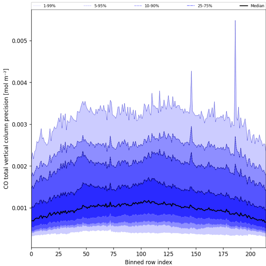
Figure 22: Along track statistics of “CO total vertical column precision” for 2025-06-29 to 2025-06-30
