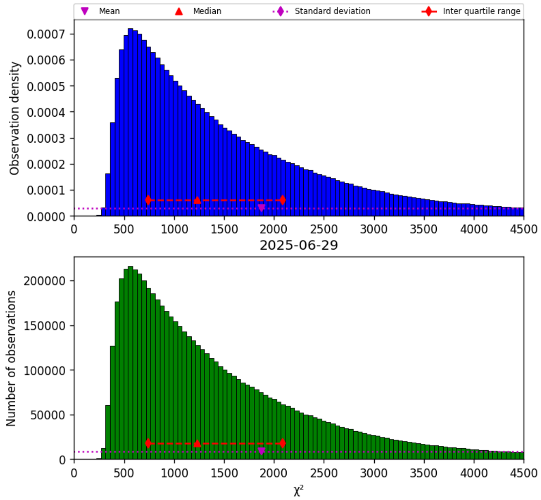
Figure 17: Histogram of “ \chi^2 ” for 2025-06-29 to 2025-06-30
