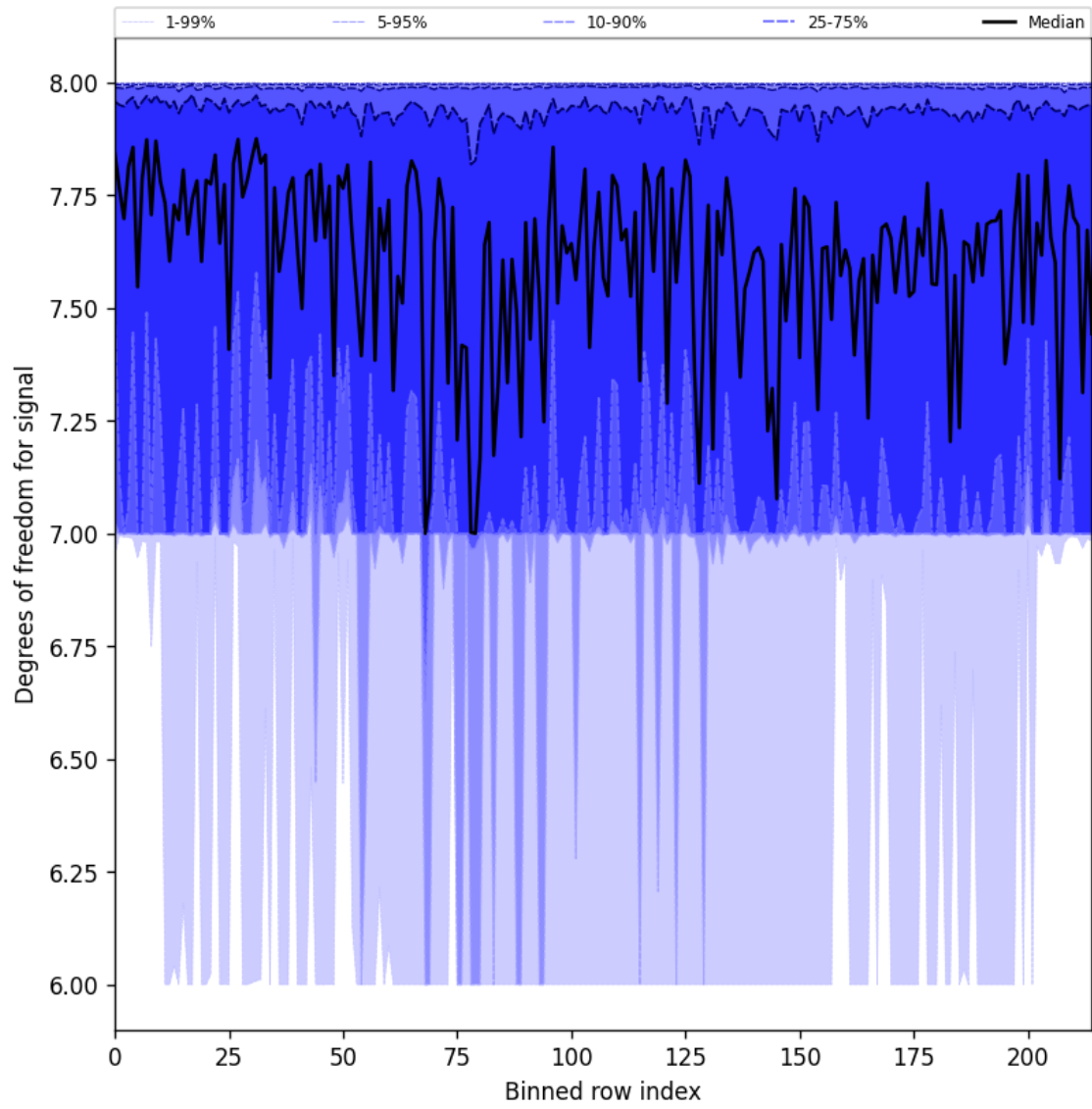
Figure 25: Along track statistics of “Degrees of freedom for signal” for 2025-06-29 to 2025-06-30
