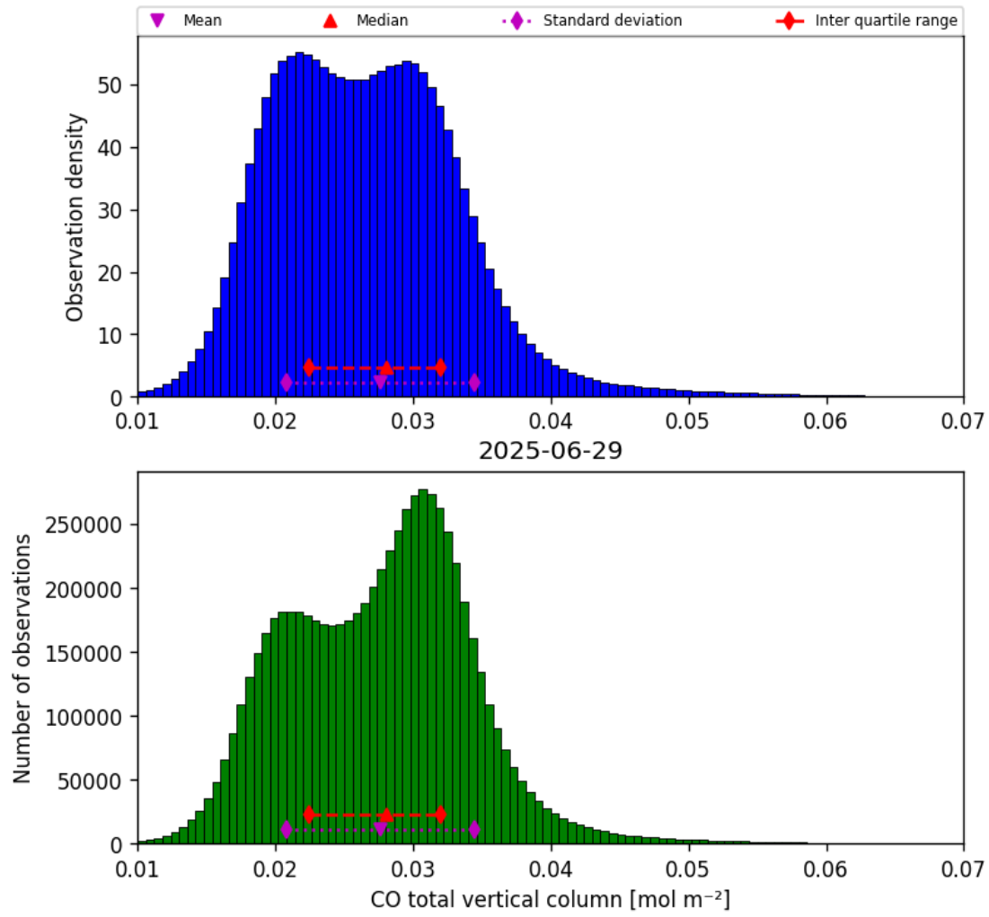
Figure 14: Histogram of “CO total vertical column” for 2025-06-29 to 2025-06-30
