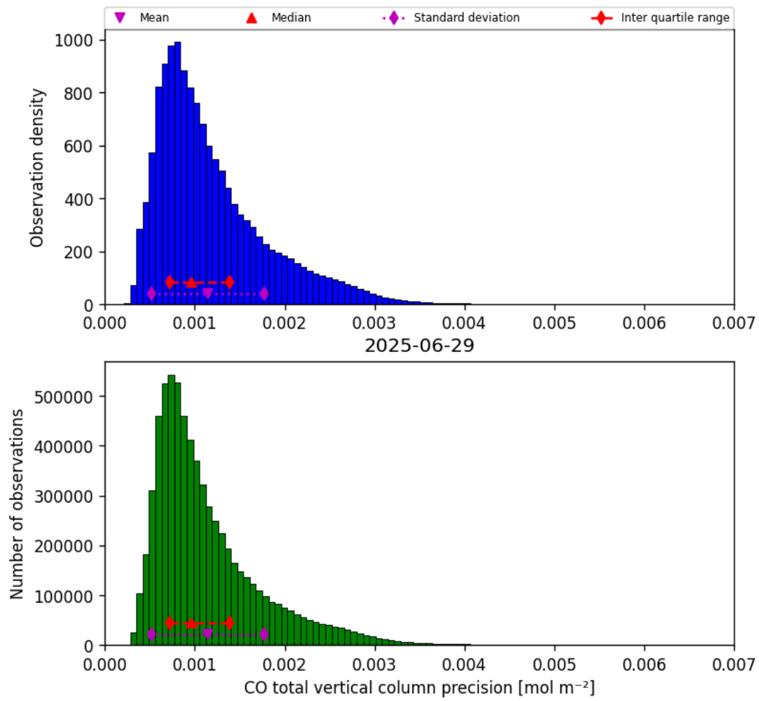
Figure 15: Histogram of “CO total vertical column precision” for 2025-06-29 to 2025-06-30
