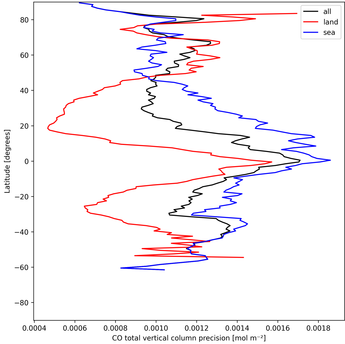
Figure 8: Zonal average of "CO total vertical column precision" for 2025-06-29 to 2025-06-30.
