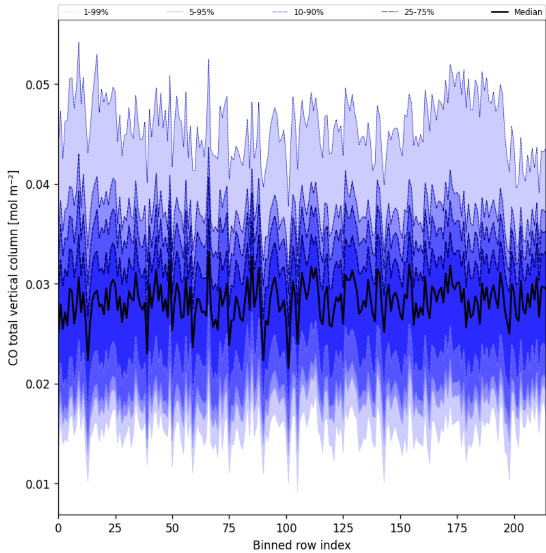
Figure 21: Along track statistics of “CO total vertical column” for 2025-06-29 to 2025-06-30
