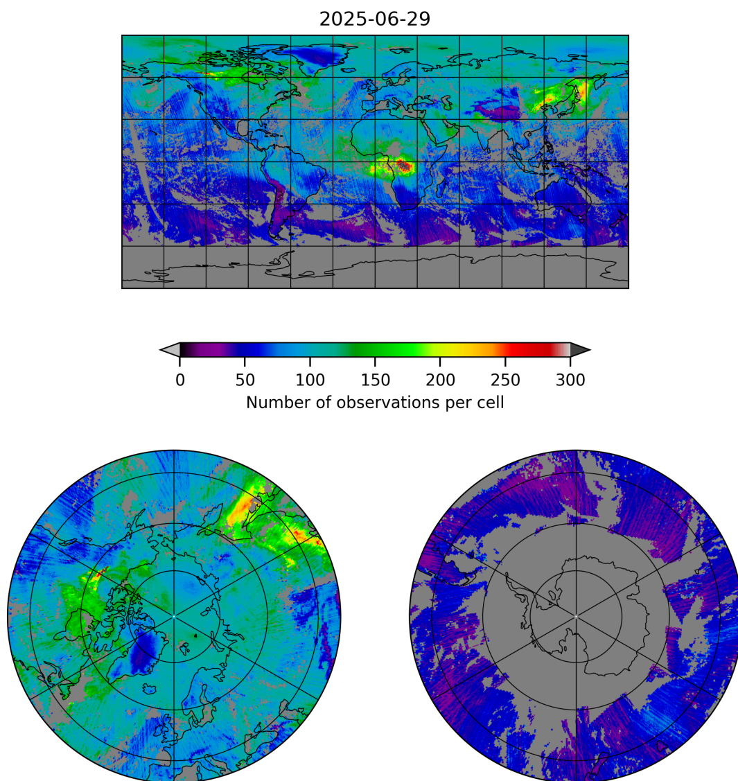
Figure 5: Map of the number of observations for 2025-06-29 to 2025-06-30
