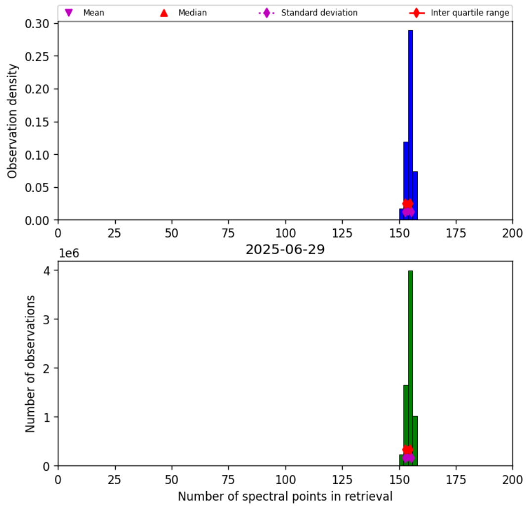
Figure 16: Histogram of “Number of spectral points in retrieval” for 2025-06-29 to 2025-06-30
