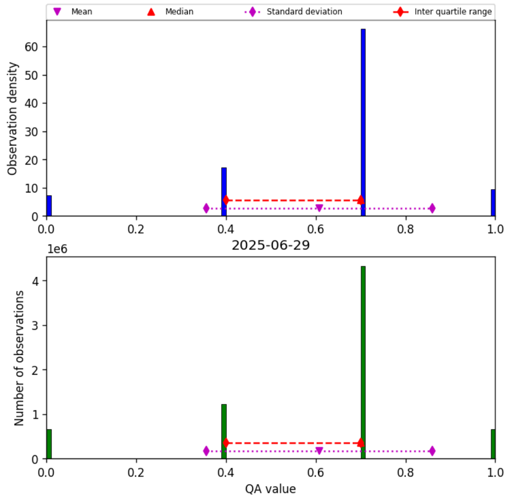
Figure 13: Histogram of “QA value” for 2025-06-29 to 2025-06-30
