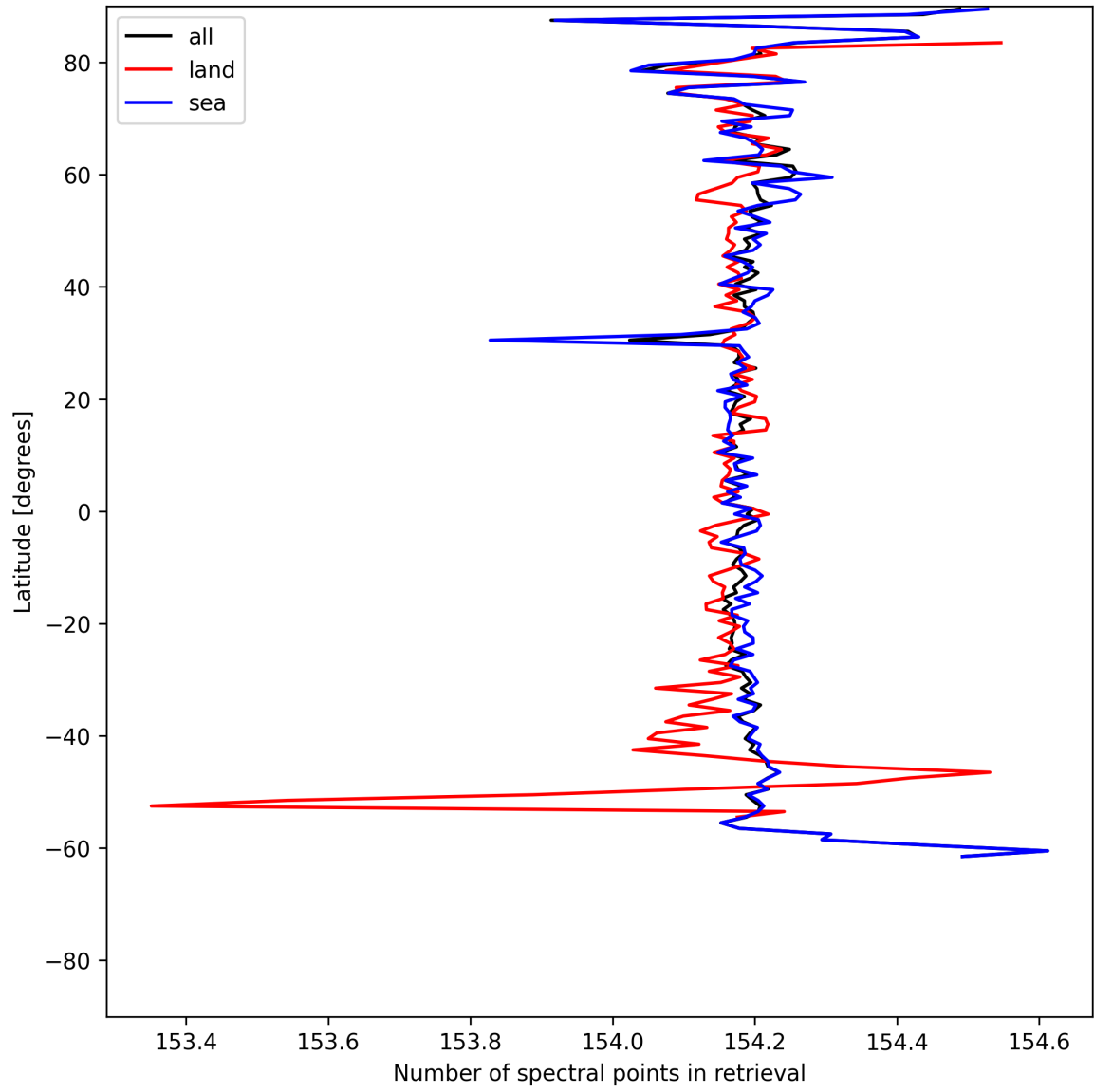
Figure 9: Zonal average of “Number of spectral points in retrieval” for 2025-06-29 to 2025-06-30.
