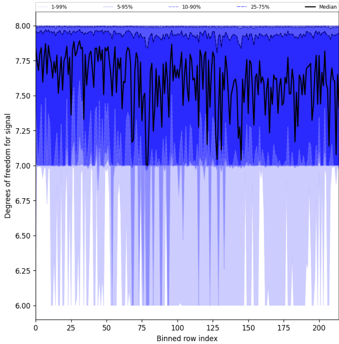
Figure 25: Along track statistics of “Degrees of freedom for signal” for 2025-06-30 to 2025-06-30
