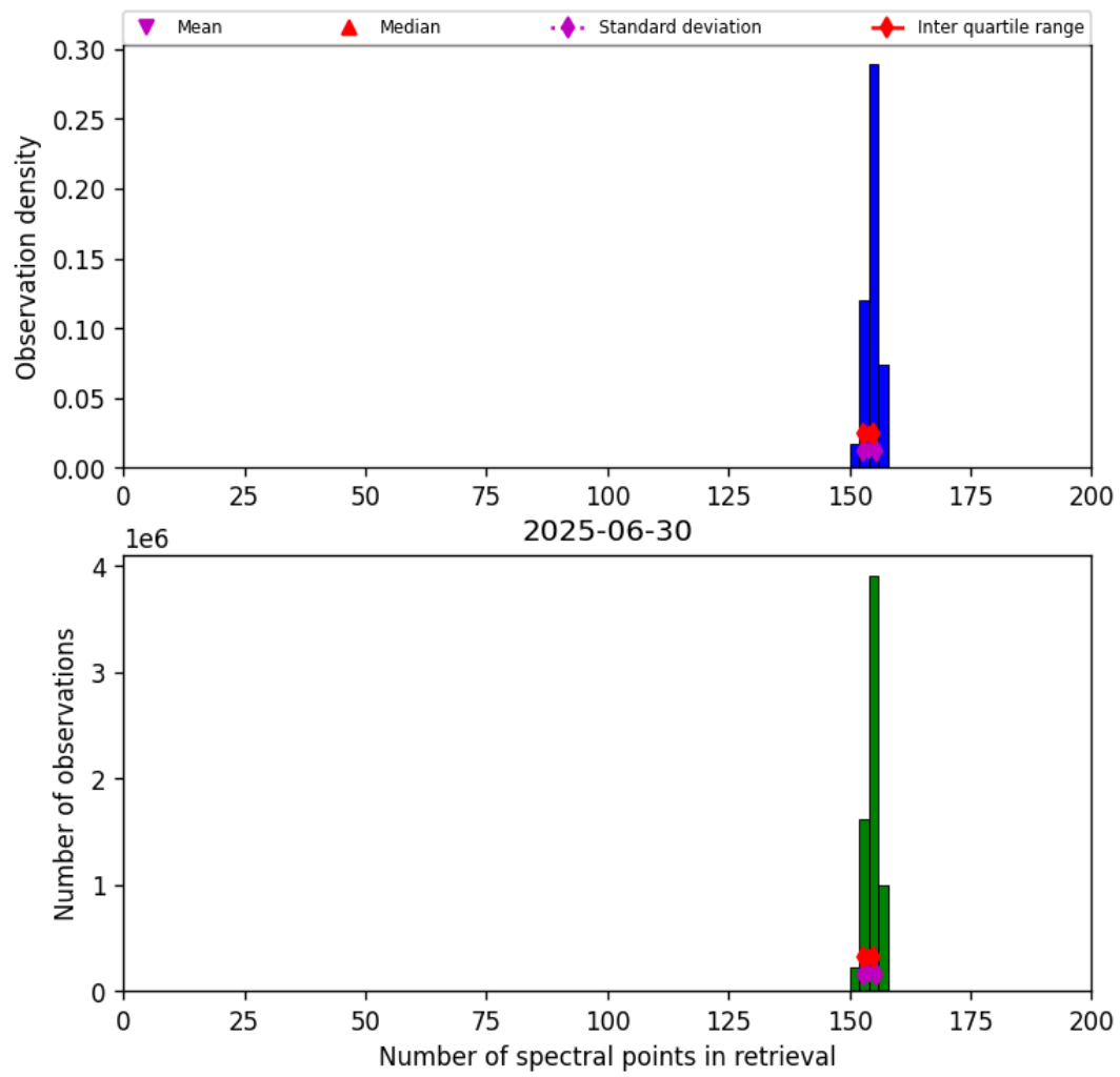
Figure 16: Histogram of “Number of spectral points in retrieval” for 2025-06-30 to 2025-06-30
