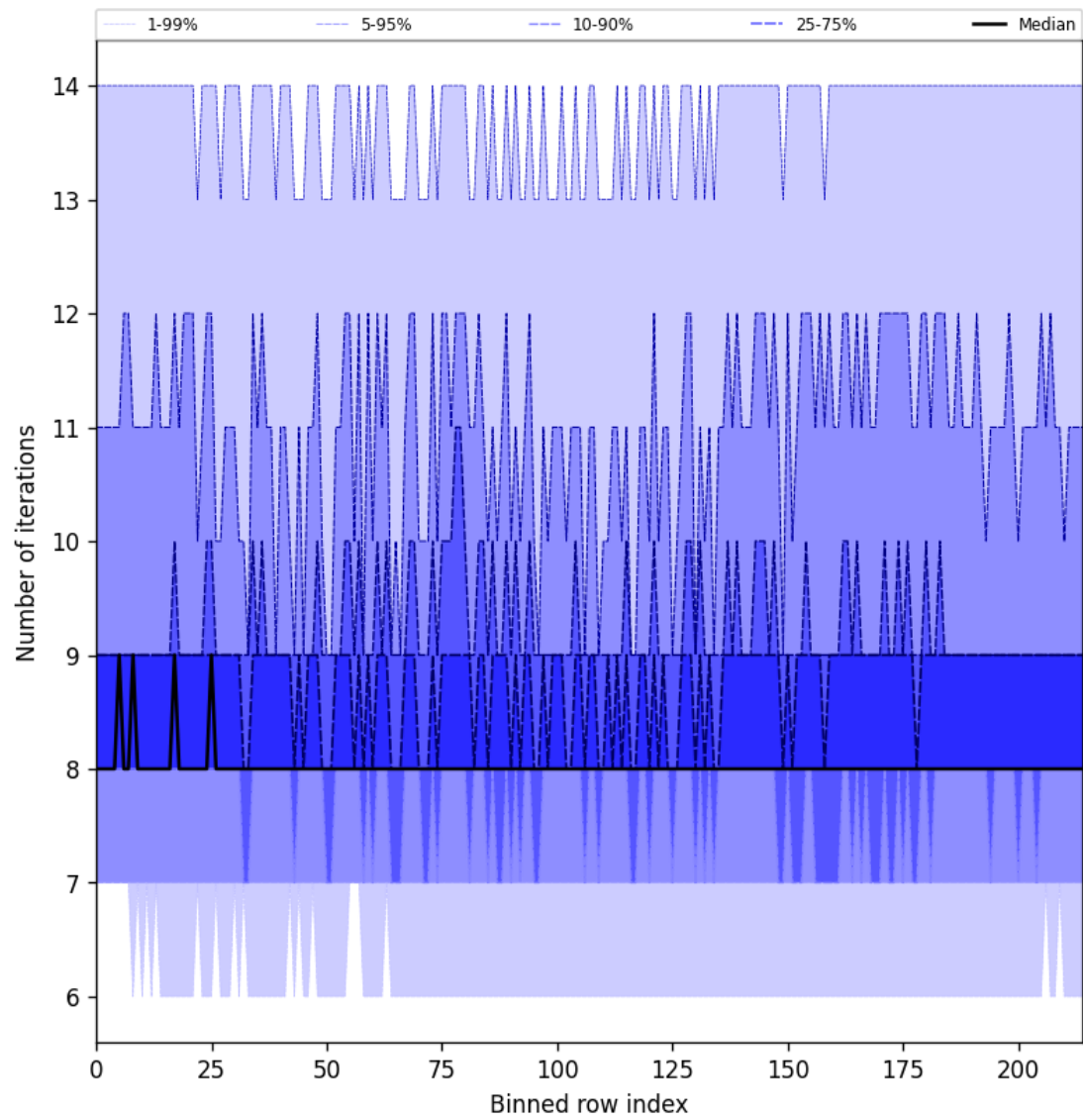
Figure 26: Along track statistics of “Number of iterations” for 2025-06-30 to 2025-06-30
