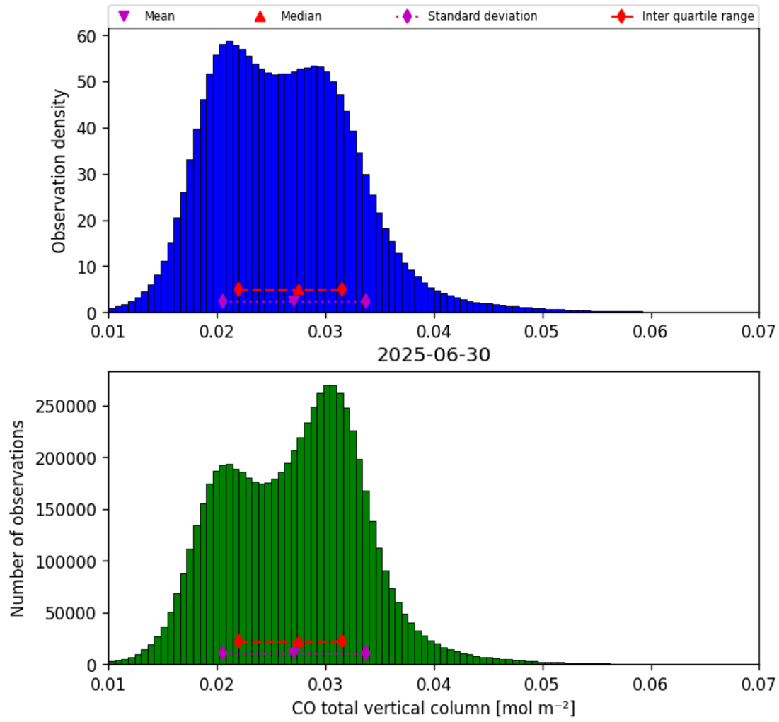
Figure 14: Histogram of “CO total vertical column” for 2025-06-30 to 2025-06-30
