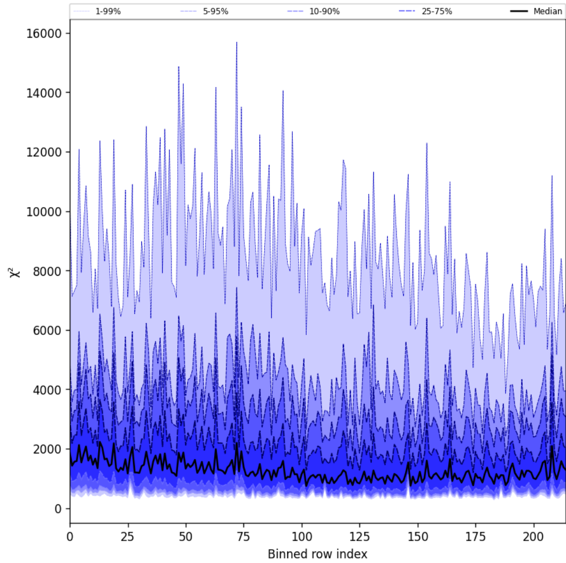
Figure 24: Along track statistics of “ \chi^2 ” for 2025-06-30 to 2025-06-30
