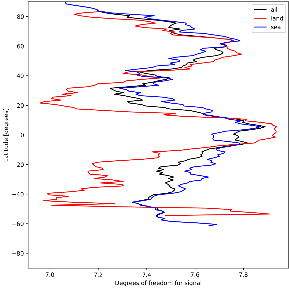
Figure 11: Zonal average of “Degrees of freedom for signal” for 2025-06-30 to 2025-06-30.
