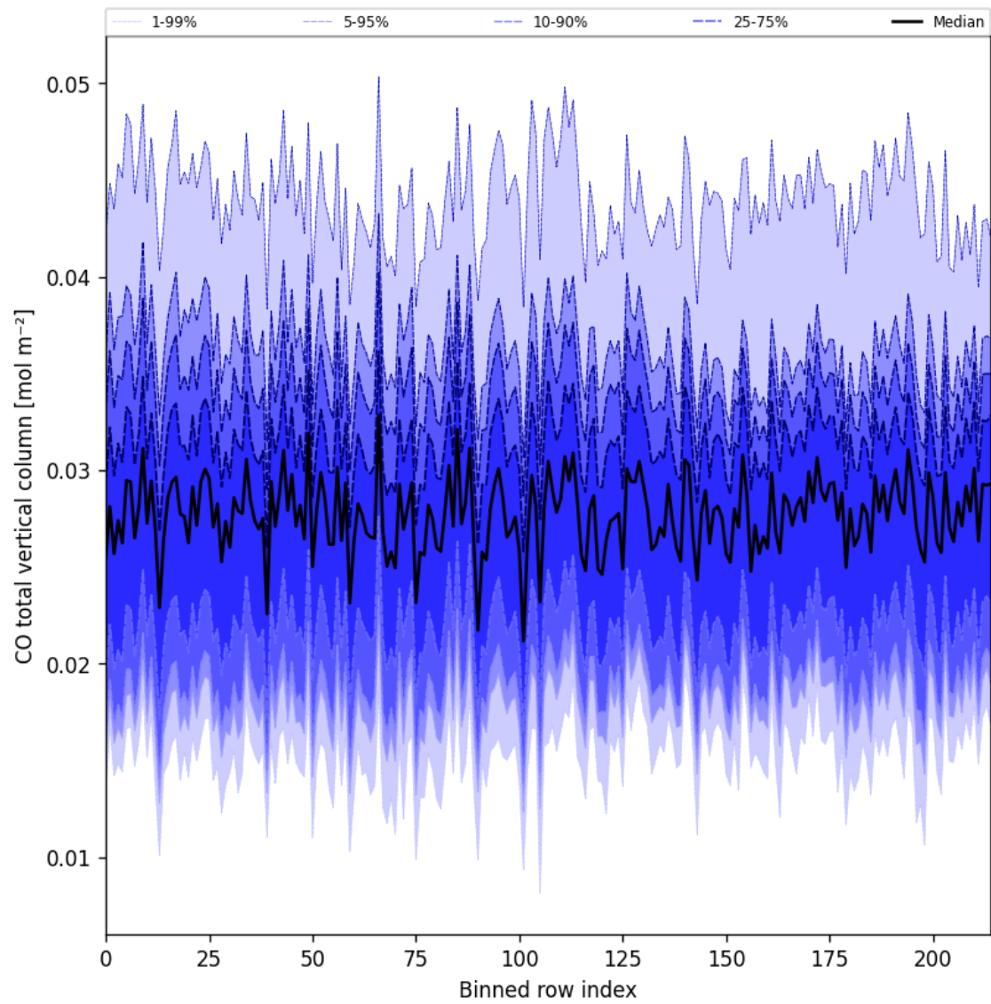
Figure 21: Along track statistics of “CO total vertical column” for 2025-06-30 to 2025-06-30
