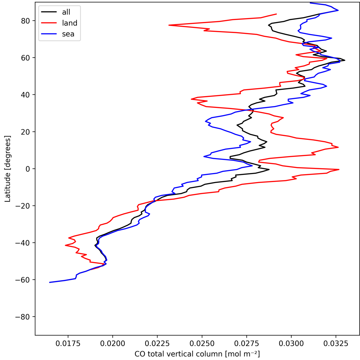
Figure 7: Zonal average of “CO total vertical column” for 2025-06-30 to 2025-06-30.
