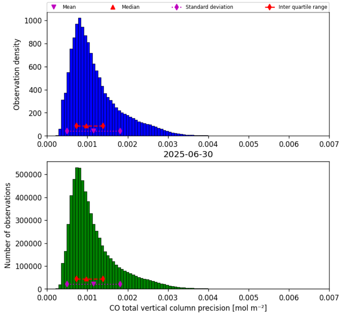
Figure 15: Histogram of “CO total vertical column precision” for 2025-06-30 to 2025-06-30
