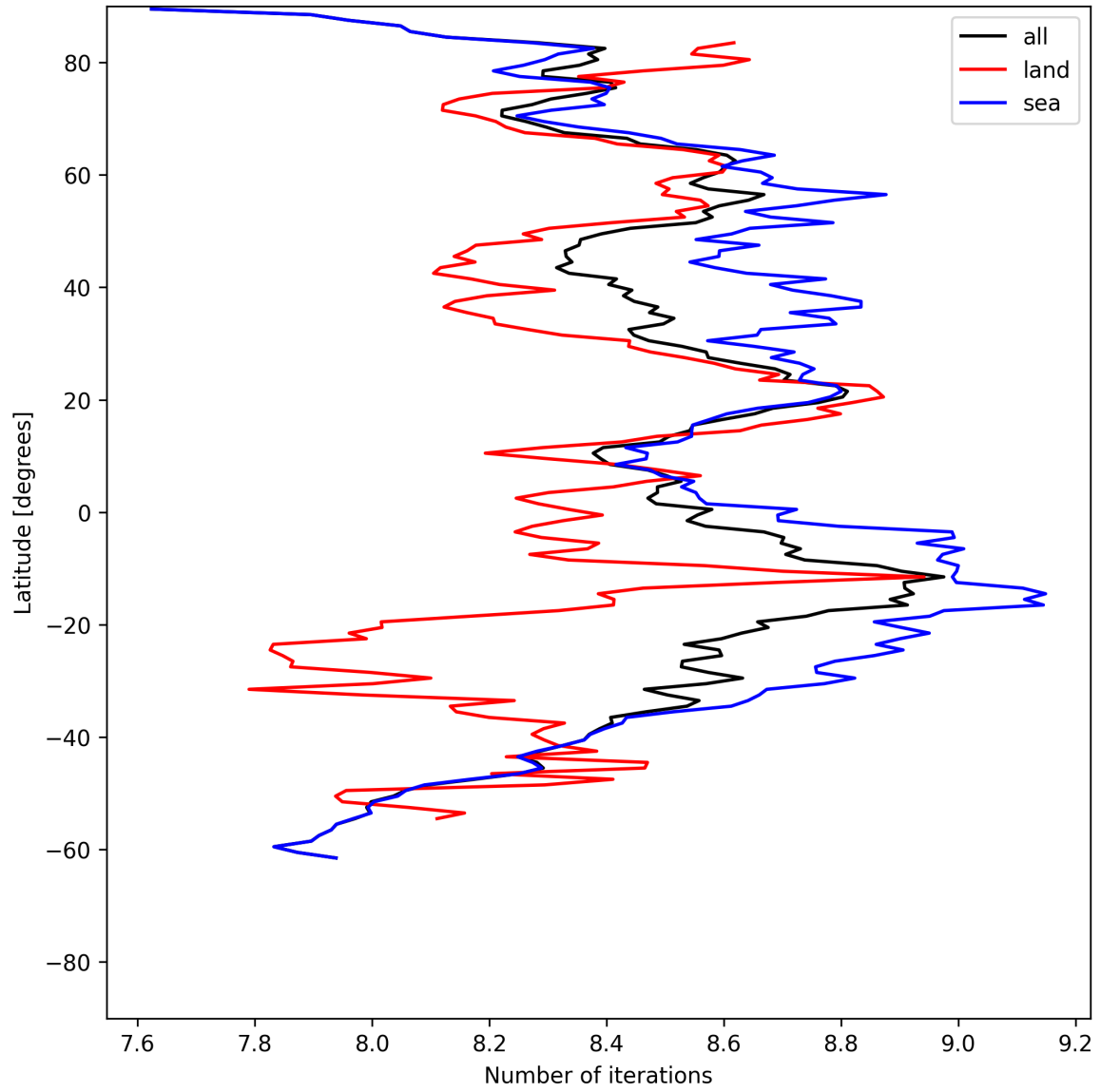
Figure 12: Zonal average of “Number of iterations” for 2025-06-30 to 2025-06-30.
