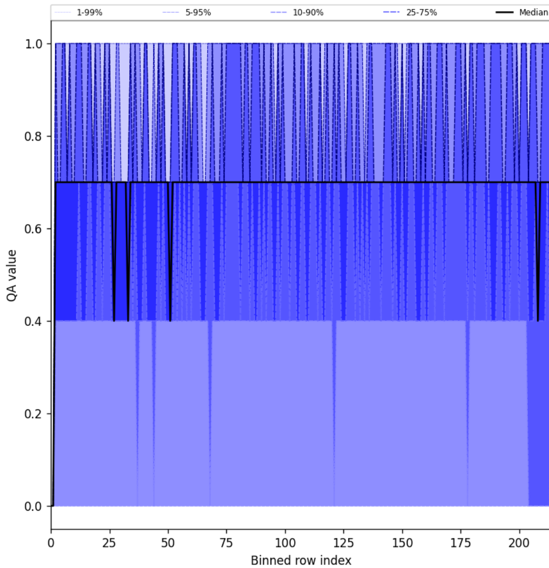
Figure 20: Along track statistics of “QA value” for 2025-06-30 to 2025-06-30
