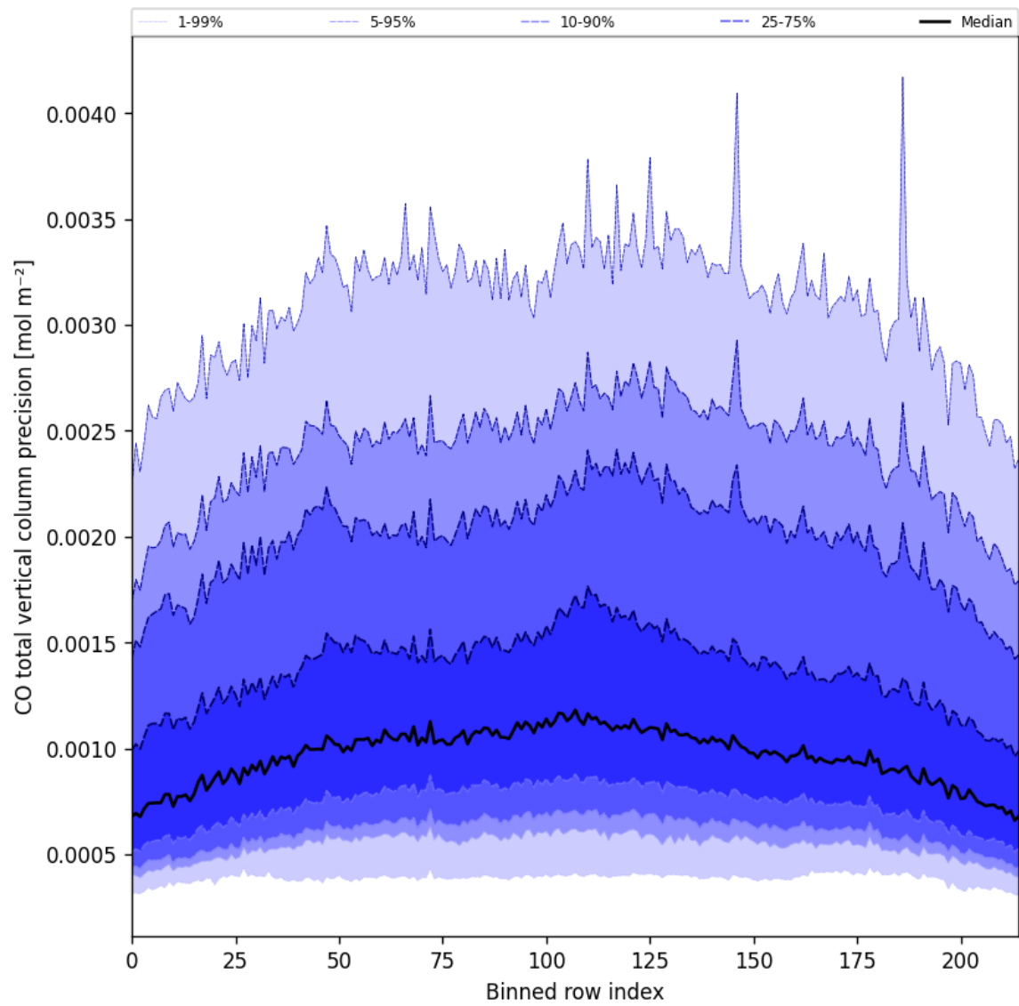
Figure 22: Along track statistics of “CO total vertical column precision” for 2025-06-30 to 2025-06-30
