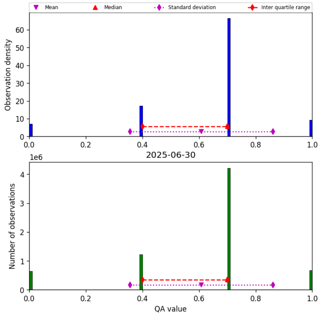
Figure 13: Histogram of “QA value” for 2025-06-30 to 2025-06-30
