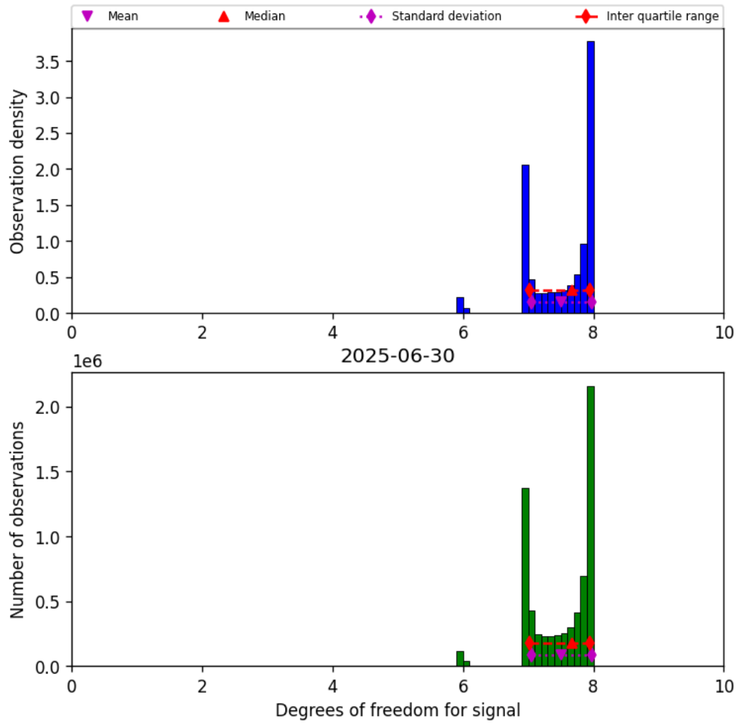
Figure 18: Histogram of “Degrees of freedom for signal” for 2025-06-30 to 2025-06-30
