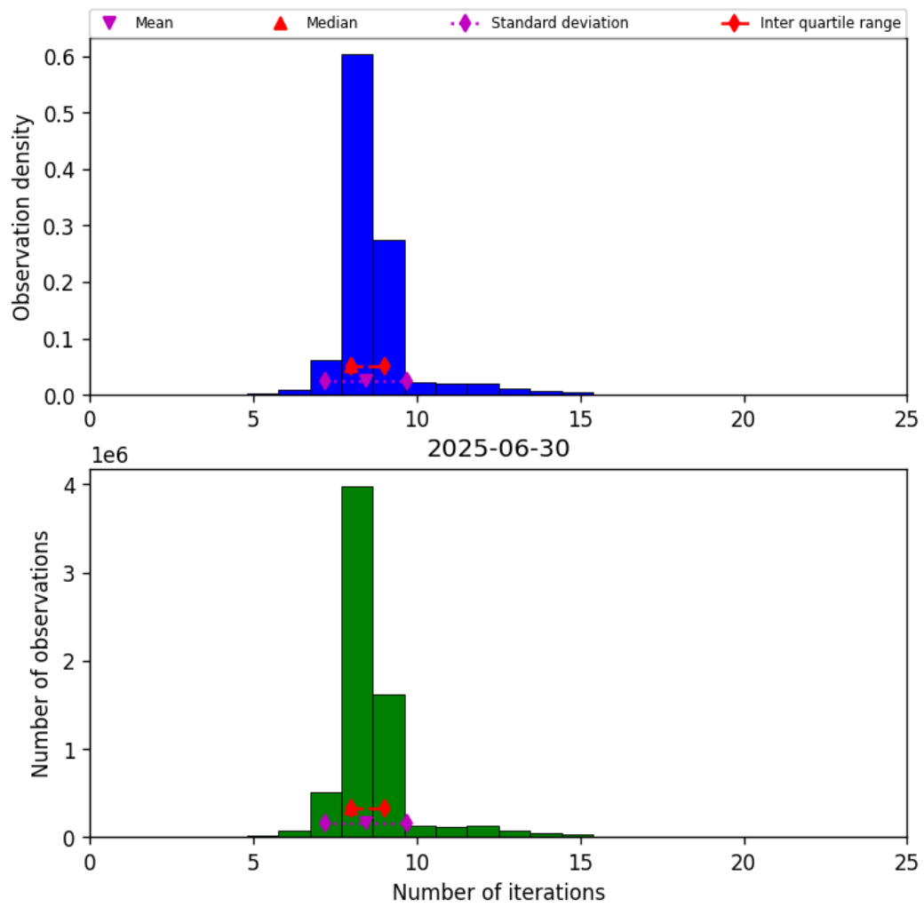
Figure 19: Histogram of “Number of iterations” for 2025-06-30 to 2025-06-30
