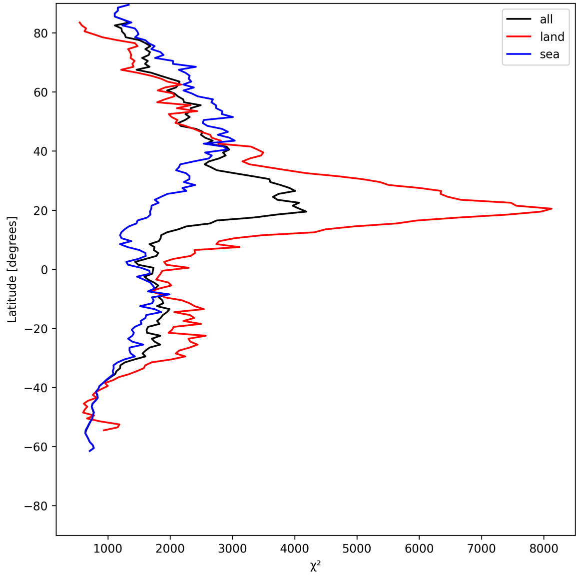
Figure 10: Zonal average of “ \chi^2 ” for 2025-06-30 to 2025-06-30.
