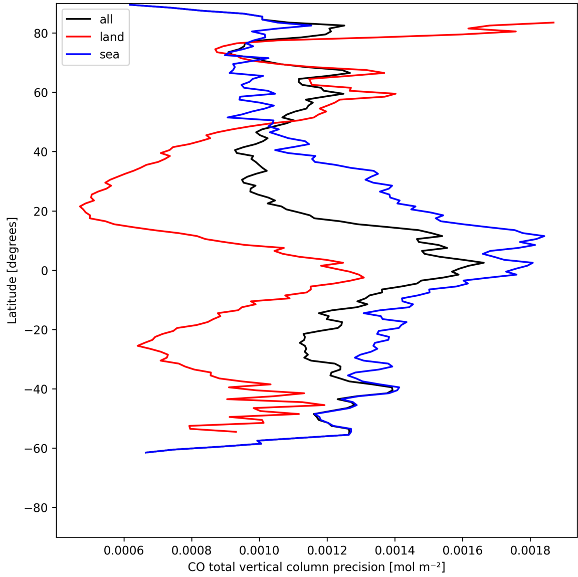
Figure 8: Zonal average of “CO total vertical column precision” for 2025-06-30 to 2025-06-30.
