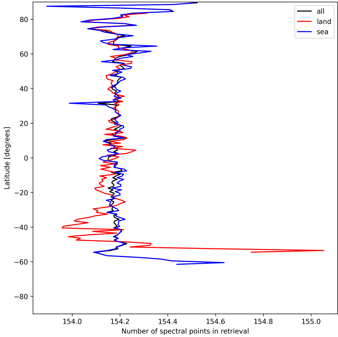
Figure 9: Zonal average of “Number of spectral points in retrieval” for 2025-06-30 to 2025-06-30.
