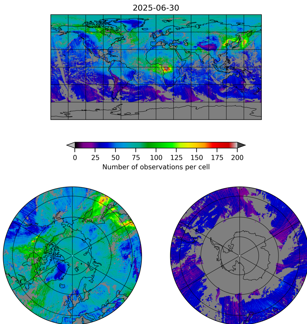
Figure 5: Map of the number of observations for 2025-06-30 to 2025-06-30
