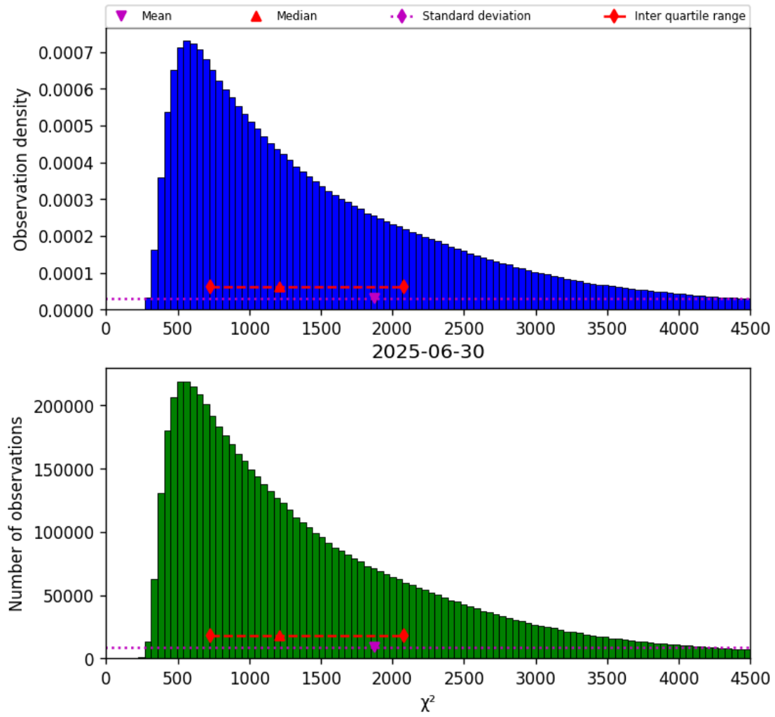
Figure 17: Histogram of " \chi^2 " for 2025-06-30 to 2025-06-30
