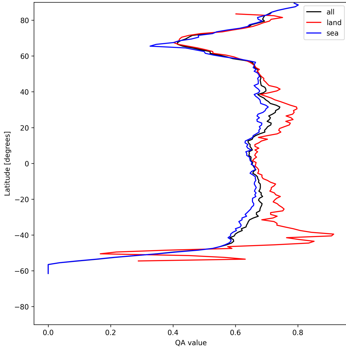
Figure 6: Zonal average of “QA value” for 2025-06-30 to 2025-06-30.
