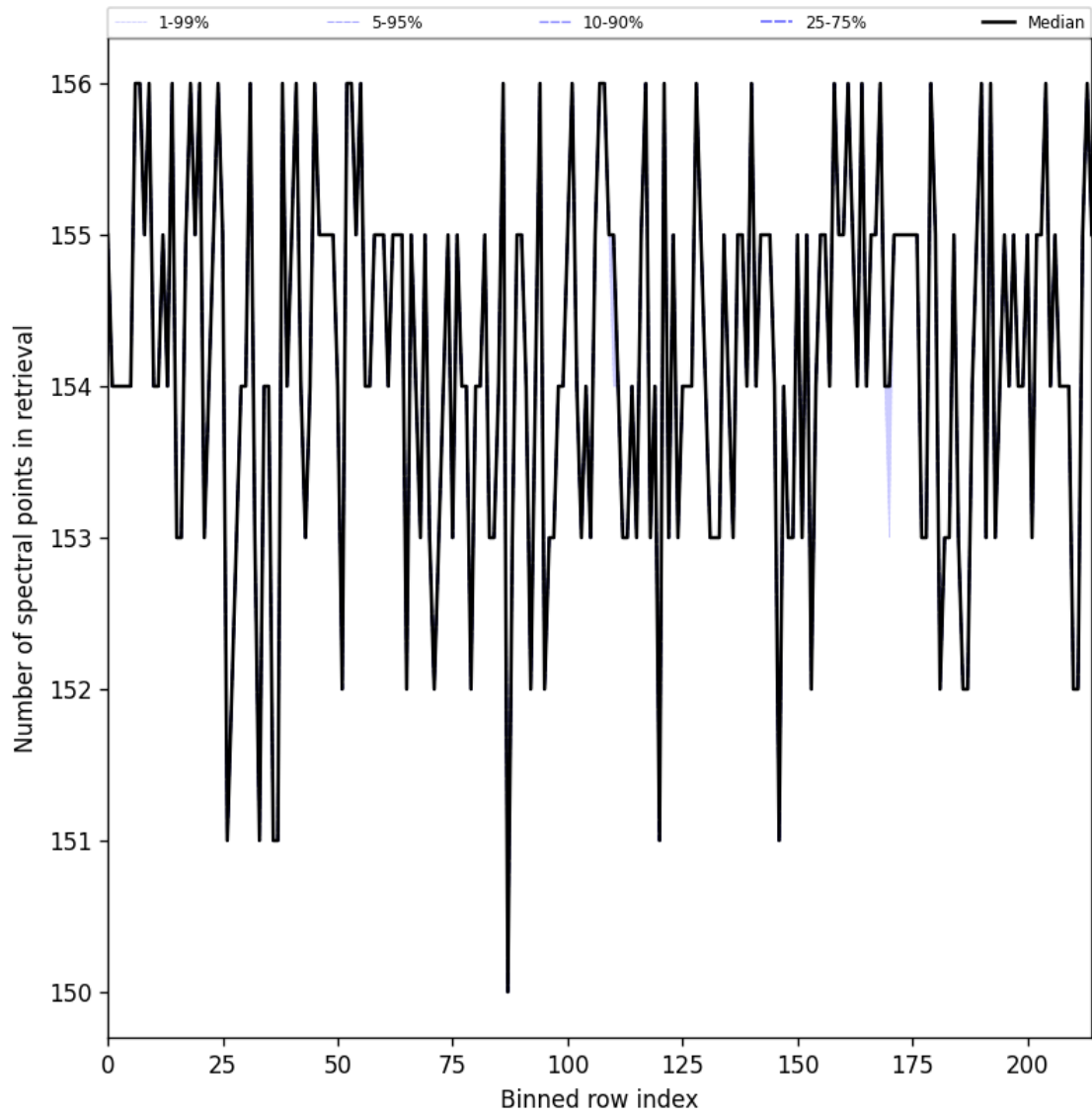
Figure 23: Along track statistics of “Number of spectral points in retrieval” for 2025-06-30 to 2025-06-30
