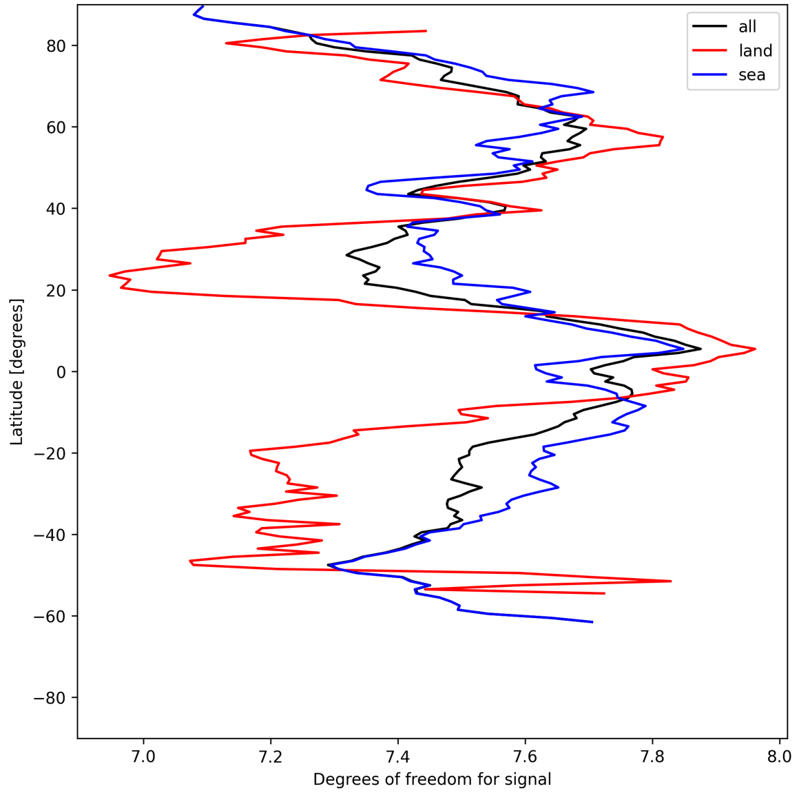
Figure 11: Zonal average of “Degrees of freedom for signal” for 2025-07-01 to 2025-07-02.
