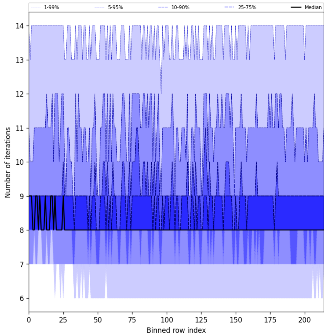
Figure 26: Along track statistics of “Number of iterations” for 2025-07-01 to 2025-07-02
