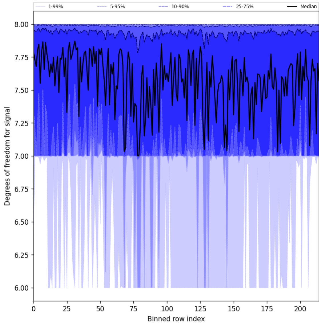
Figure 25: Along track statistics of “Degrees of freedom for signal” for 2025-07-01 to 2025-07-02
