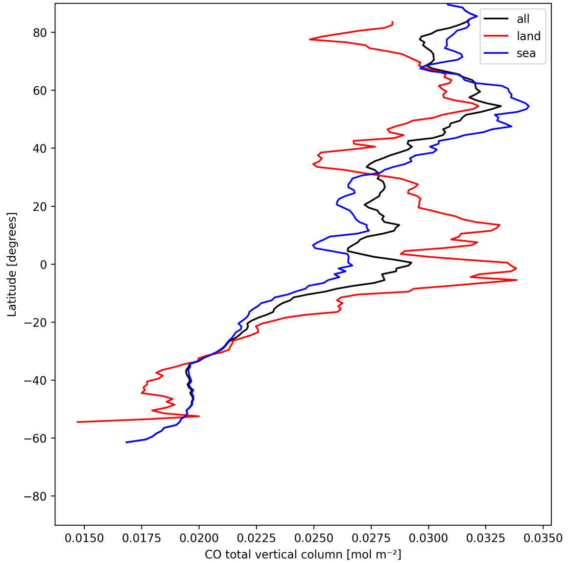
Figure 7: Zonal average of “CO total vertical column” for 2025-07-01 to 2025-07-02.
