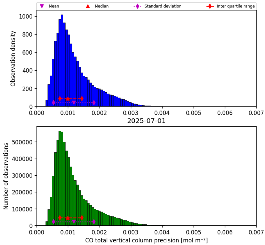
Figure 15: Histogram of “CO total vertical column precision” for 2025-07-01 to 2025-07-02
