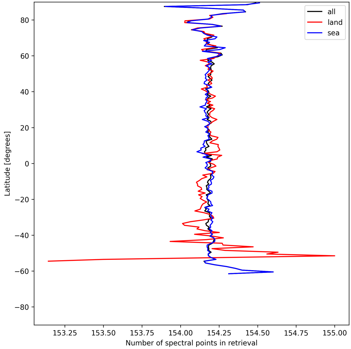
Figure 9: Zonal average of “Number of spectral points in retrieval” for 2025-07-01 to 2025-07-02.
