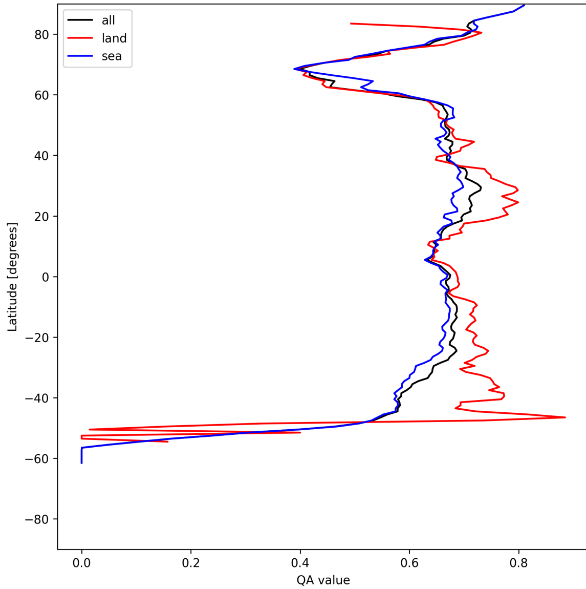
Figure 6: Zonal average of “QA value” for 2025-07-01 to 2025-07-02.
