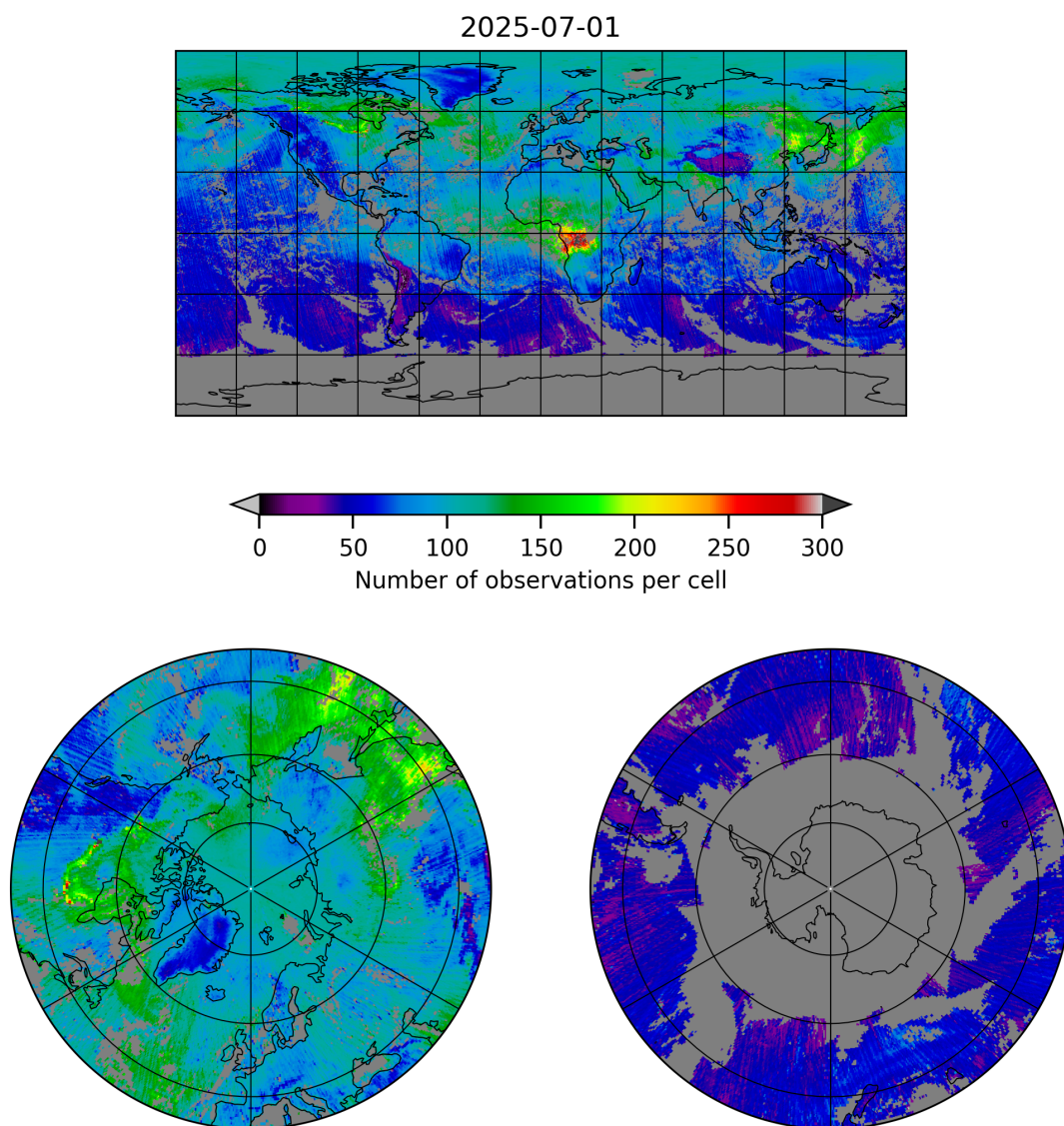
Figure 5: Map of the number of observations for 2025-07-01 to 2025-07-02
