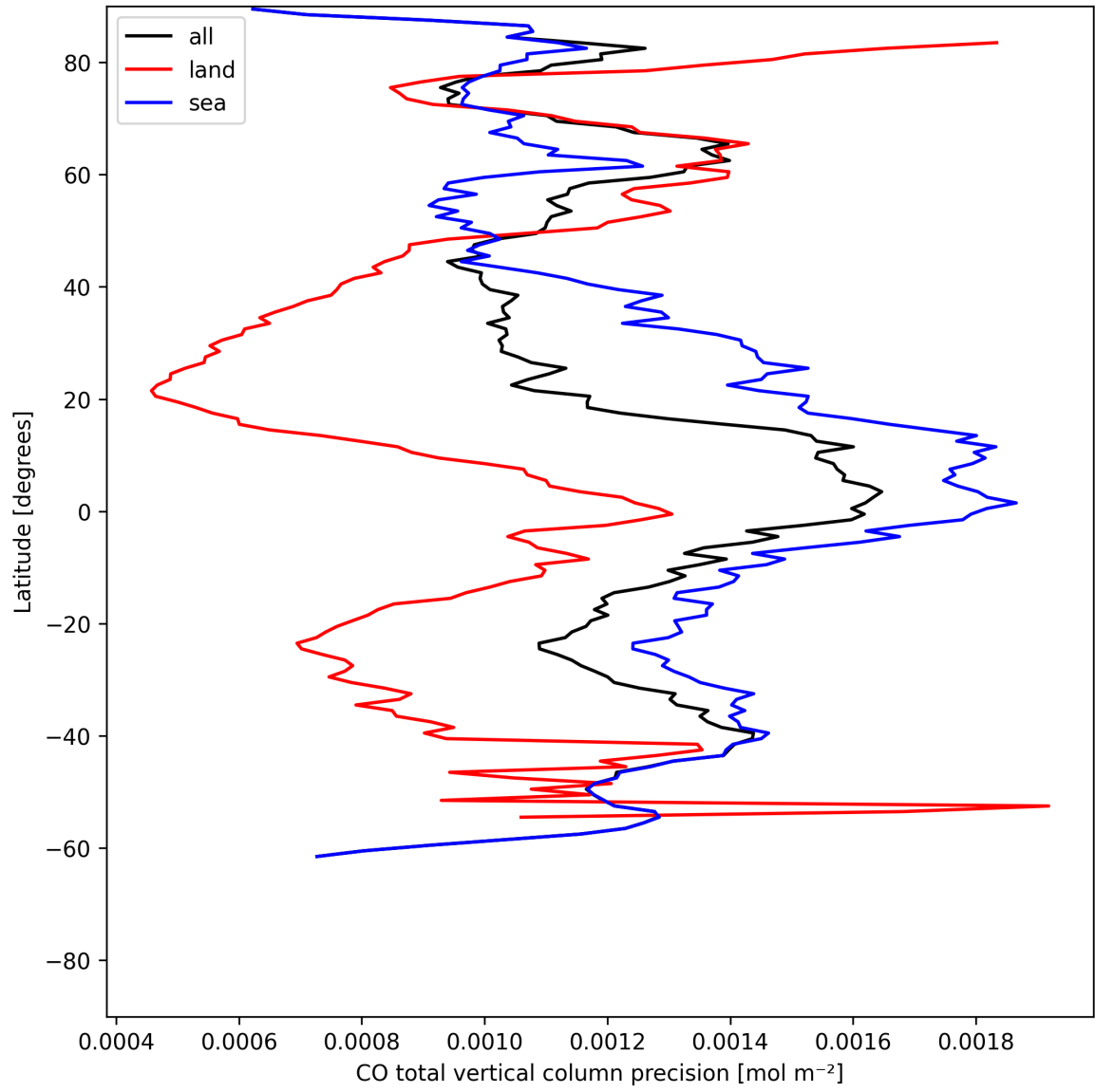
Figure 8: Zonal average of "CO total vertical column precision" for 2025-07-01 to 2025-07-02.
