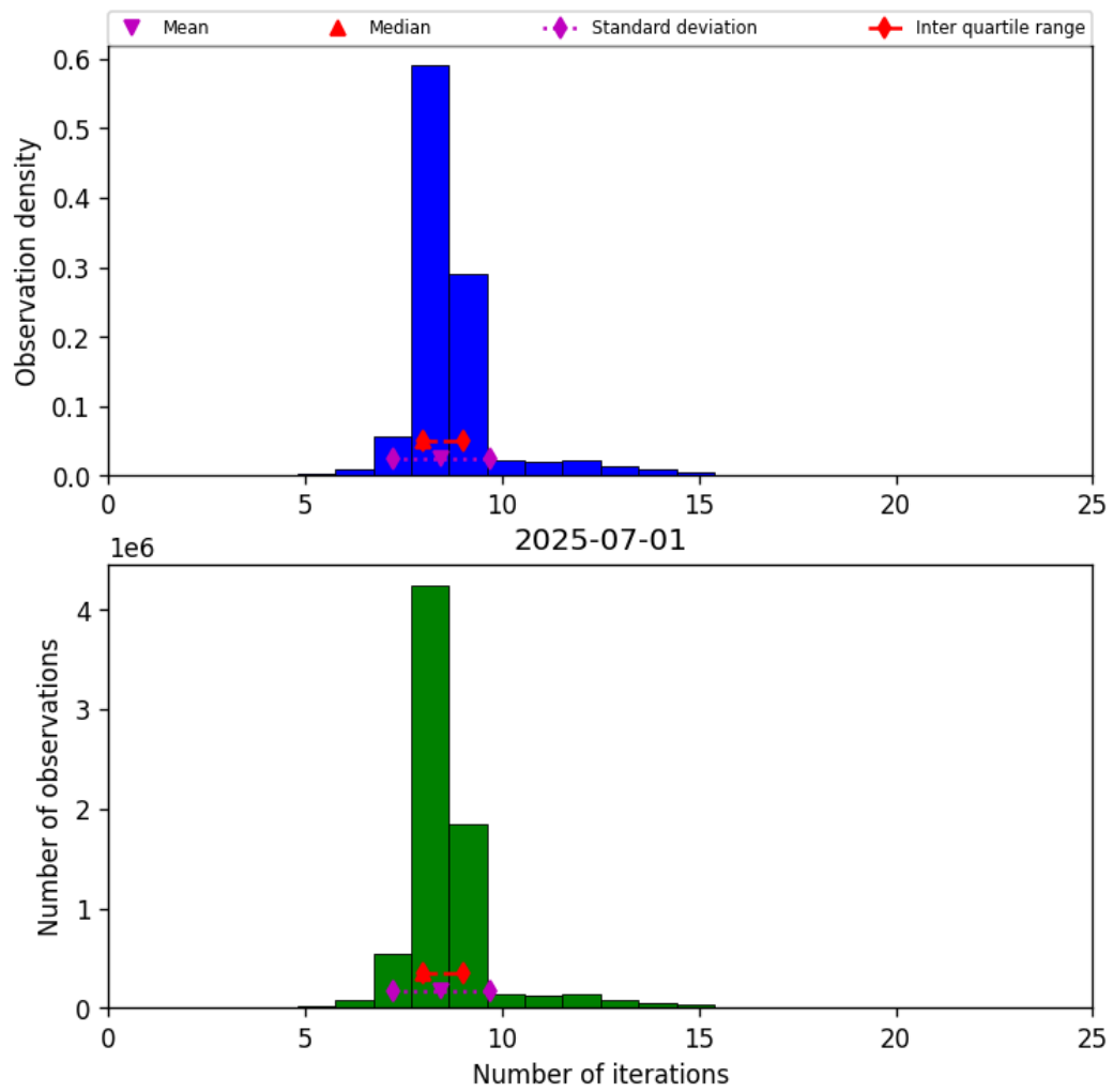
Figure 19: Histogram of “Number of iterations” for 2025-07-01 to 2025-07-02
