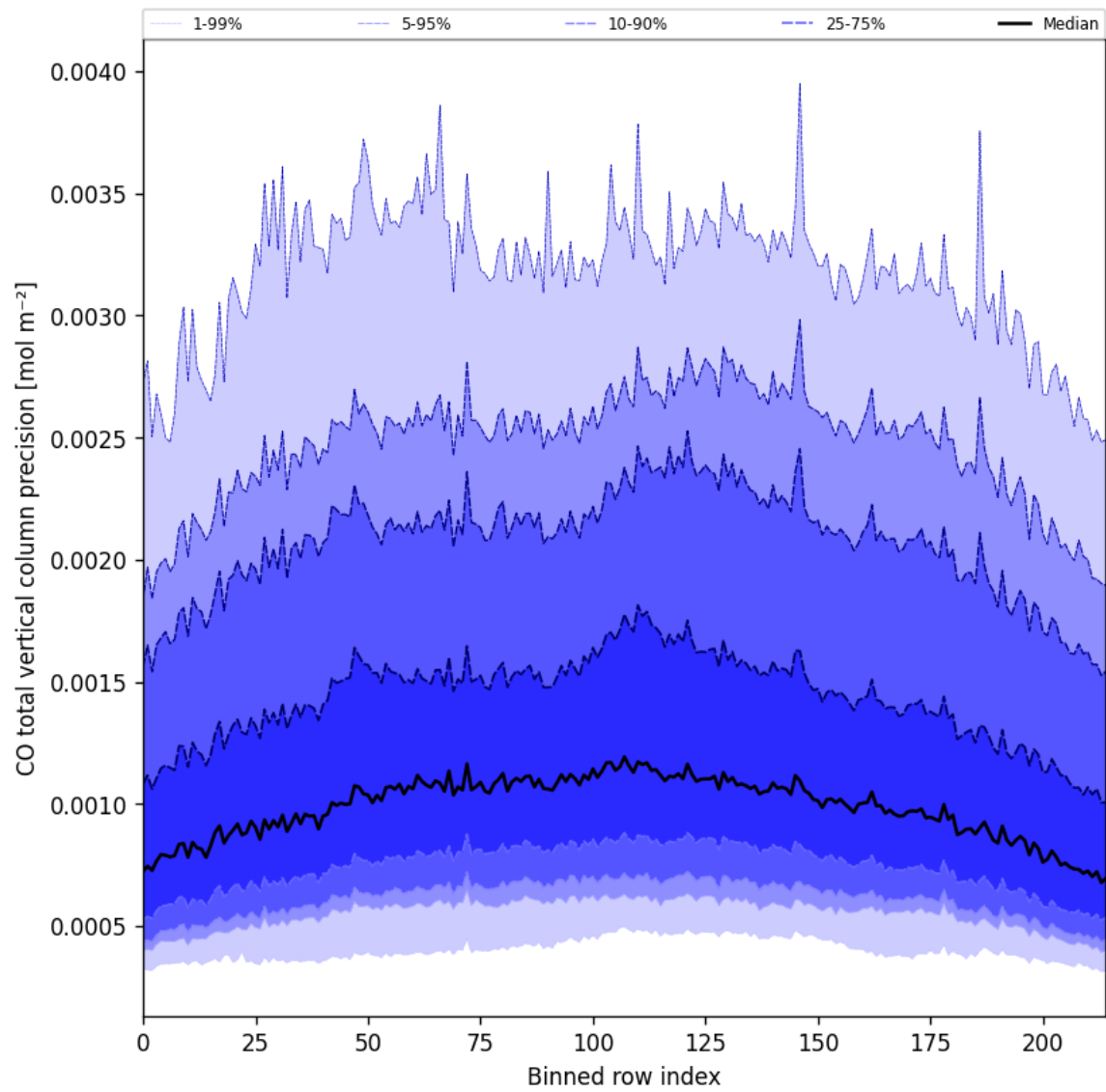
Figure 22: Along track statistics of “CO total vertical column precision” for 2025-07-01 to 2025-07-02
