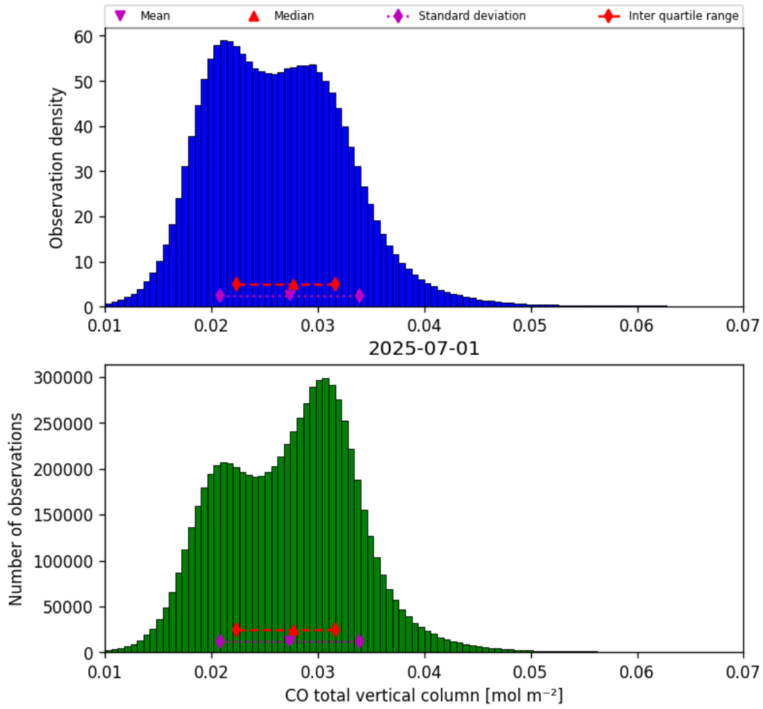
Figure 14: Histogram of “CO total vertical column” for 2025-07-01 to 2025-07-02
