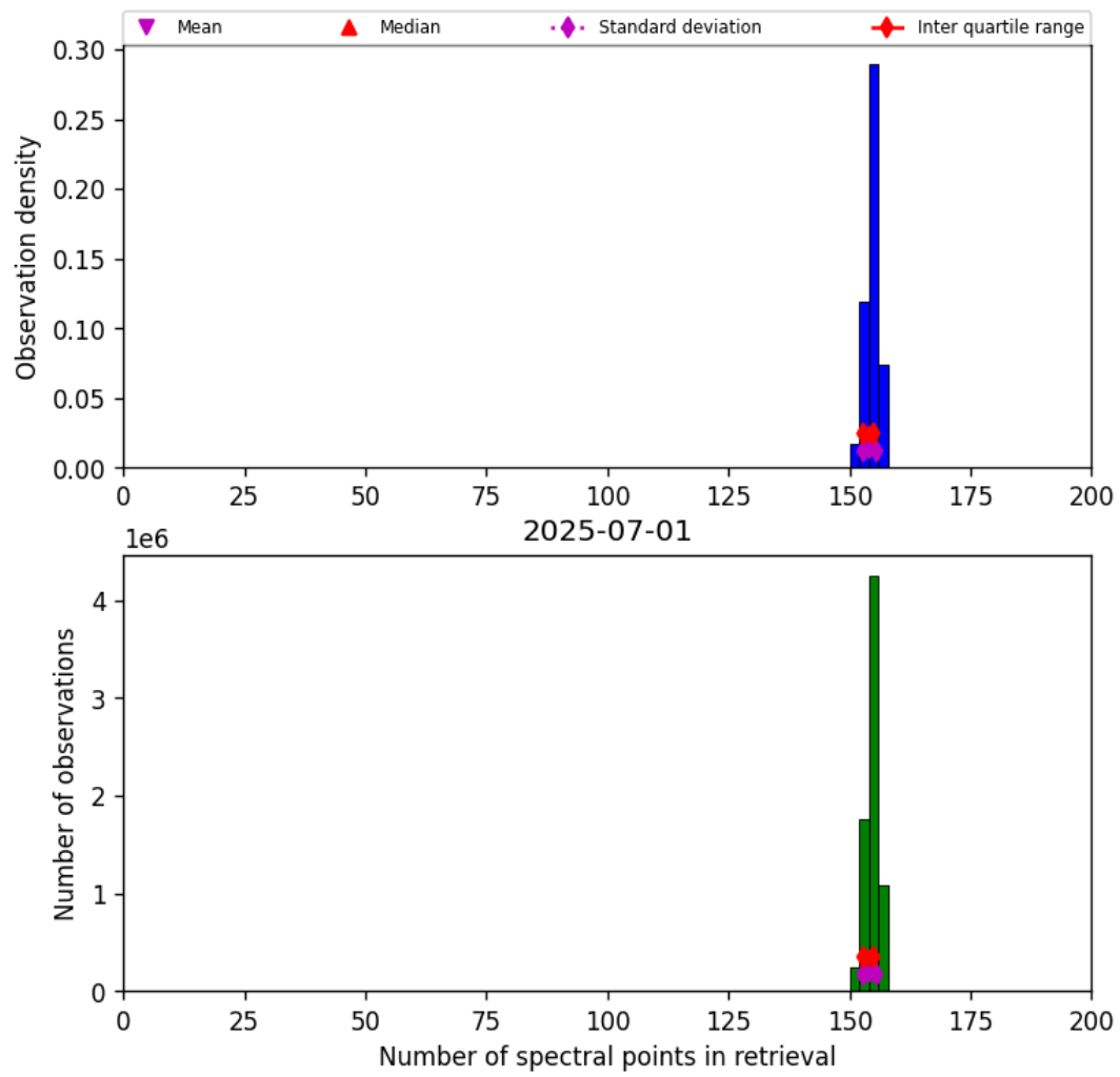
Figure 16: Histogram of “Number of spectral points in retrieval” for 2025-07-01 to 2025-07-02
