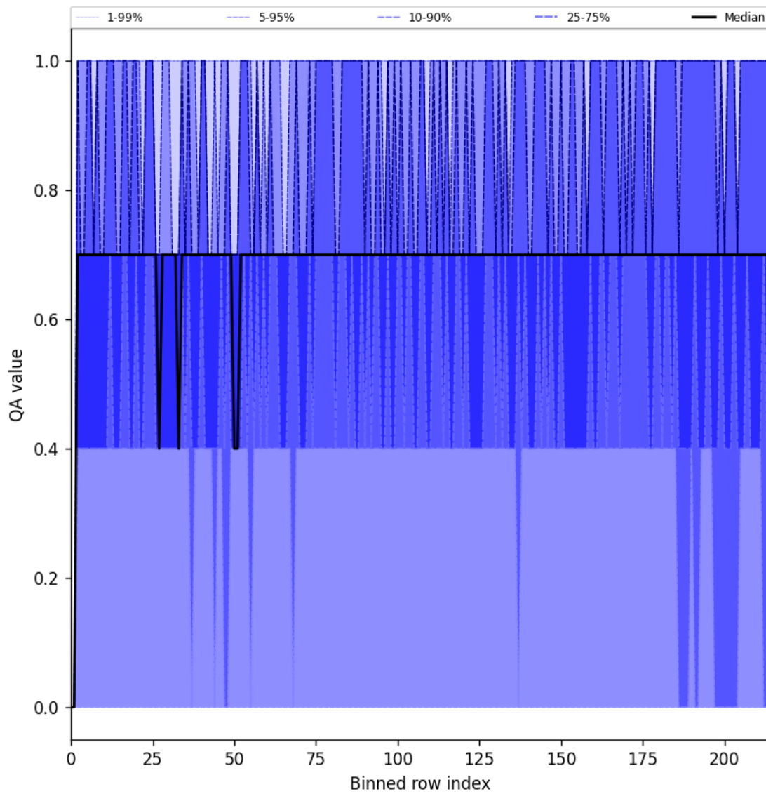
Figure 20: Along track statistics of “QA value” for 2025-07-01 to 2025-07-02
