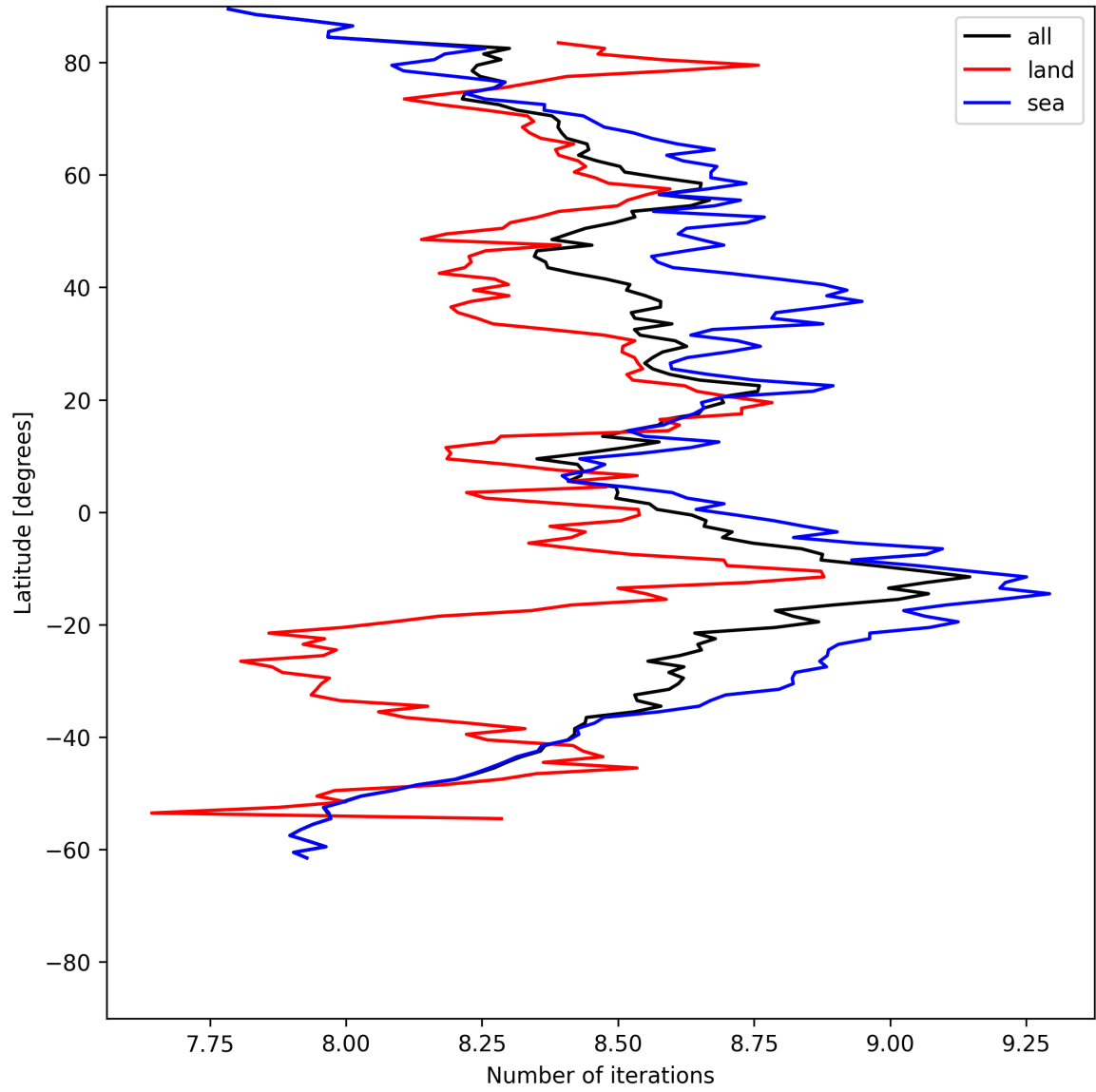
Figure 12: Zonal average of “Number of iterations” for 2025-07-01 to 2025-07-02.
