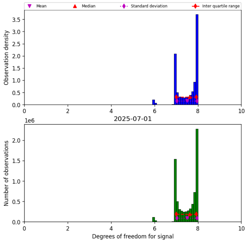
Figure 18: Histogram of “Degrees of freedom for signal” for 2025-07-01 to 2025-07-02
