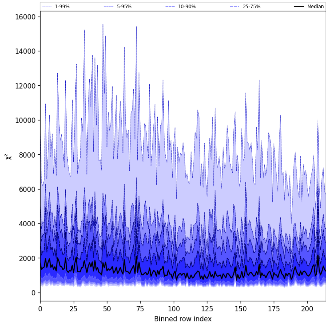
Figure 24: Along track statistics of “ \chi^2 ” for 2025-07-01 to 2025-07-02
