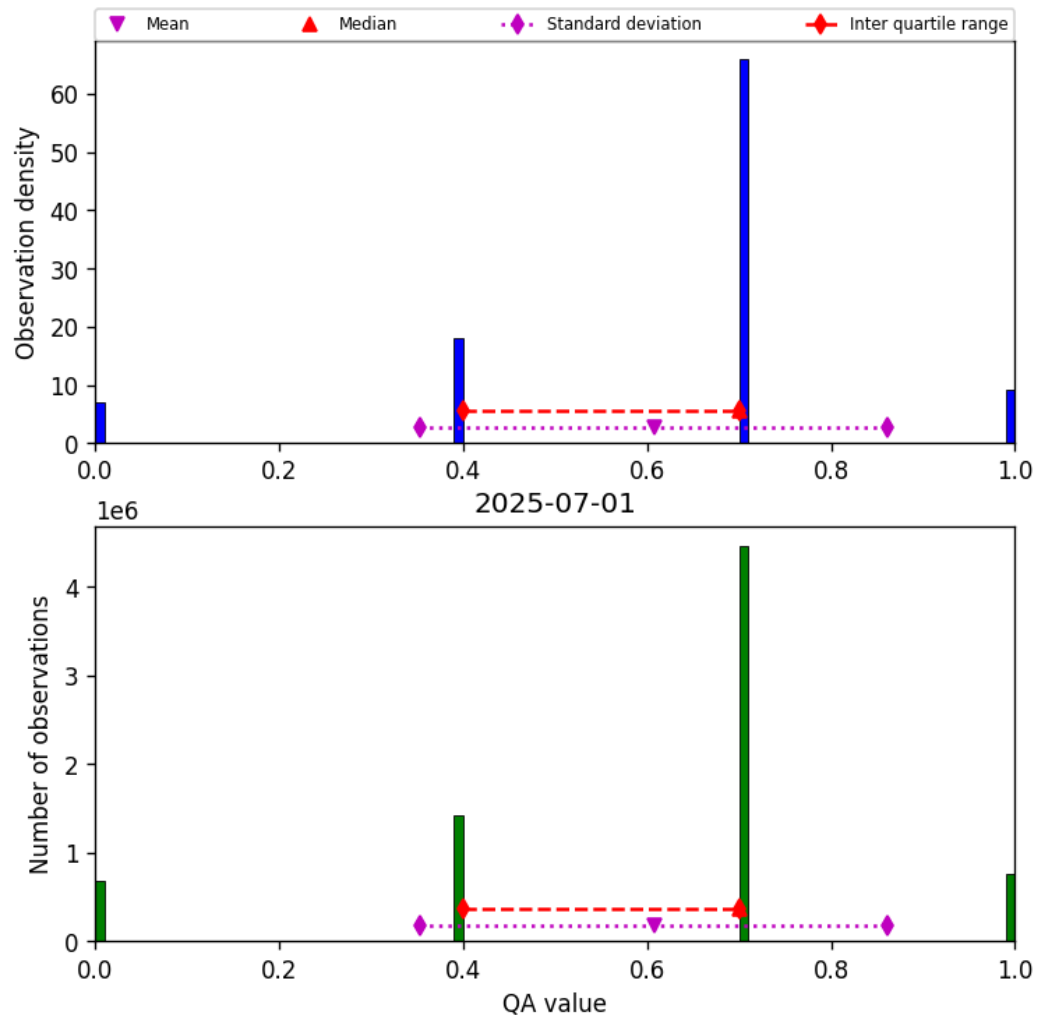
Figure 13: Histogram of “QA value” for 2025-07-01 to 2025-07-02
