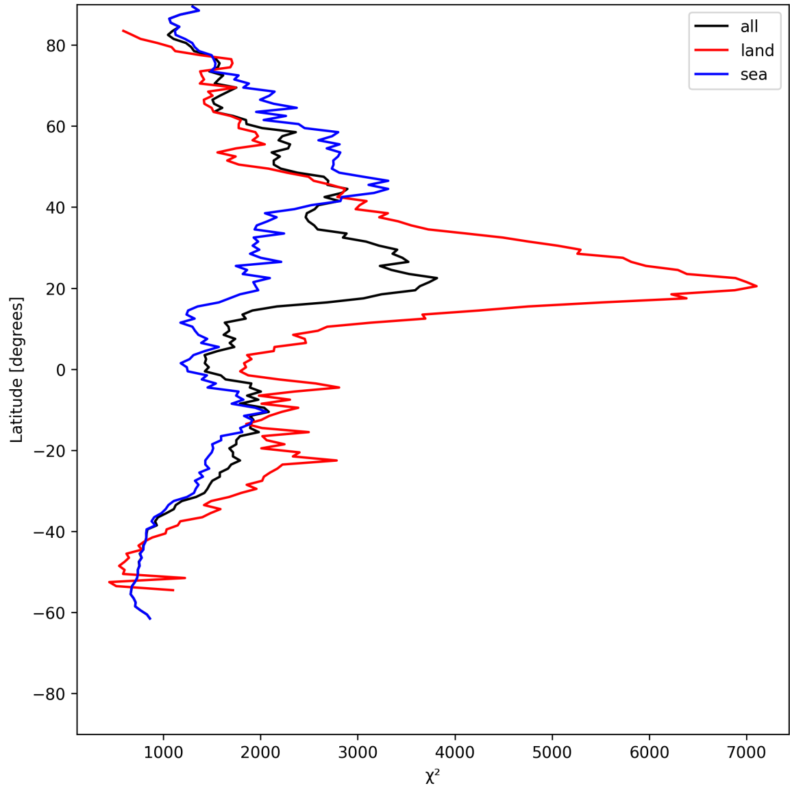
Figure 10: Zonal average of “ \chi^2 ” for 2025-07-01 to 2025-07-02.
