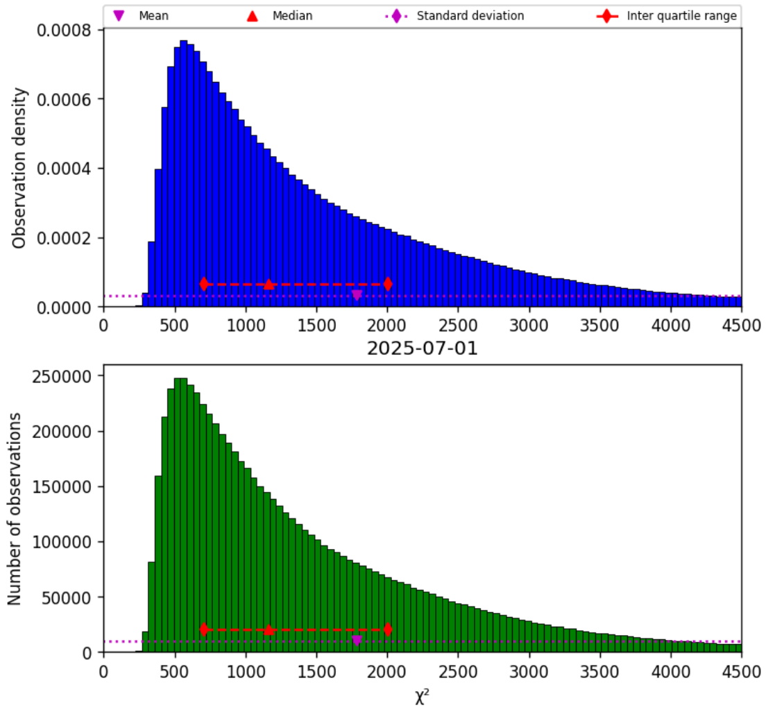
Figure 17: Histogram of “ \chi^2 ” for 2025-07-01 to 2025-07-02
