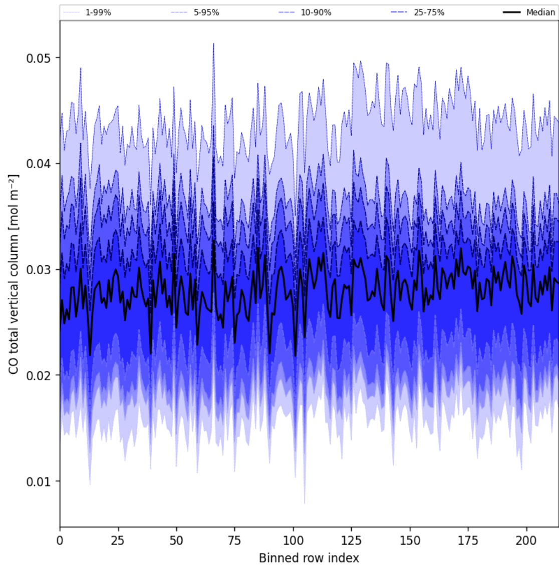
Figure 21: Along track statistics of “CO total vertical column” for 2025-07-01 to 2025-07-02
