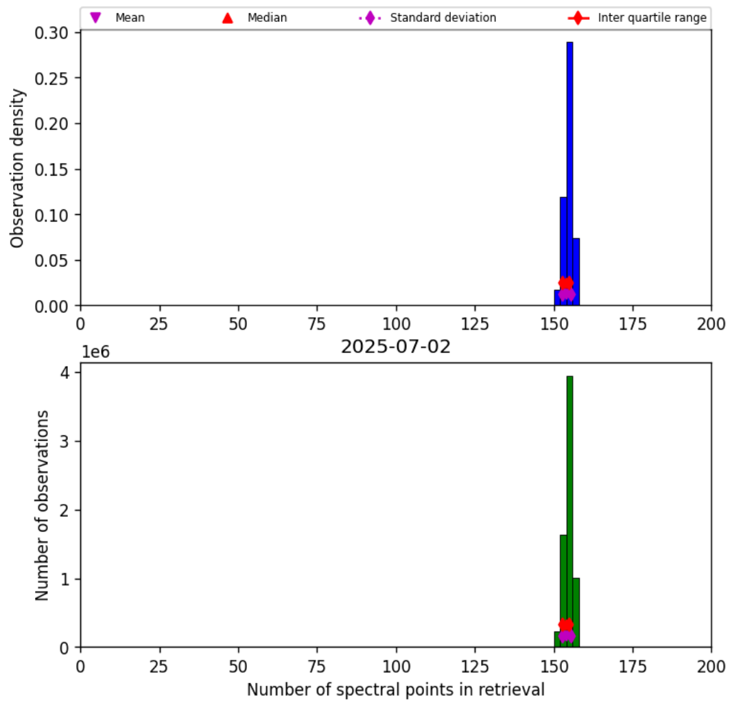
Figure 16: Histogram of “Number of spectral points in retrieval” for 2025-07-02 to 2025-07-03
