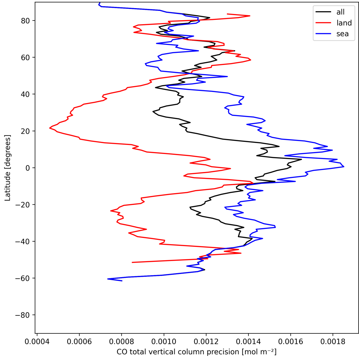
Figure 8: Zonal average of “CO total vertical column precision” for 2025-07-02 to 2025-07-03.
