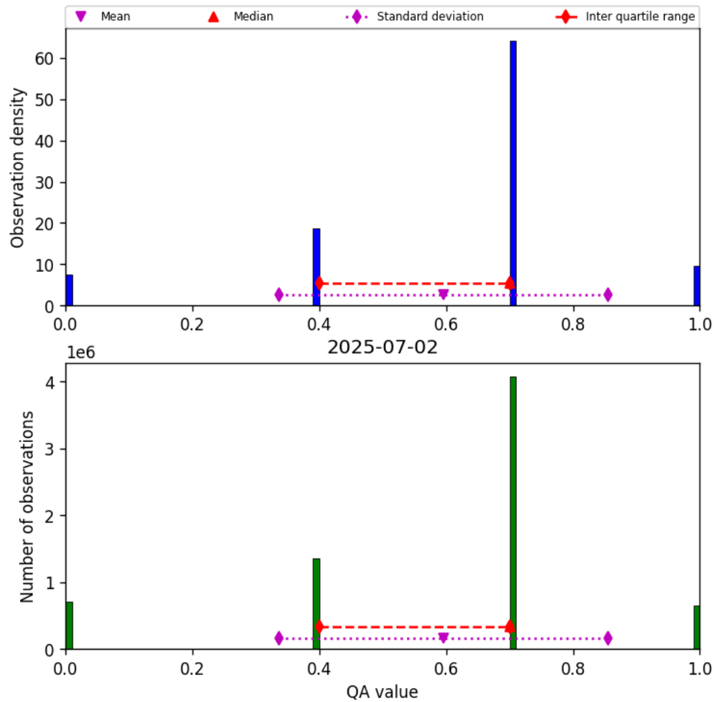
Figure 13: Histogram of “QA value” for 2025-07-02 to 2025-07-03
