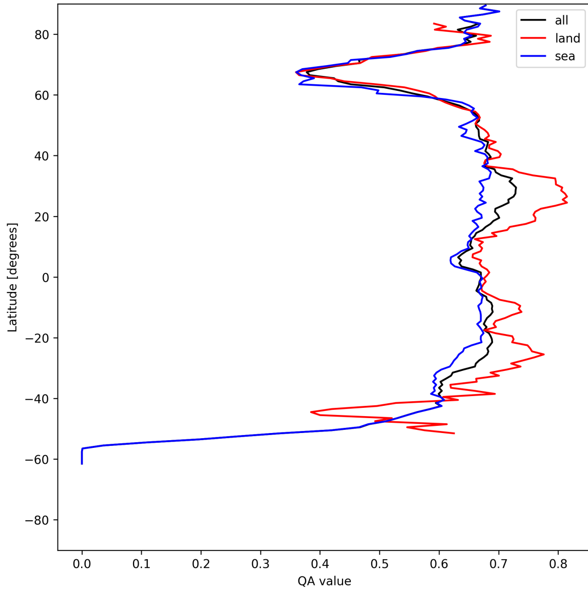
Figure 6: Zonal average of “QA value” for 2025-07-02 to 2025-07-03.
