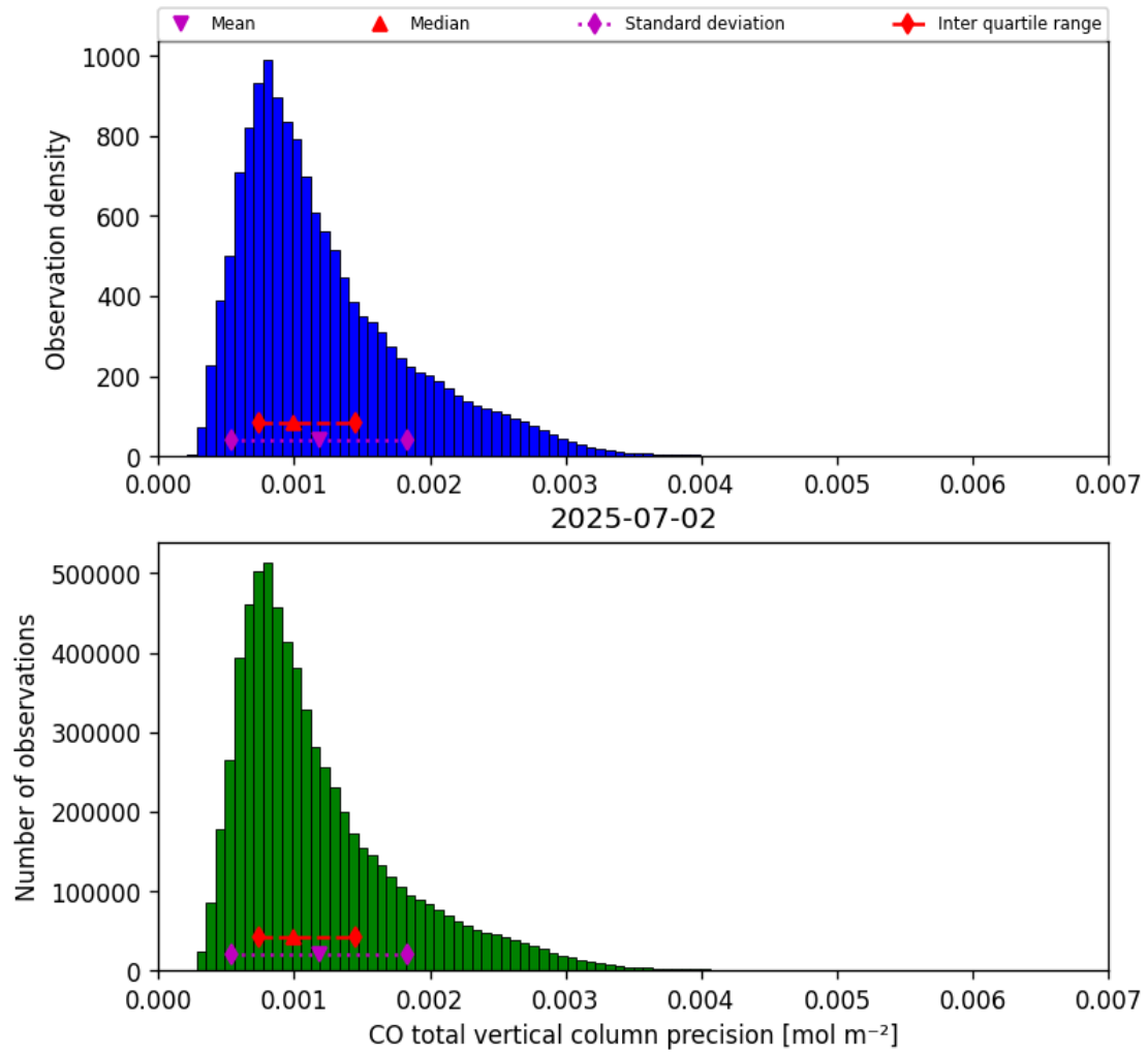
Figure 15: Histogram of “CO total vertical column precision” for 2025-07-02 to 2025-07-03
