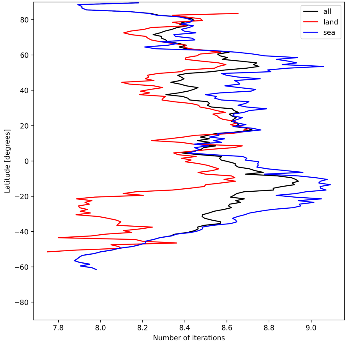
Figure 12: Zonal average of “Number of iterations” for 2025-07-02 to 2025-07-03.
