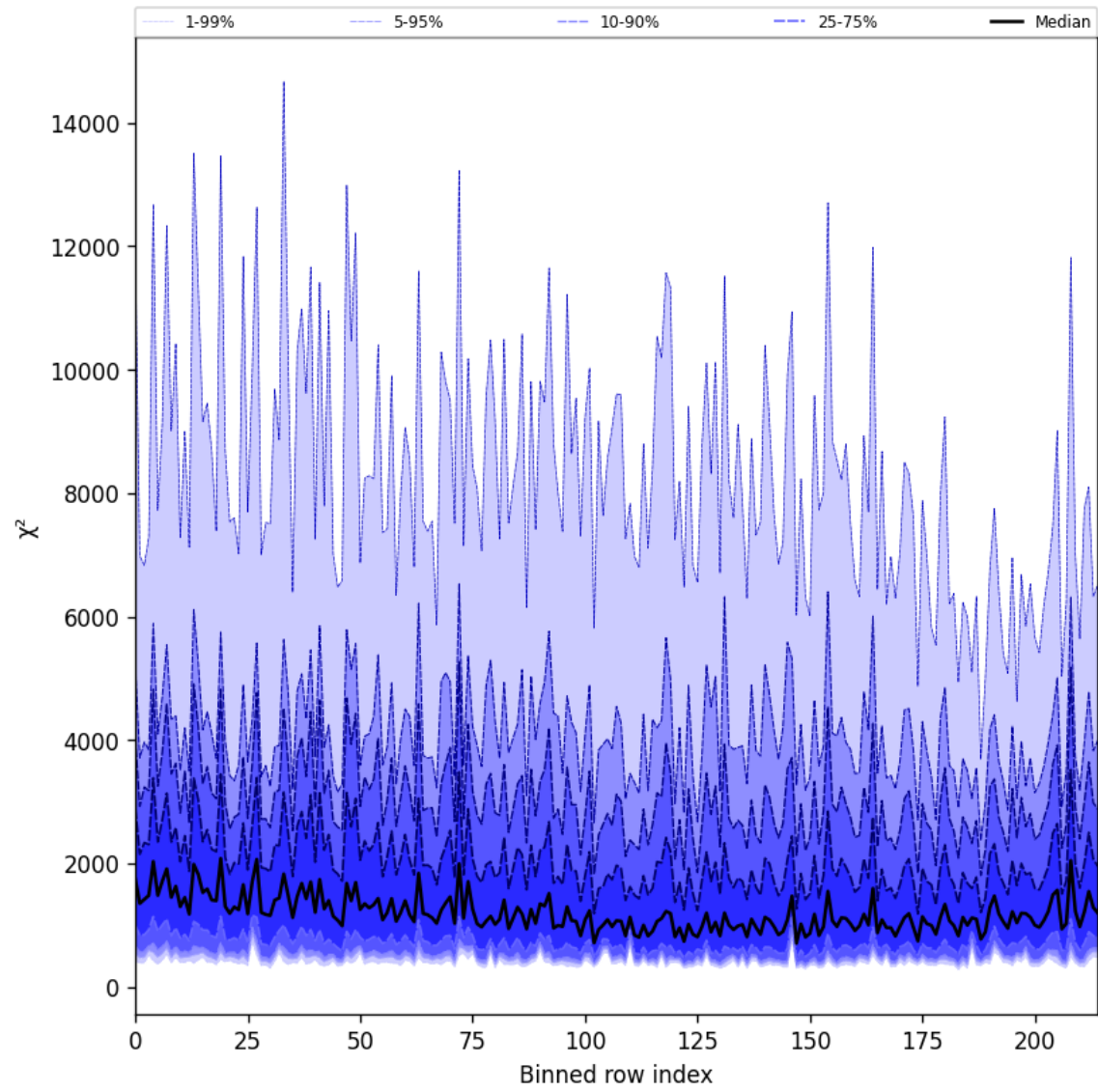
Figure 24: Along track statistics of “ \chi^2 ” for 2025-07-02 to 2025-07-03
