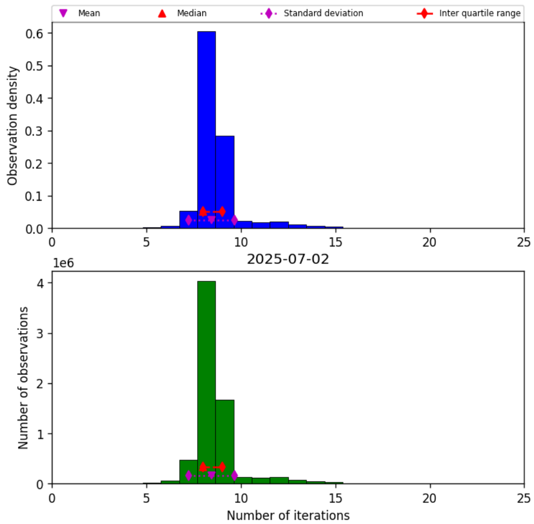
Figure 19: Histogram of “Number of iterations” for 2025-07-02 to 2025-07-03
