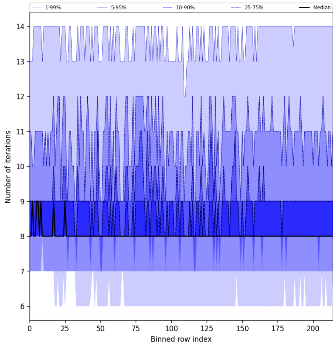
Figure 26: Along track statistics of “Number of iterations” for 2025-07-02 to 2025-07-03
