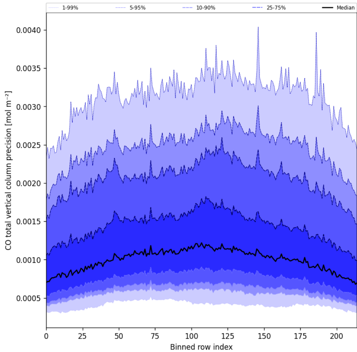
Figure 22: Along track statistics of “CO total vertical column precision” for 2025-07-02 to 2025-07-03
