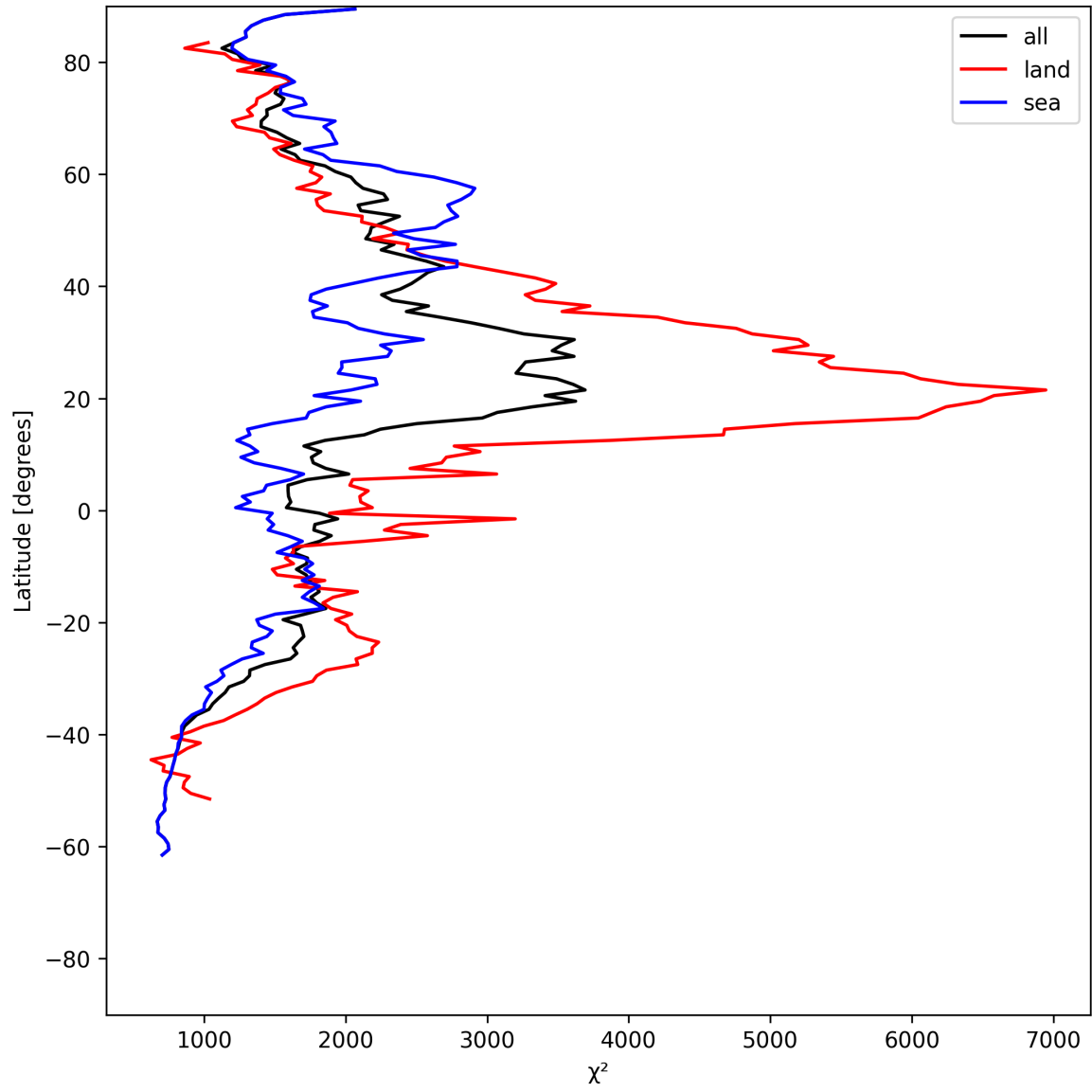
Figure 10: Zonal average of “ \chi^2 ” for 2025-07-02 to 2025-07-03.
