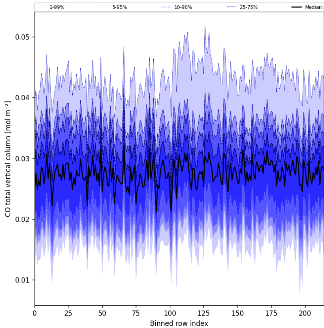
Figure 21: Along track statistics of “CO total vertical column” for 2025-07-02 to 2025-07-03
