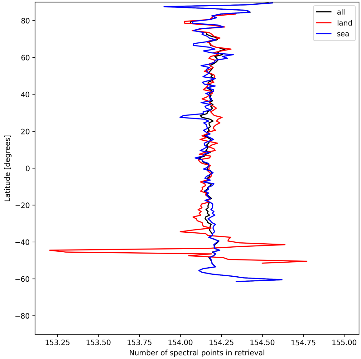
Figure 9: Zonal average of “Number of spectral points in retrieval” for 2025-07-02 to 2025-07-03.
