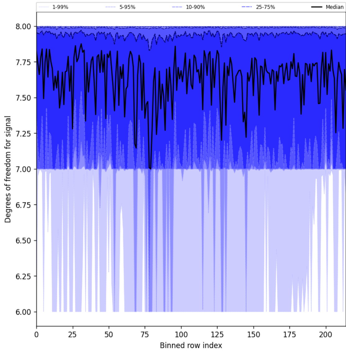
Figure 25: Along track statistics of “Degrees of freedom for signal” for 2025-07-02 to 2025-07-03
