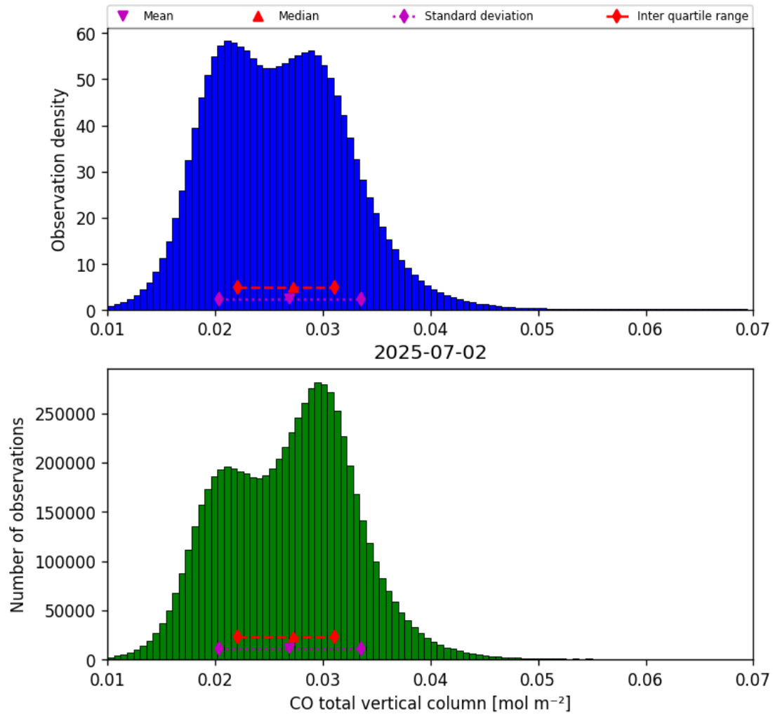
Figure 14: Histogram of “CO total vertical column” for 2025-07-02 to 2025-07-03
