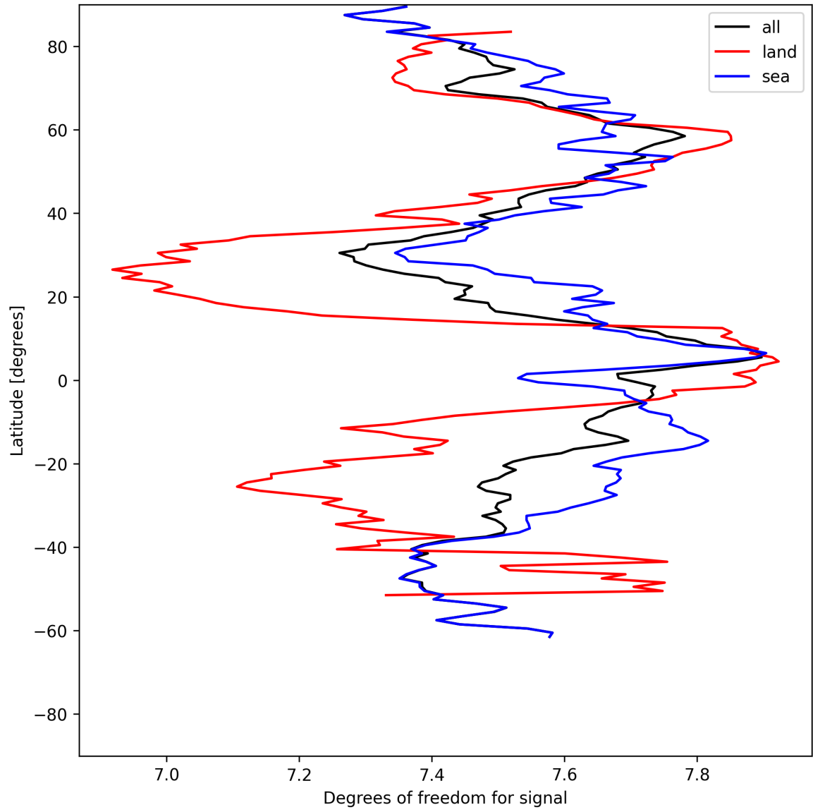
Figure 11: Zonal average of “Degrees of freedom for signal” for 2025-07-02 to 2025-07-03.
