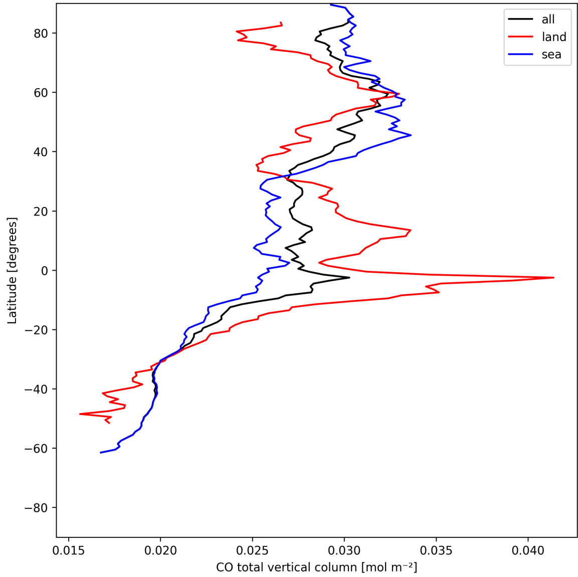
Figure 7: Zonal average of “CO total vertical column” for 2025-07-02 to 2025-07-03.
