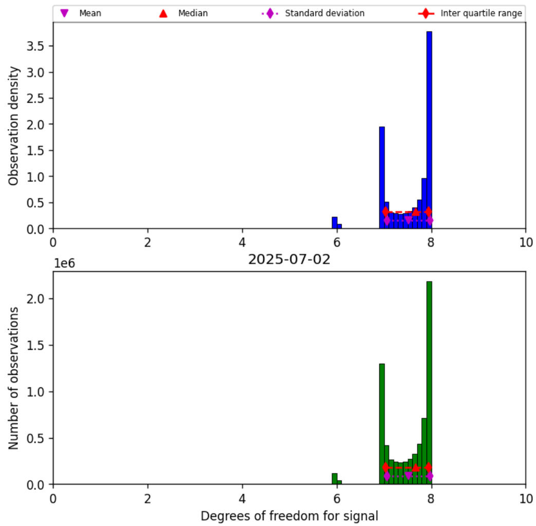
Figure 18: Histogram of “Degrees of freedom for signal” for 2025-07-02 to 2025-07-03
