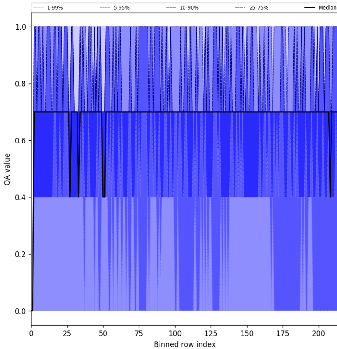
Figure 20: Along track statistics of “QA value” for 2025-07-02 to 2025-07-03
