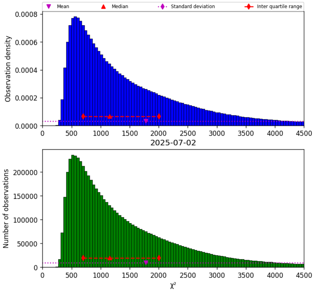
Figure 17: Histogram of " \chi^2 " for 2025-07-02 to 2025-07-03
