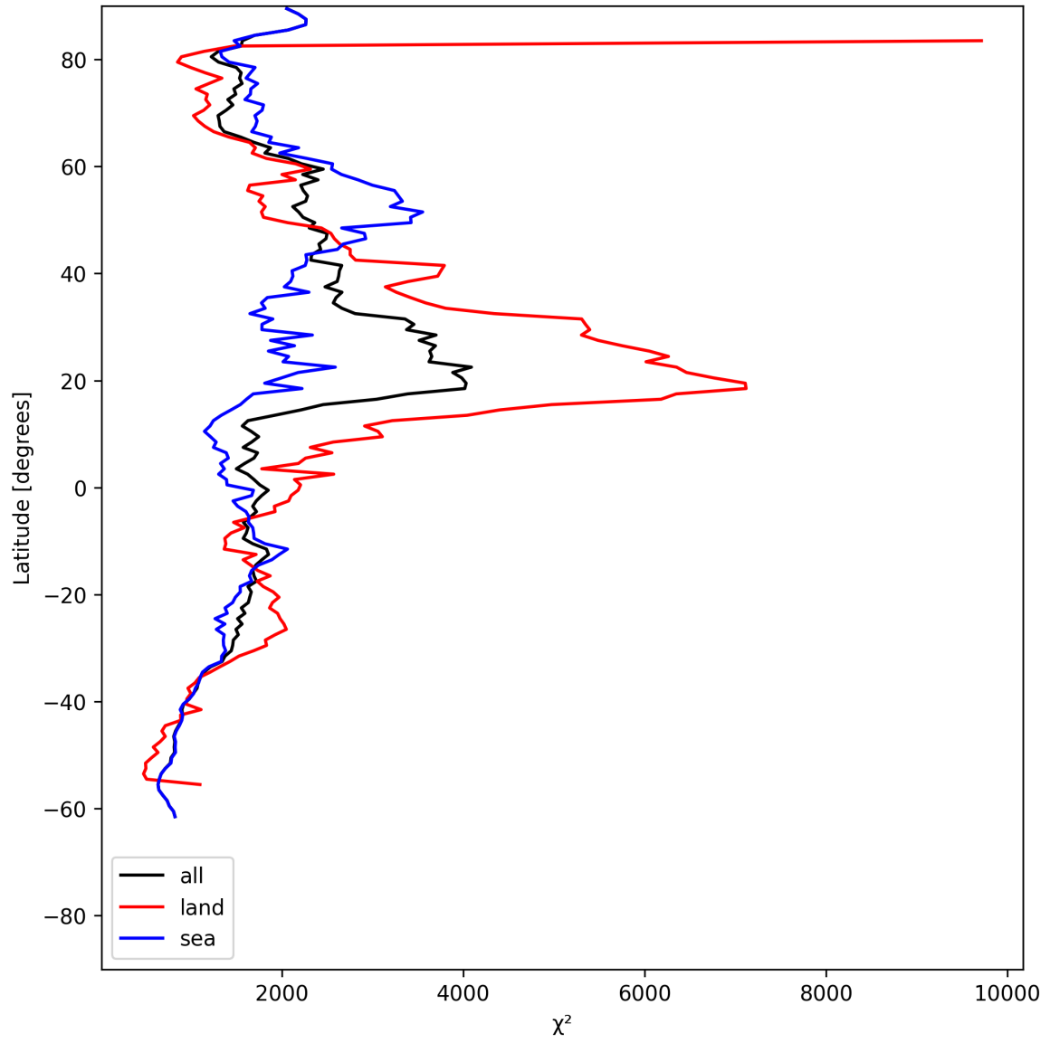
Figure 10: Zonal average of “ \chi^2 ” for 2025-07-04 to 2025-07-05.
