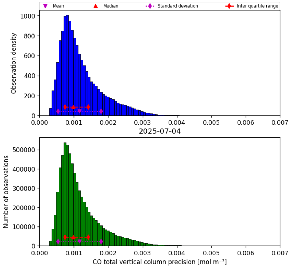
Figure 15: Histogram of “CO total vertical column precision” for 2025-07-04 to 2025-07-05
