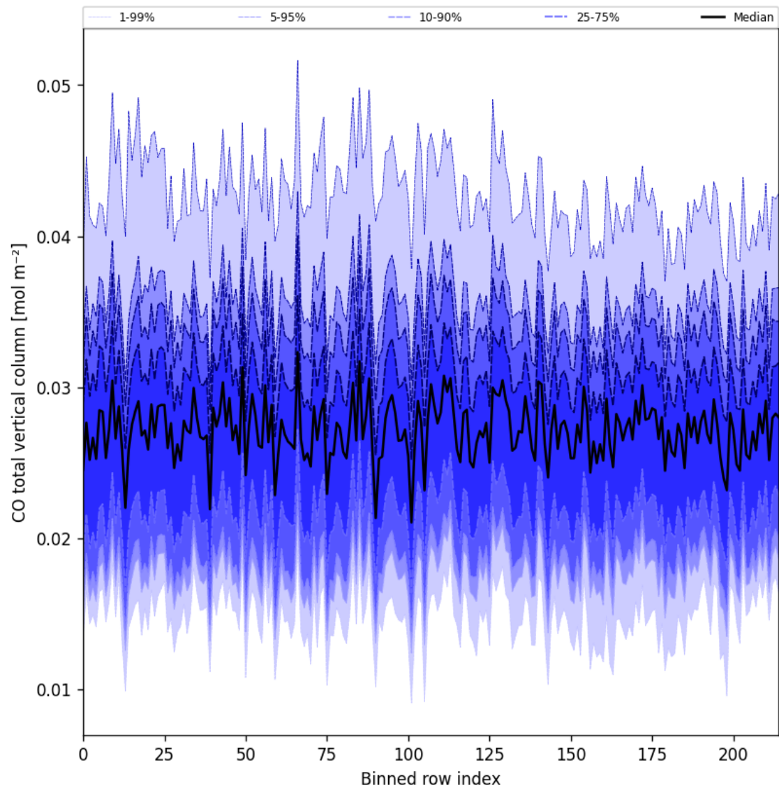
Figure 21: Along track statistics of “CO total vertical column” for 2025-07-04 to 2025-07-05
