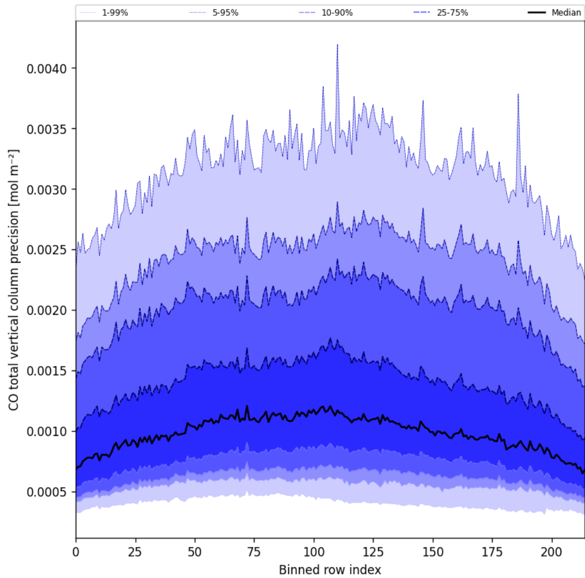
Figure 22: Along track statistics of “CO total vertical column precision” for 2025-07-04 to 2025-07-05
