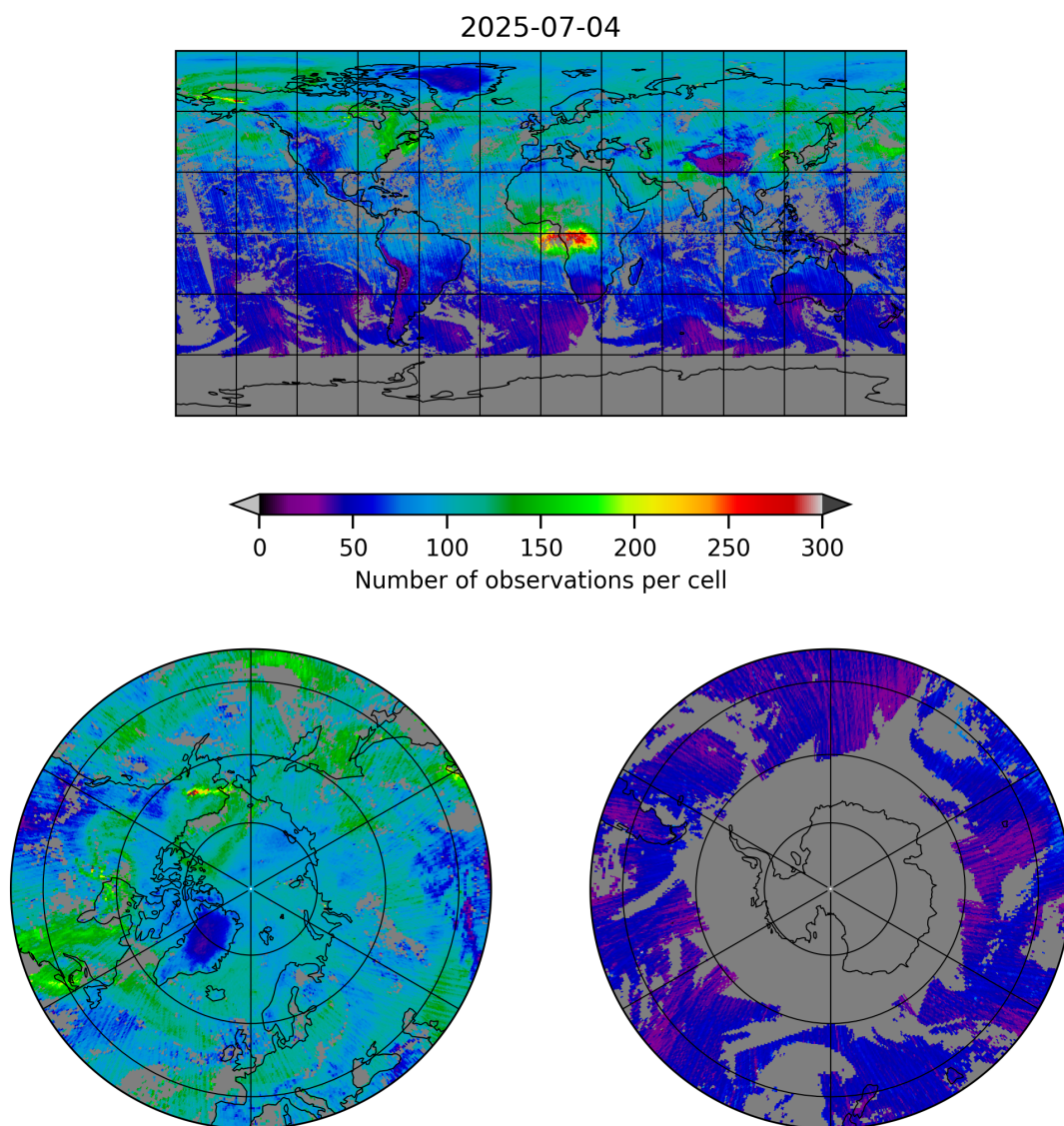
Figure 5: Map of the number of observations for 2025-07-04 to 2025-07-05
