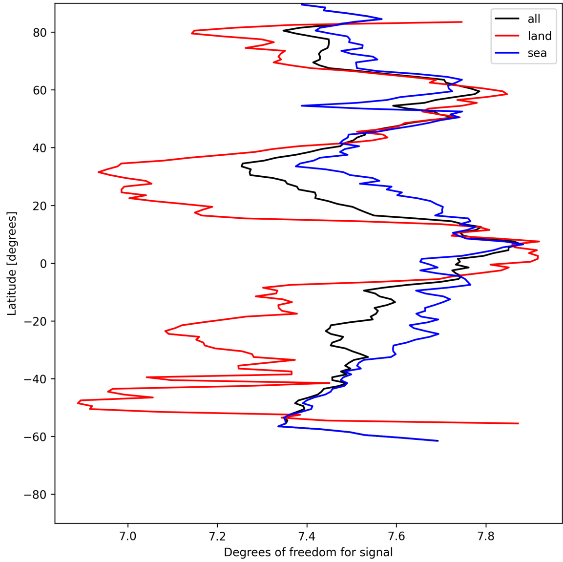
Figure 11: Zonal average of “Degrees of freedom for signal” for 2025-07-04 to 2025-07-05.
