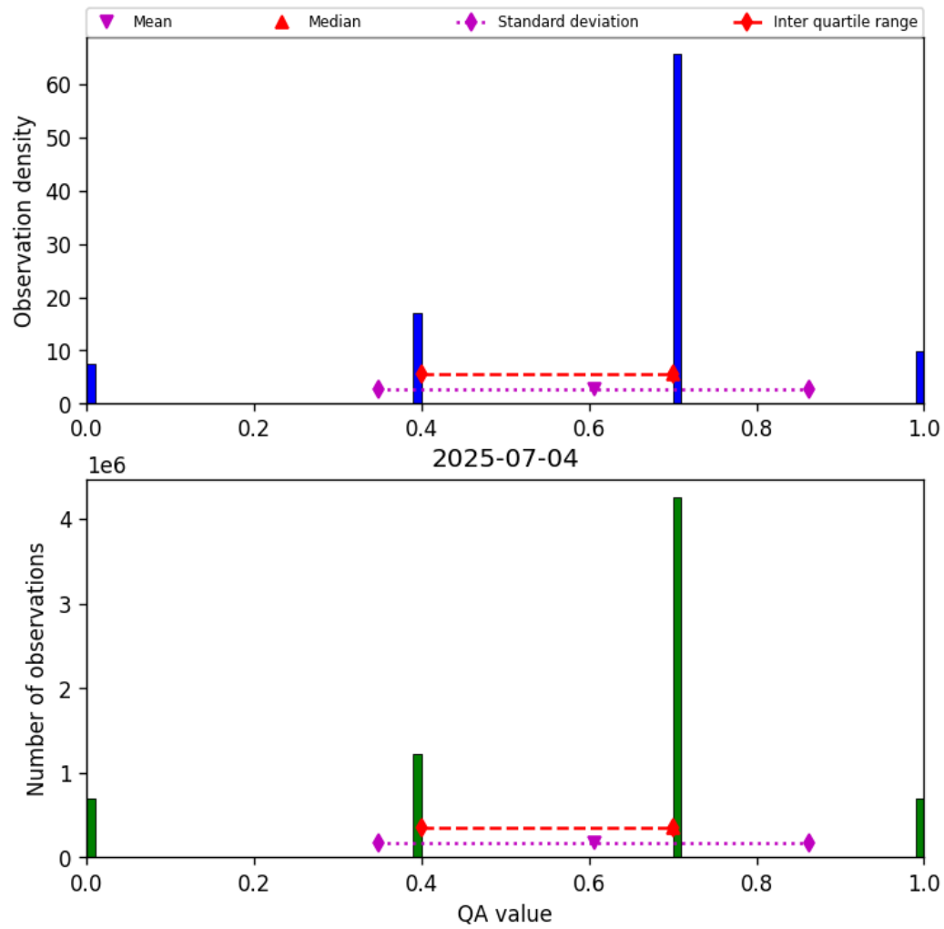
Figure 13: Histogram of “QA value” for 2025-07-04 to 2025-07-05
