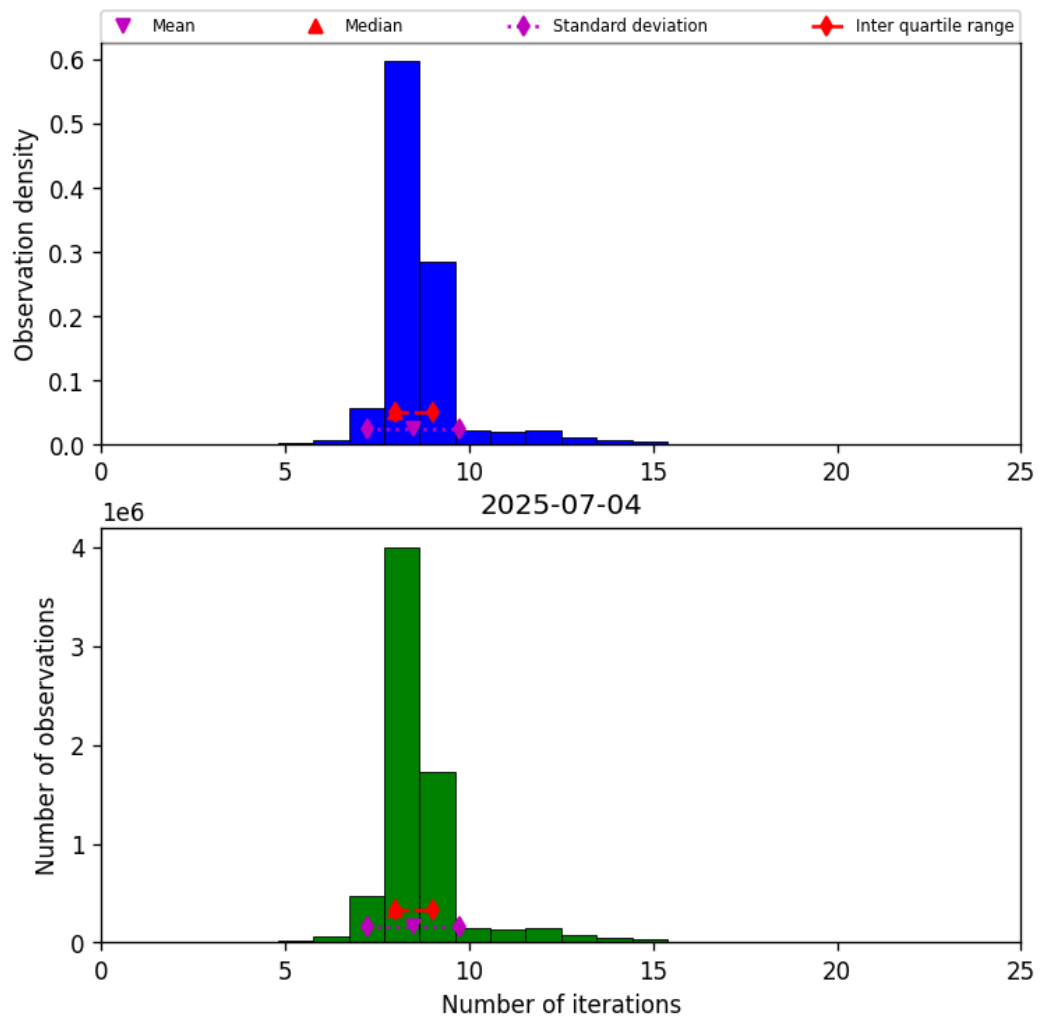
Figure 19: Histogram of “Number of iterations” for 2025-07-04 to 2025-07-05
