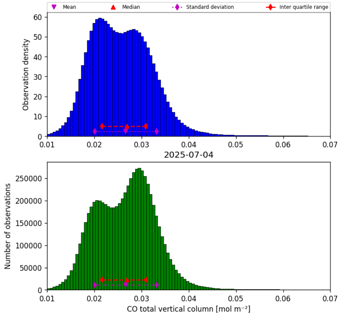
Figure 14: Histogram of “CO total vertical column” for 2025-07-04 to 2025-07-05
