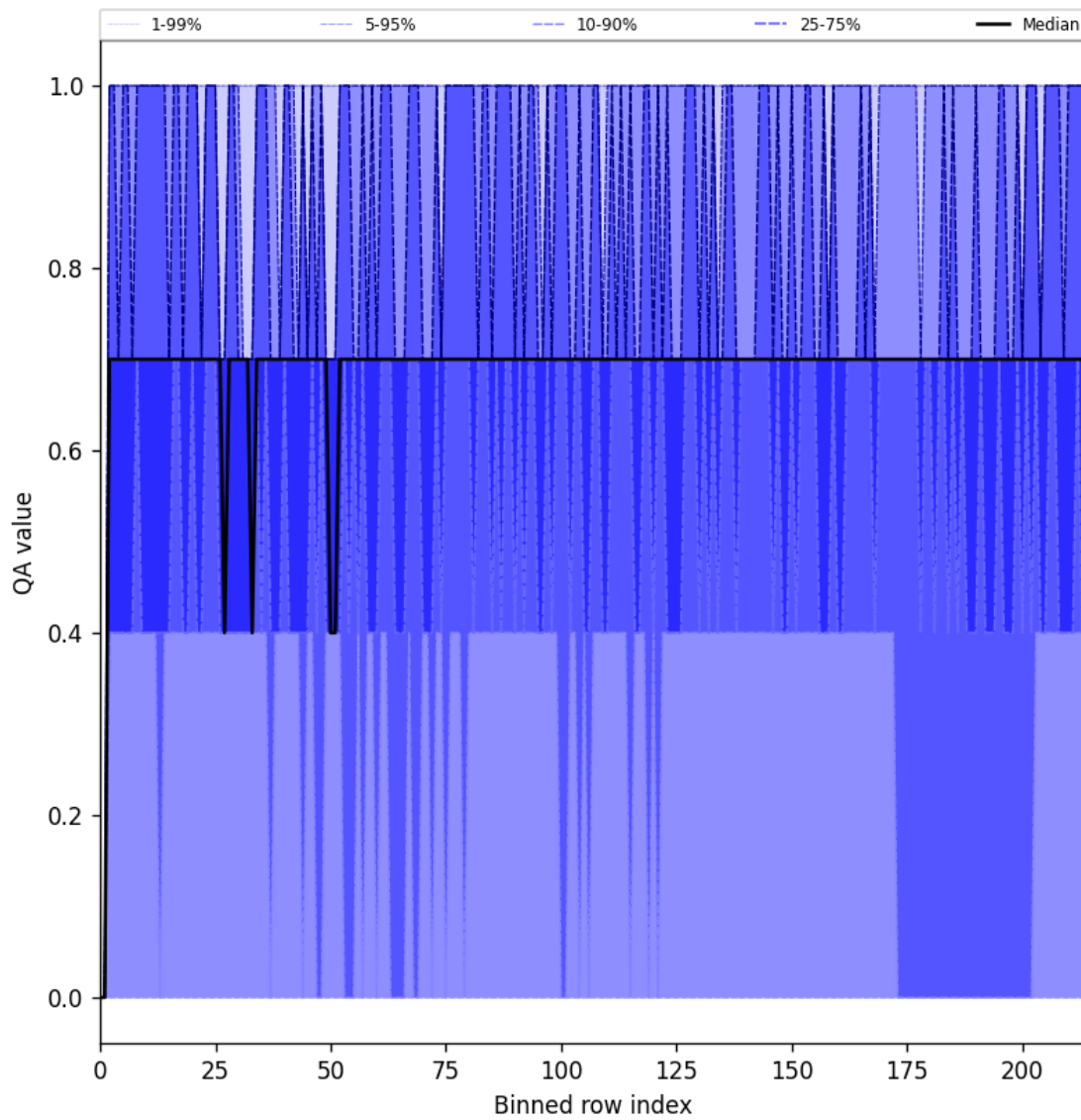
Figure 20: Along track statistics of “QA value” for 2025-07-04 to 2025-07-05
