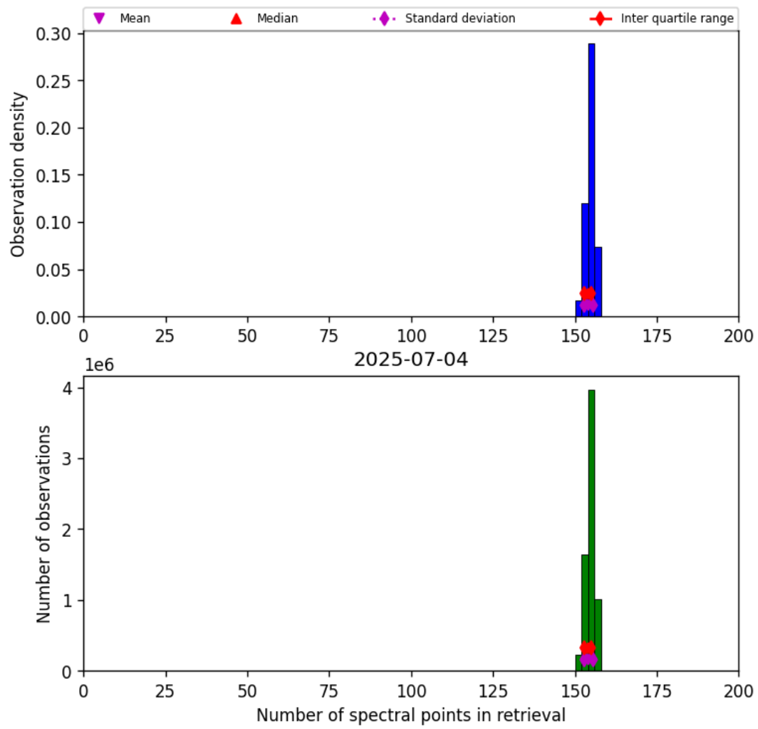
Figure 16: Histogram of “Number of spectral points in retrieval” for 2025-07-04 to 2025-07-05
