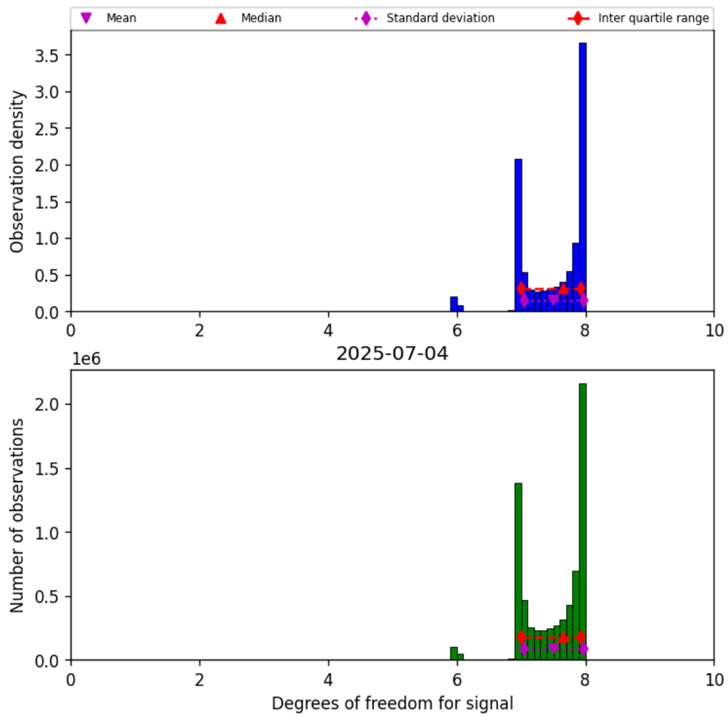
Figure 18: Histogram of “Degrees of freedom for signal” for 2025-07-04 to 2025-07-05
