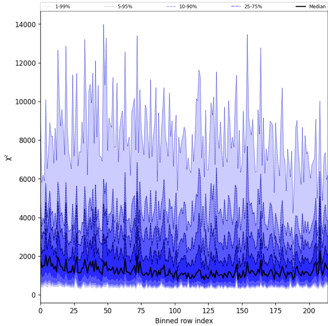
Figure 24: Along track statistics of “ \chi^2 ” for 2025-07-04 to 2025-07-05
