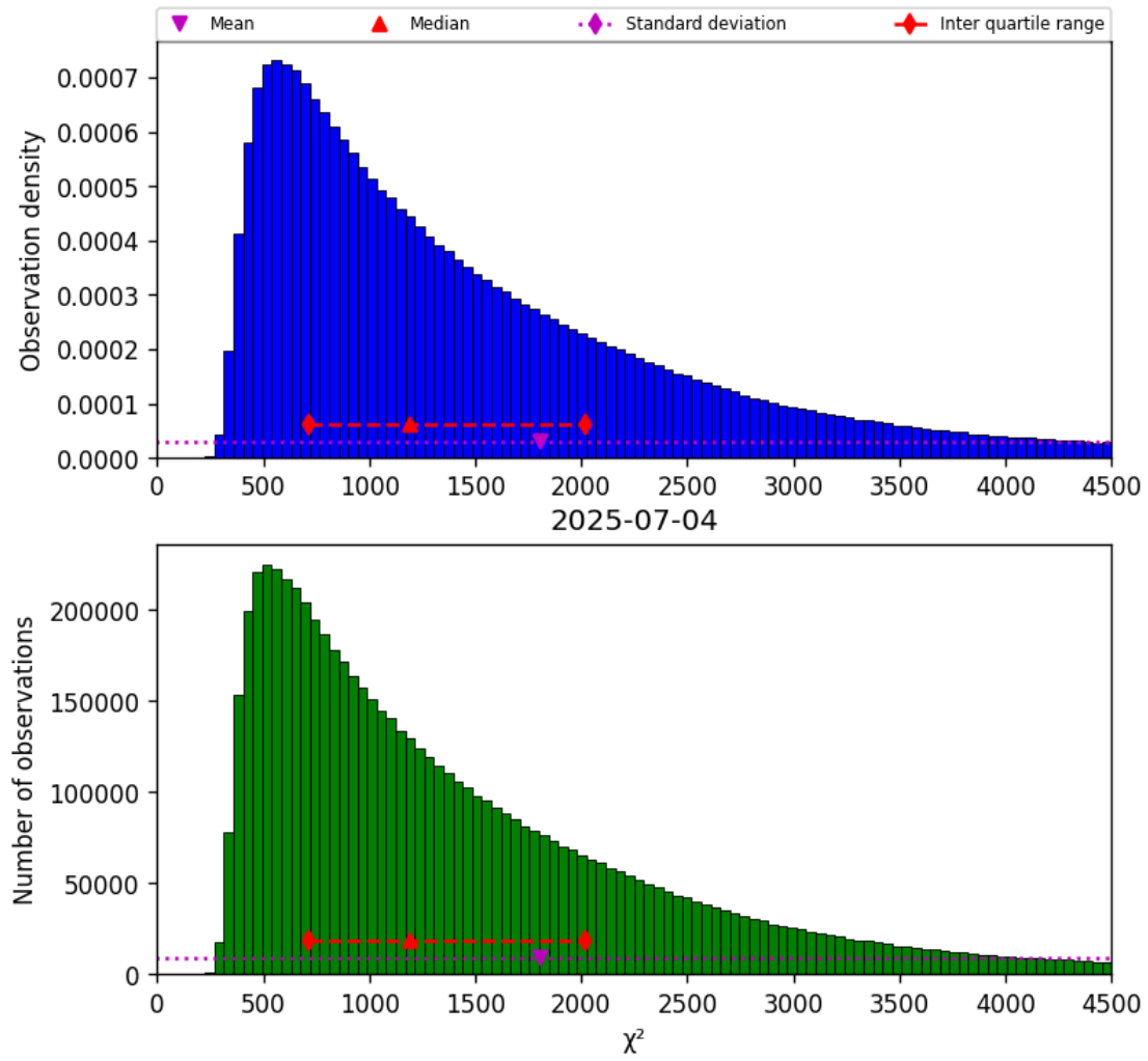
Figure 17: Histogram of " \chi^2 " for 2025-07-04 to 2025-07-05
