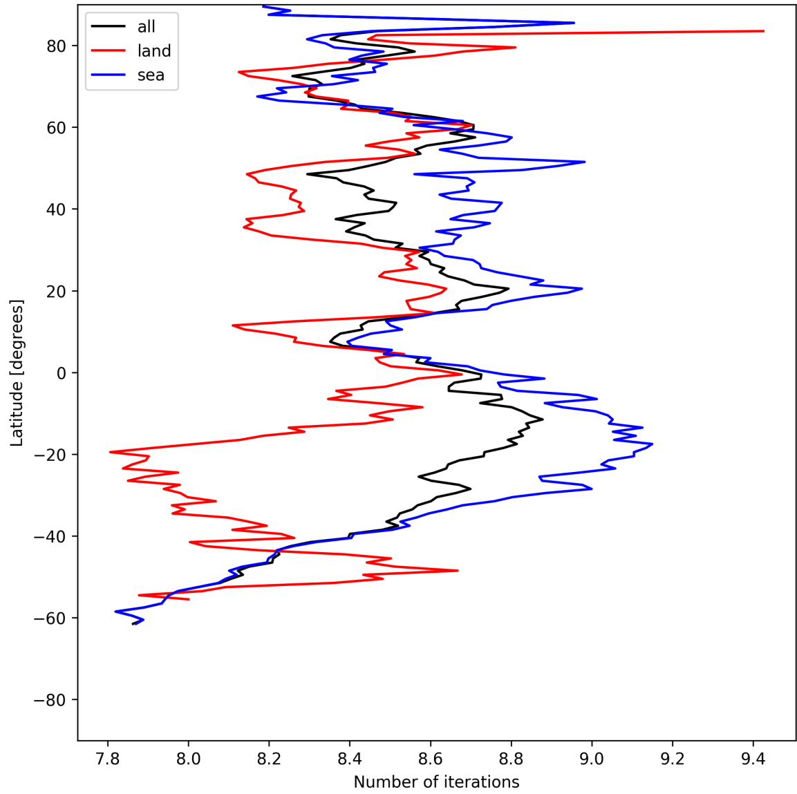
Figure 12: Zonal average of “Number of iterations” for 2025-07-04 to 2025-07-05.
