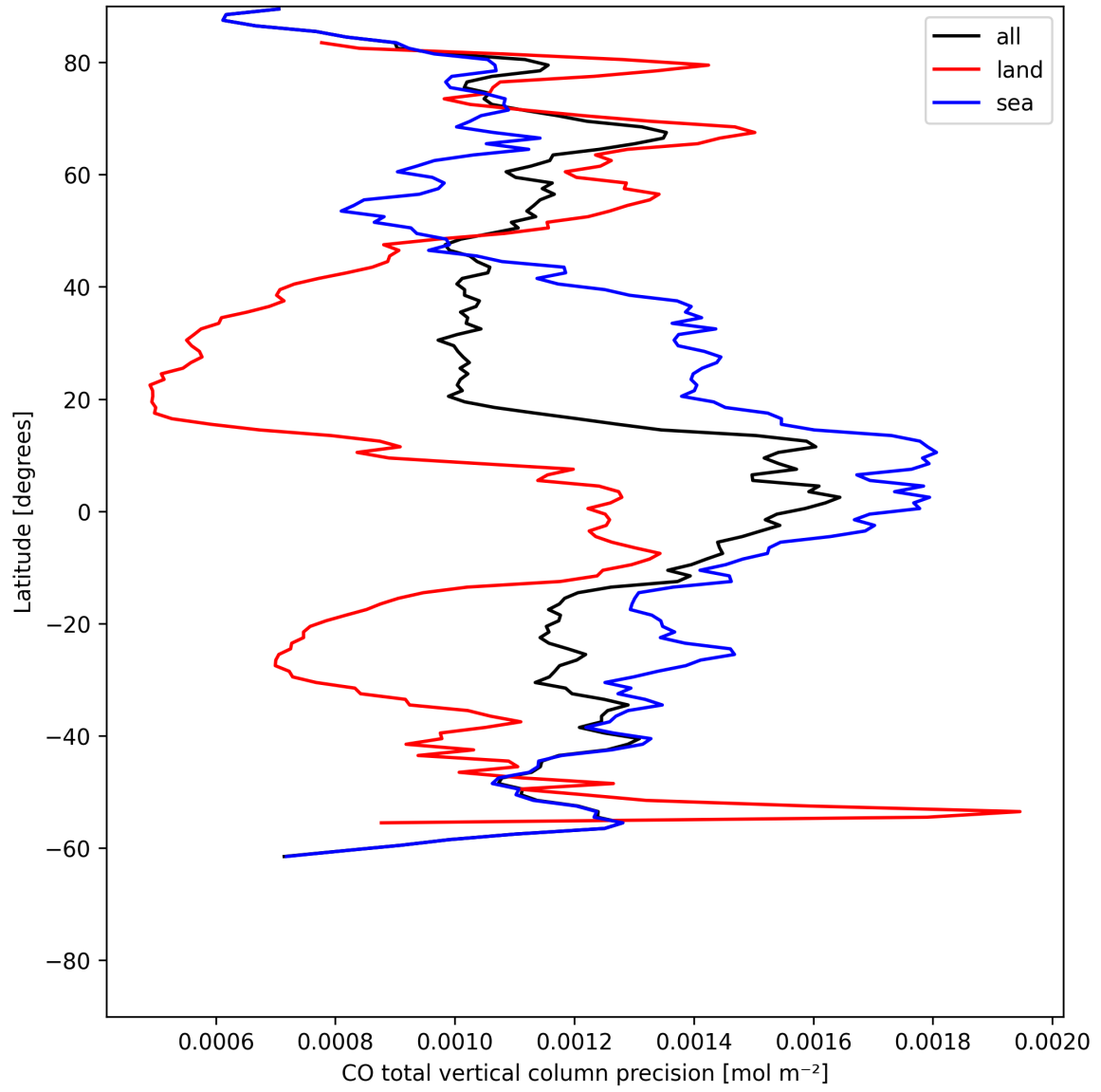
Figure 8: Zonal average of “CO total vertical column precision” for 2025-07-04 to 2025-07-05.
