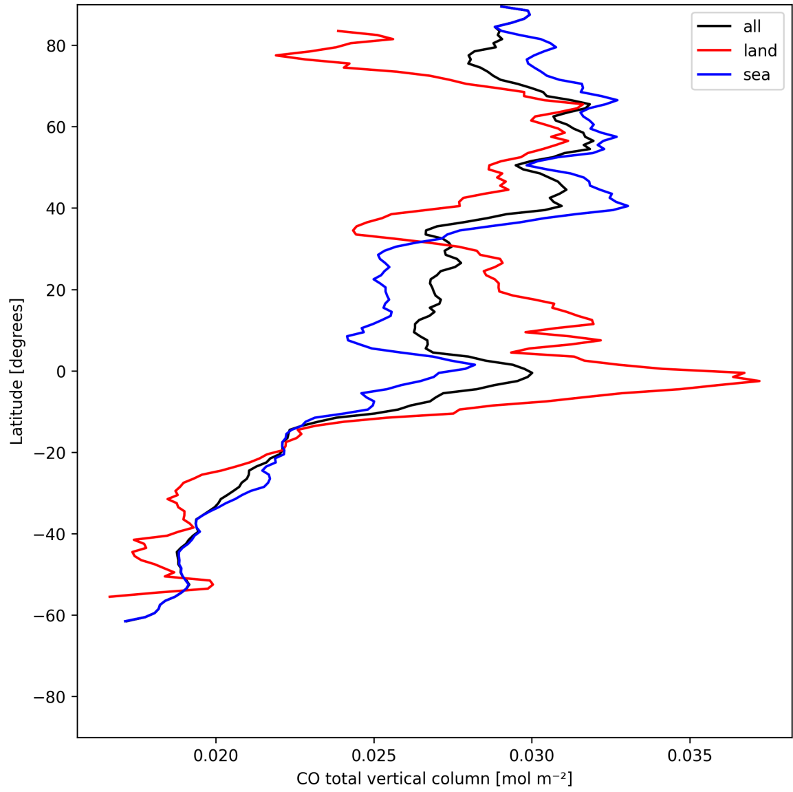
Figure 7: Zonal average of “CO total vertical column” for 2025-07-04 to 2025-07-05.
