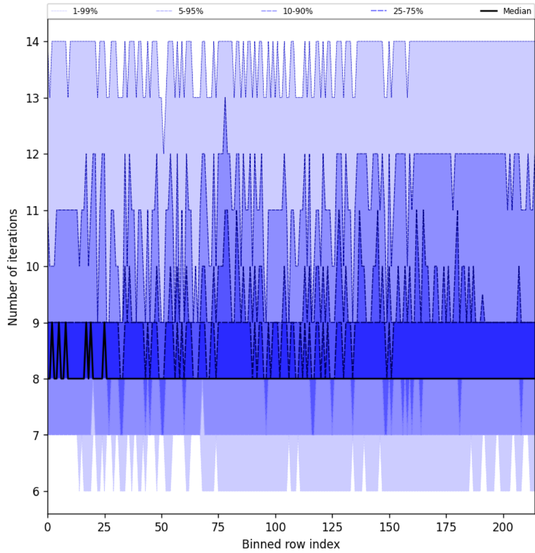
Figure 26: Along track statistics of “Number of iterations” for 2025-07-04 to 2025-07-05
