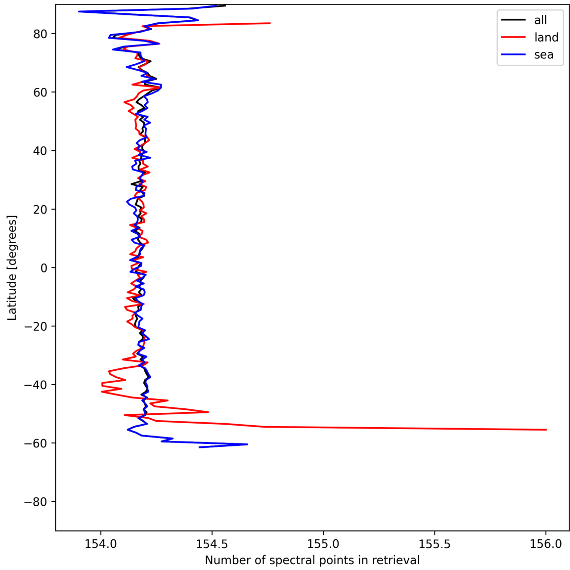
Figure 9: Zonal average of “Number of spectral points in retrieval” for 2025-07-04 to 2025-07-05.
