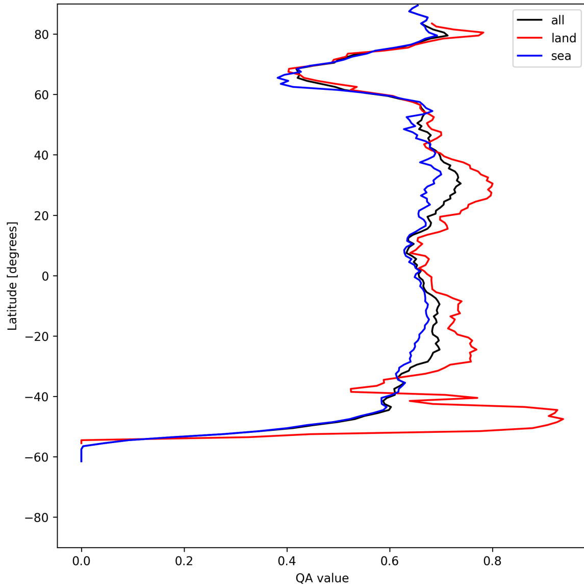
Figure 6: Zonal average of “QA value” for 2025-07-04 to 2025-07-05.
