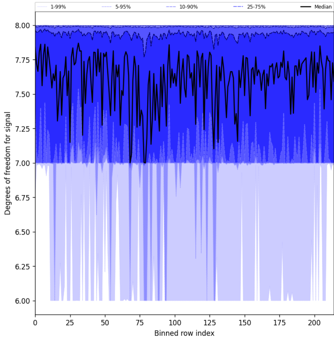
Figure 25: Along track statistics of “Degrees of freedom for signal” for 2025-07-04 to 2025-07-05
