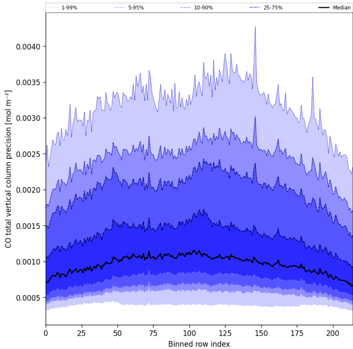
Figure 22: Along track statistics of “CO total vertical column precision” for 2025-07-05 to 2025-07-06
