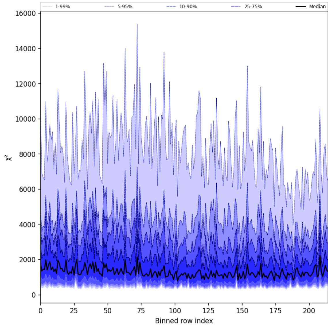
Figure 24: Along track statistics of “ \chi^2 ” for 2025-07-05 to 2025-07-06
