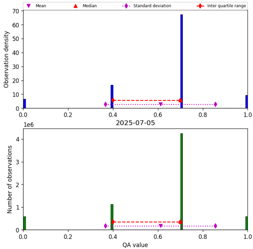
Figure 13: Histogram of “QA value” for 2025-07-05 to 2025-07-06
