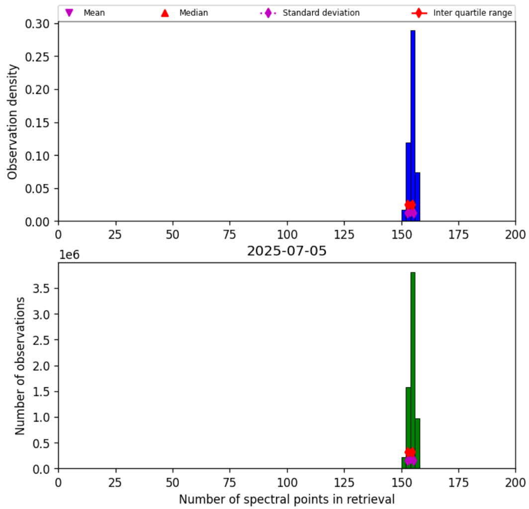
Figure 16: Histogram of “Number of spectral points in retrieval” for 2025-07-05 to 2025-07-06
