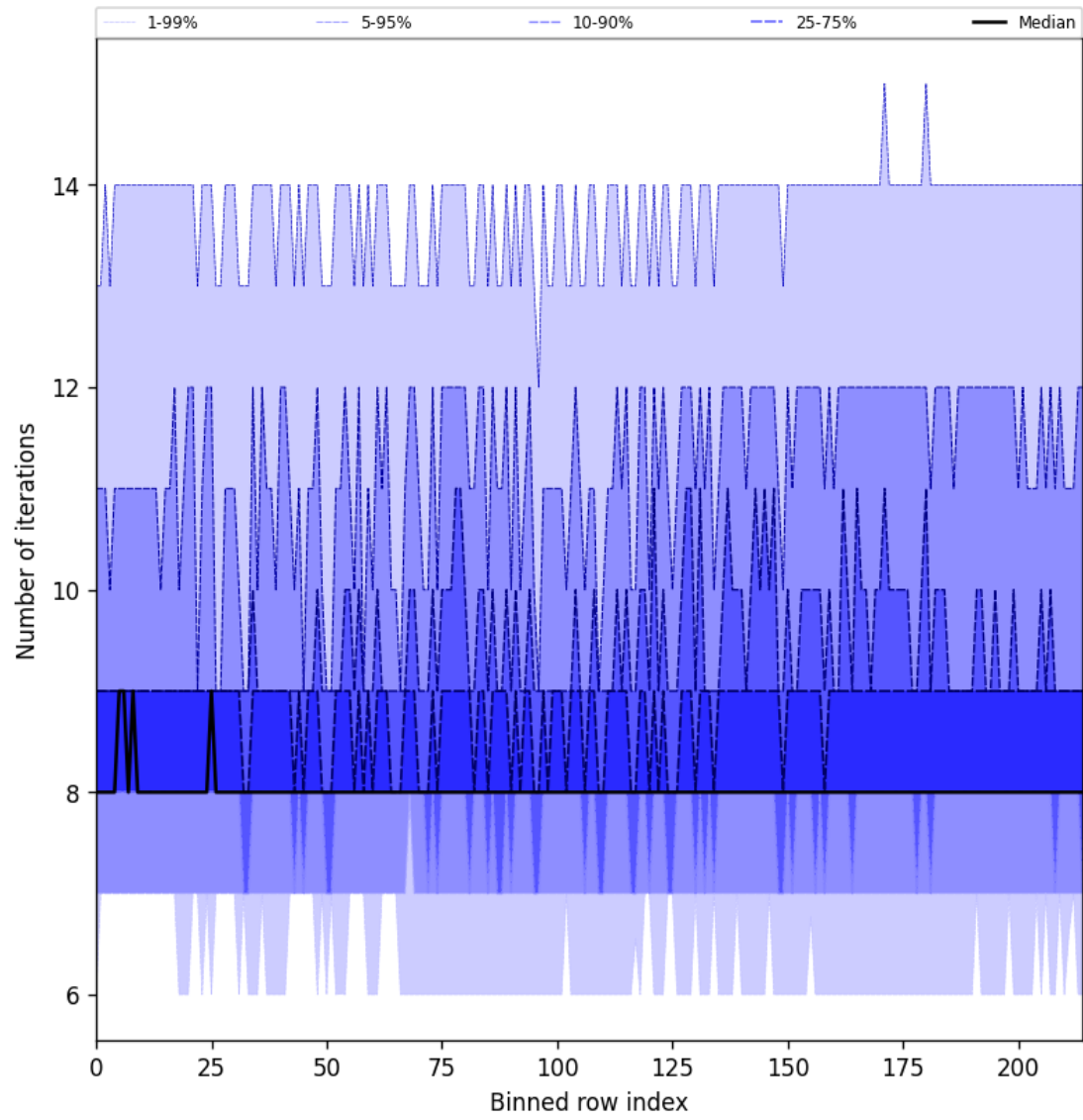
Figure 26: Along track statistics of “Number of iterations” for 2025-07-05 to 2025-07-06
