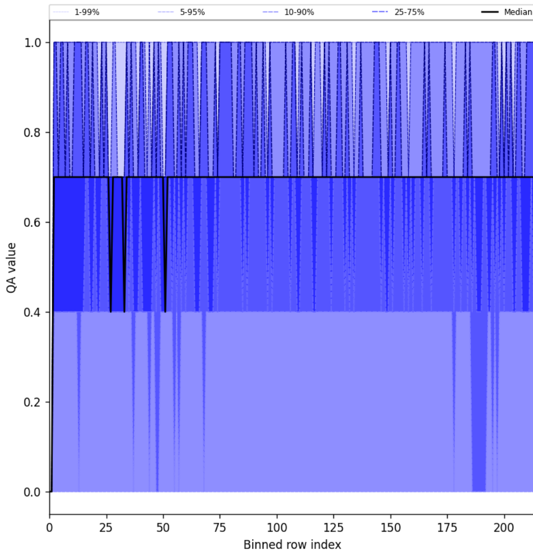
Figure 20: Along track statistics of “QA value” for 2025-07-05 to 2025-07-06
