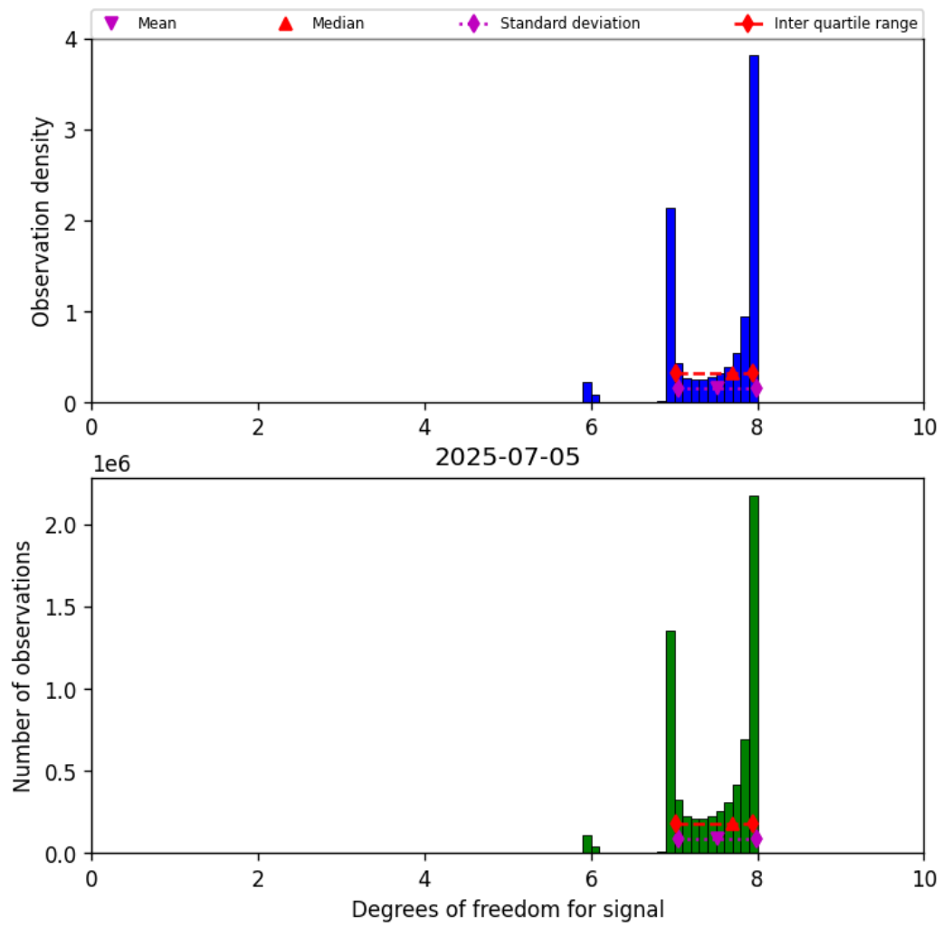
Figure 18: Histogram of “Degrees of freedom for signal” for 2025-07-05 to 2025-07-06
