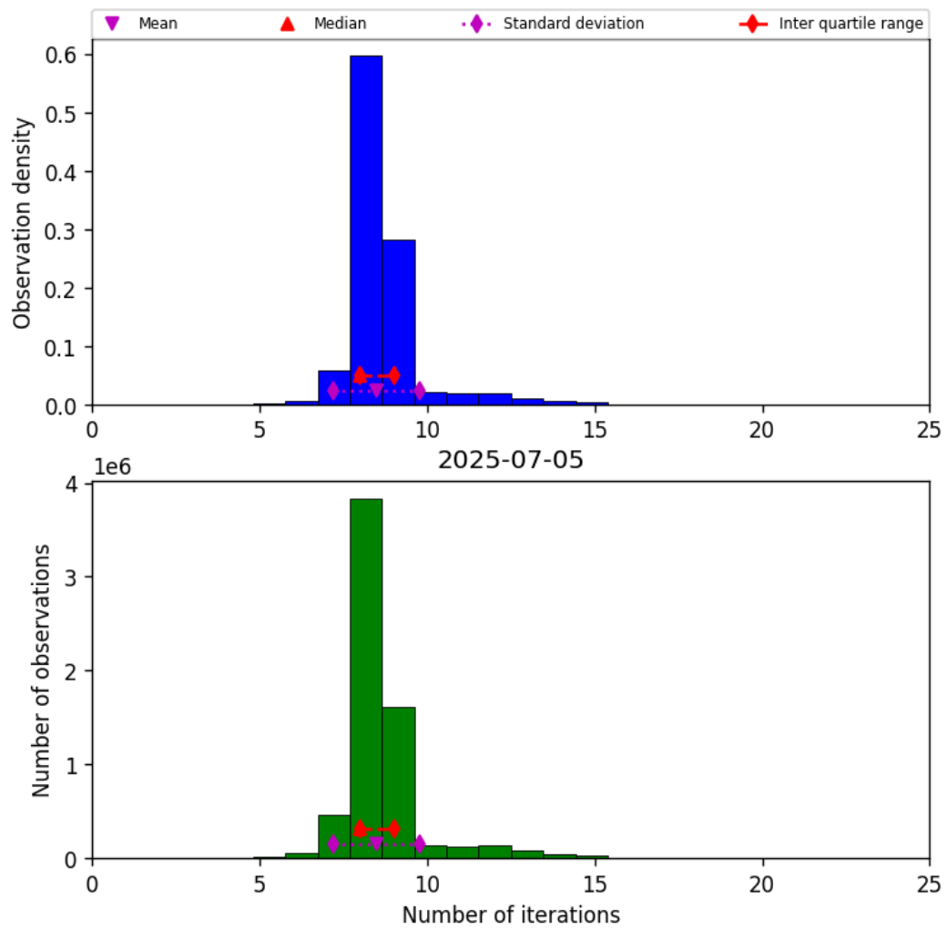
Figure 19: Histogram of “Number of iterations” for 2025-07-05 to 2025-07-06
