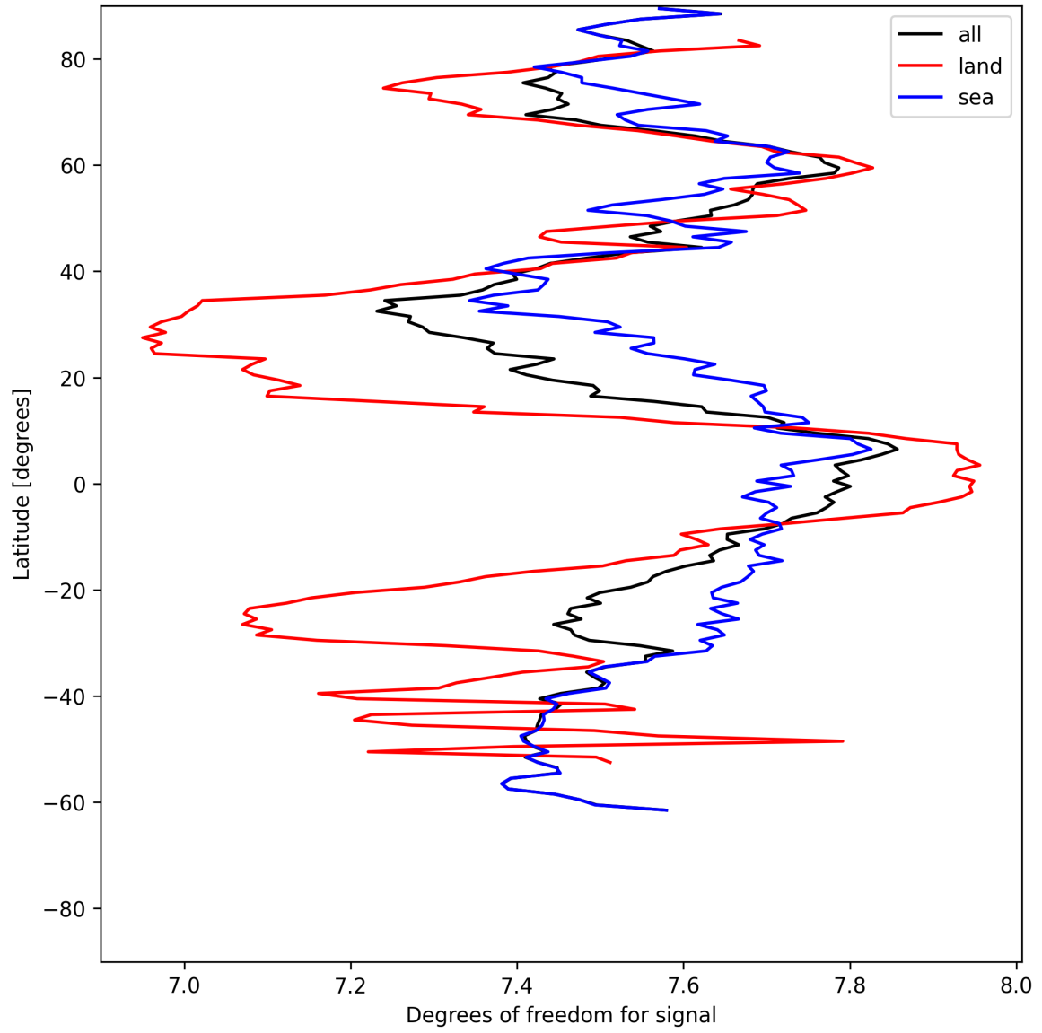
Figure 11: Zonal average of “Degrees of freedom for signal” for 2025-07-05 to 2025-07-06.
