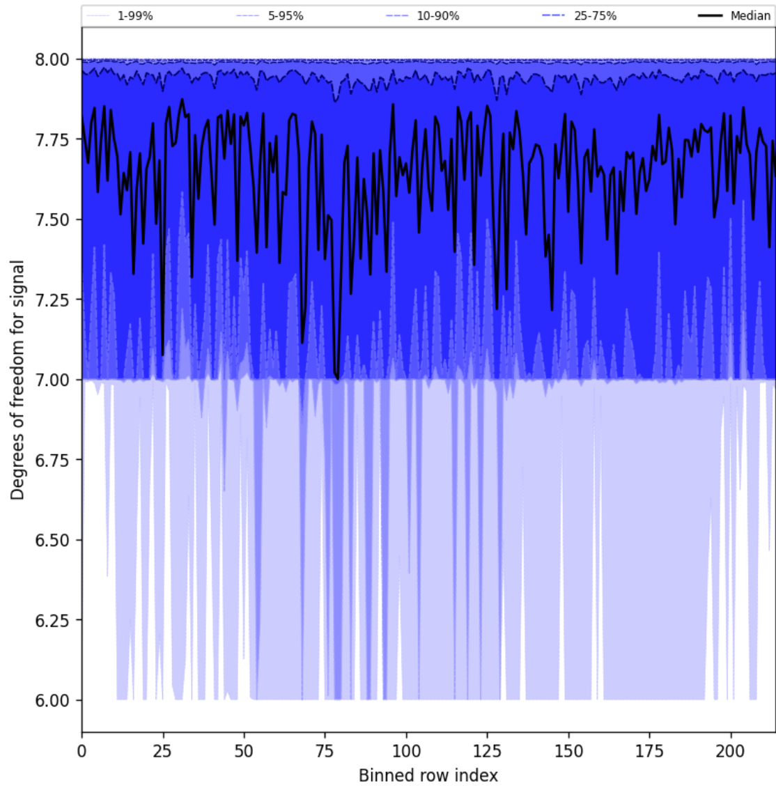
Figure 25: Along track statistics of “Degrees of freedom for signal” for 2025-07-05 to 2025-07-06
