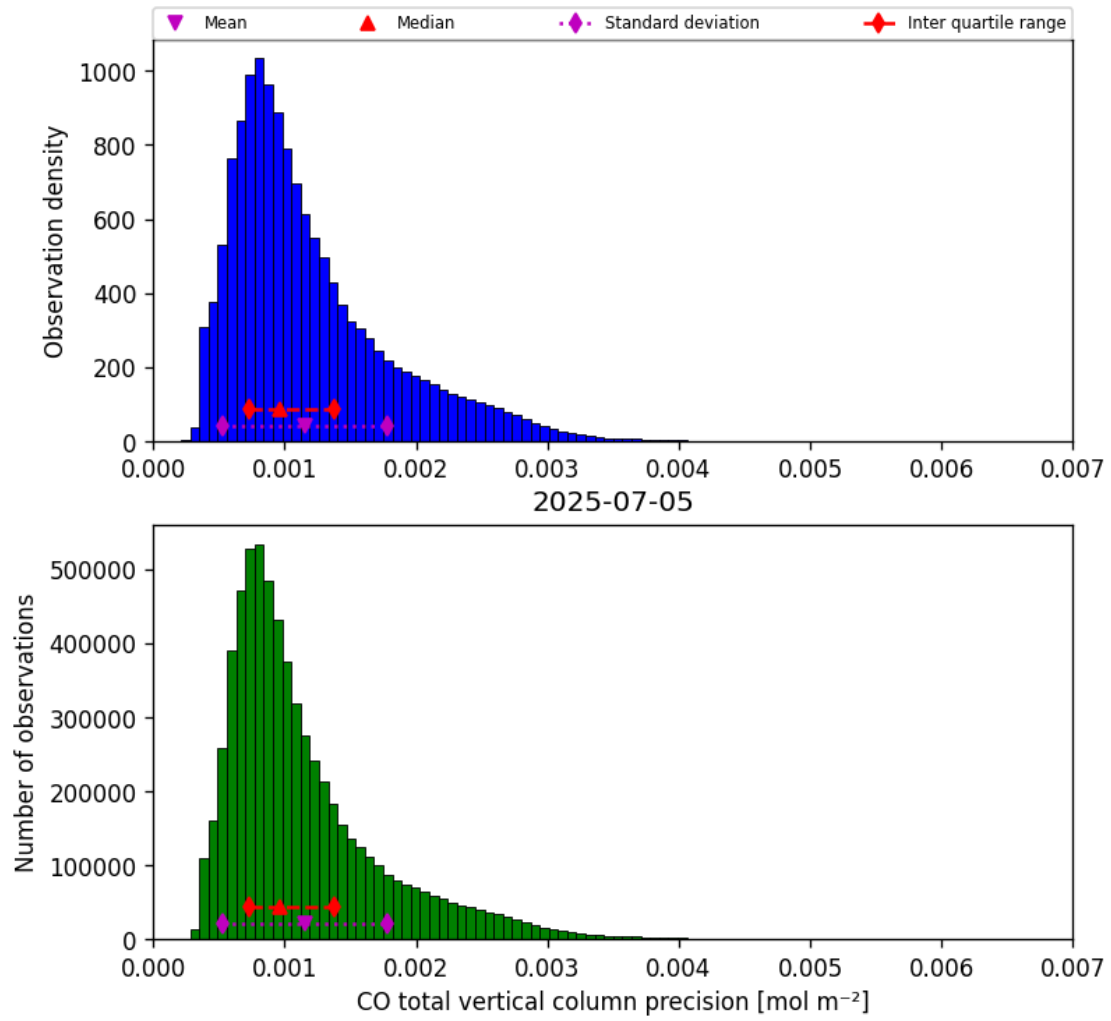
Figure 15: Histogram of “CO total vertical column precision” for 2025-07-05 to 2025-07-06
