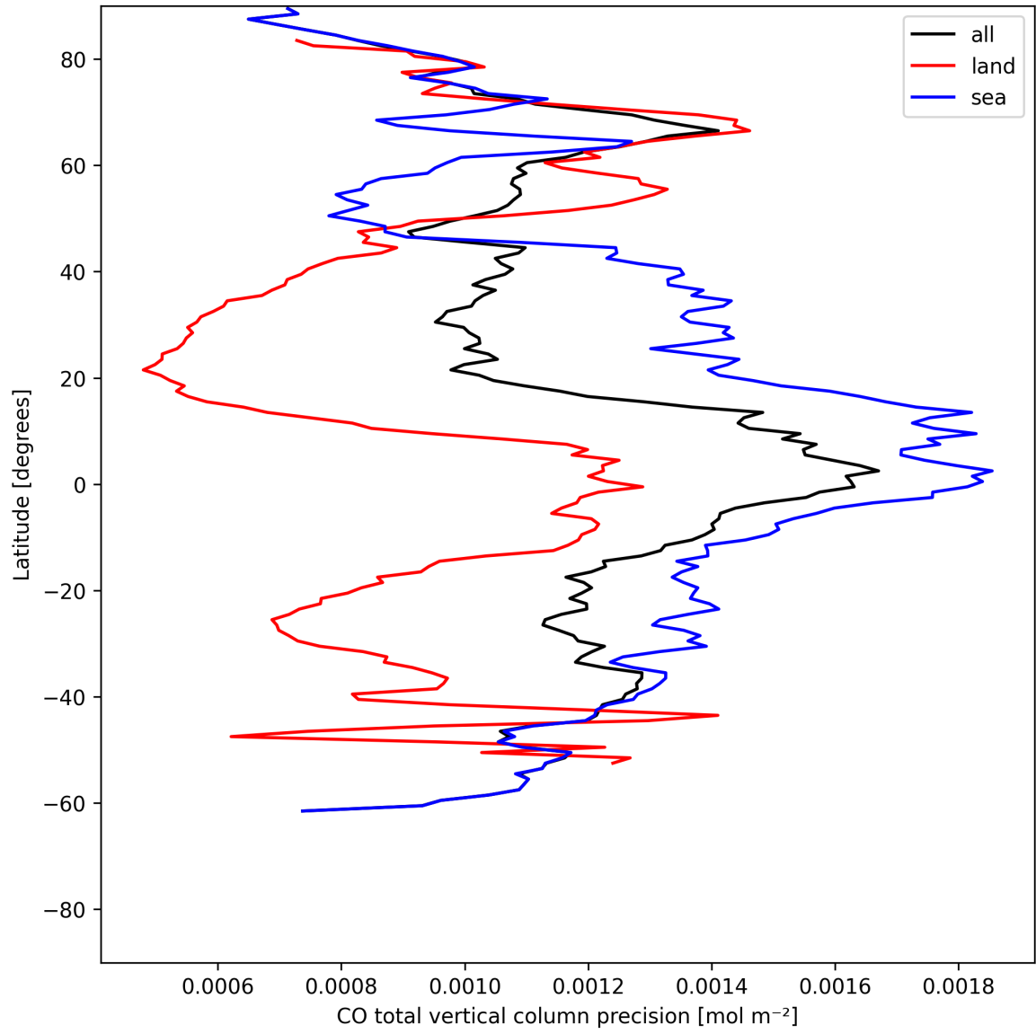
Figure 8: Zonal average of "CO total vertical column precision" for 2025-07-05 to 2025-07-06.
