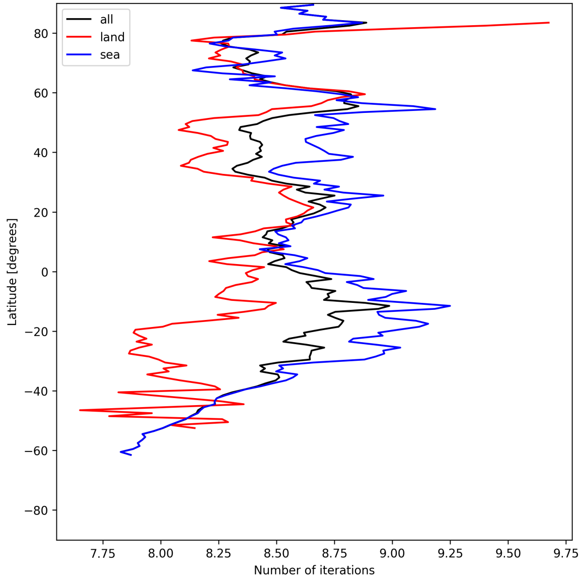
Figure 12: Zonal average of “Number of iterations” for 2025-07-05 to 2025-07-06.
