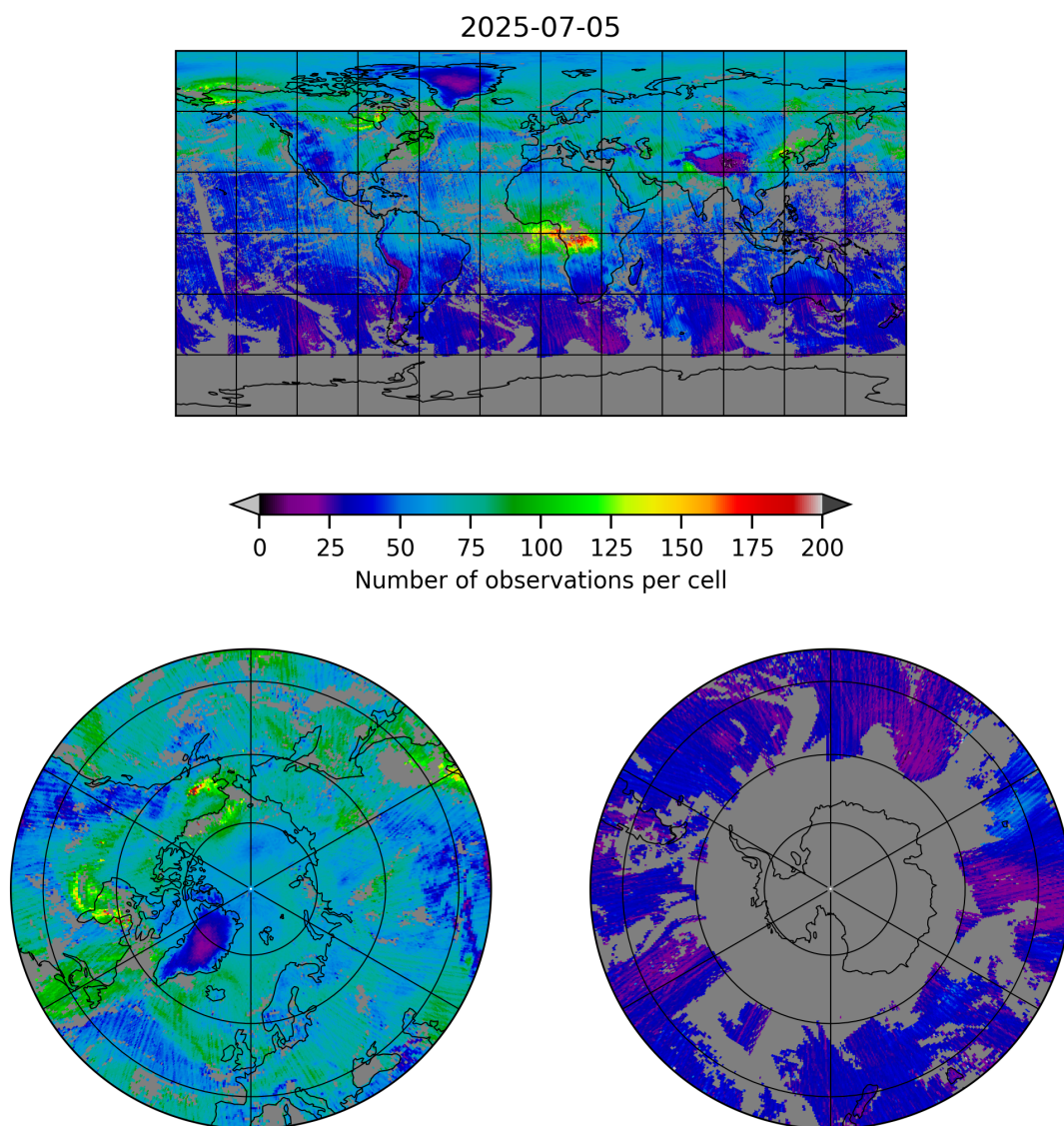
Figure 5: Map of the number of observations for 2025-07-05 to 2025-07-06
