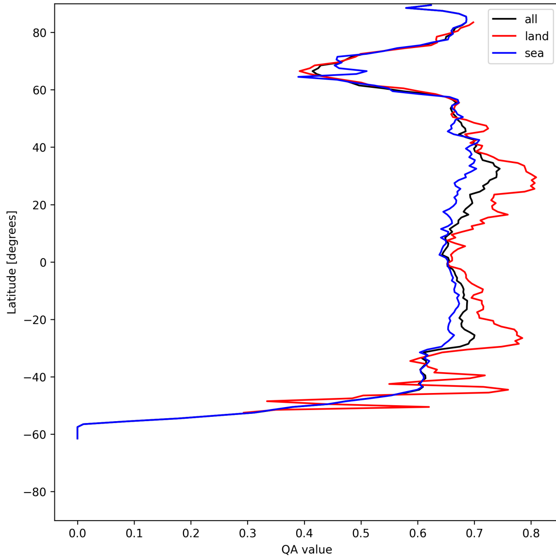
Figure 6: Zonal average of “QA value” for 2025-07-05 to 2025-07-06.
