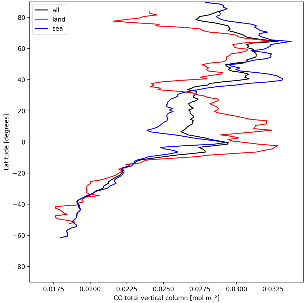
Figure 7: Zonal average of “CO total vertical column” for 2025-07-05 to 2025-07-06.
