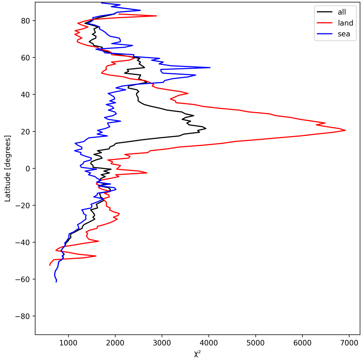
Figure 10: Zonal average of “ \chi^2 ” for 2025-07-05 to 2025-07-06.
