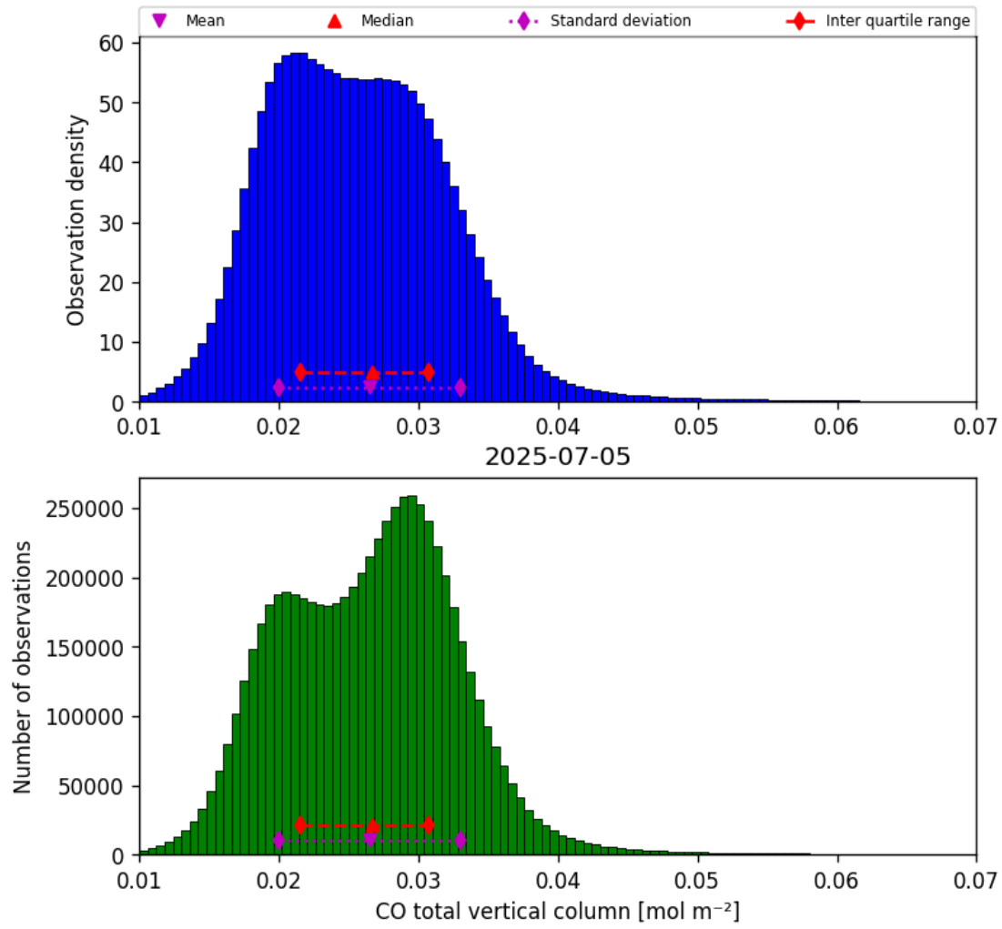
Figure 14: Histogram of “CO total vertical column” for 2025-07-05 to 2025-07-06
