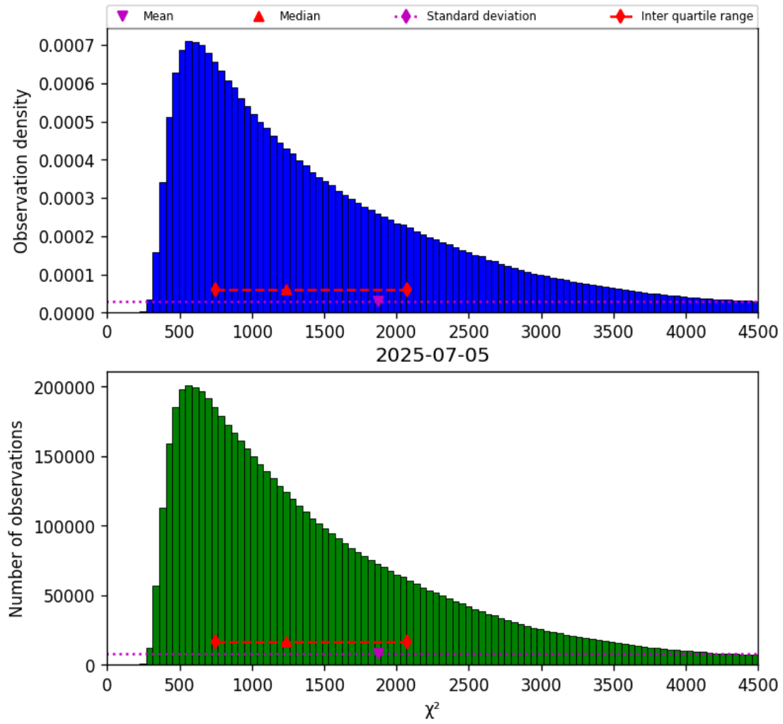
Figure 17: Histogram of " \chi^2 " for 2025-07-05 to 2025-07-06
