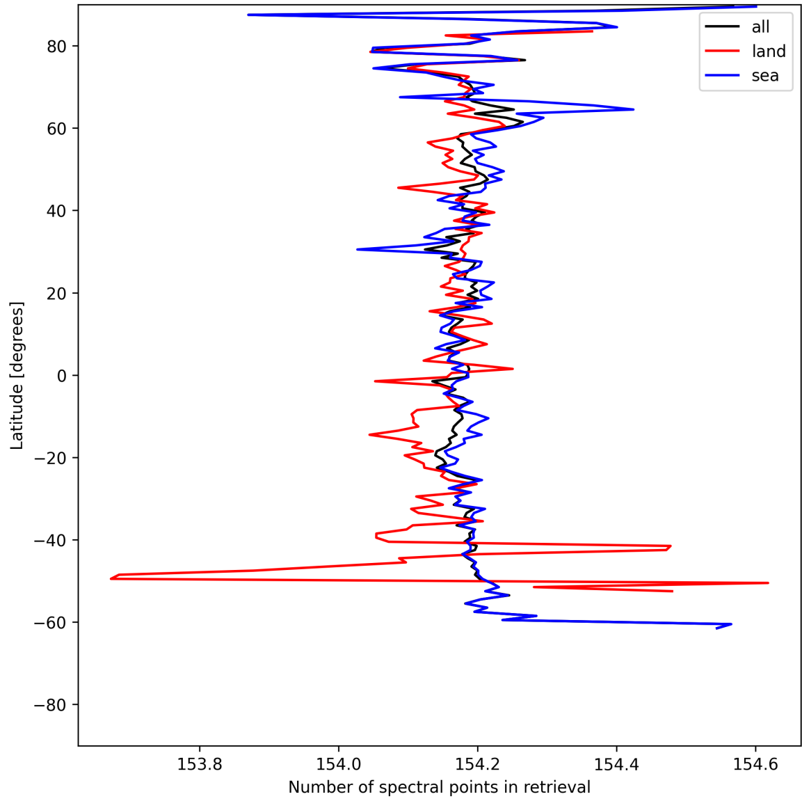
Figure 9: Zonal average of “Number of spectral points in retrieval” for 2025-07-05 to 2025-07-06.
