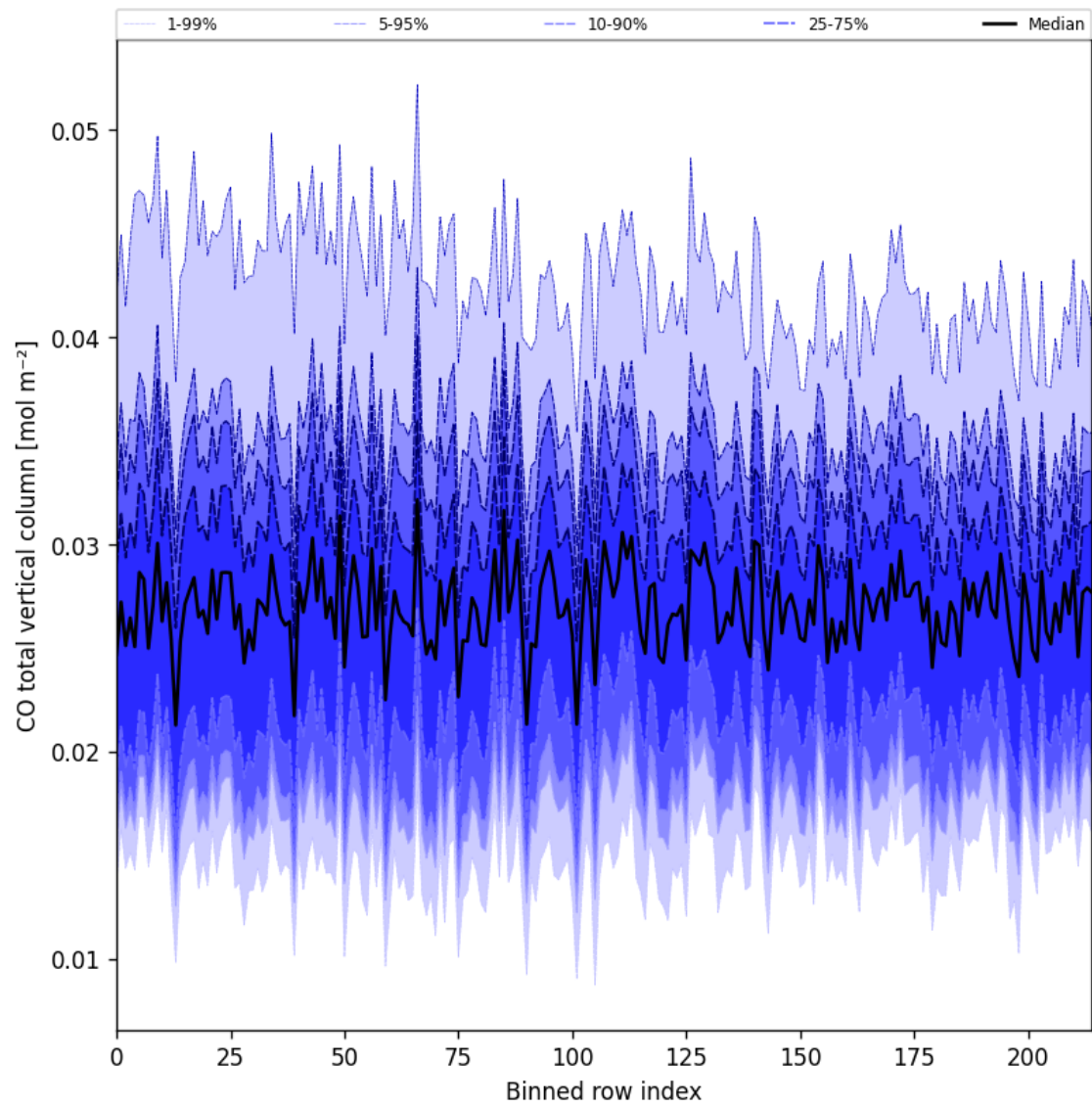
Figure 21: Along track statistics of “CO total vertical column” for 2025-07-05 to 2025-07-06
